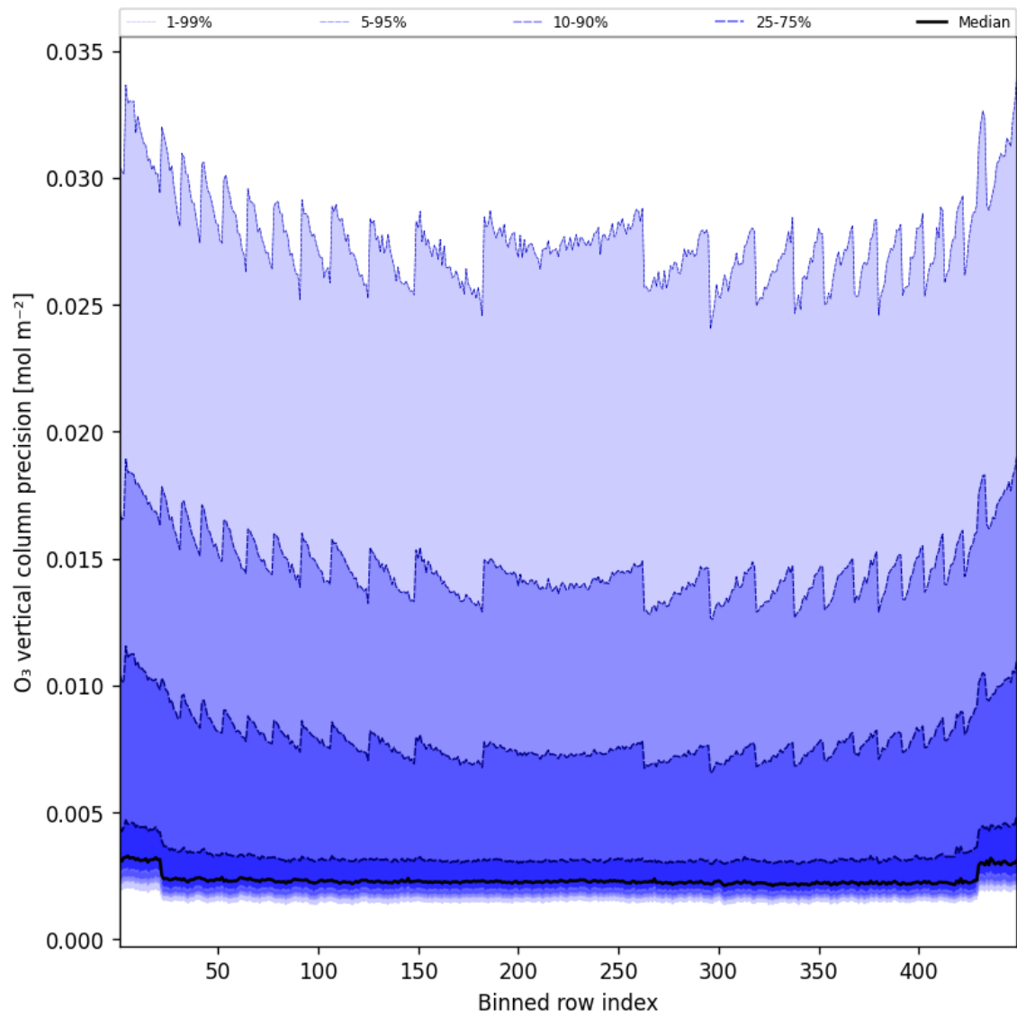
Figure 42: Along track statistics of “O 3 vertical column precision” for 2025-04-10 to 2025-04-11
