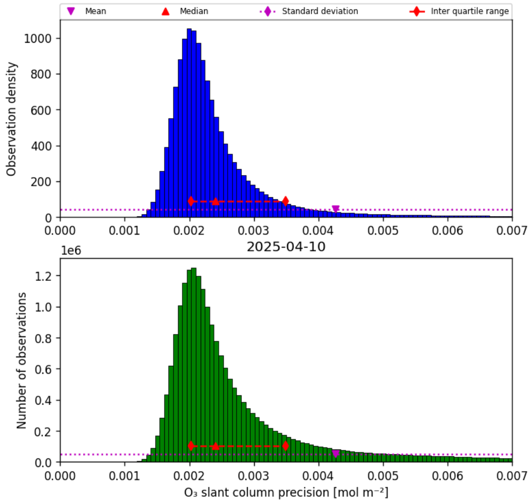
Figure 32: Histogram of “O 3 slant column precision” for 2025-04-10 to 2025-04-11
