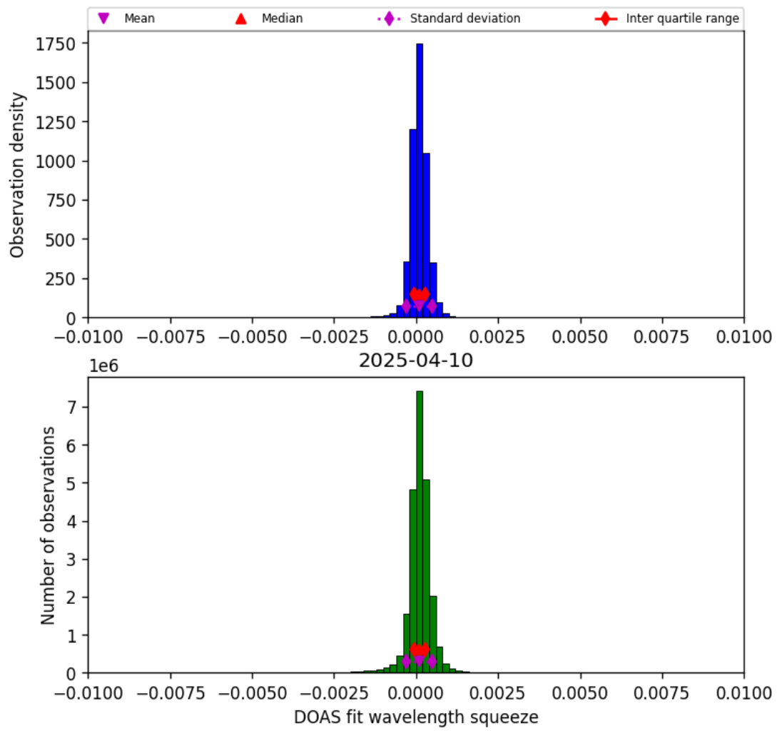
Figure 36: Histogram of “DOAS fit wavelength squeeze” for 2025-04-10 to 2025-04-11
