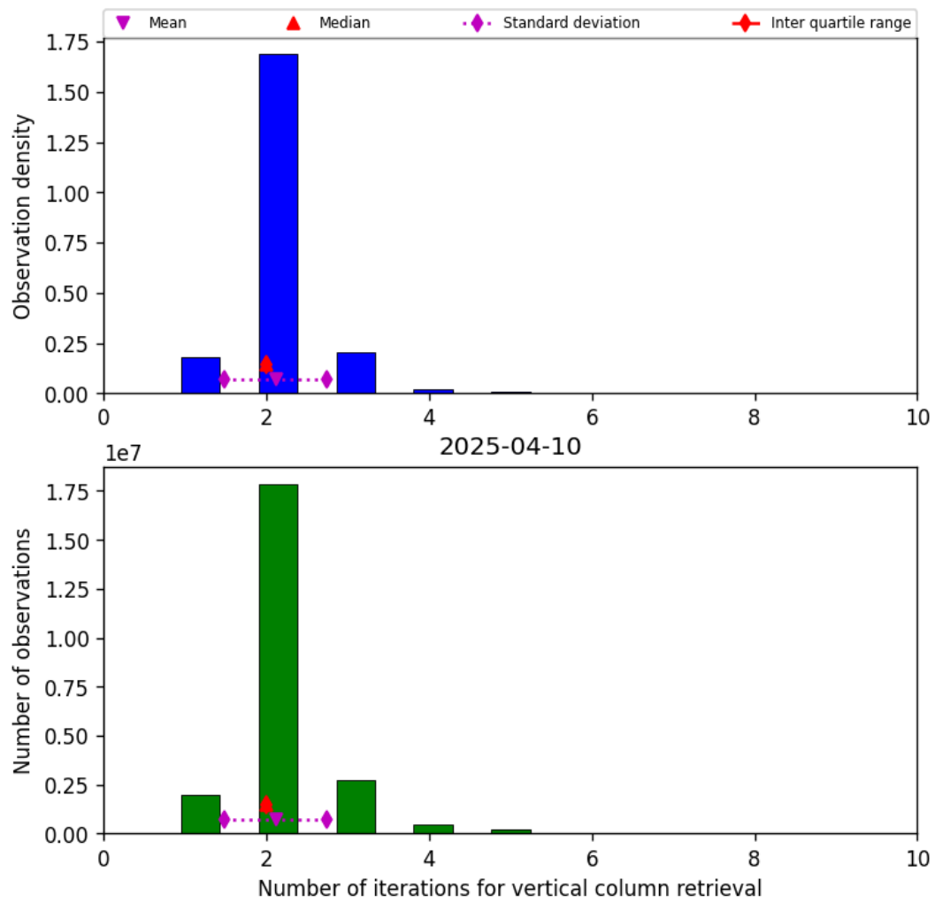
Figure 39: Histogram of “Number of iterations for vertical column retrieval” for 2025-04-10 to 2025-04-11
