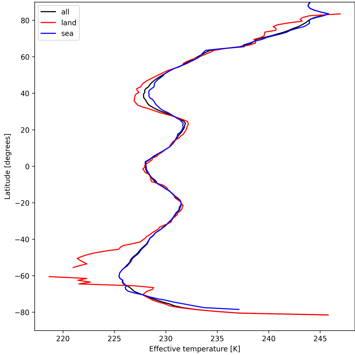
Figure 26: Zonal average of “Effective temperature” for 2025-04-10 to 2025-04-11.
