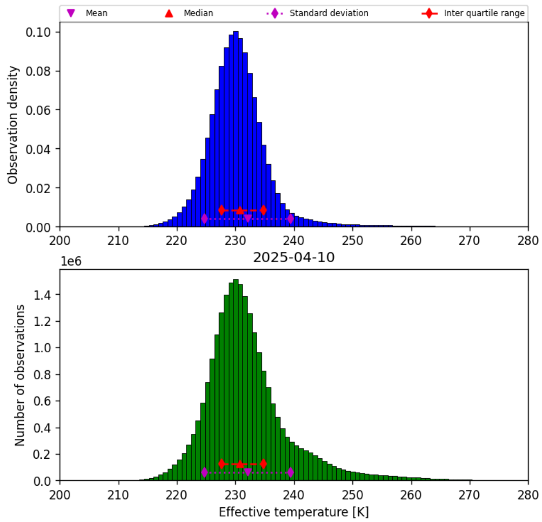
Figure 38: Histogram of “Effective temperature” for 2025-04-10 to 2025-04-11
