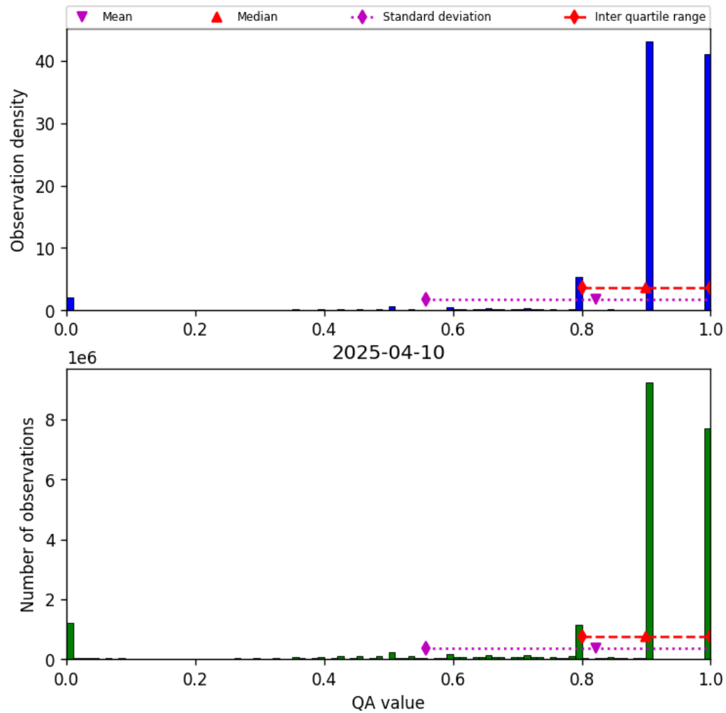
Figure 28: Histogram of “QA value” for 2025-04-10 to 2025-04-11
