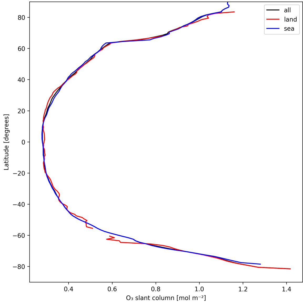
Figure 19: Zonal average of “O 3 slant column” for 2025-04-10 to 2025-04-11.
