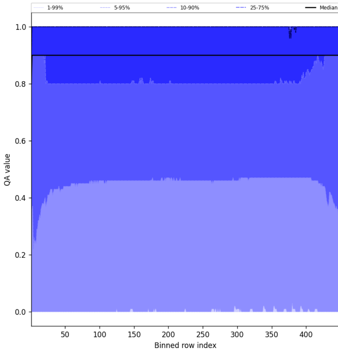
Figure 40: Along track statistics of “QA value” for 2025-04-10 to 2025-04-11
