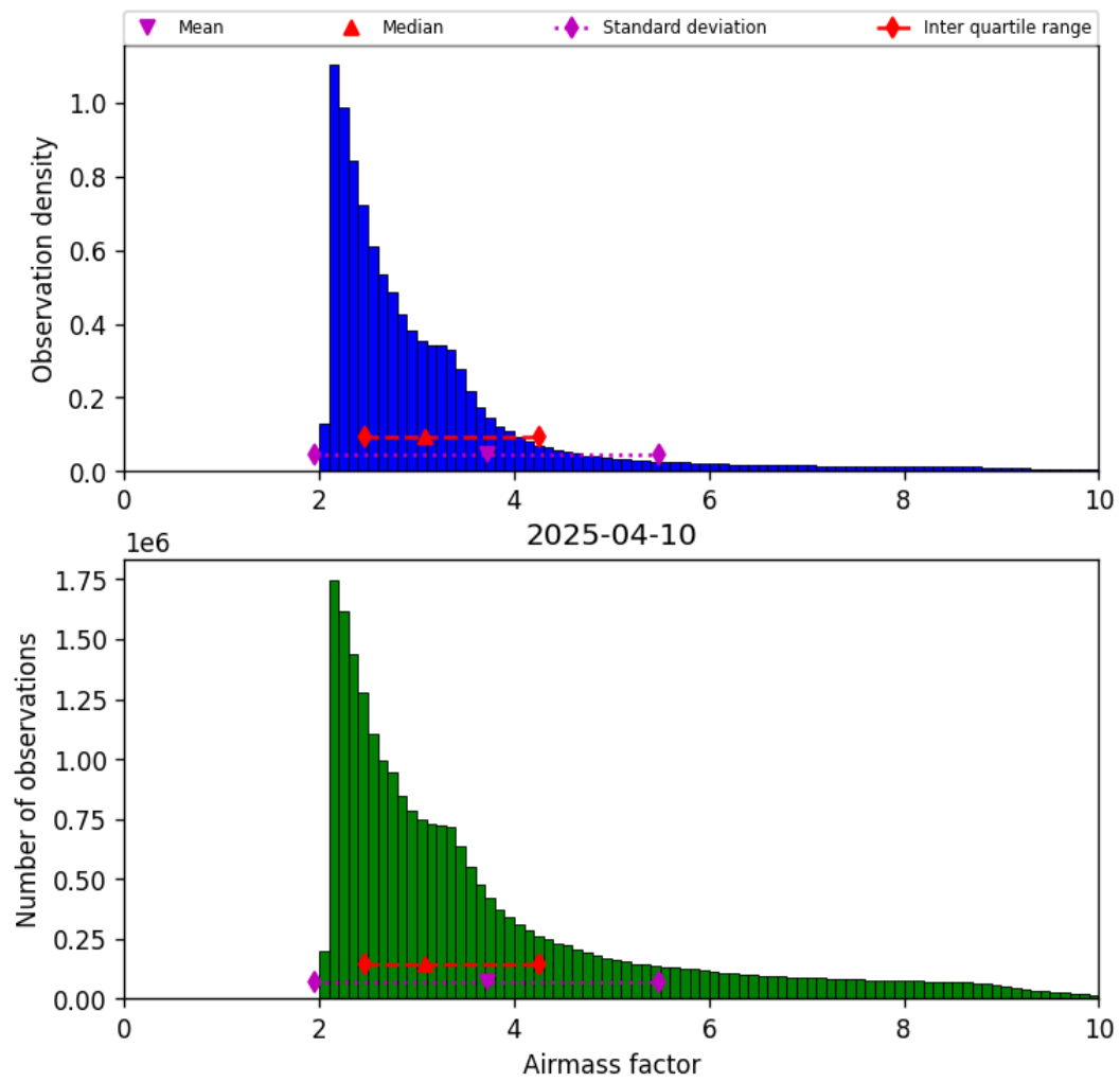
Figure 37: Histogram of “Airmass factor” for 2025-04-10 to 2025-04-11
