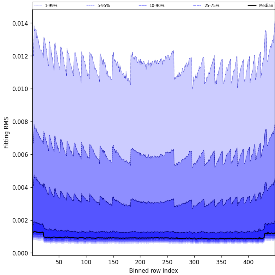
Figure 46: Along track statistics of “Fitting RMS” for 2025-04-10 to 2025-04-11
