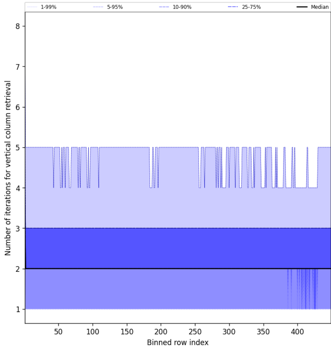
Figure 51: Along track statistics of “Number of iterations for vertical column retrieval” for 2025-04-10 to 2025-04-11
