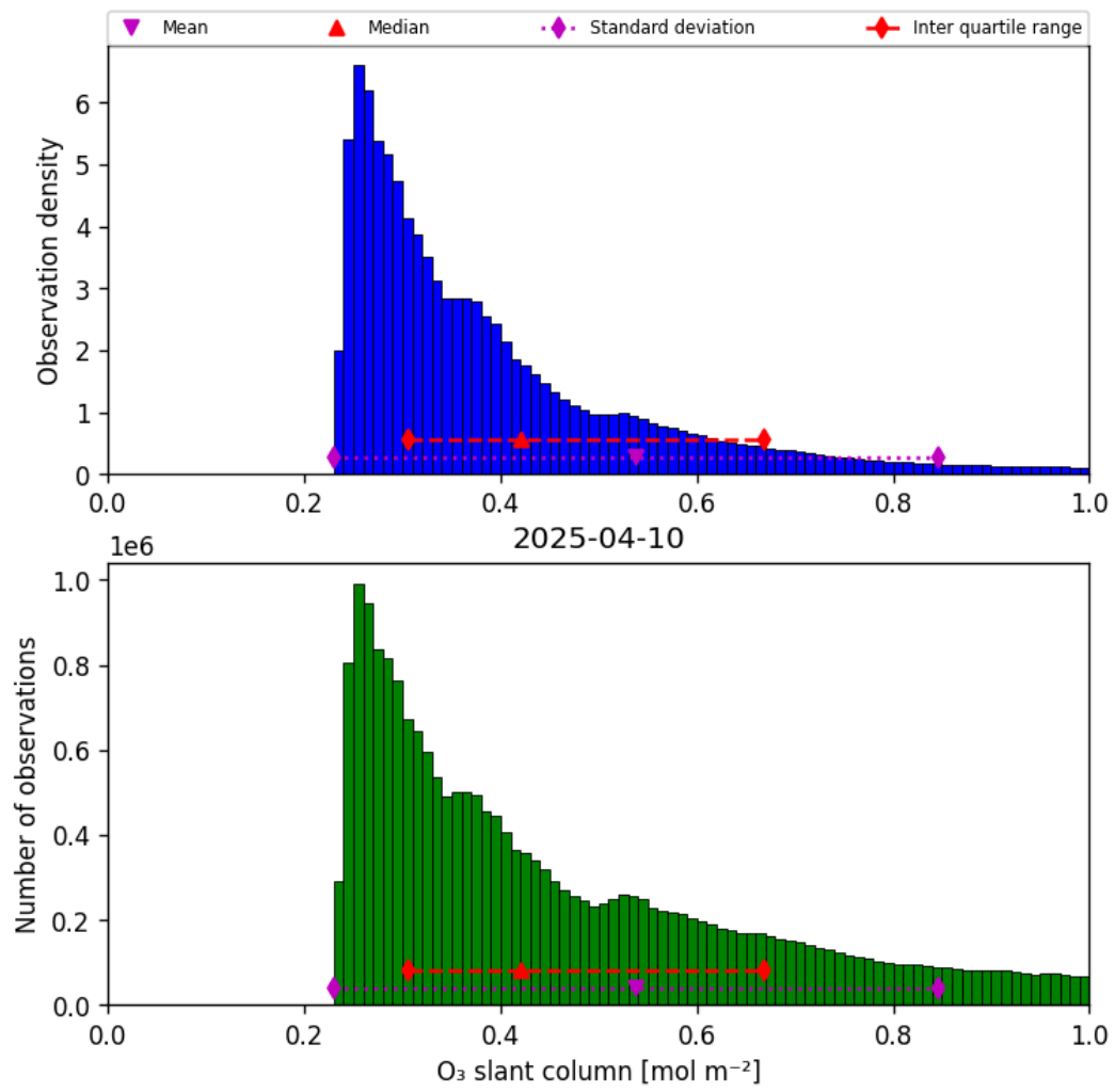
Figure 31: Histogram of “O 3 slant column” for 2025-04-10 to 2025-04-11
