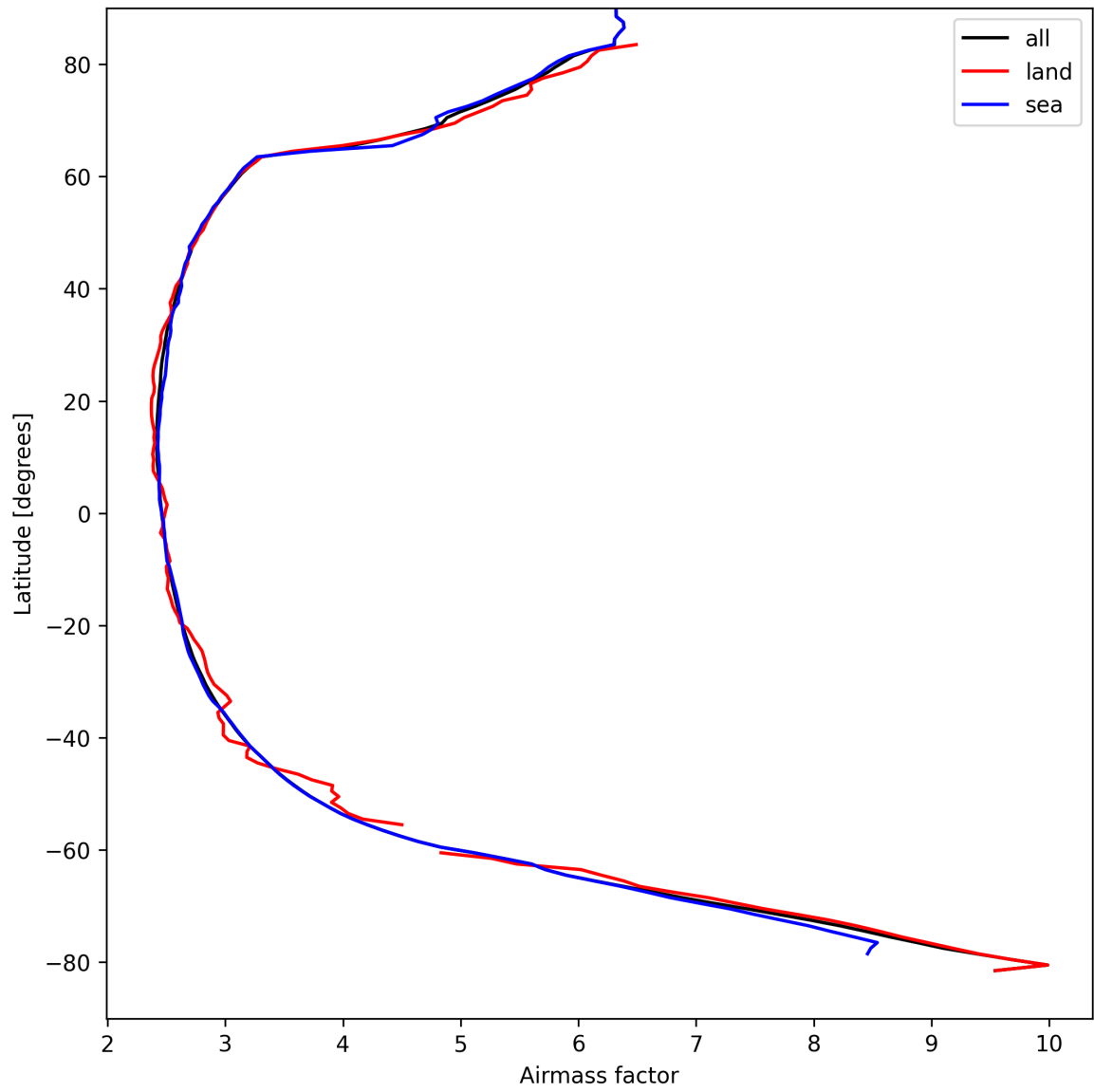
Figure 25: Zonal average of “Airmass factor” for 2025-04-10 to 2025-04-11.
