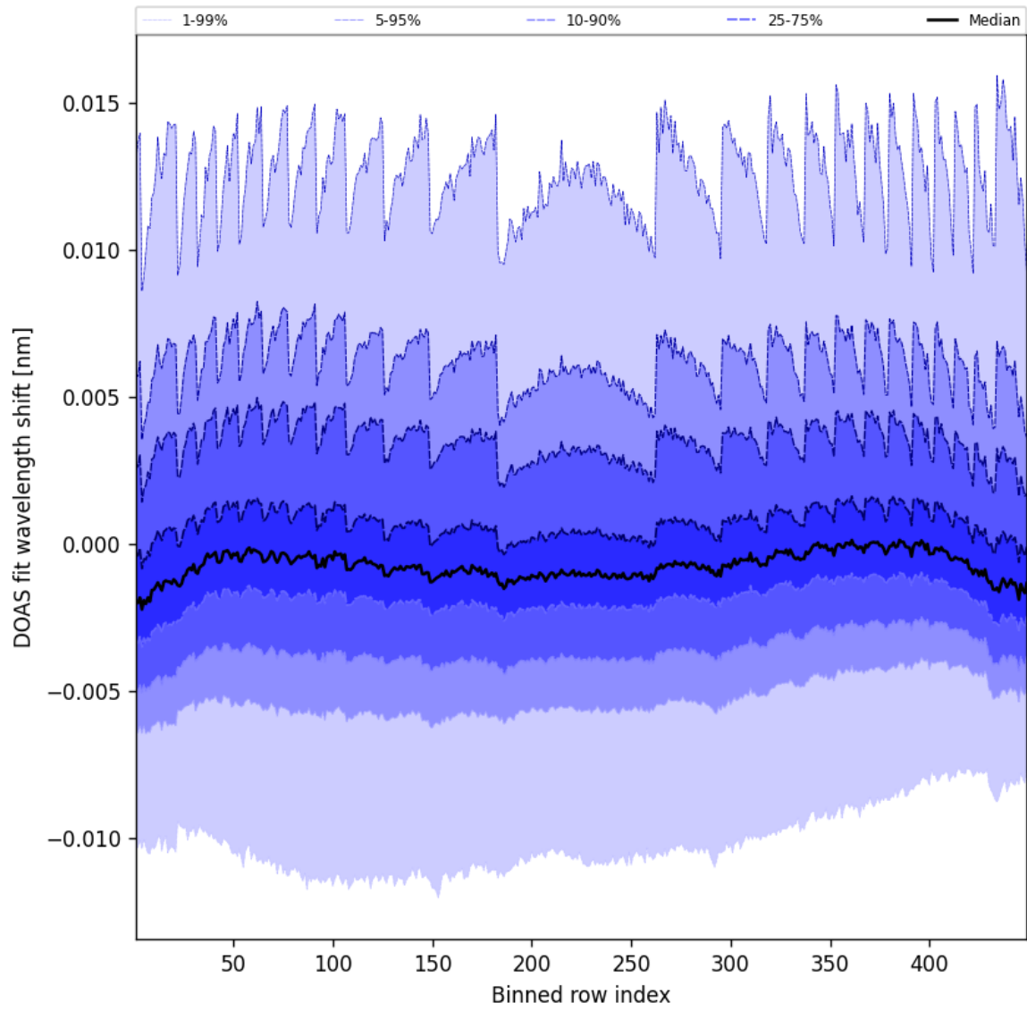
Figure 47: Along track statistics of “DOAS fit wavelength shift” for 2025-04-10 to 2025-04-11
