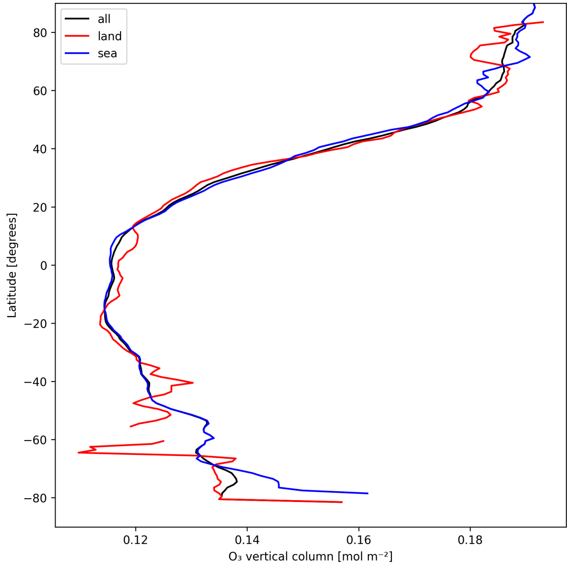
Figure 17: Zonal average of “O 3 vertical column” for 2025-04-10 to 2025-04-11.
