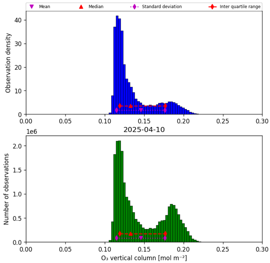
Figure 29: Histogram of “O 3 vertical column” for 2025-04-10 to 2025-04-11
