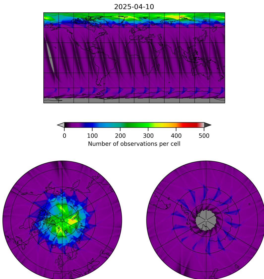
Figure 15: Map of the number of observations for 2025-04-10 to 2025-04-11
