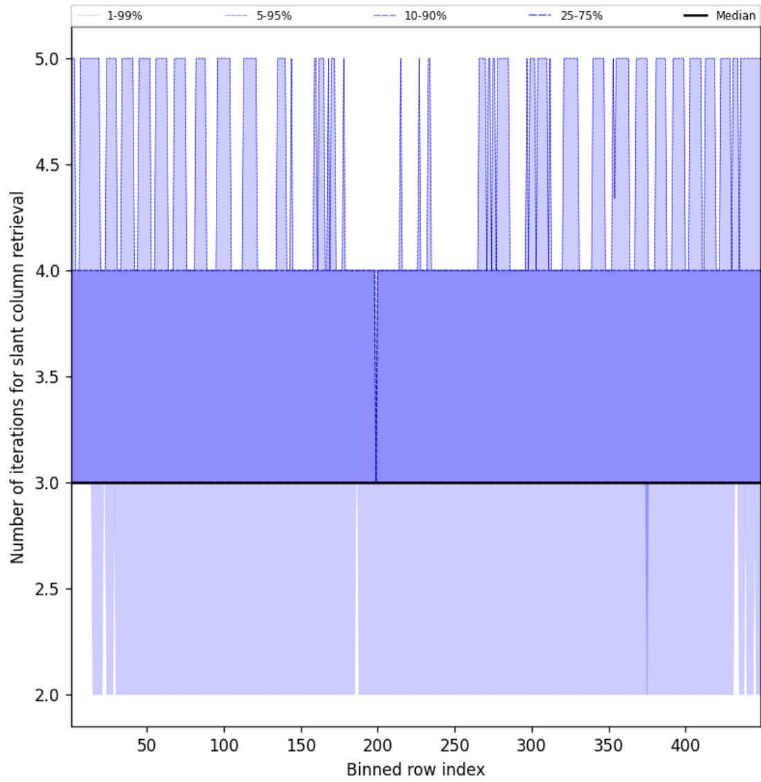
Figure 45: Along track statistics of “Number of iterations for slant column retrieval” for 2025-04-10 to 2025-04-11
