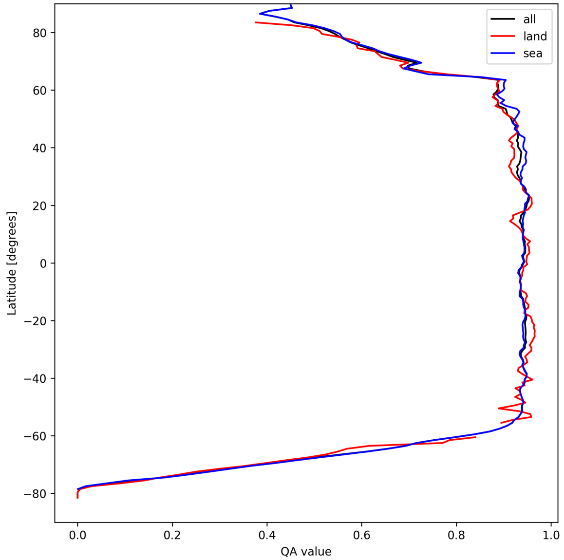
Figure 16: Zonal average of “QA value” for 2025-04-10 to 2025-04-11.
