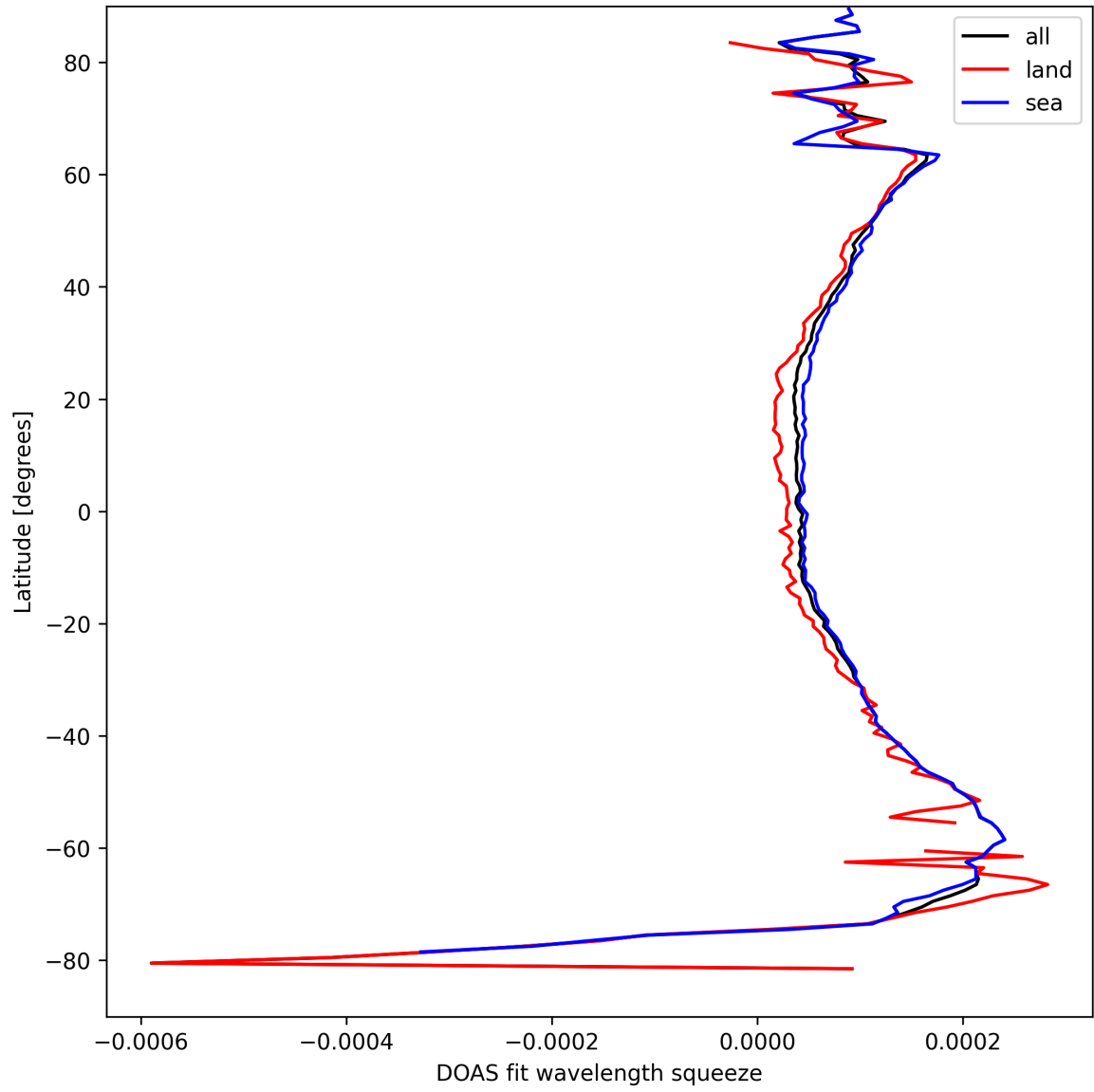
Figure 24: Zonal average of “DOAS fit wavelength squeeze” for 2025-04-10 to 2025-04-11.
