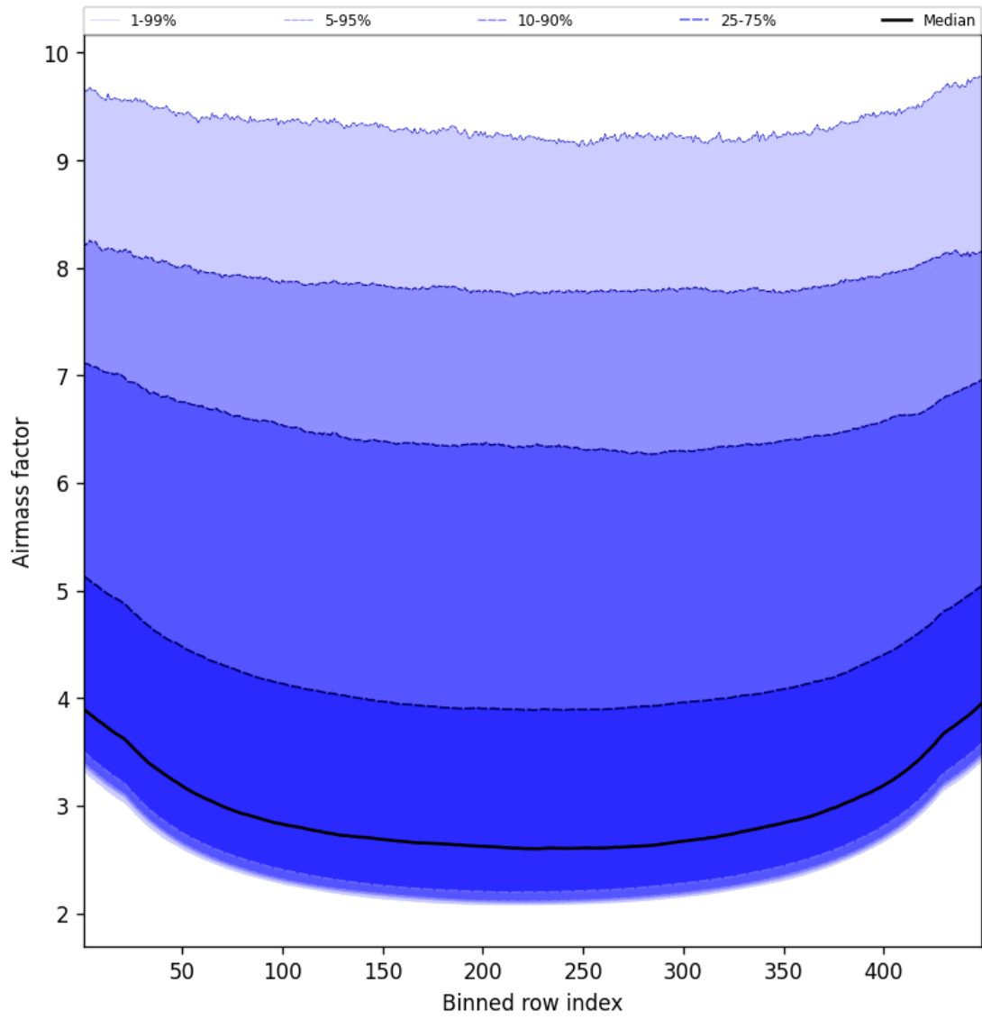
Figure 49: Along track statistics of “Airmass factor” for 2025-04-10 to 2025-04-11
