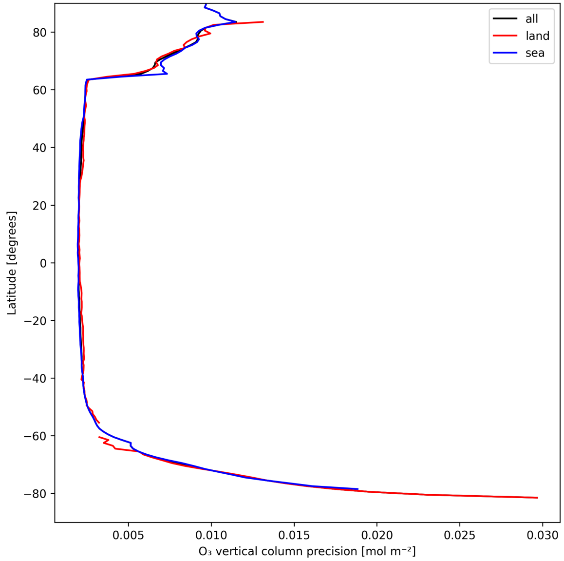
Figure 18: Zonal average of "O 3 vertical column precision" for 2025-04-10 to 2025-04-11.
