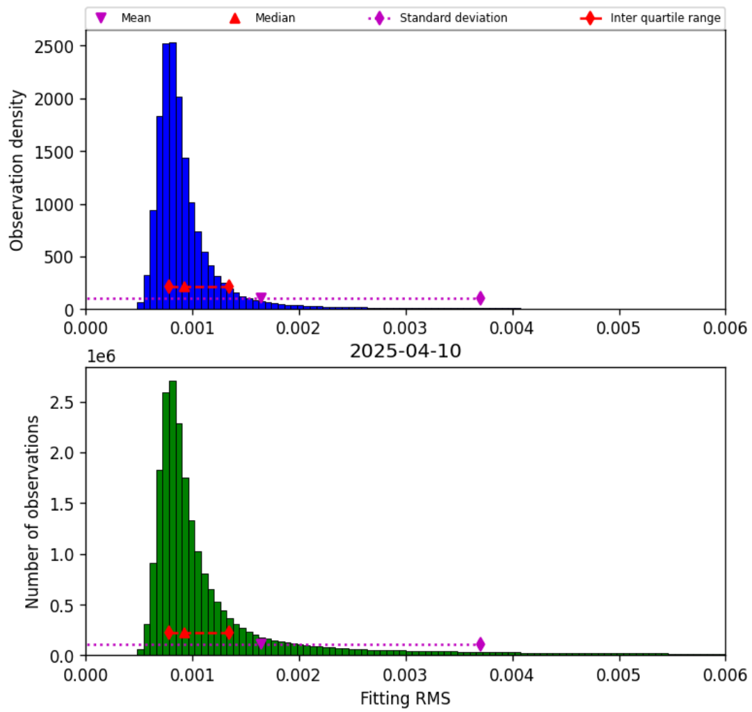
Figure 34: Histogram of “Fitting RMS” for 2025-04-10 to 2025-04-11
