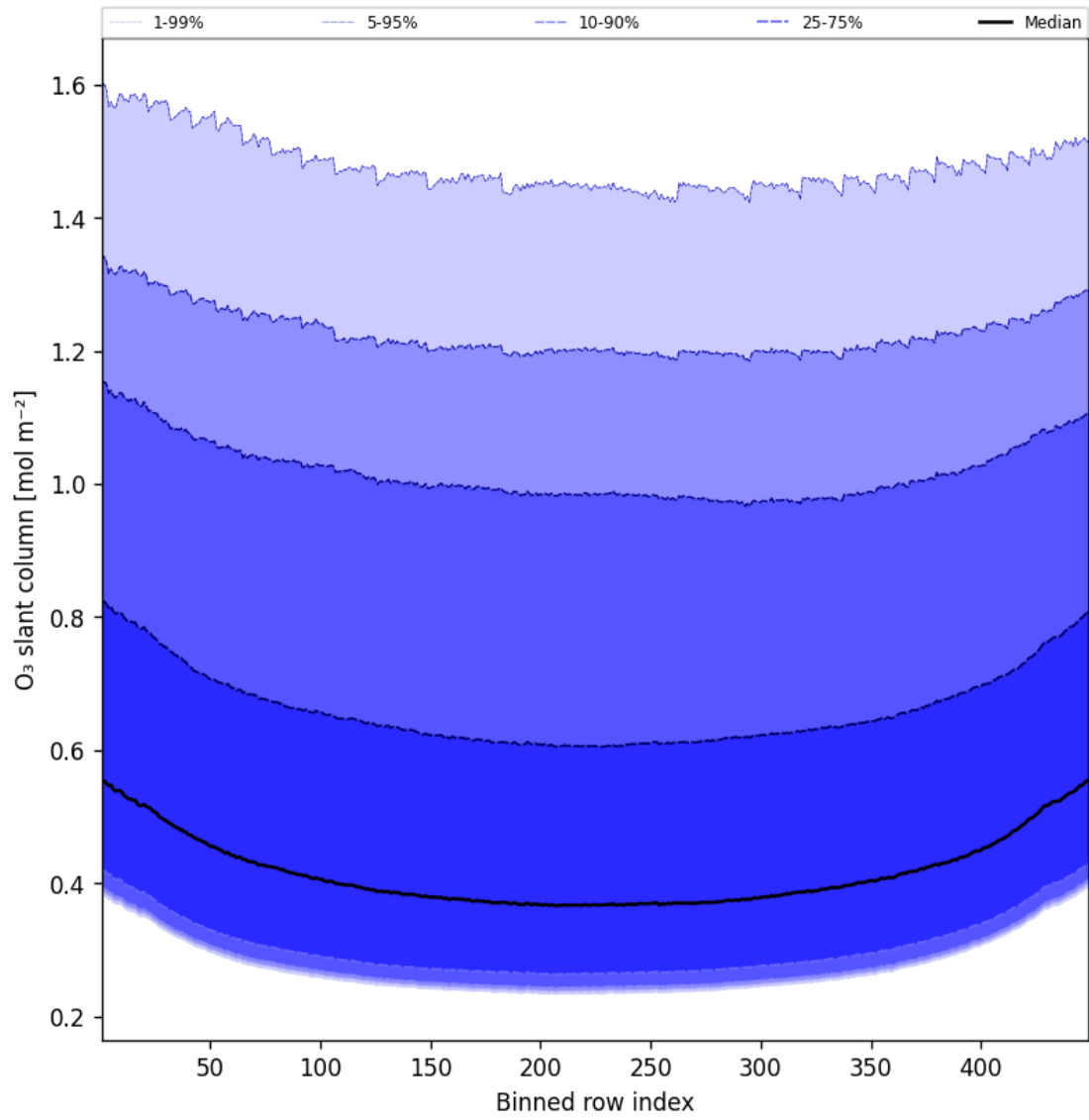
Figure 43: Along track statistics of “O 3 slant column” for 2025-04-10 to 2025-04-11
