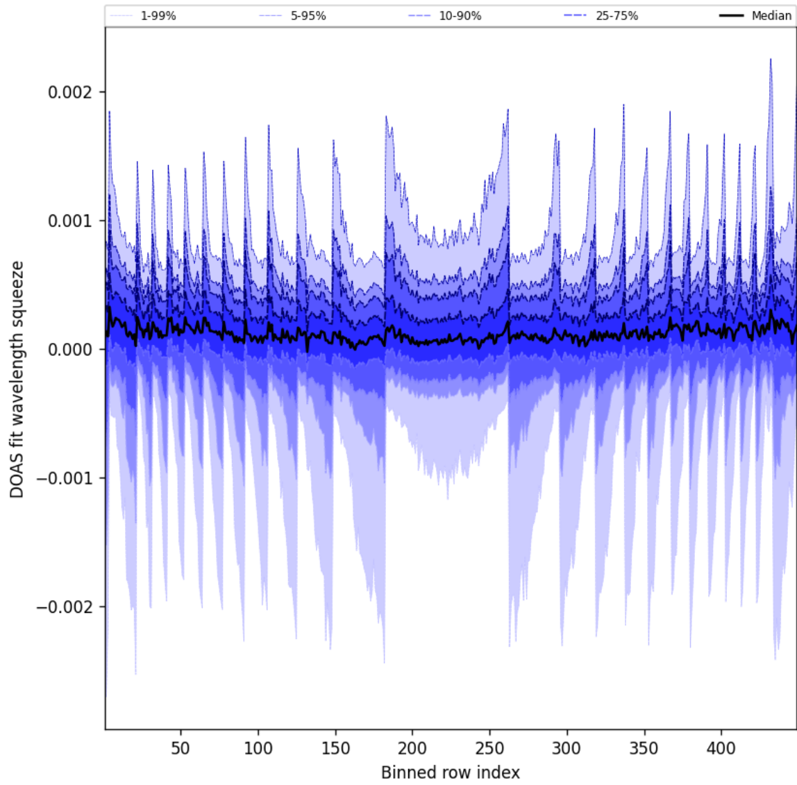
Figure 48: Along track statistics of “DOAS fit wavelength squeeze” for 2025-04-10 to 2025-04-11
