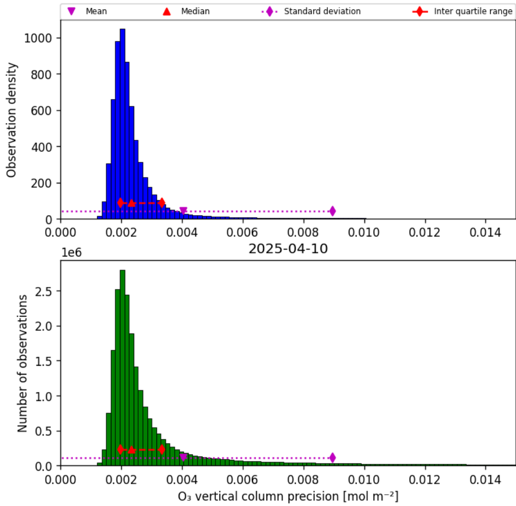
Figure 30: Histogram of “O 3 vertical column precision” for 2025-04-10 to 2025-04-11
