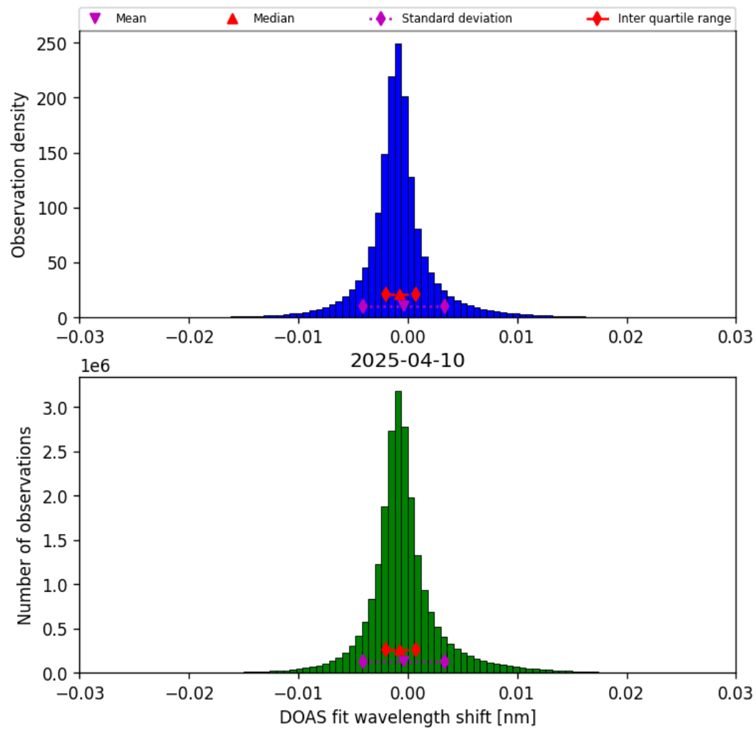
Figure 35: Histogram of “DOAS fit wavelength shift” for 2025-04-10 to 2025-04-11
