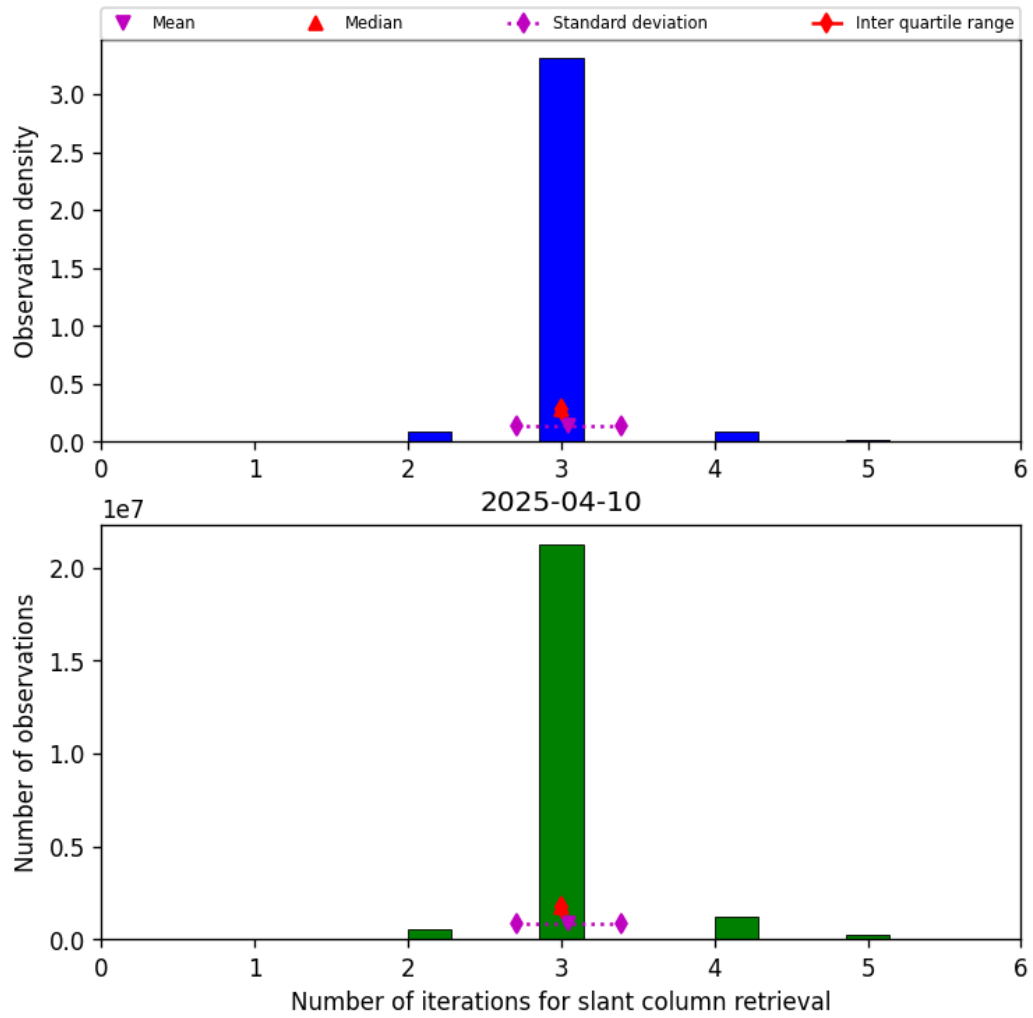
Figure 33: Histogram of “Number of iterations for slant column retrieval” for 2025-04-10 to 2025-04-11
