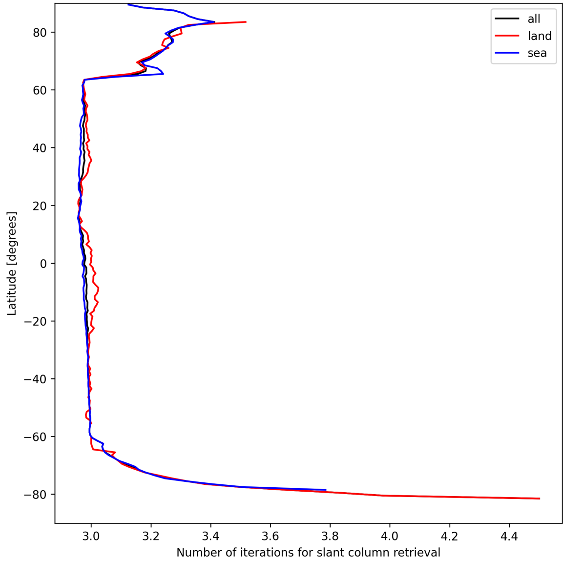
Figure 21: Zonal average of “Number of iterations for slant column retrieval” for 2025-04-10 to 2025-04-11.
