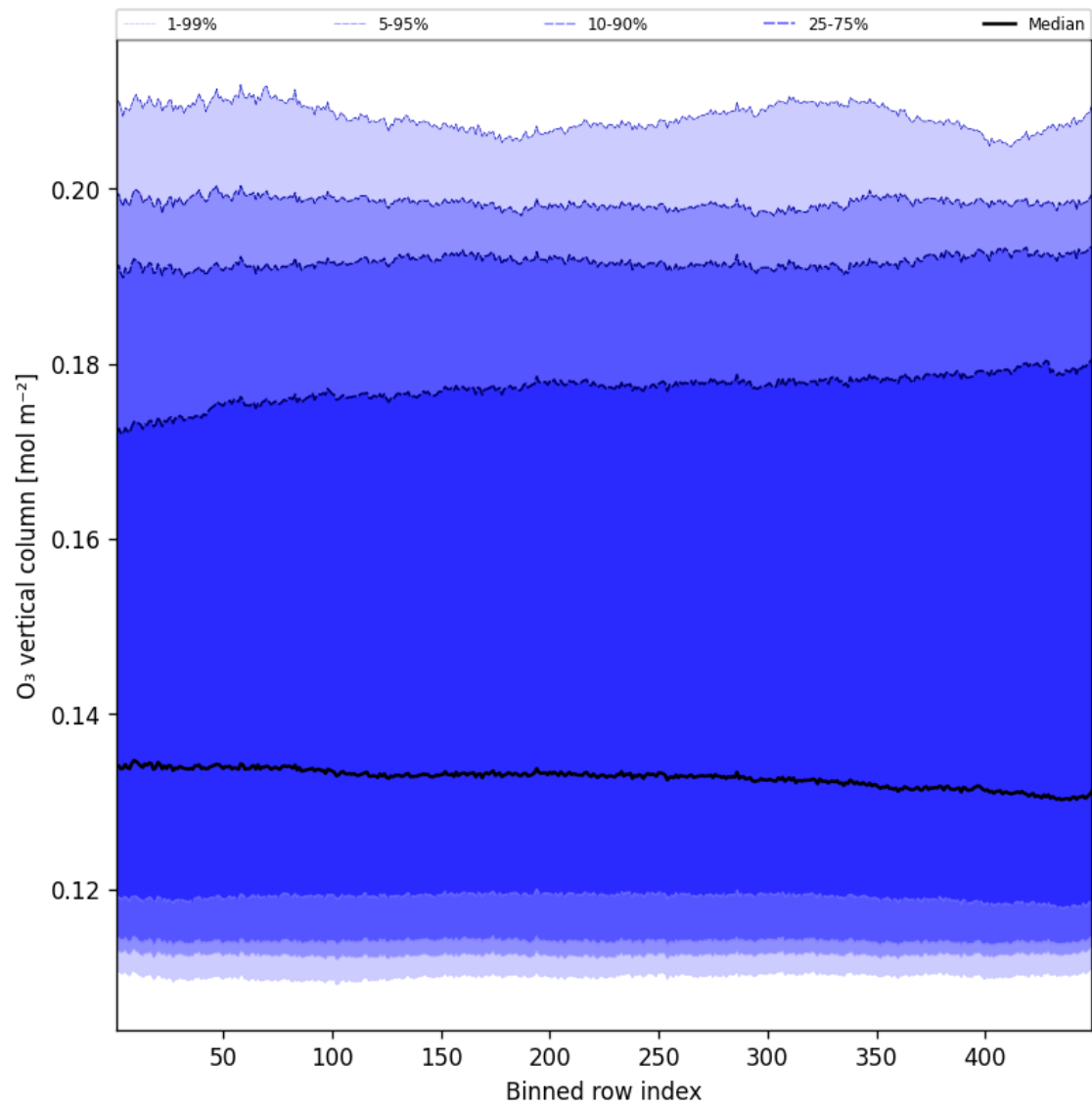
Figure 41: Along track statistics of “O 3 vertical column” for 2025-04-10 to 2025-04-11
