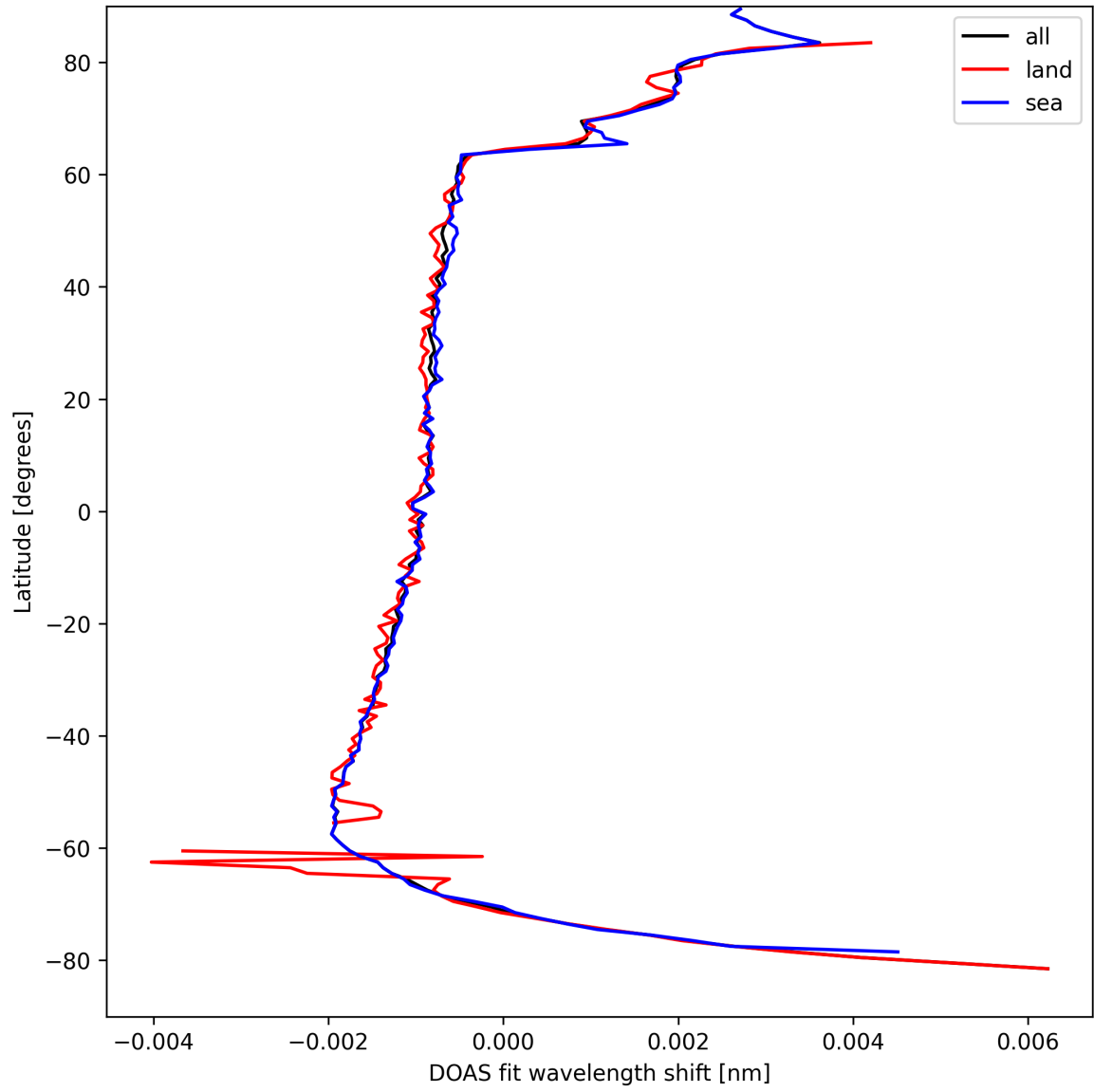
Figure 23: Zonal average of “DOAS fit wavelength shift” for 2025-04-10 to 2025-04-11.
