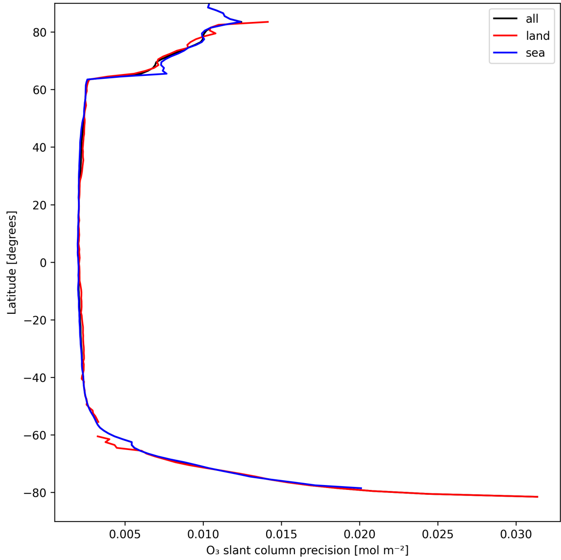
Figure 20: Zonal average of “O 3 slant column precision” for 2025-04-10 to 2025-04-11.
