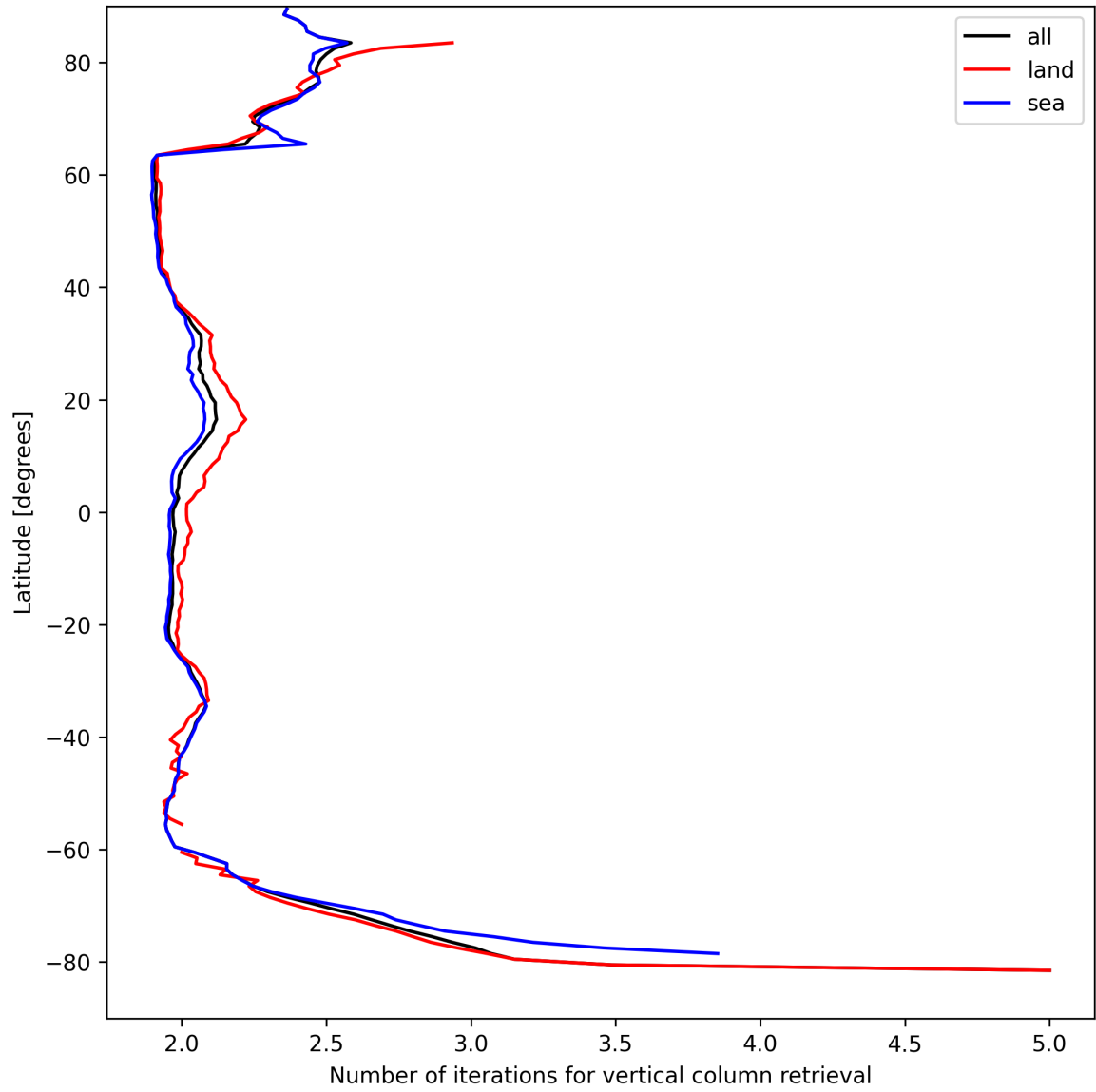
Figure 27: Zonal average of “Number of iterations for vertical column retrieval” for 2025-04-10 to 2025-04-11.
