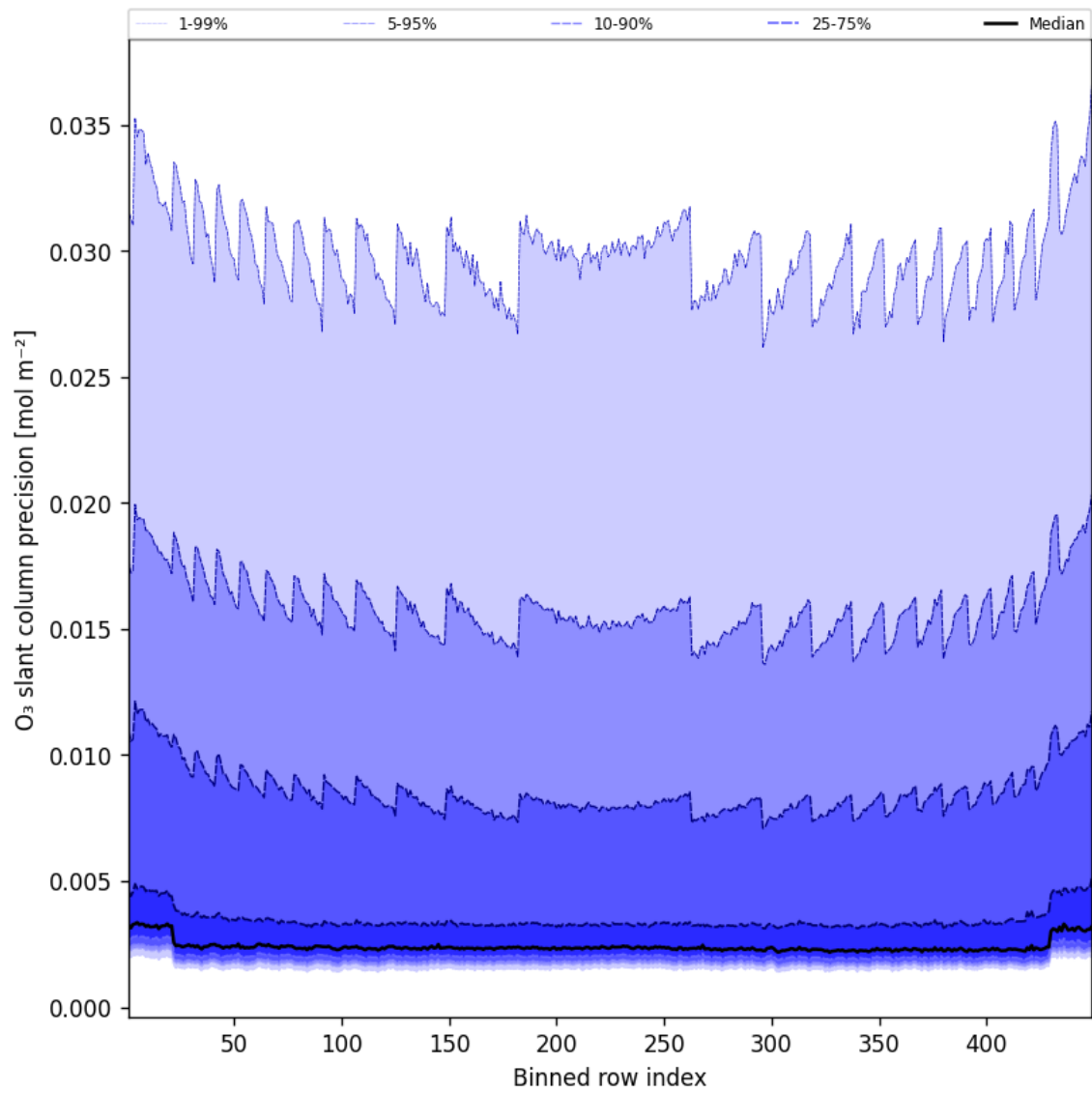
Figure 44: Along track statistics of “O 3 slant column precision” for 2025-04-10 to 2025-04-11
