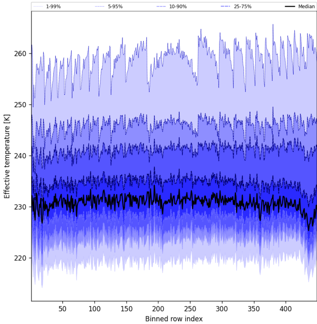
Figure 50: Along track statistics of “Effective temperature” for 2025-04-10 to 2025-04-11
