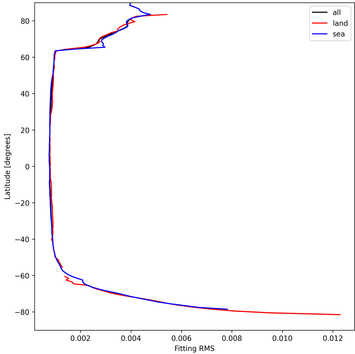
Figure 22: Zonal average of “Fitting RMS” for 2025-04-10 to 2025-04-11.
