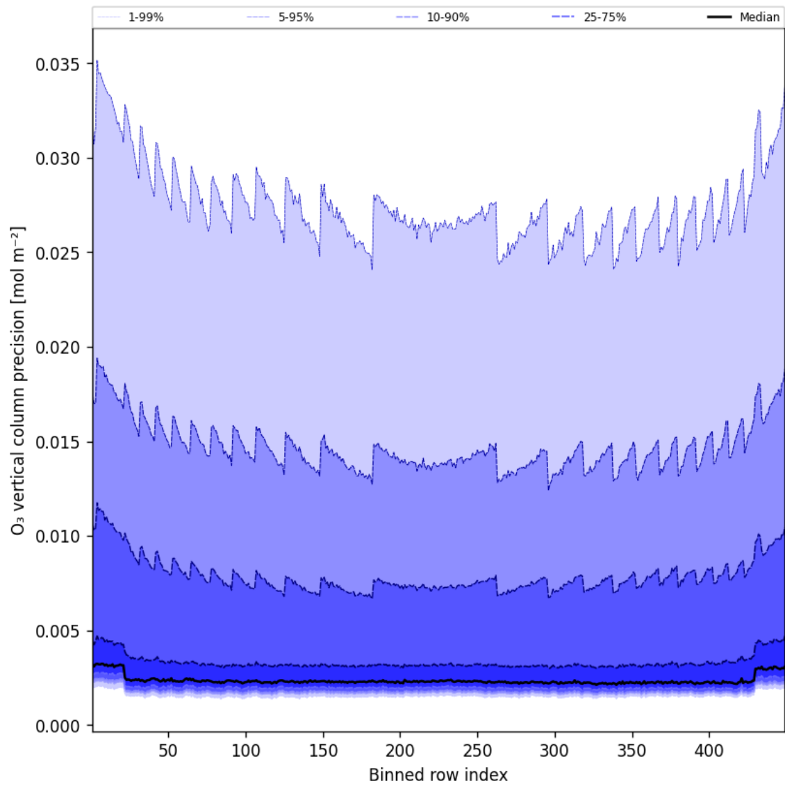
Figure 42: Along track statistics of “O 3 vertical column precision” for 2025-04-11 to 2025-04-11
