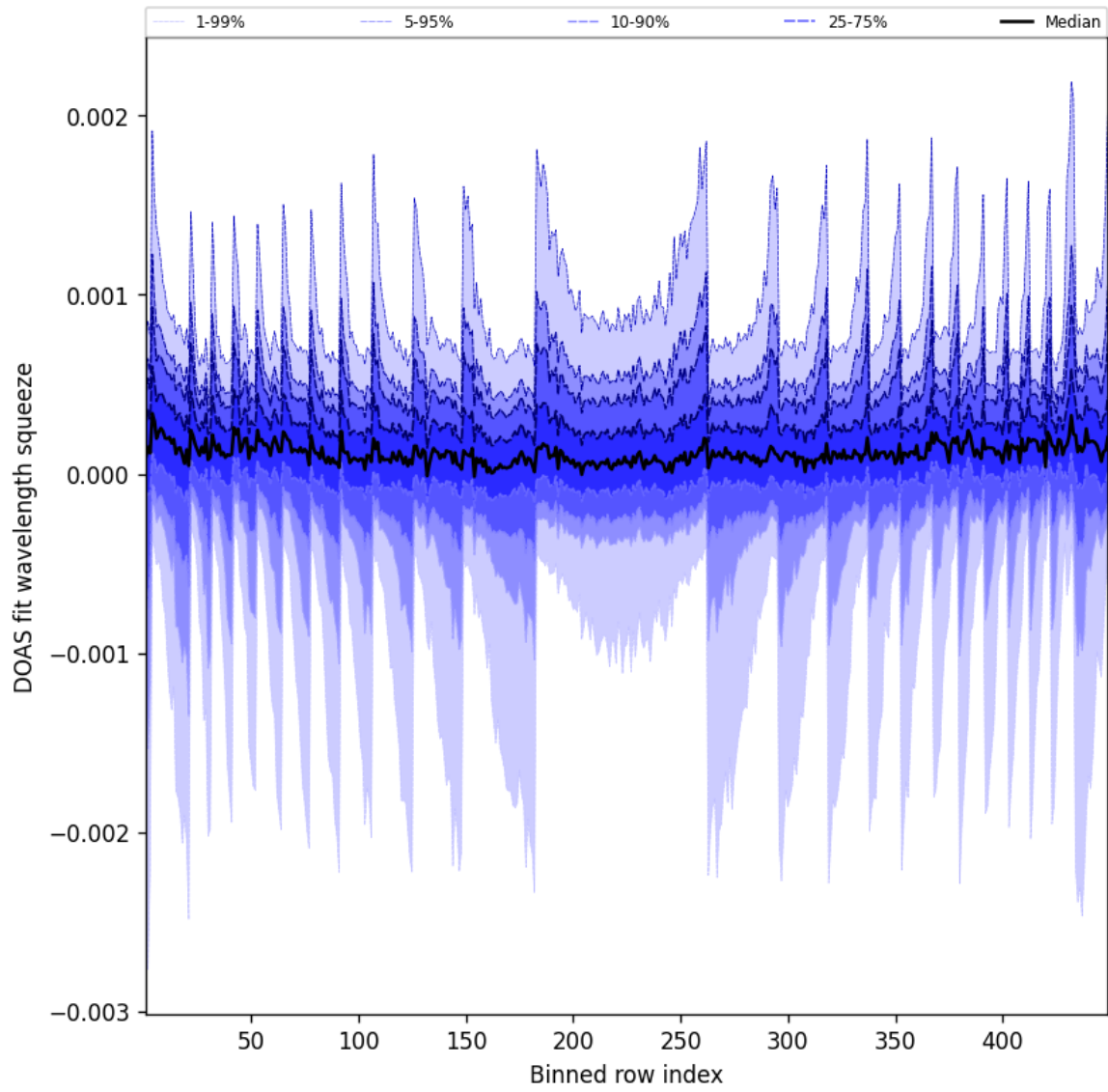
Figure 48: Along track statistics of “DOAS fit wavelength squeeze” for 2025-04-11 to 2025-04-11
