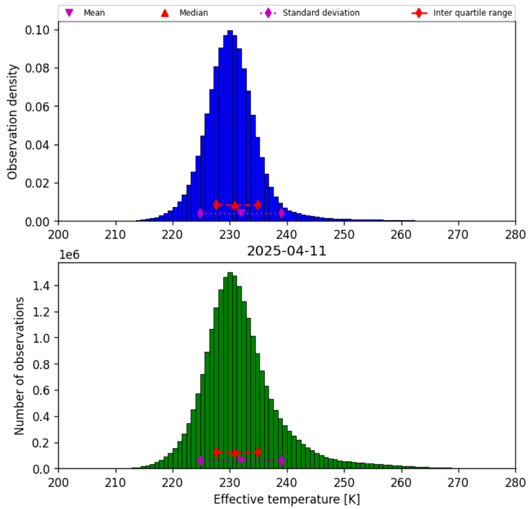
Figure 38: Histogram of “Effective temperature” for 2025-04-11 to 2025-04-11
