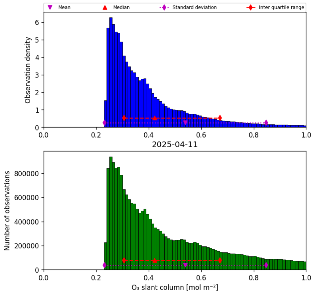
Figure 31: Histogram of “O 3 slant column” for 2025-04-11 to 2025-04-11
