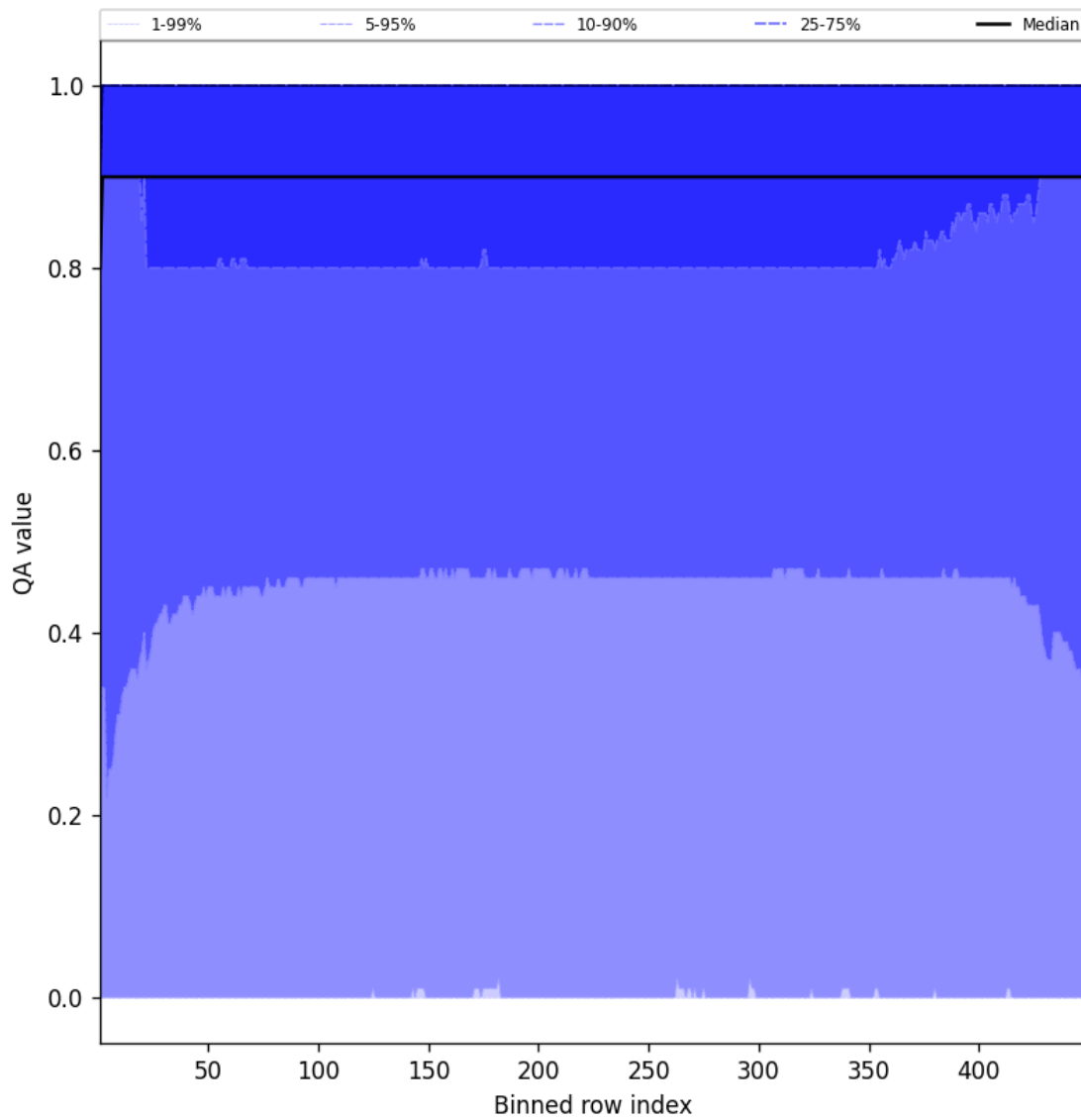
Figure 40: Along track statistics of “QA value” for 2025-04-11 to 2025-04-11
