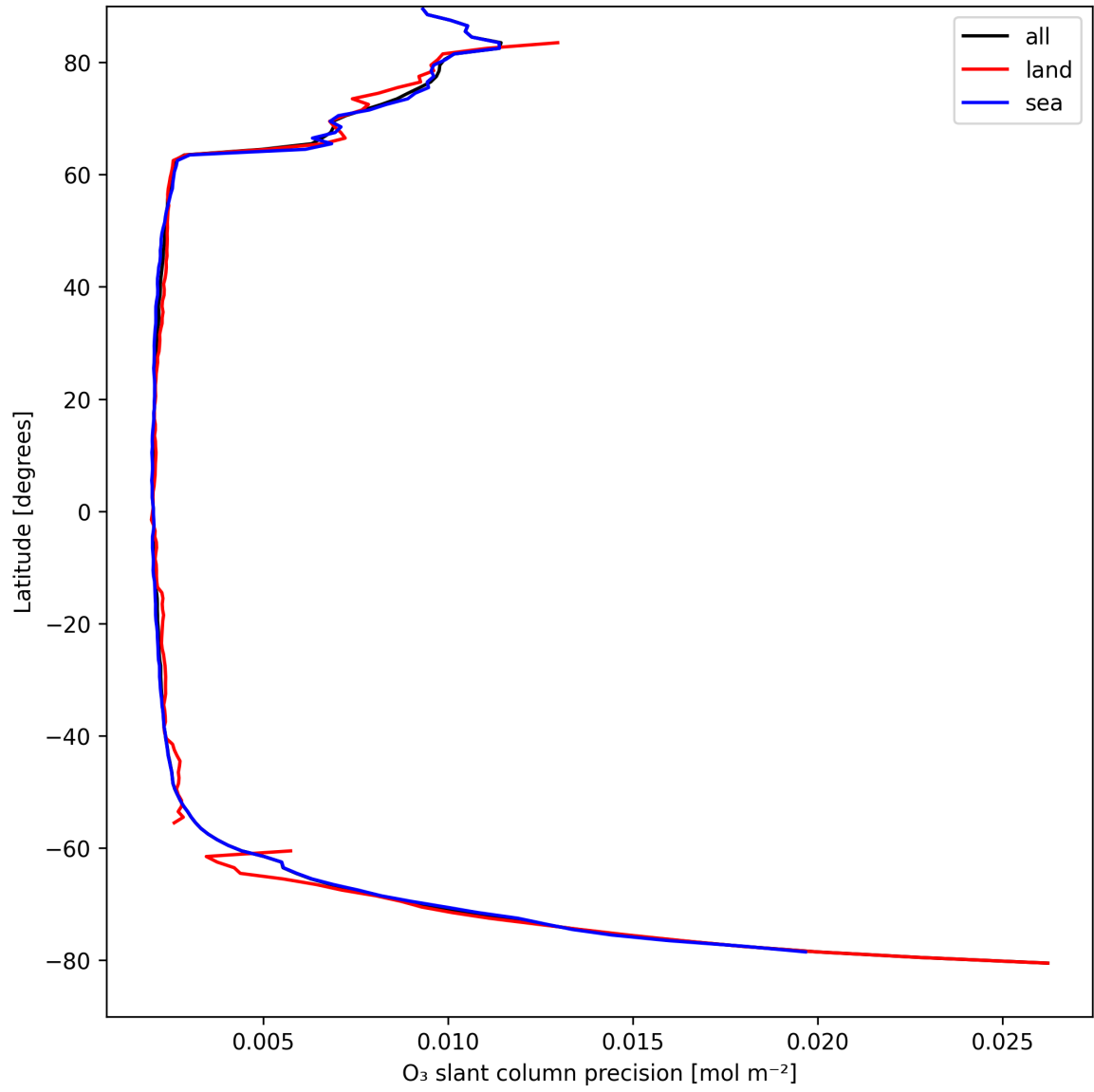
Figure 20: Zonal average of “O 3 slant column precision” for 2025-04-11 to 2025-04-11.
