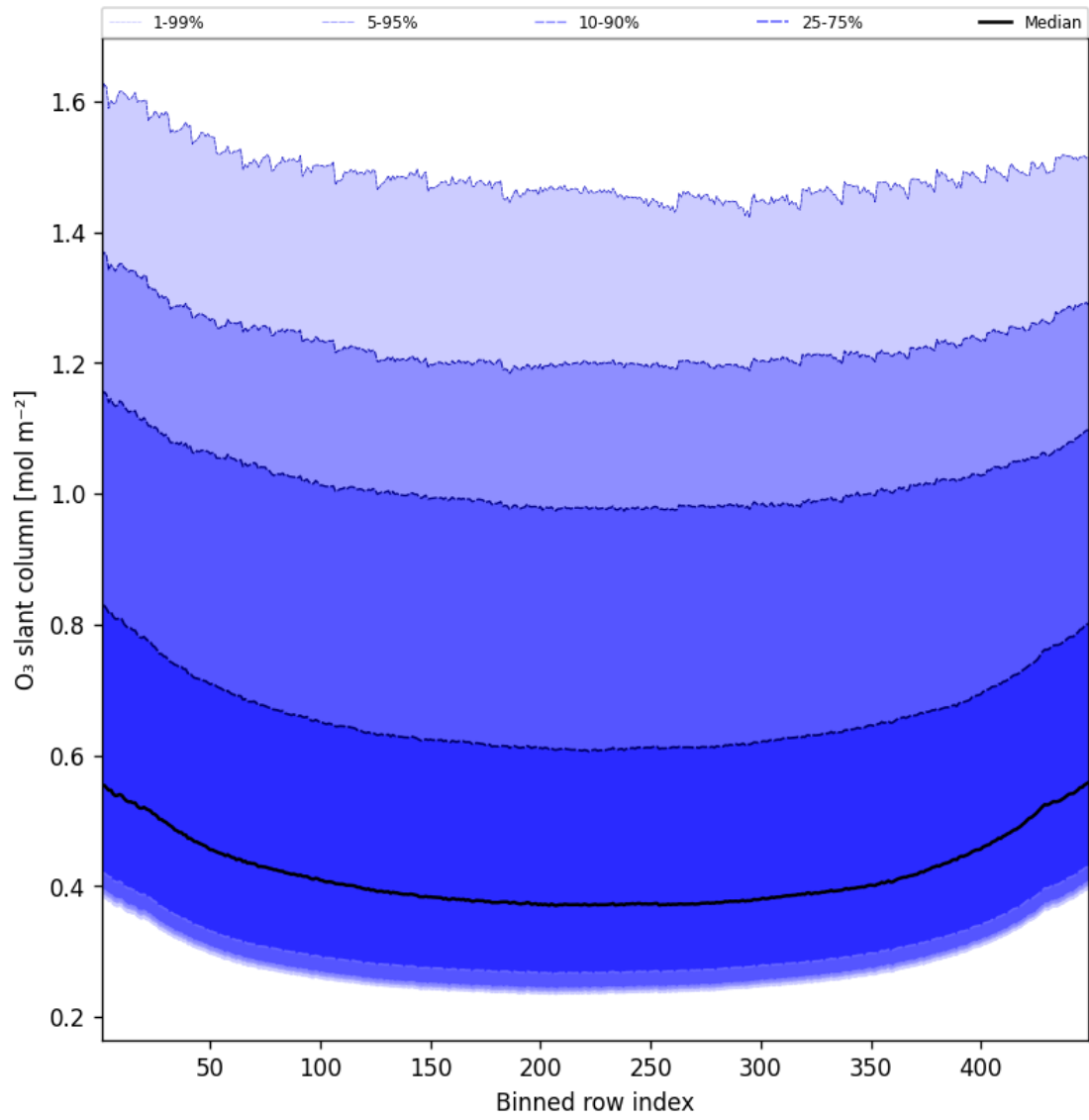
Figure 43: Along track statistics of “O 3 slant column” for 2025-04-11 to 2025-04-11
