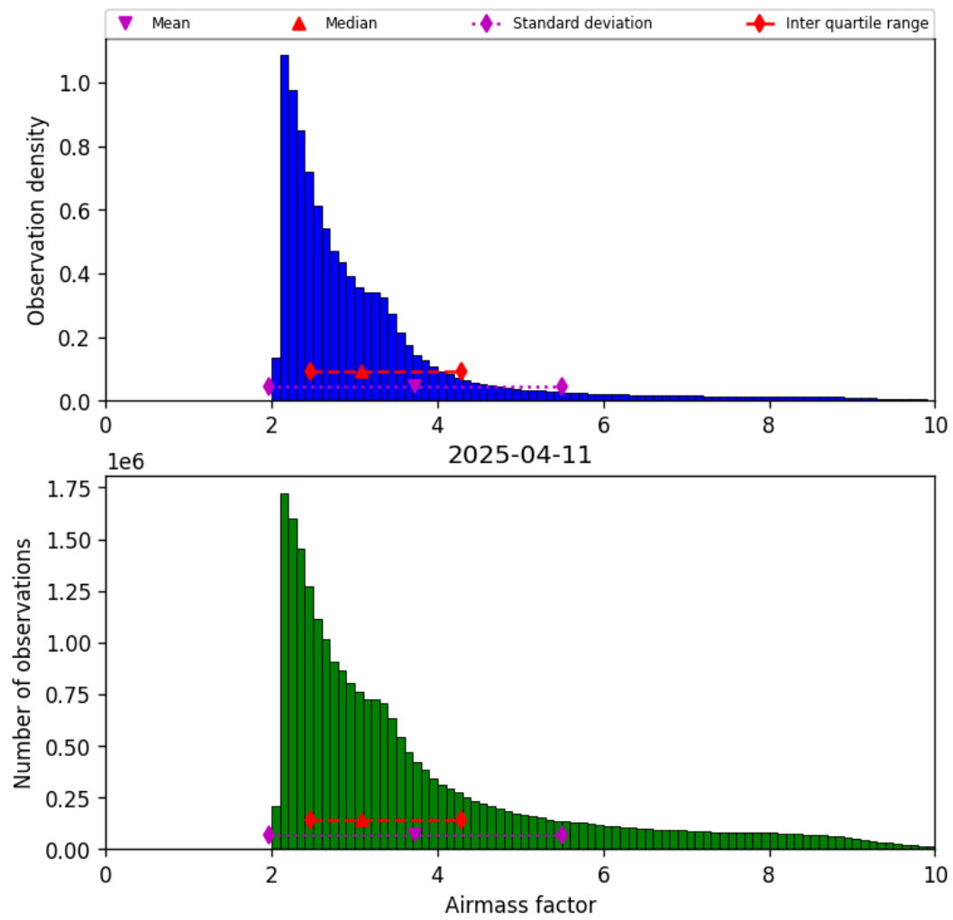
Figure 37: Histogram of “Airmass factor” for 2025-04-11 to 2025-04-11
