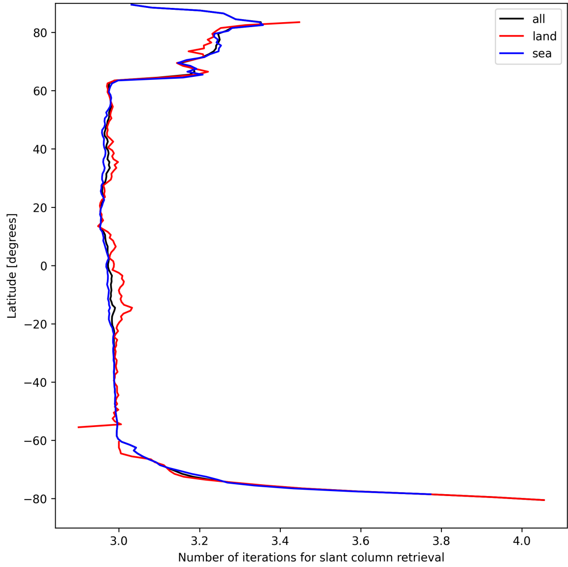
Figure 21: Zonal average of “Number of iterations for slant column retrieval” for 2025-04-11 to 2025-04-11.
