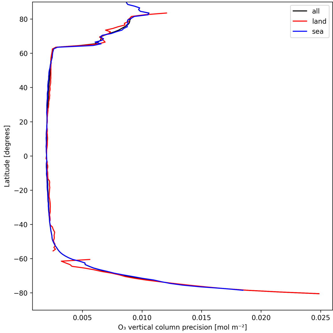
Figure 18: Zonal average of “O 3 vertical column precision” for 2025-04-11 to 2025-04-11.
