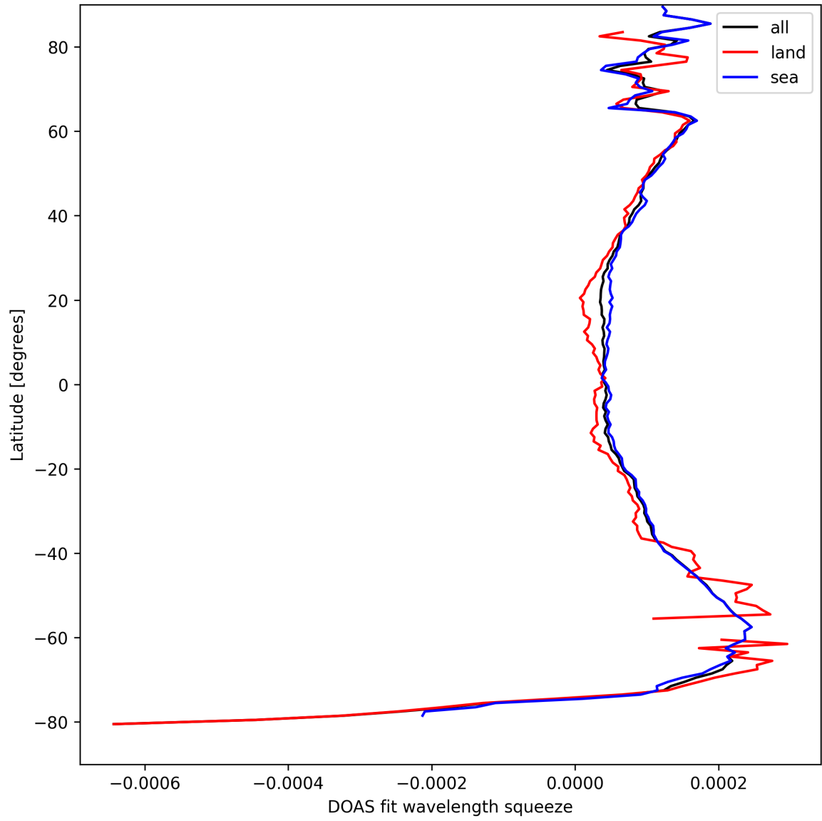
Figure 24: Zonal average of “DOAS fit wavelength squeeze” for 2025-04-11 to 2025-04-11.
