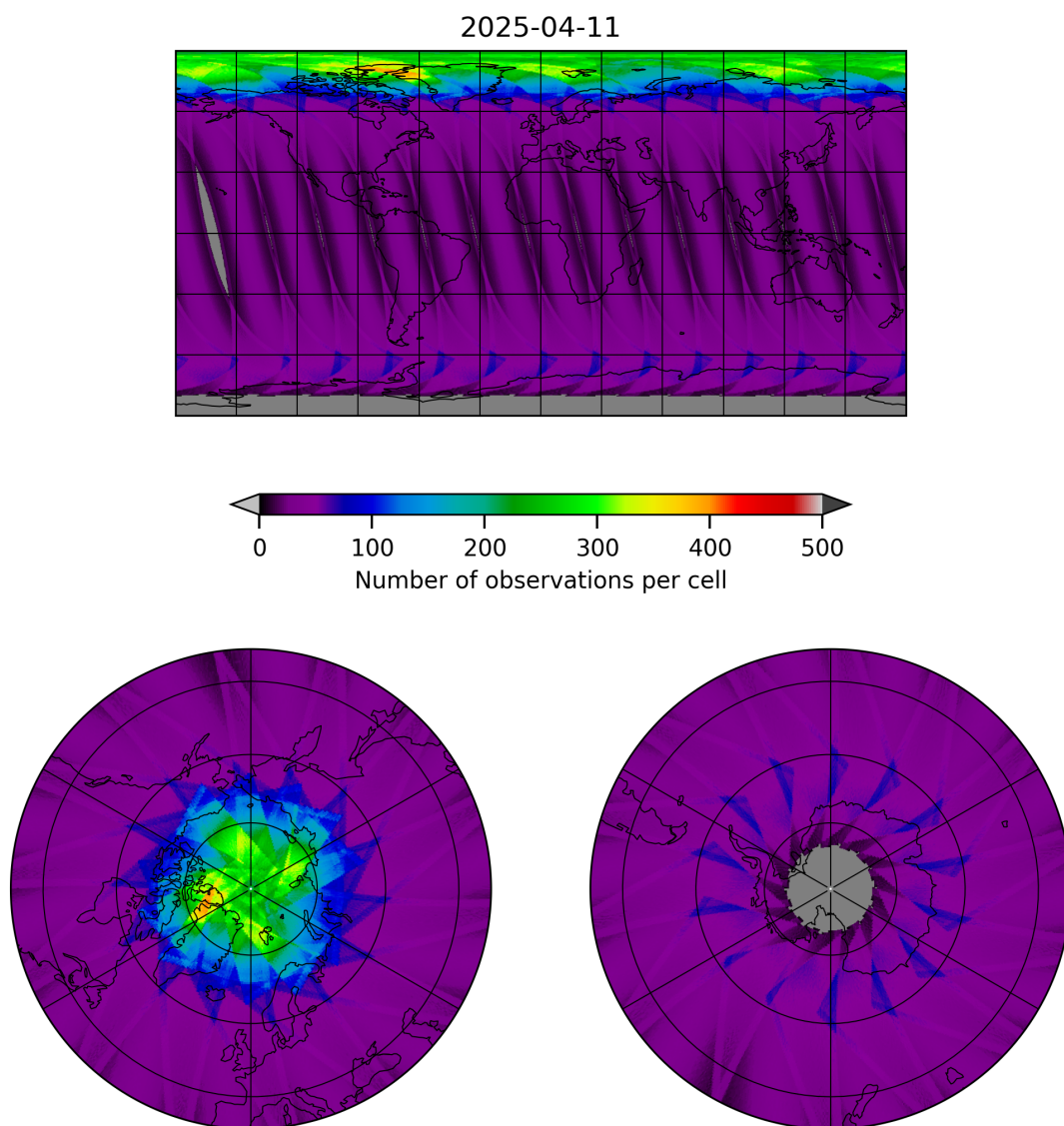
Figure 15: Map of the number of observations for 2025-04-11 to 2025-04-11
