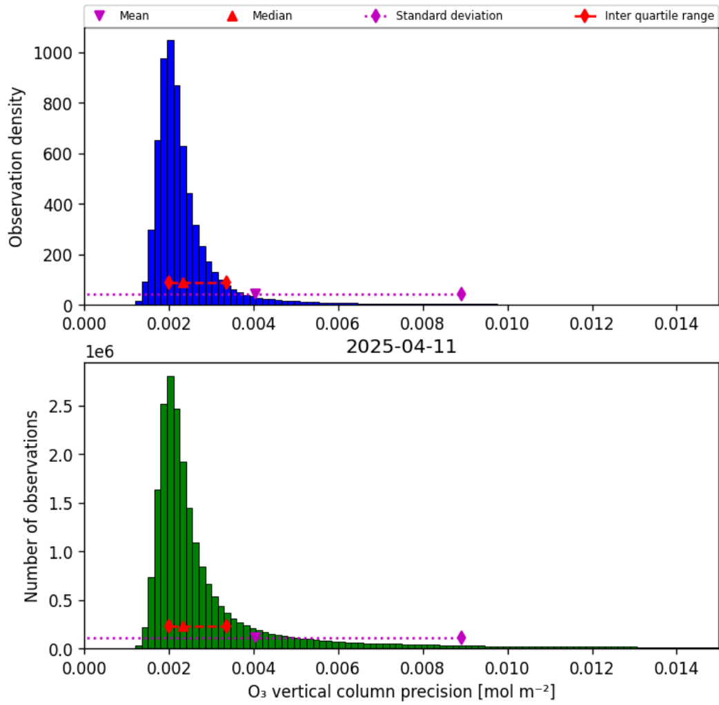
Figure 30: Histogram of “O 3 vertical column precision” for 2025-04-11 to 2025-04-11
