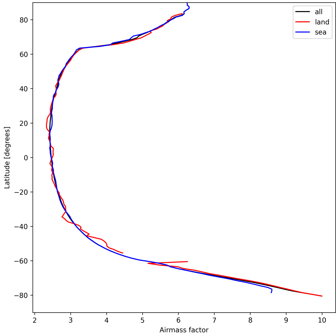
Figure 25: Zonal average of “Airmass factor” for 2025-04-11 to 2025-04-11.
