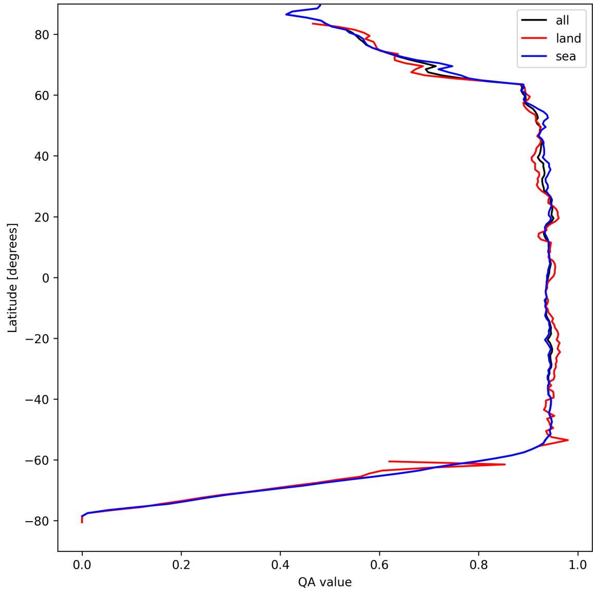
Figure 16: Zonal average of “QA value” for 2025-04-11 to 2025-04-11.
