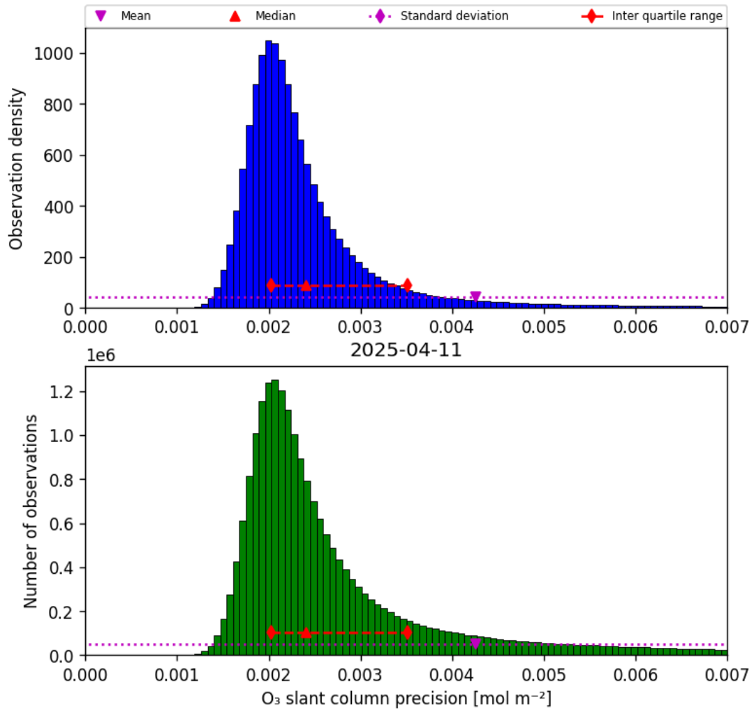
Figure 32: Histogram of “O 3 slant column precision” for 2025-04-11 to 2025-04-11
