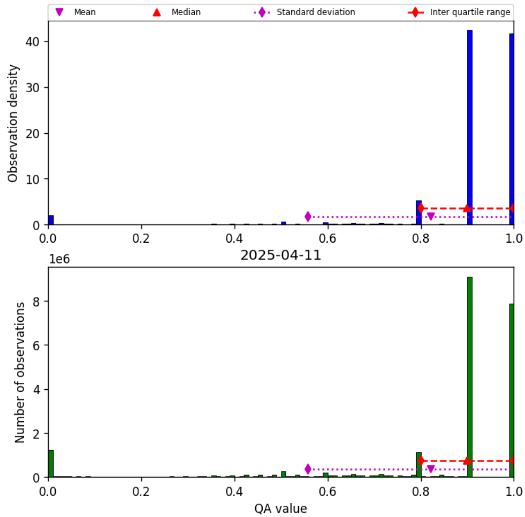
Figure 28: Histogram of “QA value” for 2025-04-11 to 2025-04-11
