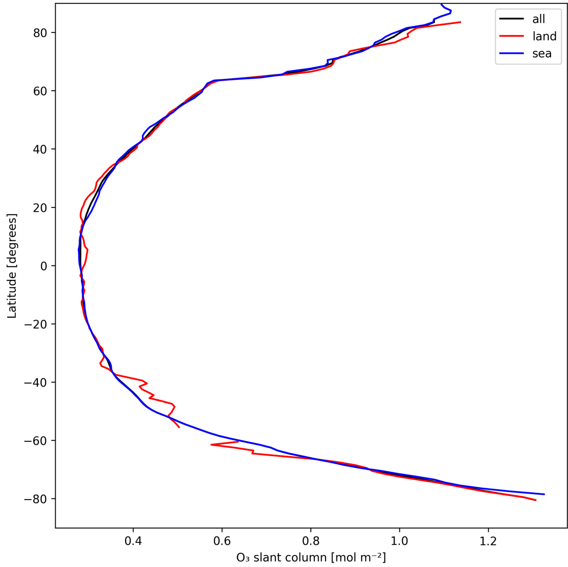
Figure 19: Zonal average of “O 3 slant column” for 2025-04-11 to 2025-04-11.
