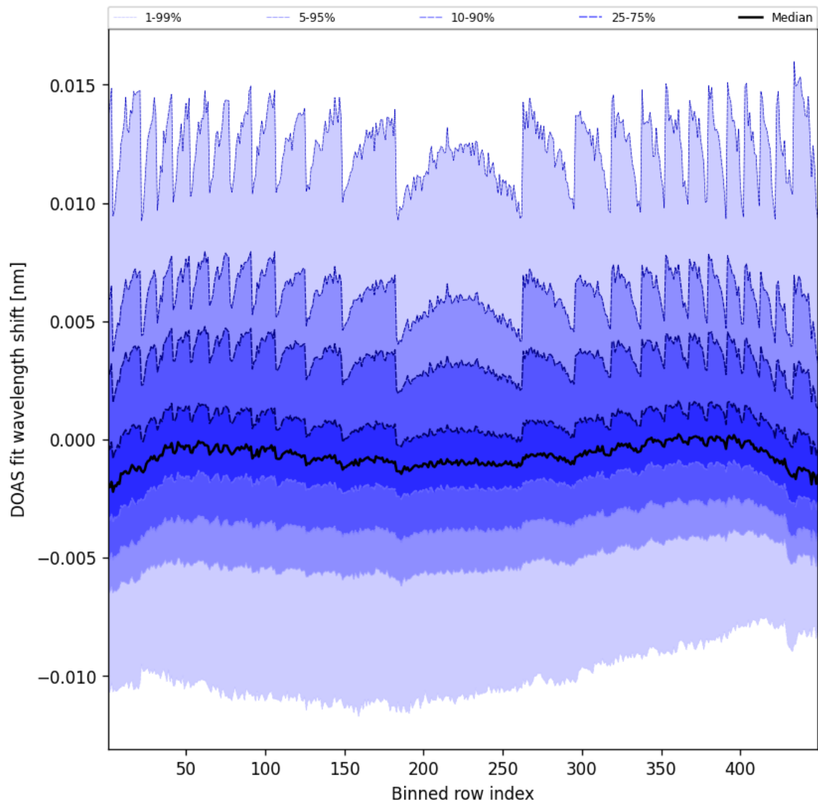
Figure 47: Along track statistics of “DOAS fit wavelength shift” for 2025-04-11 to 2025-04-11
