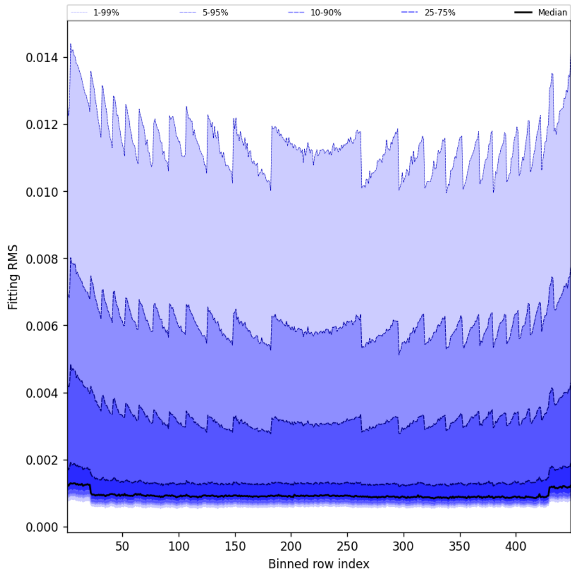
Figure 46: Along track statistics of “Fitting RMS” for 2025-04-11 to 2025-04-11
