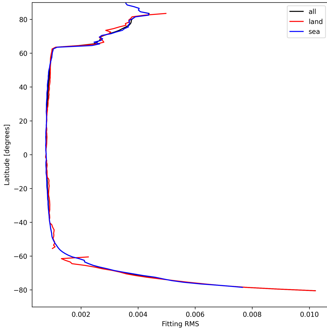
Figure 22: Zonal average of “Fitting RMS” for 2025-04-11 to 2025-04-11.
