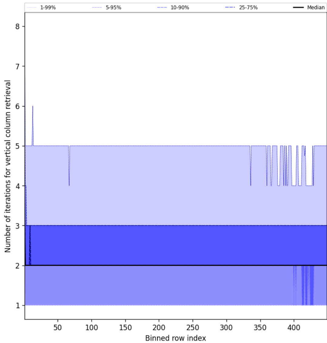
Figure 51: Along track statistics of “Number of iterations for vertical column retrieval” for 2025-04-11 to 2025-04-11
