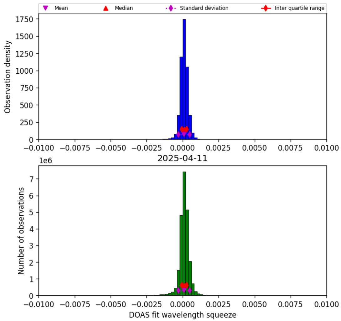
Figure 36: Histogram of “DOAS fit wavelength squeeze” for 2025-04-11 to 2025-04-11
