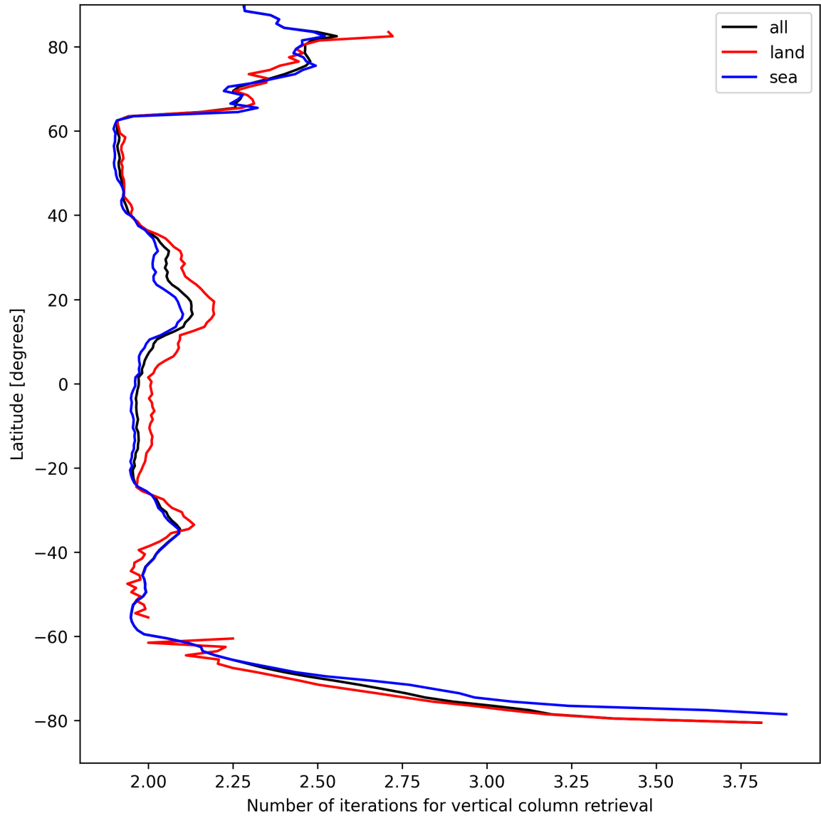
Figure 27: Zonal average of “Number of iterations for vertical column retrieval” for 2025-04-11 to 2025-04-11.
