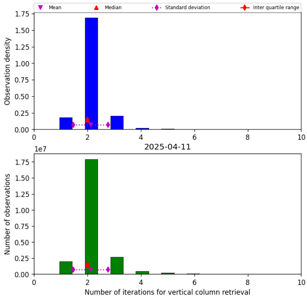
Figure 39: Histogram of “Number of iterations for vertical column retrieval” for 2025-04-11 to 2025-04-11
