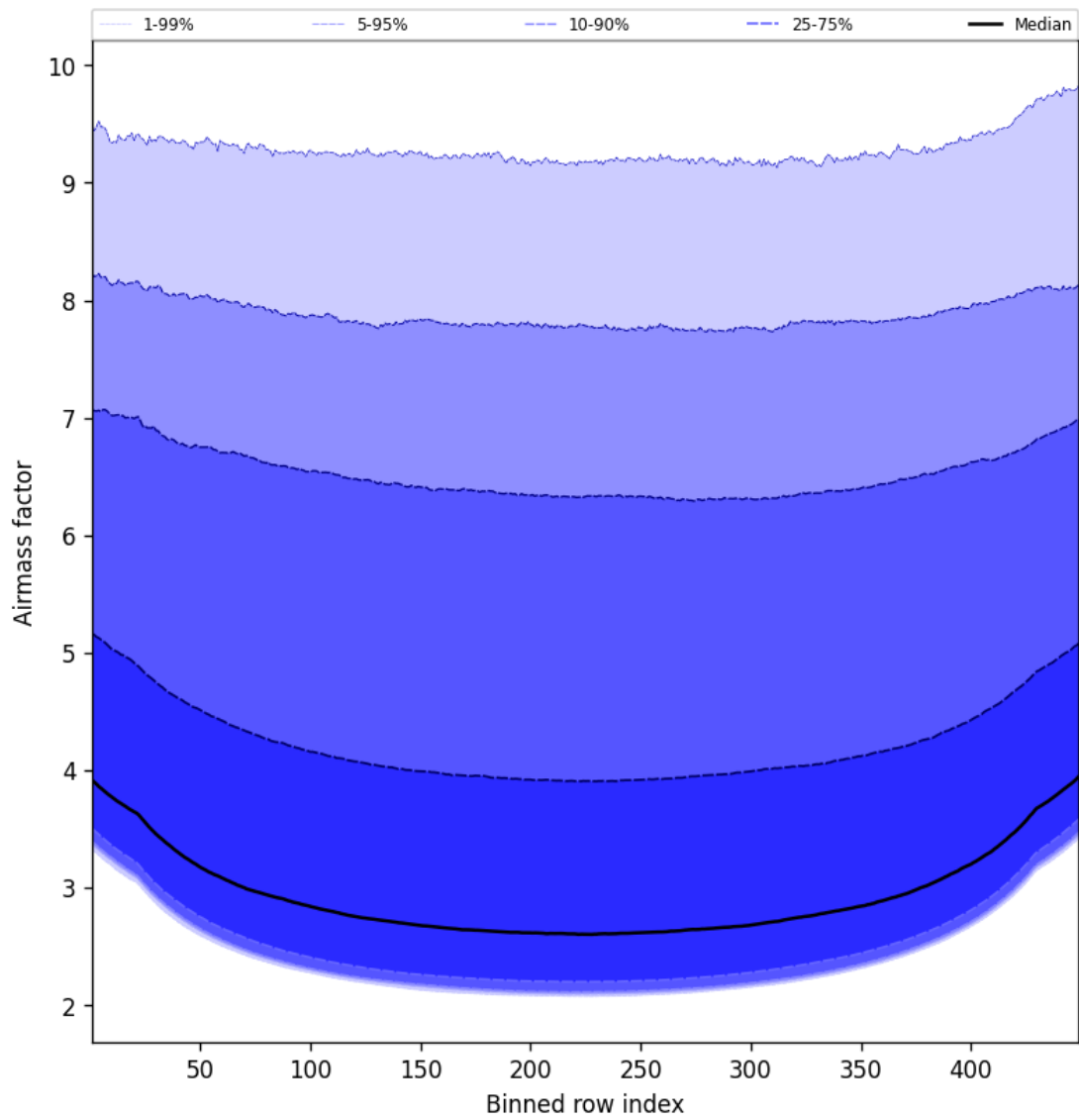
Figure 49: Along track statistics of “Airmass factor” for 2025-04-11 to 2025-04-11
