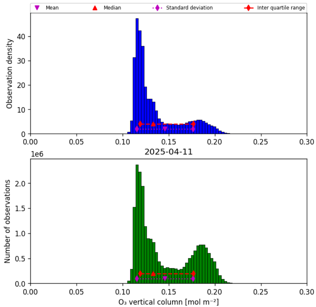
Figure 29: Histogram of “O 3 vertical column” for 2025-04-11 to 2025-04-11
