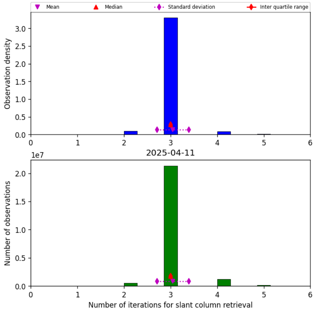
Figure 33: Histogram of “Number of iterations for slant column retrieval” for 2025-04-11 to 2025-04-11
