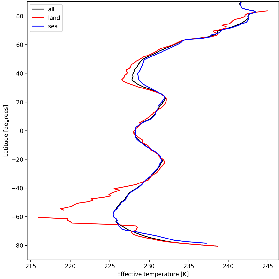
Figure 26: Zonal average of “Effective temperature” for 2025-04-11 to 2025-04-11.
