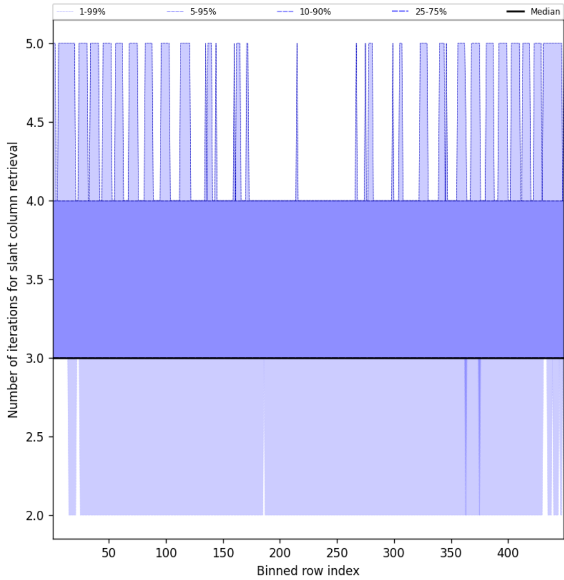
Figure 45: Along track statistics of “Number of iterations for slant column retrieval” for 2025-04-11 to 2025-04-11
