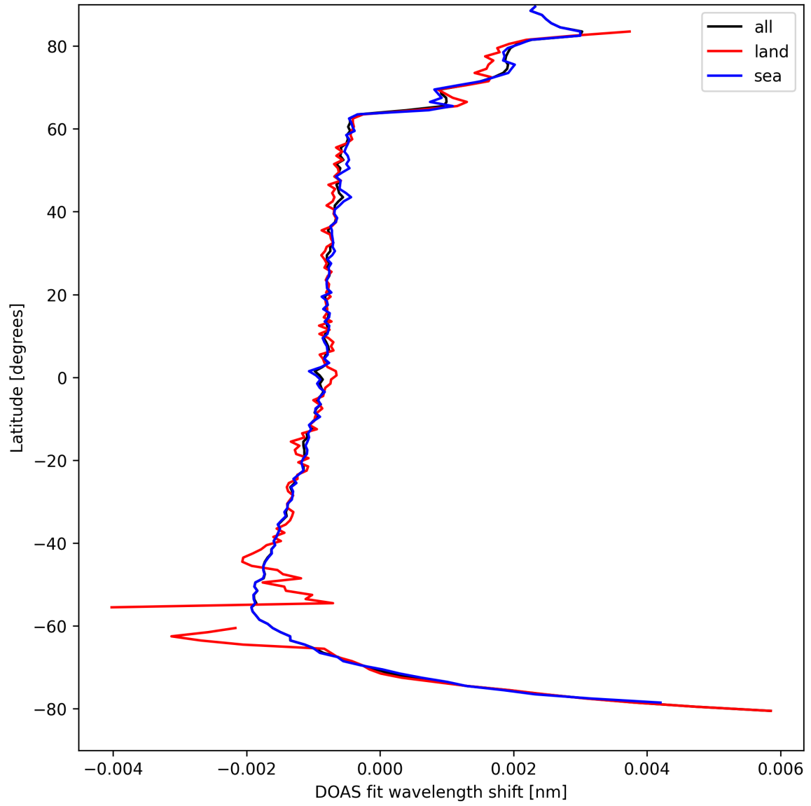
Figure 23: Zonal average of “DOAS fit wavelength shift” for 2025-04-11 to 2025-04-11.
