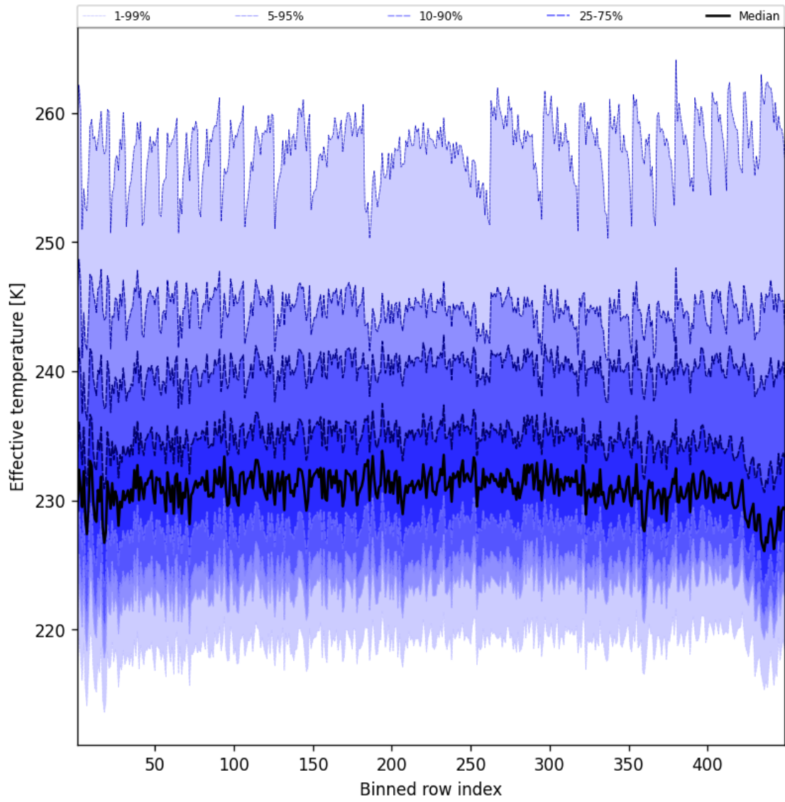
Figure 50: Along track statistics of “Effective temperature” for 2025-04-11 to 2025-04-11
