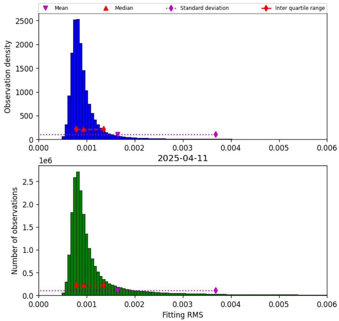
Figure 34: Histogram of “Fitting RMS” for 2025-04-11 to 2025-04-11
