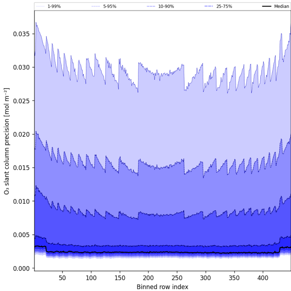
Figure 44: Along track statistics of “O 3 slant column precision” for 2025-04-11 to 2025-04-11
