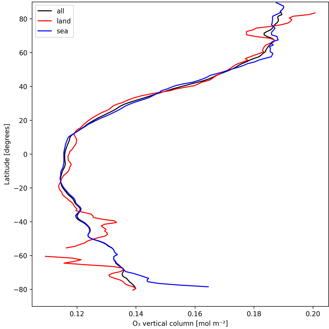
Figure 17: Zonal average of “O 3 vertical column” for 2025-04-11 to 2025-04-11.
