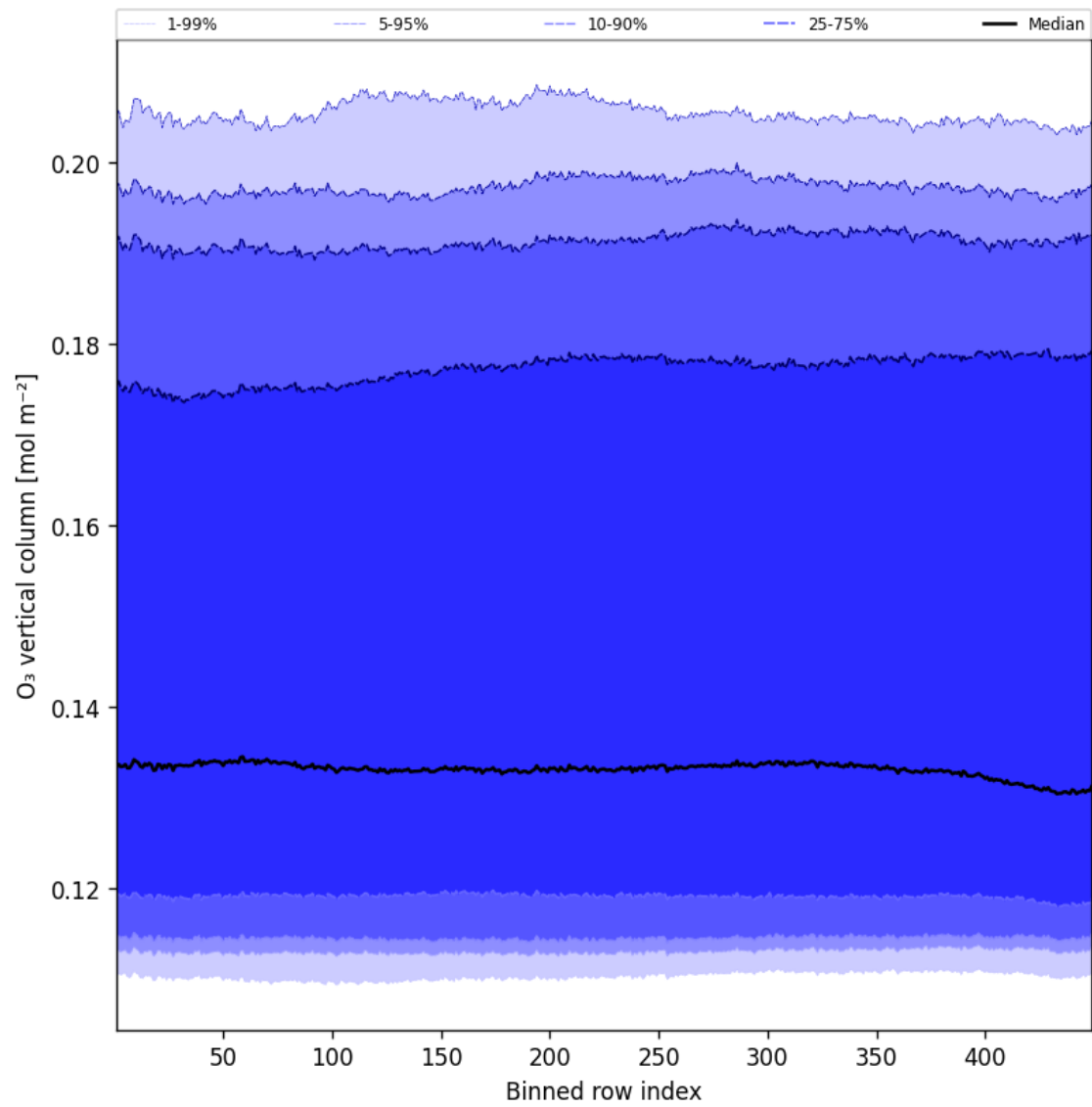
Figure 41: Along track statistics of “O 3 vertical column” for 2025-04-11 to 2025-04-11
