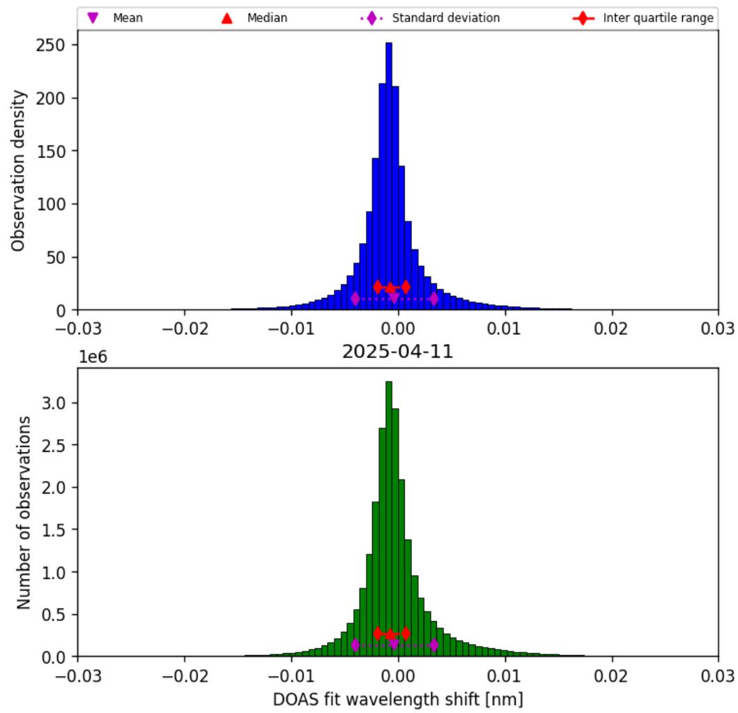
Figure 35: Histogram of “DOAS fit wavelength shift” for 2025-04-11 to 2025-04-11
