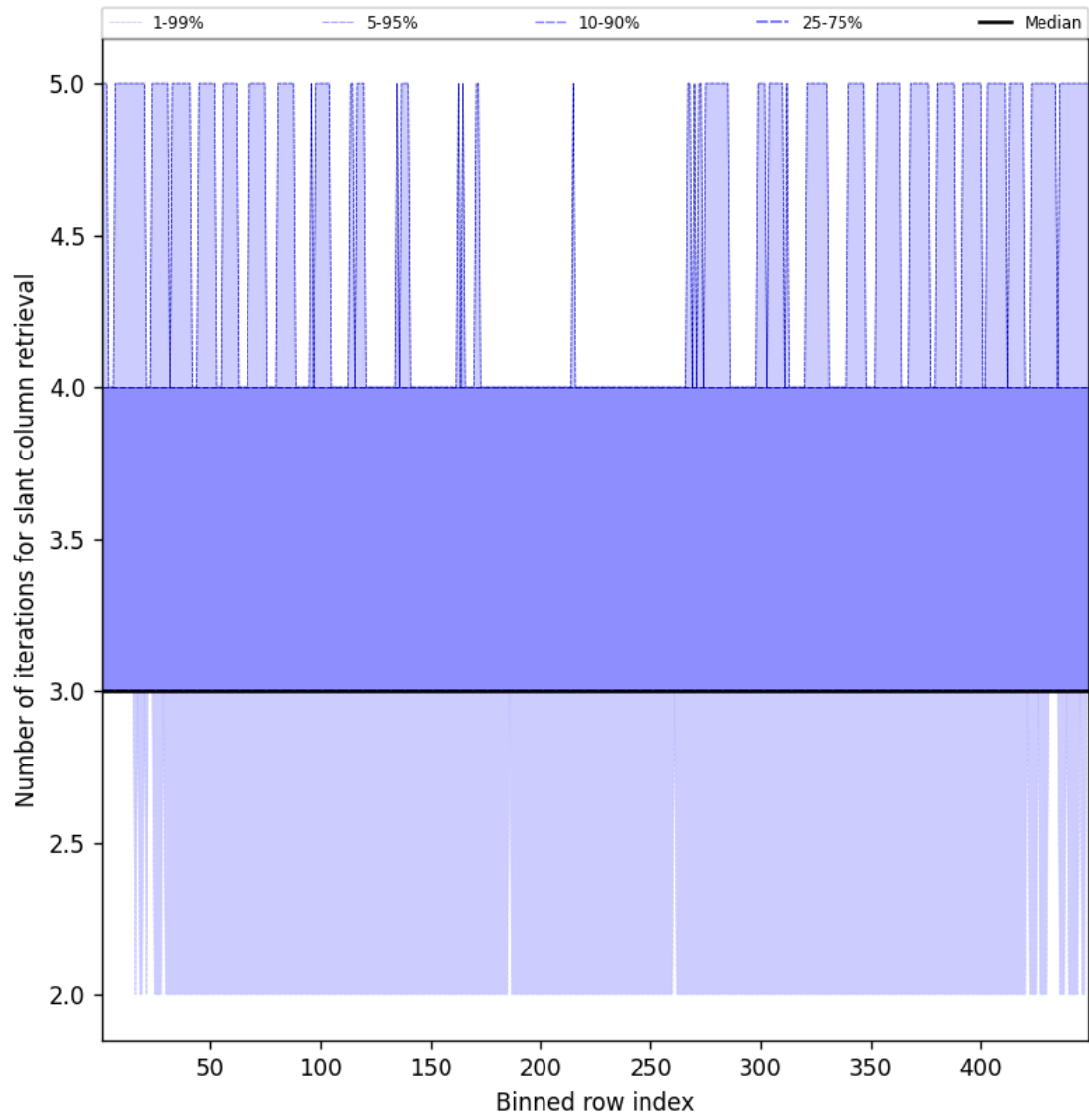
Figure 45: Along track statistics of “Number of iterations for slant column retrieval” for 2025-04-12 to 2025-04-13
