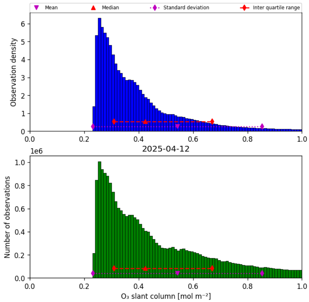
Figure 31: Histogram of “O 3 slant column” for 2025-04-12 to 2025-04-13
