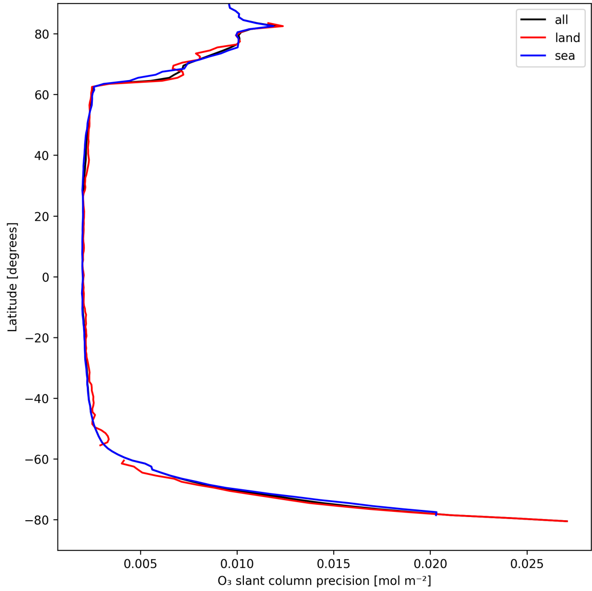
Figure 20: Zonal average of "O 3 slant column precision" for 2025-04-12 to 2025-04-13.
