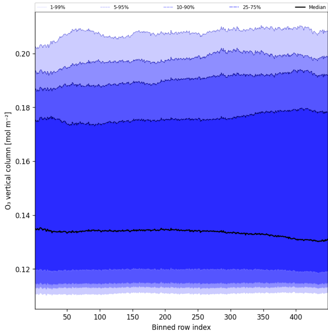
Figure 41: Along track statistics of “O 3 vertical column” for 2025-04-12 to 2025-04-13
