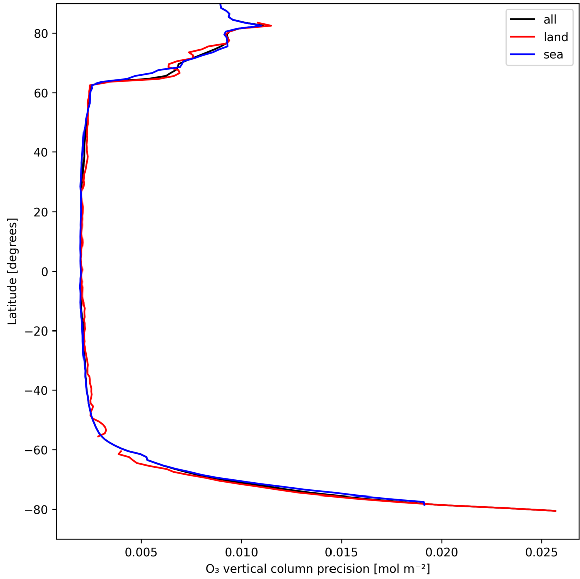
Figure 18: Zonal average of “O 3 vertical column precision” for 2025-04-12 to 2025-04-13.
