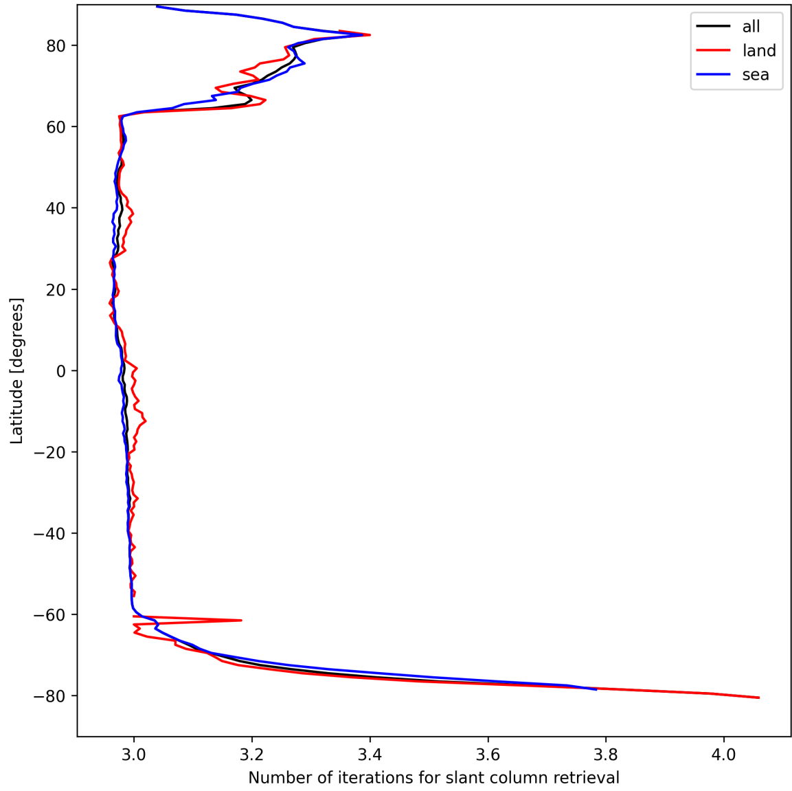
Figure 21: Zonal average of “Number of iterations for slant column retrieval” for 2025-04-12 to 2025-04-13.
