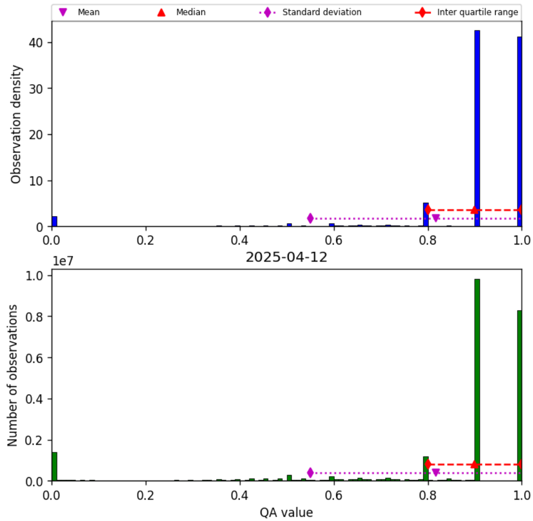
Figure 28: Histogram of “QA value” for 2025-04-12 to 2025-04-13
