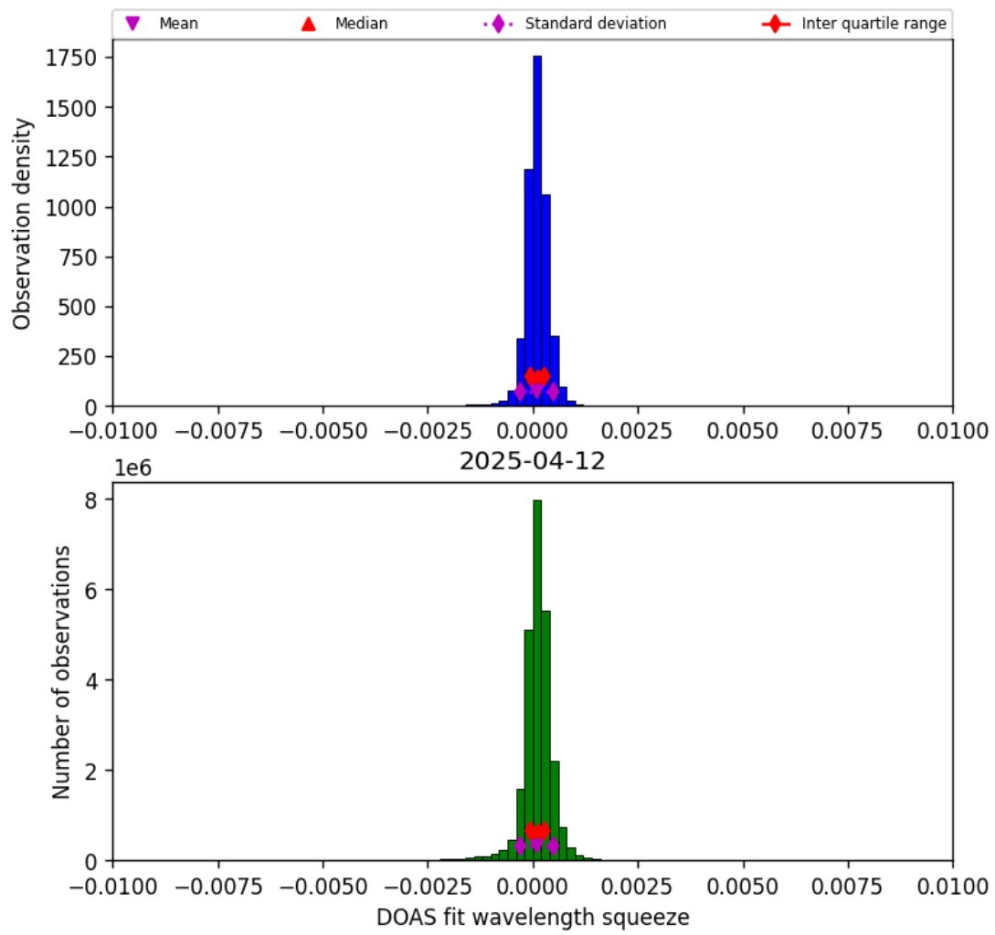
Figure 36: Histogram of “DOAS fit wavelength squeeze” for 2025-04-12 to 2025-04-13
