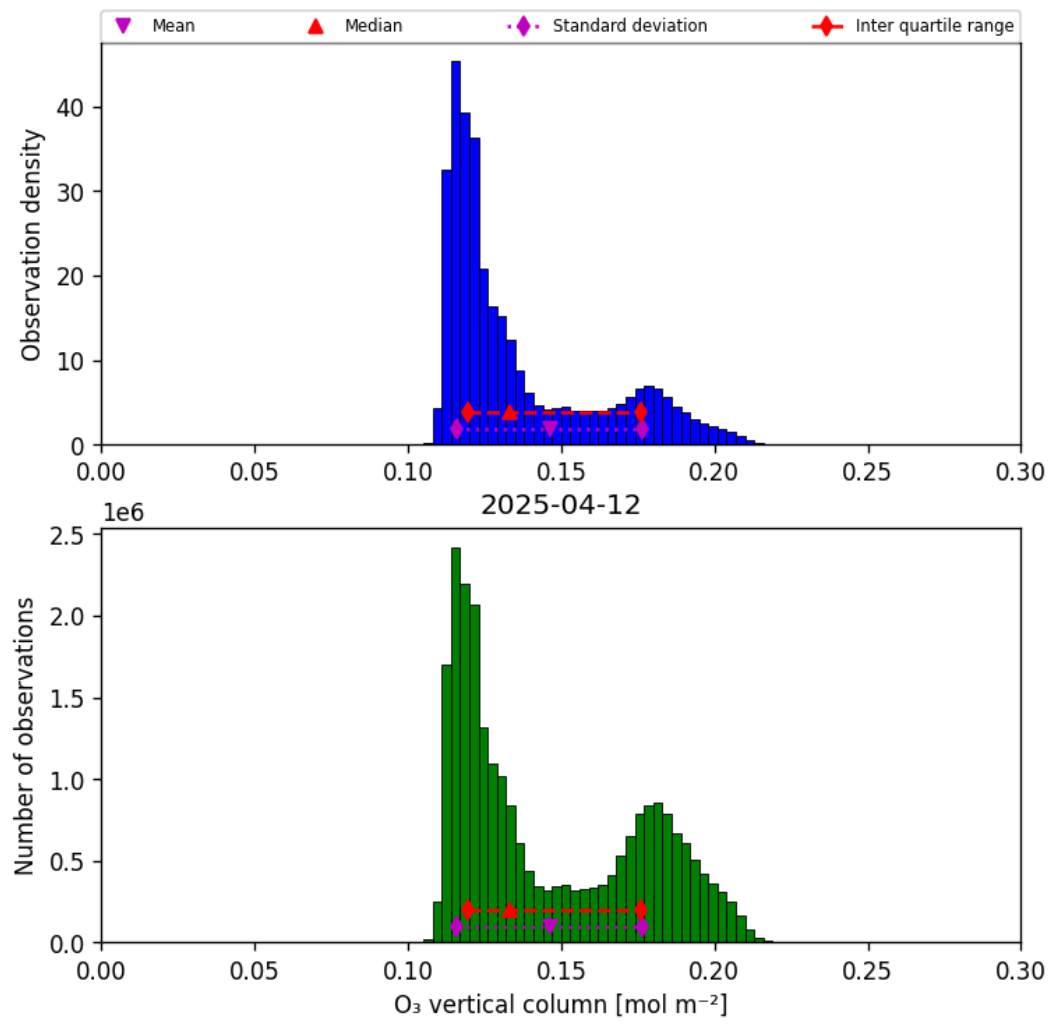
Figure 29: Histogram of “O 3 vertical column” for 2025-04-12 to 2025-04-13
