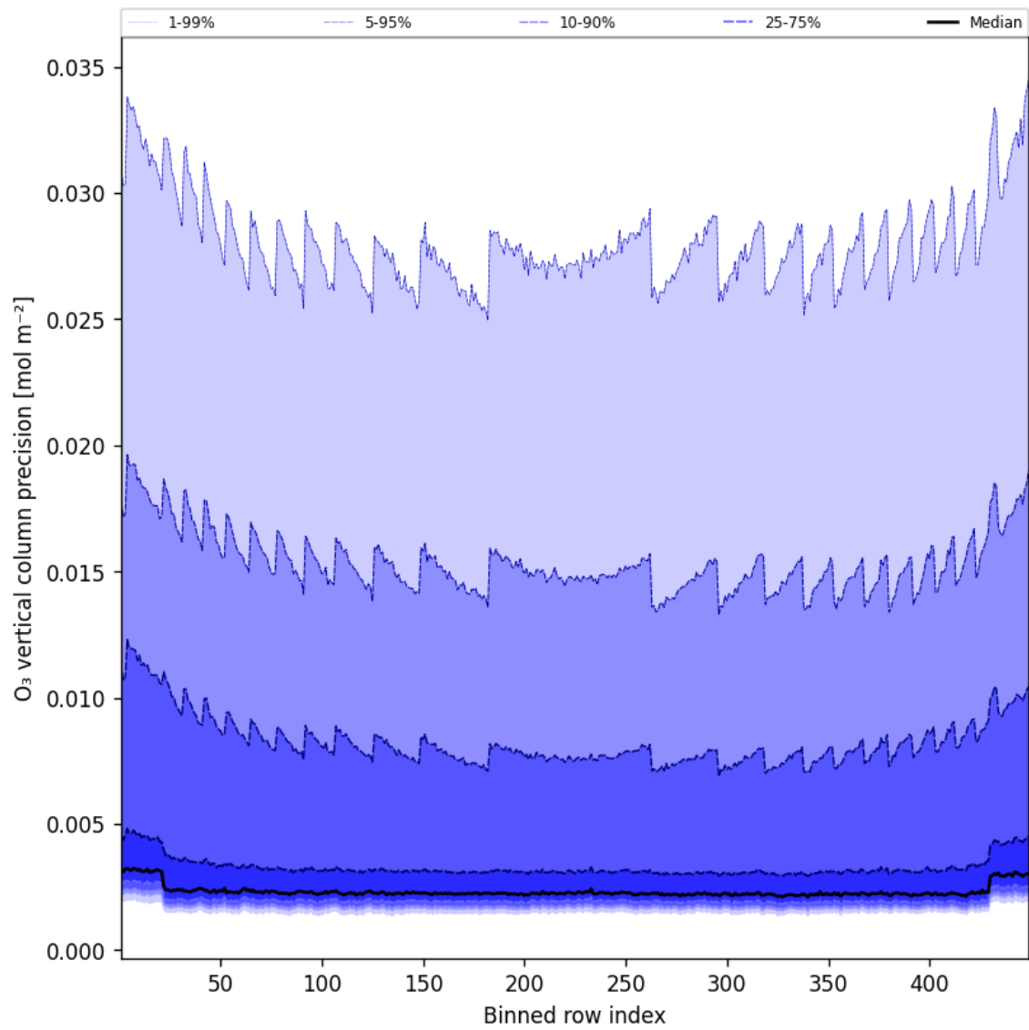
Figure 42: Along track statistics of “O 3 vertical column precision” for 2025-04-12 to 2025-04-13
