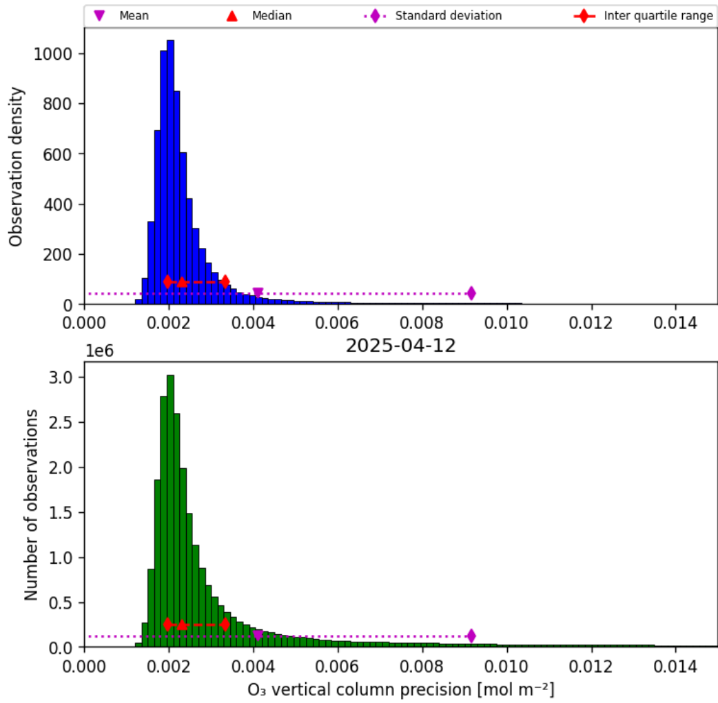
Figure 30: Histogram of “O 3 vertical column precision” for 2025-04-12 to 2025-04-13
