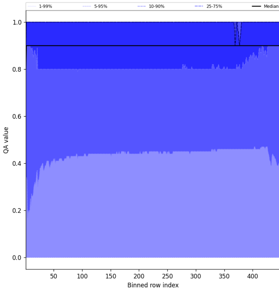
Figure 40: Along track statistics of “QA value” for 2025-04-12 to 2025-04-13
