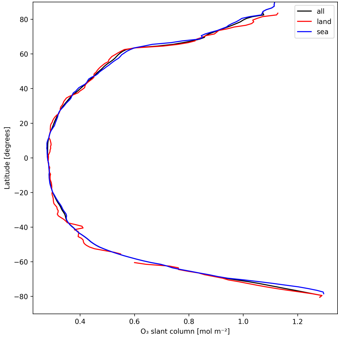
Figure 19: Zonal average of “O 3 slant column” for 2025-04-12 to 2025-04-13.
