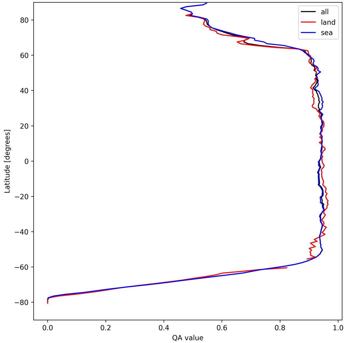
Figure 16: Zonal average of “QA value” for 2025-04-12 to 2025-04-13.
