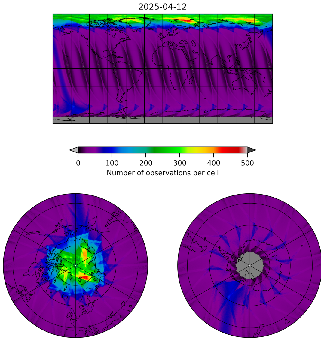
Figure 15: Map of the number of observations for 2025-04-12 to 2025-04-13
