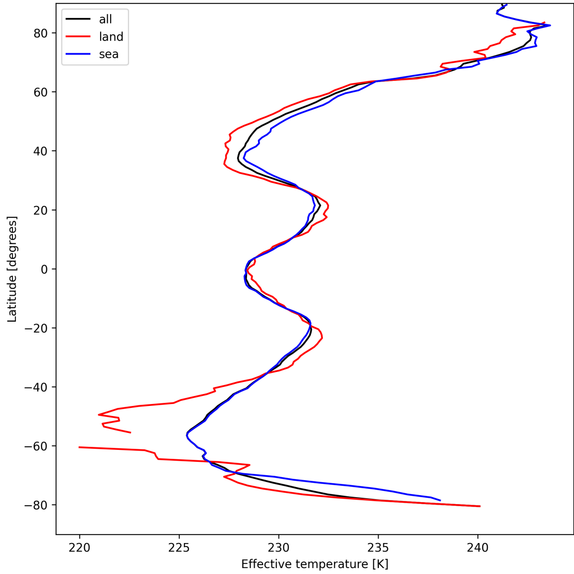
Figure 26: Zonal average of “Effective temperature” for 2025-04-12 to 2025-04-13.
