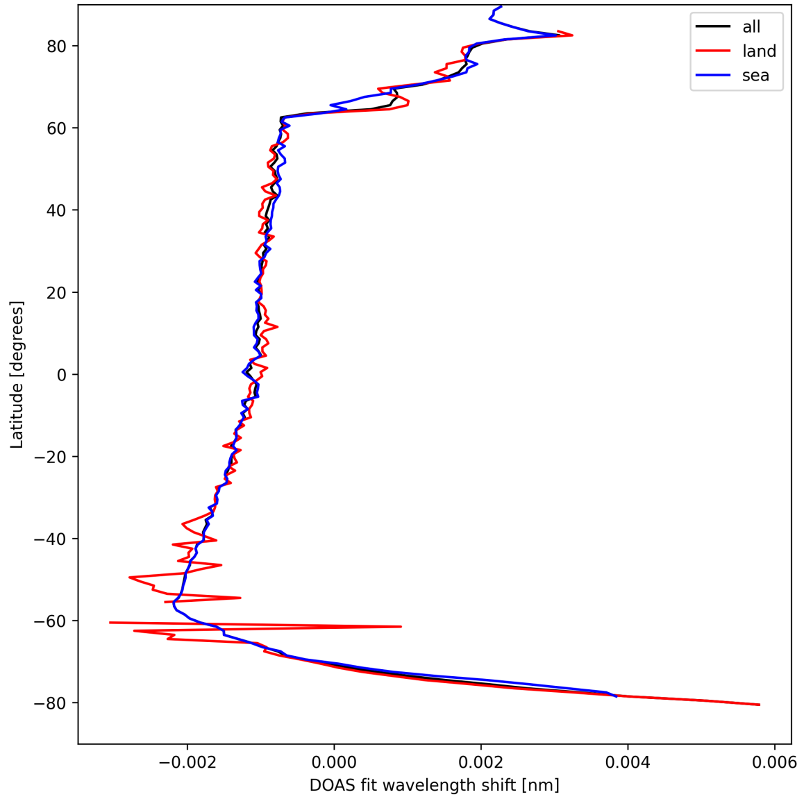
Figure 23: Zonal average of “DOAS fit wavelength shift” for 2025-04-12 to 2025-04-13.
