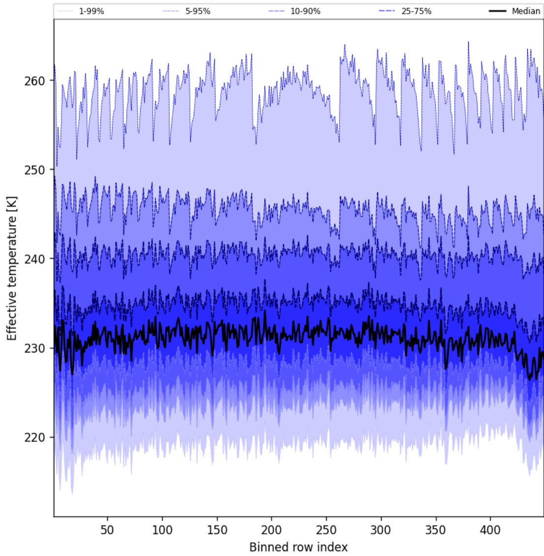
Figure 50: Along track statistics of “Effective temperature” for 2025-04-12 to 2025-04-13
