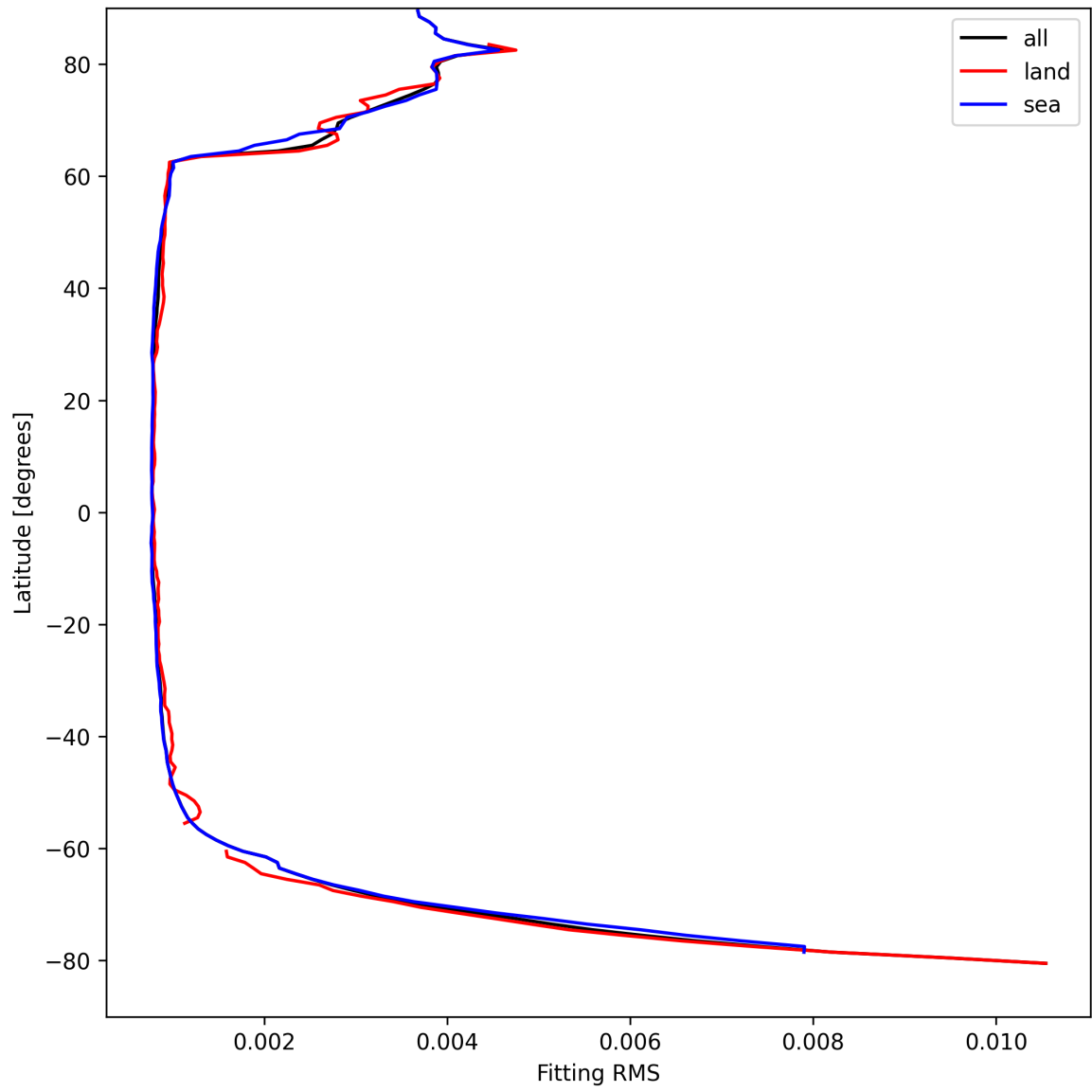
Figure 22: Zonal average of “Fitting RMS” for 2025-04-12 to 2025-04-13.
