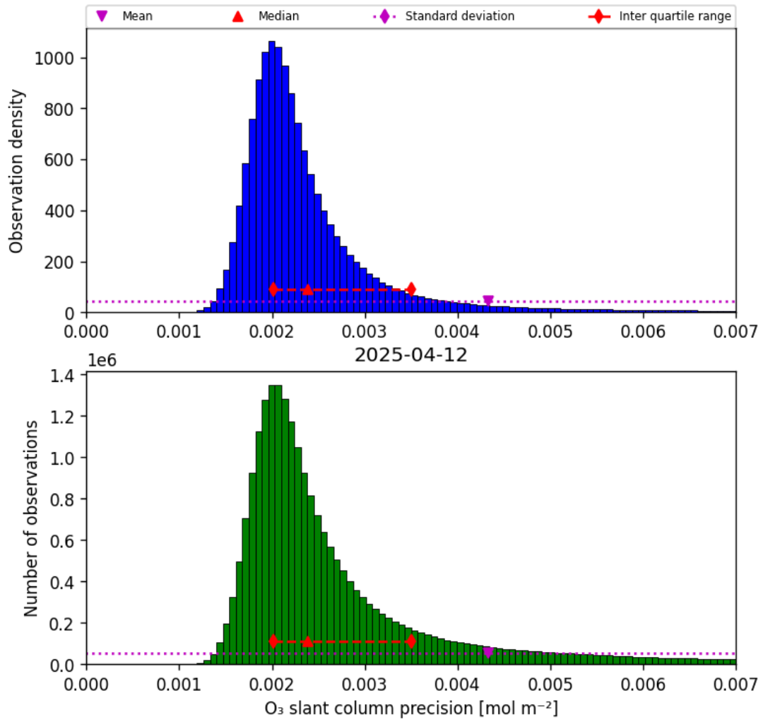
Figure 32: Histogram of “O 3 slant column precision” for 2025-04-12 to 2025-04-13
