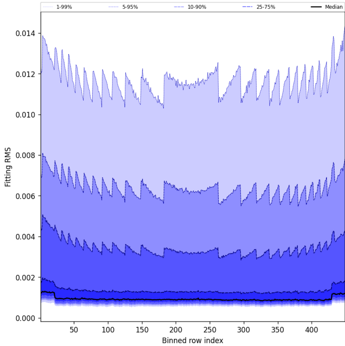
Figure 46: Along track statistics of “Fitting RMS” for 2025-04-12 to 2025-04-13
