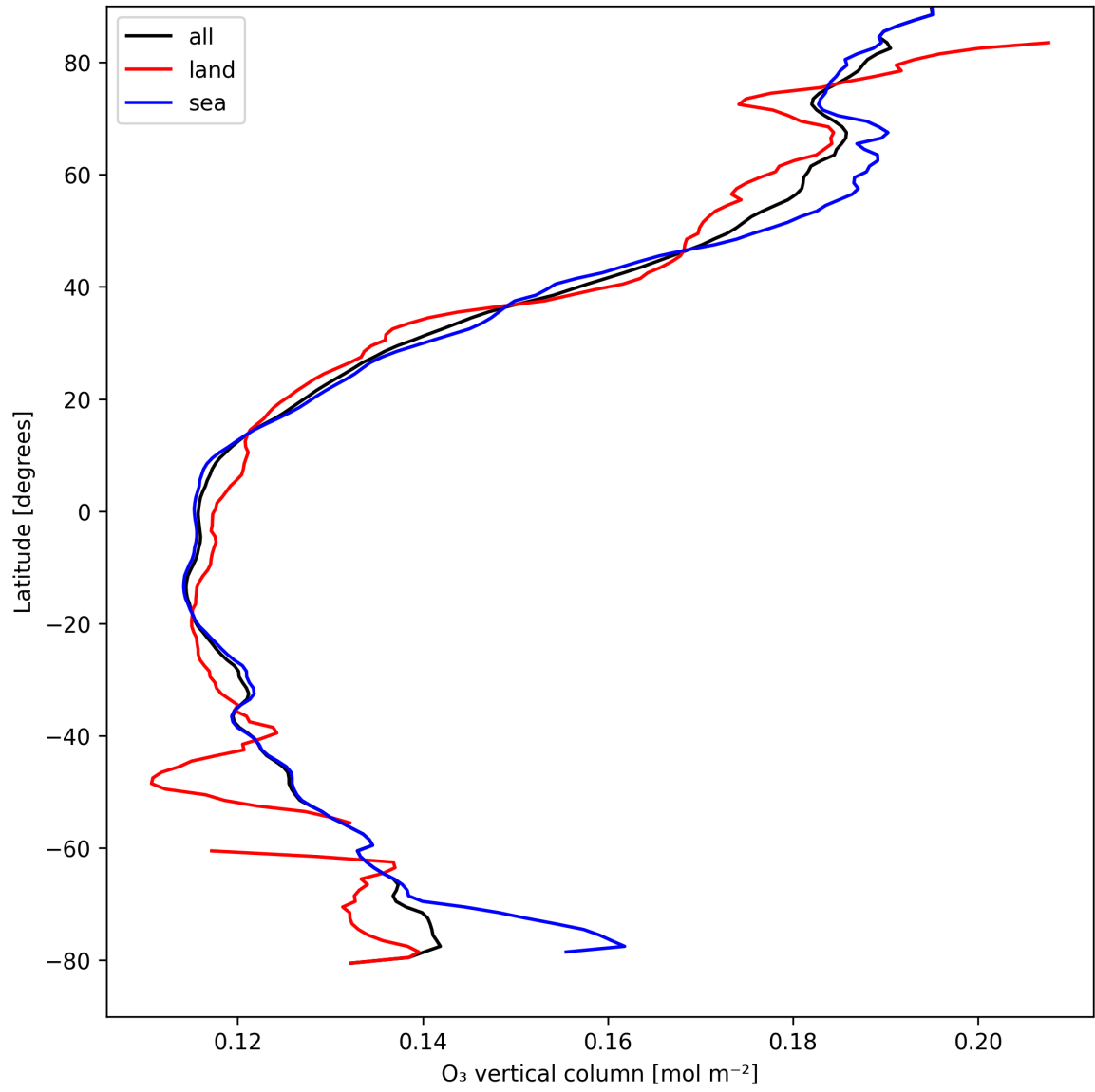
Figure 17: Zonal average of “O 3 vertical column” for 2025-04-12 to 2025-04-13.
