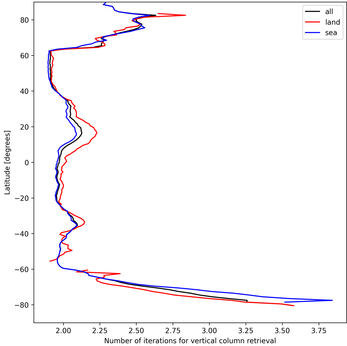
Figure 27: Zonal average of “Number of iterations for vertical column retrieval” for 2025-04-12 to 2025-04-13.
