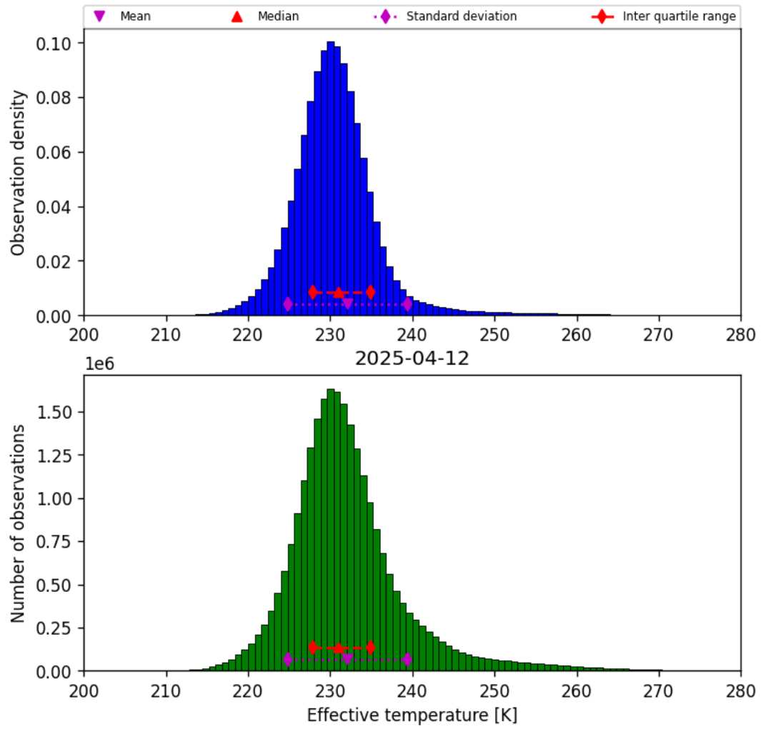
Figure 38: Histogram of “Effective temperature” for 2025-04-12 to 2025-04-13
