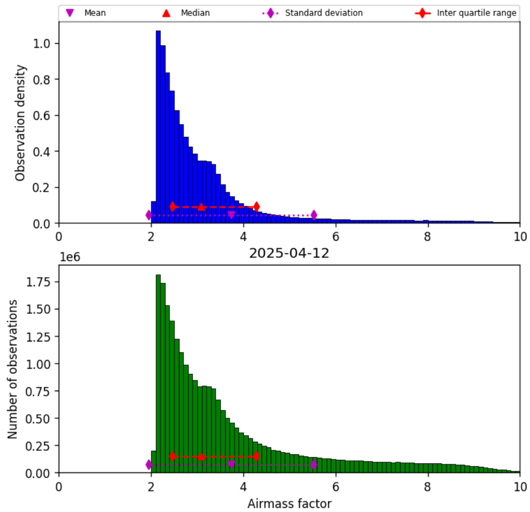
Figure 37: Histogram of “Airmass factor” for 2025-04-12 to 2025-04-13
