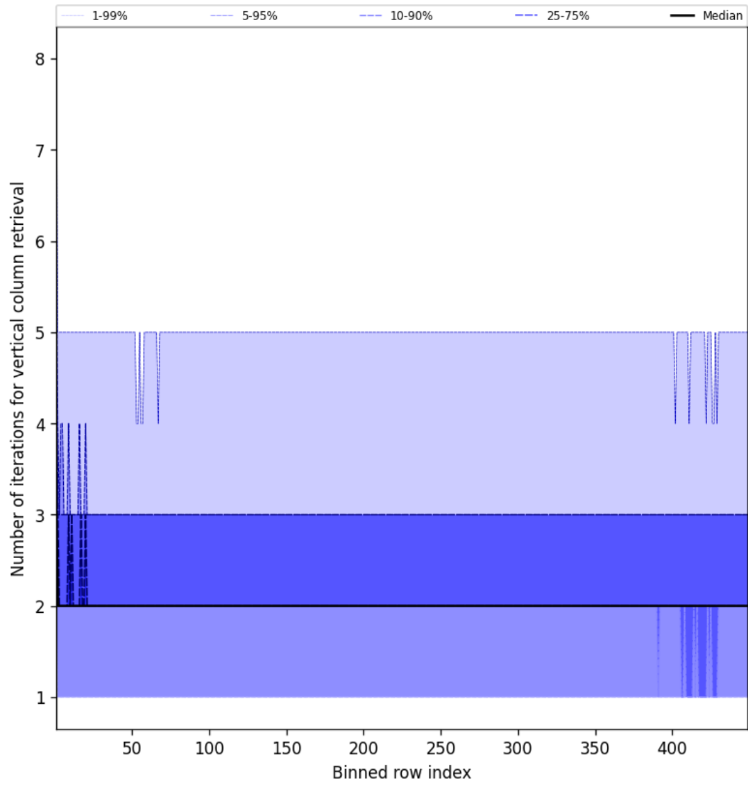
Figure 51: Along track statistics of “Number of iterations for vertical column retrieval” for 2025-04-12 to 2025-04-13
