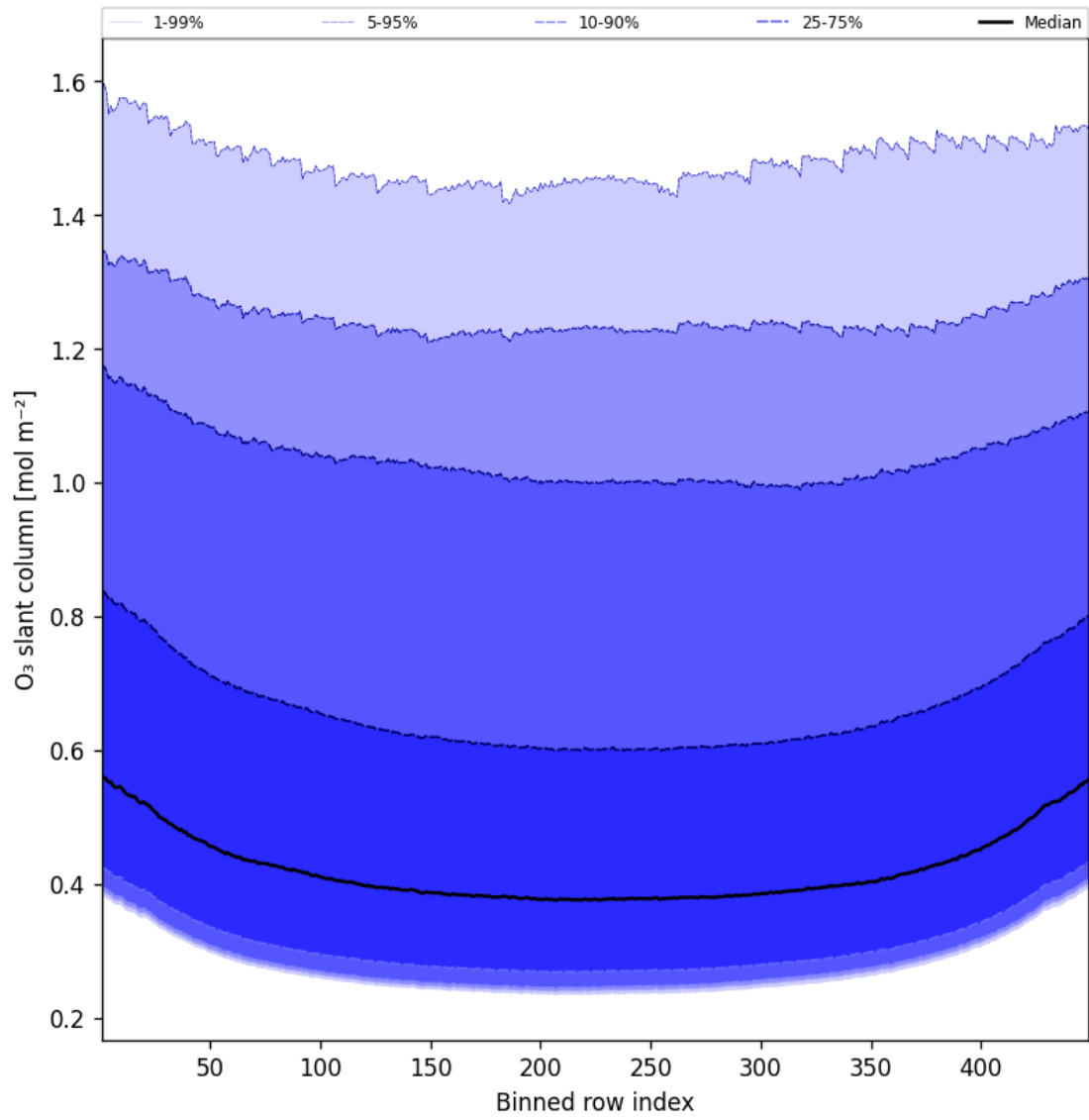
Figure 43: Along track statistics of “O 3 slant column” for 2025-04-12 to 2025-04-13
