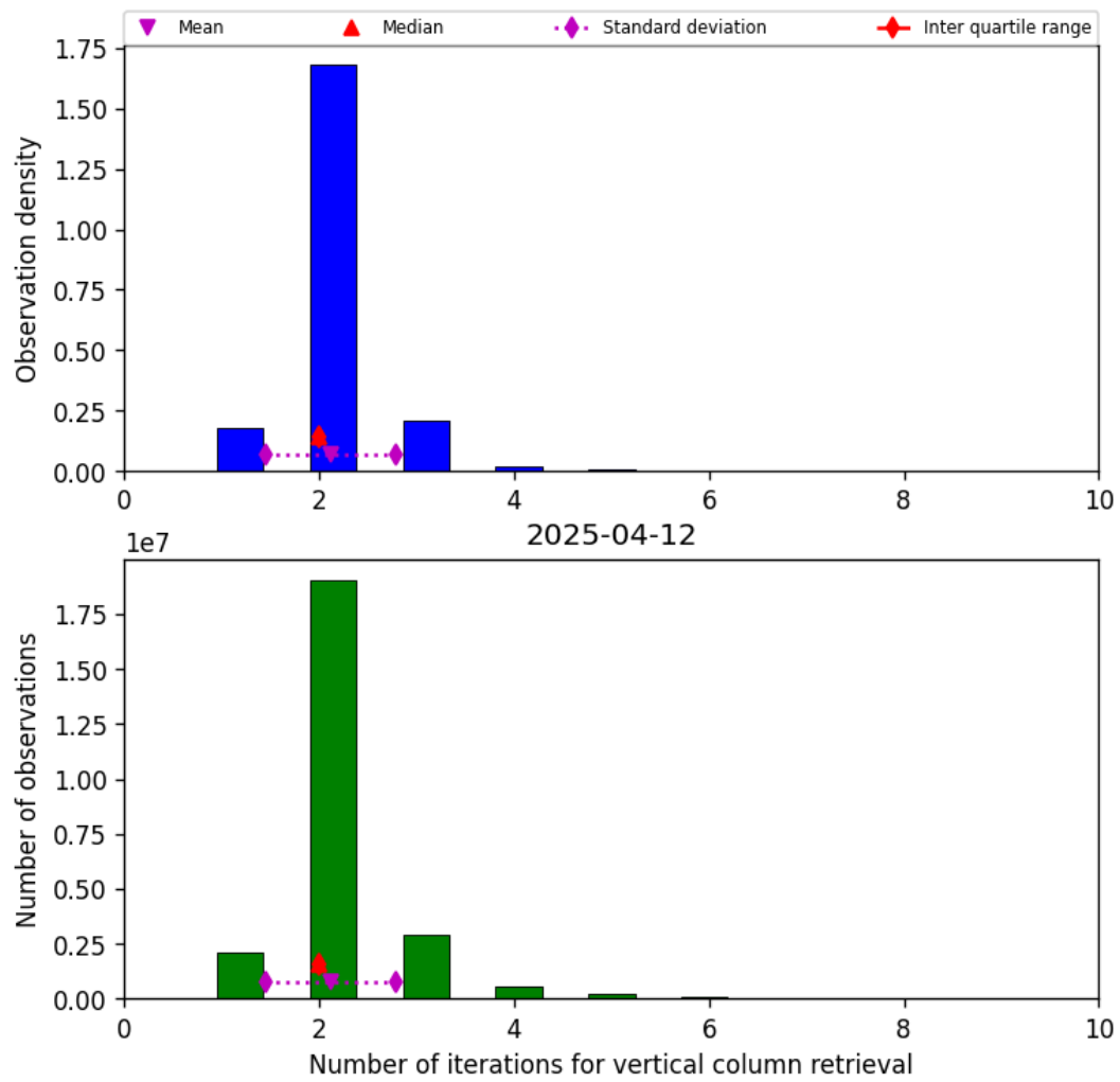
Figure 39: Histogram of “Number of iterations for vertical column retrieval” for 2025-04-12 to 2025-04-13
