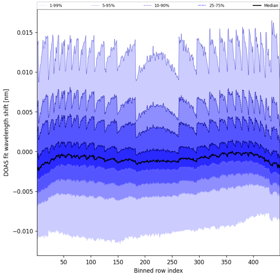
Figure 47: Along track statistics of “DOAS fit wavelength shift” for 2025-04-12 to 2025-04-13
