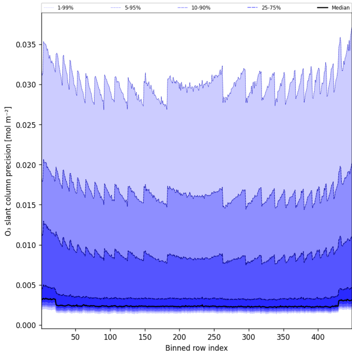
Figure 44: Along track statistics of “O 3 slant column precision” for 2025-04-12 to 2025-04-13
