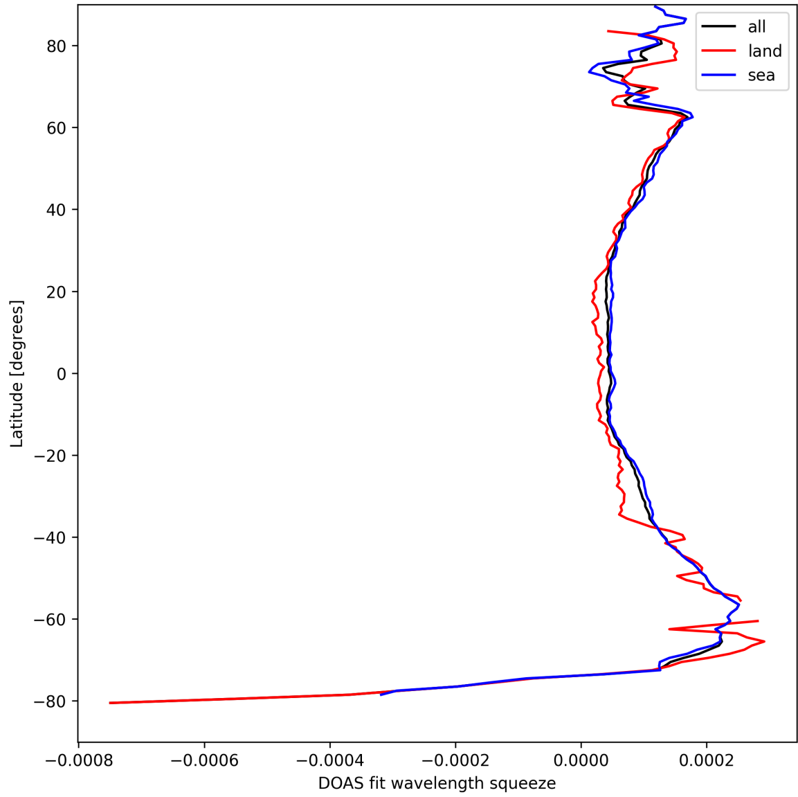
Figure 24: Zonal average of “DOAS fit wavelength squeeze” for 2025-04-12 to 2025-04-13.
