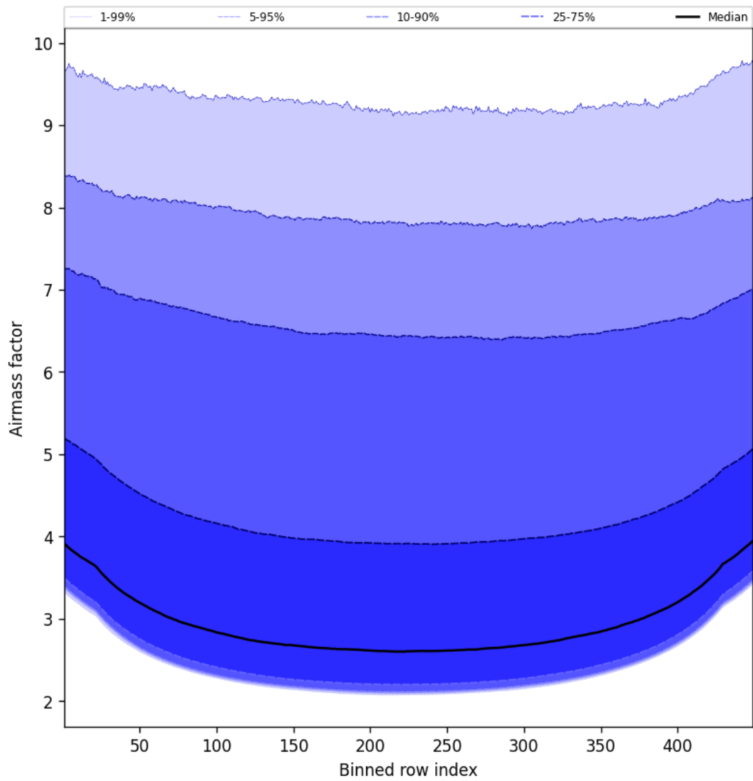
Figure 49: Along track statistics of “Airmass factor” for 2025-04-12 to 2025-04-13
