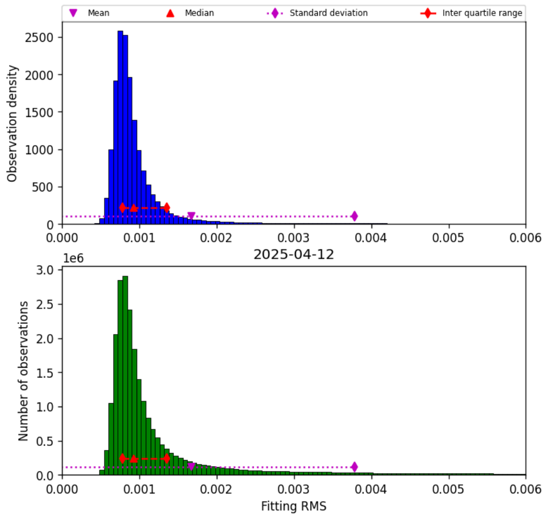
Figure 34: Histogram of “Fitting RMS” for 2025-04-12 to 2025-04-13
