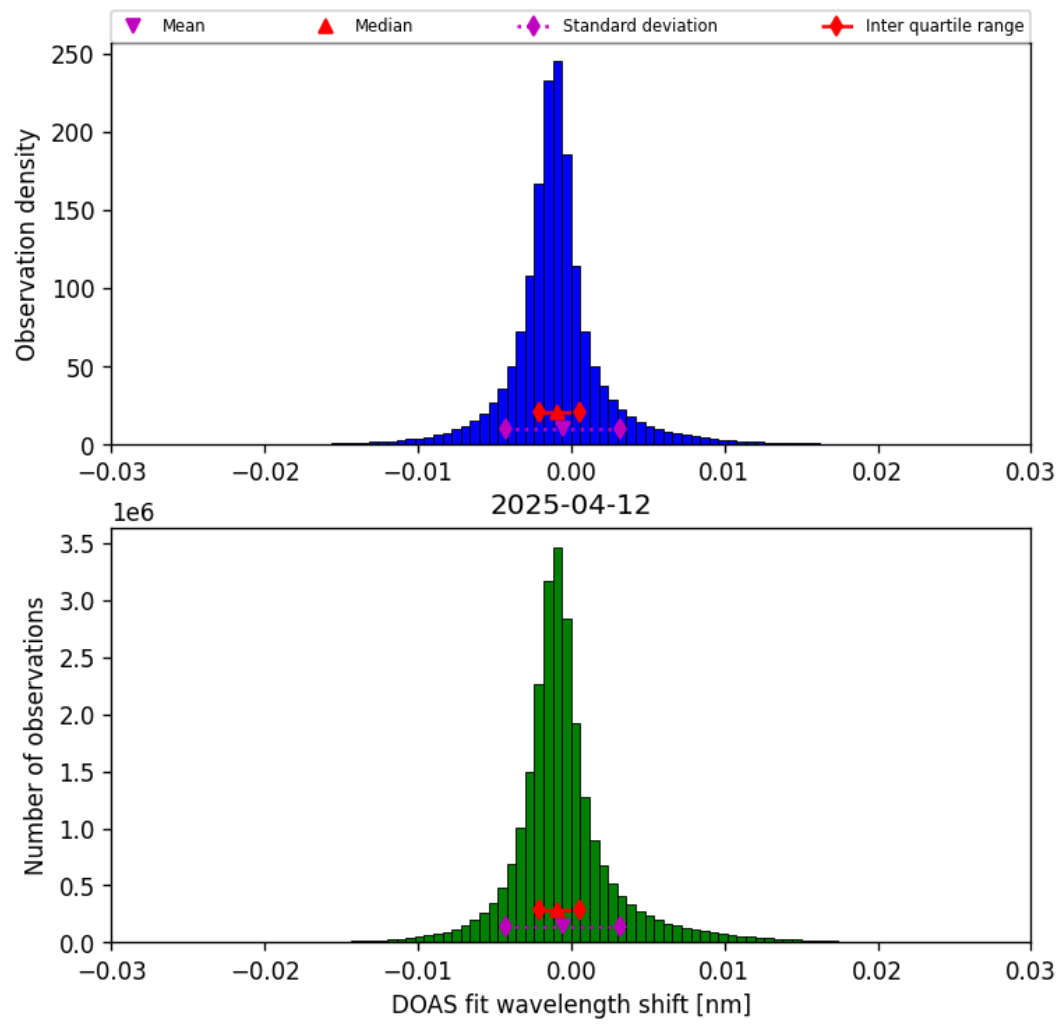
Figure 35: Histogram of “DOAS fit wavelength shift” for 2025-04-12 to 2025-04-13
