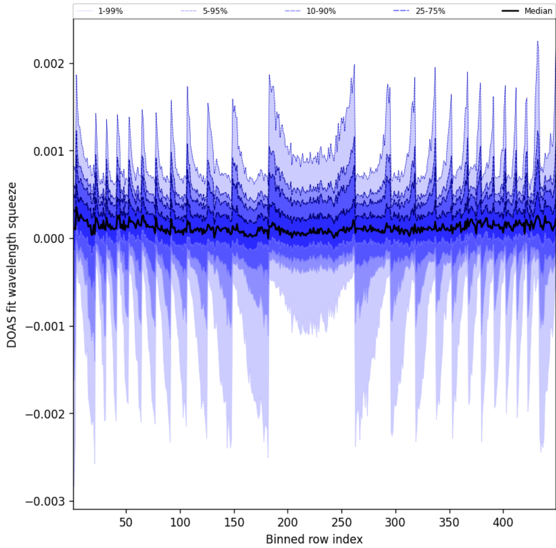
Figure 48: Along track statistics of “DOAS fit wavelength squeeze” for 2025-04-12 to 2025-04-13
