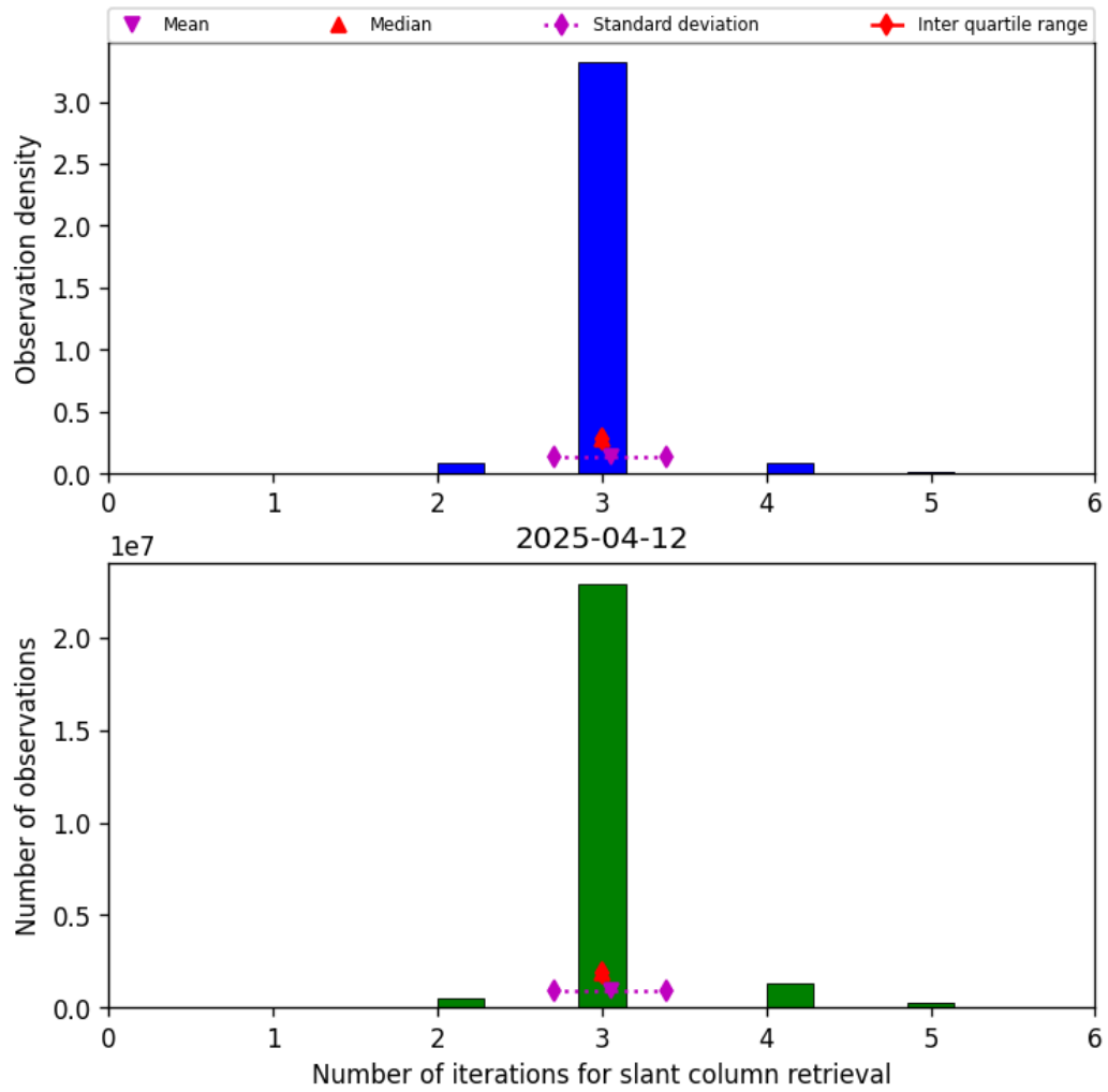
Figure 33: Histogram of “Number of iterations for slant column retrieval” for 2025-04-12 to 2025-04-13
