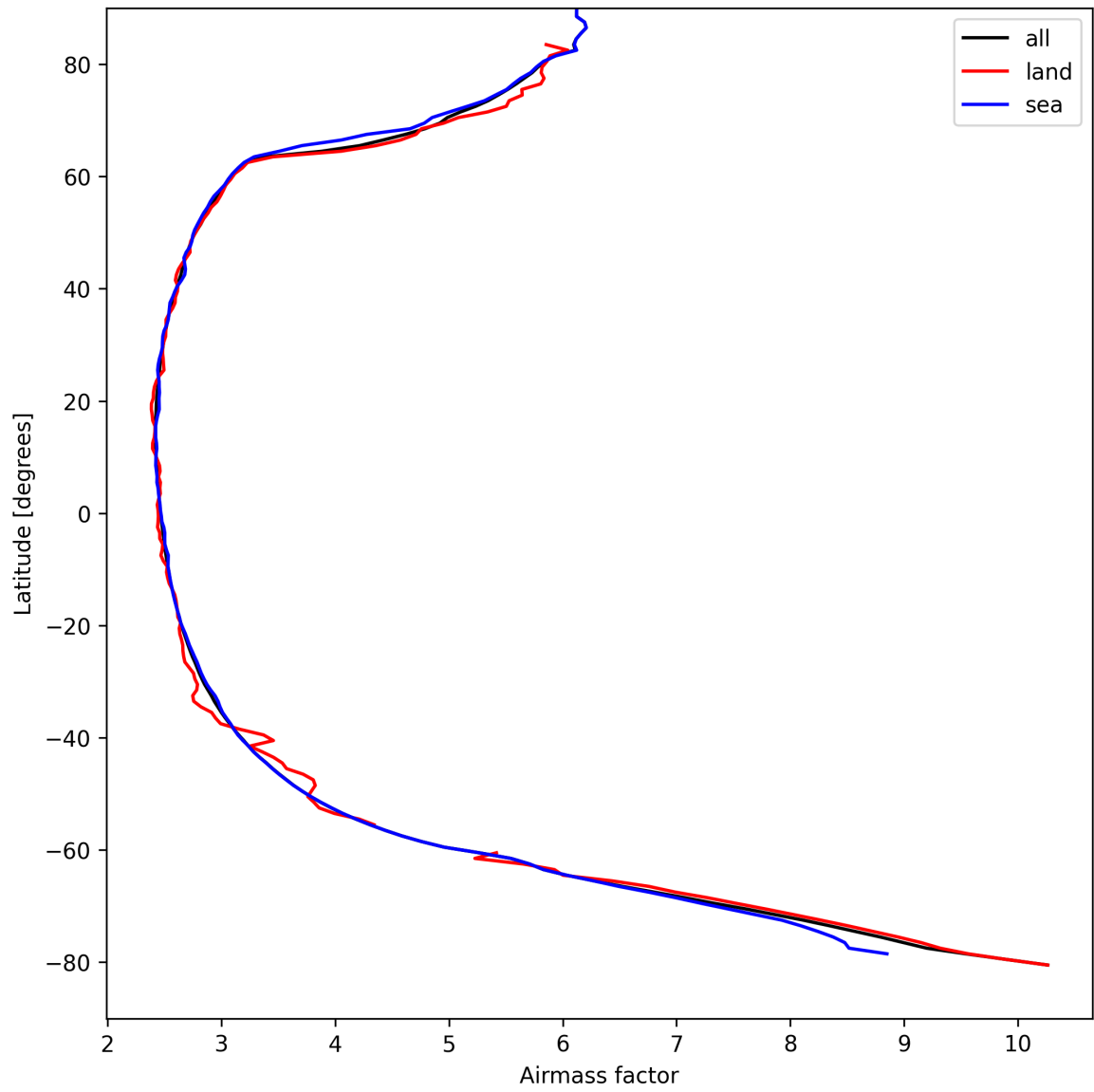
Figure 25: Zonal average of “Airmass factor” for 2025-04-12 to 2025-04-13.
