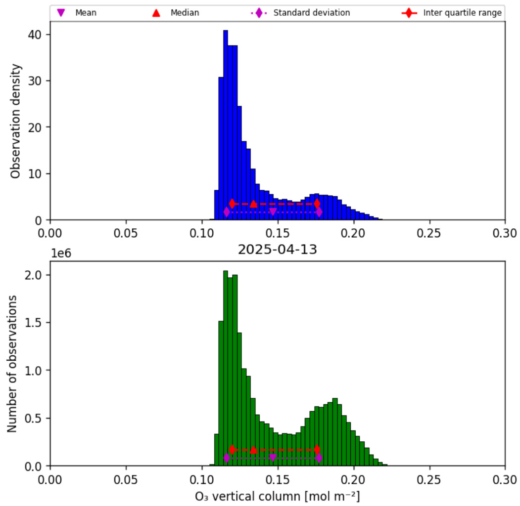
Figure 29: Histogram of “O 3 vertical column” for 2025-04-13 to 2025-04-14
