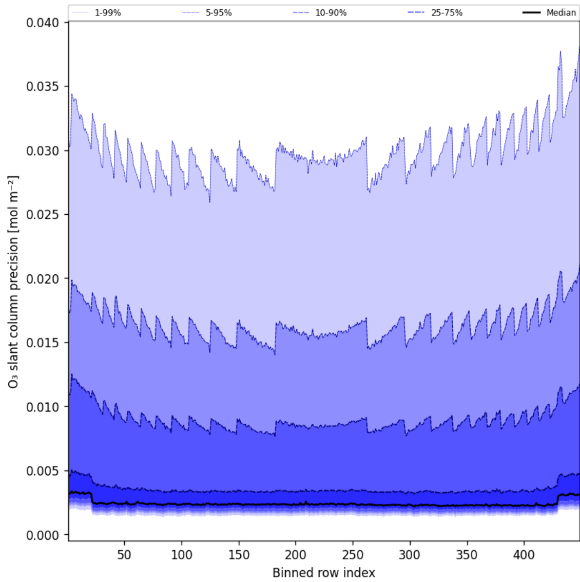
Figure 44: Along track statistics of “O 3 slant column precision” for 2025-04-13 to 2025-04-14
