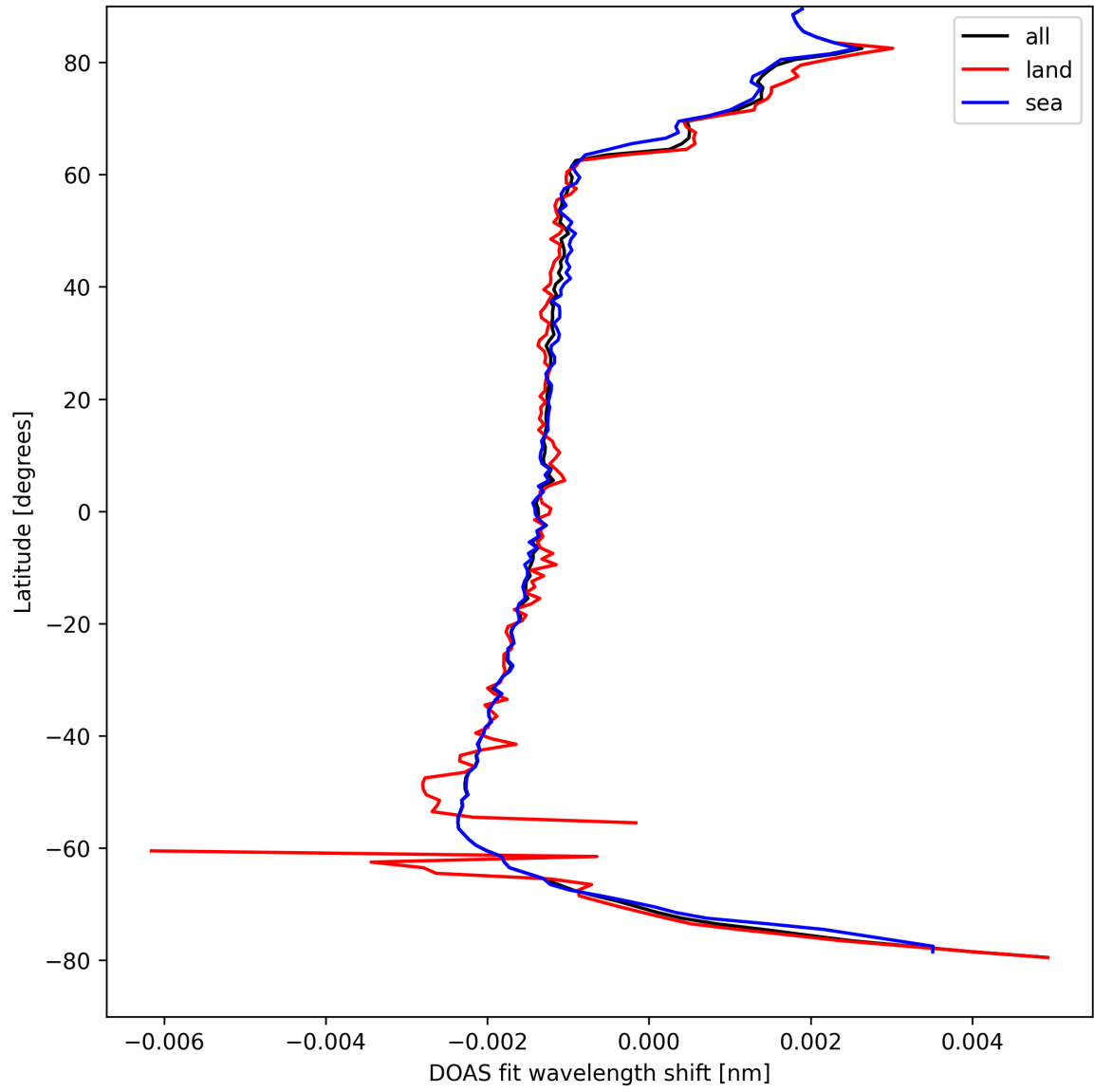
Figure 23: Zonal average of “DOAS fit wavelength shift” for 2025-04-13 to 2025-04-14.
