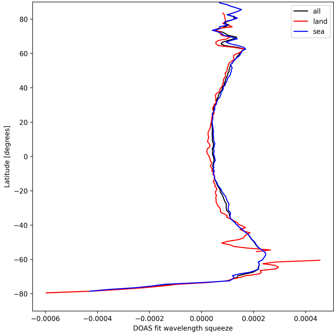
Figure 24: Zonal average of “DOAS fit wavelength squeeze” for 2025-04-13 to 2025-04-14.
