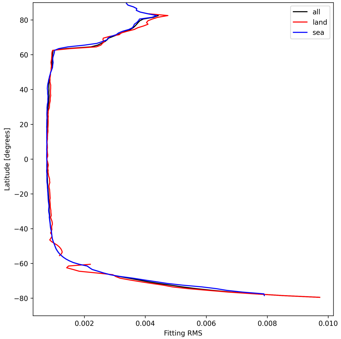
Figure 22: Zonal average of “Fitting RMS” for 2025-04-13 to 2025-04-14.
