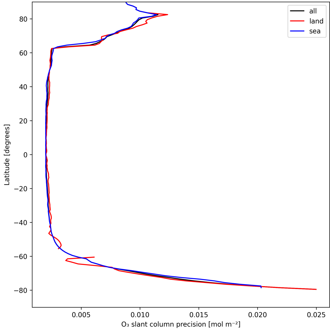
Figure 20: Zonal average of "O 3 slant column precision" for 2025-04-13 to 2025-04-14.
