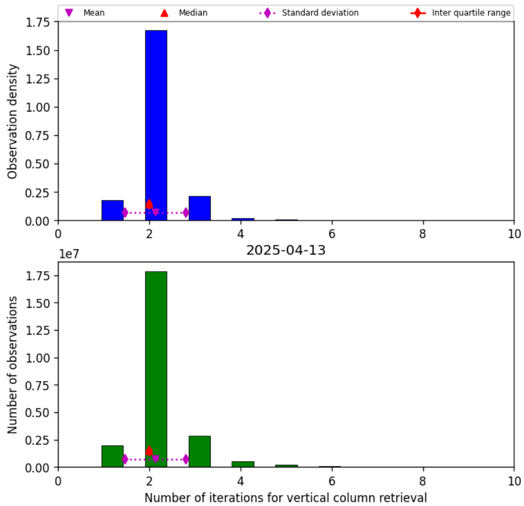
Figure 39: Histogram of “Number of iterations for vertical column retrieval” for 2025-04-13 to 2025-04-14
