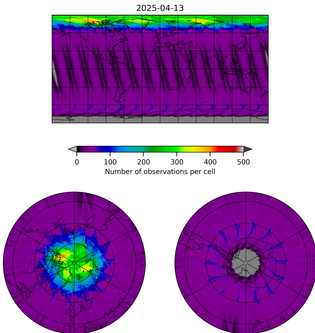
Figure 15: Map of the number of observations for 2025-04-13 to 2025-04-14
