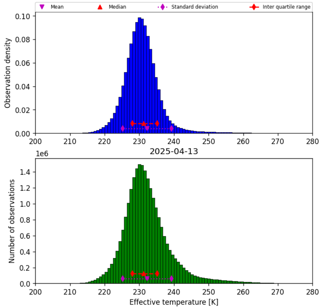
Figure 38: Histogram of “Effective temperature” for 2025-04-13 to 2025-04-14
