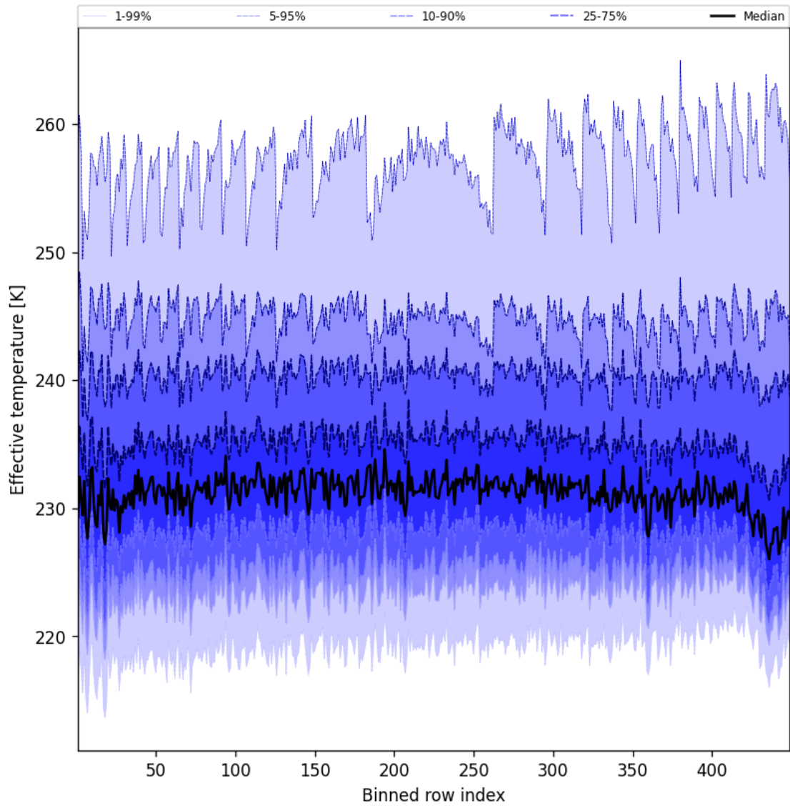
Figure 50: Along track statistics of “Effective temperature” for 2025-04-13 to 2025-04-14
