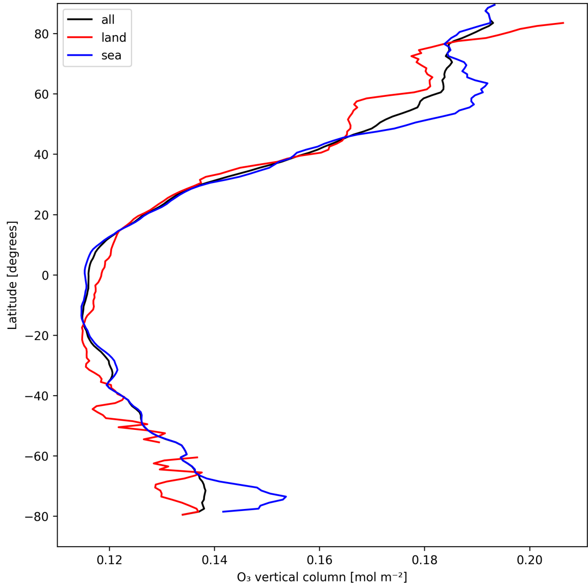
Figure 17: Zonal average of “O 3 vertical column” for 2025-04-13 to 2025-04-14.
