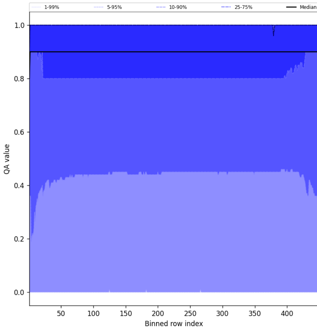
Figure 40: Along track statistics of “QA value” for 2025-04-13 to 2025-04-14
