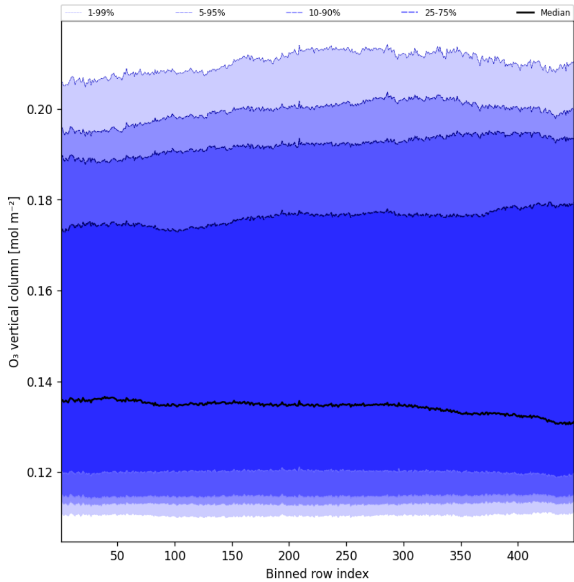
Figure 41: Along track statistics of “O 3 vertical column” for 2025-04-13 to 2025-04-14
