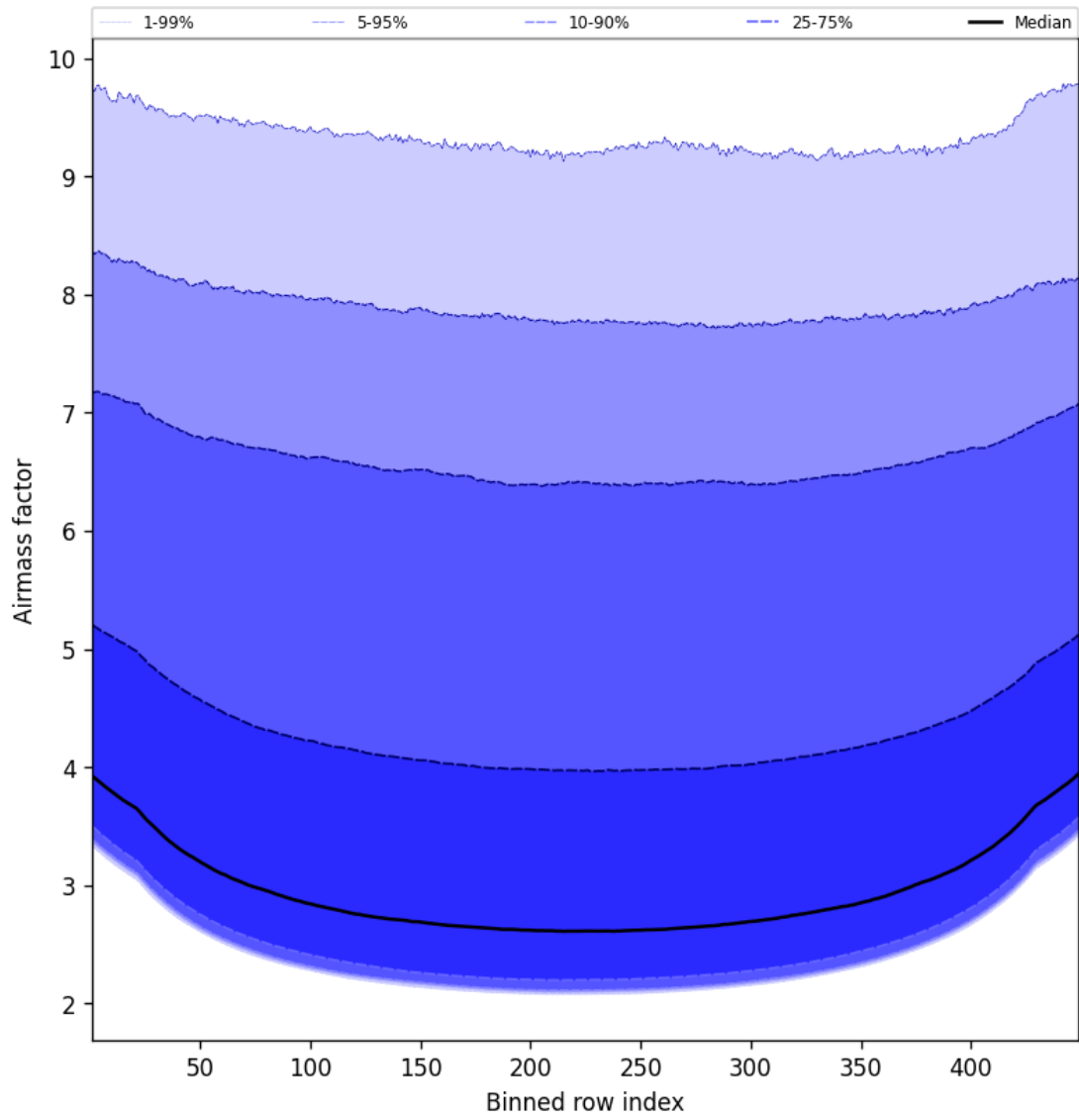
Figure 49: Along track statistics of “Airmass factor” for 2025-04-13 to 2025-04-14
