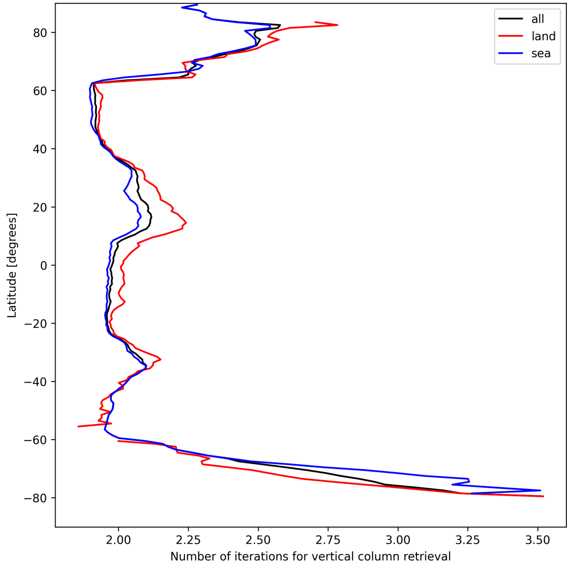
Figure 27: Zonal average of “Number of iterations for vertical column retrieval” for 2025-04-13 to 2025-04-14.
