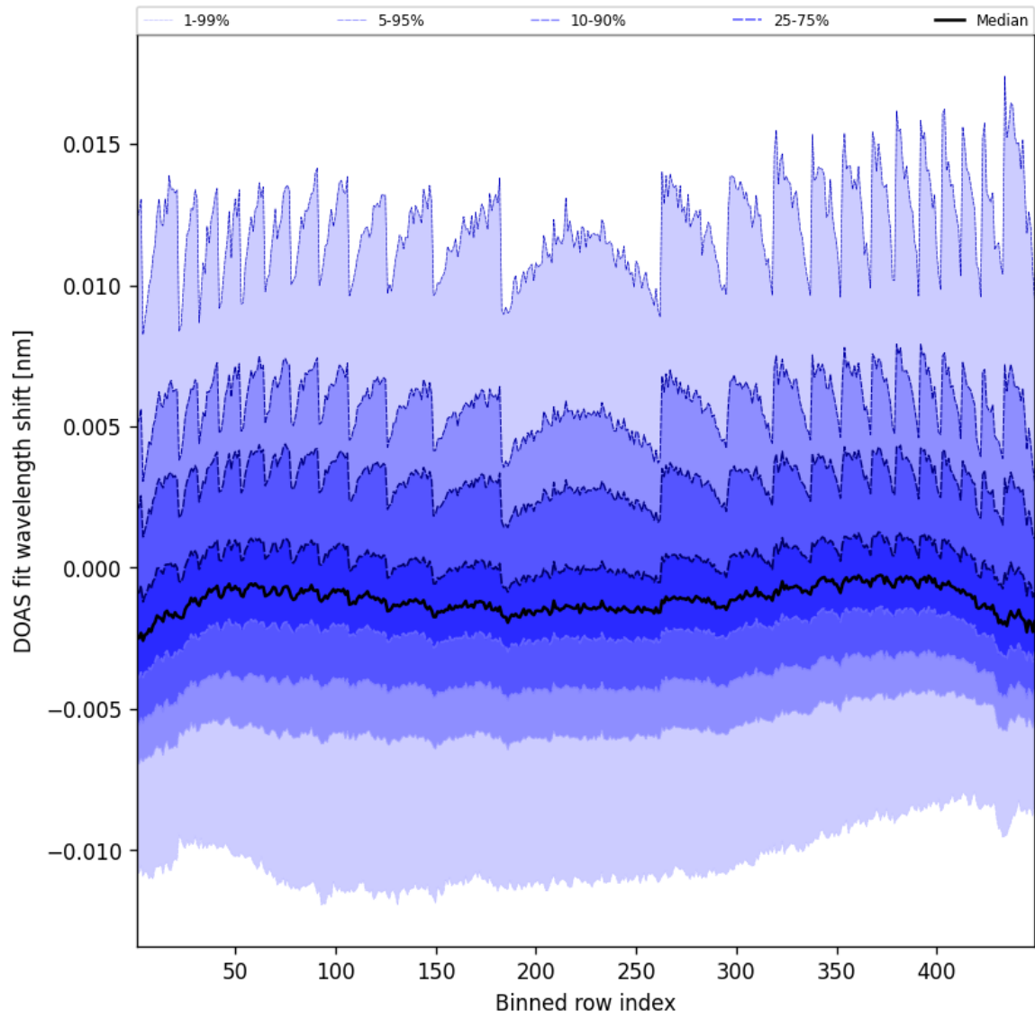
Figure 47: Along track statistics of “DOAS fit wavelength shift” for 2025-04-13 to 2025-04-14
