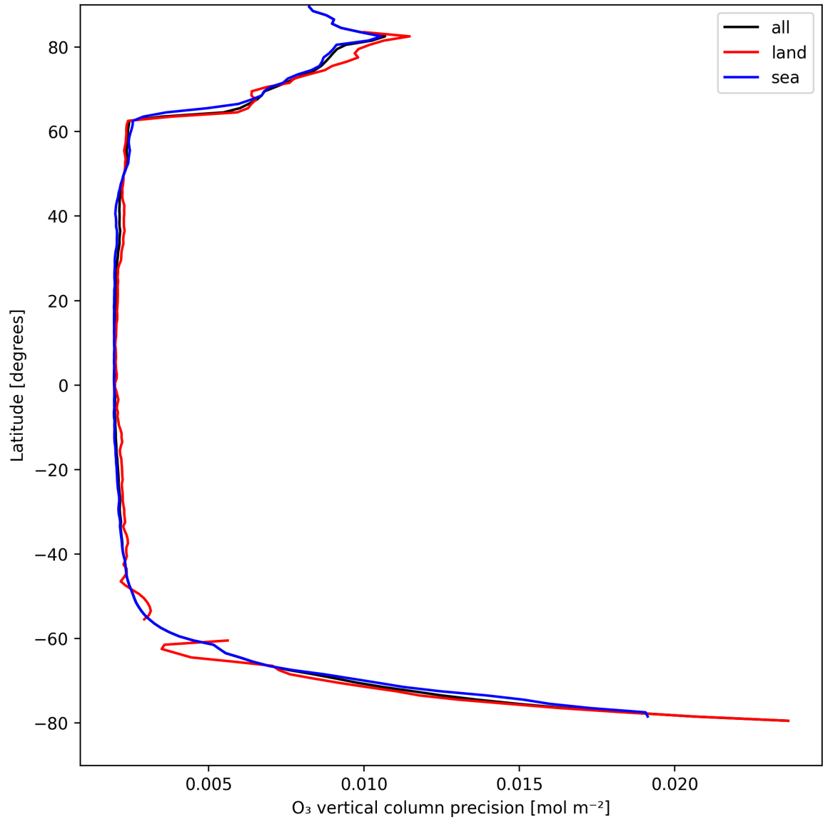
Figure 18: Zonal average of "O 3 vertical column precision" for 2025-04-13 to 2025-04-14.
