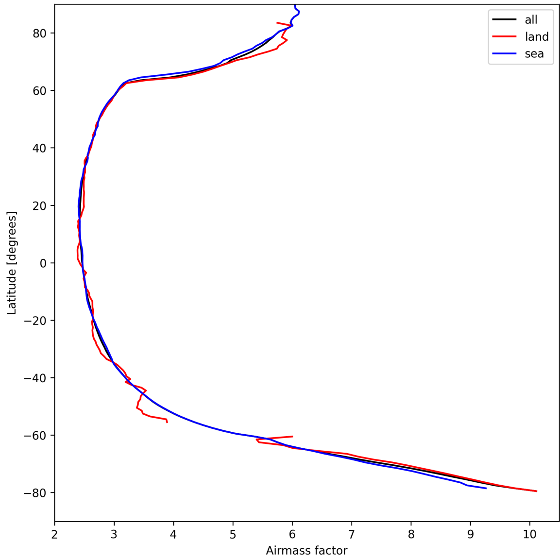
Figure 25: Zonal average of “Airmass factor” for 2025-04-13 to 2025-04-14.
