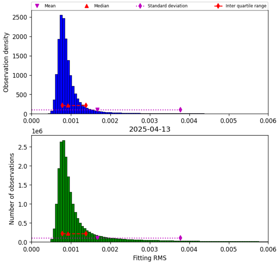
Figure 34: Histogram of “Fitting RMS” for 2025-04-13 to 2025-04-14
