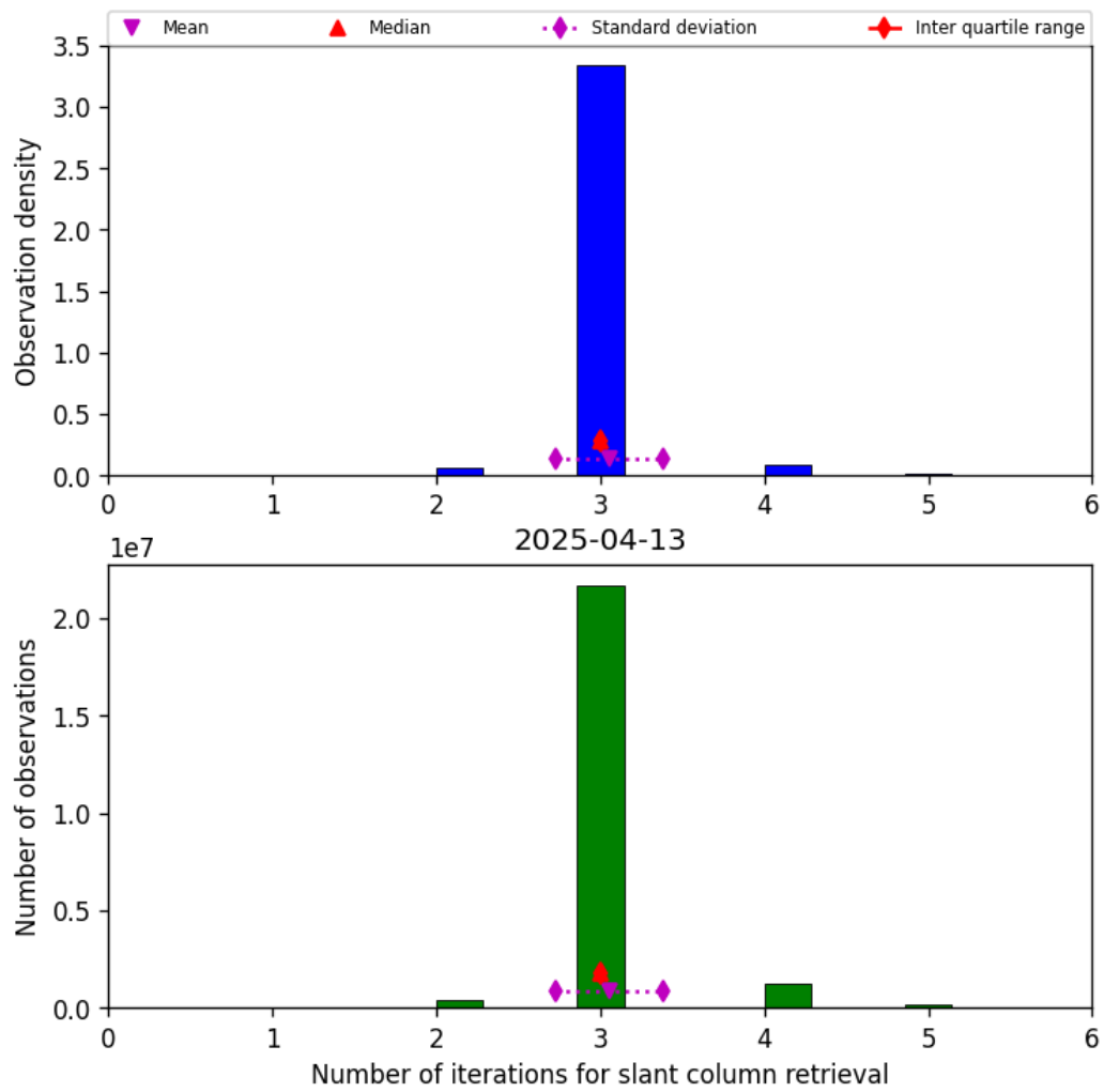
Figure 33: Histogram of “Number of iterations for slant column retrieval” for 2025-04-13 to 2025-04-14
