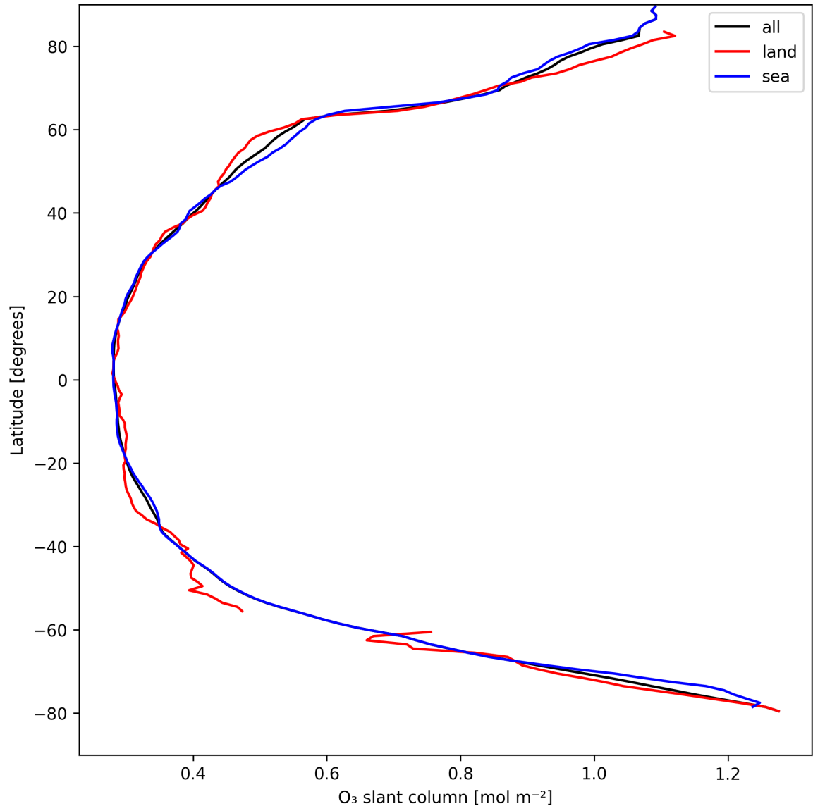
Figure 19: Zonal average of “O 3 slant column” for 2025-04-13 to 2025-04-14.
