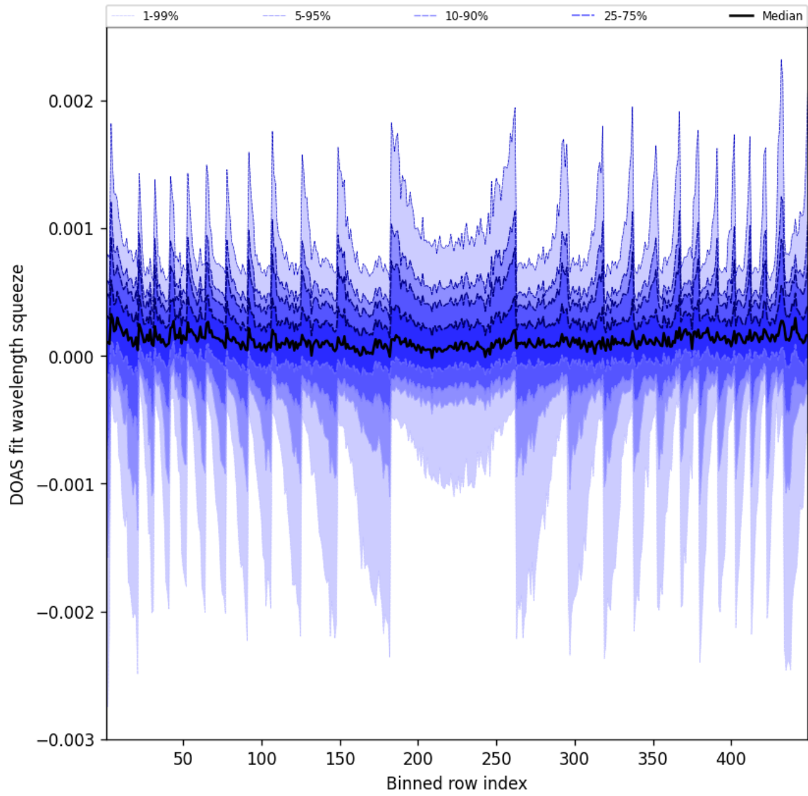
Figure 48: Along track statistics of “DOAS fit wavelength squeeze” for 2025-04-13 to 2025-04-14
