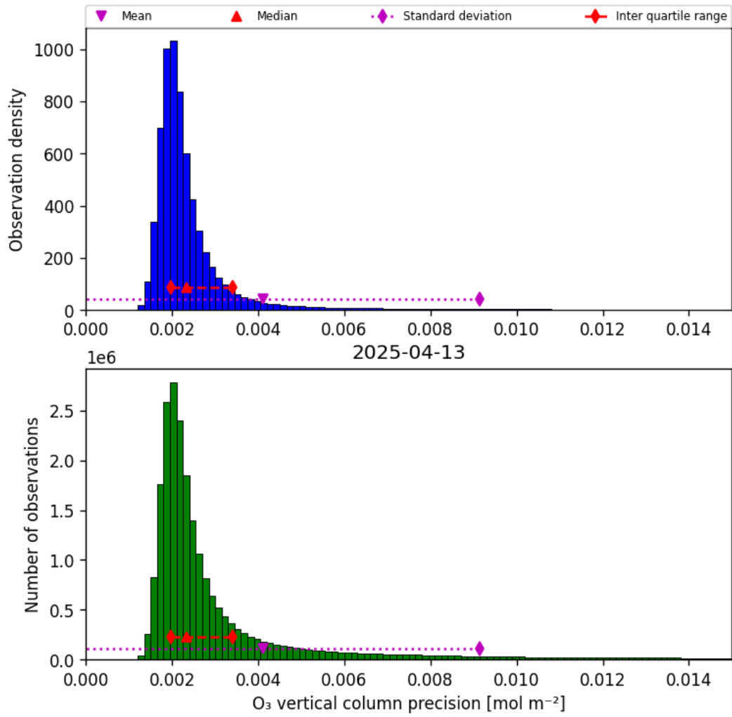
Figure 30: Histogram of “O 3 vertical column precision” for 2025-04-13 to 2025-04-14
