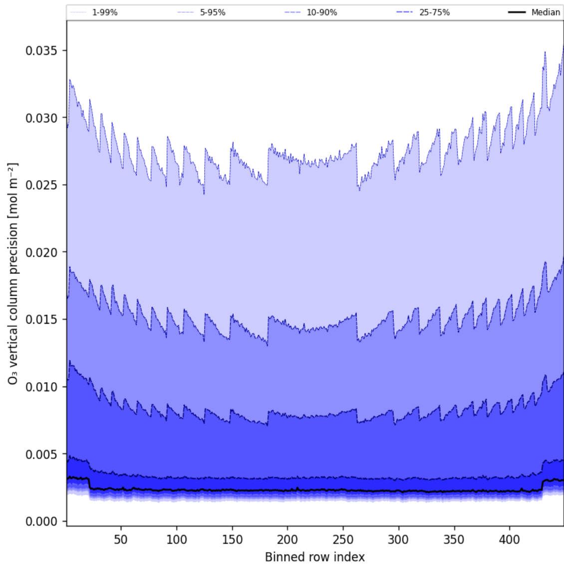
Figure 42: Along track statistics of “O 3 vertical column precision” for 2025-04-13 to 2025-04-14
