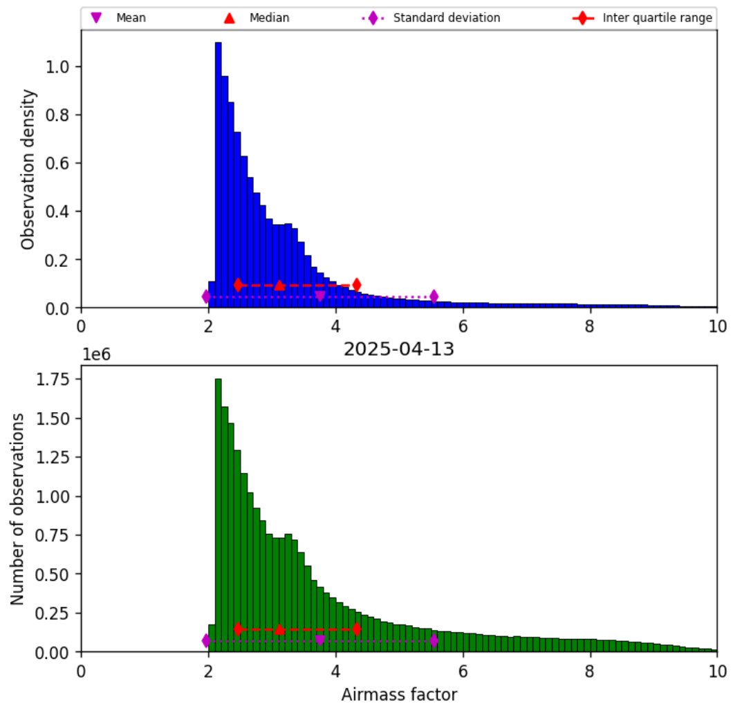
Figure 37: Histogram of “Airmass factor” for 2025-04-13 to 2025-04-14
