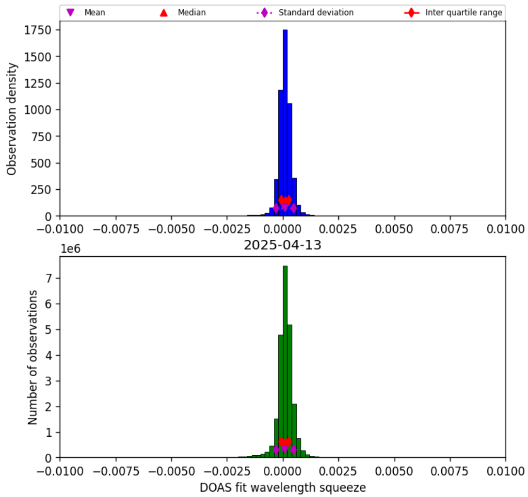
Figure 36: Histogram of “DOAS fit wavelength squeeze” for 2025-04-13 to 2025-04-14
