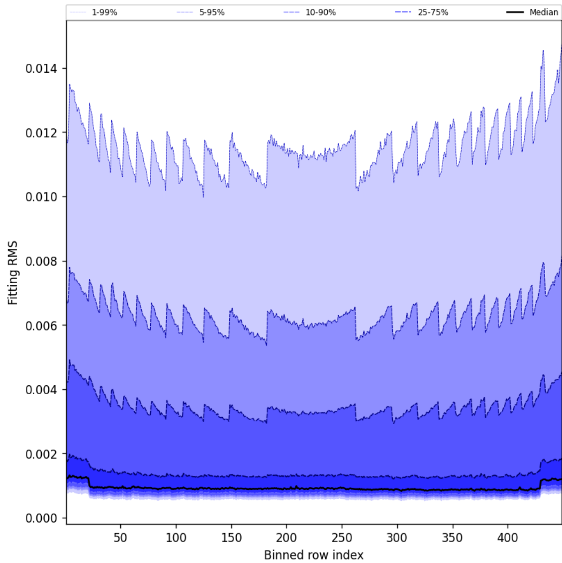
Figure 46: Along track statistics of “Fitting RMS” for 2025-04-13 to 2025-04-14
