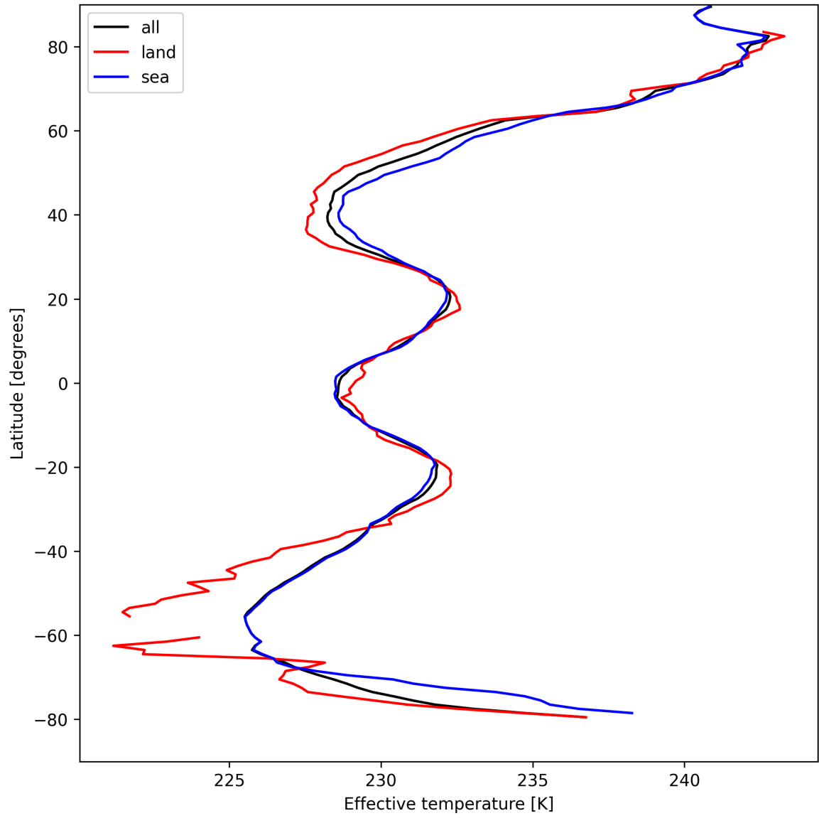
Figure 26: Zonal average of "Effective temperature" for 2025-04-13 to 2025-04-14.
