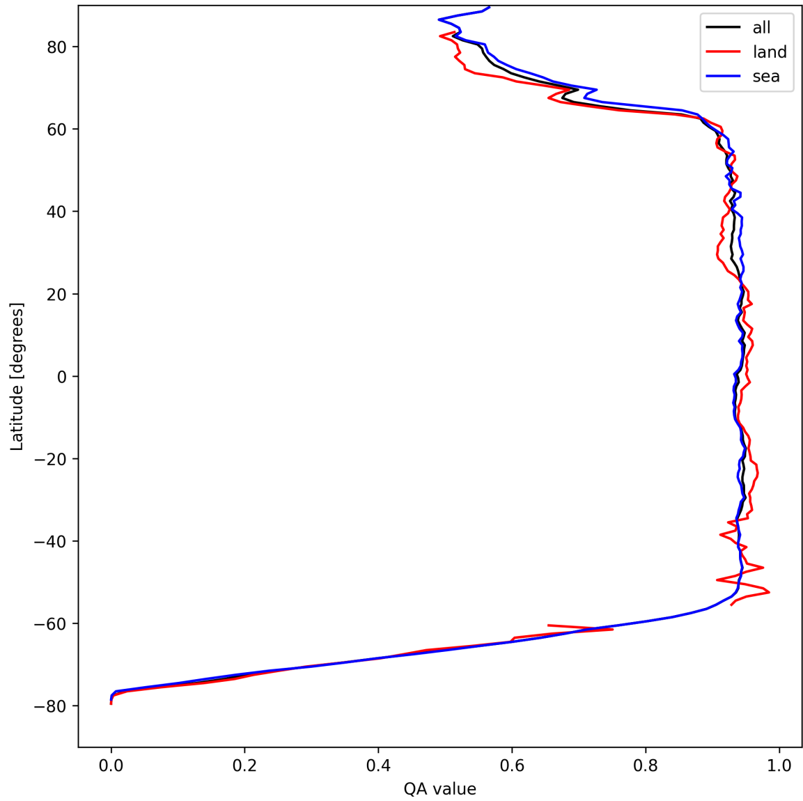
Figure 16: Zonal average of “QA value” for 2025-04-13 to 2025-04-14.
