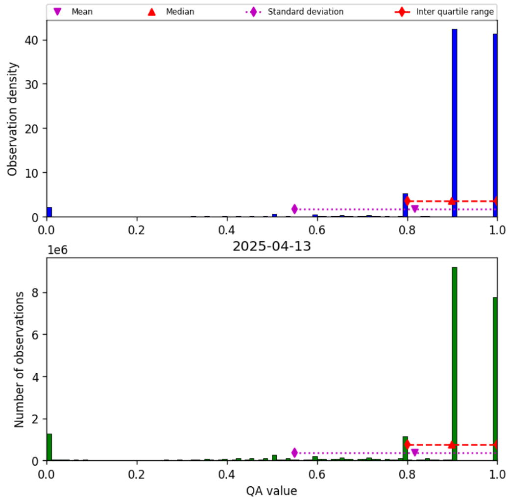
Figure 28: Histogram of “QA value” for 2025-04-13 to 2025-04-14
