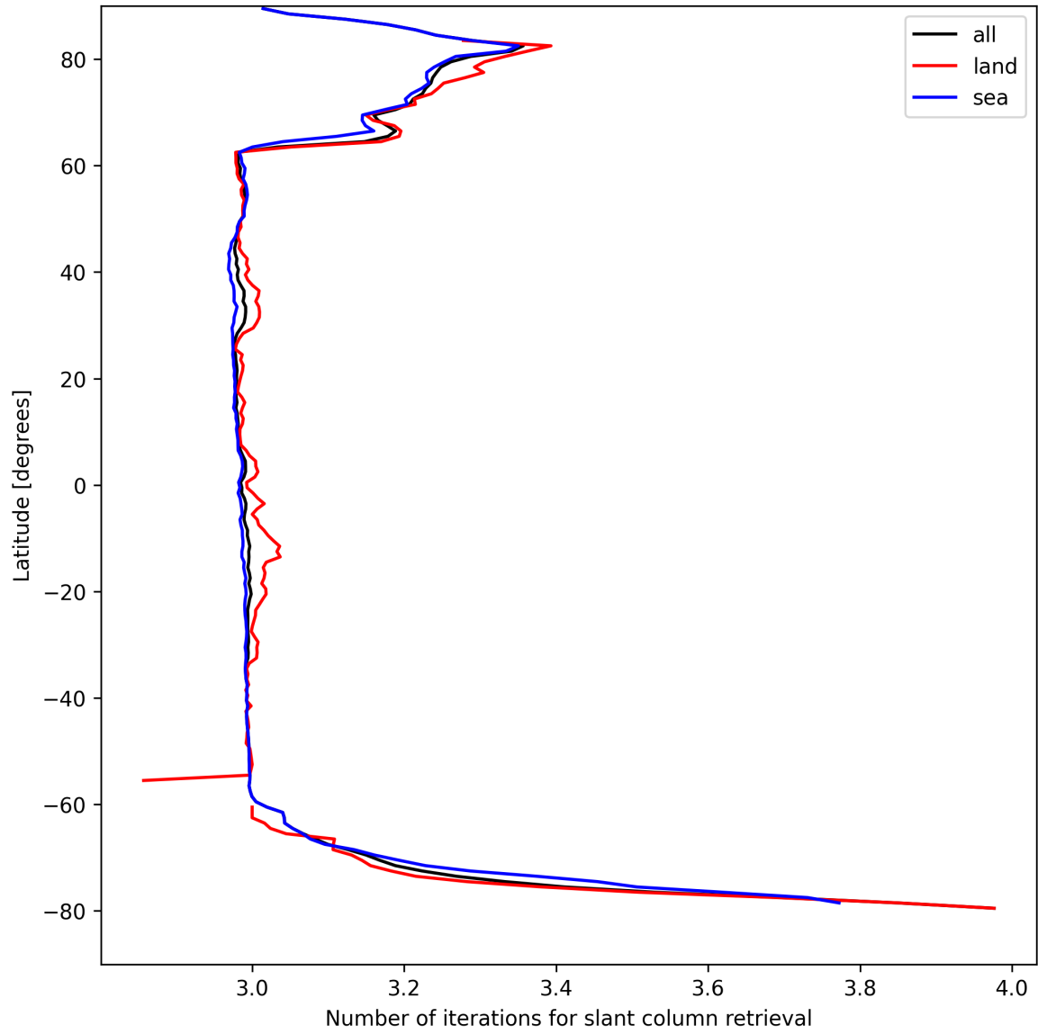
Figure 21: Zonal average of “Number of iterations for slant column retrieval” for 2025-04-13 to 2025-04-14.
