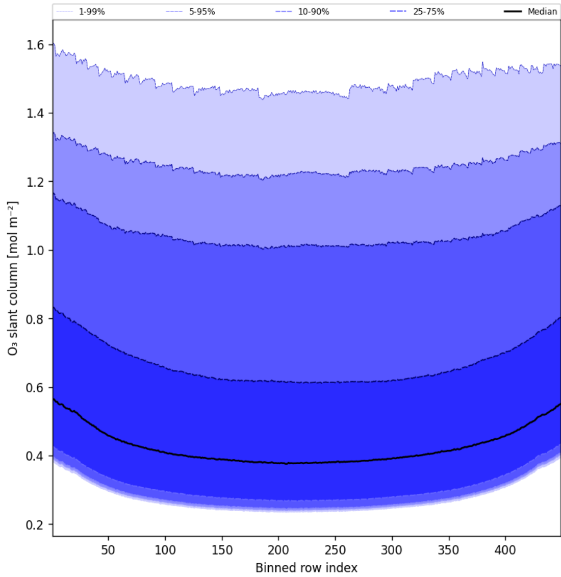
Figure 43: Along track statistics of “O 3 slant column” for 2025-04-13 to 2025-04-14
