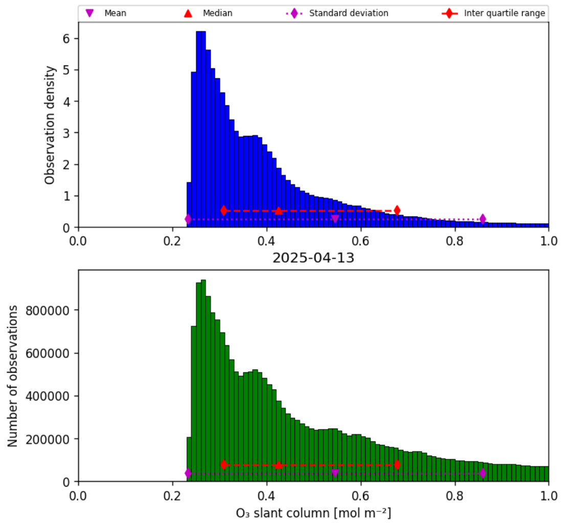
Figure 31: Histogram of “O 3 slant column” for 2025-04-13 to 2025-04-14
