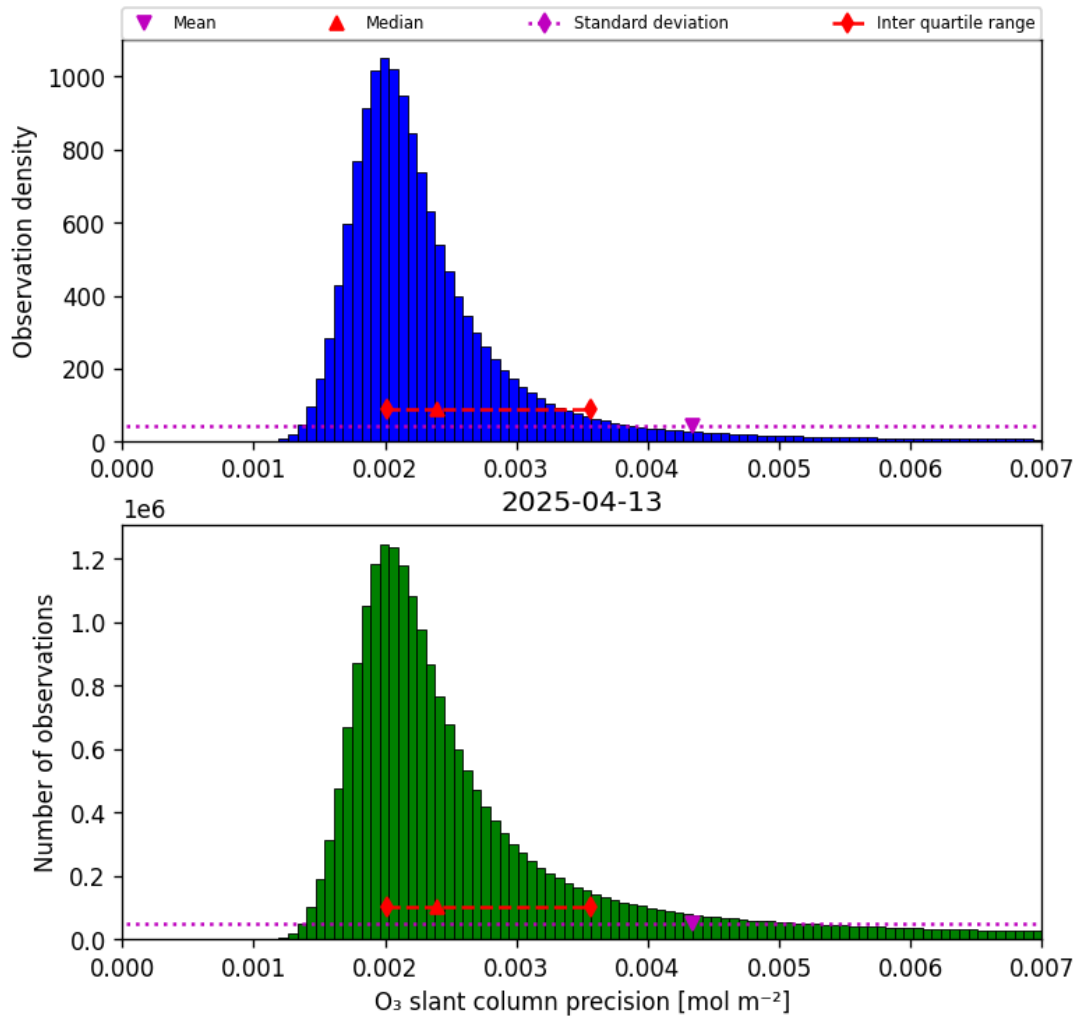
Figure 32: Histogram of “O 3 slant column precision” for 2025-04-13 to 2025-04-14
