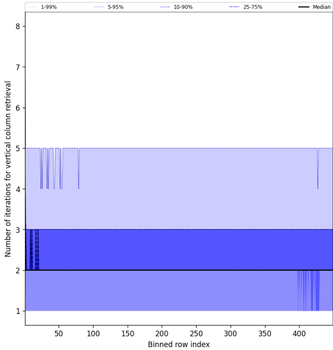
Figure 51: Along track statistics of “Number of iterations for vertical column retrieval” for 2025-04-13 to 2025-04-14
