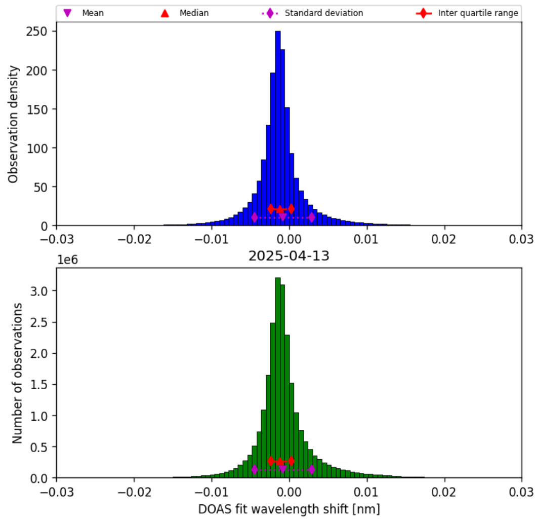
Figure 35: Histogram of “DOAS fit wavelength shift” for 2025-04-13 to 2025-04-14
