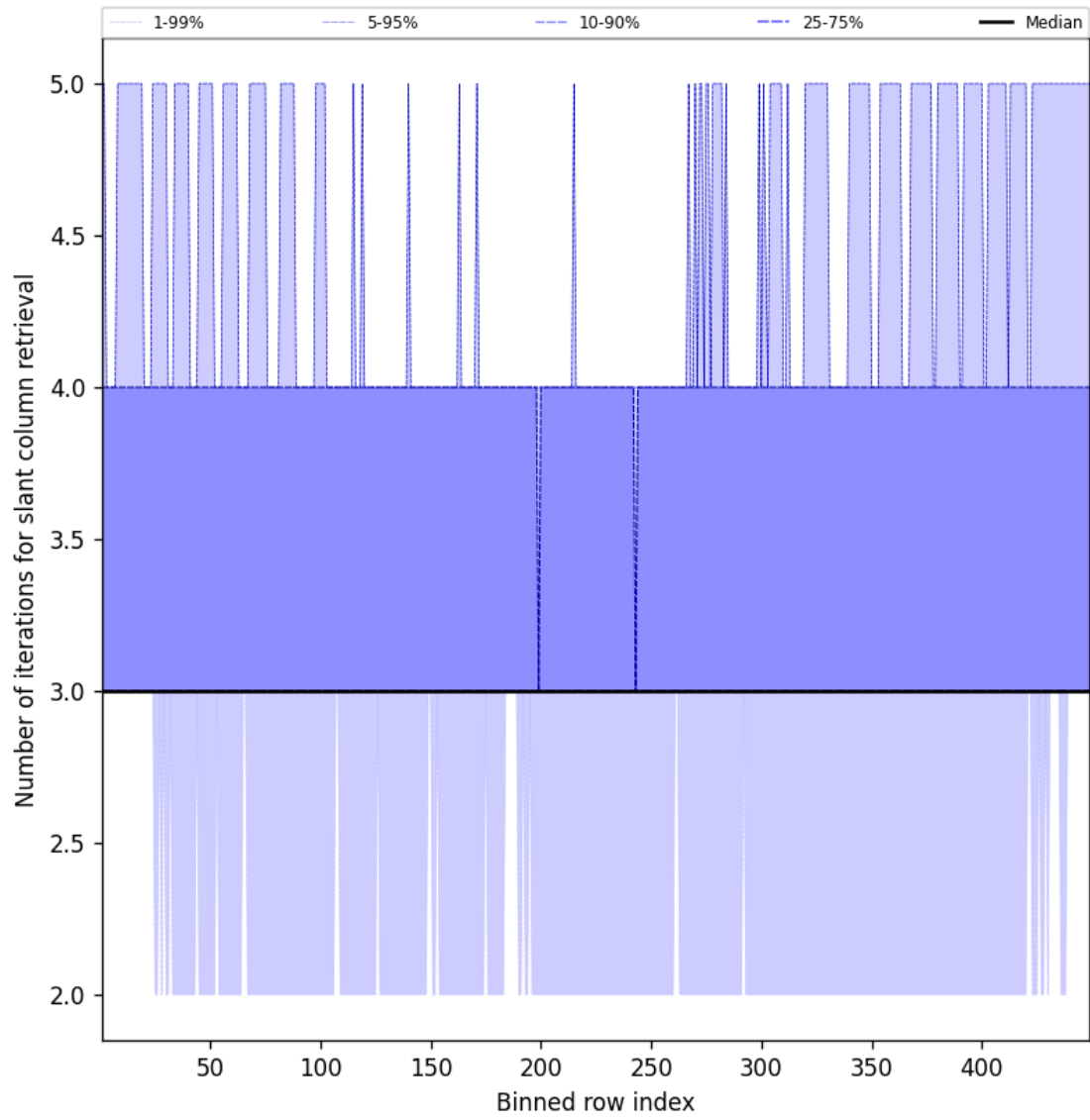
Figure 45: Along track statistics of “Number of iterations for slant column retrieval” for 2025-04-13 to 2025-04-14
