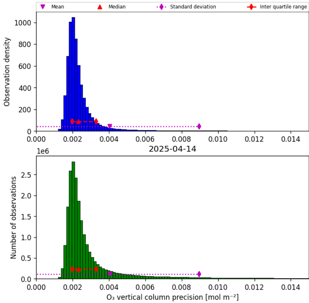
Figure 30: Histogram of “O 3 vertical column precision” for 2025-04-14 to 2025-04-15
