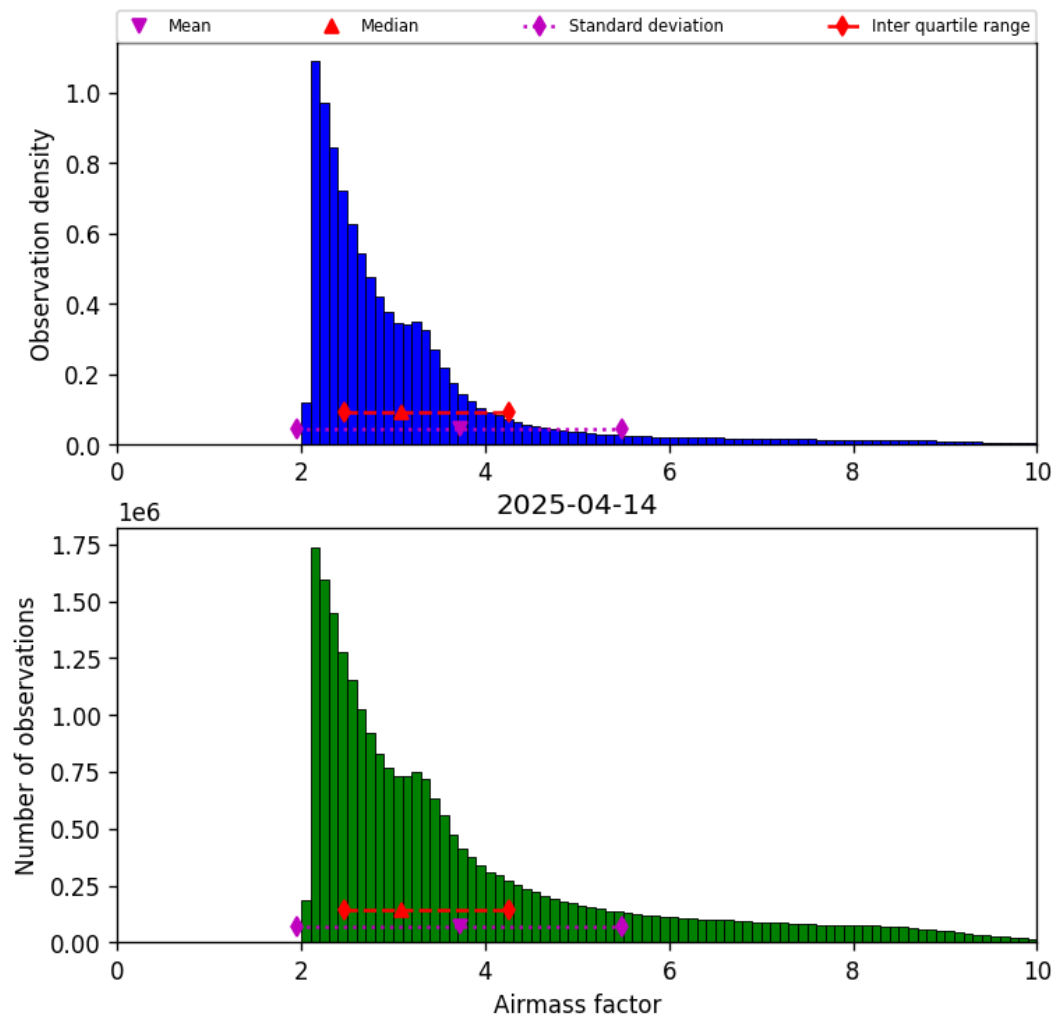
Figure 37: Histogram of “Airmass factor” for 2025-04-14 to 2025-04-15
