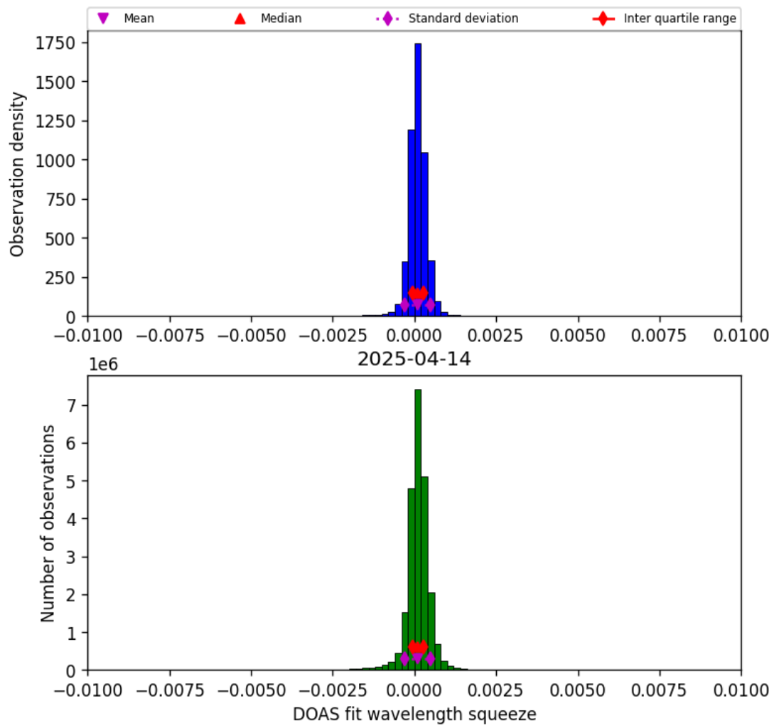
Figure 36: Histogram of “DOAS fit wavelength squeeze” for 2025-04-14 to 2025-04-15
