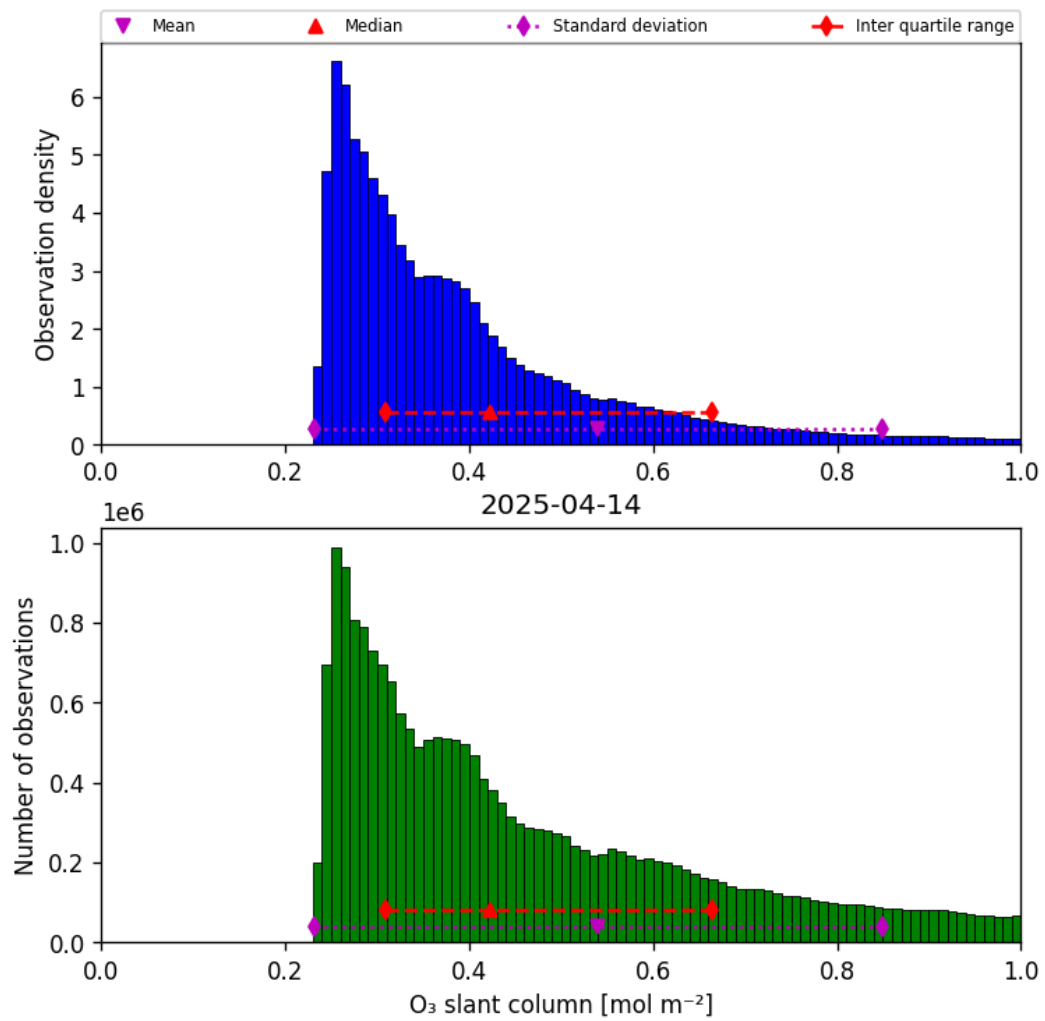
Figure 31: Histogram of “O 3 slant column” for 2025-04-14 to 2025-04-15
