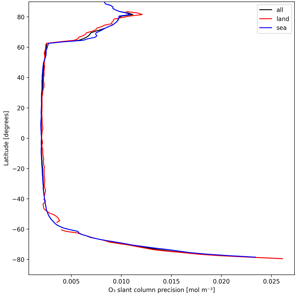
Figure 20: Zonal average of “O 3 slant column precision” for 2025-04-14 to 2025-04-15.
