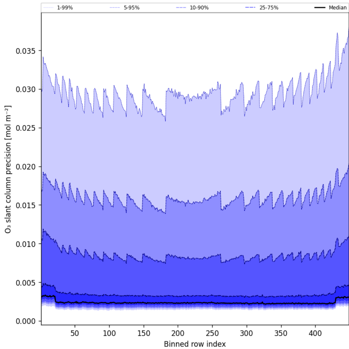
Figure 44: Along track statistics of "O 3 slant column precision" for 2025-04-14 to 2025-04-15
