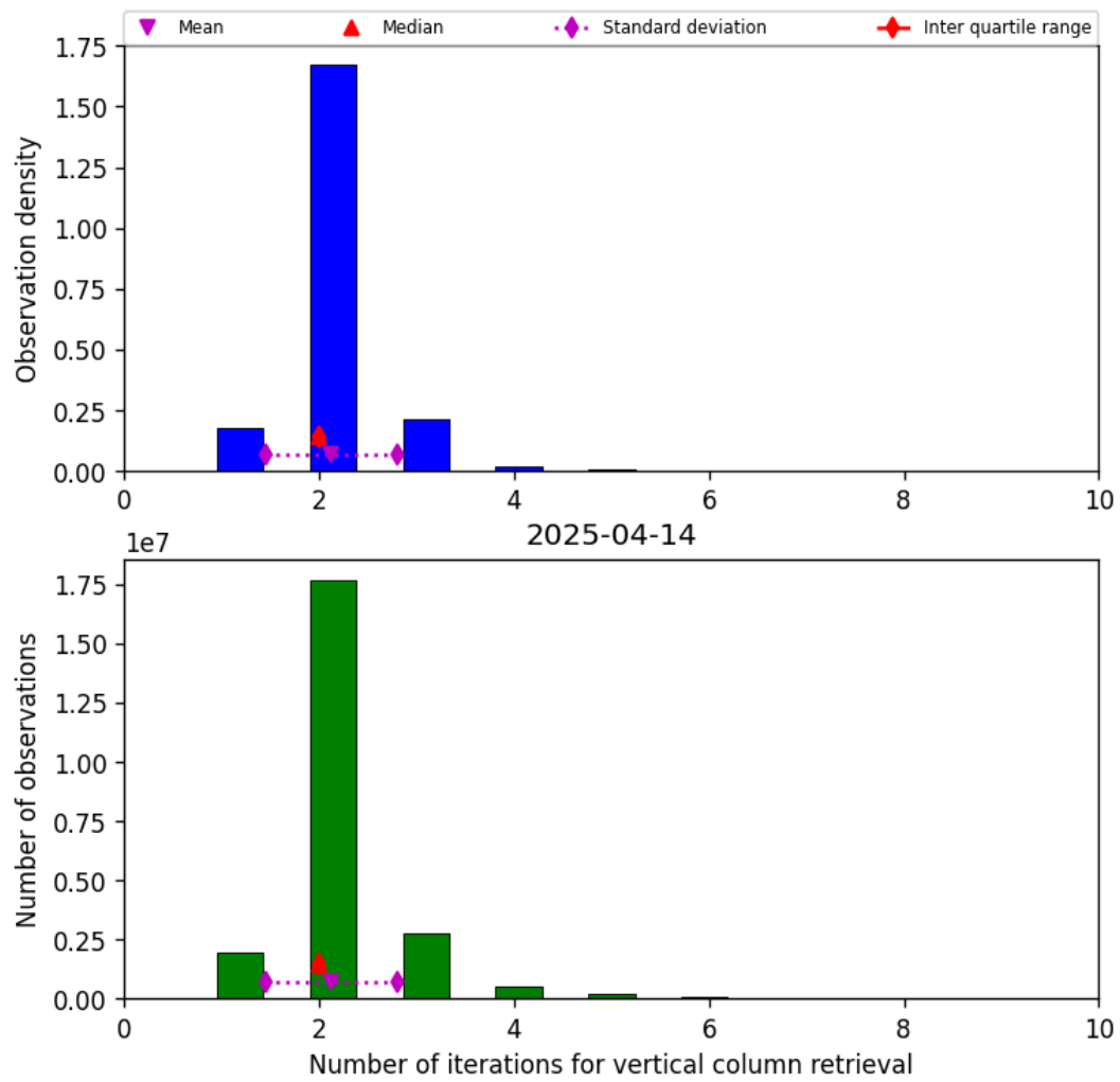
Figure 39: Histogram of “Number of iterations for vertical column retrieval” for 2025-04-14 to 2025-04-15
