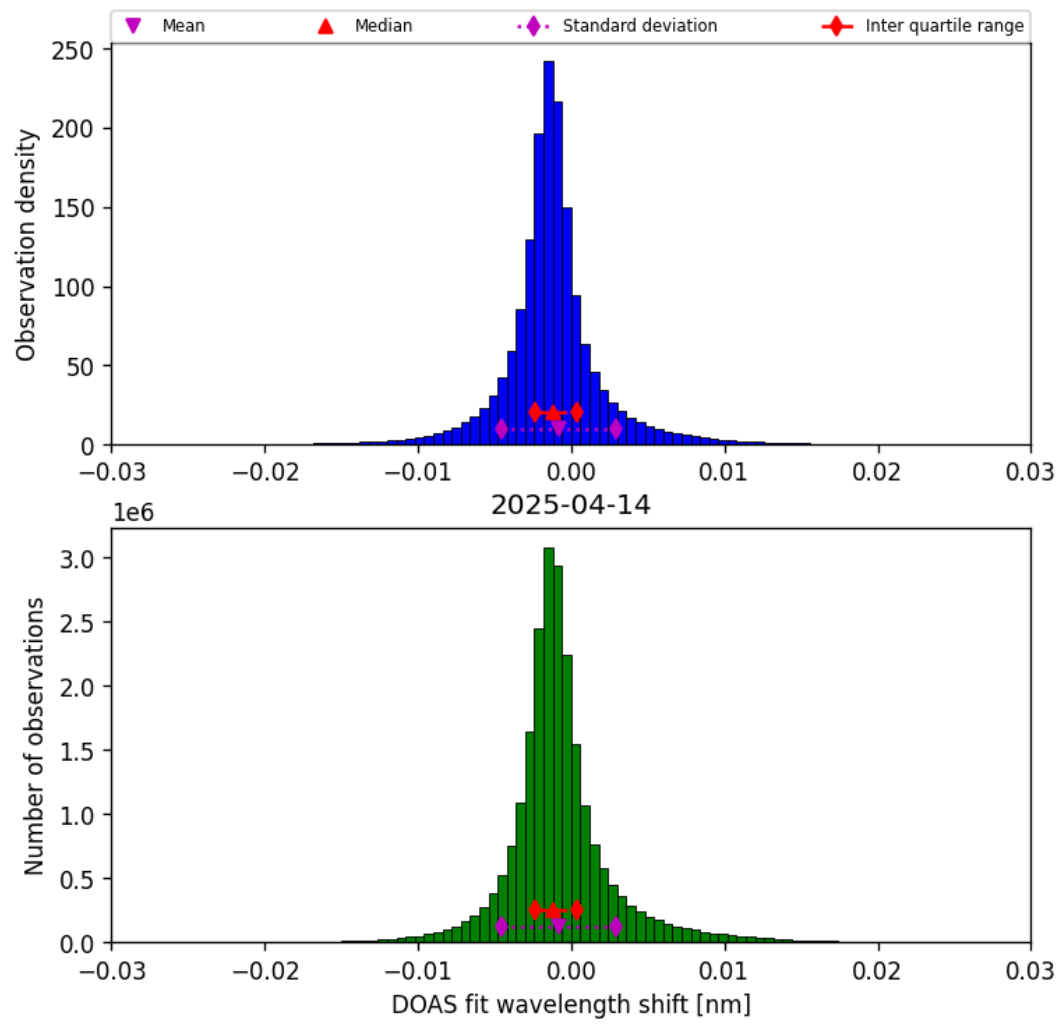
Figure 35: Histogram of “DOAS fit wavelength shift” for 2025-04-14 to 2025-04-15
