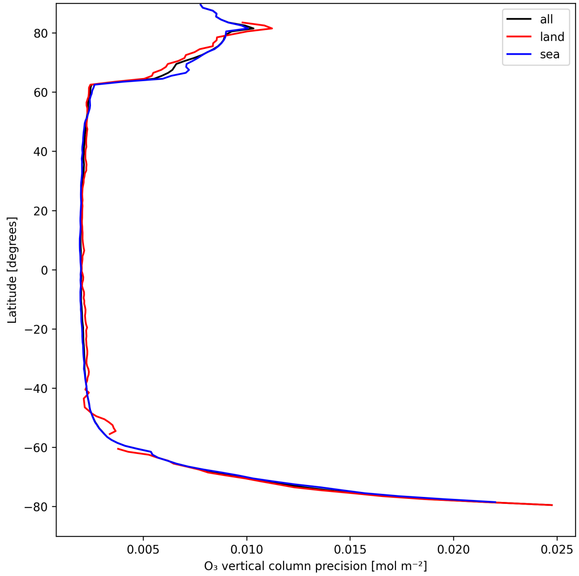
Figure 18: Zonal average of “O 3 vertical column precision” for 2025-04-14 to 2025-04-15.
