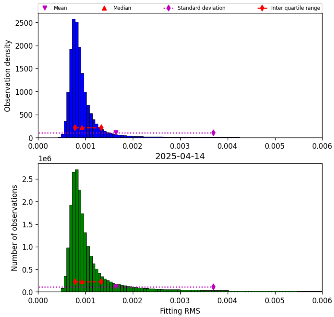
Figure 34: Histogram of “Fitting RMS” for 2025-04-14 to 2025-04-15
