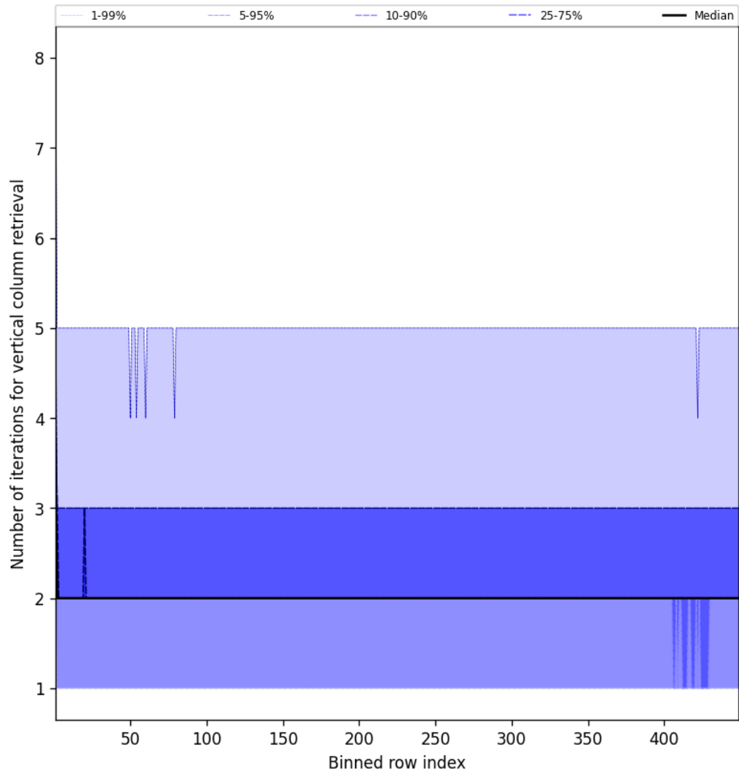
Figure 51: Along track statistics of “Number of iterations for vertical column retrieval” for 2025-04-14 to 2025-04-15
