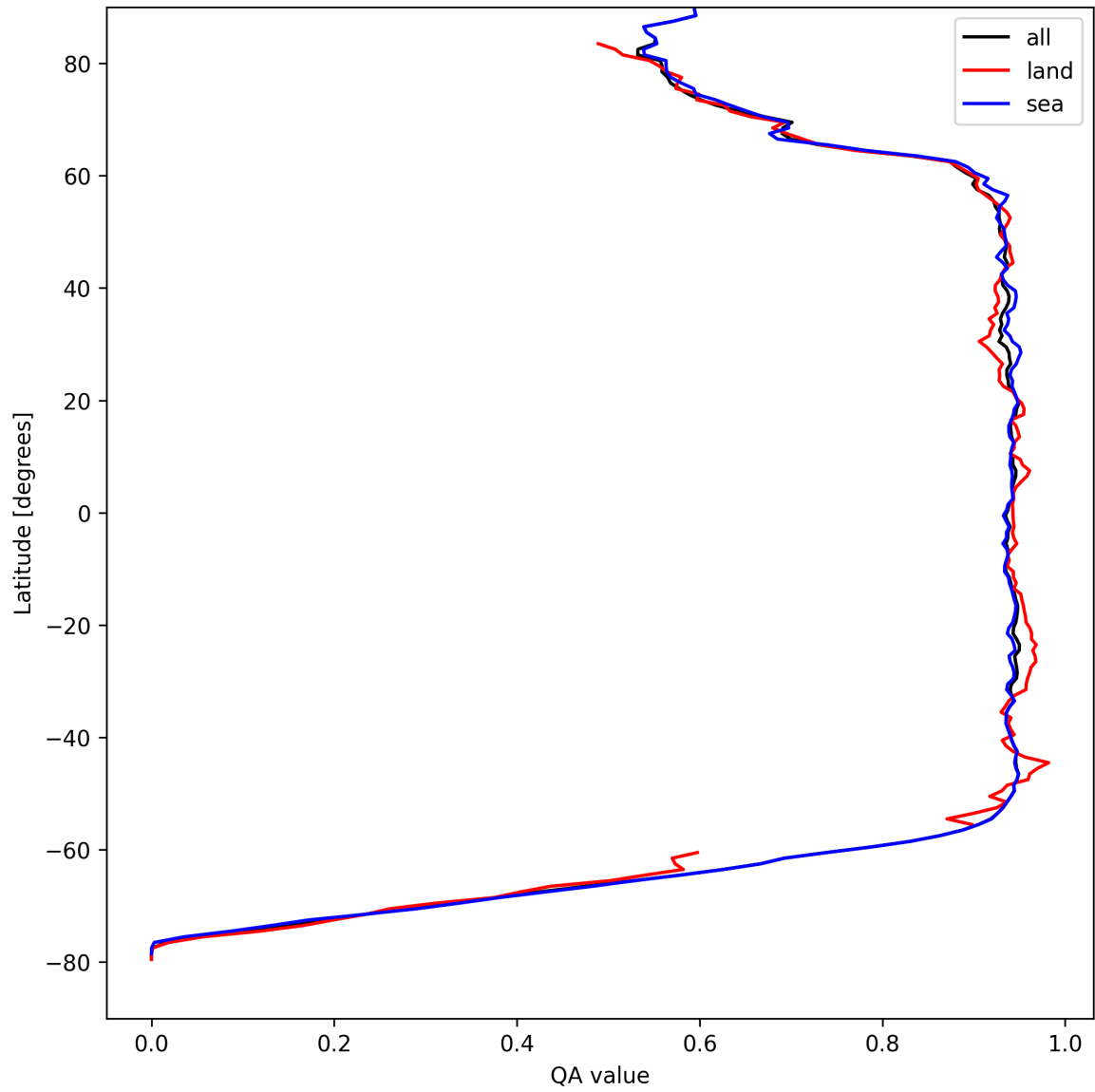
Figure 16: Zonal average of “QA value” for 2025-04-14 to 2025-04-15.
