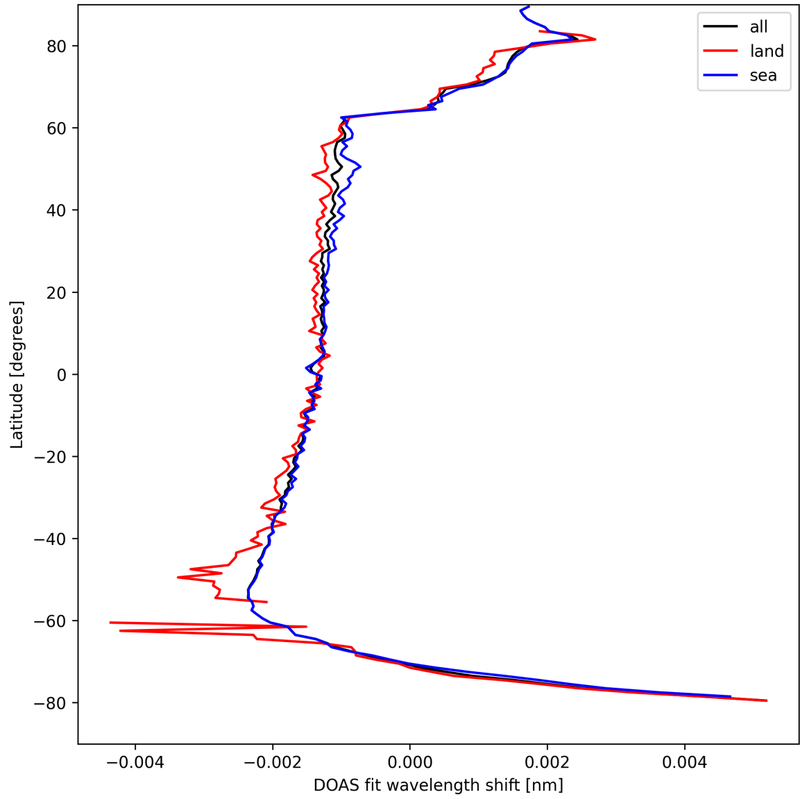
Figure 23: Zonal average of “DOAS fit wavelength shift” for 2025-04-14 to 2025-04-15.
