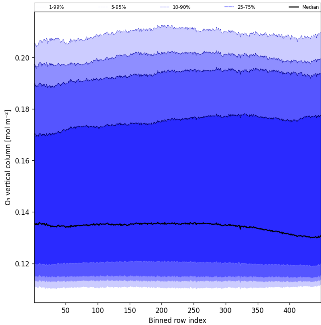
Figure 41: Along track statistics of “O 3 vertical column” for 2025-04-14 to 2025-04-15
