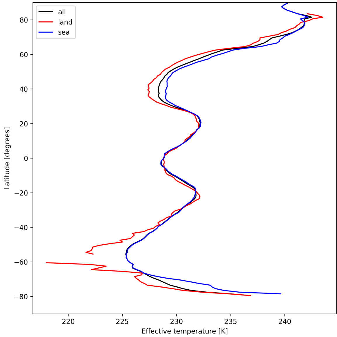
Figure 26: Zonal average of “Effective temperature” for 2025-04-14 to 2025-04-15.
