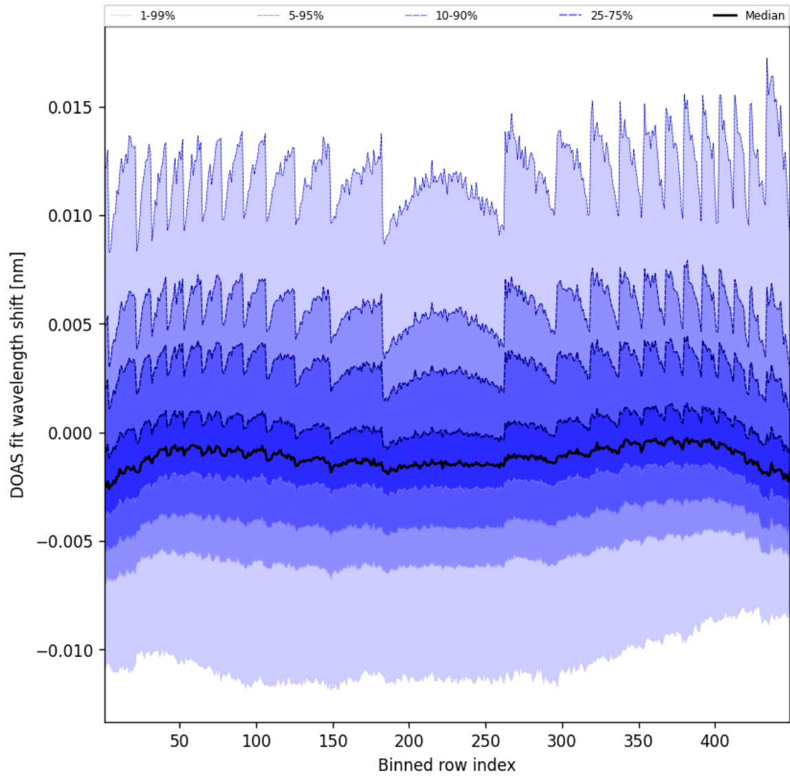
Figure 47: Along track statistics of “DOAS fit wavelength shift” for 2025-04-14 to 2025-04-15
