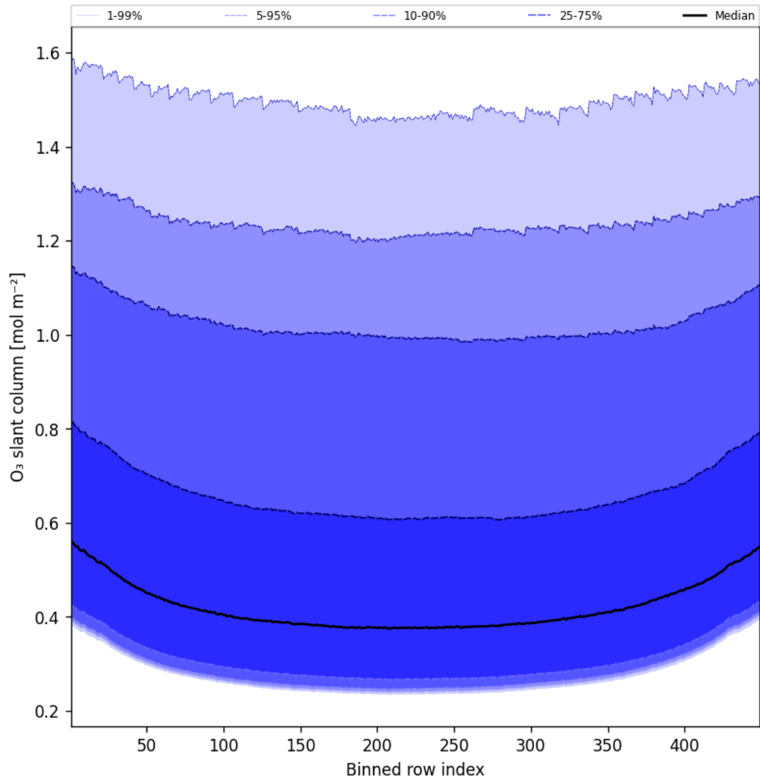
Figure 43: Along track statistics of “O 3 slant column” for 2025-04-14 to 2025-04-15
