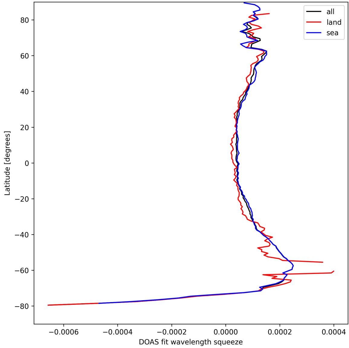
Figure 24: Zonal average of “DOAS fit wavelength squeeze” for 2025-04-14 to 2025-04-15.
