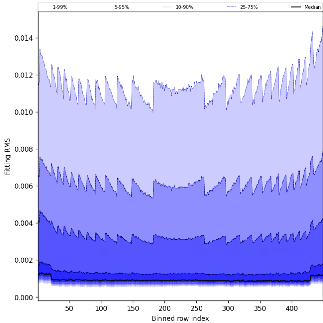
Figure 46: Along track statistics of “Fitting RMS” for 2025-04-14 to 2025-04-15
