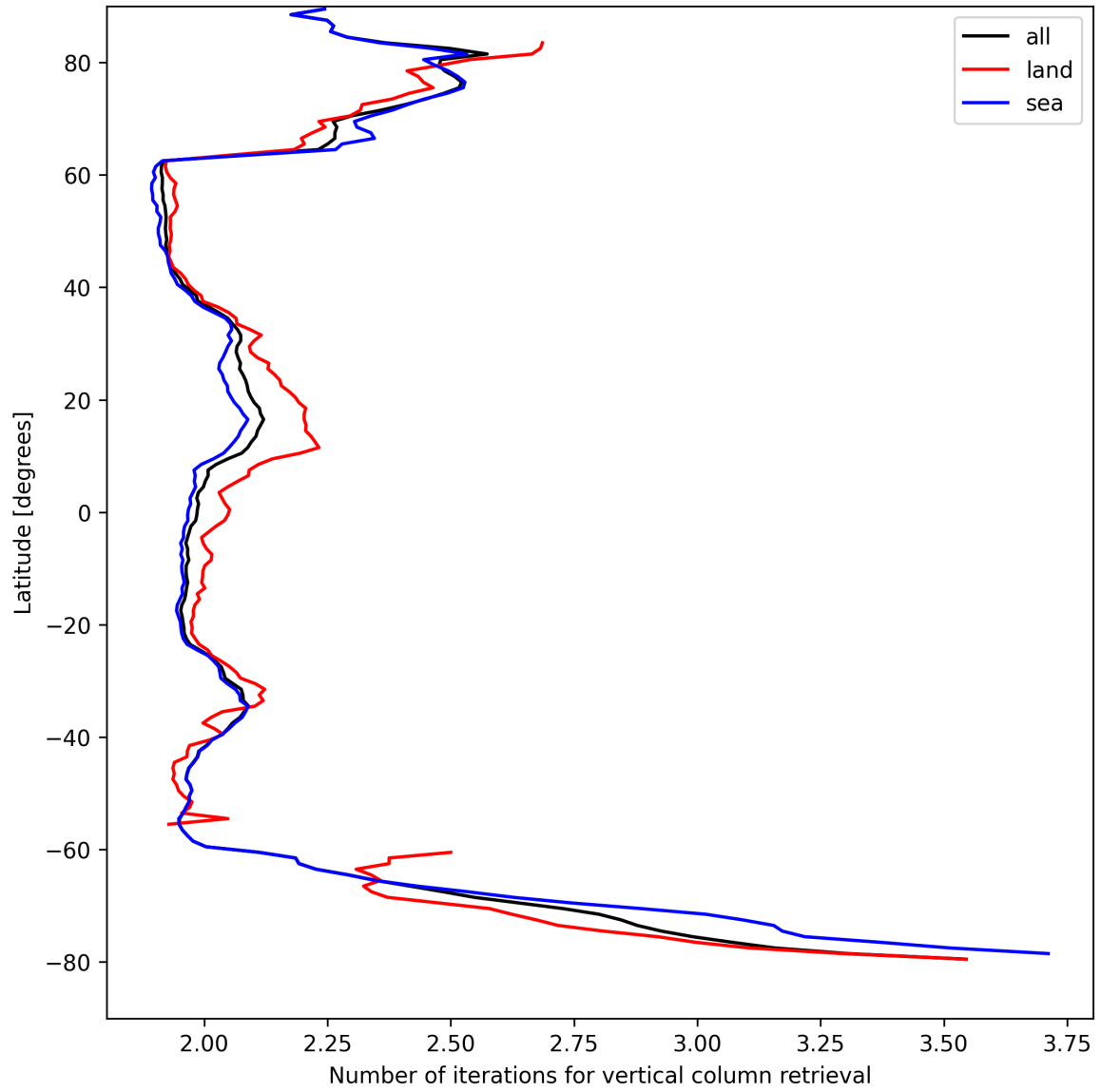
Figure 27: Zonal average of “Number of iterations for vertical column retrieval” for 2025-04-14 to 2025-04-15.
