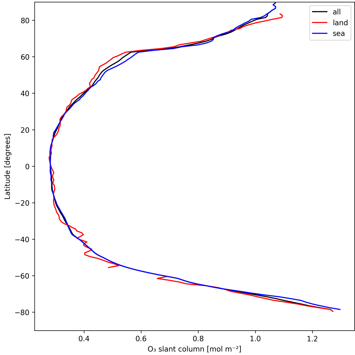
Figure 19: Zonal average of “O 3 slant column” for 2025-04-14 to 2025-04-15.
