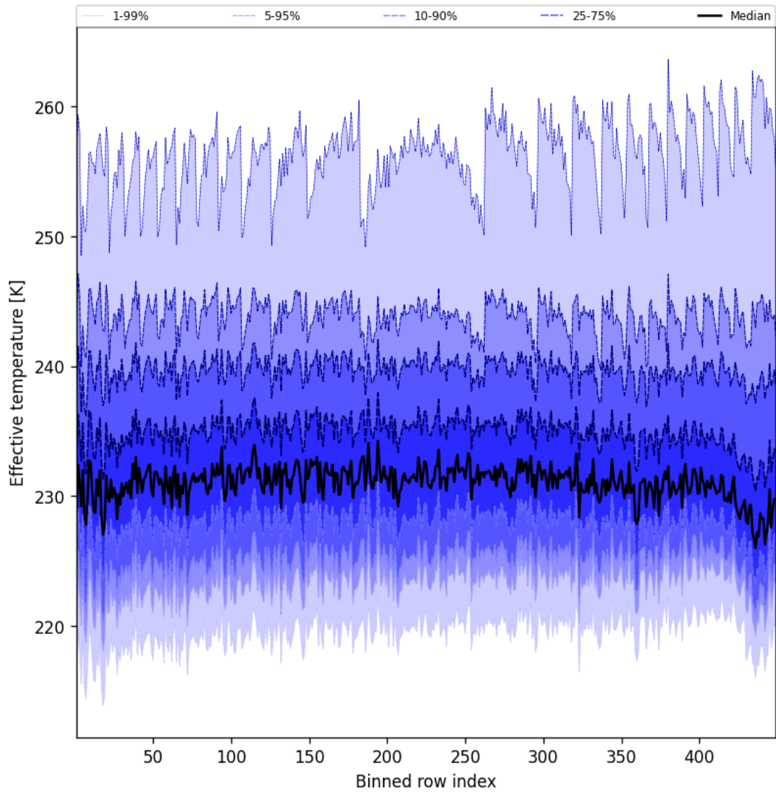
Figure 50: Along track statistics of “Effective temperature” for 2025-04-14 to 2025-04-15
