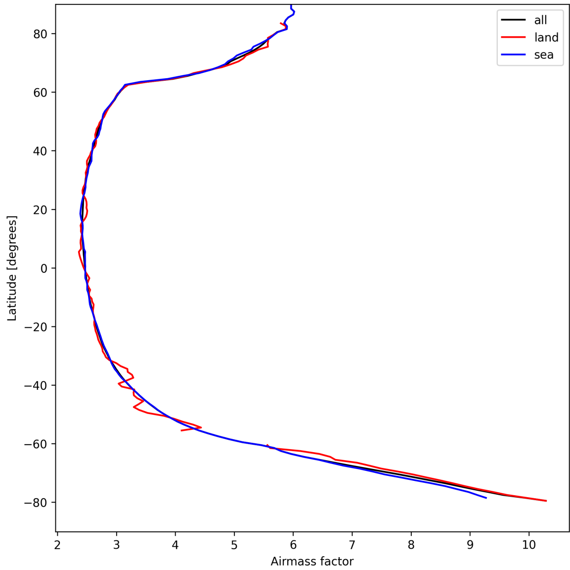
Figure 25: Zonal average of “Airmass factor” for 2025-04-14 to 2025-04-15.
