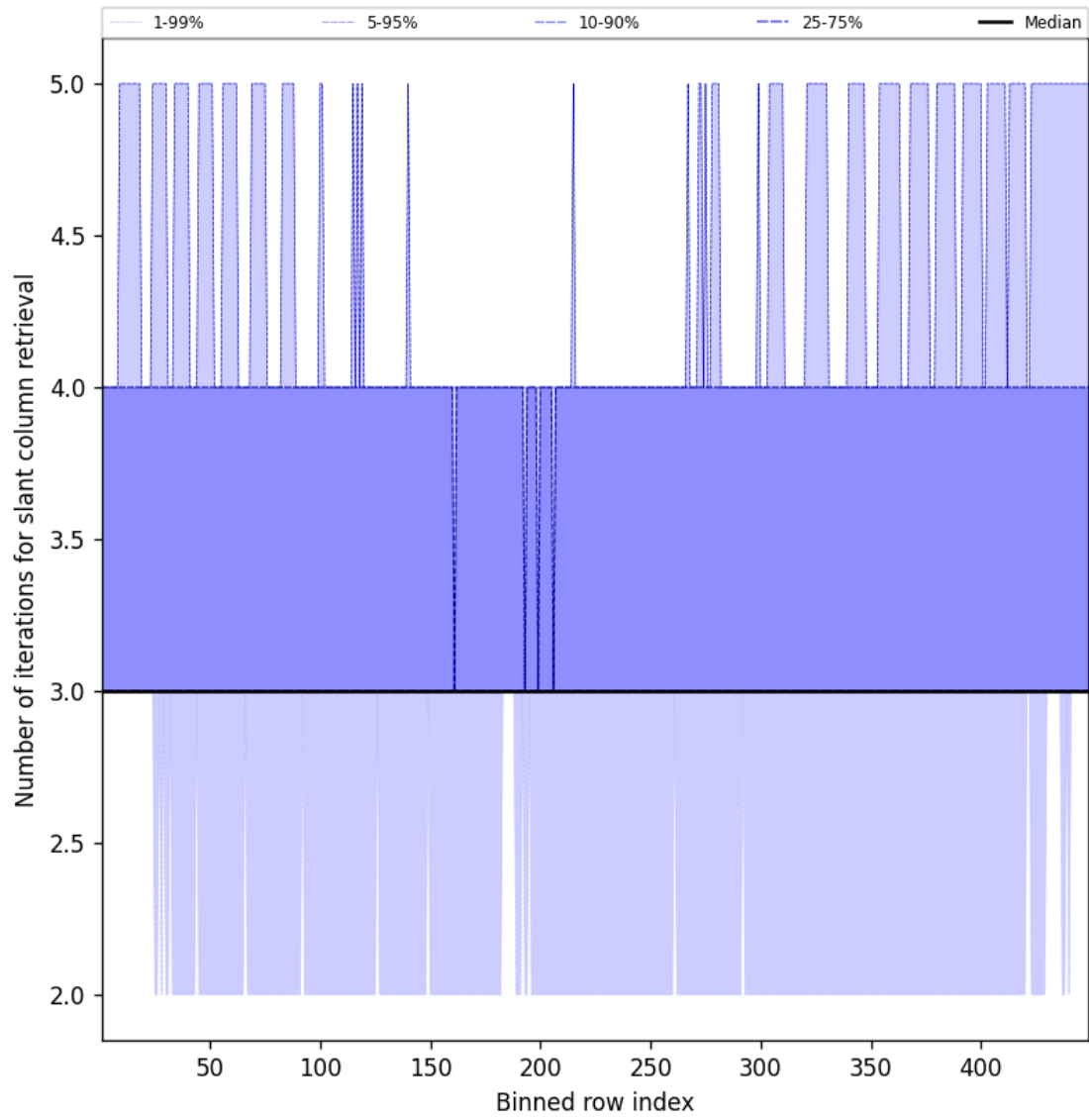
Figure 45: Along track statistics of “Number of iterations for slant column retrieval” for 2025-04-14 to 2025-04-15
