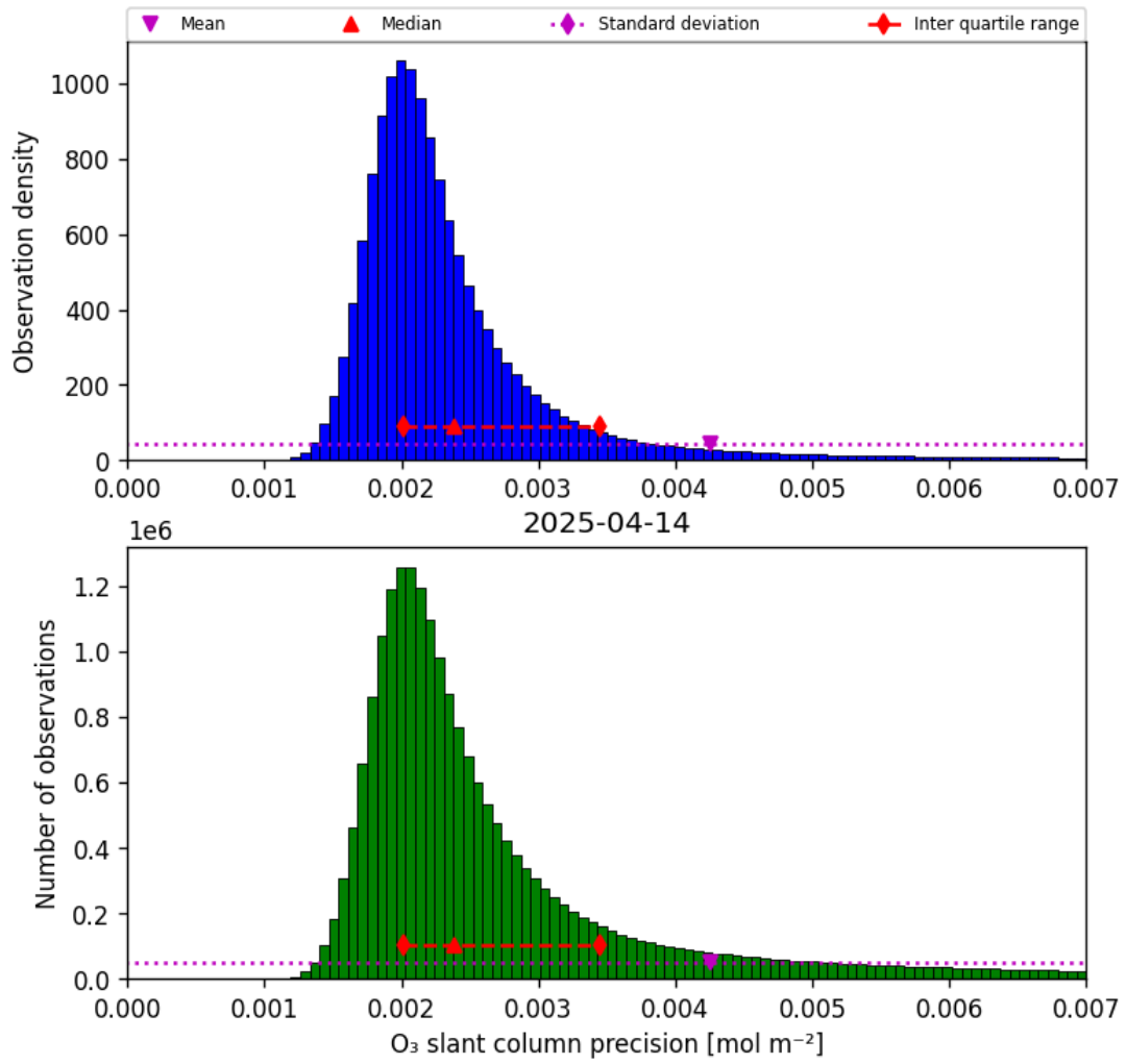
Figure 32: Histogram of "O 3 slant column precision" for 2025-04-14 to 2025-04-15
