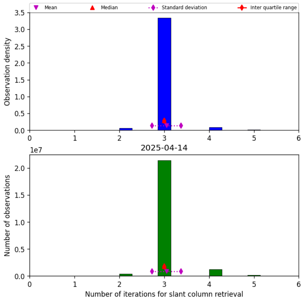
Figure 33: Histogram of "Number of iterations for slant column retrieval" for 2025-04-14 to 2025-04-15
