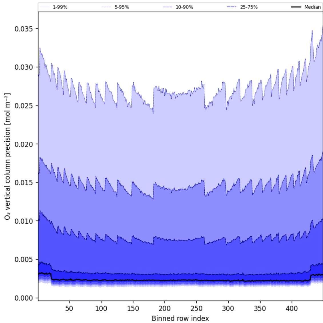
Figure 42: Along track statistics of “O 3 vertical column precision” for 2025-04-14 to 2025-04-15
