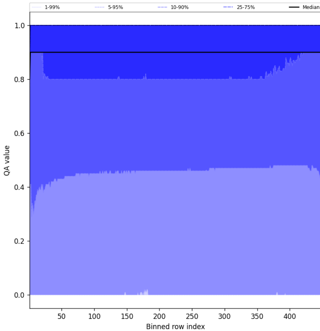
Figure 40: Along track statistics of “QA value” for 2025-04-14 to 2025-04-15
