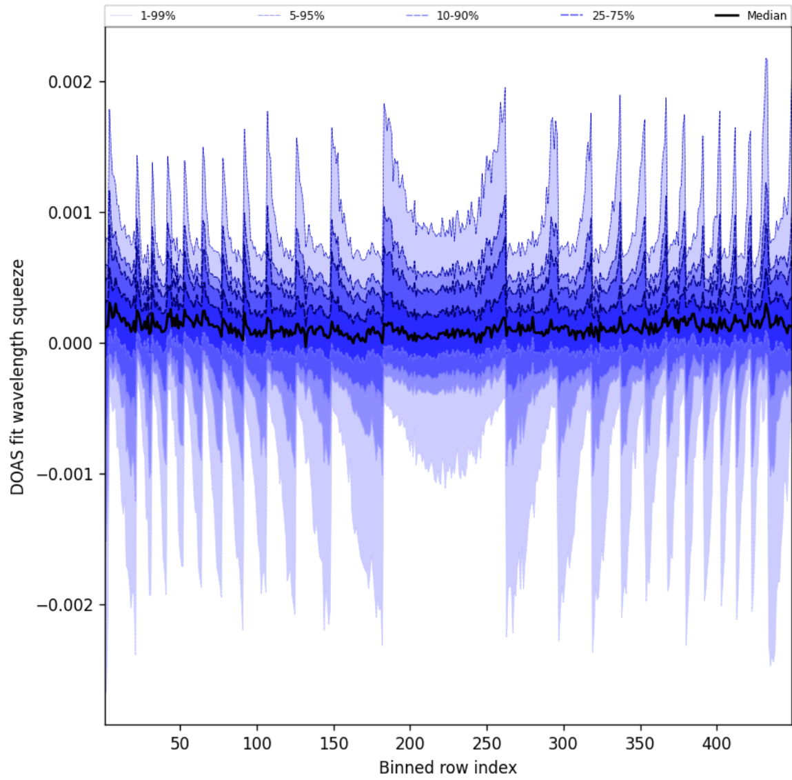
Figure 48: Along track statistics of “DOAS fit wavelength squeeze” for 2025-04-14 to 2025-04-15
