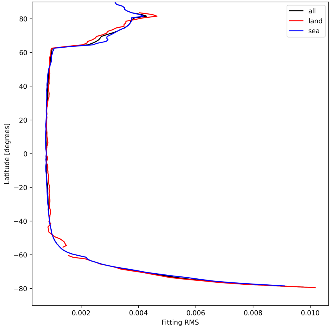
Figure 22: Zonal average of “Fitting RMS” for 2025-04-14 to 2025-04-15.
