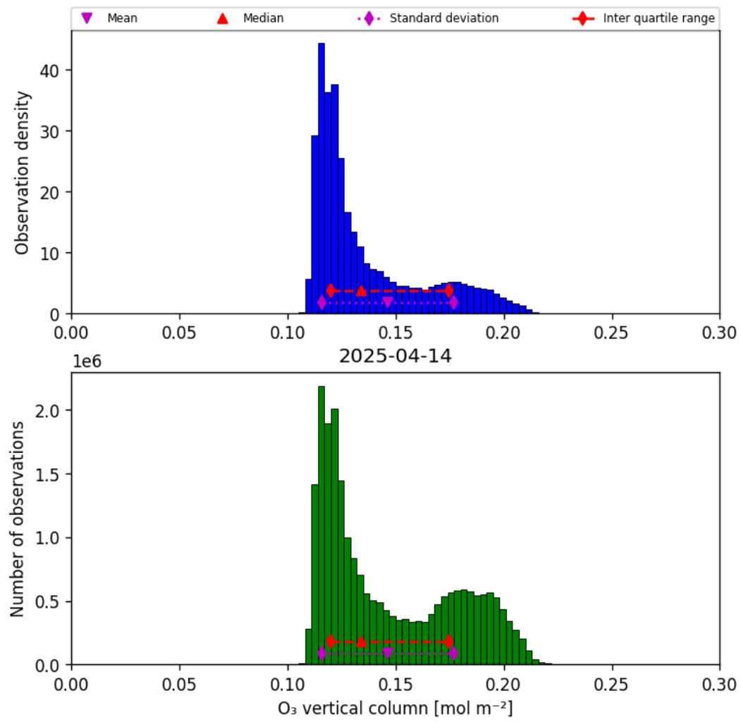
Figure 29: Histogram of “O 3 vertical column” for 2025-04-14 to 2025-04-15
