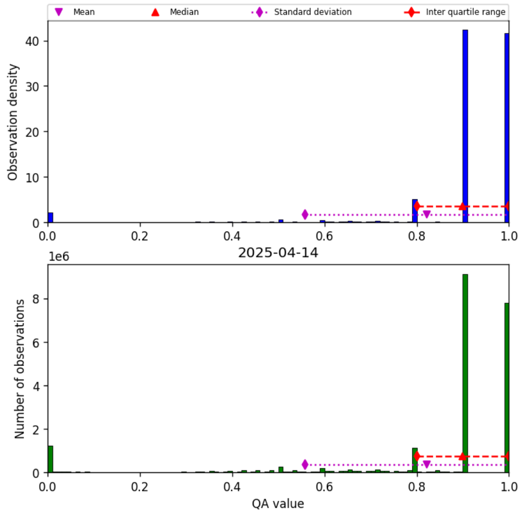
Figure 28: Histogram of “QA value” for 2025-04-14 to 2025-04-15
