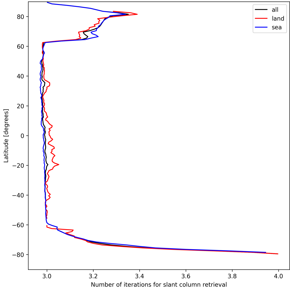
Figure 21: Zonal average of “Number of iterations for slant column retrieval” for 2025-04-14 to 2025-04-15.
