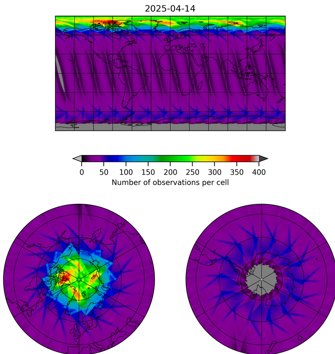
Figure 15: Map of the number of observations for 2025-04-14 to 2025-04-15
