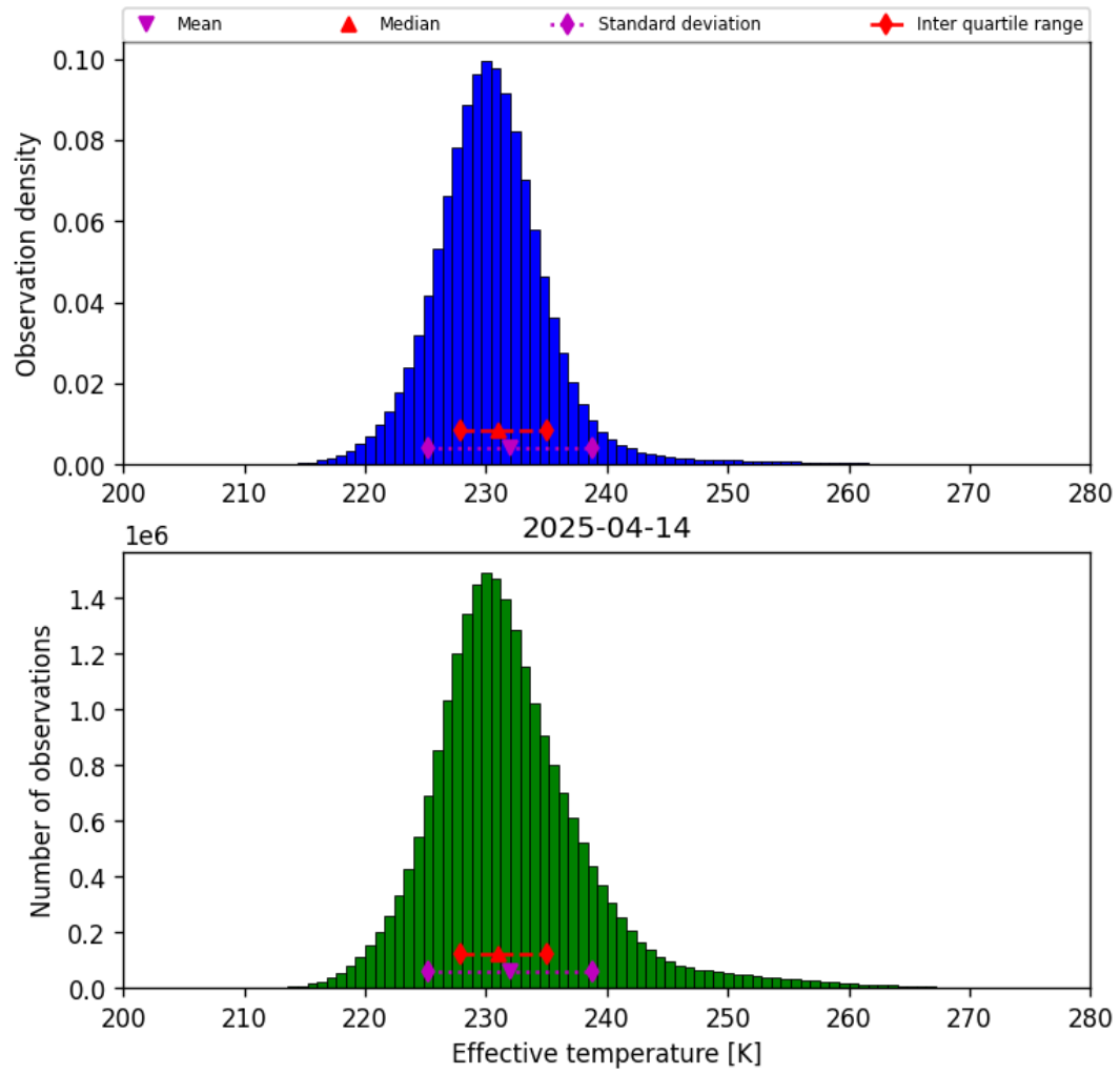
Figure 38: Histogram of “Effective temperature” for 2025-04-14 to 2025-04-15
