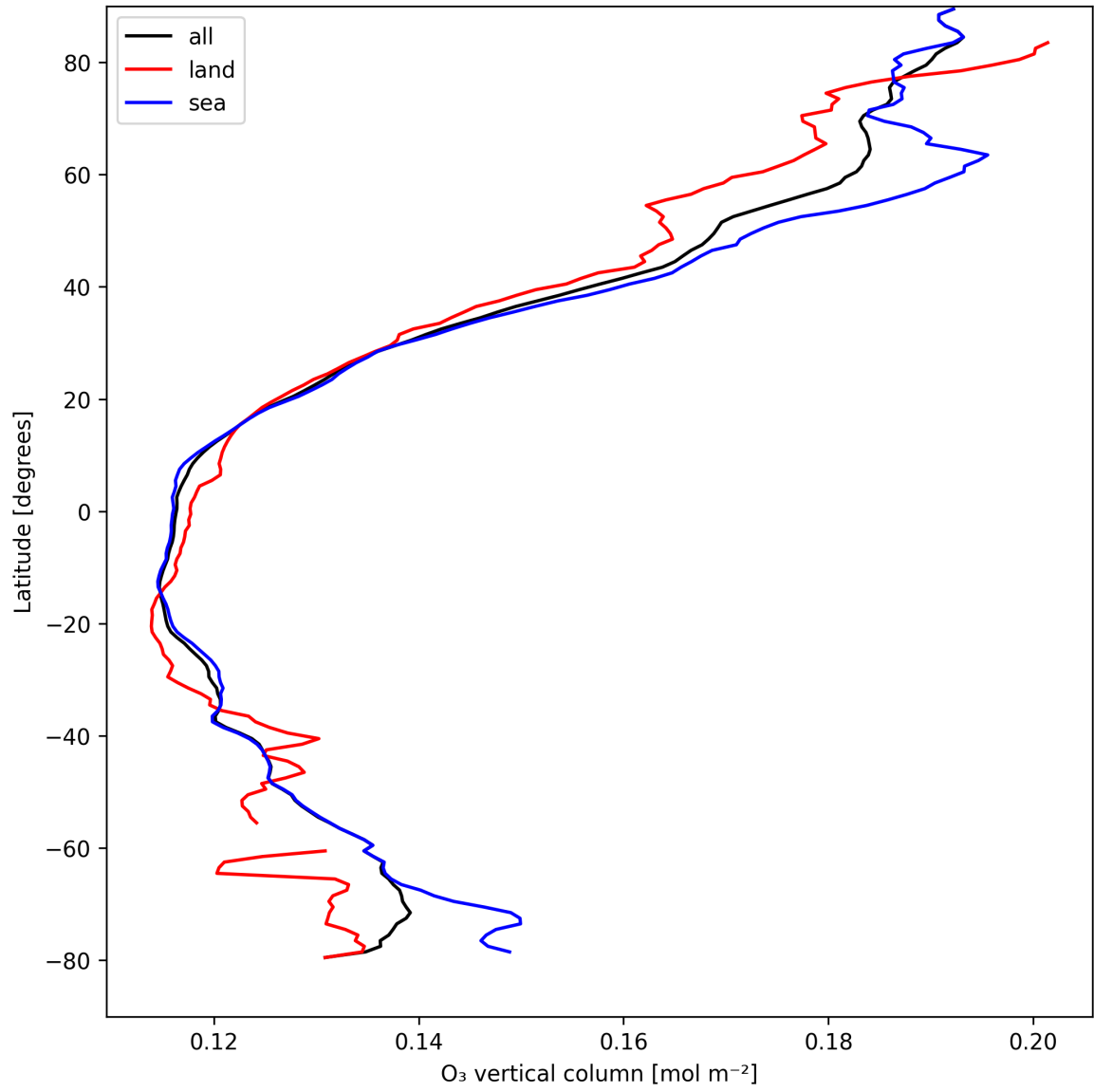
Figure 17: Zonal average of “O 3 vertical column” for 2025-04-14 to 2025-04-15.
