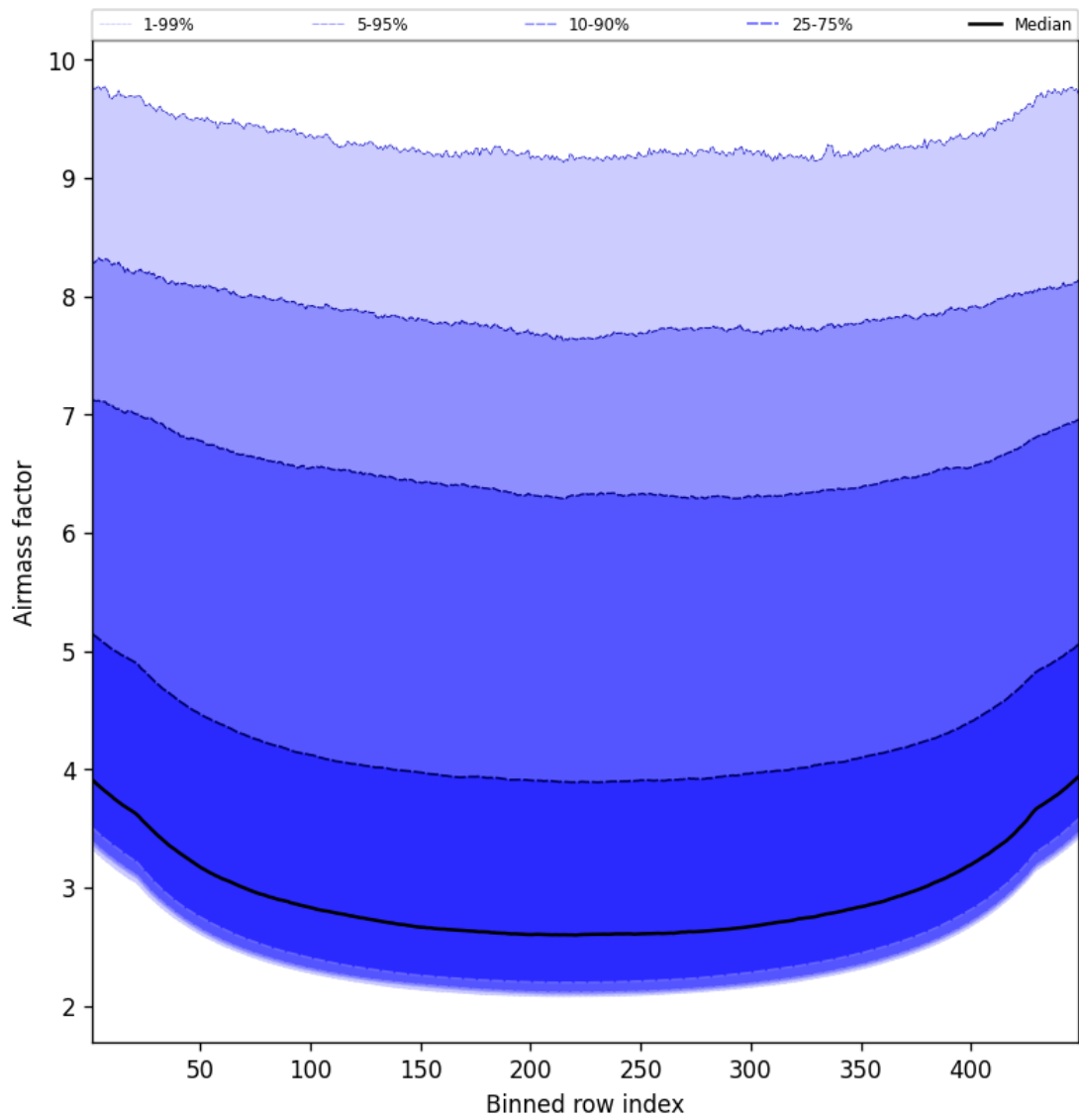
Figure 49: Along track statistics of “Airmass factor” for 2025-04-14 to 2025-04-15
