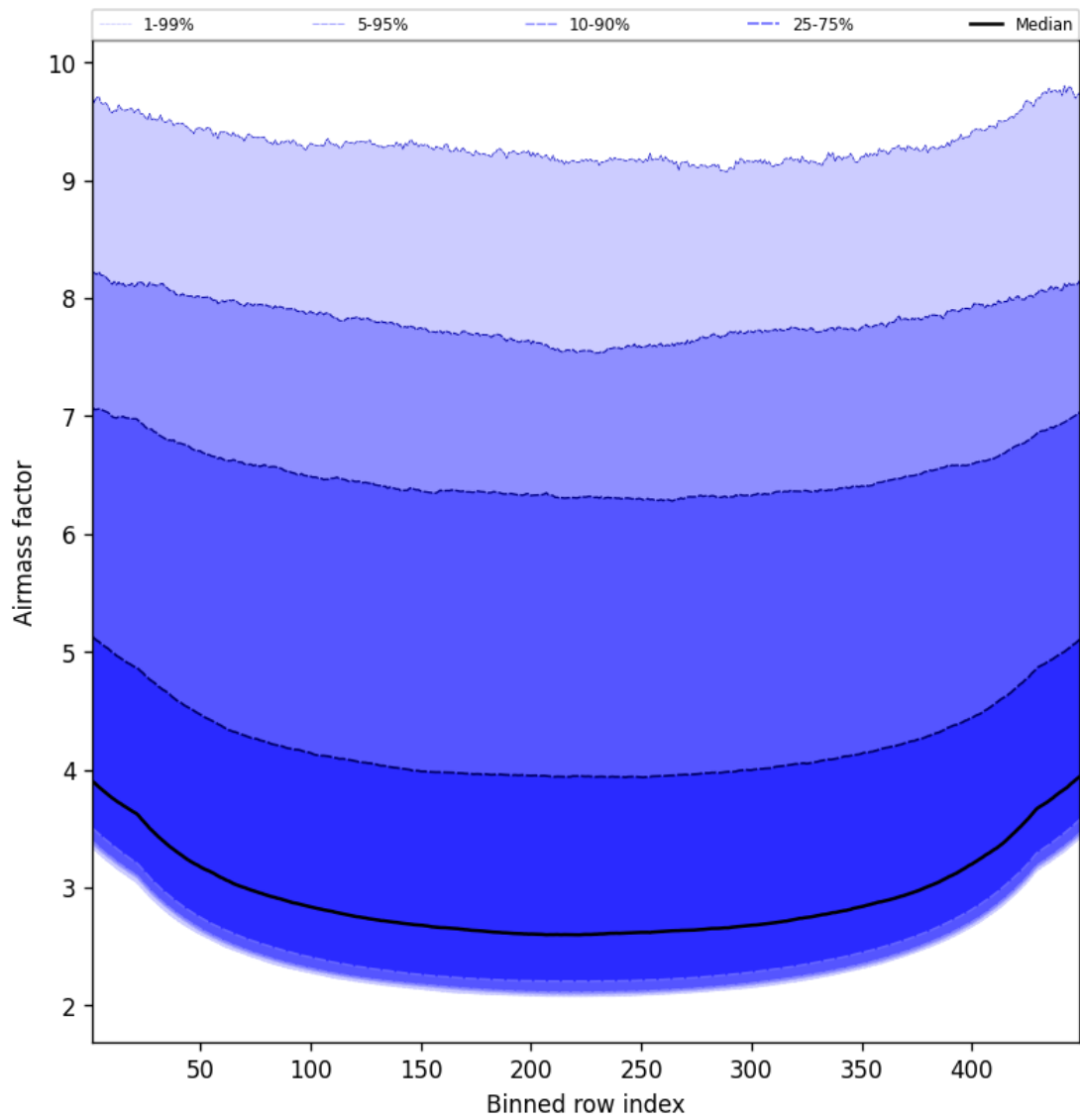
Figure 49: Along track statistics of “Airmass factor” for 2025-04-15 to 2025-04-16
