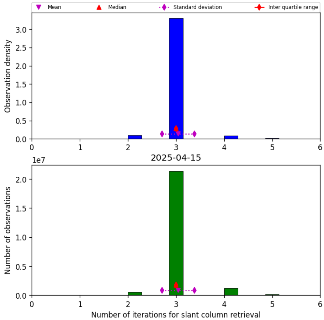
Figure 33: Histogram of “Number of iterations for slant column retrieval” for 2025-04-15 to 2025-04-16
