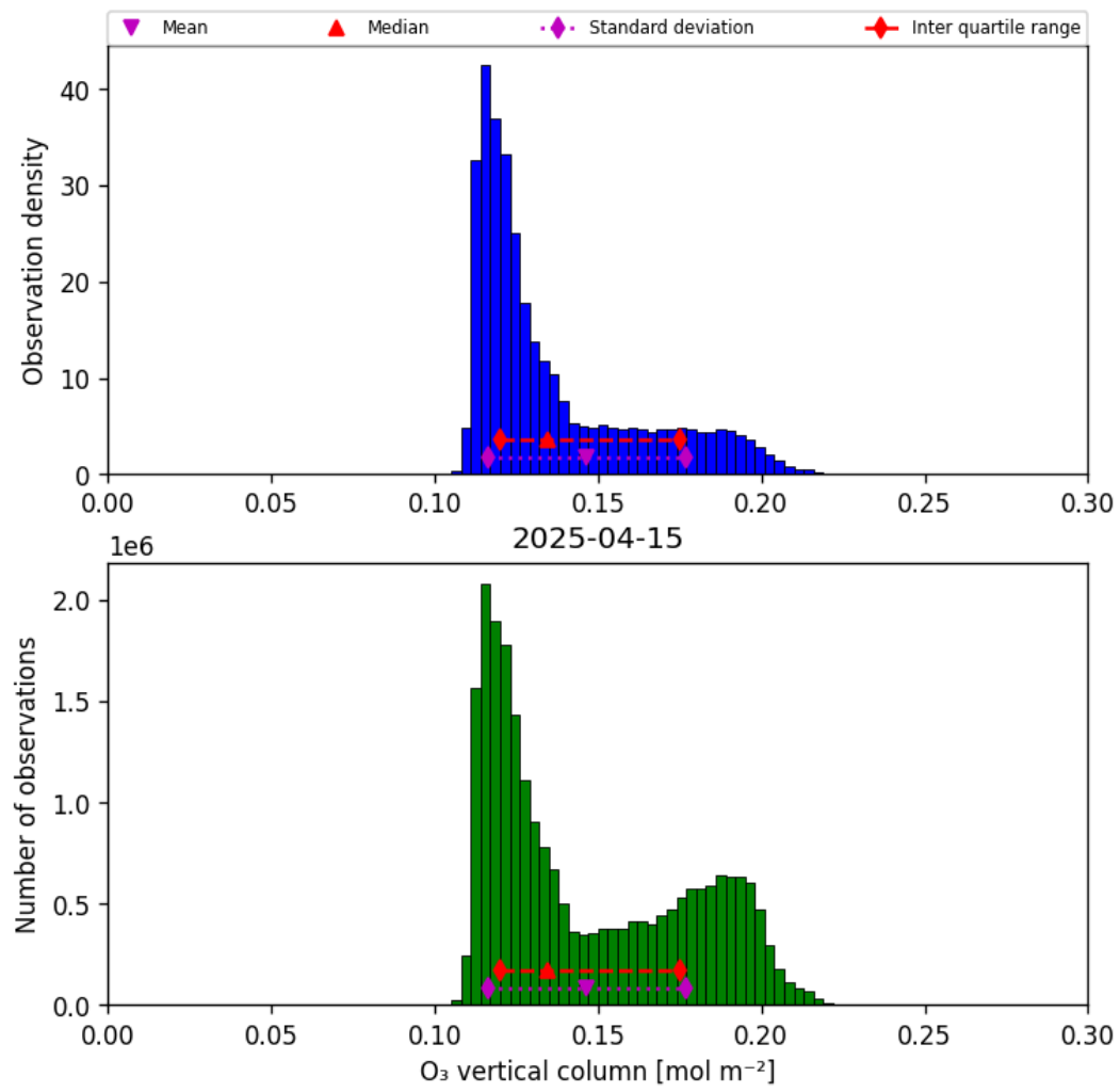
Figure 29: Histogram of “O 3 vertical column” for 2025-04-15 to 2025-04-16
