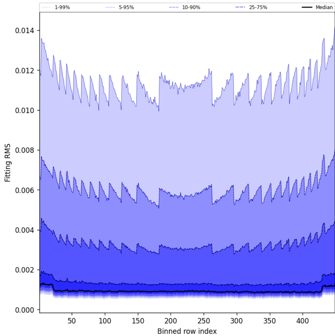
Figure 46: Along track statistics of “Fitting RMS” for 2025-04-15 to 2025-04-16
