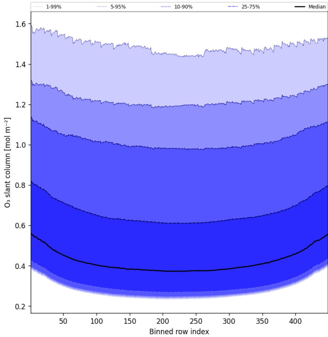
Figure 43: Along track statistics of “O 3 slant column” for 2025-04-15 to 2025-04-16
