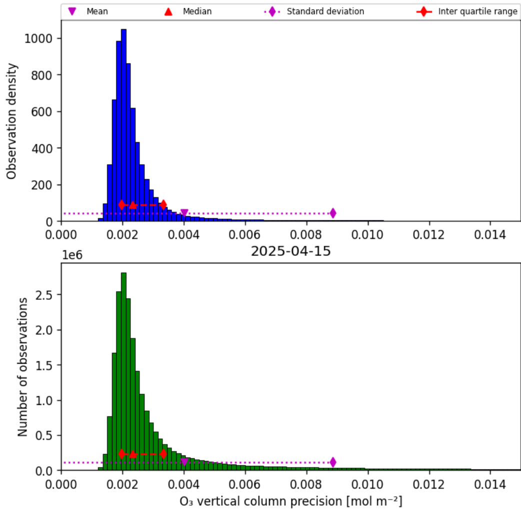
Figure 30: Histogram of “O 3 vertical column precision” for 2025-04-15 to 2025-04-16
