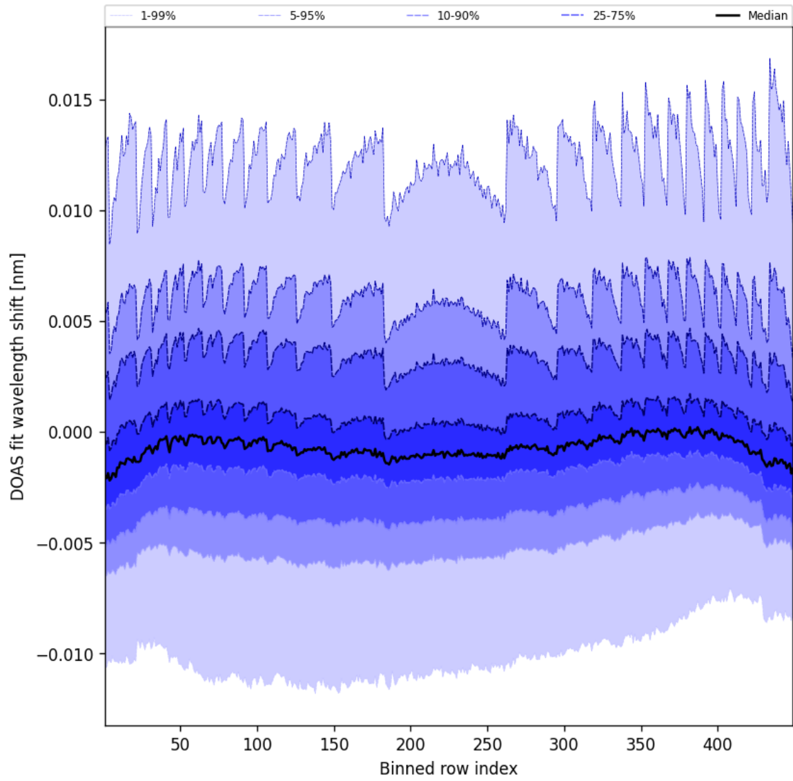
Figure 47: Along track statistics of “DOAS fit wavelength shift” for 2025-04-15 to 2025-04-16
