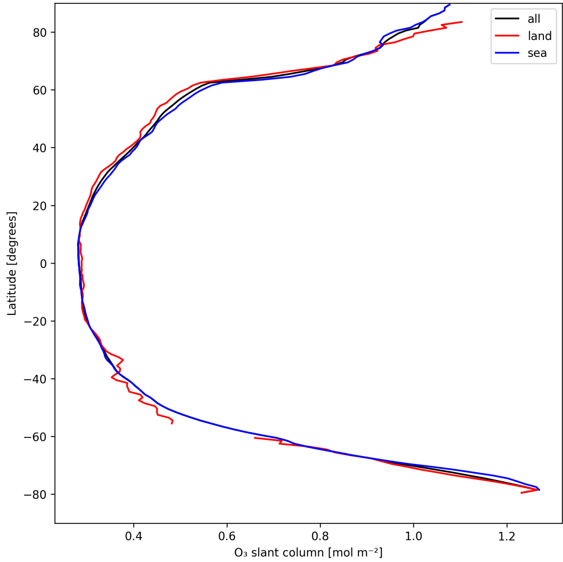
Figure 19: Zonal average of “O 3 slant column” for 2025-04-15 to 2025-04-16.
