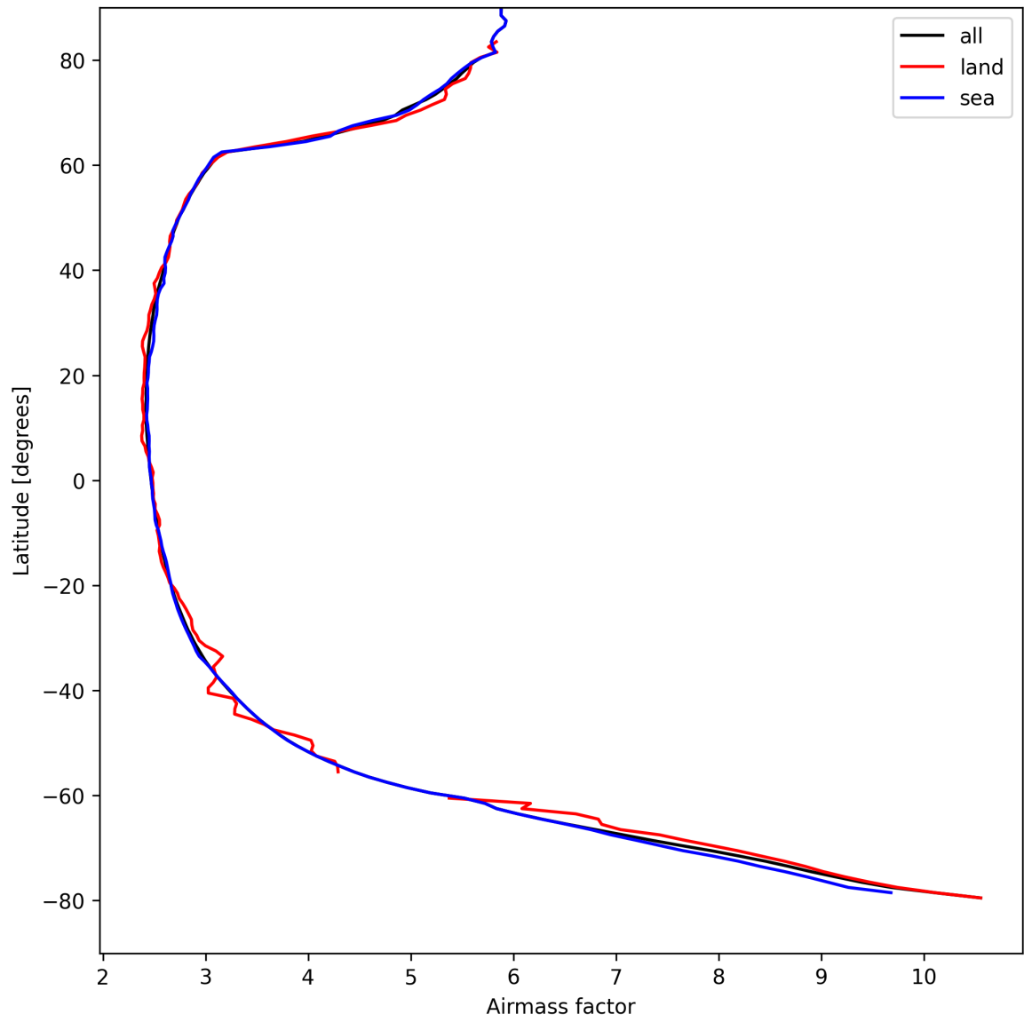
Figure 25: Zonal average of “Airmass factor” for 2025-04-15 to 2025-04-16.
