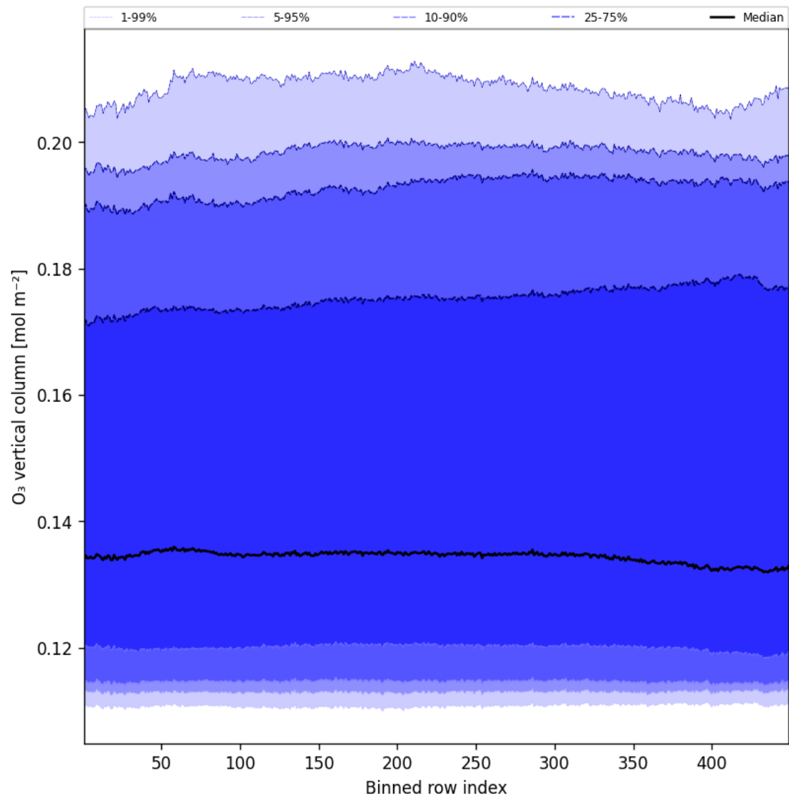
Figure 41: Along track statistics of “O 3 vertical column” for 2025-04-15 to 2025-04-16
