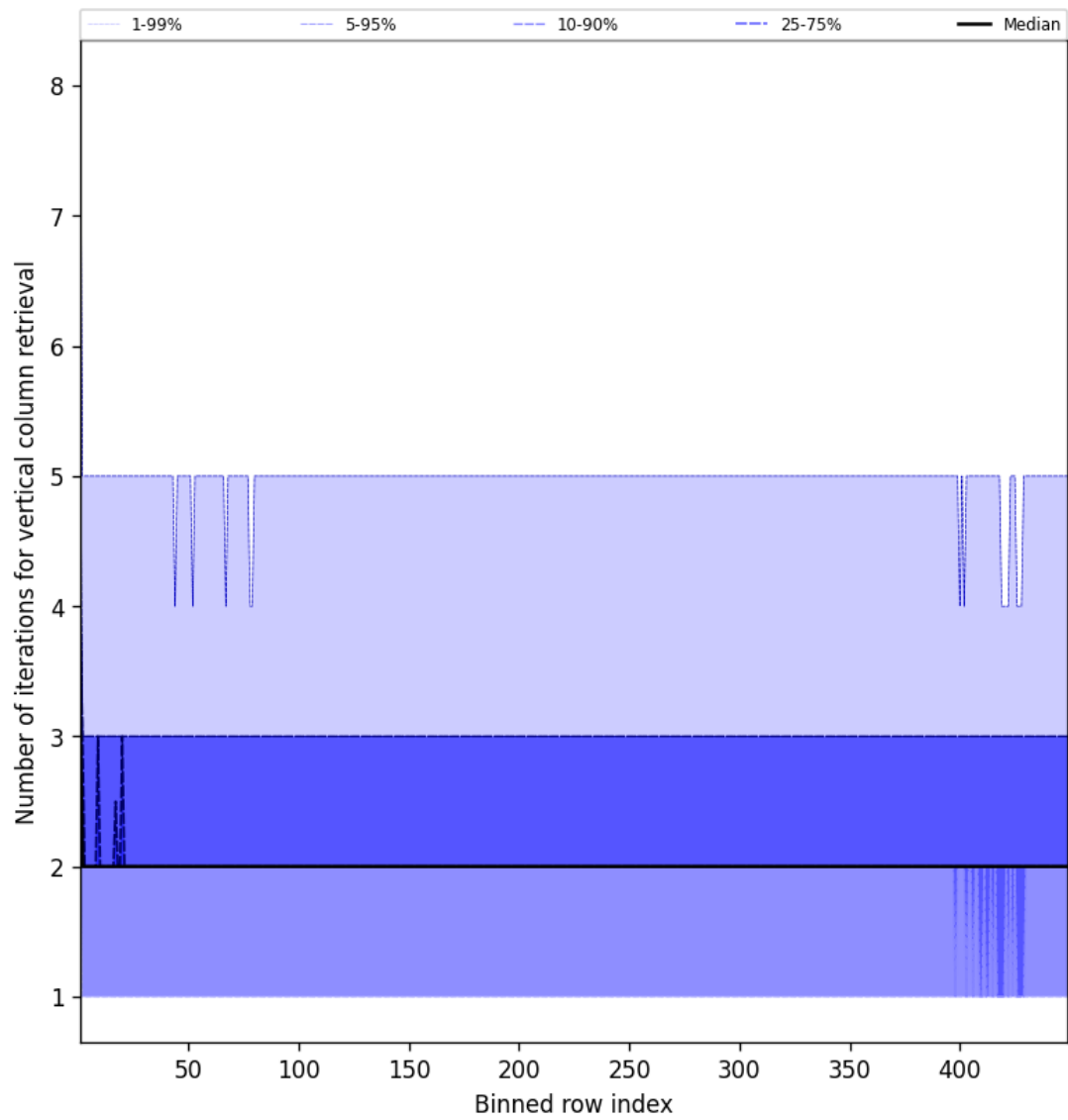
Figure 51: Along track statistics of “Number of iterations for vertical column retrieval” for 2025-04-15 to 2025-04-16
