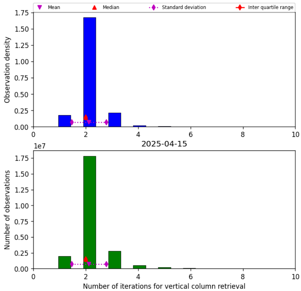
Figure 39: Histogram of “Number of iterations for vertical column retrieval” for 2025-04-15 to 2025-04-16
