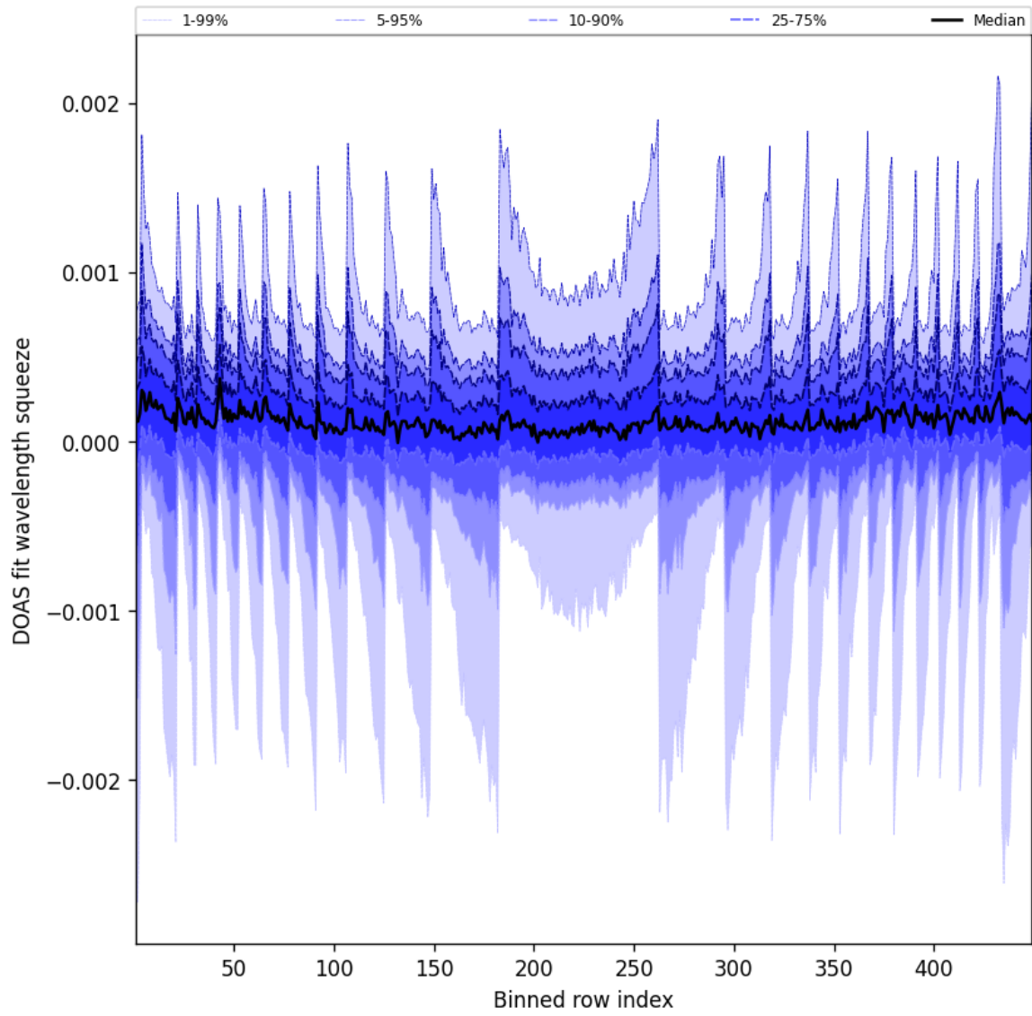
Figure 48: Along track statistics of “DOAS fit wavelength squeeze” for 2025-04-15 to 2025-04-16
