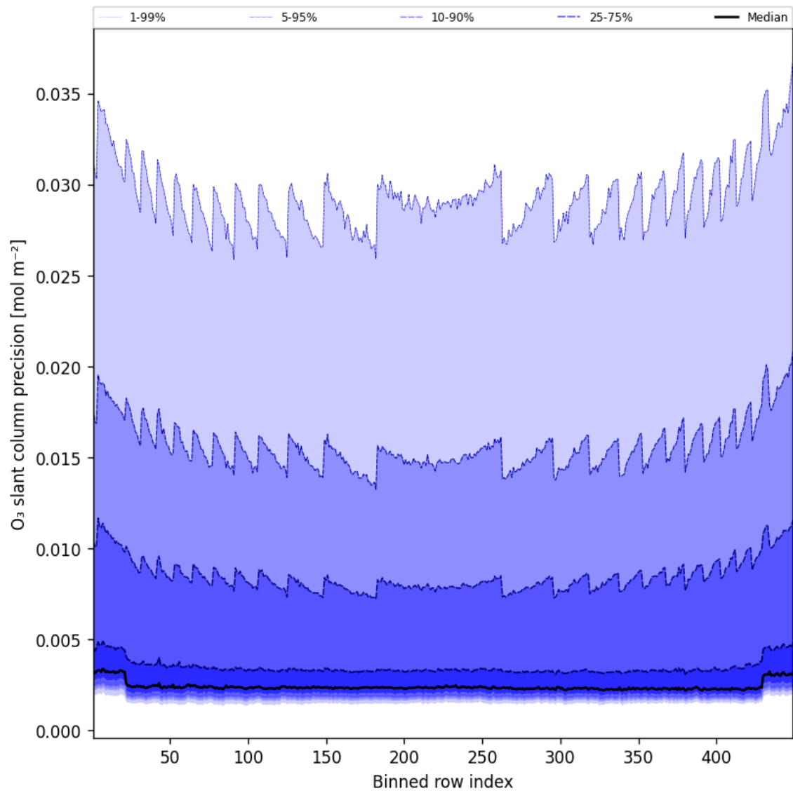
Figure 44: Along track statistics of “O 3 slant column precision” for 2025-04-15 to 2025-04-16
