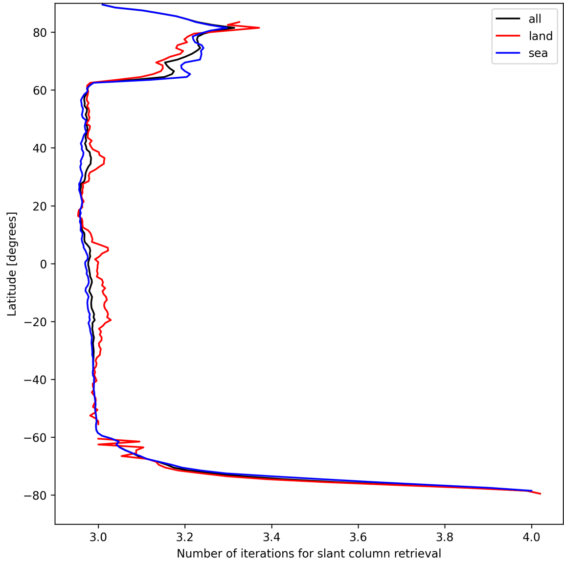
Figure 21: Zonal average of “Number of iterations for slant column retrieval” for 2025-04-15 to 2025-04-16.
