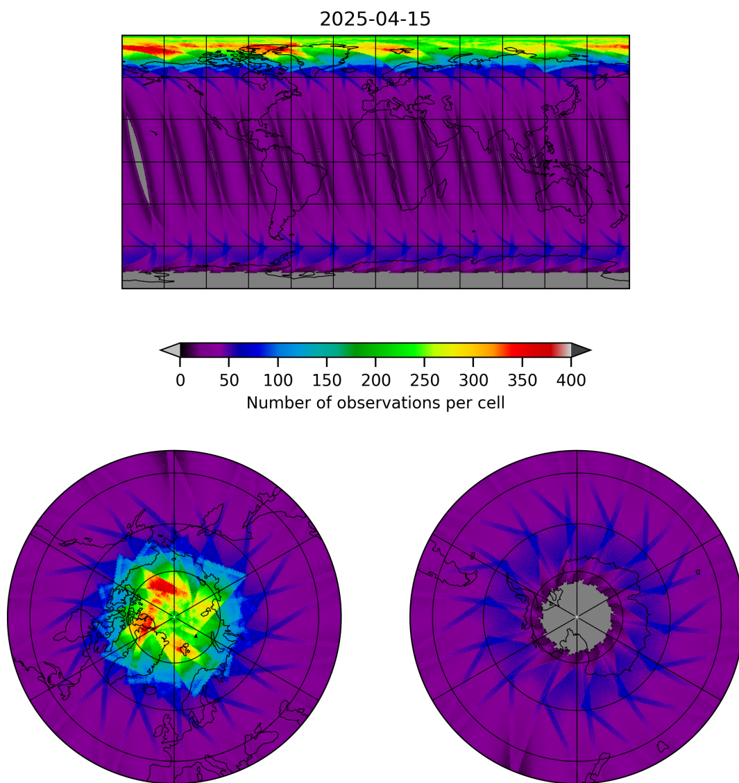
Figure 15: Map of the number of observations for 2025-04-15 to 2025-04-16
