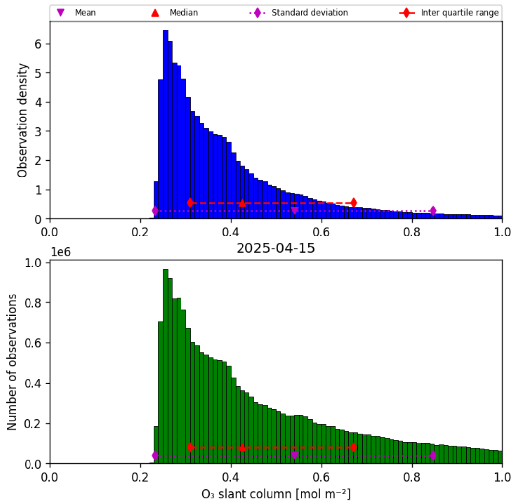
Figure 31: Histogram of “O 3 slant column” for 2025-04-15 to 2025-04-16
