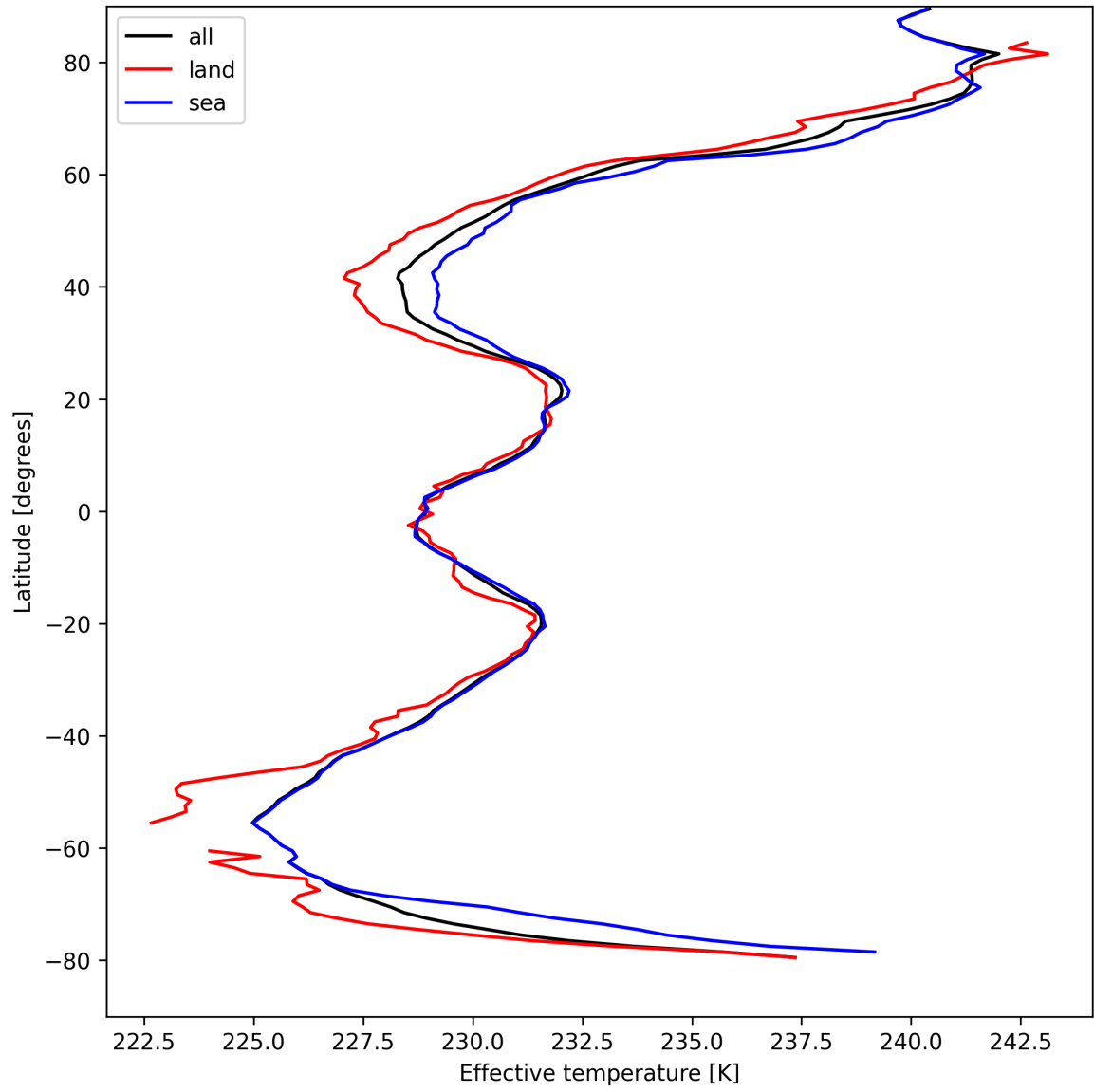
Figure 26: Zonal average of “Effective temperature” for 2025-04-15 to 2025-04-16.
