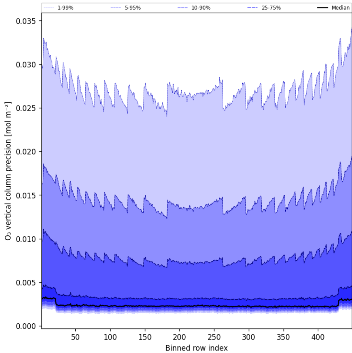
Figure 42: Along track statistics of “O 3 vertical column precision” for 2025-04-15 to 2025-04-16
