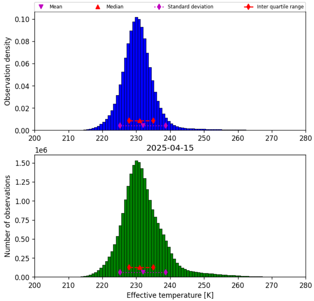
Figure 38: Histogram of “Effective temperature” for 2025-04-15 to 2025-04-16
