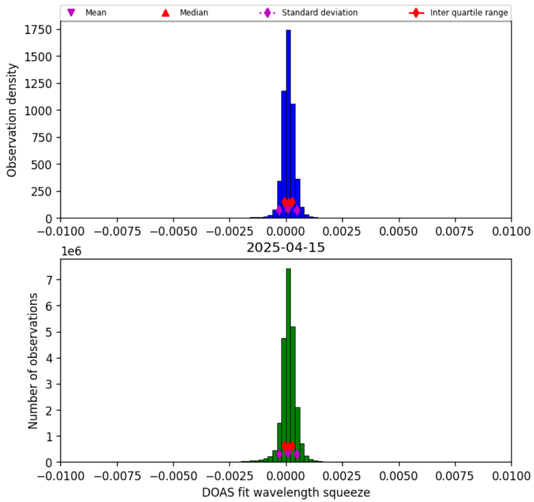
Figure 36: Histogram of “DOAS fit wavelength squeeze” for 2025-04-15 to 2025-04-16
