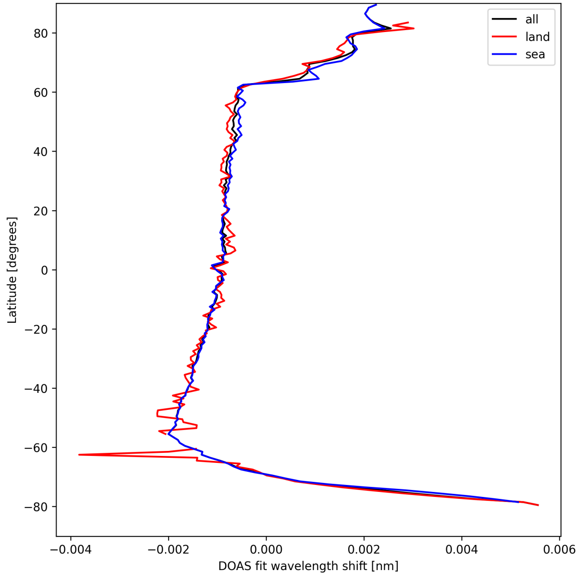
Figure 23: Zonal average of “DOAS fit wavelength shift” for 2025-04-15 to 2025-04-16.
