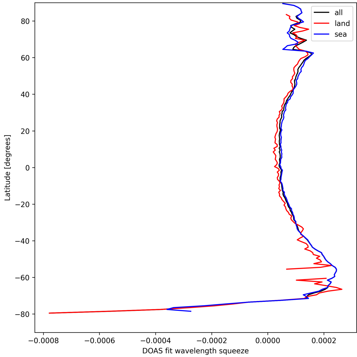
Figure 24: Zonal average of “DOAS fit wavelength squeeze” for 2025-04-15 to 2025-04-16.
