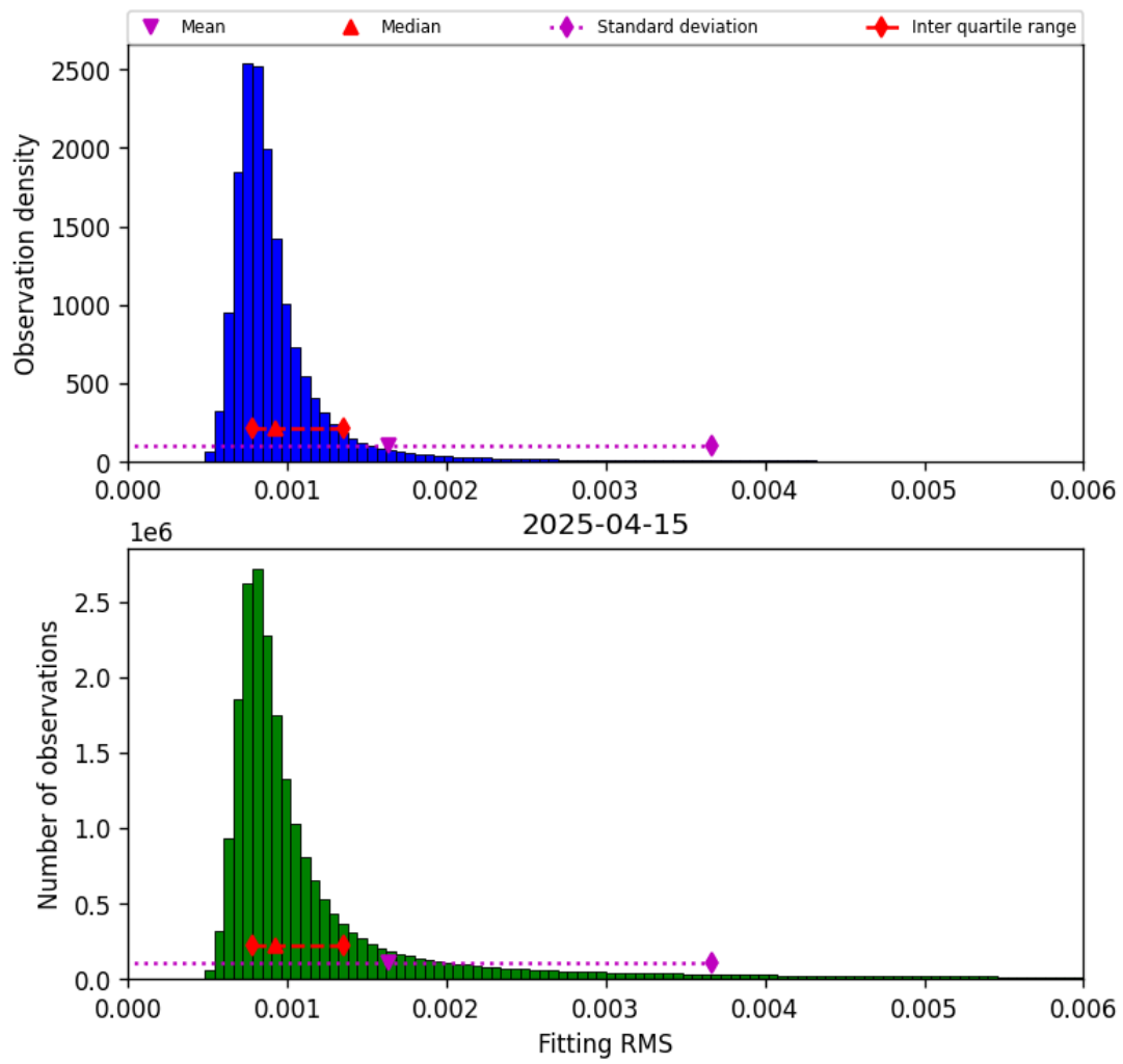
Figure 34: Histogram of “Fitting RMS” for 2025-04-15 to 2025-04-16
