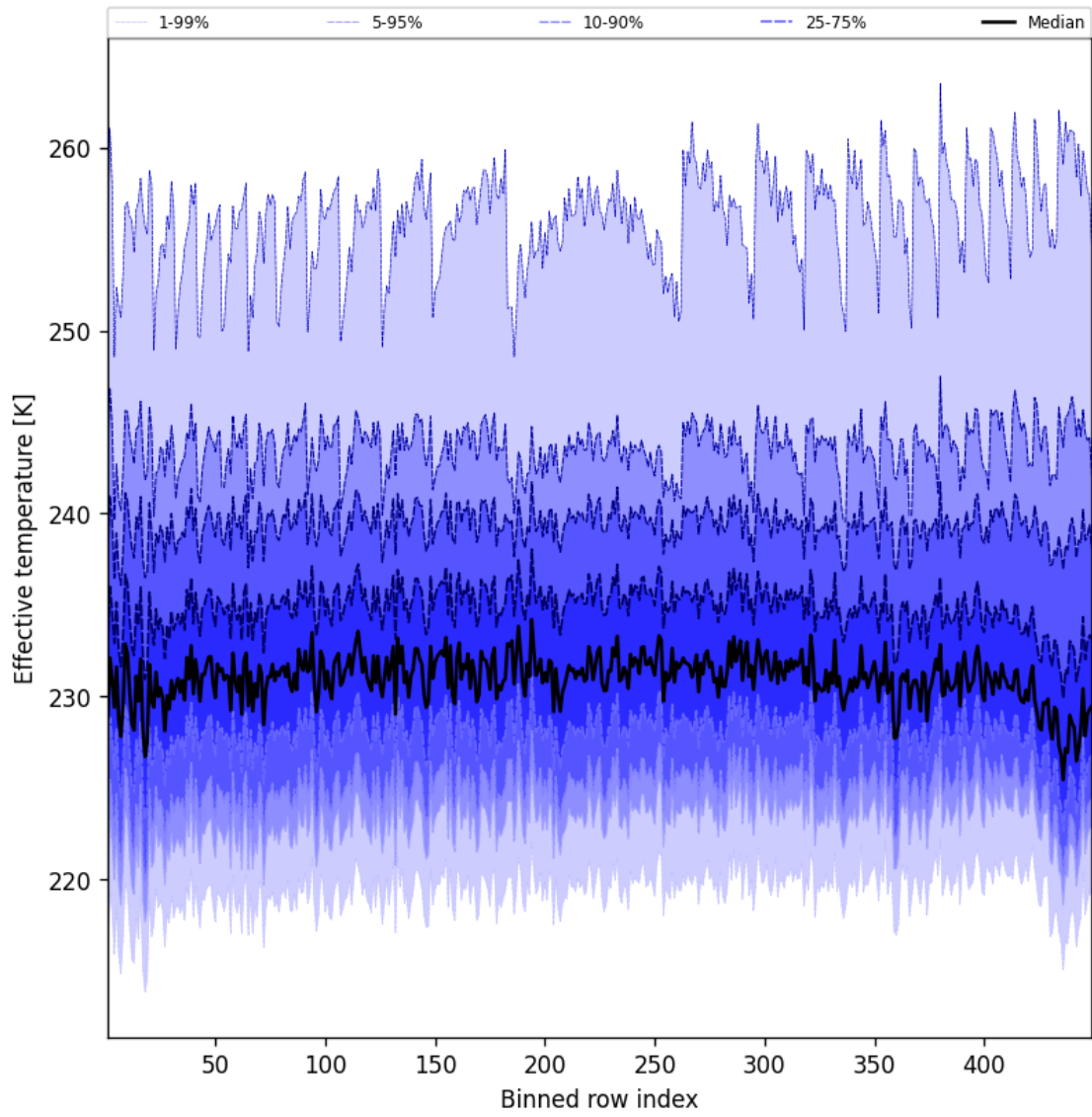
Figure 50: Along track statistics of “Effective temperature” for 2025-04-15 to 2025-04-16
