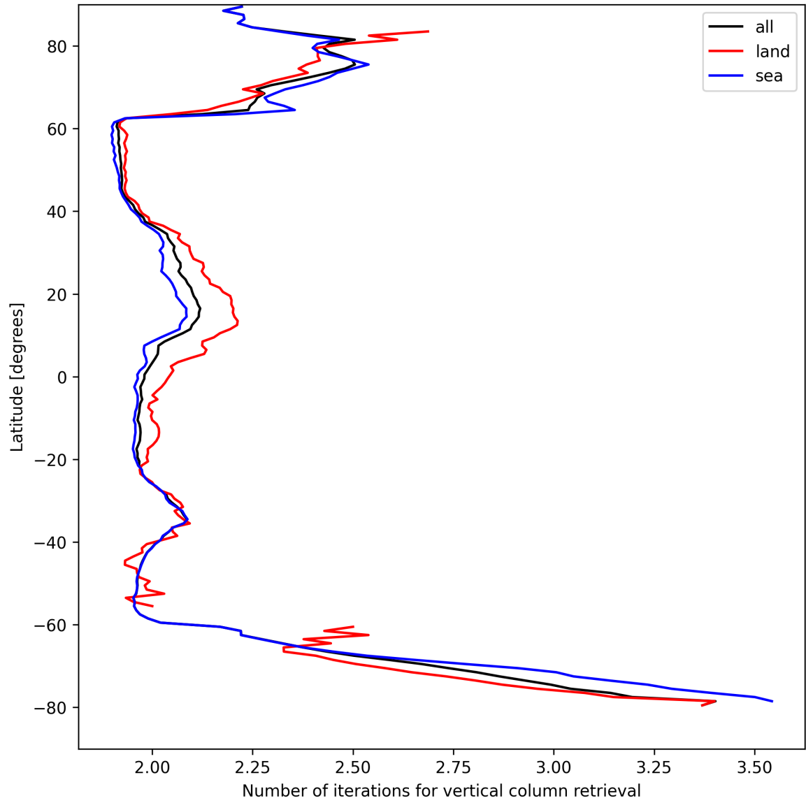
Figure 27: Zonal average of “Number of iterations for vertical column retrieval” for 2025-04-15 to 2025-04-16.
