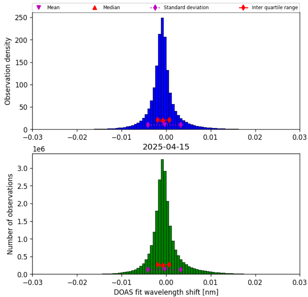
Figure 35: Histogram of “DOAS fit wavelength shift” for 2025-04-15 to 2025-04-16
