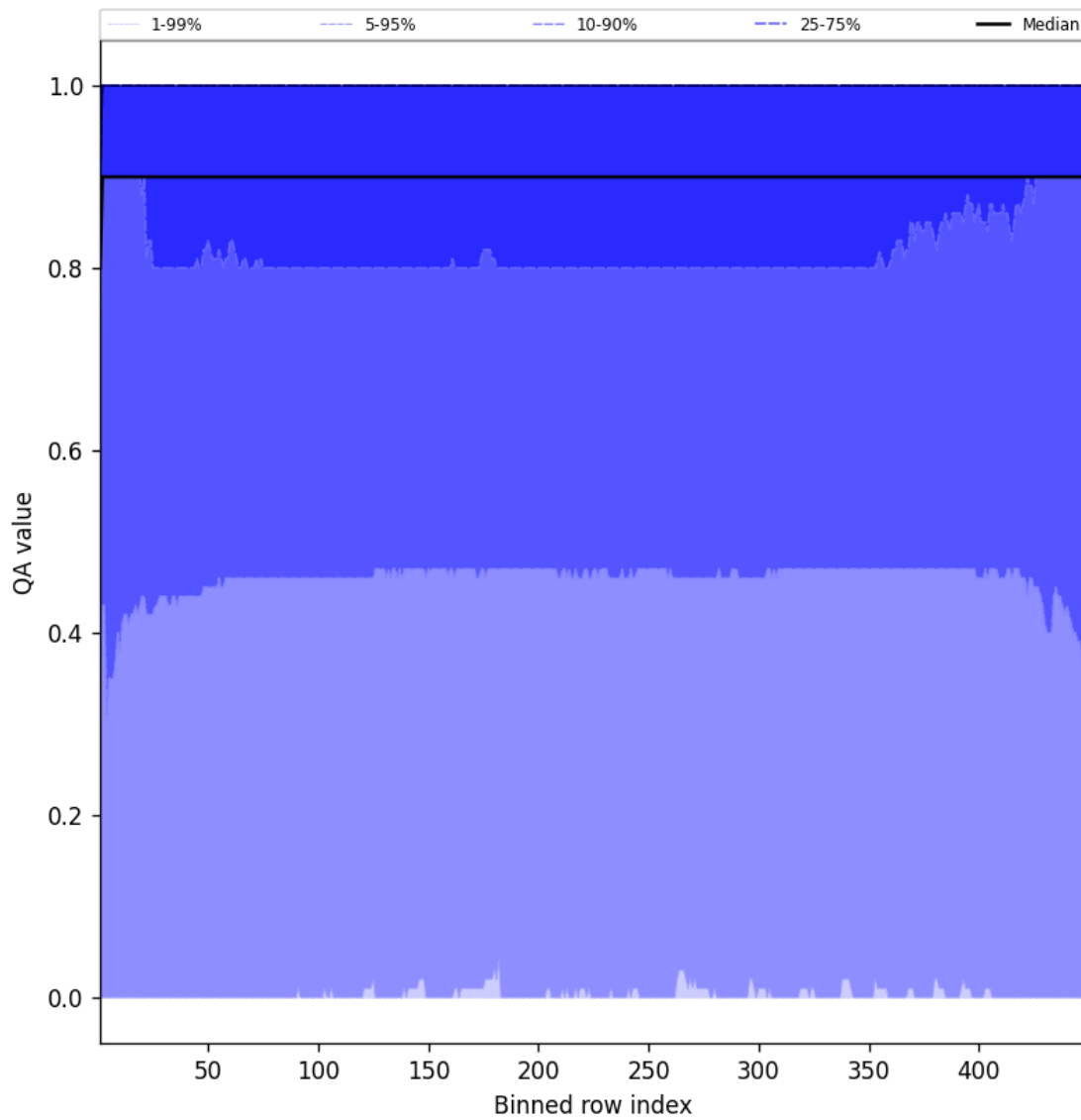
Figure 40: Along track statistics of “QA value” for 2025-04-15 to 2025-04-16
