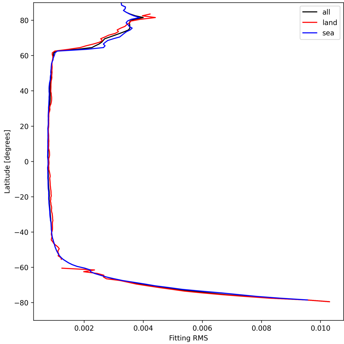
Figure 22: Zonal average of “Fitting RMS” for 2025-04-15 to 2025-04-16.
