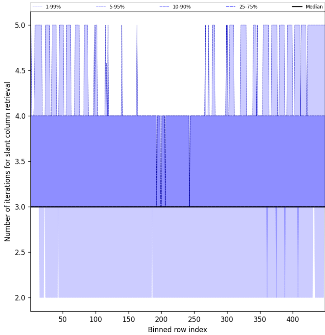
Figure 45: Along track statistics of “Number of iterations for slant column retrieval” for 2025-04-15 to 2025-04-16
