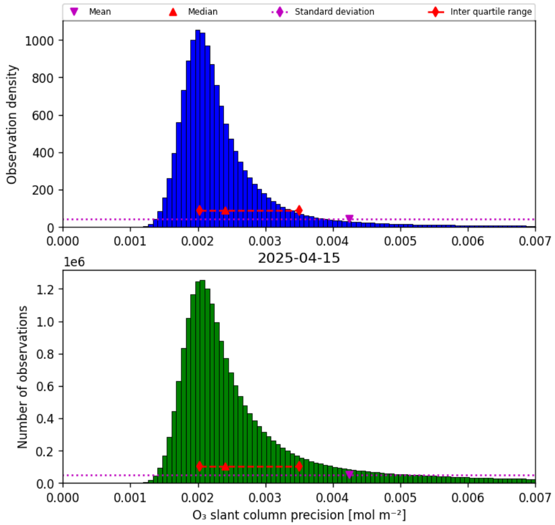
Figure 32: Histogram of "O 3 slant column precision" for 2025-04-15 to 2025-04-16
