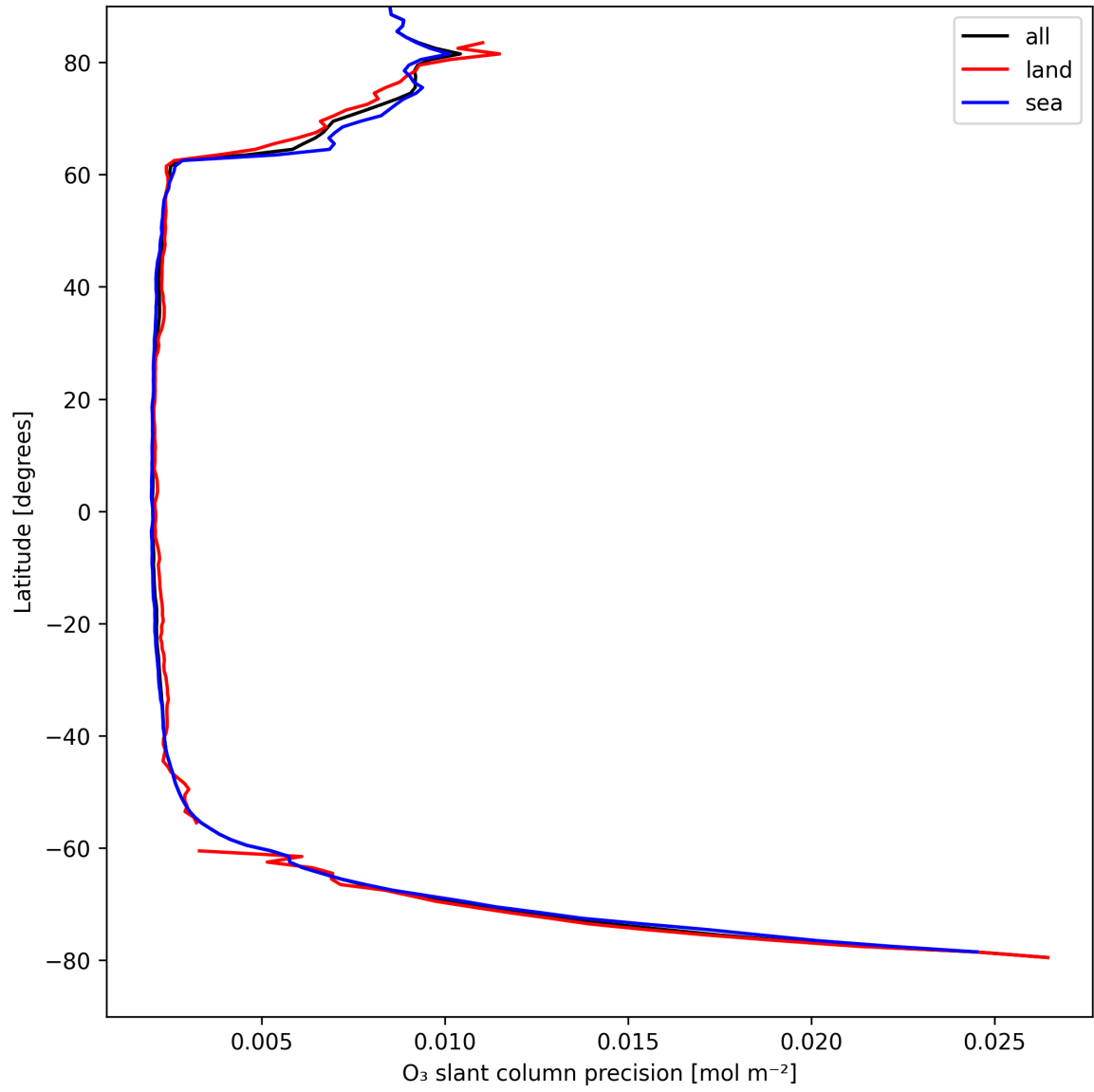
Figure 20: Zonal average of "O 3 slant column precision" for 2025-04-15 to 2025-04-16.
