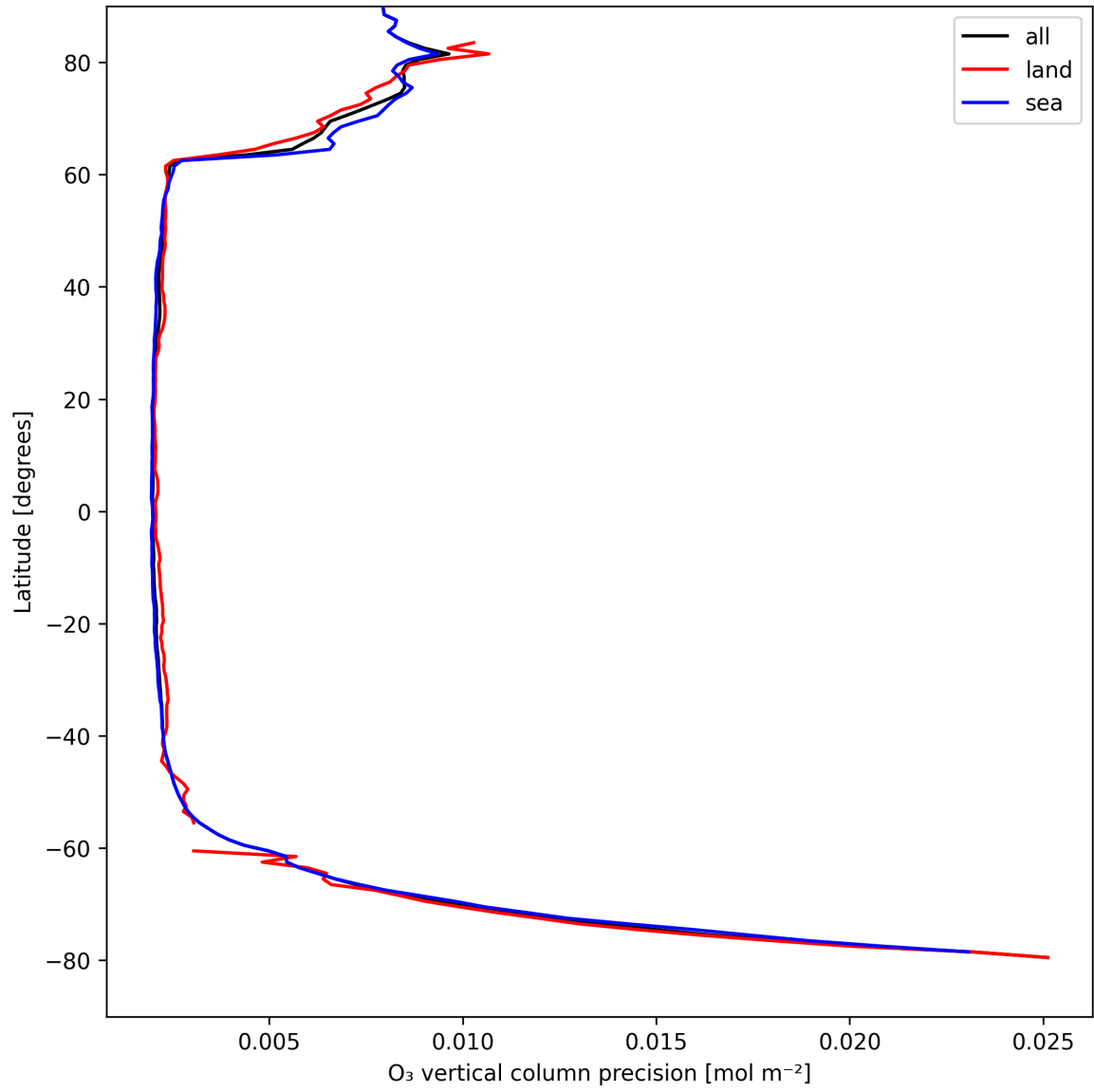
Figure 18: Zonal average of "O 3 vertical column precision" for 2025-04-15 to 2025-04-16.
