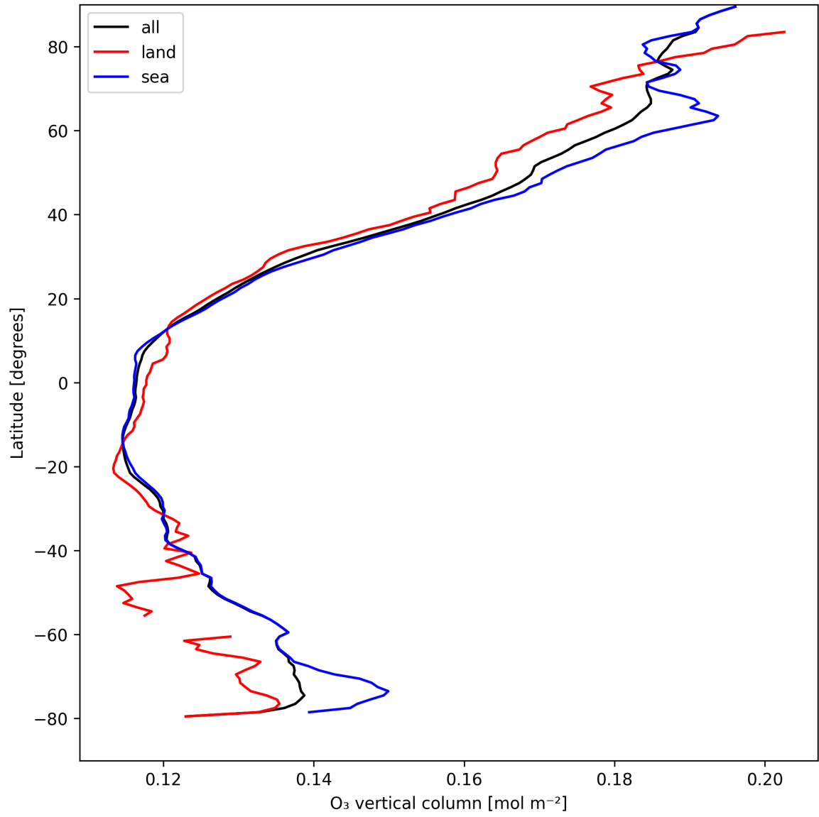
Figure 17: Zonal average of “O 3 vertical column” for 2025-04-15 to 2025-04-16.
