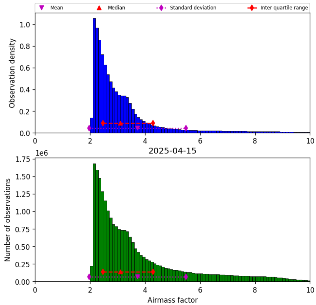
Figure 37: Histogram of “Airmass factor” for 2025-04-15 to 2025-04-16
