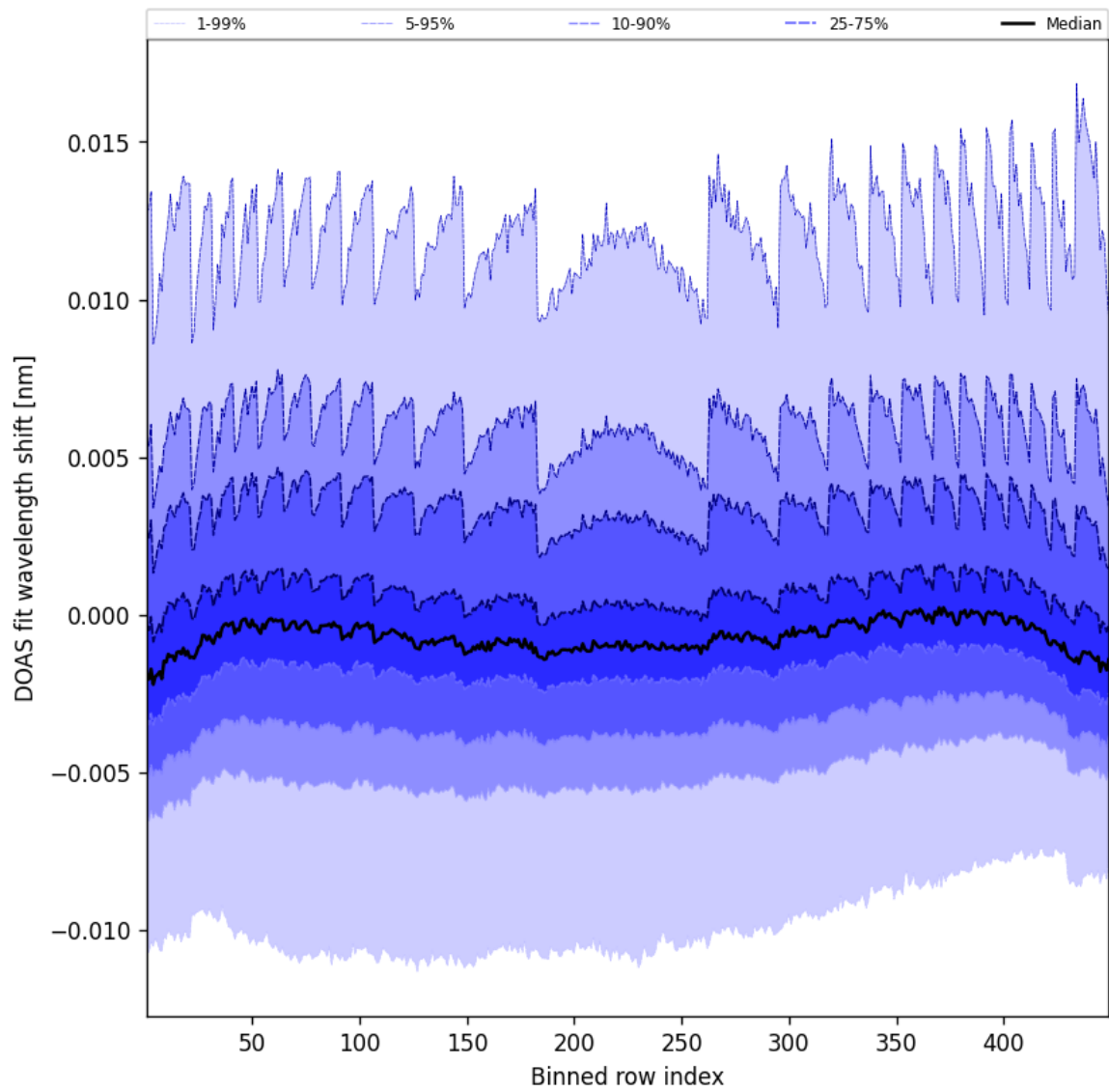
Figure 47: Along track statistics of "DOAS fit wavelength shift" for 2025-04-16 to 2025-04-16
