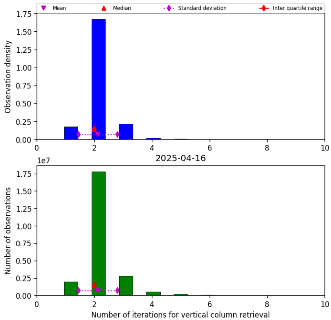
Figure 39: Histogram of “Number of iterations for vertical column retrieval” for 2025-04-16 to 2025-04-16
