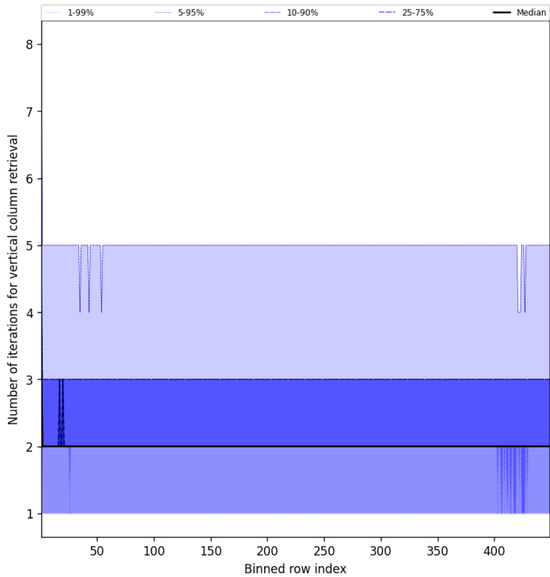
Figure 51: Along track statistics of “Number of iterations for vertical column retrieval” for 2025-04-16 to 2025-04-16
