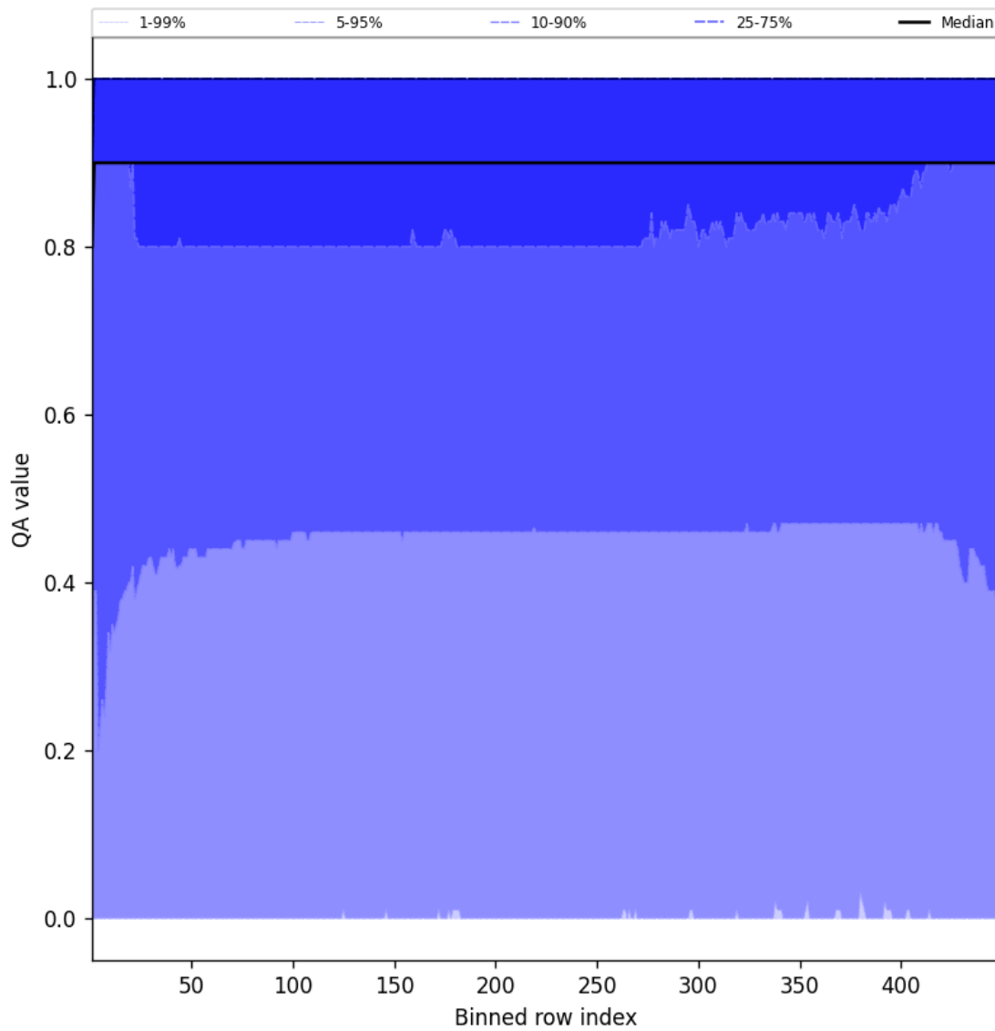
Figure 40: Along track statistics of “QA value” for 2025-04-16 to 2025-04-16
