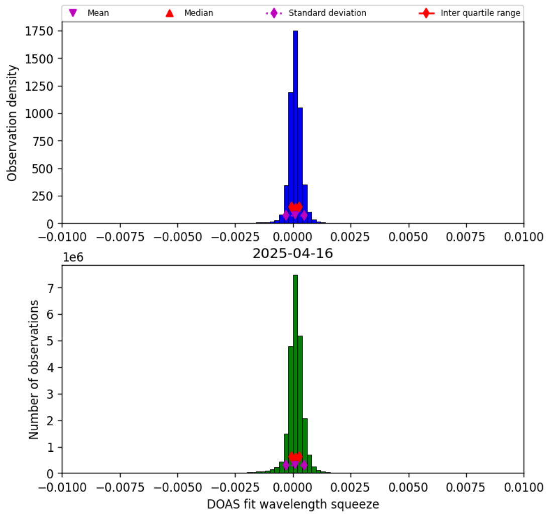
Figure 36: Histogram of “DOAS fit wavelength squeeze” for 2025-04-16 to 2025-04-16
