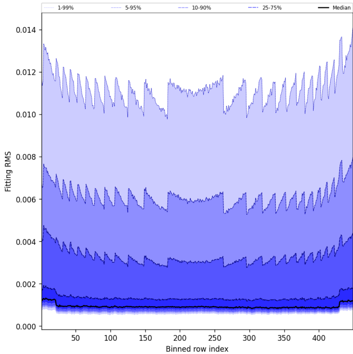
Figure 46: Along track statistics of “Fitting RMS” for 2025-04-16 to 2025-04-16
