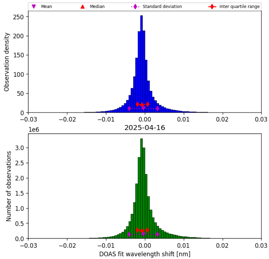
Figure 35: Histogram of “DOAS fit wavelength shift” for 2025-04-16 to 2025-04-16
