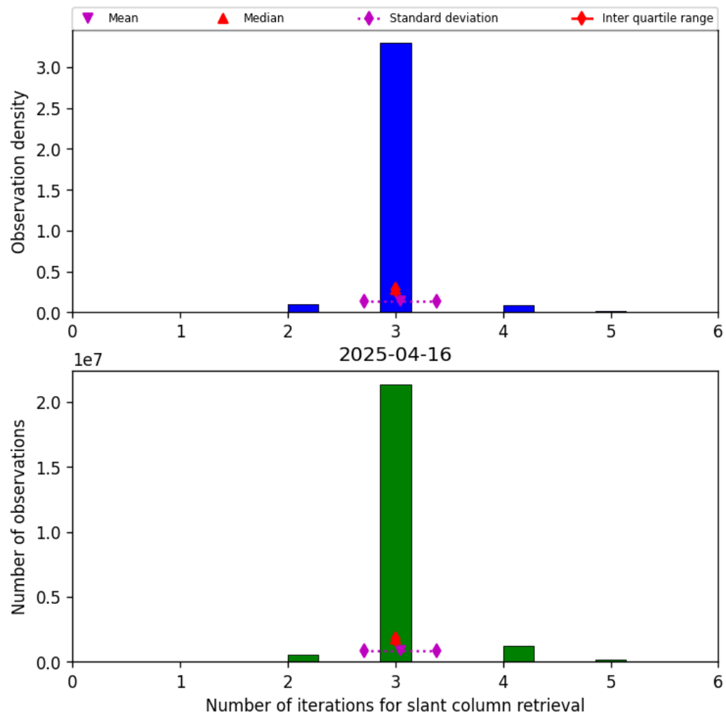
Figure 33: Histogram of “Number of iterations for slant column retrieval” for 2025-04-16 to 2025-04-16
