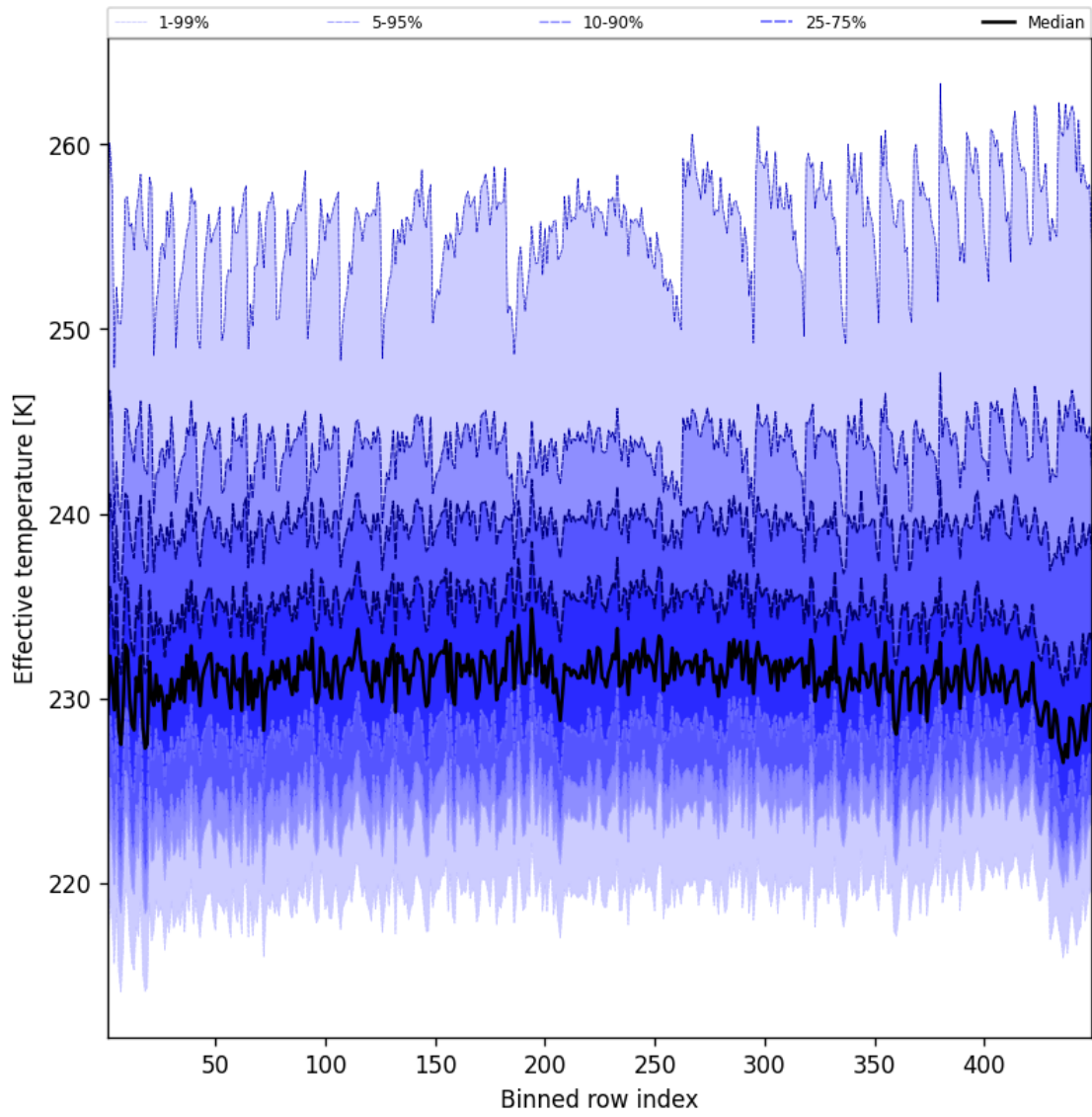
Figure 50: Along track statistics of “Effective temperature” for 2025-04-16 to 2025-04-16
