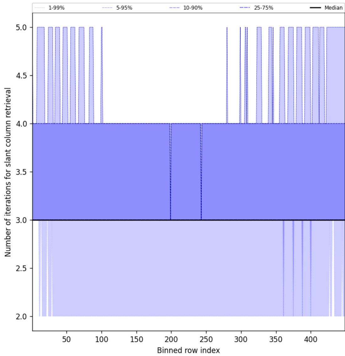
Figure 45: Along track statistics of “Number of iterations for slant column retrieval” for 2025-04-16 to 2025-04-16
