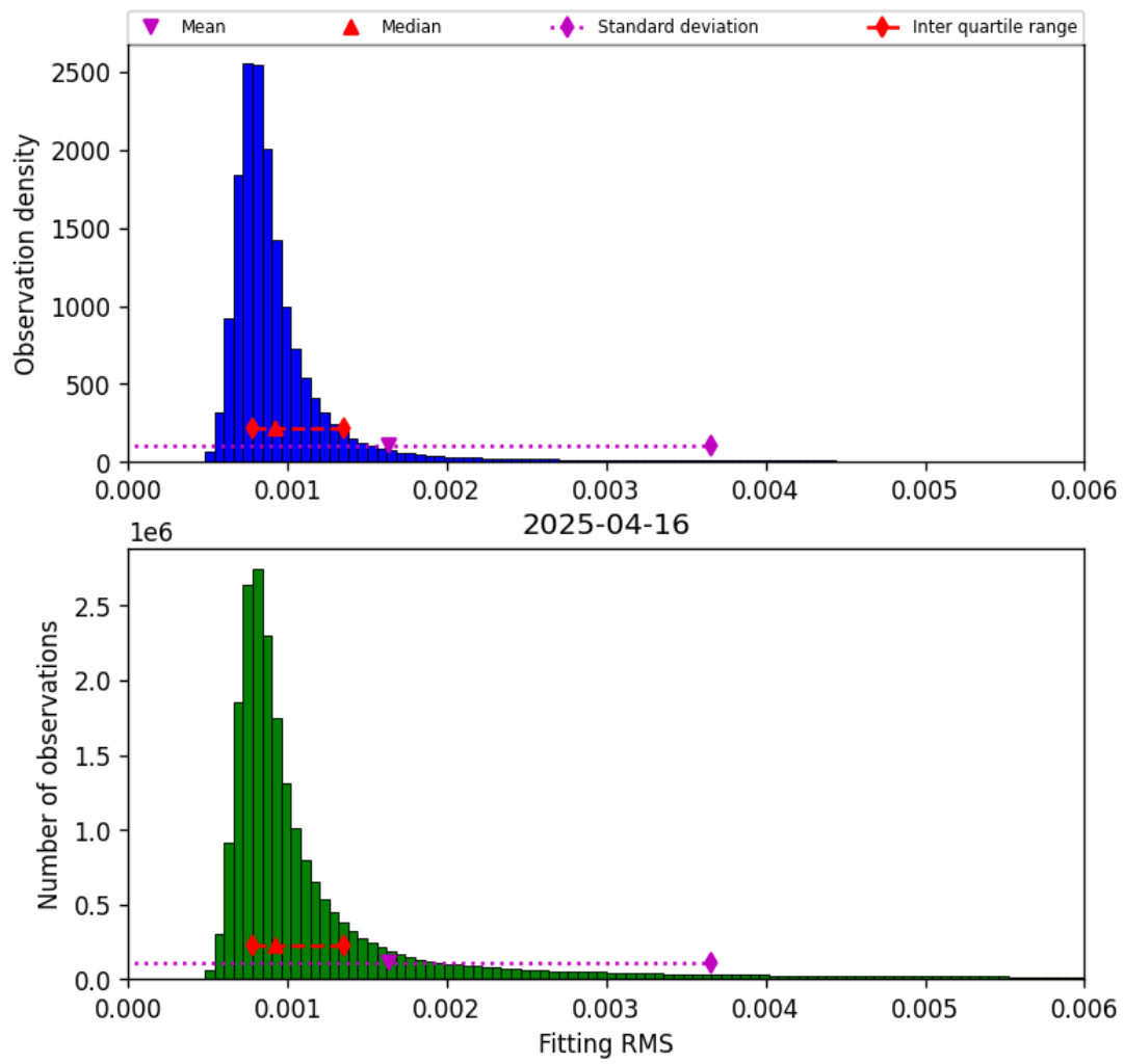
Figure 34: Histogram of “Fitting RMS” for 2025-04-16 to 2025-04-16
