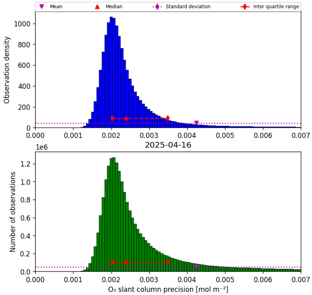
Figure 32: Histogram of “O 3 slant column precision” for 2025-04-16 to 2025-04-16
