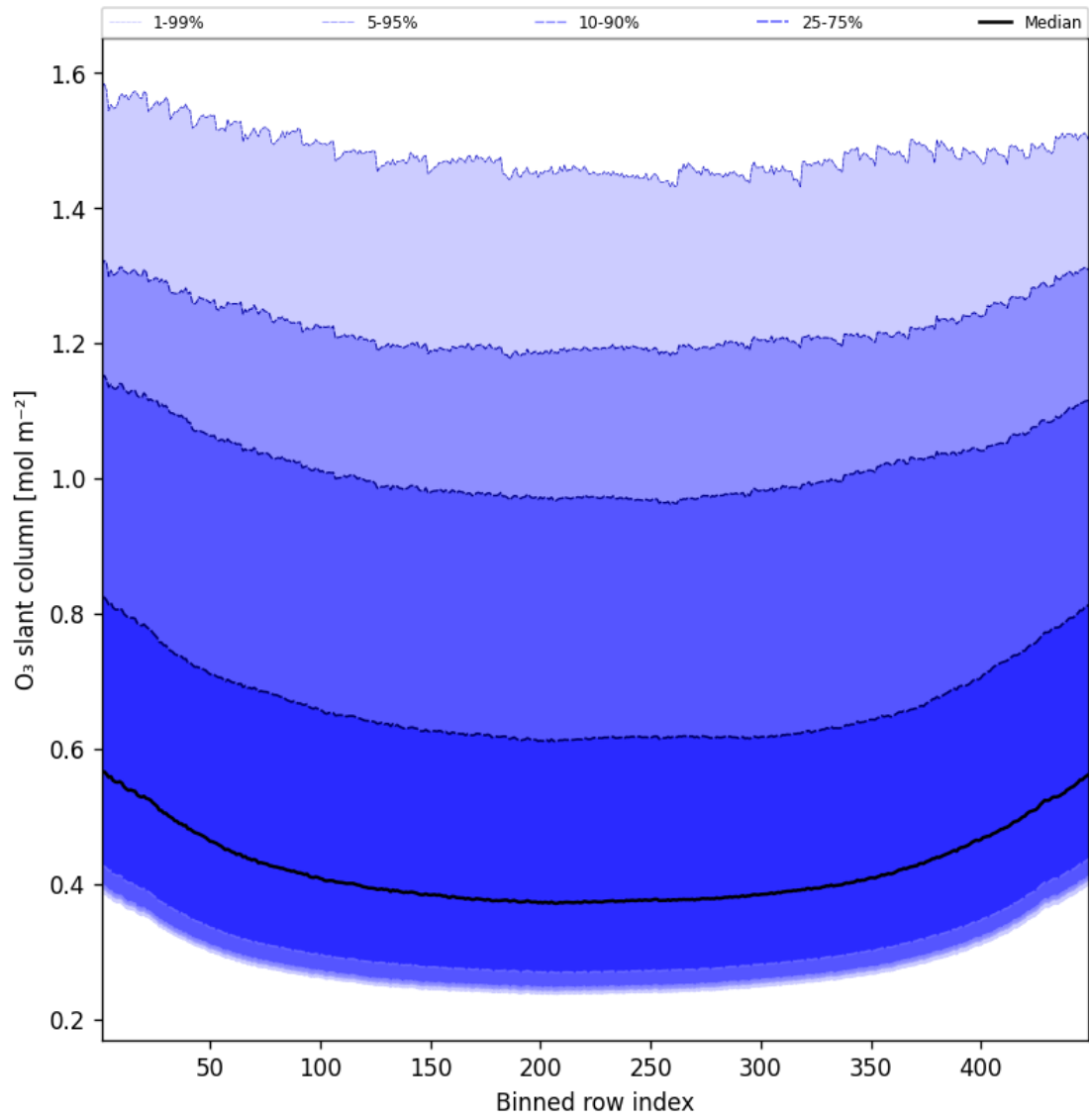
Figure 43: Along track statistics of “O 3 slant column” for 2025-04-17 to 2025-04-18
