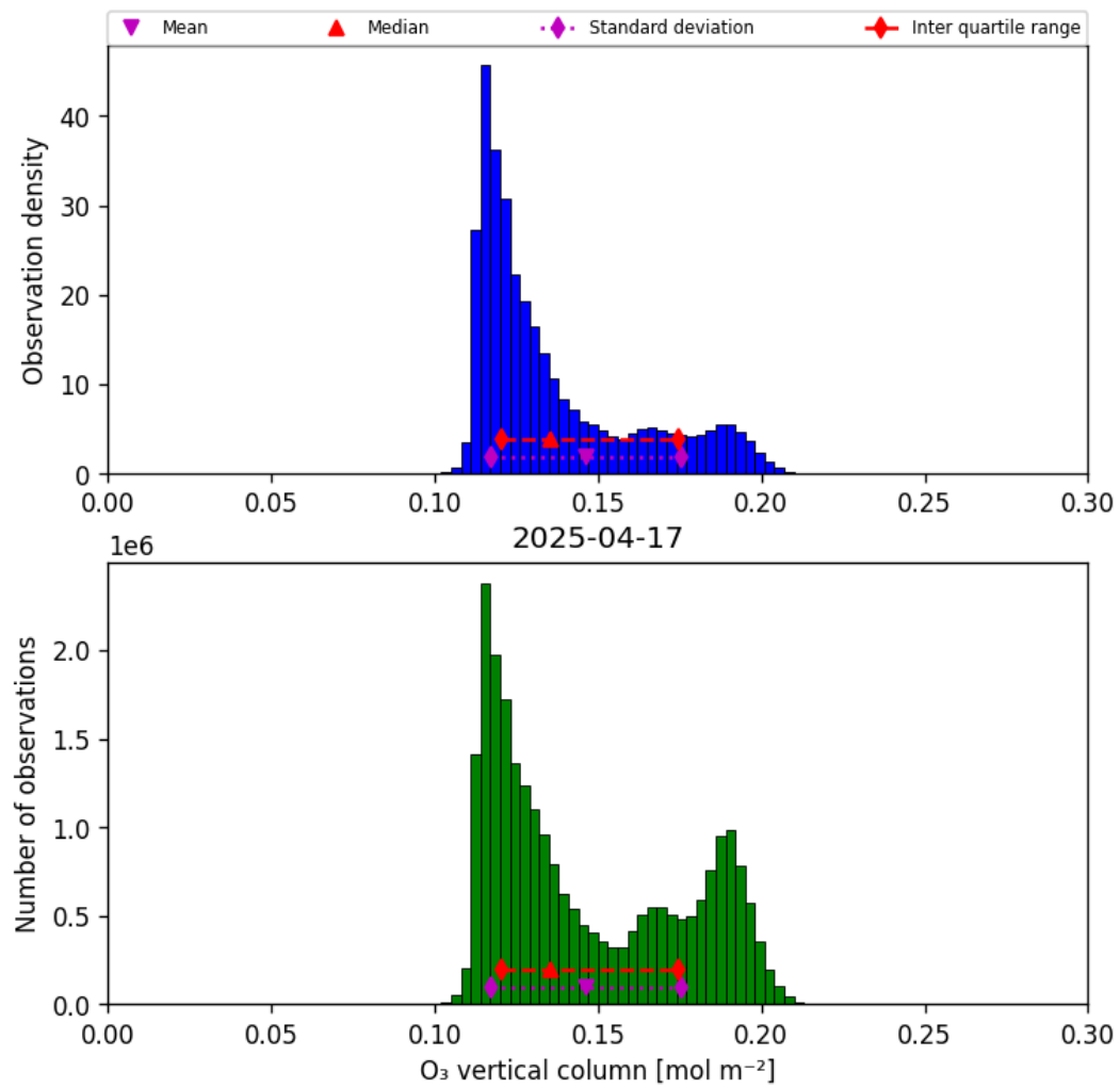
Figure 29: Histogram of “O 3 vertical column” for 2025-04-17 to 2025-04-18
