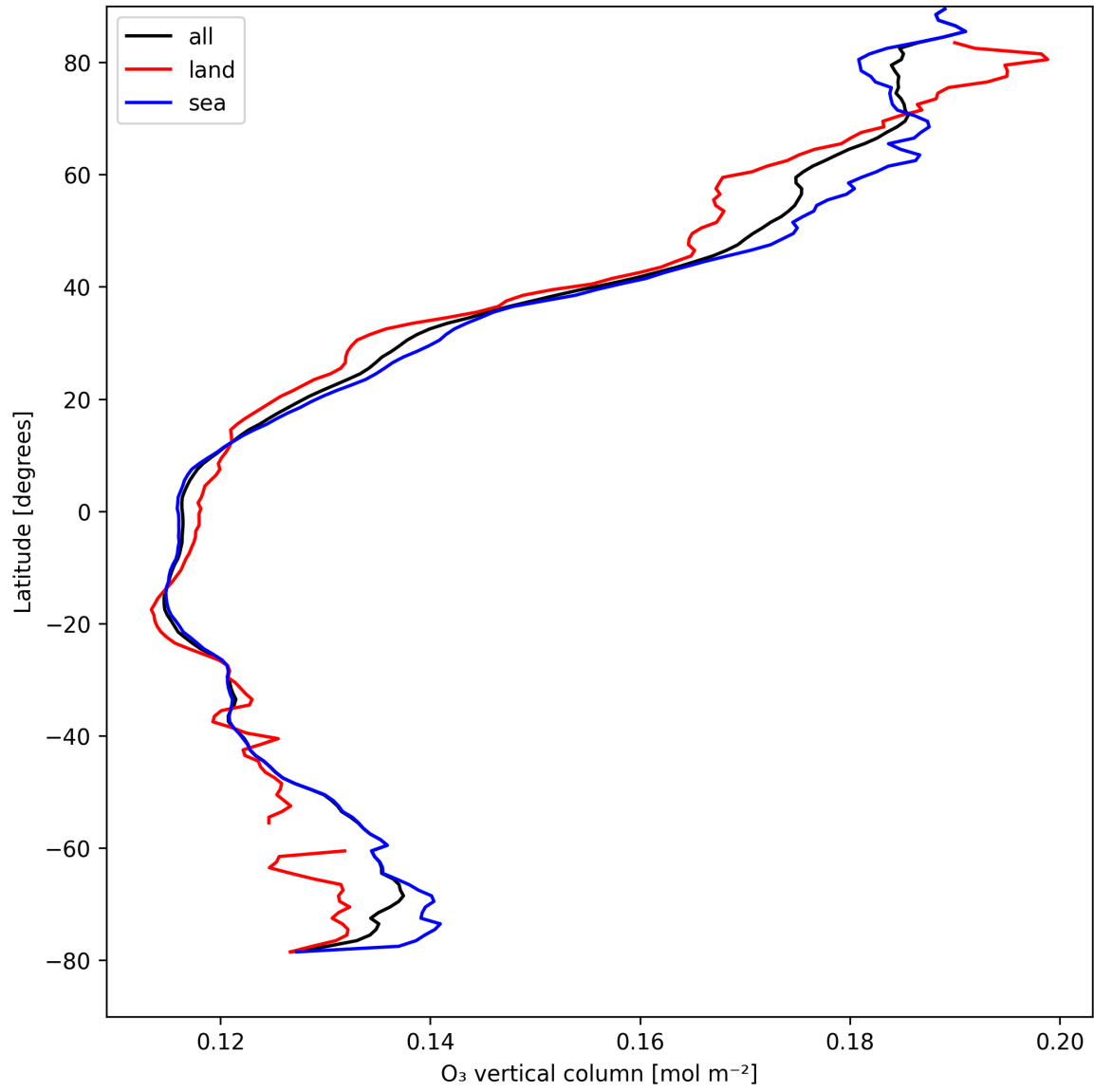
Figure 17: Zonal average of “O 3 vertical column” for 2025-04-17 to 2025-04-18.
