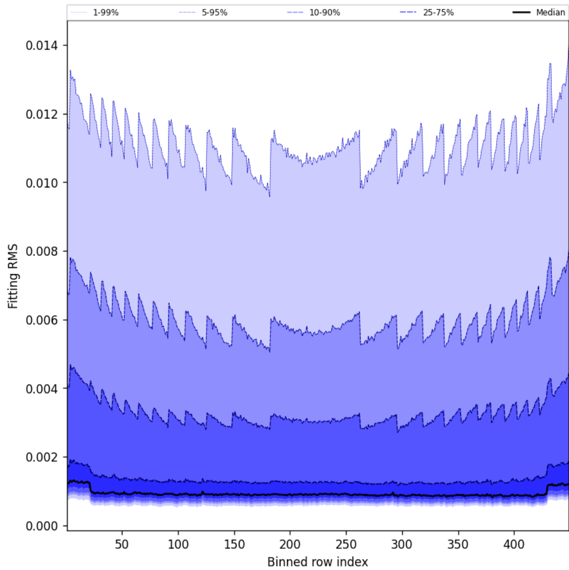
Figure 46: Along track statistics of “Fitting RMS” for 2025-04-17 to 2025-04-18
