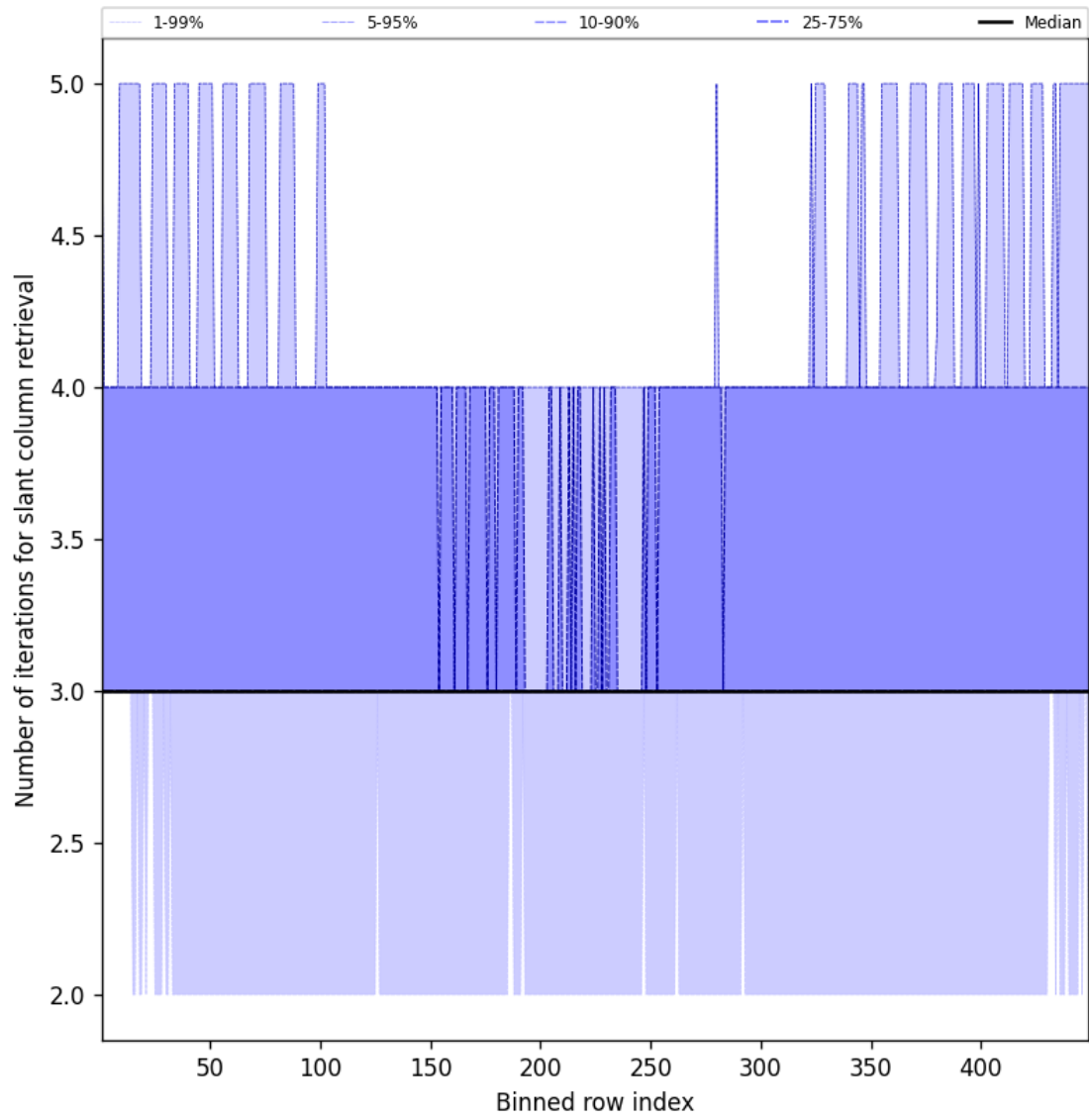
Figure 45: Along track statistics of “Number of iterations for slant column retrieval” for 2025-04-17 to 2025-04-18
