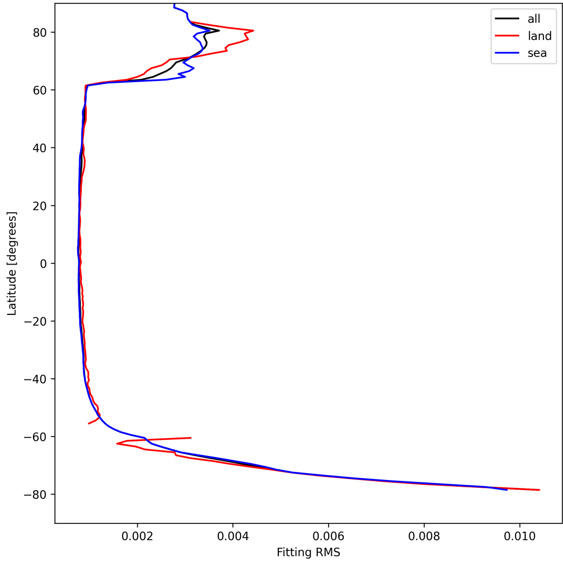
Figure 22: Zonal average of “Fitting RMS” for 2025-04-17 to 2025-04-18.
