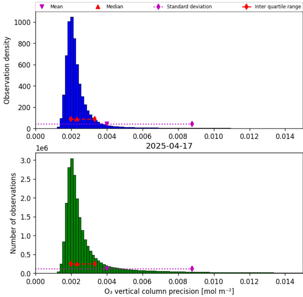
Figure 30: Histogram of “O 3 vertical column precision” for 2025-04-17 to 2025-04-18
