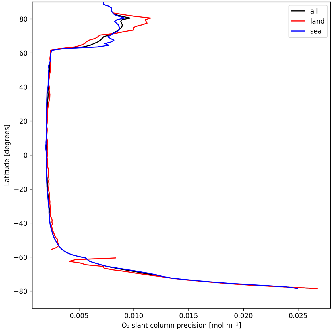
Figure 20: Zonal average of “O 3 slant column precision” for 2025-04-17 to 2025-04-18.
