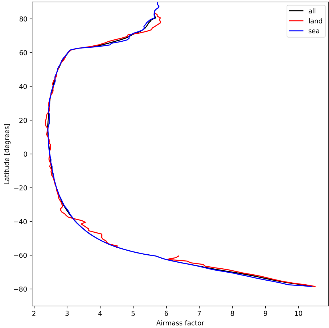
Figure 25: Zonal average of “Airmass factor” for 2025-04-17 to 2025-04-18.
