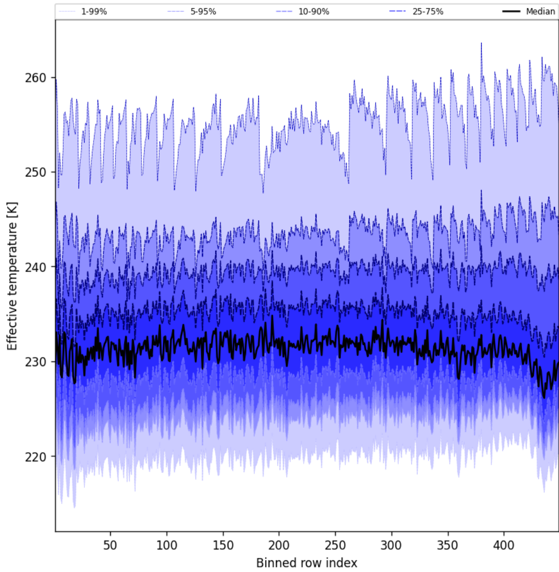
Figure 50: Along track statistics of “Effective temperature” for 2025-04-17 to 2025-04-18
