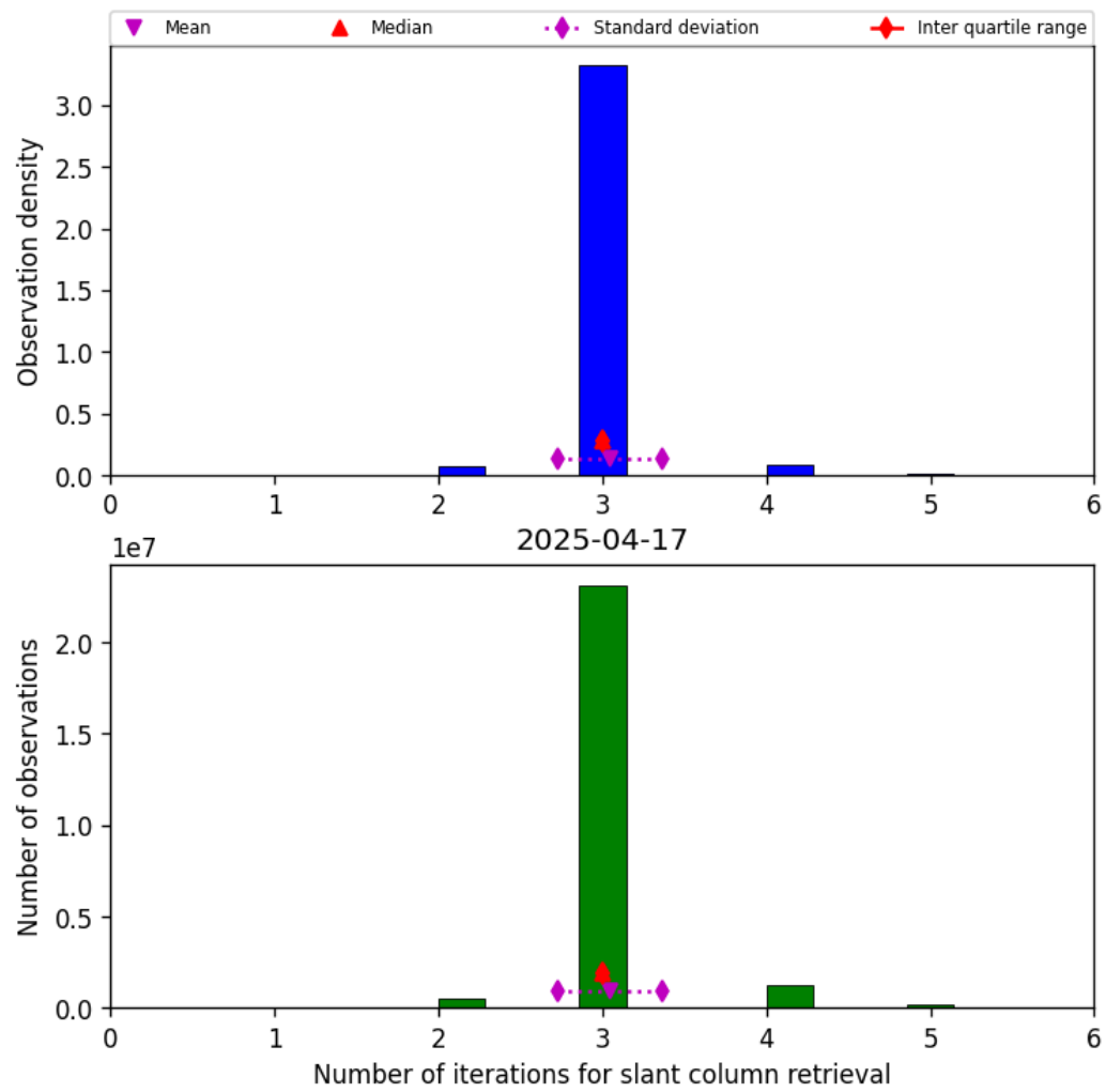
Figure 33: Histogram of “Number of iterations for slant column retrieval” for 2025-04-17 to 2025-04-18
