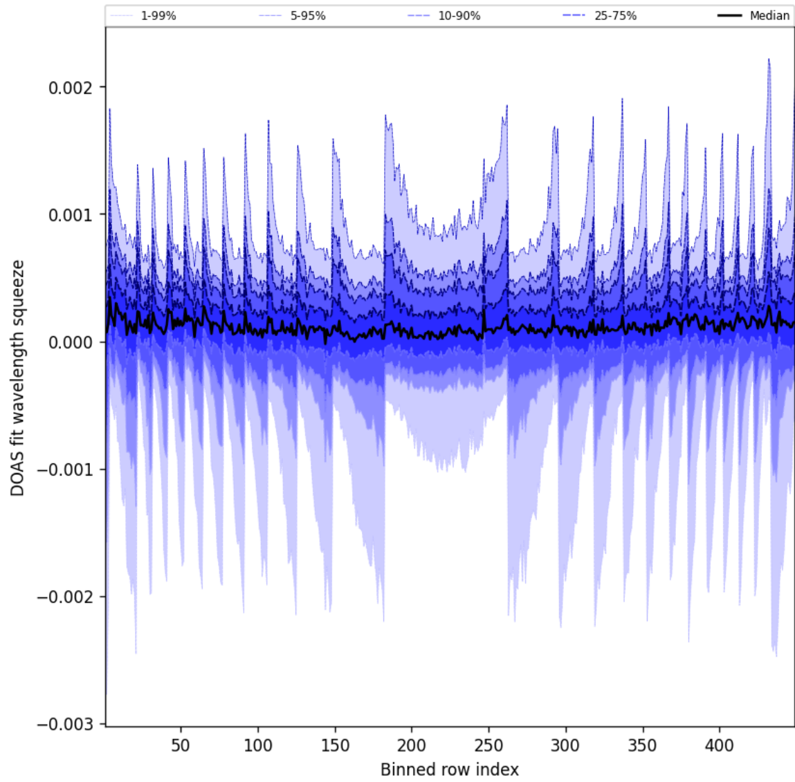
Figure 48: Along track statistics of “DOAS fit wavelength squeeze” for 2025-04-17 to 2025-04-18
