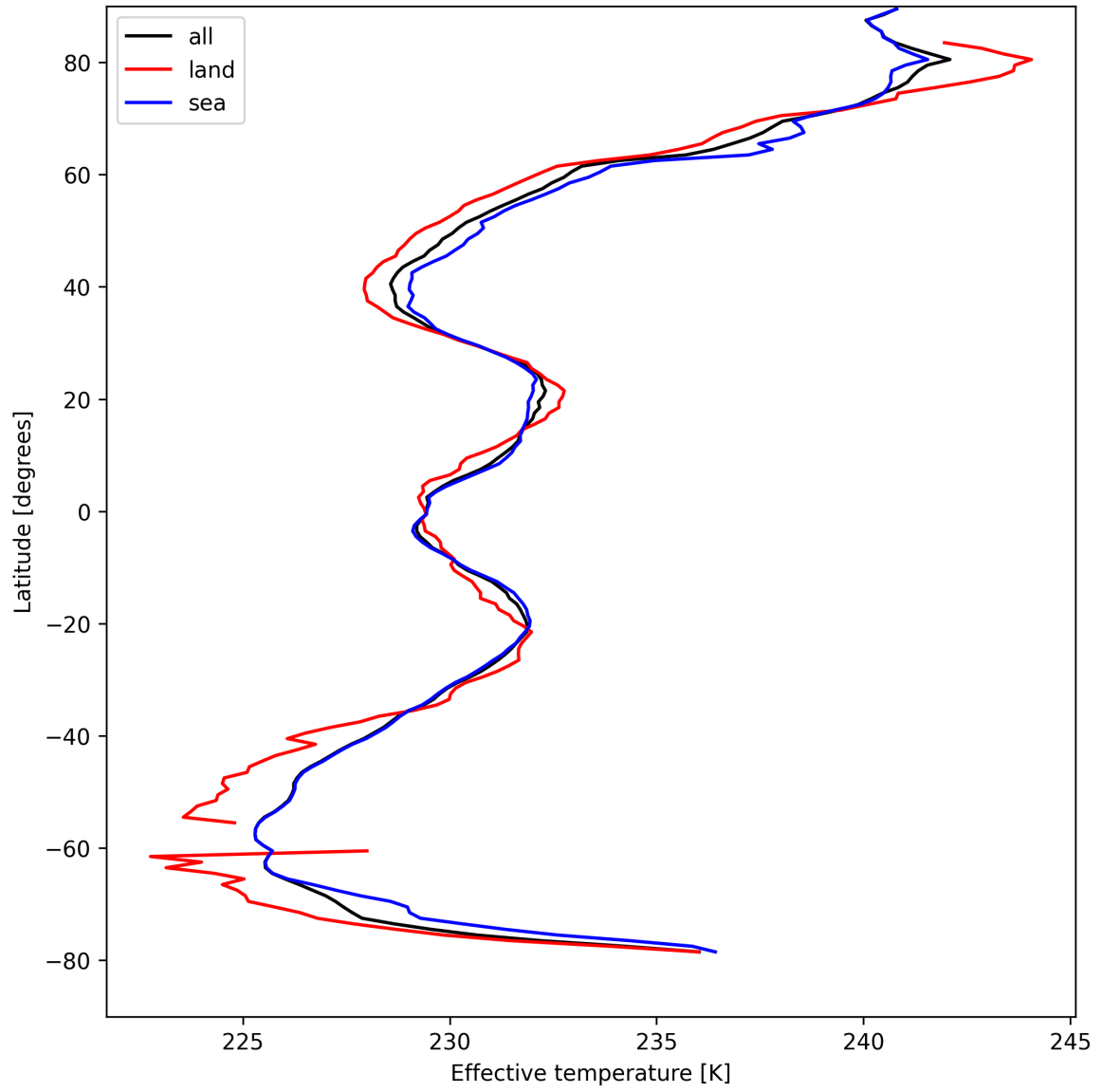
Figure 26: Zonal average of “Effective temperature” for 2025-04-17 to 2025-04-18.
