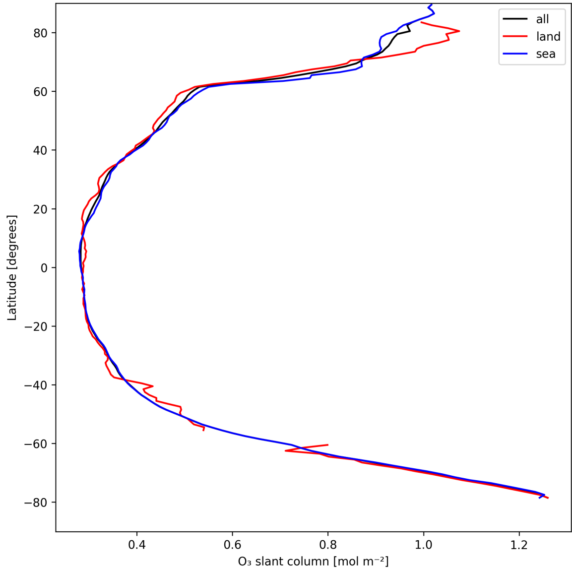
Figure 19: Zonal average of “O 3 slant column” for 2025-04-17 to 2025-04-18.
