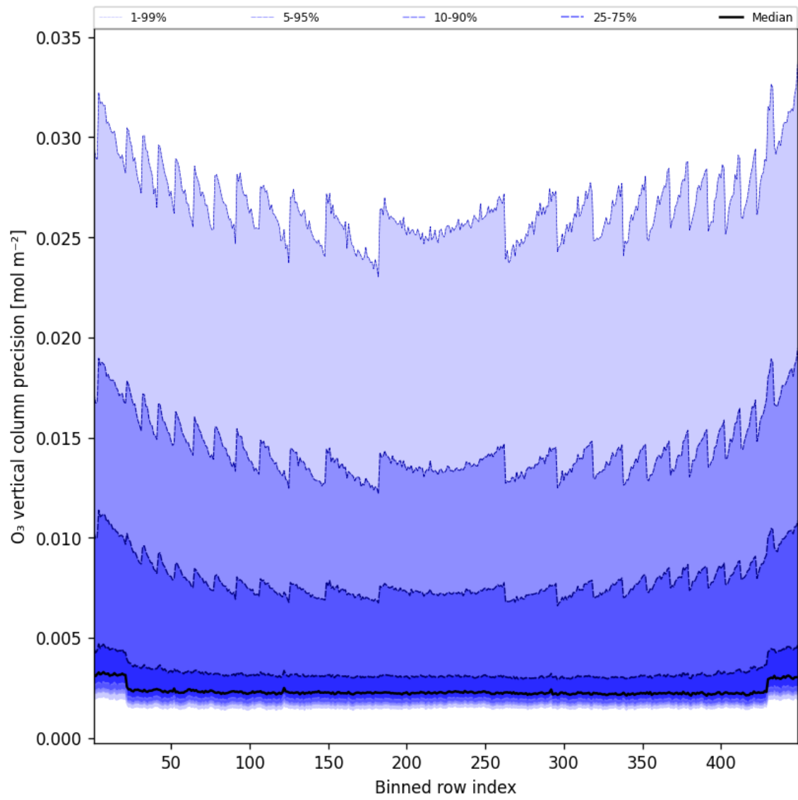
Figure 42: Along track statistics of “O 3 vertical column precision” for 2025-04-17 to 2025-04-18
