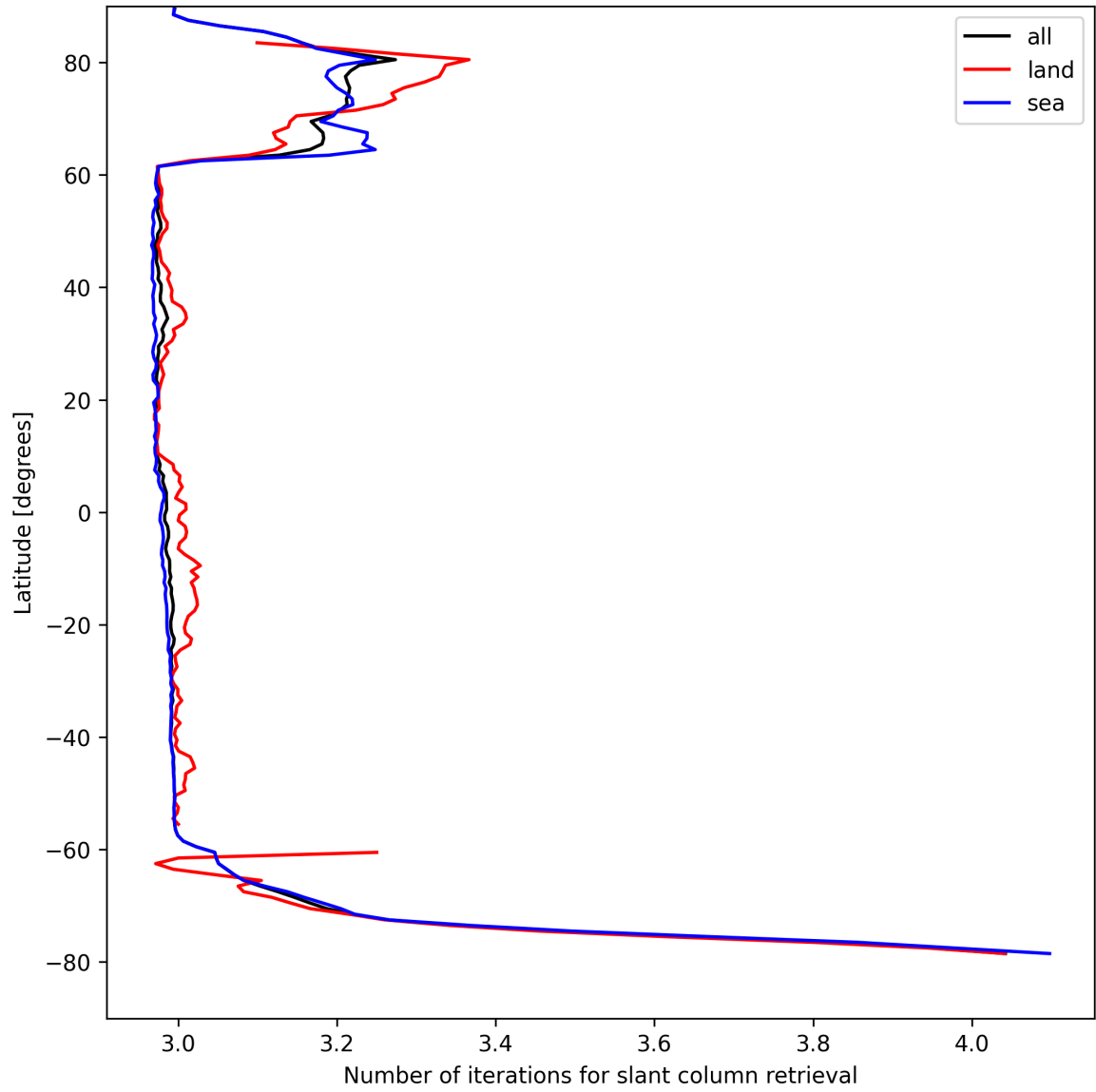
Figure 21: Zonal average of “Number of iterations for slant column retrieval” for 2025-04-17 to 2025-04-18.
