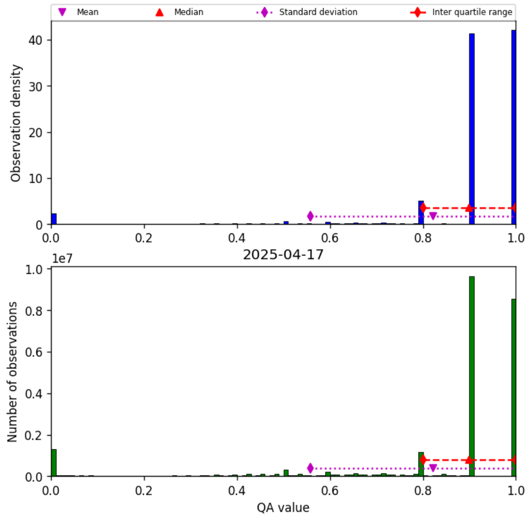
Figure 28: Histogram of “QA value” for 2025-04-17 to 2025-04-18
