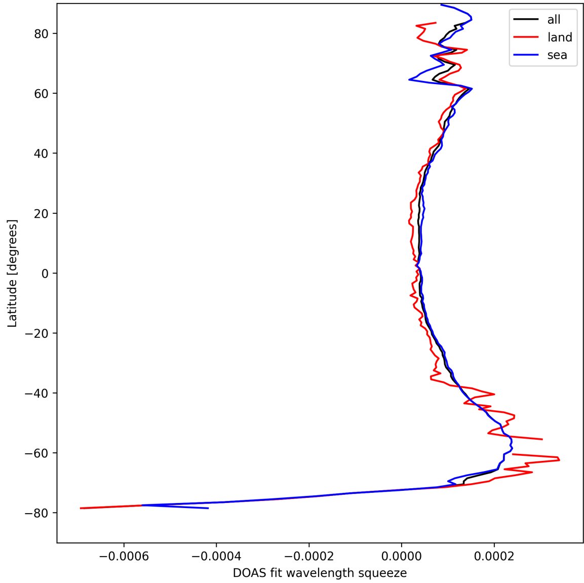
Figure 24: Zonal average of “DOAS fit wavelength squeeze” for 2025-04-17 to 2025-04-18.
