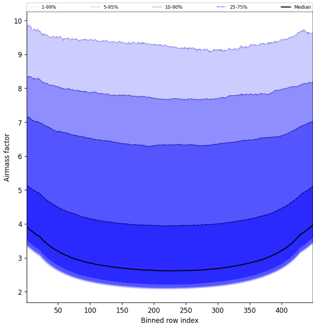
Figure 49: Along track statistics of “Airmass factor” for 2025-04-17 to 2025-04-18
