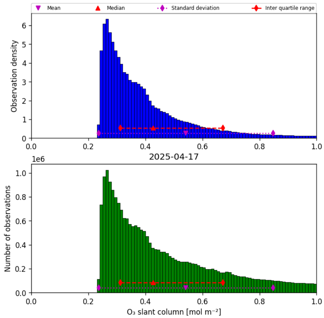
Figure 31: Histogram of “O 3 slant column” for 2025-04-17 to 2025-04-18
