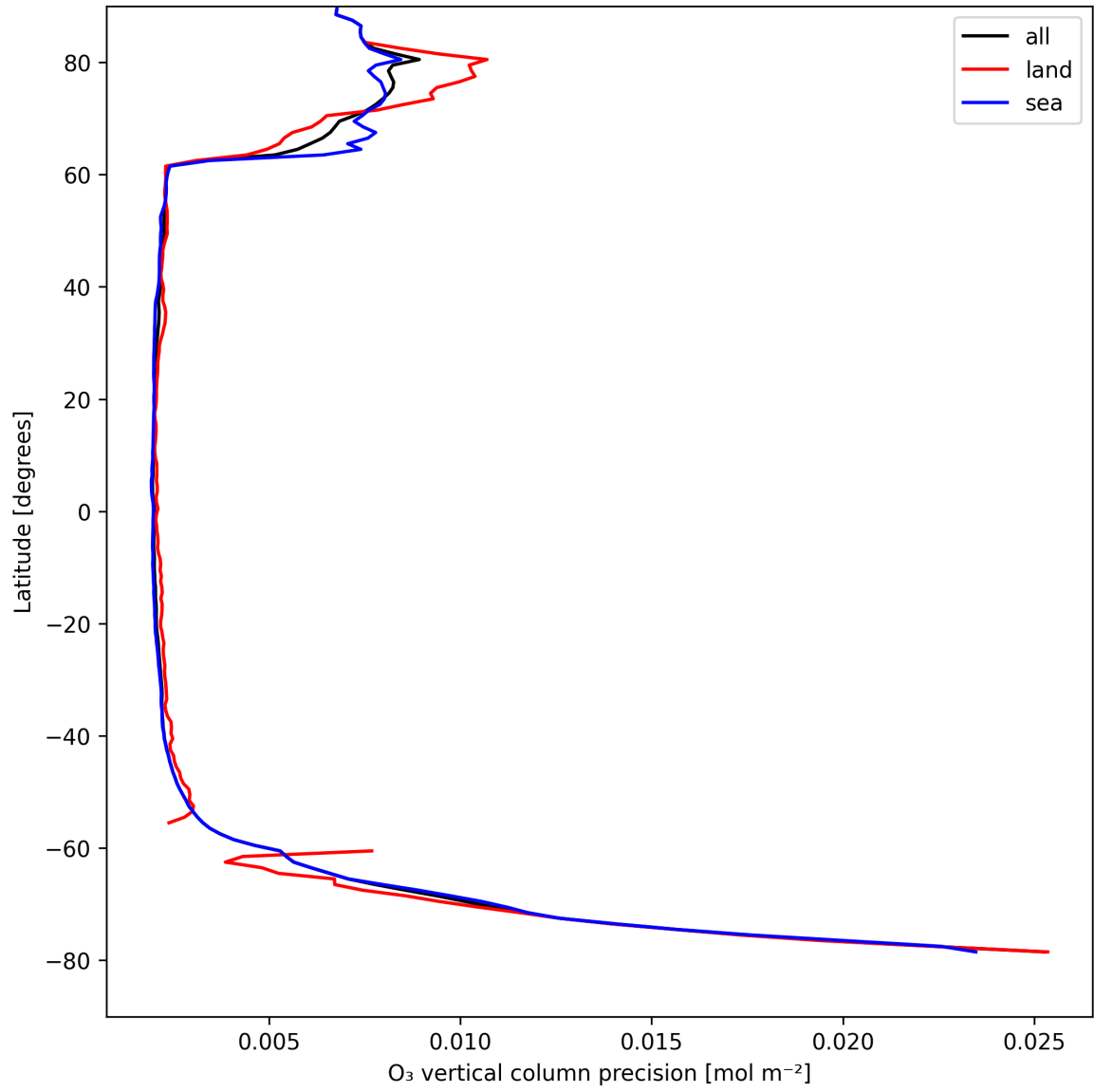
Figure 18: Zonal average of “O 3 vertical column precision” for 2025-04-17 to 2025-04-18.
