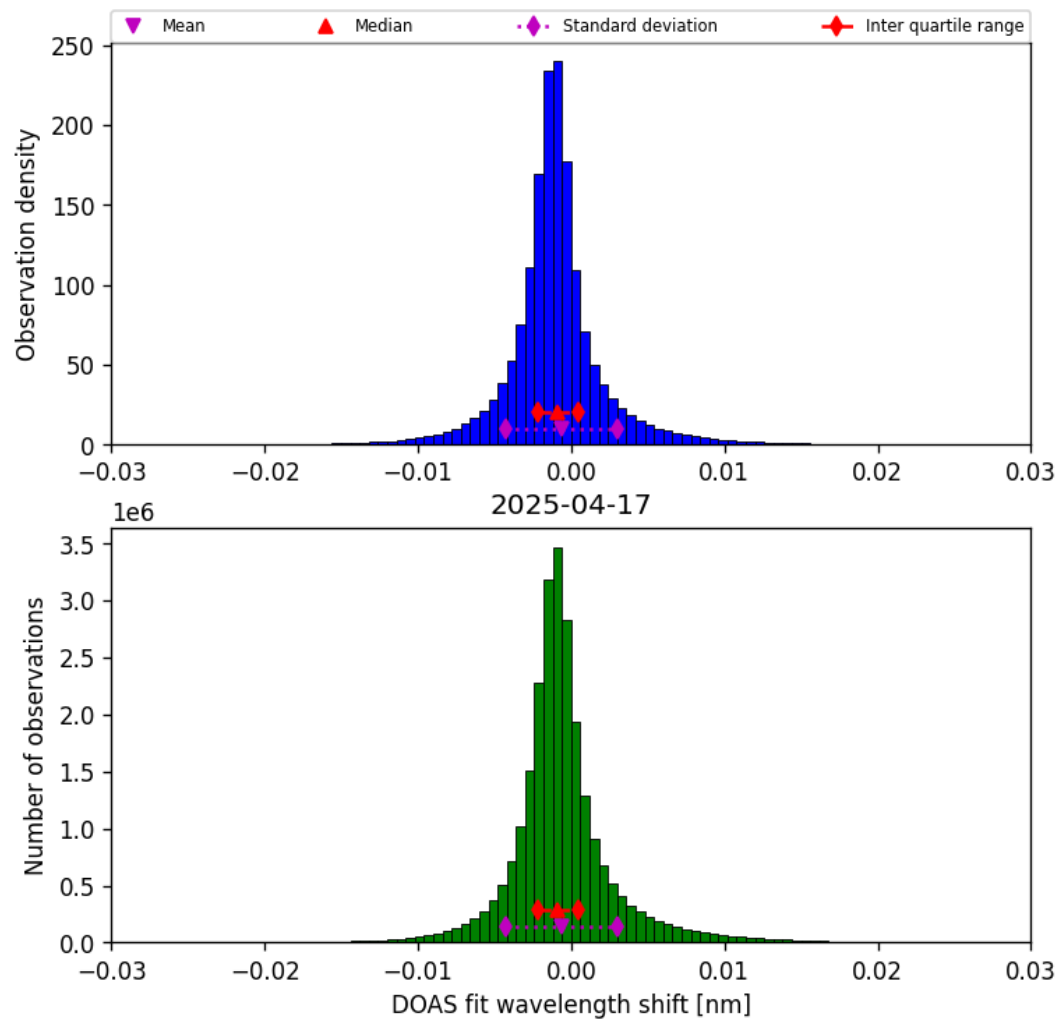
Figure 35: Histogram of “DOAS fit wavelength shift” for 2025-04-17 to 2025-04-18
