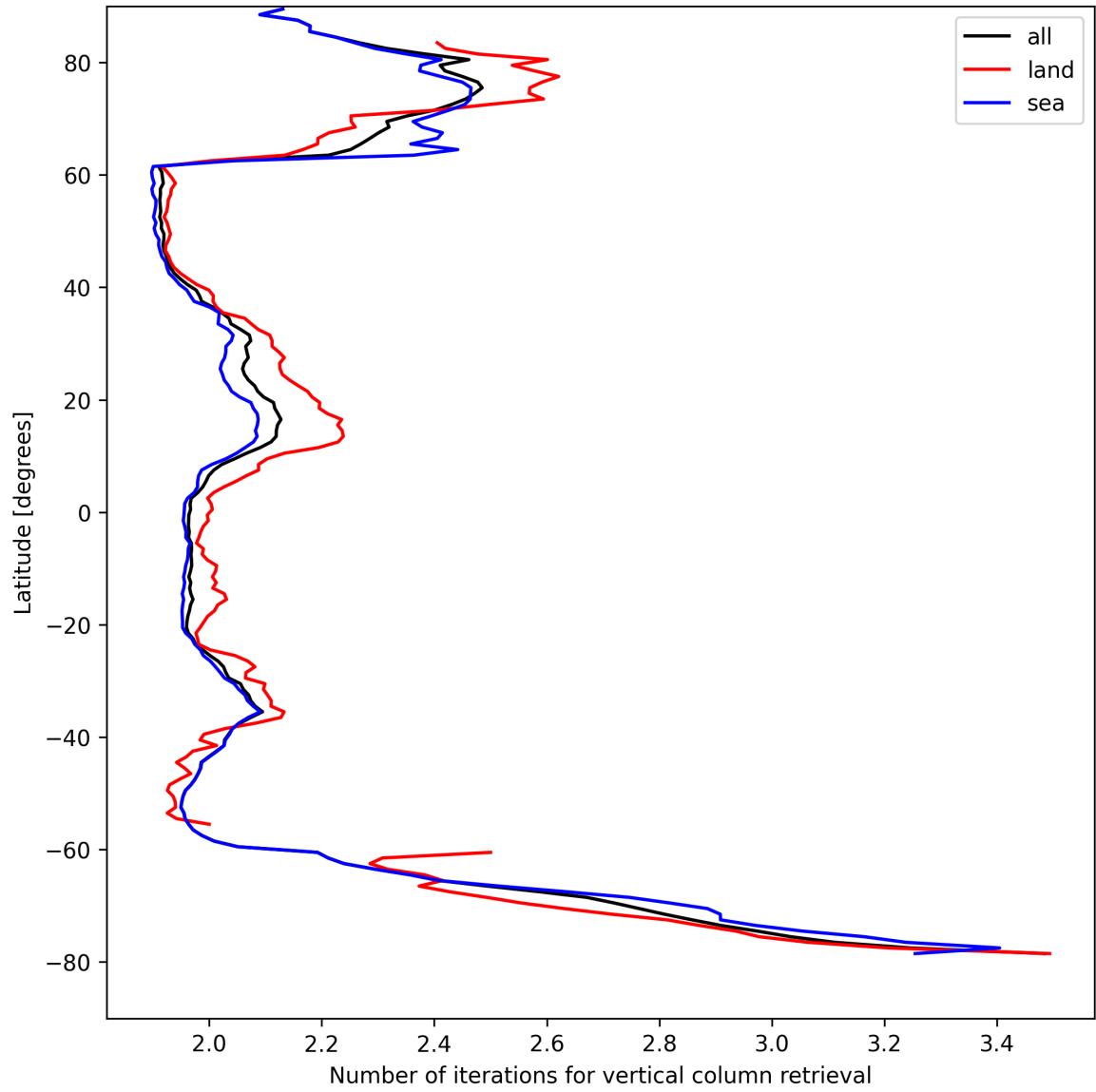
Figure 27: Zonal average of “Number of iterations for vertical column retrieval” for 2025-04-17 to 2025-04-18.
