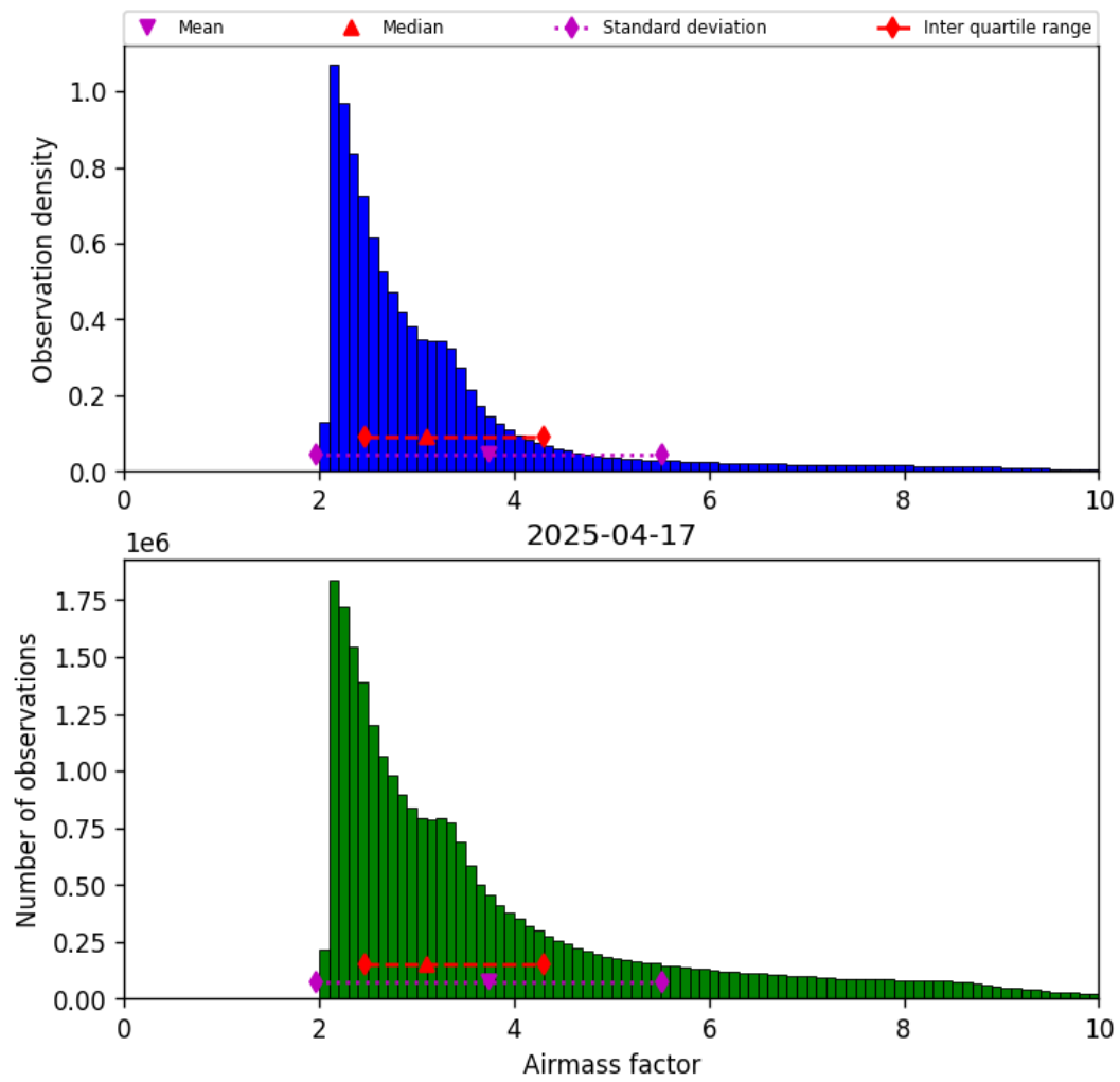
Figure 37: Histogram of “Airmass factor” for 2025-04-17 to 2025-04-18
