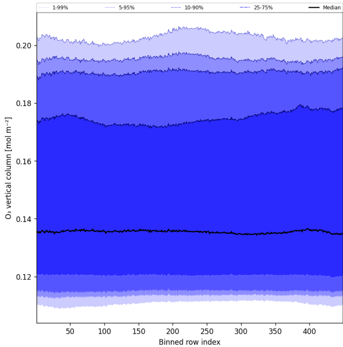
Figure 41: Along track statistics of “ O_3 vertical column” for 2025-04-17 to 2025-04-18
