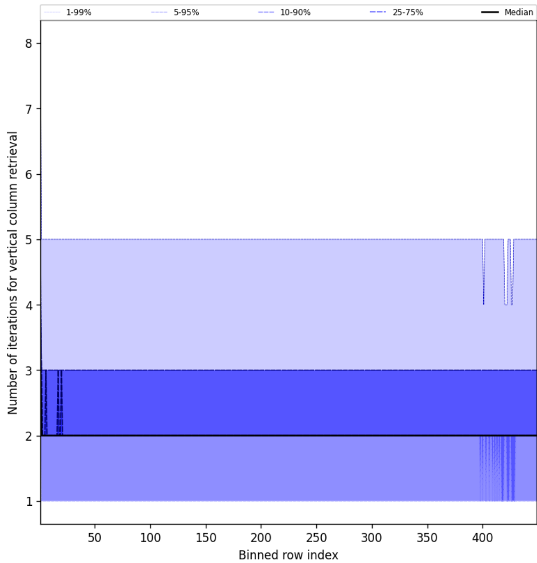
Figure 51: Along track statistics of “Number of iterations for vertical column retrieval” for 2025-04-17 to 2025-04-18
