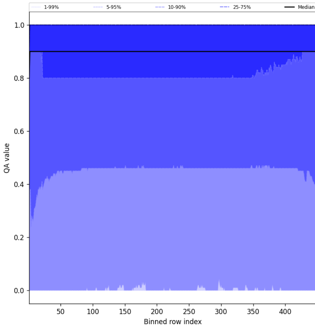
Figure 40: Along track statistics of “QA value” for 2025-04-17 to 2025-04-18
