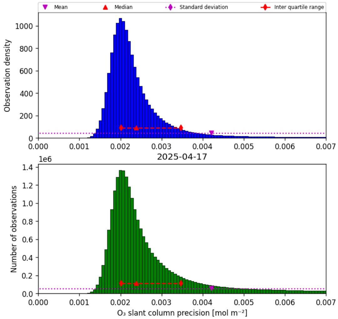
Figure 32: Histogram of “O 3 slant column precision” for 2025-04-17 to 2025-04-18
