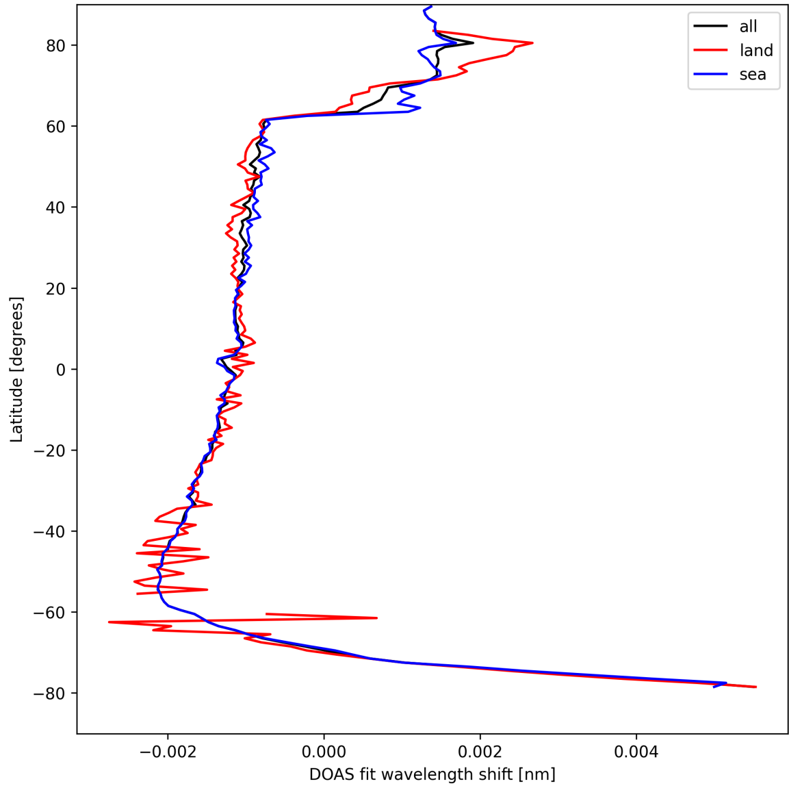
Figure 23: Zonal average of “DOAS fit wavelength shift” for 2025-04-17 to 2025-04-18.
