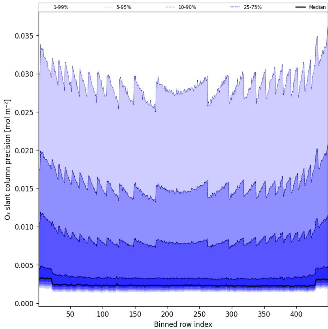
Figure 44: Along track statistics of “O 3 slant column precision” for 2025-04-17 to 2025-04-18
