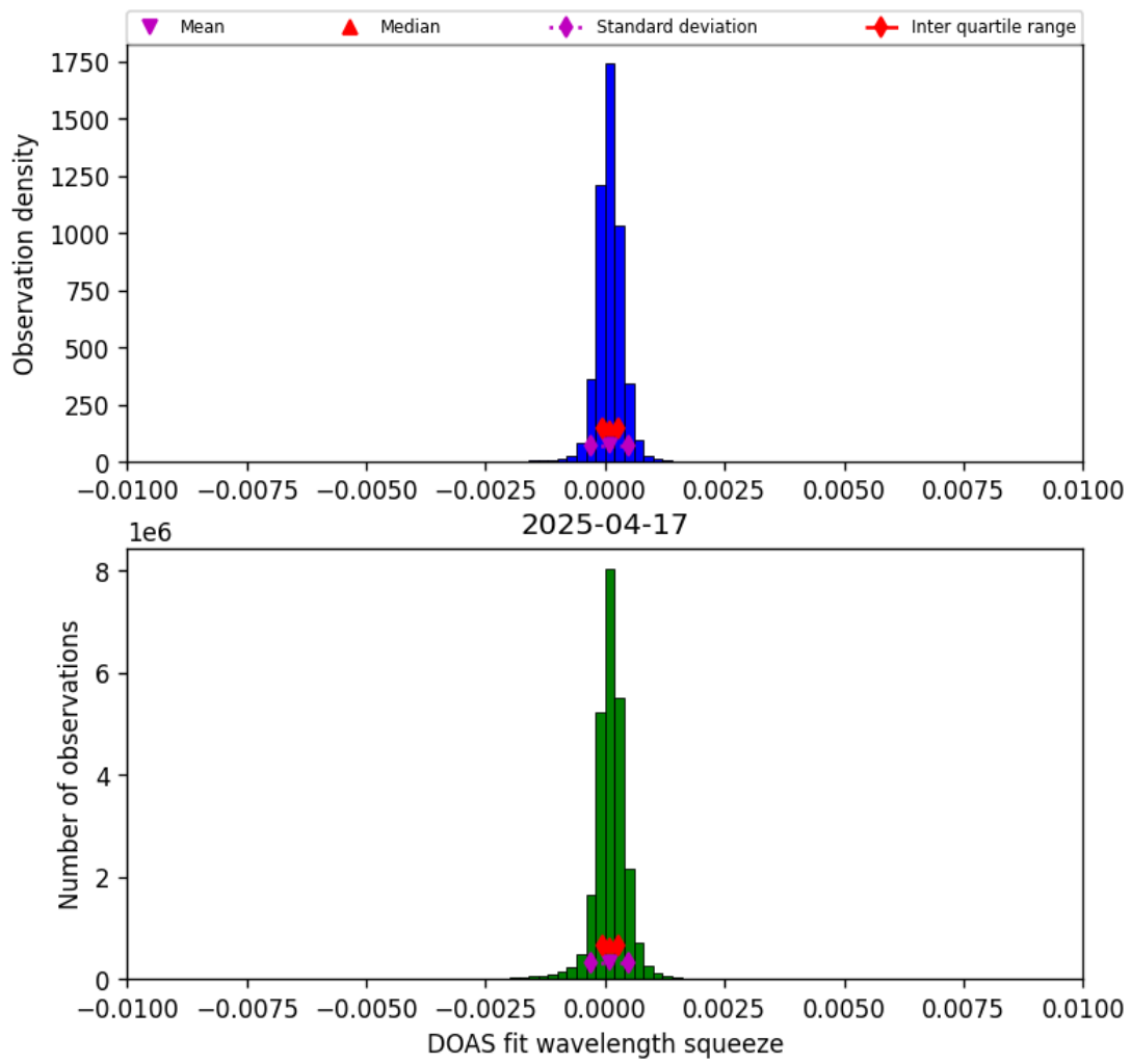
Figure 36: Histogram of “DOAS fit wavelength squeeze” for 2025-04-17 to 2025-04-18
