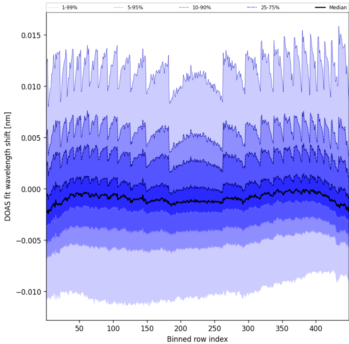
Figure 47: Along track statistics of “DOAS fit wavelength shift” for 2025-04-17 to 2025-04-18
