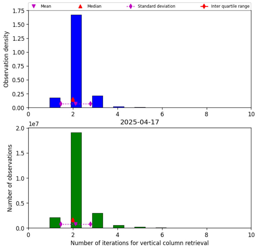
Figure 39: Histogram of “Number of iterations for vertical column retrieval” for 2025-04-17 to 2025-04-18
