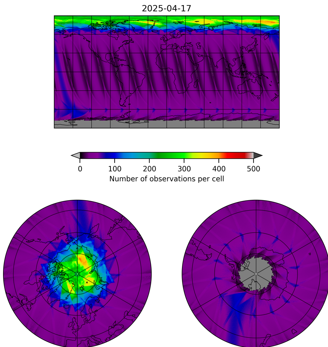
Figure 15: Map of the number of observations for 2025-04-17 to 2025-04-18
