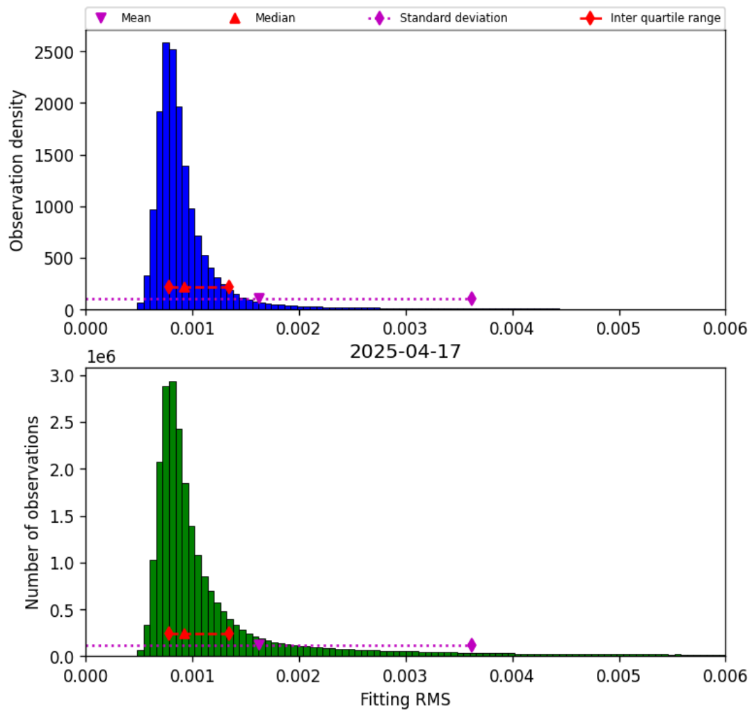
Figure 34: Histogram of “Fitting RMS” for 2025-04-17 to 2025-04-18
