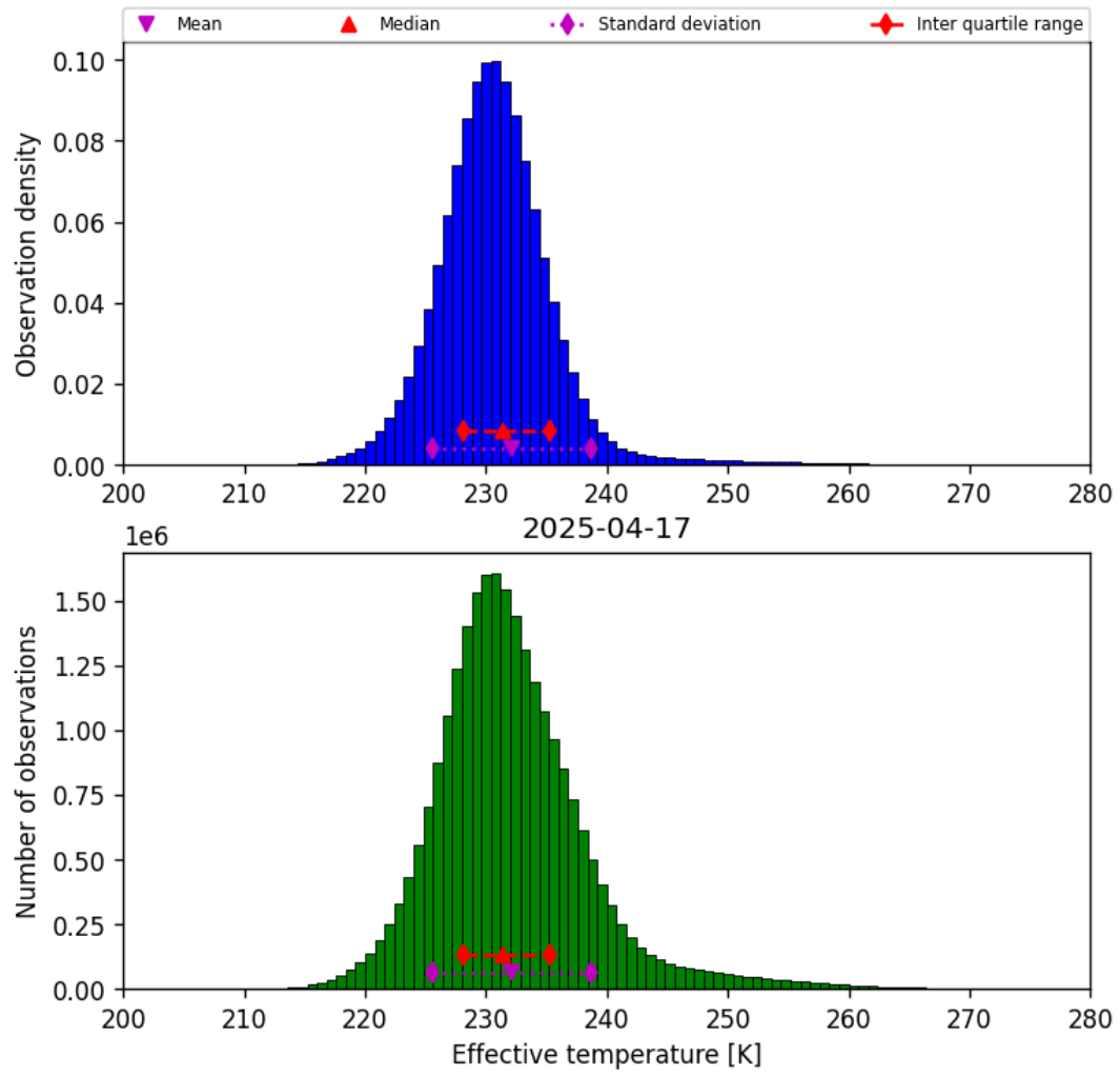
Figure 38: Histogram of “Effective temperature” for 2025-04-17 to 2025-04-18
