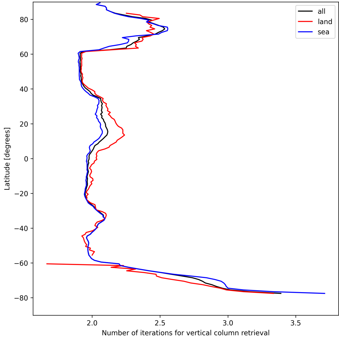
Figure 27: Zonal average of “Number of iterations for vertical column retrieval” for 2025-04-19 to 2025-04-20.
