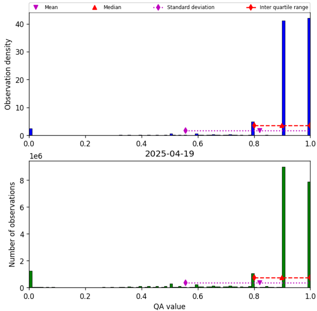
Figure 28: Histogram of “QA value” for 2025-04-19 to 2025-04-20
