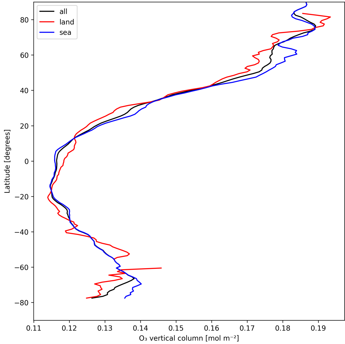
Figure 17: Zonal average of “O 3 vertical column” for 2025-04-19 to 2025-04-20.
