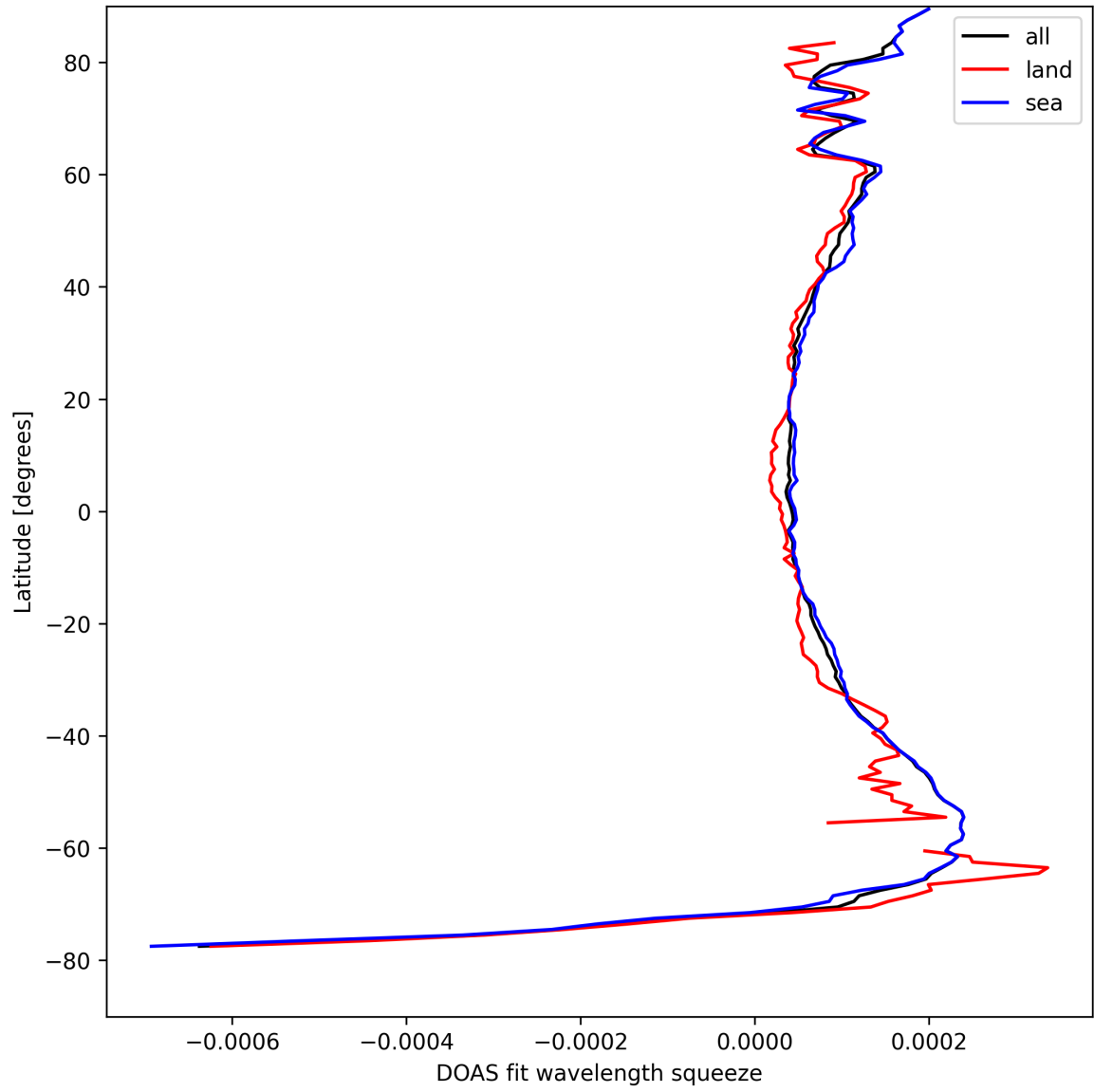
Figure 24: Zonal average of “DOAS fit wavelength squeeze” for 2025-04-19 to 2025-04-20.
