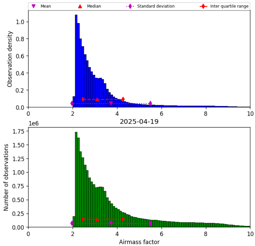
Figure 37: Histogram of “Airmass factor” for 2025-04-19 to 2025-04-20
