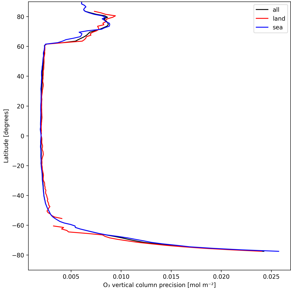
Figure 18: Zonal average of “O 3 vertical column precision” for 2025-04-19 to 2025-04-20.
