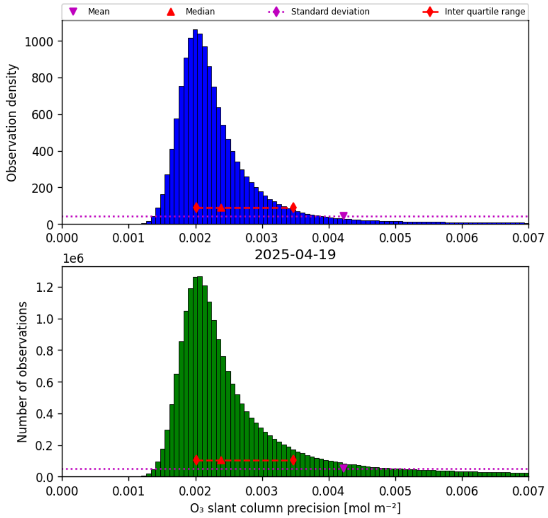
Figure 32: Histogram of “O 3 slant column precision” for 2025-04-19 to 2025-04-20
