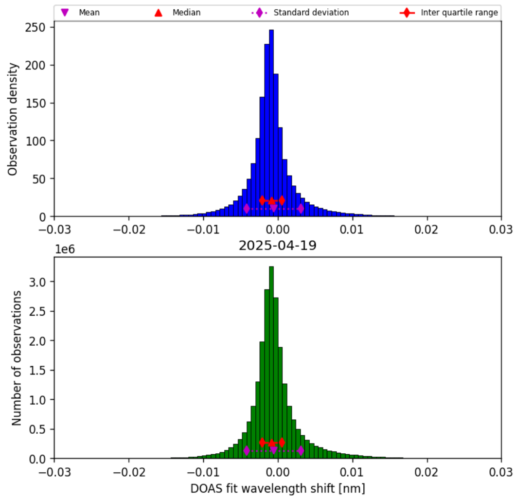
Figure 35: Histogram of “DOAS fit wavelength shift” for 2025-04-19 to 2025-04-20
