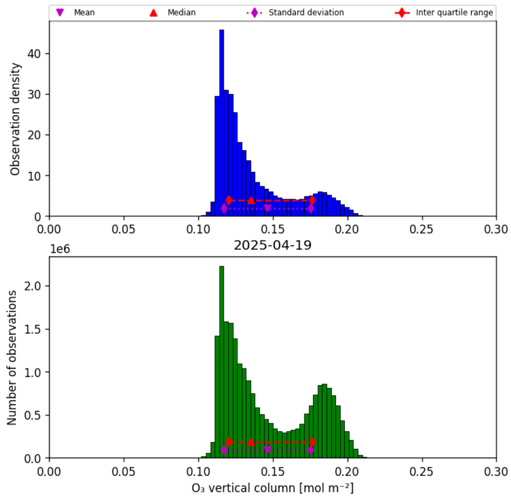
Figure 29: Histogram of “O 3 vertical column” for 2025-04-19 to 2025-04-20
