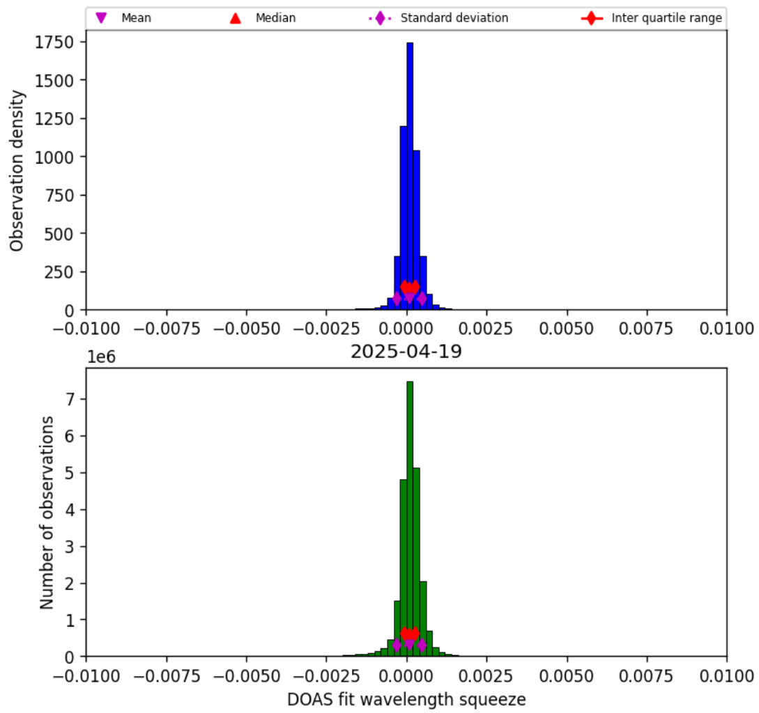
Figure 36: Histogram of “DOAS fit wavelength squeeze” for 2025-04-19 to 2025-04-20
