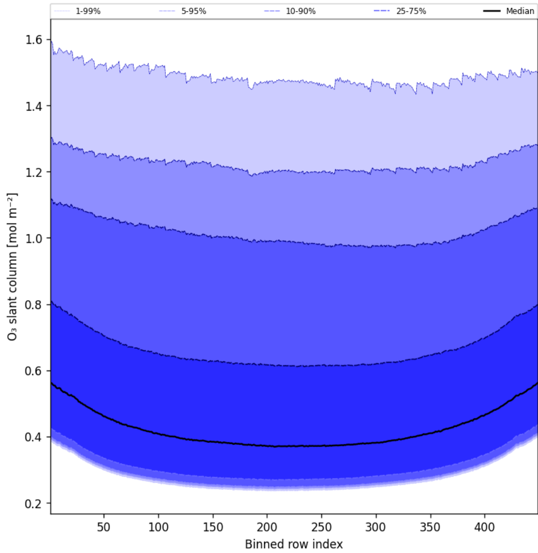
Figure 43: Along track statistics of “O 3 slant column” for 2025-04-19 to 2025-04-20
