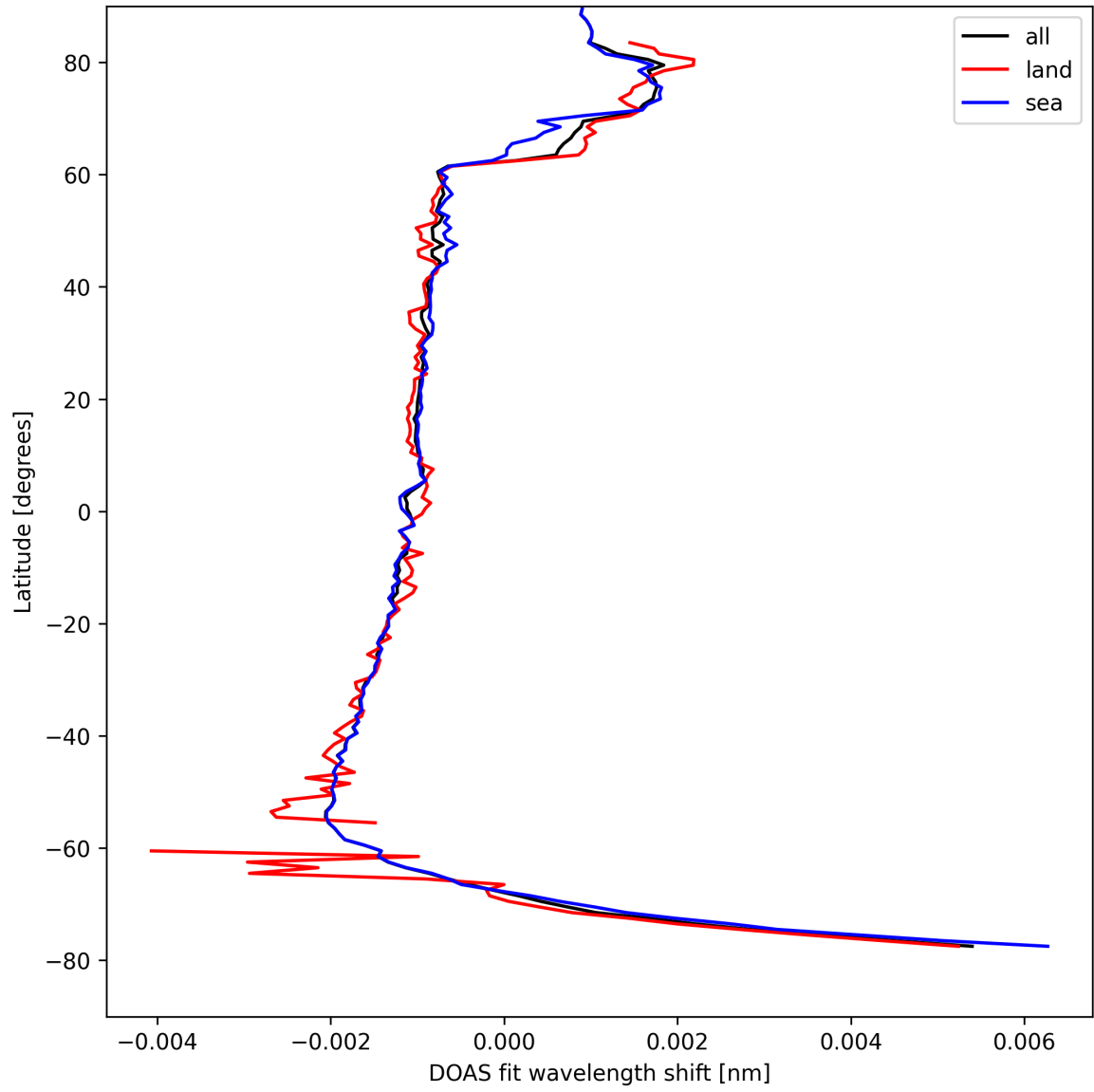
Figure 23: Zonal average of “DOAS fit wavelength shift” for 2025-04-19 to 2025-04-20.
