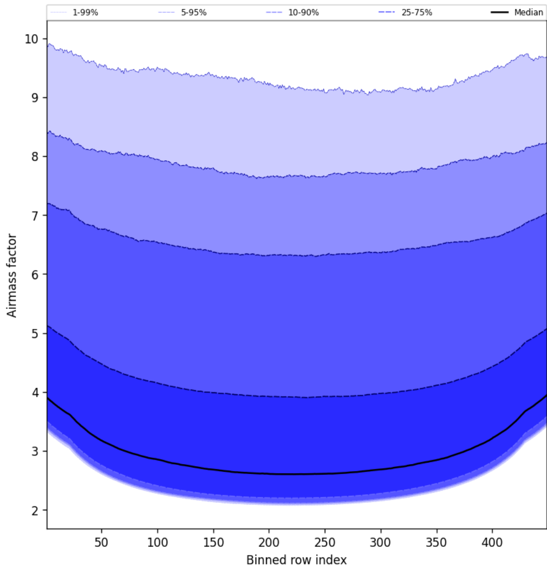
Figure 49: Along track statistics of “Airmass factor” for 2025-04-19 to 2025-04-20
