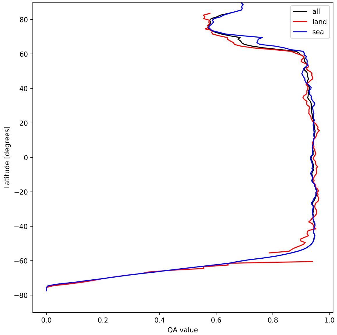
Figure 16: Zonal average of “QA value” for 2025-04-19 to 2025-04-20.
