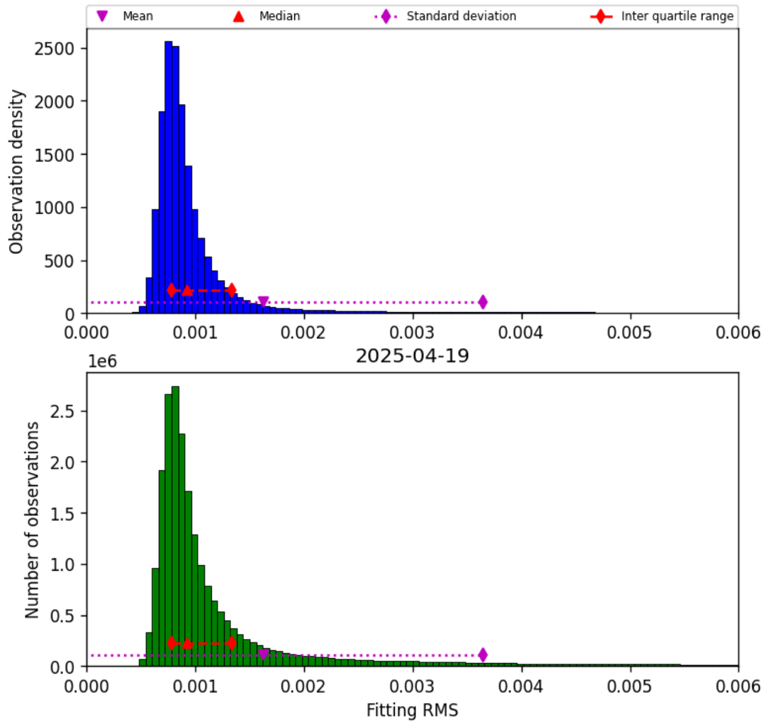
Figure 34: Histogram of “Fitting RMS” for 2025-04-19 to 2025-04-20
