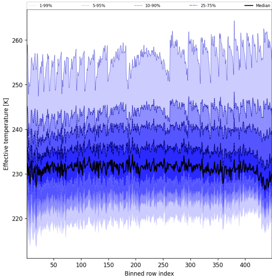
Figure 50: Along track statistics of “Effective temperature” for 2025-04-19 to 2025-04-20
