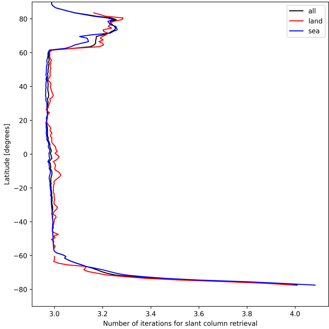
Figure 21: Zonal average of “Number of iterations for slant column retrieval” for 2025-04-19 to 2025-04-20.
