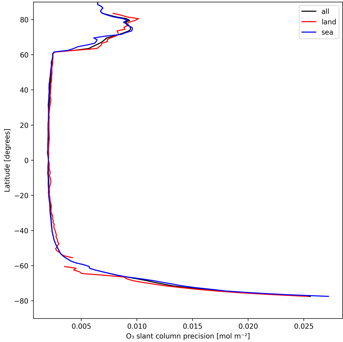
Figure 20: Zonal average of "O 3 slant column precision" for 2025-04-19 to 2025-04-20.
