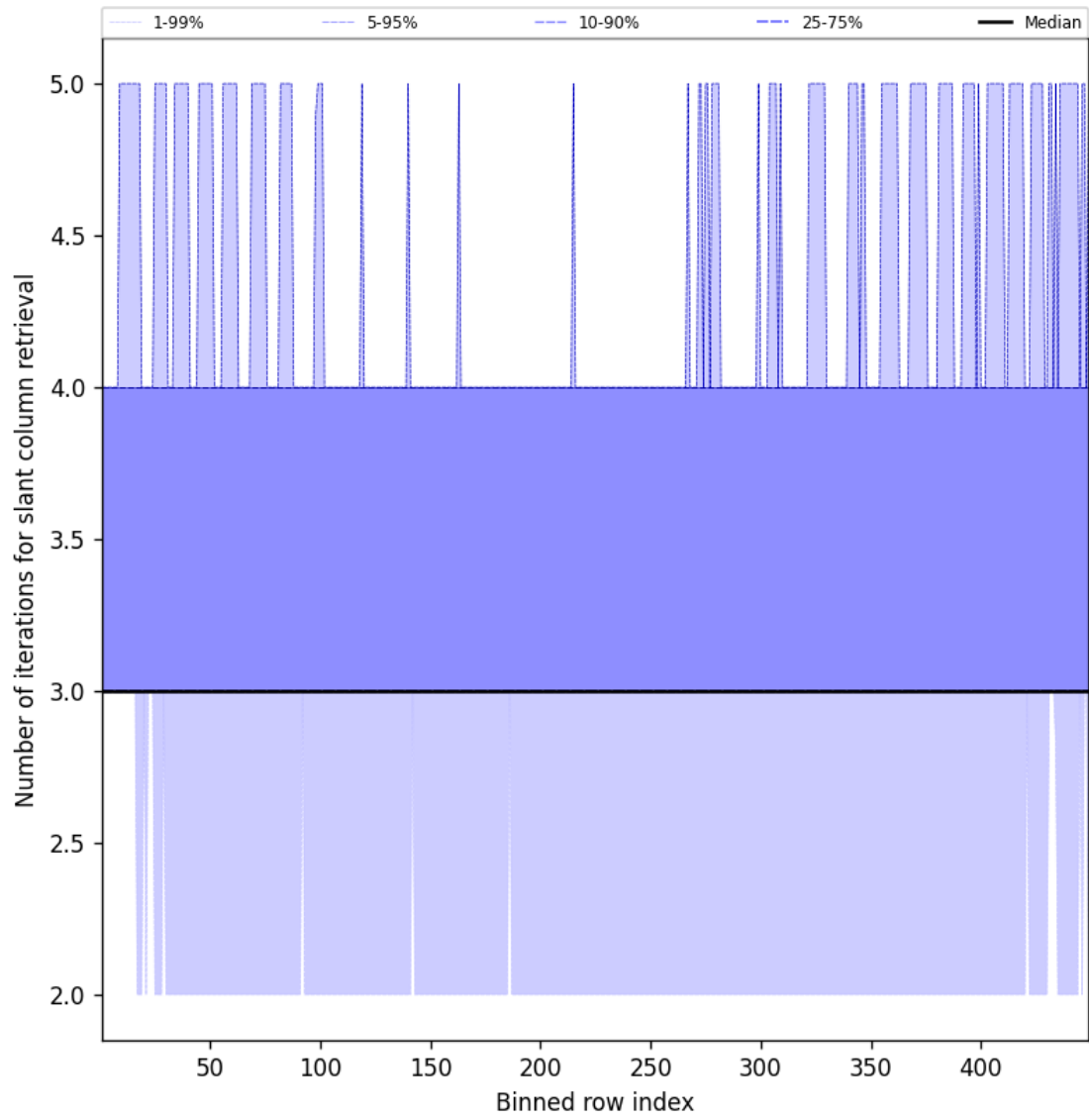
Figure 45: Along track statistics of “Number of iterations for slant column retrieval” for 2025-04-19 to 2025-04-20
