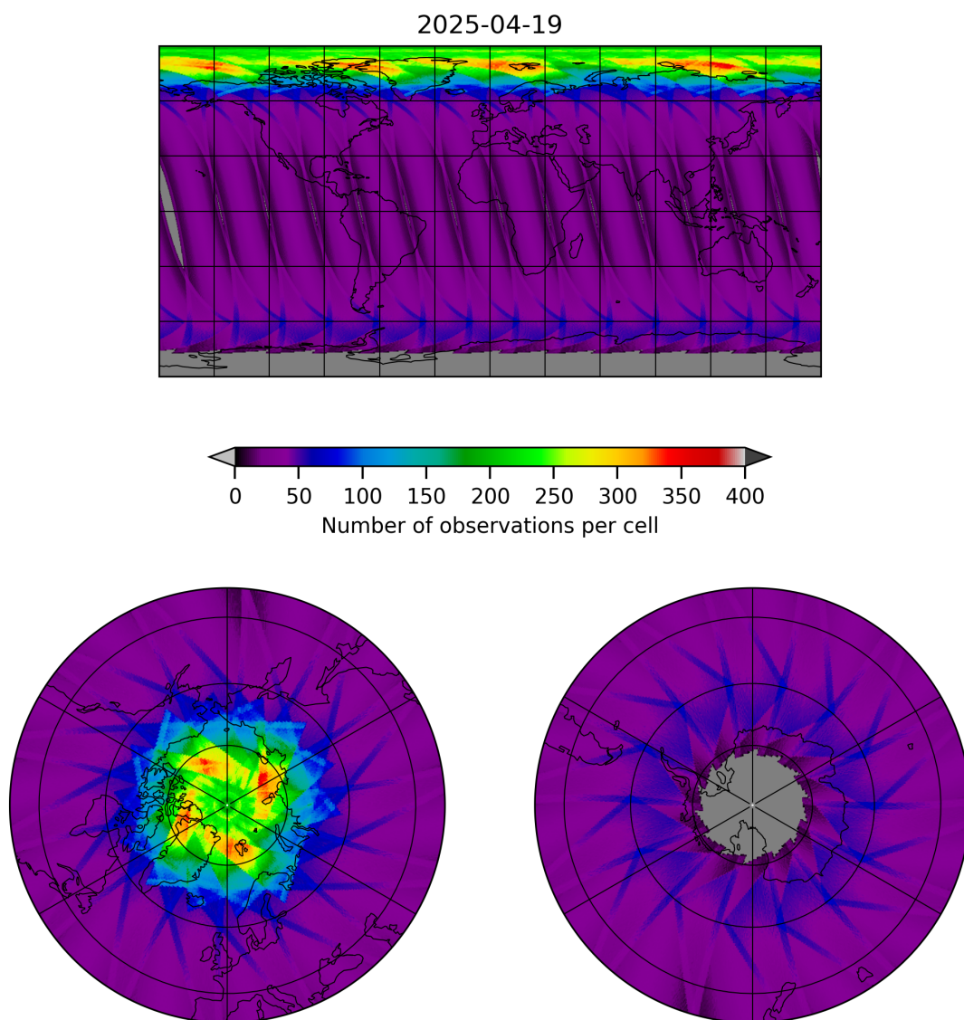
Figure 15: Map of the number of observations for 2025-04-19 to 2025-04-20
