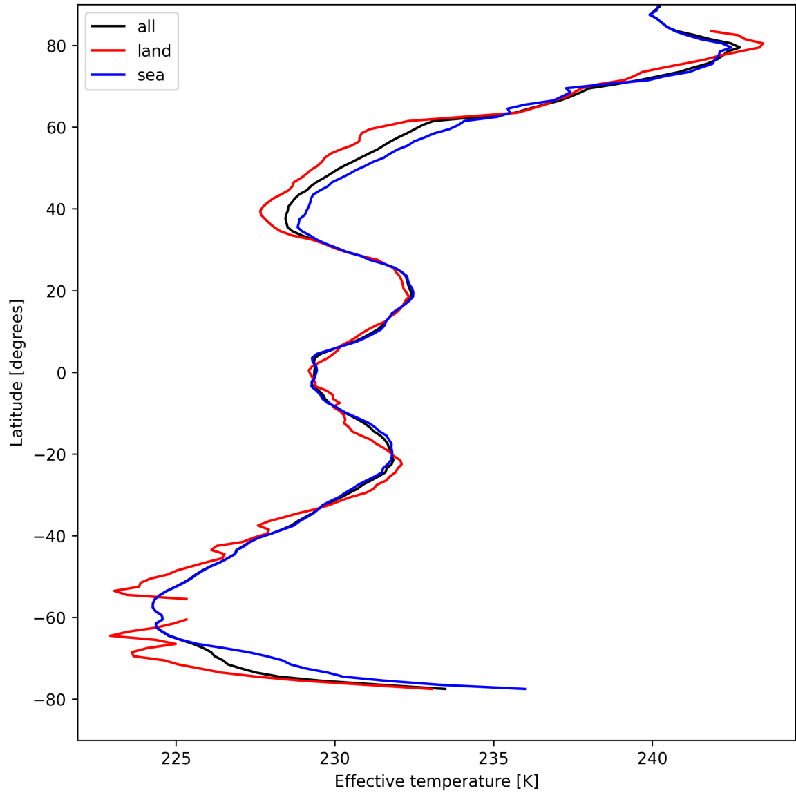
Figure 26: Zonal average of “Effective temperature” for 2025-04-19 to 2025-04-20.
