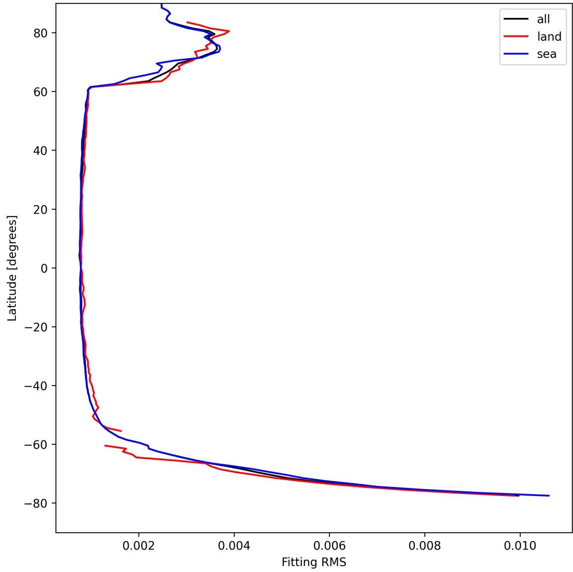
Figure 22: Zonal average of “Fitting RMS” for 2025-04-19 to 2025-04-20.
