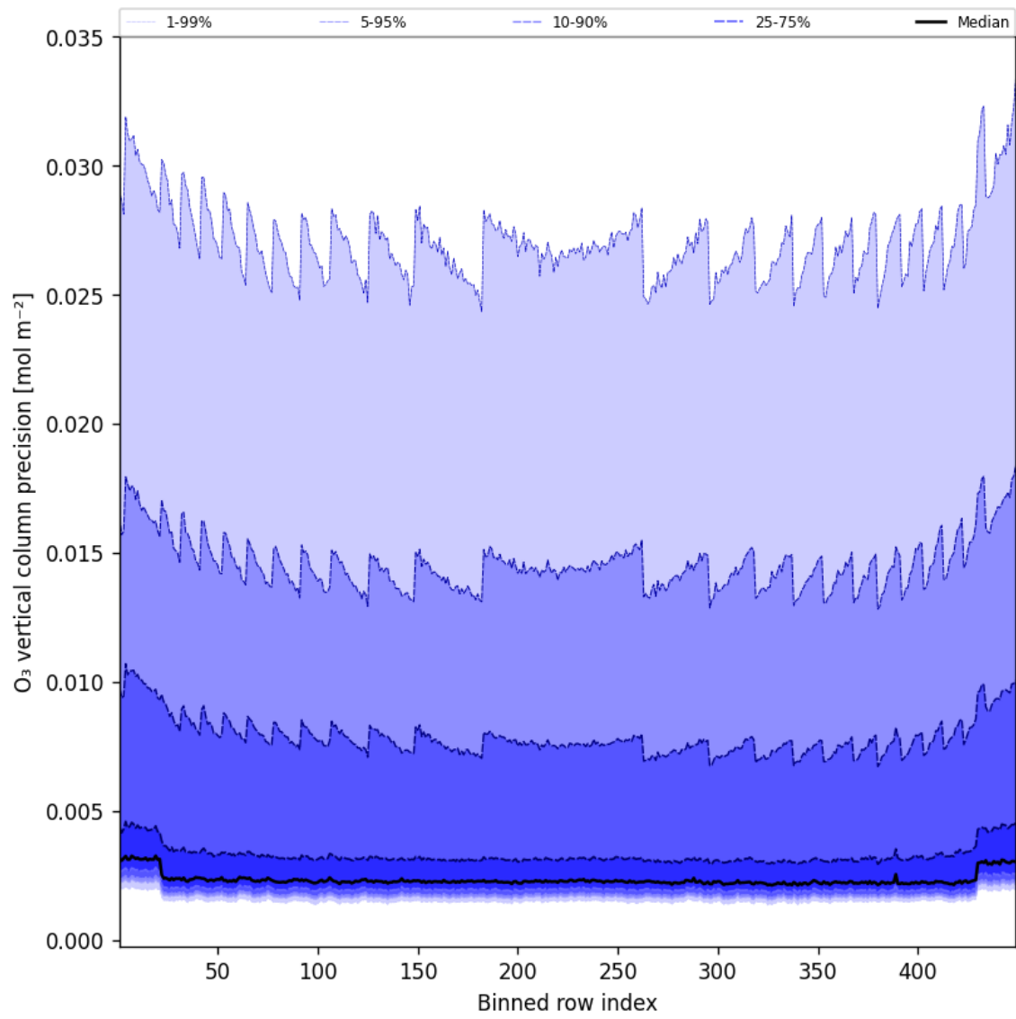
Figure 42: Along track statistics of “O 3 vertical column precision” for 2025-04-19 to 2025-04-20
