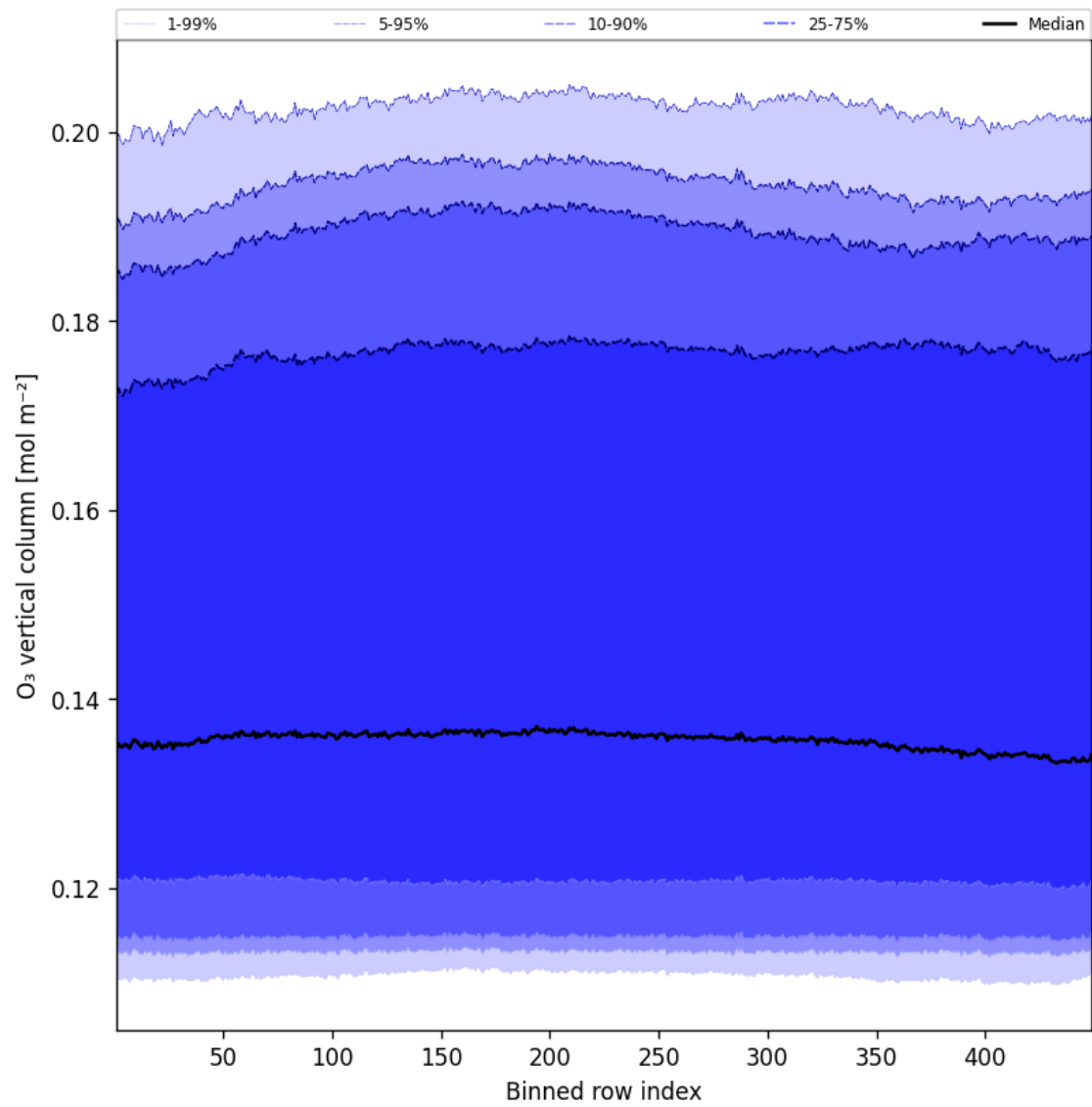
Figure 41: Along track statistics of “O 3 vertical column” for 2025-04-19 to 2025-04-20
