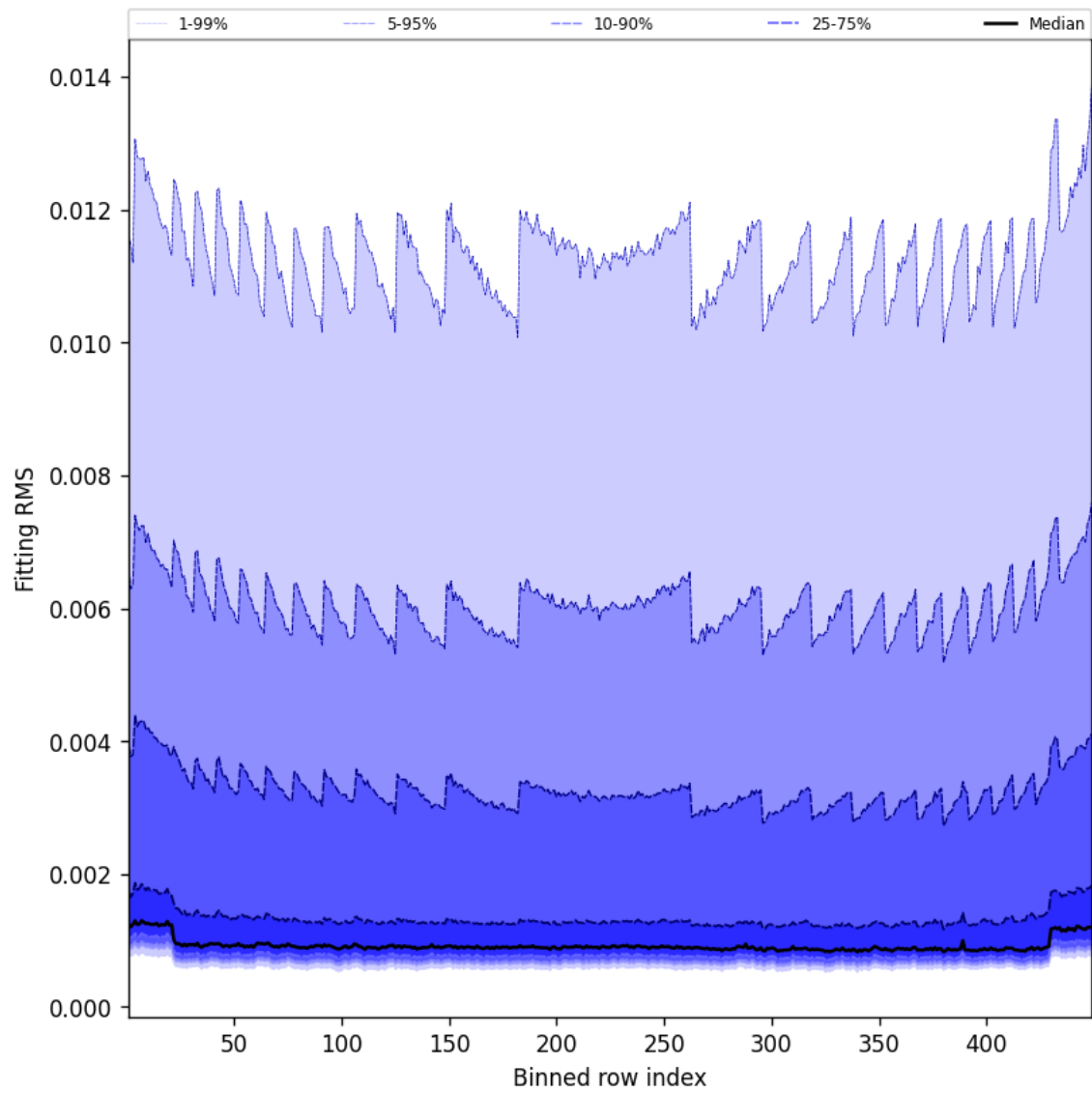
Figure 46: Along track statistics of “Fitting RMS” for 2025-04-19 to 2025-04-20
