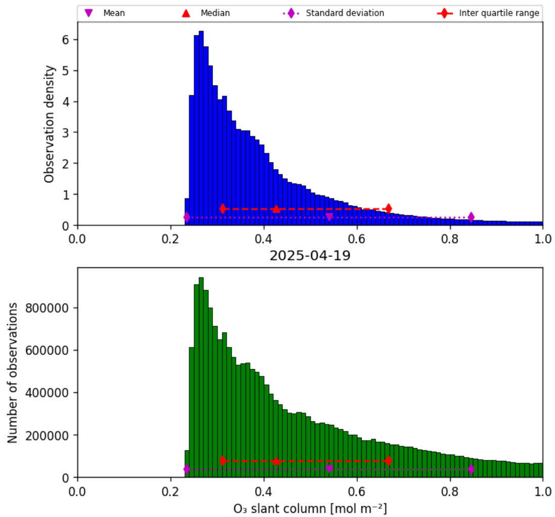
Figure 31: Histogram of “O 3 slant column” for 2025-04-19 to 2025-04-20
