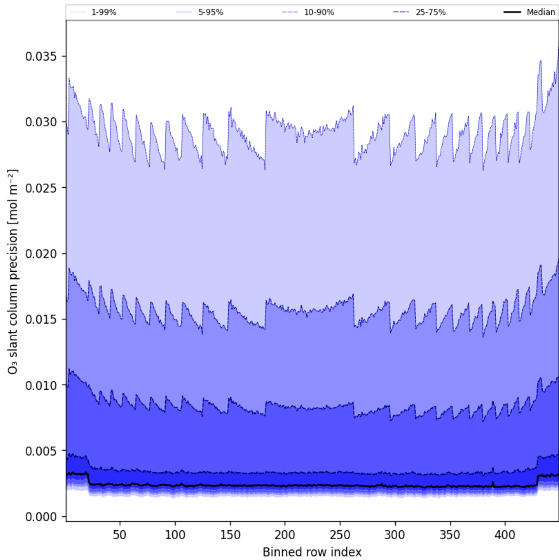
Figure 44: Along track statistics of “O 3 slant column precision” for 2025-04-19 to 2025-04-20
