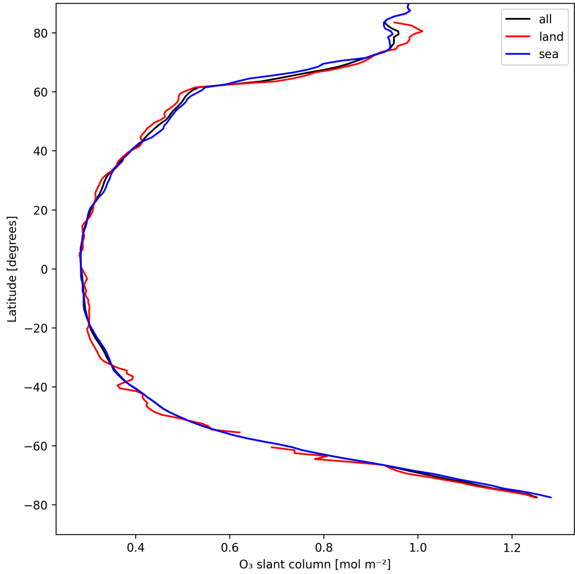
Figure 19: Zonal average of “O 3 slant column” for 2025-04-19 to 2025-04-20.
