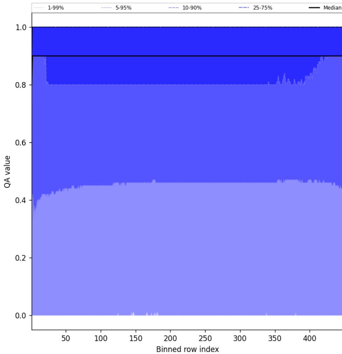
Figure 40: Along track statistics of “QA value” for 2025-04-19 to 2025-04-20
