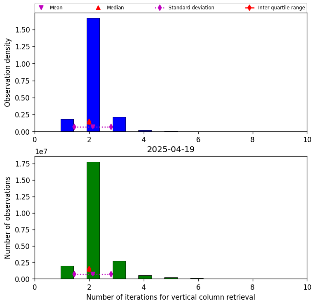
Figure 39: Histogram of “Number of iterations for vertical column retrieval” for 2025-04-19 to 2025-04-20
