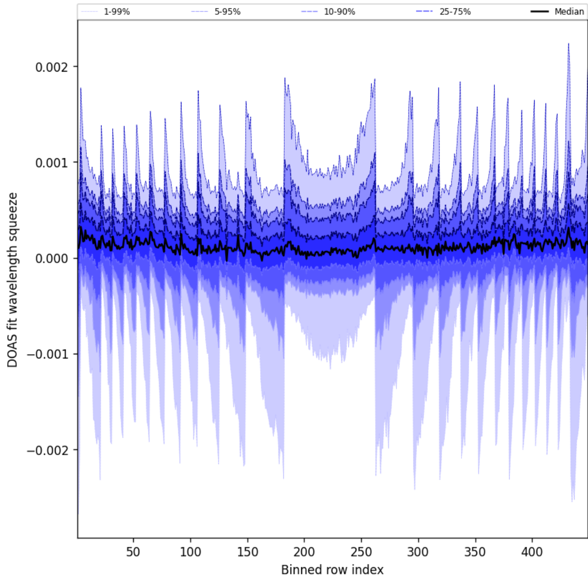
Figure 48: Along track statistics of “DOAS fit wavelength squeeze” for 2025-04-19 to 2025-04-20
