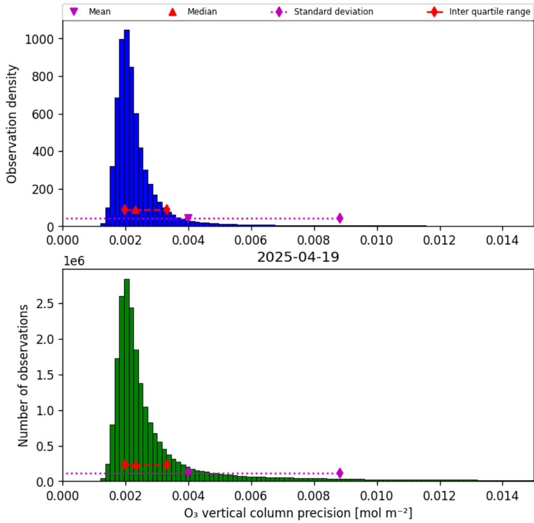
Figure 30: Histogram of “O 3 vertical column precision” for 2025-04-19 to 2025-04-20
