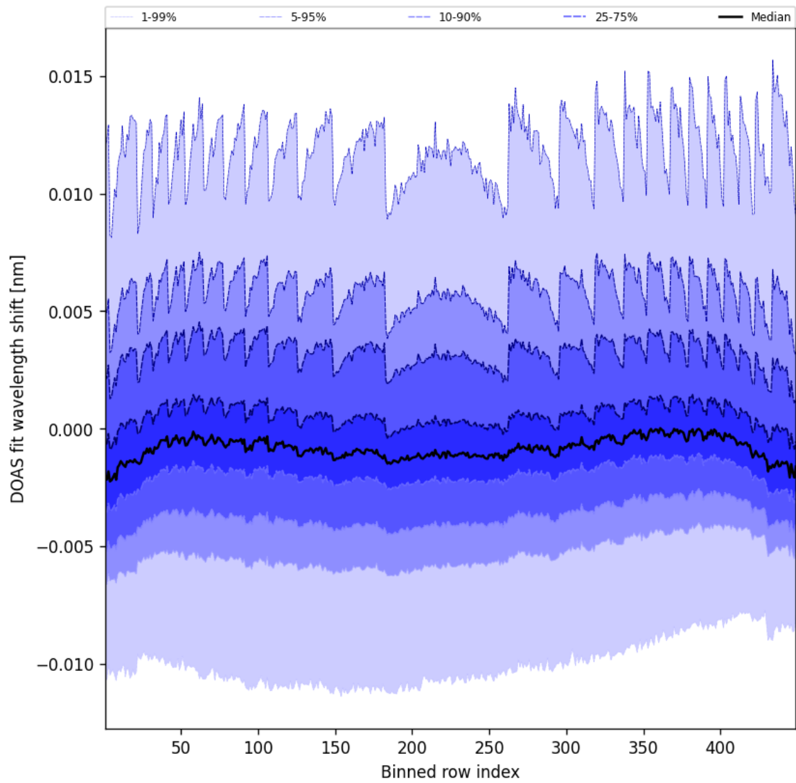
Figure 47: Along track statistics of “DOAS fit wavelength shift” for 2025-04-19 to 2025-04-20
