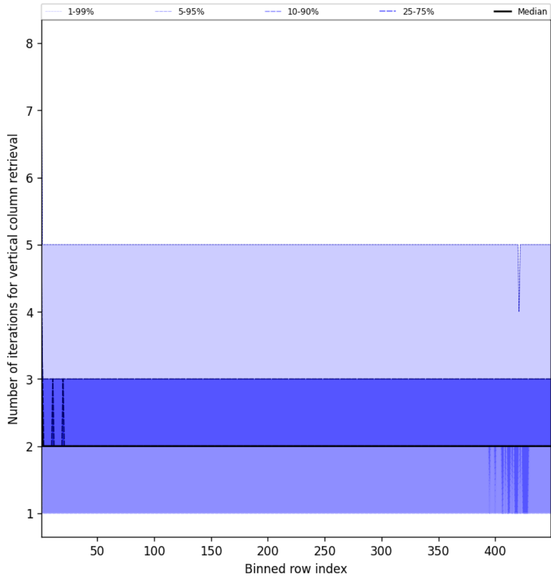
Figure 51: Along track statistics of “Number of iterations for vertical column retrieval” for 2025-04-19 to 2025-04-20
