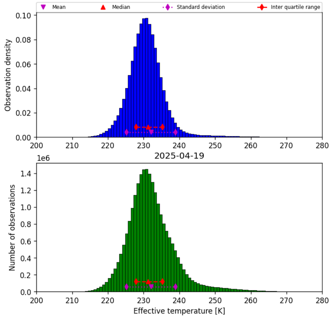
Figure 38: Histogram of “Effective temperature” for 2025-04-19 to 2025-04-20
