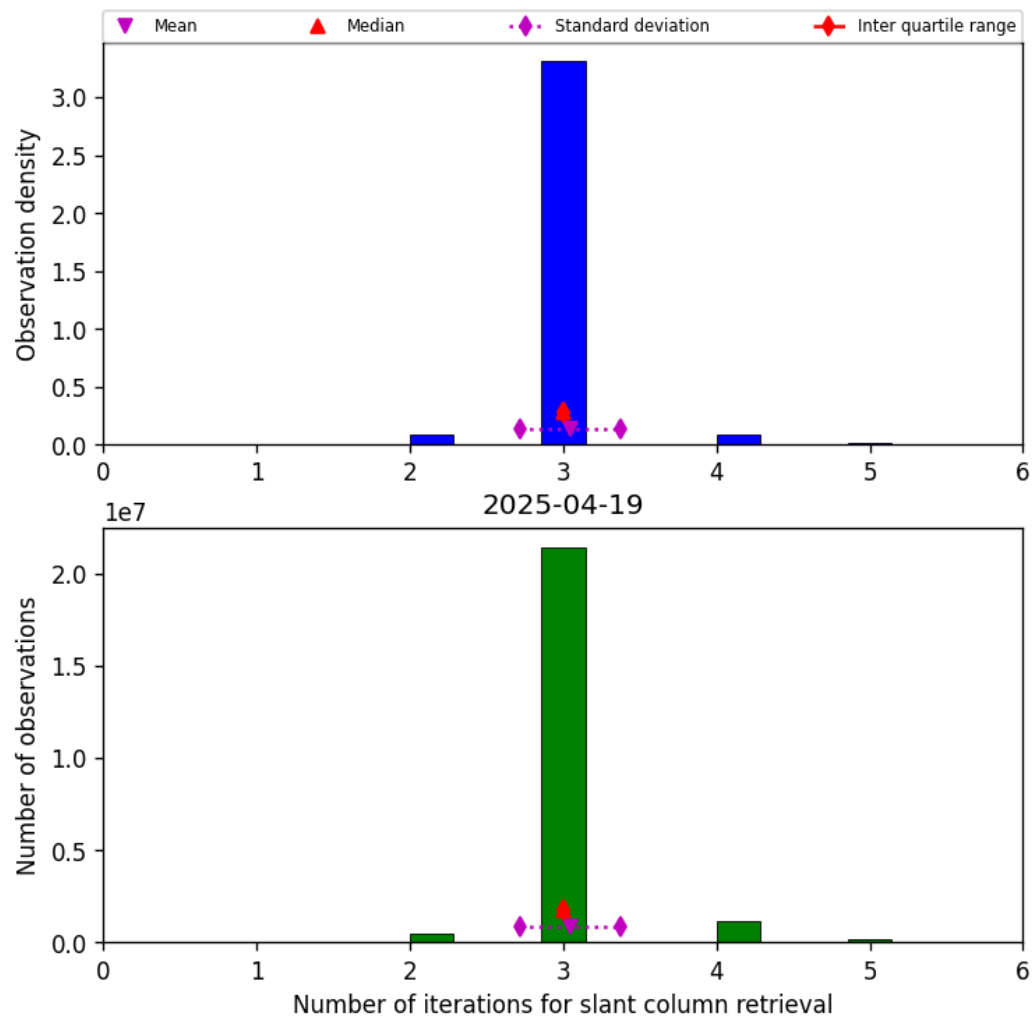
Figure 33: Histogram of “Number of iterations for slant column retrieval” for 2025-04-19 to 2025-04-20
