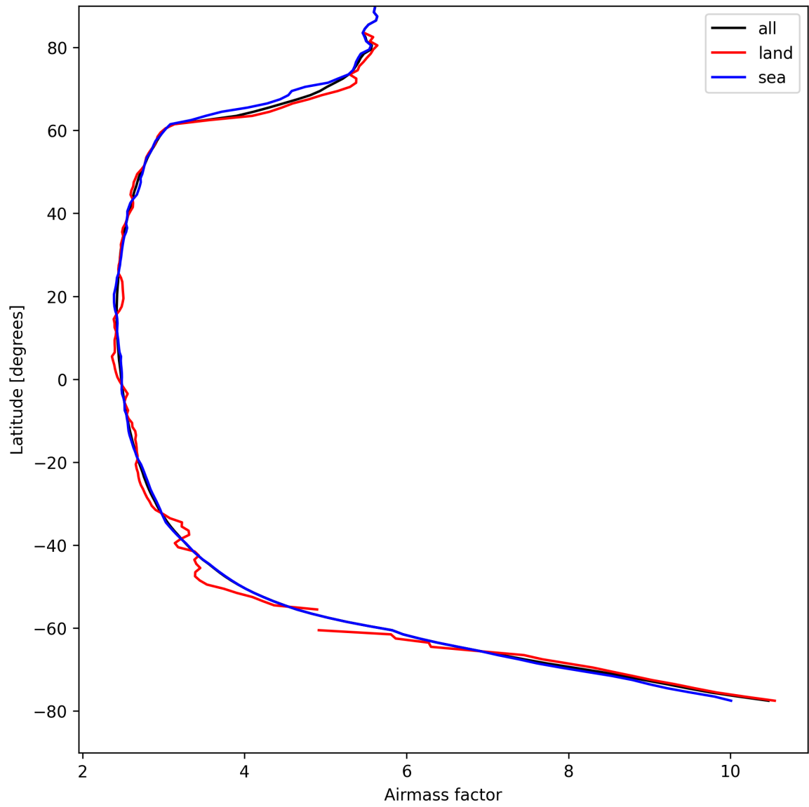
Figure 25: Zonal average of “Airmass factor” for 2025-04-19 to 2025-04-20.
