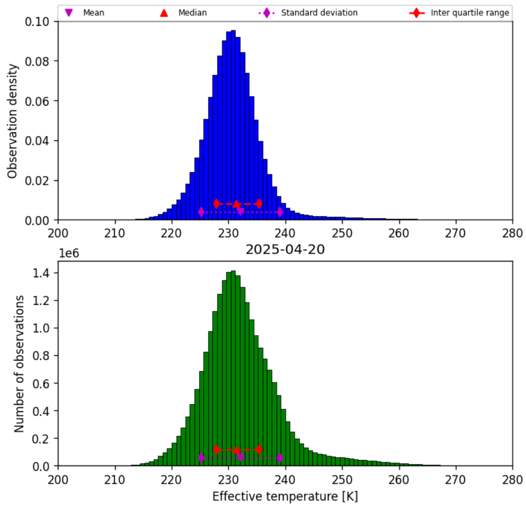
Figure 38: Histogram of “Effective temperature” for 2025-04-20 to 2025-04-21
