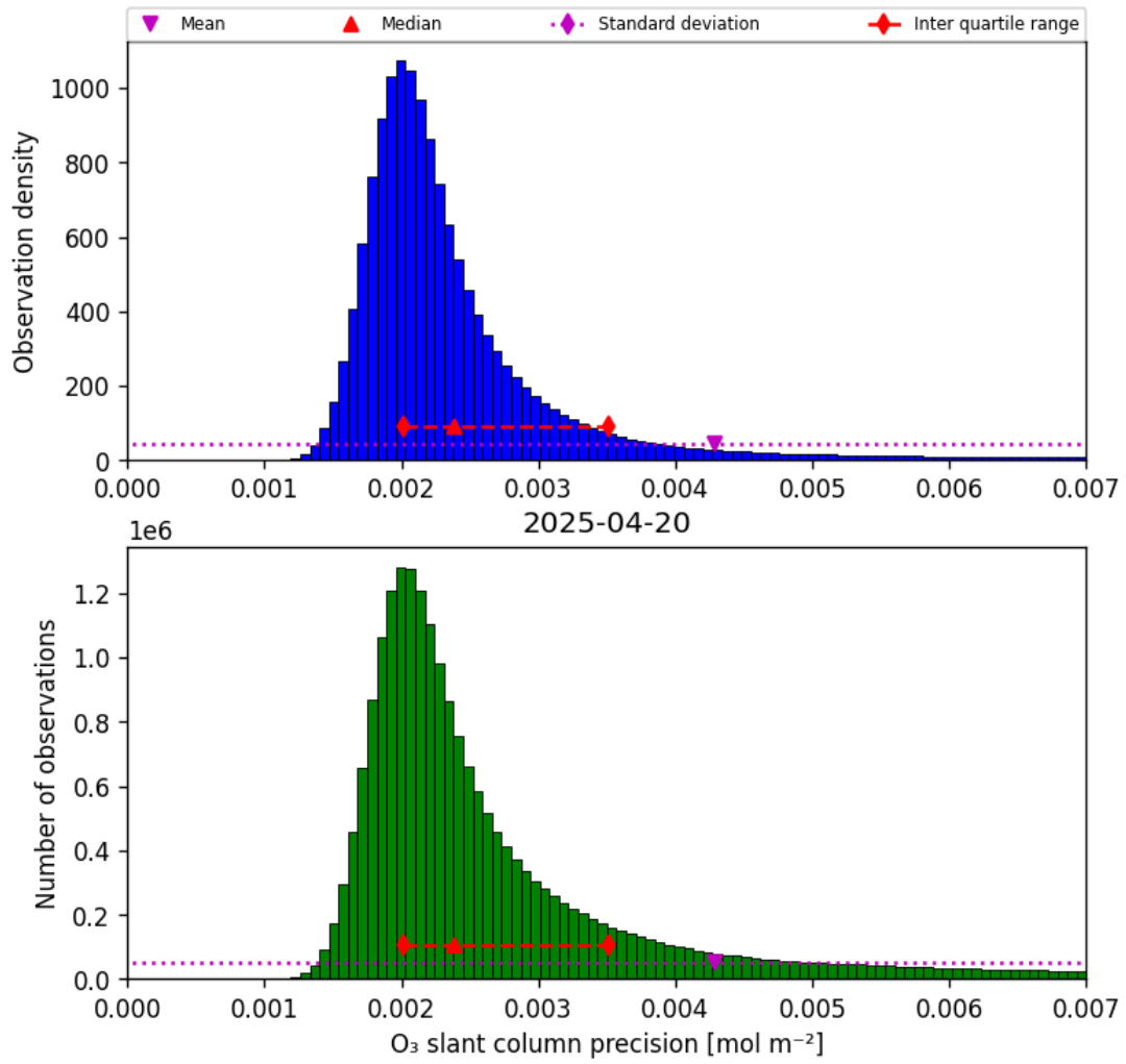
Figure 32: Histogram of “O 3 slant column precision” for 2025-04-20 to 2025-04-21
