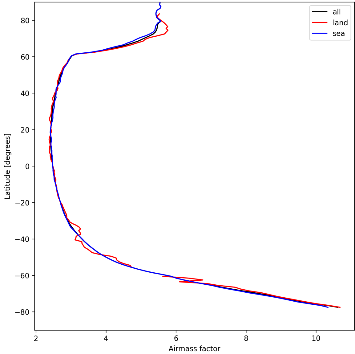
Figure 25: Zonal average of “Airmass factor” for 2025-04-20 to 2025-04-21.
