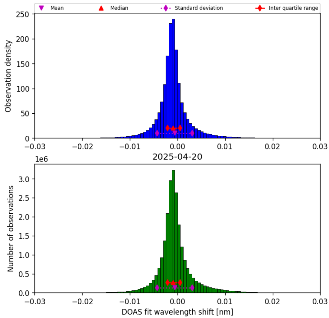
Figure 35: Histogram of “DOAS fit wavelength shift” for 2025-04-20 to 2025-04-21
