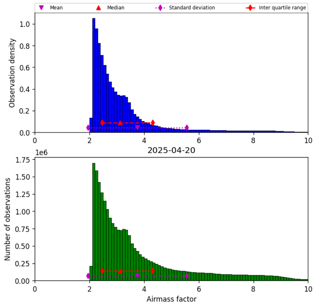
Figure 37: Histogram of “Airmass factor” for 2025-04-20 to 2025-04-21
