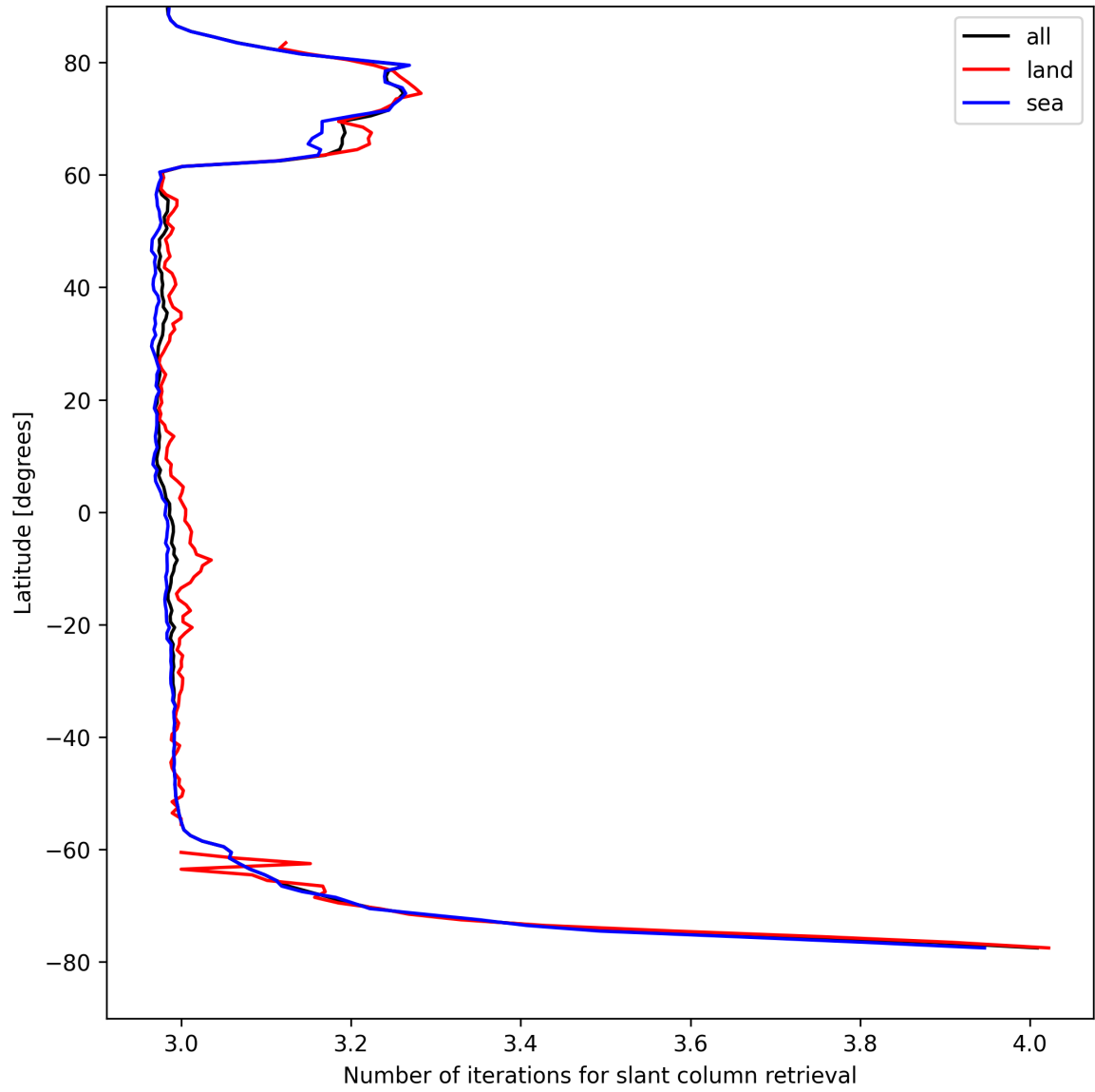
Figure 21: Zonal average of “Number of iterations for slant column retrieval” for 2025-04-20 to 2025-04-21.
