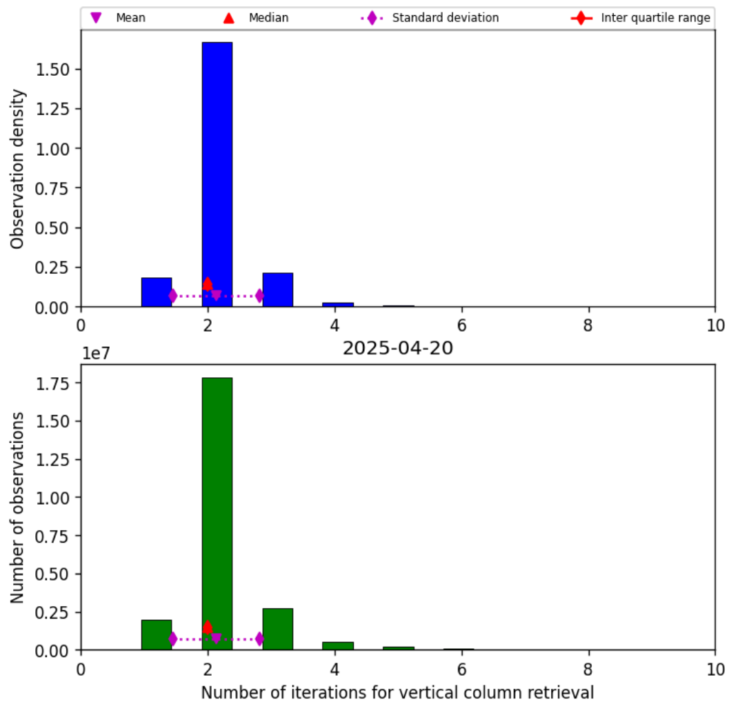
Figure 39: Histogram of “Number of iterations for vertical column retrieval” for 2025-04-20 to 2025-04-21
