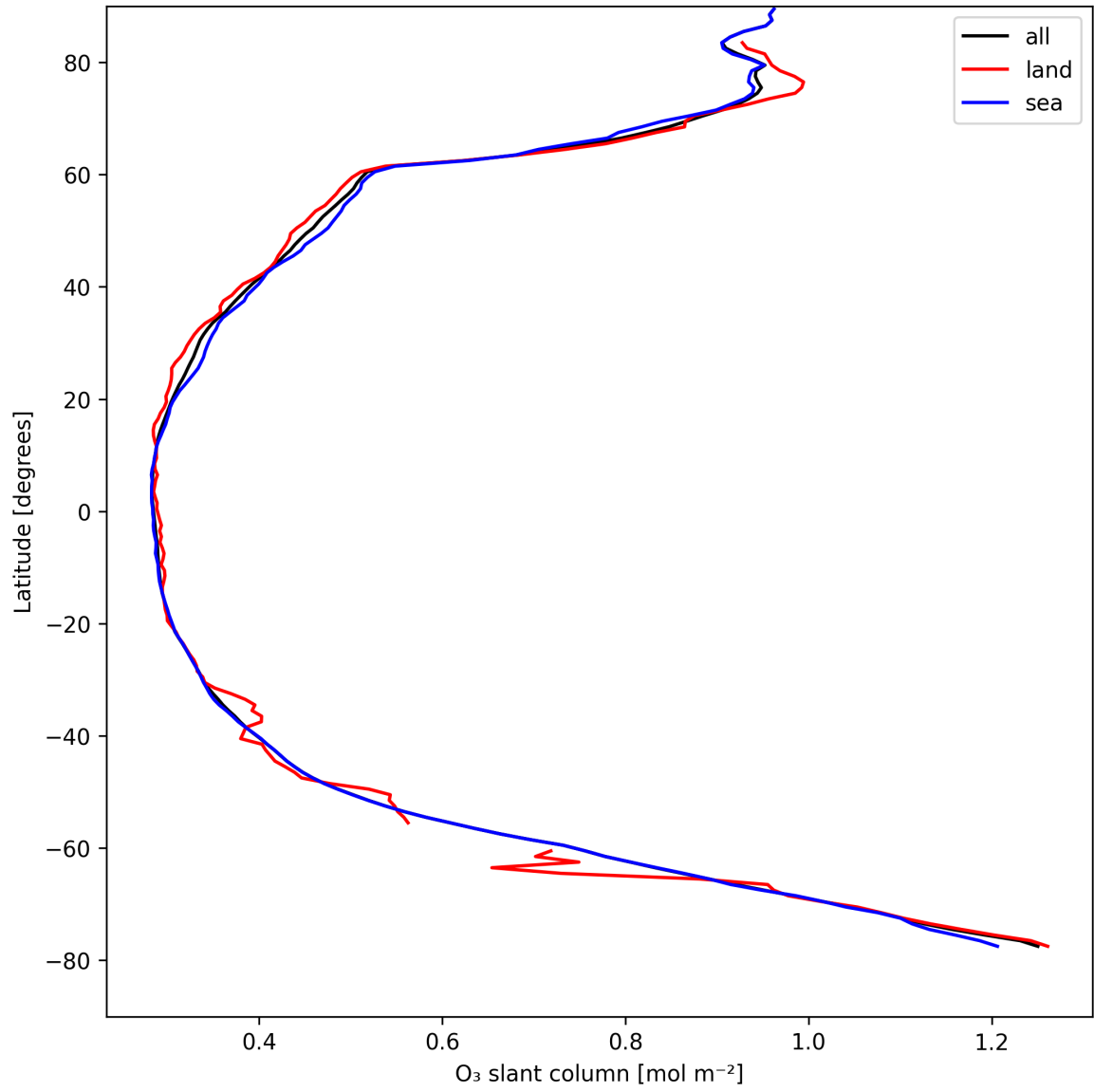
Figure 19: Zonal average of “O 3 slant column” for 2025-04-20 to 2025-04-21.
