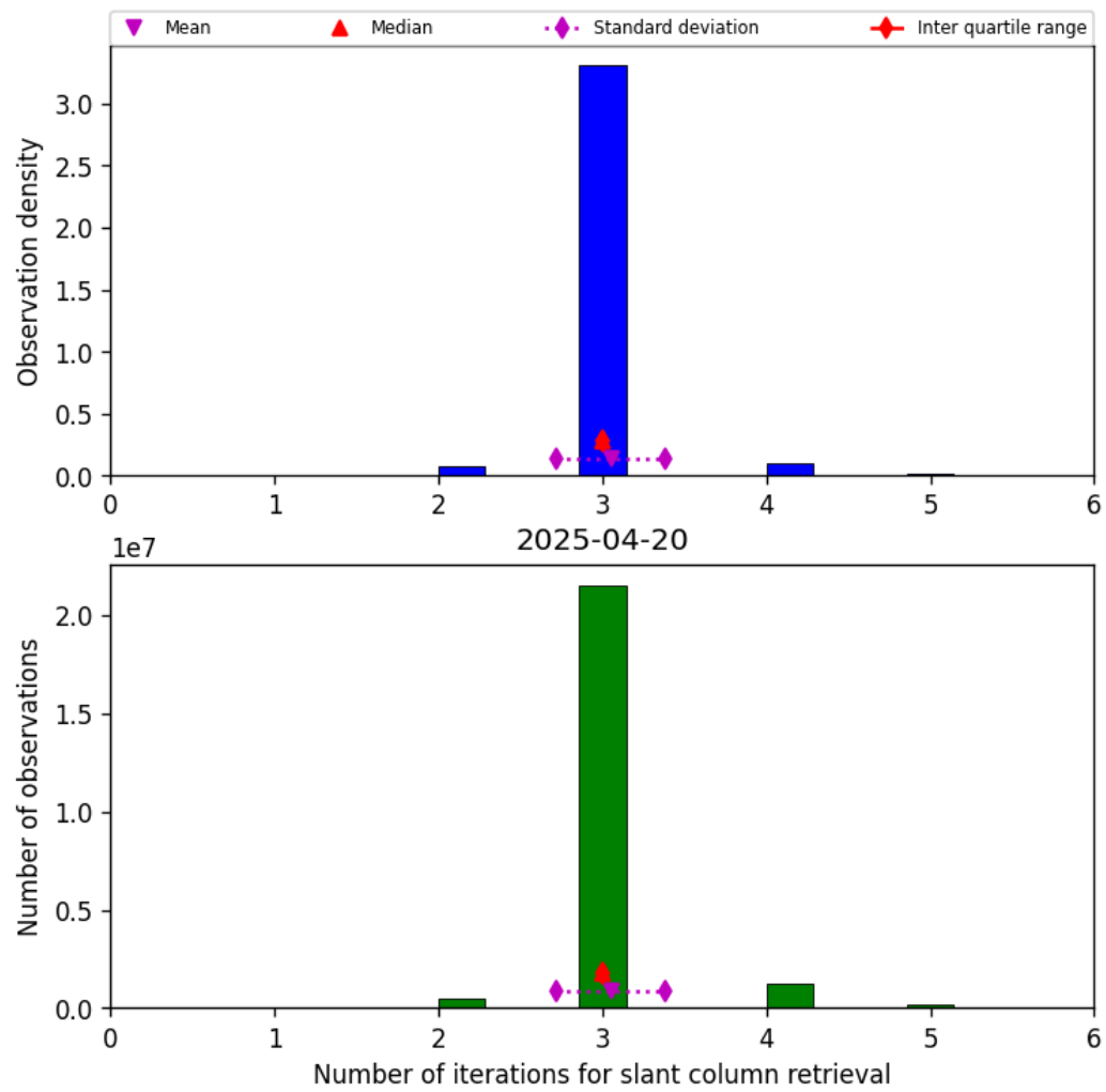
Figure 33: Histogram of "Number of iterations for slant column retrieval" for 2025-04-20 to 2025-04-21
