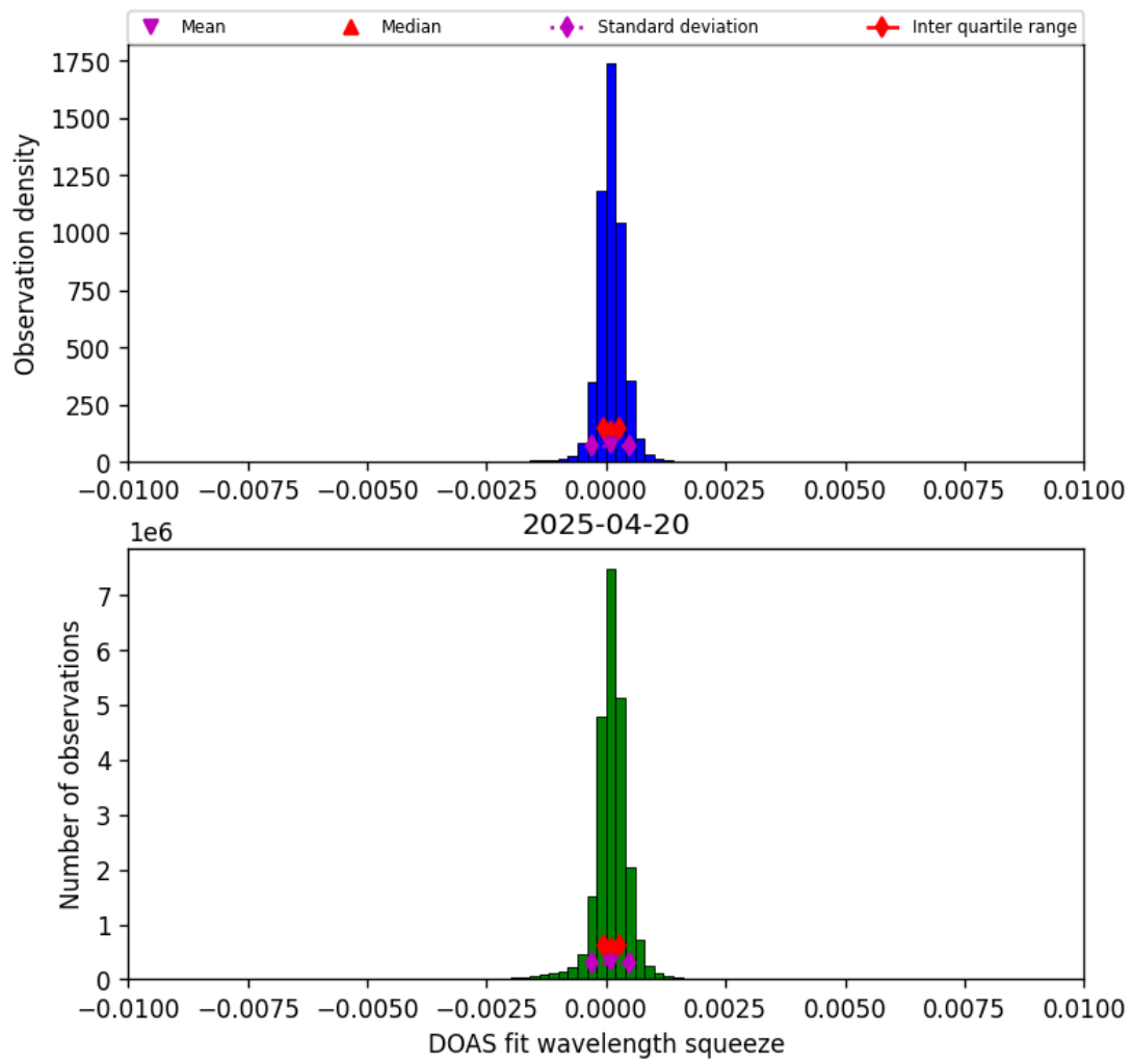
Figure 36: Histogram of “DOAS fit wavelength squeeze” for 2025-04-20 to 2025-04-21
