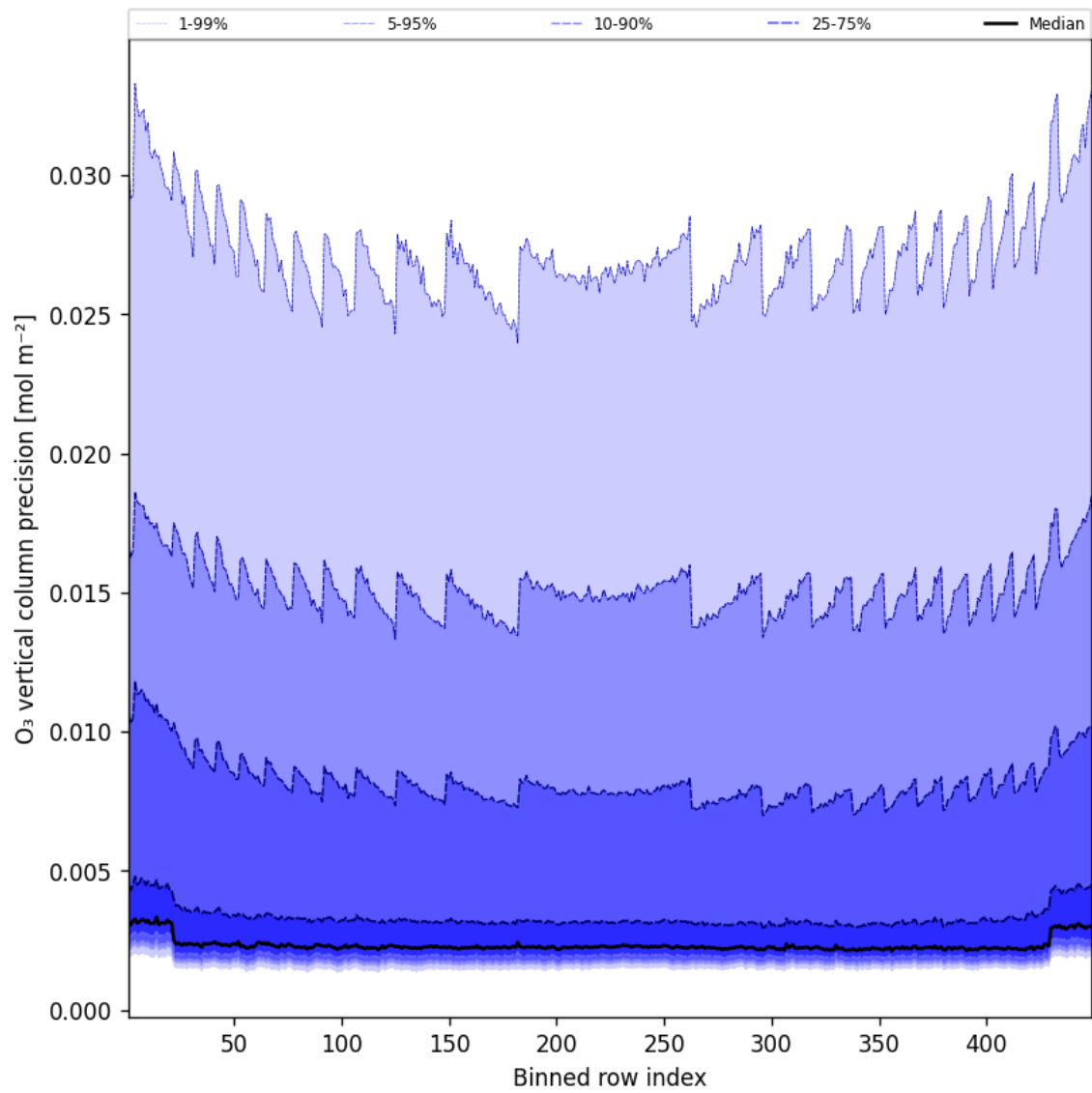
Figure 42: Along track statistics of “O 3 vertical column precision” for 2025-04-20 to 2025-04-21
