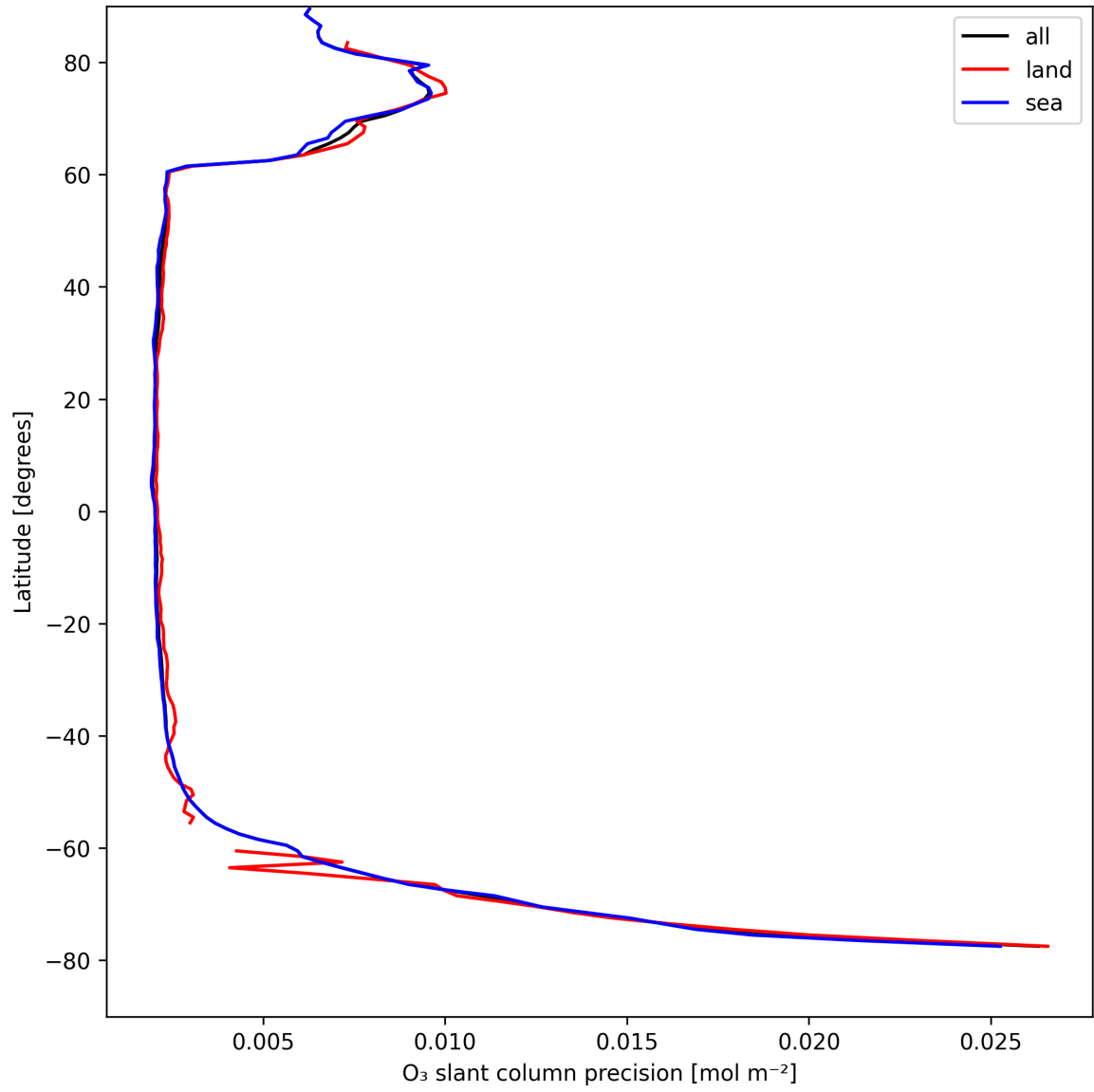
Figure 20: Zonal average of “O 3 slant column precision” for 2025-04-20 to 2025-04-21.
