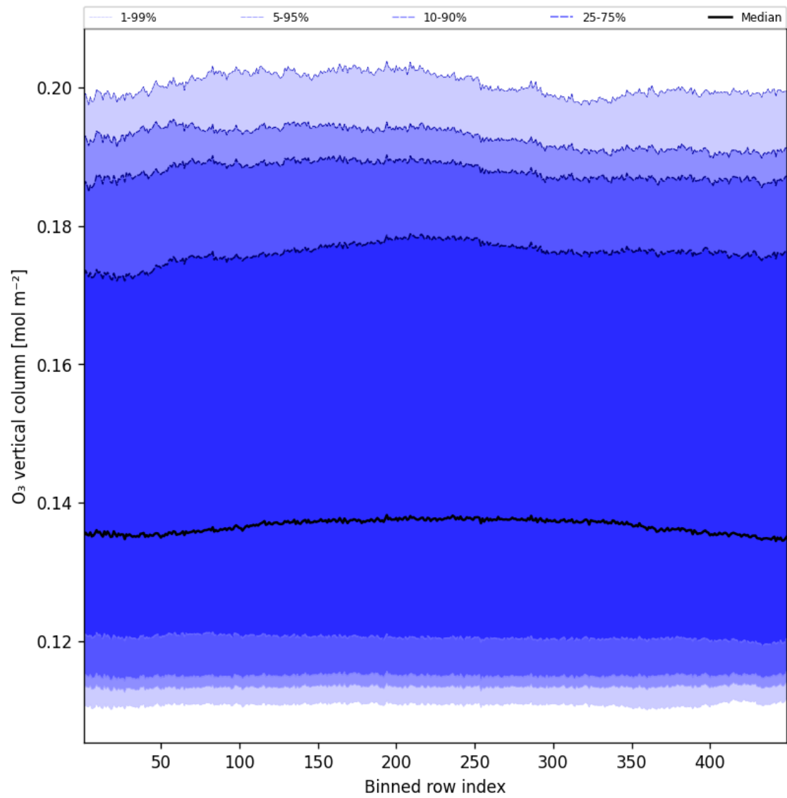
Figure 41: Along track statistics of “O 3 vertical column” for 2025-04-20 to 2025-04-21
