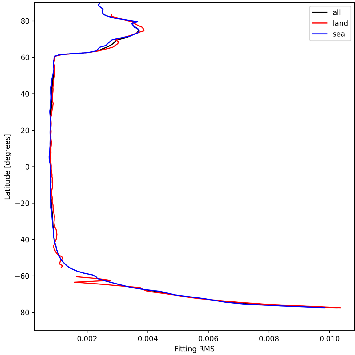
Figure 22: Zonal average of “Fitting RMS” for 2025-04-20 to 2025-04-21.
