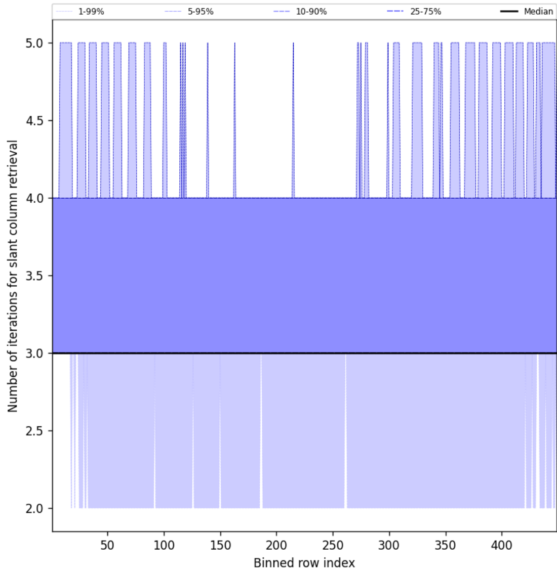
Figure 45: Along track statistics of “Number of iterations for slant column retrieval” for 2025-04-20 to 2025-04-21
