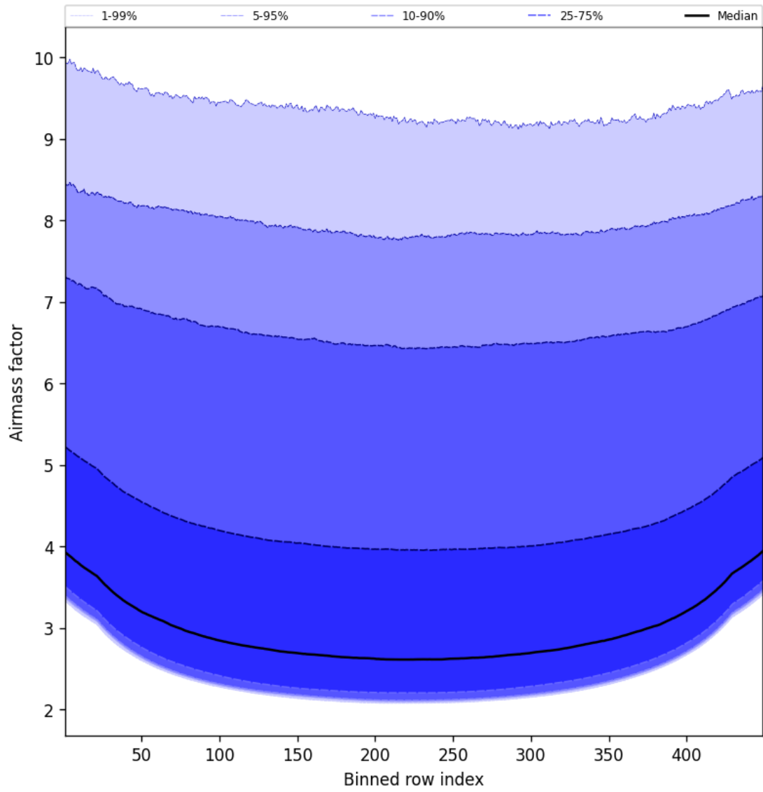
Figure 49: Along track statistics of “Airmass factor” for 2025-04-20 to 2025-04-21
