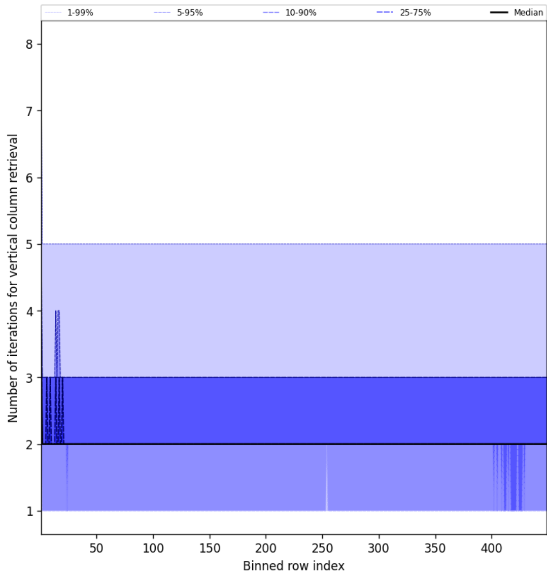
Figure 51: Along track statistics of “Number of iterations for vertical column retrieval” for 2025-04-20 to 2025-04-21
