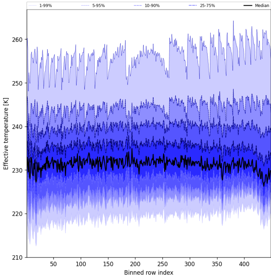
Figure 50: Along track statistics of "Effective temperature" for 2025-04-20 to 2025-04-21
