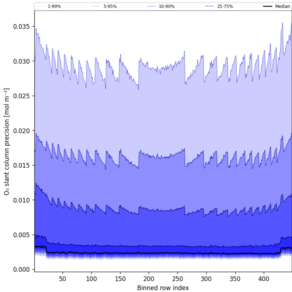
Figure 44: Along track statistics of “O 3 slant column precision” for 2025-04-20 to 2025-04-21
