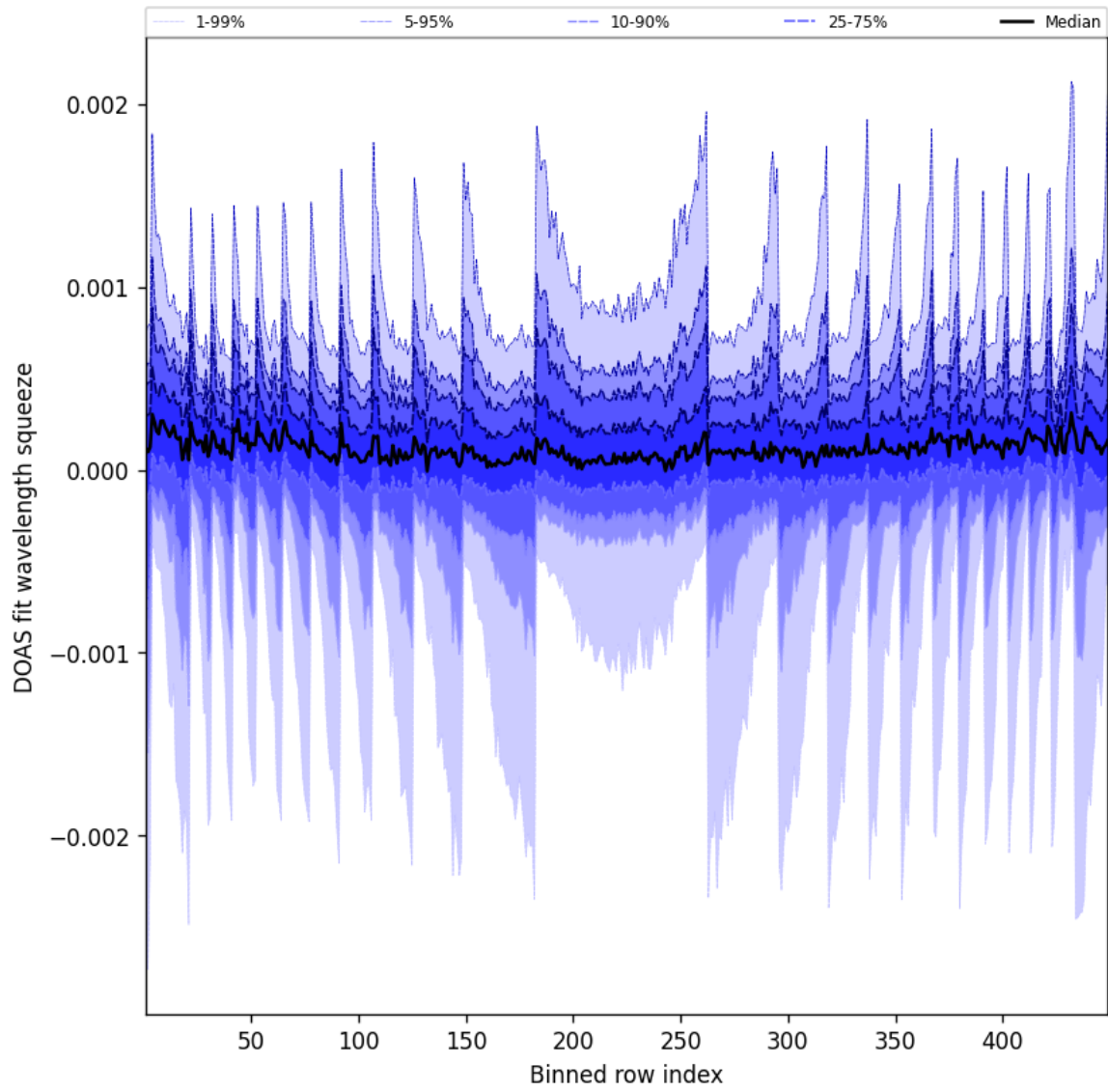
Figure 48: Along track statistics of “DOAS fit wavelength squeeze” for 2025-04-20 to 2025-04-21
