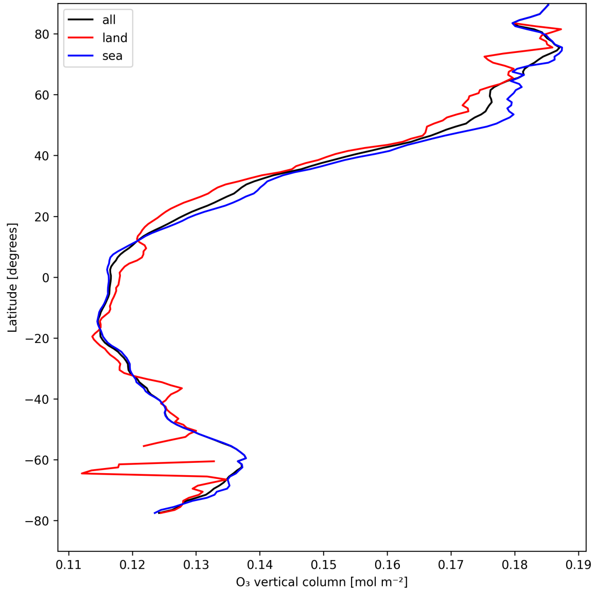
Figure 17: Zonal average of “O 3 vertical column” for 2025-04-20 to 2025-04-21.
