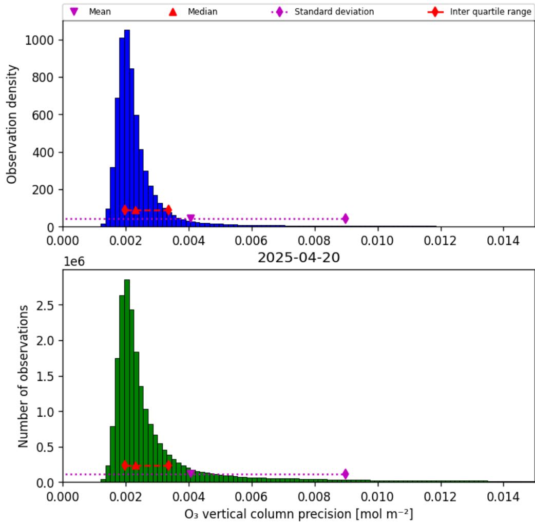
Figure 30: Histogram of “O 3 vertical column precision” for 2025-04-20 to 2025-04-21
