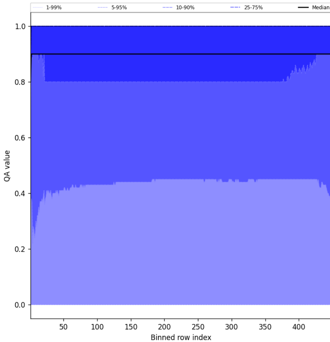
Figure 40: Along track statistics of “QA value” for 2025-04-20 to 2025-04-21
