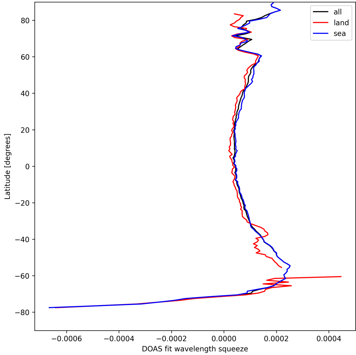
Figure 24: Zonal average of “DOAS fit wavelength squeeze” for 2025-04-20 to 2025-04-21.
