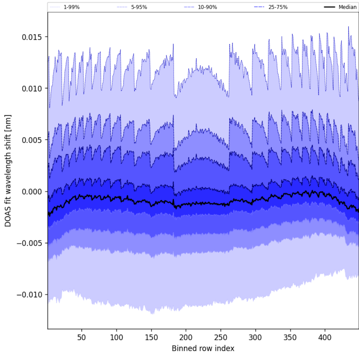
Figure 47: Along track statistics of “DOAS fit wavelength shift” for 2025-04-20 to 2025-04-21
