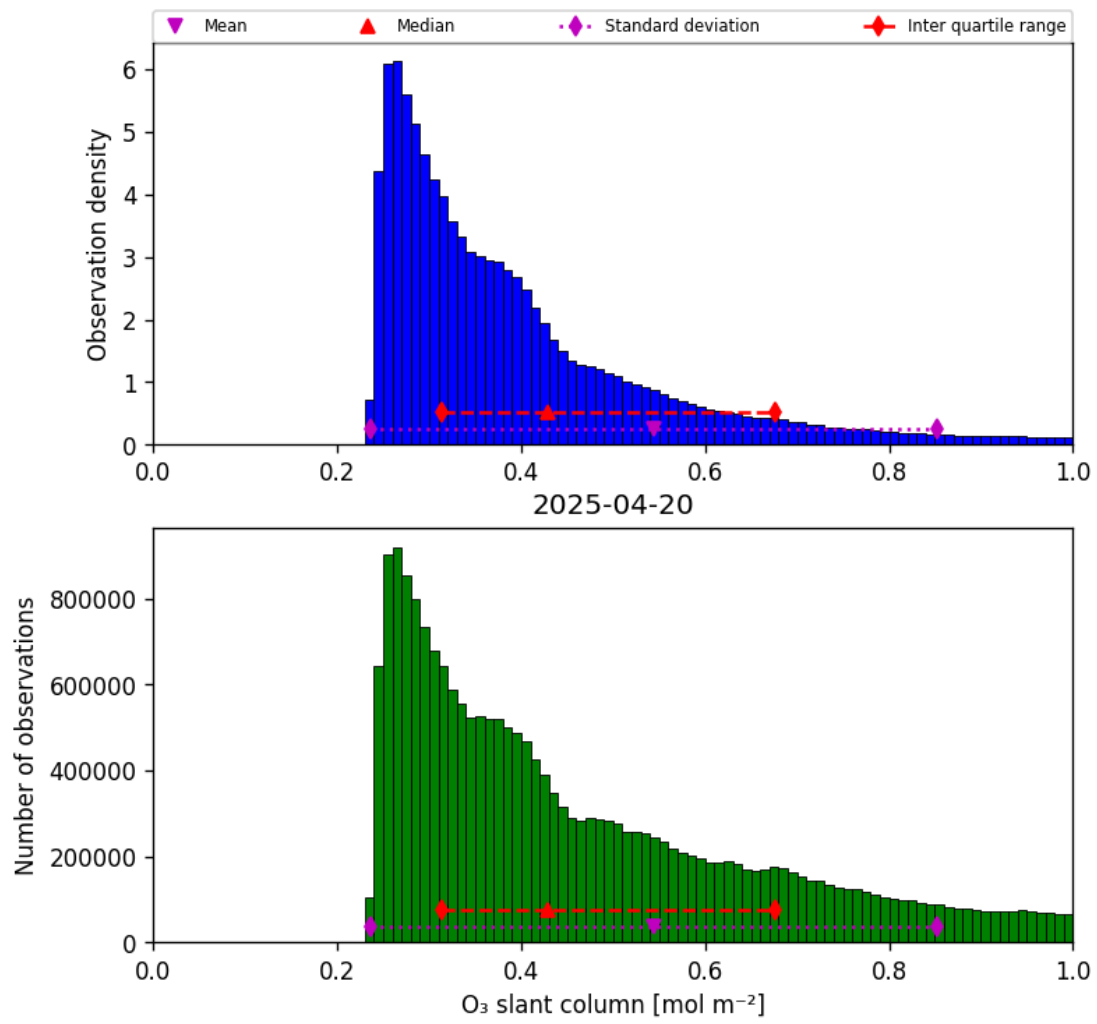
Figure 31: Histogram of “O 3 slant column” for 2025-04-20 to 2025-04-21
