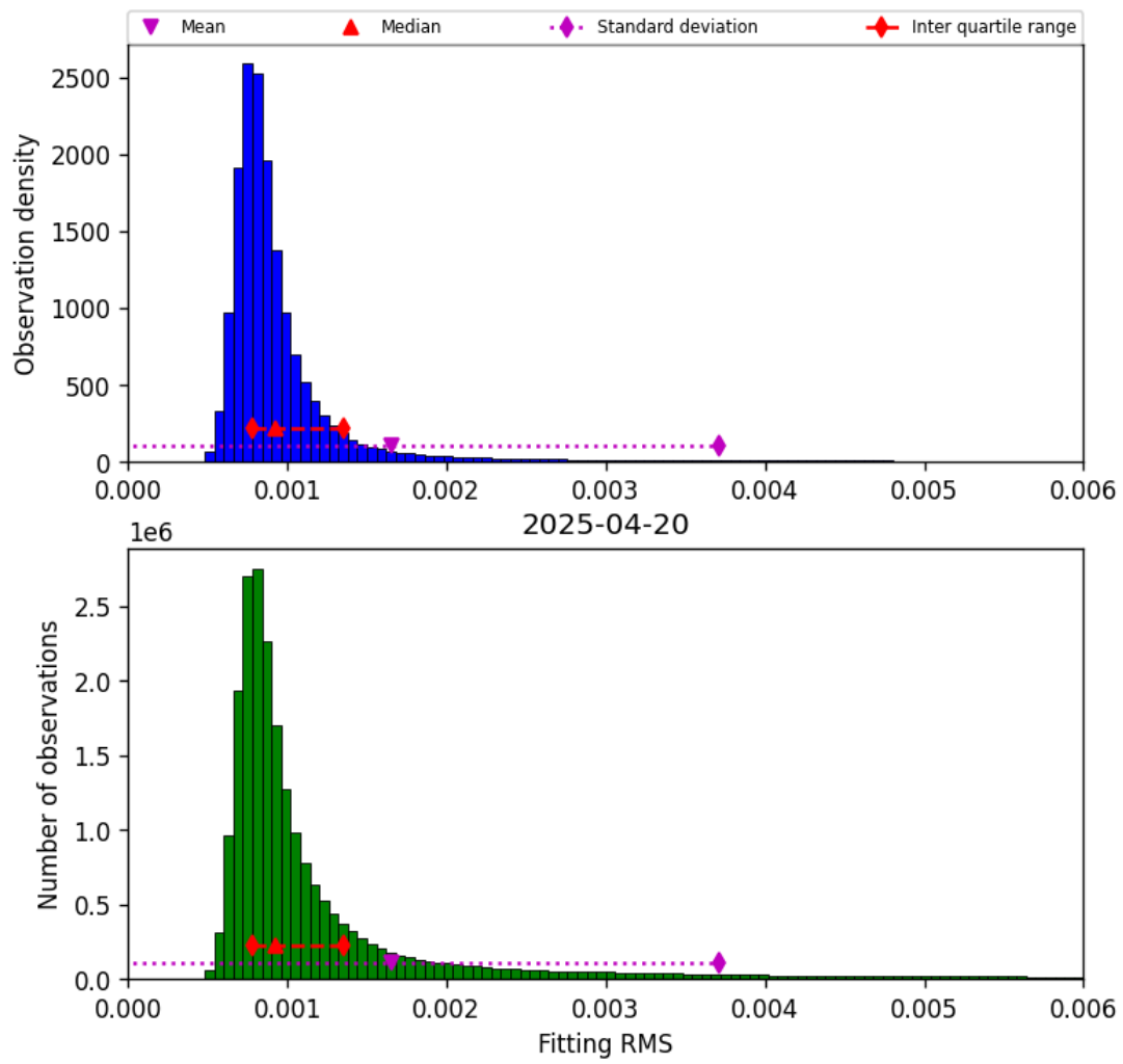
Figure 34: Histogram of “Fitting RMS” for 2025-04-20 to 2025-04-21
