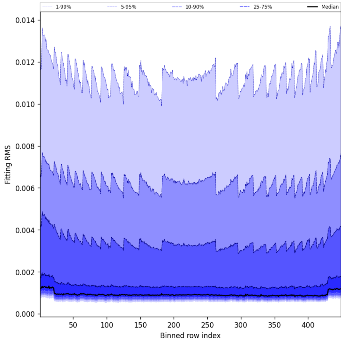
Figure 46: Along track statistics of “Fitting RMS” for 2025-04-20 to 2025-04-21
