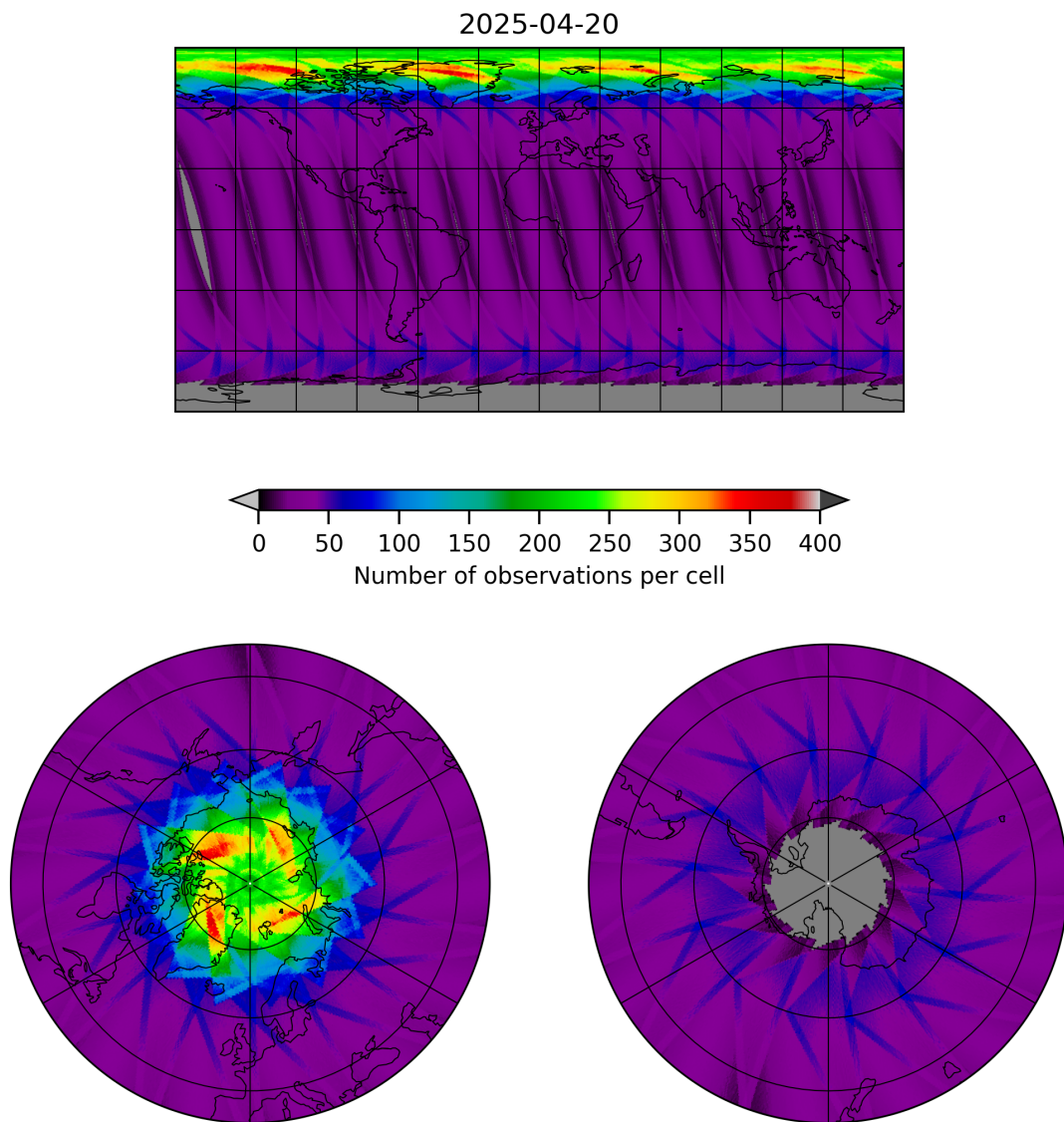
Figure 15: Map of the number of observations for 2025-04-20 to 2025-04-21
