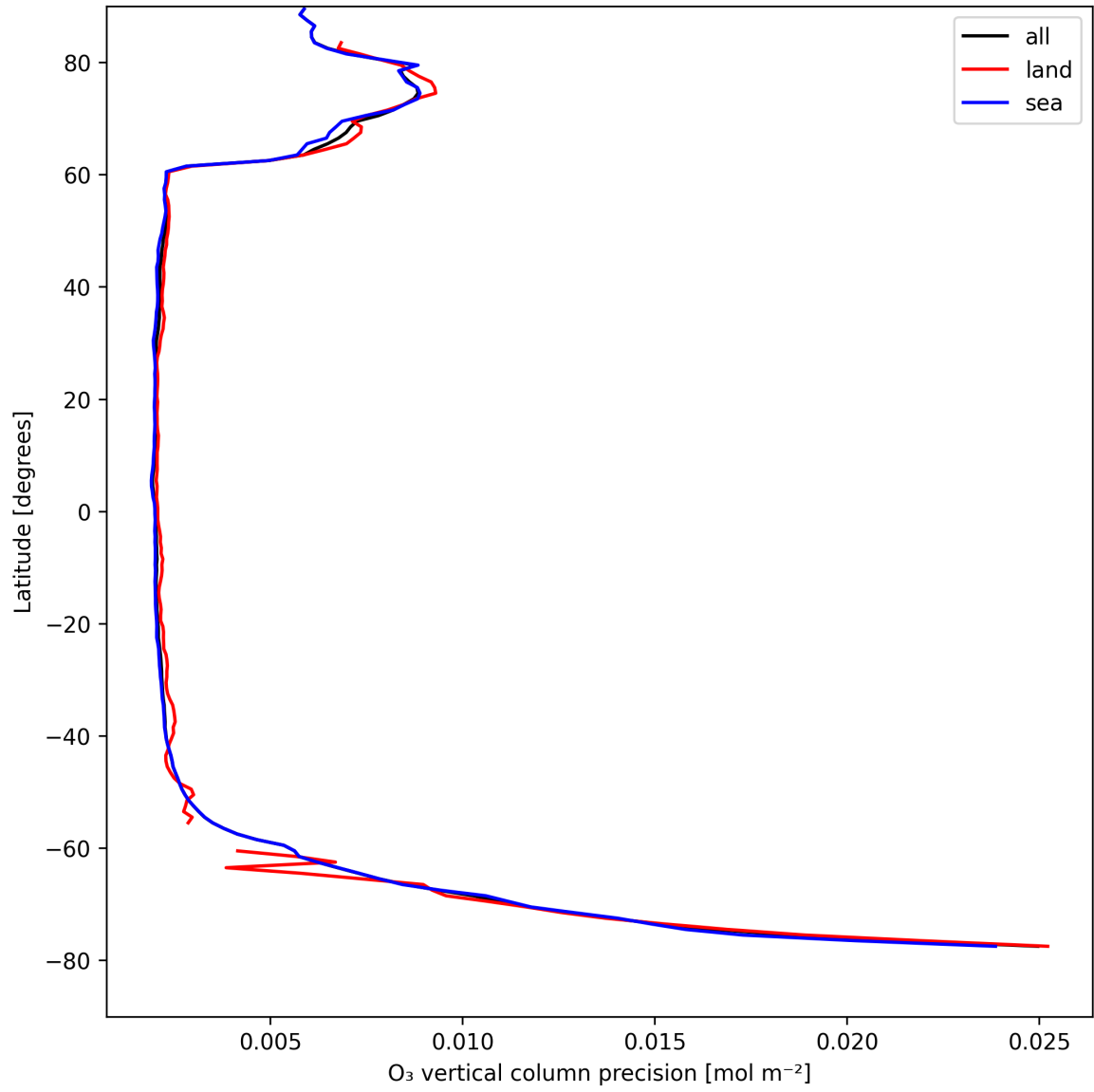
Figure 18: Zonal average of “O 3 vertical column precision” for 2025-04-20 to 2025-04-21.
