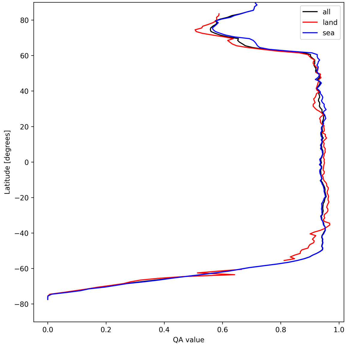
Figure 16: Zonal average of “QA value” for 2025-04-20 to 2025-04-21.
