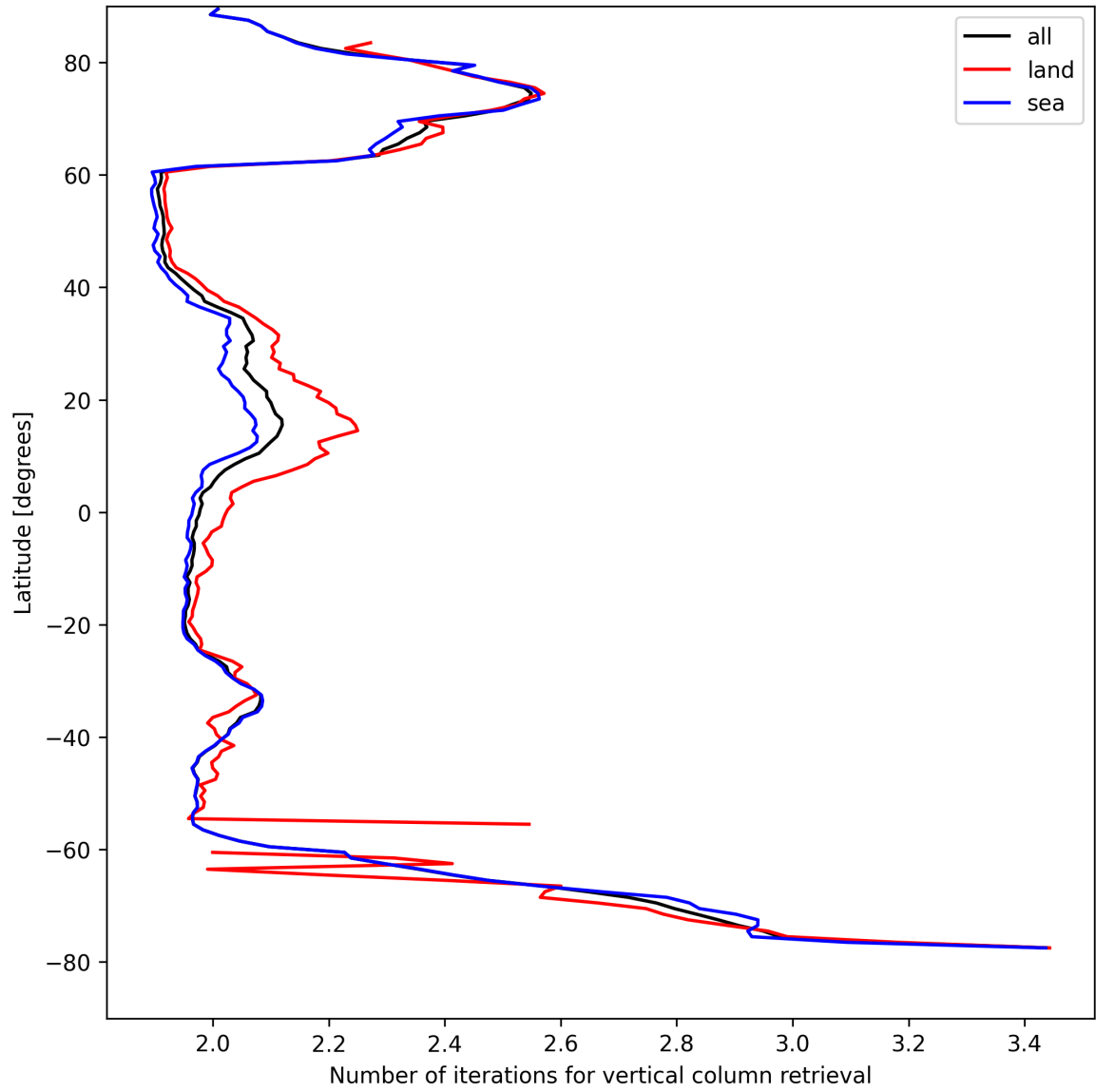
Figure 27: Zonal average of “Number of iterations for vertical column retrieval” for 2025-04-20 to 2025-04-21.
