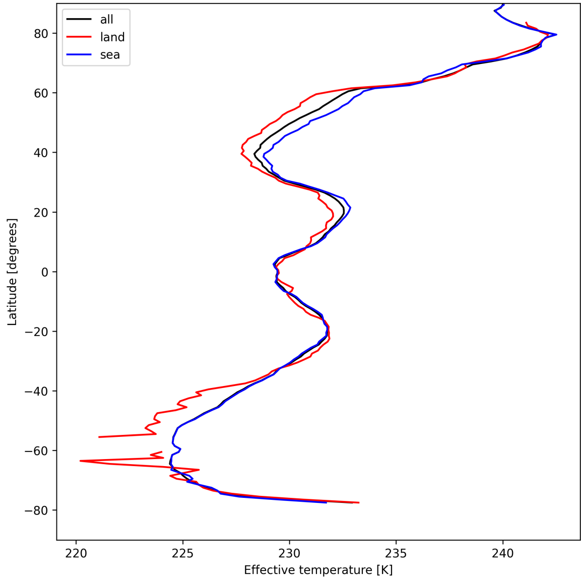
Figure 26: Zonal average of “Effective temperature” for 2025-04-20 to 2025-04-21.
