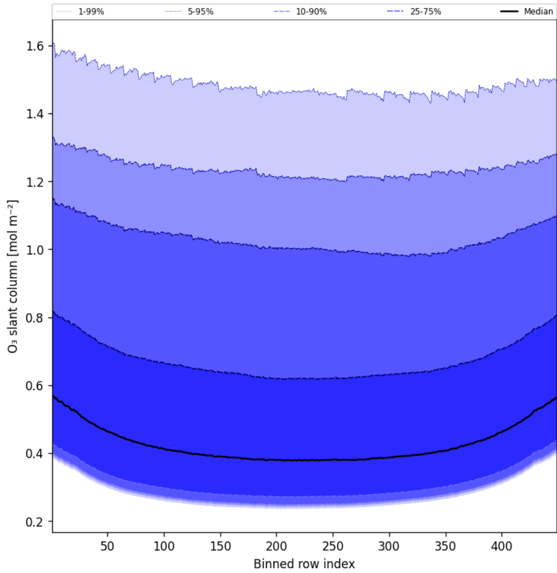
Figure 43: Along track statistics of “O 3 slant column” for 2025-04-20 to 2025-04-21
