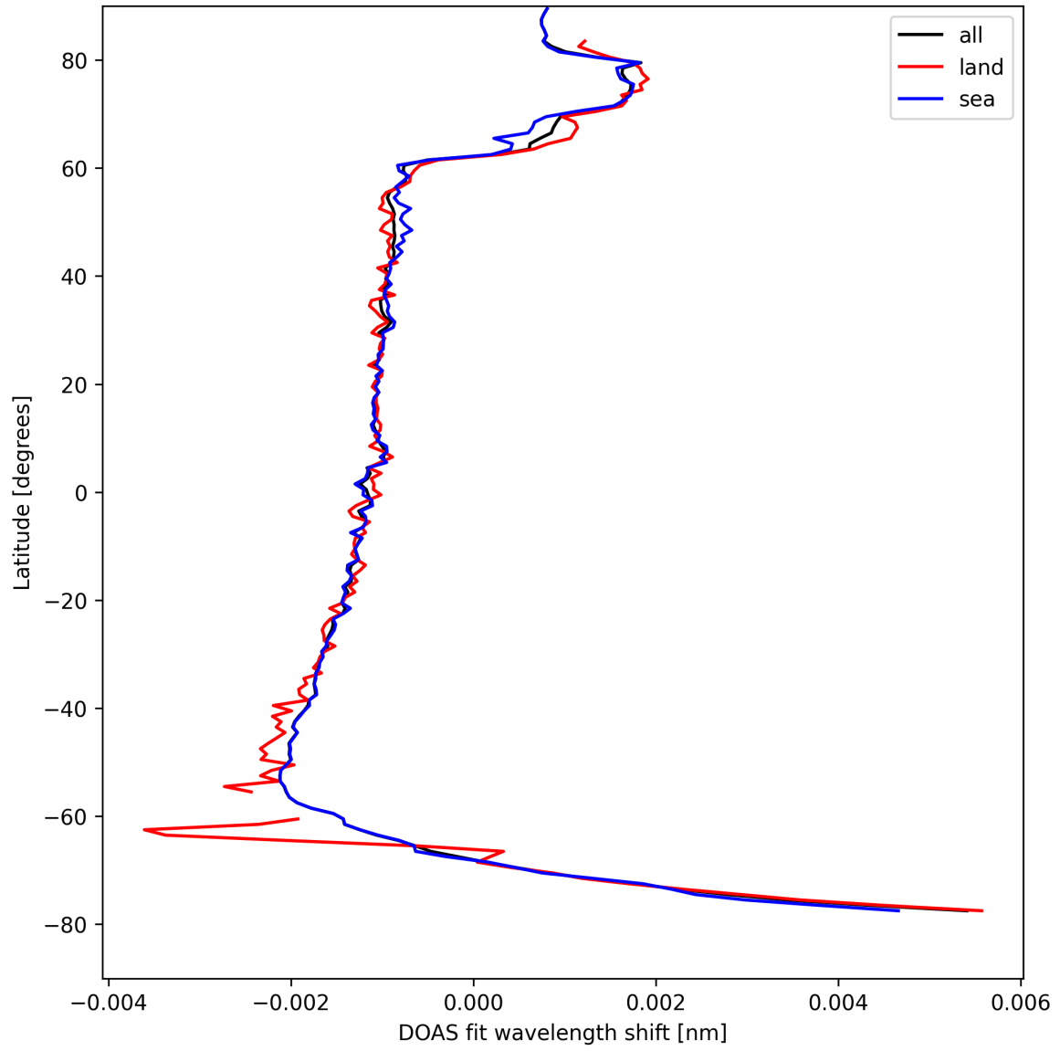
Figure 23: Zonal average of “DOAS fit wavelength shift” for 2025-04-20 to 2025-04-21.
