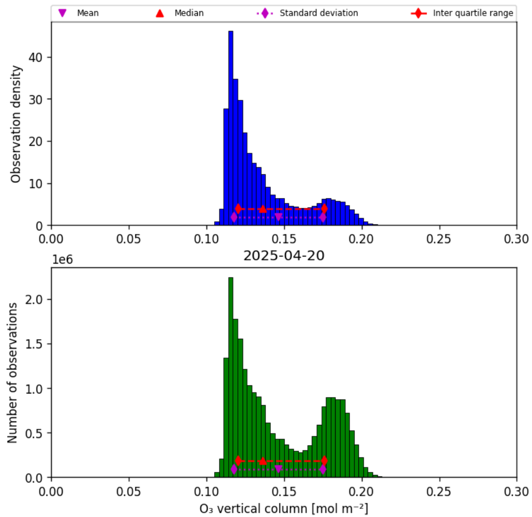
Figure 29: Histogram of “O 3 vertical column” for 2025-04-20 to 2025-04-21
