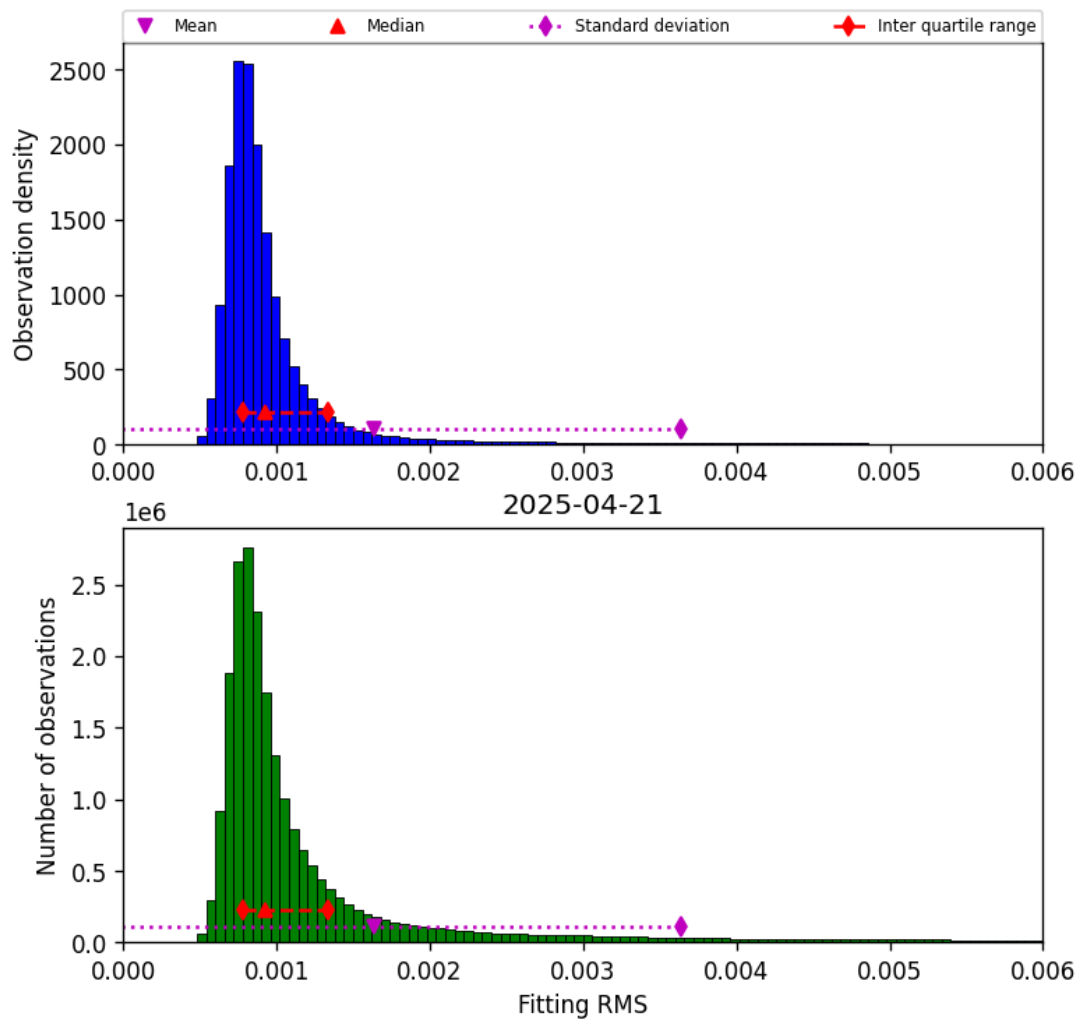
Figure 34: Histogram of “Fitting RMS” for 2025-04-21 to 2025-04-22
