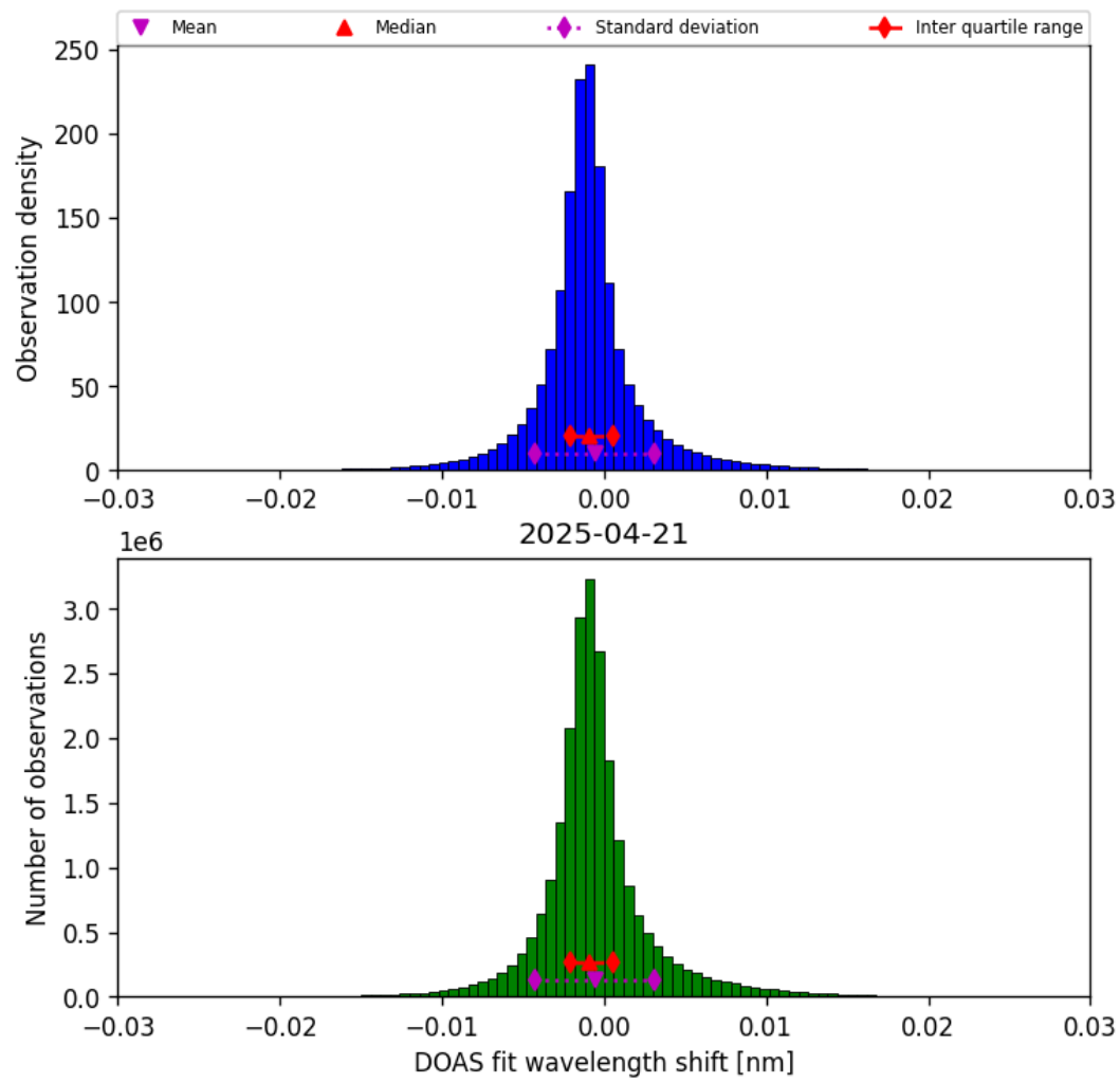
Figure 35: Histogram of “DOAS fit wavelength shift” for 2025-04-21 to 2025-04-22
