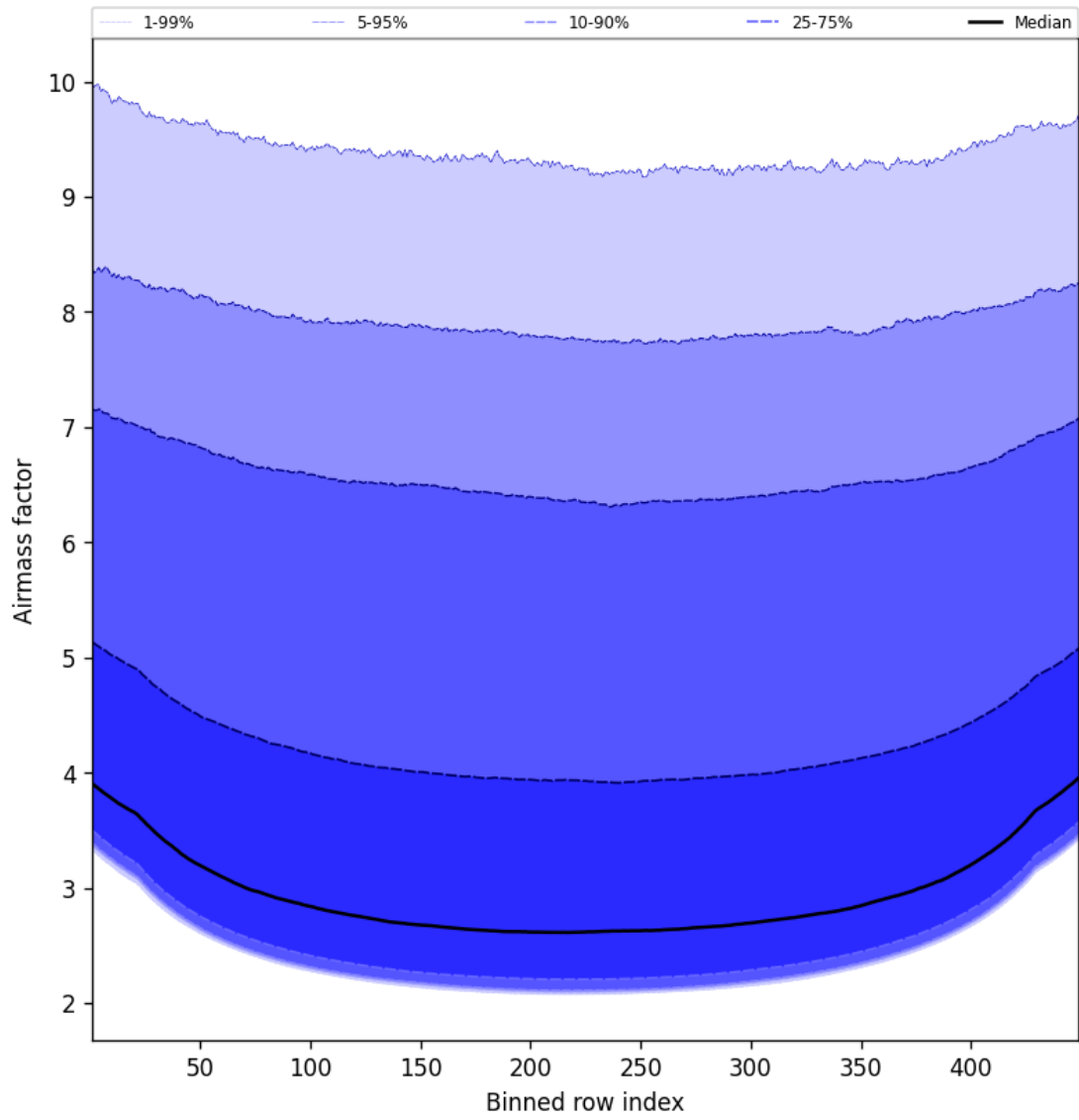
Figure 49: Along track statistics of “Airmass factor” for 2025-04-21 to 2025-04-22
