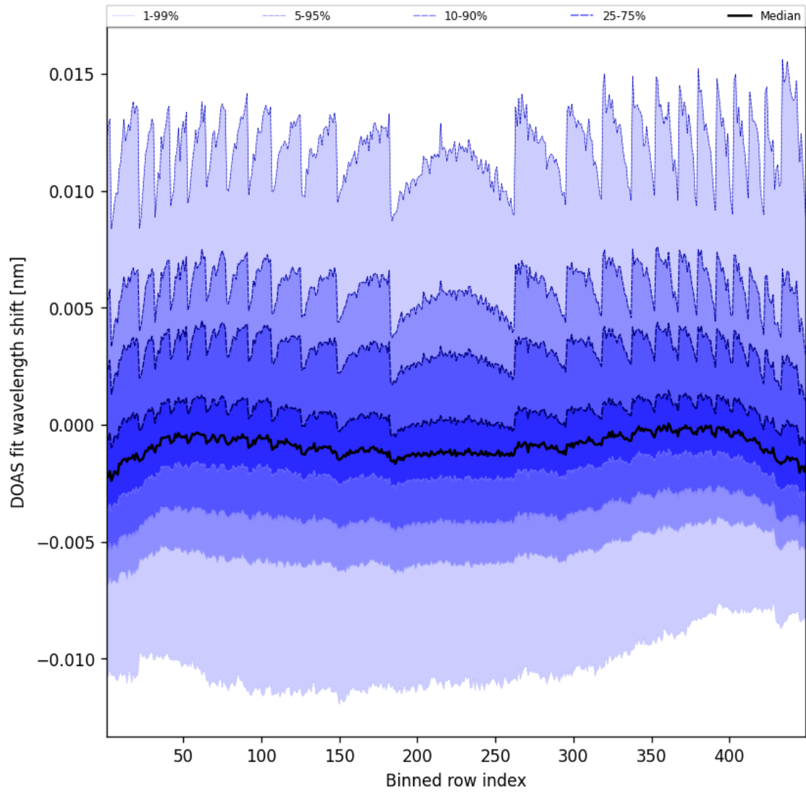
Figure 47: Along track statistics of “DOAS fit wavelength shift” for 2025-04-21 to 2025-04-22
