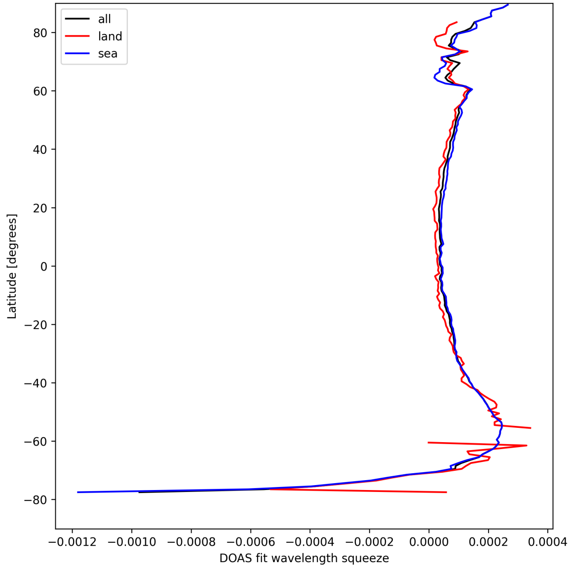
Figure 24: Zonal average of “DOAS fit wavelength squeeze” for 2025-04-21 to 2025-04-22.
