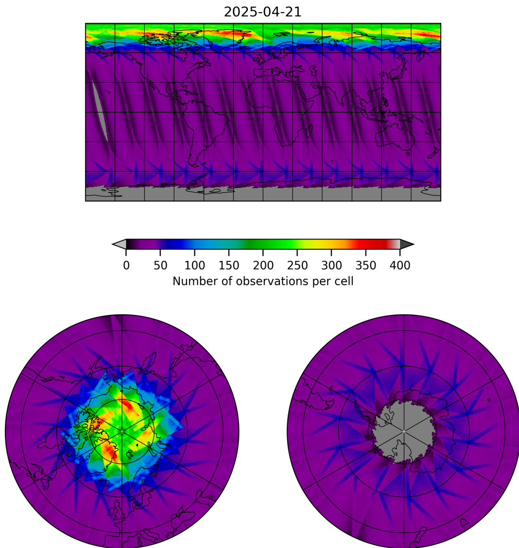
Figure 15: Map of the number of observations for 2025-04-21 to 2025-04-22
