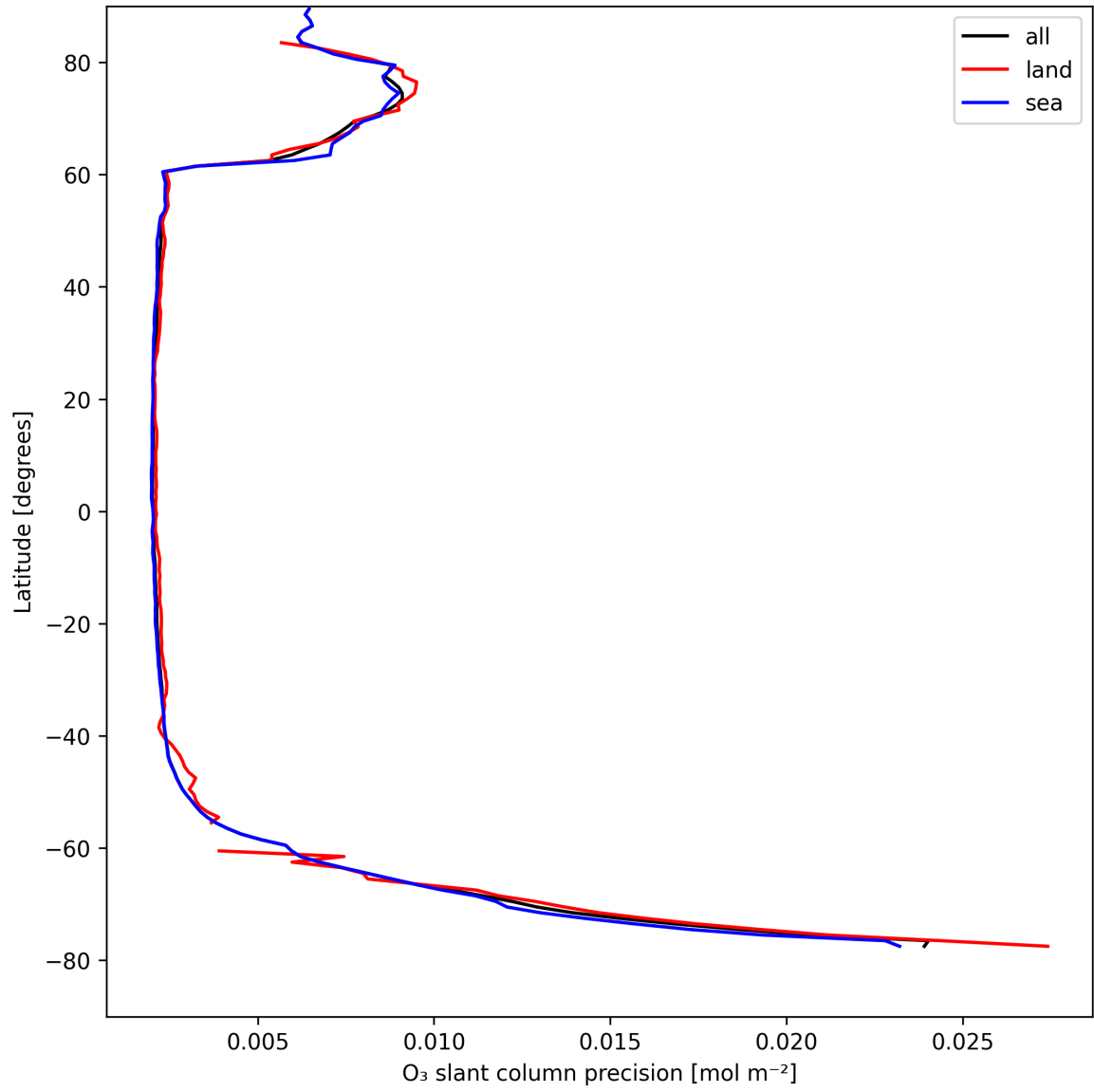
Figure 20: Zonal average of “O 3 slant column precision” for 2025-04-21 to 2025-04-22.
