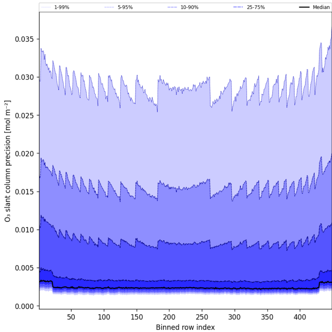
Figure 44: Along track statistics of “O 3 slant column precision” for 2025-04-21 to 2025-04-22
