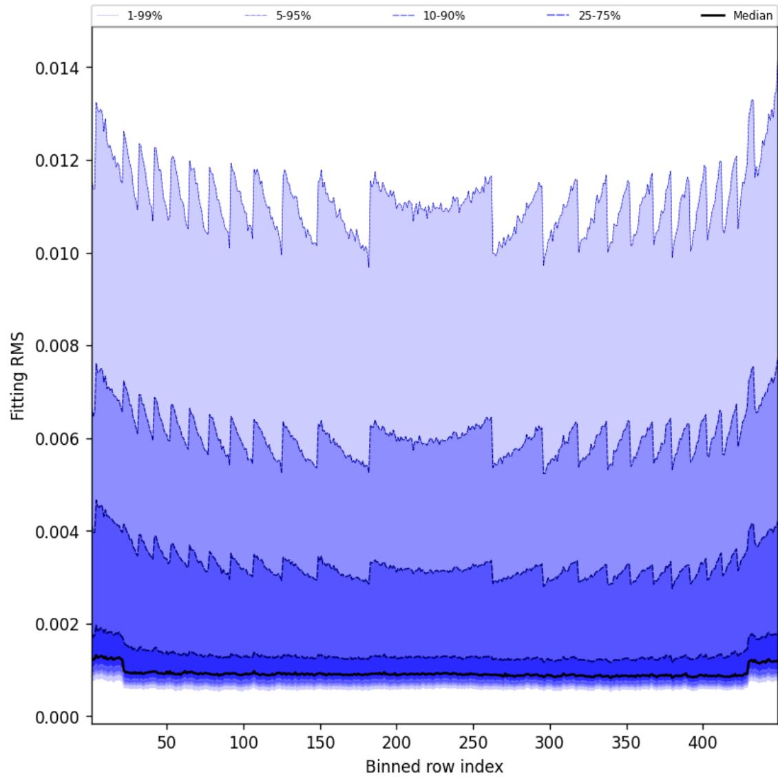
Figure 46: Along track statistics of “Fitting RMS” for 2025-04-21 to 2025-04-22
