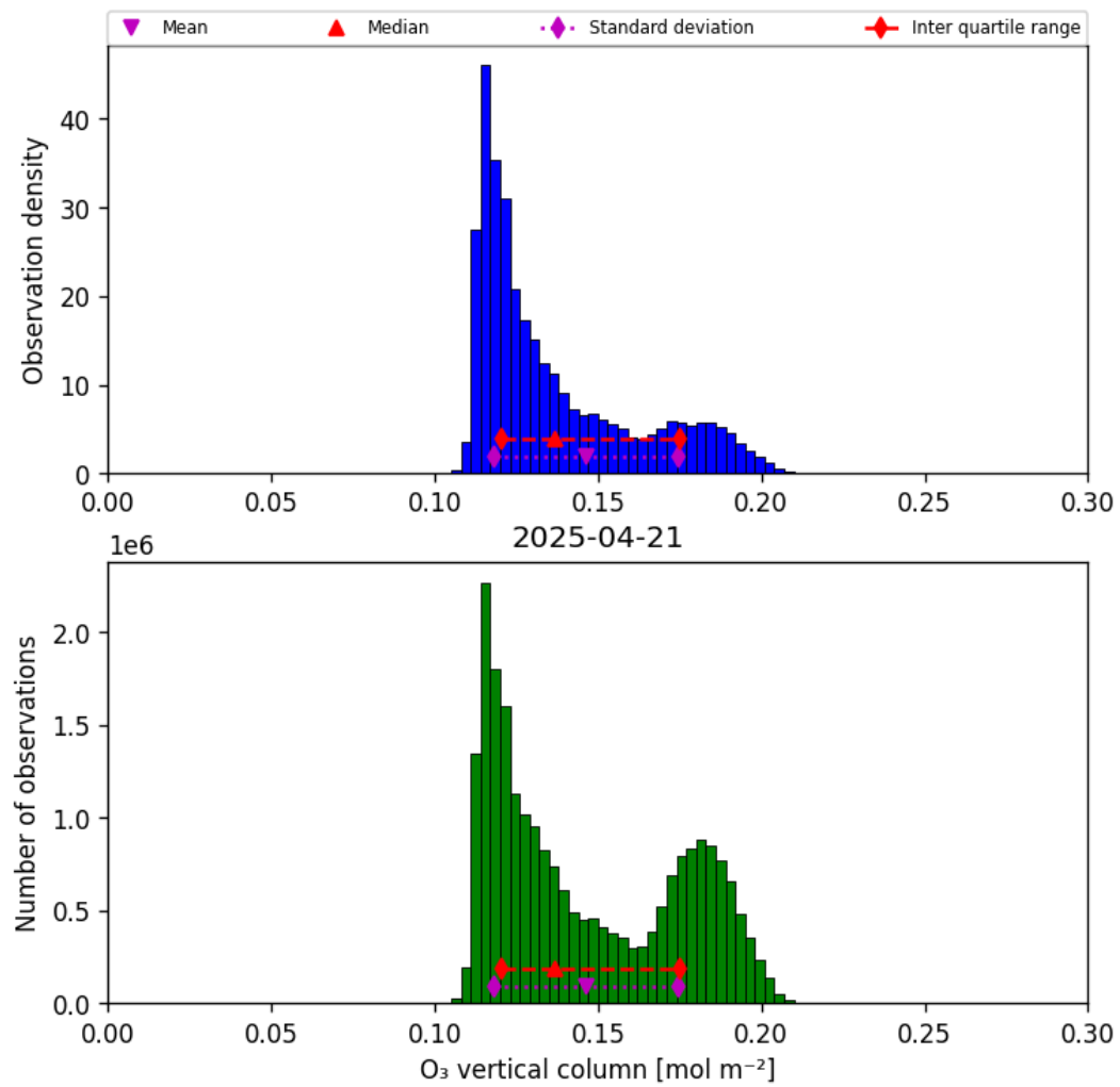
Figure 29: Histogram of “O 3 vertical column” for 2025-04-21 to 2025-04-22
