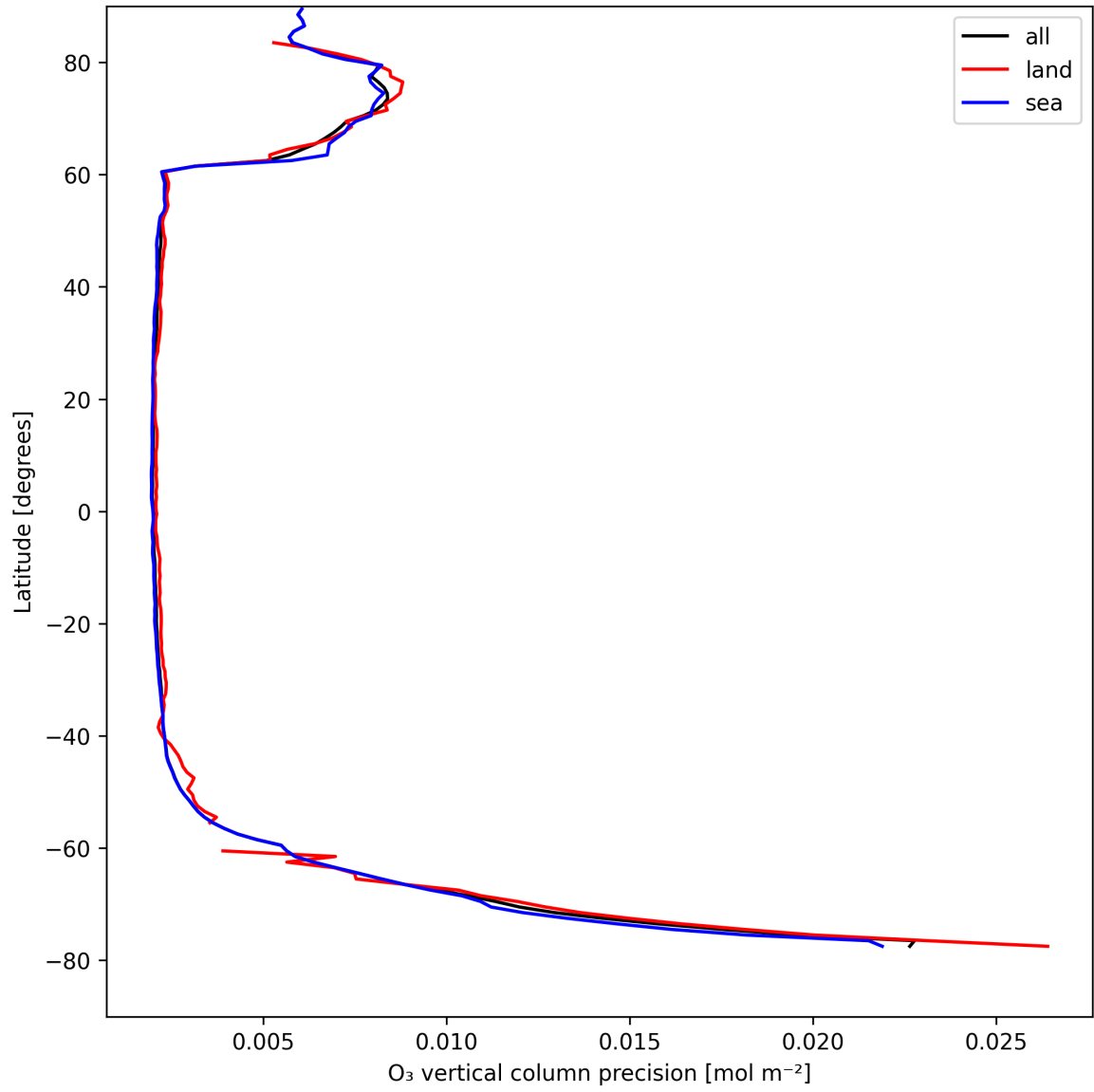
Figure 18: Zonal average of “O 3 vertical column precision” for 2025-04-21 to 2025-04-22.
