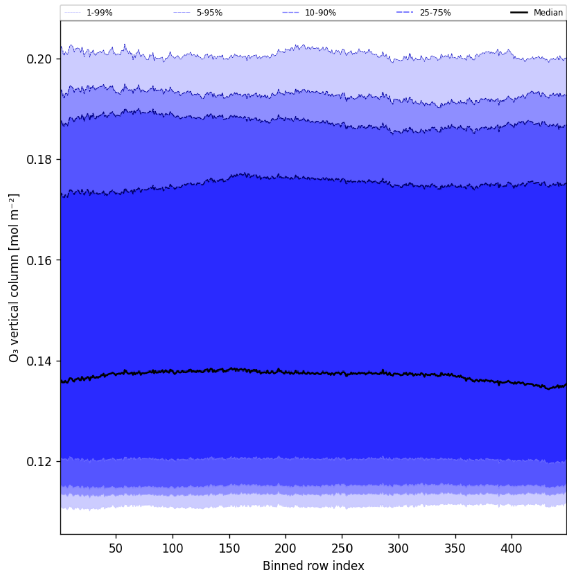
Figure 41: Along track statistics of “O 3 vertical column” for 2025-04-21 to 2025-04-22
