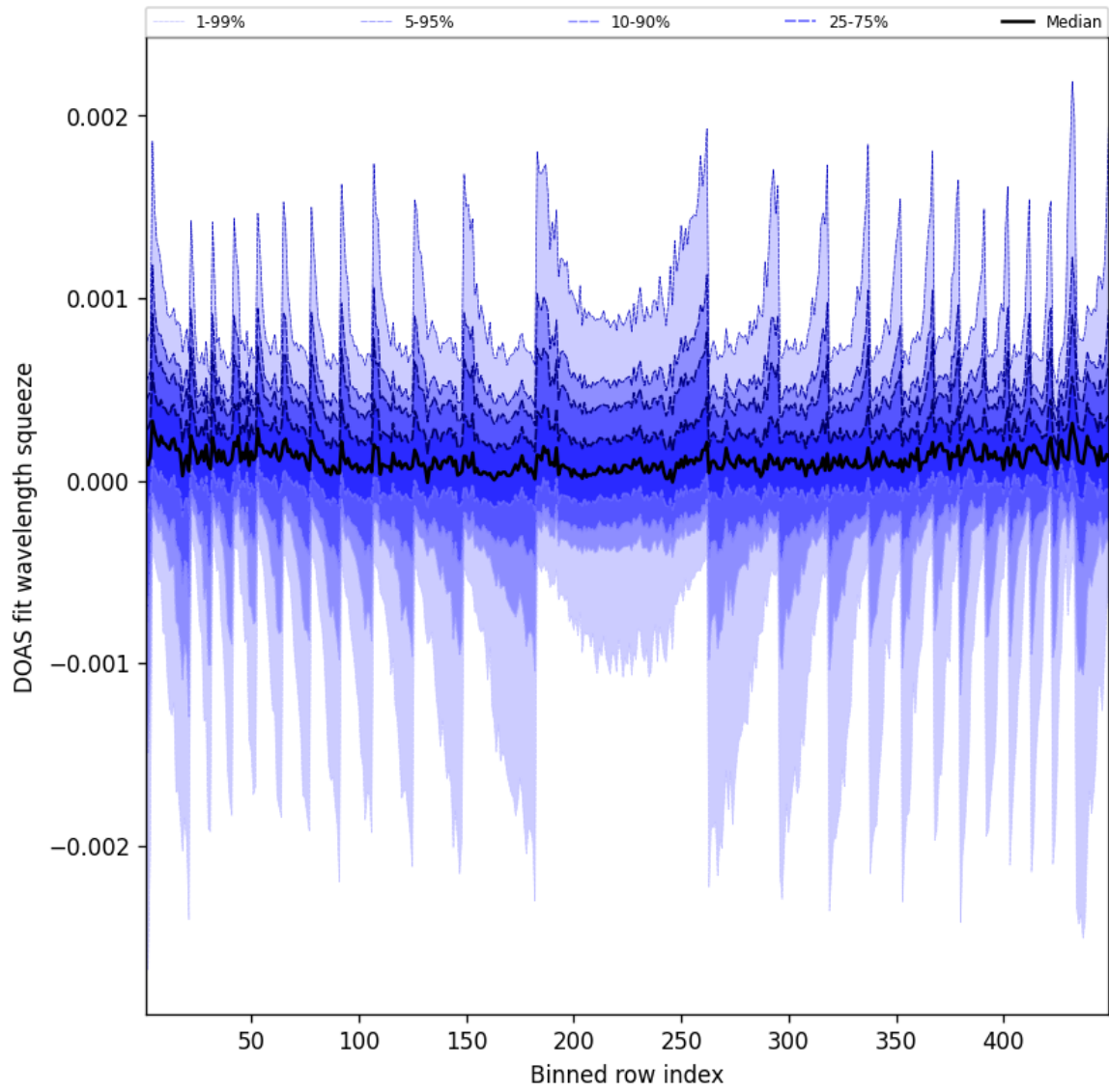
Figure 48: Along track statistics of “DOAS fit wavelength squeeze” for 2025-04-21 to 2025-04-22
