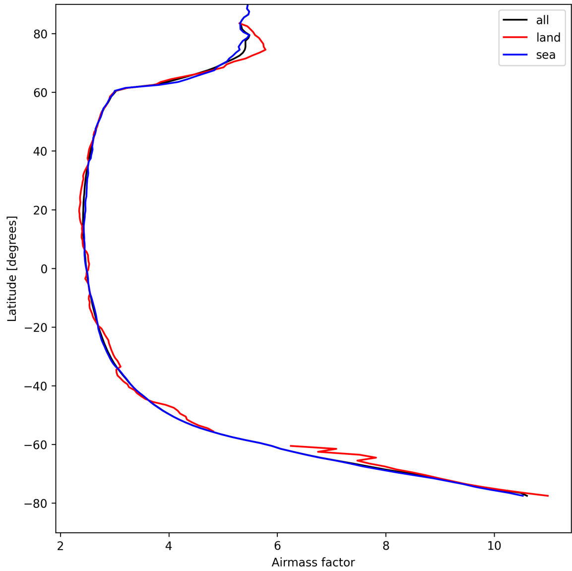
Figure 25: Zonal average of “Airmass factor” for 2025-04-21 to 2025-04-22.
