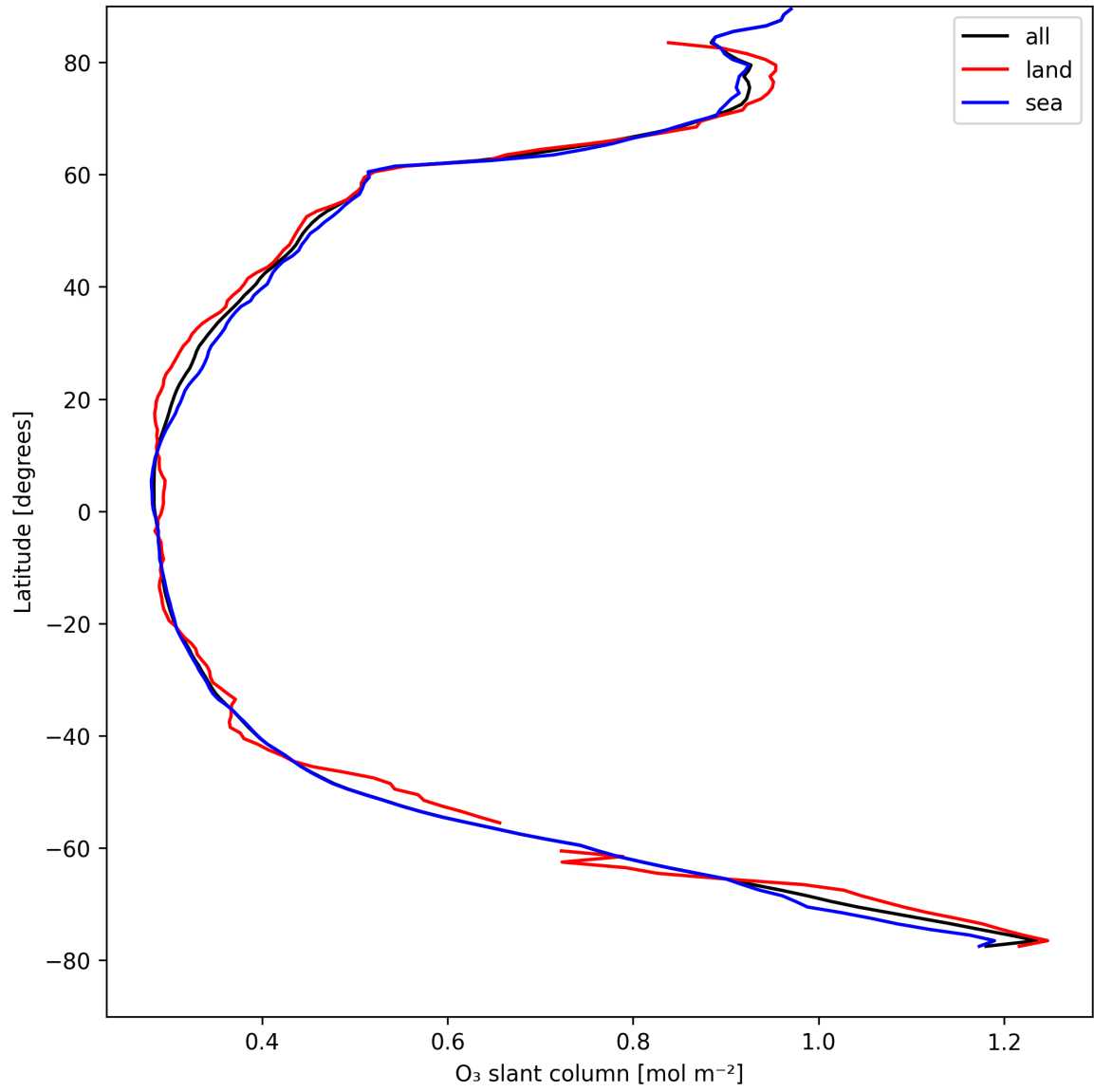
Figure 19: Zonal average of “O 3 slant column” for 2025-04-21 to 2025-04-22.
