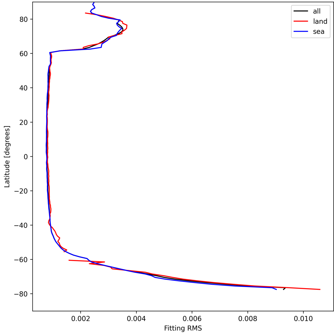
Figure 22: Zonal average of “Fitting RMS” for 2025-04-21 to 2025-04-22.
