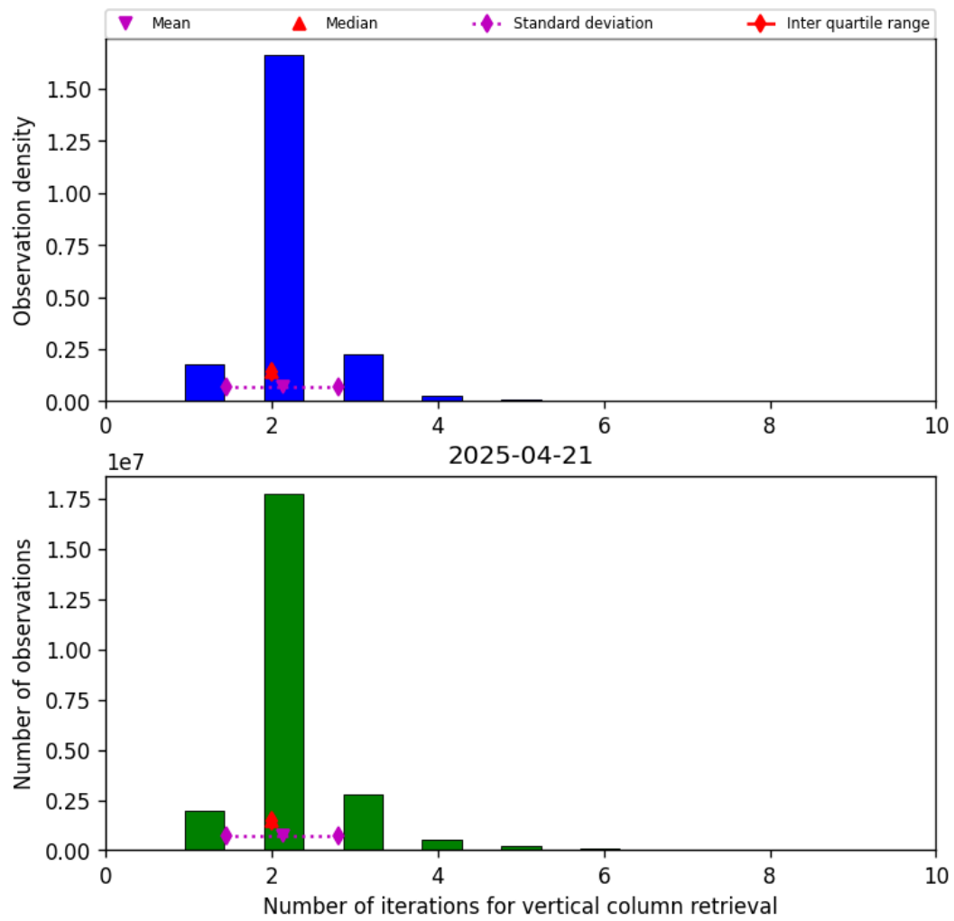
Figure 39: Histogram of “Number of iterations for vertical column retrieval” for 2025-04-21 to 2025-04-22
