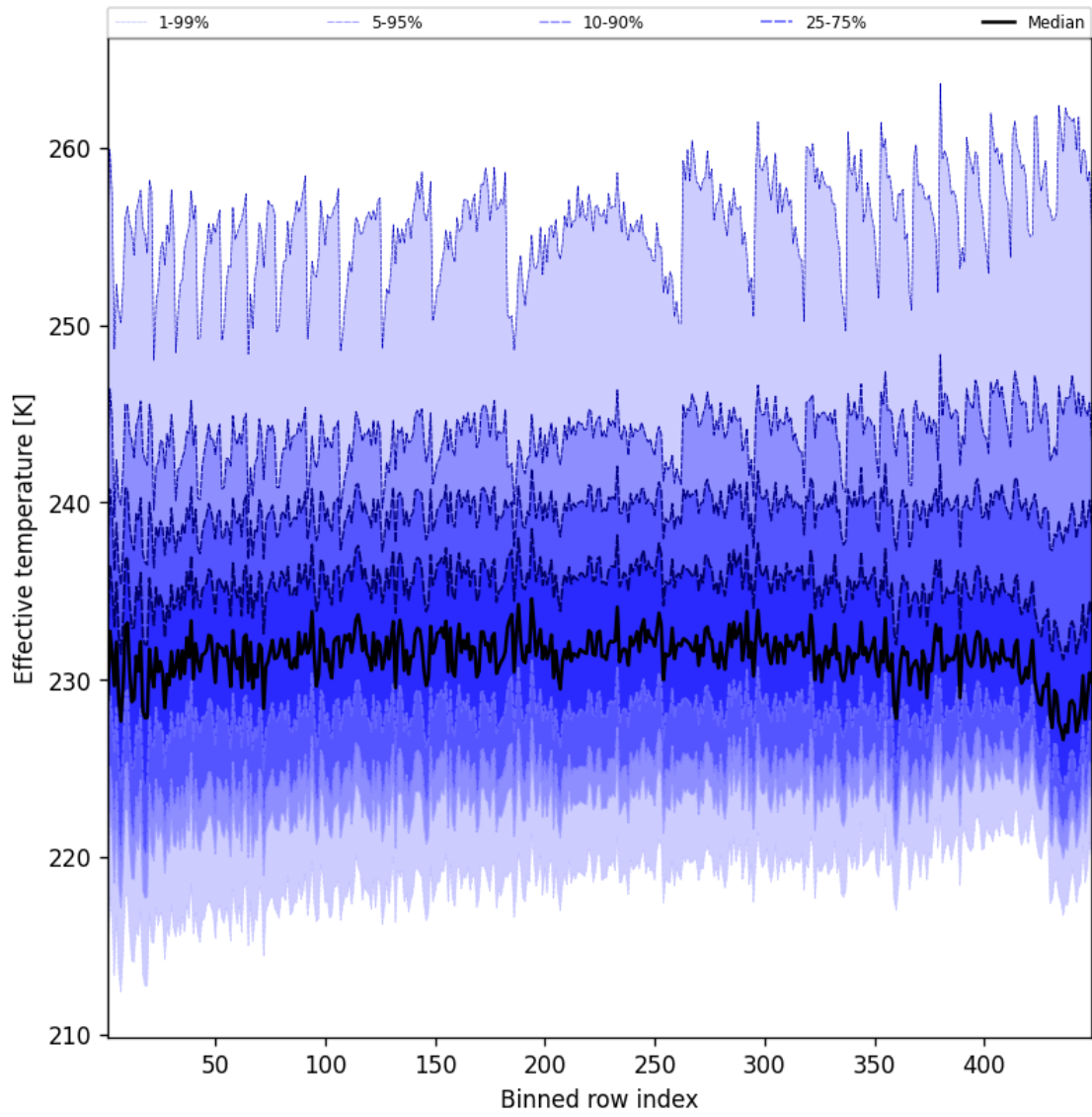
Figure 50: Along track statistics of “Effective temperature” for 2025-04-21 to 2025-04-22
