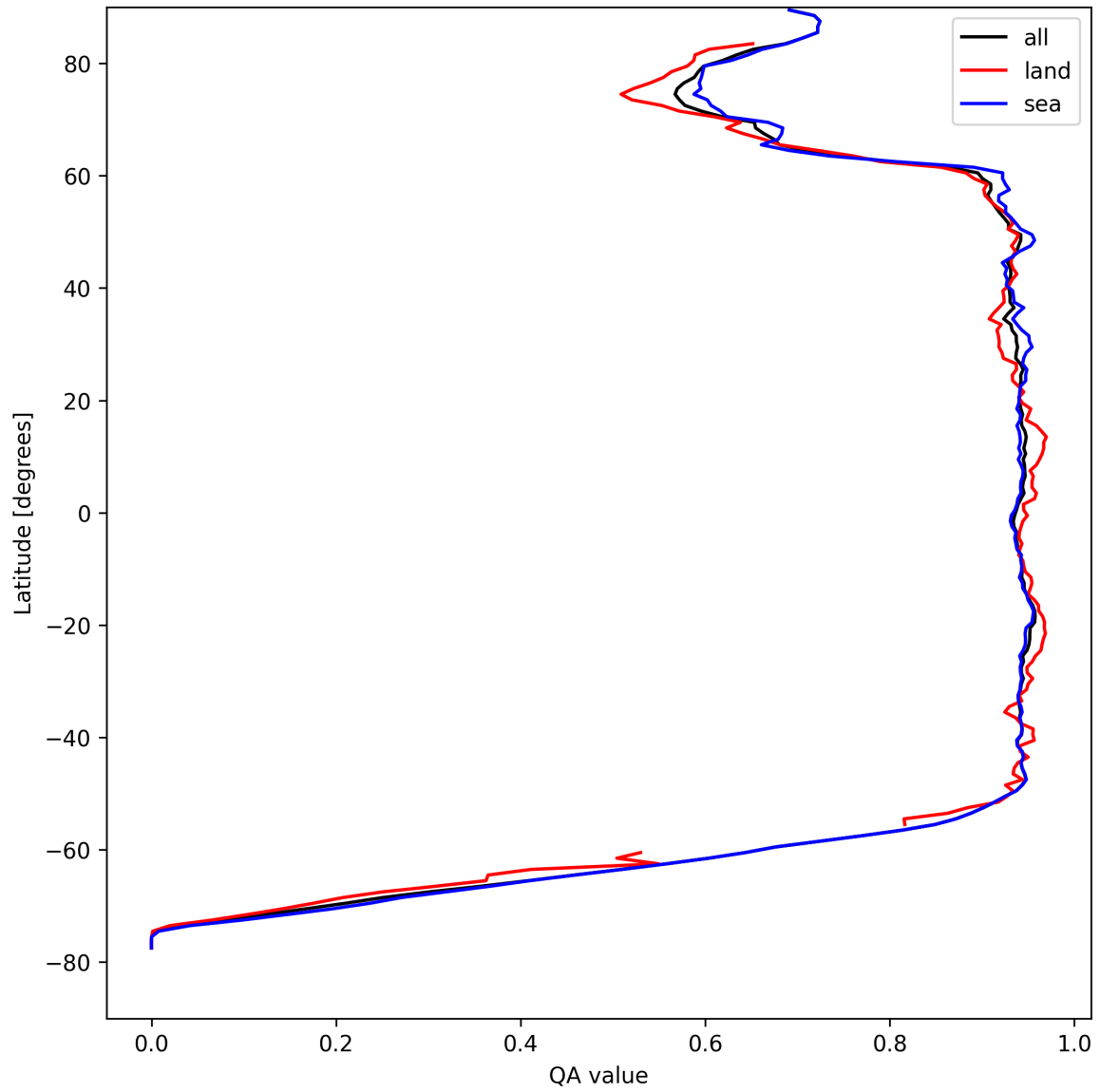
Figure 16: Zonal average of “QA value” for 2025-04-21 to 2025-04-22.
