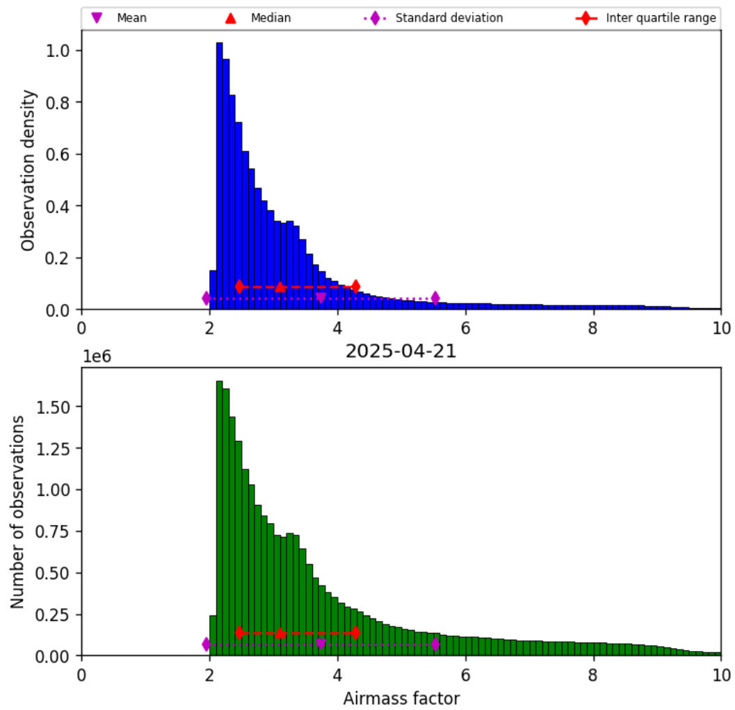
Figure 37: Histogram of “Airmass factor” for 2025-04-21 to 2025-04-22
