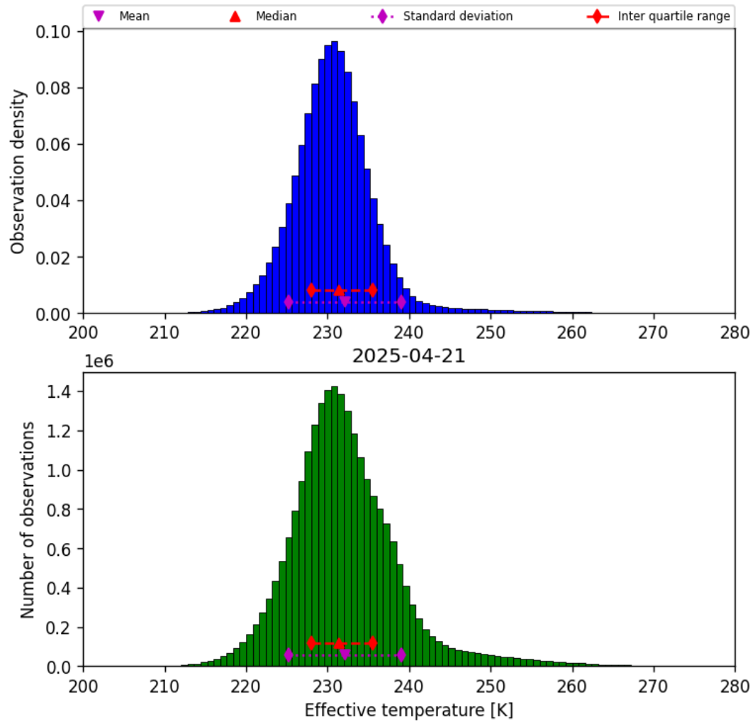
Figure 38: Histogram of “Effective temperature” for 2025-04-21 to 2025-04-22
