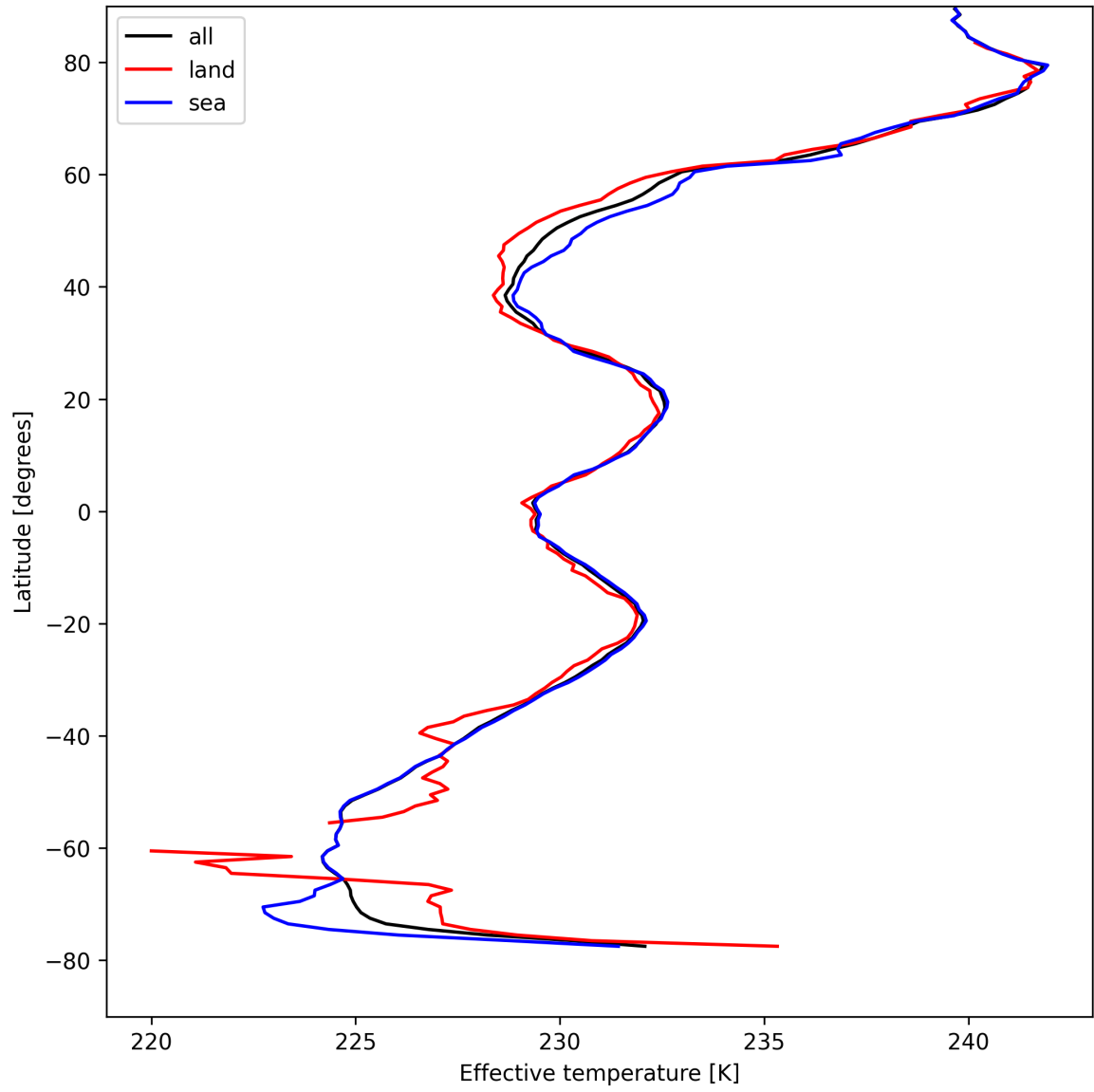
Figure 26: Zonal average of “Effective temperature” for 2025-04-21 to 2025-04-22.
