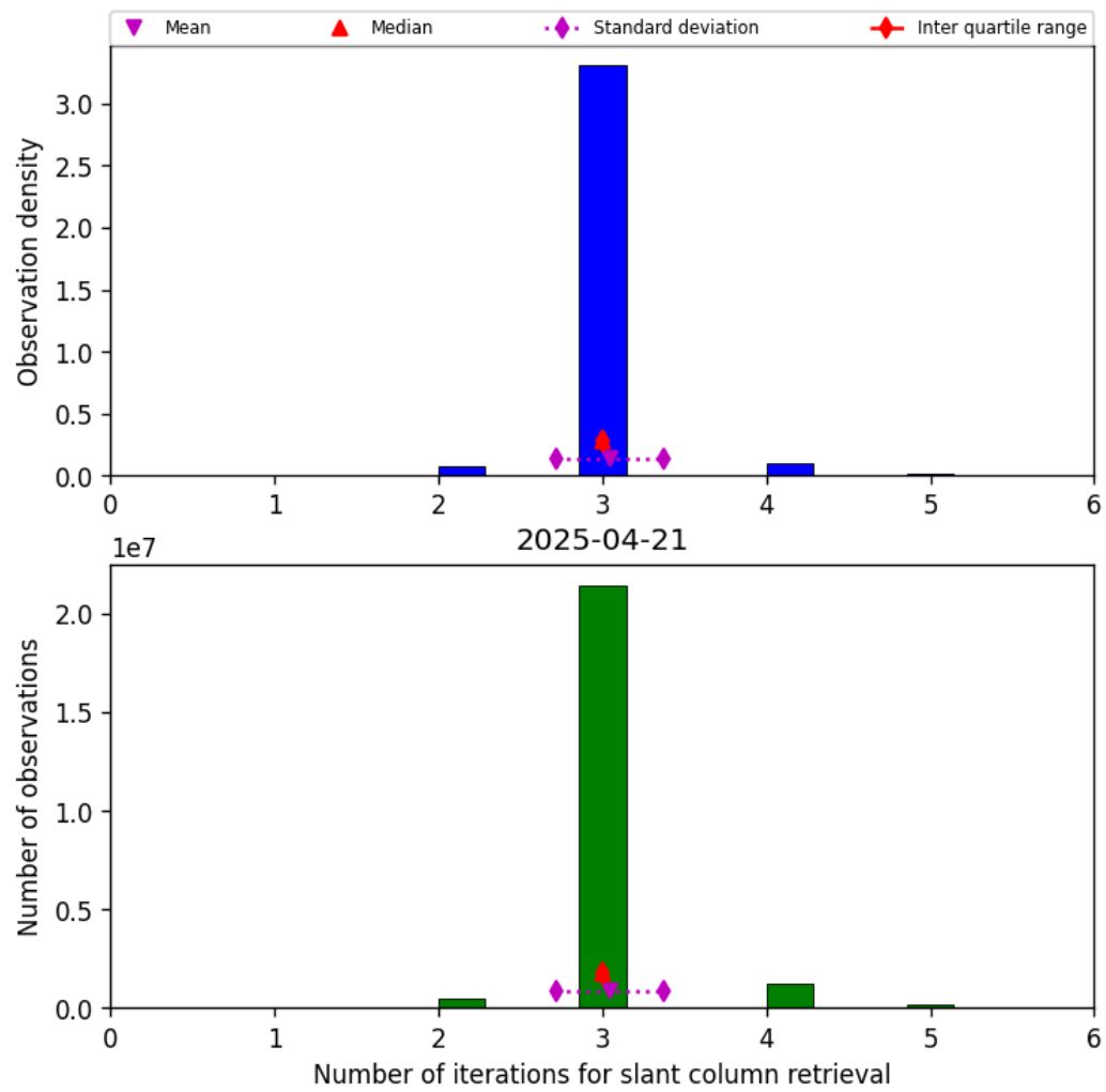
Figure 33: Histogram of "Number of iterations for slant column retrieval" for 2025-04-21 to 2025-04-22
