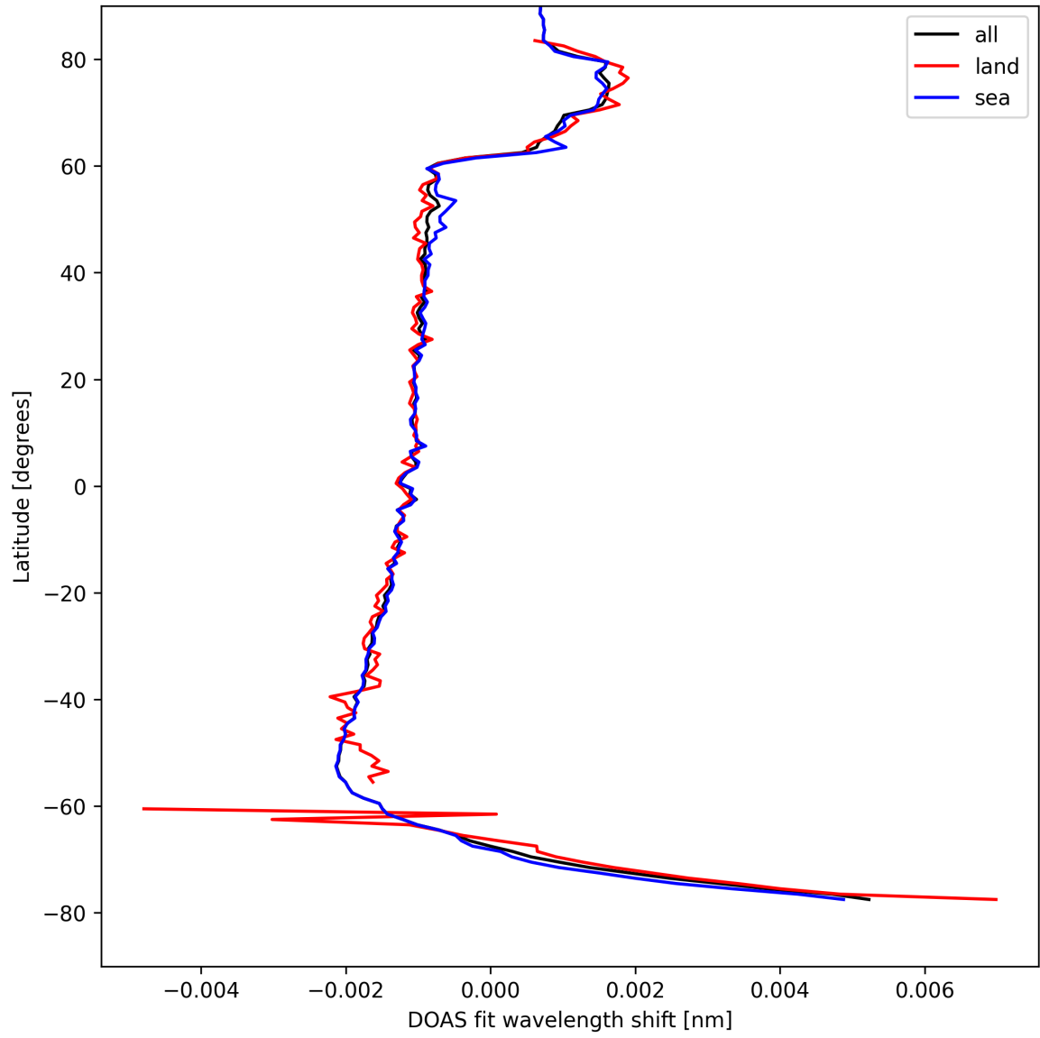
Figure 23: Zonal average of “DOAS fit wavelength shift” for 2025-04-21 to 2025-04-22.
