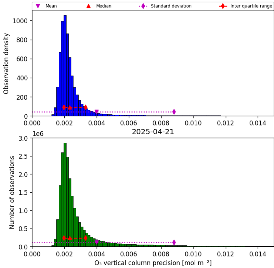
Figure 30: Histogram of “O 3 vertical column precision” for 2025-04-21 to 2025-04-22
