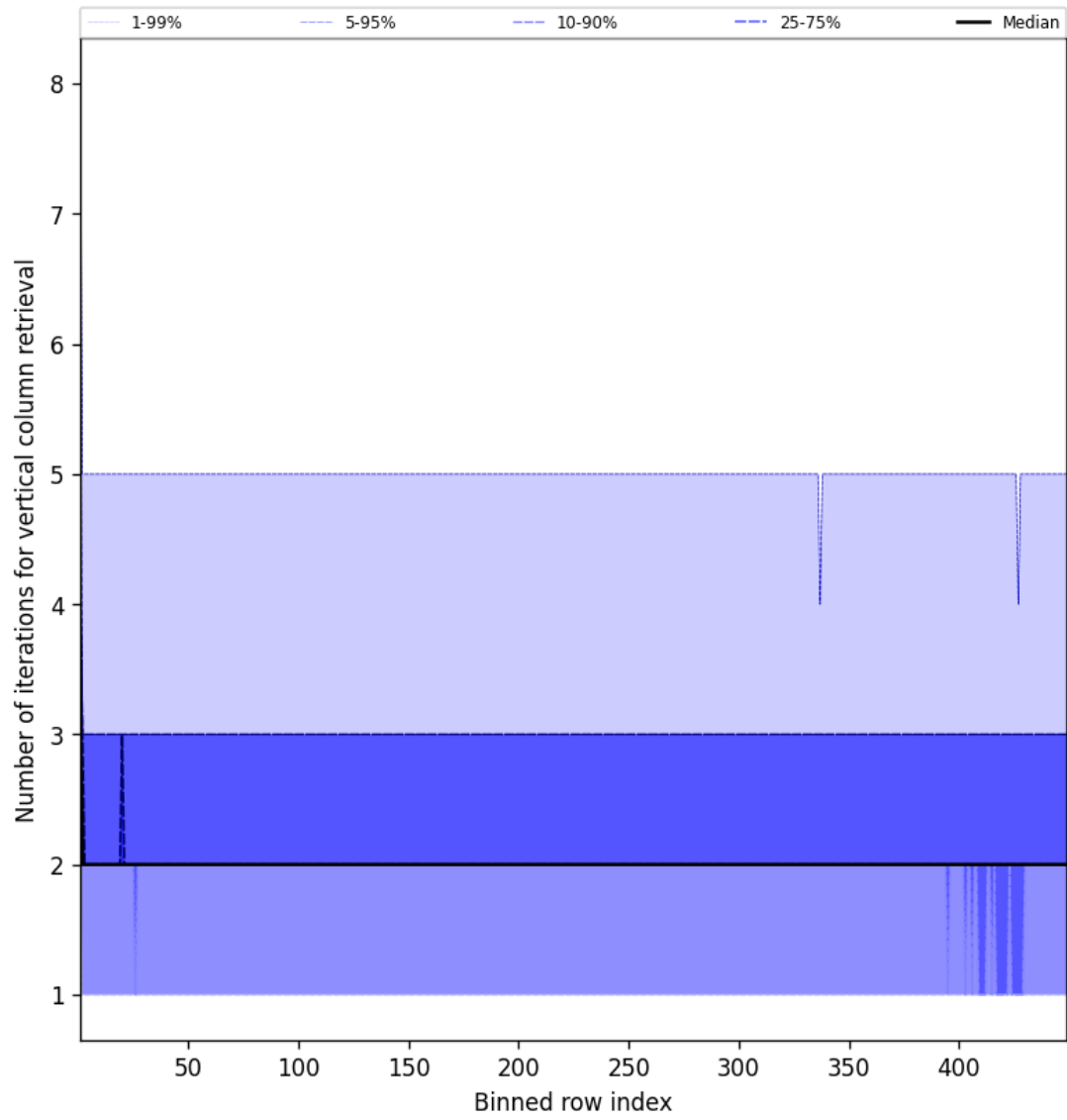
Figure 51: Along track statistics of “Number of iterations for vertical column retrieval” for 2025-04-21 to 2025-04-22
