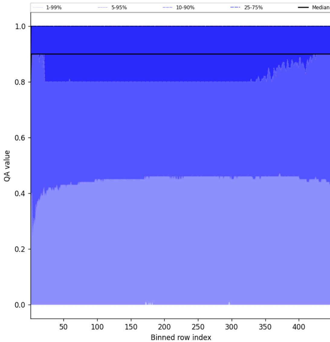
Figure 40: Along track statistics of “QA value” for 2025-04-21 to 2025-04-22
