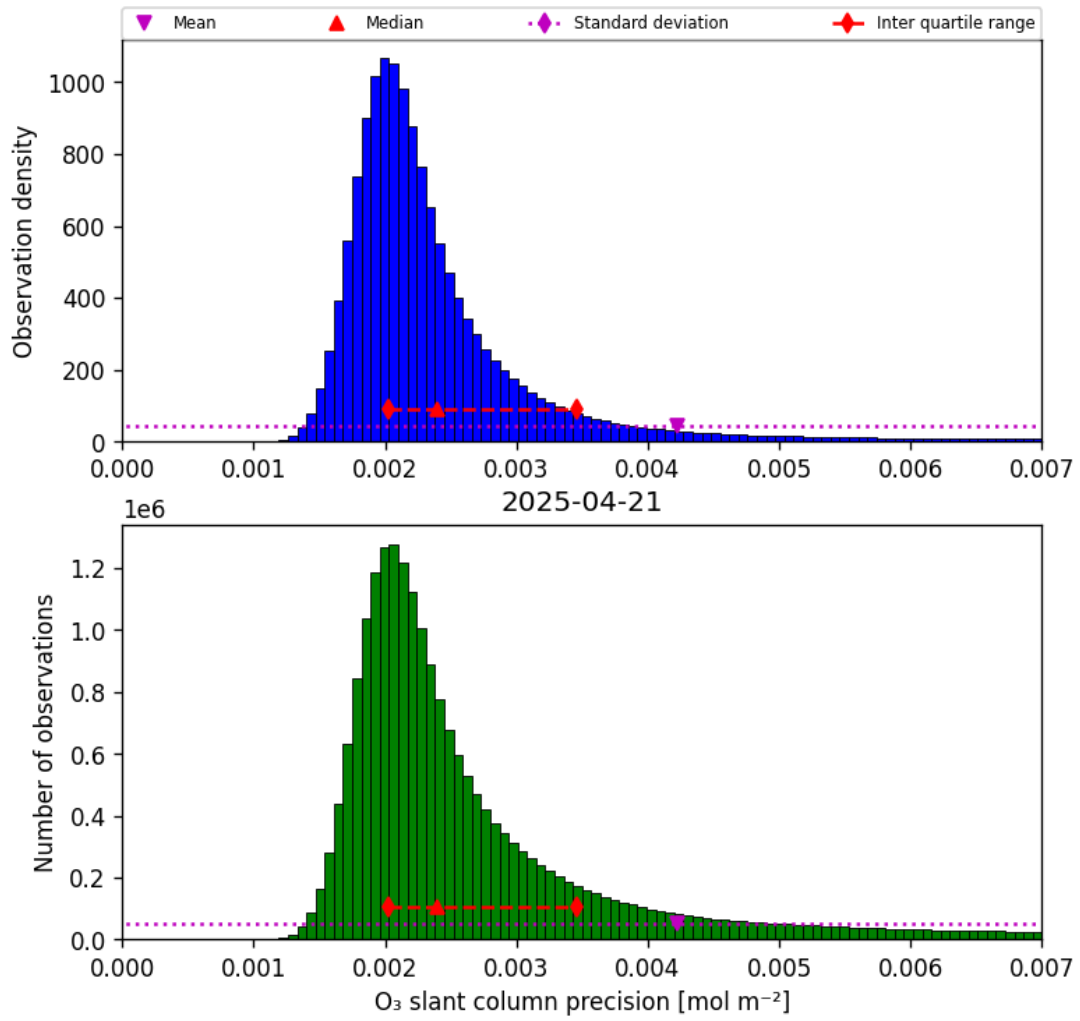
Figure 32: Histogram of “O 3 slant column precision” for 2025-04-21 to 2025-04-22
