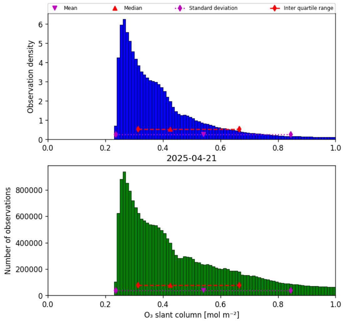
Figure 31: Histogram of “O 3 slant column” for 2025-04-21 to 2025-04-22
