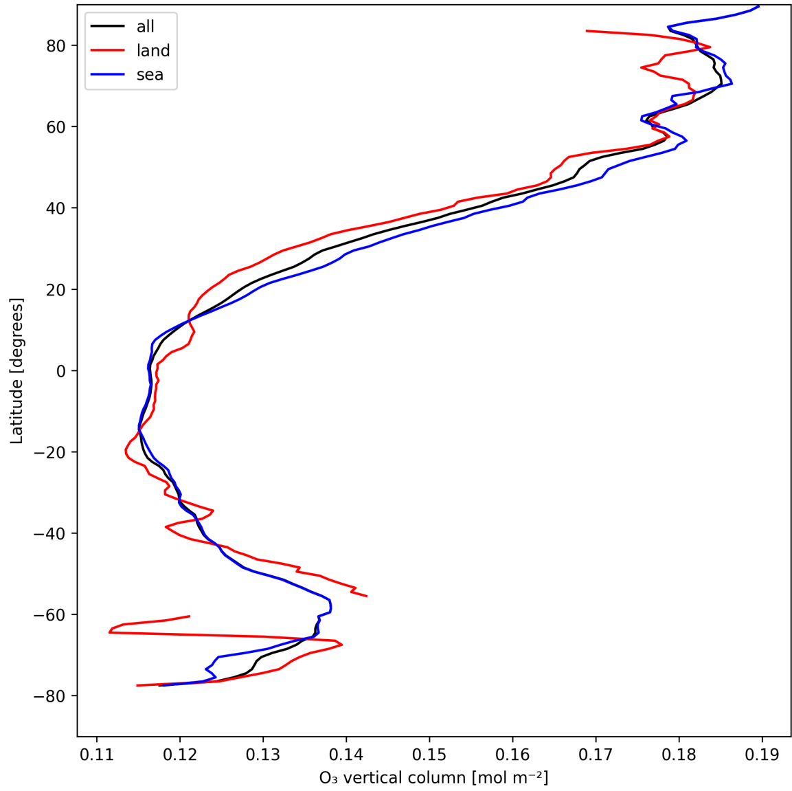
Figure 17: Zonal average of “O 3 vertical column” for 2025-04-21 to 2025-04-22.
