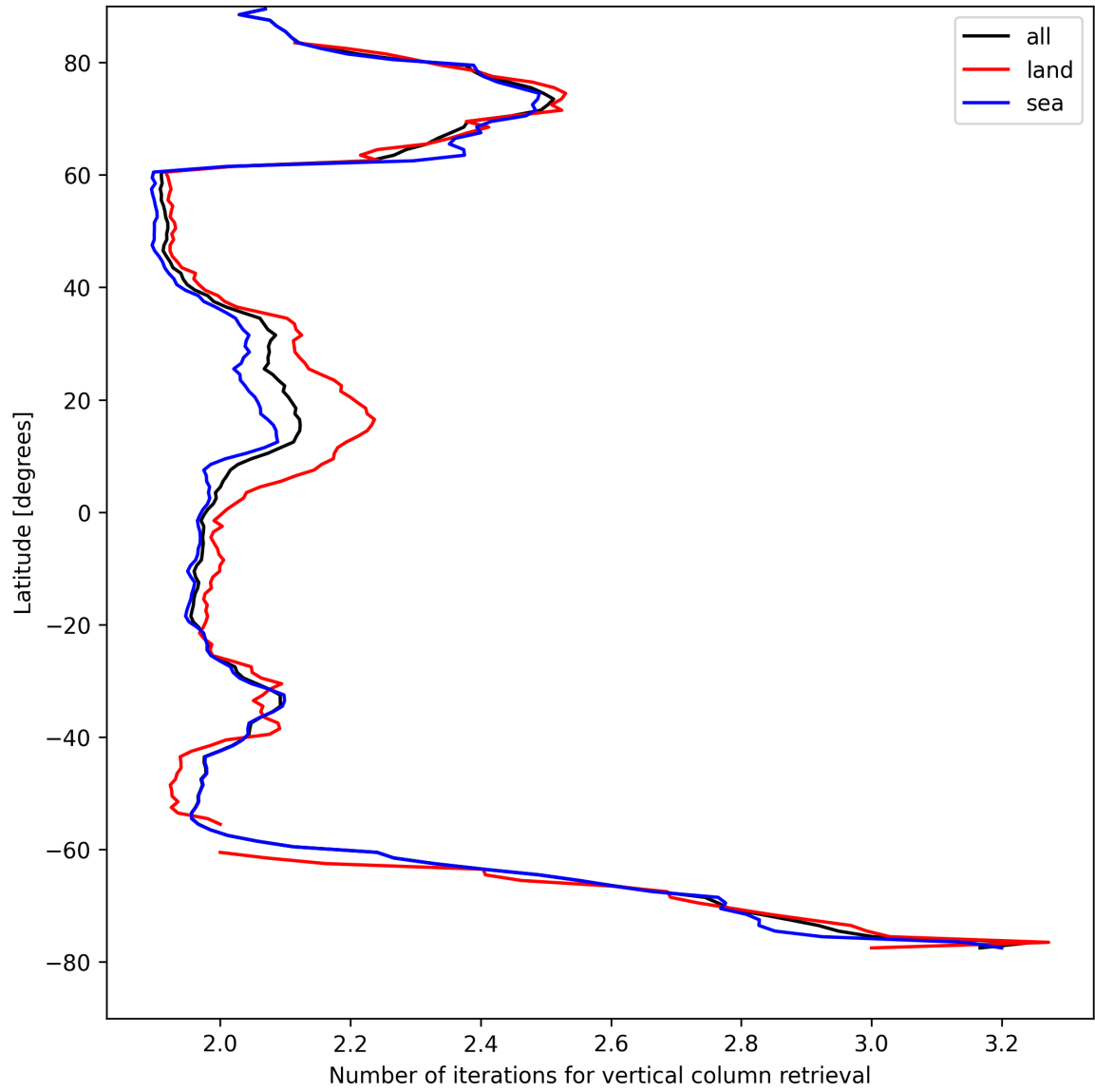
Figure 27: Zonal average of “Number of iterations for vertical column retrieval” for 2025-04-21 to 2025-04-22.
