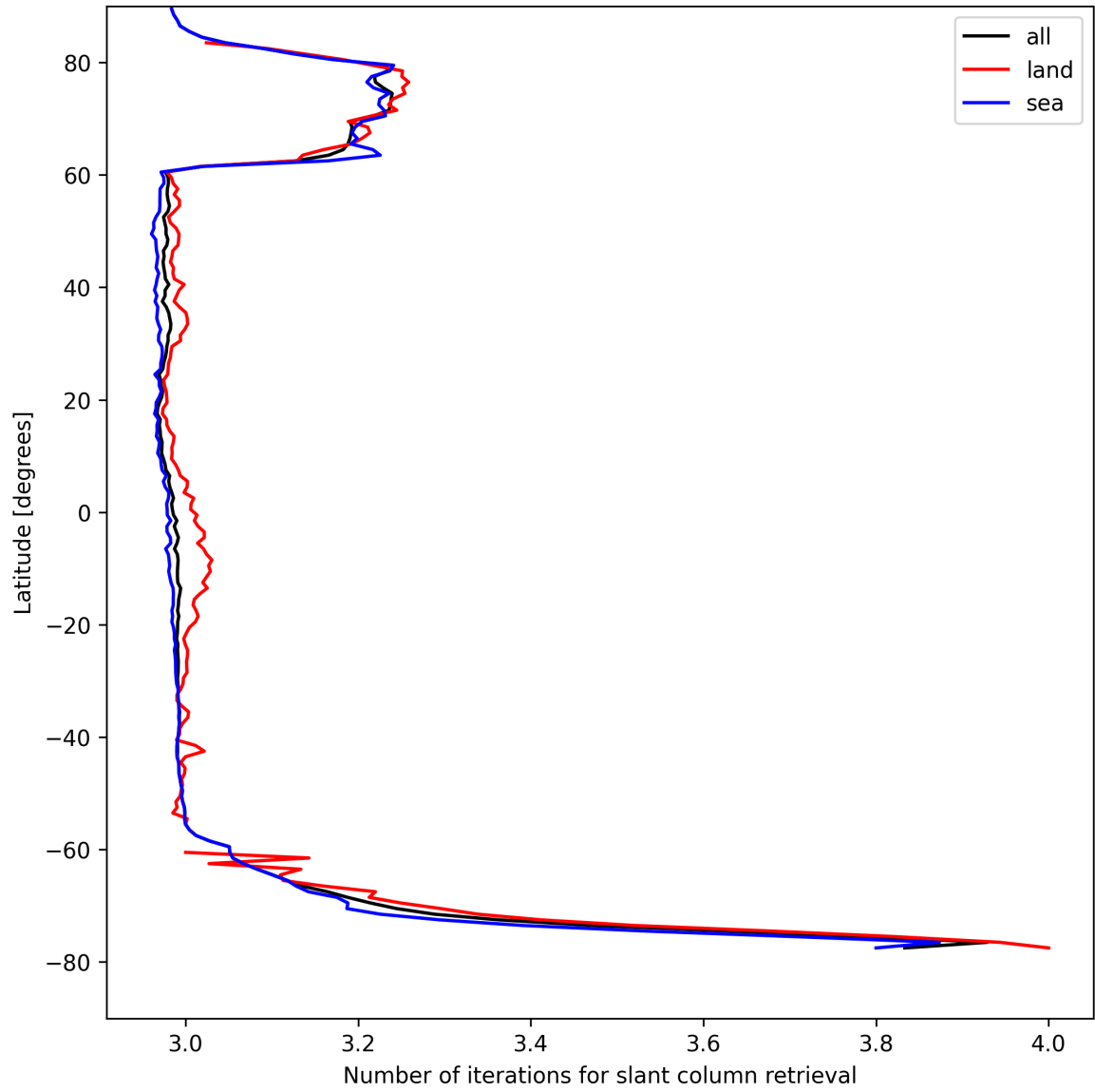
Figure 21: Zonal average of “Number of iterations for slant column retrieval” for 2025-04-21 to 2025-04-22.
