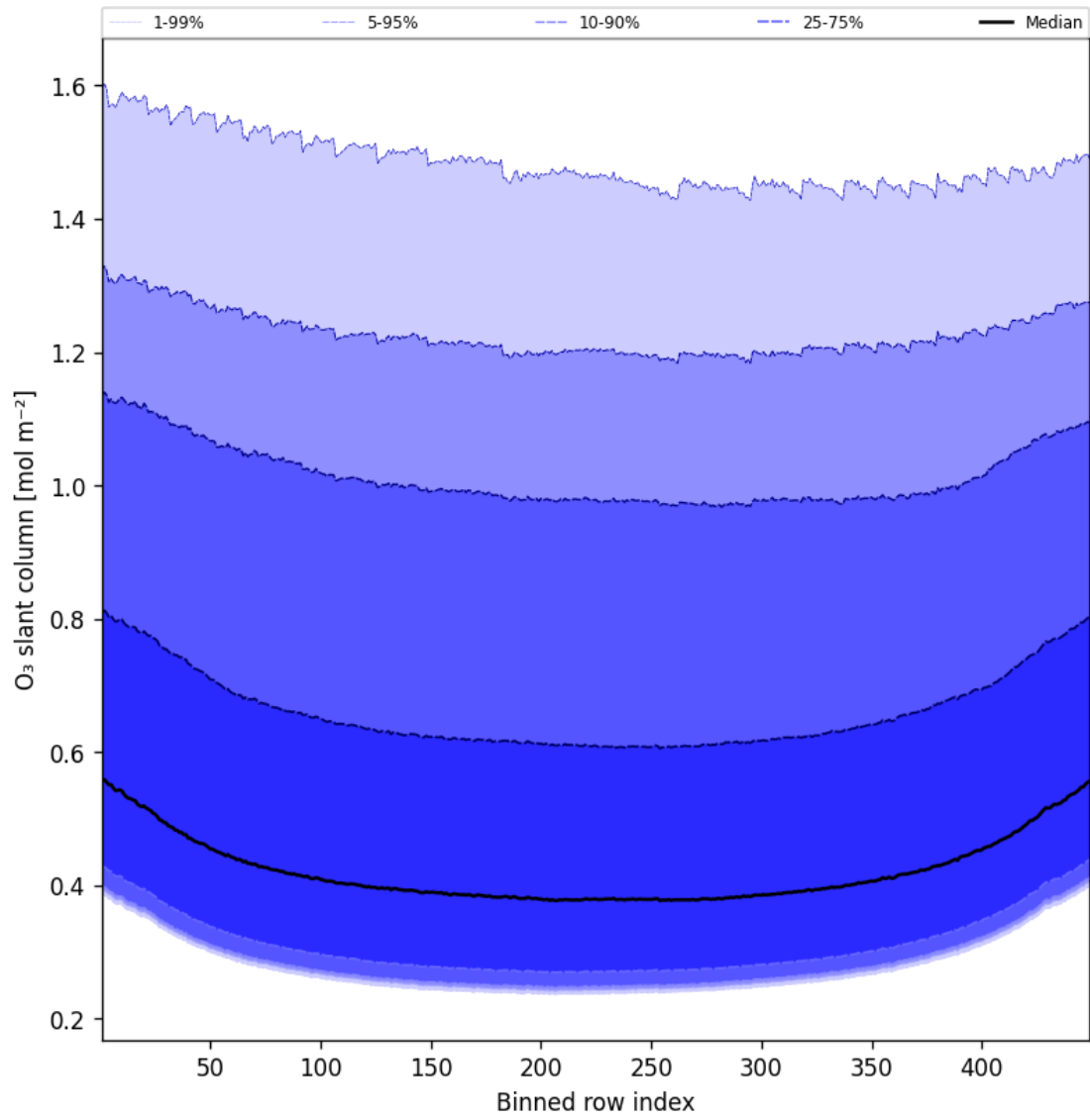
Figure 43: Along track statistics of “O 3 slant column” for 2025-04-21 to 2025-04-22
