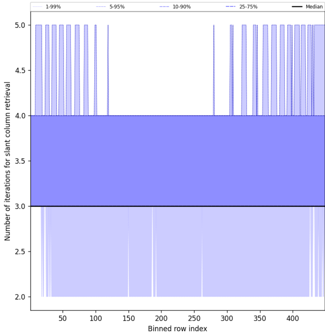
Figure 45: Along track statistics of “Number of iterations for slant column retrieval” for 2025-04-21 to 2025-04-22
