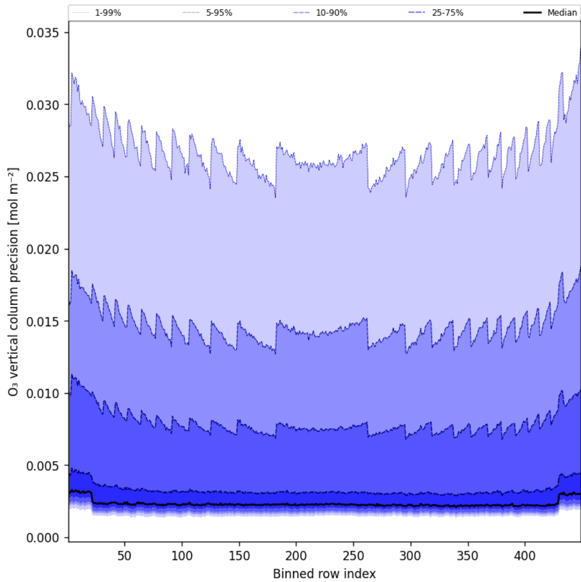
Figure 42: Along track statistics of “O 3 vertical column precision” for 2025-04-21 to 2025-04-22
