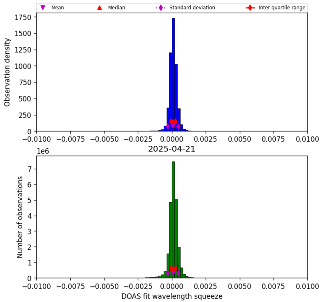
Figure 36: Histogram of “DOAS fit wavelength squeeze” for 2025-04-21 to 2025-04-22
