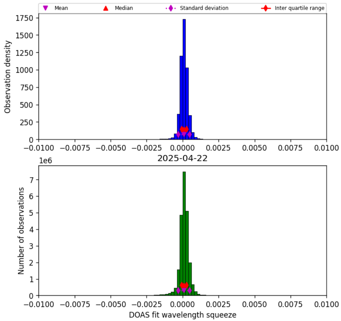
Figure 36: Histogram of “DOAS fit wavelength squeeze” for 2025-04-22 to 2025-04-22
