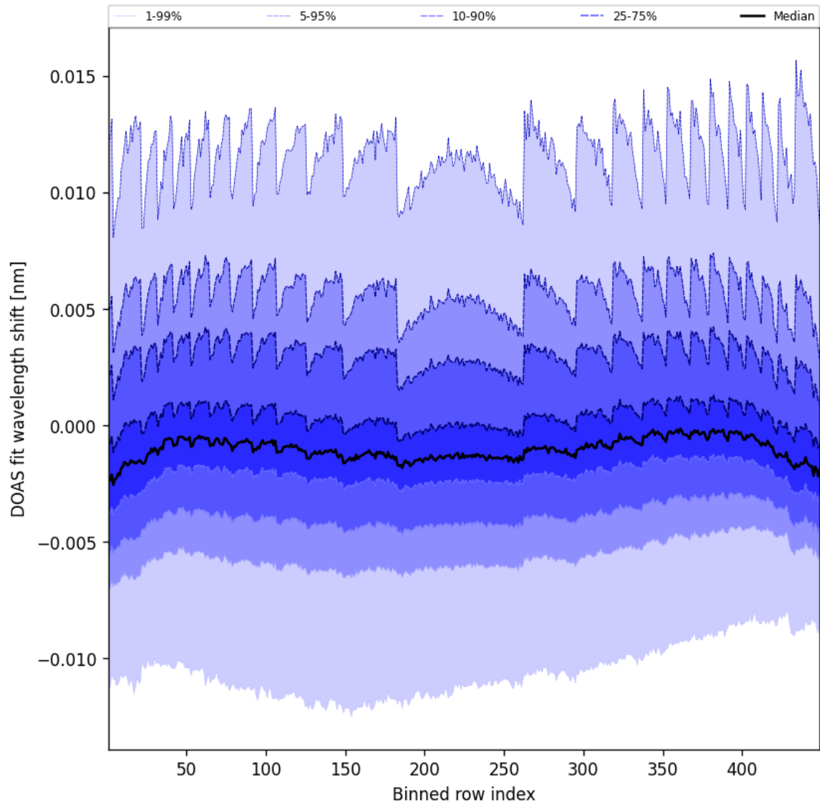
Figure 47: Along track statistics of “DOAS fit wavelength shift” for 2025-04-22 to 2025-04-22
