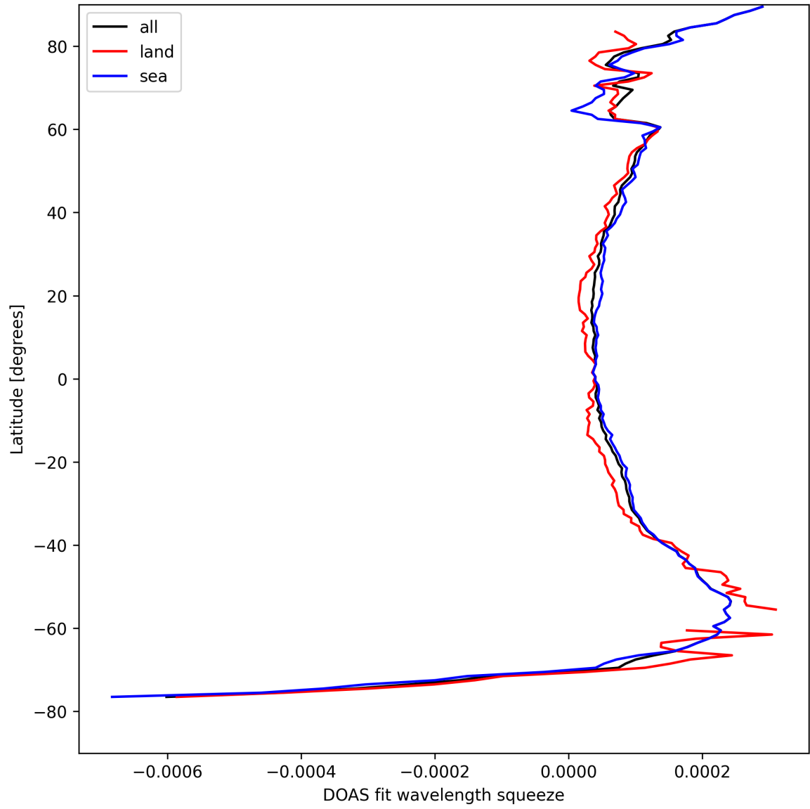
Figure 24: Zonal average of “DOAS fit wavelength squeeze” for 2025-04-22 to 2025-04-22.
