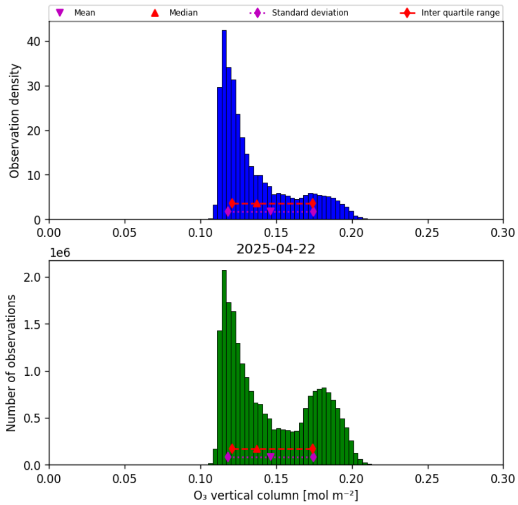
Figure 29: Histogram of “O 3 vertical column” for 2025-04-22 to 2025-04-22
