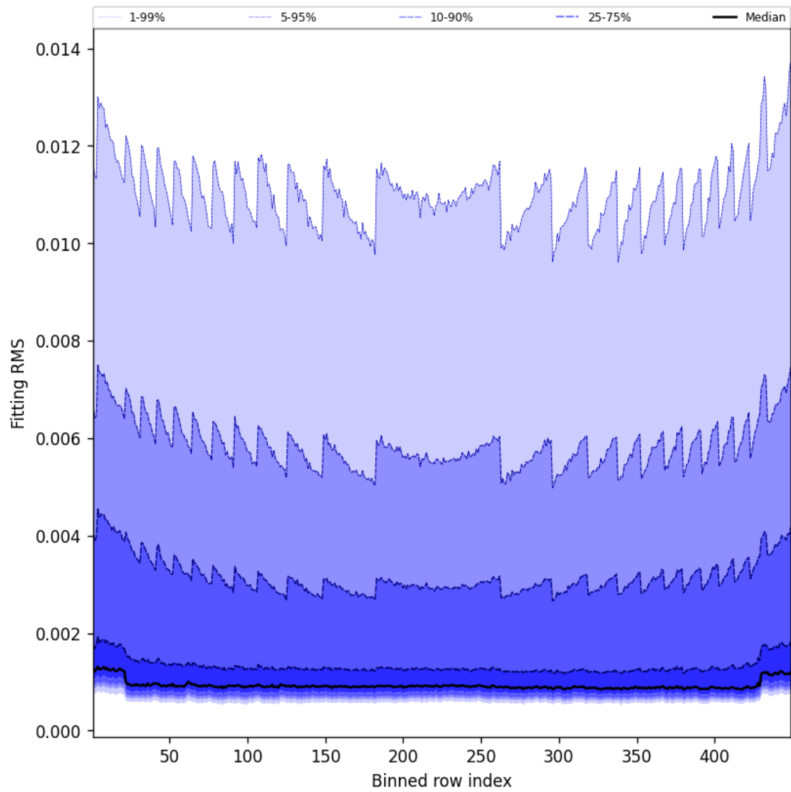
Figure 46: Along track statistics of “Fitting RMS” for 2025-04-22 to 2025-04-22
