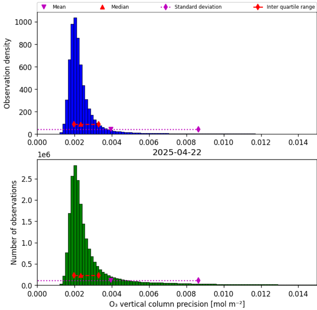
Figure 30: Histogram of “O 3 vertical column precision” for 2025-04-22 to 2025-04-22
