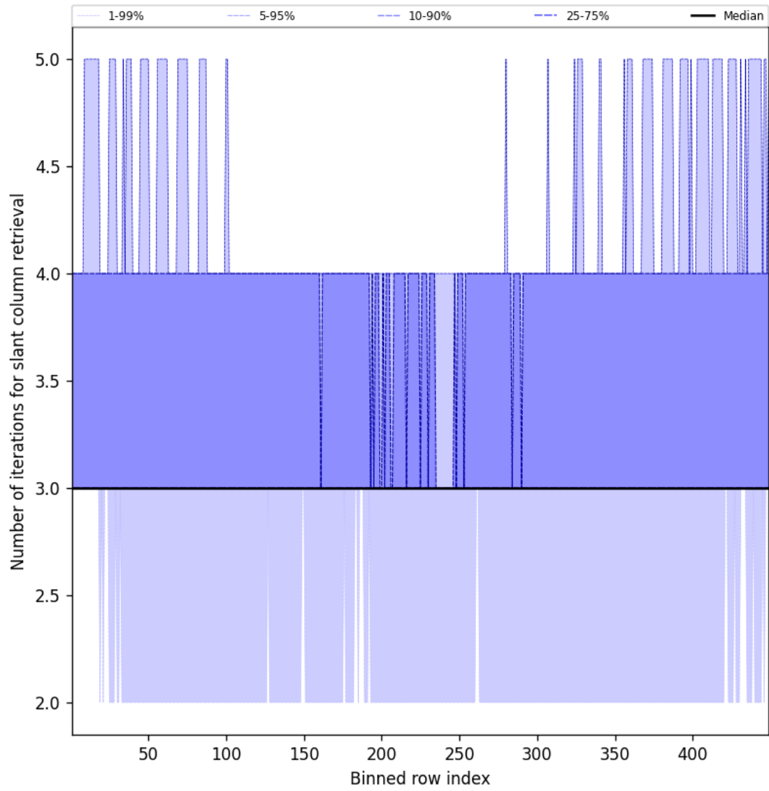
Figure 45: Along track statistics of “Number of iterations for slant column retrieval” for 2025-04-22 to 2025-04-22
