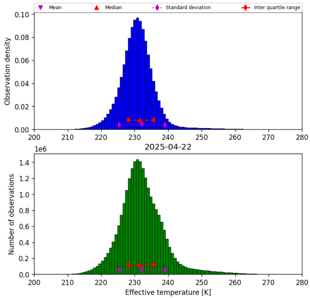
Figure 38: Histogram of “Effective temperature” for 2025-04-22 to 2025-04-22
