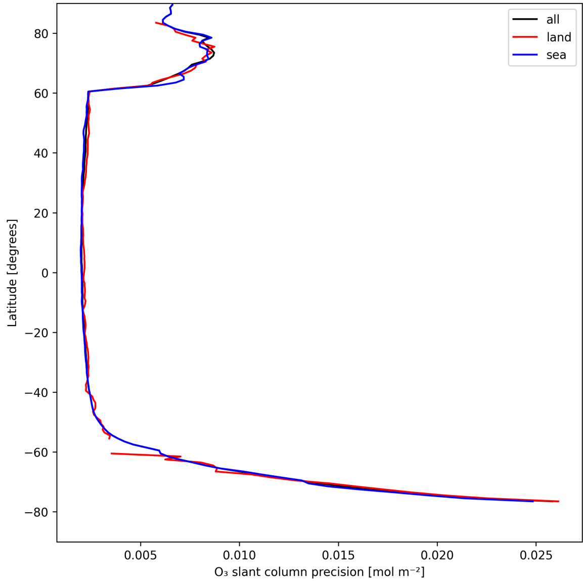
Figure 20: Zonal average of “O 3 slant column precision” for 2025-04-22 to 2025-04-22.
