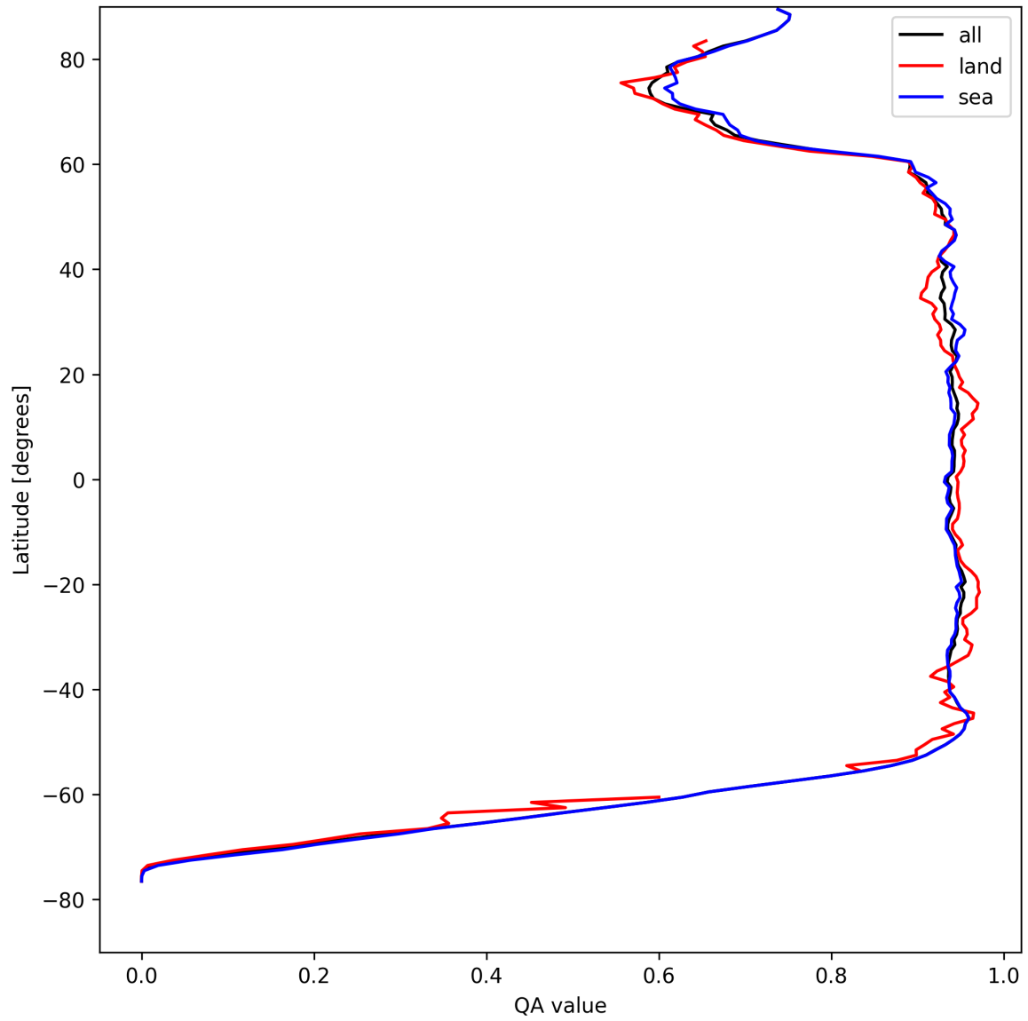
Figure 16: Zonal average of “QA value” for 2025-04-22 to 2025-04-22.
