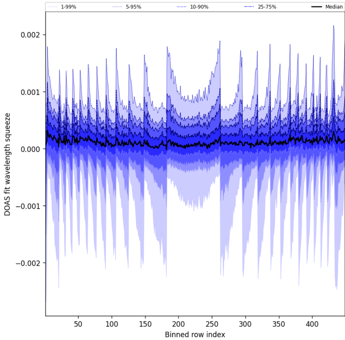
Figure 48: Along track statistics of “DOAS fit wavelength squeeze” for 2025-04-22 to 2025-04-22
