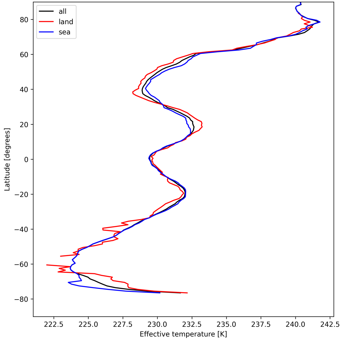
Figure 26: Zonal average of “Effective temperature” for 2025-04-22 to 2025-04-22.
