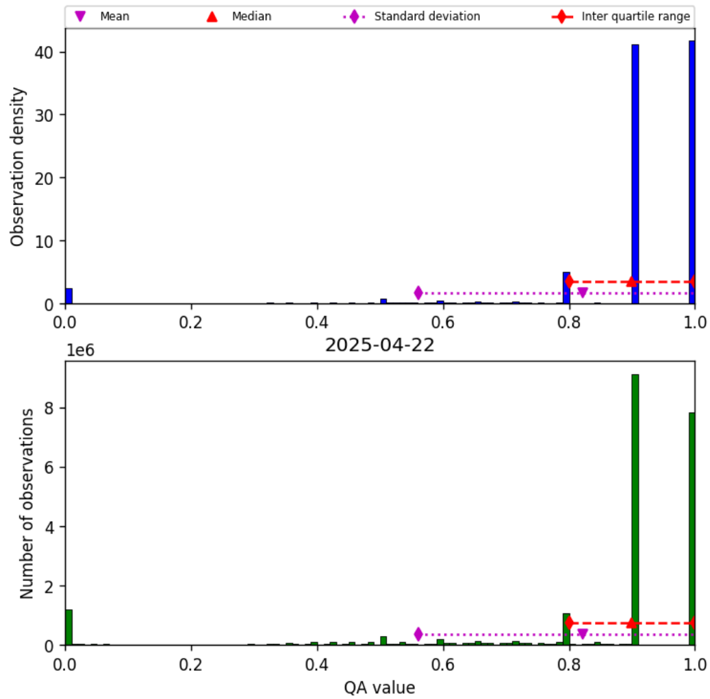
Figure 28: Histogram of “QA value” for 2025-04-22 to 2025-04-22
