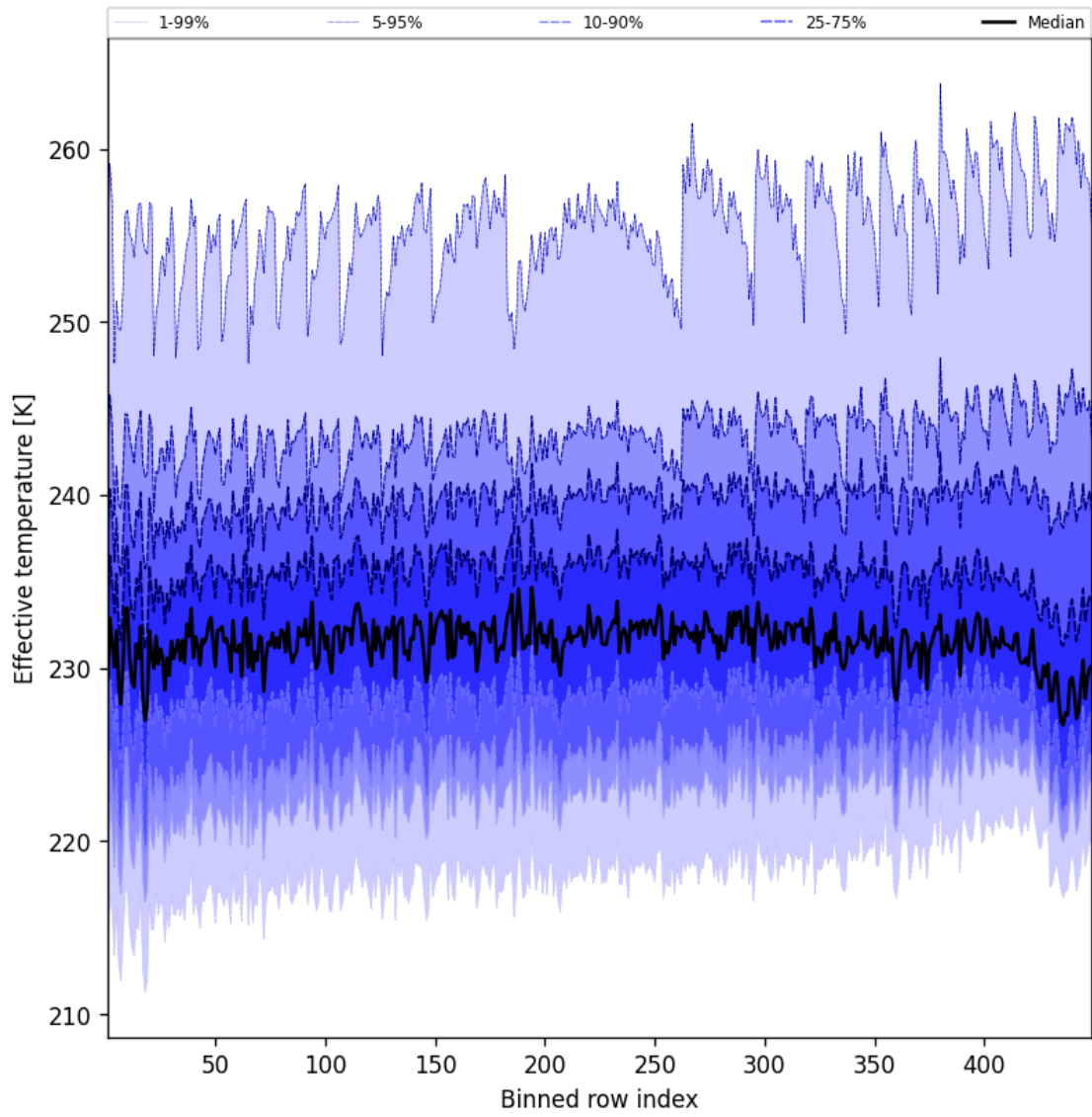
Figure 50: Along track statistics of “Effective temperature” for 2025-04-22 to 2025-04-22
