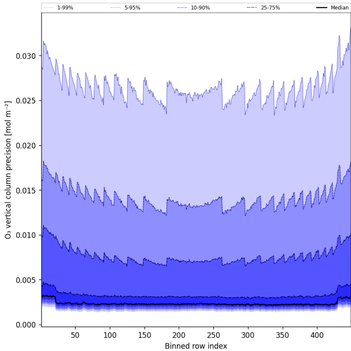
Figure 42: Along track statistics of “O 3 vertical column precision” for 2025-04-22 to 2025-04-22
