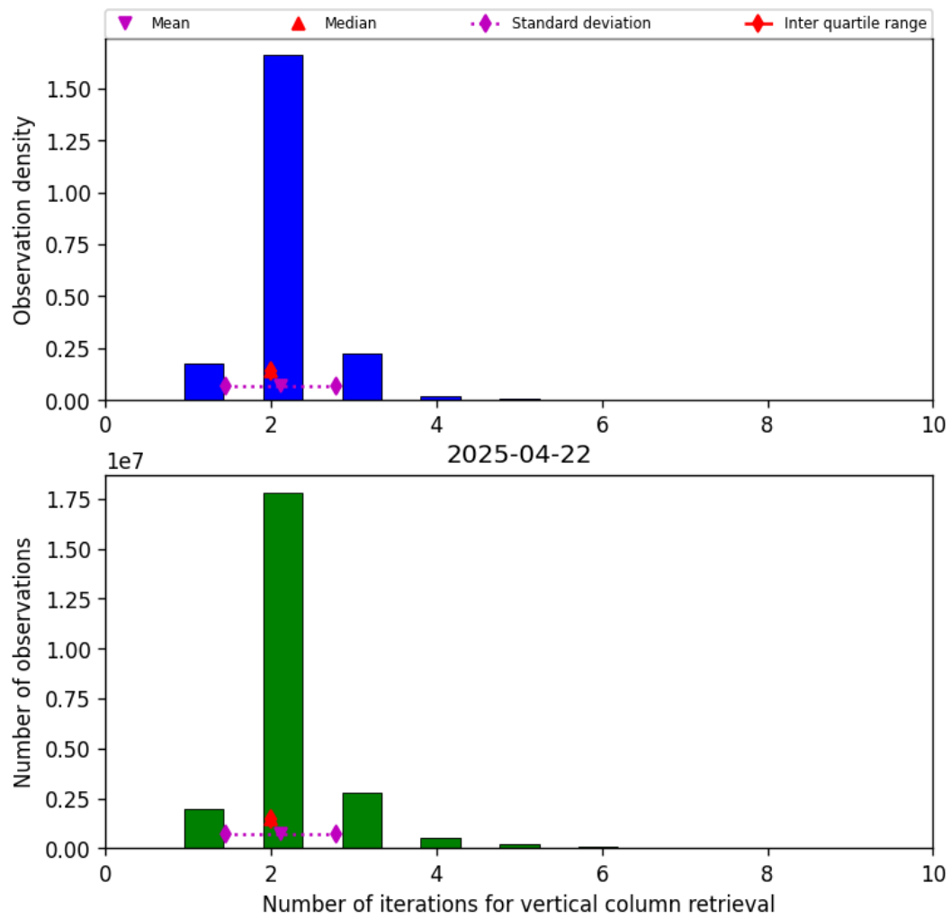
Figure 39: Histogram of “Number of iterations for vertical column retrieval” for 2025-04-22 to 2025-04-22
