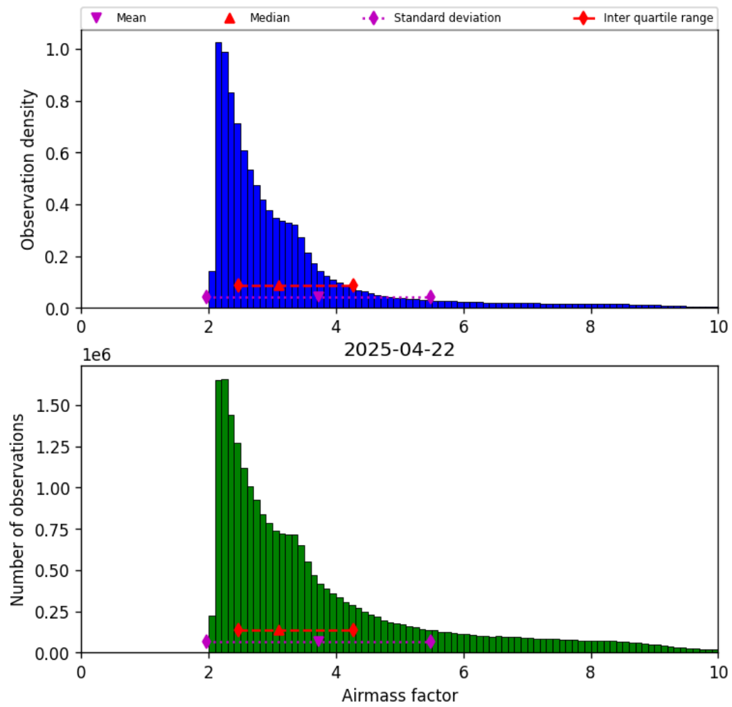
Figure 37: Histogram of “Airmass factor” for 2025-04-22 to 2025-04-22
