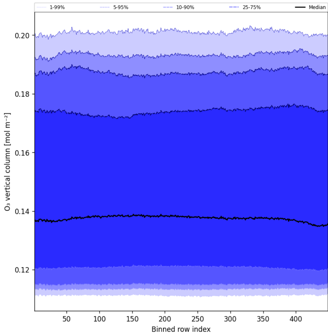
Figure 41: Along track statistics of “O 3 vertical column” for 2025-04-22 to 2025-04-22
