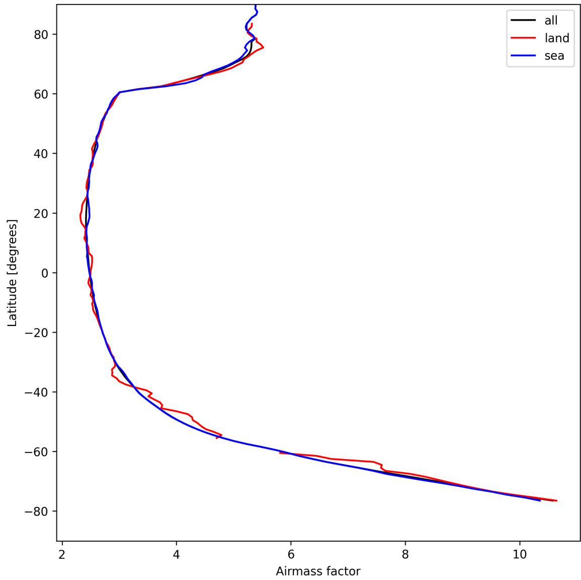
Figure 25: Zonal average of “Airmass factor” for 2025-04-22 to 2025-04-22.
