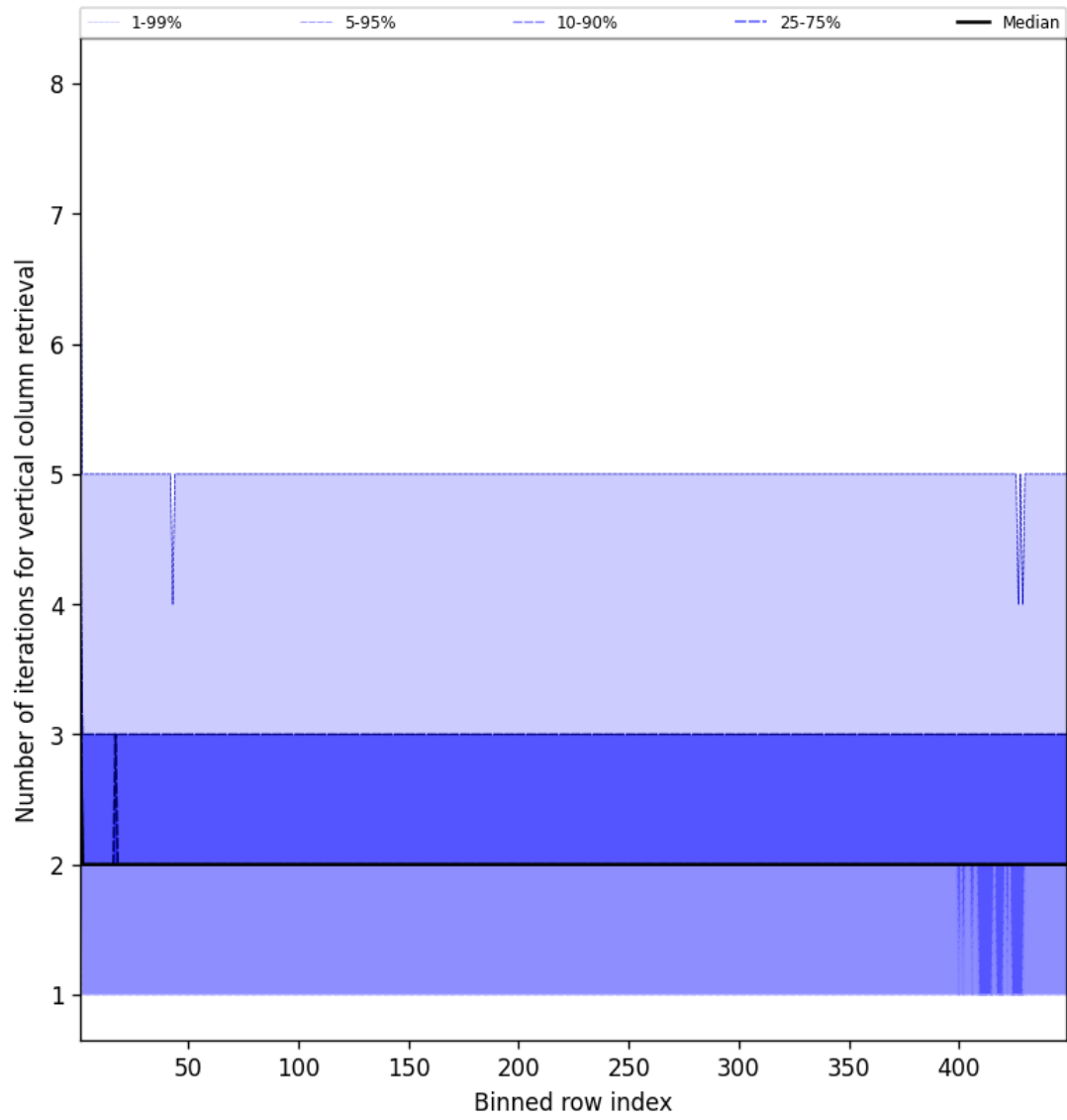
Figure 51: Along track statistics of “Number of iterations for vertical column retrieval” for 2025-04-22 to 2025-04-22
