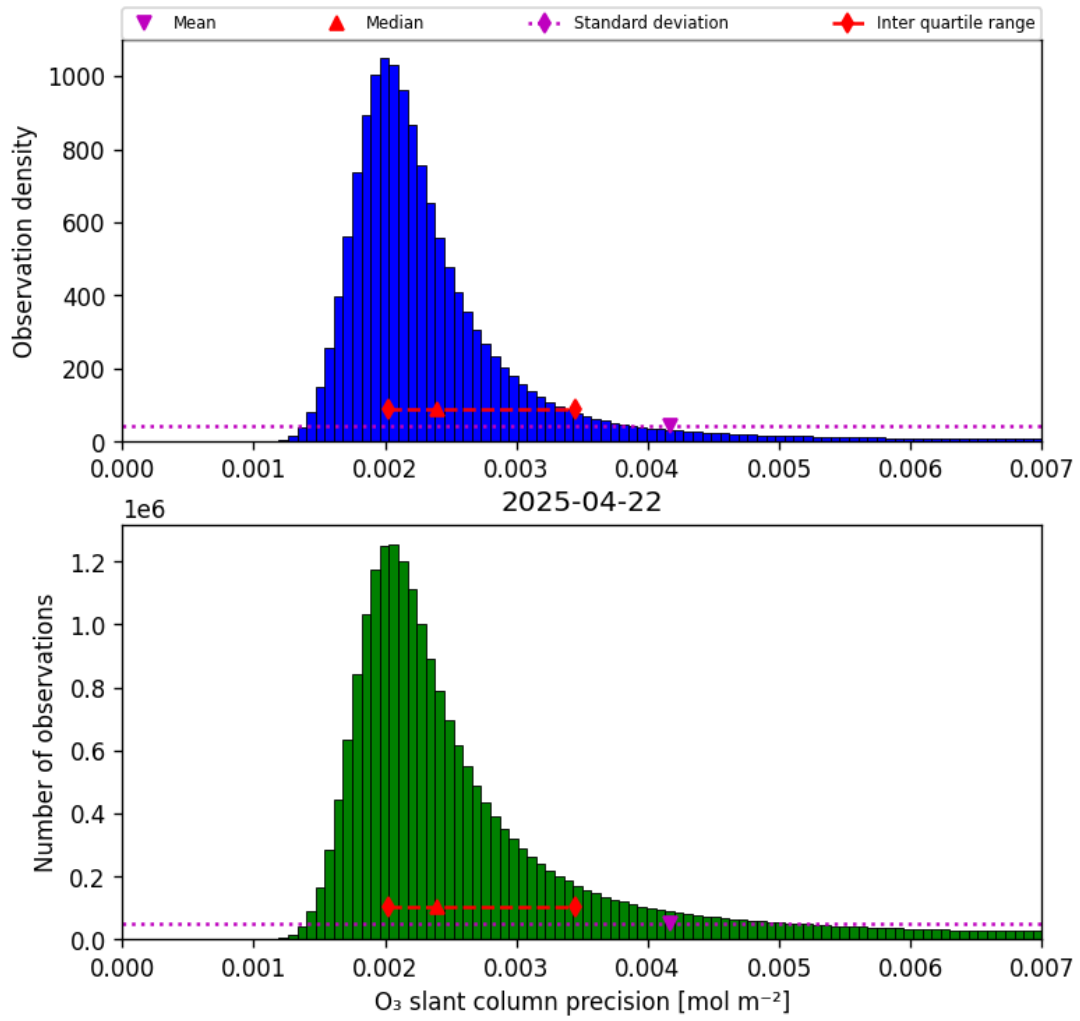
Figure 32: Histogram of “O 3 slant column precision” for 2025-04-22 to 2025-04-22
