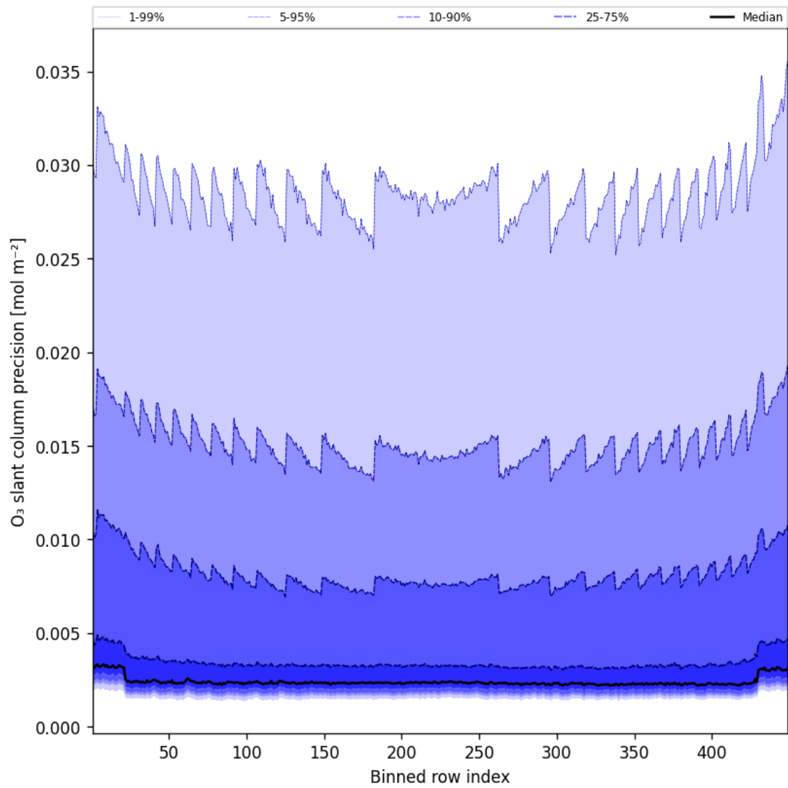
Figure 44: Along track statistics of “O 3 slant column precision” for 2025-04-22 to 2025-04-22
