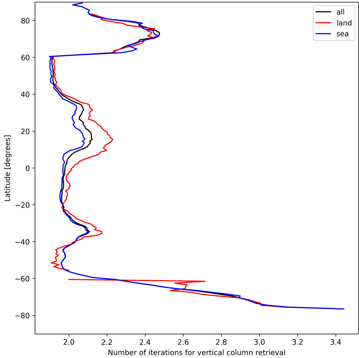
Figure 27: Zonal average of “Number of iterations for vertical column retrieval” for 2025-04-22 to 2025-04-22.
