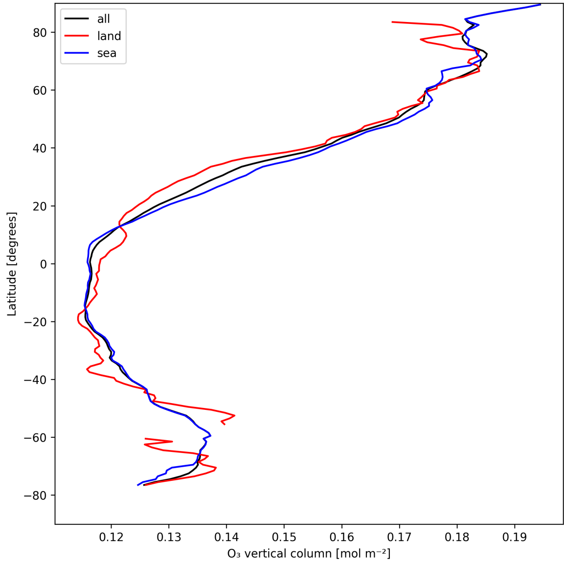
Figure 17: Zonal average of “O 3 vertical column” for 2025-04-22 to 2025-04-22.
