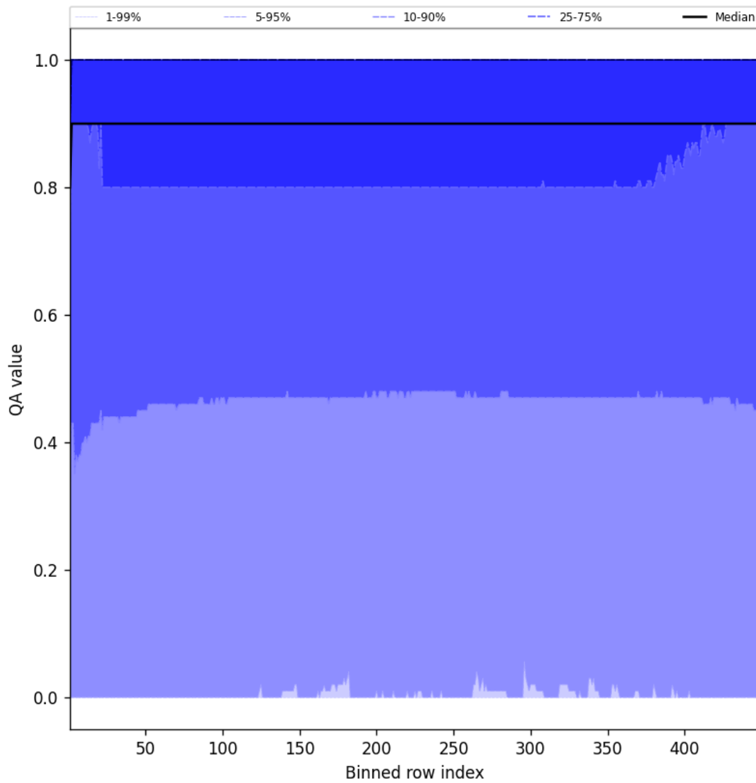
Figure 40: Along track statistics of “QA value” for 2025-04-22 to 2025-04-22
