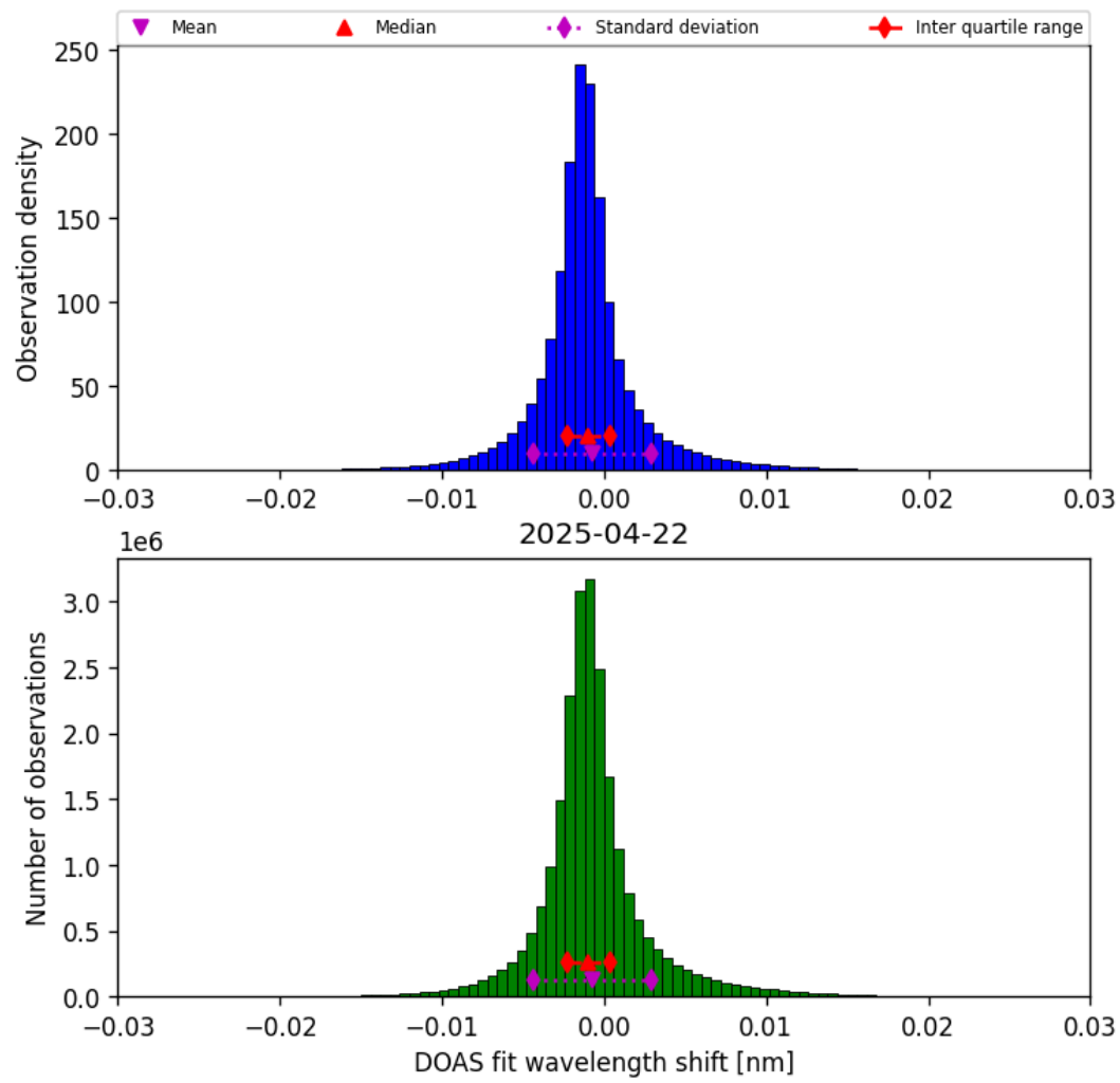
Figure 35: Histogram of “DOAS fit wavelength shift” for 2025-04-22 to 2025-04-22
