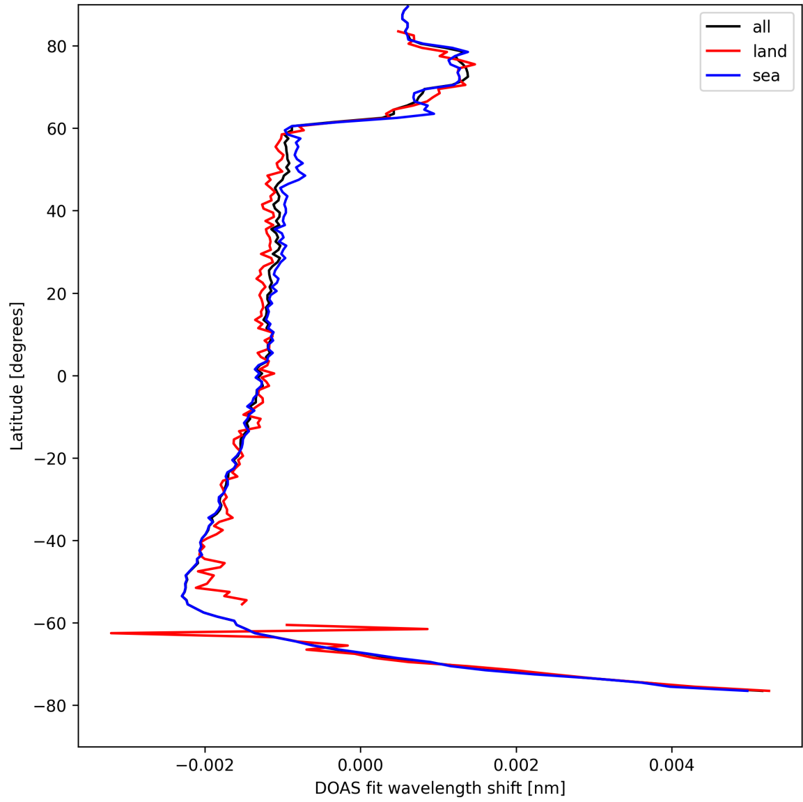
Figure 23: Zonal average of “DOAS fit wavelength shift” for 2025-04-22 to 2025-04-22.
