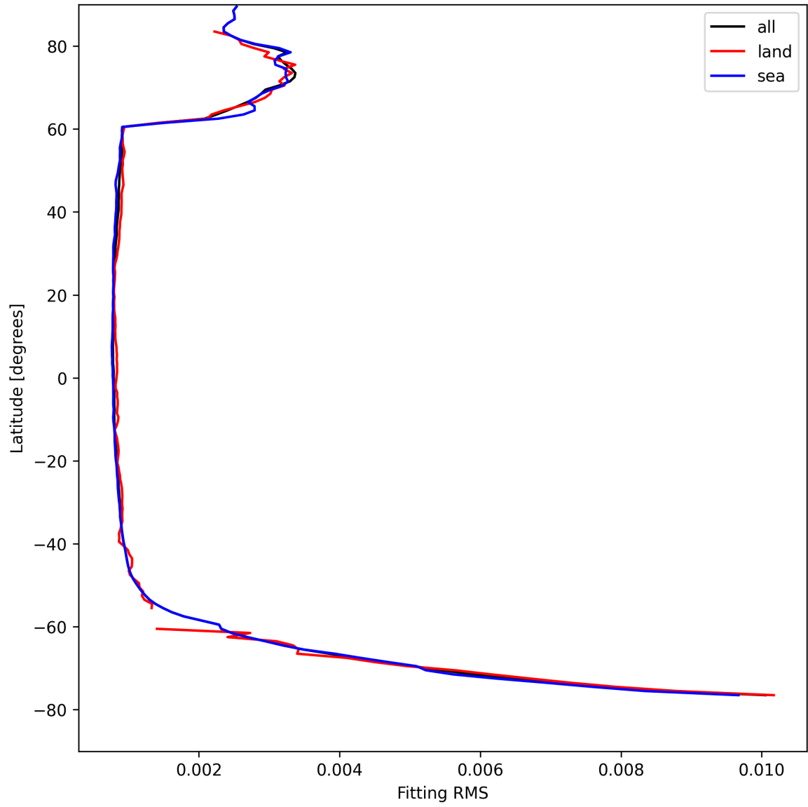
Figure 22: Zonal average of “Fitting RMS” for 2025-04-22 to 2025-04-22.
