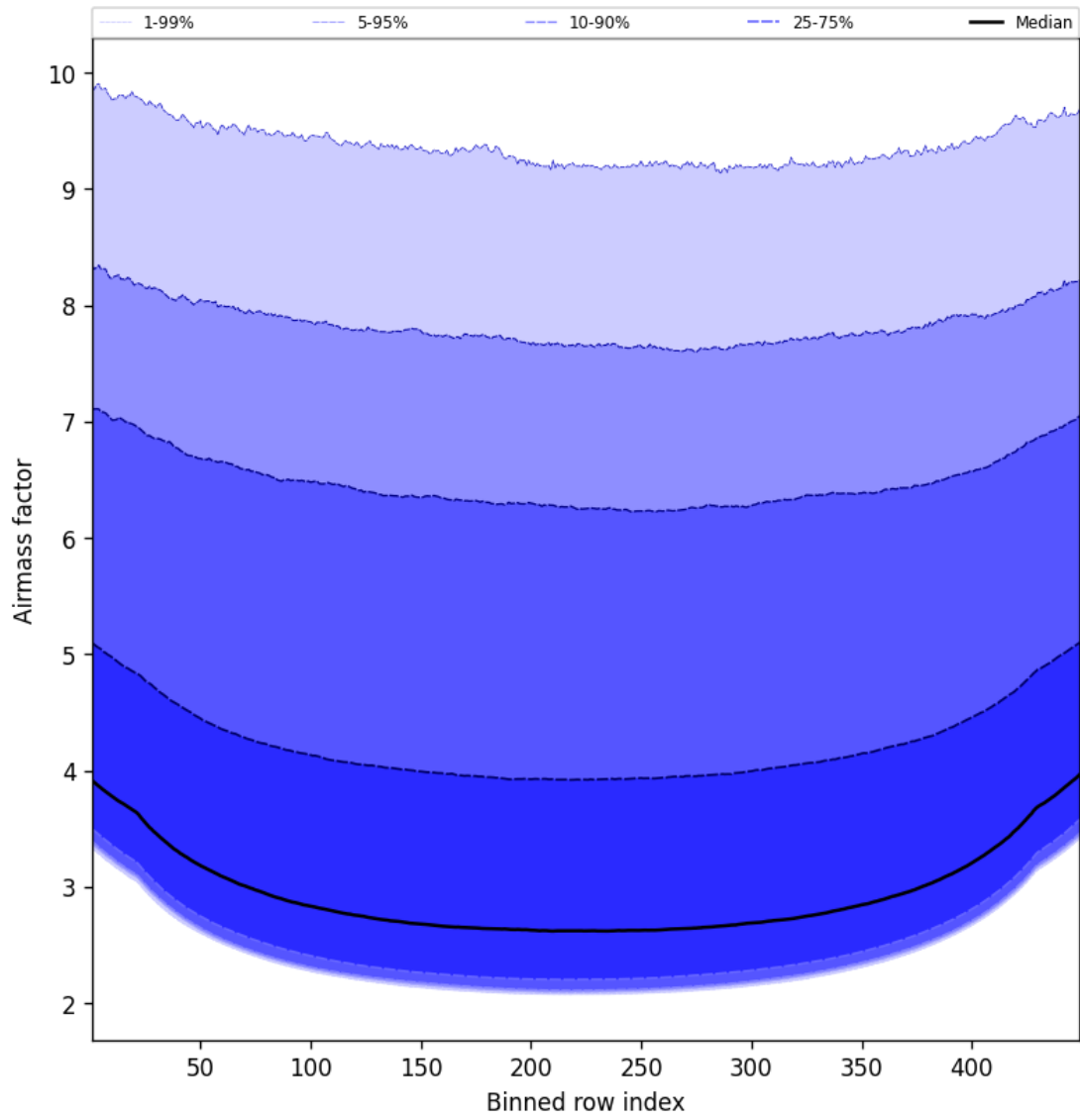
Figure 49: Along track statistics of “Airmass factor” for 2025-04-22 to 2025-04-22
