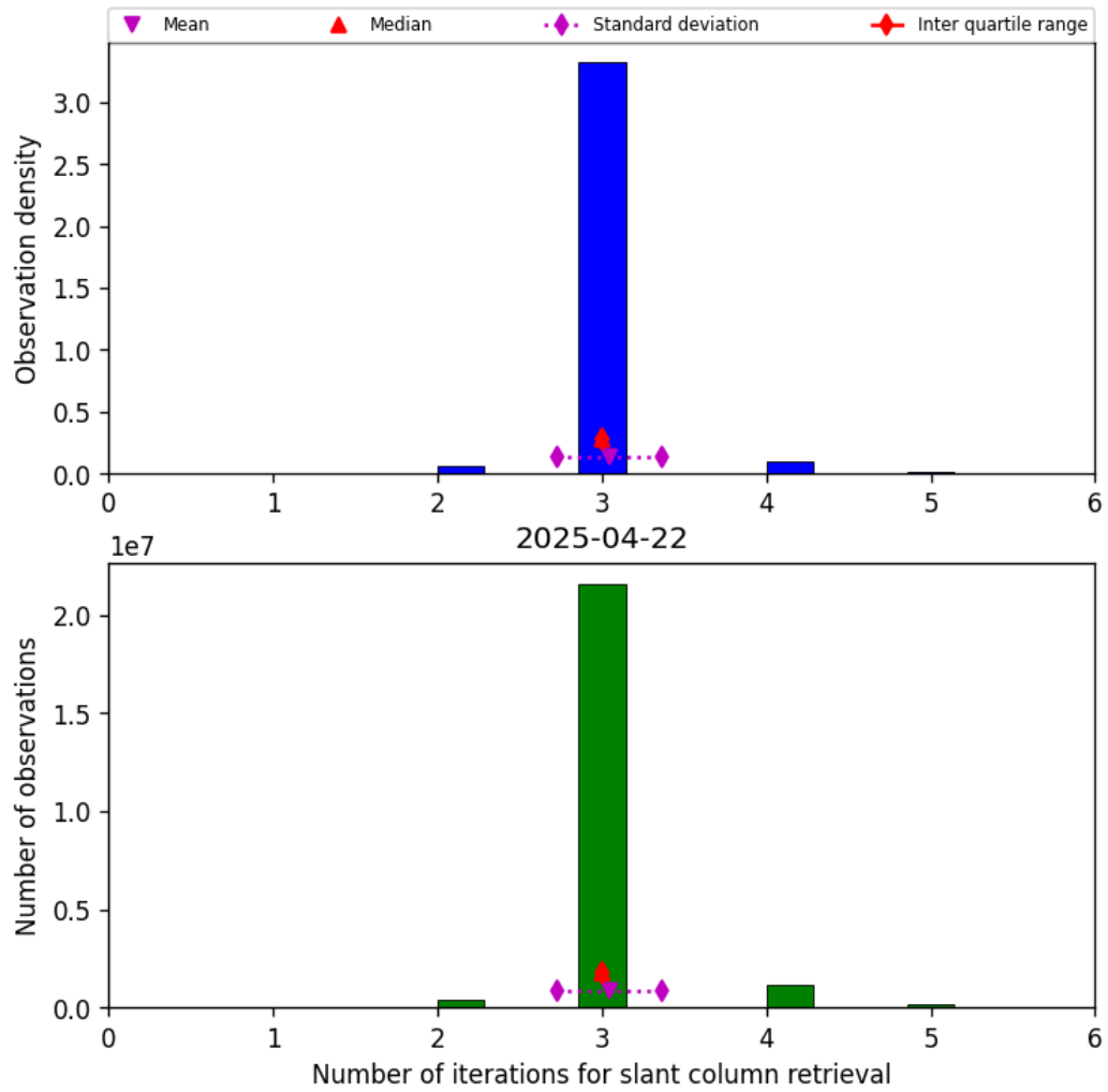
Figure 33: Histogram of "Number of iterations for slant column retrieval" for 2025-04-22 to 2025-04-22
