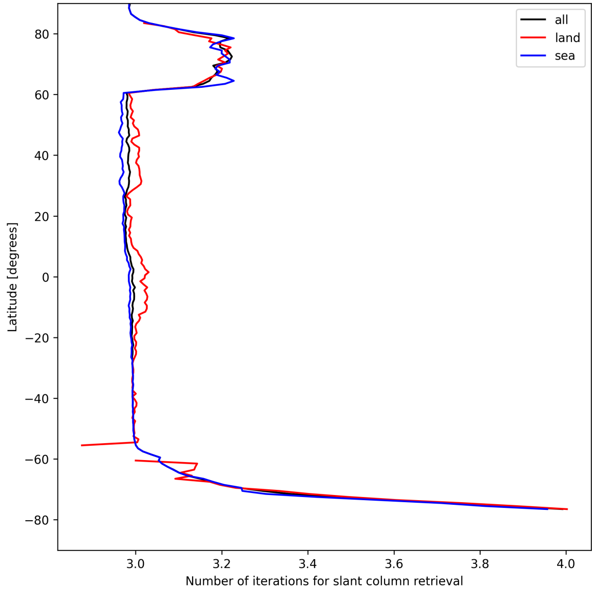
Figure 21: Zonal average of “Number of iterations for slant column retrieval” for 2025-04-22 to 2025-04-22.
