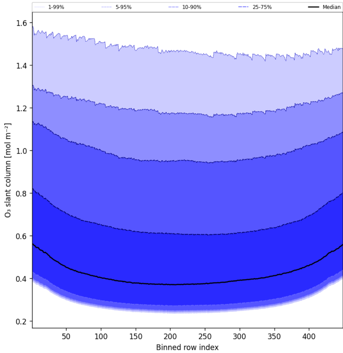
Figure 43: Along track statistics of “O 3 slant column” for 2025-04-22 to 2025-04-22
