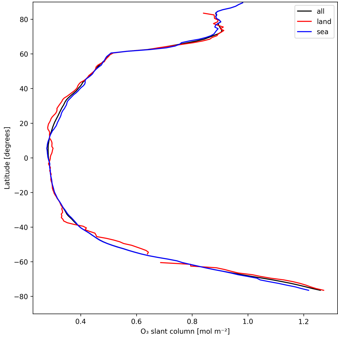
Figure 19: Zonal average of “O 3 slant column” for 2025-04-22 to 2025-04-22.
