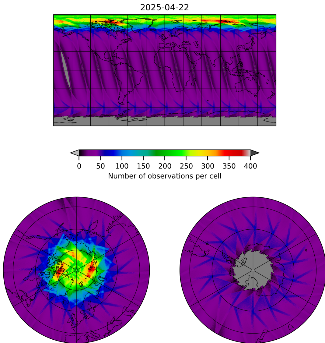
Figure 15: Map of the number of observations for 2025-04-22 to 2025-04-22
