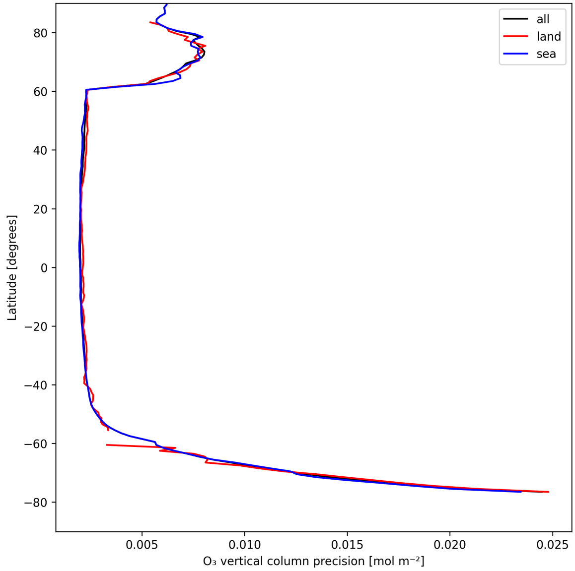
Figure 18: Zonal average of “O 3 vertical column precision” for 2025-04-22 to 2025-04-22.
