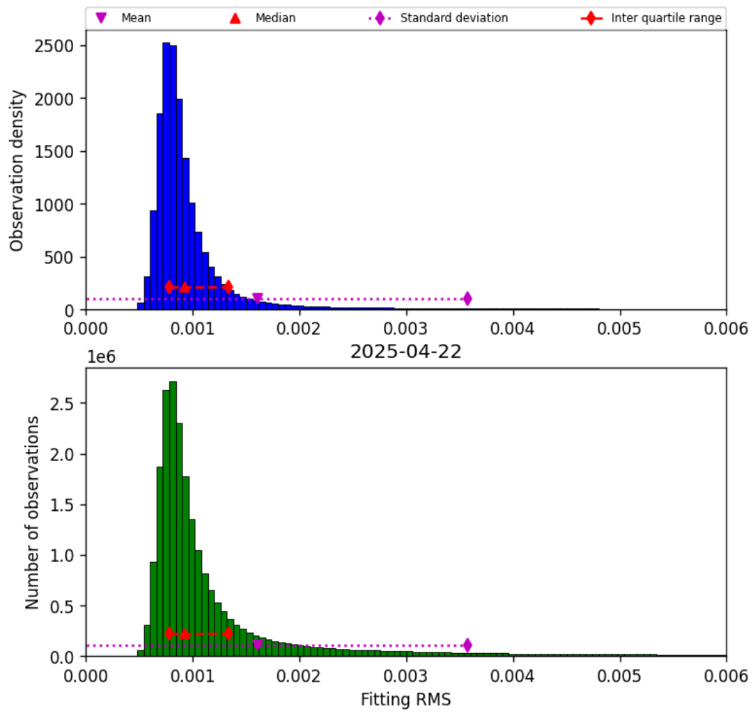
Figure 34: Histogram of “Fitting RMS” for 2025-04-22 to 2025-04-22
