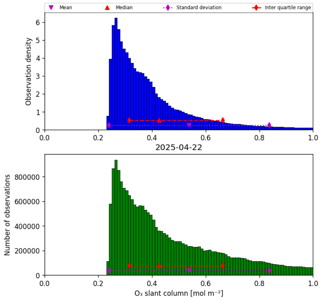
Figure 31: Histogram of “O 3 slant column” for 2025-04-22 to 2025-04-22
