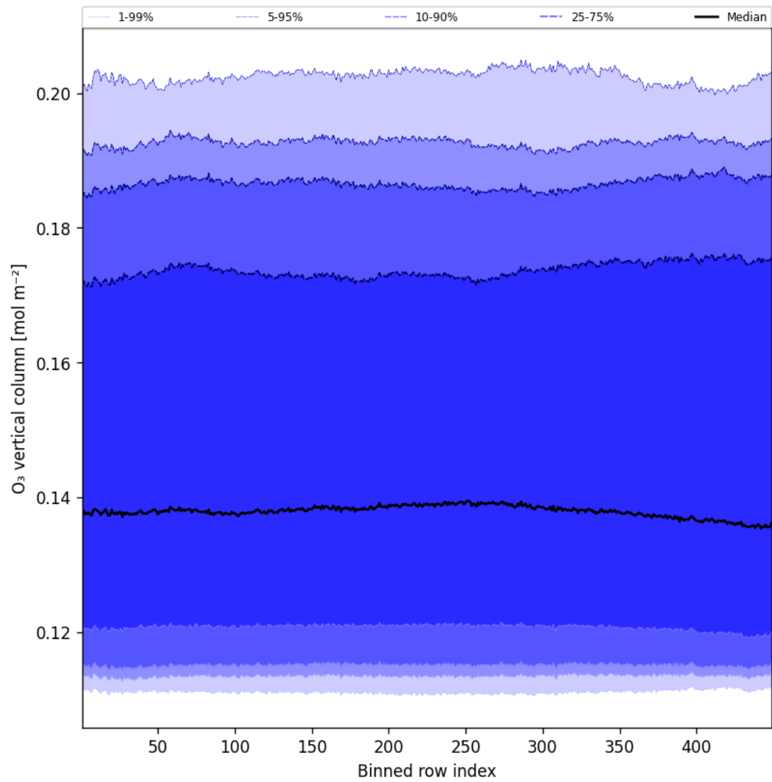
Figure 41: Along track statistics of “ O_3 vertical column” for 2025-04-23 to 2025-04-24
