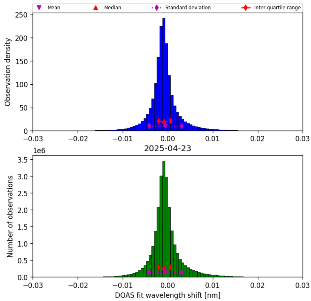
Figure 35: Histogram of “DOAS fit wavelength shift” for 2025-04-23 to 2025-04-24
