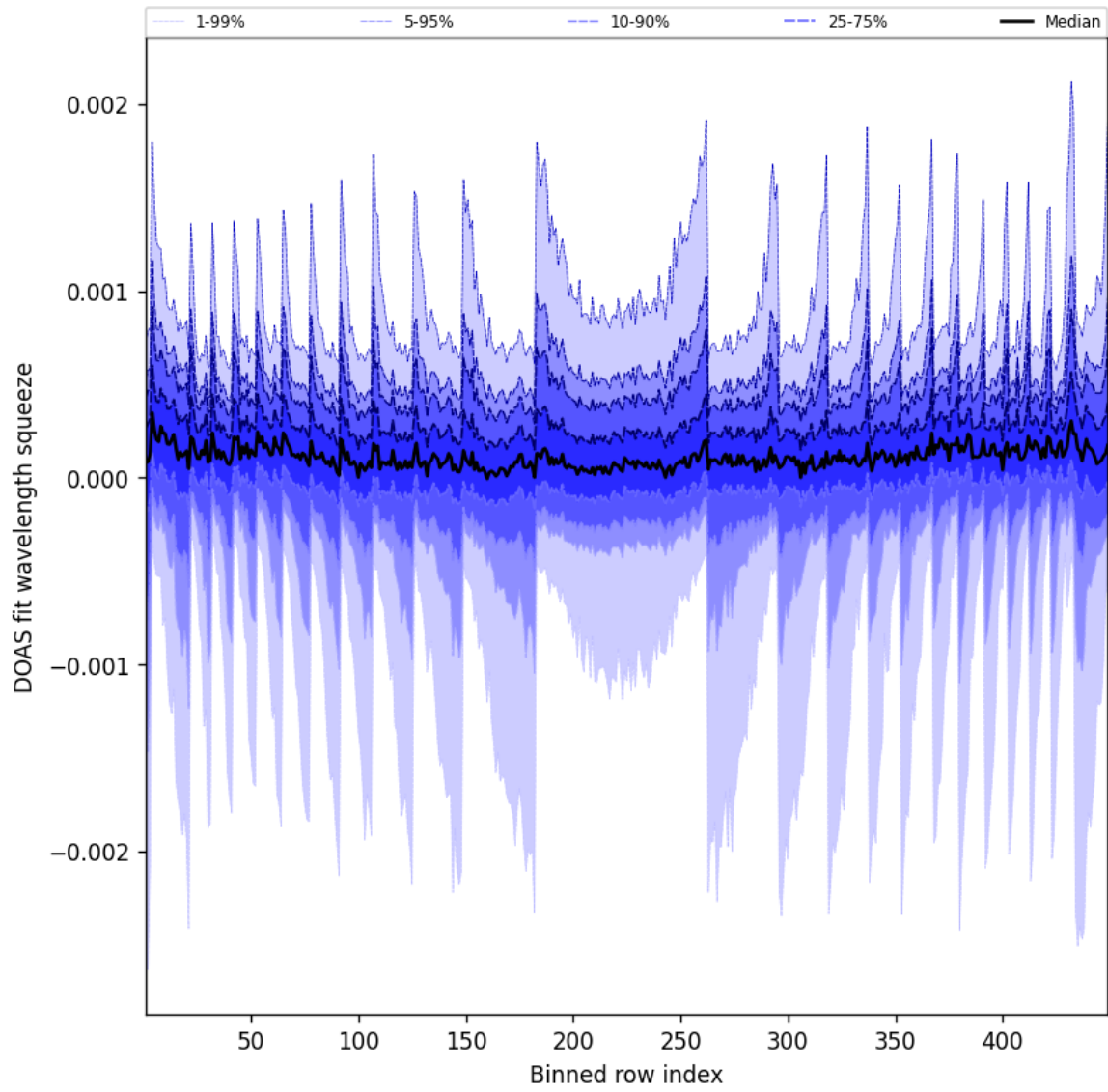
Figure 48: Along track statistics of “DOAS fit wavelength squeeze” for 2025-04-23 to 2025-04-24
