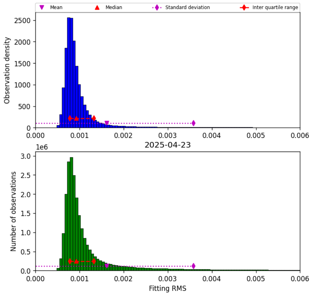
Figure 34: Histogram of “Fitting RMS” for 2025-04-23 to 2025-04-24
