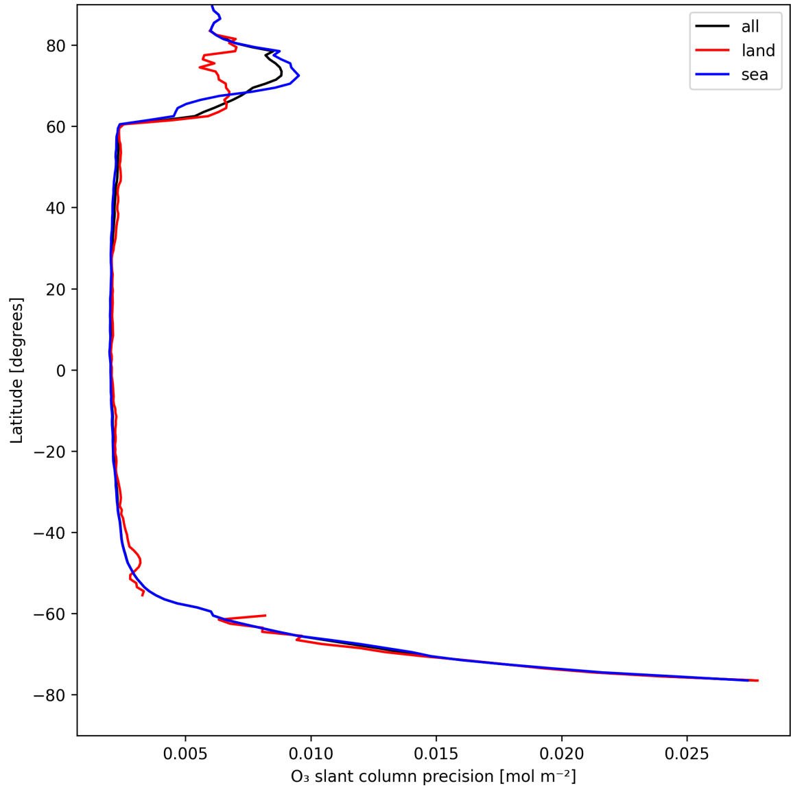
Figure 20: Zonal average of "O 3 slant column precision" for 2025-04-23 to 2025-04-24.
