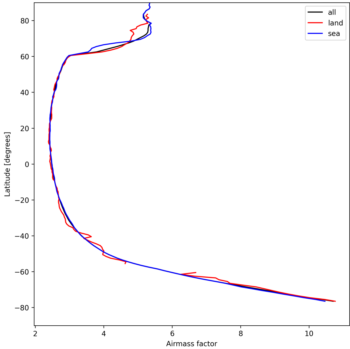
Figure 25: Zonal average of “Airmass factor” for 2025-04-23 to 2025-04-24.
