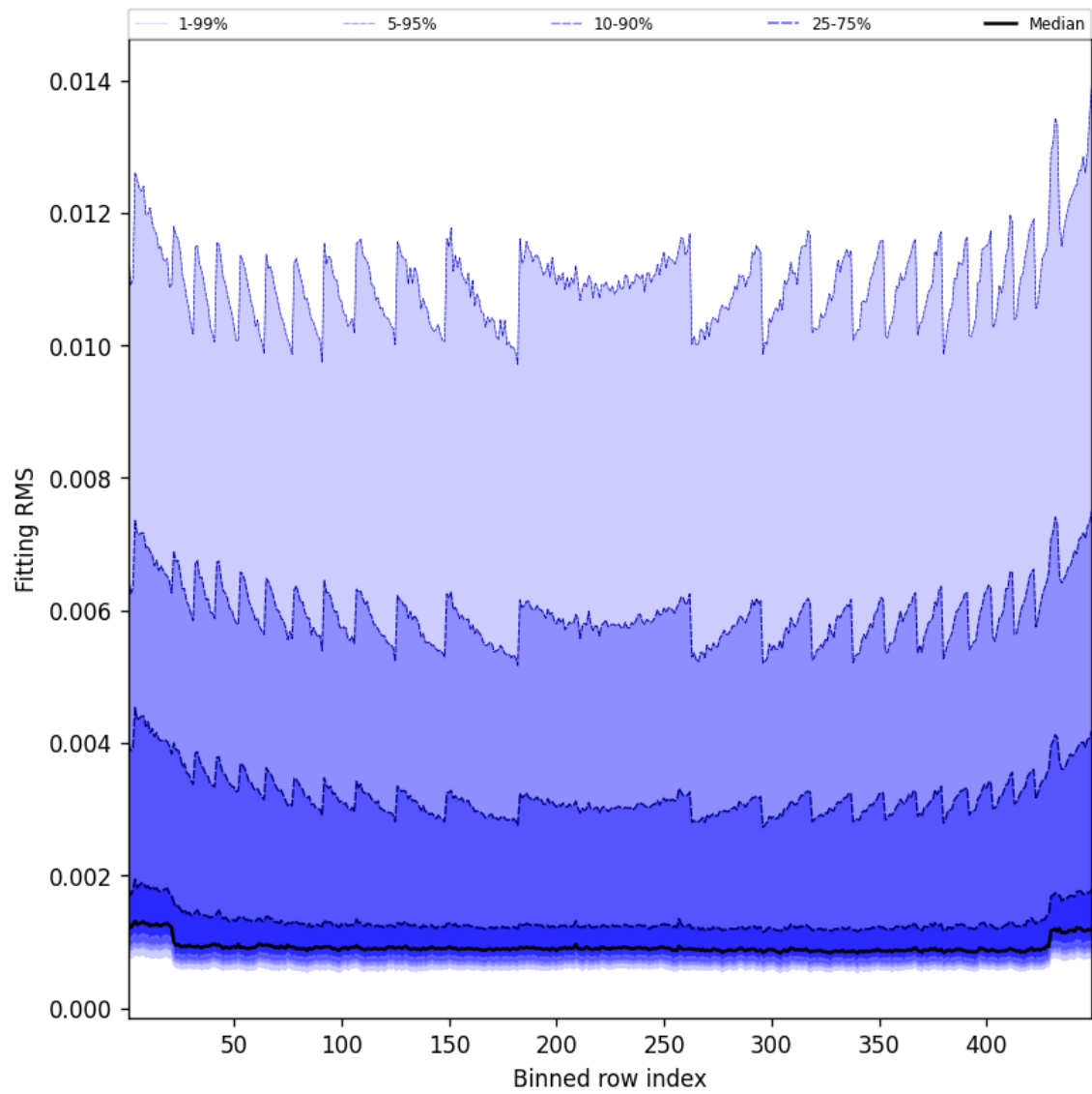
Figure 46: Along track statistics of “Fitting RMS” for 2025-04-23 to 2025-04-24
