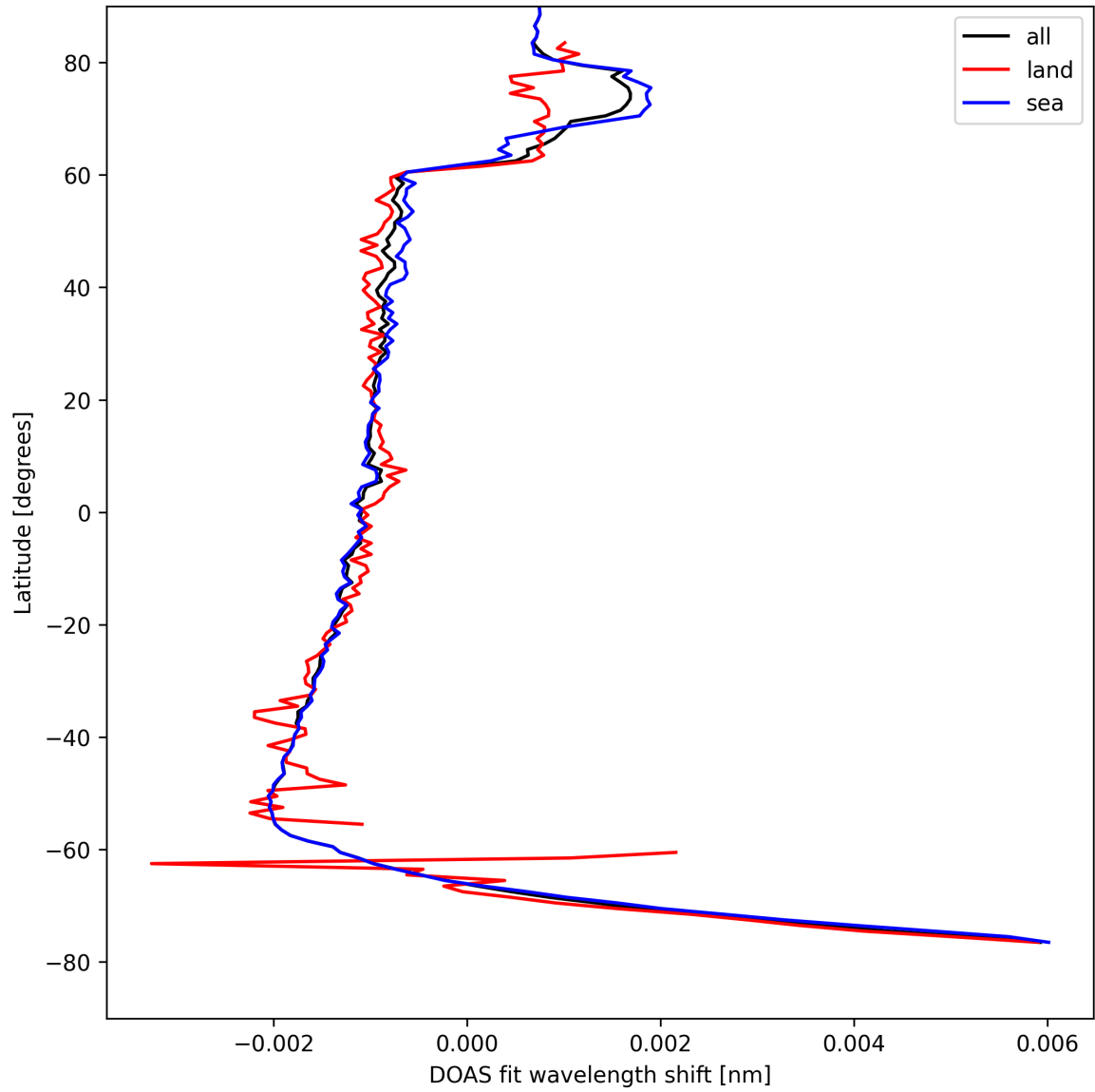
Figure 23: Zonal average of “DOAS fit wavelength shift” for 2025-04-23 to 2025-04-24.
