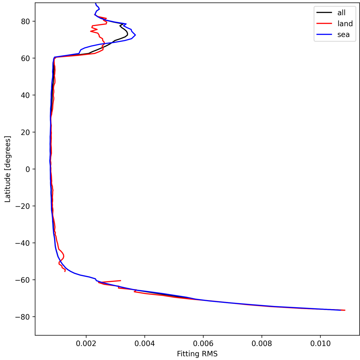
Figure 22: Zonal average of “Fitting RMS” for 2025-04-23 to 2025-04-24.
