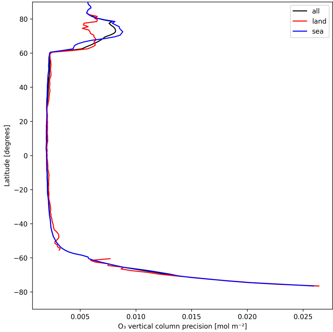
Figure 18: Zonal average of "O 3 vertical column precision" for 2025-04-23 to 2025-04-24.
