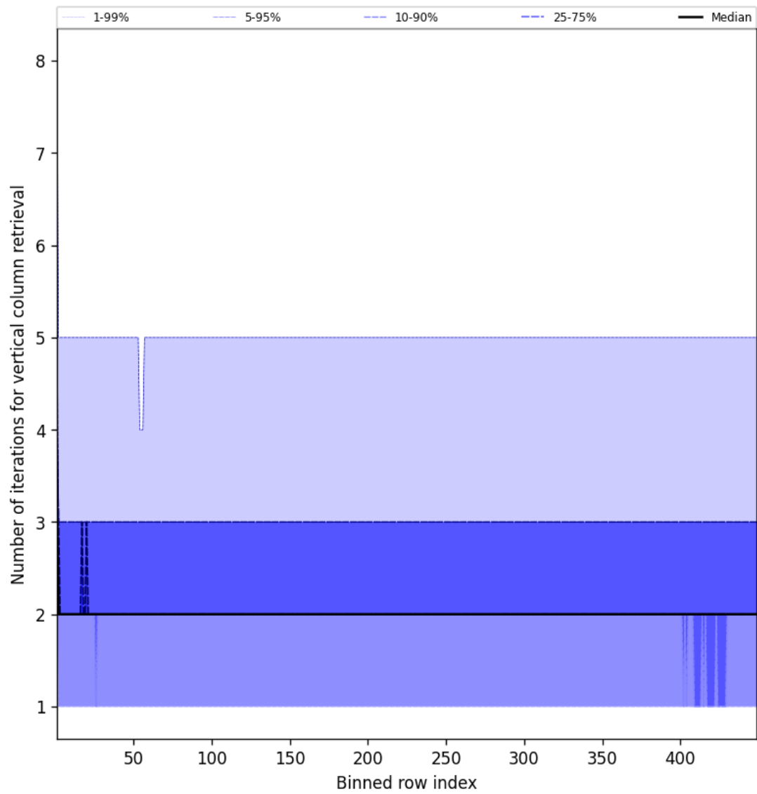
Figure 51: Along track statistics of “Number of iterations for vertical column retrieval” for 2025-04-23 to 2025-04-24
