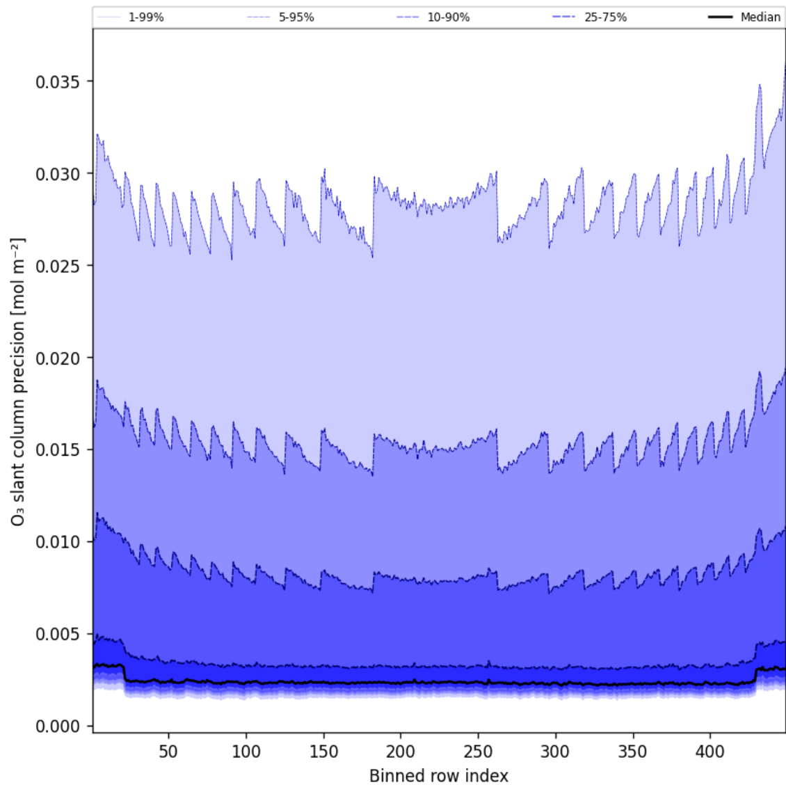
Figure 44: Along track statistics of “O 3 slant column precision” for 2025-04-23 to 2025-04-24
