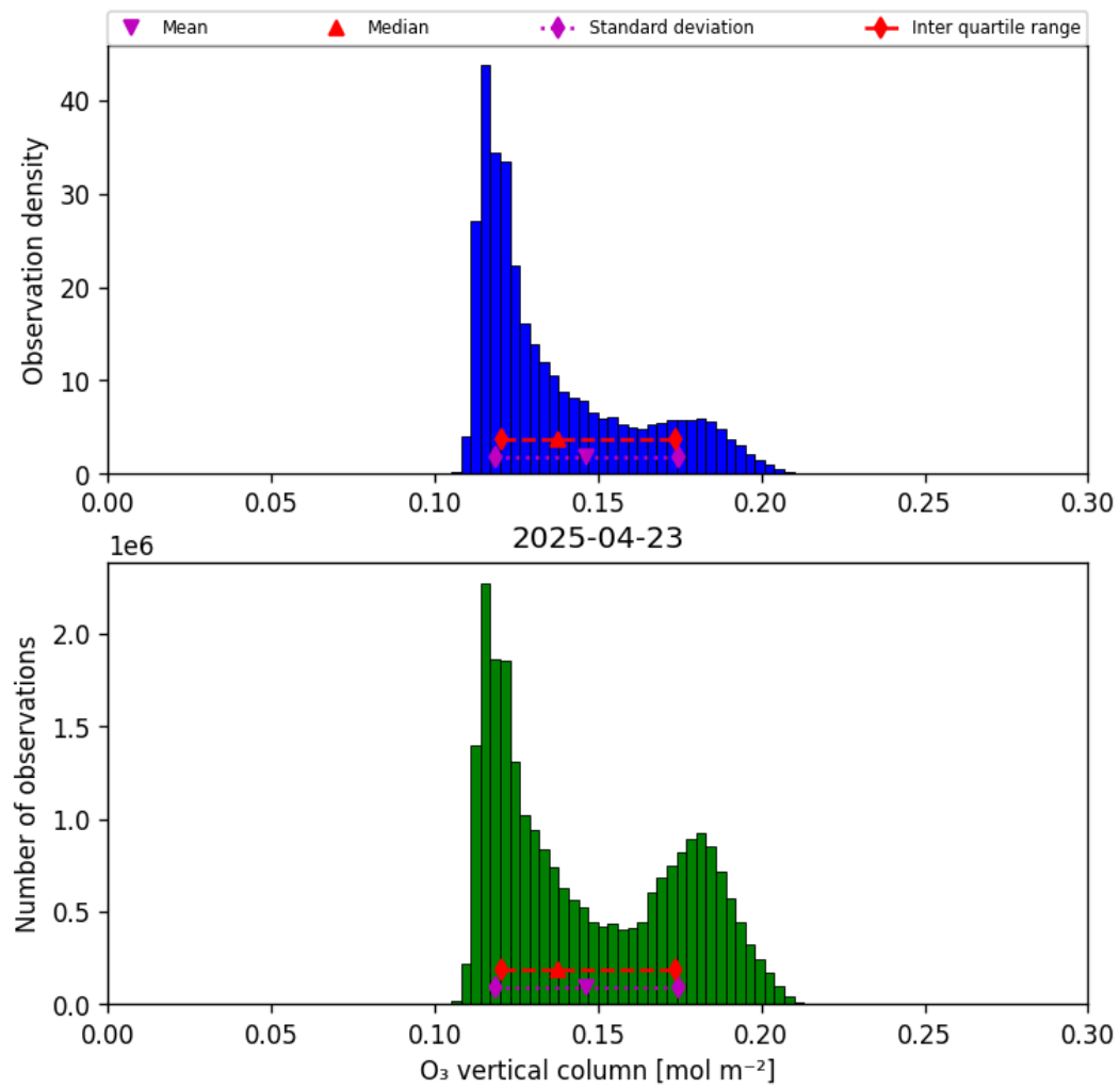
Figure 29: Histogram of “O 3 vertical column” for 2025-04-23 to 2025-04-24
