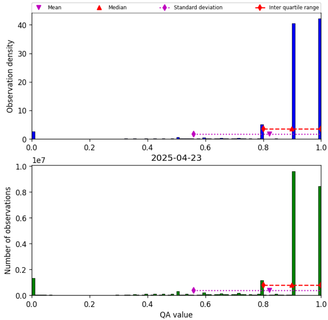
Figure 28: Histogram of “QA value” for 2025-04-23 to 2025-04-24
