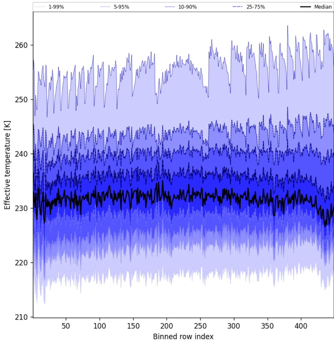
Figure 50: Along track statistics of “Effective temperature” for 2025-04-23 to 2025-04-24
