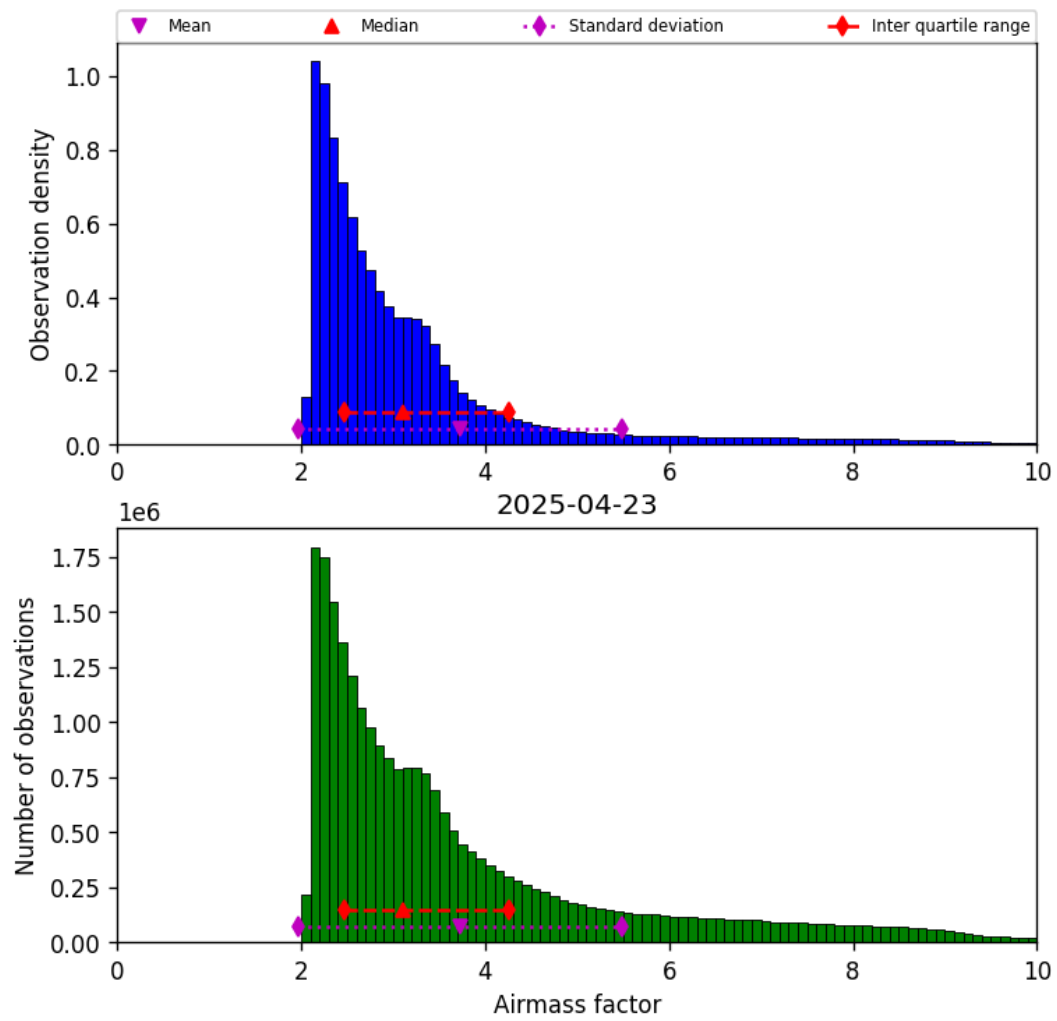
Figure 37: Histogram of “Airmass factor” for 2025-04-23 to 2025-04-24
