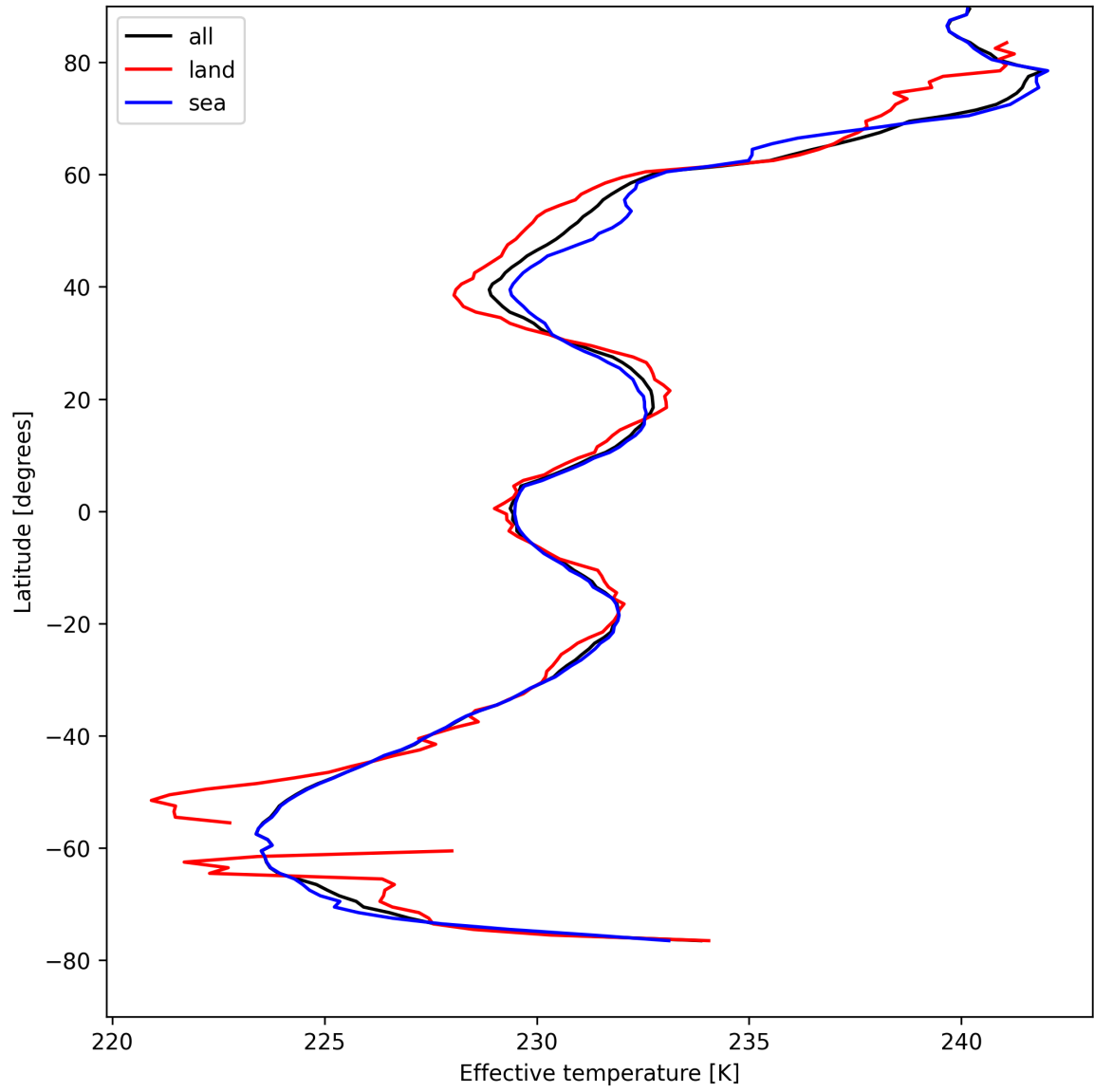
Figure 26: Zonal average of “Effective temperature” for 2025-04-23 to 2025-04-24.
