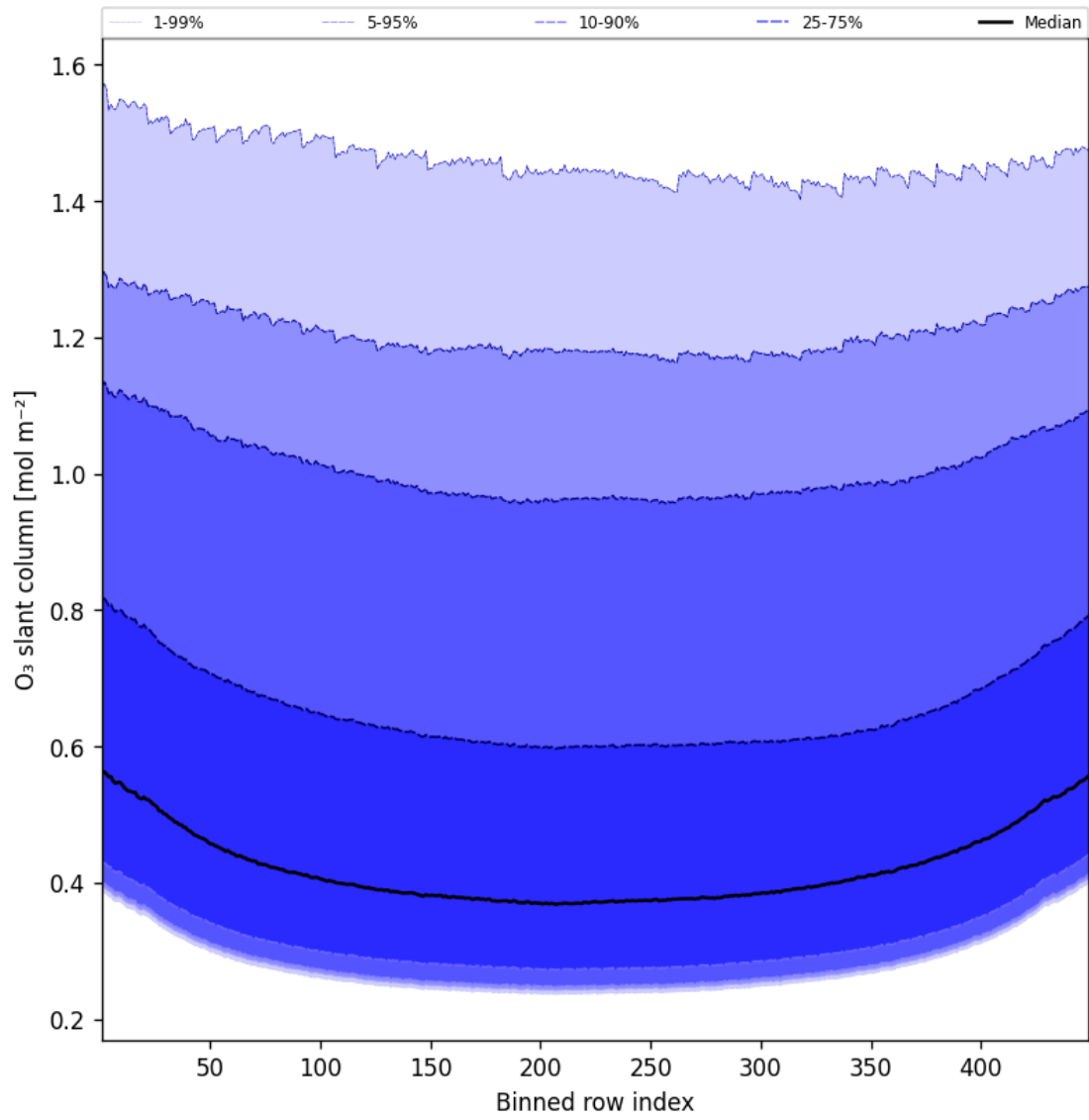
Figure 43: Along track statistics of “O 3 slant column” for 2025-04-23 to 2025-04-24
