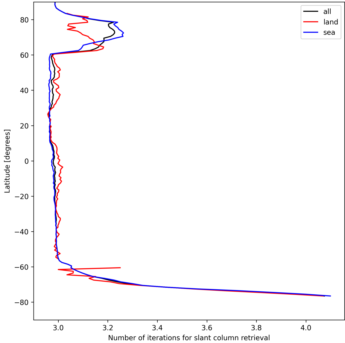
Figure 21: Zonal average of “Number of iterations for slant column retrieval” for 2025-04-23 to 2025-04-24.
