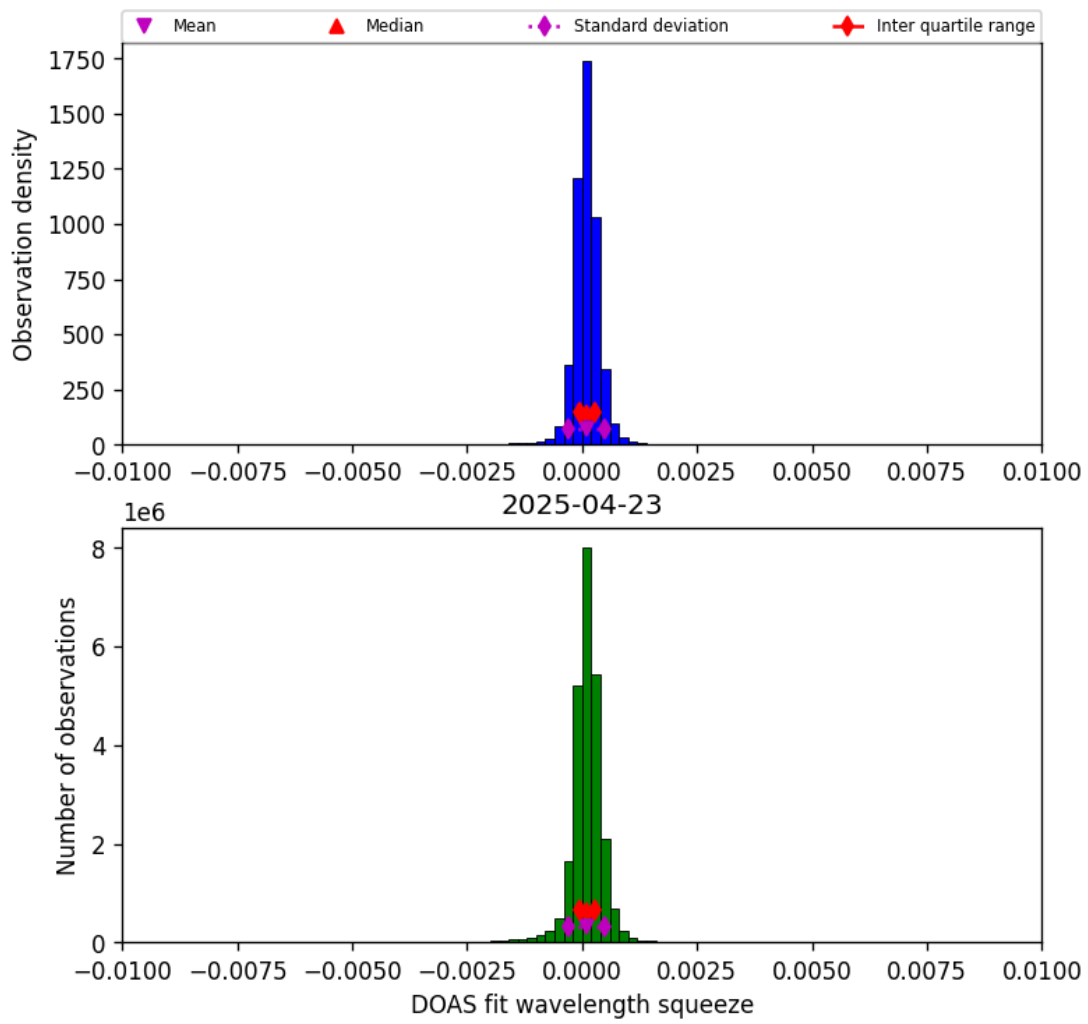
Figure 36: Histogram of “DOAS fit wavelength squeeze” for 2025-04-23 to 2025-04-24
