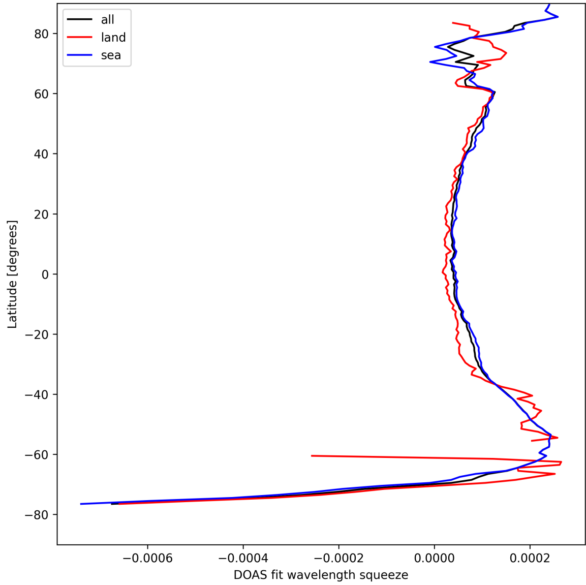
Figure 24: Zonal average of “DOAS fit wavelength squeeze” for 2025-04-23 to 2025-04-24.
