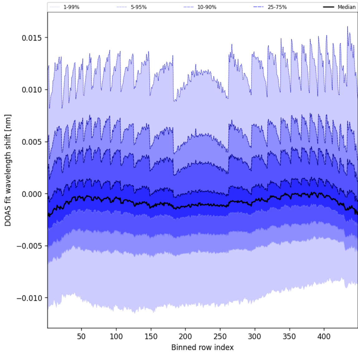
Figure 47: Along track statistics of “DOAS fit wavelength shift” for 2025-04-23 to 2025-04-24
