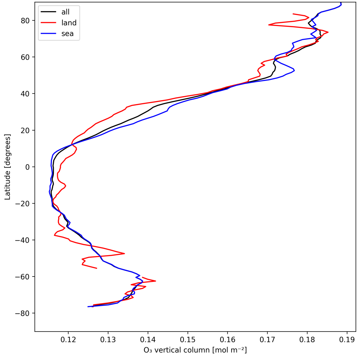
Figure 17: Zonal average of “O 3 vertical column” for 2025-04-23 to 2025-04-24.
