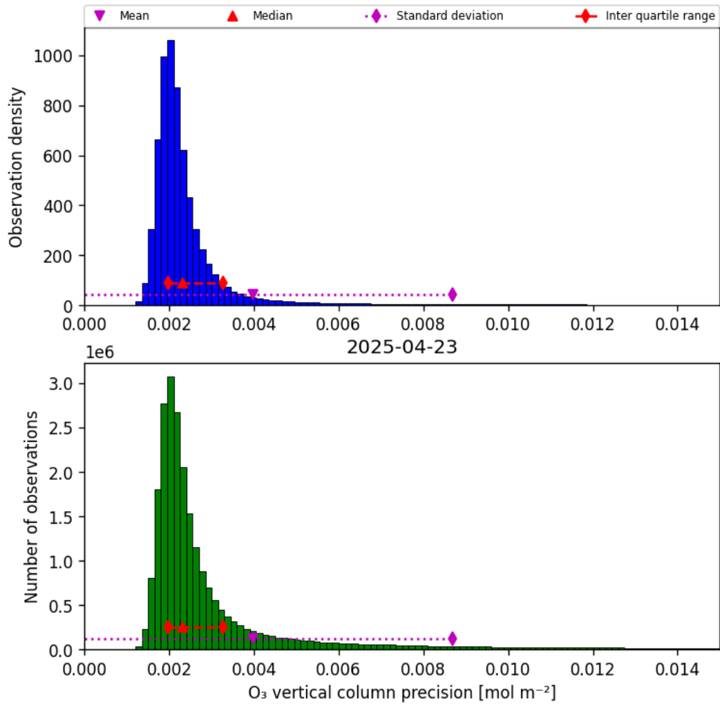
Figure 30: Histogram of “O 3 vertical column precision” for 2025-04-23 to 2025-04-24
