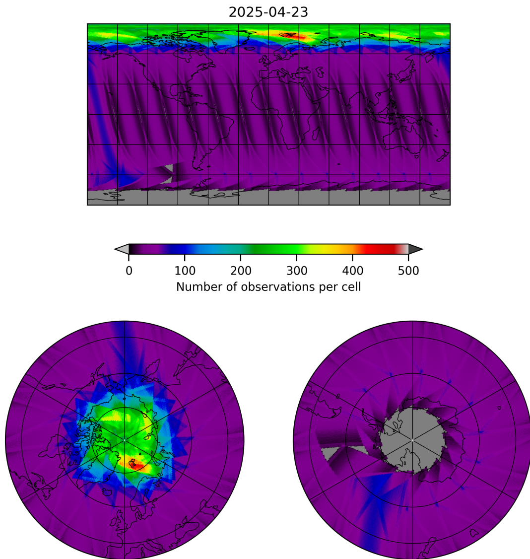
Figure 15: Map of the number of observations for 2025-04-23 to 2025-04-24
