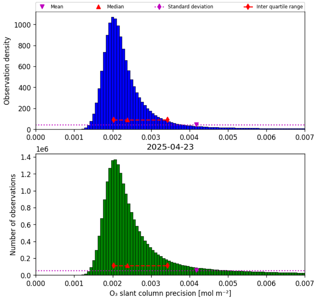
Figure 32: Histogram of “O 3 slant column precision” for 2025-04-23 to 2025-04-24
