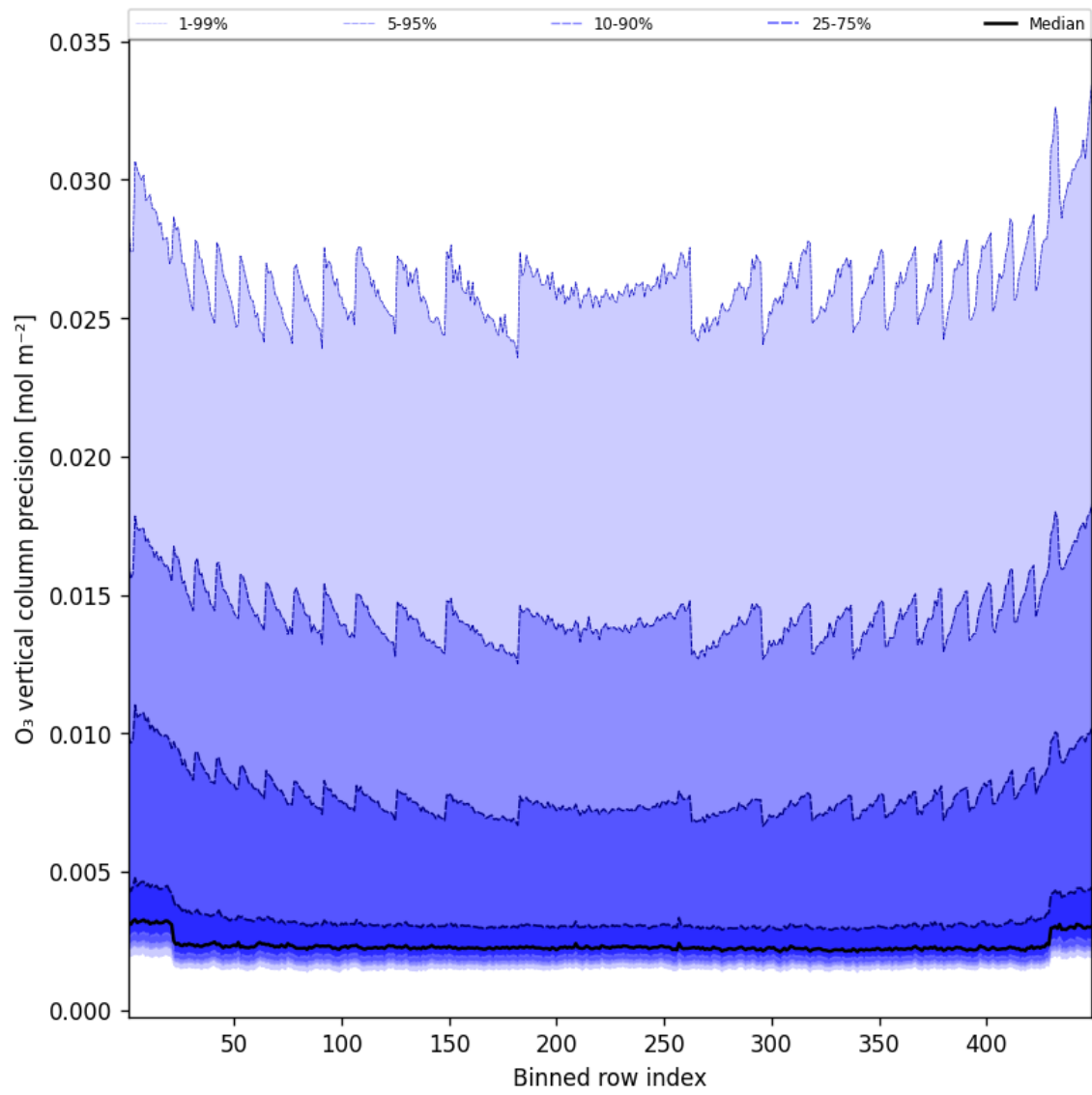
Figure 42: Along track statistics of “O 3 vertical column precision” for 2025-04-23 to 2025-04-24
