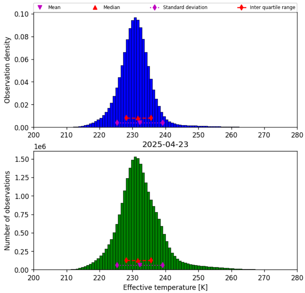
Figure 38: Histogram of “Effective temperature” for 2025-04-23 to 2025-04-24
