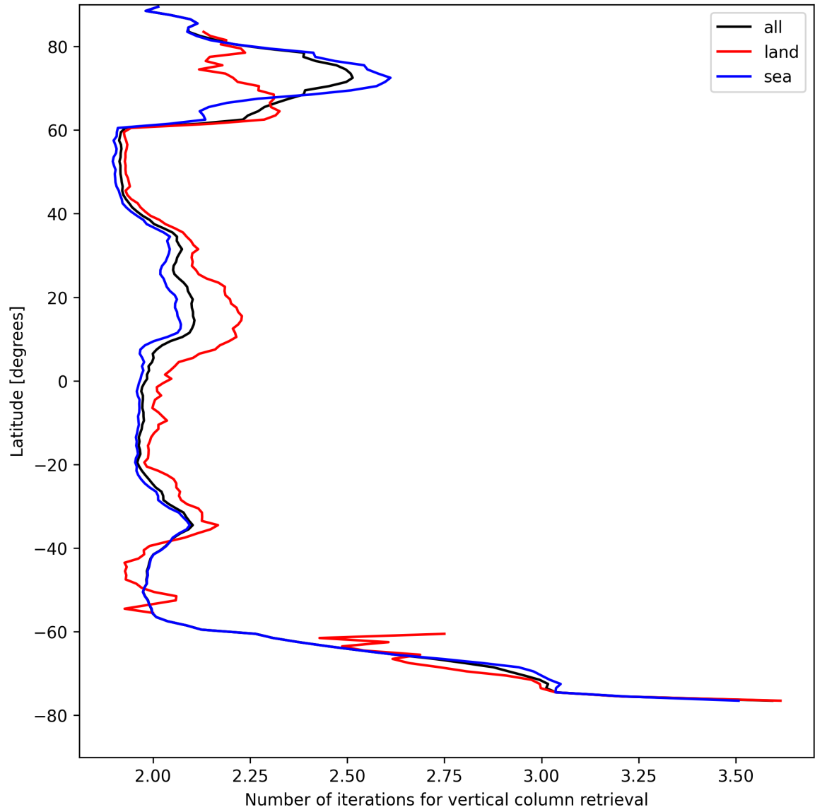
Figure 27: Zonal average of “Number of iterations for vertical column retrieval” for 2025-04-23 to 2025-04-24.
