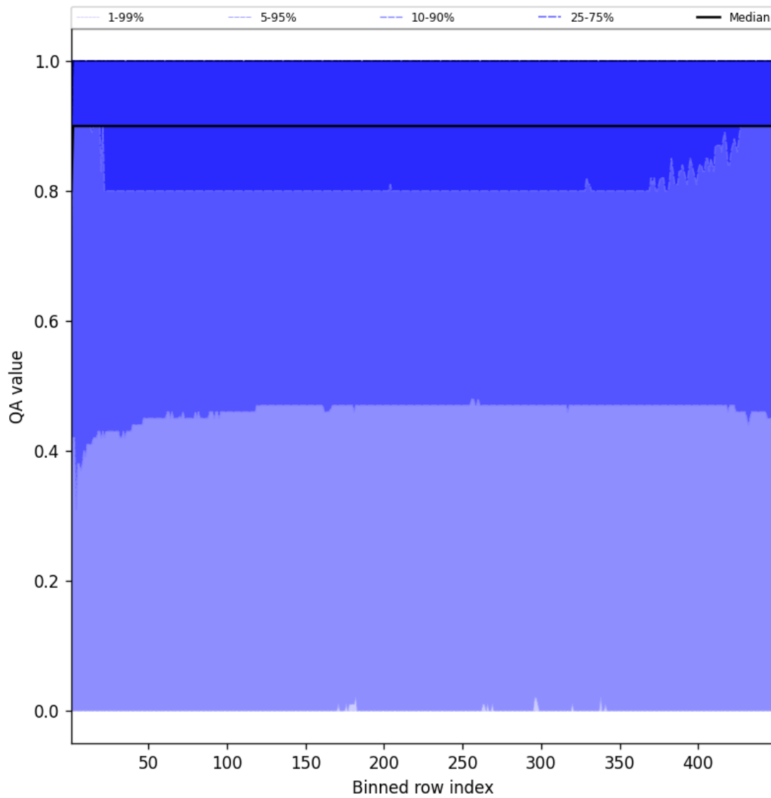
Figure 40: Along track statistics of “QA value” for 2025-04-23 to 2025-04-24
