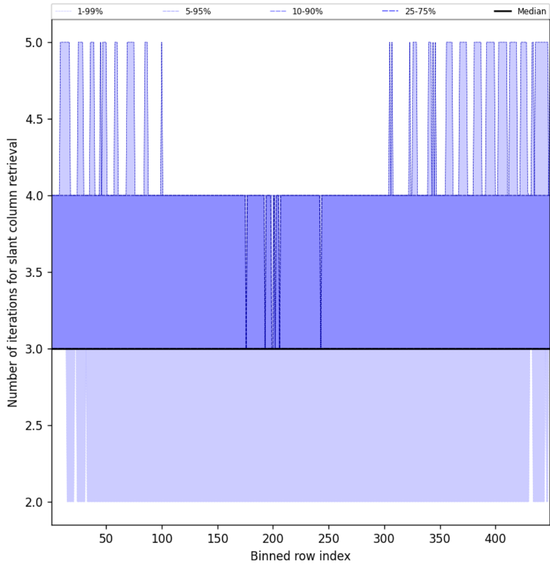
Figure 45: Along track statistics of “Number of iterations for slant column retrieval” for 2025-04-23 to 2025-04-24
