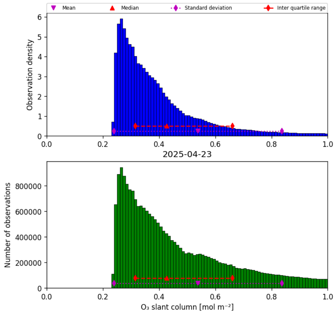
Figure 31: Histogram of “O 3 slant column” for 2025-04-23 to 2025-04-24
