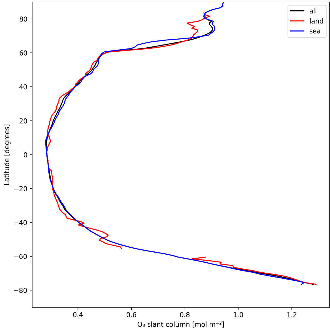
Figure 19: Zonal average of “O 3 slant column” for 2025-04-23 to 2025-04-24.
