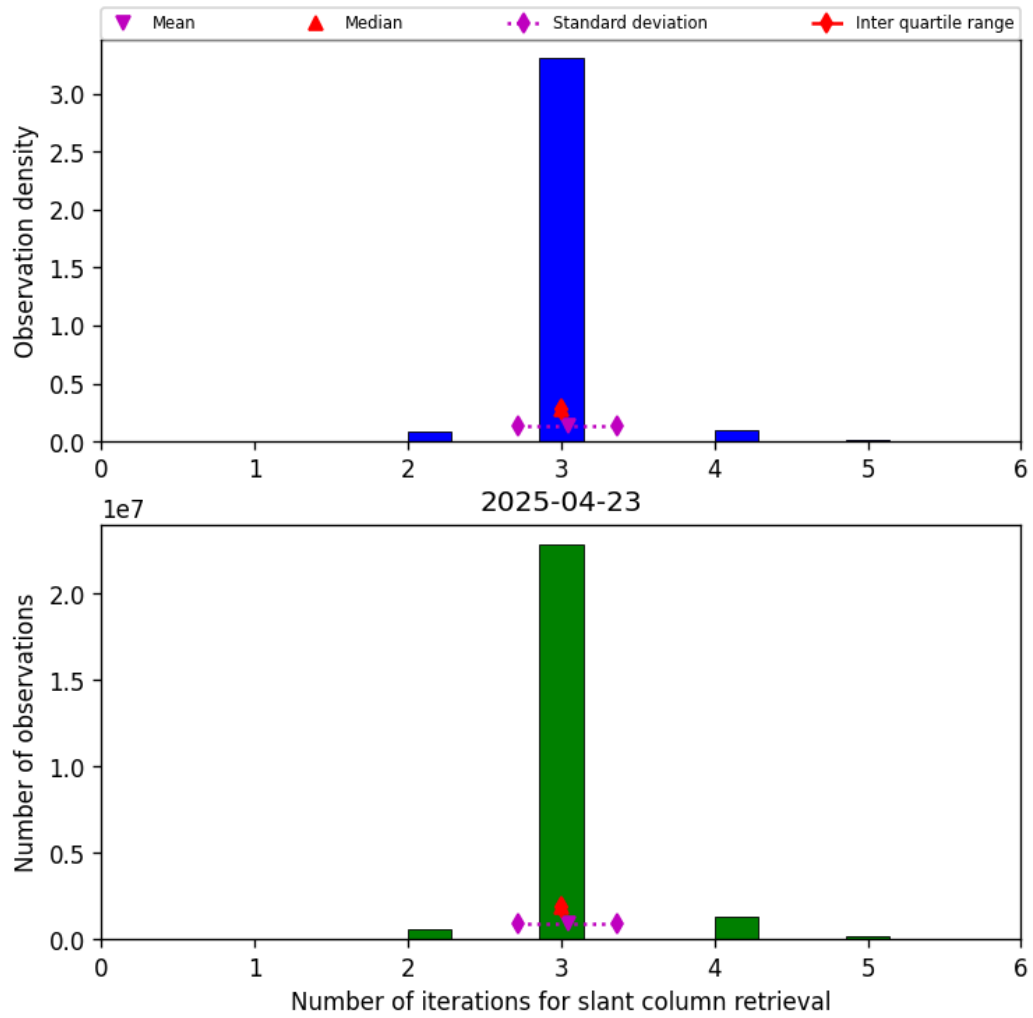
Figure 33: Histogram of “Number of iterations for slant column retrieval” for 2025-04-23 to 2025-04-24
