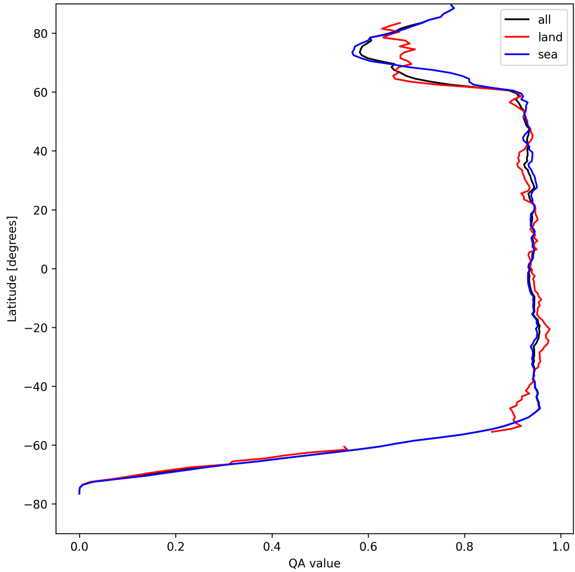
Figure 16: Zonal average of “QA value” for 2025-04-23 to 2025-04-24.
