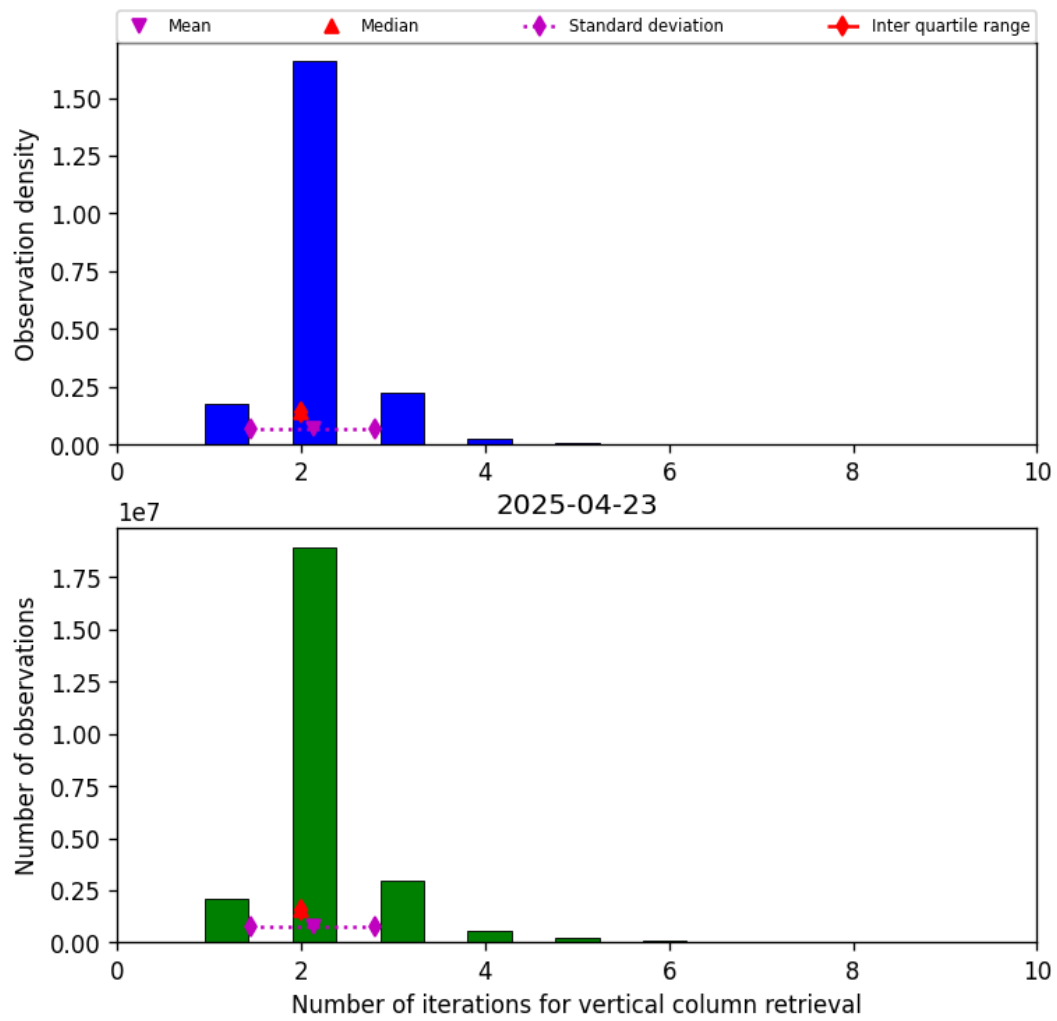
Figure 39: Histogram of “Number of iterations for vertical column retrieval” for 2025-04-23 to 2025-04-24
