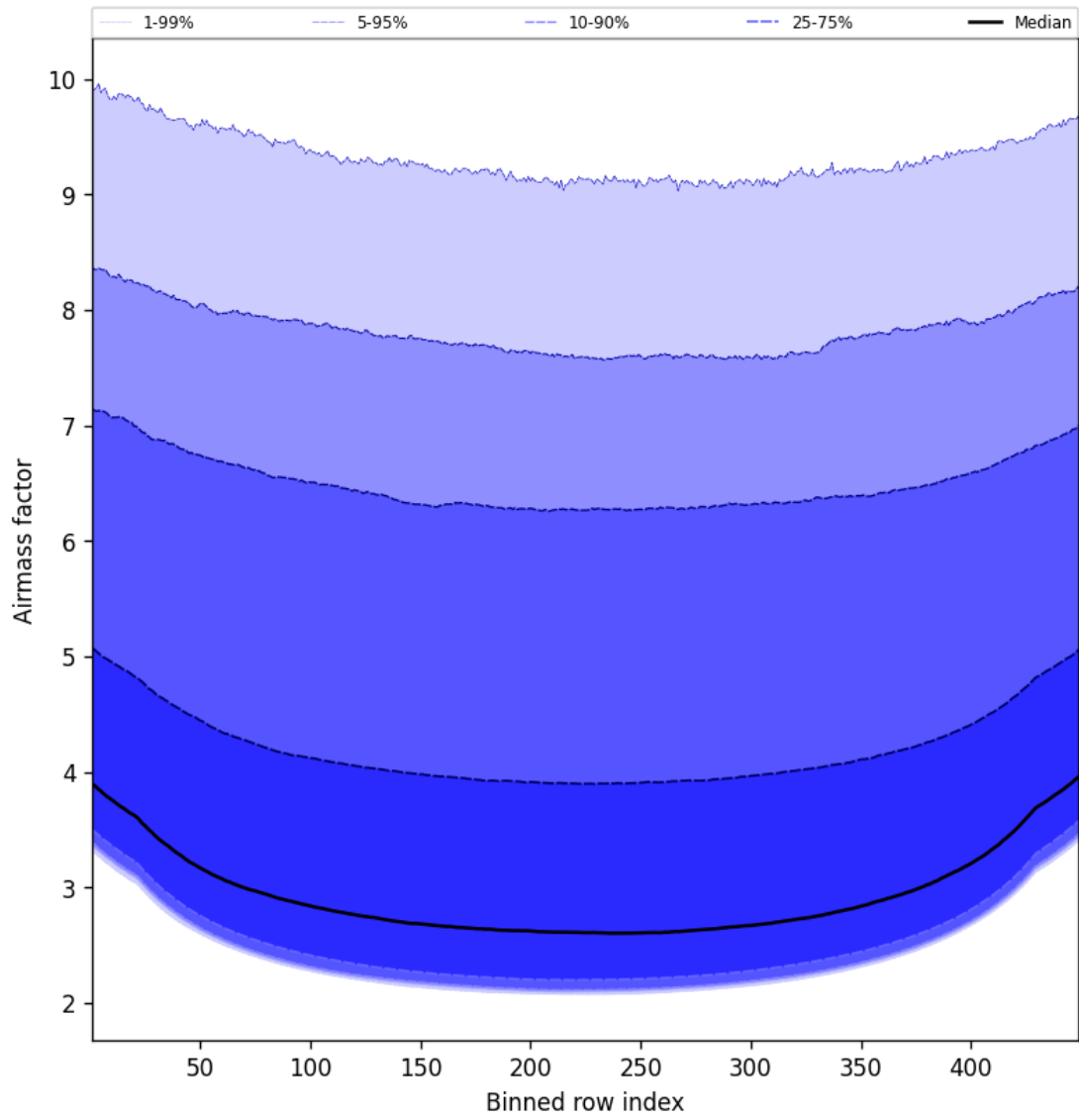
Figure 49: Along track statistics of “Airmass factor” for 2025-04-23 to 2025-04-24
