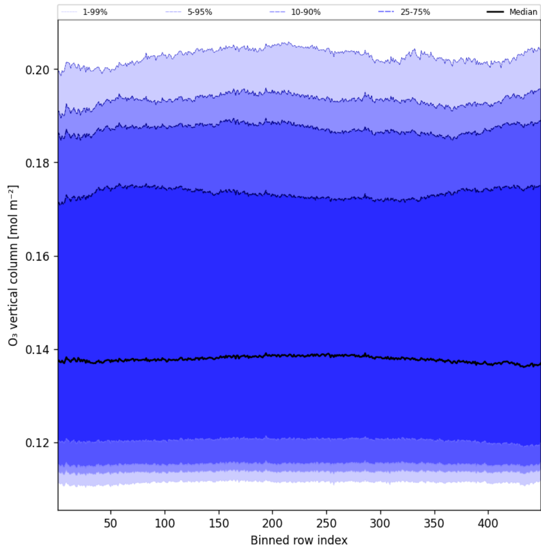
Figure 41: Along track statistics of “O 3 vertical column” for 2025-04-24 to 2025-04-25
