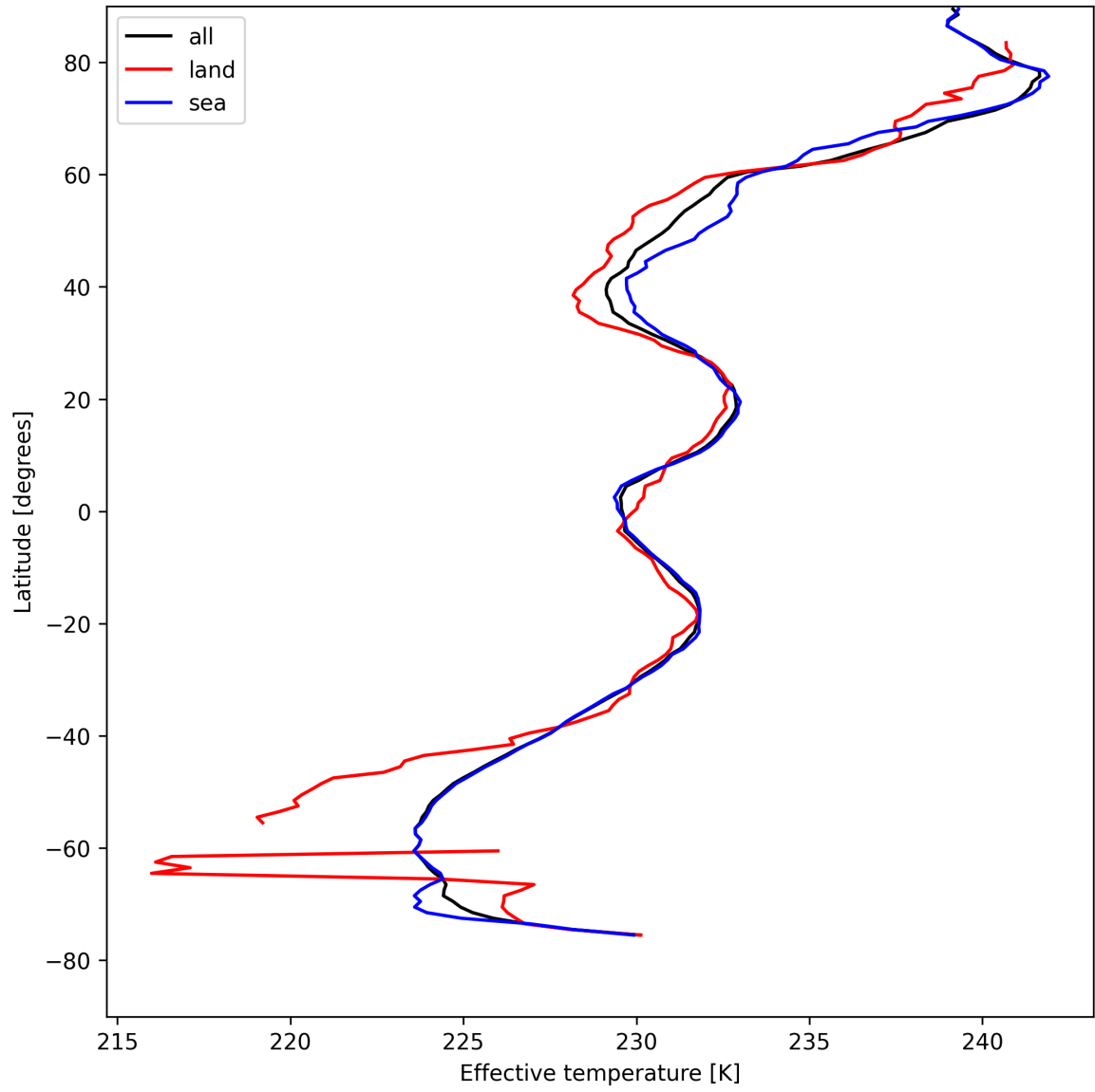
Figure 26: Zonal average of "Effective temperature" for 2025-04-24 to 2025-04-25.
