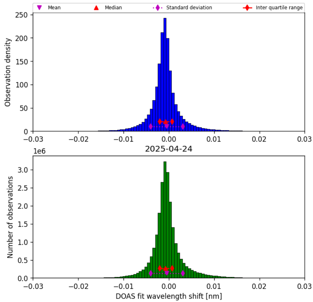
Figure 35: Histogram of “DOAS fit wavelength shift” for 2025-04-24 to 2025-04-25
