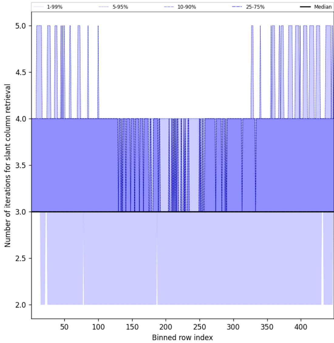
Figure 45: Along track statistics of “Number of iterations for slant column retrieval” for 2025-04-24 to 2025-04-25
