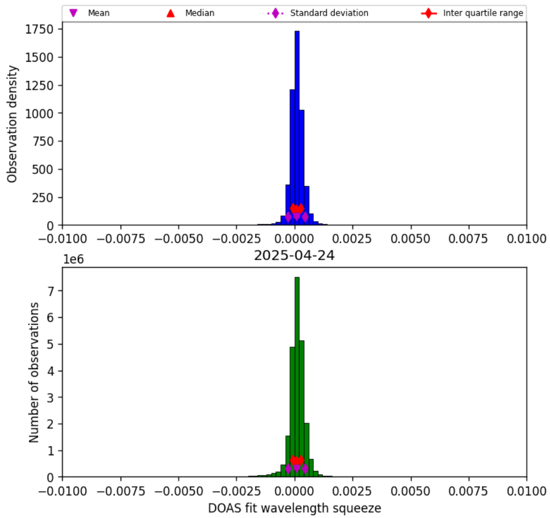
Figure 36: Histogram of “DOAS fit wavelength squeeze” for 2025-04-24 to 2025-04-25
