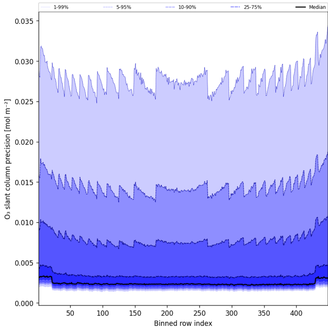
Figure 44: Along track statistics of “O 3 slant column precision” for 2025-04-24 to 2025-04-25
