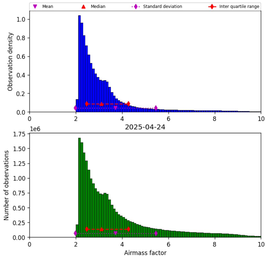
Figure 37: Histogram of “Airmass factor” for 2025-04-24 to 2025-04-25
