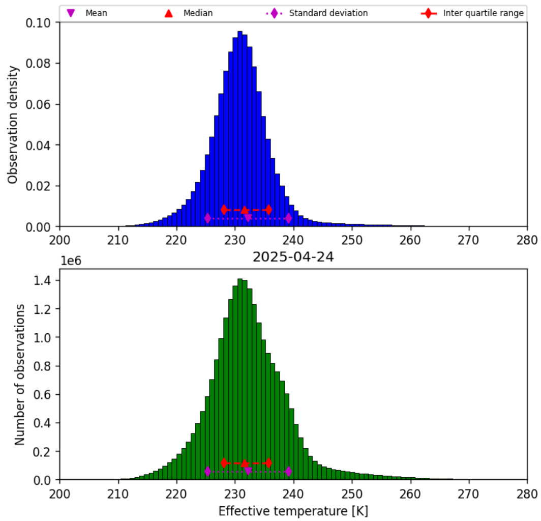
Figure 38: Histogram of “Effective temperature” for 2025-04-24 to 2025-04-25
