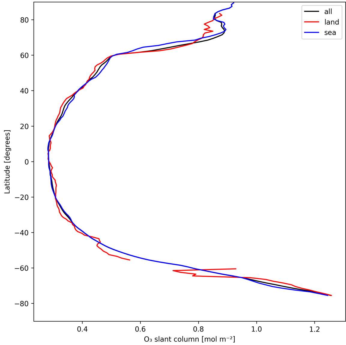
Figure 19: Zonal average of “O 3 slant column” for 2025-04-24 to 2025-04-25.
