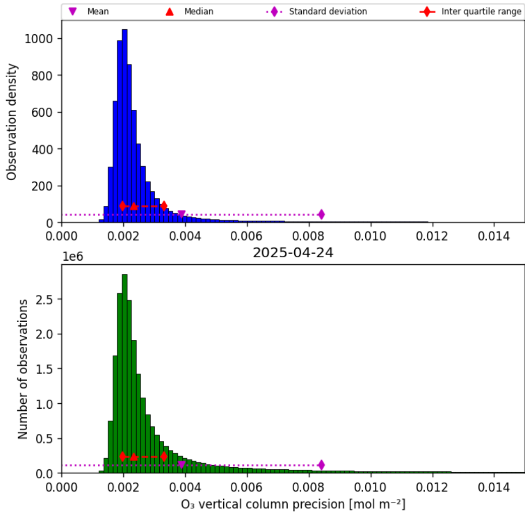
Figure 30: Histogram of “O 3 vertical column precision” for 2025-04-24 to 2025-04-25
