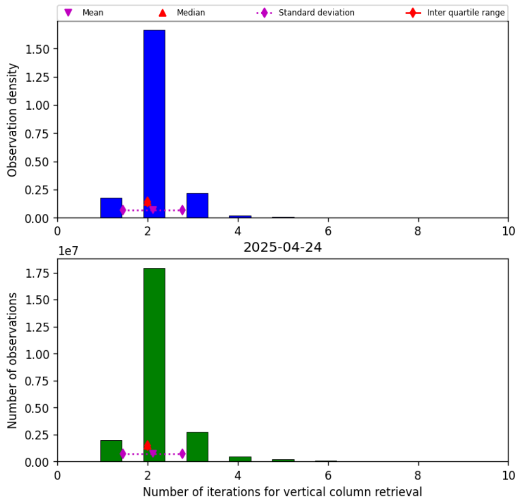
Figure 39: Histogram of “Number of iterations for vertical column retrieval” for 2025-04-24 to 2025-04-25
