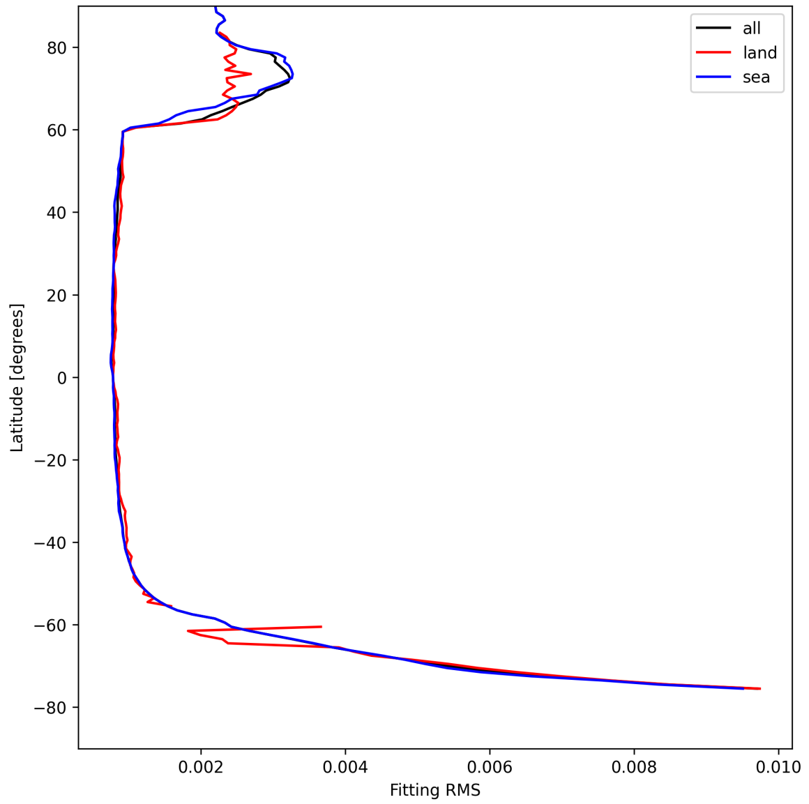
Figure 22: Zonal average of “Fitting RMS” for 2025-04-24 to 2025-04-25.
