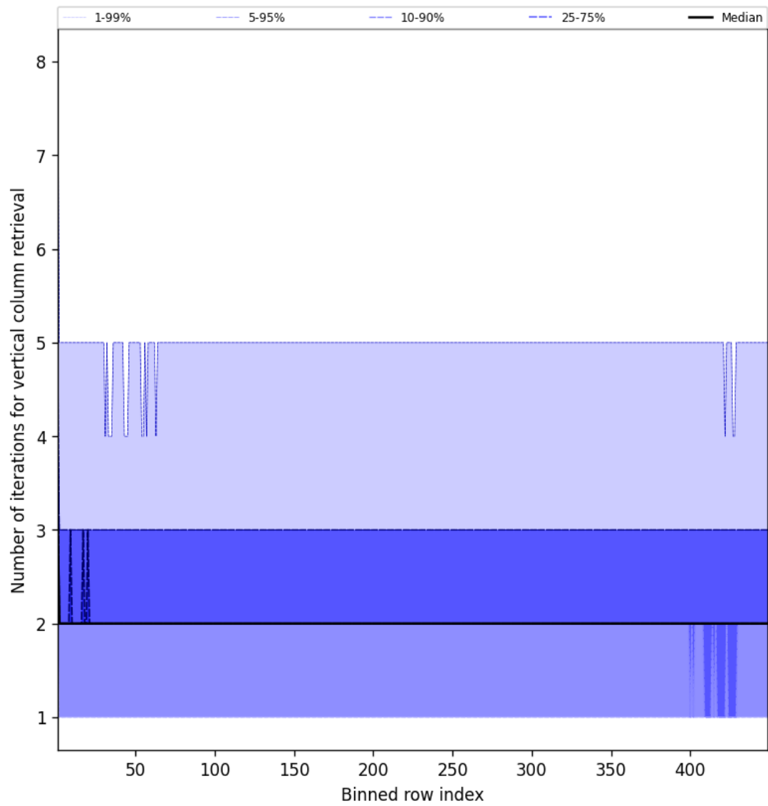
Figure 51: Along track statistics of “Number of iterations for vertical column retrieval” for 2025-04-24 to 2025-04-25
