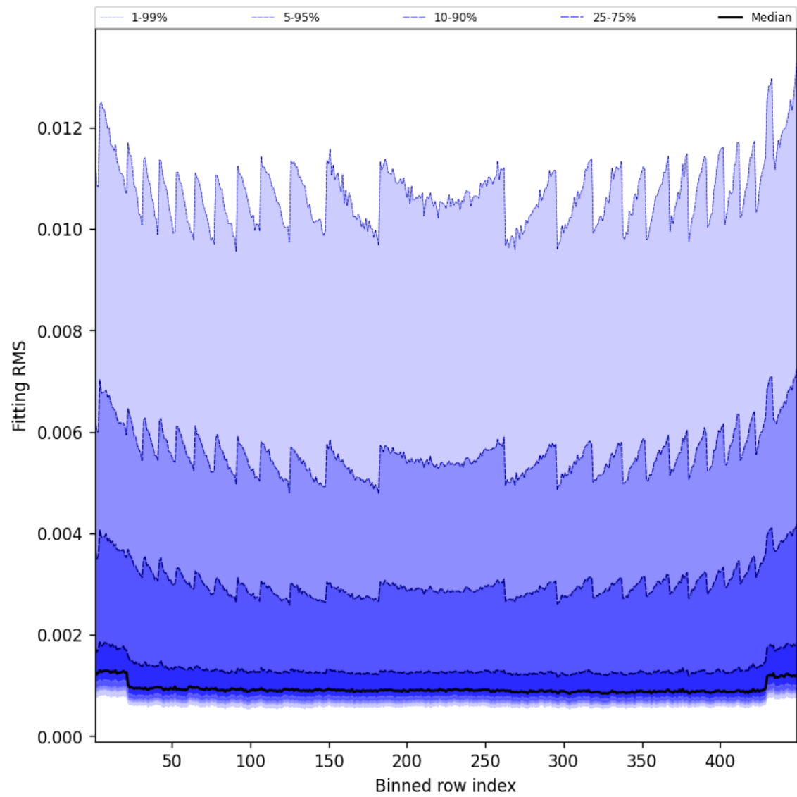
Figure 46: Along track statistics of “Fitting RMS” for 2025-04-24 to 2025-04-25
