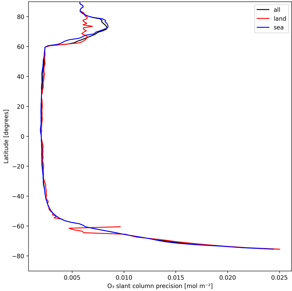
Figure 20: Zonal average of “O 3 slant column precision” for 2025-04-24 to 2025-04-25.
