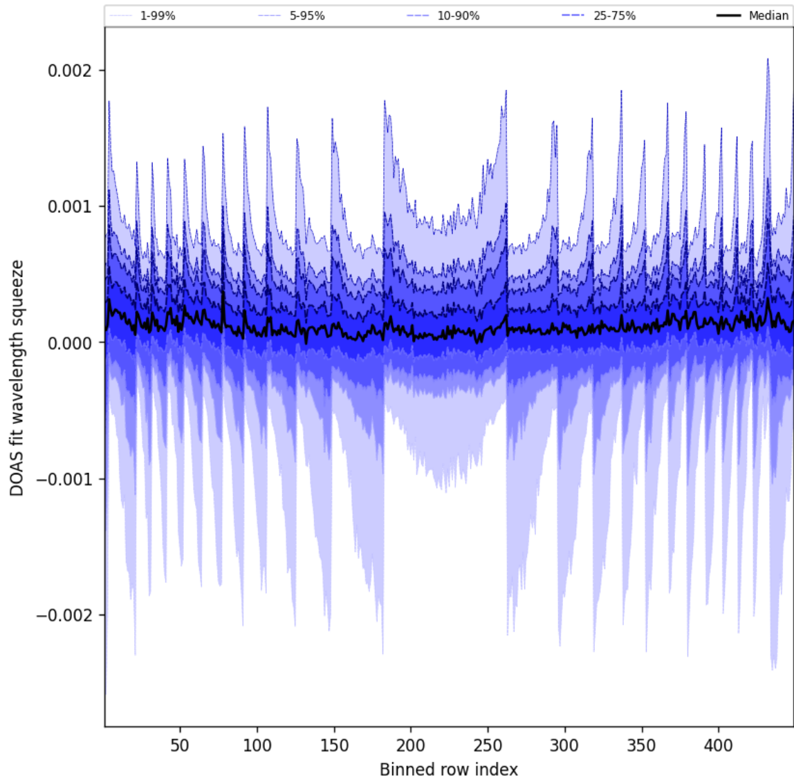
Figure 48: Along track statistics of “DOAS fit wavelength squeeze” for 2025-04-24 to 2025-04-25
