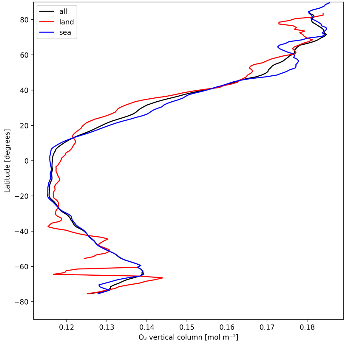
Figure 17: Zonal average of “O 3 vertical column” for 2025-04-24 to 2025-04-25.
