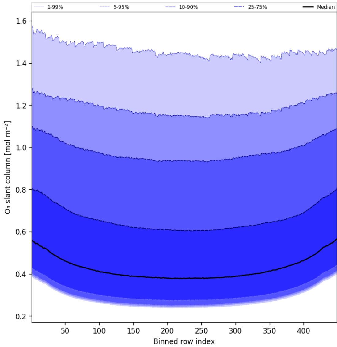
Figure 43: Along track statistics of “O 3 slant column” for 2025-04-24 to 2025-04-25
