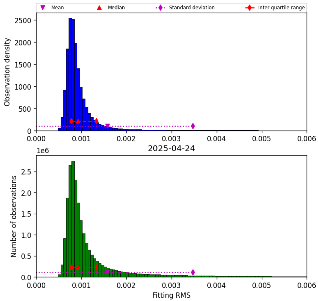
Figure 34: Histogram of “Fitting RMS” for 2025-04-24 to 2025-04-25
