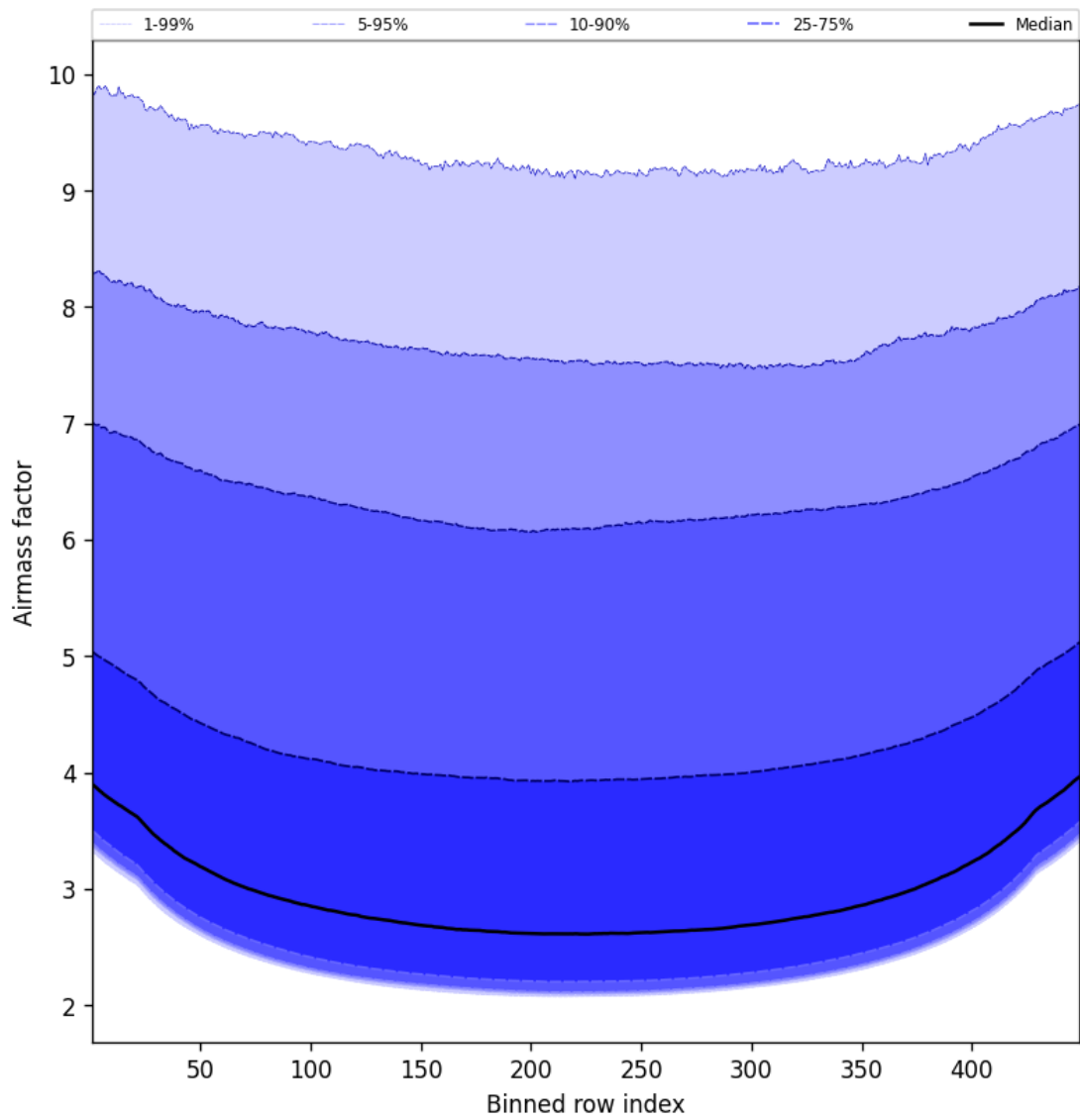
Figure 49: Along track statistics of “Airmass factor” for 2025-04-24 to 2025-04-25
