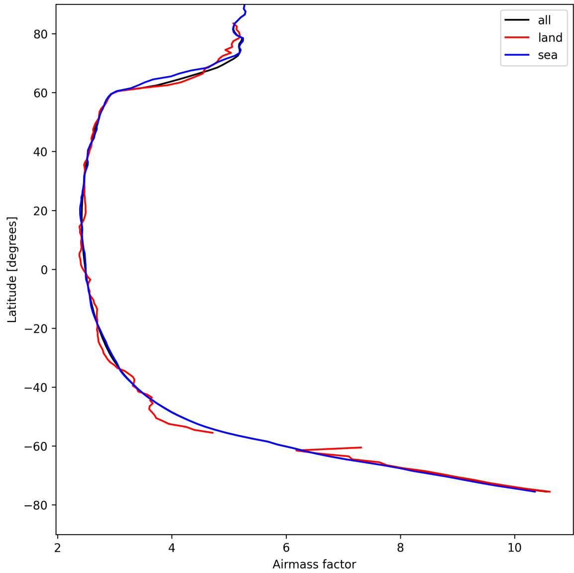
Figure 25: Zonal average of “Airmass factor” for 2025-04-24 to 2025-04-25.
