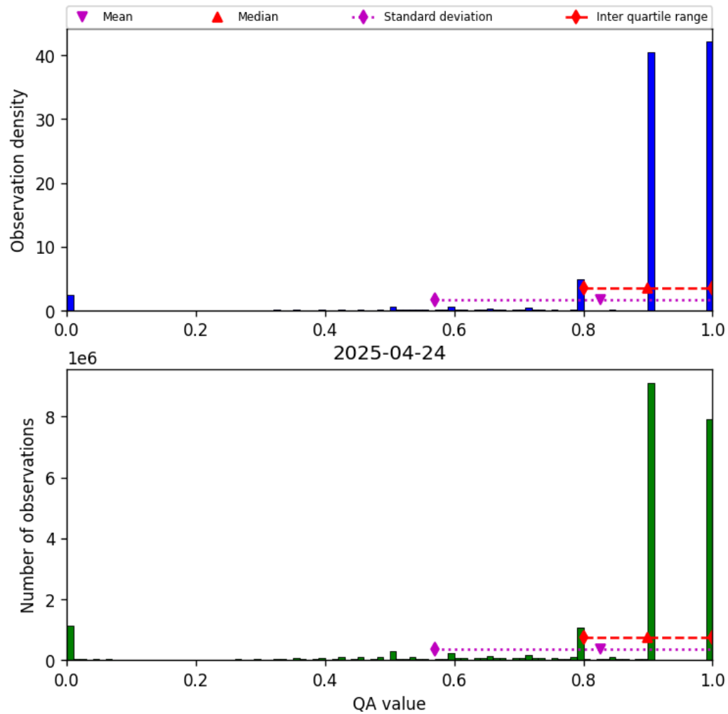
Figure 28: Histogram of “QA value” for 2025-04-24 to 2025-04-25
