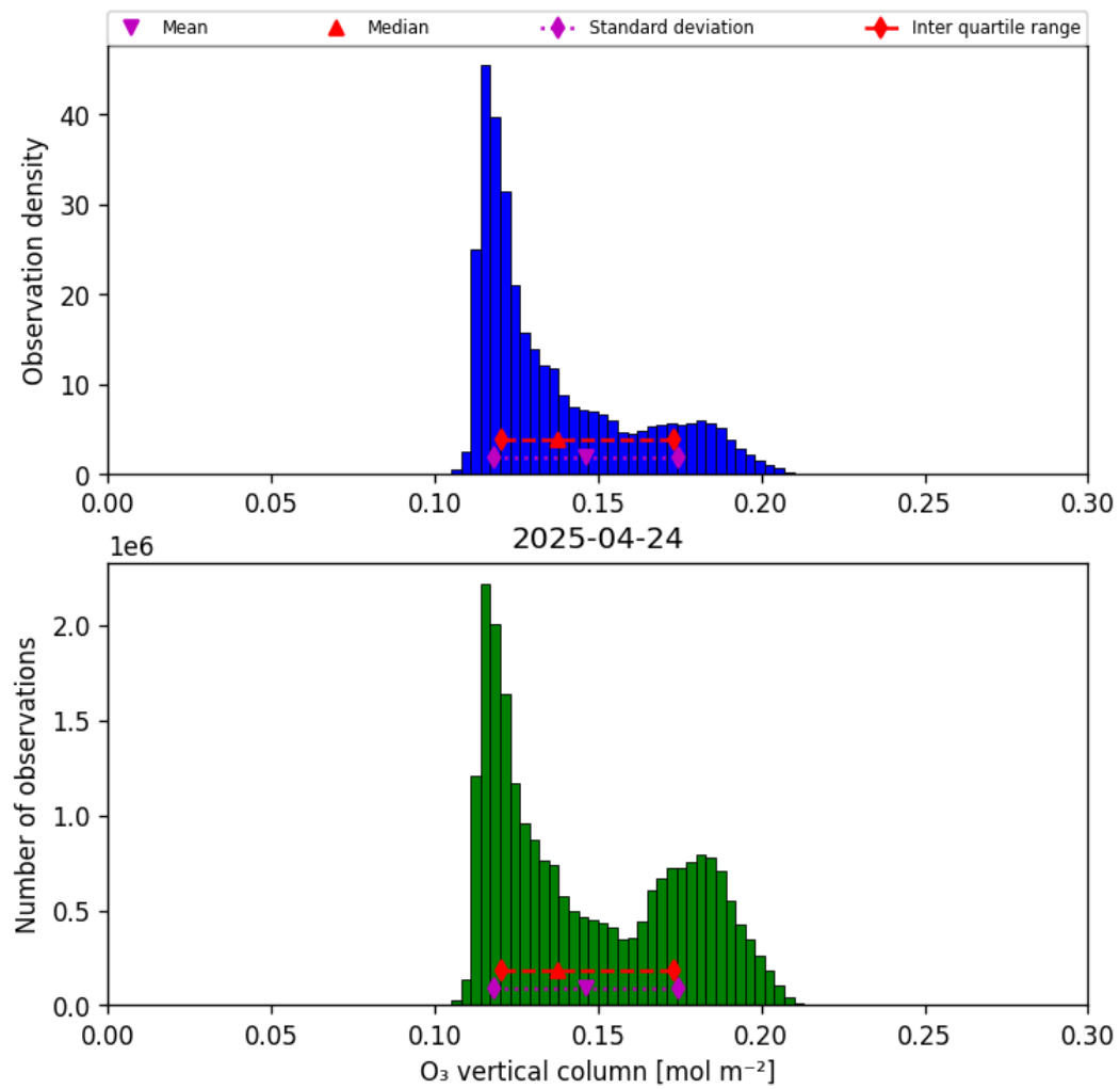
Figure 29: Histogram of “O 3 vertical column” for 2025-04-24 to 2025-04-25
