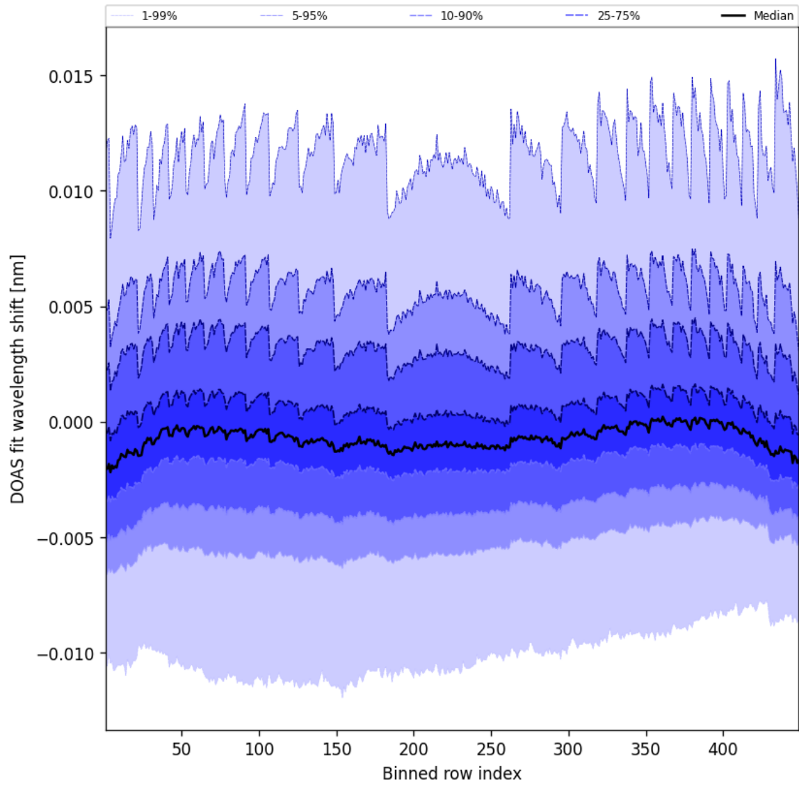
Figure 47: Along track statistics of “DOAS fit wavelength shift” for 2025-04-24 to 2025-04-25
