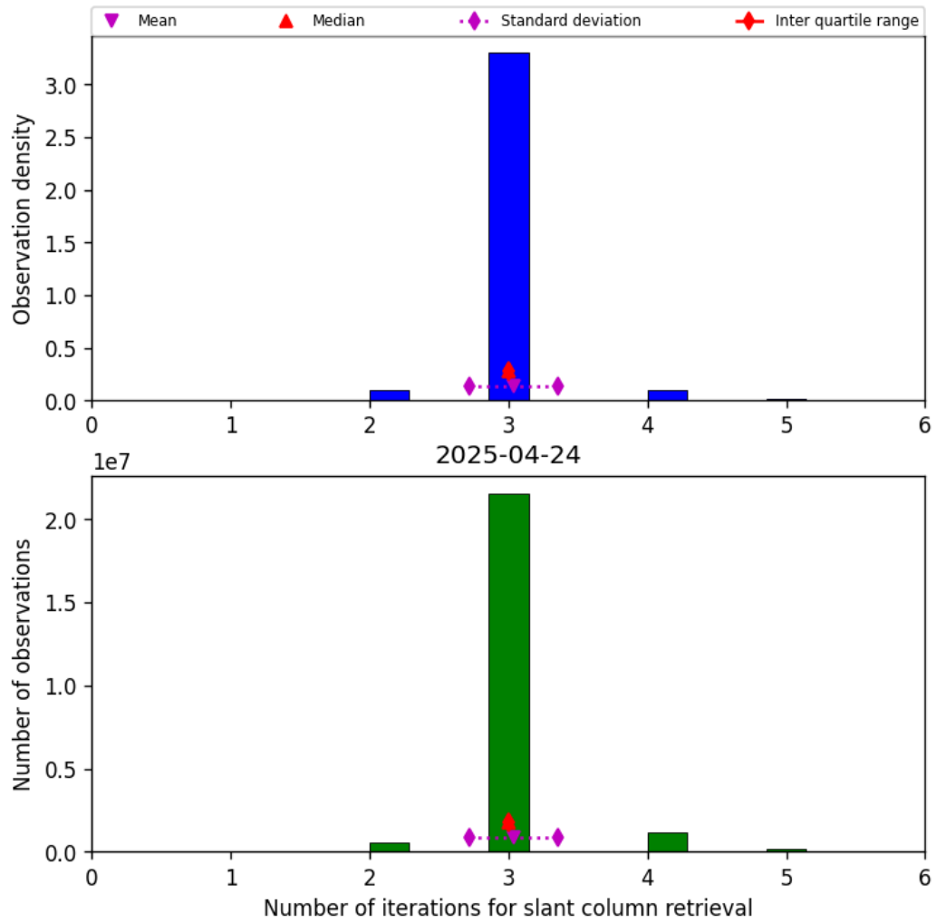
Figure 33: Histogram of “Number of iterations for slant column retrieval” for 2025-04-24 to 2025-04-25
