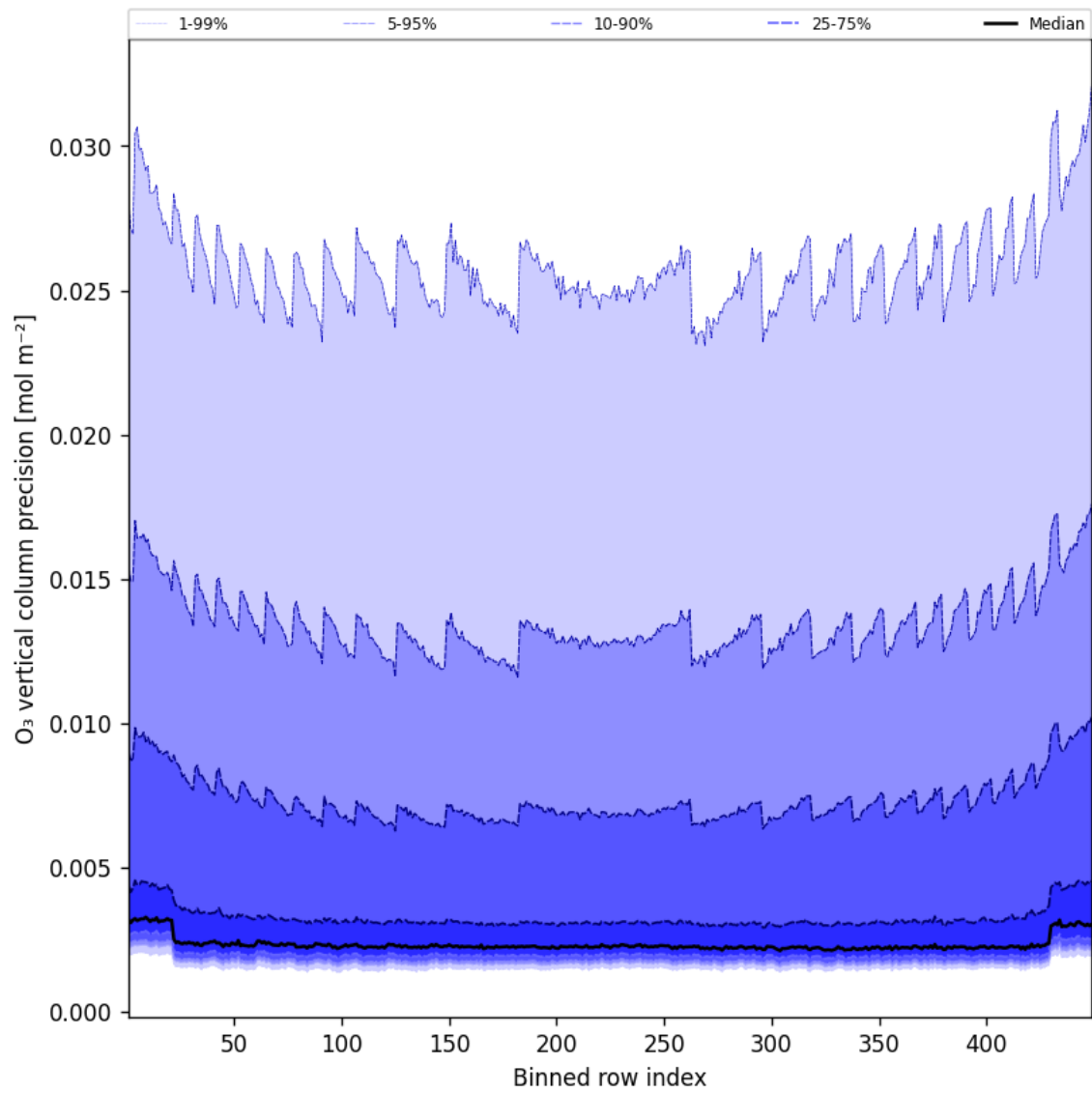
Figure 42: Along track statistics of “O 3 vertical column precision” for 2025-04-24 to 2025-04-25
