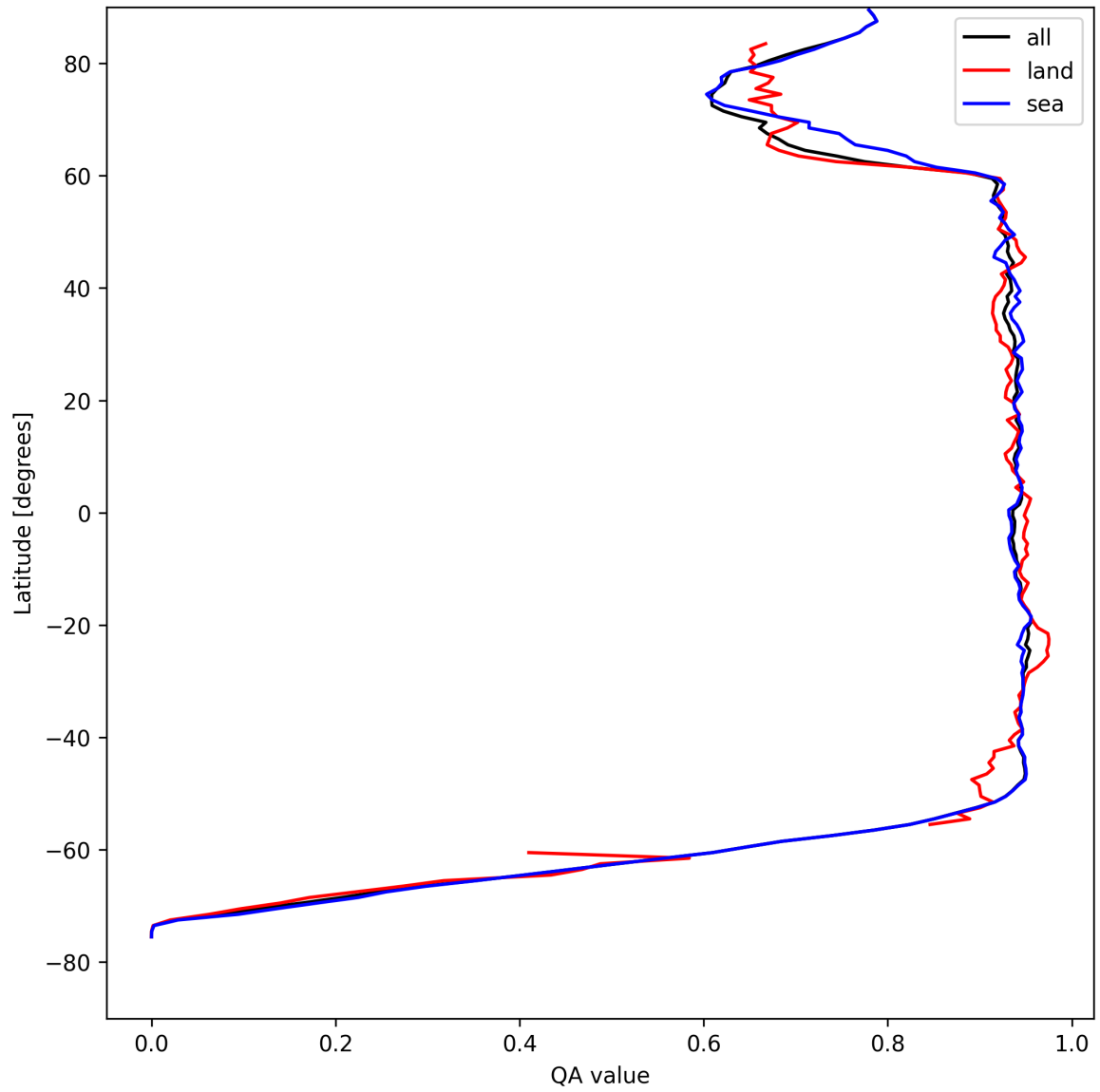
Figure 16: Zonal average of “QA value” for 2025-04-24 to 2025-04-25.
