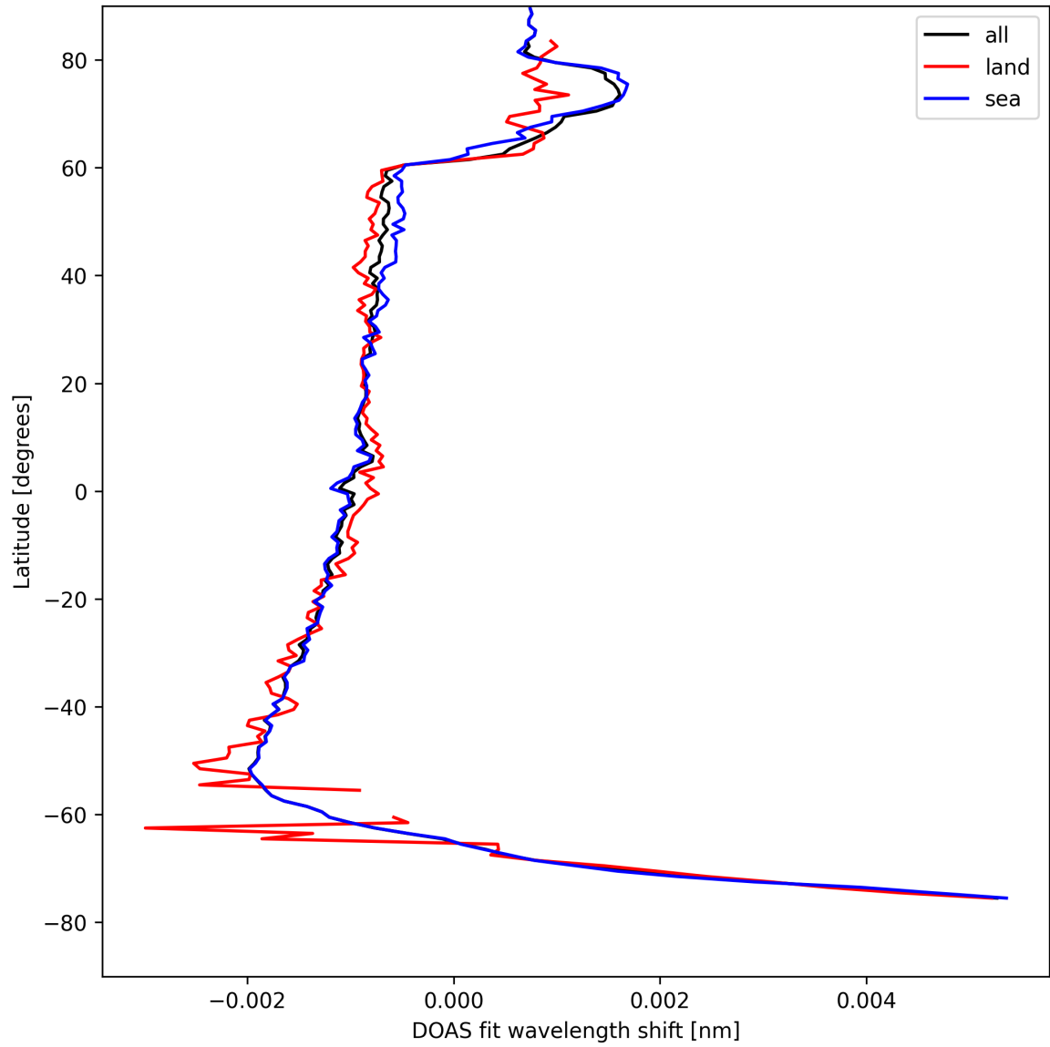
Figure 23: Zonal average of “DOAS fit wavelength shift” for 2025-04-24 to 2025-04-25.
