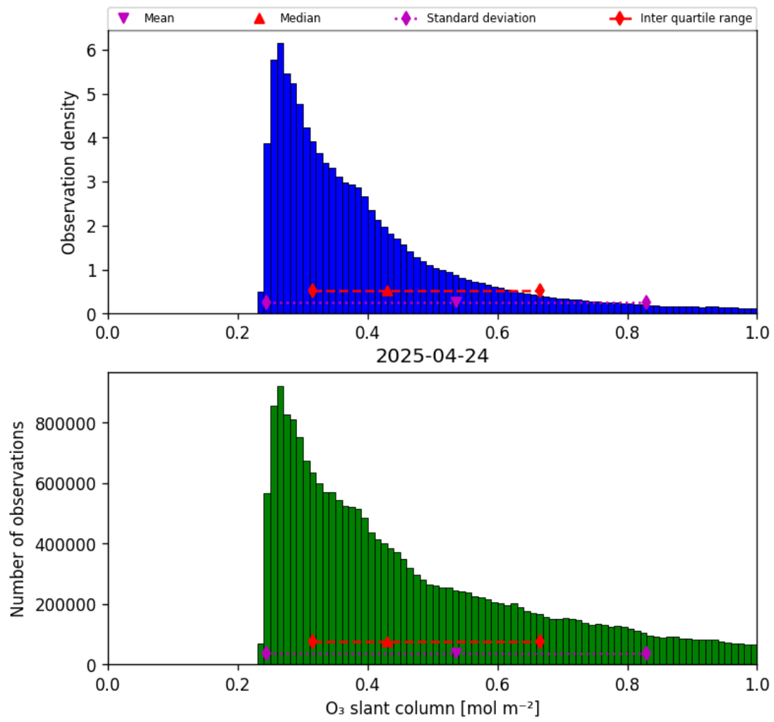
Figure 31: Histogram of “O 3 slant column” for 2025-04-24 to 2025-04-25
