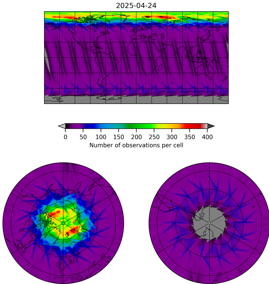
Figure 15: Map of the number of observations for 2025-04-24 to 2025-04-25
