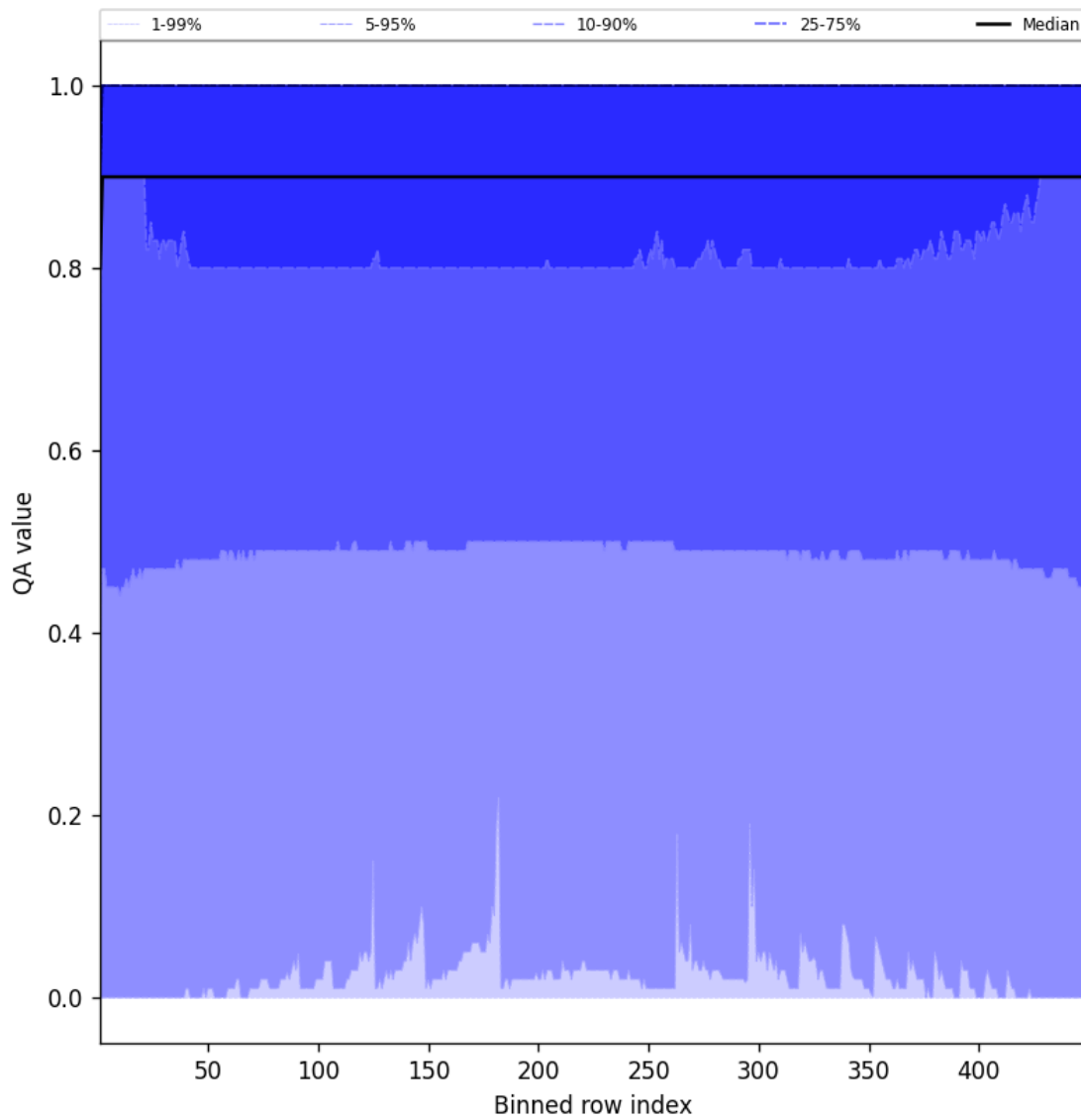
Figure 40: Along track statistics of “QA value” for 2025-04-24 to 2025-04-25
