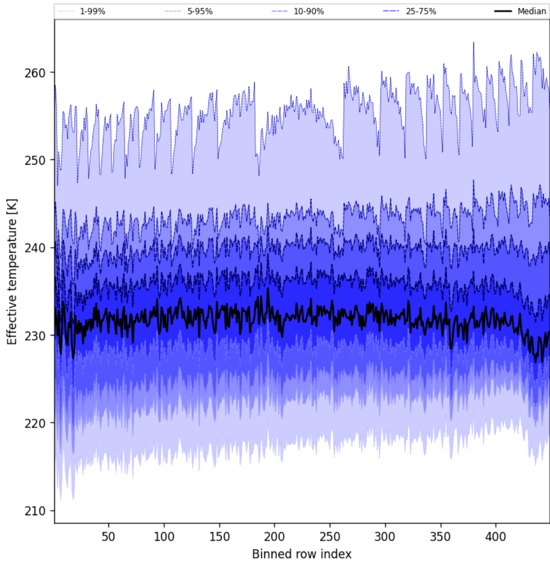
Figure 50: Along track statistics of “Effective temperature” for 2025-04-24 to 2025-04-25
