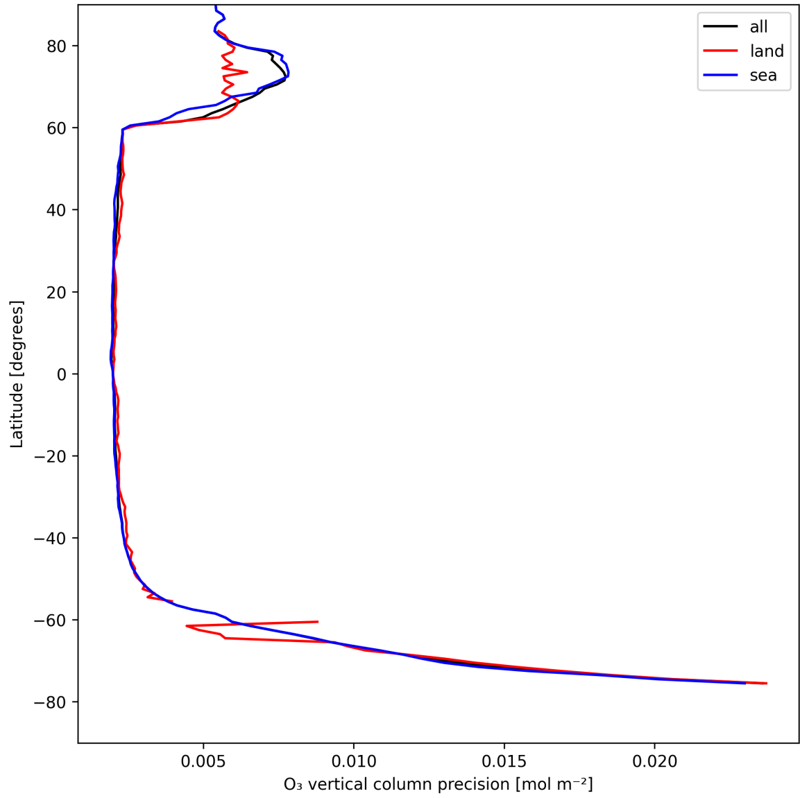
Figure 18: Zonal average of “O 3 vertical column precision” for 2025-04-24 to 2025-04-25.
