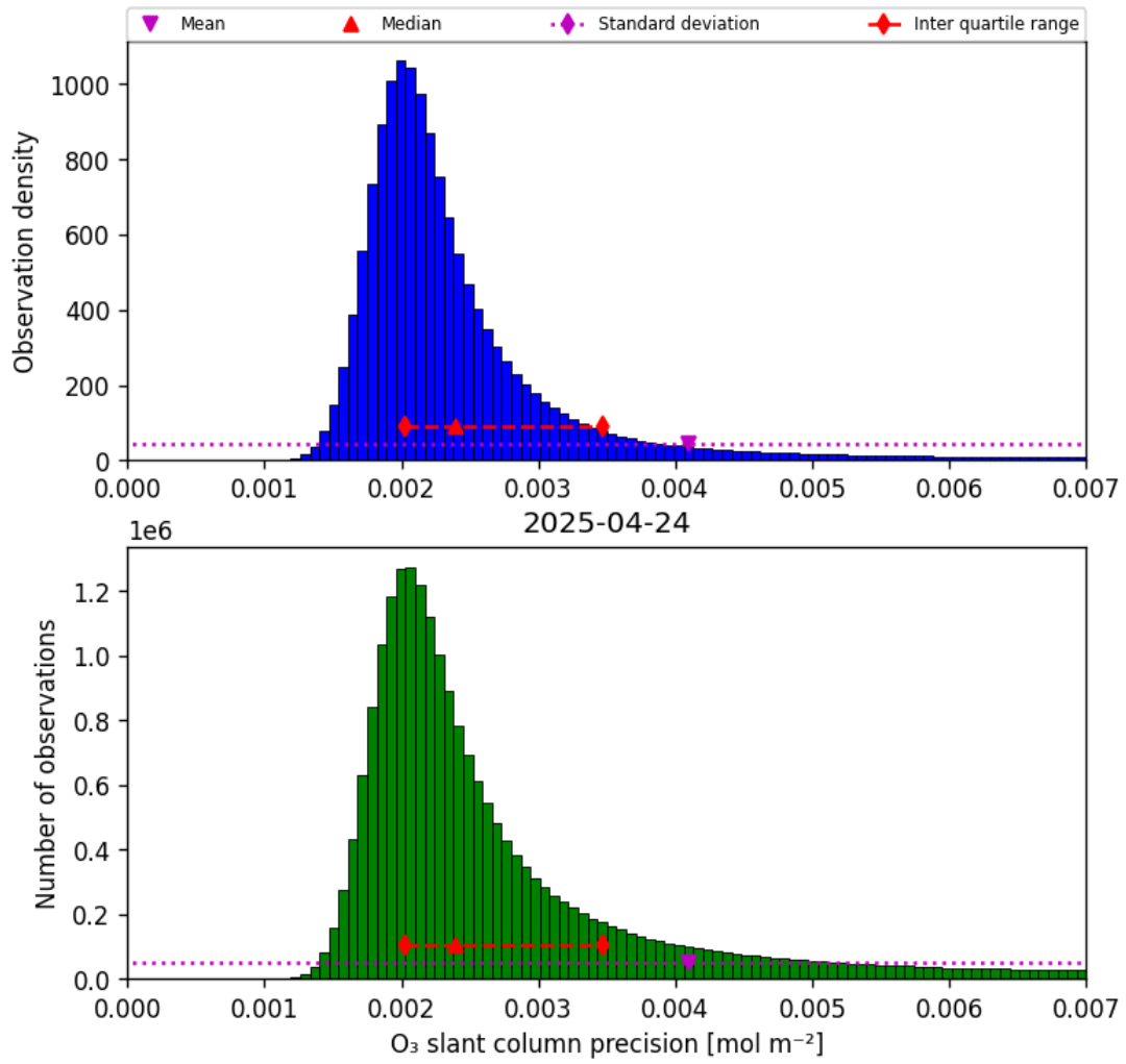
Figure 32: Histogram of “O 3 slant column precision” for 2025-04-24 to 2025-04-25
