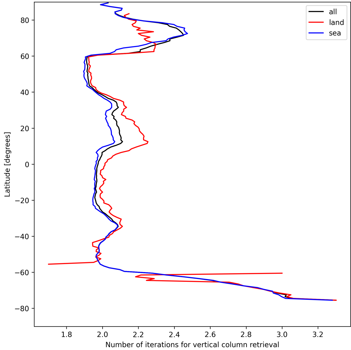
Figure 27: Zonal average of “Number of iterations for vertical column retrieval” for 2025-04-24 to 2025-04-25.
