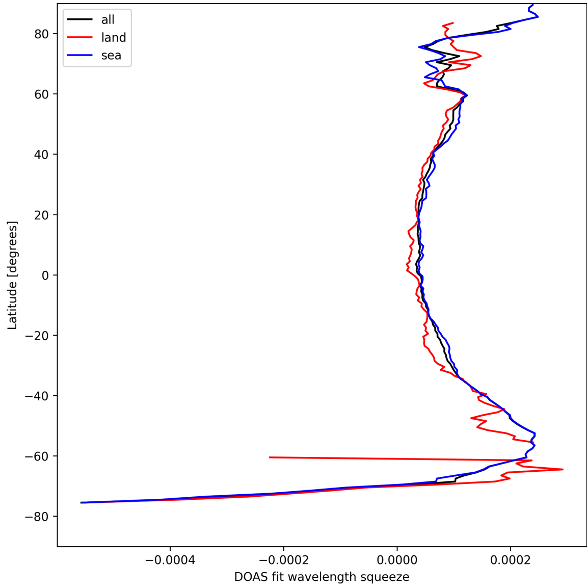
Figure 24: Zonal average of “DOAS fit wavelength squeeze” for 2025-04-24 to 2025-04-25.
