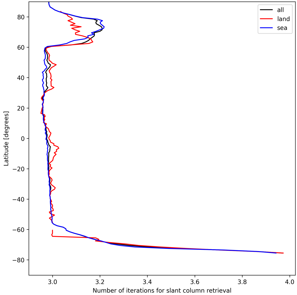
Figure 21: Zonal average of “Number of iterations for slant column retrieval” for 2025-04-24 to 2025-04-25.
