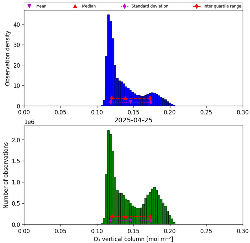
Figure 29: Histogram of “O 3 vertical column” for 2025-04-25 to 2025-04-26
