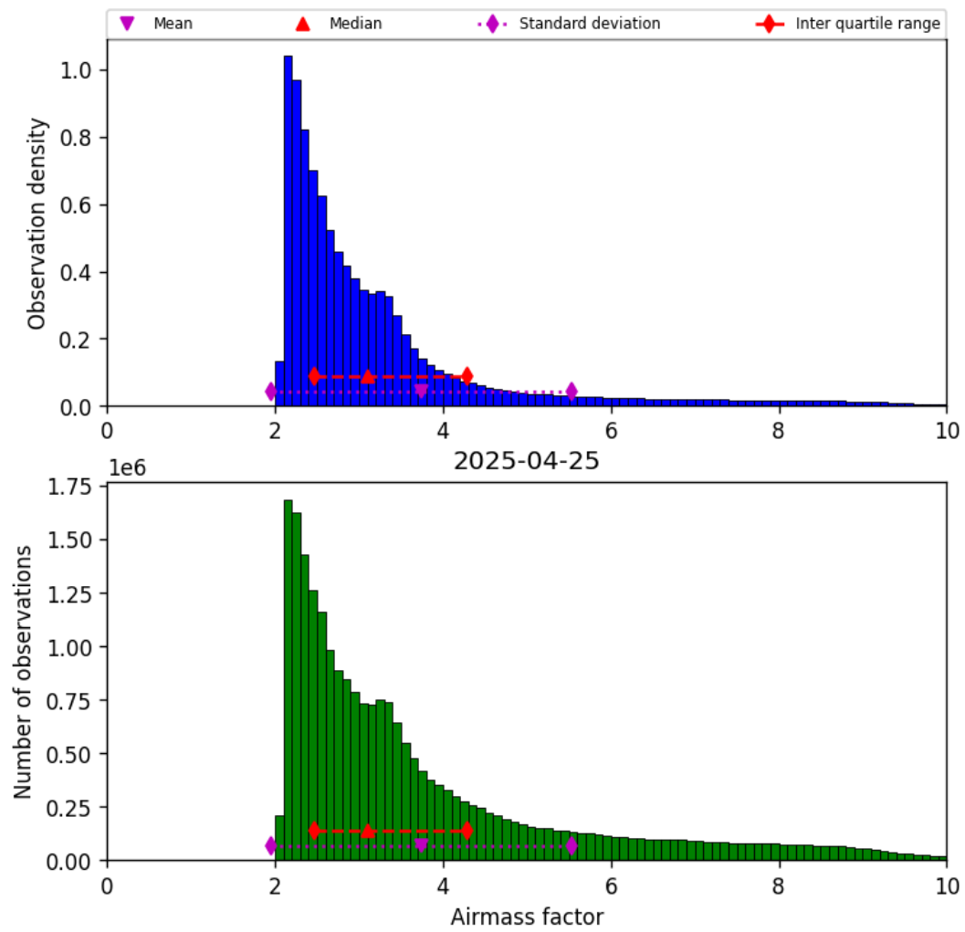
Figure 37: Histogram of “Airmass factor” for 2025-04-25 to 2025-04-26
