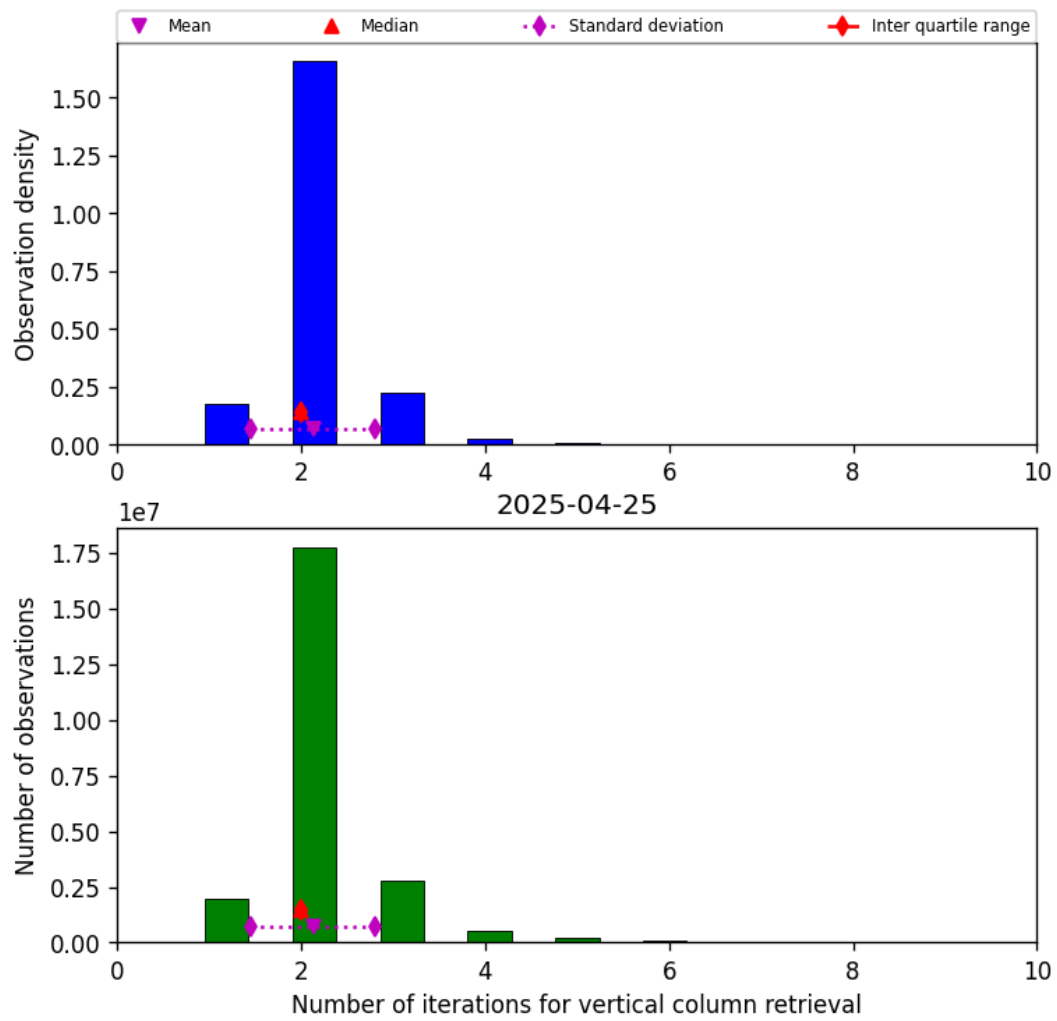
Figure 39: Histogram of “Number of iterations for vertical column retrieval” for 2025-04-25 to 2025-04-26
