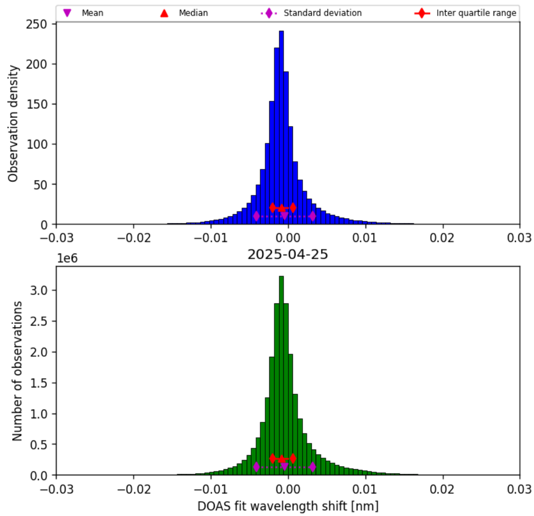
Figure 35: Histogram of “DOAS fit wavelength shift” for 2025-04-25 to 2025-04-26
