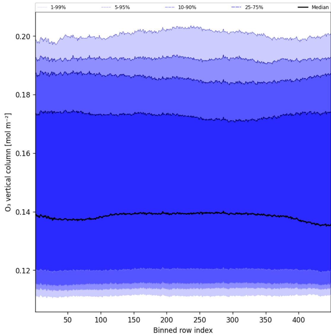
Figure 41: Along track statistics of “O 3 vertical column” for 2025-04-25 to 2025-04-26
