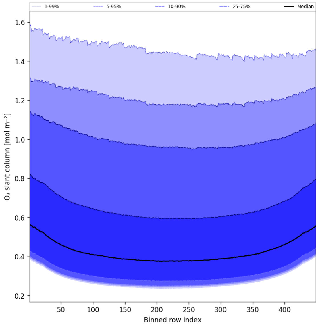
Figure 43: Along track statistics of “O 3 slant column” for 2025-04-25 to 2025-04-26
