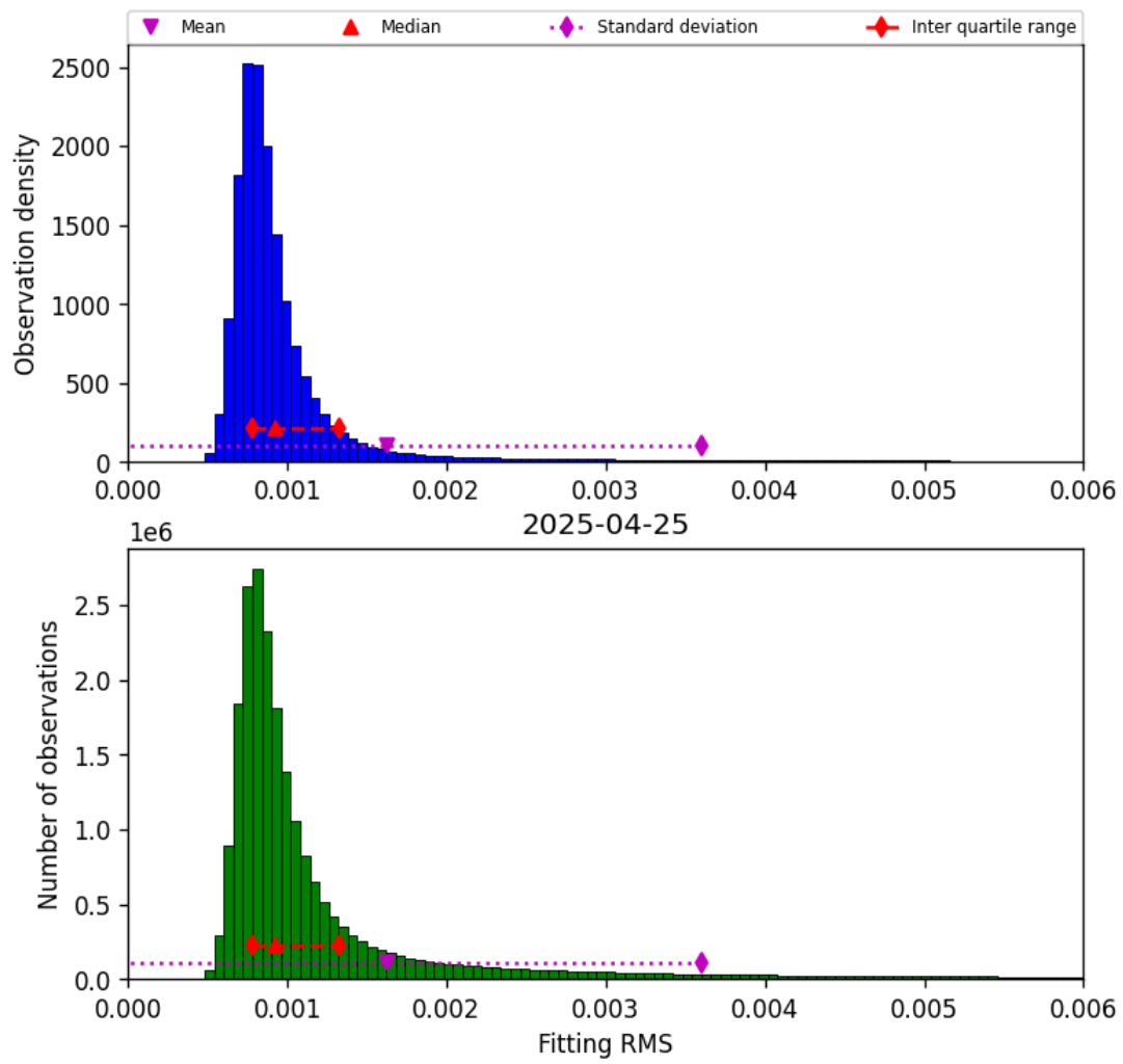
Figure 34: Histogram of “Fitting RMS” for 2025-04-25 to 2025-04-26
