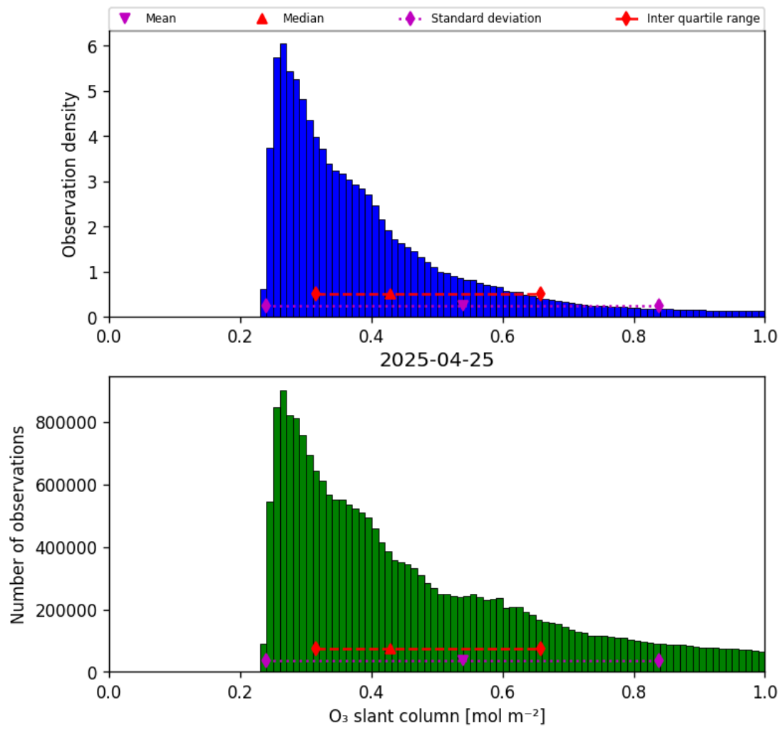
Figure 31: Histogram of “O 3 slant column” for 2025-04-25 to 2025-04-26
