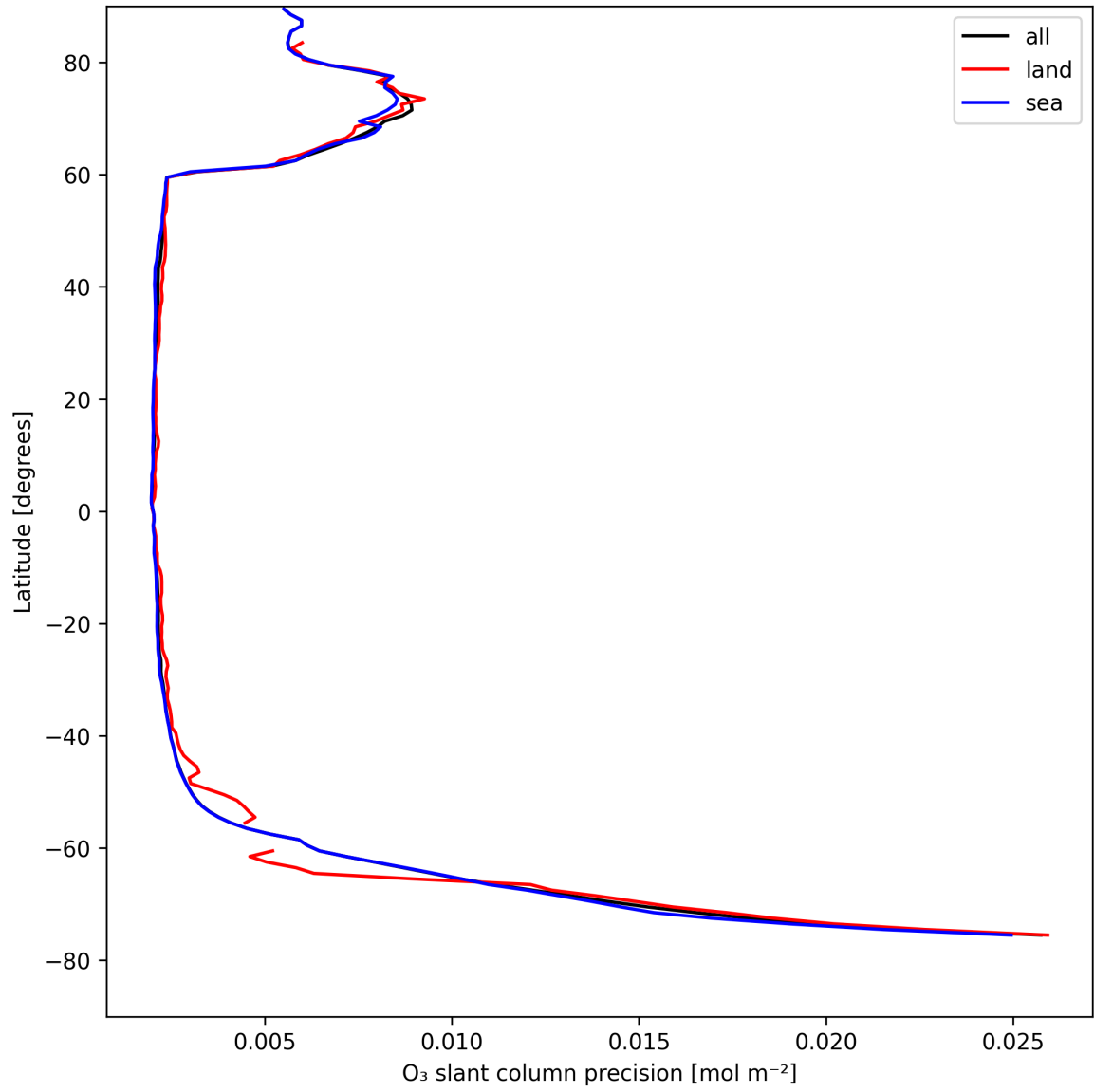
Figure 20: Zonal average of “O 3 slant column precision” for 2025-04-25 to 2025-04-26.
