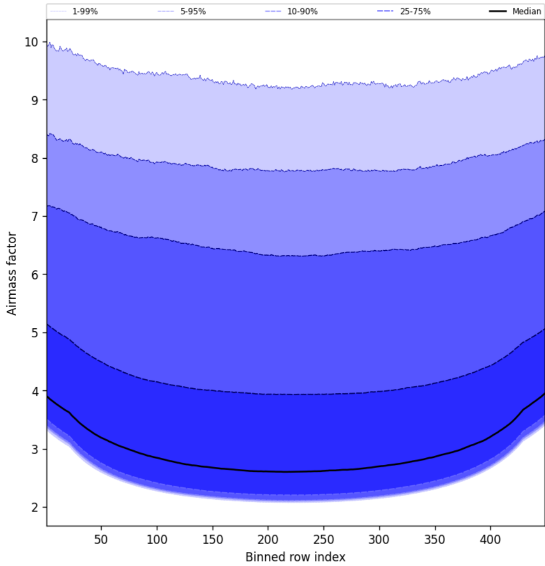
Figure 49: Along track statistics of “Airmass factor” for 2025-04-25 to 2025-04-26
