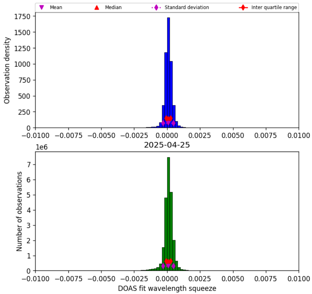
Figure 36: Histogram of “DOAS fit wavelength squeeze” for 2025-04-25 to 2025-04-26
