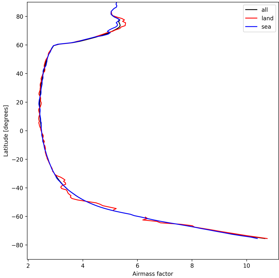
Figure 25: Zonal average of “Airmass factor” for 2025-04-25 to 2025-04-26.
