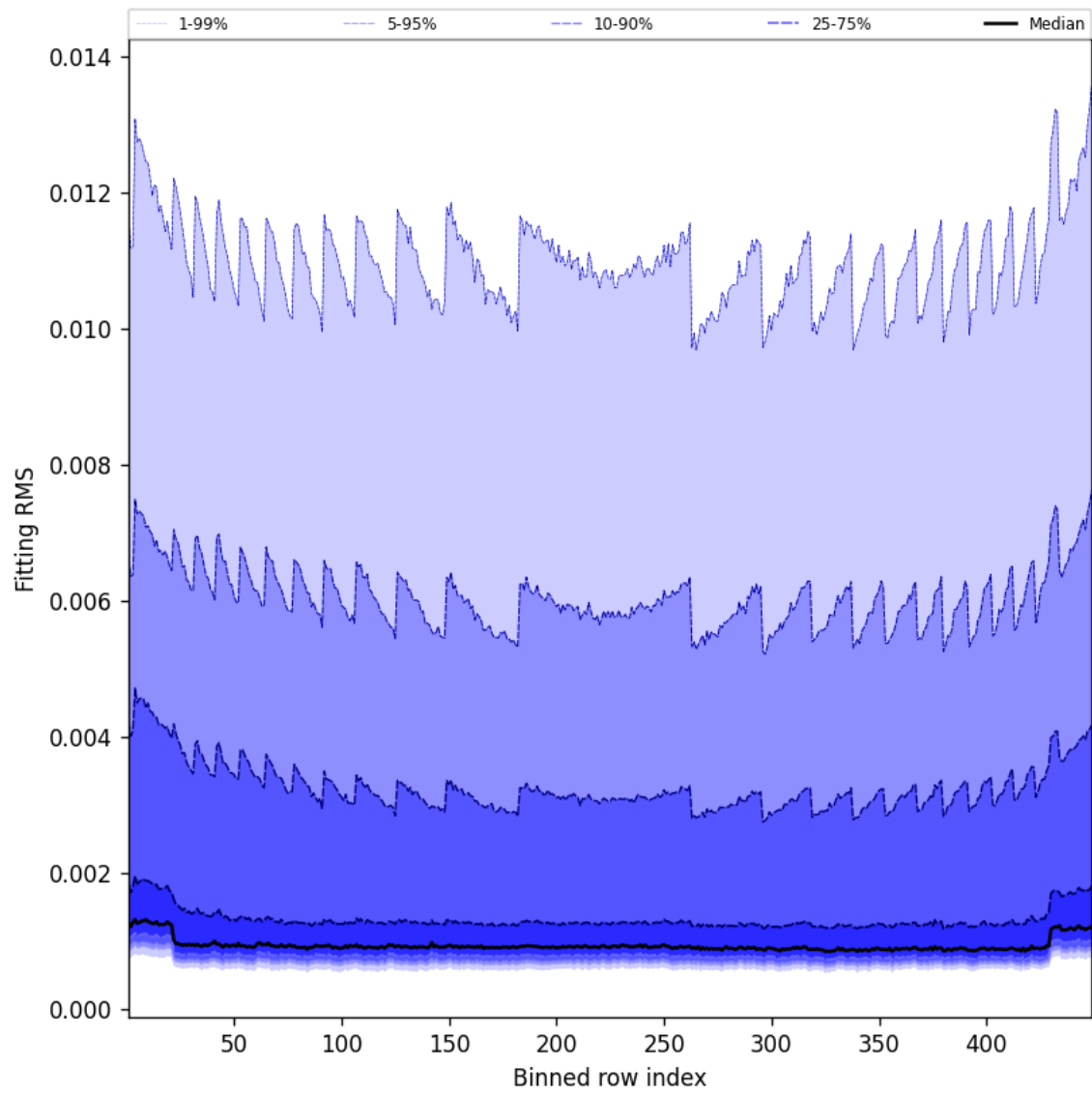
Figure 46: Along track statistics of “Fitting RMS” for 2025-04-25 to 2025-04-26
