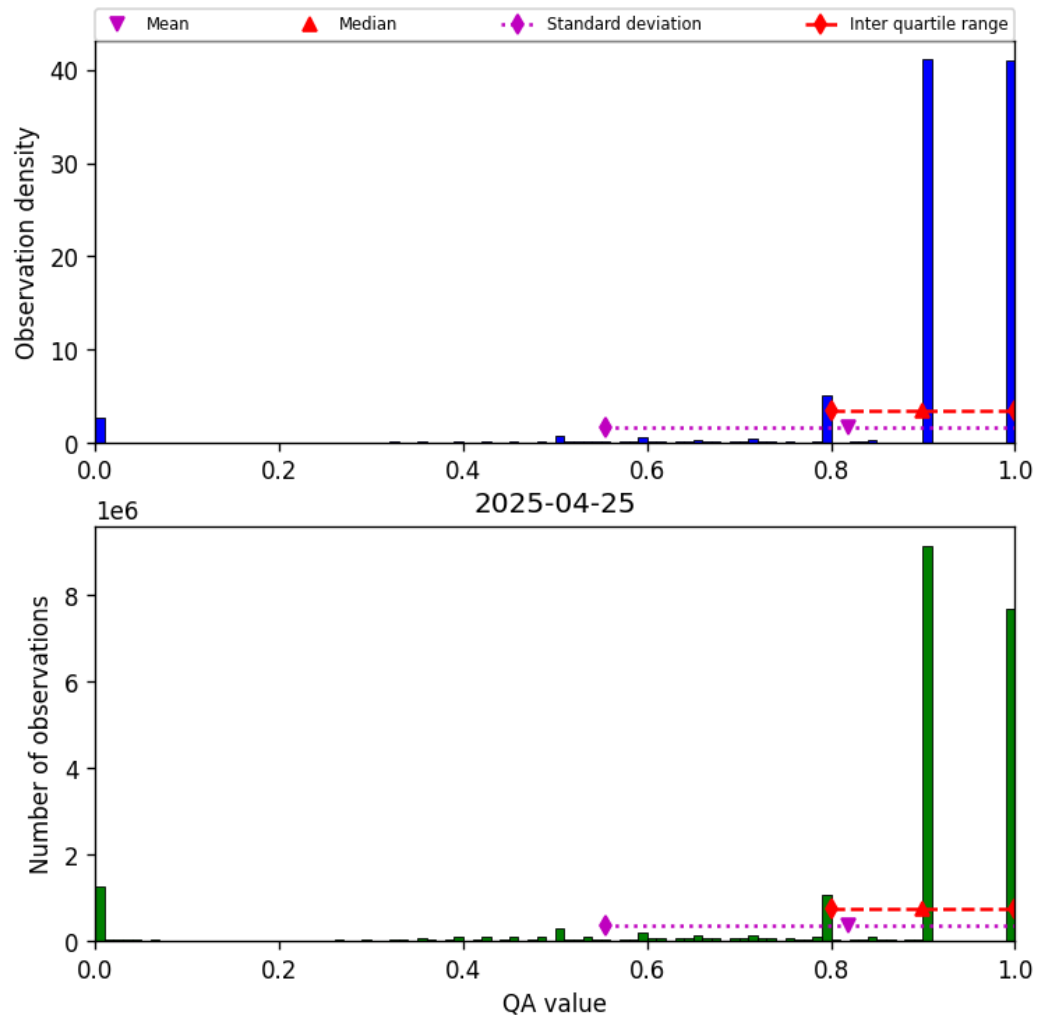
Figure 28: Histogram of “QA value” for 2025-04-25 to 2025-04-26
