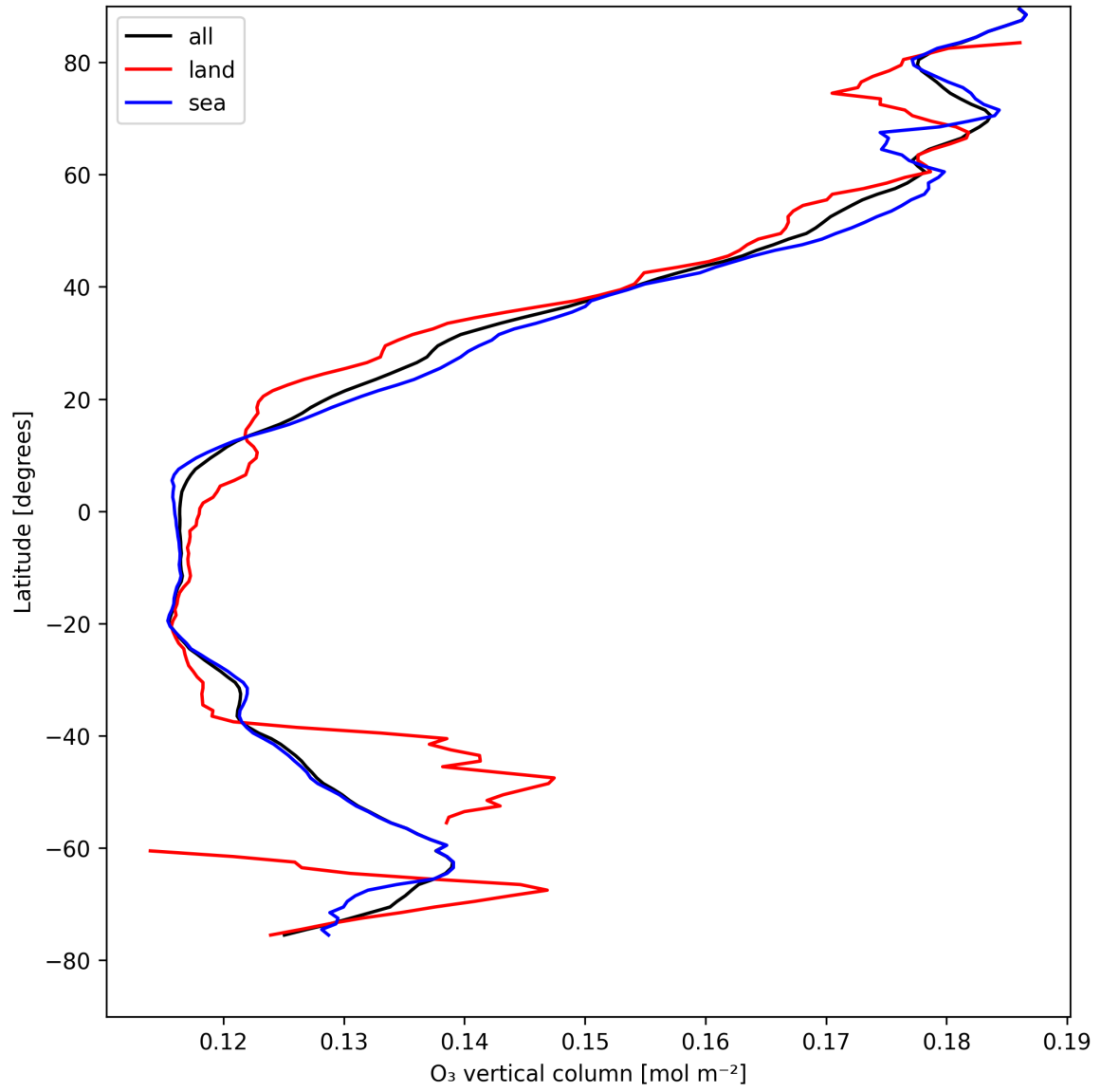
Figure 17: Zonal average of “O 3 vertical column” for 2025-04-25 to 2025-04-26.
