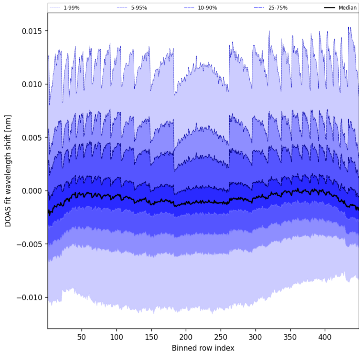
Figure 47: Along track statistics of “DOAS fit wavelength shift” for 2025-04-25 to 2025-04-26
