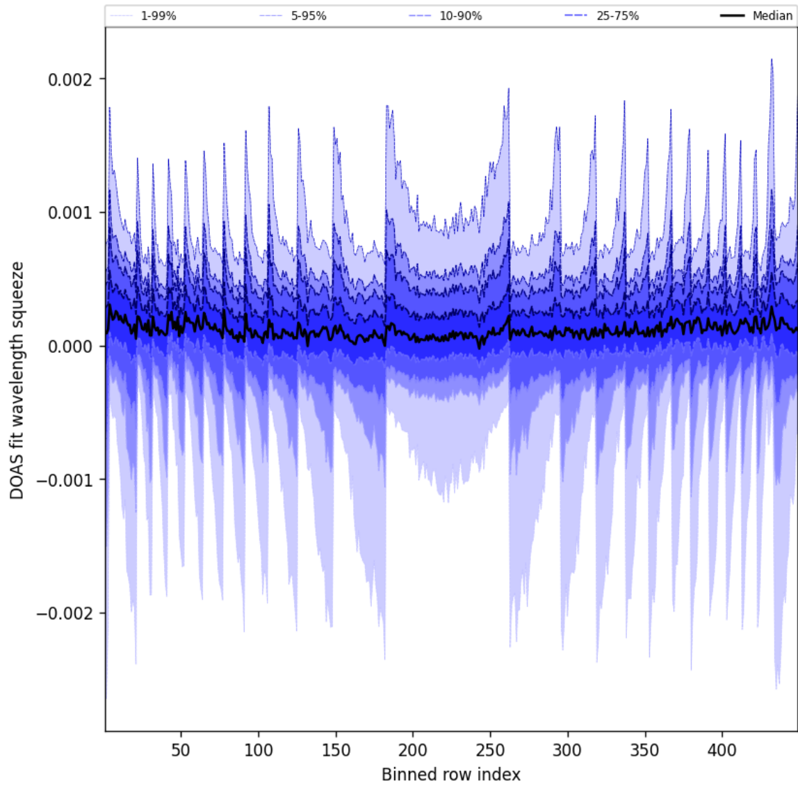
Figure 48: Along track statistics of “DOAS fit wavelength squeeze” for 2025-04-25 to 2025-04-26
