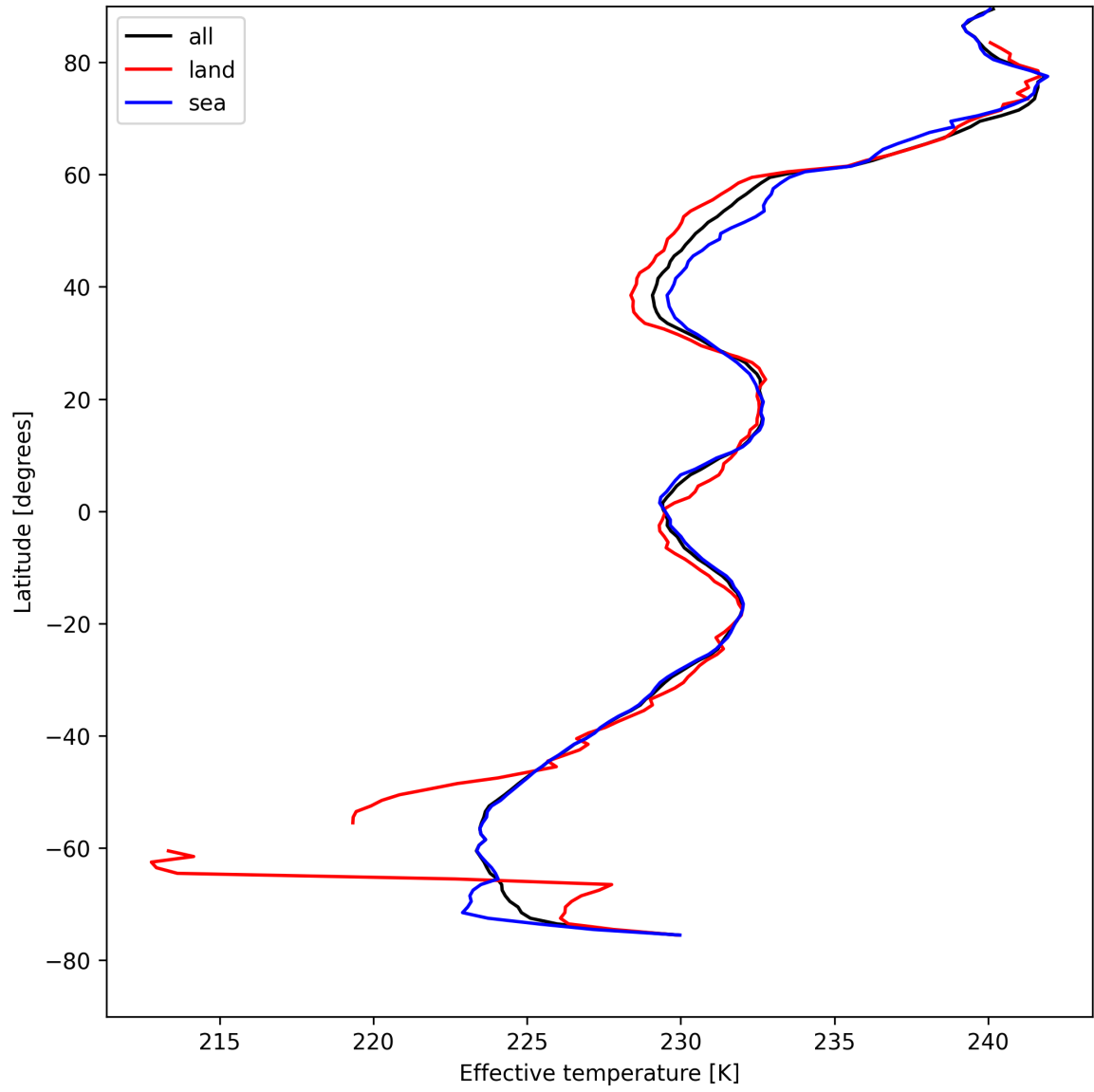
Figure 26: Zonal average of “Effective temperature” for 2025-04-25 to 2025-04-26.
