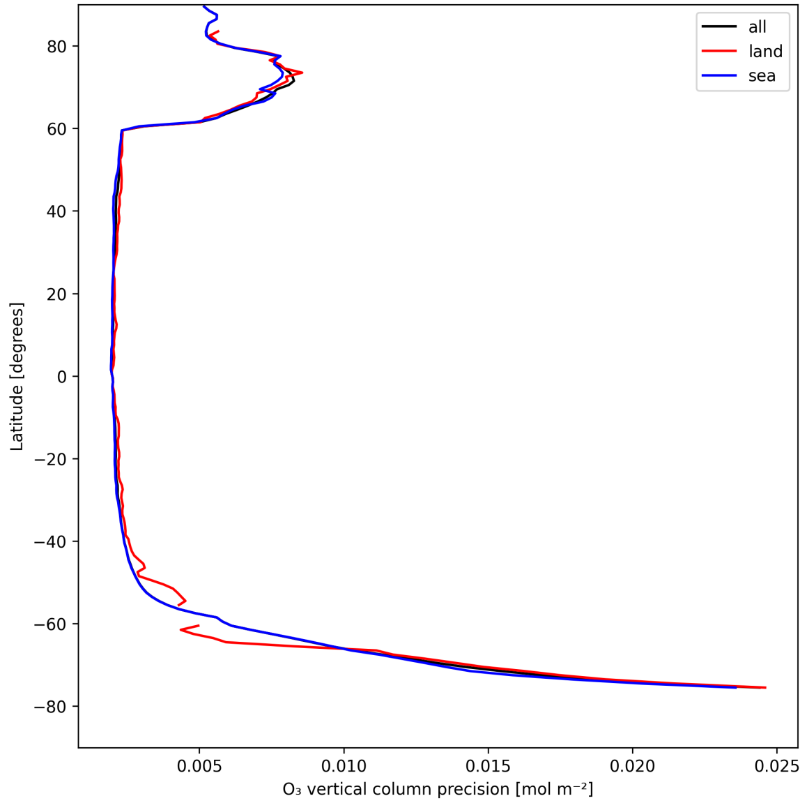
Figure 18: Zonal average of “O 3 vertical column precision” for 2025-04-25 to 2025-04-26.
