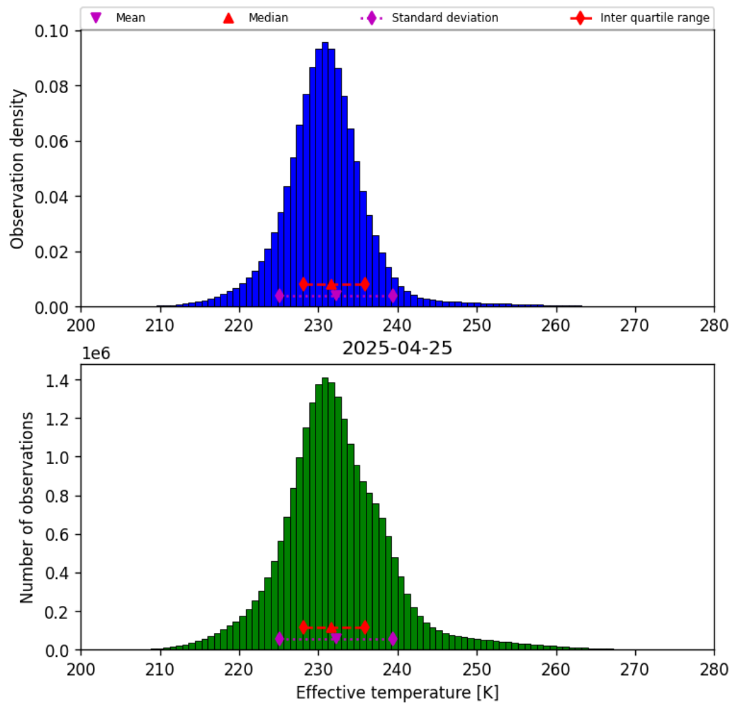
Figure 38: Histogram of “Effective temperature” for 2025-04-25 to 2025-04-26
