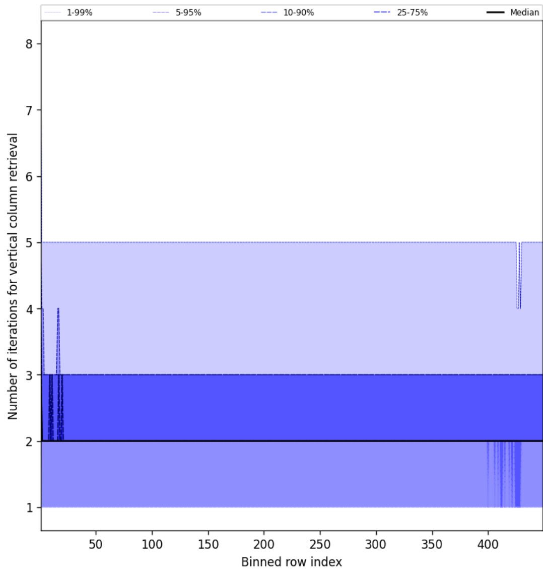
Figure 51: Along track statistics of “Number of iterations for vertical column retrieval” for 2025-04-25 to 2025-04-26
