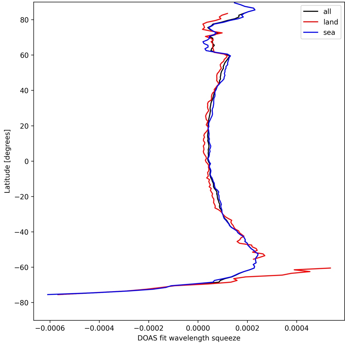
Figure 24: Zonal average of “DOAS fit wavelength squeeze” for 2025-04-25 to 2025-04-26.
