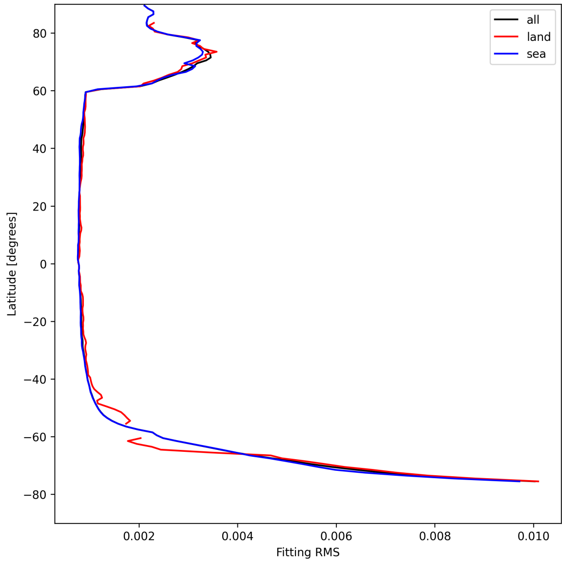
Figure 22: Zonal average of “Fitting RMS” for 2025-04-25 to 2025-04-26.
