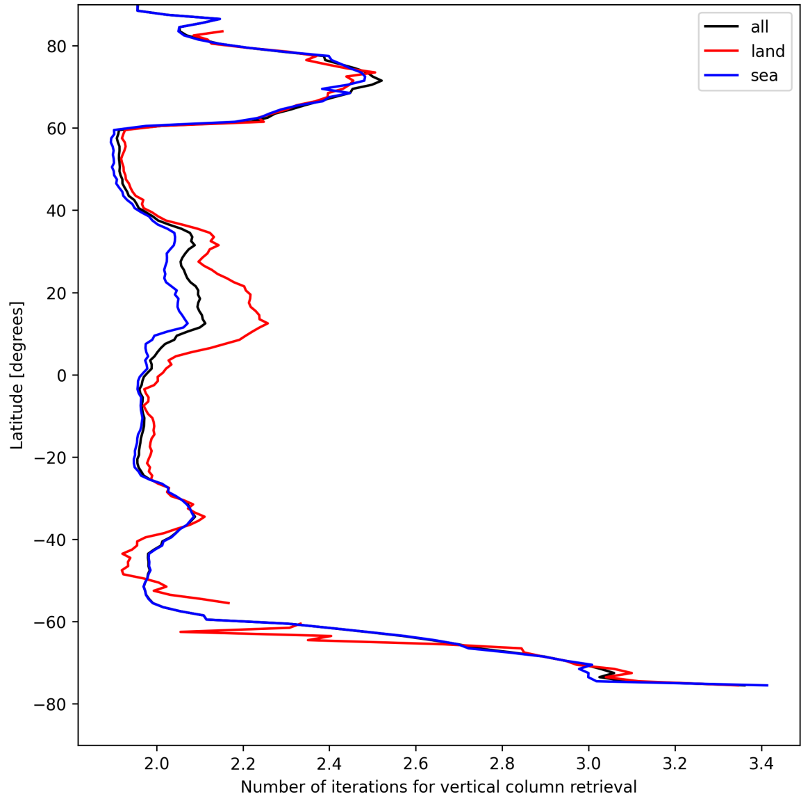
Figure 27: Zonal average of “Number of iterations for vertical column retrieval” for 2025-04-25 to 2025-04-26.
