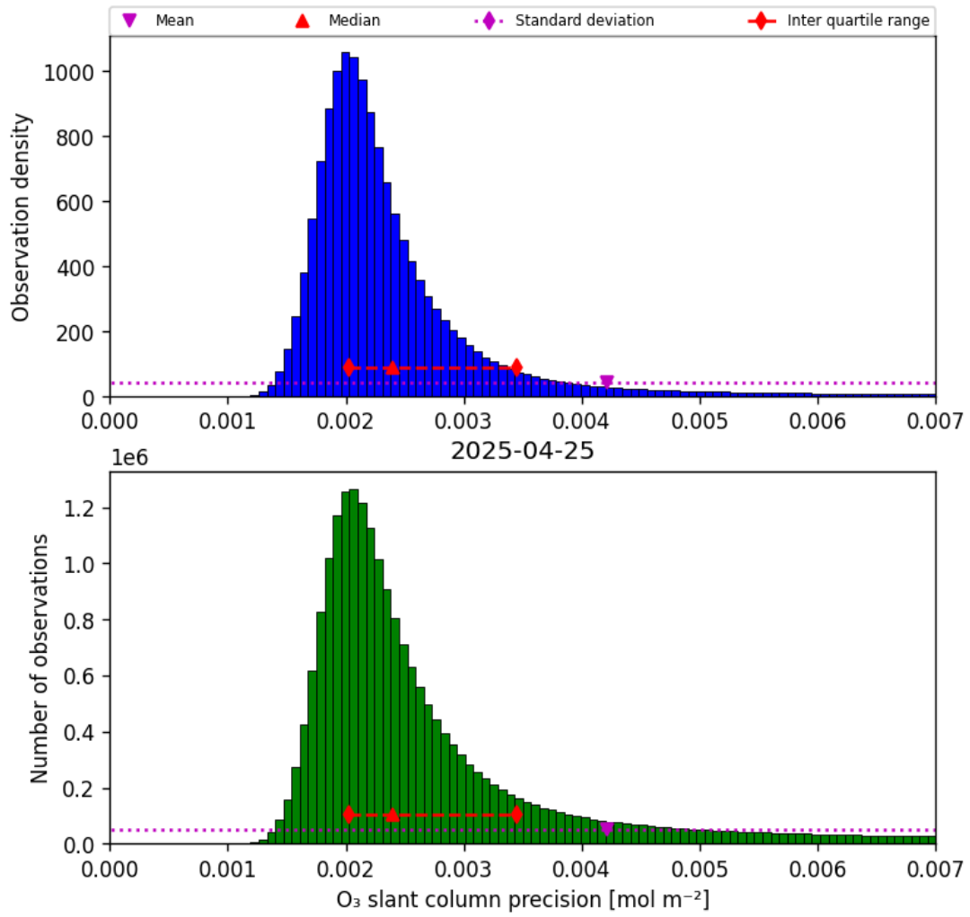
Figure 32: Histogram of “O 3 slant column precision” for 2025-04-25 to 2025-04-26
