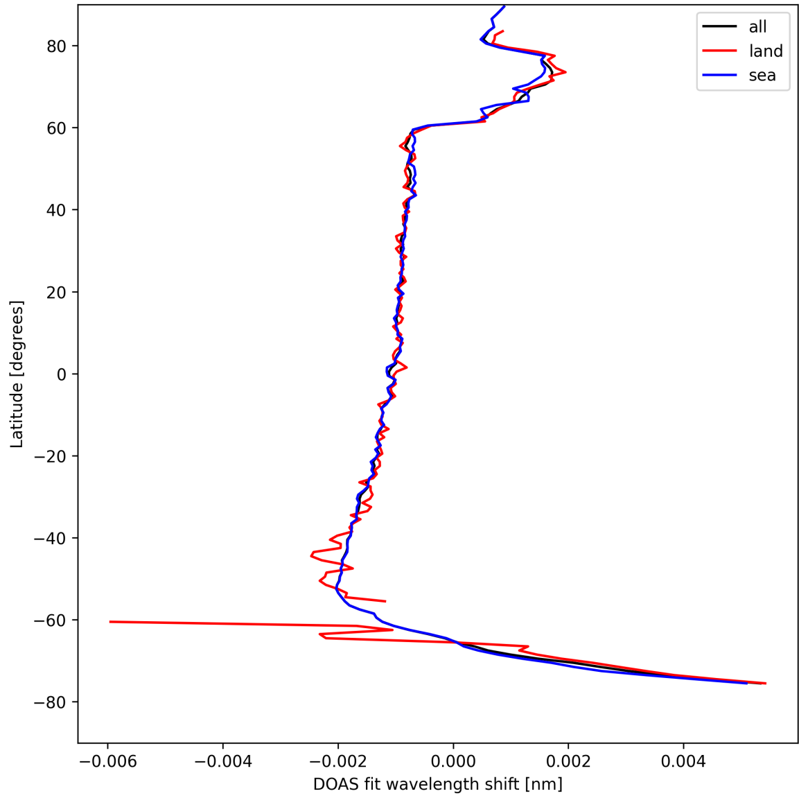
Figure 23: Zonal average of “DOAS fit wavelength shift” for 2025-04-25 to 2025-04-26.
