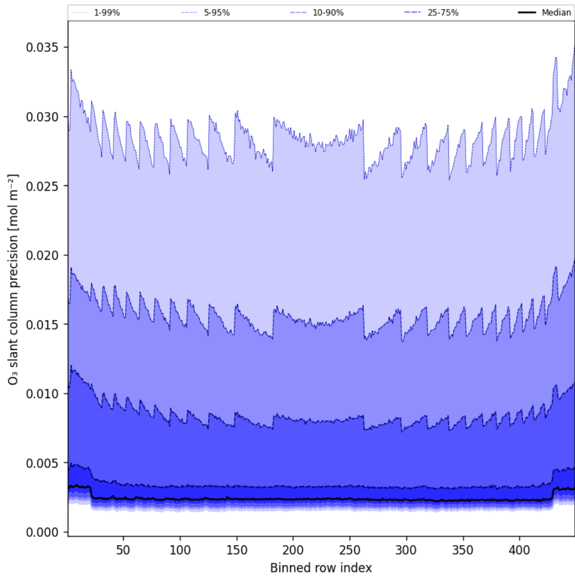
Figure 44: Along track statistics of “O 3 slant column precision” for 2025-04-25 to 2025-04-26
