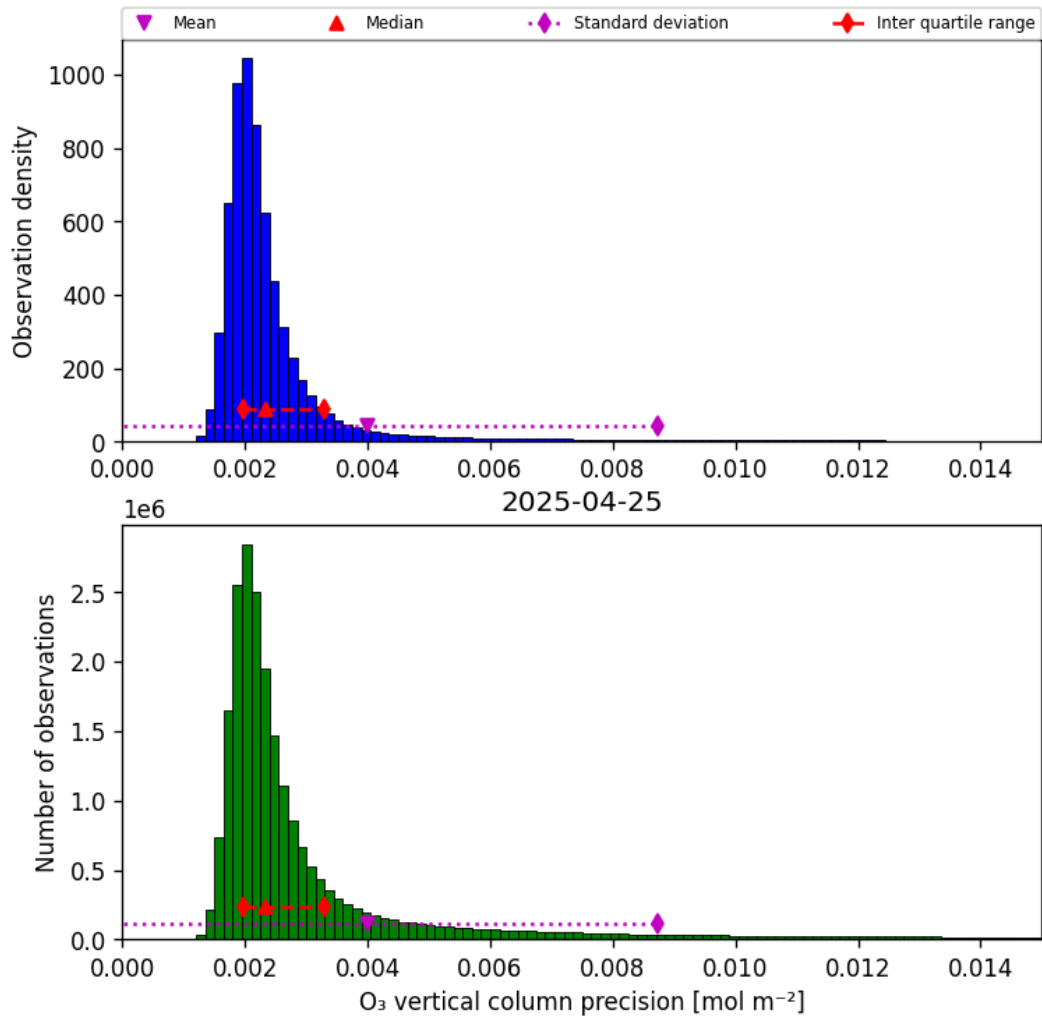
Figure 30: Histogram of “O 3 vertical column precision” for 2025-04-25 to 2025-04-26
