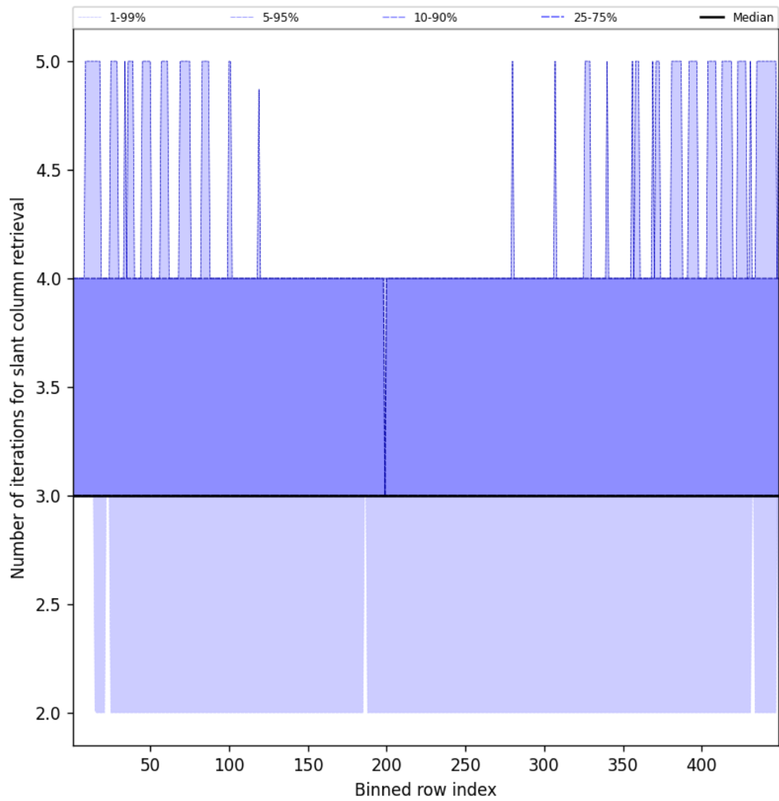
Figure 45: Along track statistics of “Number of iterations for slant column retrieval” for 2025-04-25 to 2025-04-26
