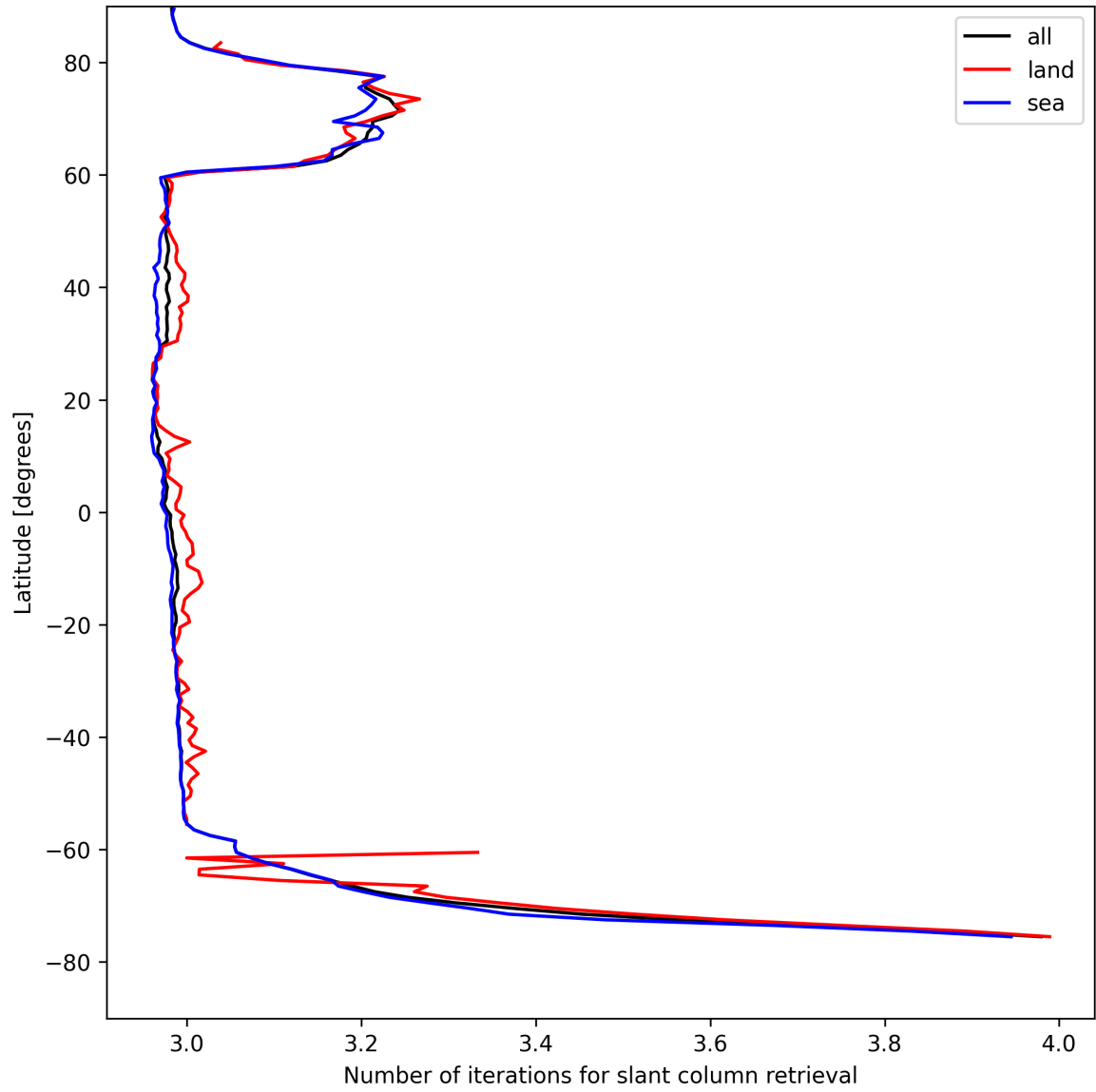
Figure 21: Zonal average of “Number of iterations for slant column retrieval” for 2025-04-25 to 2025-04-26.
