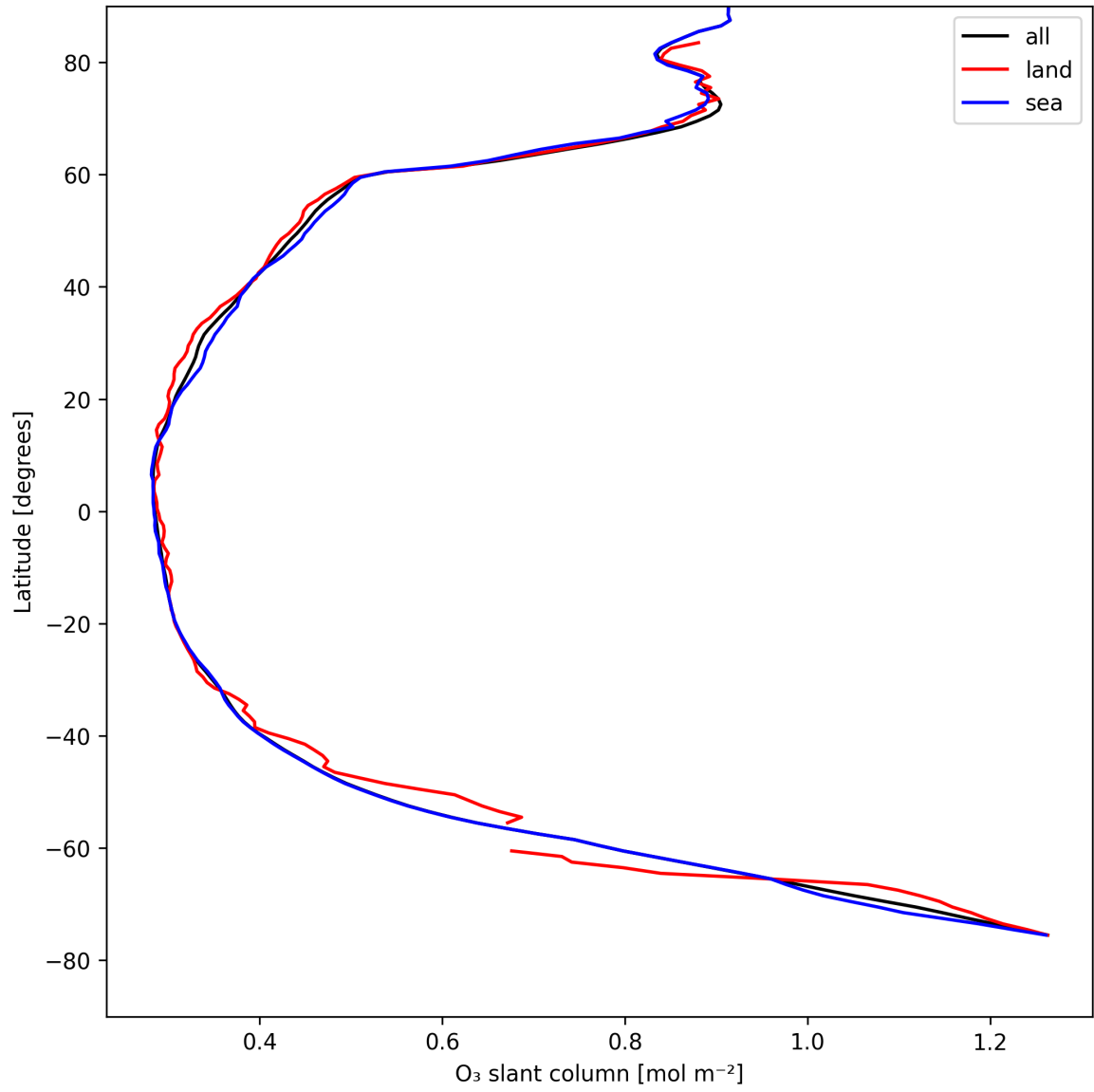
Figure 19: Zonal average of “O 3 slant column” for 2025-04-25 to 2025-04-26.
