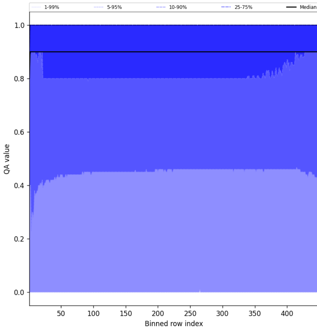
Figure 40: Along track statistics of “QA value” for 2025-04-25 to 2025-04-26
