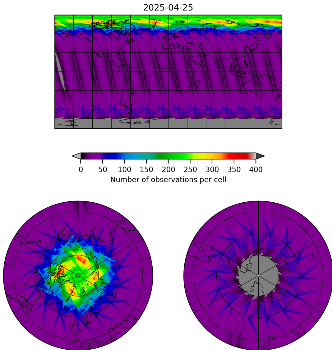
Figure 15: Map of the number of observations for 2025-04-25 to 2025-04-26
