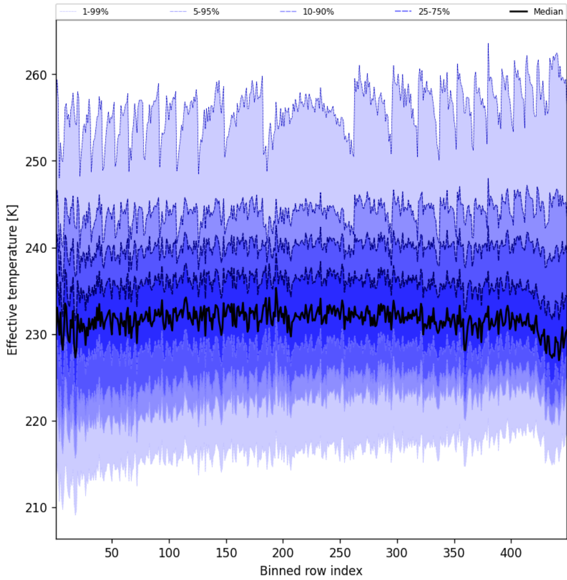
Figure 50: Along track statistics of “Effective temperature” for 2025-04-25 to 2025-04-26
