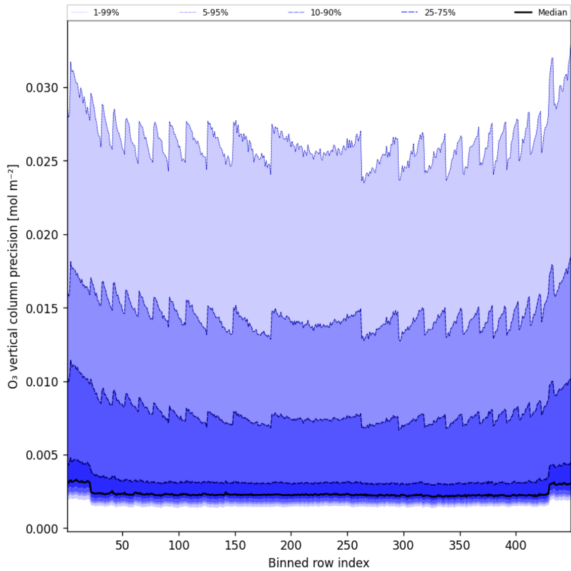
Figure 42: Along track statistics of “O 3 vertical column precision” for 2025-04-25 to 2025-04-26
