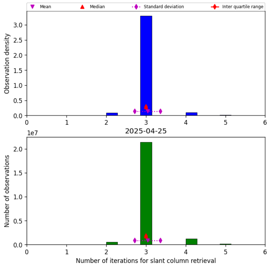
Figure 33: Histogram of “Number of iterations for slant column retrieval” for 2025-04-25 to 2025-04-26
