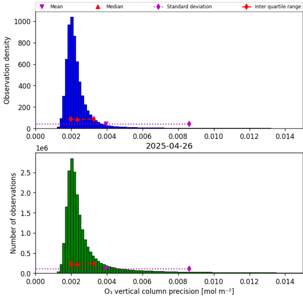
Figure 30: Histogram of “O 3 vertical column precision” for 2025-04-26 to 2025-04-27
