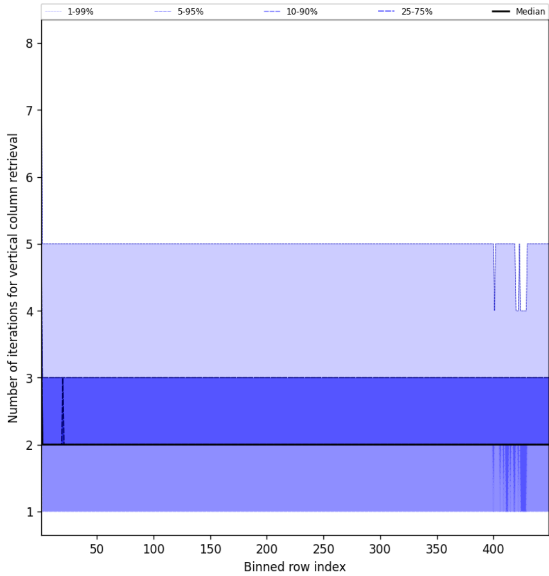
Figure 51: Along track statistics of “Number of iterations for vertical column retrieval” for 2025-04-26 to 2025-04-27
