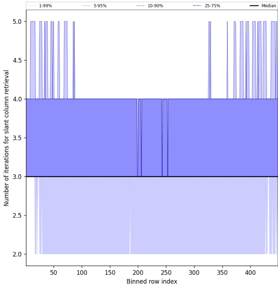
Figure 45: Along track statistics of “Number of iterations for slant column retrieval” for 2025-04-26 to 2025-04-27
