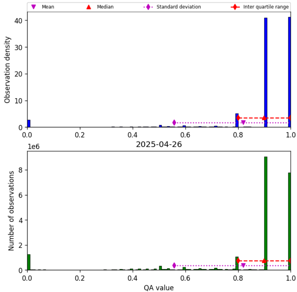
Figure 28: Histogram of “QA value” for 2025-04-26 to 2025-04-27
