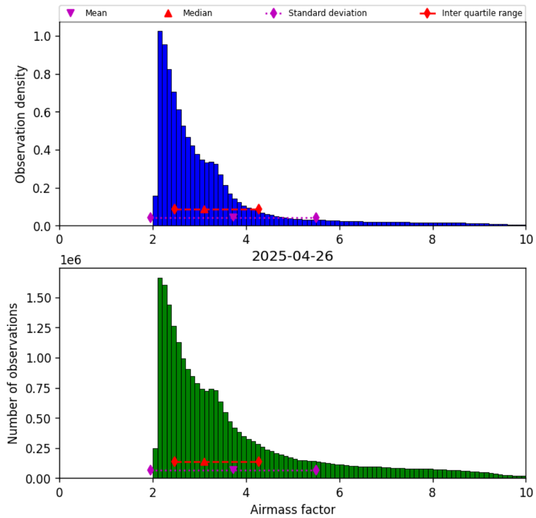
Figure 37: Histogram of “Airmass factor” for 2025-04-26 to 2025-04-27
