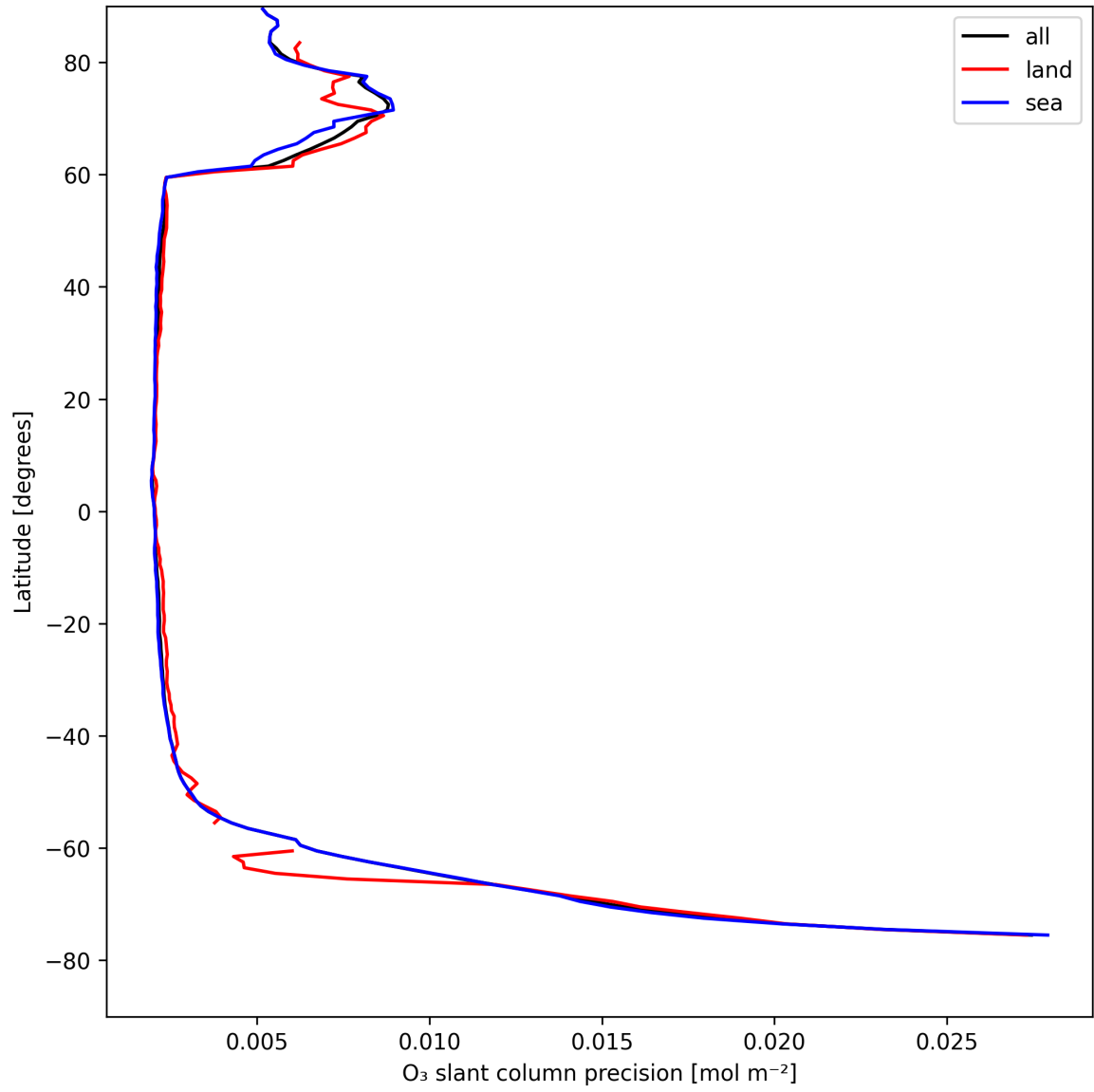
Figure 20: Zonal average of “O 3 slant column precision” for 2025-04-26 to 2025-04-27.
