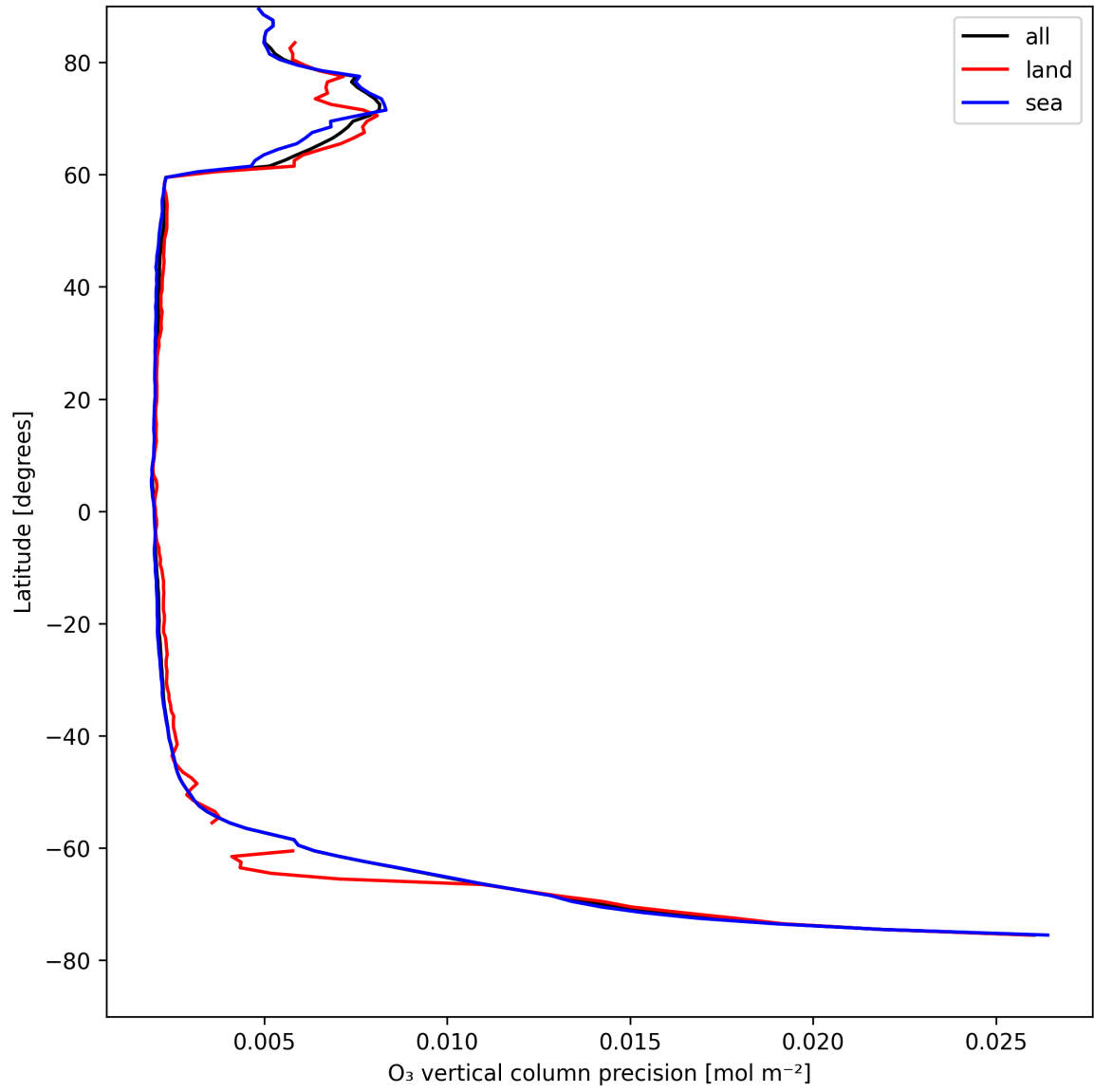
Figure 18: Zonal average of “O 3 vertical column precision” for 2025-04-26 to 2025-04-27.
