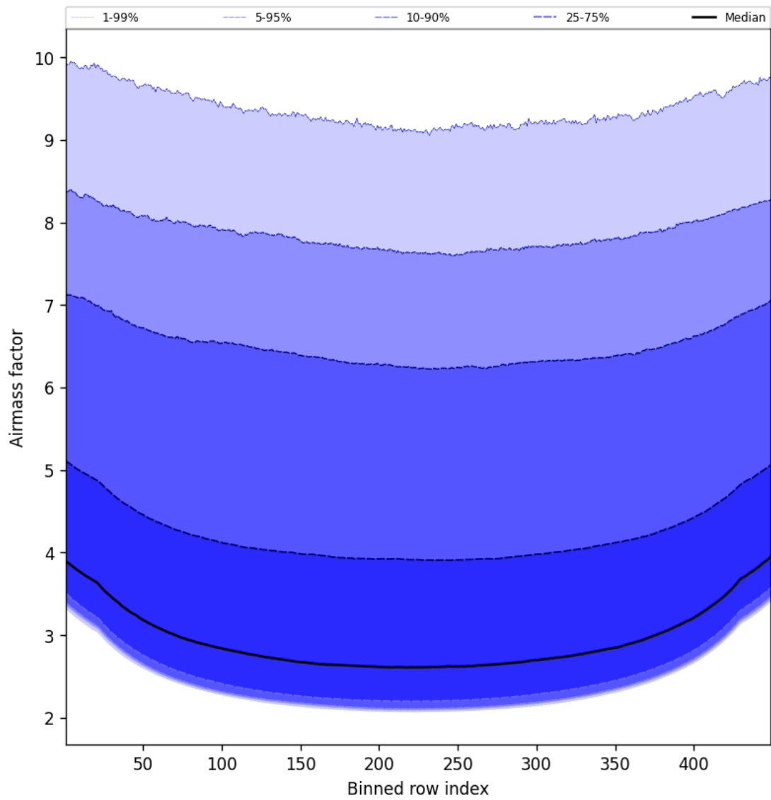
Figure 49: Along track statistics of “Airmass factor” for 2025-04-26 to 2025-04-27
