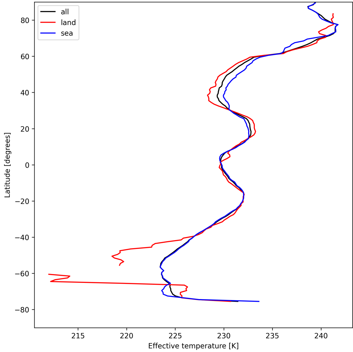
Figure 26: Zonal average of "Effective temperature" for 2025-04-26 to 2025-04-27.
