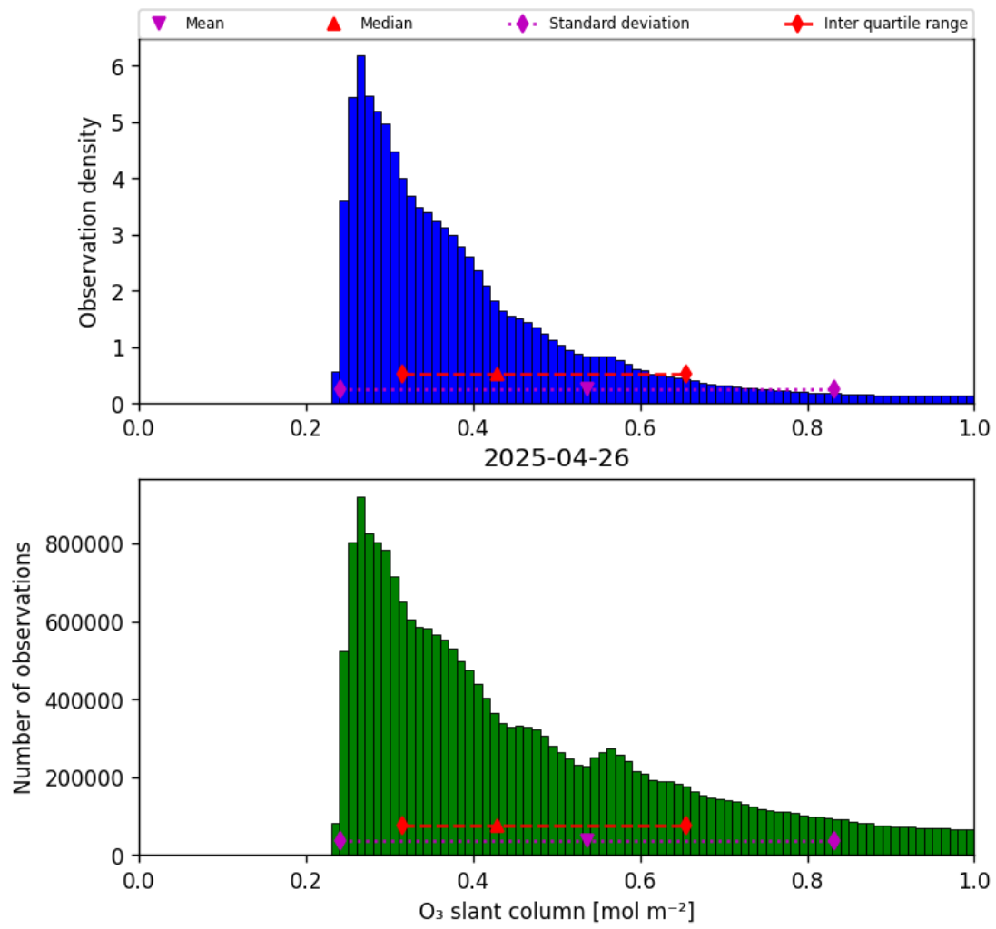
Figure 31: Histogram of “O 3 slant column” for 2025-04-26 to 2025-04-27
