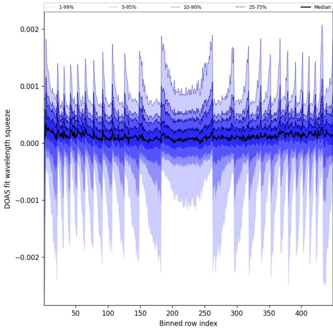
Figure 48: Along track statistics of “DOAS fit wavelength squeeze” for 2025-04-26 to 2025-04-27
