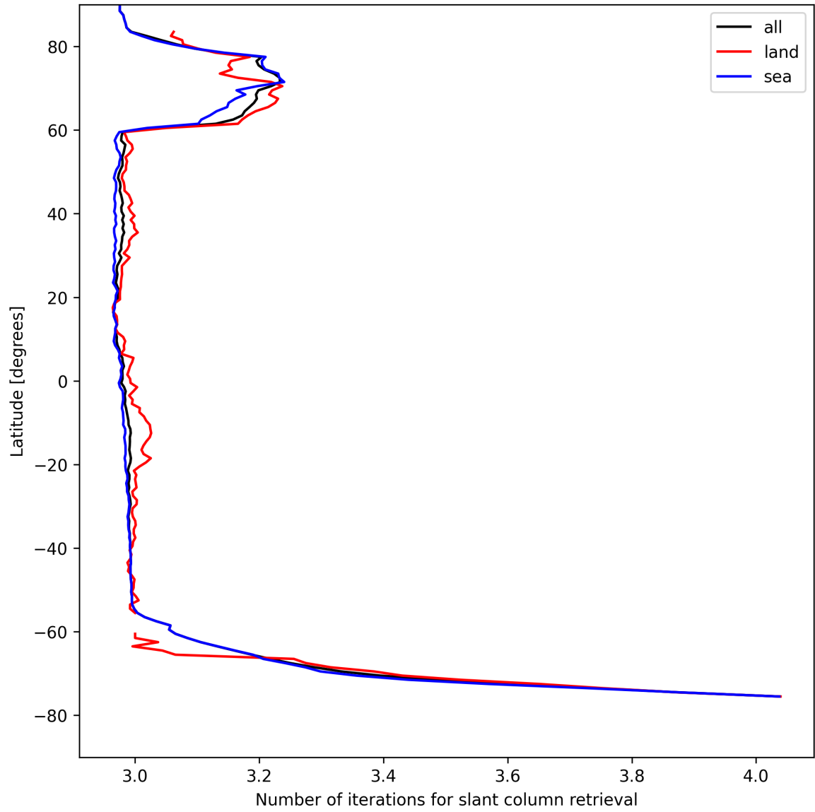
Figure 21: Zonal average of “Number of iterations for slant column retrieval” for 2025-04-26 to 2025-04-27.
