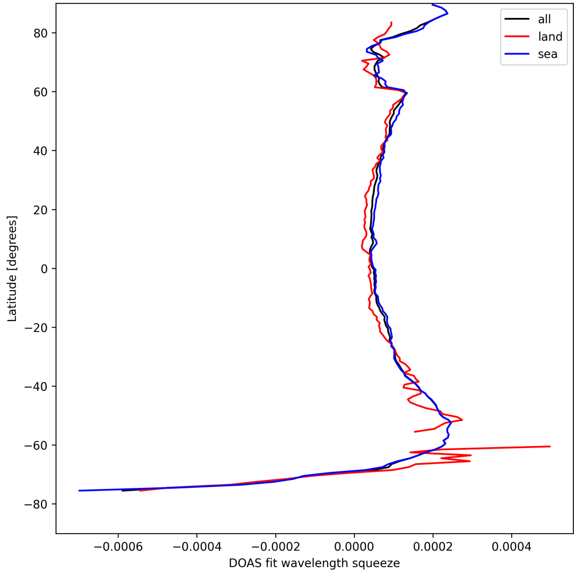
Figure 24: Zonal average of “DOAS fit wavelength squeeze” for 2025-04-26 to 2025-04-27.
