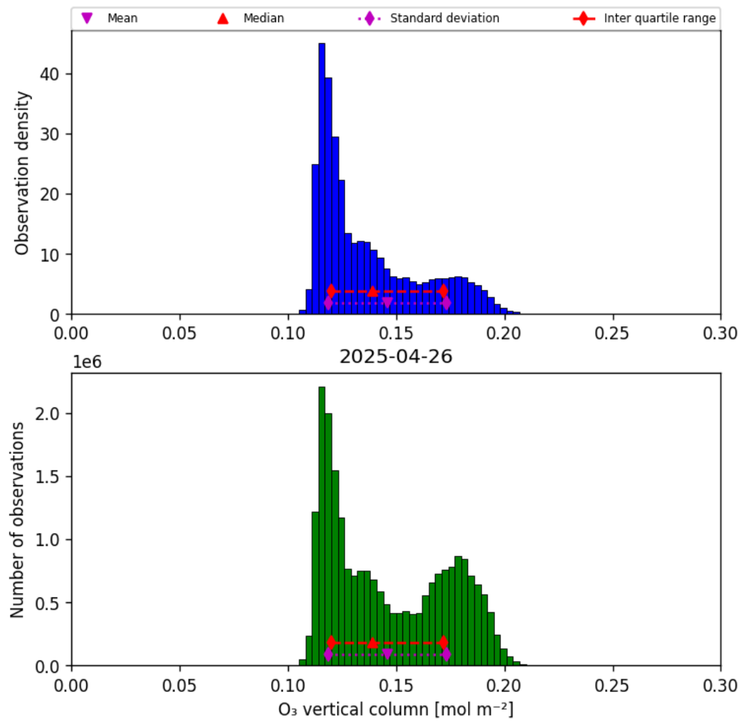
Figure 29: Histogram of “O 3 vertical column” for 2025-04-26 to 2025-04-27
