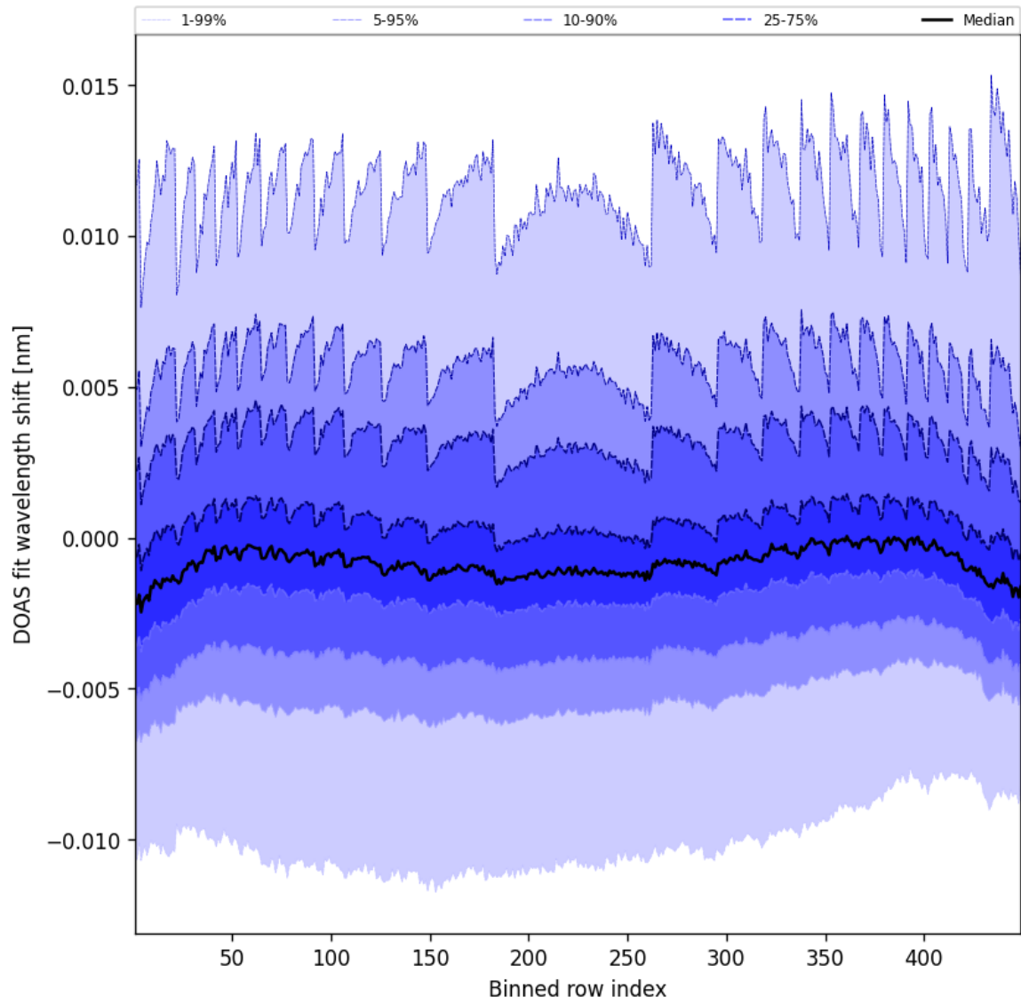
Figure 47: Along track statistics of “DOAS fit wavelength shift” for 2025-04-26 to 2025-04-27
