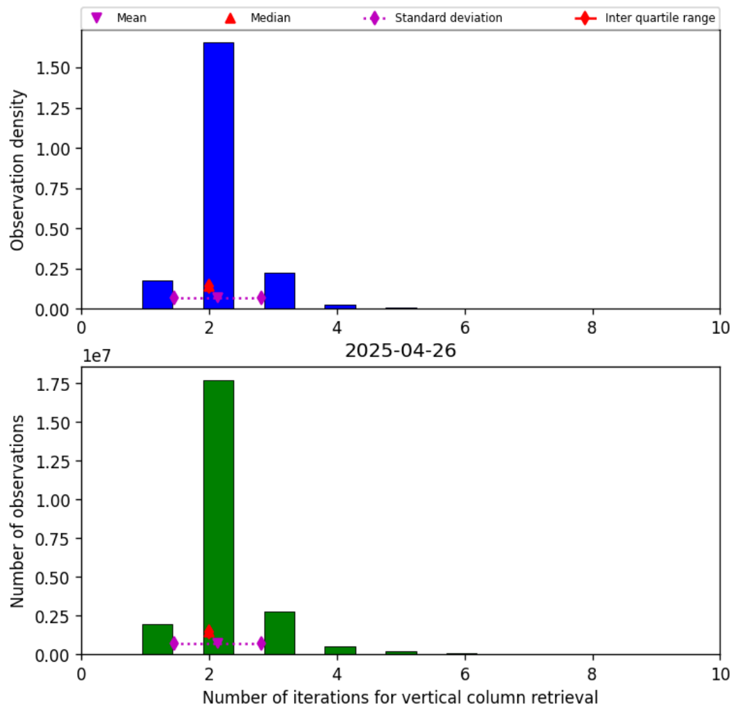
Figure 39: Histogram of “Number of iterations for vertical column retrieval” for 2025-04-26 to 2025-04-27
