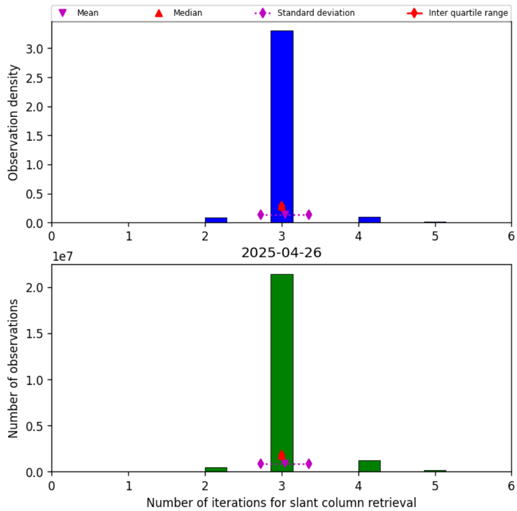
Figure 33: Histogram of “Number of iterations for slant column retrieval” for 2025-04-26 to 2025-04-27
