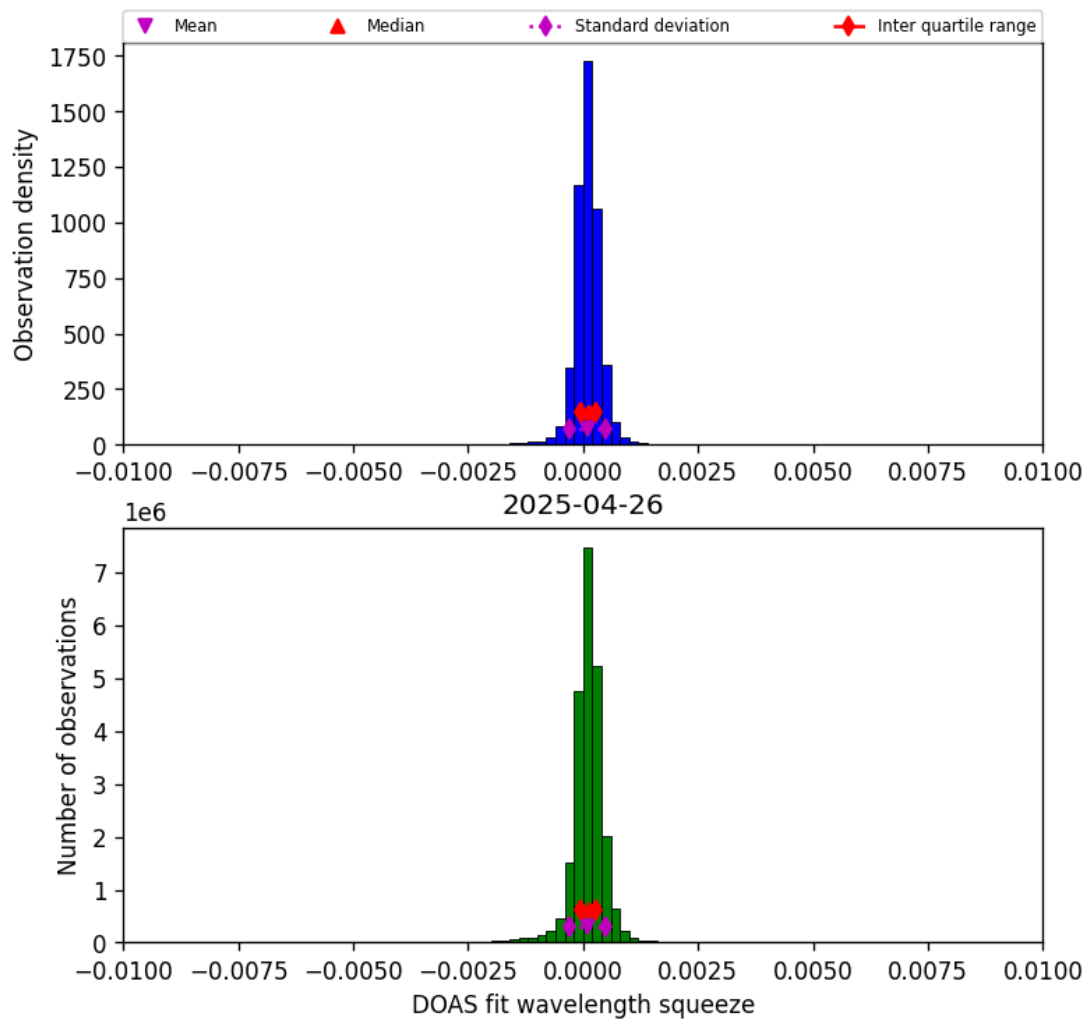
Figure 36: Histogram of “DOAS fit wavelength squeeze” for 2025-04-26 to 2025-04-27
