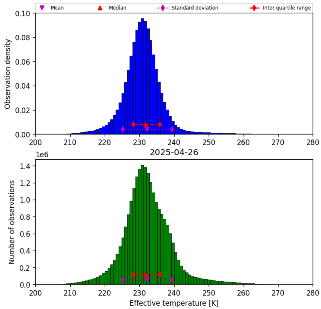
Figure 38: Histogram of “Effective temperature” for 2025-04-26 to 2025-04-27
