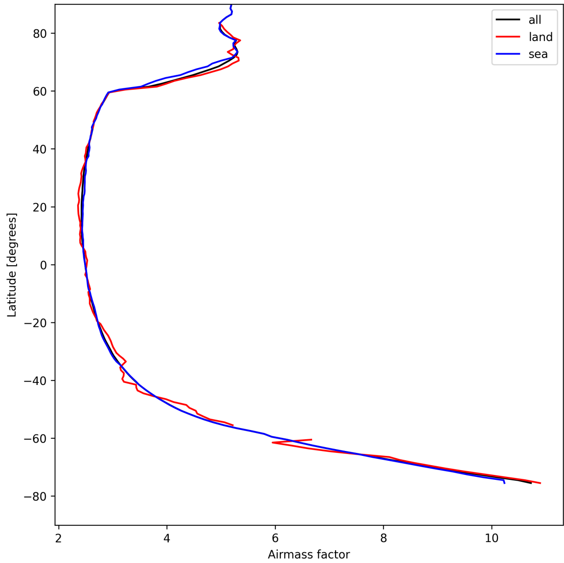
Figure 25: Zonal average of “Airmass factor” for 2025-04-26 to 2025-04-27.
