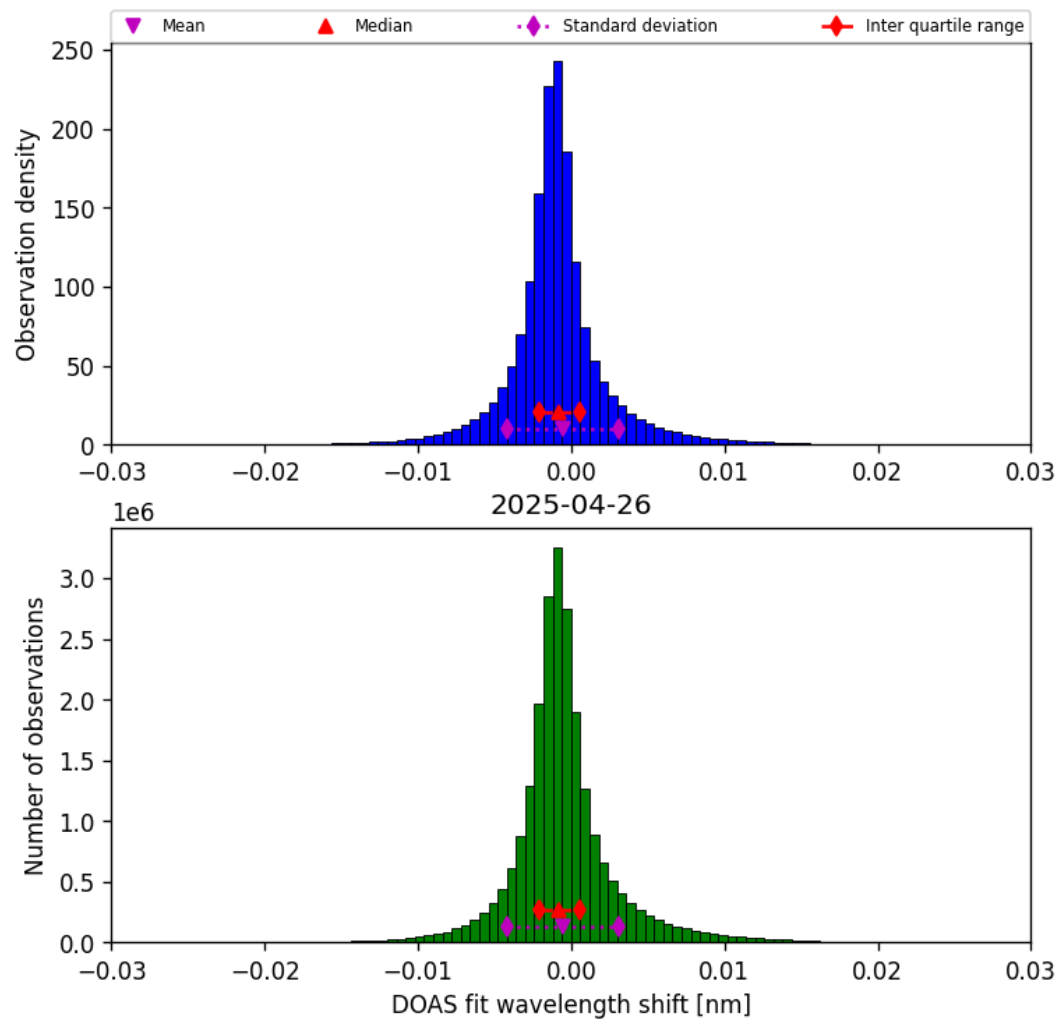
Figure 35: Histogram of “DOAS fit wavelength shift” for 2025-04-26 to 2025-04-27
