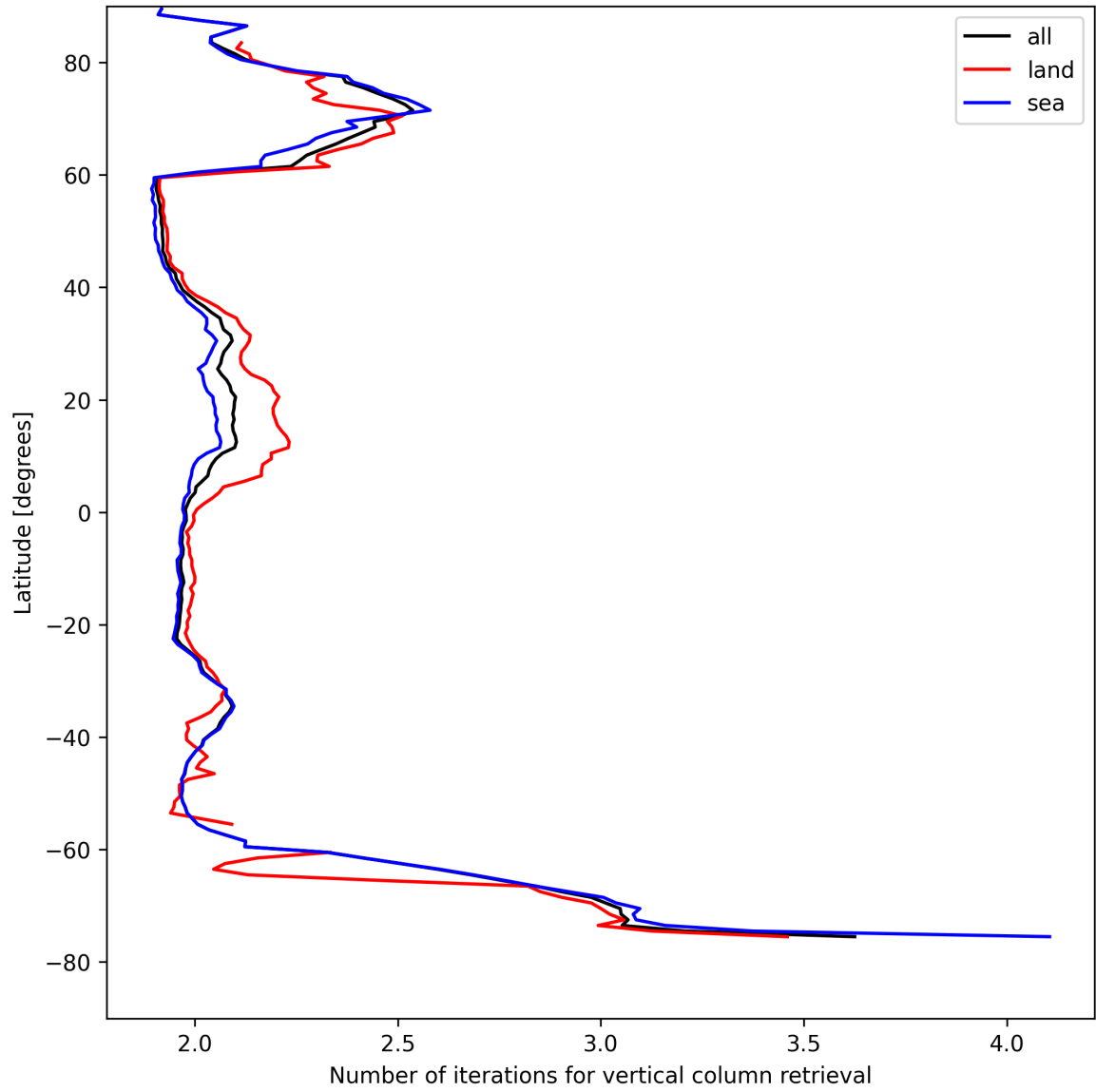
Figure 27: Zonal average of “Number of iterations for vertical column retrieval” for 2025-04-26 to 2025-04-27.
