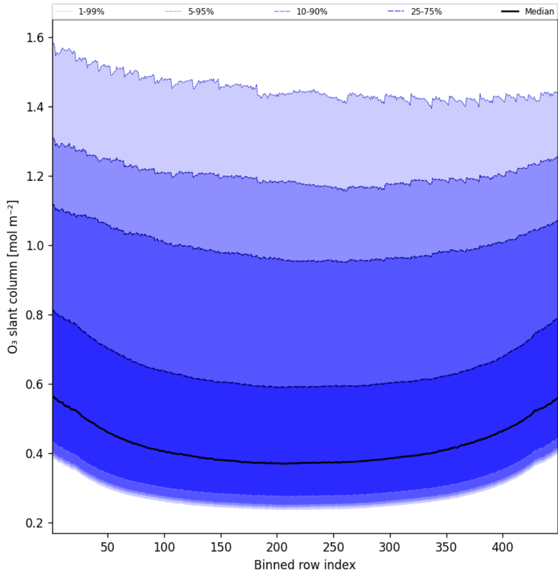
Figure 43: Along track statistics of “O 3 slant column” for 2025-04-26 to 2025-04-27
