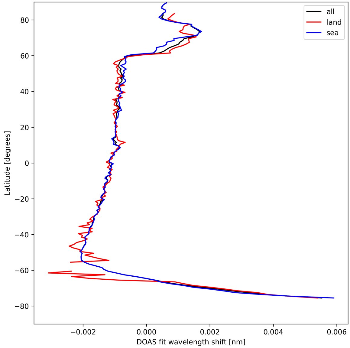
Figure 23: Zonal average of “DOAS fit wavelength shift” for 2025-04-26 to 2025-04-27.
