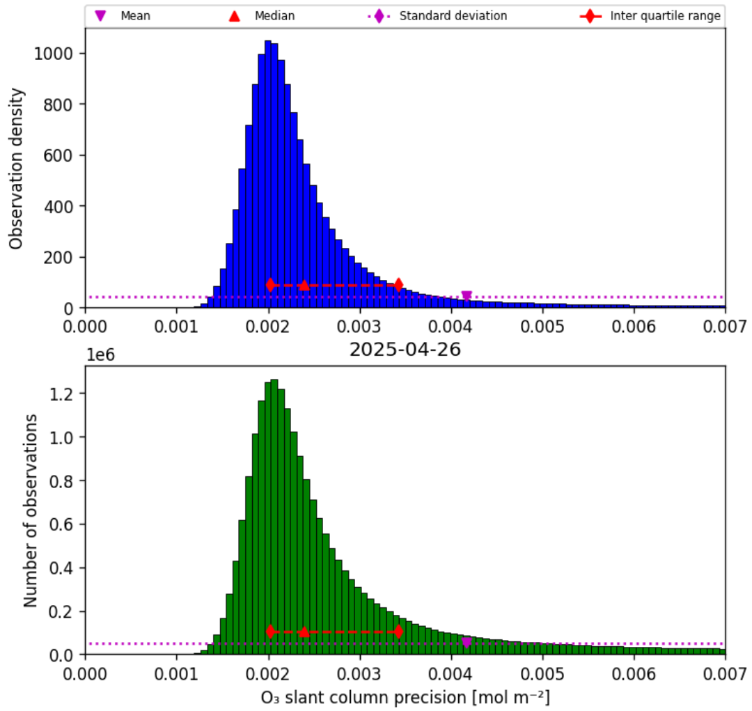
Figure 32: Histogram of “O 3 slant column precision” for 2025-04-26 to 2025-04-27
