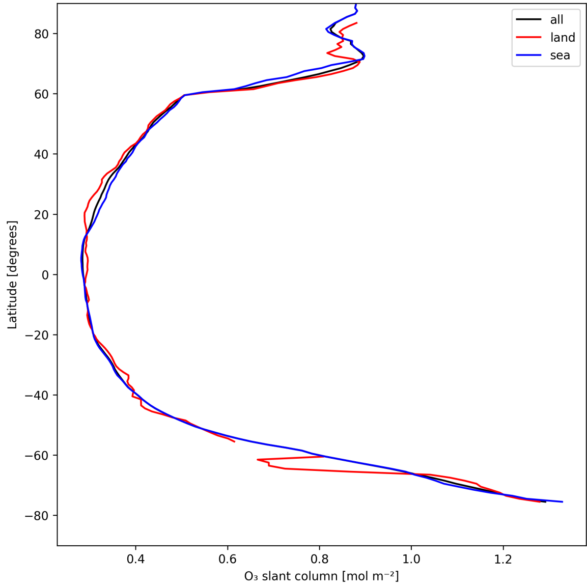
Figure 19: Zonal average of “O 3 slant column” for 2025-04-26 to 2025-04-27.
