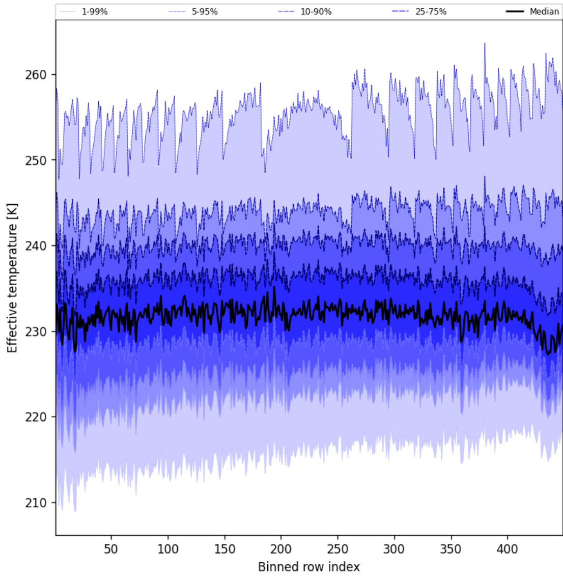
Figure 50: Along track statistics of “Effective temperature” for 2025-04-26 to 2025-04-27
