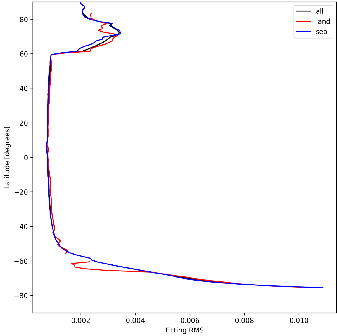
Figure 22: Zonal average of “Fitting RMS” for 2025-04-26 to 2025-04-27.
