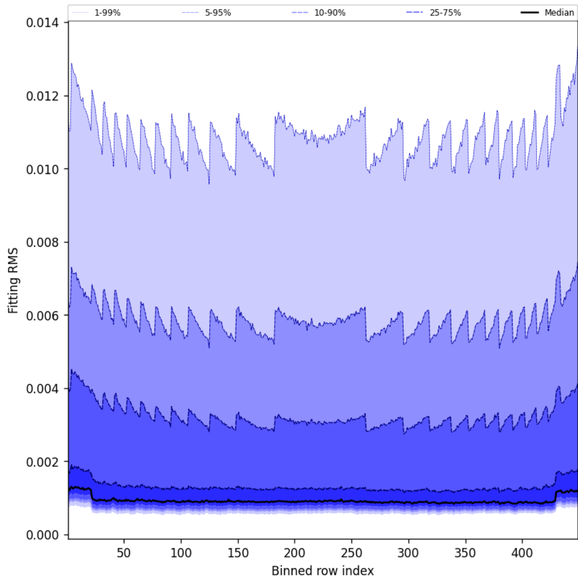
Figure 46: Along track statistics of “Fitting RMS” for 2025-04-26 to 2025-04-27
