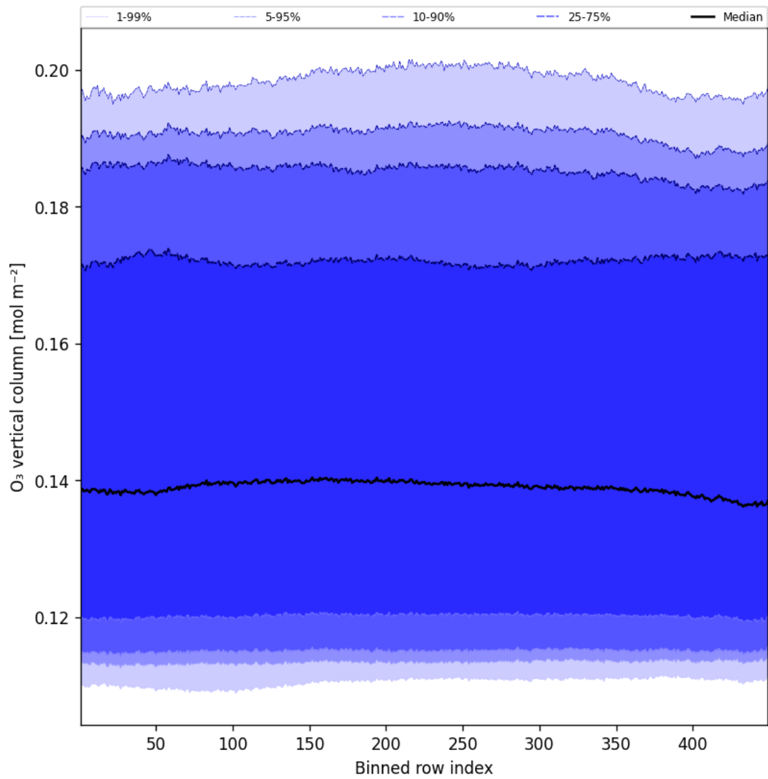
Figure 41: Along track statistics of “O 3 vertical column” for 2025-04-26 to 2025-04-27
