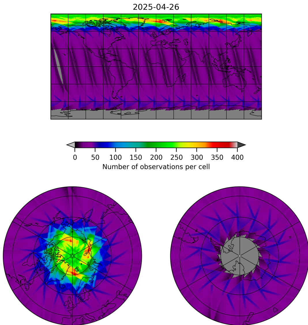
Figure 15: Map of the number of observations for 2025-04-26 to 2025-04-27
