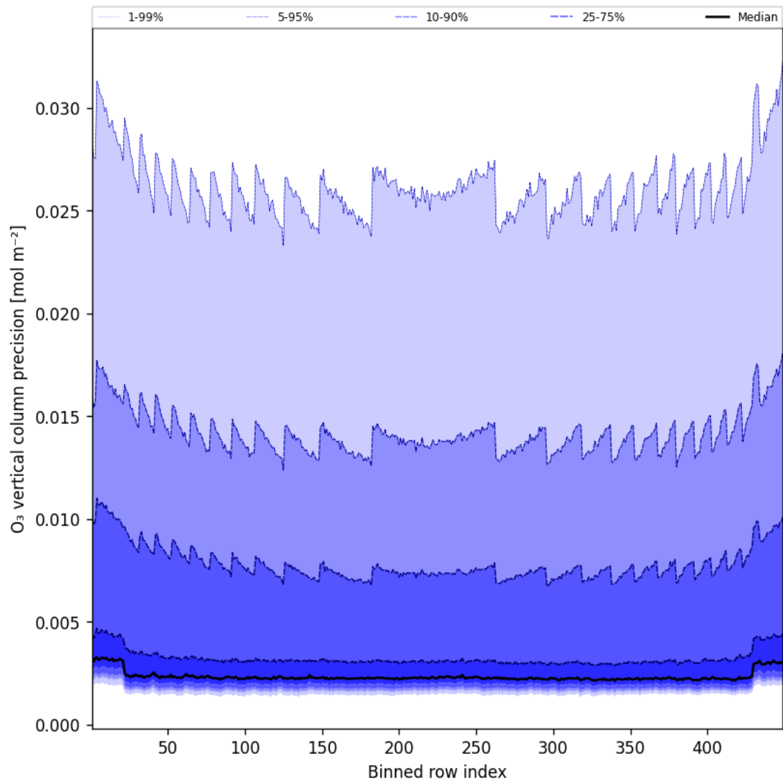
Figure 42: Along track statistics of “O 3 vertical column precision” for 2025-04-26 to 2025-04-27
