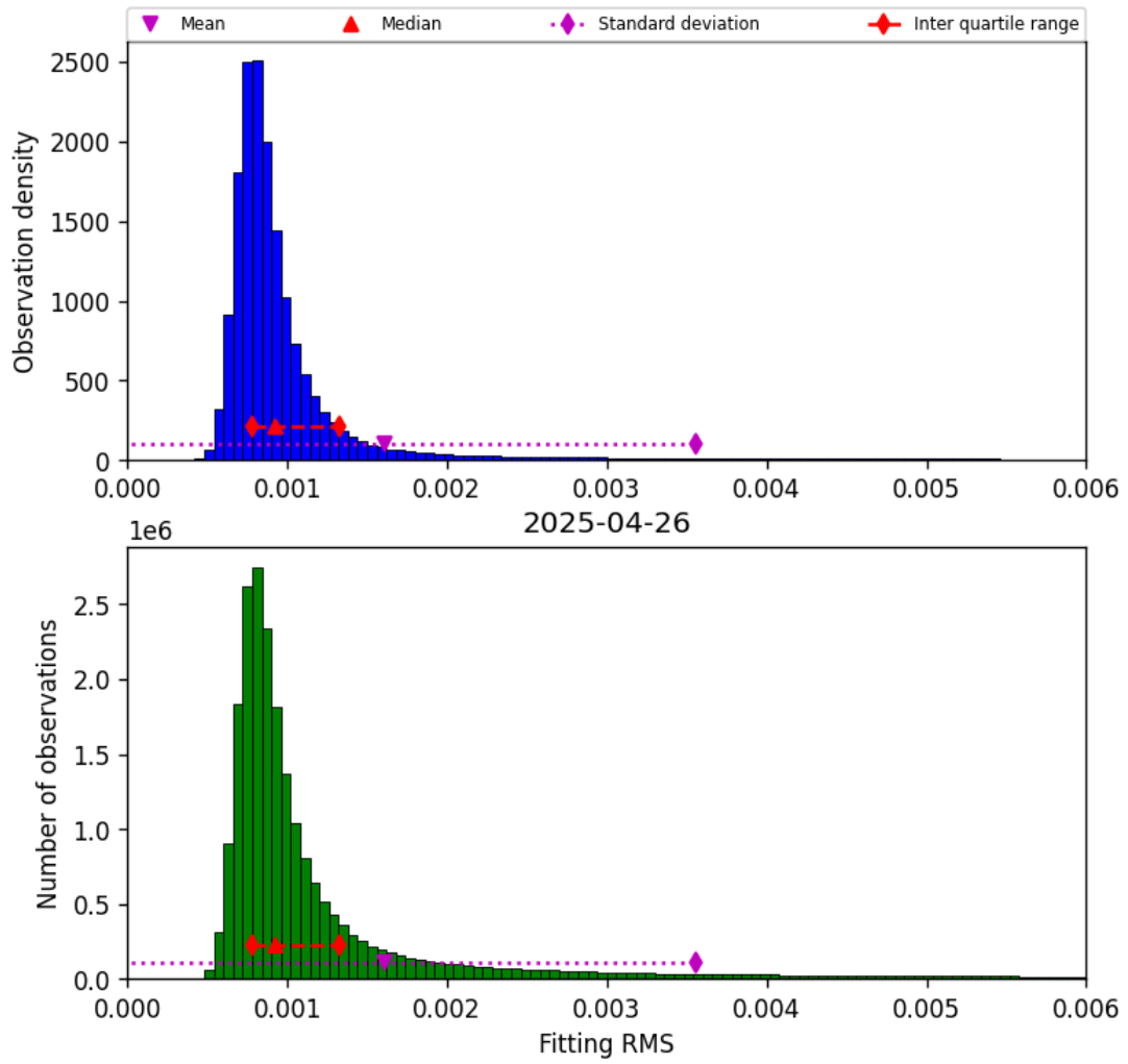
Figure 34: Histogram of “Fitting RMS” for 2025-04-26 to 2025-04-27
