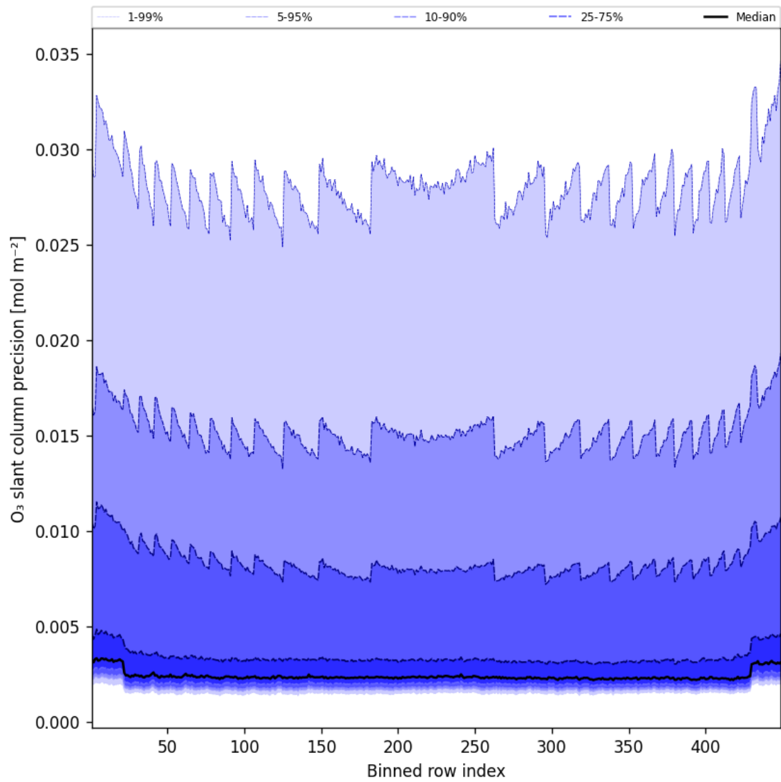
Figure 44: Along track statistics of “O 3 slant column precision” for 2025-04-26 to 2025-04-27
