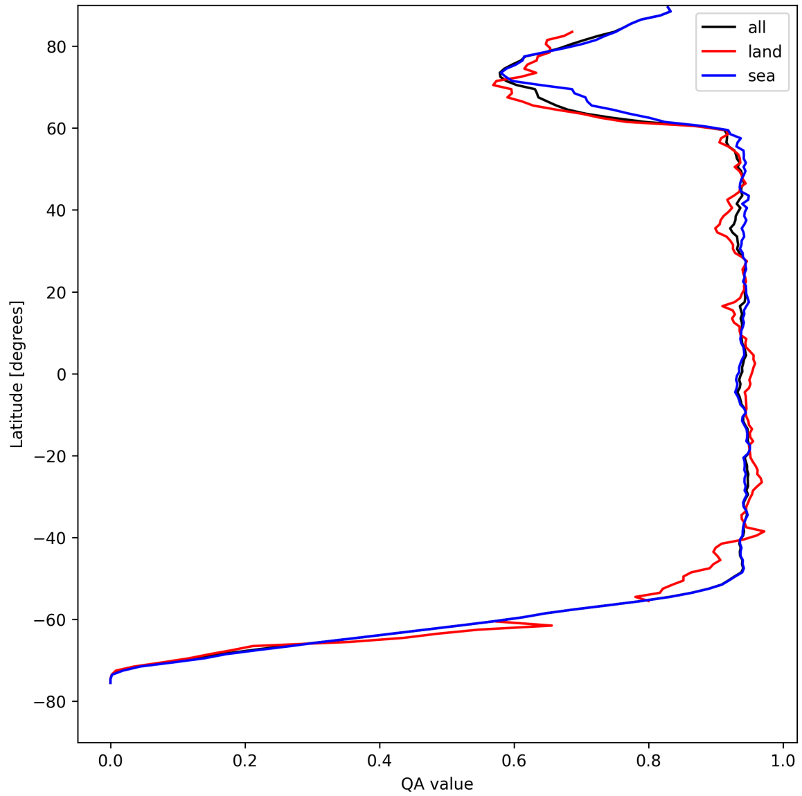
Figure 16: Zonal average of “QA value” for 2025-04-26 to 2025-04-27.
