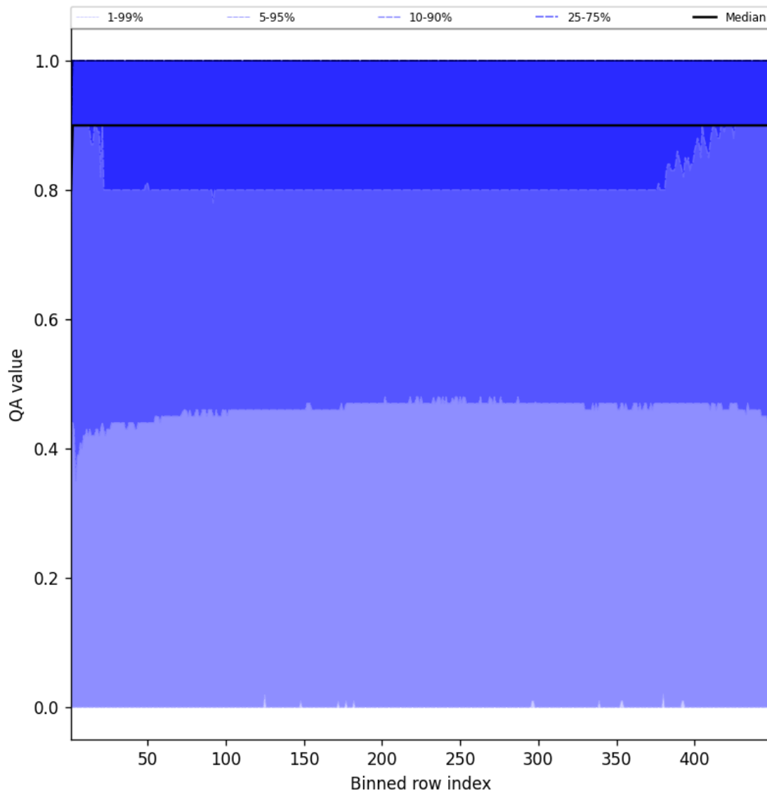
Figure 40: Along track statistics of “QA value” for 2025-04-26 to 2025-04-27
