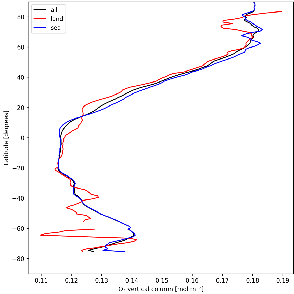
Figure 17: Zonal average of “O 3 vertical column” for 2025-04-26 to 2025-04-27.
