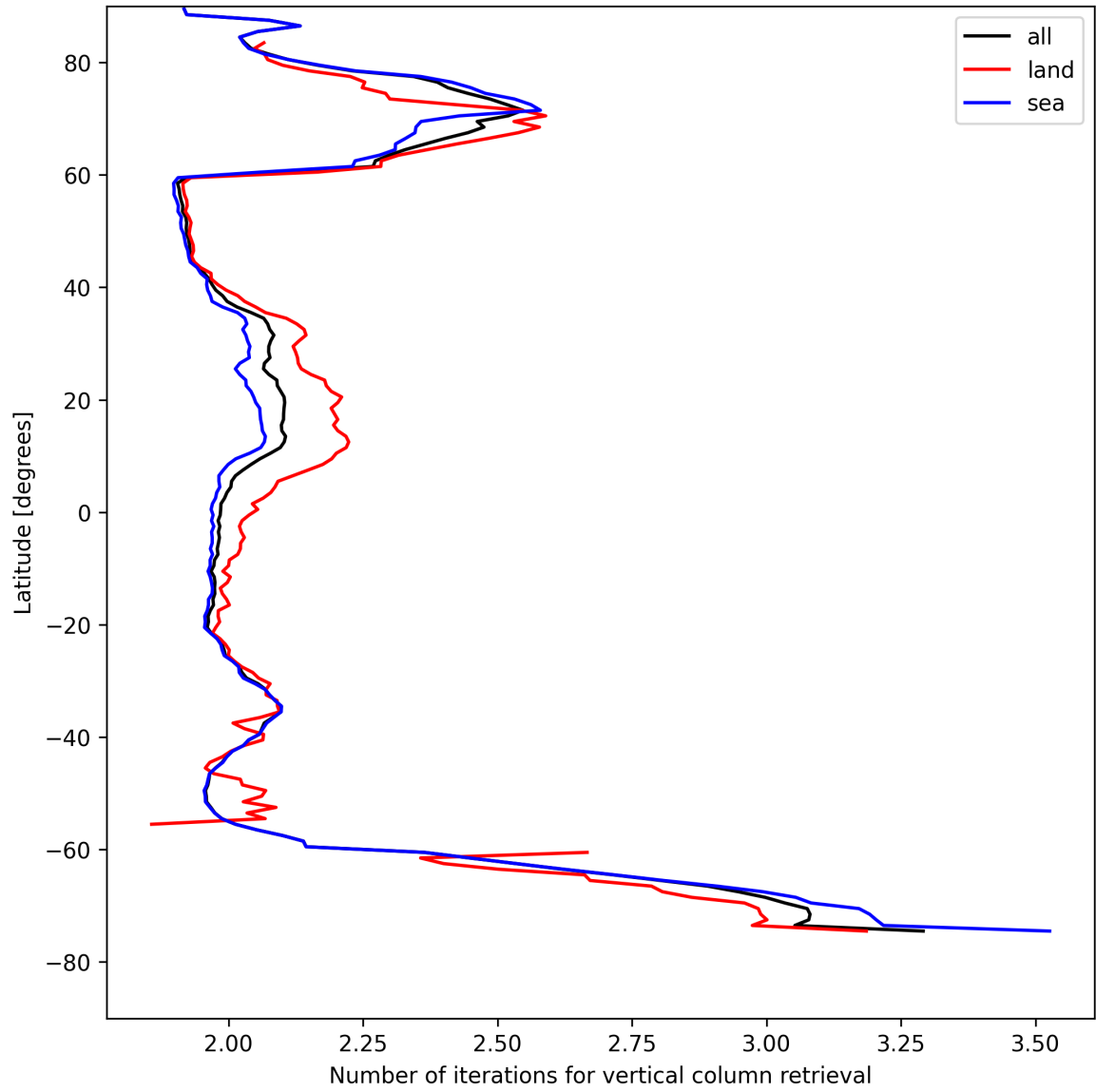
Figure 27: Zonal average of “Number of iterations for vertical column retrieval” for 2025-04-27 to 2025-04-27.
