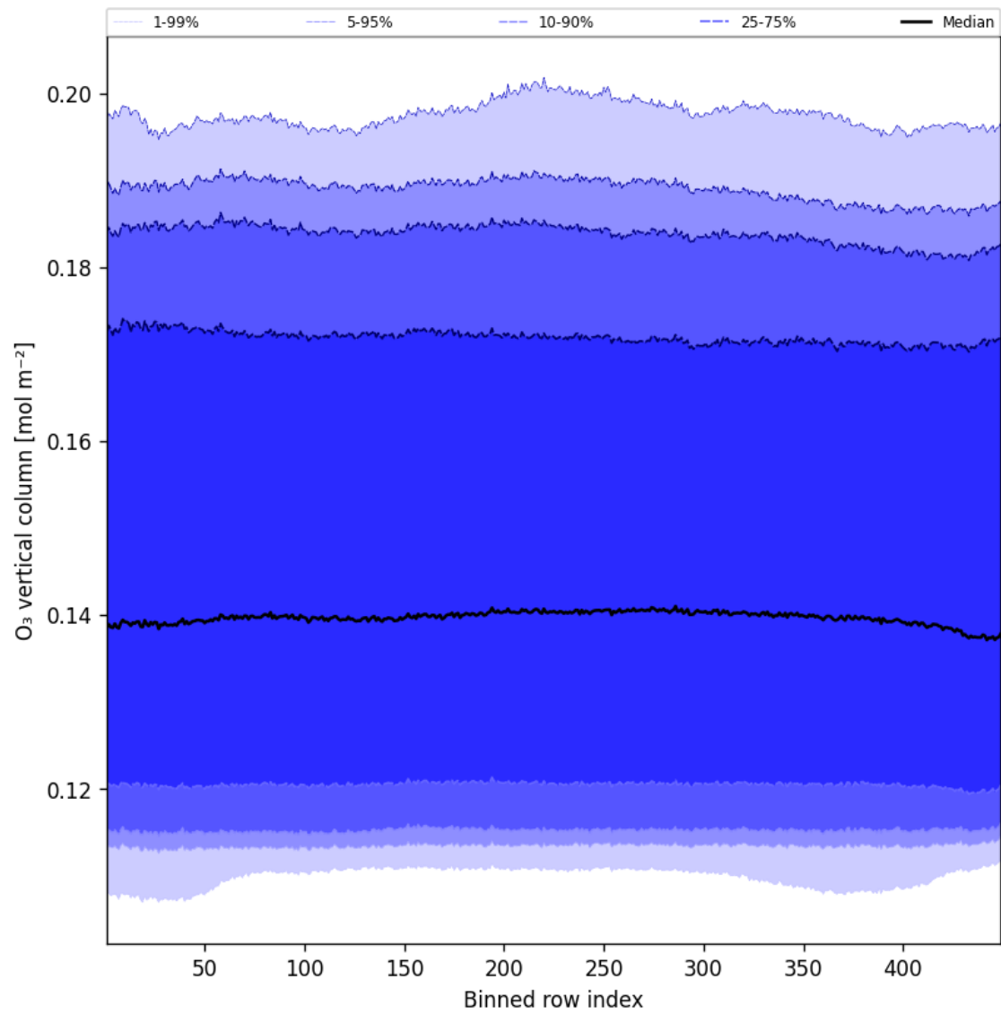
Figure 41: Along track statistics of “O 3 vertical column” for 2025-04-27 to 2025-04-27
