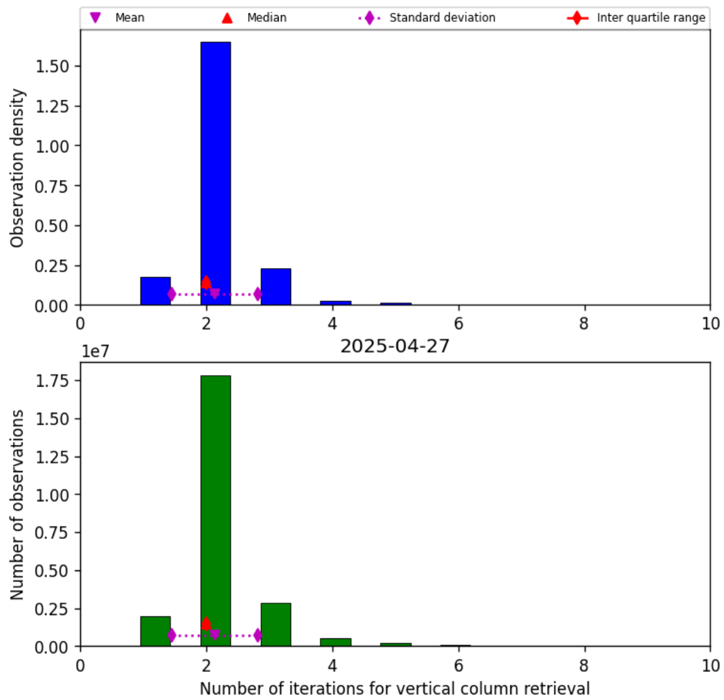
Figure 39: Histogram of “Number of iterations for vertical column retrieval” for 2025-04-27 to 2025-04-27
