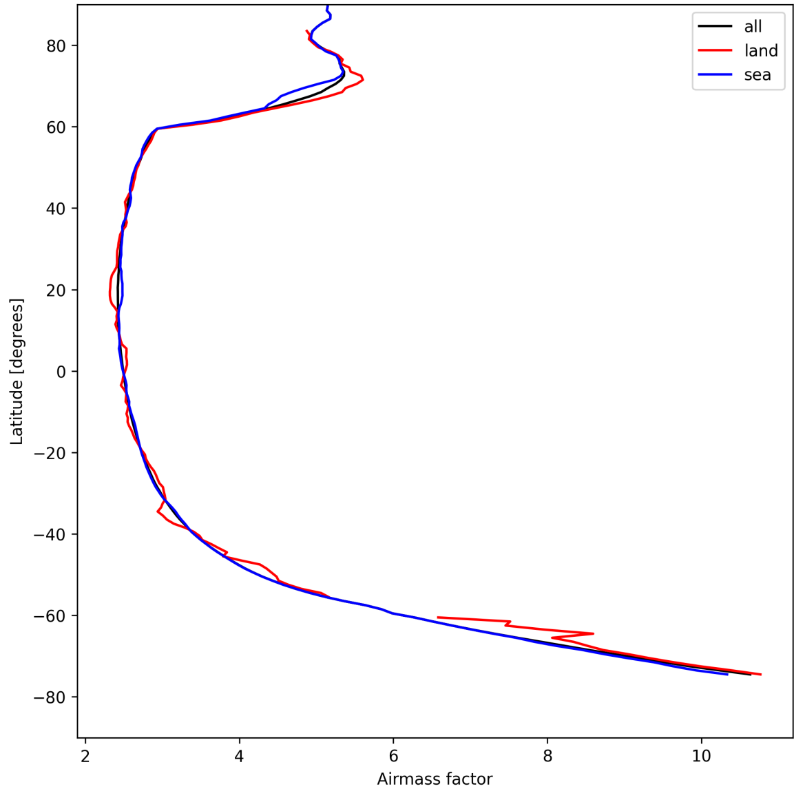
Figure 25: Zonal average of “Airmass factor” for 2025-04-27 to 2025-04-27.
