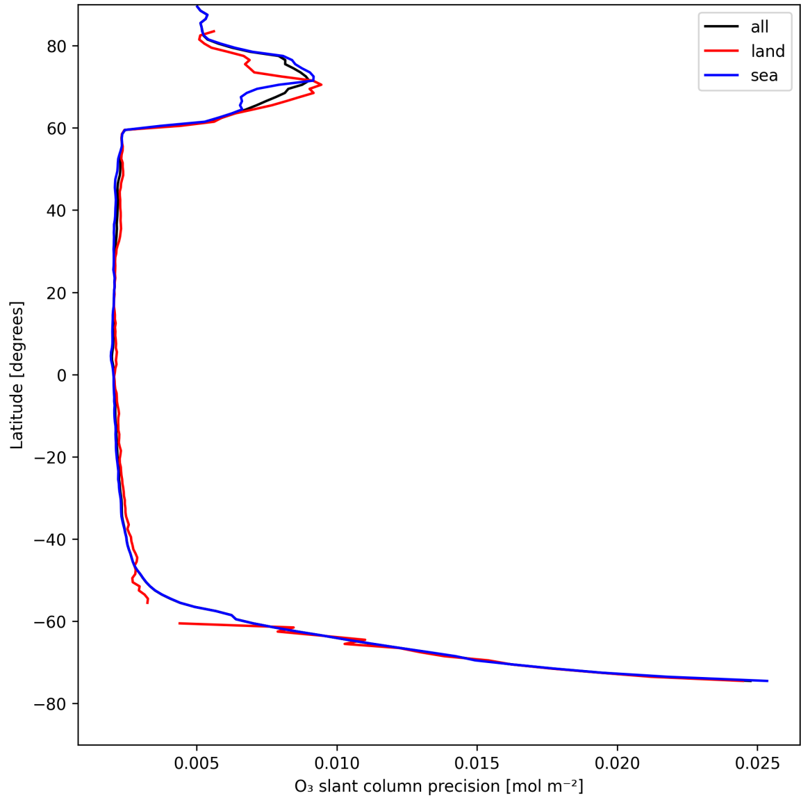
Figure 20: Zonal average of “O 3 slant column precision” for 2025-04-27 to 2025-04-27.
