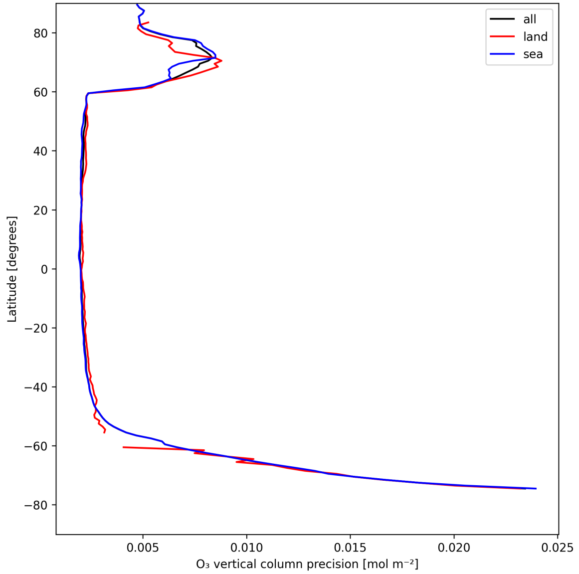
Figure 18: Zonal average of “O 3 vertical column precision” for 2025-04-27 to 2025-04-27.
