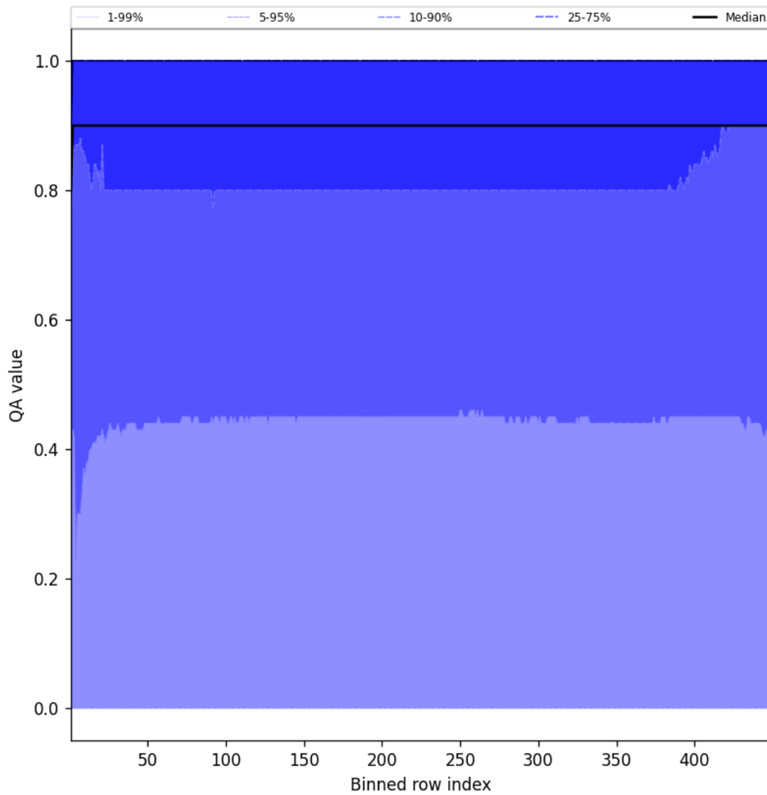
Figure 40: Along track statistics of “QA value” for 2025-04-27 to 2025-04-27
