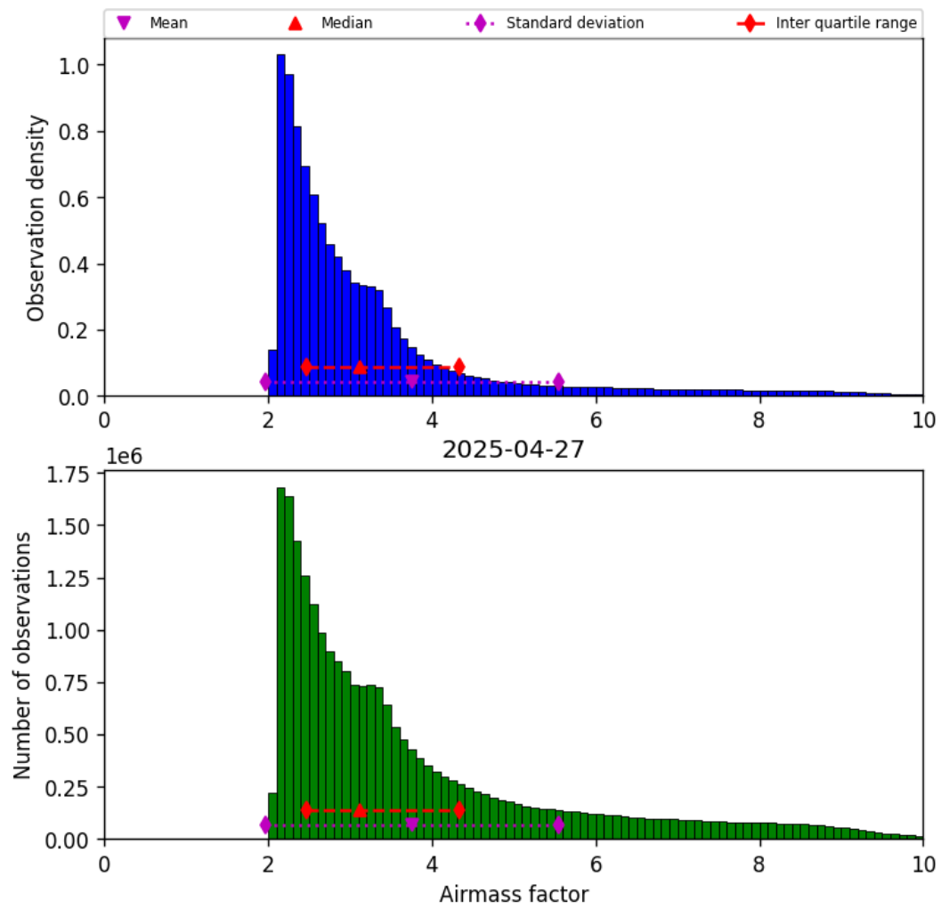
Figure 37: Histogram of “Airmass factor” for 2025-04-27 to 2025-04-27
