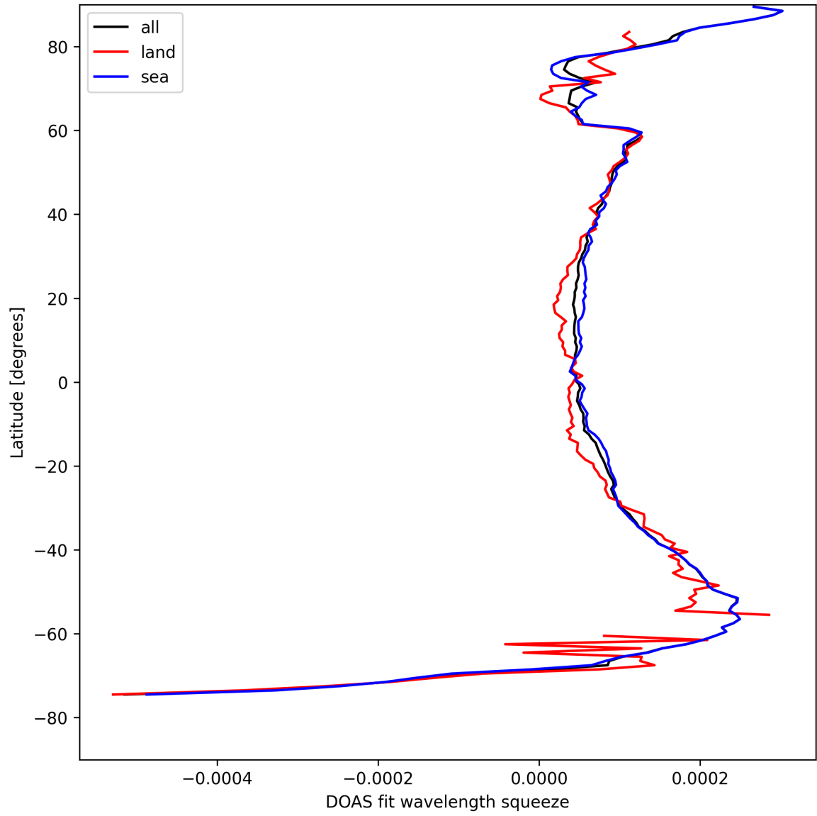
Figure 24: Zonal average of “DOAS fit wavelength squeeze” for 2025-04-27 to 2025-04-27.
