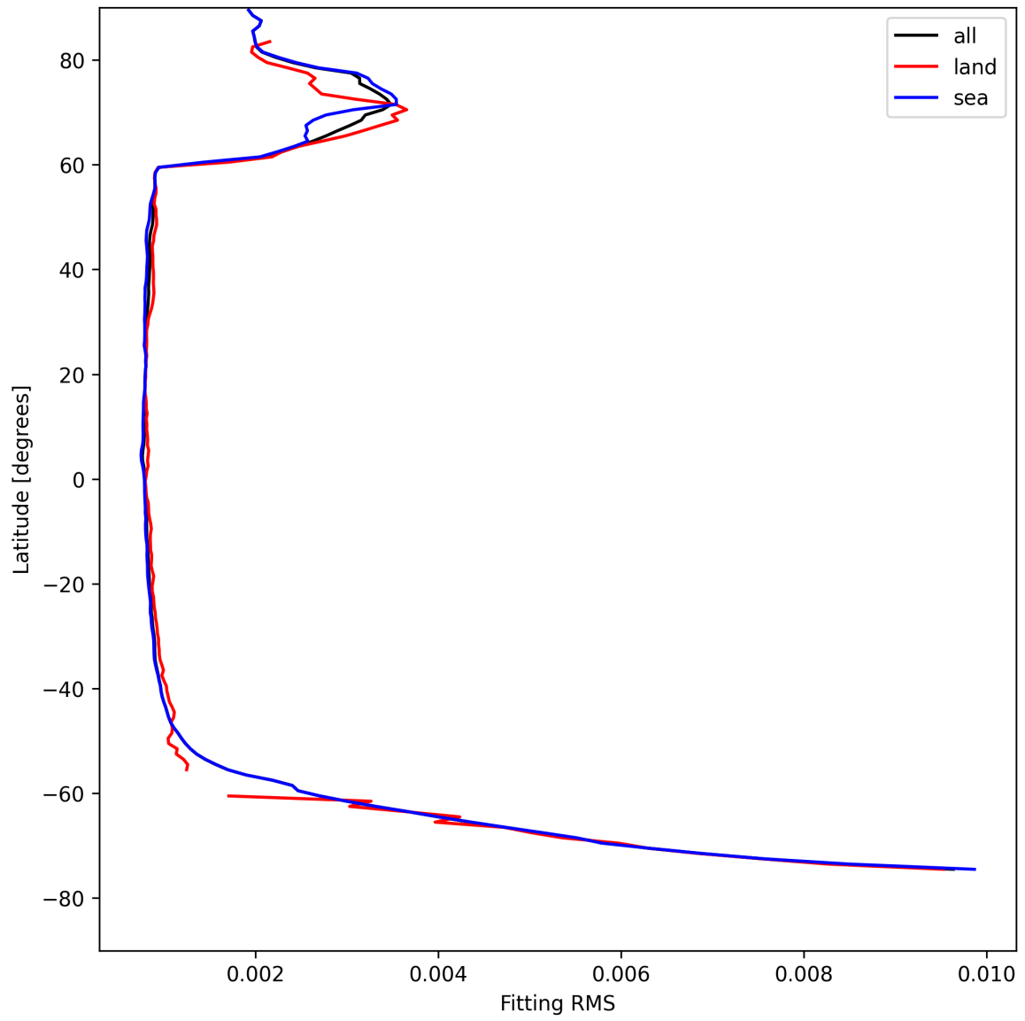
Figure 22: Zonal average of “Fitting RMS” for 2025-04-27 to 2025-04-27.
