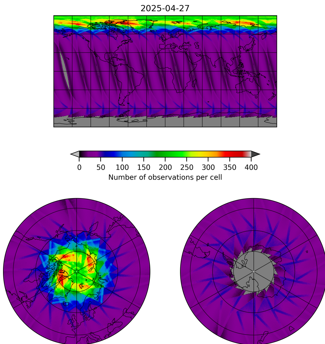
Figure 15: Map of the number of observations for 2025-04-27 to 2025-04-27
