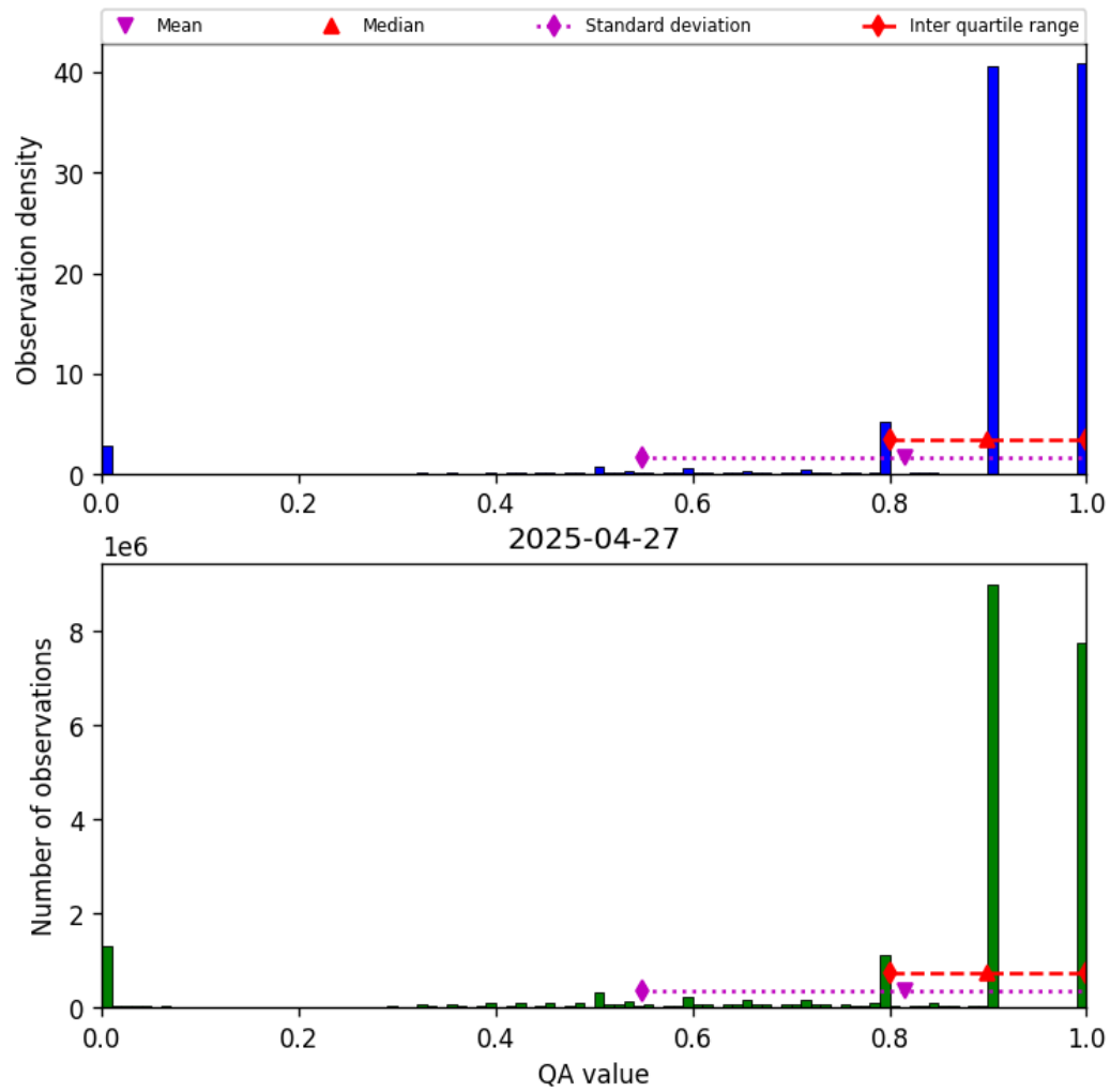
Figure 28: Histogram of “QA value” for 2025-04-27 to 2025-04-27
