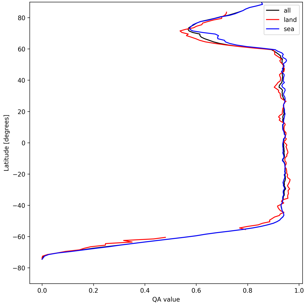
Figure 16: Zonal average of “QA value” for 2025-04-27 to 2025-04-27.
