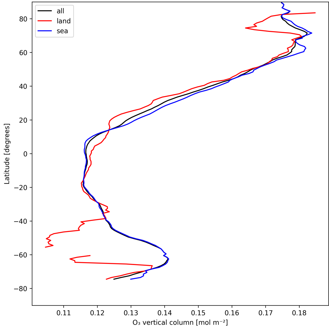
Figure 17: Zonal average of “O 3 vertical column” for 2025-04-27 to 2025-04-27.
