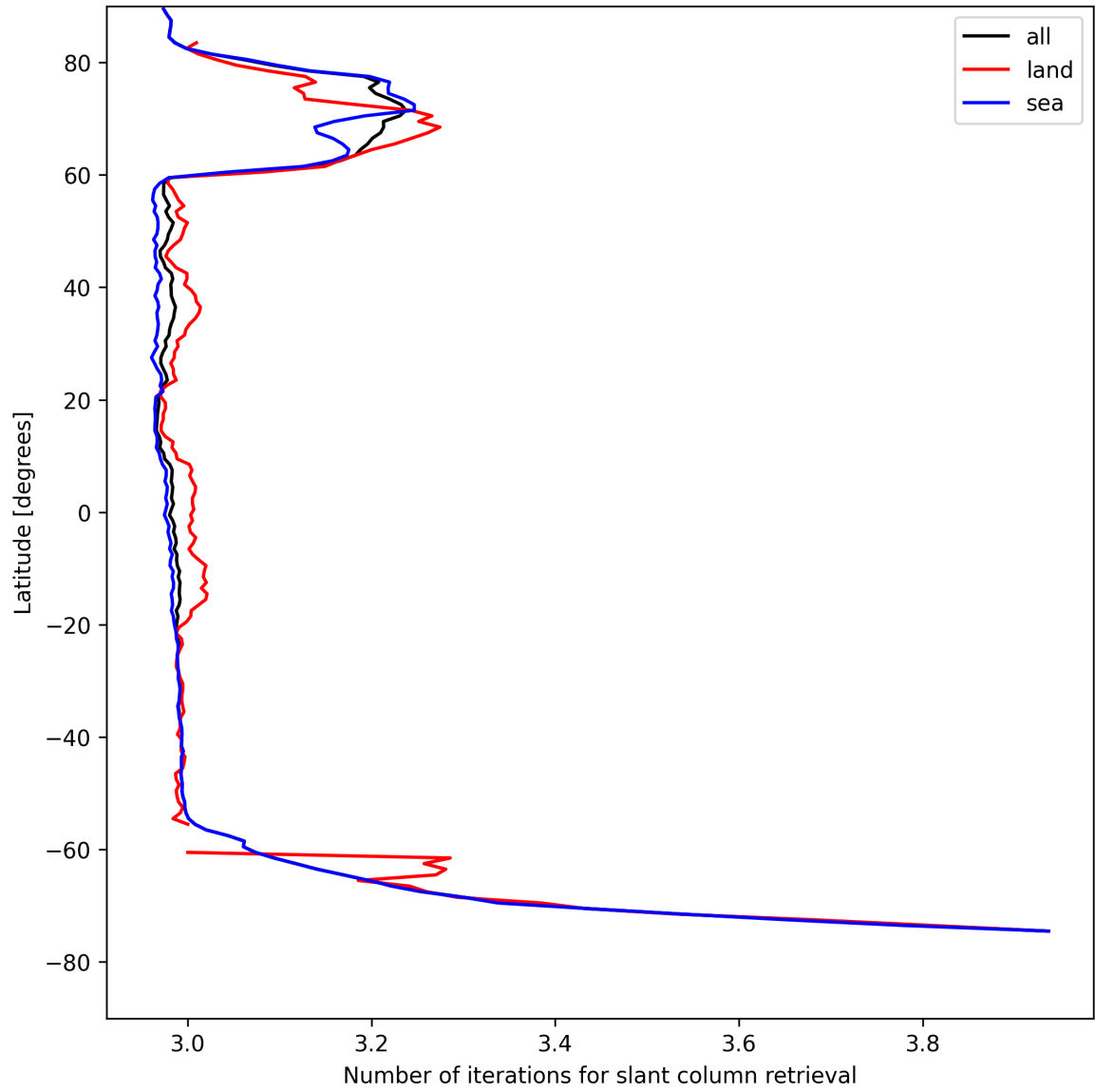
Figure 21: Zonal average of “Number of iterations for slant column retrieval” for 2025-04-27 to 2025-04-27.
