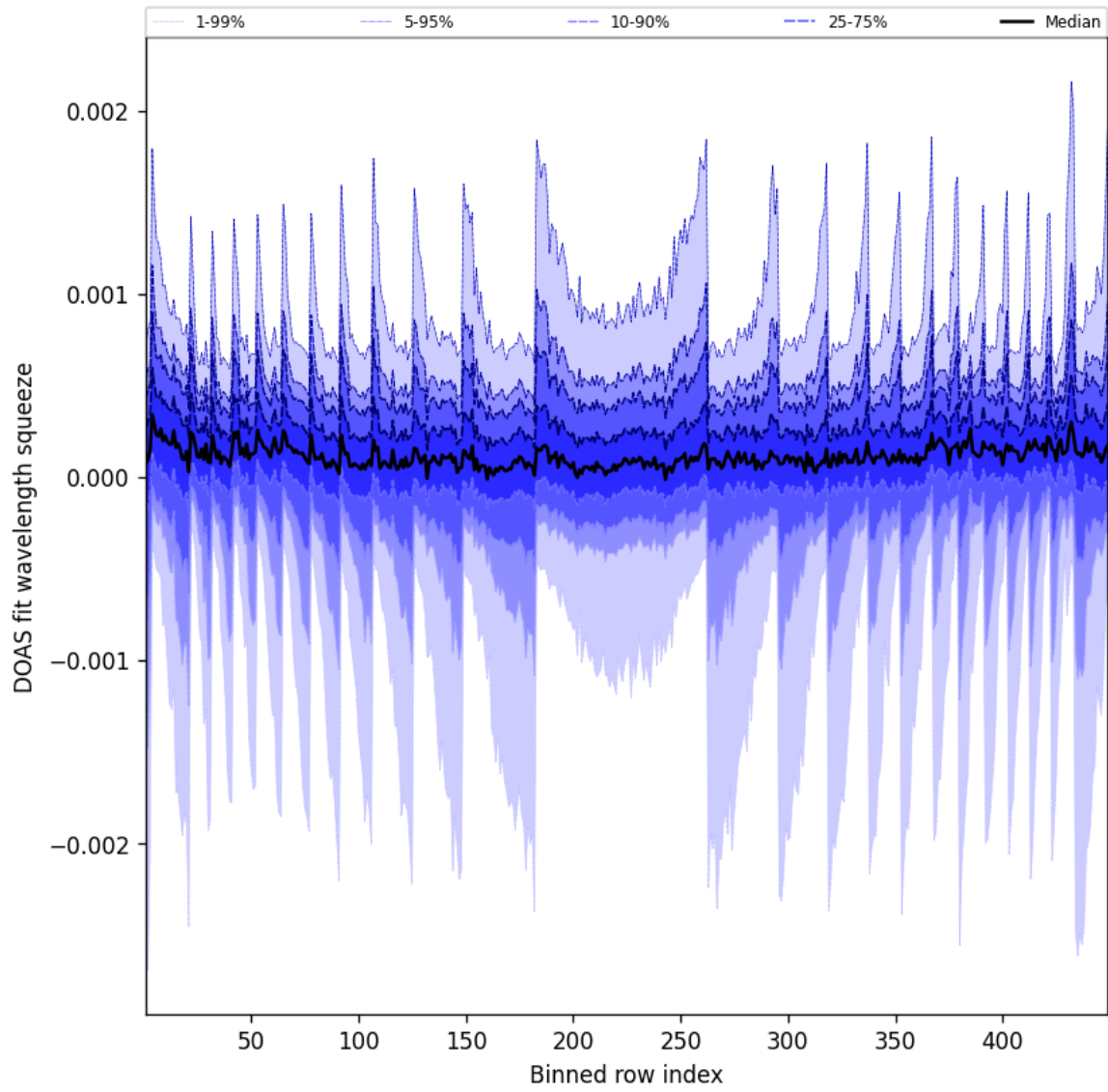
Figure 48: Along track statistics of “DOAS fit wavelength squeeze” for 2025-04-27 to 2025-04-27
