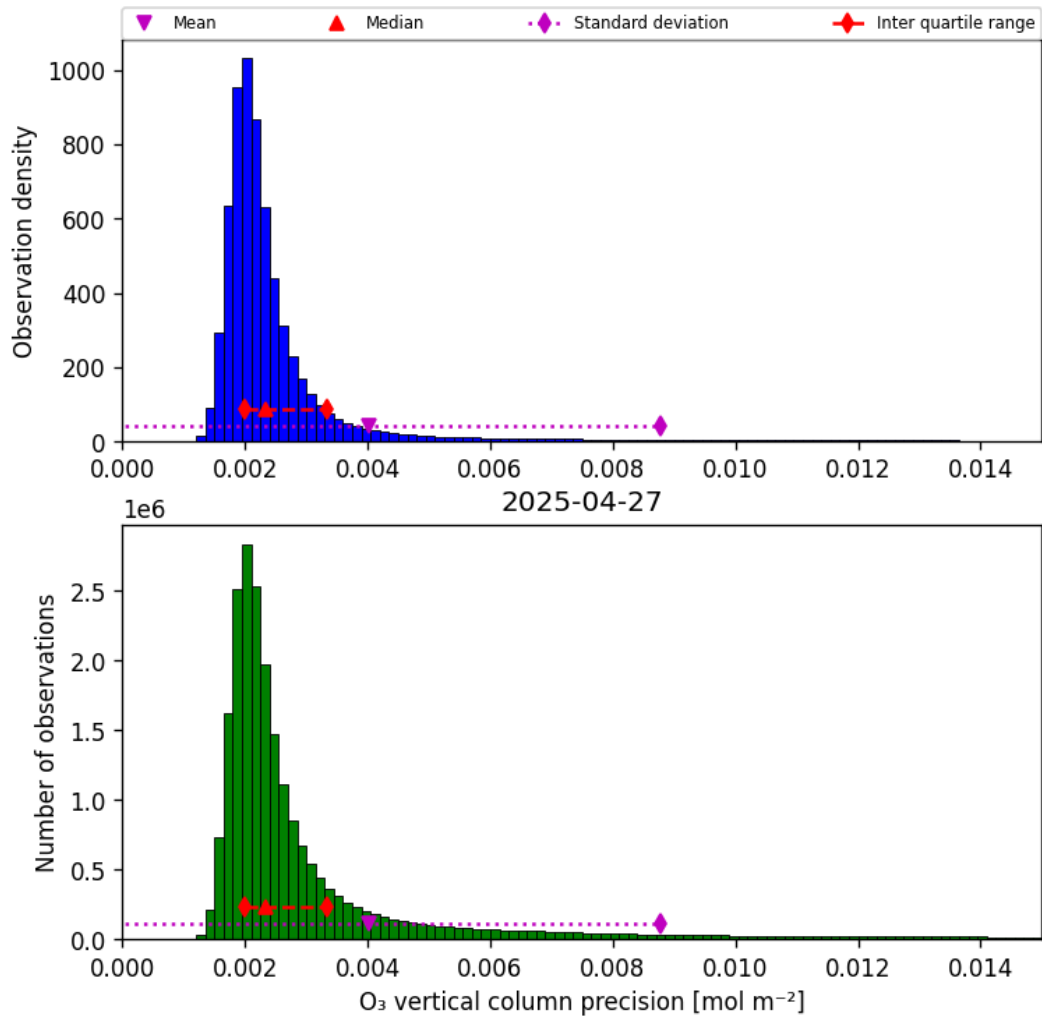
Figure 30: Histogram of “O 3 vertical column precision” for 2025-04-27 to 2025-04-27
