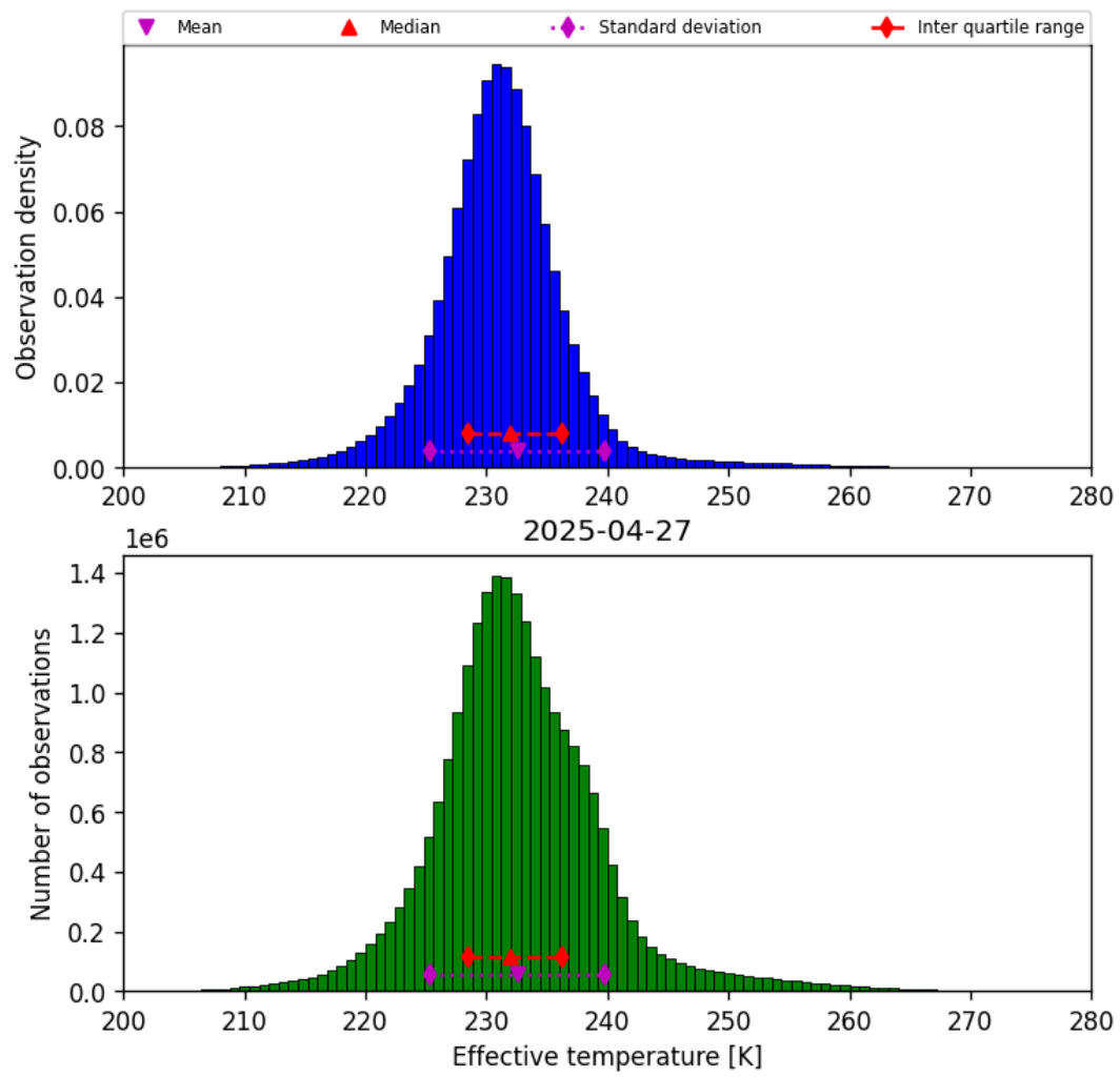
Figure 38: Histogram of “Effective temperature” for 2025-04-27 to 2025-04-27
