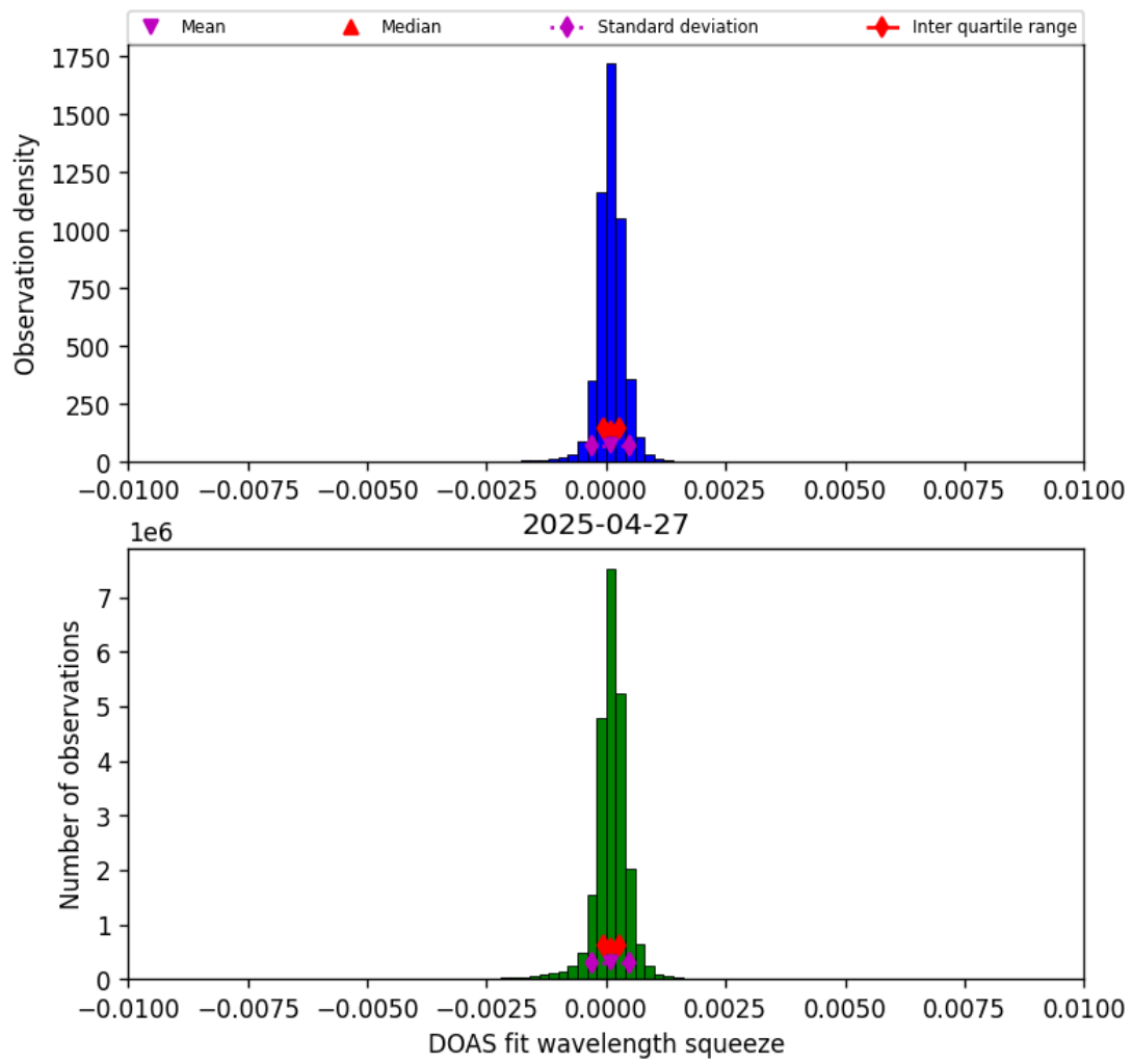
Figure 36: Histogram of “DOAS fit wavelength squeeze” for 2025-04-27 to 2025-04-27
