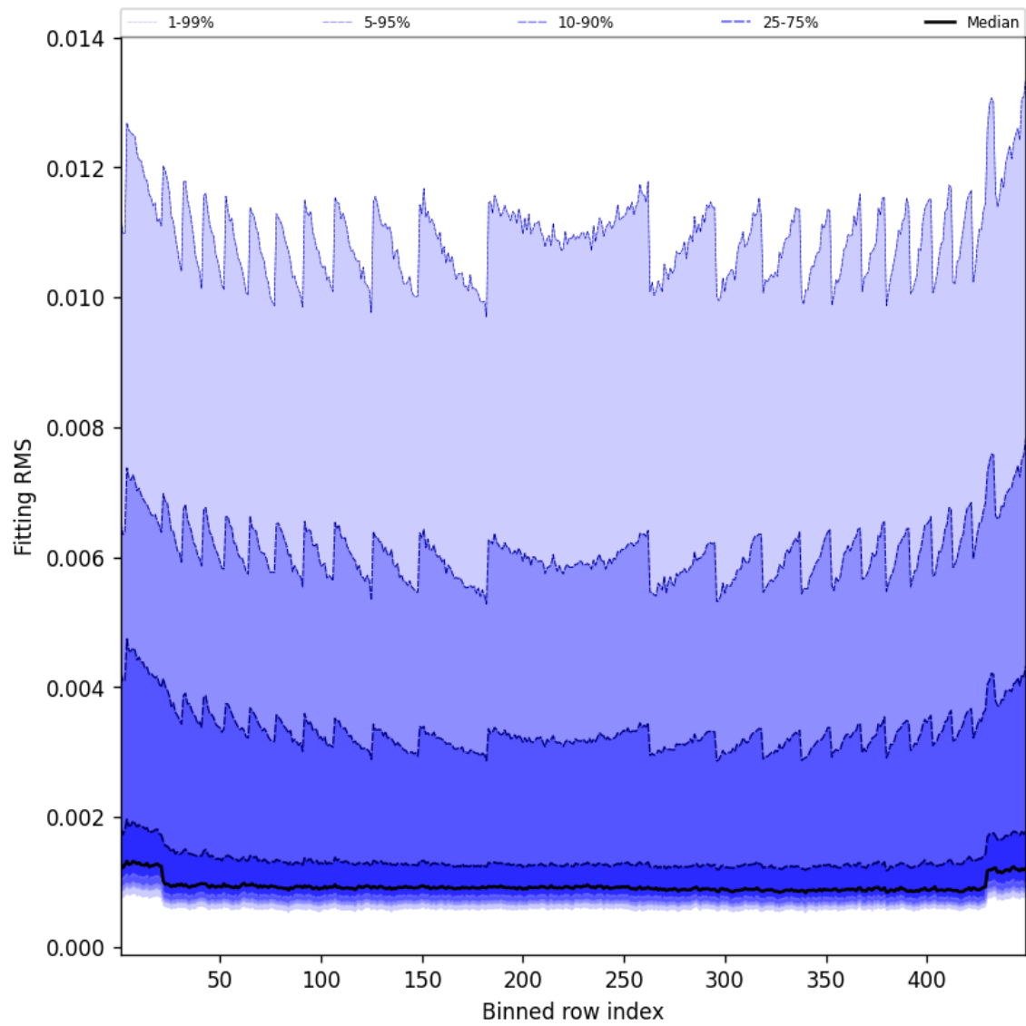
Figure 46: Along track statistics of “Fitting RMS” for 2025-04-27 to 2025-04-27
