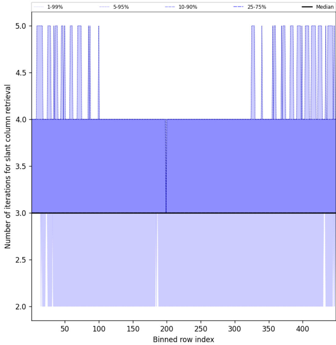
Figure 45: Along track statistics of “Number of iterations for slant column retrieval” for 2025-04-27 to 2025-04-27
