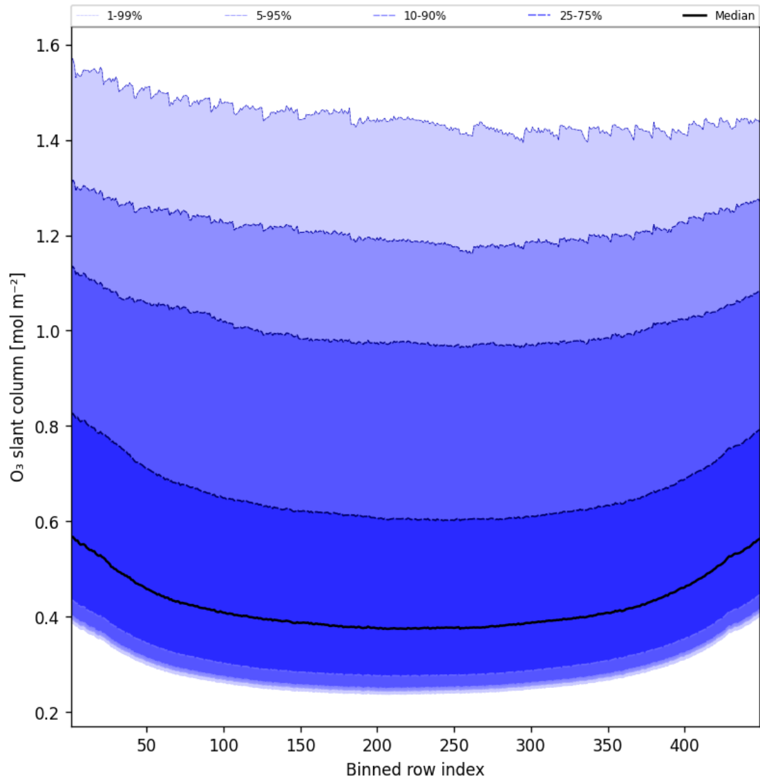
Figure 43: Along track statistics of “O 3 slant column” for 2025-04-27 to 2025-04-27
