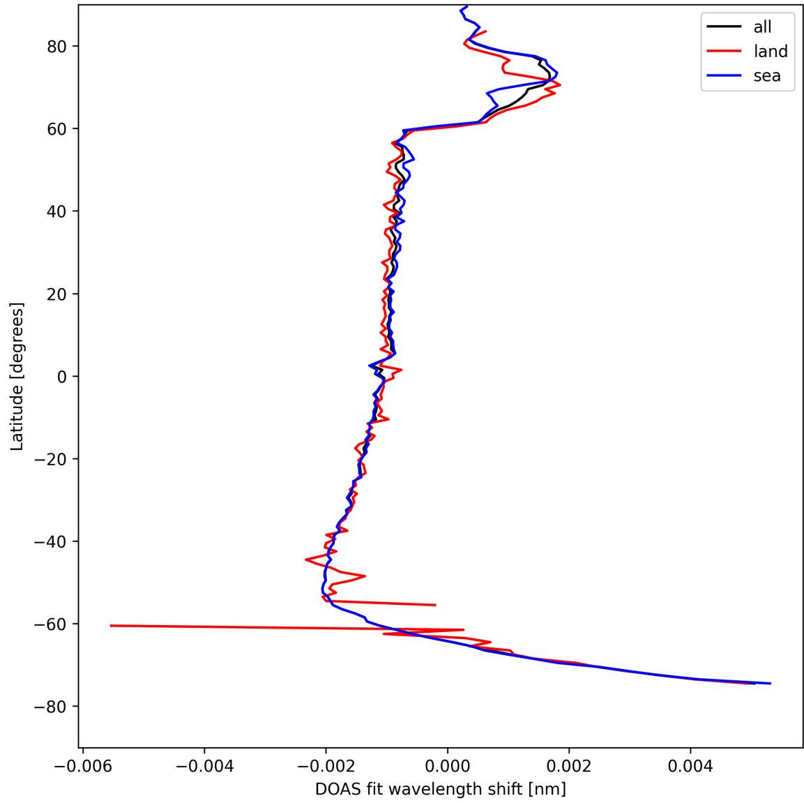
Figure 23: Zonal average of “DOAS fit wavelength shift” for 2025-04-27 to 2025-04-27.
