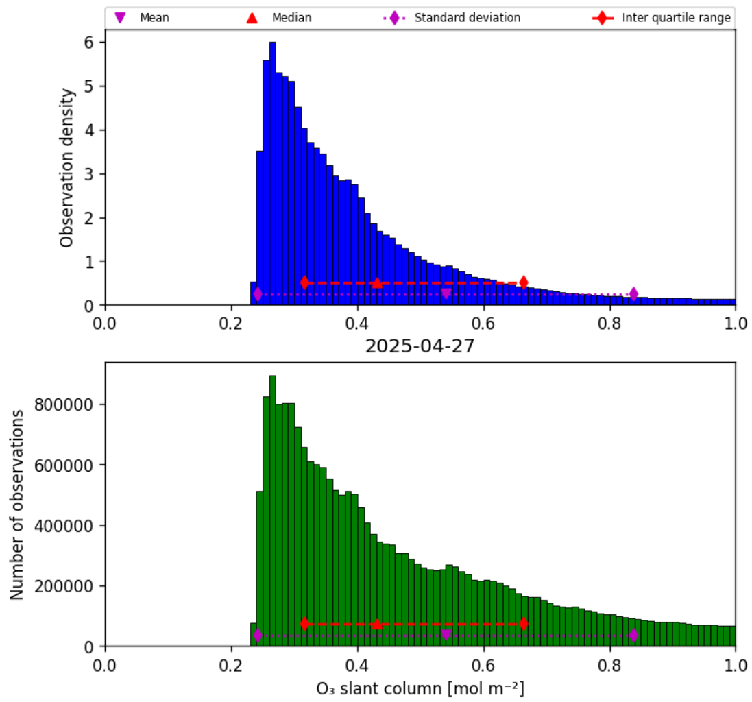
Figure 31: Histogram of “O 3 slant column” for 2025-04-27 to 2025-04-27
