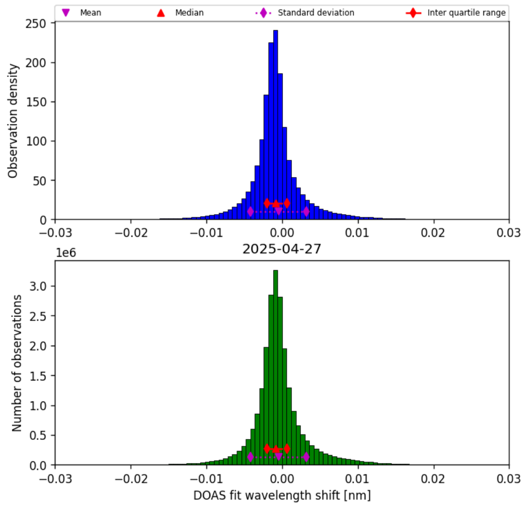
Figure 35: Histogram of “DOAS fit wavelength shift” for 2025-04-27 to 2025-04-27
