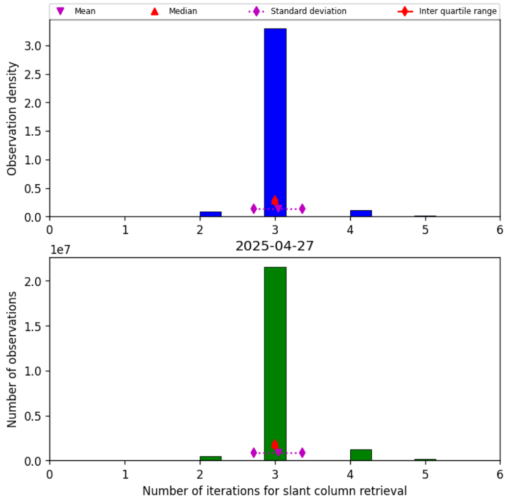
Figure 33: Histogram of "Number of iterations for slant column retrieval" for 2025-04-27 to 2025-04-27
