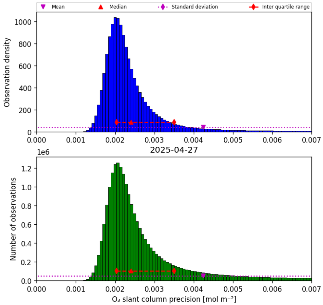
Figure 32: Histogram of “O 3 slant column precision” for 2025-04-27 to 2025-04-27
