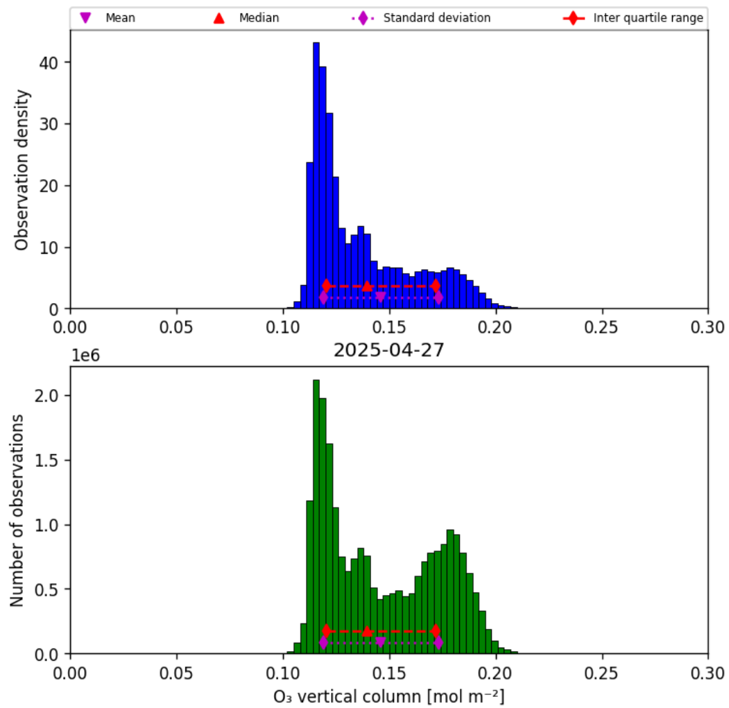
Figure 29: Histogram of “O 3 vertical column” for 2025-04-27 to 2025-04-27
