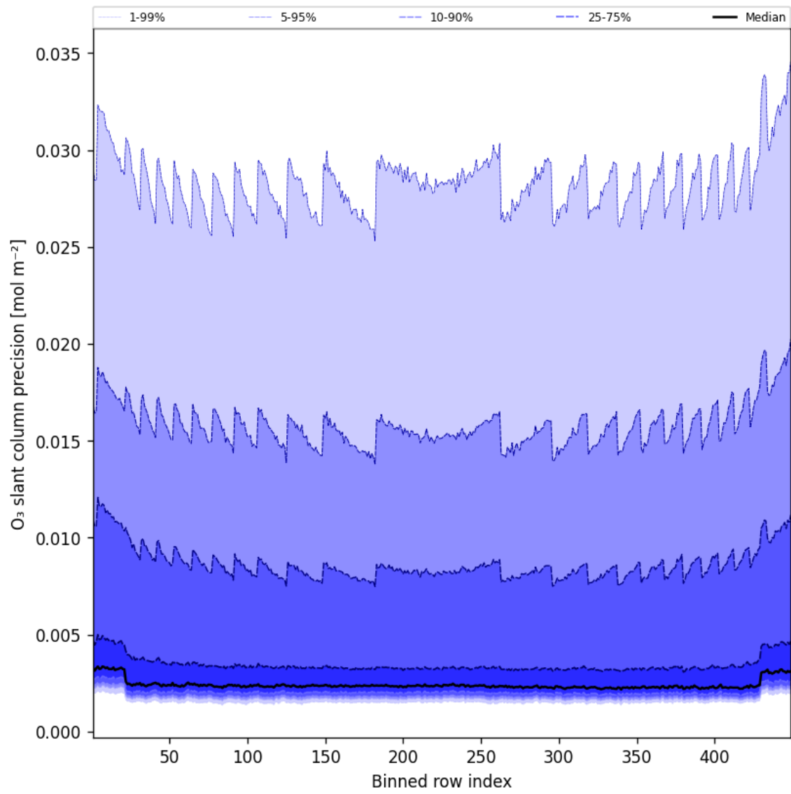
Figure 44: Along track statistics of “O 3 slant column precision” for 2025-04-27 to 2025-04-27
