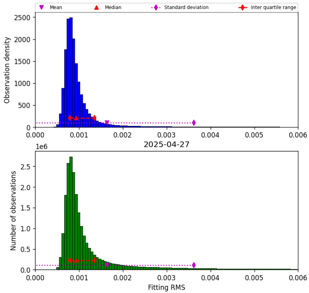
Figure 34: Histogram of “Fitting RMS” for 2025-04-27 to 2025-04-27
