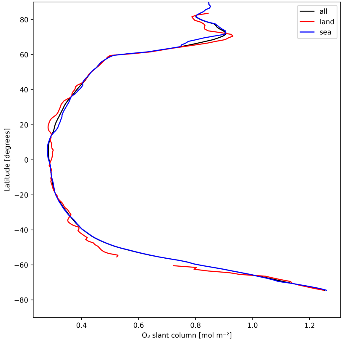
Figure 19: Zonal average of “O 3 slant column” for 2025-04-27 to 2025-04-27.
