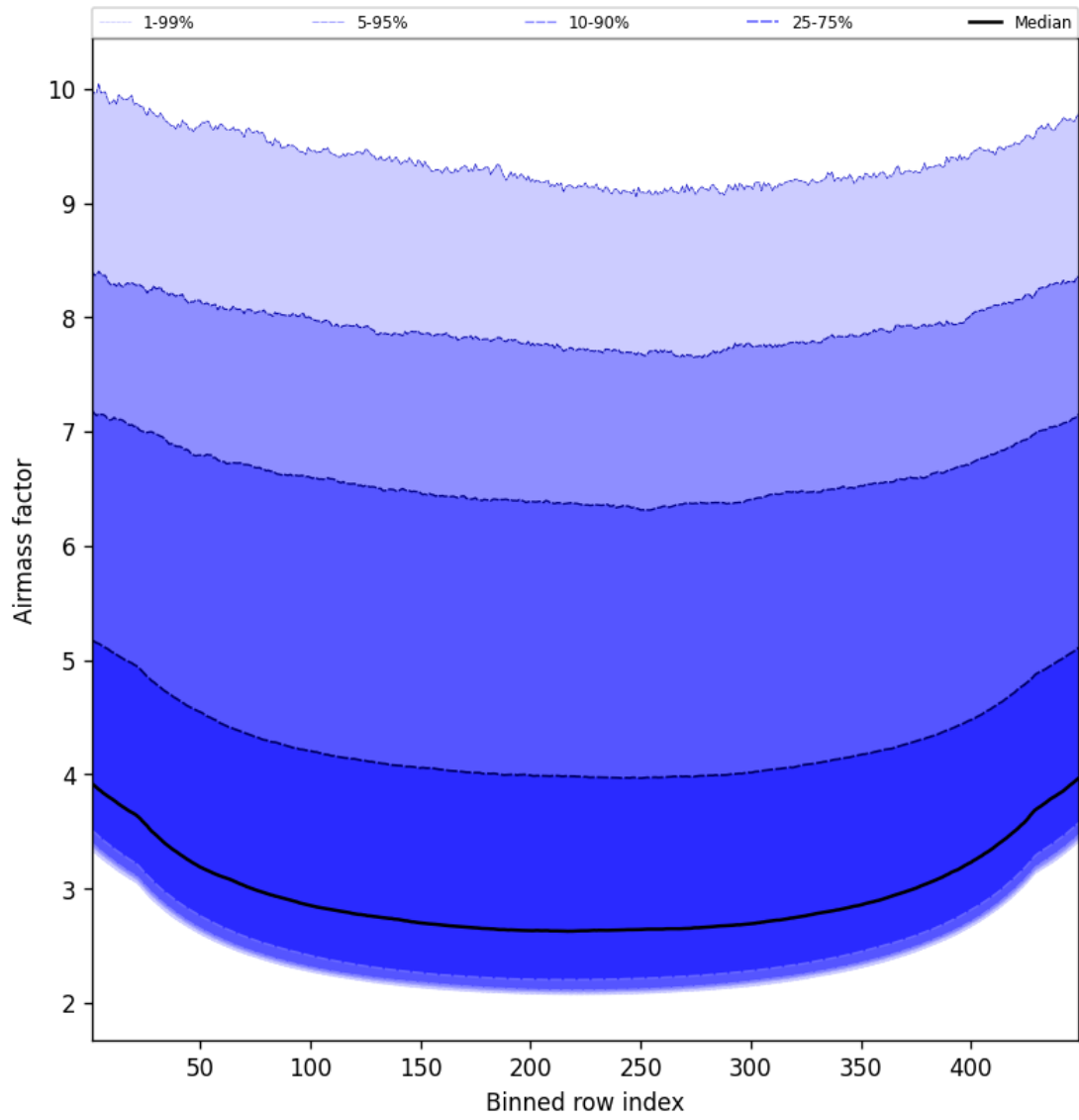
Figure 49: Along track statistics of “Airmass factor” for 2025-04-27 to 2025-04-27
