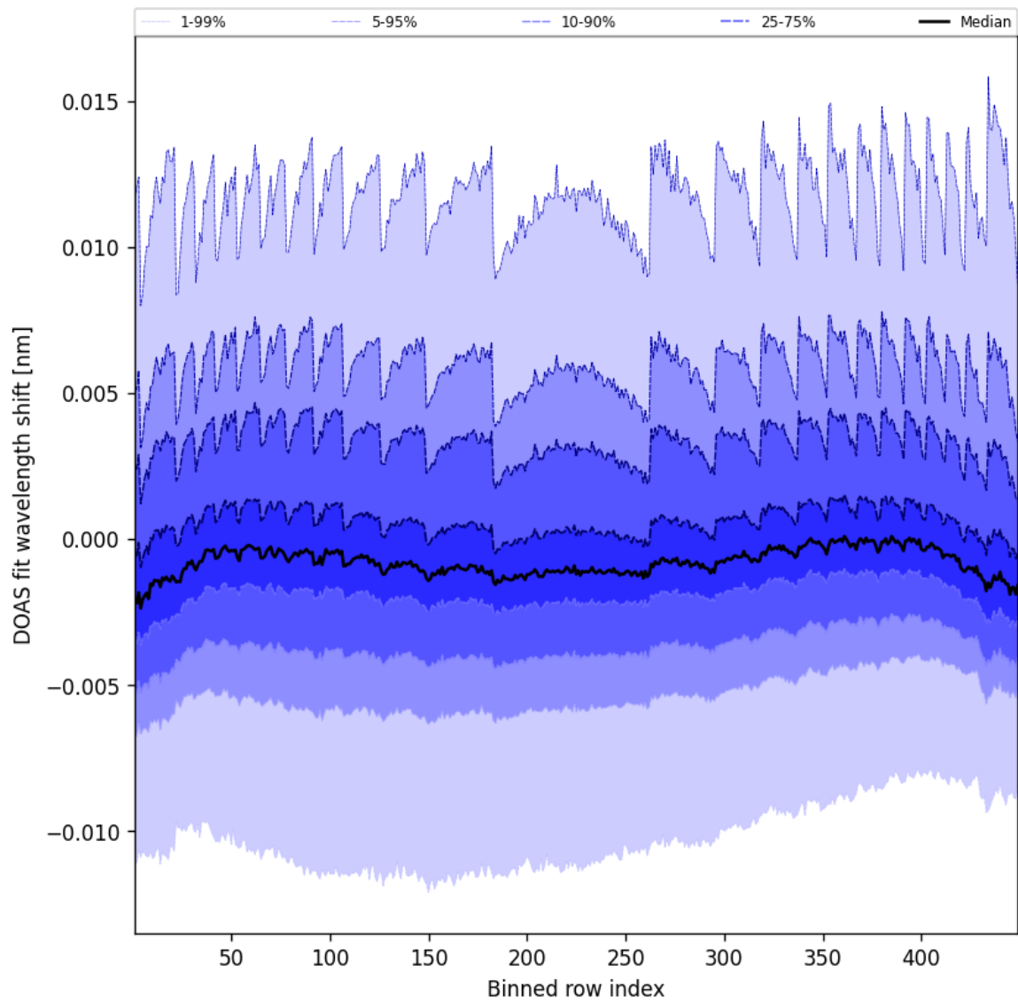
Figure 47: Along track statistics of "DOAS fit wavelength shift" for 2025-04-27 to 2025-04-27
