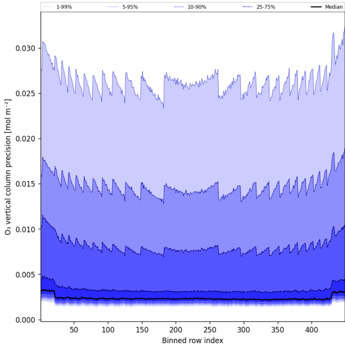
Figure 42: Along track statistics of “O 3 vertical column precision” for 2025-04-27 to 2025-04-27
