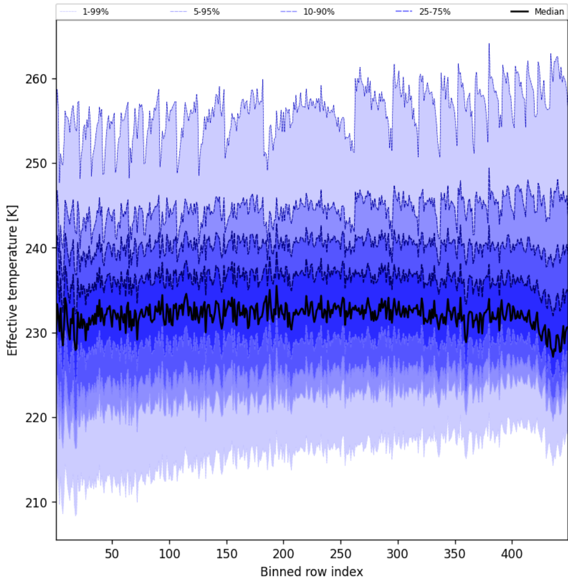
Figure 50: Along track statistics of “Effective temperature” for 2025-04-27 to 2025-04-27
