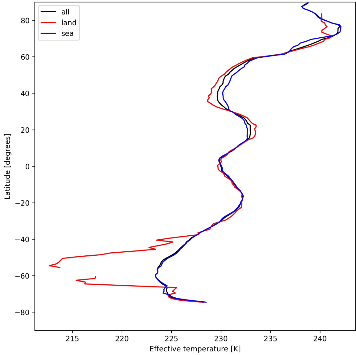
Figure 26: Zonal average of "Effective temperature" for 2025-04-27 to 2025-04-27.
