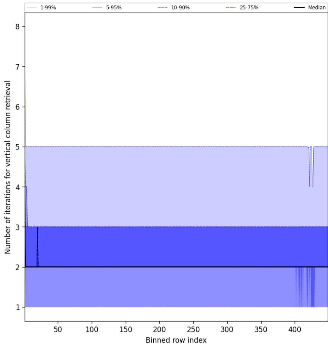
Figure 51: Along track statistics of “Number of iterations for vertical column retrieval” for 2025-04-27 to 2025-04-27
