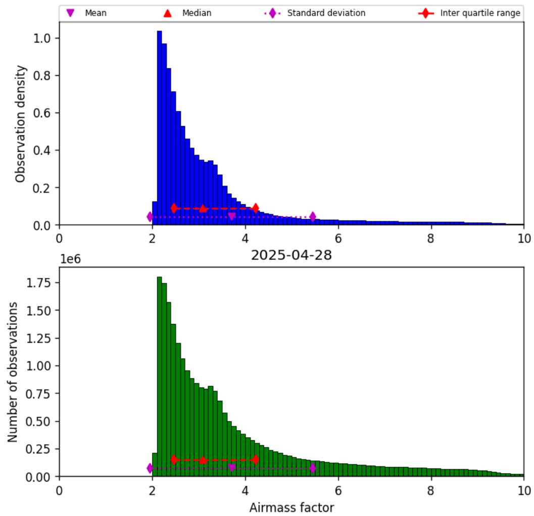
Figure 37: Histogram of “Airmass factor” for 2025-04-28 to 2025-04-29
