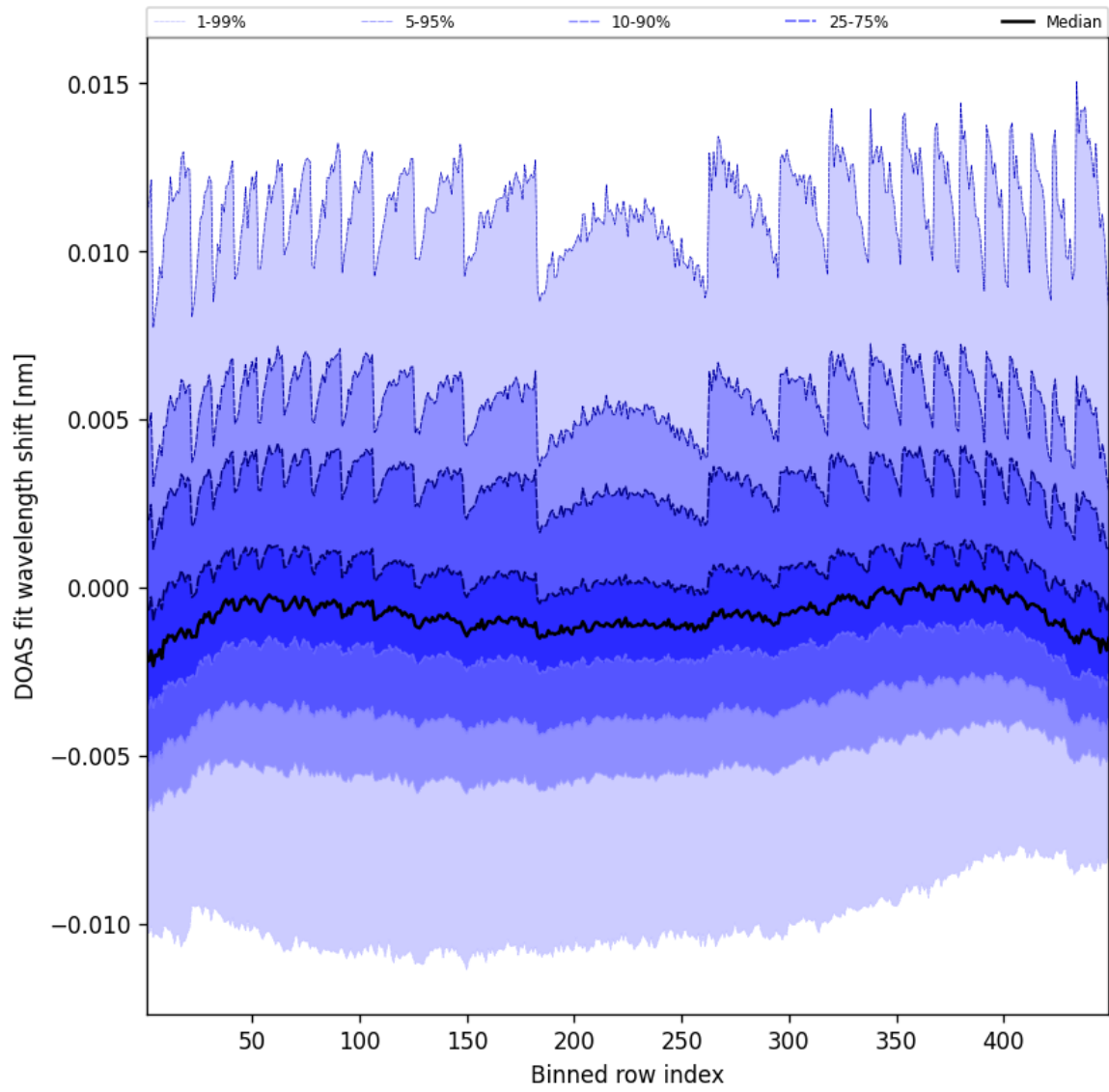
Figure 47: Along track statistics of “DOAS fit wavelength shift” for 2025-04-28 to 2025-04-29
