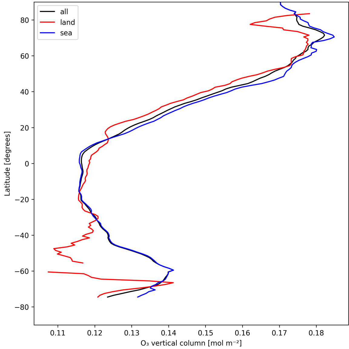
Figure 17: Zonal average of “O 3 vertical column” for 2025-04-28 to 2025-04-29.
