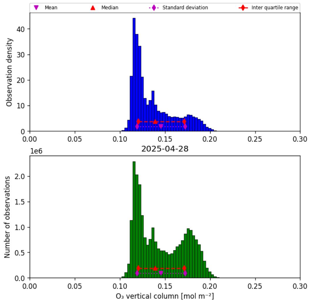
Figure 29: Histogram of “O 3 vertical column” for 2025-04-28 to 2025-04-29
