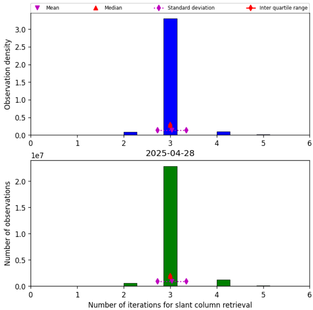
Figure 33: Histogram of “Number of iterations for slant column retrieval” for 2025-04-28 to 2025-04-29
