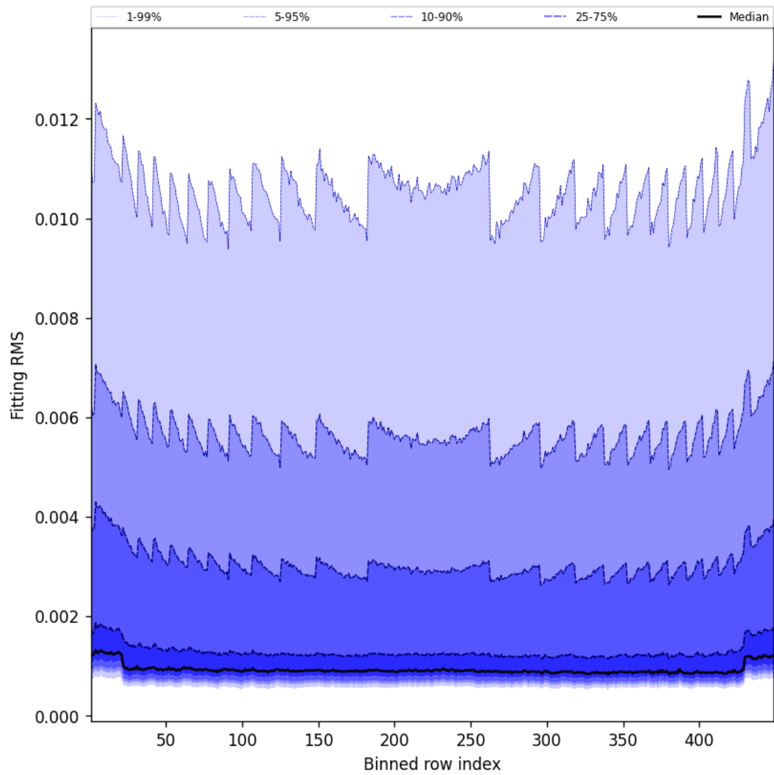
Figure 46: Along track statistics of “Fitting RMS” for 2025-04-28 to 2025-04-29
