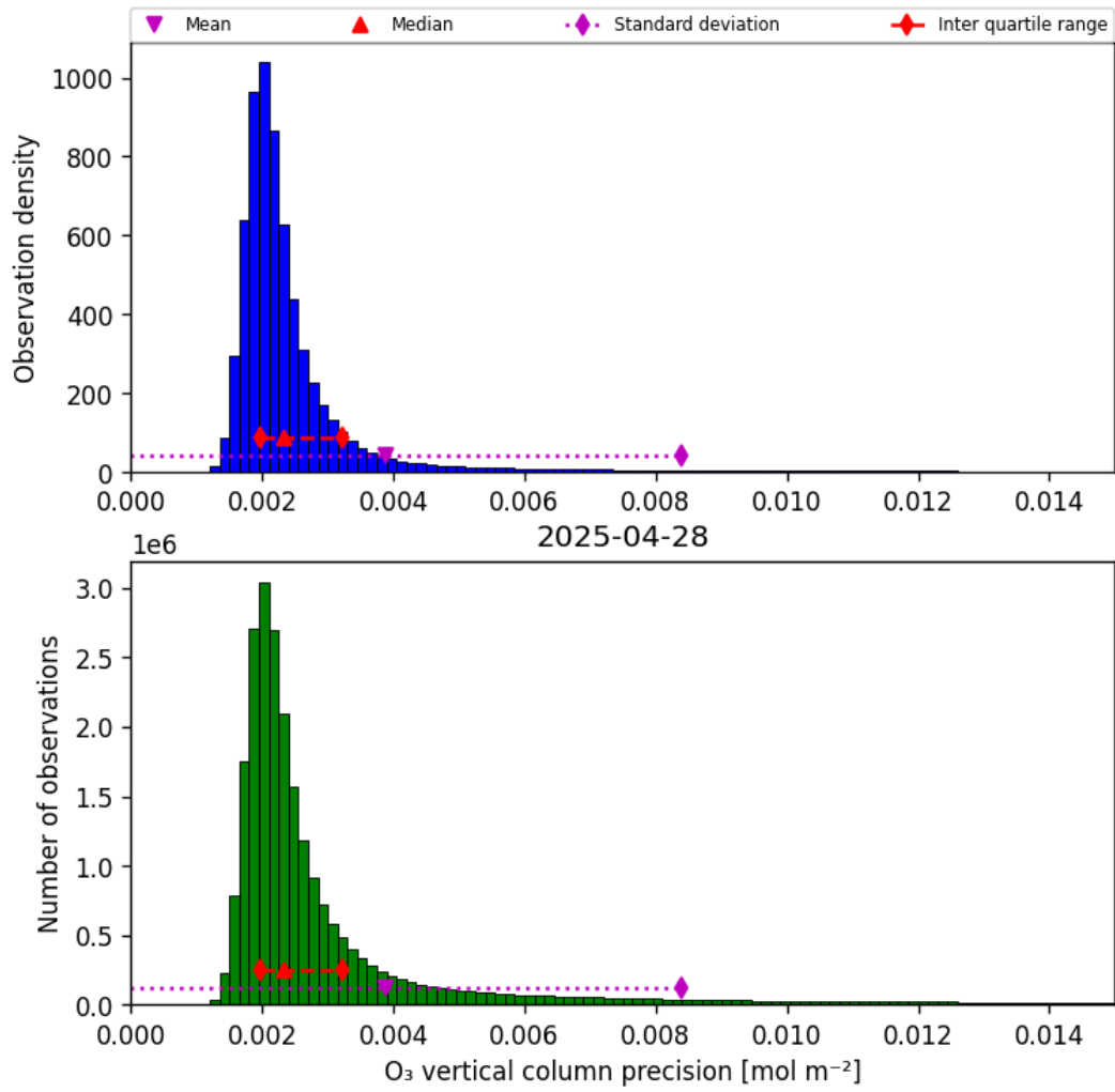
Figure 30: Histogram of “O 3 vertical column precision” for 2025-04-28 to 2025-04-29
