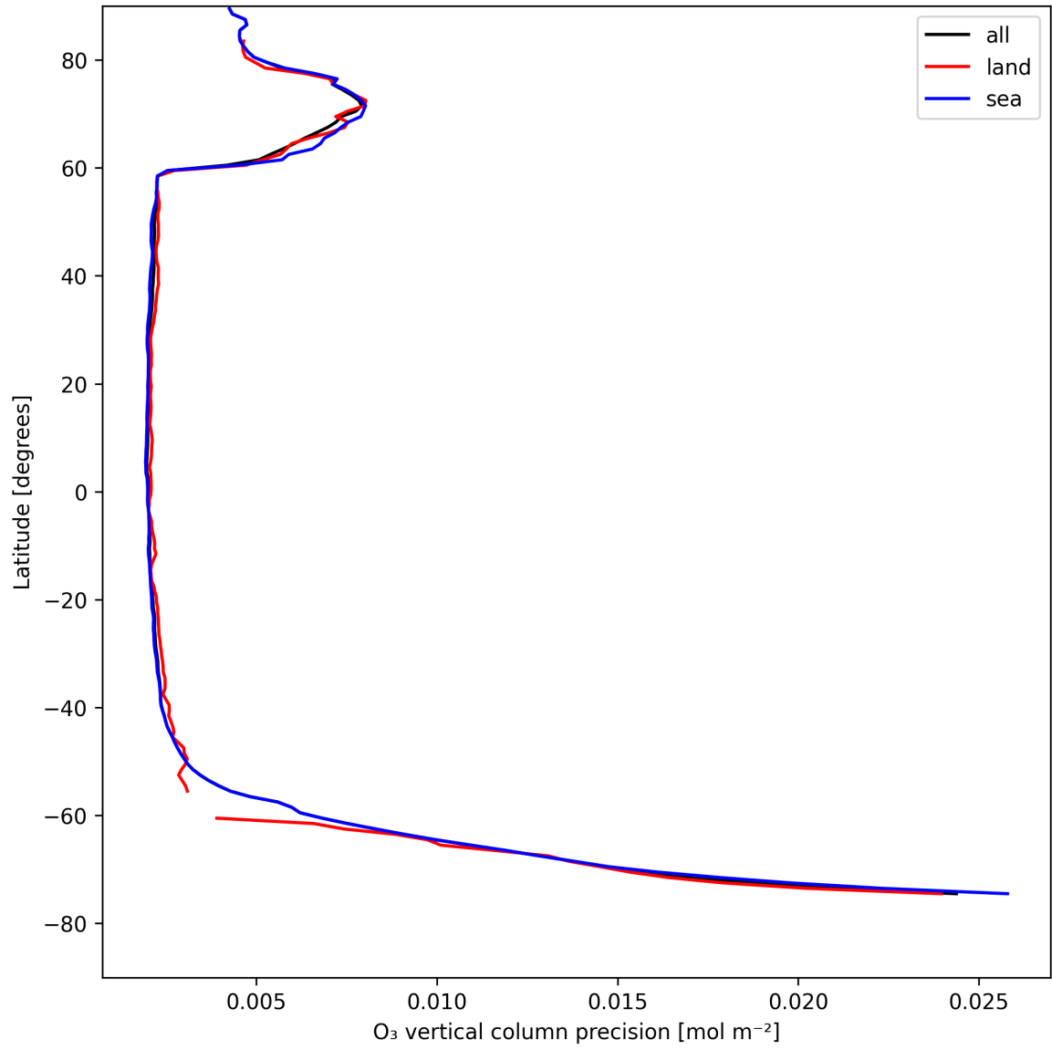
Figure 18: Zonal average of “O 3 vertical column precision” for 2025-04-28 to 2025-04-29.
