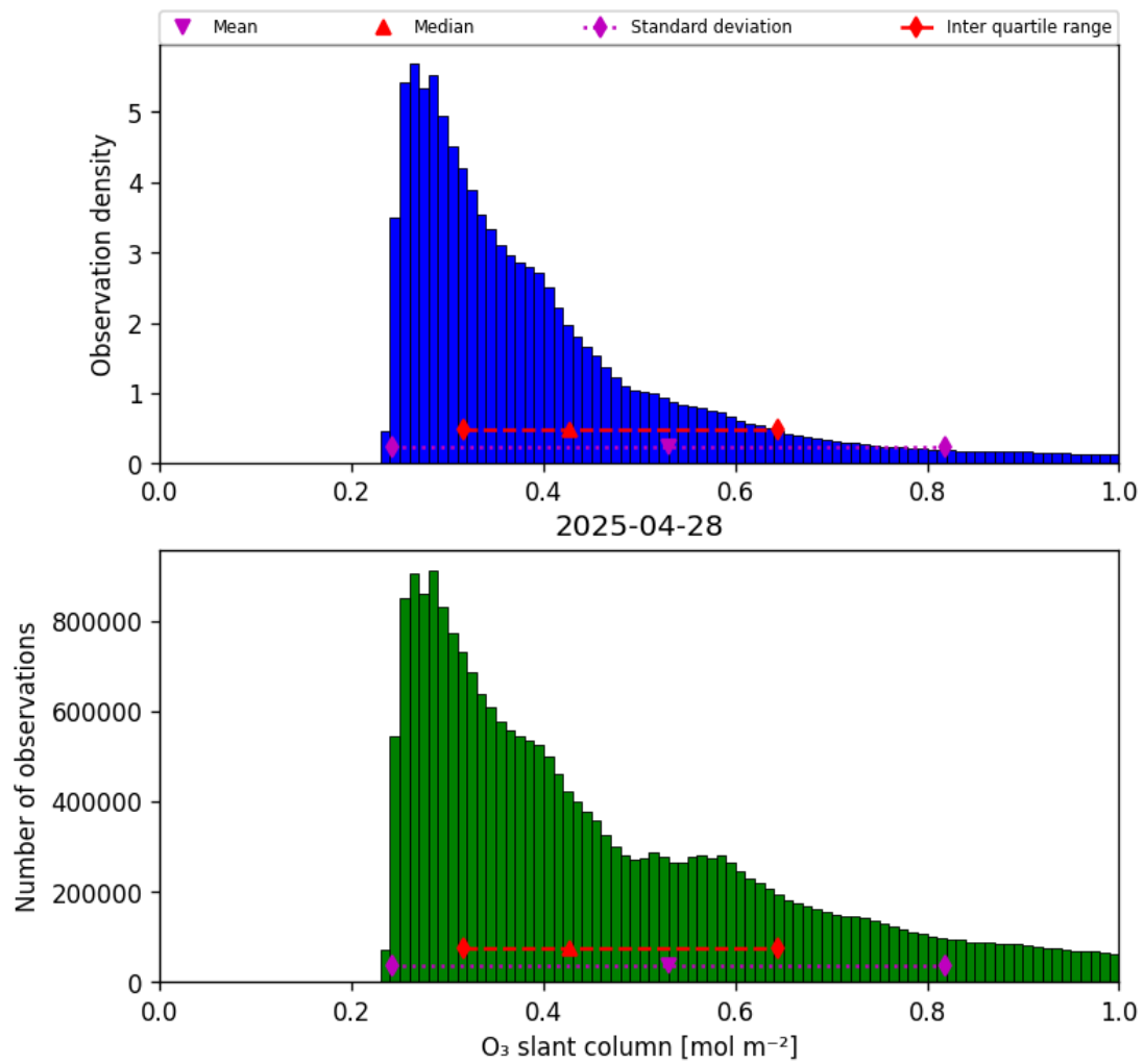
Figure 31: Histogram of “O 3 slant column” for 2025-04-28 to 2025-04-29
