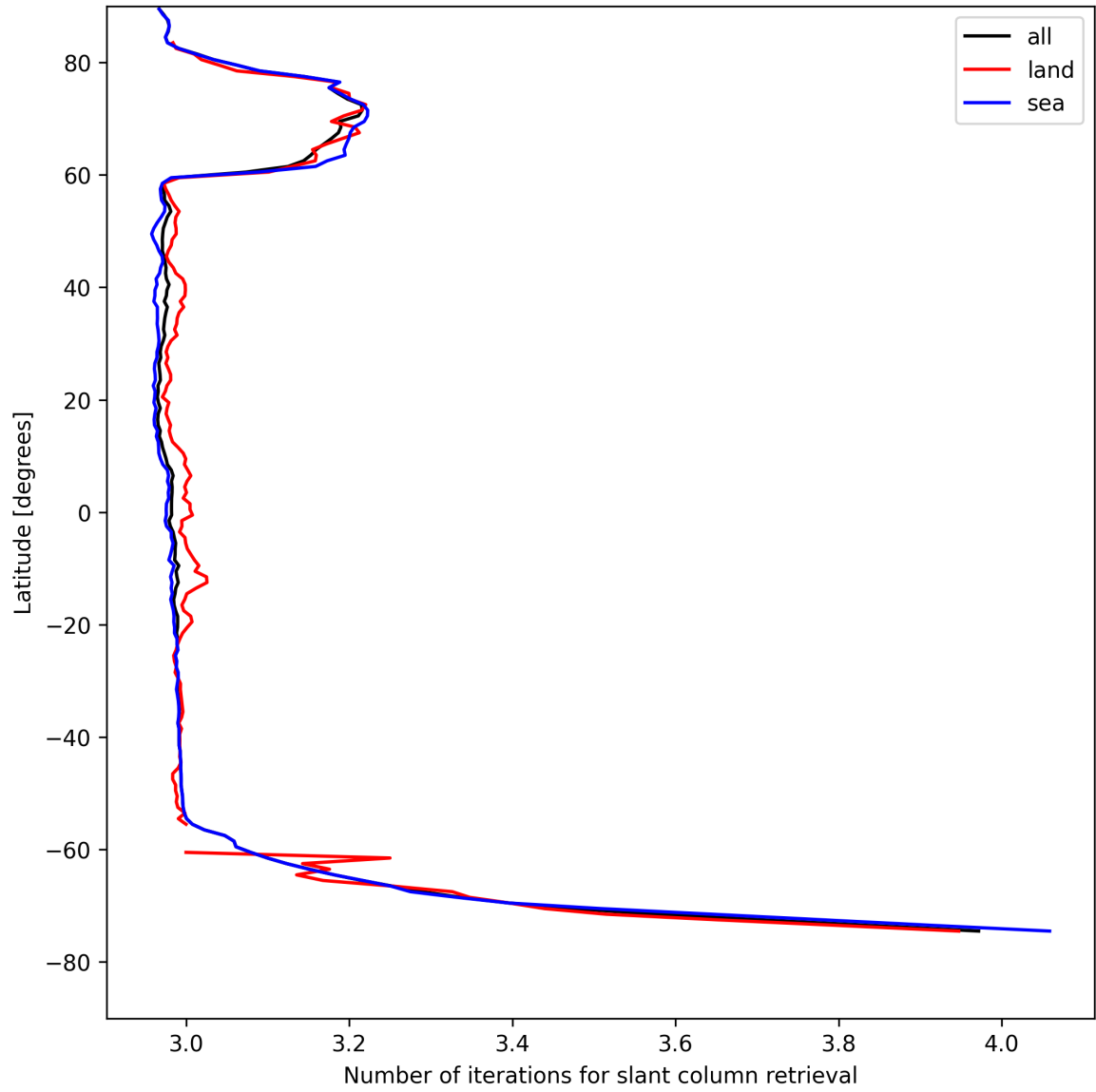
Figure 21: Zonal average of “Number of iterations for slant column retrieval” for 2025-04-28 to 2025-04-29.
