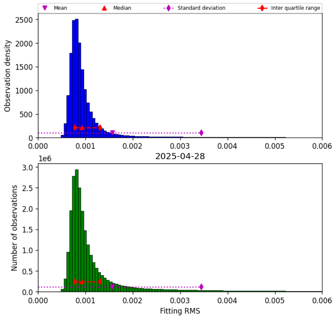
Figure 34: Histogram of “Fitting RMS” for 2025-04-28 to 2025-04-29
