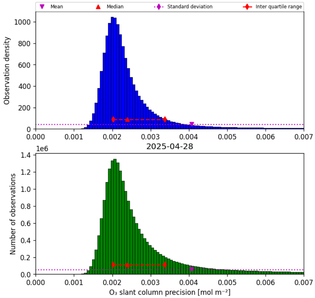
Figure 32: Histogram of “O 3 slant column precision” for 2025-04-28 to 2025-04-29
