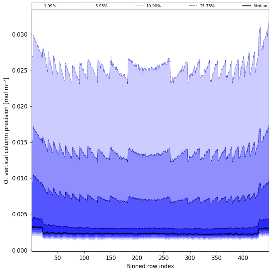
Figure 42: Along track statistics of “O 3 vertical column precision” for 2025-04-28 to 2025-04-29
