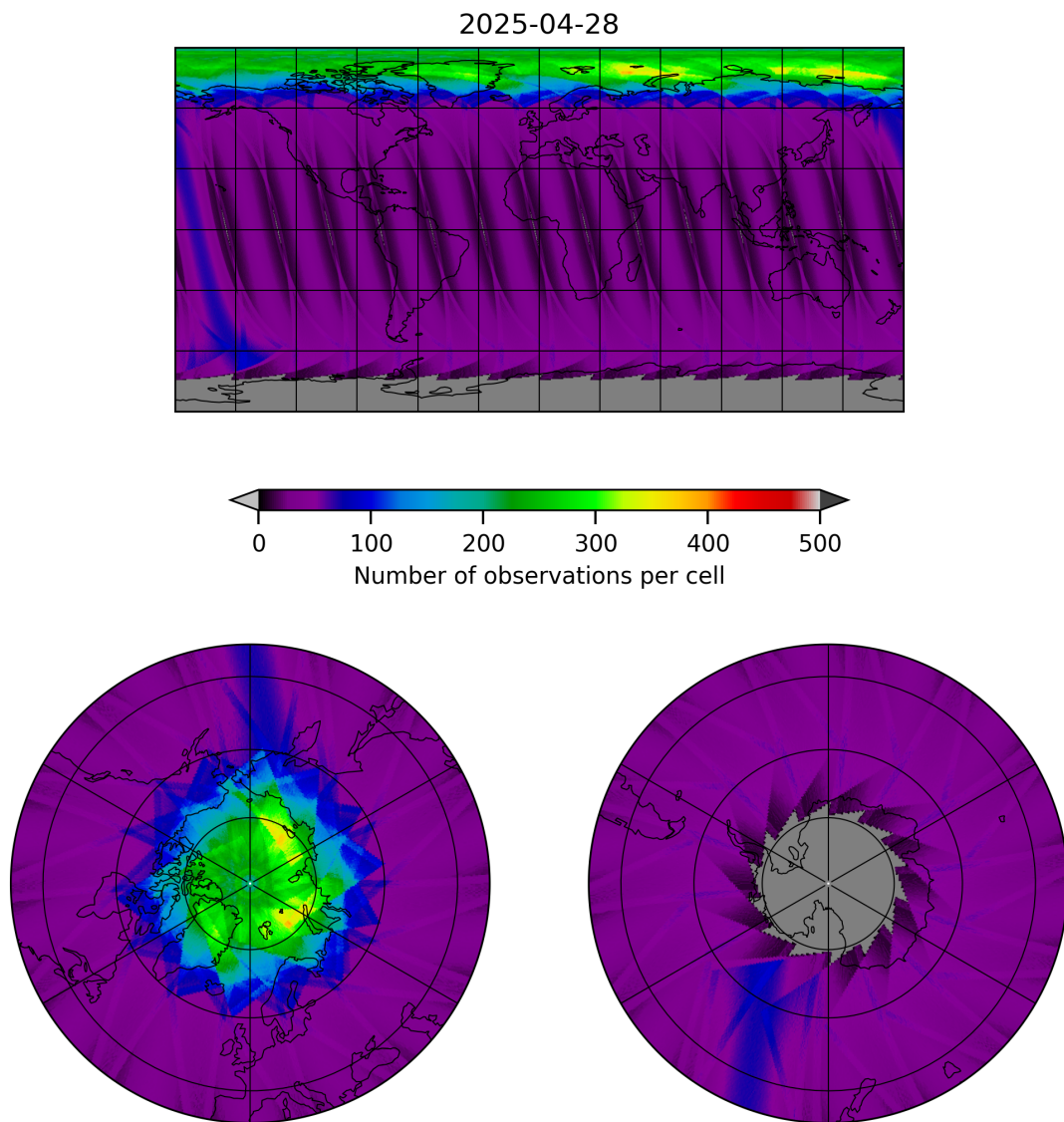
Figure 15: Map of the number of observations for 2025-04-28 to 2025-04-29
