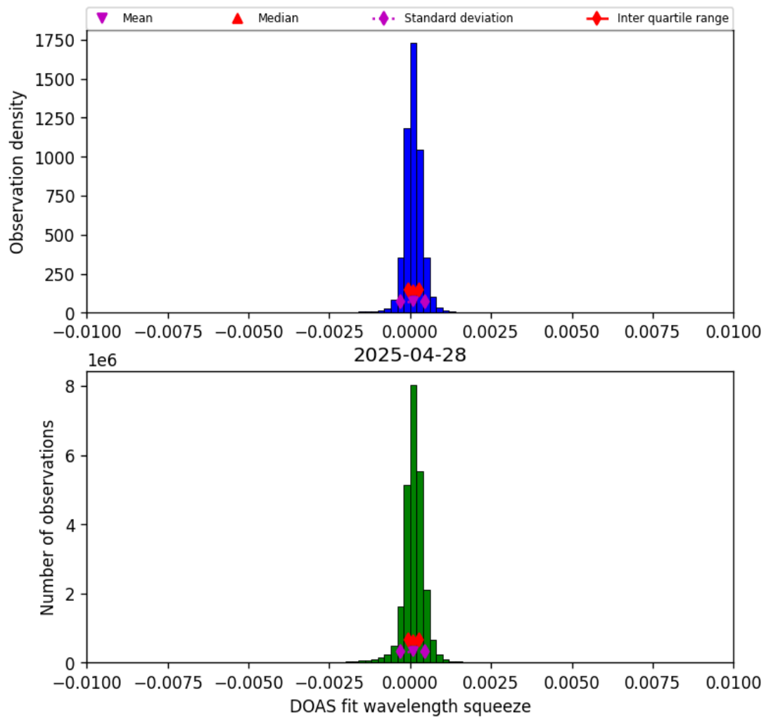
Figure 36: Histogram of “DOAS fit wavelength squeeze” for 2025-04-28 to 2025-04-29
