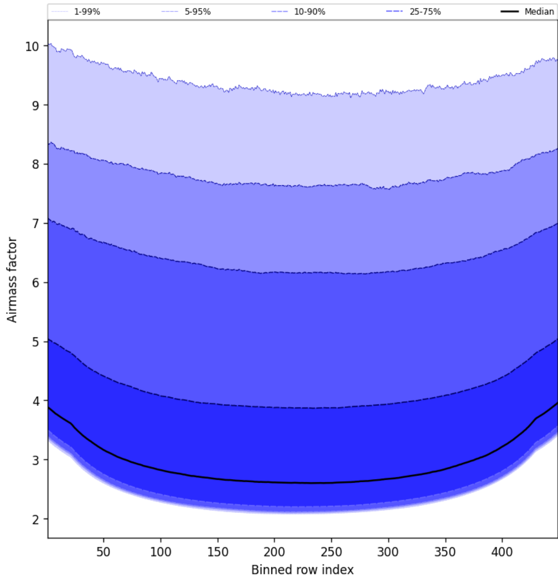
Figure 49: Along track statistics of “Airmass factor” for 2025-04-28 to 2025-04-29
