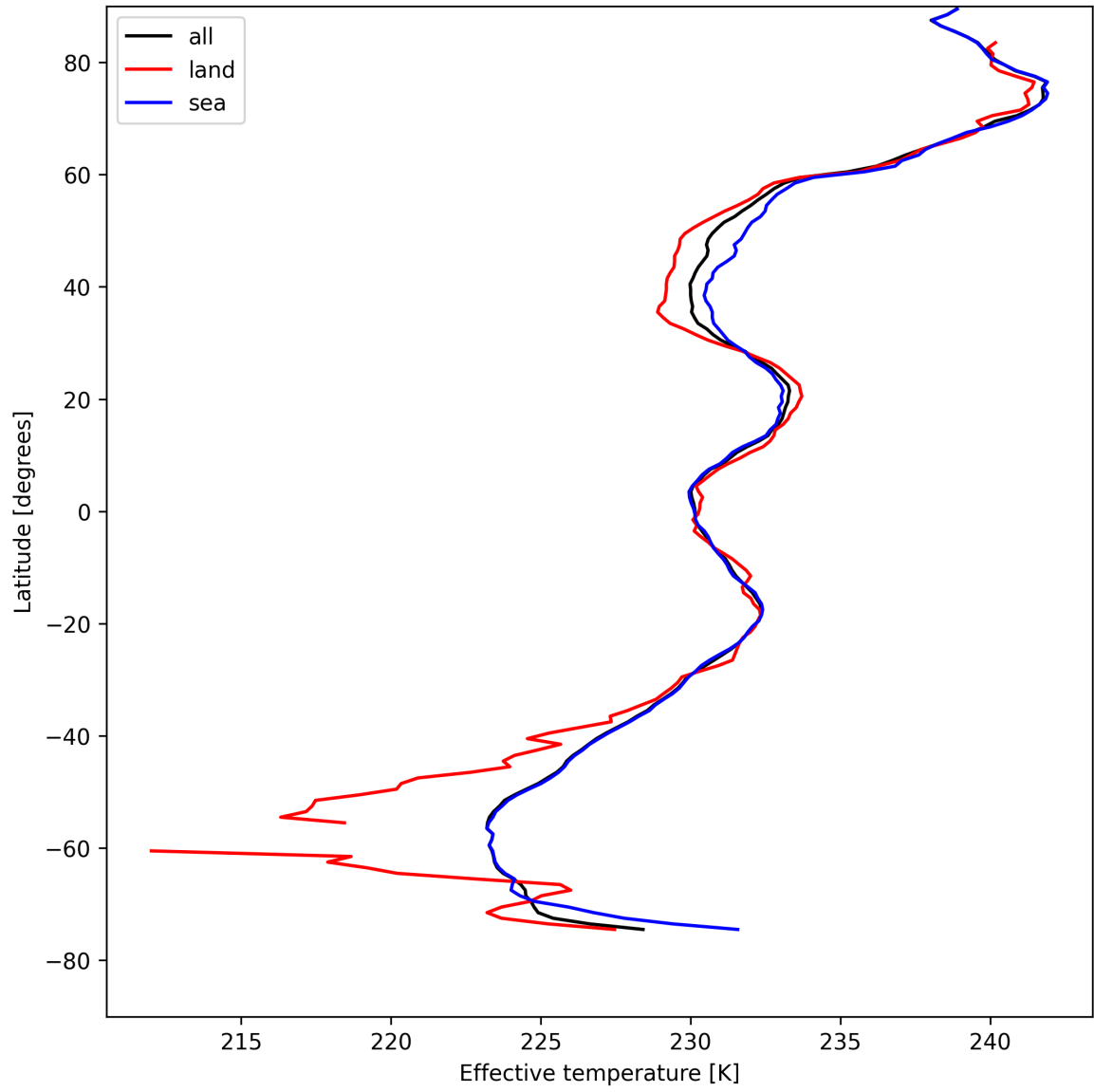
Figure 26: Zonal average of "Effective temperature" for 2025-04-28 to 2025-04-29.
