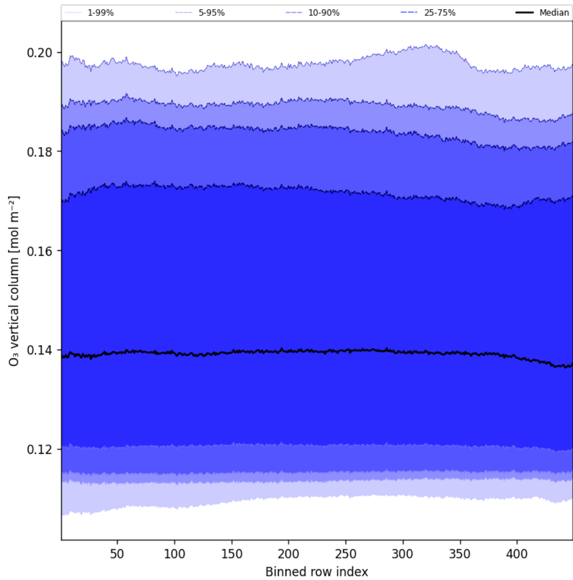
Figure 41: Along track statistics of “O 3 vertical column” for 2025-04-28 to 2025-04-29
