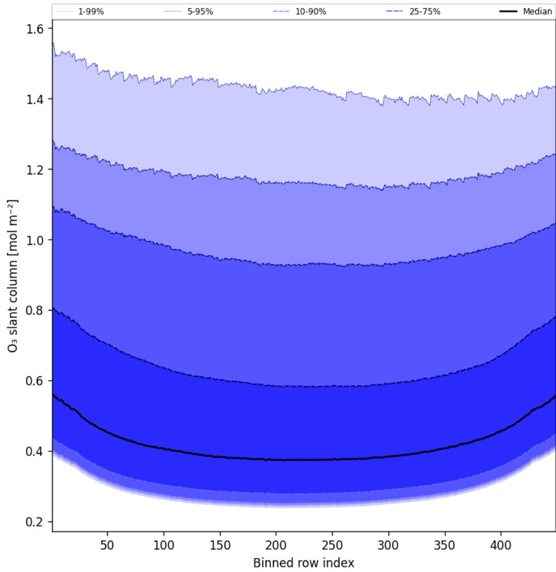
Figure 43: Along track statistics of “O 3 slant column” for 2025-04-28 to 2025-04-29
