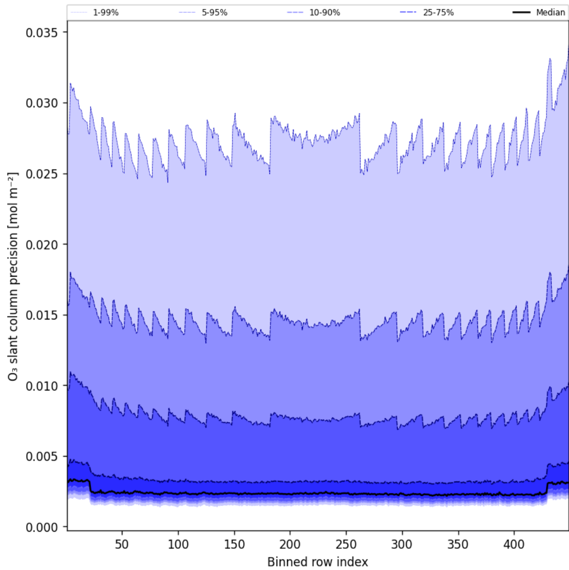
Figure 44: Along track statistics of “O 3 slant column precision” for 2025-04-28 to 2025-04-29
