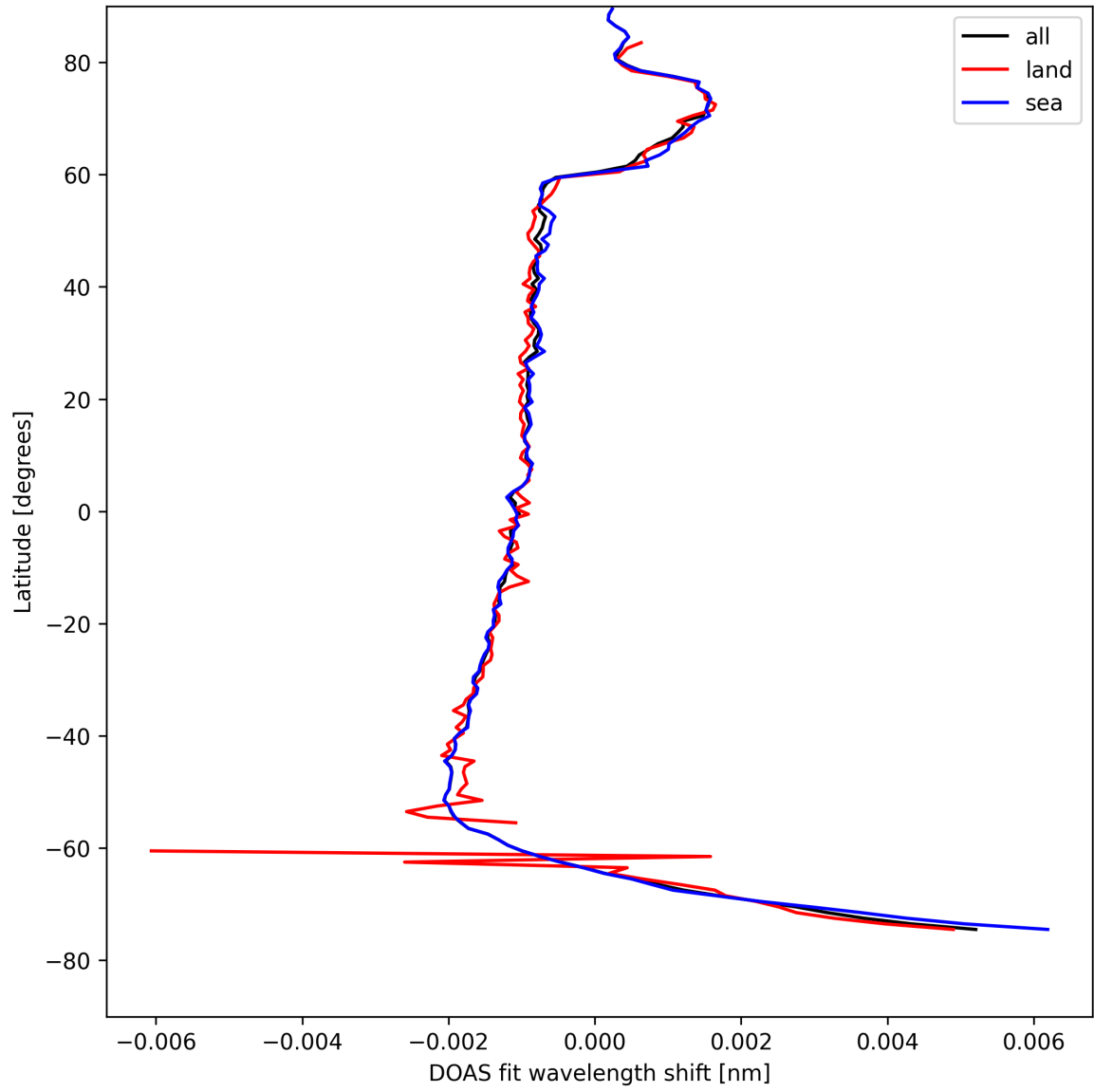
Figure 23: Zonal average of “DOAS fit wavelength shift” for 2025-04-28 to 2025-04-29.
