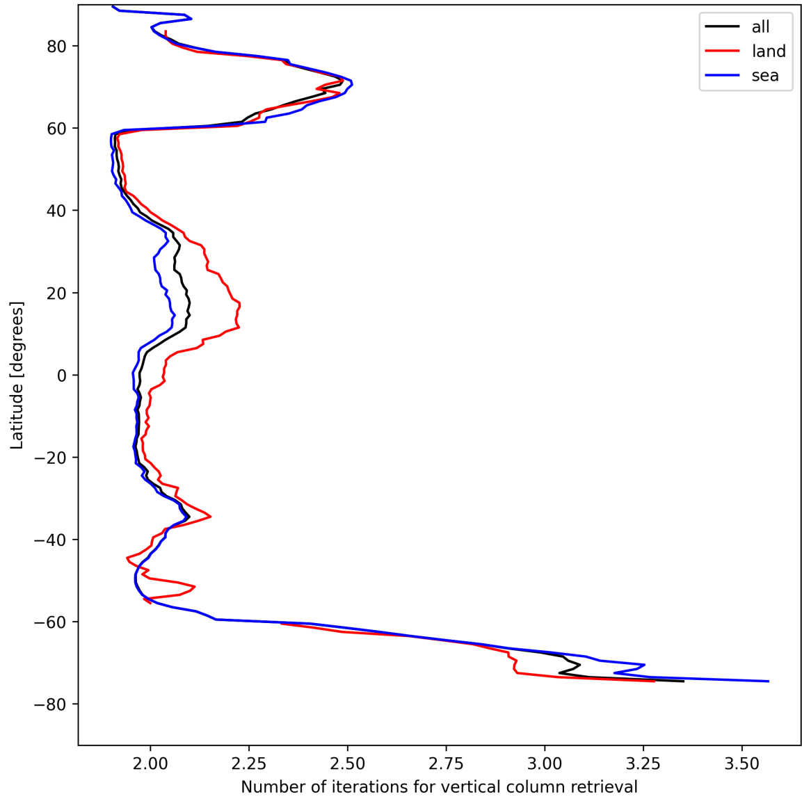
Figure 27: Zonal average of “Number of iterations for vertical column retrieval” for 2025-04-28 to 2025-04-29.
