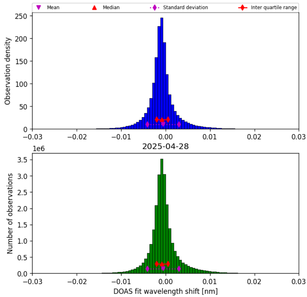
Figure 35: Histogram of “DOAS fit wavelength shift” for 2025-04-28 to 2025-04-29
