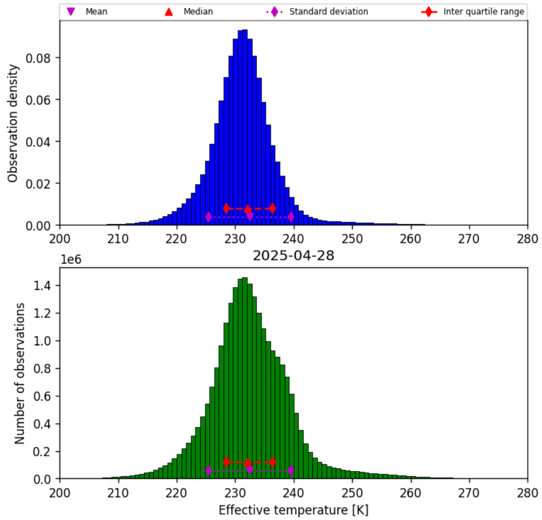
Figure 38: Histogram of “Effective temperature” for 2025-04-28 to 2025-04-29
