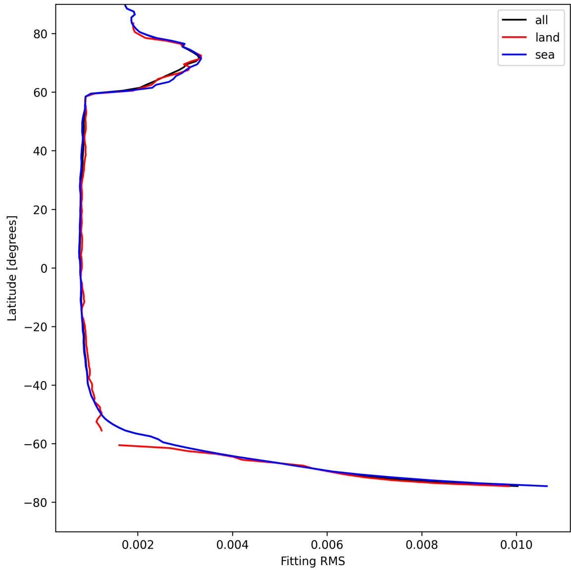
Figure 22: Zonal average of “Fitting RMS” for 2025-04-28 to 2025-04-29.
