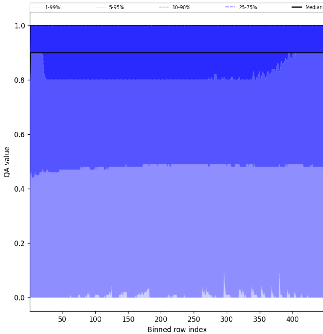
Figure 40: Along track statistics of “QA value” for 2025-04-28 to 2025-04-29
