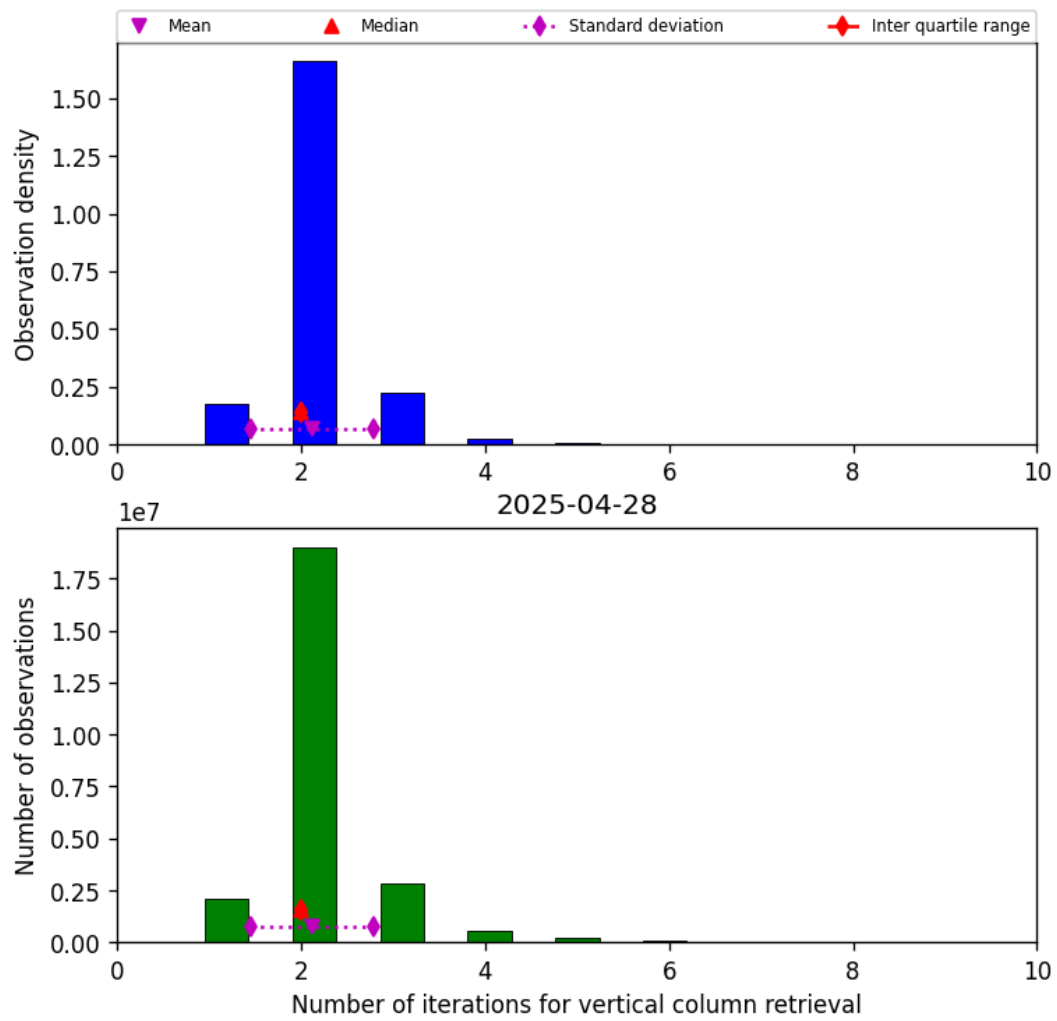
Figure 39: Histogram of “Number of iterations for vertical column retrieval” for 2025-04-28 to 2025-04-29
