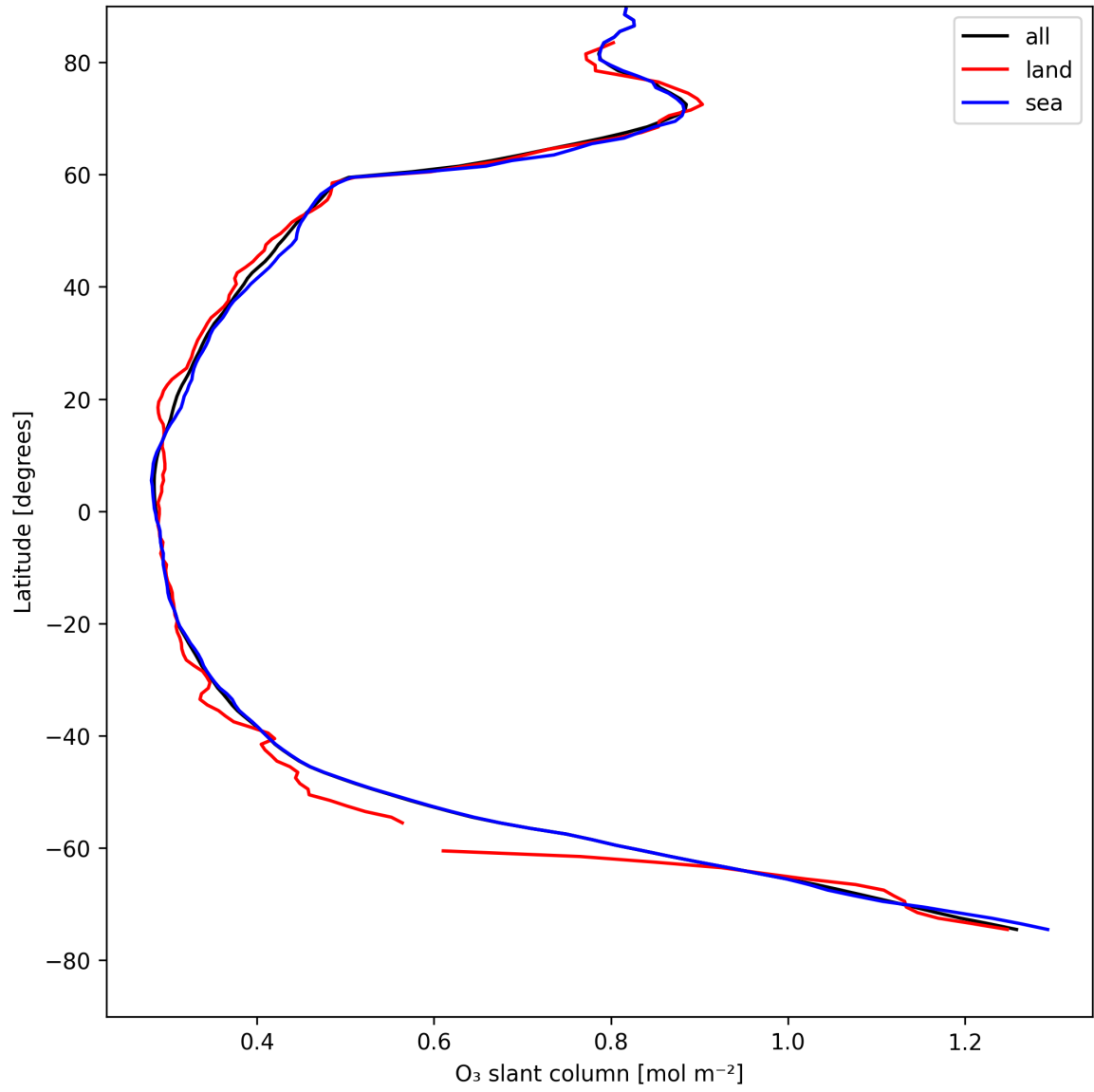
Figure 19: Zonal average of “O 3 slant column” for 2025-04-28 to 2025-04-29.
