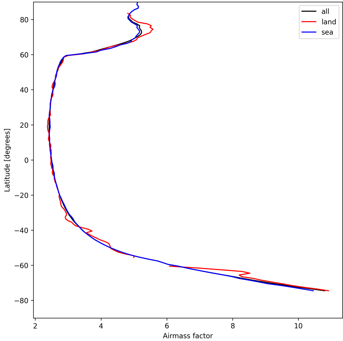
Figure 25: Zonal average of “Airmass factor” for 2025-04-28 to 2025-04-29.
