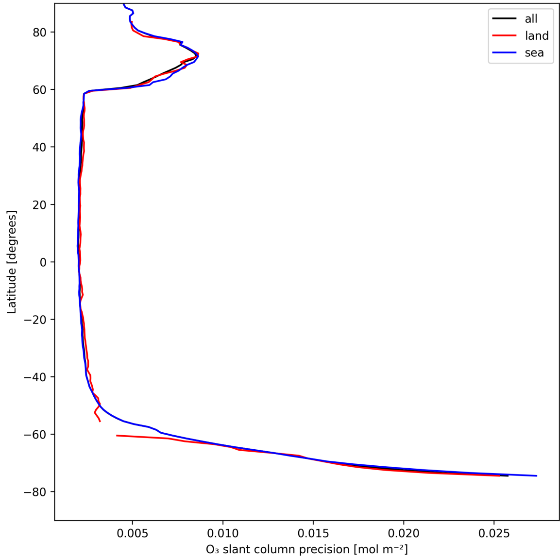
Figure 20: Zonal average of "O 3 slant column precision" for 2025-04-28 to 2025-04-29.
