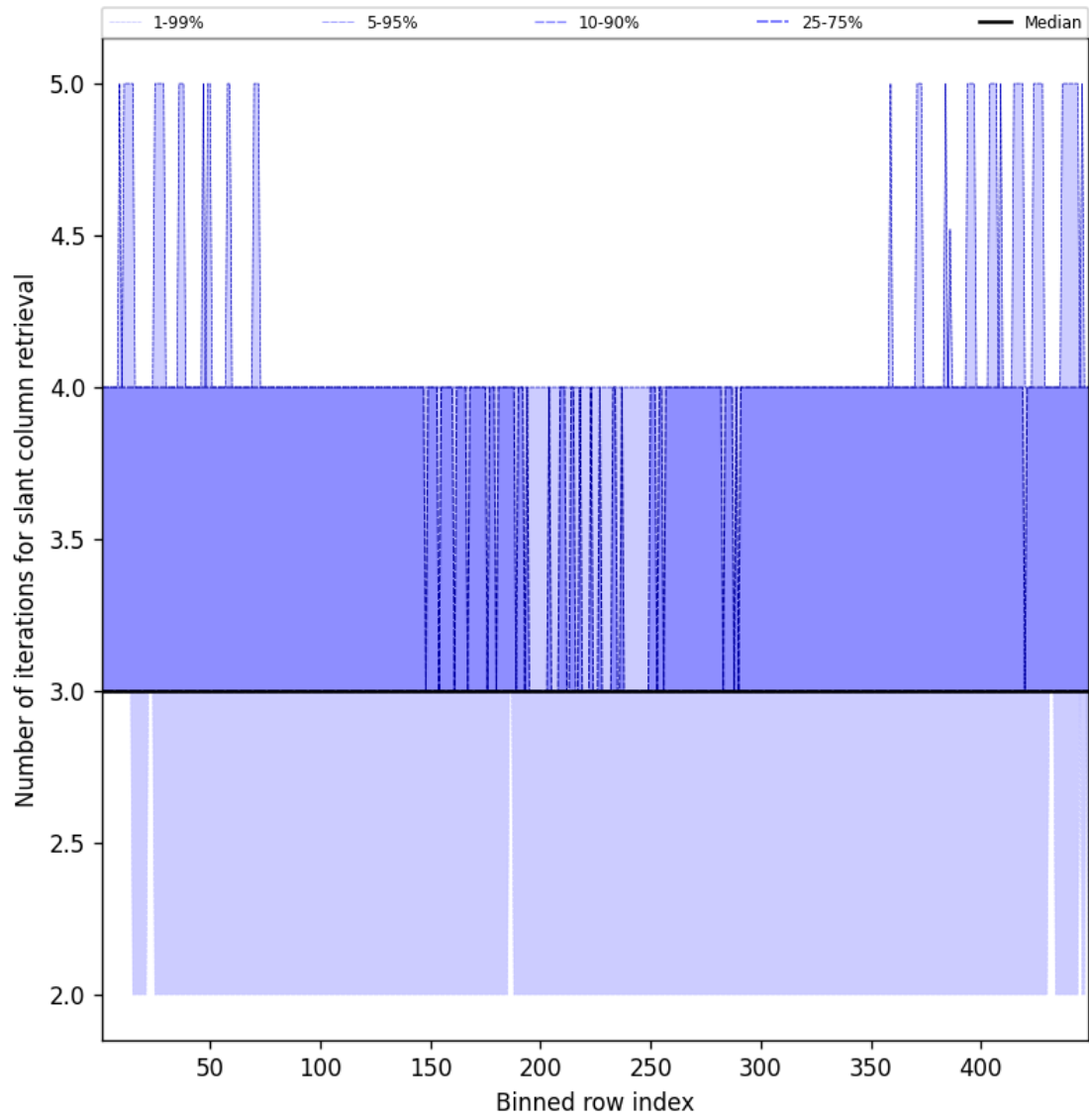
Figure 45: Along track statistics of “Number of iterations for slant column retrieval” for 2025-04-28 to 2025-04-29
