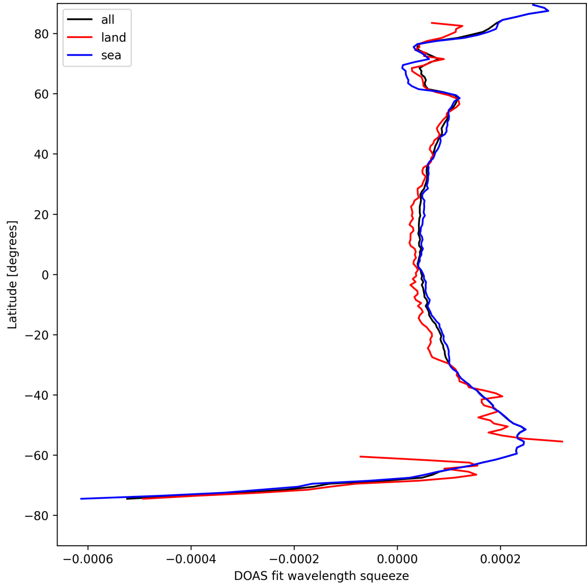
Figure 24: Zonal average of “DOAS fit wavelength squeeze” for 2025-04-28 to 2025-04-29.
