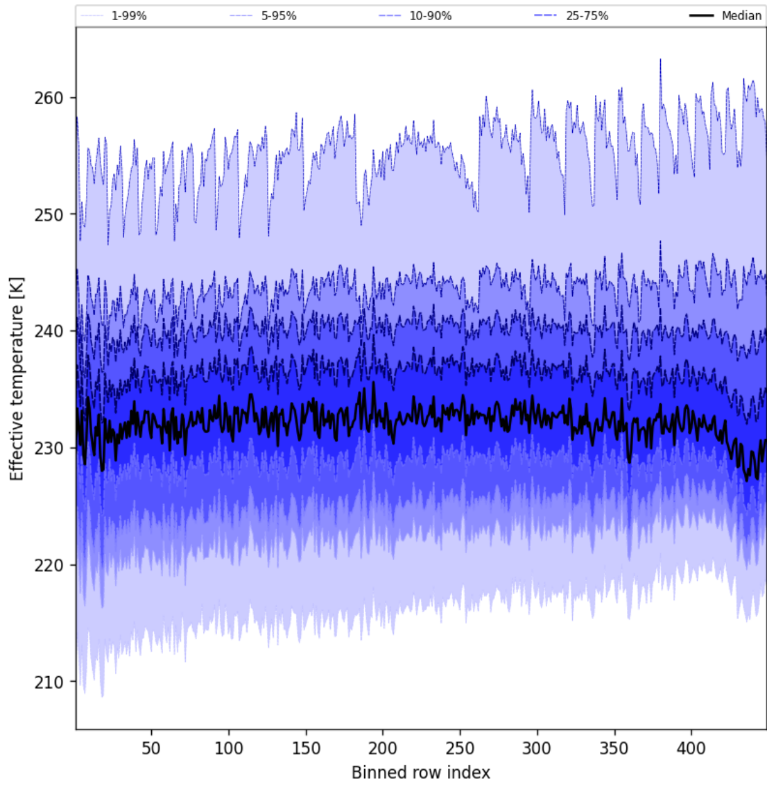
Figure 50: Along track statistics of “Effective temperature” for 2025-04-28 to 2025-04-29
