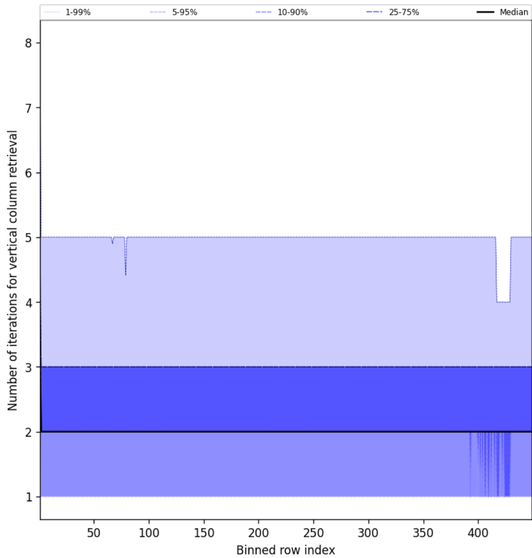
Figure 51: Along track statistics of “Number of iterations for vertical column retrieval” for 2025-04-28 to 2025-04-29
