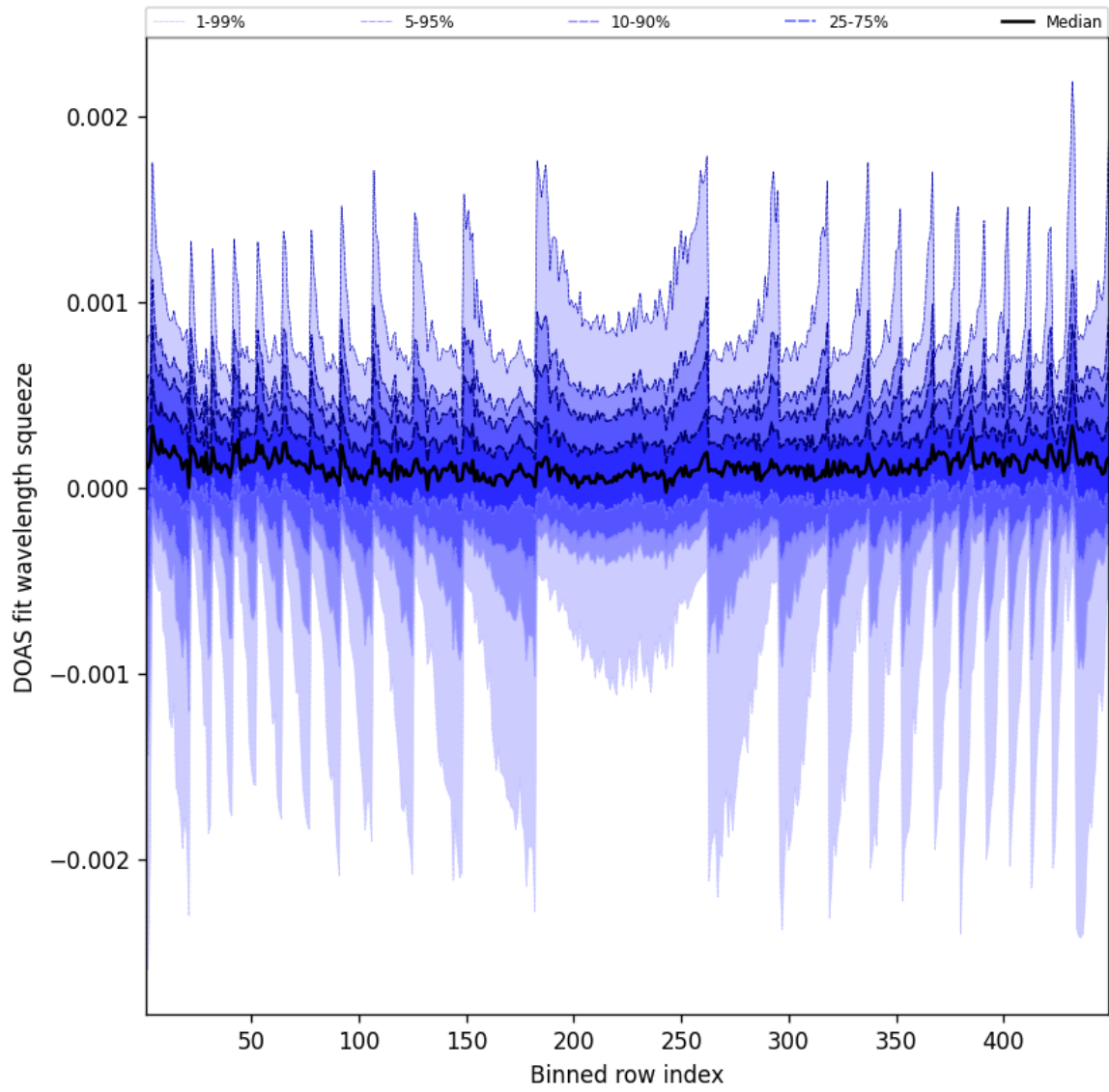
Figure 48: Along track statistics of “DOAS fit wavelength squeeze” for 2025-04-28 to 2025-04-29
