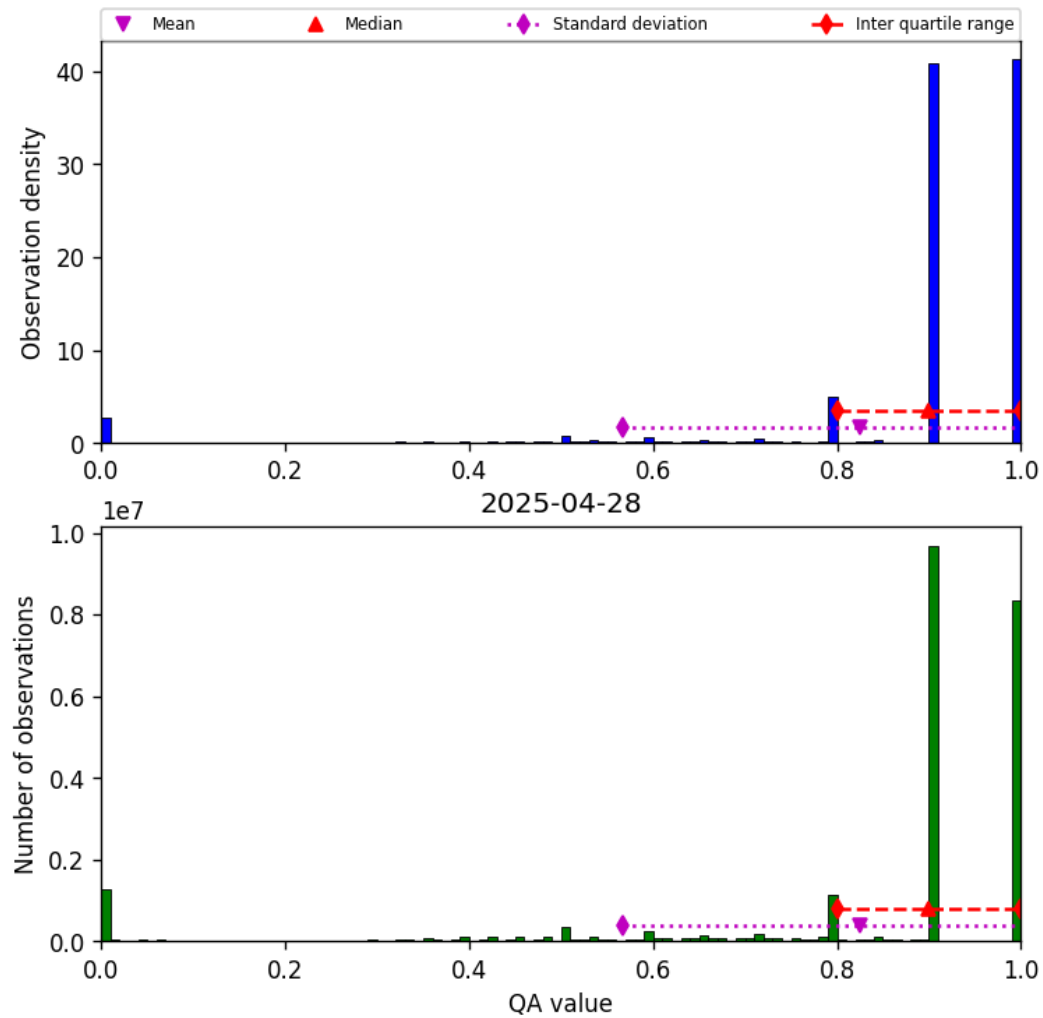
Figure 28: Histogram of “QA value” for 2025-04-28 to 2025-04-29
