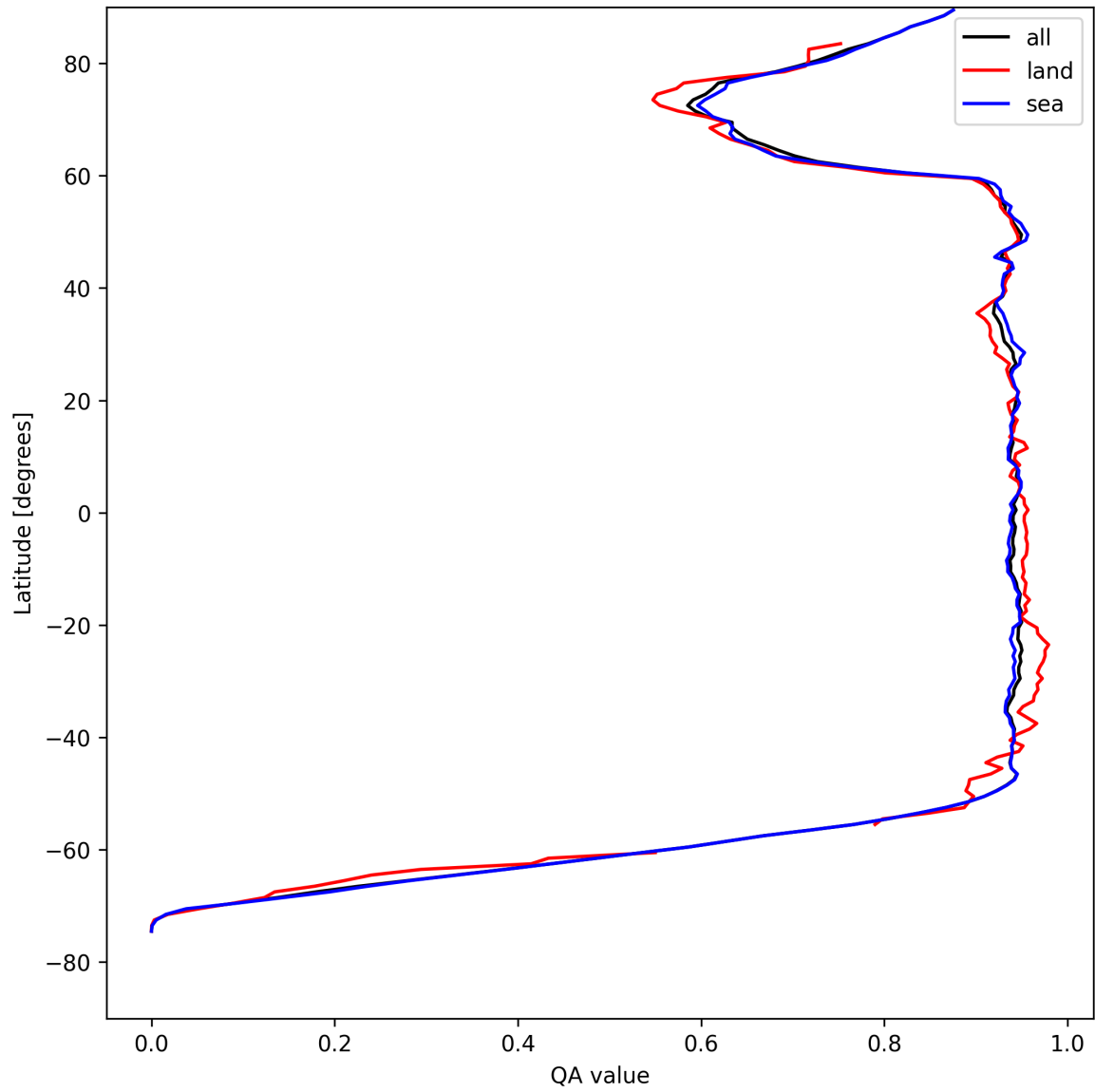
Figure 16: Zonal average of “QA value” for 2025-04-28 to 2025-04-29.
