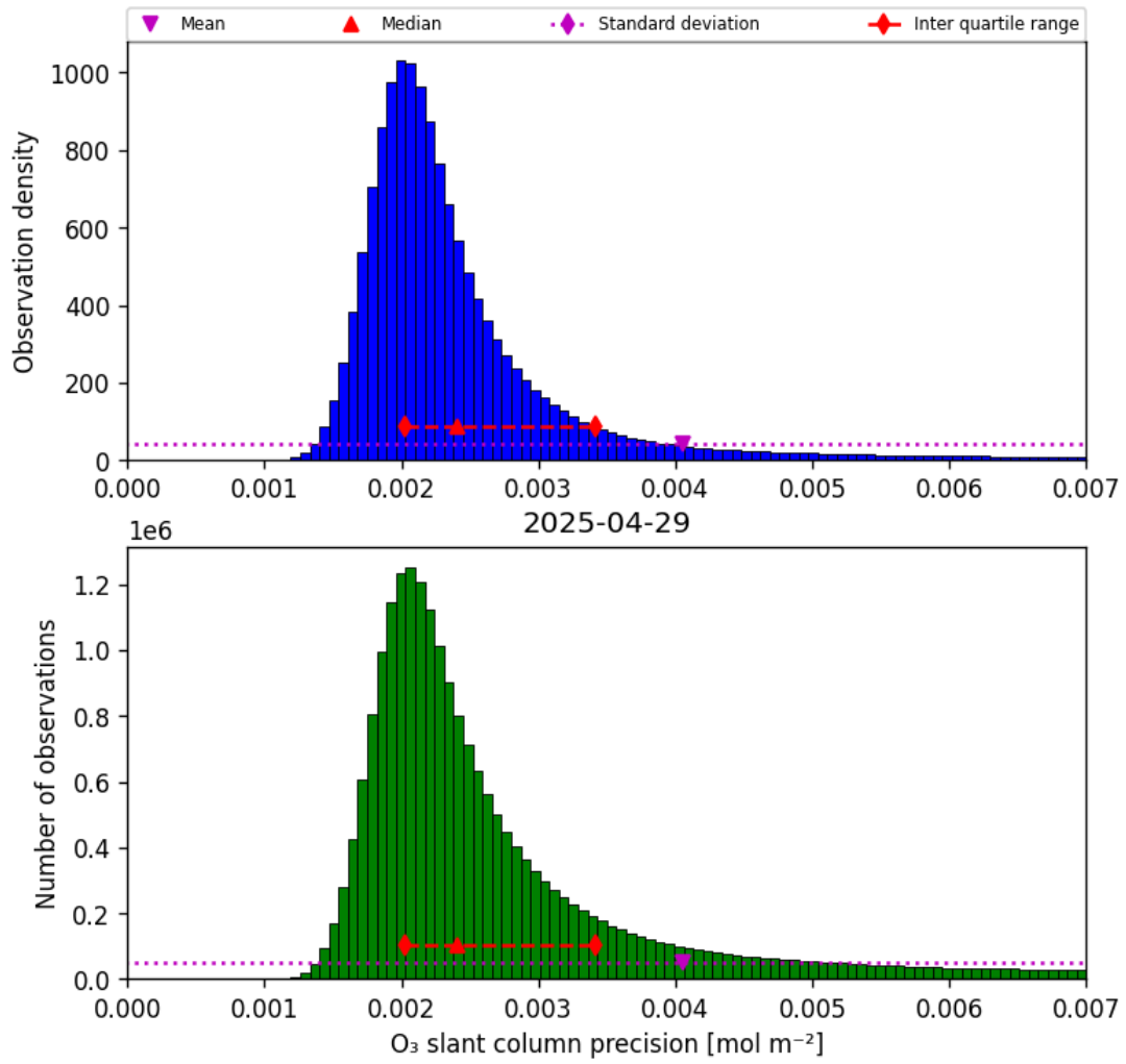
Figure 32: Histogram of “O 3 slant column precision” for 2025-04-29 to 2025-04-30
