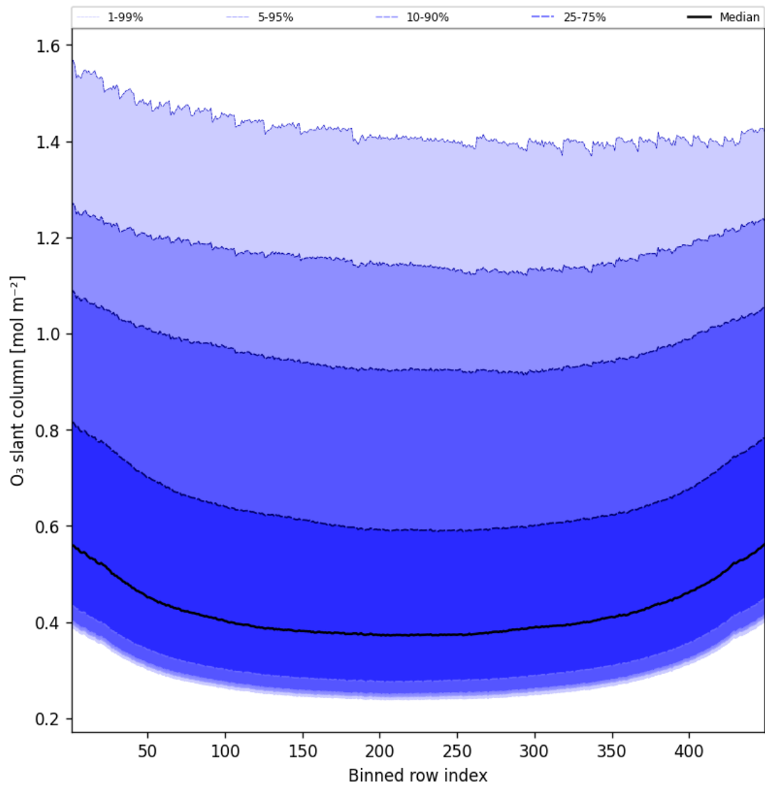
Figure 43: Along track statistics of “O 3 slant column” for 2025-04-29 to 2025-04-30
