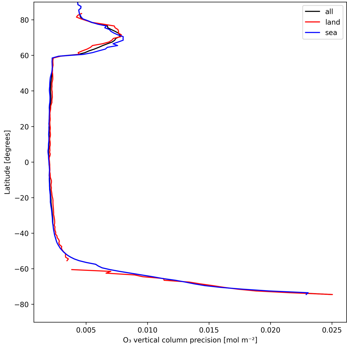
Figure 18: Zonal average of “O 3 vertical column precision” for 2025-04-29 to 2025-04-30.
