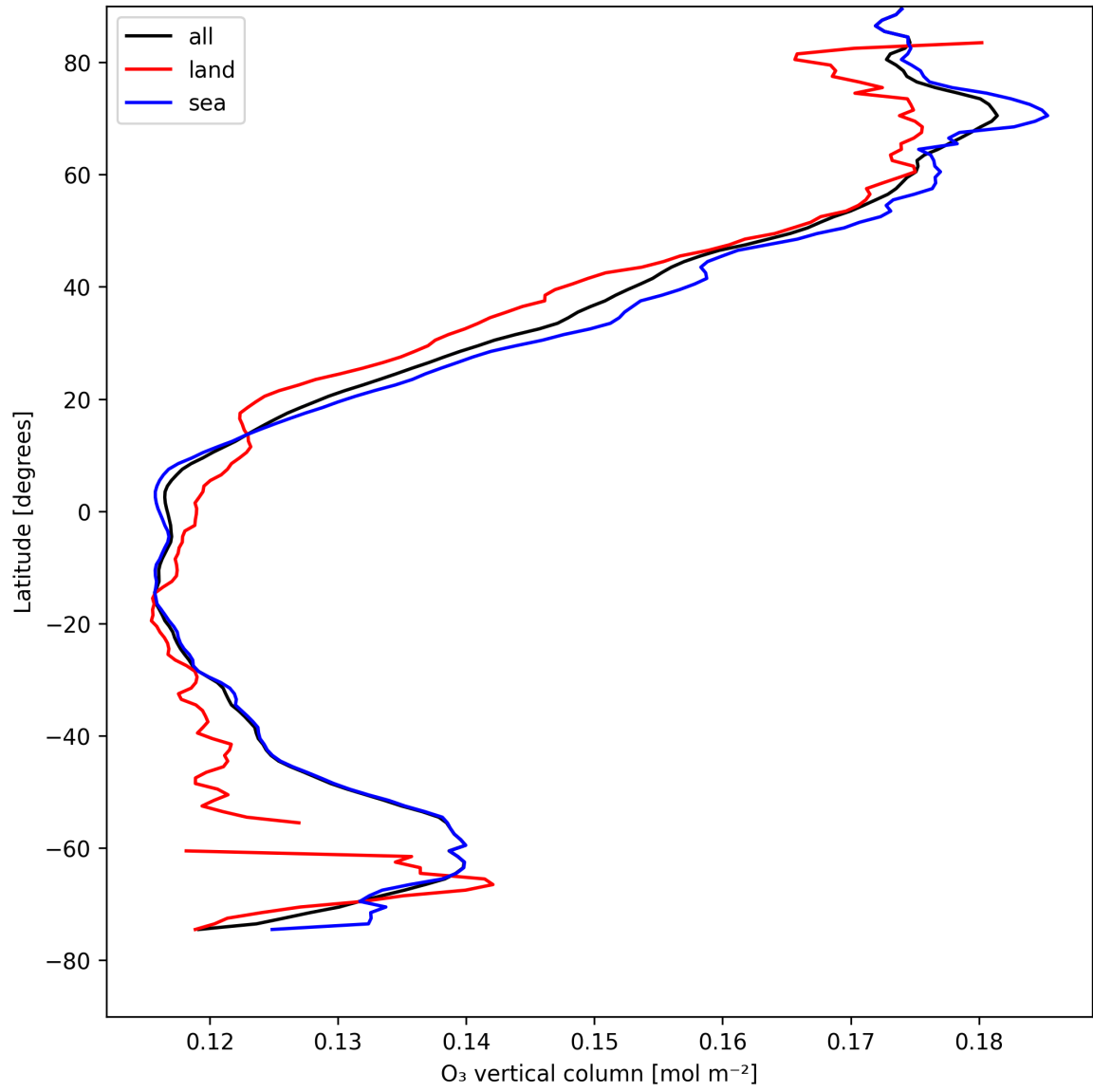
Figure 17: Zonal average of “O 3 vertical column” for 2025-04-29 to 2025-04-30.
