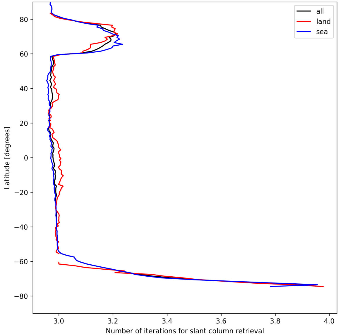
Figure 21: Zonal average of “Number of iterations for slant column retrieval” for 2025-04-29 to 2025-04-30.
