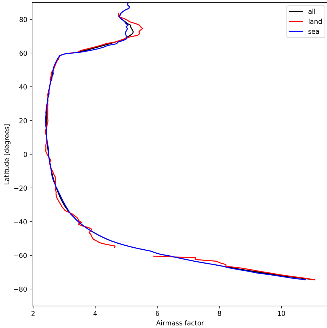
Figure 25: Zonal average of “Airmass factor” for 2025-04-29 to 2025-04-30.
