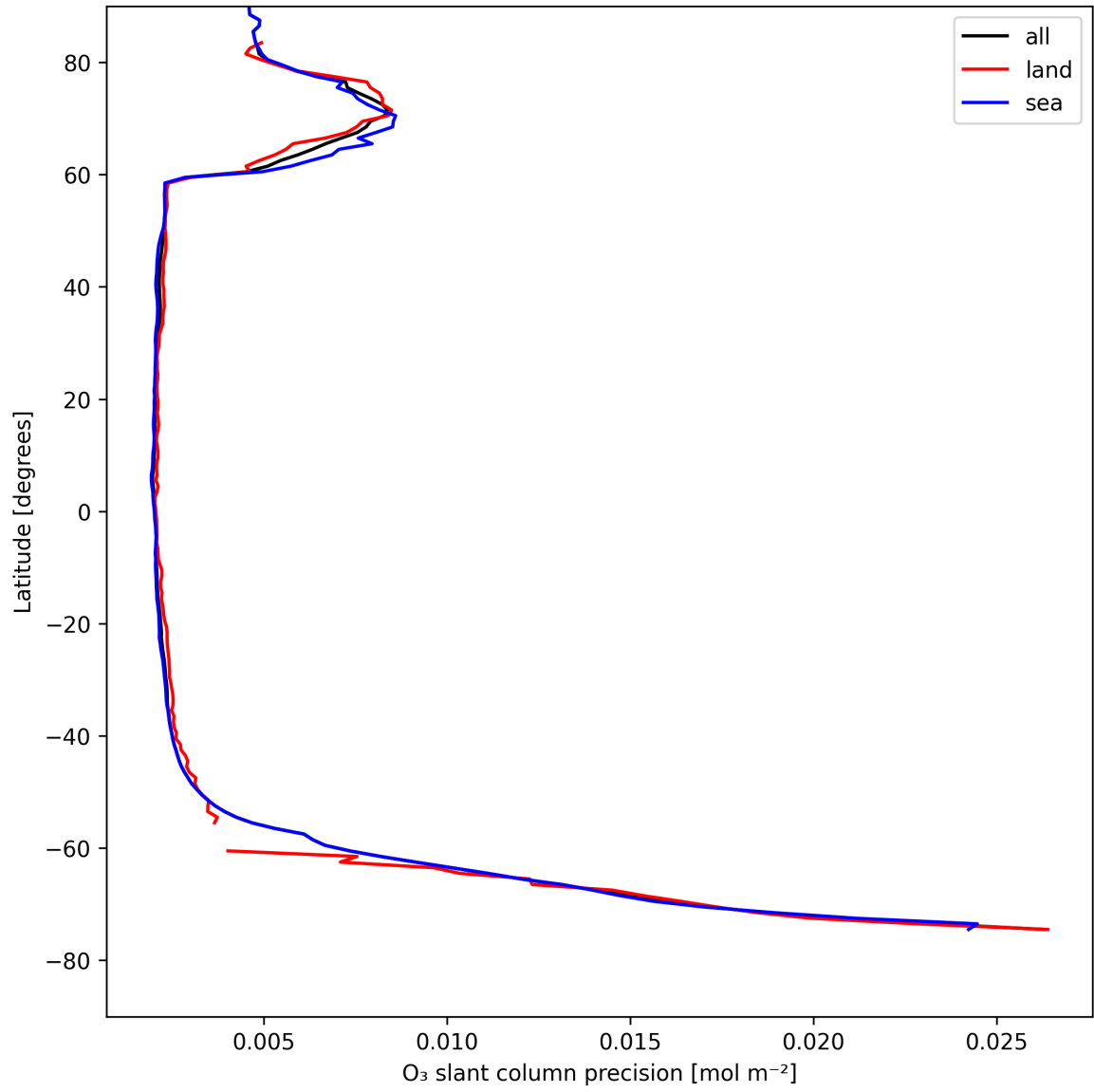
Figure 20: Zonal average of "O 3 slant column precision" for 2025-04-29 to 2025-04-30.
