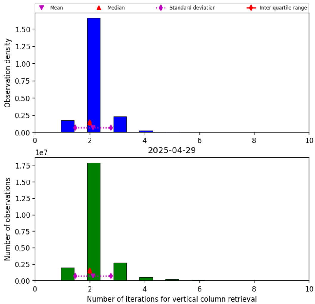
Figure 39: Histogram of “Number of iterations for vertical column retrieval” for 2025-04-29 to 2025-04-30
