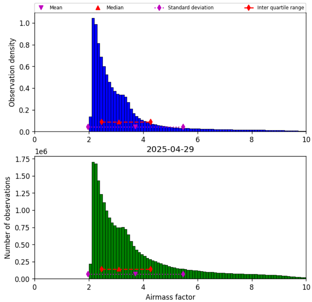
Figure 37: Histogram of “Airmass factor” for 2025-04-29 to 2025-04-30
