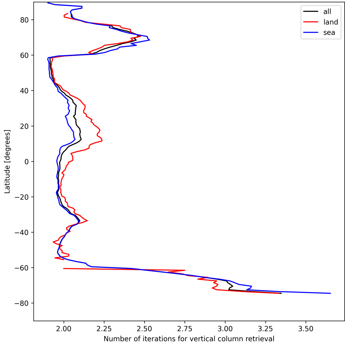
Figure 27: Zonal average of “Number of iterations for vertical column retrieval” for 2025-04-29 to 2025-04-30.
