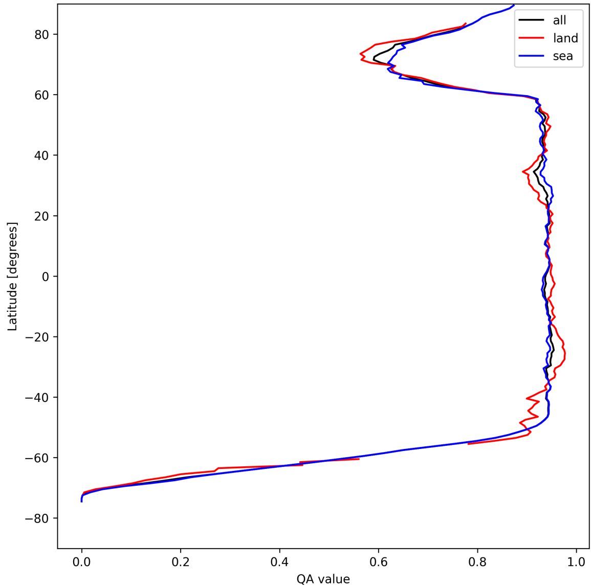
Figure 16: Zonal average of “QA value” for 2025-04-29 to 2025-04-30.
