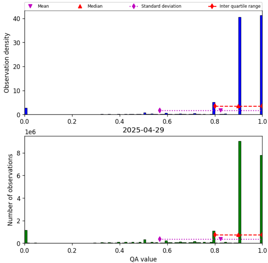
Figure 28: Histogram of “QA value” for 2025-04-29 to 2025-04-30
