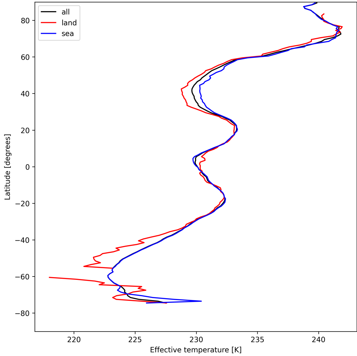
Figure 26: Zonal average of “Effective temperature” for 2025-04-29 to 2025-04-30.
