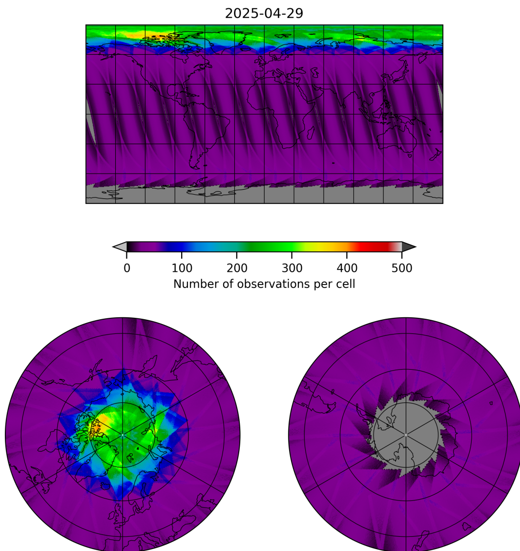
Figure 15: Map of the number of observations for 2025-04-29 to 2025-04-30
