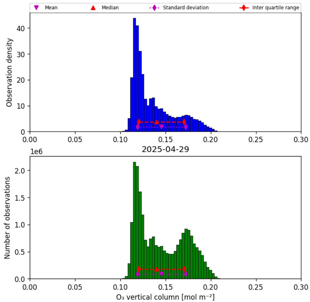
Figure 29: Histogram of “O 3 vertical column” for 2025-04-29 to 2025-04-30
