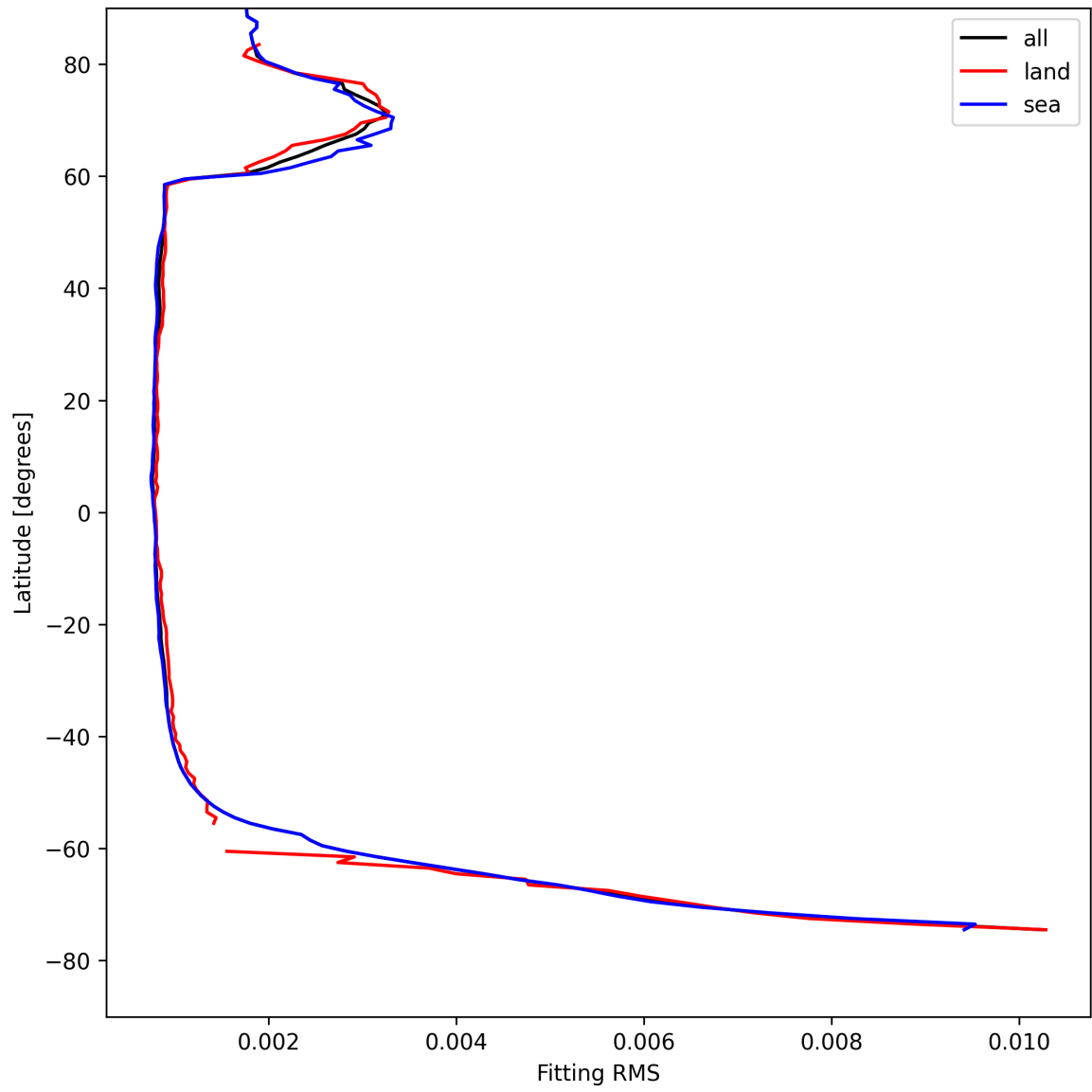
Figure 22: Zonal average of “Fitting RMS” for 2025-04-29 to 2025-04-30.
