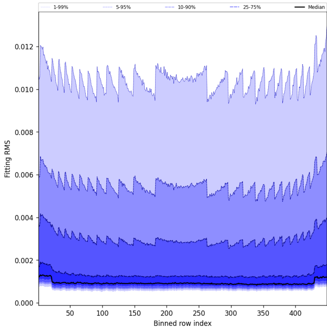
Figure 46: Along track statistics of “Fitting RMS” for 2025-04-29 to 2025-04-30
