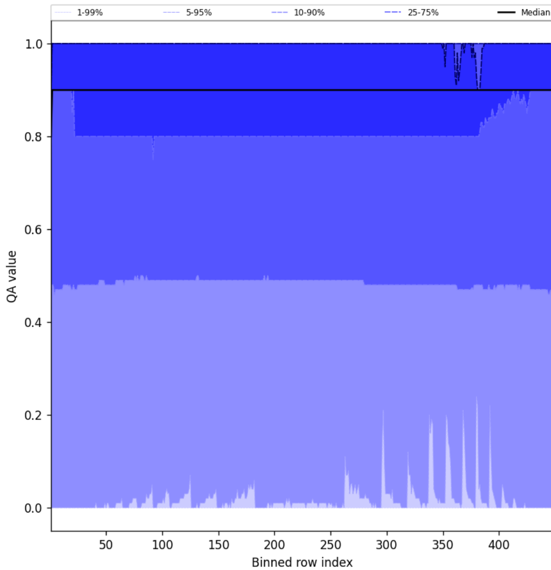
Figure 40: Along track statistics of “QA value” for 2025-04-29 to 2025-04-30
