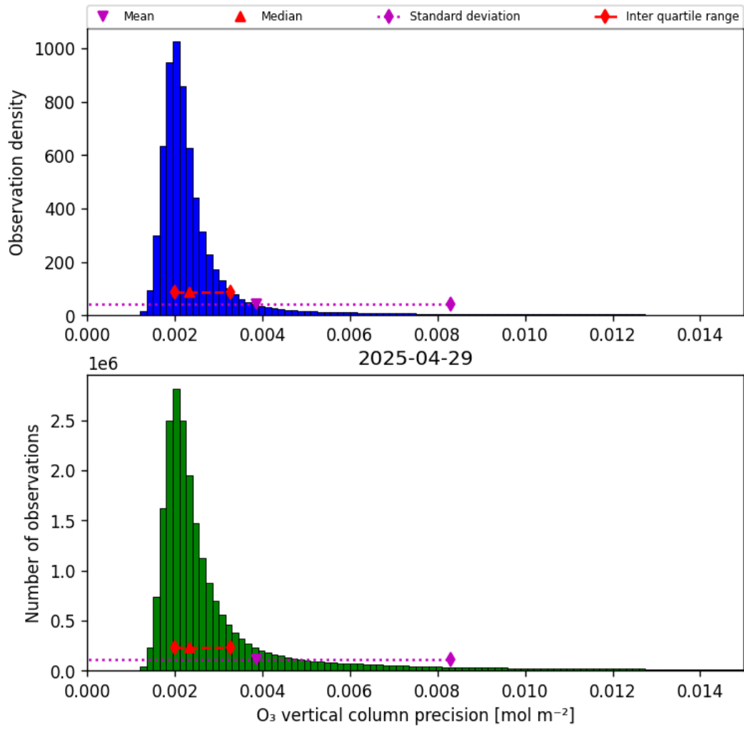
Figure 30: Histogram of “O 3 vertical column precision” for 2025-04-29 to 2025-04-30
