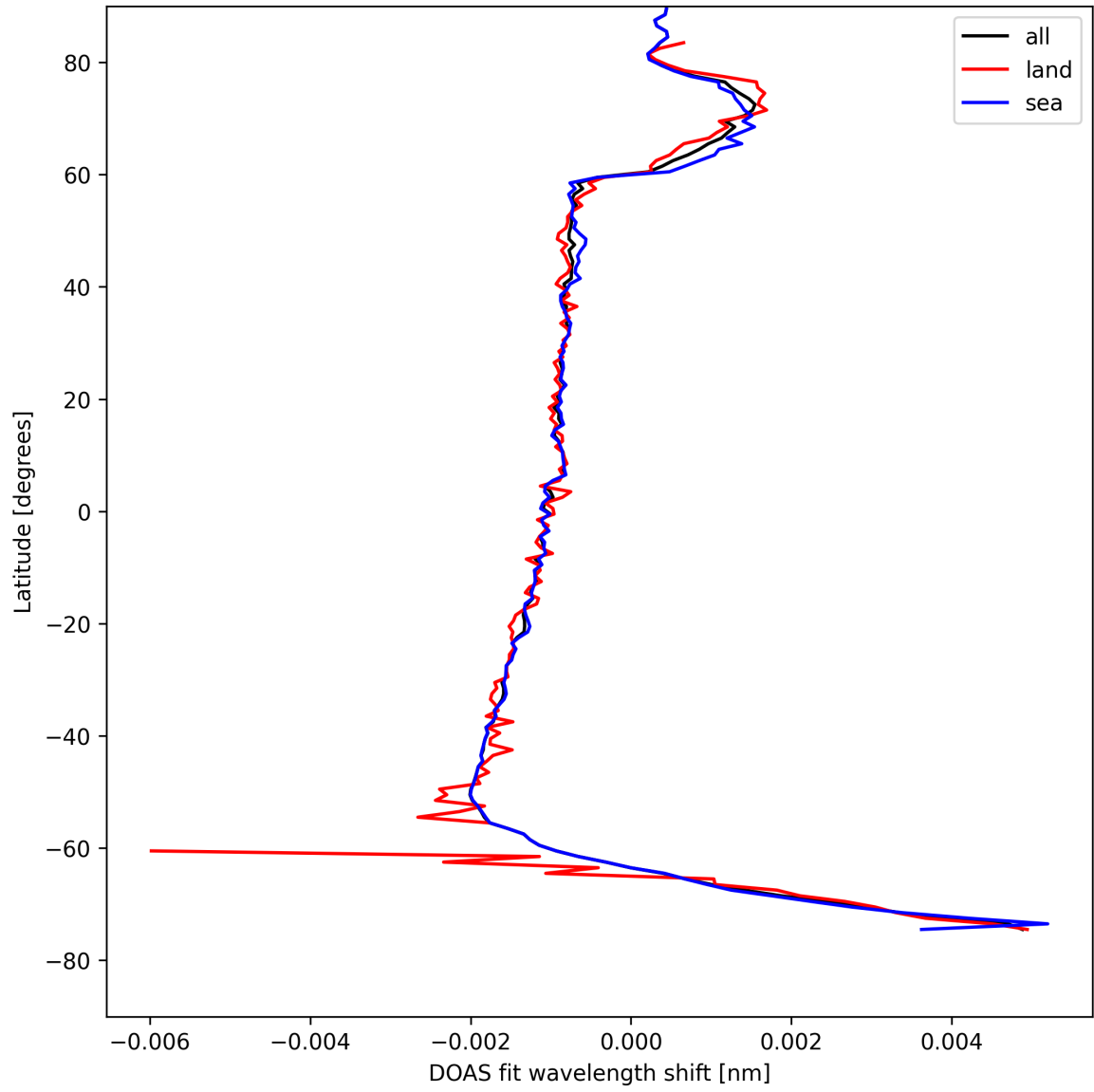
Figure 23: Zonal average of “DOAS fit wavelength shift” for 2025-04-29 to 2025-04-30.
