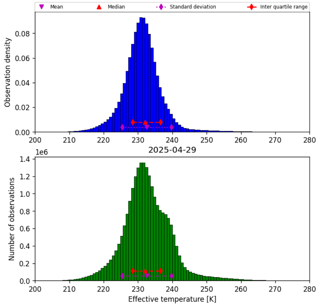
Figure 38: Histogram of “Effective temperature” for 2025-04-29 to 2025-04-30
