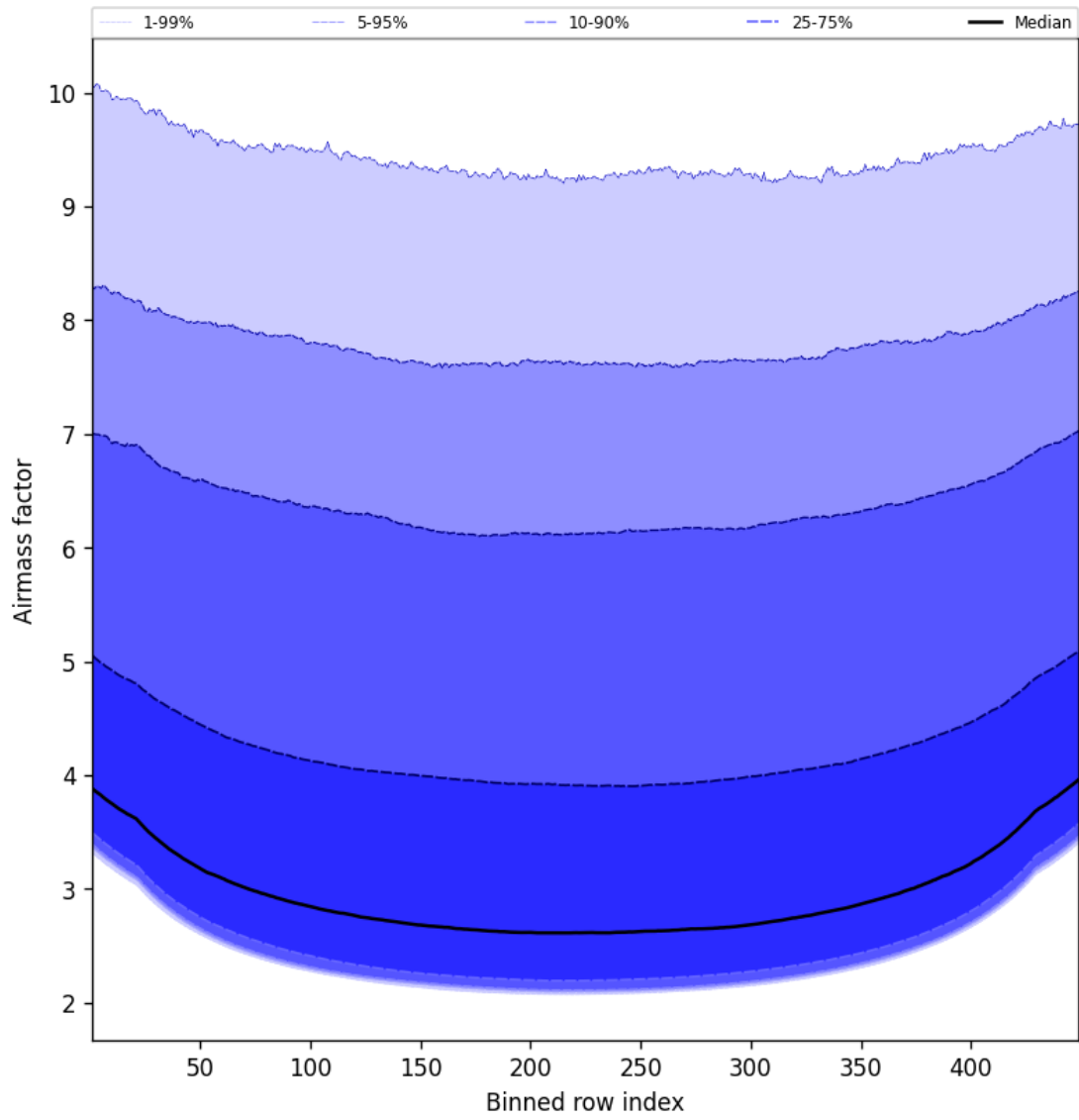
Figure 49: Along track statistics of “Airmass factor” for 2025-04-29 to 2025-04-30
