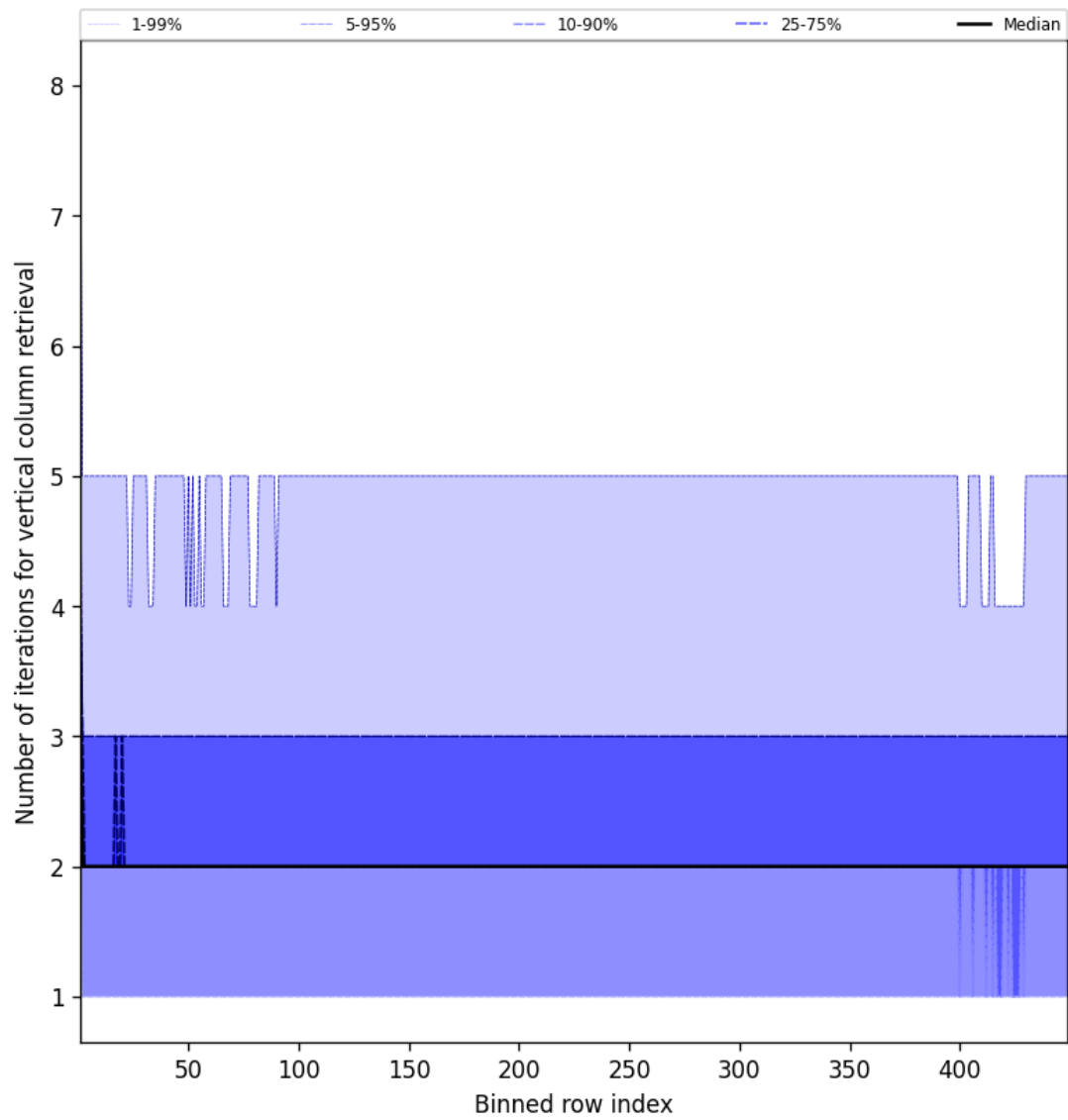
Figure 51: Along track statistics of “Number of iterations for vertical column retrieval” for 2025-04-29 to 2025-04-30
