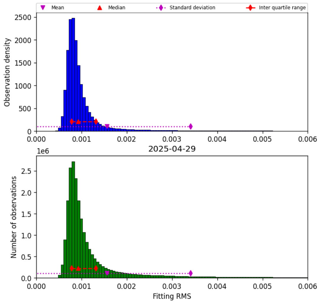
Figure 34: Histogram of “Fitting RMS” for 2025-04-29 to 2025-04-30
