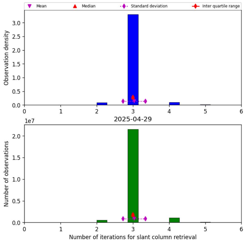
Figure 33: Histogram of "Number of iterations for slant column retrieval" for 2025-04-29 to 2025-04-30
