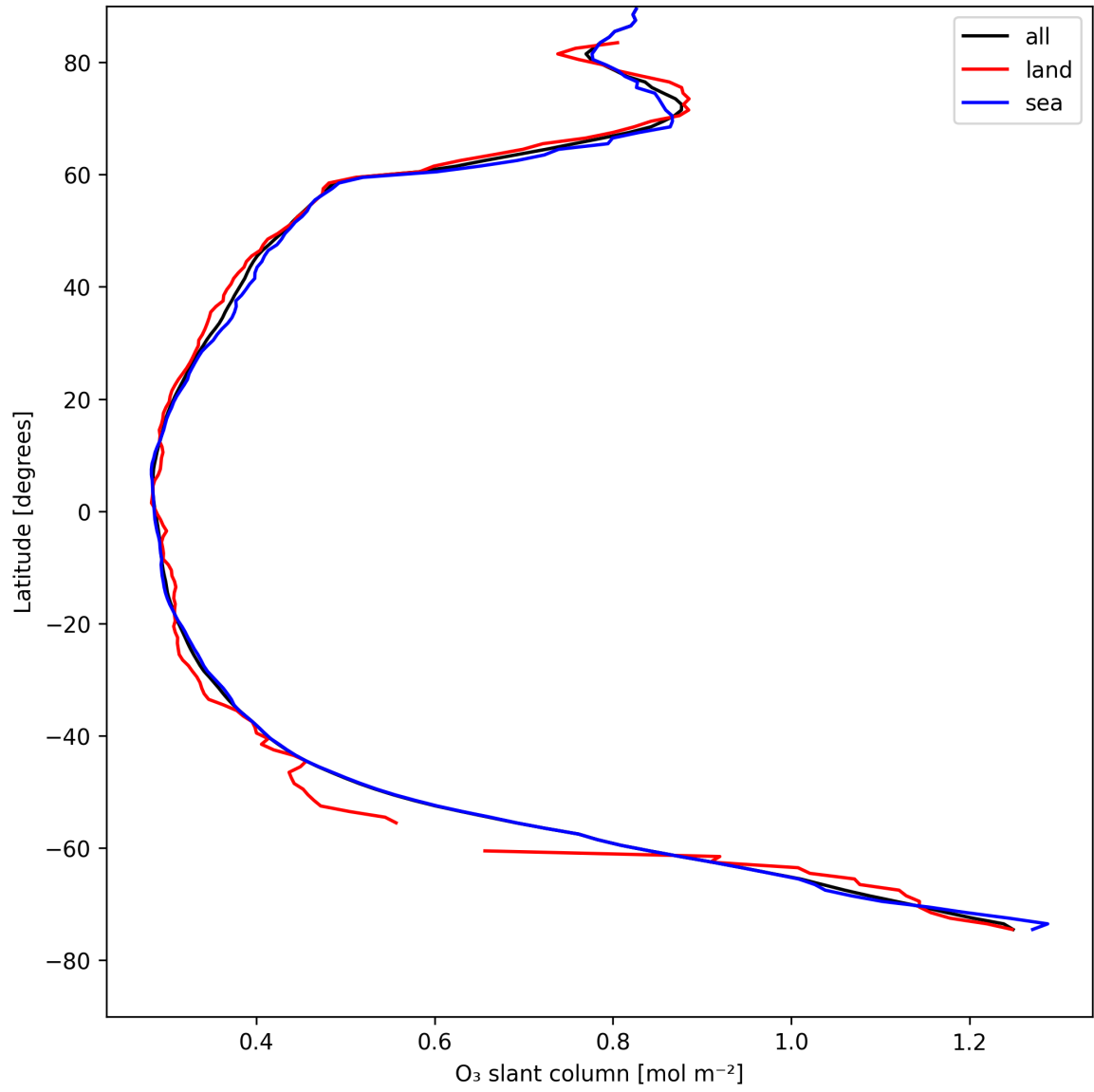
Figure 19: Zonal average of “O 3 slant column” for 2025-04-29 to 2025-04-30.
