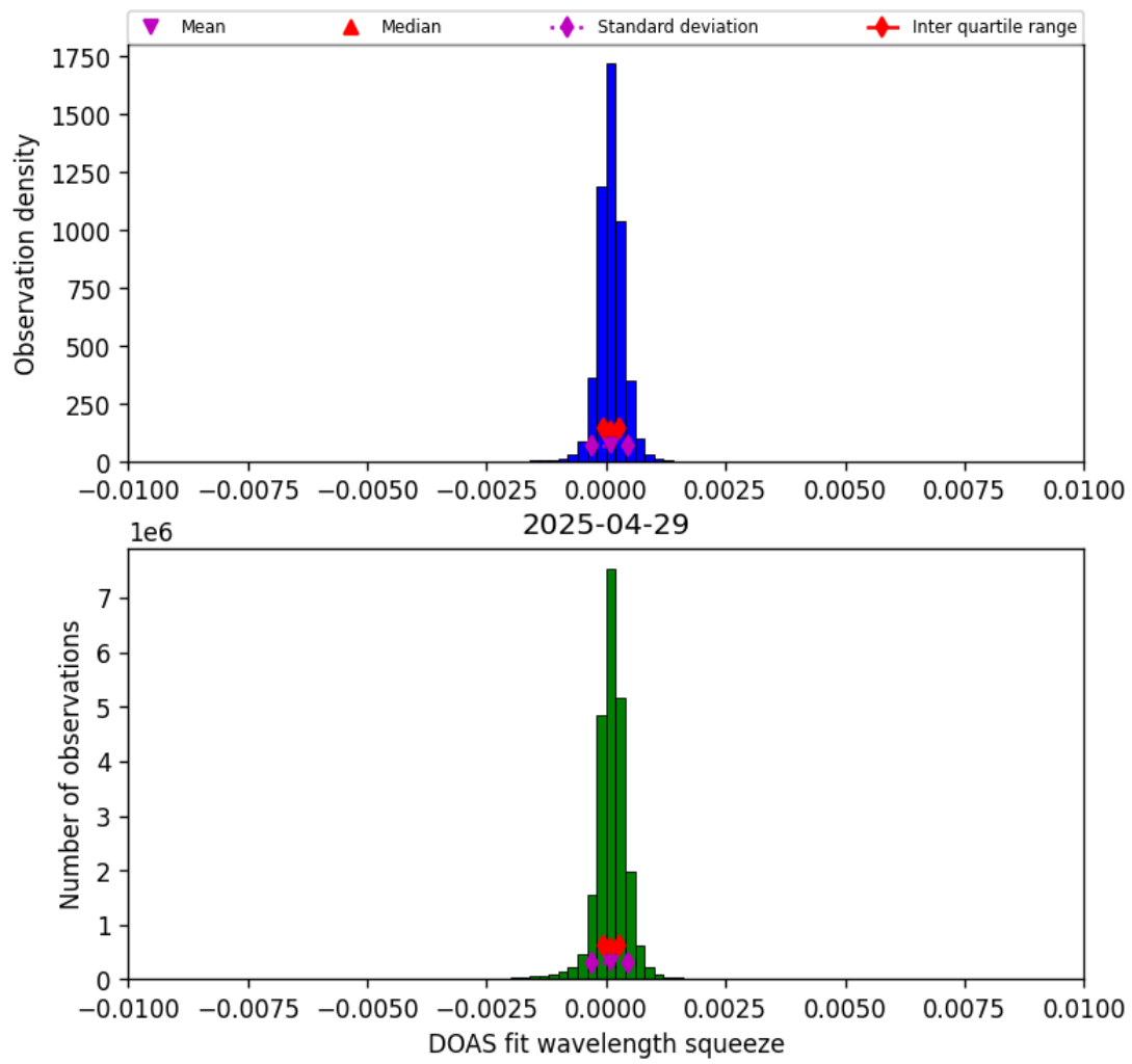
Figure 36: Histogram of “DOAS fit wavelength squeeze” for 2025-04-29 to 2025-04-30
