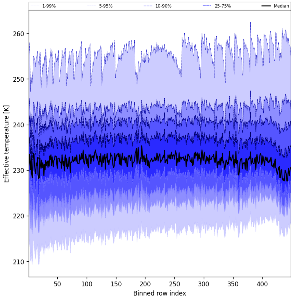
Figure 50: Along track statistics of “Effective temperature” for 2025-04-29 to 2025-04-30
