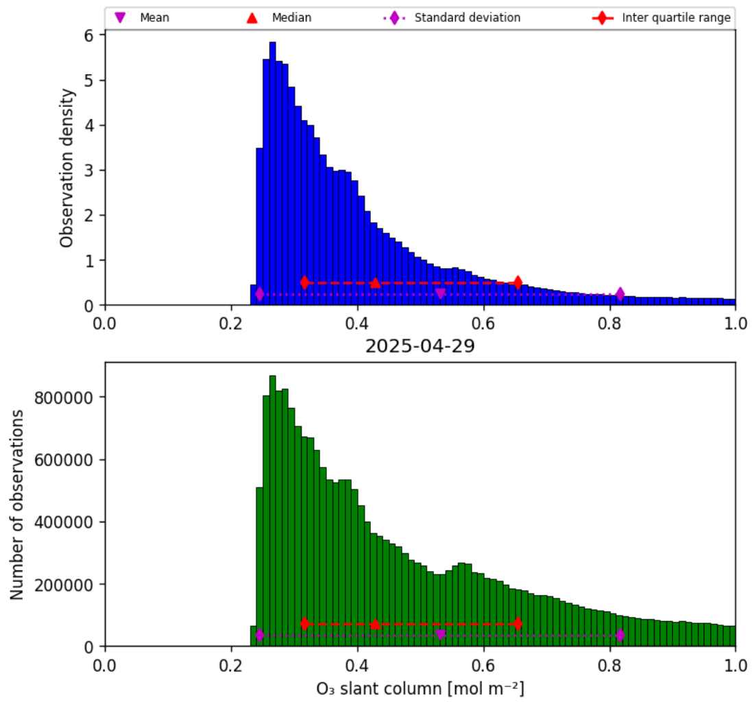
Figure 31: Histogram of “O 3 slant column” for 2025-04-29 to 2025-04-30
