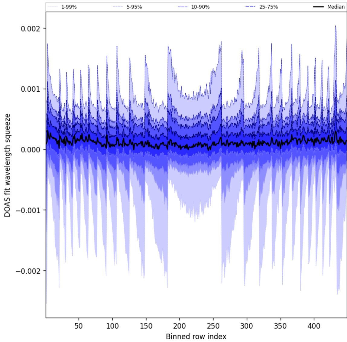
Figure 48: Along track statistics of “DOAS fit wavelength squeeze” for 2025-04-29 to 2025-04-30
