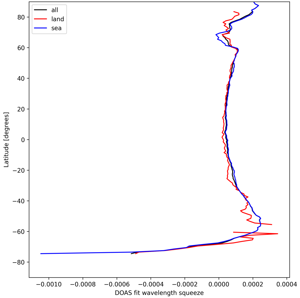
Figure 24: Zonal average of “DOAS fit wavelength squeeze” for 2025-04-29 to 2025-04-30.
