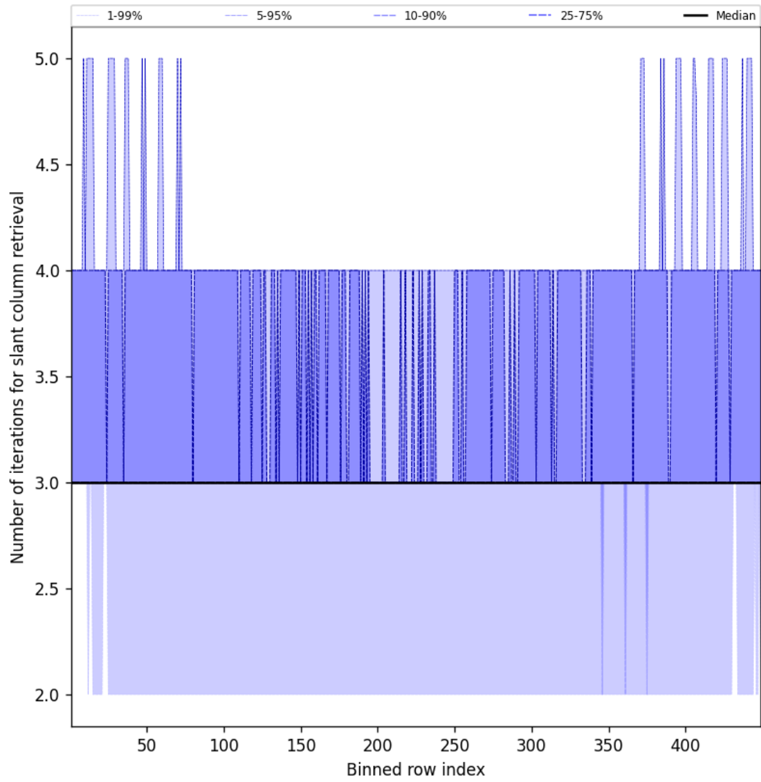
Figure 45: Along track statistics of “Number of iterations for slant column retrieval” for 2025-04-29 to 2025-04-30
