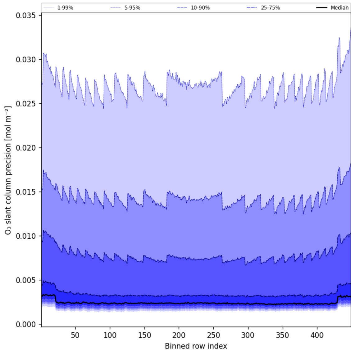
Figure 44: Along track statistics of “O 3 slant column precision” for 2025-04-29 to 2025-04-30
