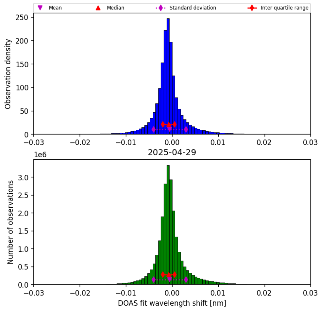
Figure 35: Histogram of “DOAS fit wavelength shift” for 2025-04-29 to 2025-04-30
