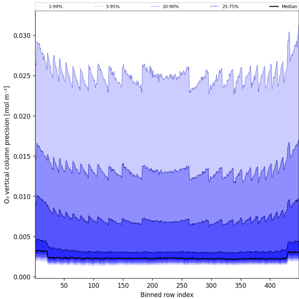
Figure 42: Along track statistics of “O 3 vertical column precision” for 2025-04-29 to 2025-04-30
