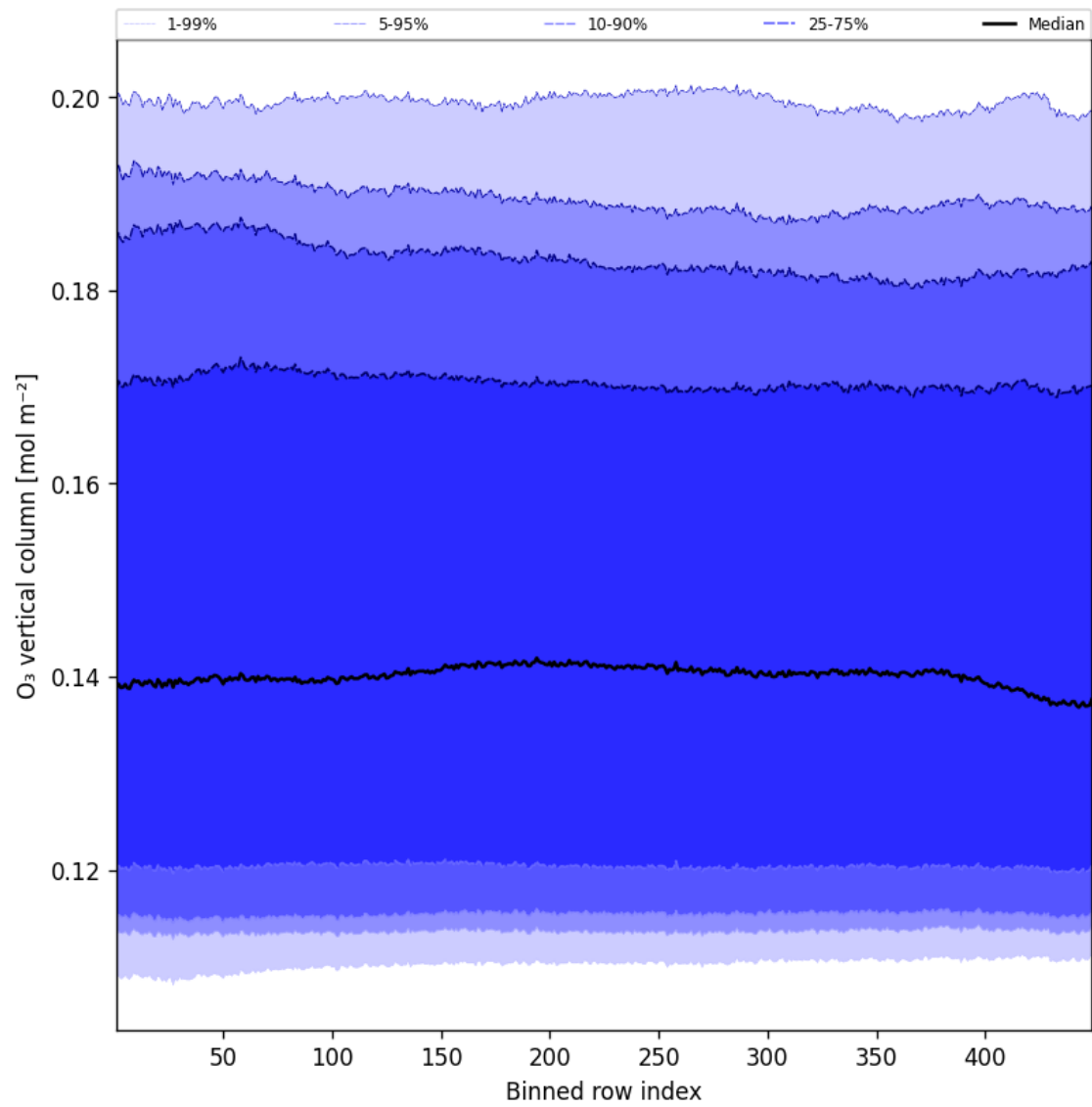
Figure 41: Along track statistics of “O 3 vertical column” for 2025-04-29 to 2025-04-30
