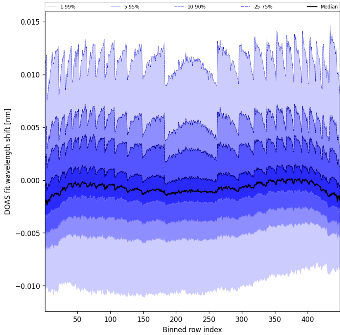
Figure 47: Along track statistics of “DOAS fit wavelength shift” for 2025-04-29 to 2025-04-30
