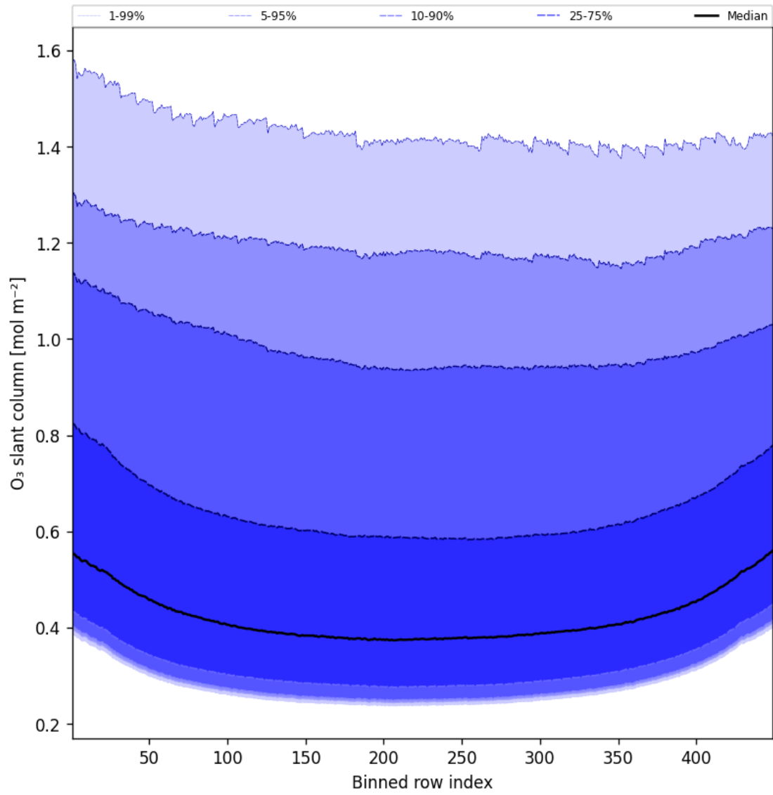
Figure 43: Along track statistics of “O 3 slant column” for 2025-04-30 to 2025-05-01
