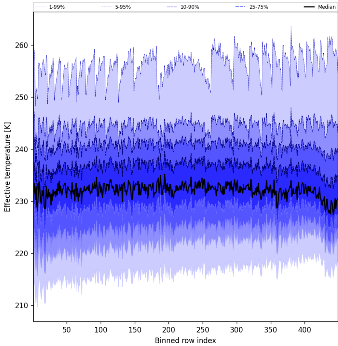
Figure 50: Along track statistics of “Effective temperature” for 2025-04-30 to 2025-05-01
