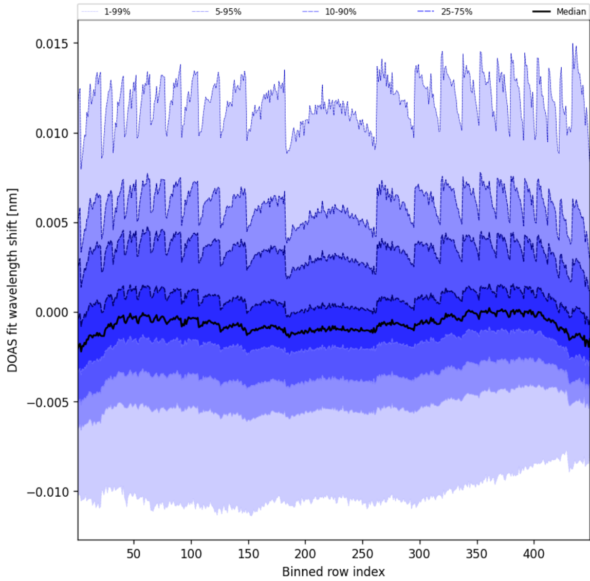
Figure 47: Along track statistics of “DOAS fit wavelength shift” for 2025-04-30 to 2025-05-01
