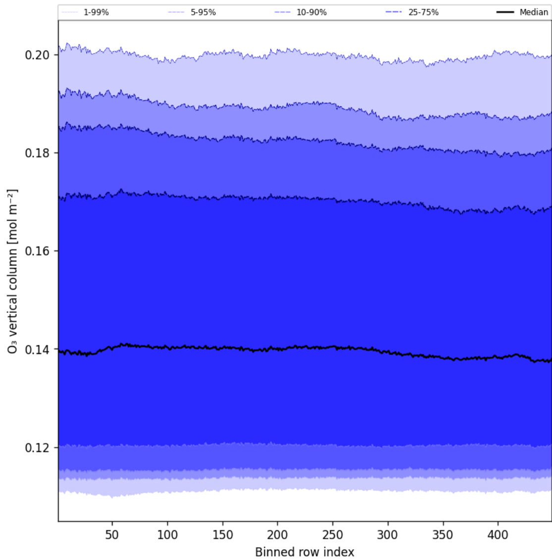
Figure 41: Along track statistics of “ O_3 vertical column” for 2025-04-30 to 2025-05-01
