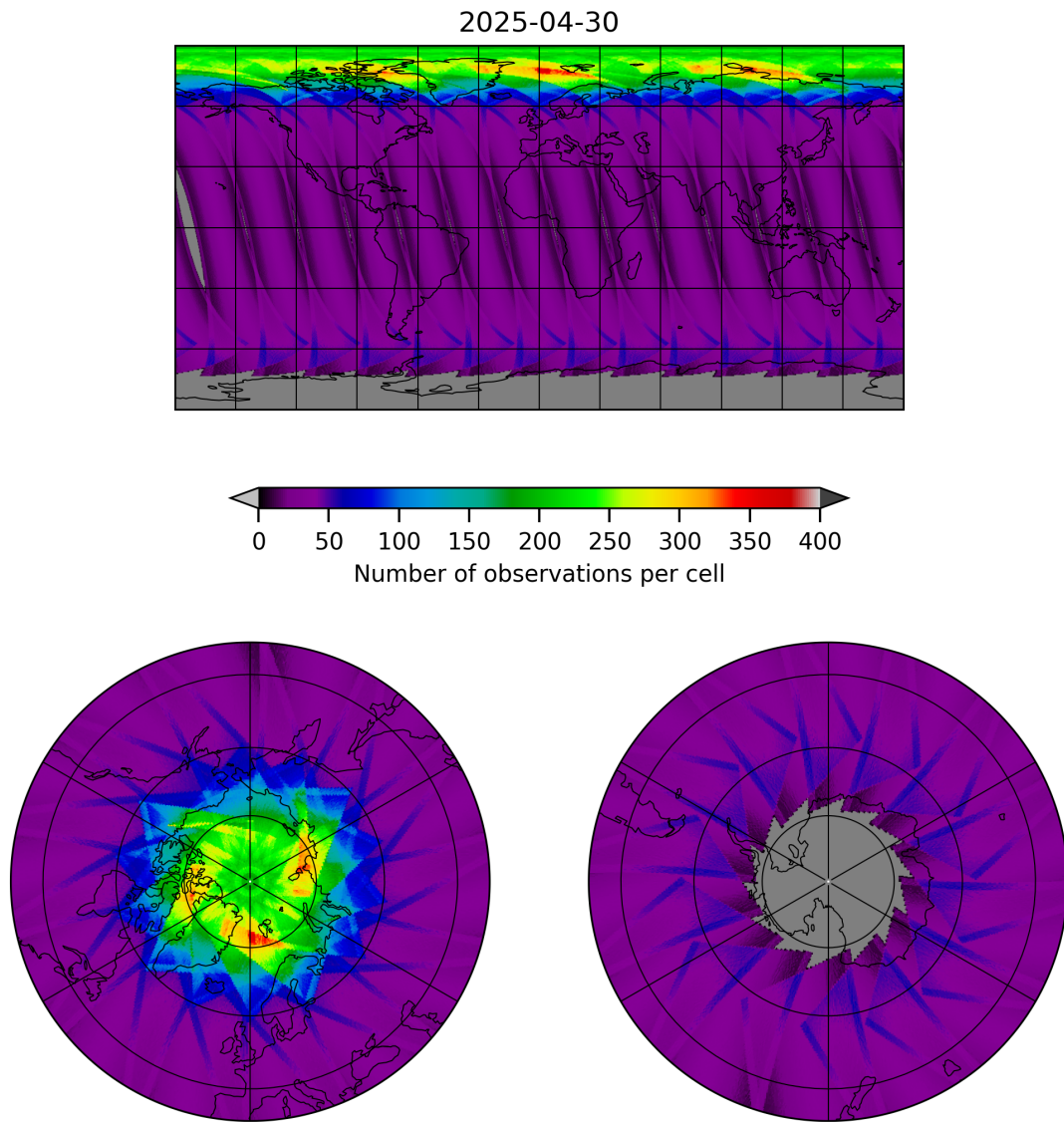
Figure 15: Map of the number of observations for 2025-04-30 to 2025-05-01
