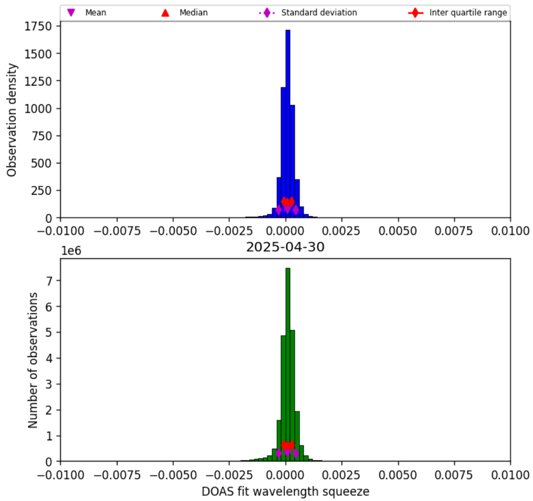
Figure 36: Histogram of “DOAS fit wavelength squeeze” for 2025-04-30 to 2025-05-01
