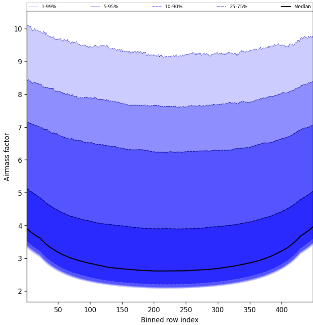
Figure 49: Along track statistics of “Airmass factor” for 2025-04-30 to 2025-05-01
