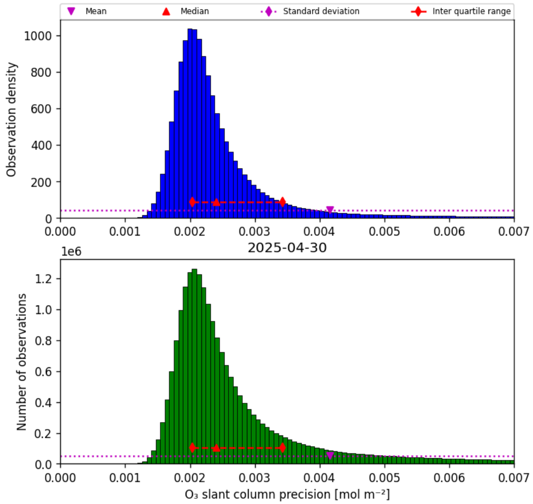
Figure 32: Histogram of “O 3 slant column precision” for 2025-04-30 to 2025-05-01
