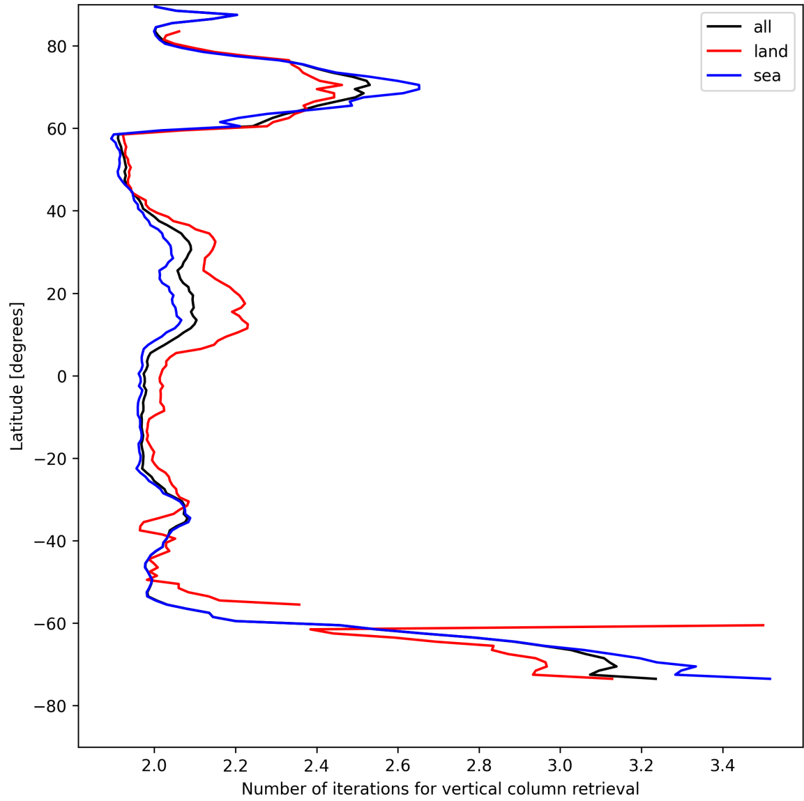
Figure 27: Zonal average of “Number of iterations for vertical column retrieval” for 2025-04-30 to 2025-05-01.
