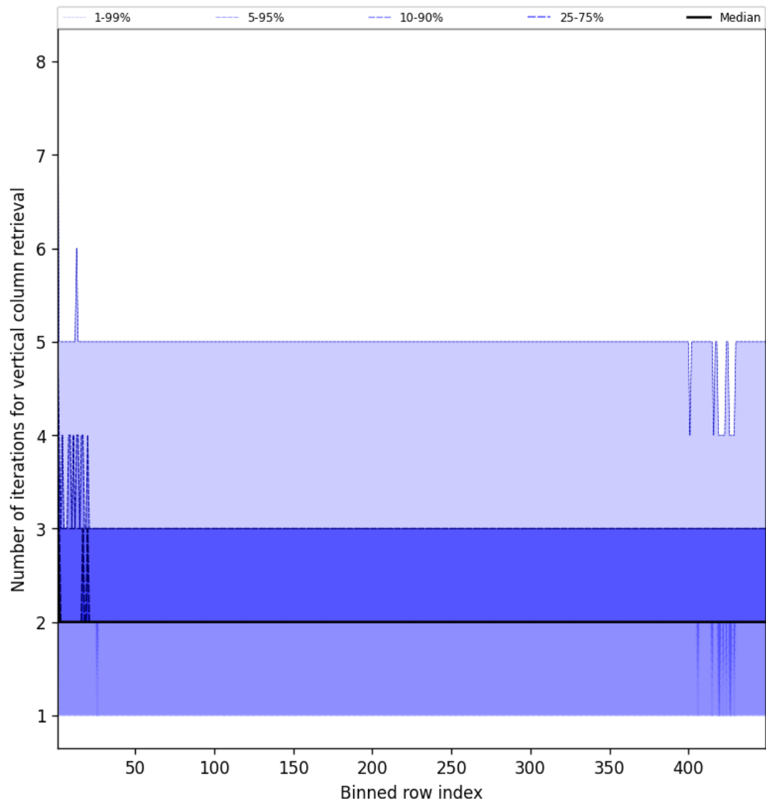
Figure 51: Along track statistics of “Number of iterations for vertical column retrieval” for 2025-04-30 to 2025-05-01
