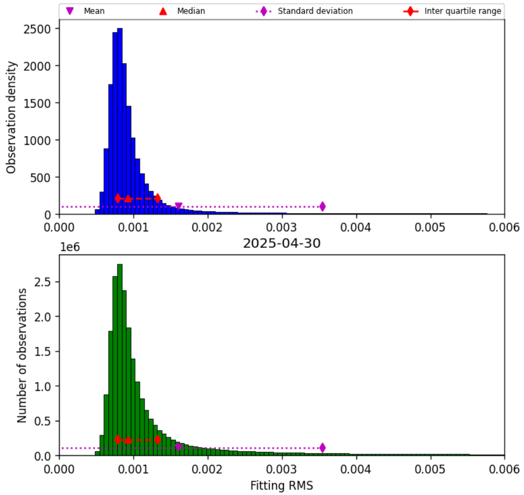
Figure 34: Histogram of “Fitting RMS” for 2025-04-30 to 2025-05-01
