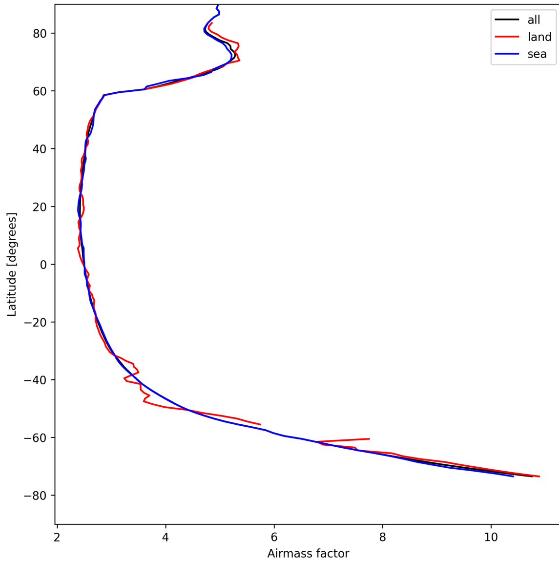
Figure 25: Zonal average of “Airmass factor” for 2025-04-30 to 2025-05-01.
