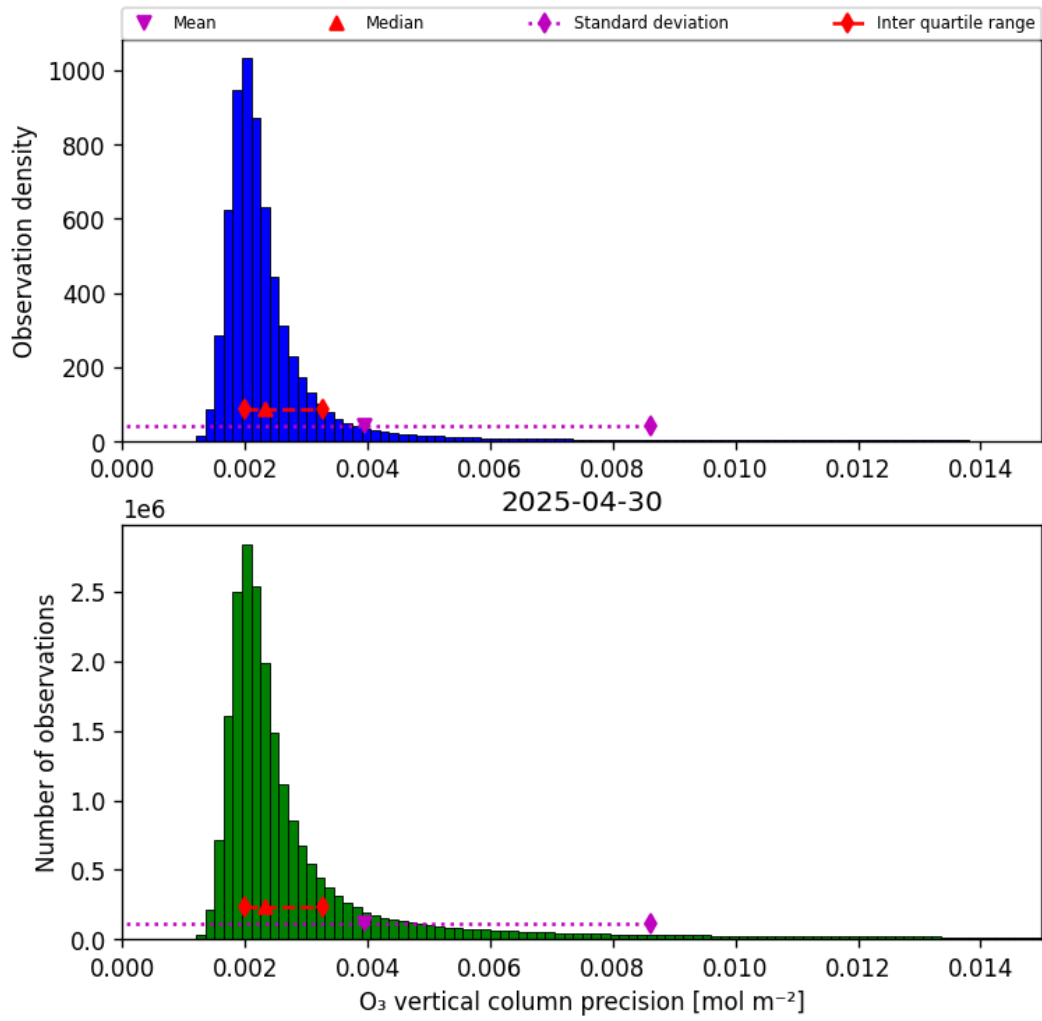
Figure 30: Histogram of “O 3 vertical column precision” for 2025-04-30 to 2025-05-01
