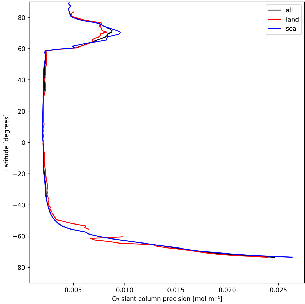
Figure 20: Zonal average of "O 3 slant column precision" for 2025-04-30 to 2025-05-01.
