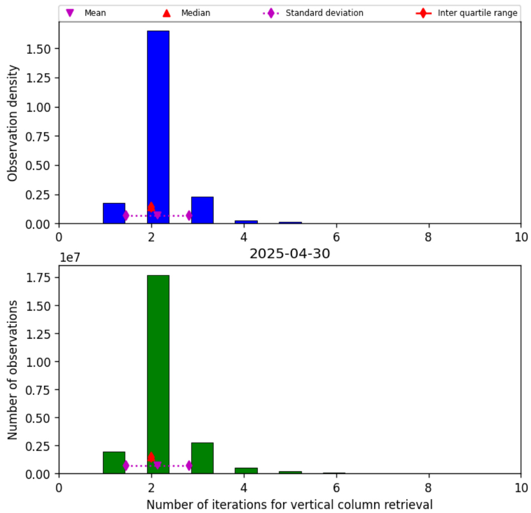
Figure 39: Histogram of “Number of iterations for vertical column retrieval” for 2025-04-30 to 2025-05-01
