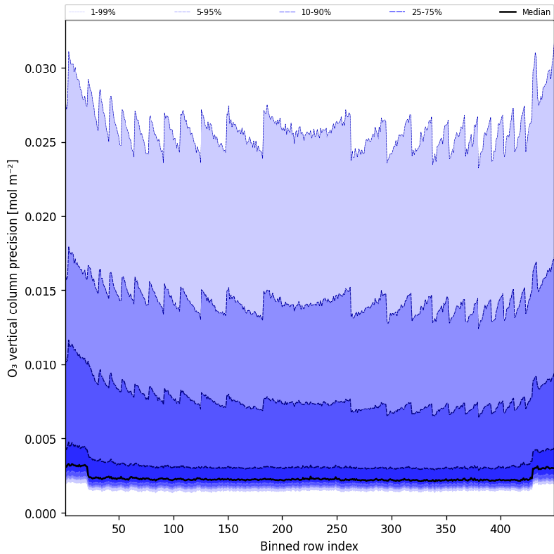
Figure 42: Along track statistics of “O 3 vertical column precision” for 2025-04-30 to 2025-05-01
