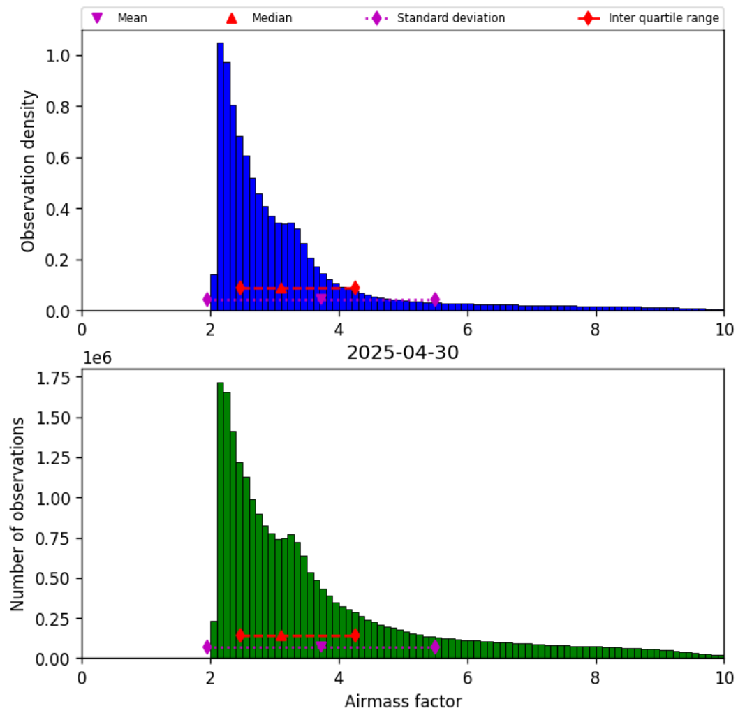
Figure 37: Histogram of “Airmass factor” for 2025-04-30 to 2025-05-01
