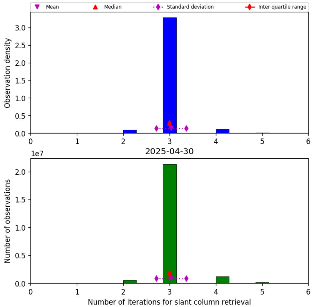
Figure 33: Histogram of “Number of iterations for slant column retrieval” for 2025-04-30 to 2025-05-01
