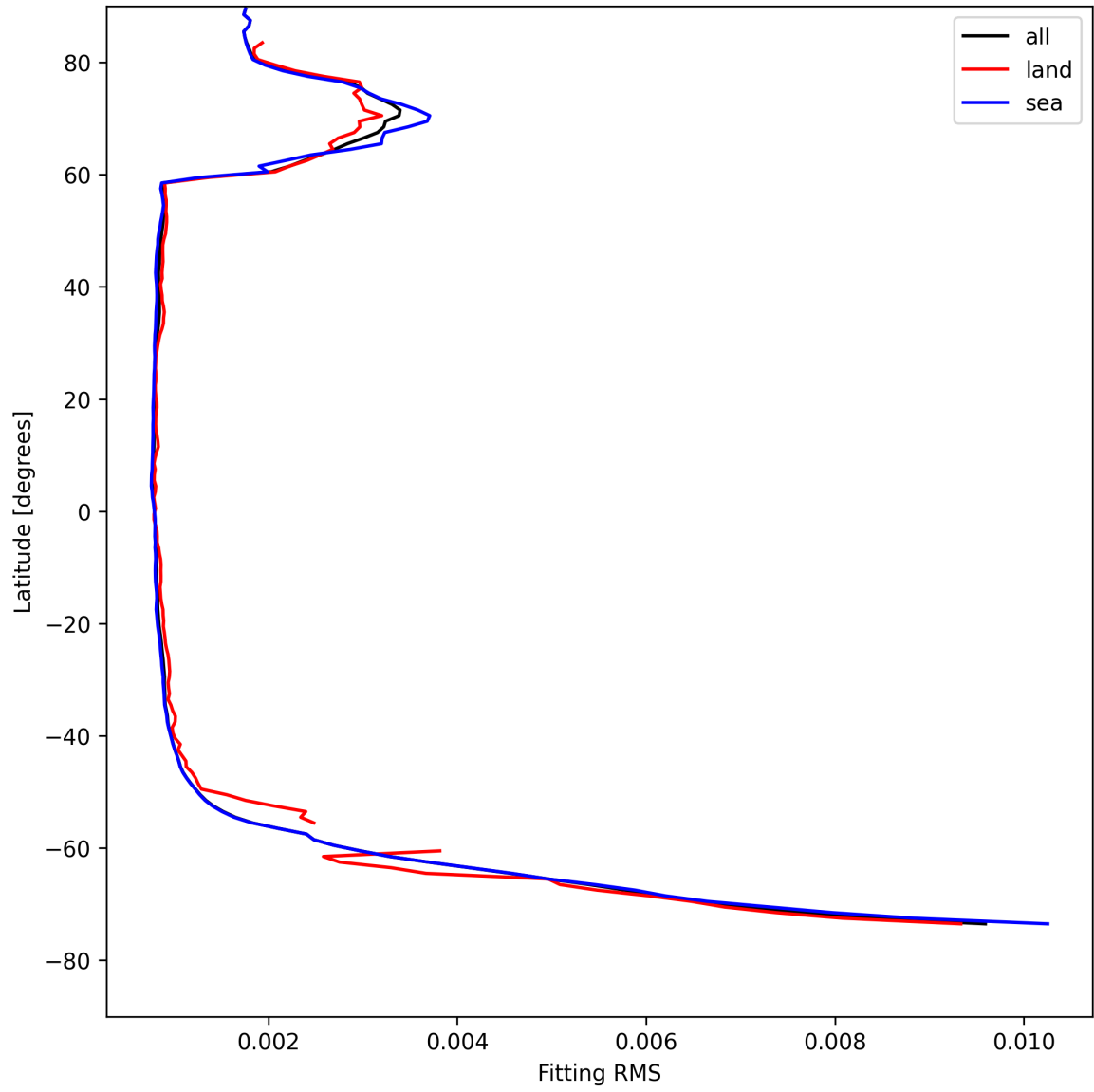
Figure 22: Zonal average of “Fitting RMS” for 2025-04-30 to 2025-05-01.
