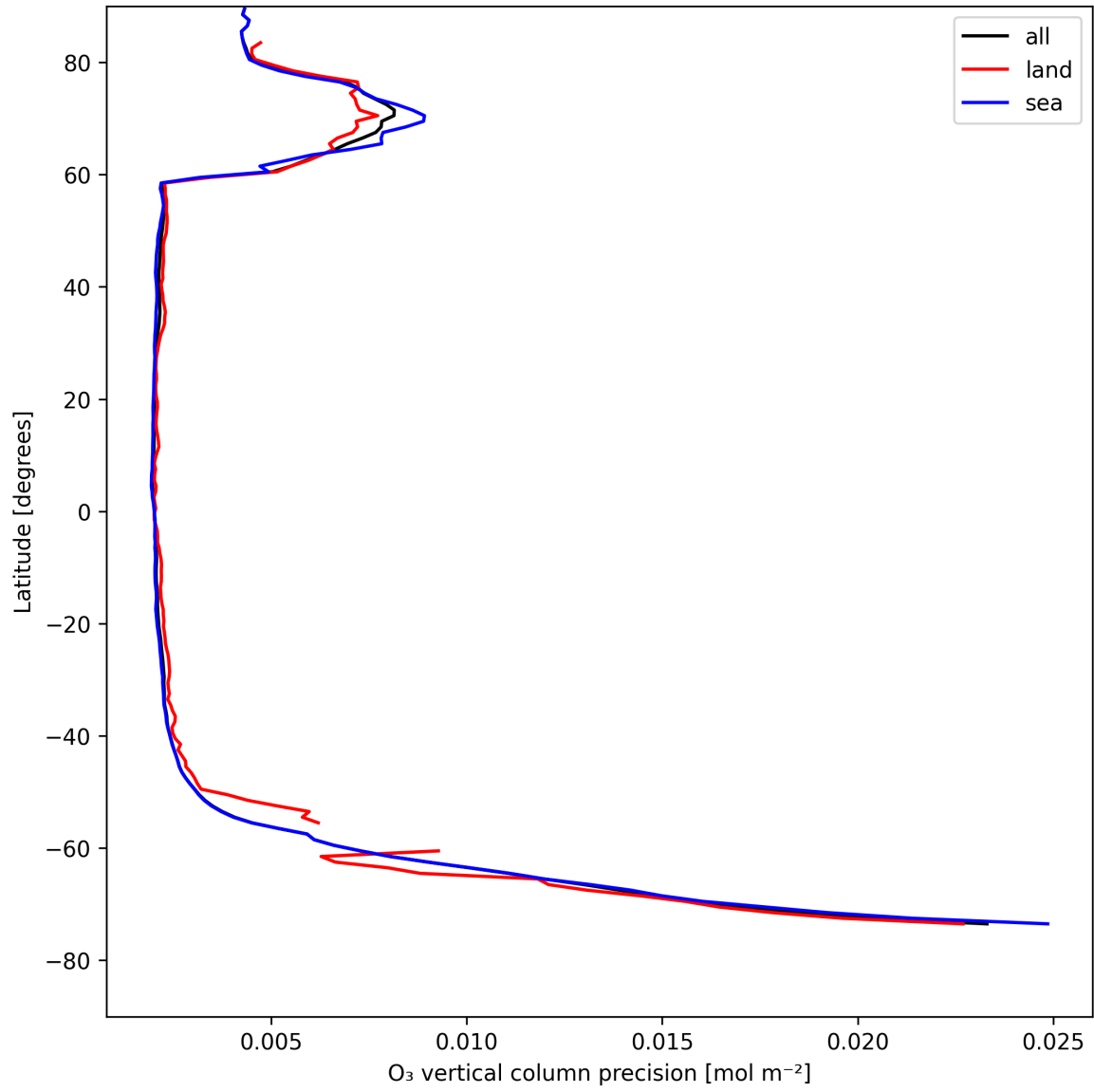
Figure 18: Zonal average of “O 3 vertical column precision” for 2025-04-30 to 2025-05-01.
