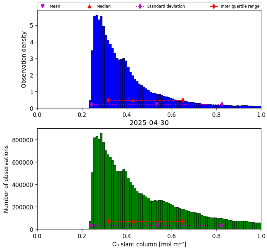
Figure 31: Histogram of “O 3 slant column” for 2025-04-30 to 2025-05-01
