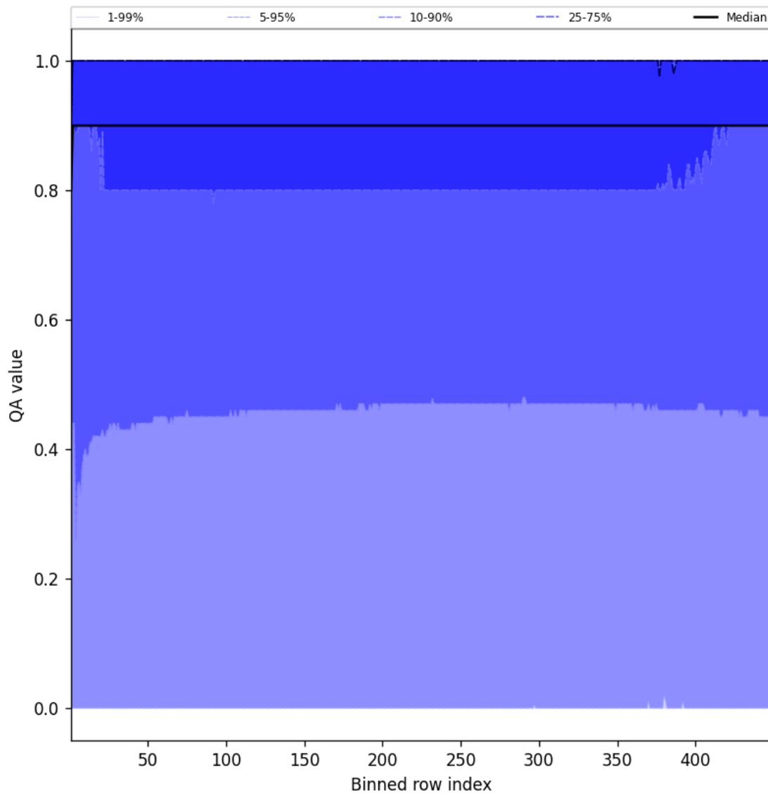
Figure 40: Along track statistics of “QA value” for 2025-04-30 to 2025-05-01
