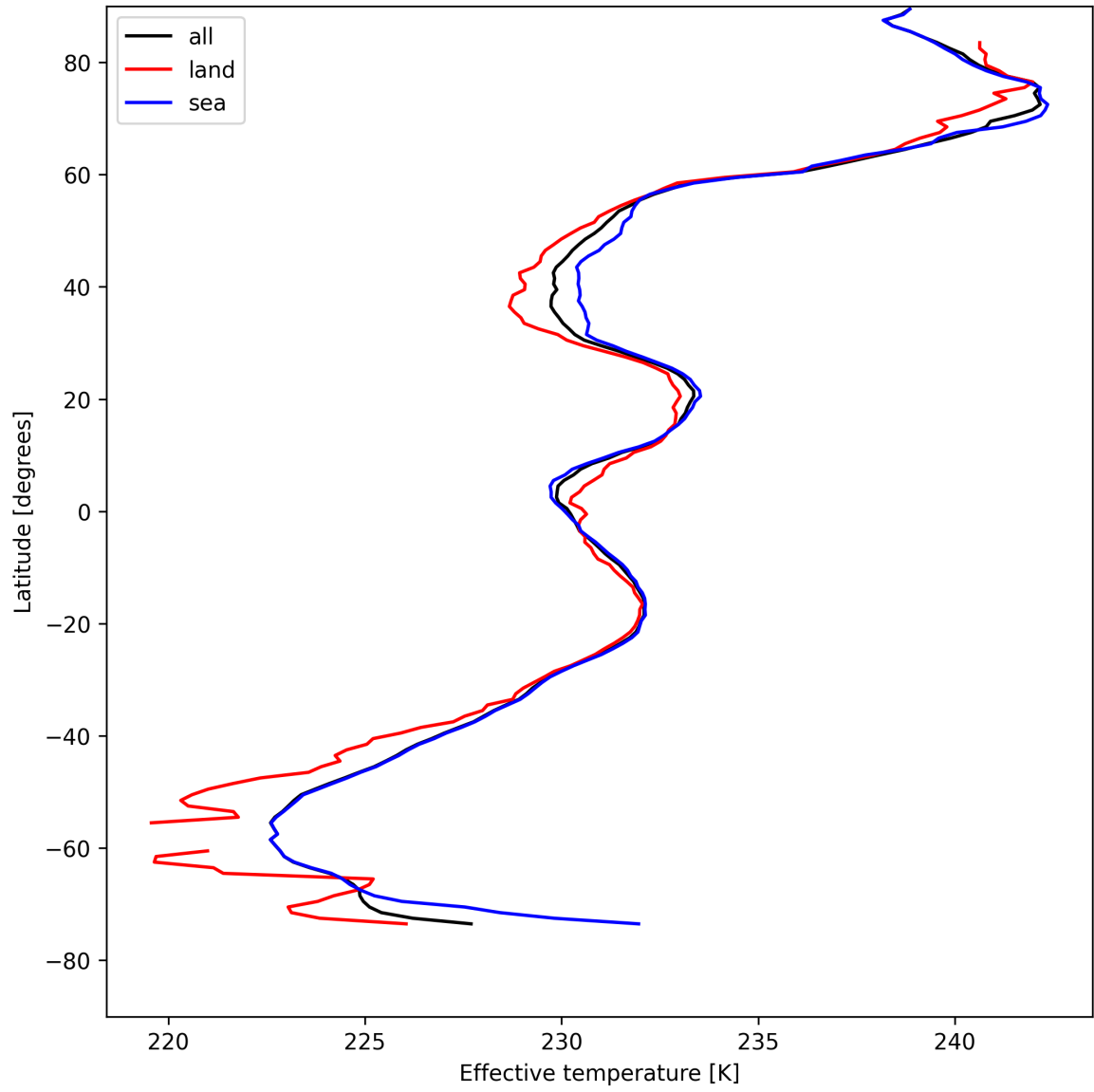
Figure 26: Zonal average of “Effective temperature” for 2025-04-30 to 2025-05-01.
