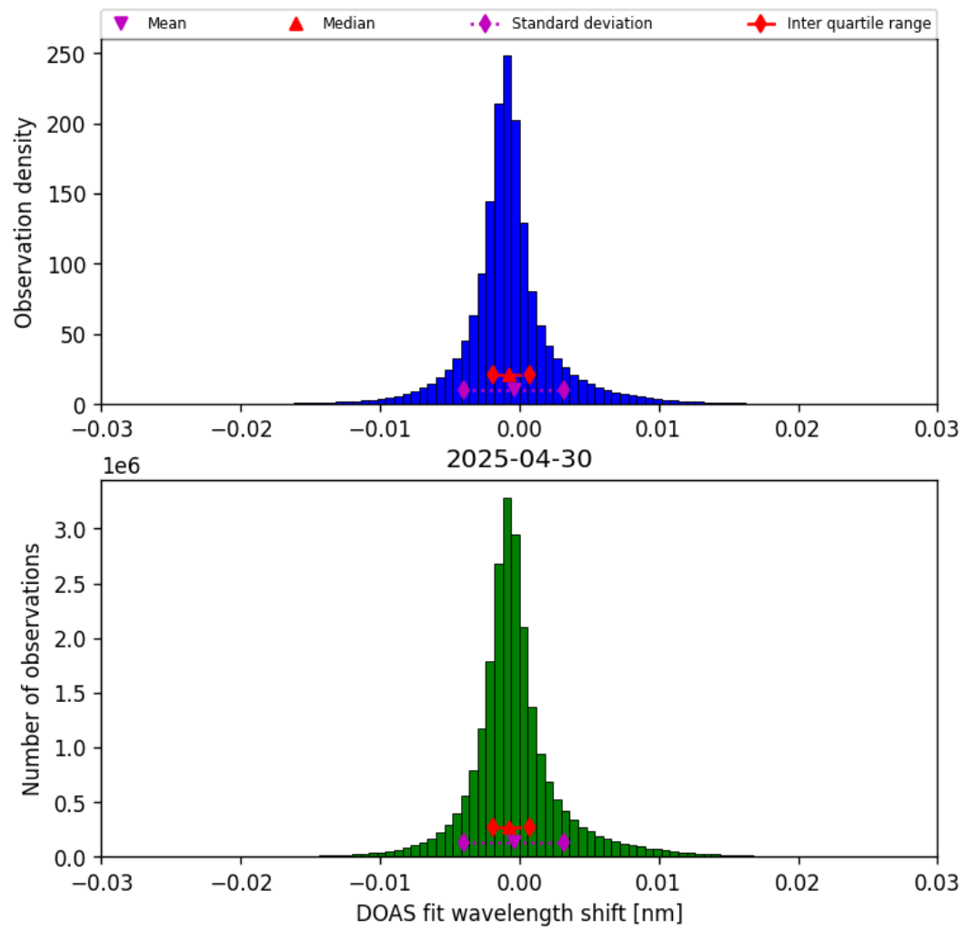
Figure 35: Histogram of “DOAS fit wavelength shift” for 2025-04-30 to 2025-05-01
