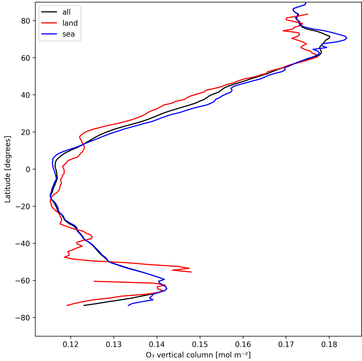
Figure 17: Zonal average of “O 3 vertical column” for 2025-04-30 to 2025-05-01.
