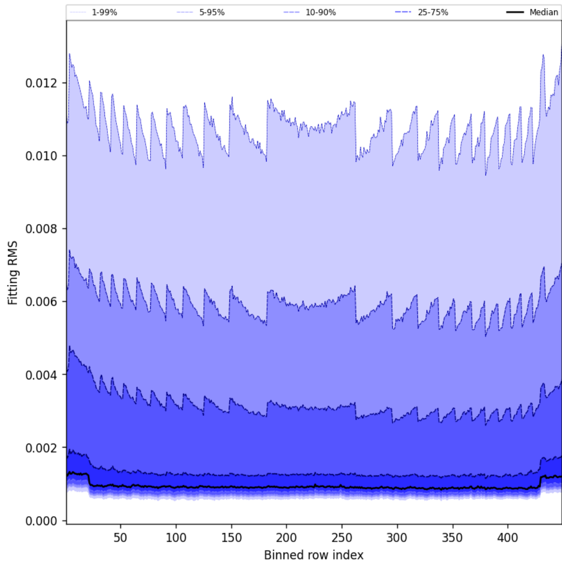
Figure 46: Along track statistics of “Fitting RMS” for 2025-04-30 to 2025-05-01
