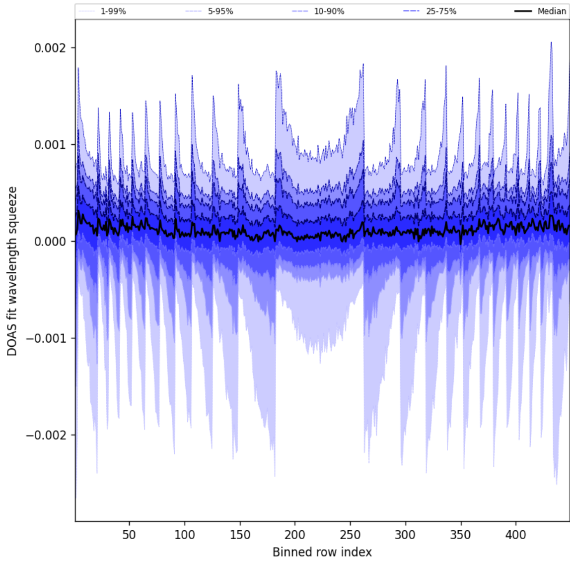
Figure 48: Along track statistics of “DOAS fit wavelength squeeze” for 2025-04-30 to 2025-05-01
