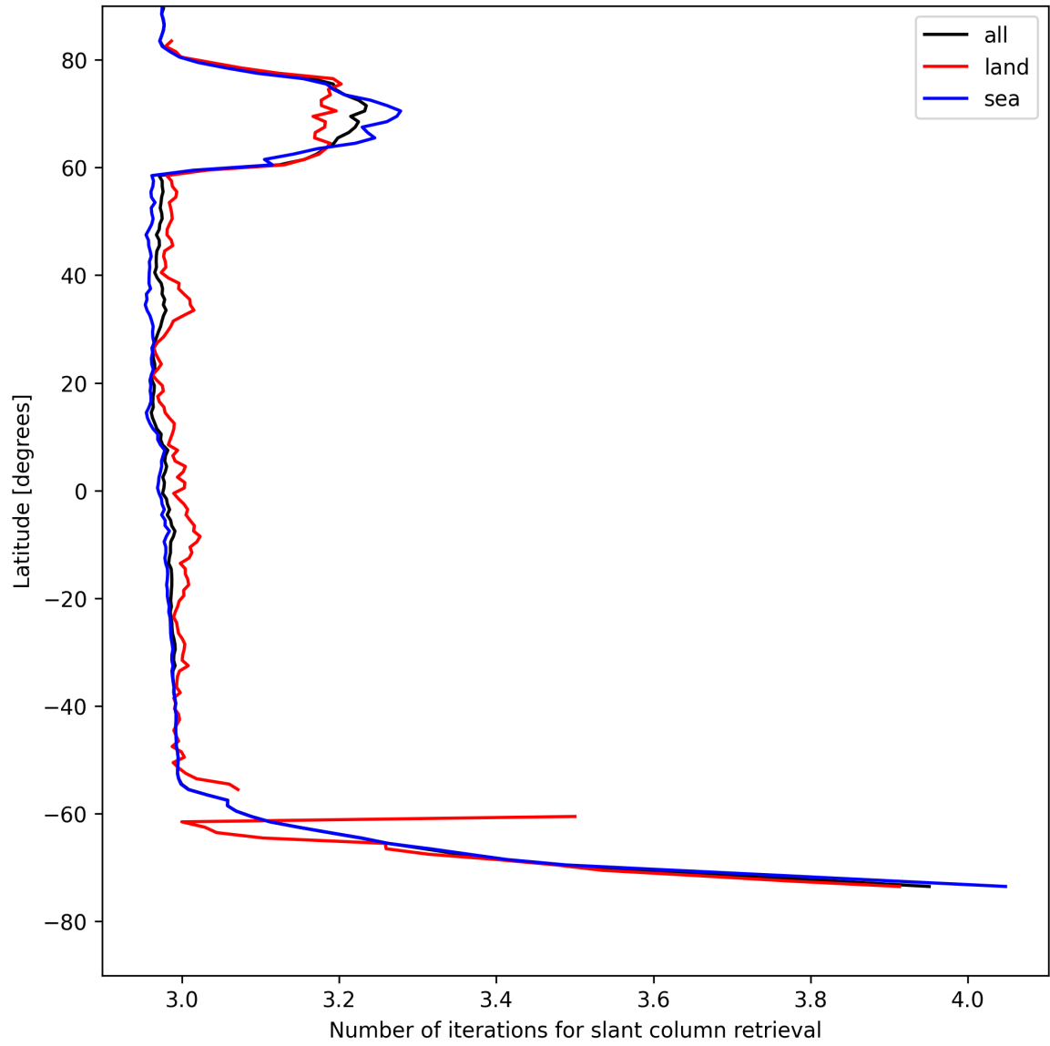
Figure 21: Zonal average of “Number of iterations for slant column retrieval” for 2025-04-30 to 2025-05-01.
