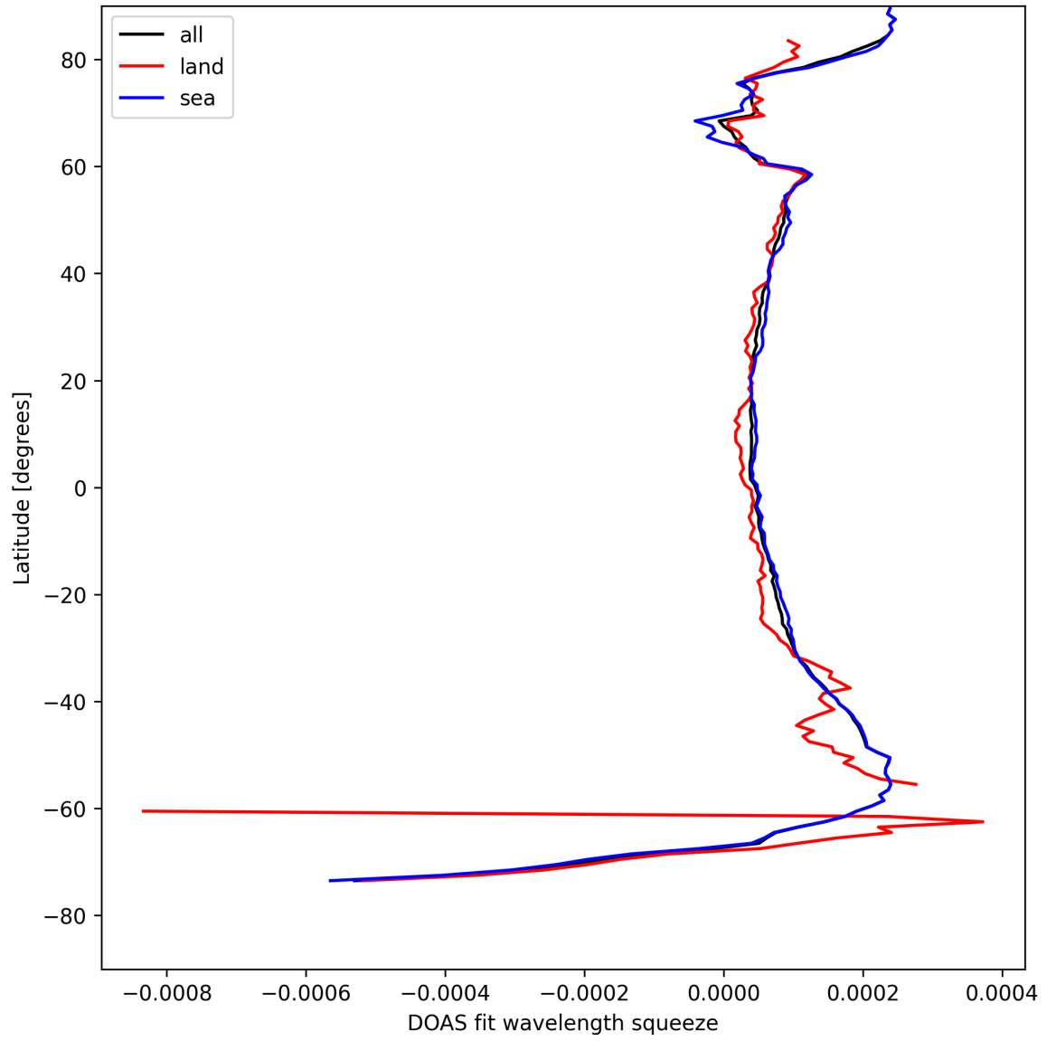
Figure 24: Zonal average of “DOAS fit wavelength squeeze” for 2025-04-30 to 2025-05-01.
