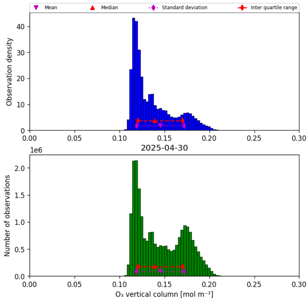
Figure 29: Histogram of “O 3 vertical column” for 2025-04-30 to 2025-05-01
