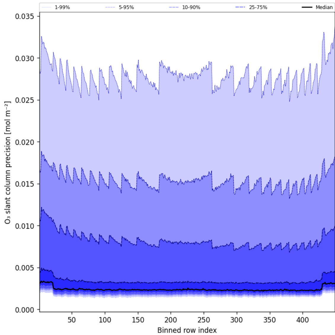
Figure 44: Along track statistics of “O 3 slant column precision” for 2025-04-30 to 2025-05-01
