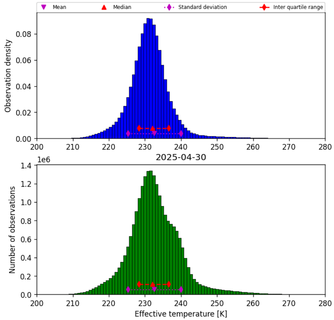
Figure 38: Histogram of “Effective temperature” for 2025-04-30 to 2025-05-01
