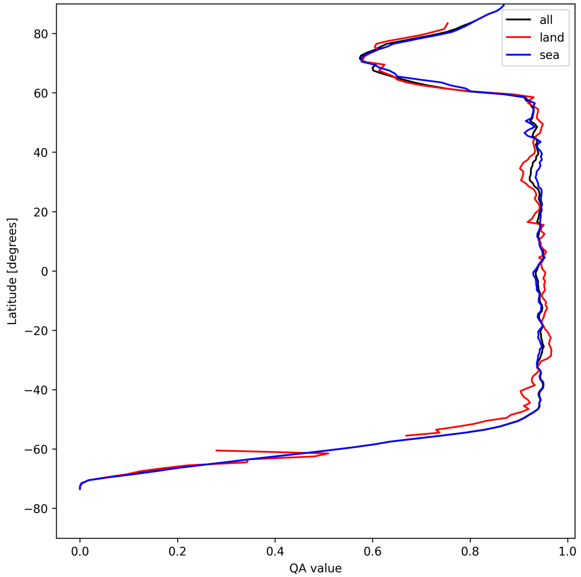
Figure 16: Zonal average of “QA value” for 2025-04-30 to 2025-05-01.
