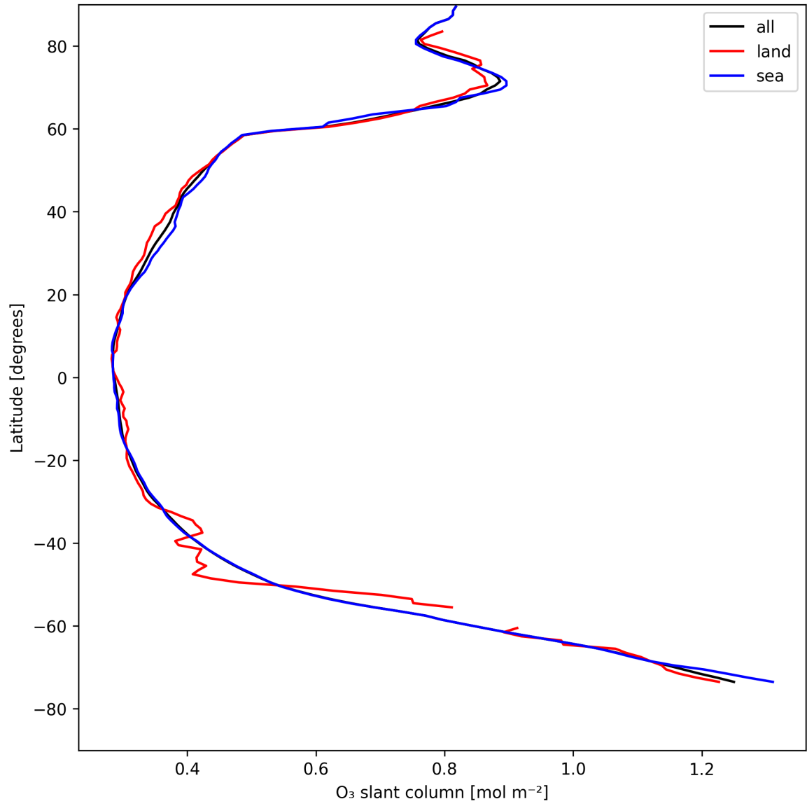
Figure 19: Zonal average of “O 3 slant column” for 2025-04-30 to 2025-05-01.
