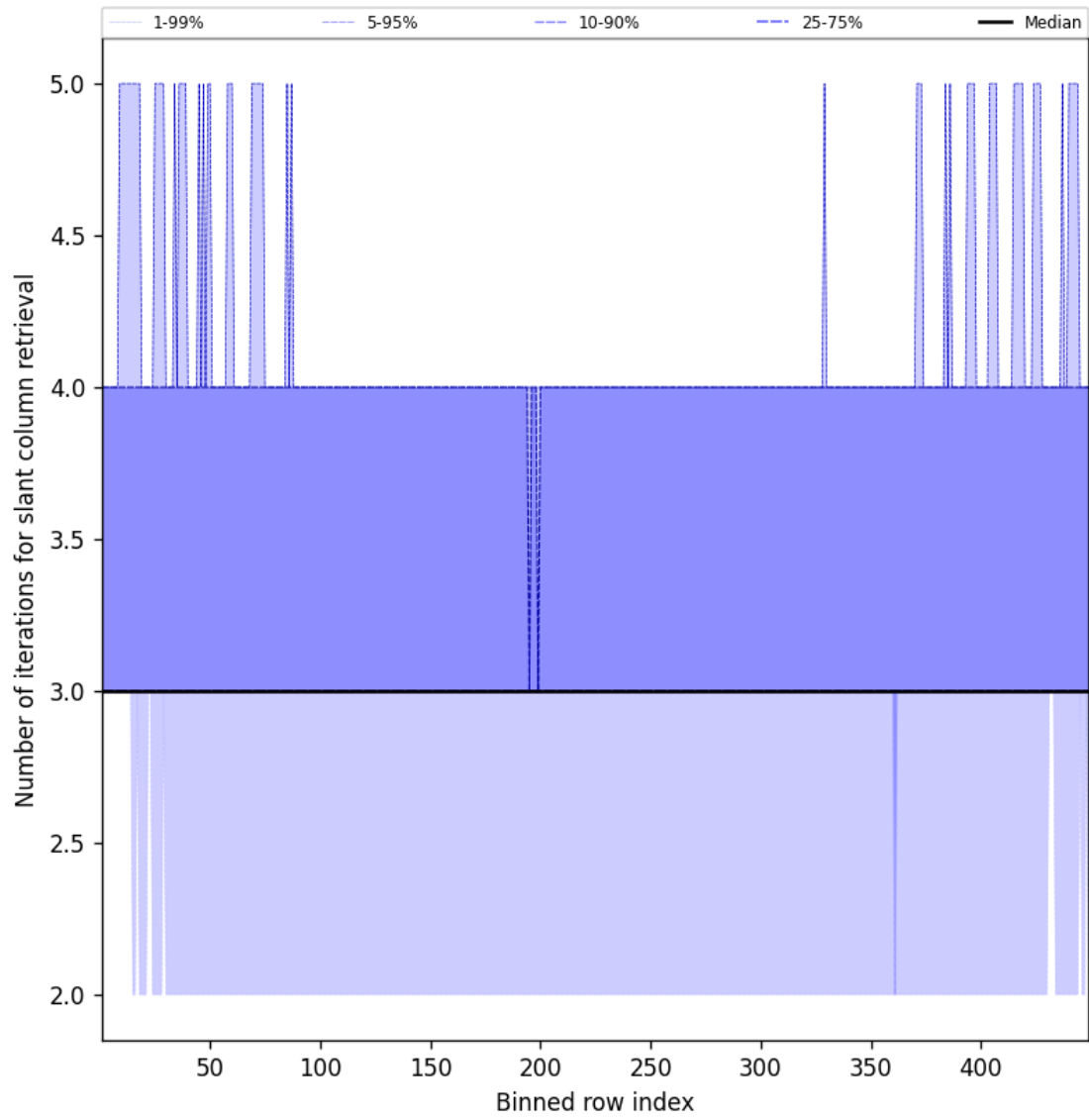
Figure 45: Along track statistics of “Number of iterations for slant column retrieval” for 2025-04-30 to 2025-05-01
