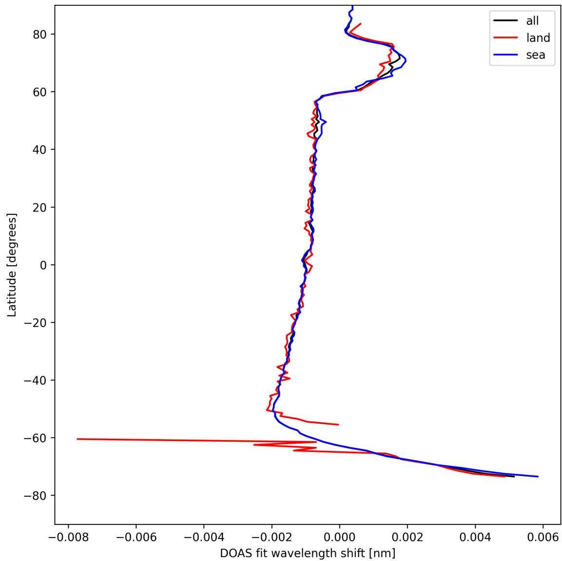
Figure 23: Zonal average of “DOAS fit wavelength shift” for 2025-04-30 to 2025-05-01.
