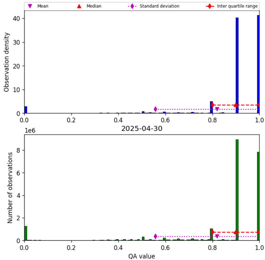
Figure 28: Histogram of “QA value” for 2025-04-30 to 2025-05-01
