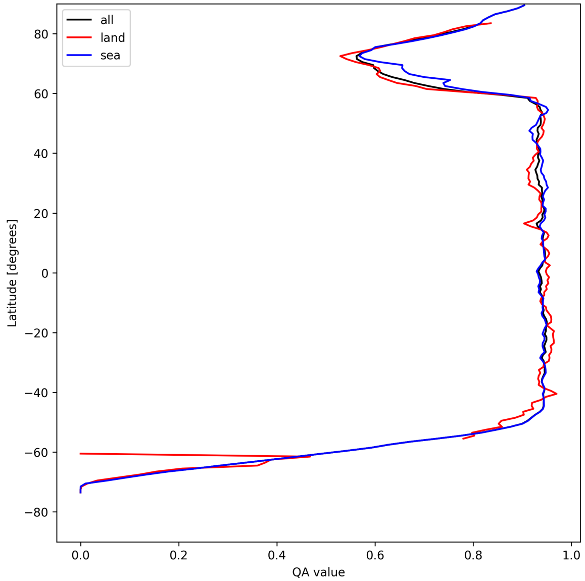
Figure 16: Zonal average of “QA value” for 2025-05-01 to 2025-05-02.
