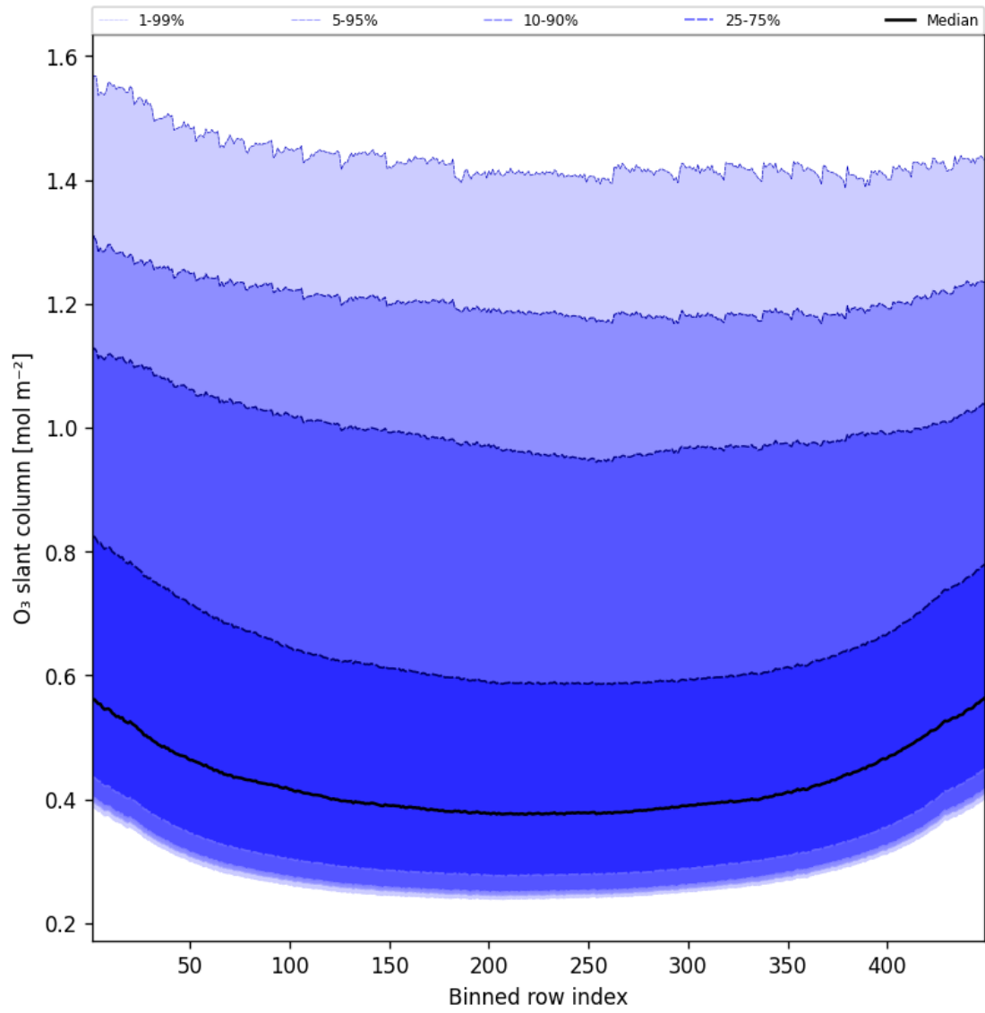
Figure 43: Along track statistics of “O 3 slant column” for 2025-05-01 to 2025-05-02
