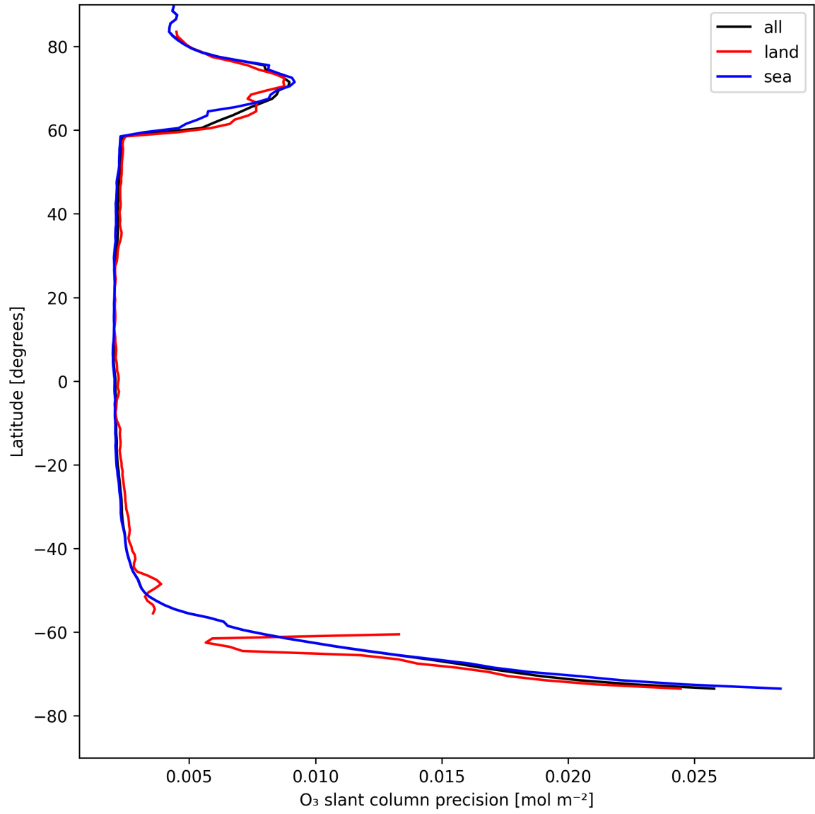
Figure 20: Zonal average of “O 3 slant column precision” for 2025-05-01 to 2025-05-02.
