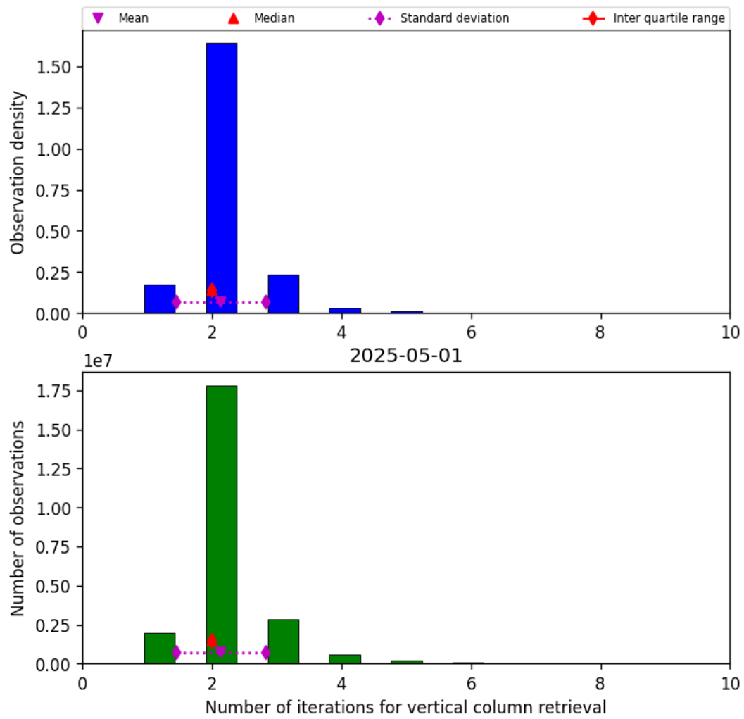
Figure 39: Histogram of “Number of iterations for vertical column retrieval” for 2025-05-01 to 2025-05-02
