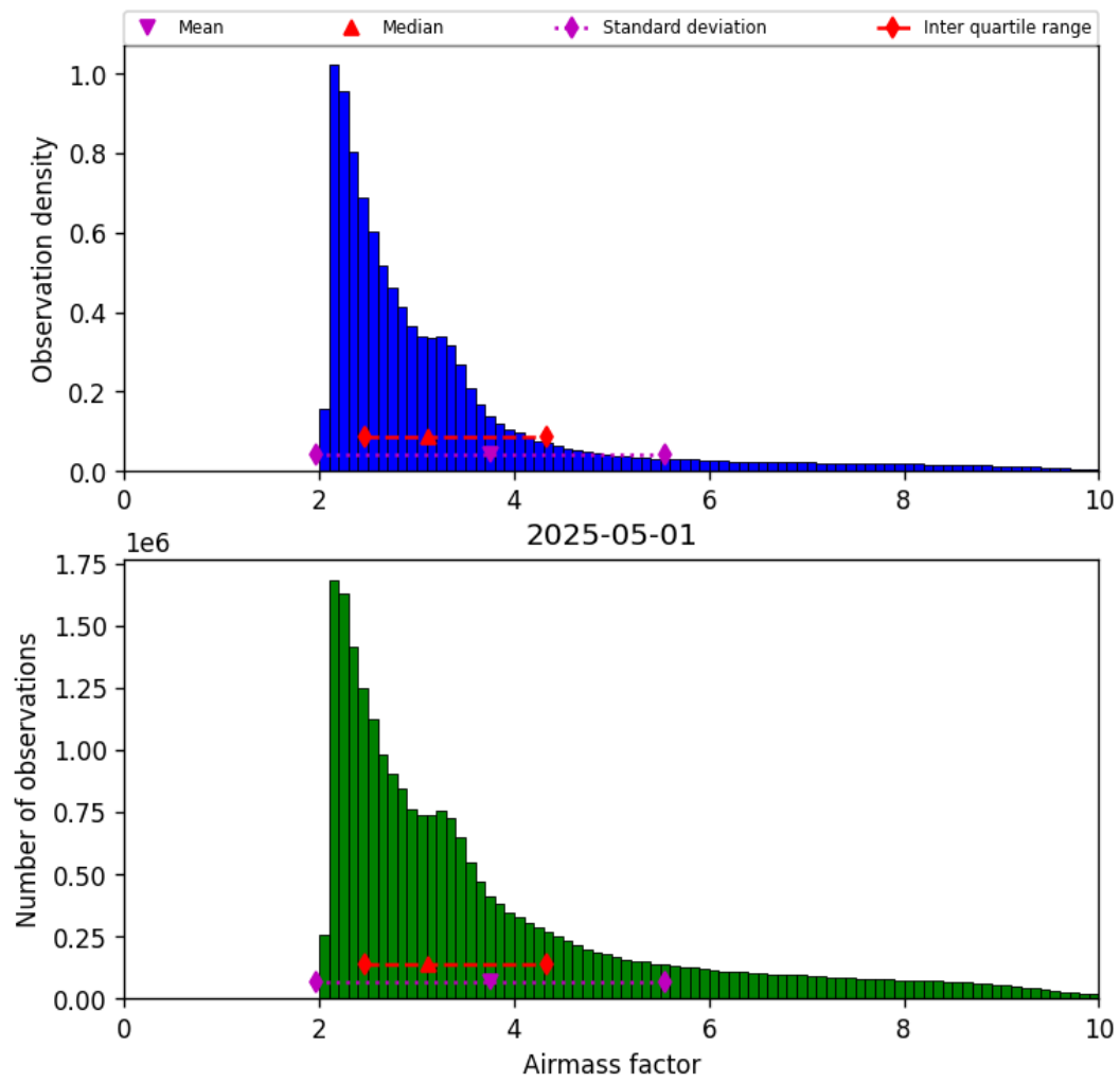
Figure 37: Histogram of “Airmass factor” for 2025-05-01 to 2025-05-02
