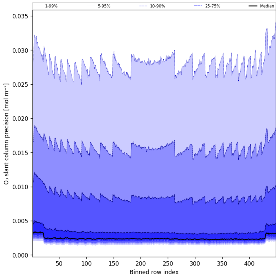
Figure 44: Along track statistics of “O 3 slant column precision” for 2025-05-01 to 2025-05-02
