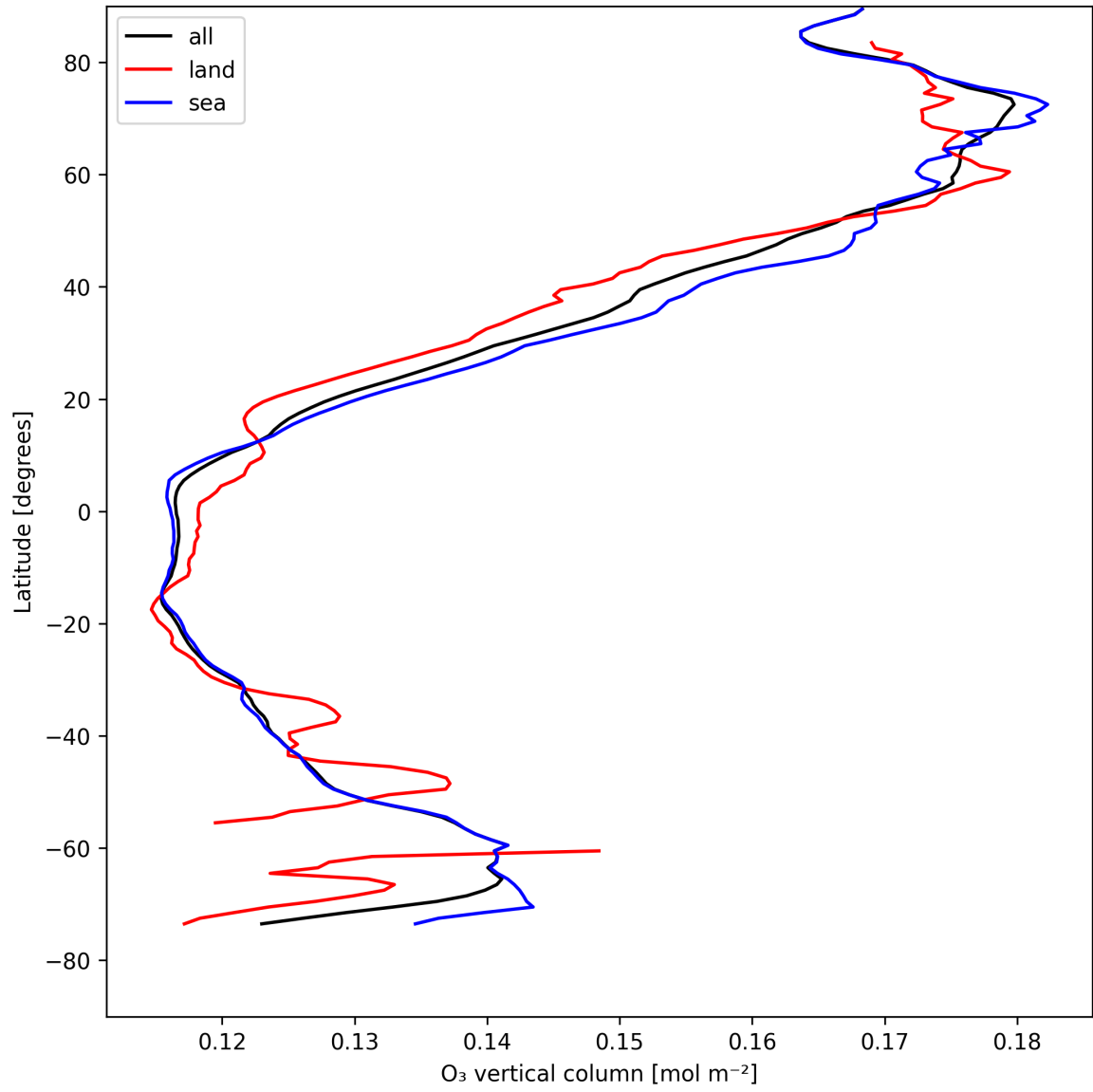
Figure 17: Zonal average of “O 3 vertical column” for 2025-05-01 to 2025-05-02.
