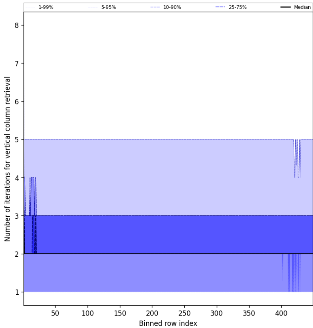
Figure 51: Along track statistics of “Number of iterations for vertical column retrieval” for 2025-05-01 to 2025-05-02
