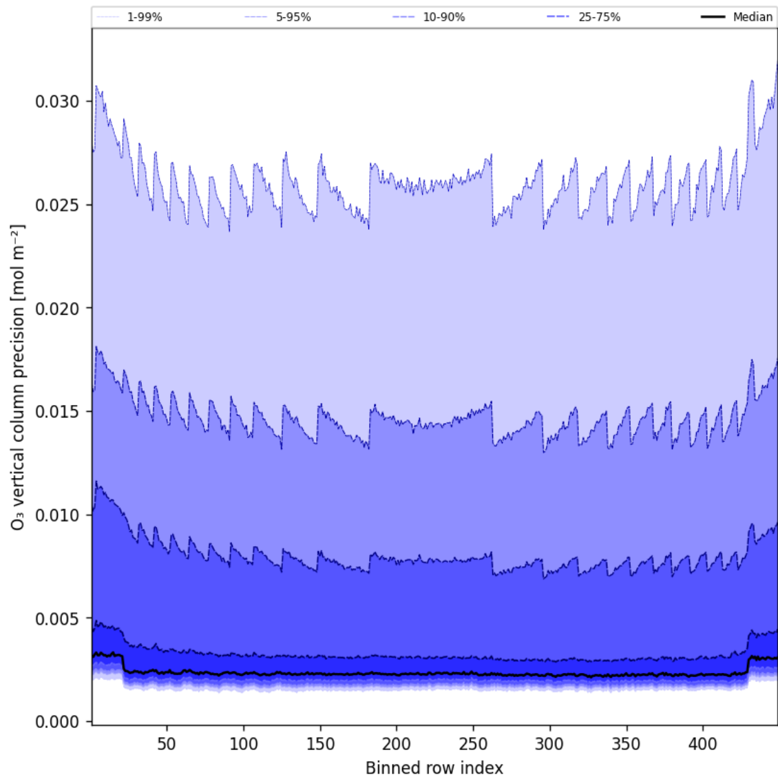
Figure 42: Along track statistics of “O 3 vertical column precision” for 2025-05-01 to 2025-05-02
