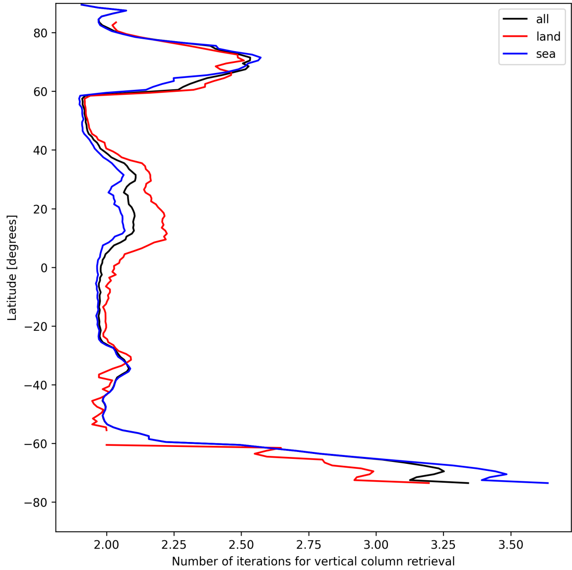
Figure 27: Zonal average of “Number of iterations for vertical column retrieval” for 2025-05-01 to 2025-05-02.
