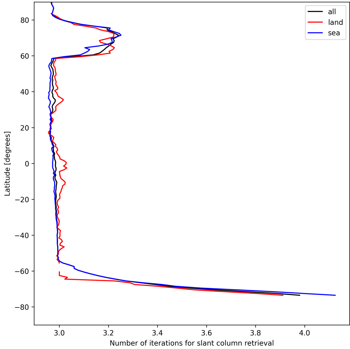
Figure 21: Zonal average of “Number of iterations for slant column retrieval” for 2025-05-01 to 2025-05-02.
