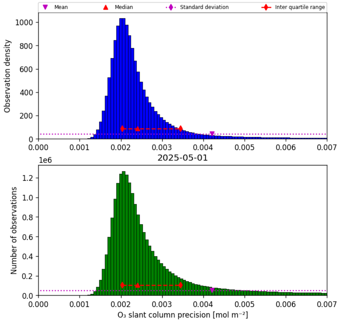
Figure 32: Histogram of “O 3 slant column precision” for 2025-05-01 to 2025-05-02
