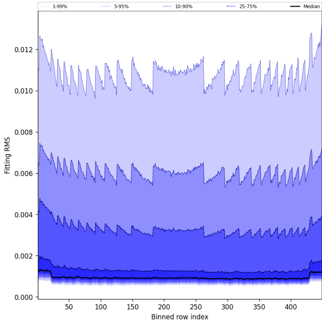
Figure 46: Along track statistics of “Fitting RMS” for 2025-05-01 to 2025-05-02
