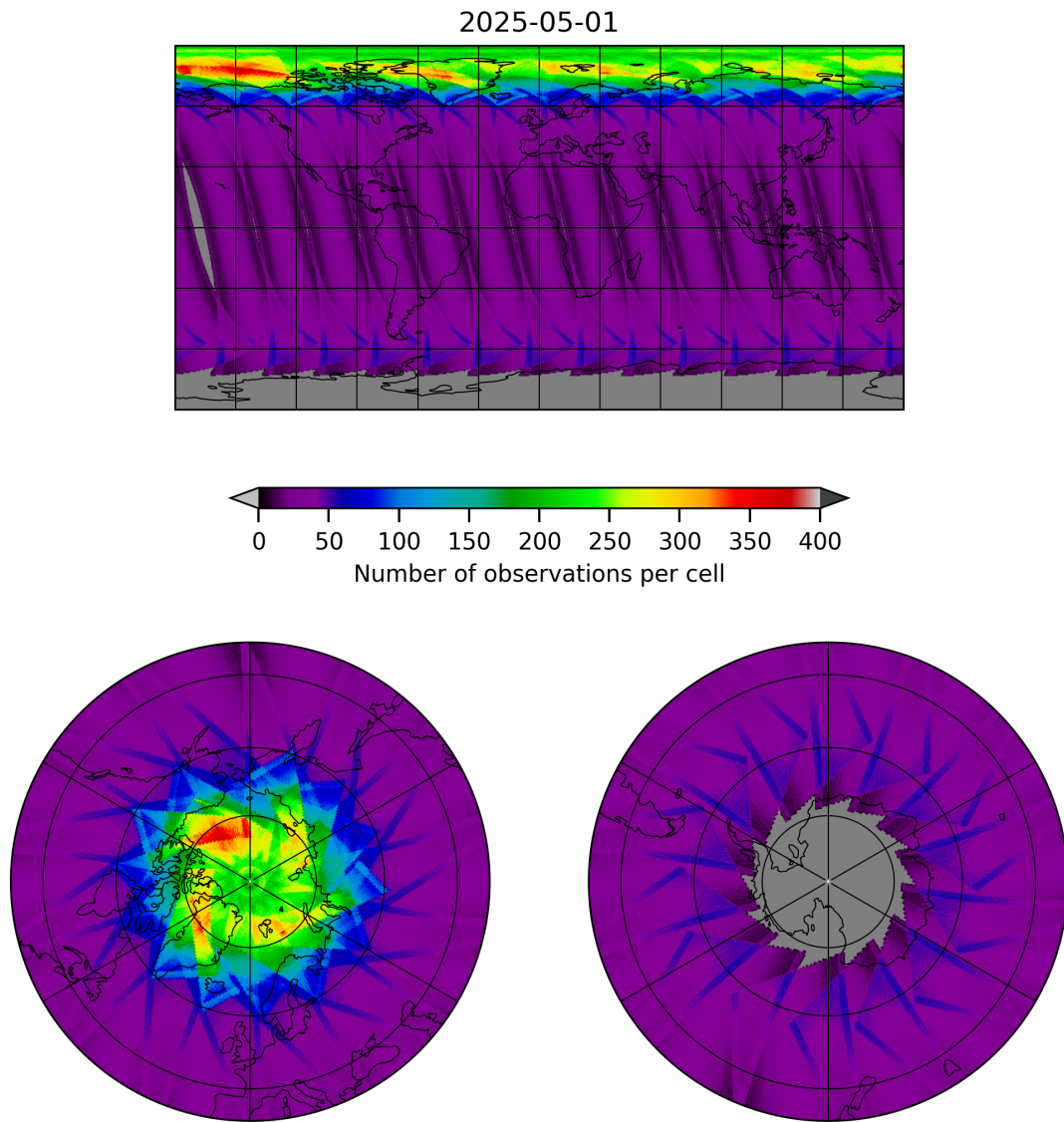
Figure 15: Map of the number of observations for 2025-05-01 to 2025-05-02
