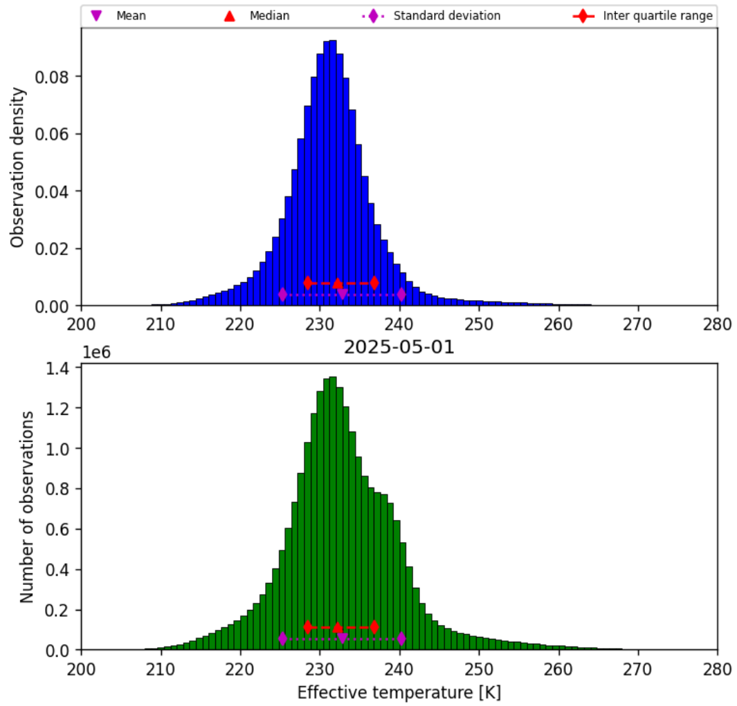
Figure 38: Histogram of “Effective temperature” for 2025-05-01 to 2025-05-02
