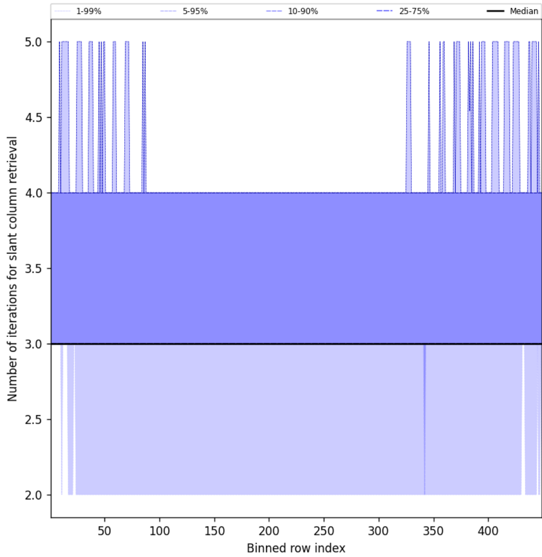
Figure 45: Along track statistics of “Number of iterations for slant column retrieval” for 2025-05-01 to 2025-05-02
