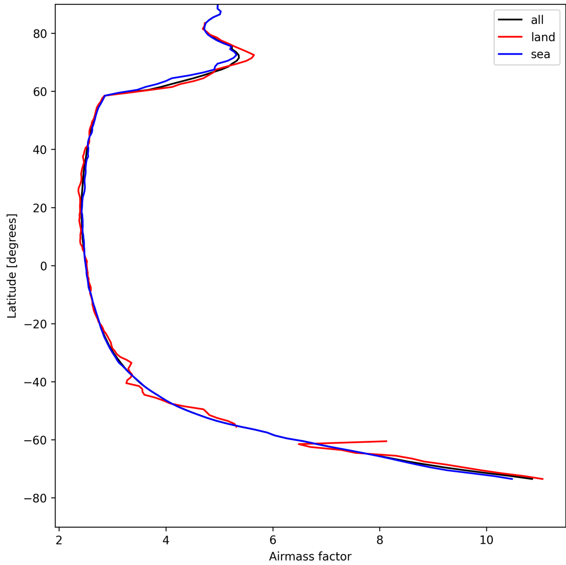
Figure 25: Zonal average of “Airmass factor” for 2025-05-01 to 2025-05-02.
