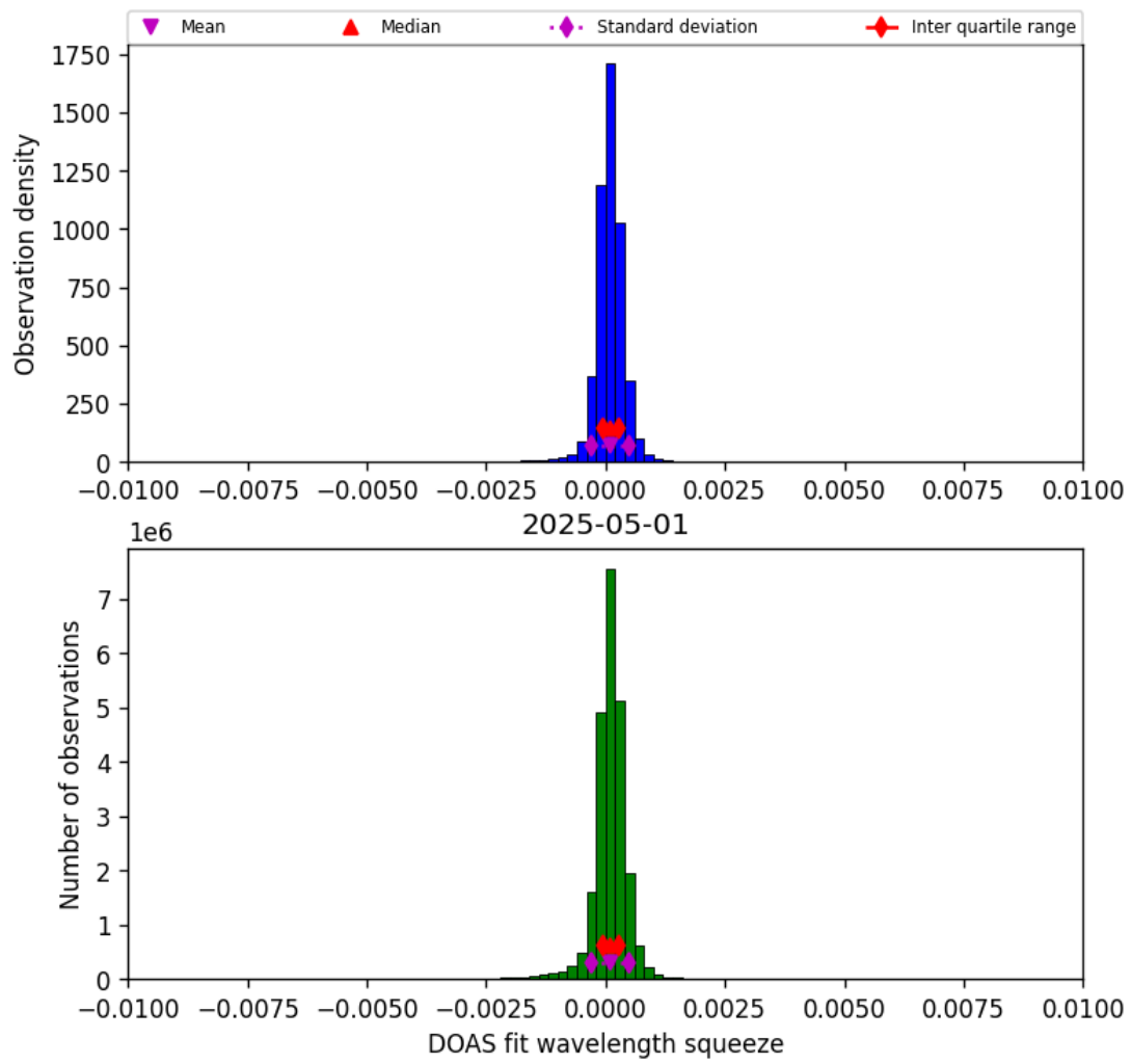
Figure 36: Histogram of “DOAS fit wavelength squeeze” for 2025-05-01 to 2025-05-02
