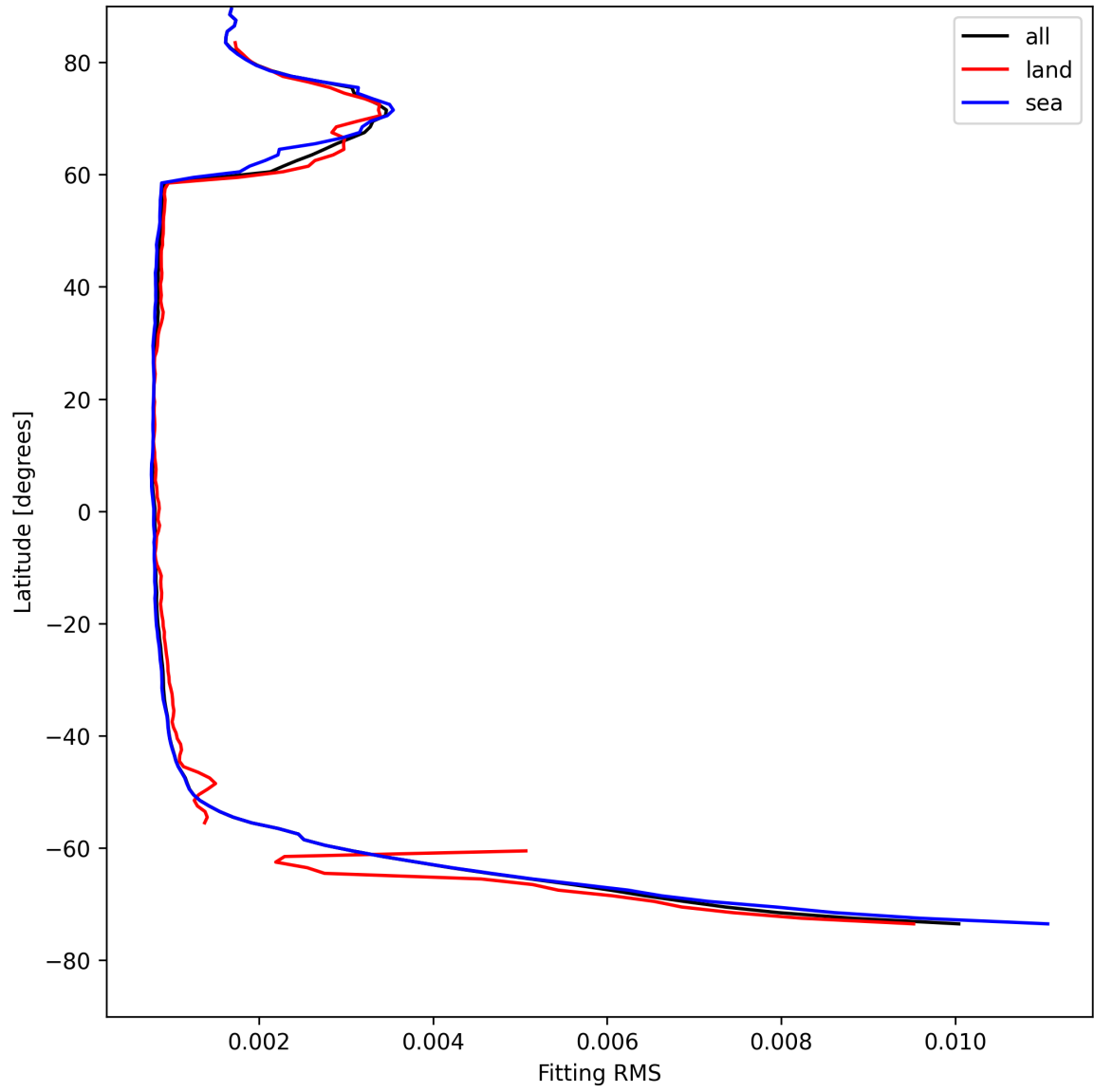
Figure 22: Zonal average of “Fitting RMS” for 2025-05-01 to 2025-05-02.
