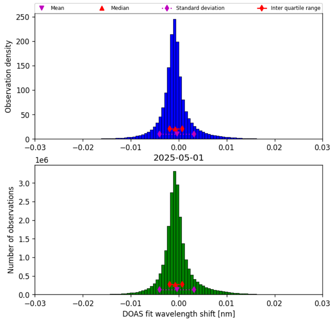
Figure 35: Histogram of “DOAS fit wavelength shift” for 2025-05-01 to 2025-05-02
