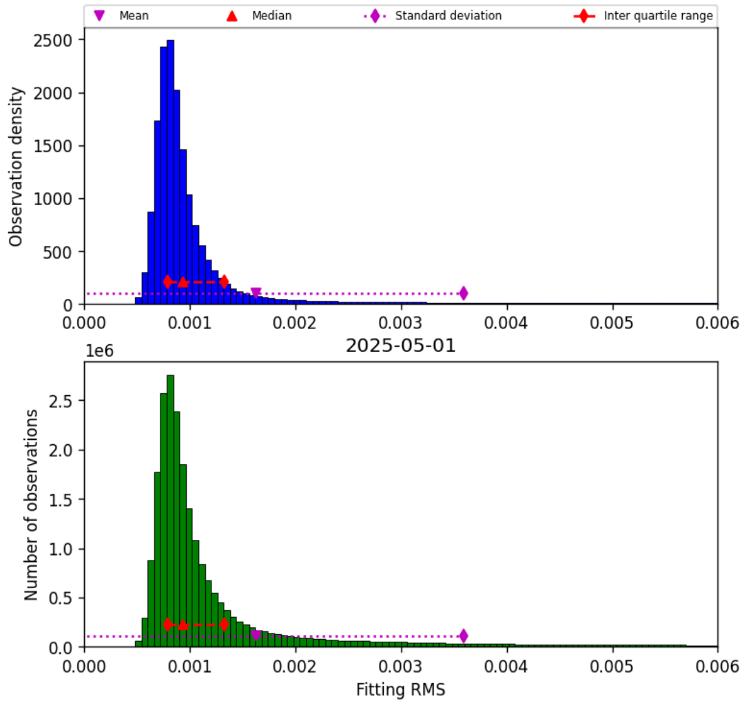
Figure 34: Histogram of “Fitting RMS” for 2025-05-01 to 2025-05-02
