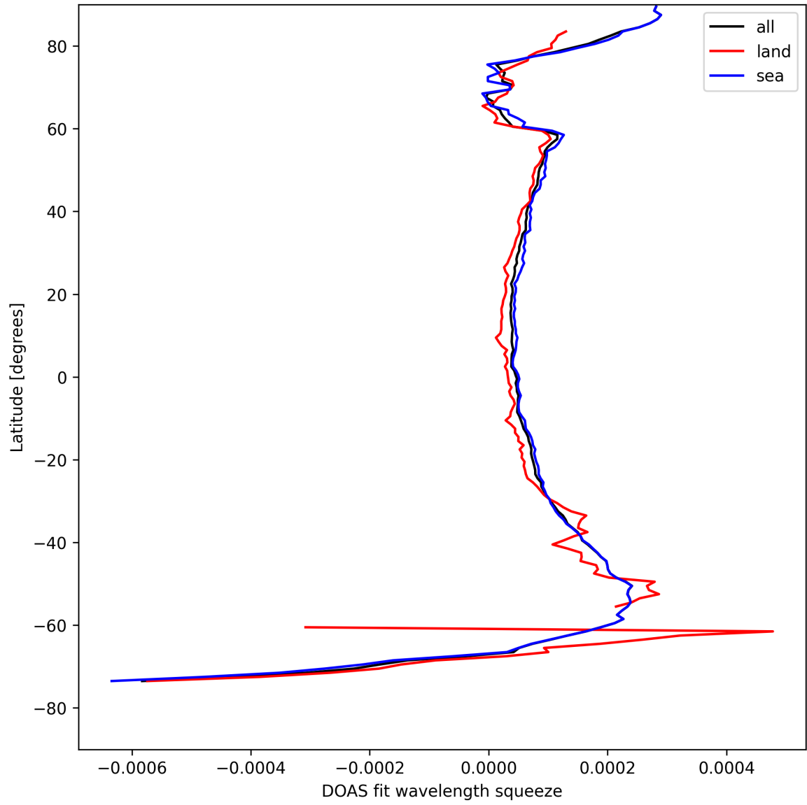
Figure 24: Zonal average of “DOAS fit wavelength squeeze” for 2025-05-01 to 2025-05-02.
