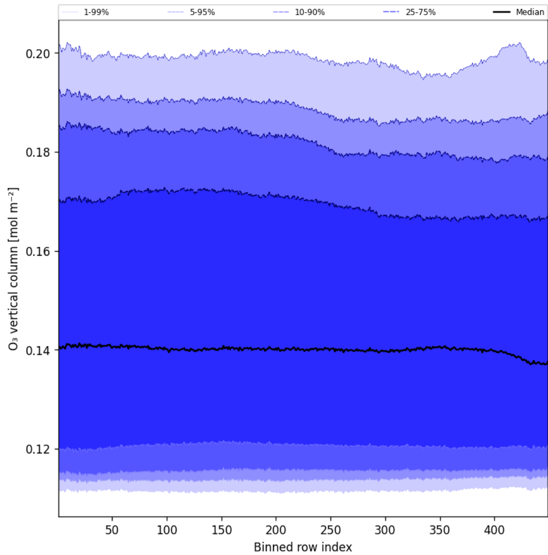
Figure 41: Along track statistics of “O 3 vertical column” for 2025-05-01 to 2025-05-02
