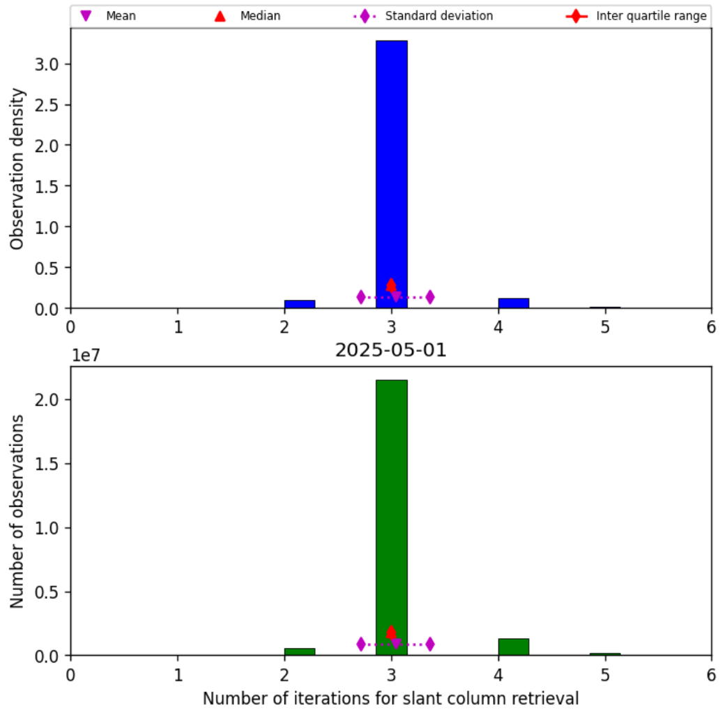
Figure 33: Histogram of “Number of iterations for slant column retrieval” for 2025-05-01 to 2025-05-02
