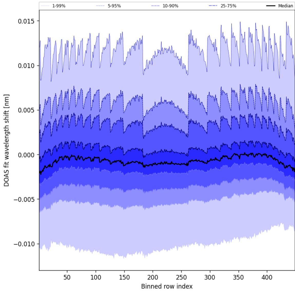
Figure 47: Along track statistics of “DOAS fit wavelength shift” for 2025-05-01 to 2025-05-02
