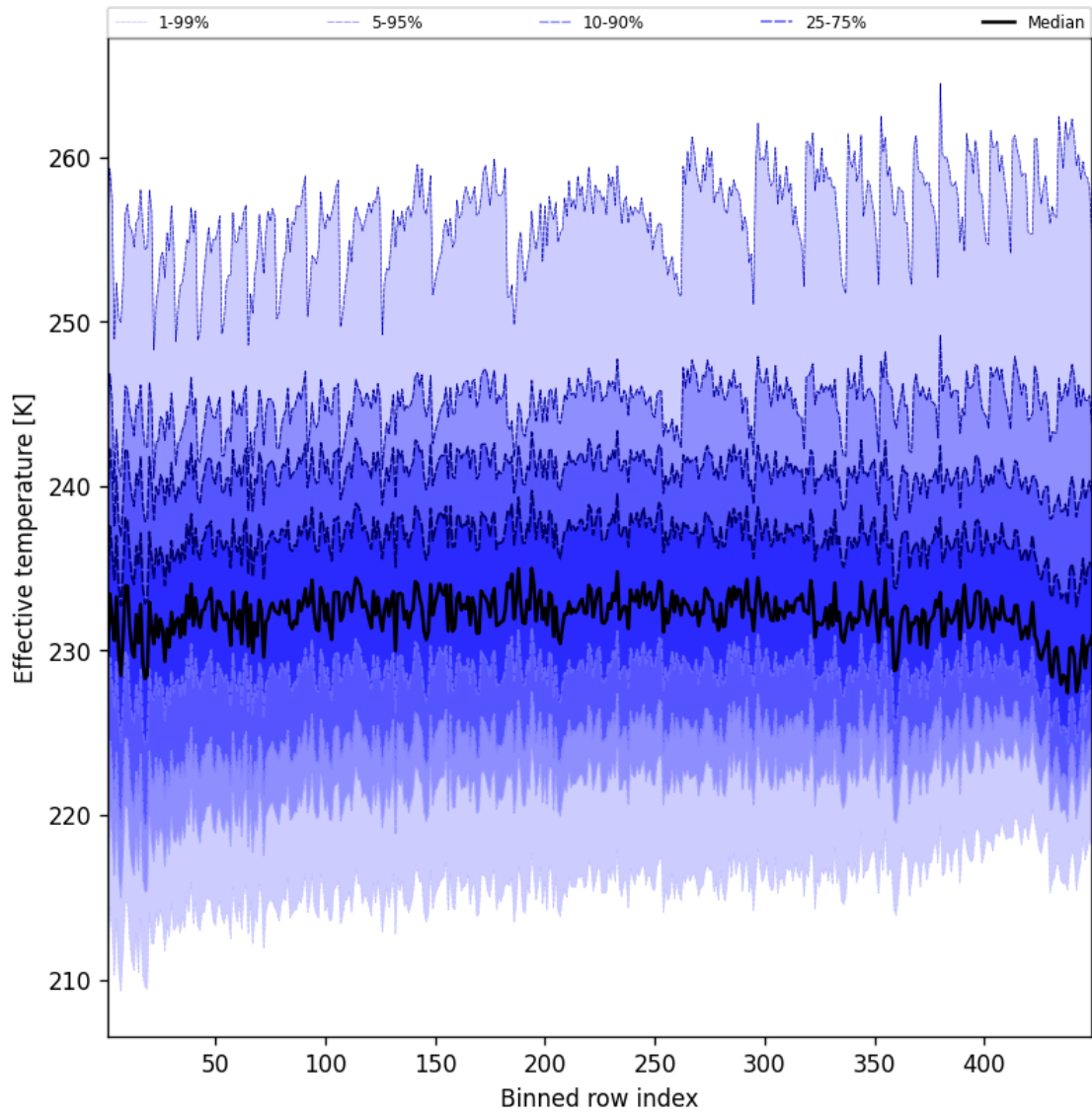
Figure 50: Along track statistics of “Effective temperature” for 2025-05-01 to 2025-05-02
