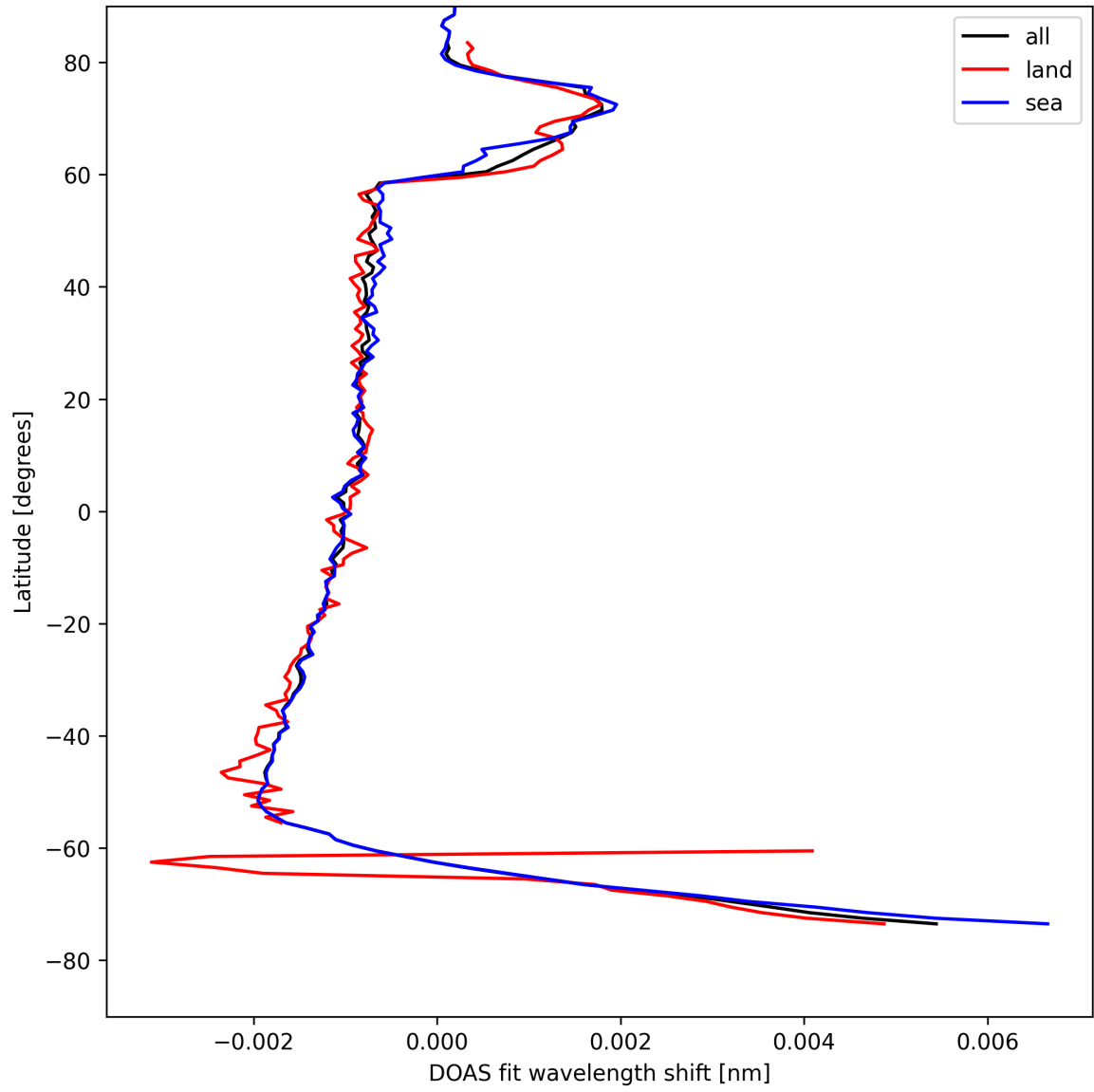
Figure 23: Zonal average of “DOAS fit wavelength shift” for 2025-05-01 to 2025-05-02.
