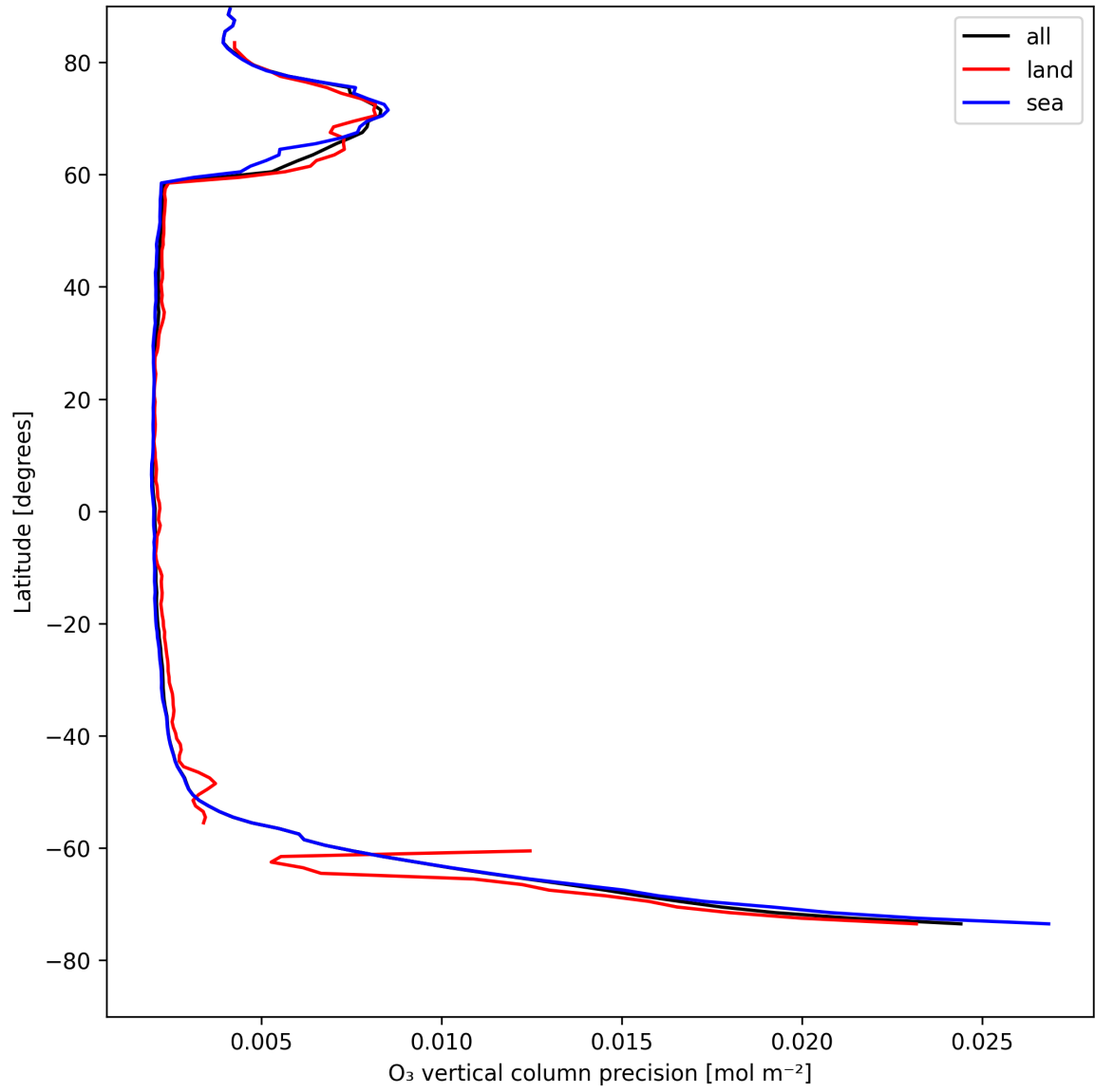
Figure 18: Zonal average of “O 3 vertical column precision” for 2025-05-01 to 2025-05-02.
