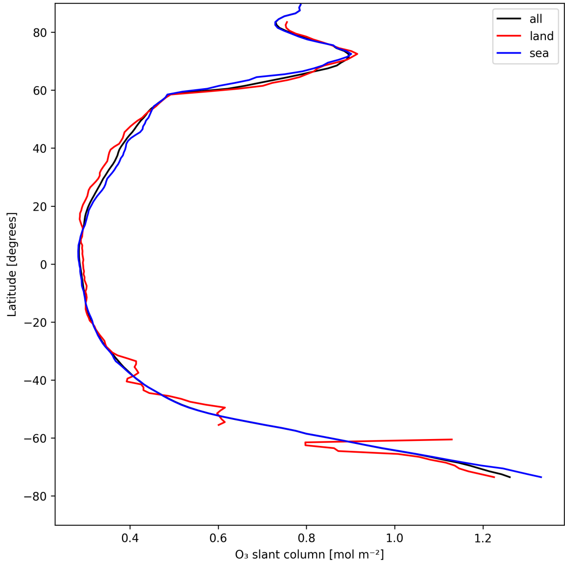
Figure 19: Zonal average of “O 3 slant column” for 2025-05-01 to 2025-05-02.
