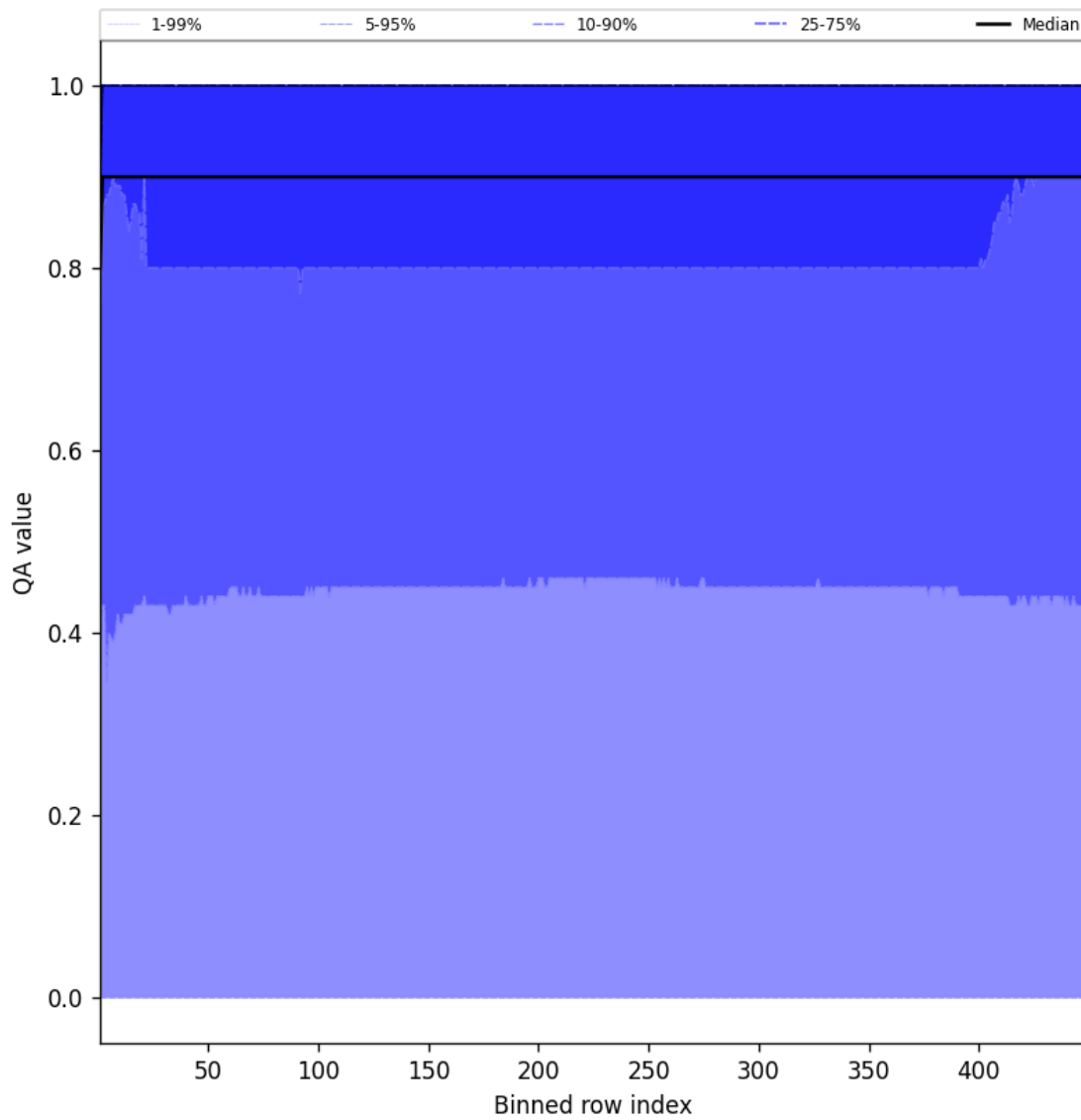
Figure 40: Along track statistics of “QA value” for 2025-05-01 to 2025-05-02
