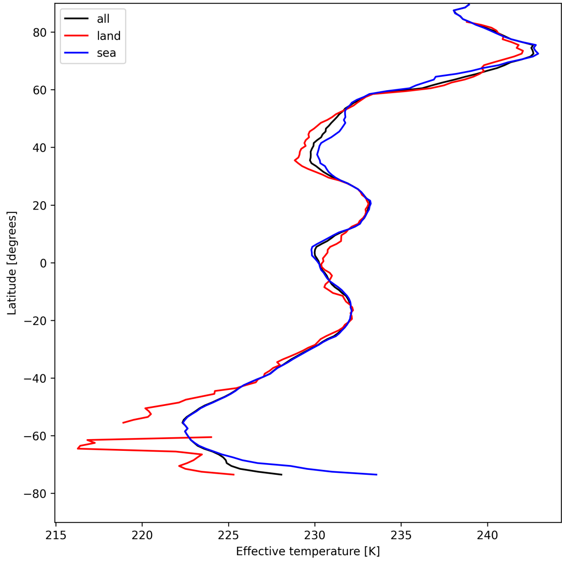
Figure 26: Zonal average of "Effective temperature" for 2025-05-01 to 2025-05-02.
