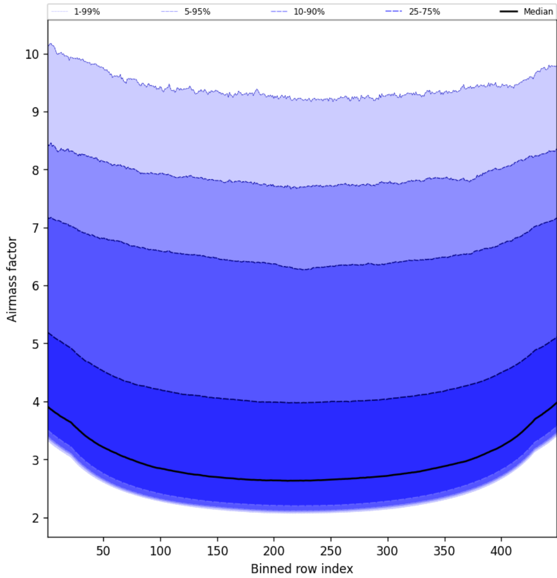
Figure 49: Along track statistics of “Airmass factor” for 2025-05-01 to 2025-05-02
