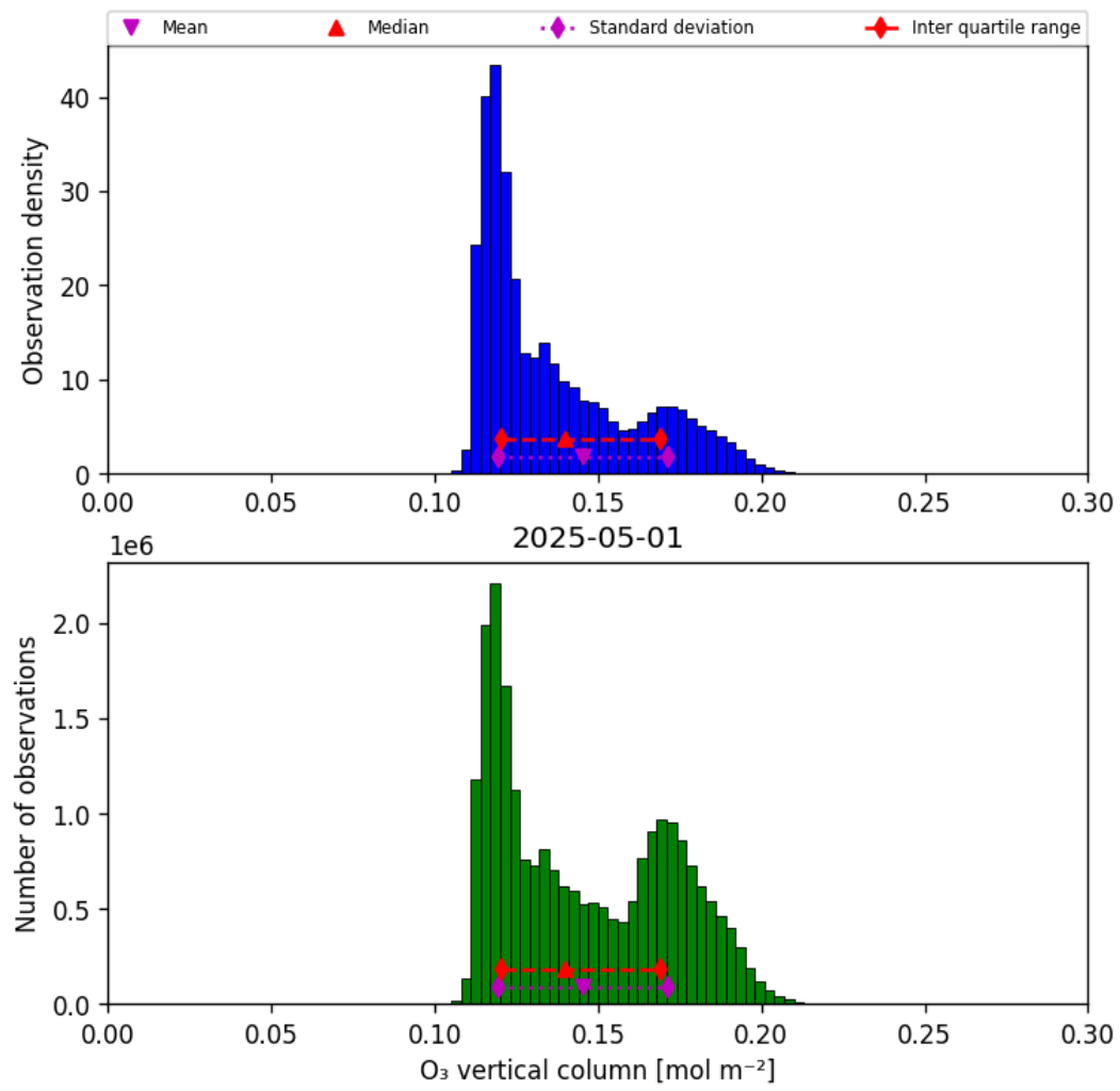
Figure 29: Histogram of “O 3 vertical column” for 2025-05-01 to 2025-05-02
