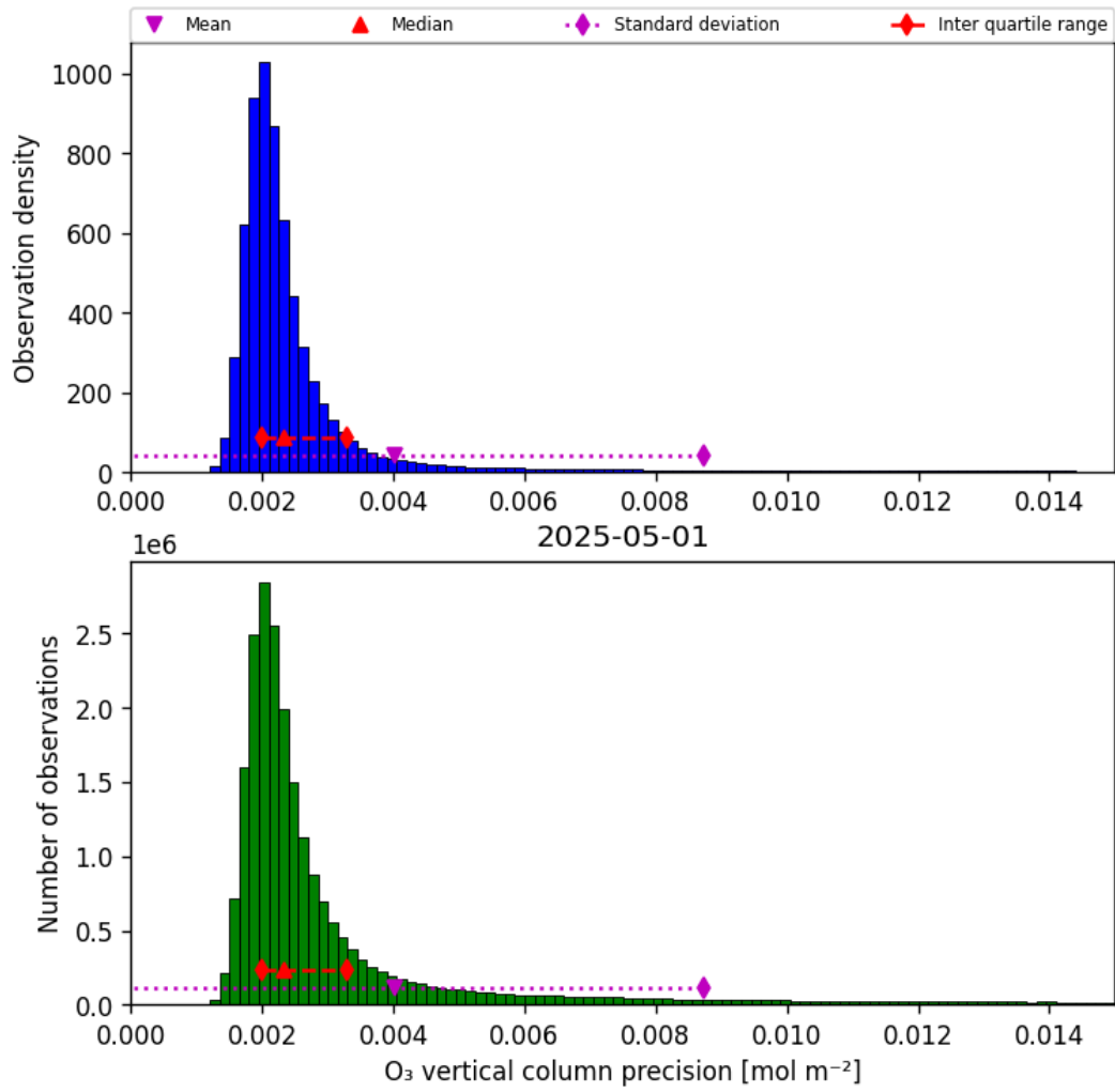
Figure 30: Histogram of “O 3 vertical column precision” for 2025-05-01 to 2025-05-02
