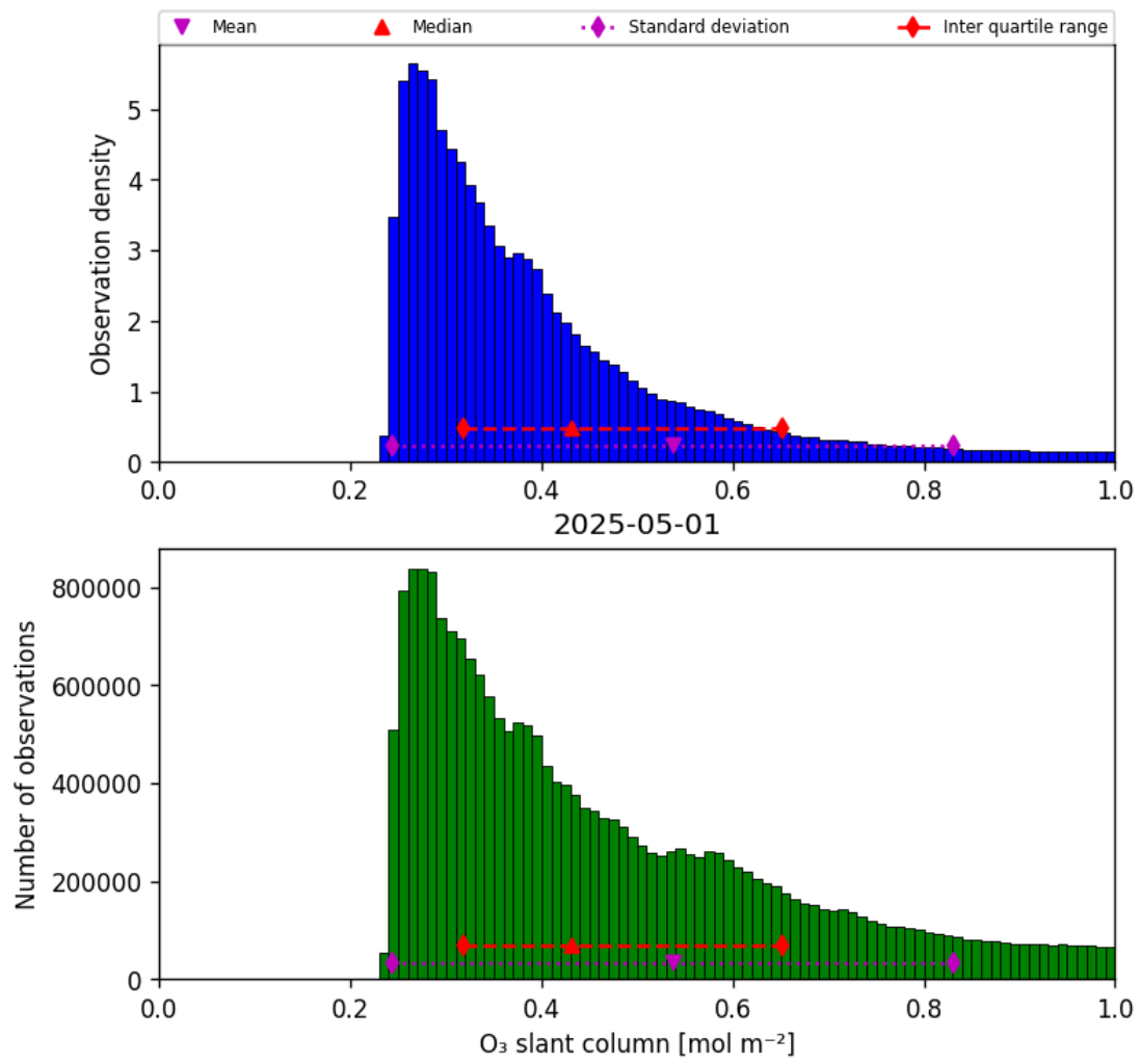
Figure 31: Histogram of “O 3 slant column” for 2025-05-01 to 2025-05-02
