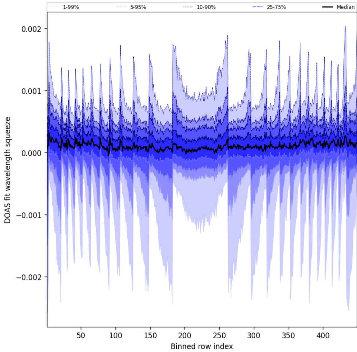
Figure 48: Along track statistics of “DOAS fit wavelength squeeze” for 2025-05-01 to 2025-05-02
