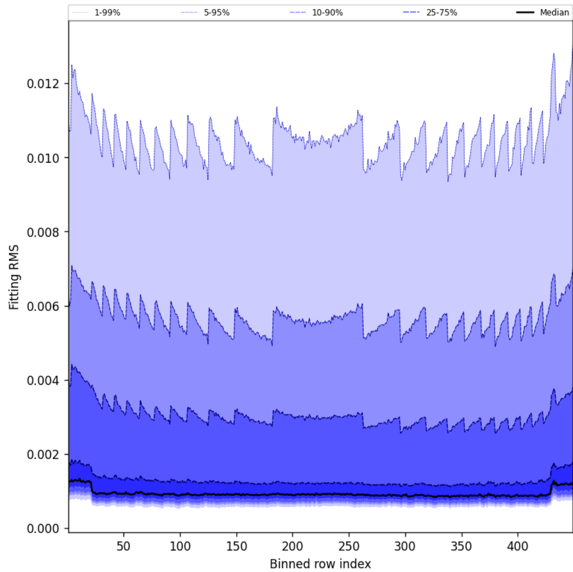
Figure 46: Along track statistics of “Fitting RMS” for 2025-05-02 to 2025-05-02
