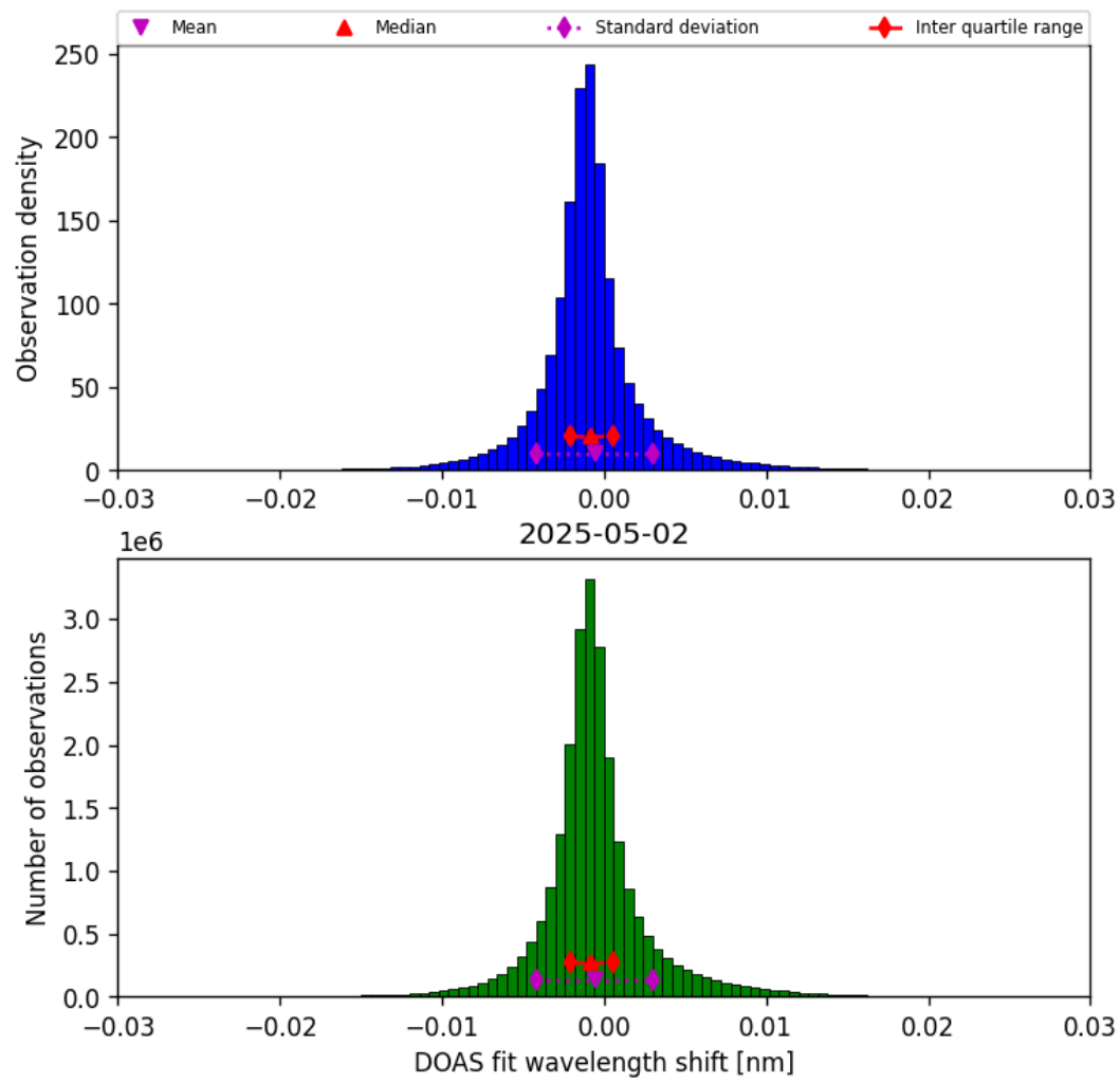
Figure 35: Histogram of “DOAS fit wavelength shift” for 2025-05-02 to 2025-05-02
