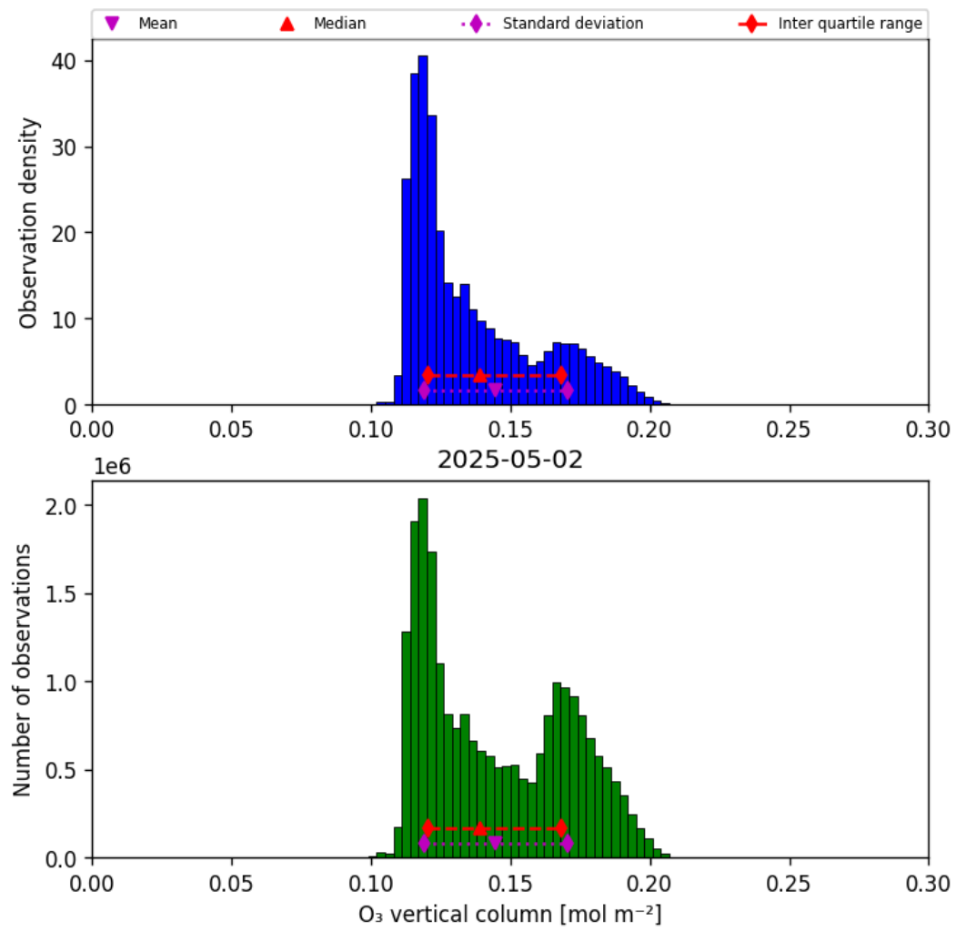
Figure 29: Histogram of “O 3 vertical column” for 2025-05-02 to 2025-05-02
