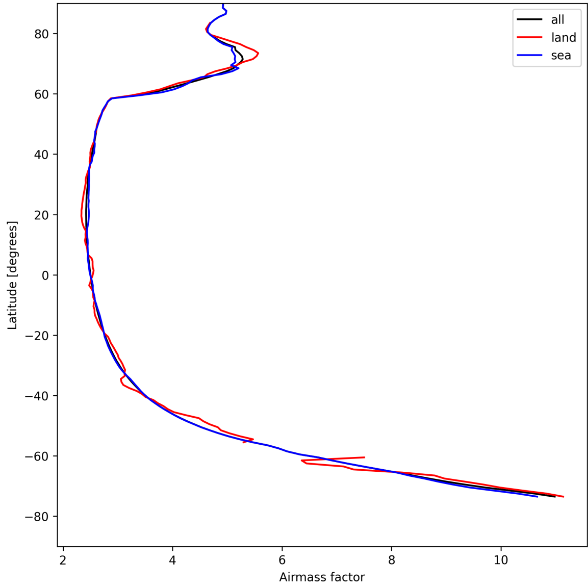
Figure 25: Zonal average of “Airmass factor” for 2025-05-02 to 2025-05-02.
