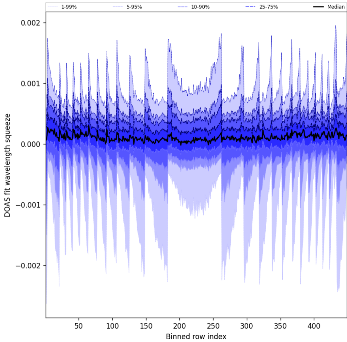
Figure 48: Along track statistics of “DOAS fit wavelength squeeze” for 2025-05-02 to 2025-05-02
