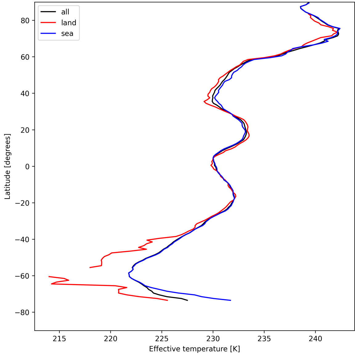
Figure 26: Zonal average of “Effective temperature” for 2025-05-02 to 2025-05-02.
