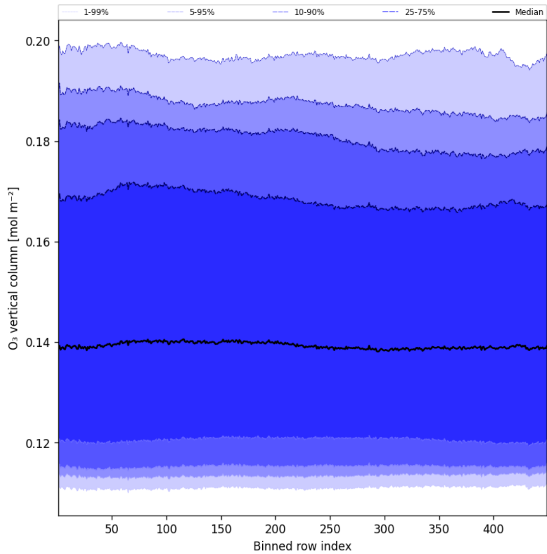
Figure 41: Along track statistics of “ \text{O}_3 vertical column” for 2025-05-02 to 2025-05-02
