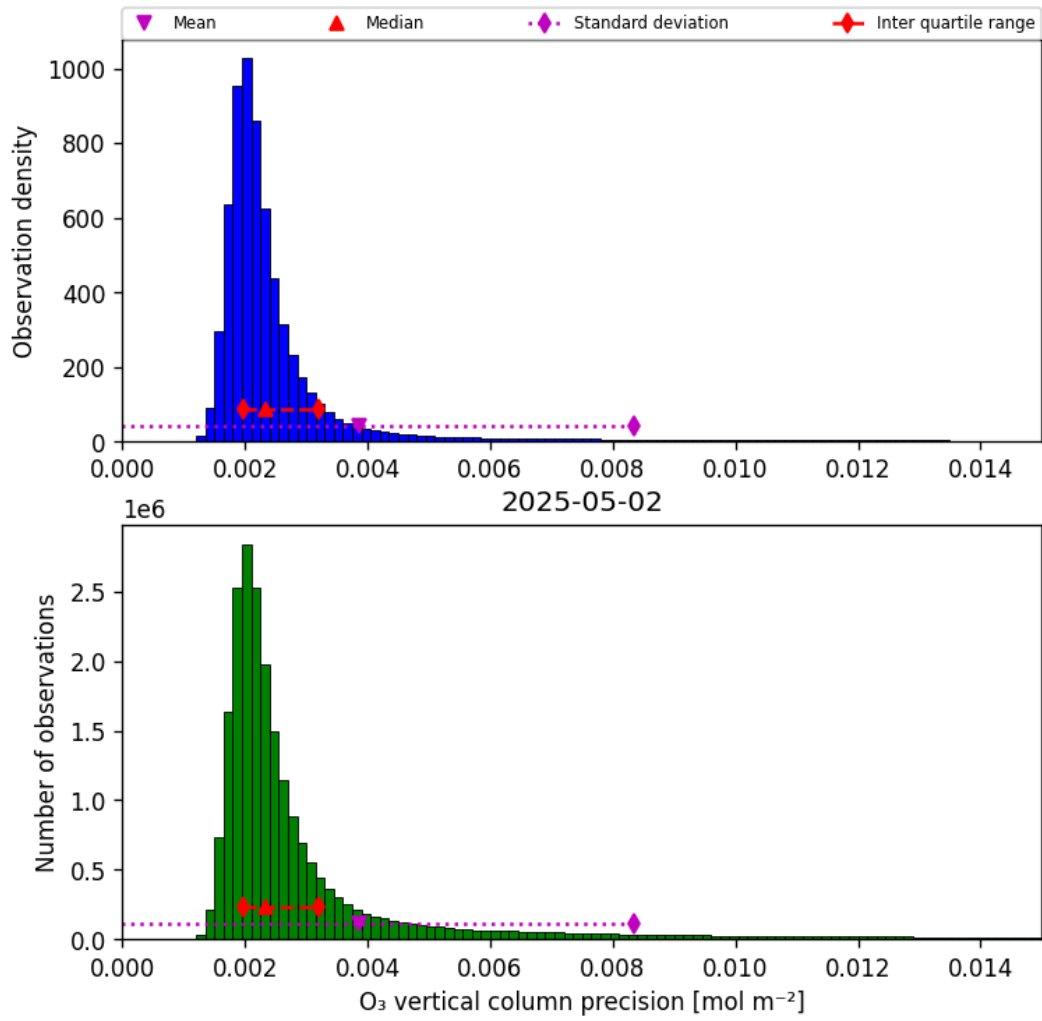
Figure 30: Histogram of “O 3 vertical column precision” for 2025-05-02 to 2025-05-02
