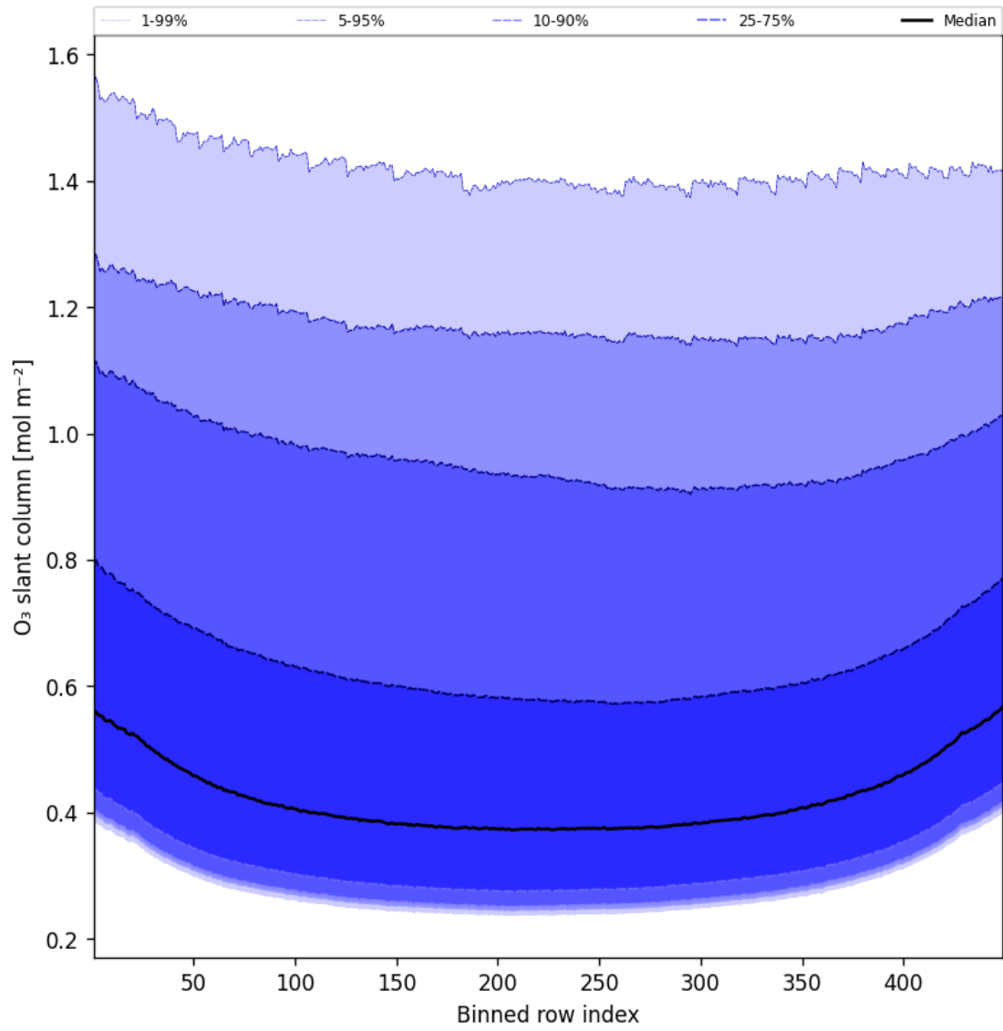
Figure 43: Along track statistics of “O 3 slant column” for 2025-05-02 to 2025-05-02
