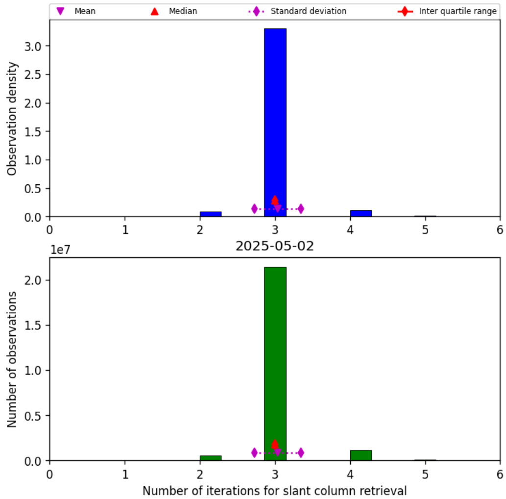
Figure 33: Histogram of “Number of iterations for slant column retrieval” for 2025-05-02 to 2025-05-02
