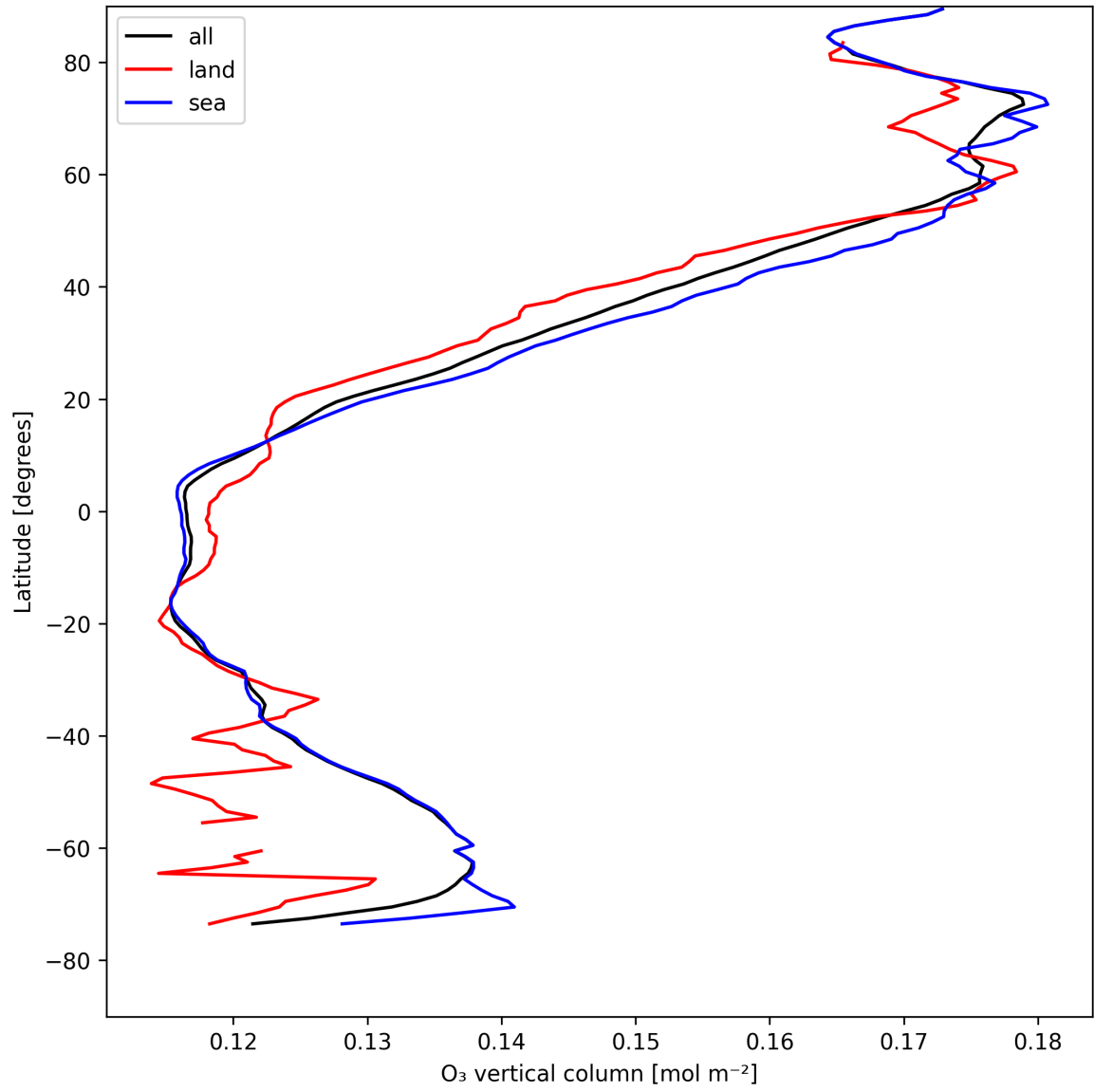
Figure 17: Zonal average of “O 3 vertical column” for 2025-05-02 to 2025-05-02.
