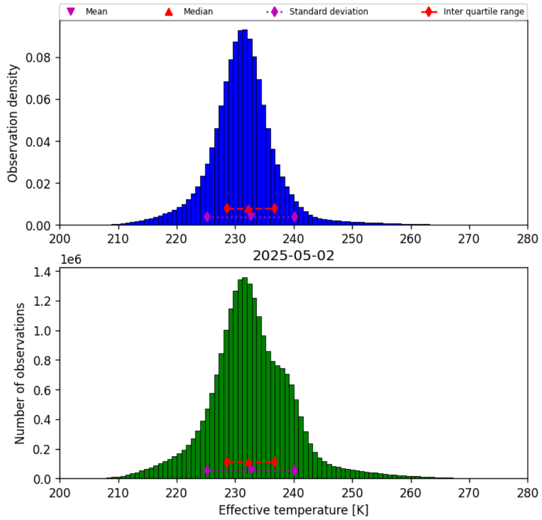
Figure 38: Histogram of “Effective temperature” for 2025-05-02 to 2025-05-02
