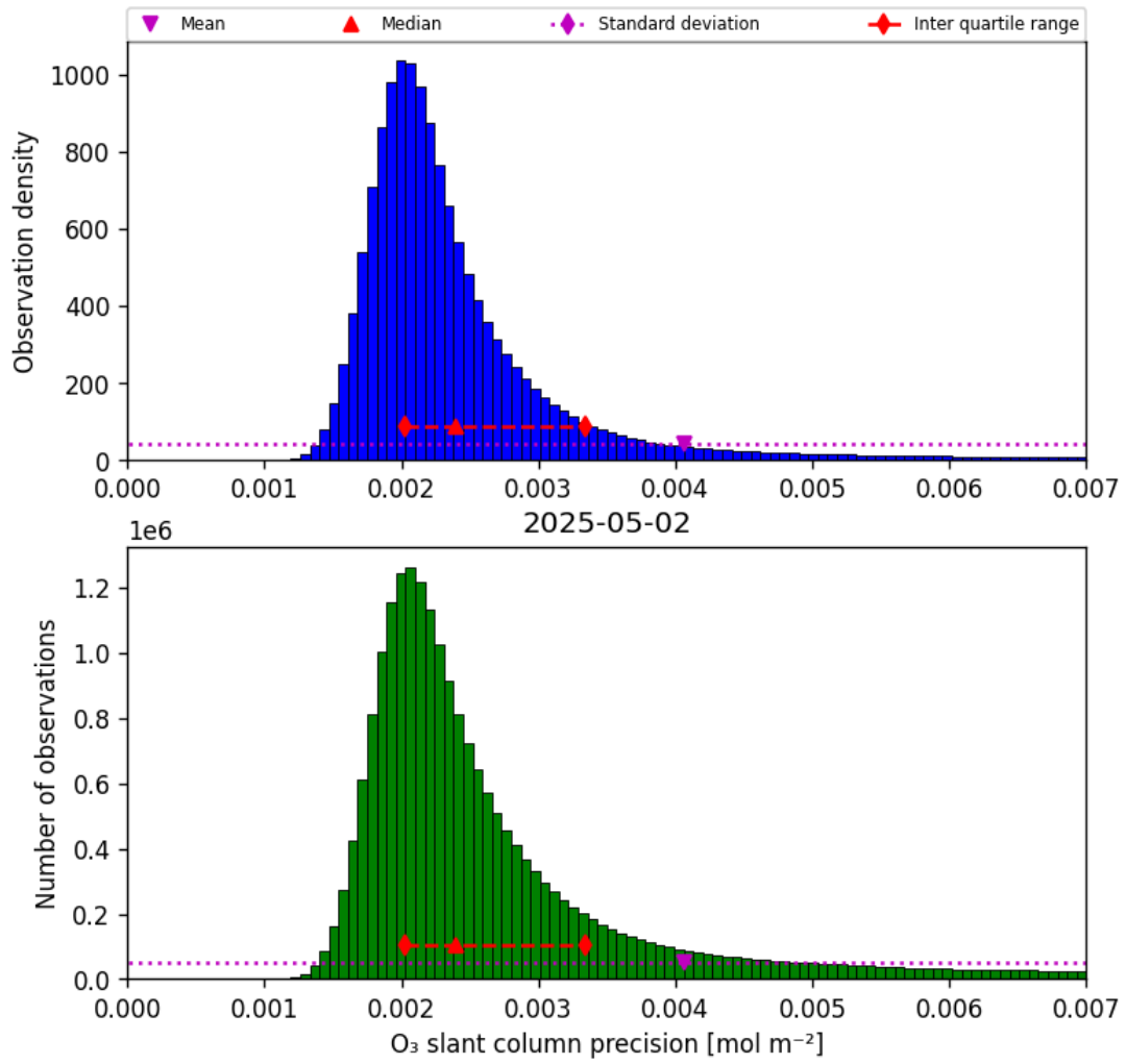
Figure 32: Histogram of “O 3 slant column precision” for 2025-05-02 to 2025-05-02
