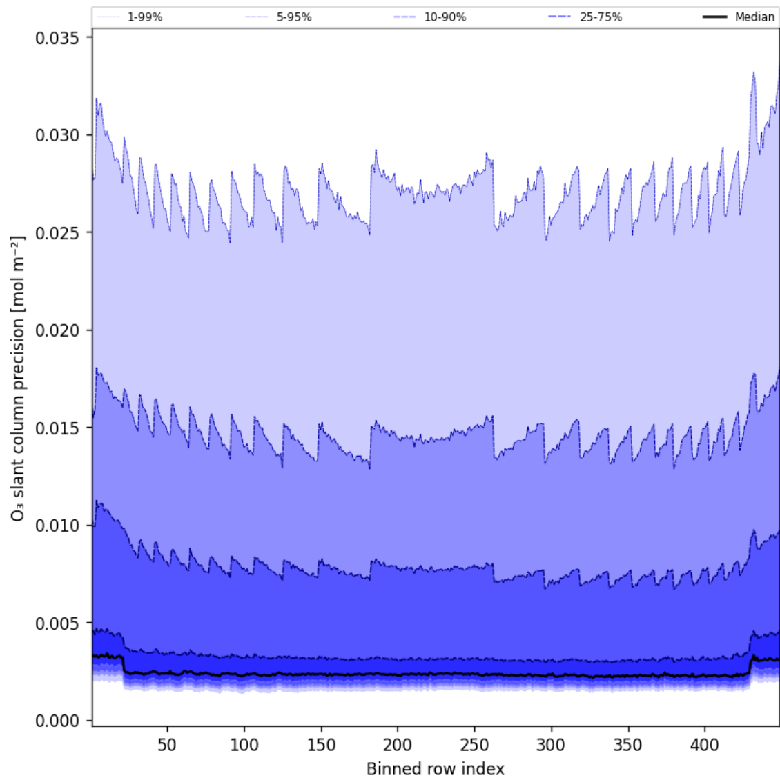
Figure 44: Along track statistics of “O 3 slant column precision” for 2025-05-02 to 2025-05-02
