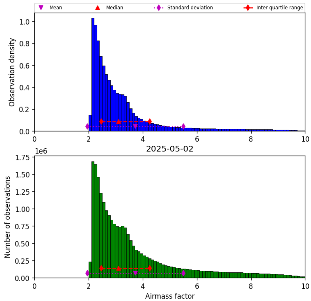
Figure 37: Histogram of “Airmass factor” for 2025-05-02 to 2025-05-02
