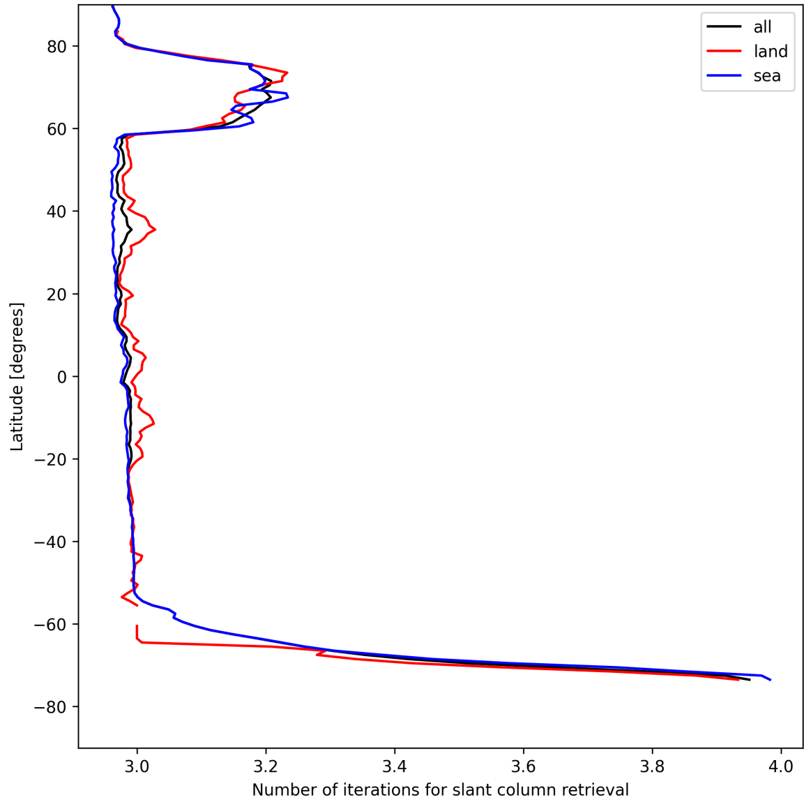
Figure 21: Zonal average of “Number of iterations for slant column retrieval” for 2025-05-02 to 2025-05-02.
