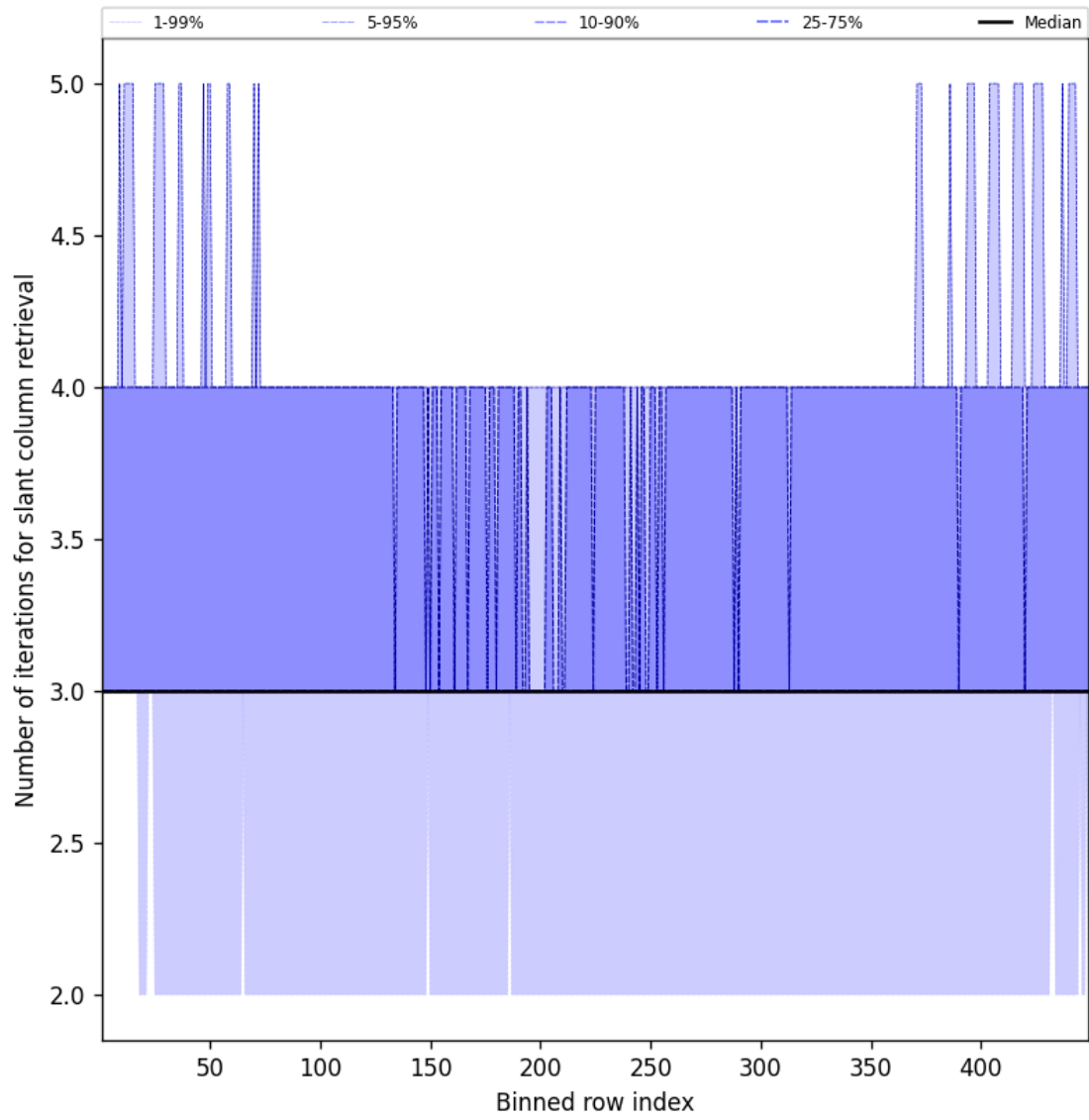
Figure 45: Along track statistics of “Number of iterations for slant column retrieval” for 2025-05-02 to 2025-05-02
