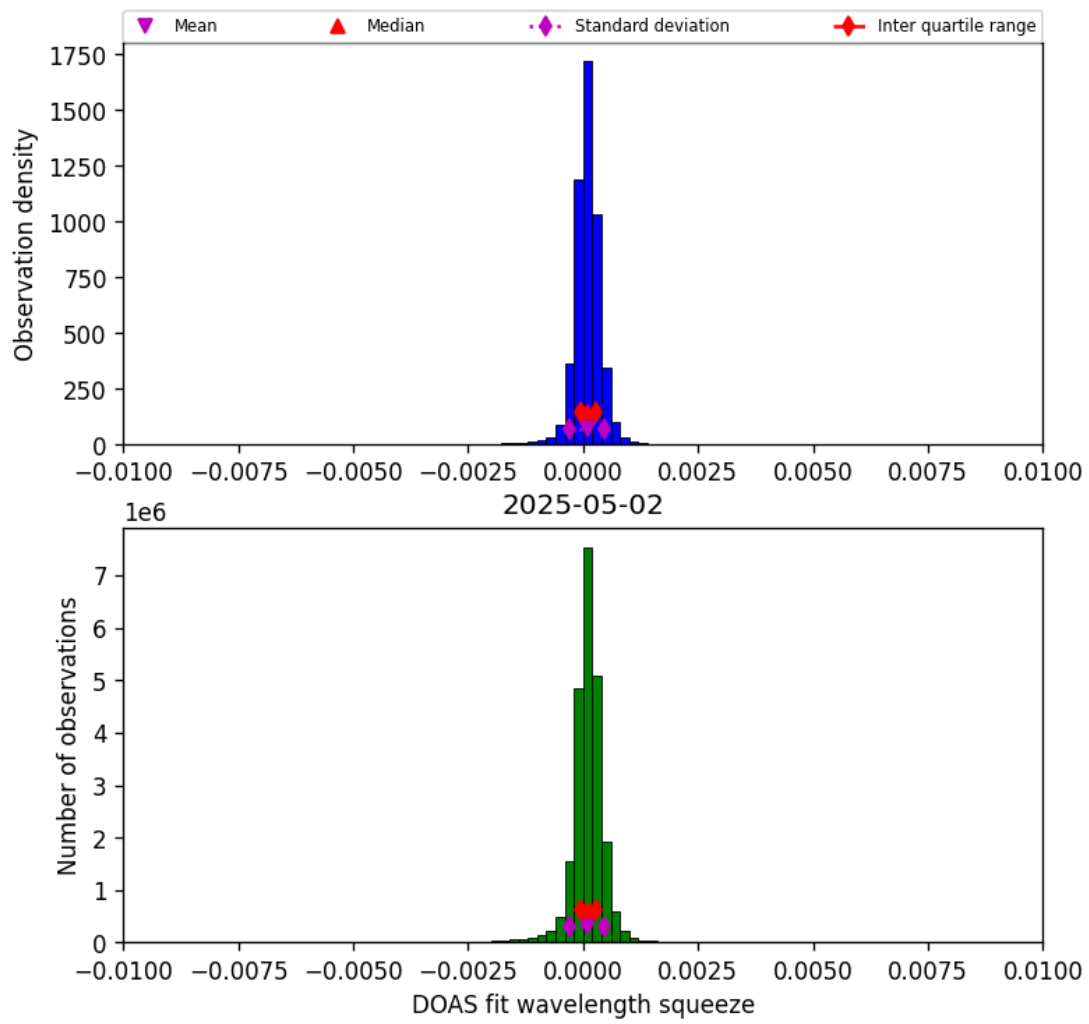
Figure 36: Histogram of “DOAS fit wavelength squeeze” for 2025-05-02 to 2025-05-02
