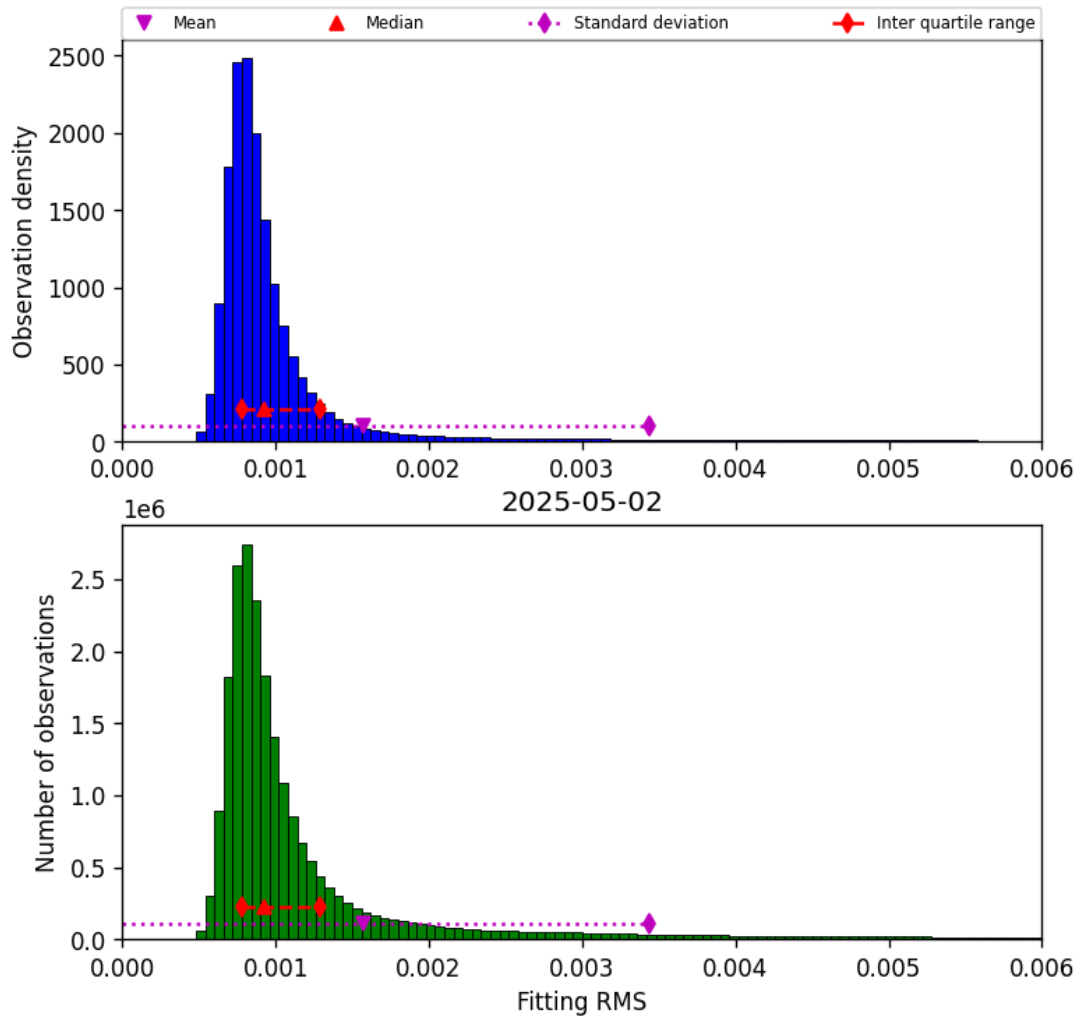
Figure 34: Histogram of “Fitting RMS” for 2025-05-02 to 2025-05-02
