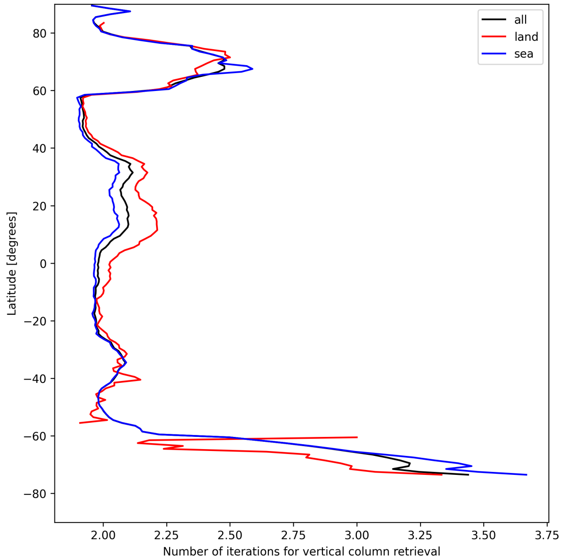
Figure 27: Zonal average of “Number of iterations for vertical column retrieval” for 2025-05-02 to 2025-05-02.
