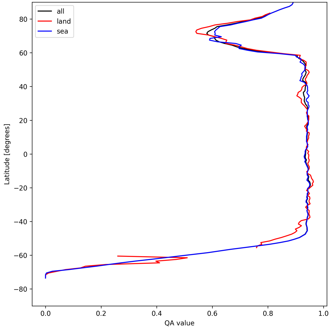
Figure 16: Zonal average of “QA value” for 2025-05-02 to 2025-05-02.
