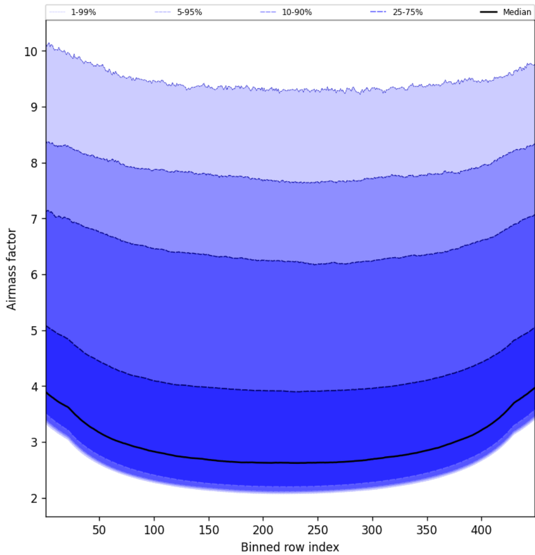
Figure 49: Along track statistics of “Airmass factor” for 2025-05-02 to 2025-05-02
