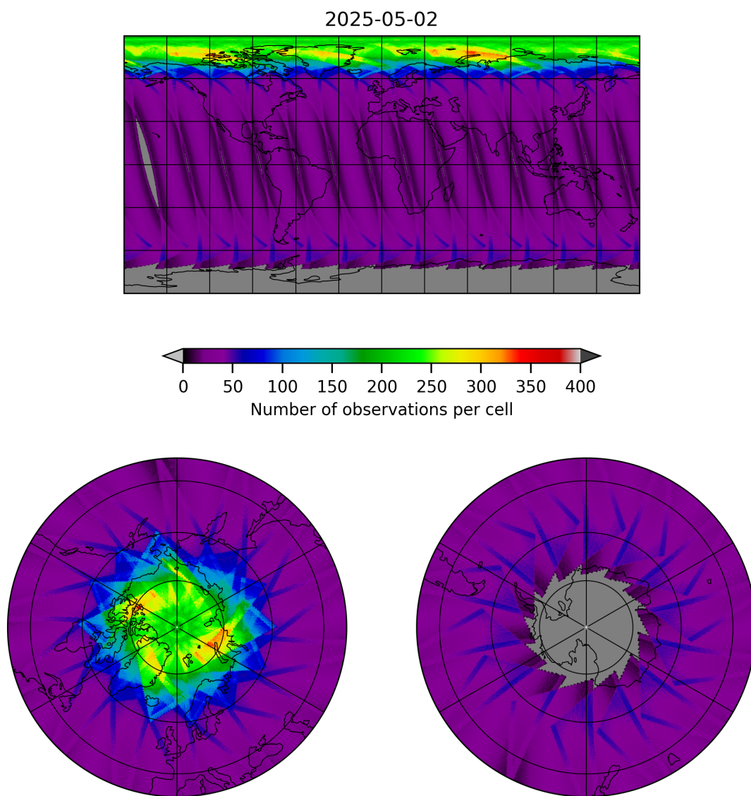
Figure 15: Map of the number of observations for 2025-05-02 to 2025-05-02
