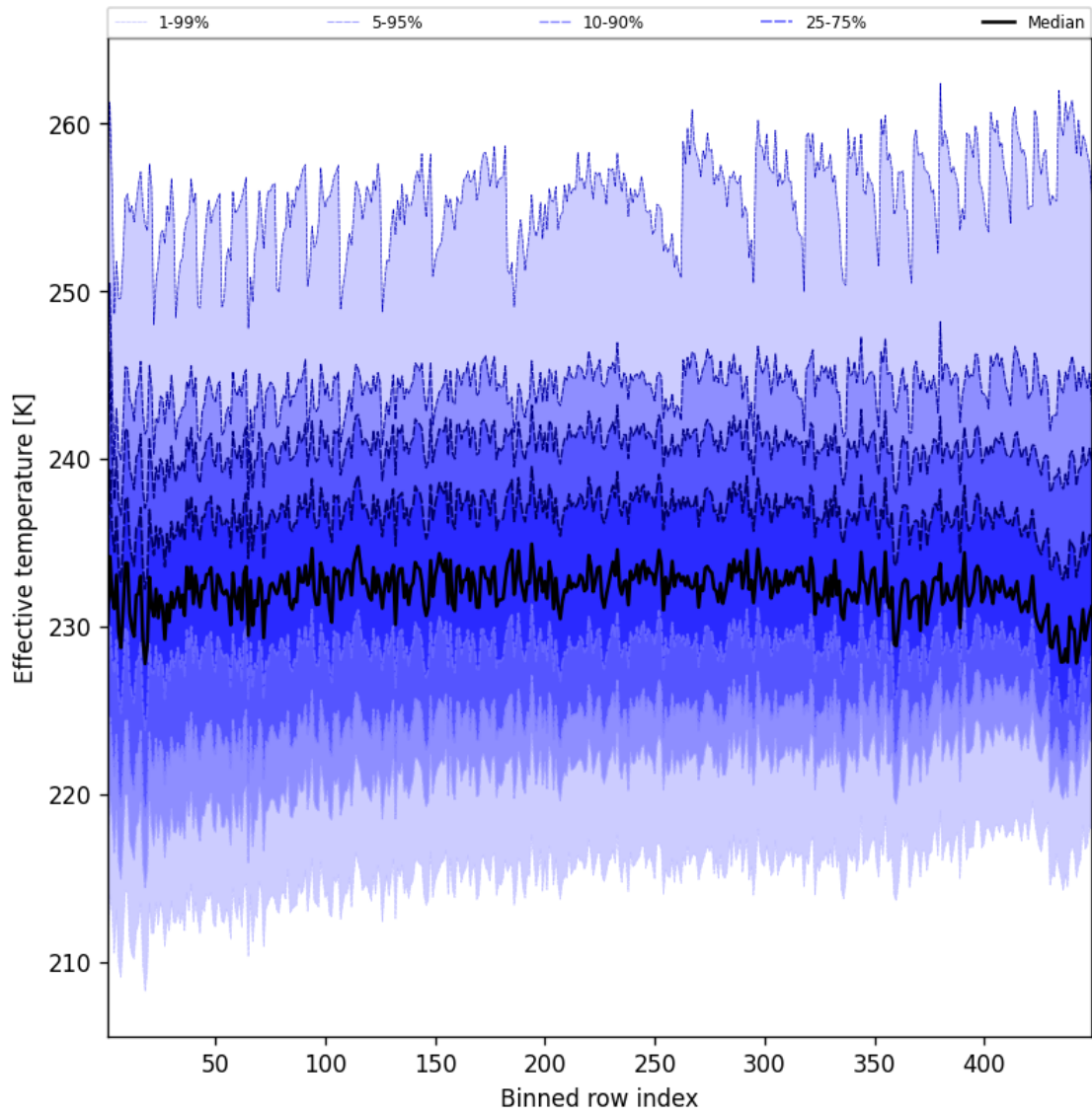
Figure 50: Along track statistics of “Effective temperature” for 2025-05-02 to 2025-05-02
