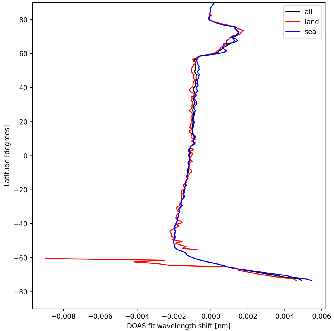
Figure 23: Zonal average of "DOAS fit wavelength shift" for 2025-05-02 to 2025-05-02.
