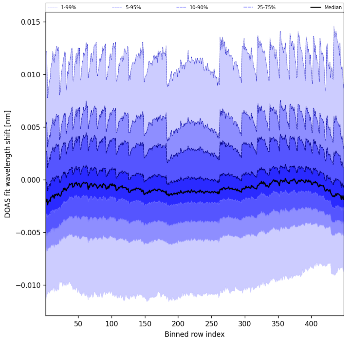
Figure 47: Along track statistics of “DOAS fit wavelength shift” for 2025-05-02 to 2025-05-02
