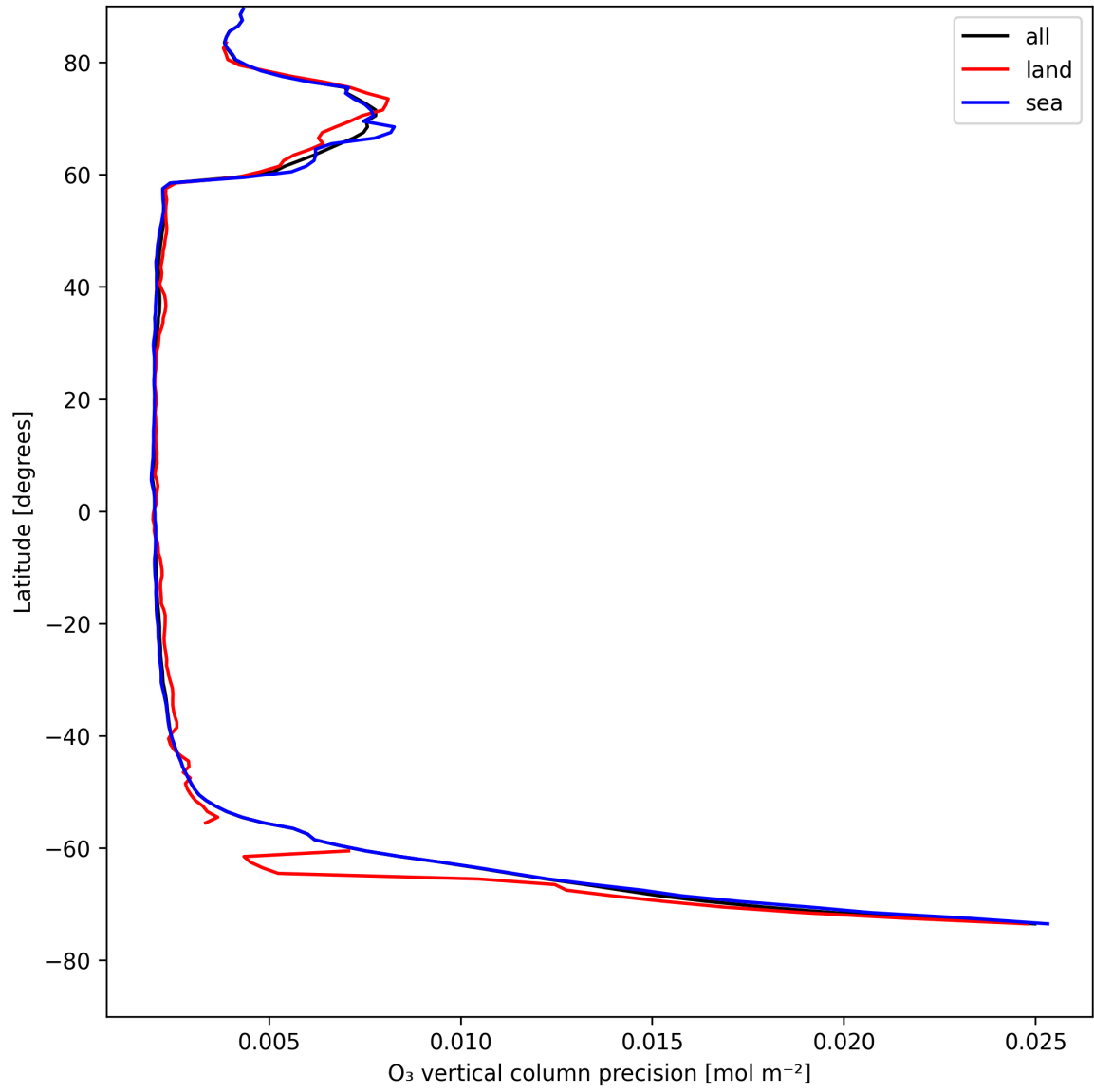
Figure 18: Zonal average of “O 3 vertical column precision” for 2025-05-02 to 2025-05-02.
