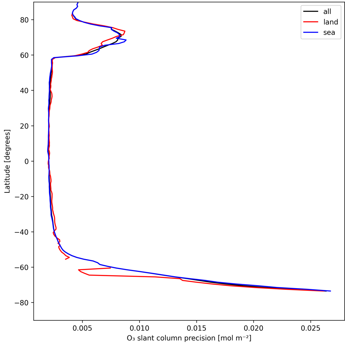
Figure 20: Zonal average of “O 3 slant column precision” for 2025-05-02 to 2025-05-02.
