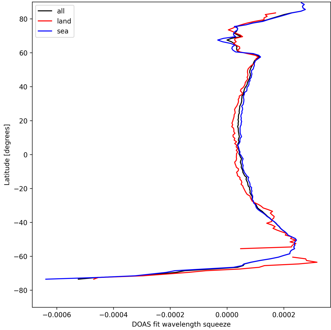
Figure 24: Zonal average of “DOAS fit wavelength squeeze” for 2025-05-02 to 2025-05-02.
