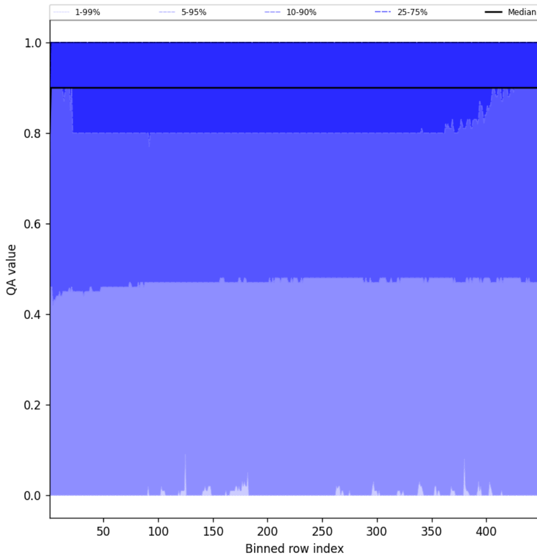
Figure 40: Along track statistics of “QA value” for 2025-05-02 to 2025-05-02
