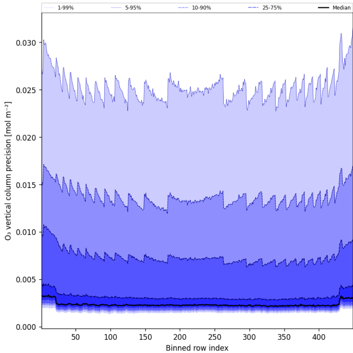
Figure 42: Along track statistics of “O 3 vertical column precision” for 2025-05-02 to 2025-05-02
