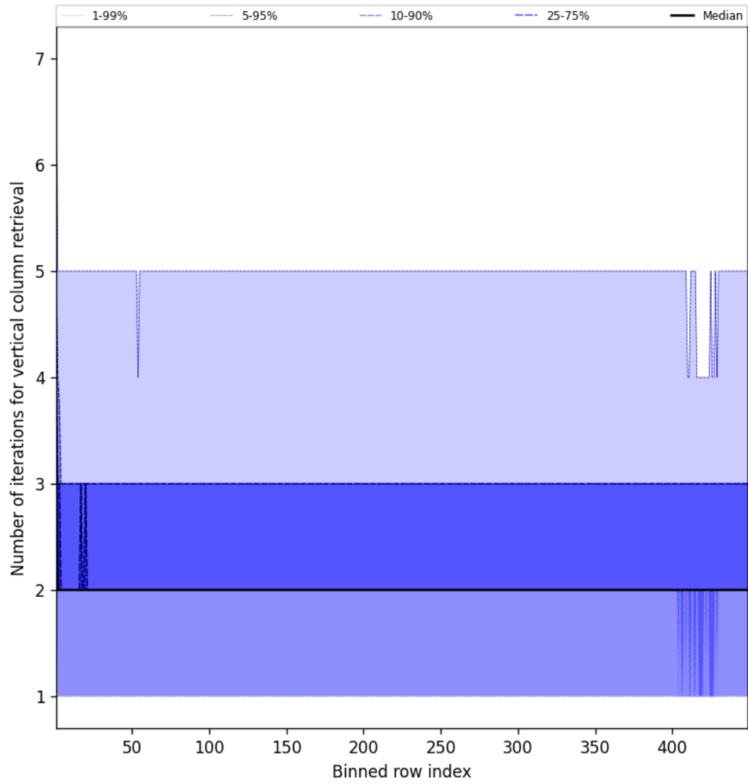
Figure 51: Along track statistics of “Number of iterations for vertical column retrieval” for 2025-05-02 to 2025-05-02
