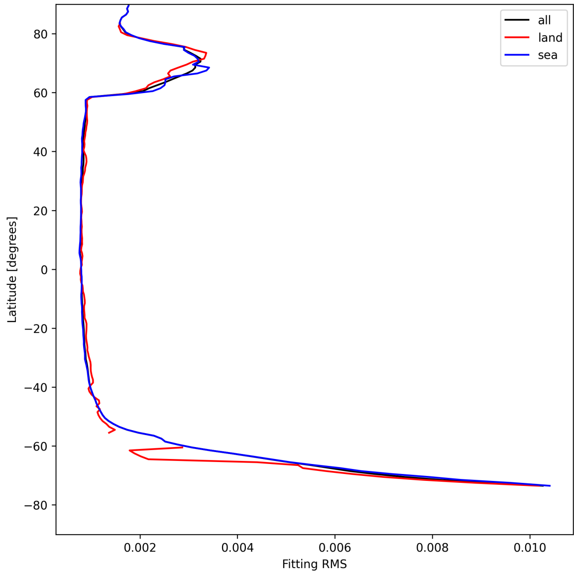
Figure 22: Zonal average of “Fitting RMS” for 2025-05-02 to 2025-05-02.
