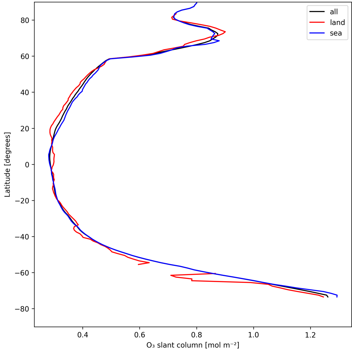
Figure 19: Zonal average of “O 3 slant column” for 2025-05-02 to 2025-05-02.
