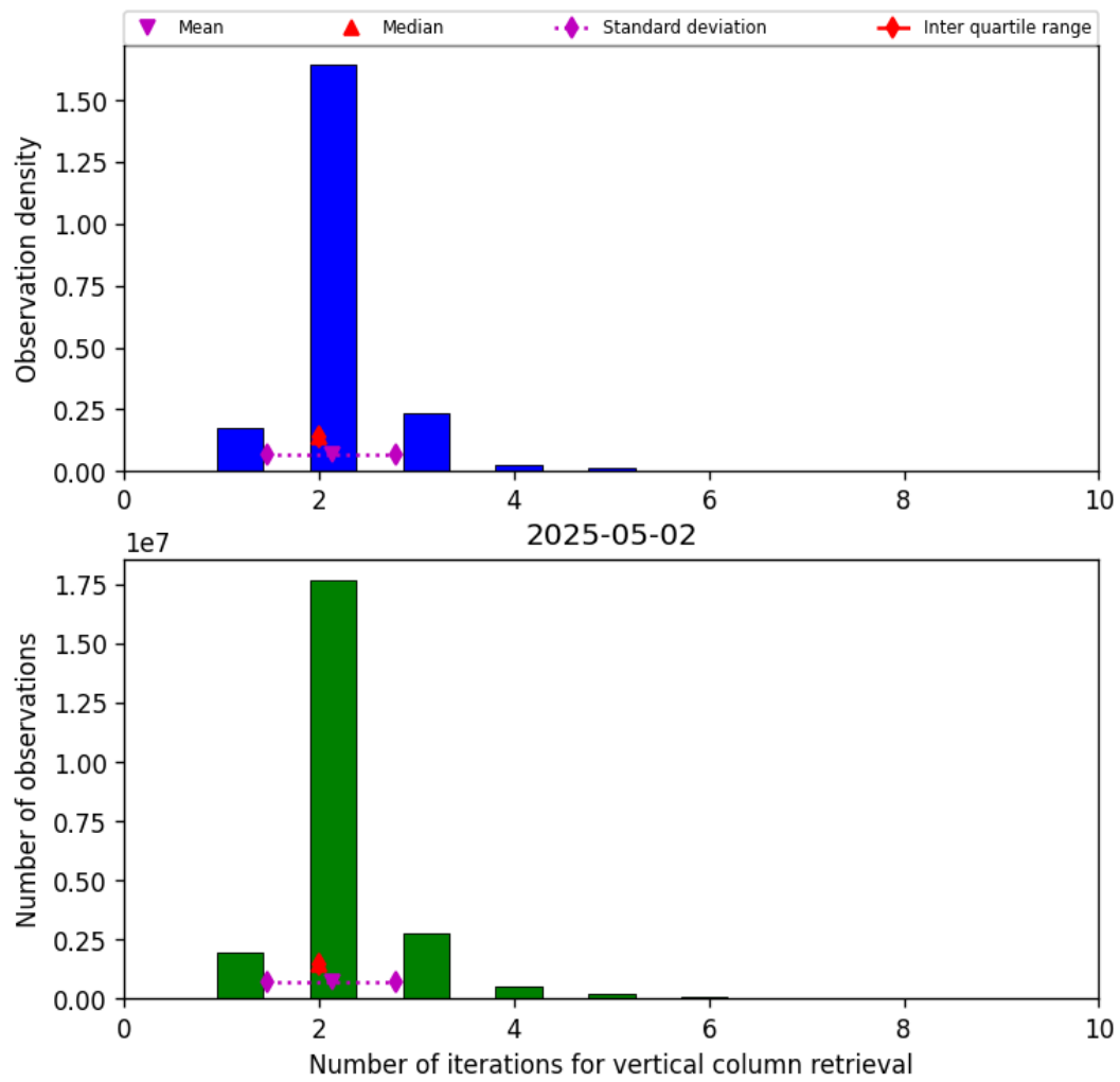
Figure 39: Histogram of “Number of iterations for vertical column retrieval” for 2025-05-02 to 2025-05-02
