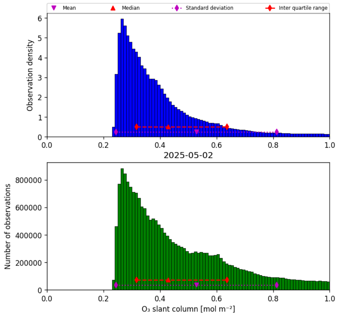
Figure 31: Histogram of “O 3 slant column” for 2025-05-02 to 2025-05-02
