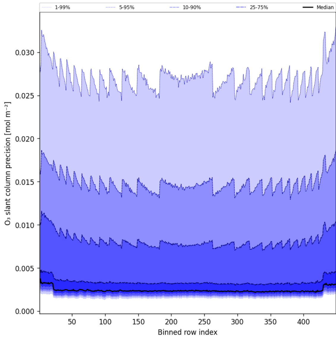
Figure 44: Along track statistics of “O 3 slant column precision” for 2025-05-03 to 2025-05-03
