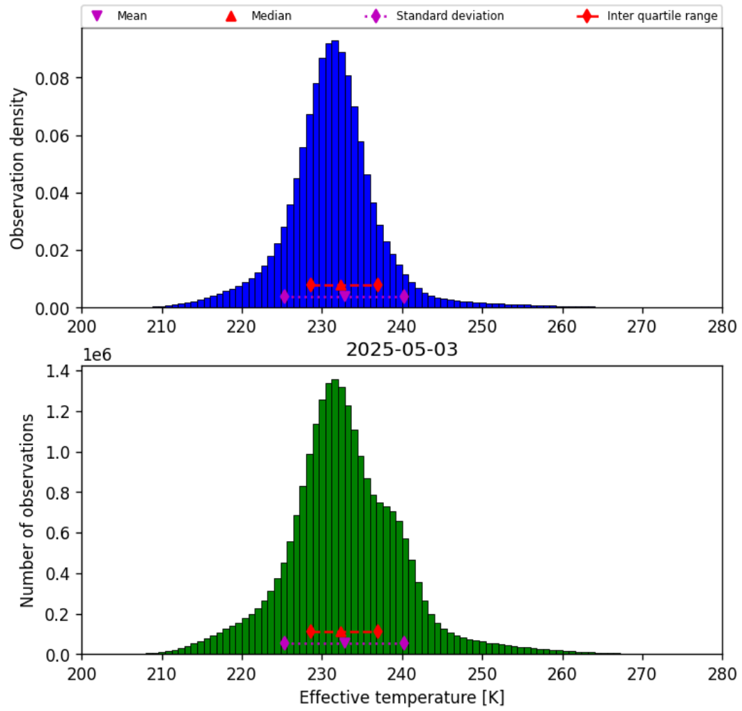
Figure 38: Histogram of “Effective temperature” for 2025-05-03 to 2025-05-03
