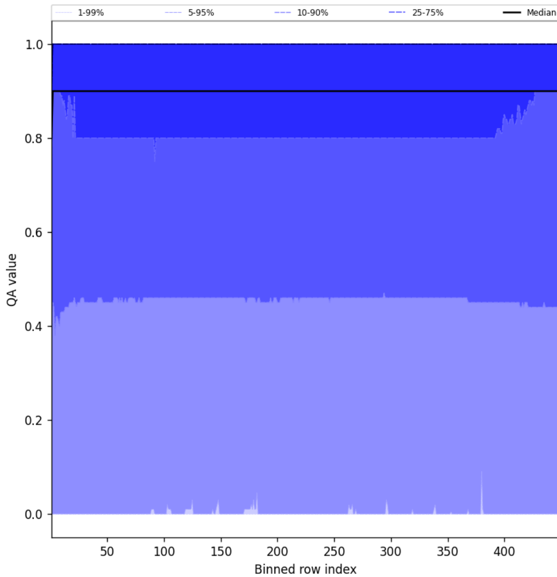
Figure 40: Along track statistics of “QA value” for 2025-05-03 to 2025-05-03
