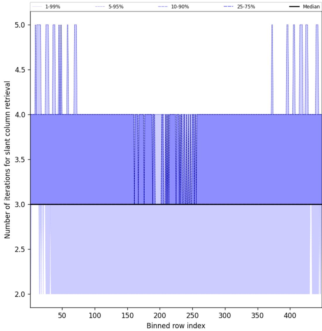
Figure 45: Along track statistics of “Number of iterations for slant column retrieval” for 2025-05-03 to 2025-05-03
