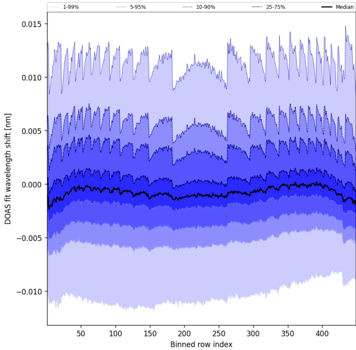
Figure 47: Along track statistics of “DOAS fit wavelength shift” for 2025-05-03 to 2025-05-03
