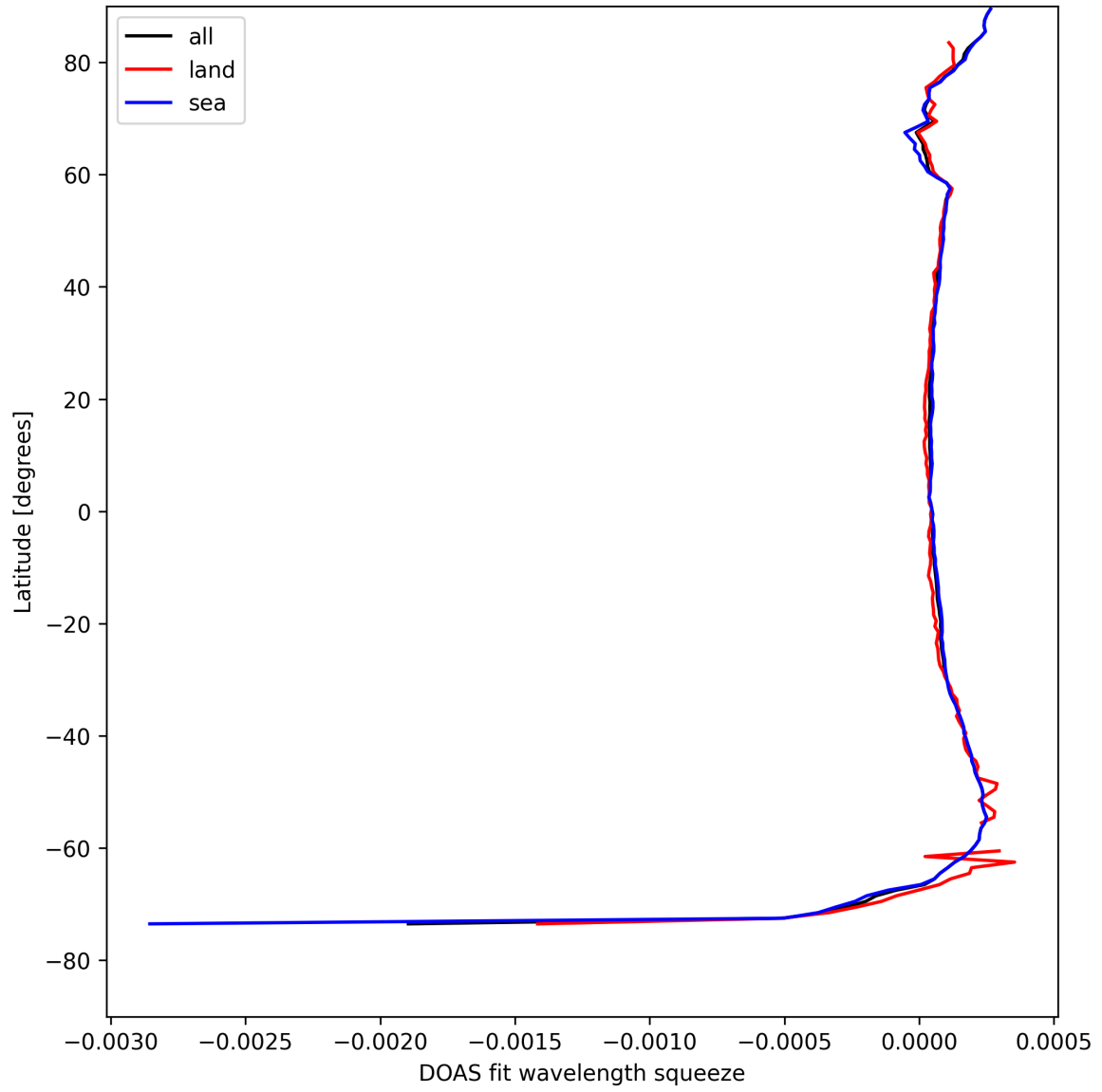
Figure 24: Zonal average of “DOAS fit wavelength squeeze” for 2025-05-03 to 2025-05-03.
