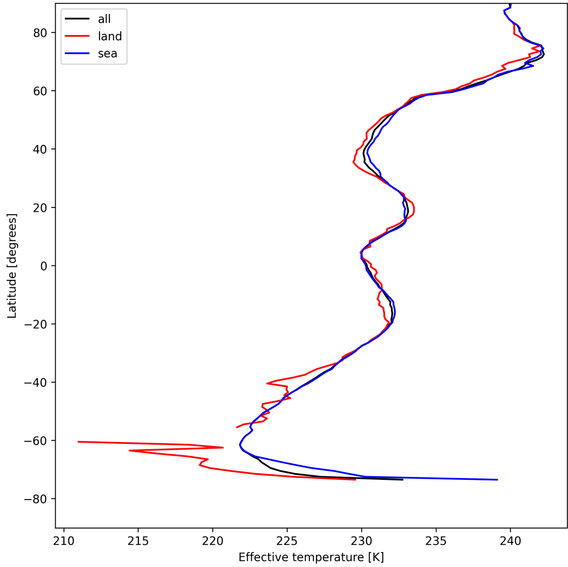
Figure 26: Zonal average of “Effective temperature” for 2025-05-03 to 2025-05-03.
