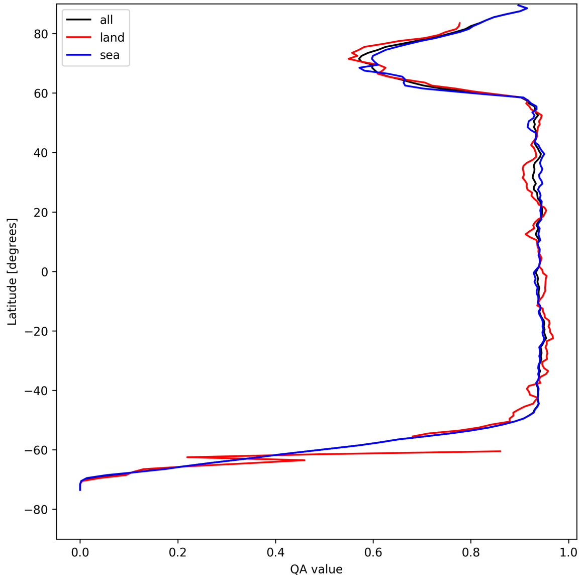
Figure 16: Zonal average of “QA value” for 2025-05-03 to 2025-05-03.
