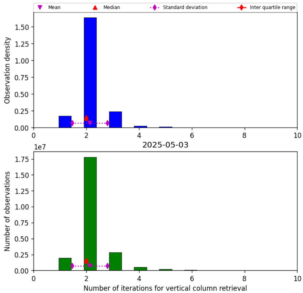
Figure 39: Histogram of “Number of iterations for vertical column retrieval” for 2025-05-03 to 2025-05-03
