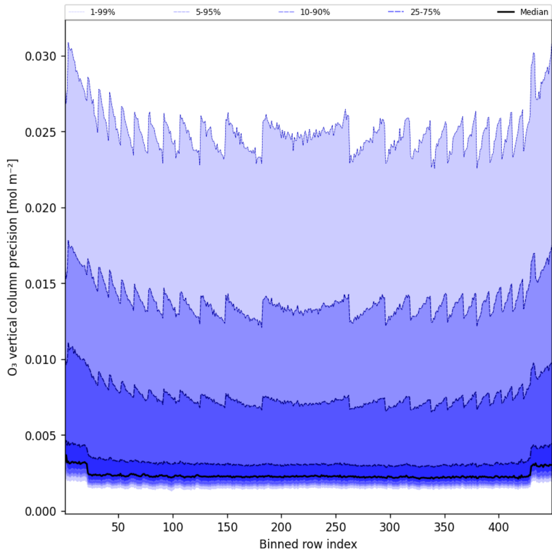
Figure 42: Along track statistics of “O 3 vertical column precision” for 2025-05-03 to 2025-05-03
