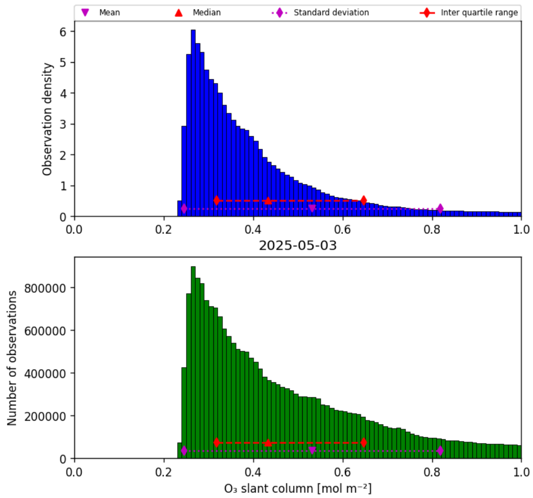
Figure 31: Histogram of “O 3 slant column” for 2025-05-03 to 2025-05-03
