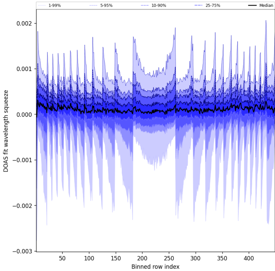
Figure 48: Along track statistics of “DOAS fit wavelength squeeze” for 2025-05-03 to 2025-05-03
