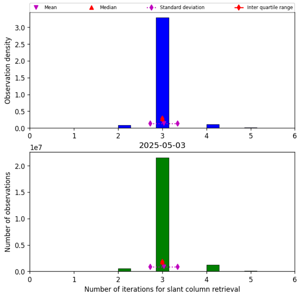
Figure 33: Histogram of "Number of iterations for slant column retrieval" for 2025-05-03 to 2025-05-03
