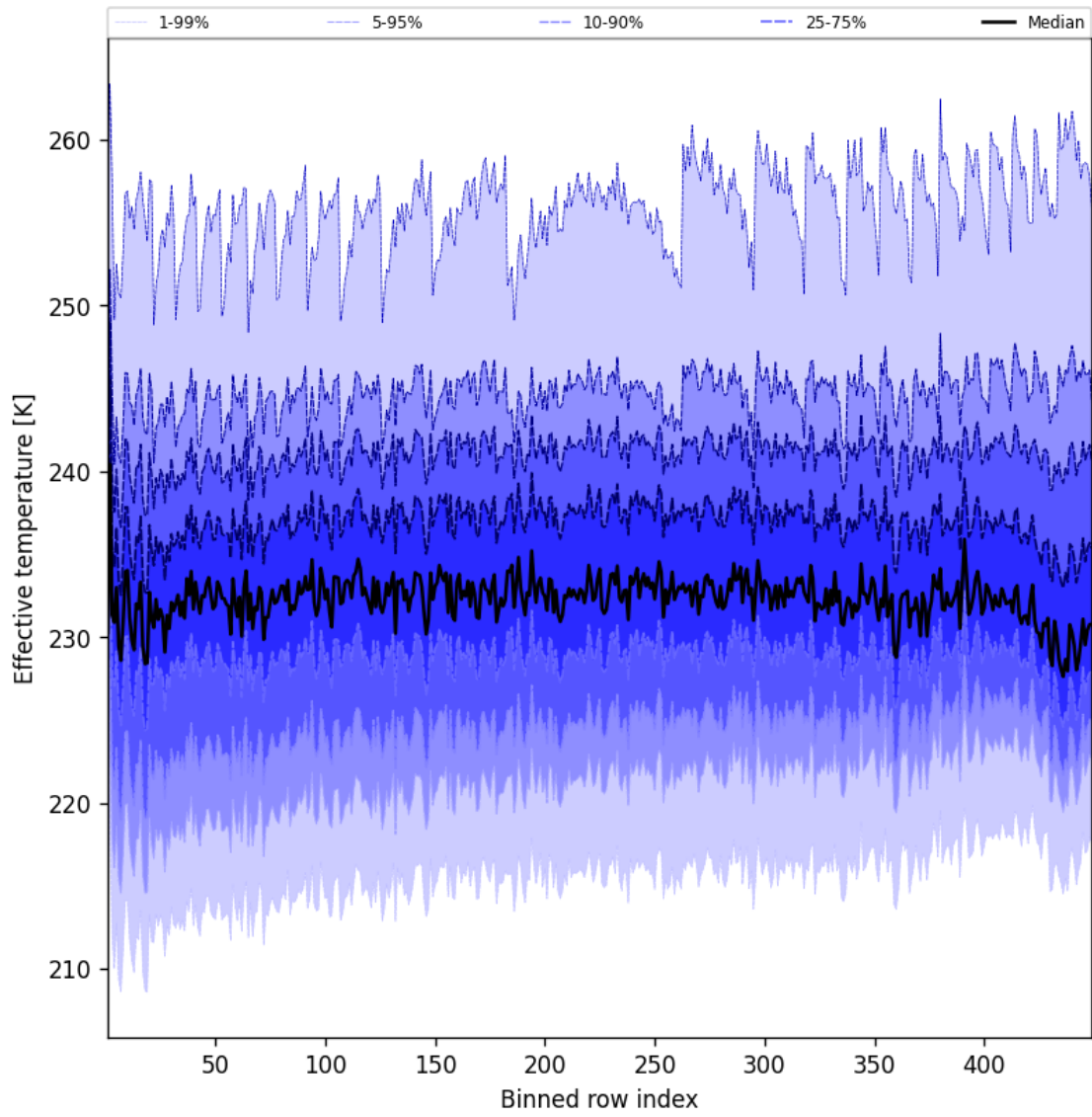
Figure 50: Along track statistics of “Effective temperature” for 2025-05-03 to 2025-05-03
