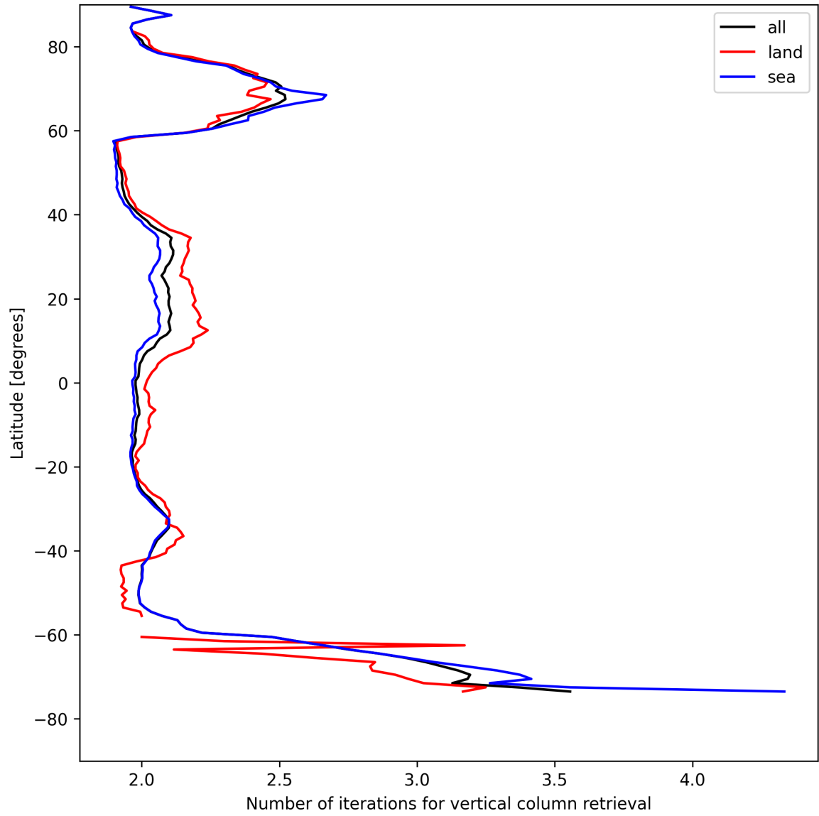
Figure 27: Zonal average of “Number of iterations for vertical column retrieval” for 2025-05-03 to 2025-05-03.
