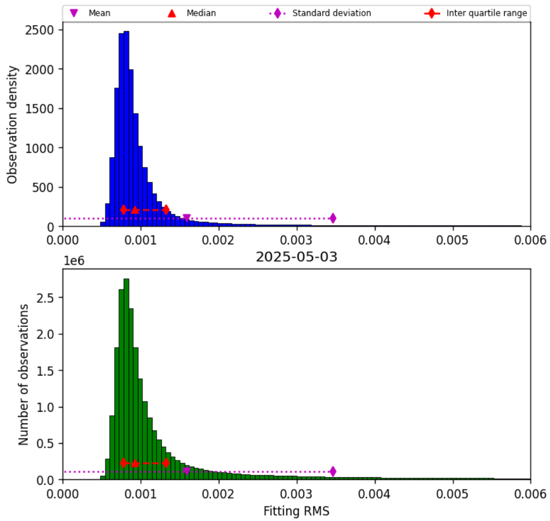
Figure 34: Histogram of “Fitting RMS” for 2025-05-03 to 2025-05-03
