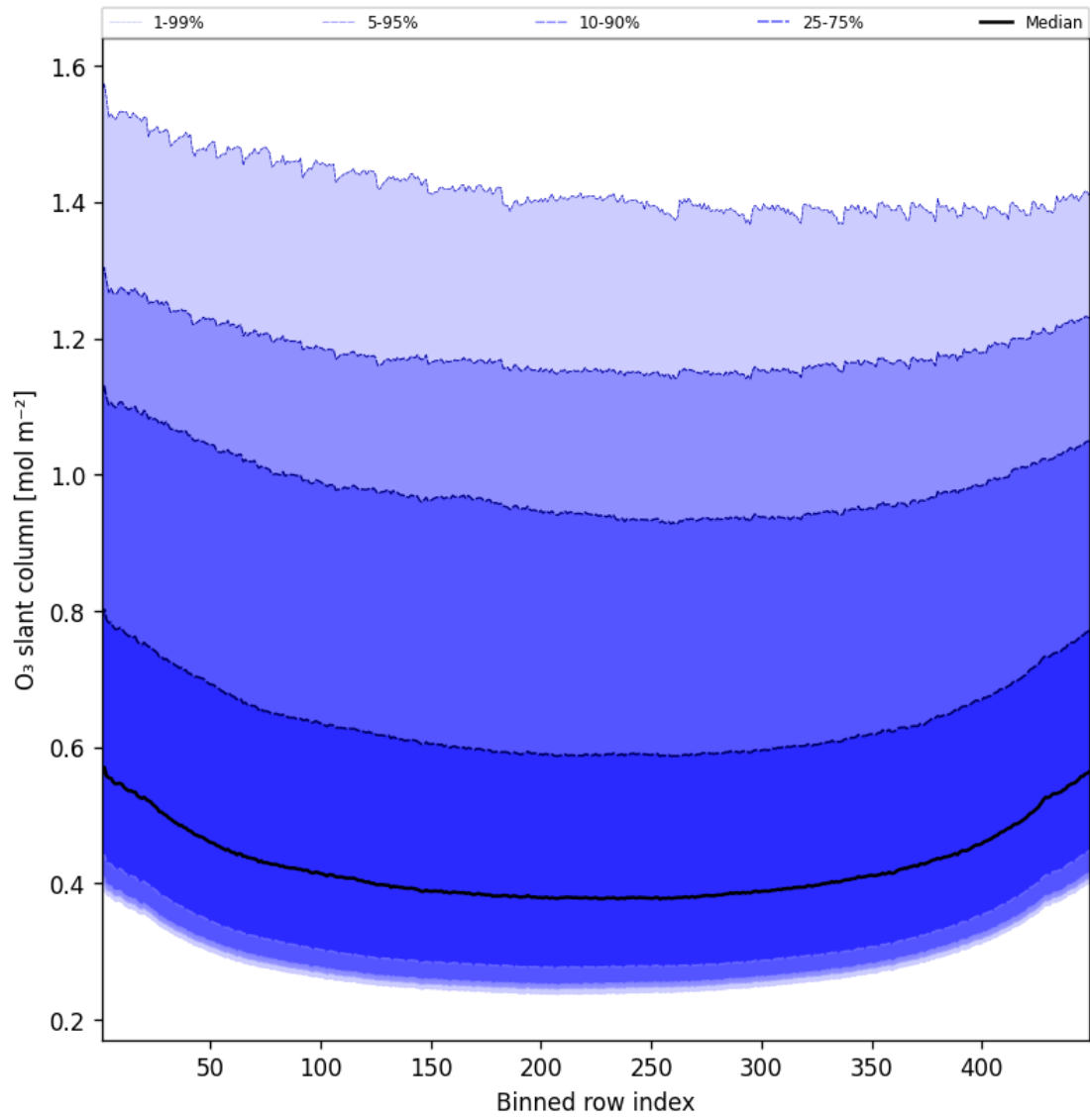
Figure 43: Along track statistics of “O 3 slant column” for 2025-05-03 to 2025-05-03
