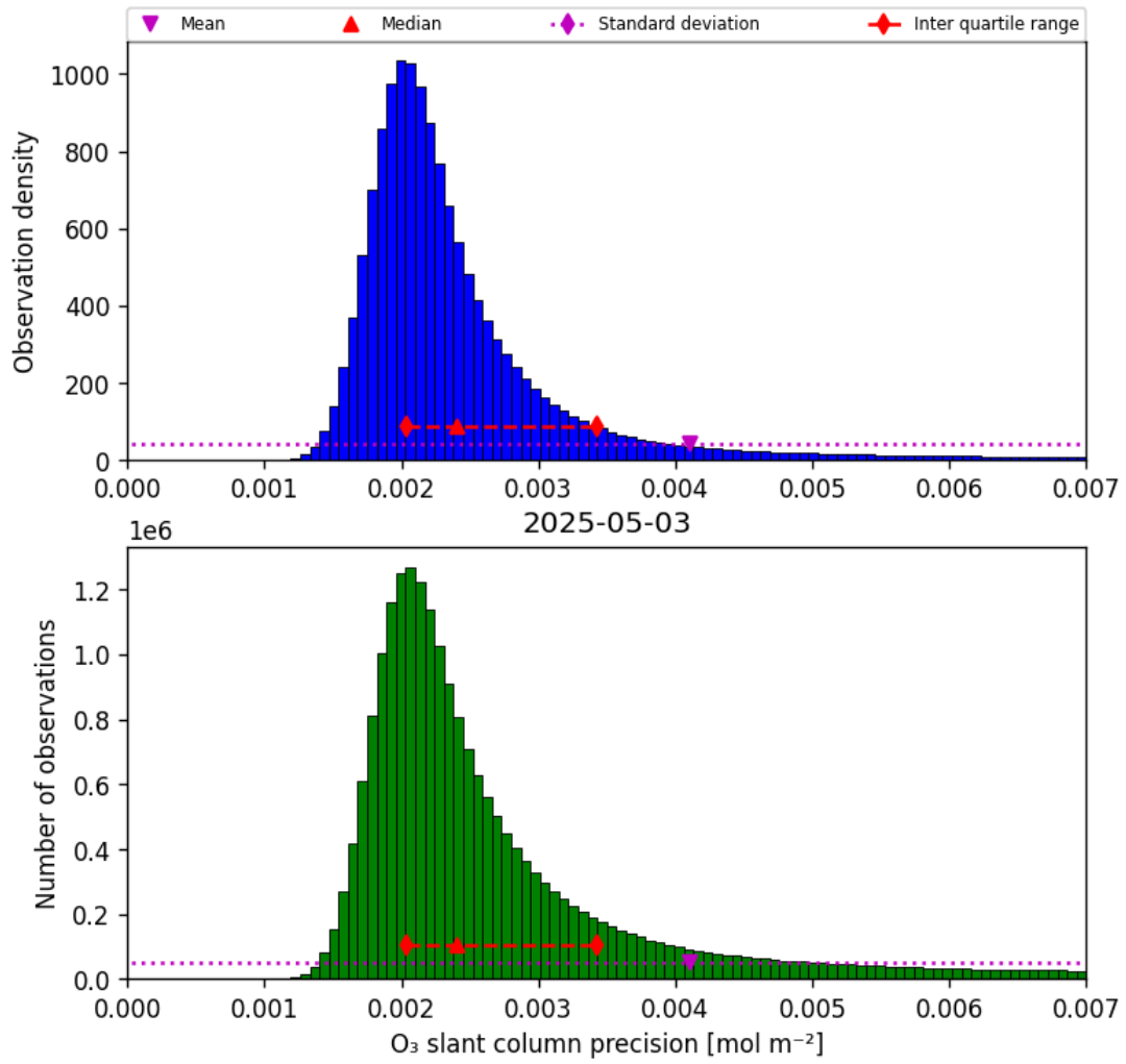
Figure 32: Histogram of “O 3 slant column precision” for 2025-05-03 to 2025-05-03
