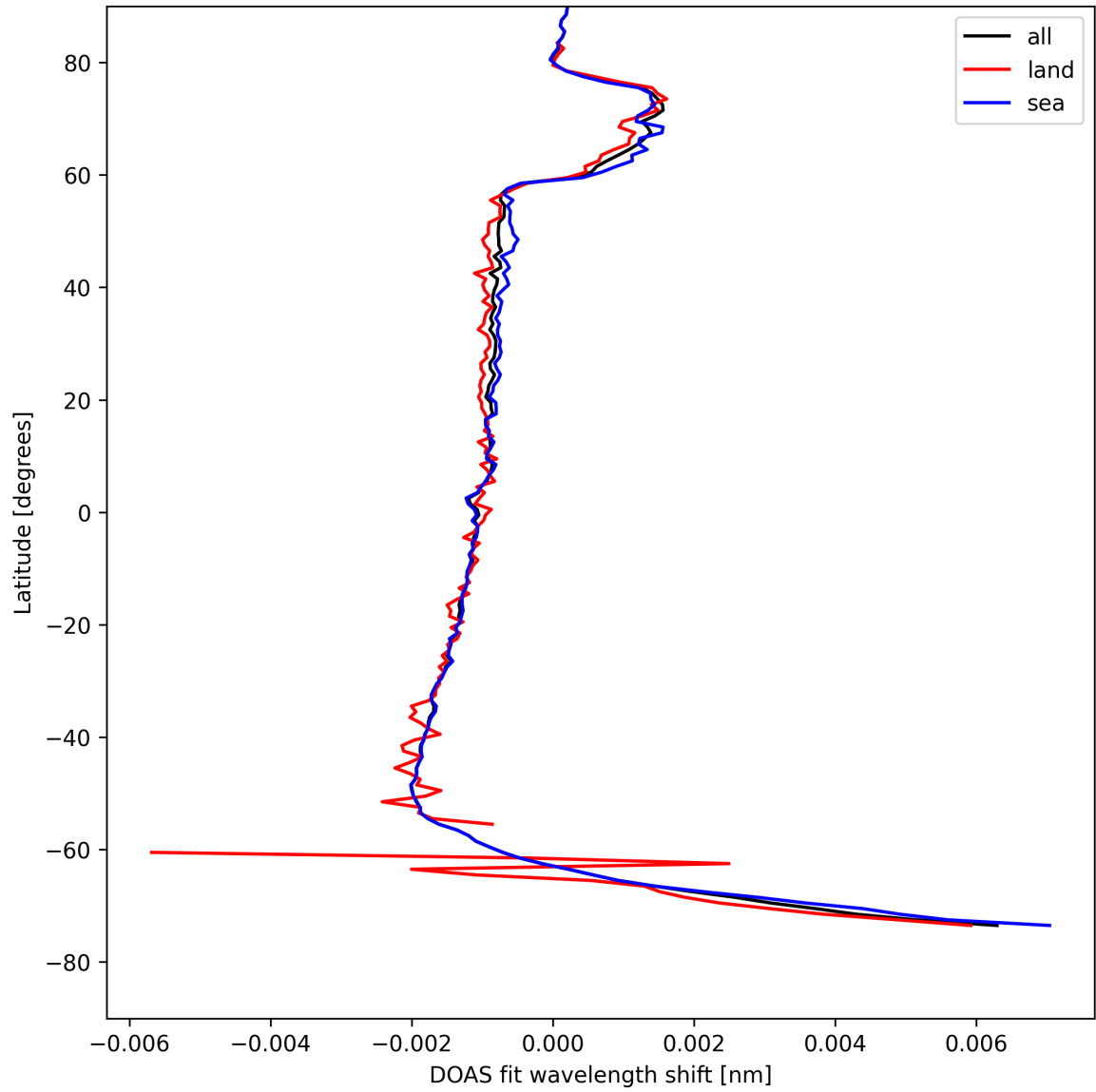
Figure 23: Zonal average of "DOAS fit wavelength shift" for 2025-05-03 to 2025-05-03.
