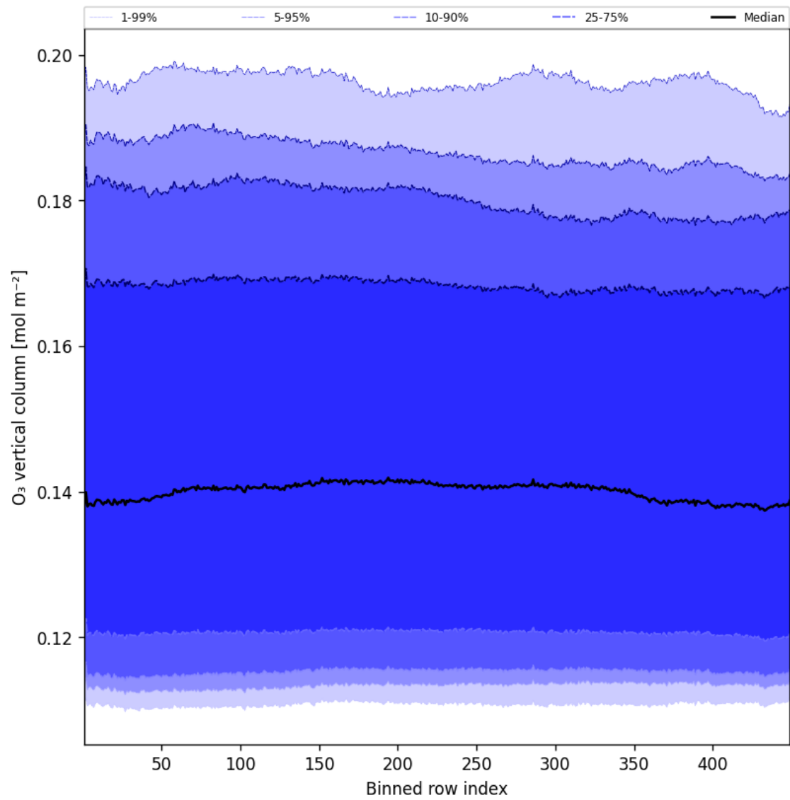
Figure 41: Along track statistics of “O 3 vertical column” for 2025-05-03 to 2025-05-03
