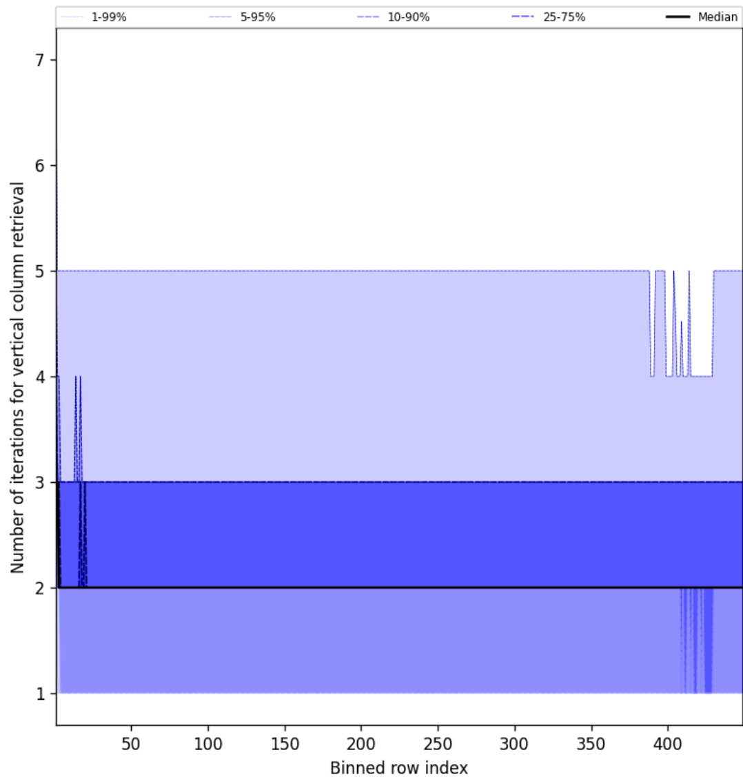
Figure 51: Along track statistics of “Number of iterations for vertical column retrieval” for 2025-05-03 to 2025-05-03
