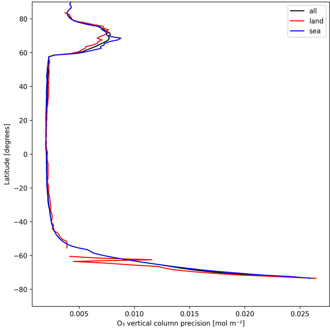
Figure 18: Zonal average of “O 3 vertical column precision” for 2025-05-03 to 2025-05-03.
