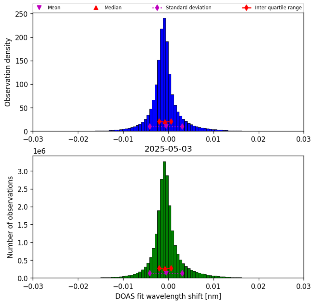
Figure 35: Histogram of “DOAS fit wavelength shift” for 2025-05-03 to 2025-05-03
