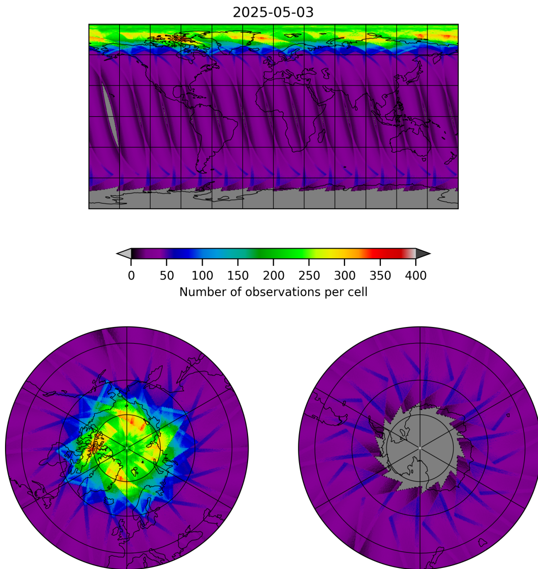
Figure 15: Map of the number of observations for 2025-05-03 to 2025-05-03
