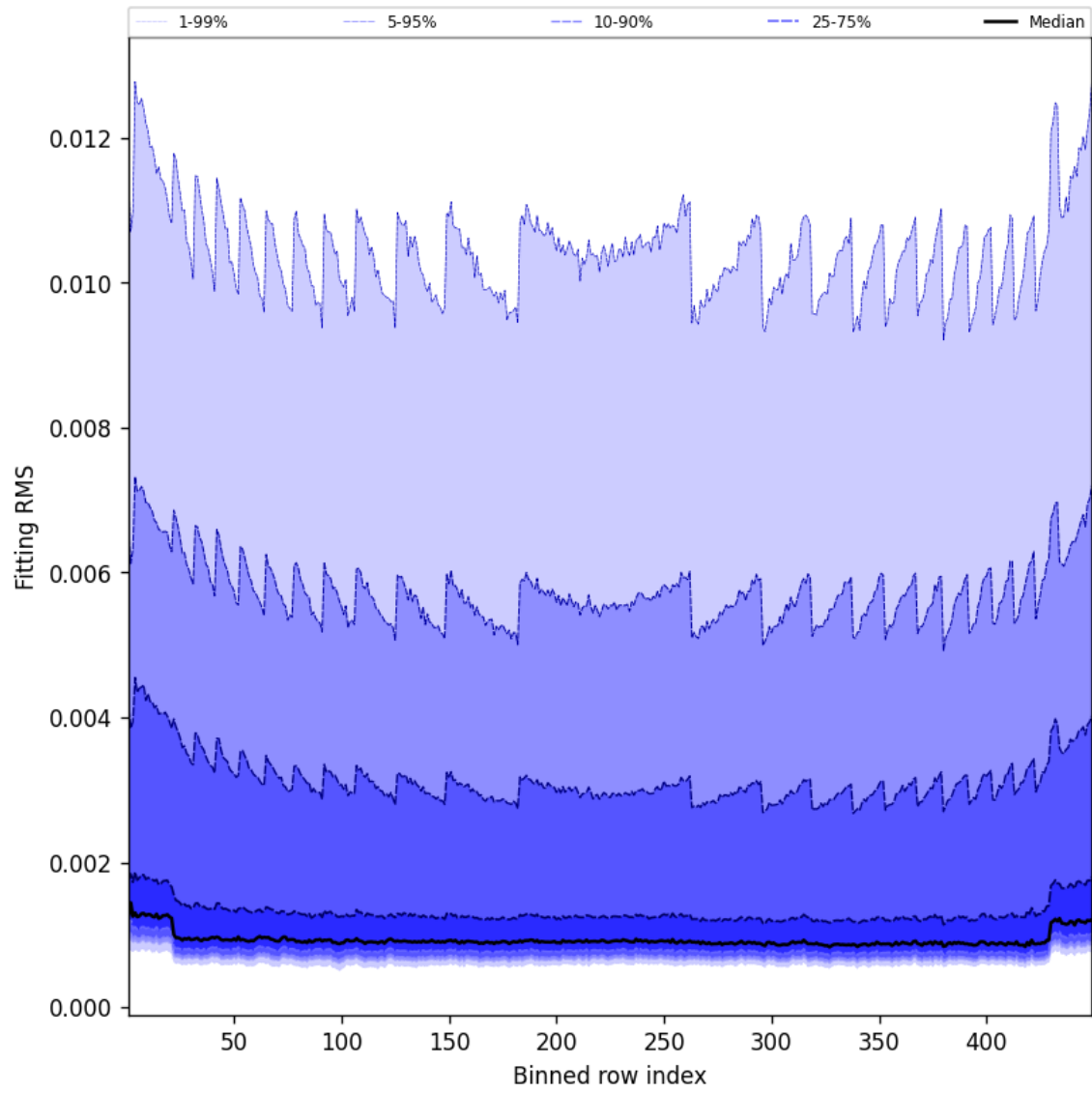
Figure 46: Along track statistics of “Fitting RMS” for 2025-05-03 to 2025-05-03
