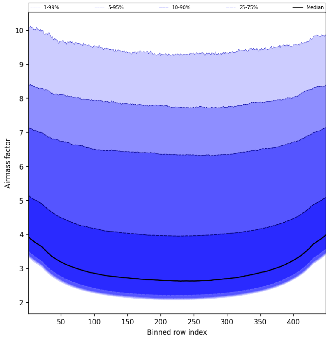
Figure 49: Along track statistics of “Airmass factor” for 2025-05-03 to 2025-05-03
