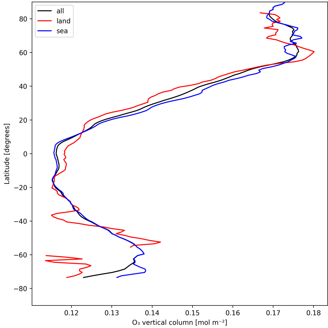
Figure 17: Zonal average of “O 3 vertical column” for 2025-05-03 to 2025-05-03.
