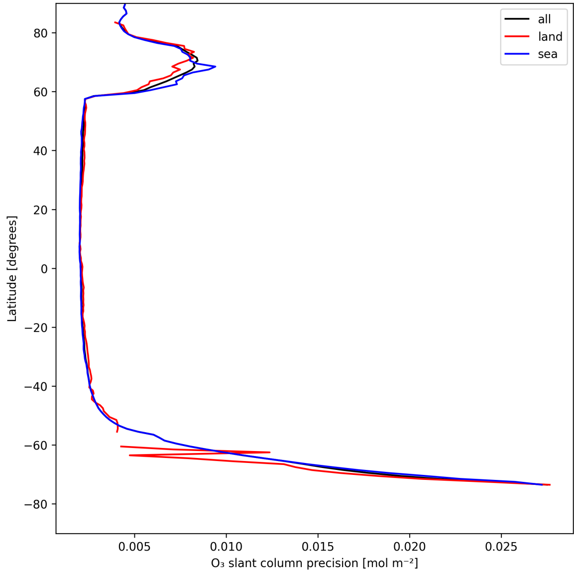
Figure 20: Zonal average of “O 3 slant column precision” for 2025-05-03 to 2025-05-03.
