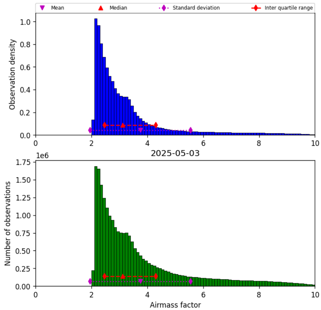
Figure 37: Histogram of “Airmass factor” for 2025-05-03 to 2025-05-03
