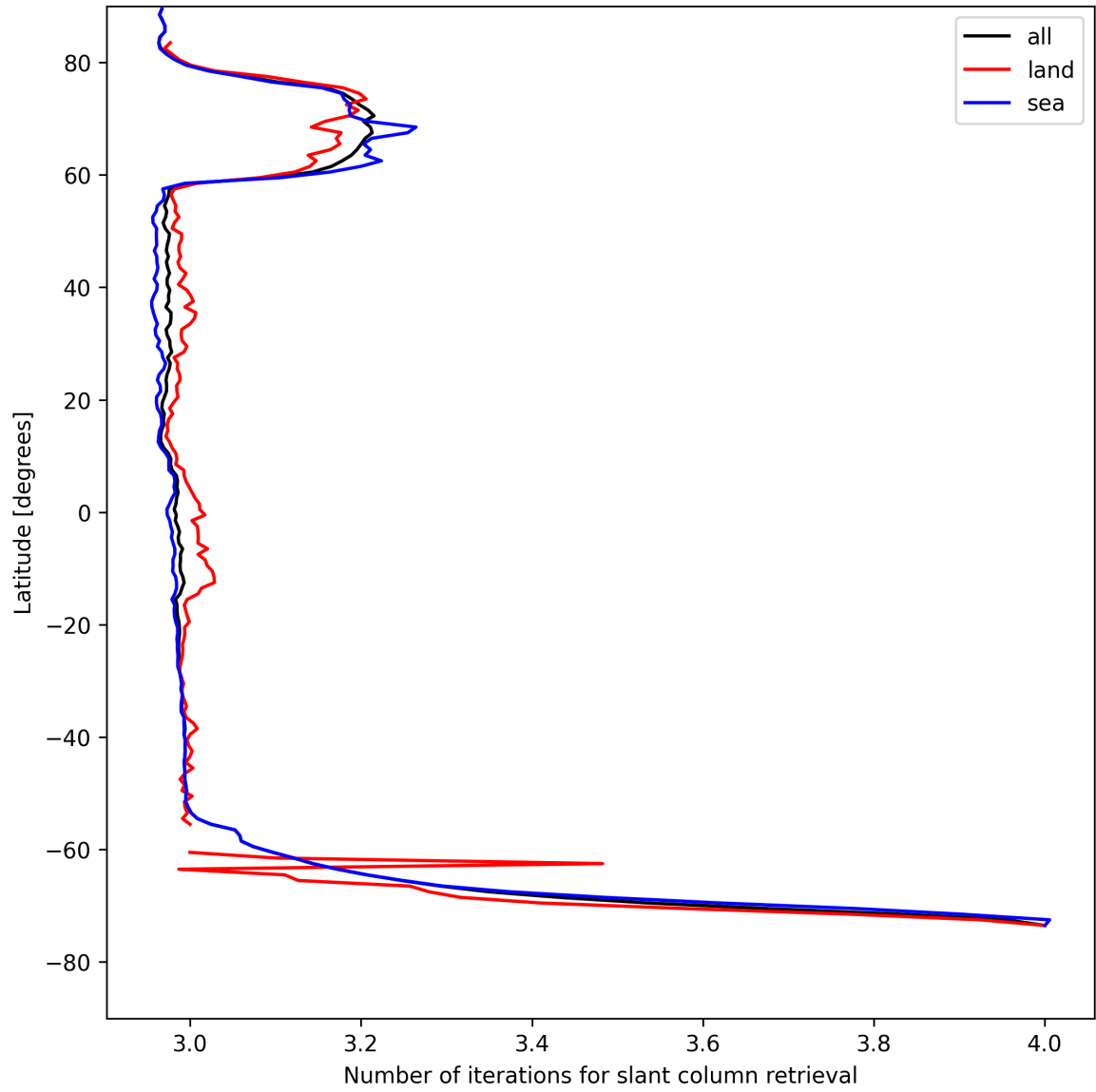
Figure 21: Zonal average of “Number of iterations for slant column retrieval” for 2025-05-03 to 2025-05-03.
