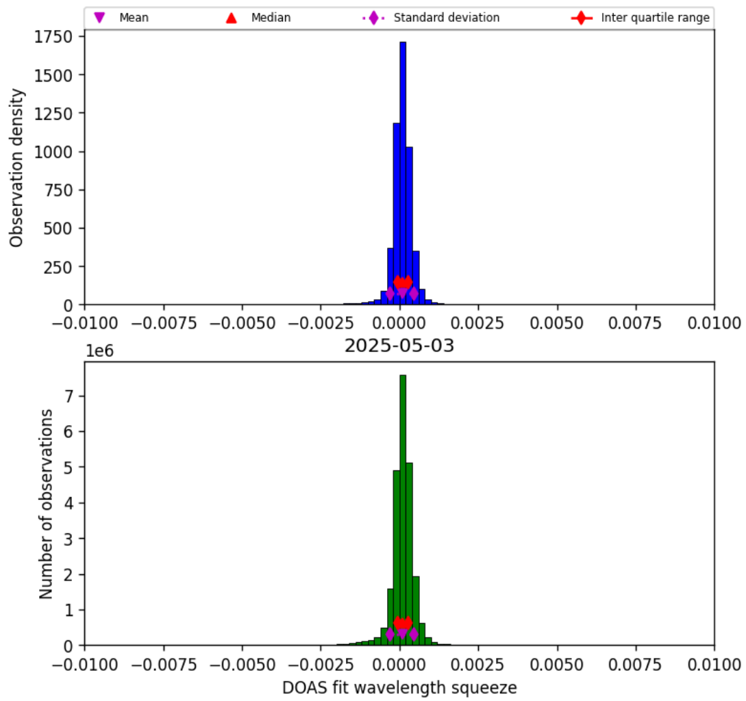
Figure 36: Histogram of “DOAS fit wavelength squeeze” for 2025-05-03 to 2025-05-03
