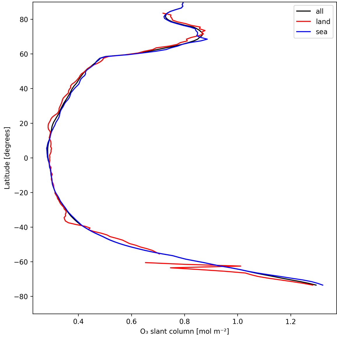
Figure 19: Zonal average of “O 3 slant column” for 2025-05-03 to 2025-05-03.
