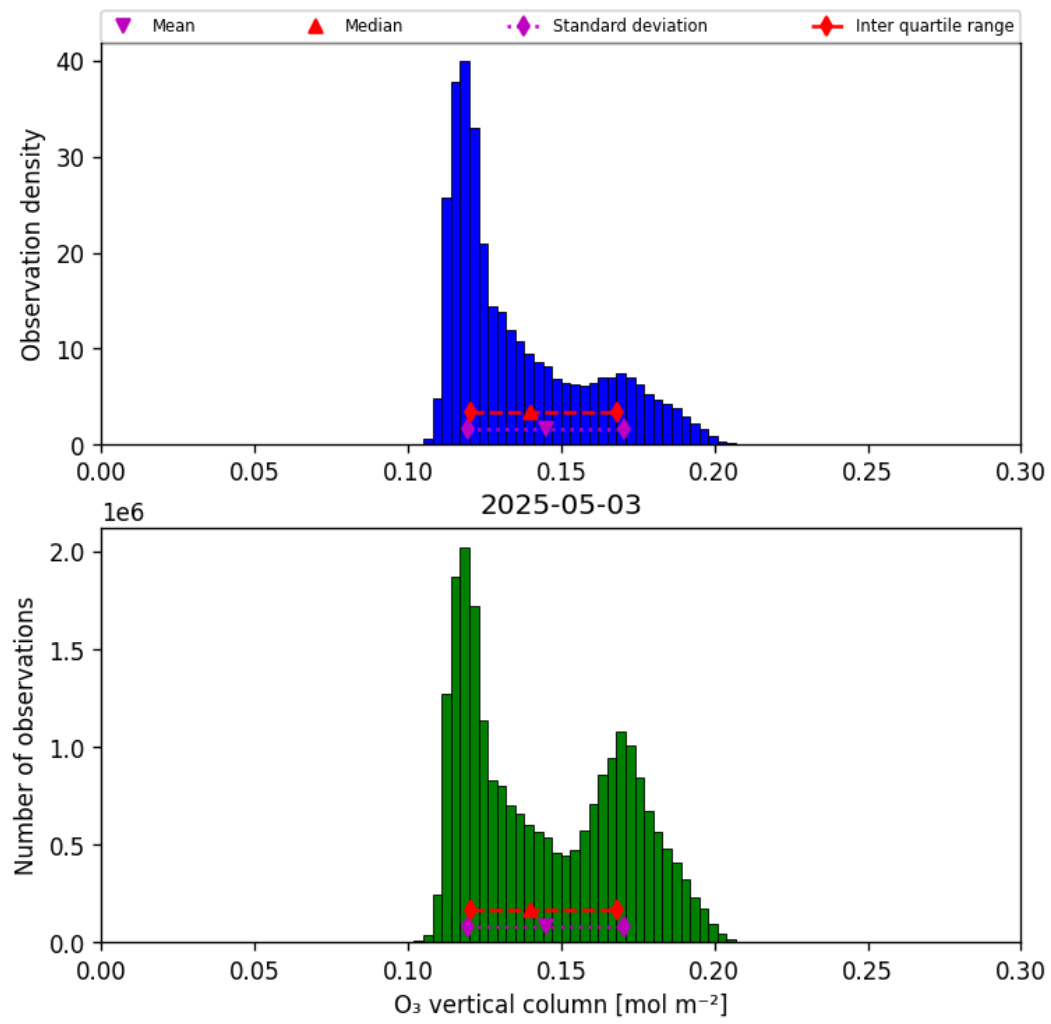
Figure 29: Histogram of “O 3 vertical column” for 2025-05-03 to 2025-05-03
