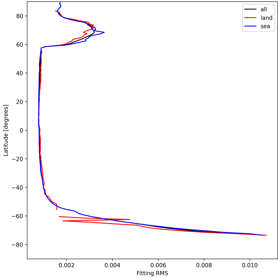
Figure 22: Zonal average of “Fitting RMS” for 2025-05-03 to 2025-05-03.
