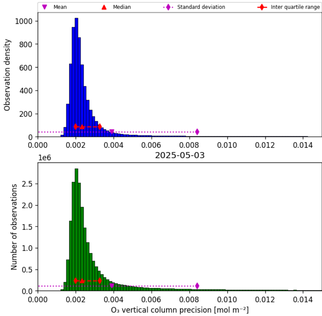
Figure 30: Histogram of "O 3 vertical column precision" for 2025-05-03 to 2025-05-03
