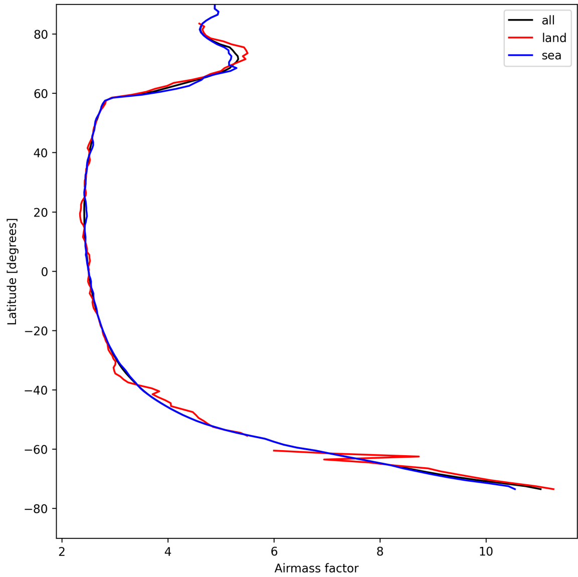
Figure 25: Zonal average of “Airmass factor” for 2025-05-03 to 2025-05-03.
