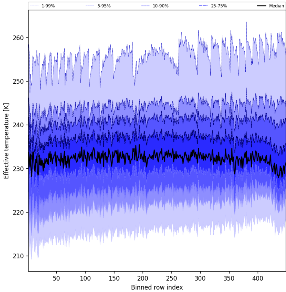
Figure 50: Along track statistics of “Effective temperature” for 2025-05-04 to 2025-05-05
