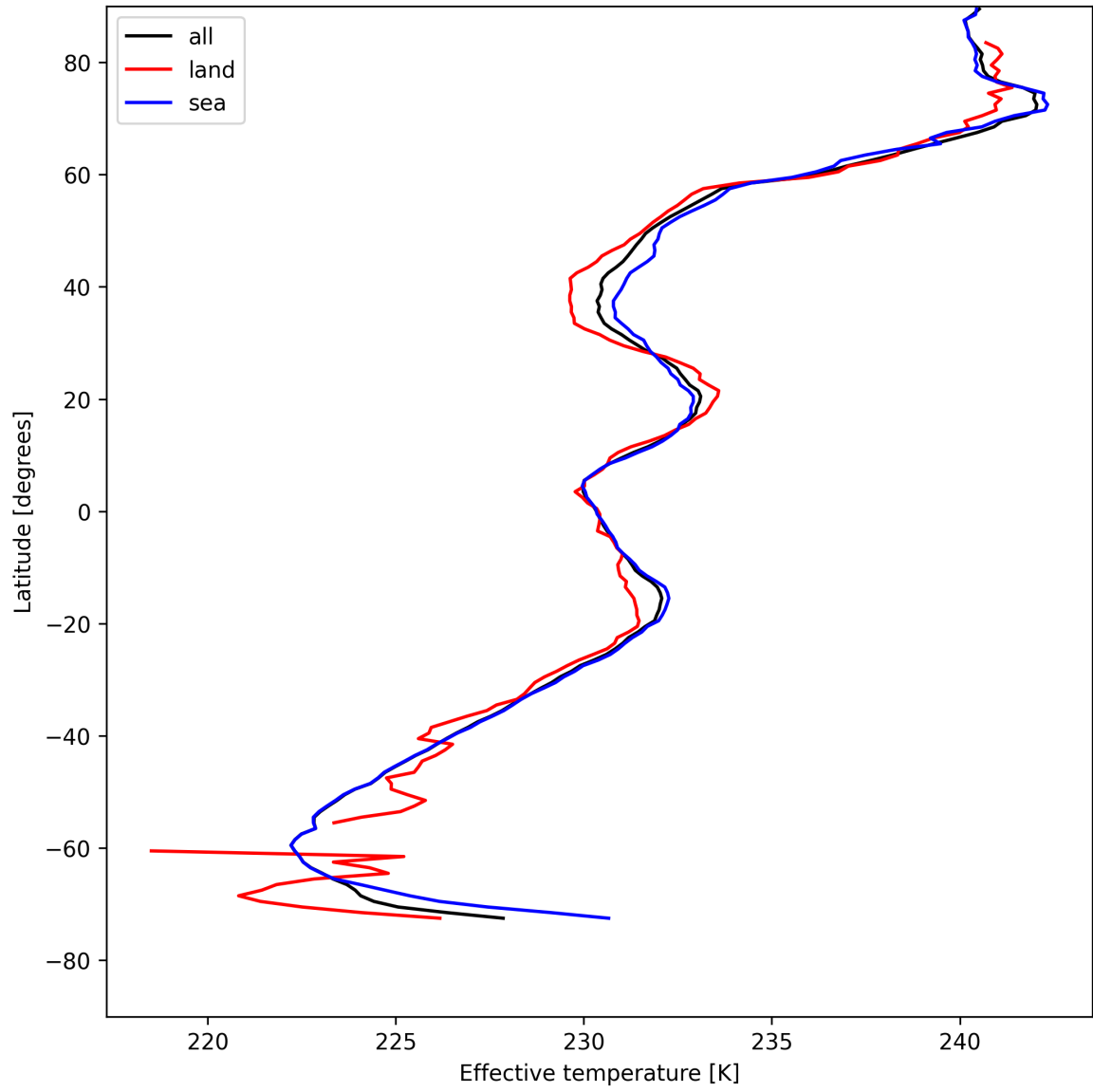
Figure 26: Zonal average of “Effective temperature” for 2025-05-04 to 2025-05-05.
