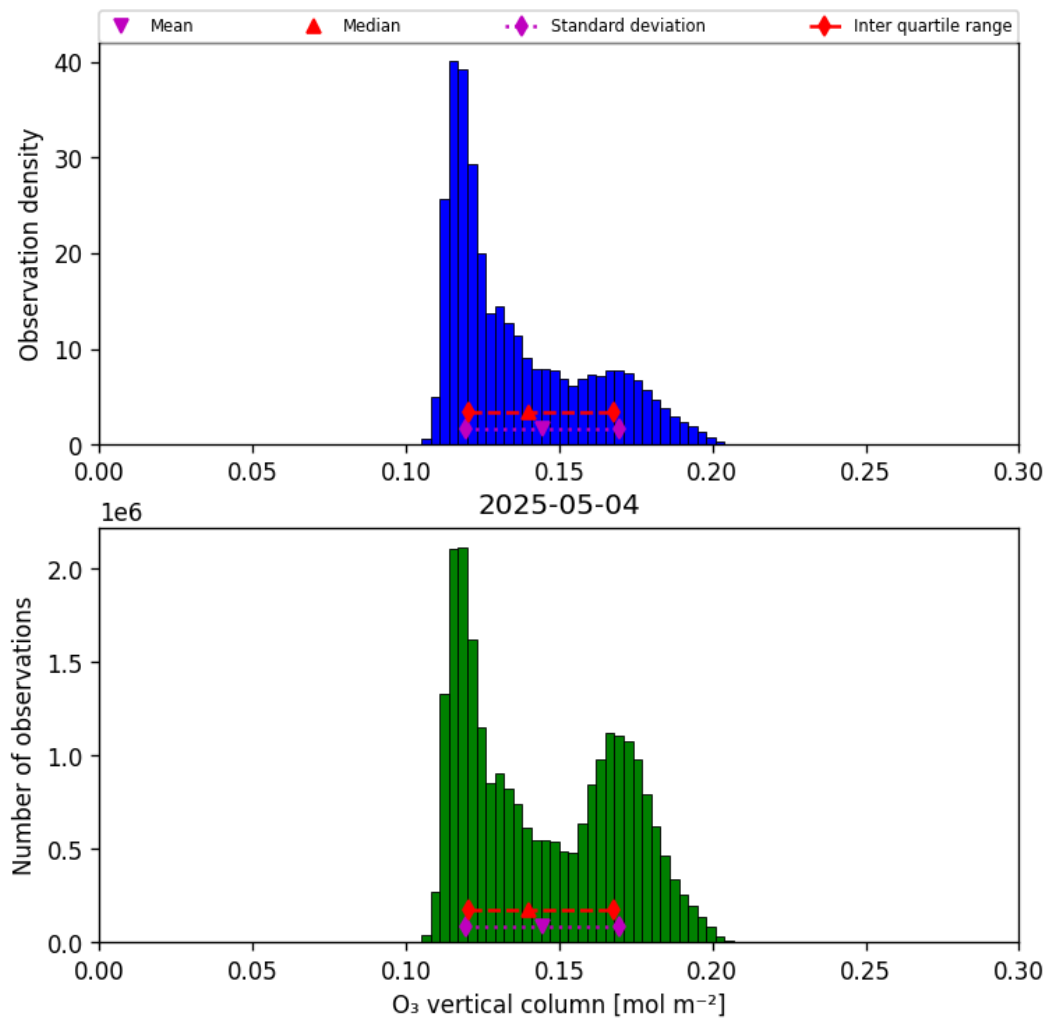
Figure 29: Histogram of “O 3 vertical column” for 2025-05-04 to 2025-05-05
