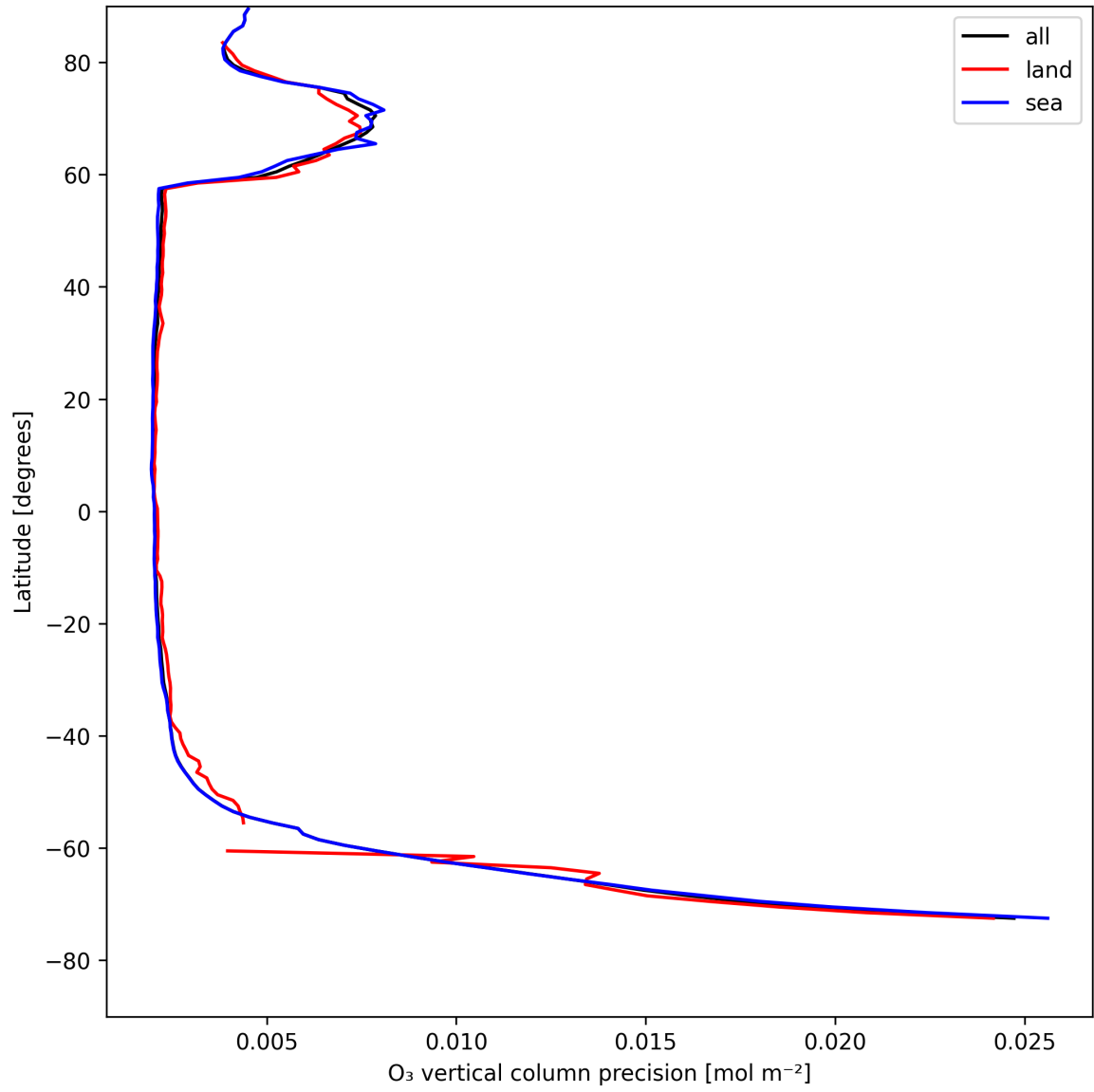
Figure 18: Zonal average of "O 3 vertical column precision" for 2025-05-04 to 2025-05-05.
