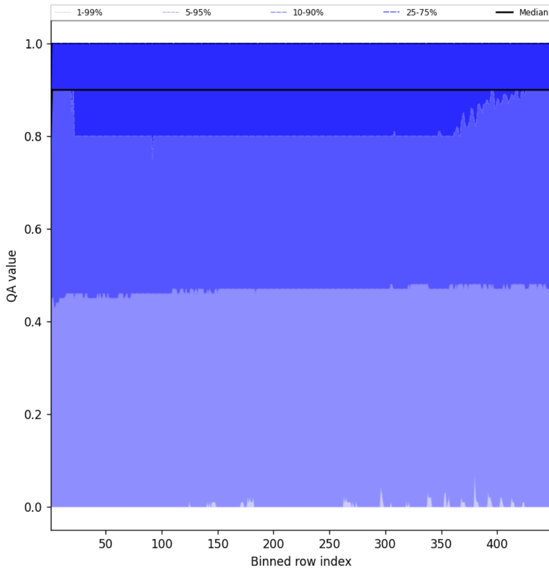
Figure 40: Along track statistics of “QA value” for 2025-05-04 to 2025-05-05
