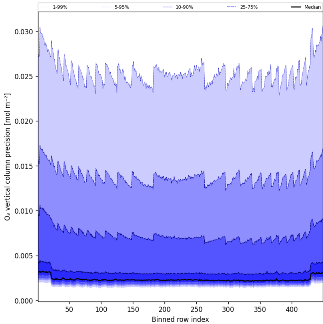
Figure 42: Along track statistics of “O 3 vertical column precision” for 2025-05-04 to 2025-05-05
