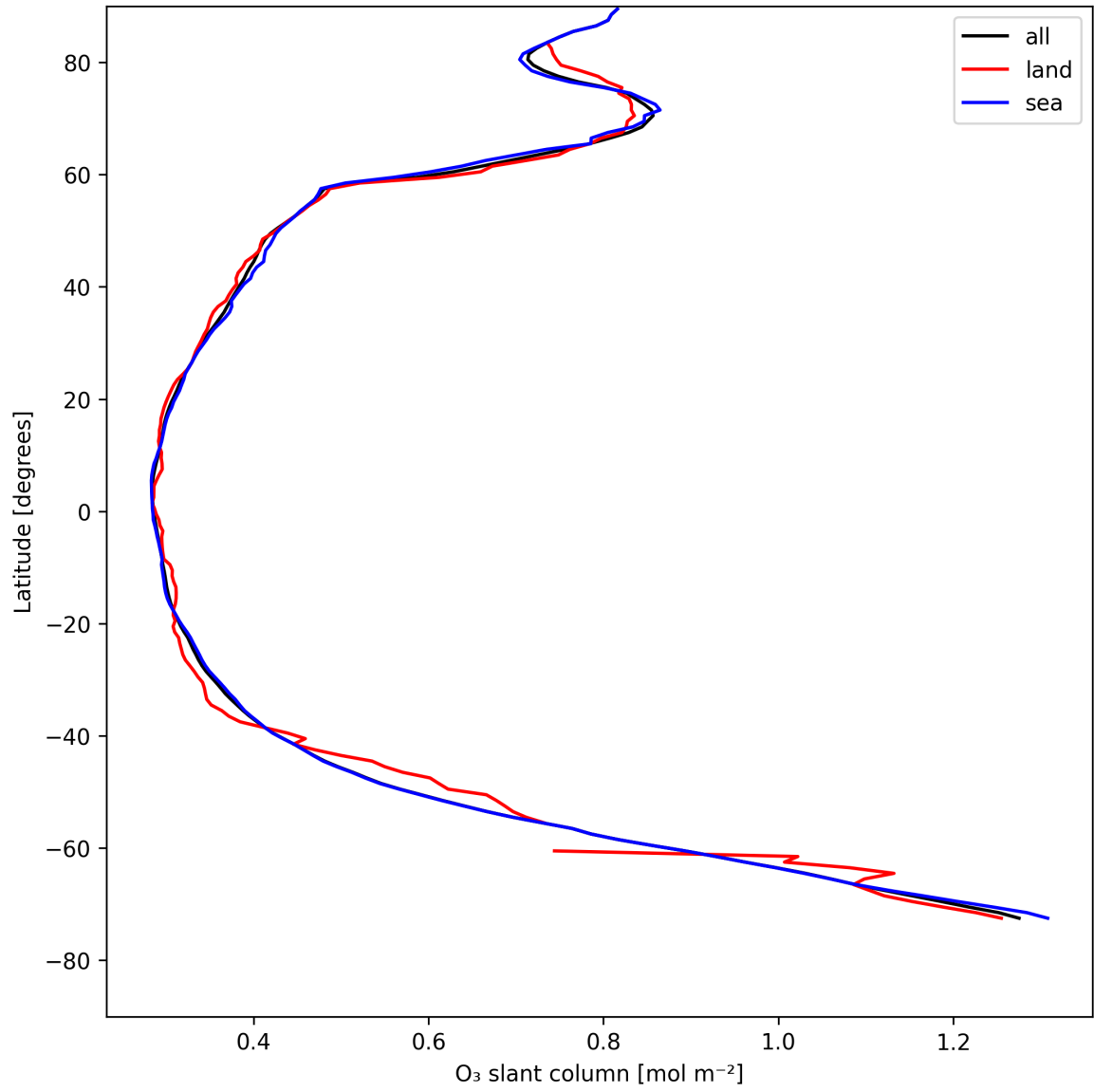
Figure 19: Zonal average of “O 3 slant column” for 2025-05-04 to 2025-05-05.
