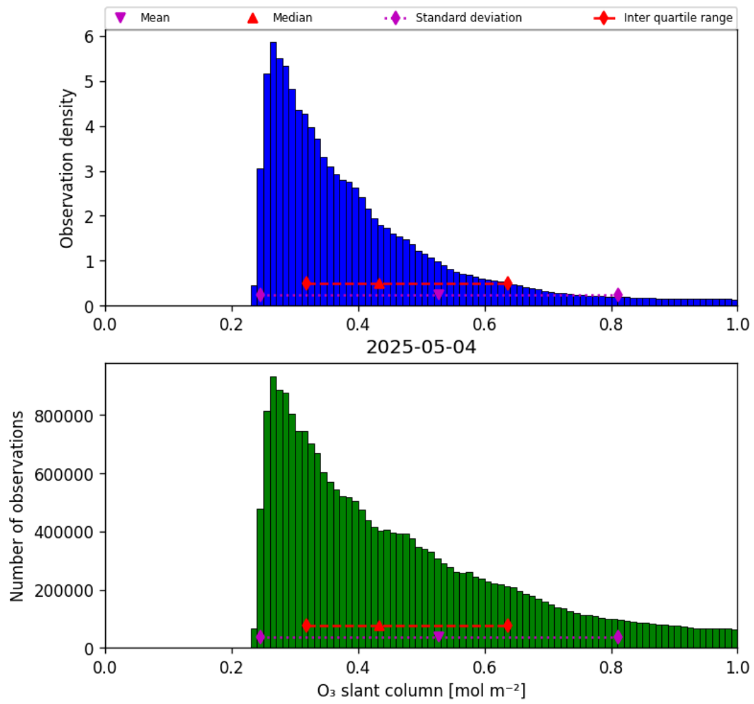
Figure 31: Histogram of “O 3 slant column” for 2025-05-04 to 2025-05-05
