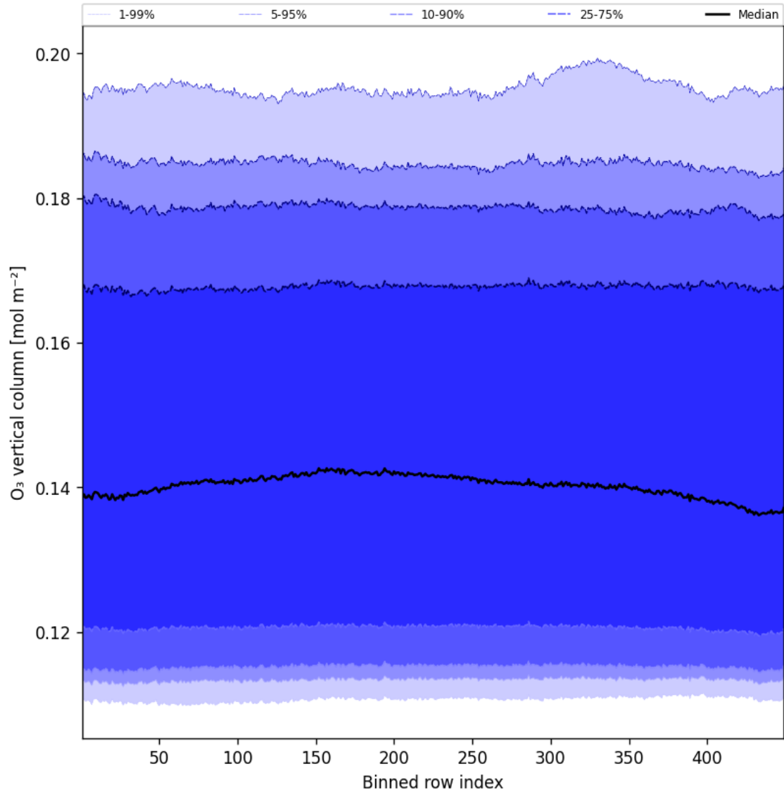
Figure 41: Along track statistics of “O 3 vertical column” for 2025-05-04 to 2025-05-05
