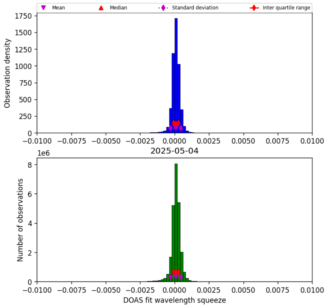
Figure 36: Histogram of “DOAS fit wavelength squeeze” for 2025-05-04 to 2025-05-05
