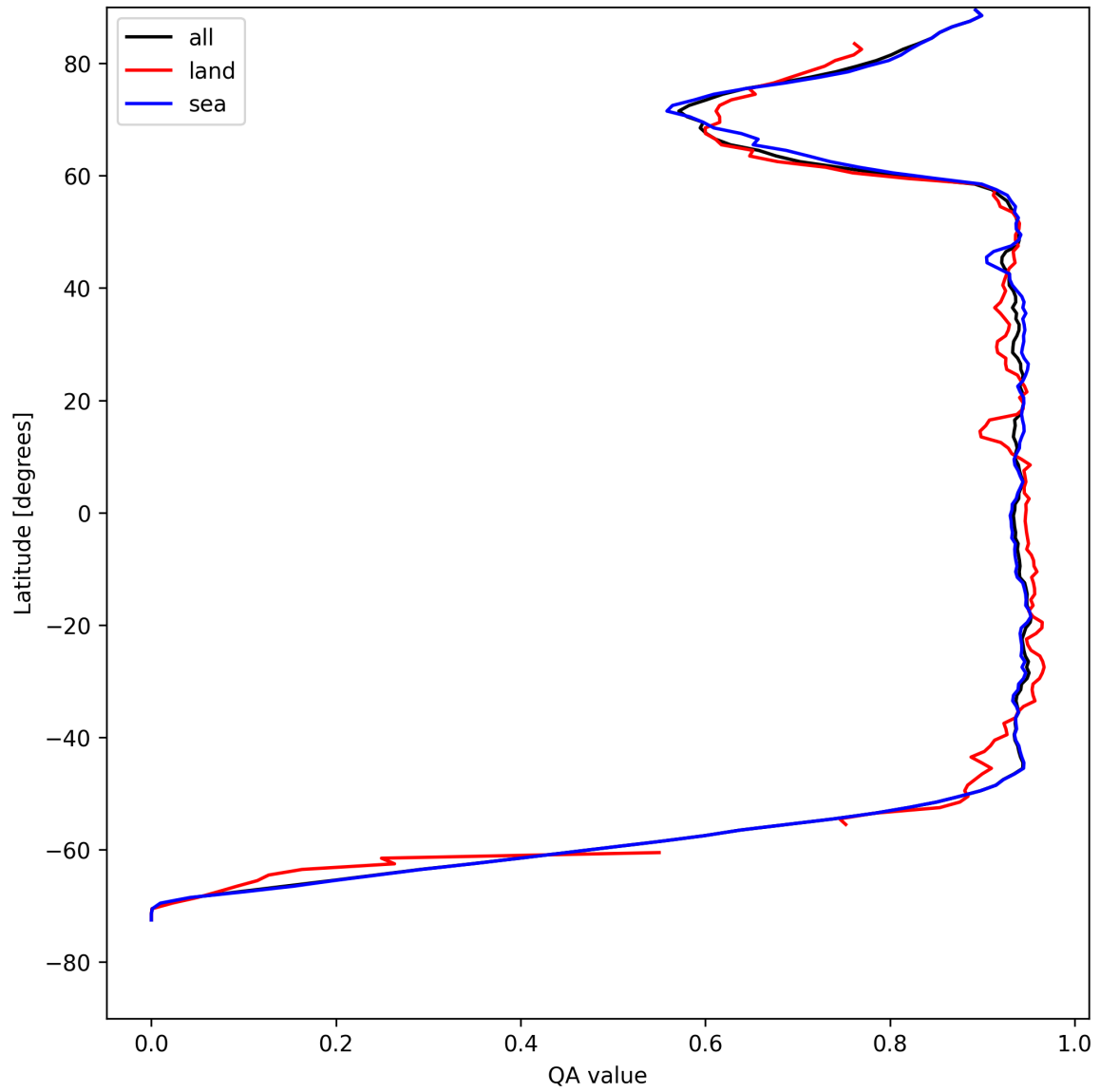
Figure 16: Zonal average of “QA value” for 2025-05-04 to 2025-05-05.
