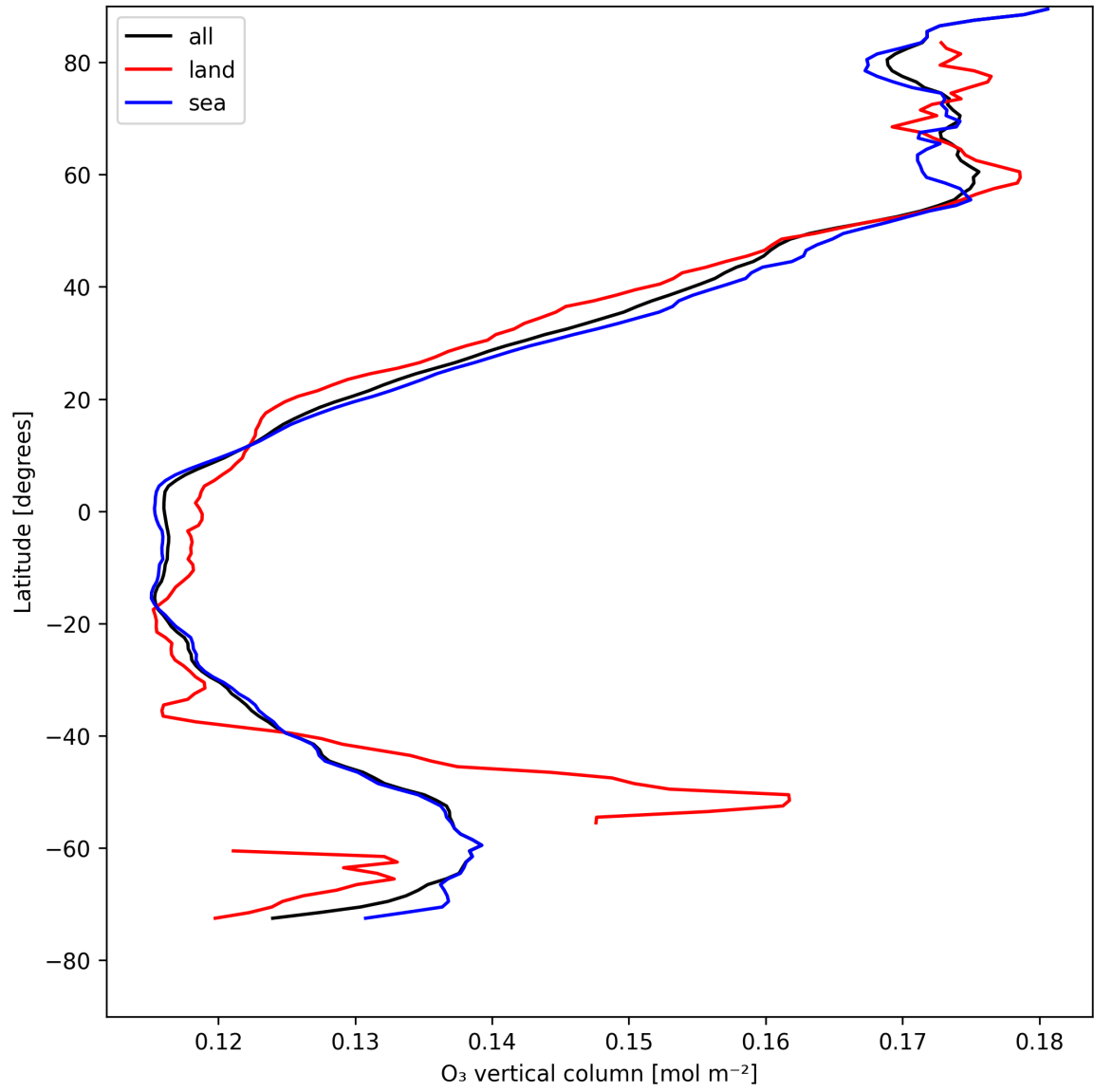
Figure 17: Zonal average of “O 3 vertical column” for 2025-05-04 to 2025-05-05.
