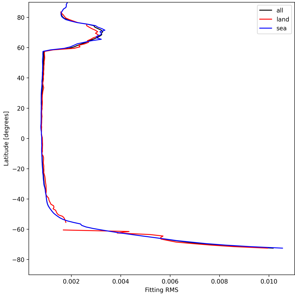
Figure 22: Zonal average of “Fitting RMS” for 2025-05-04 to 2025-05-05.
