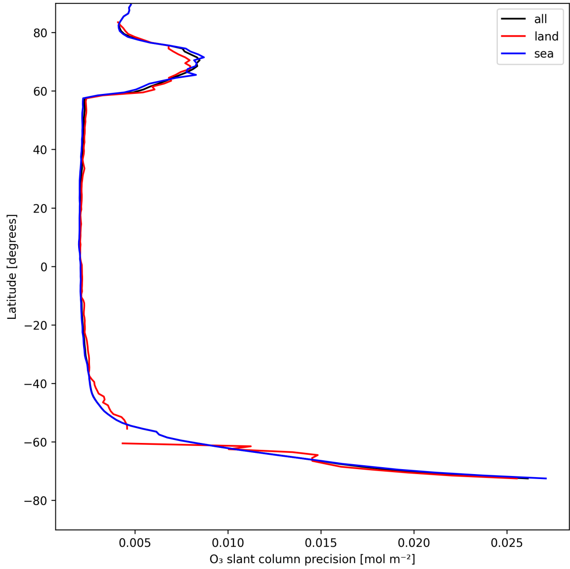
Figure 20: Zonal average of “O 3 slant column precision” for 2025-05-04 to 2025-05-05.
