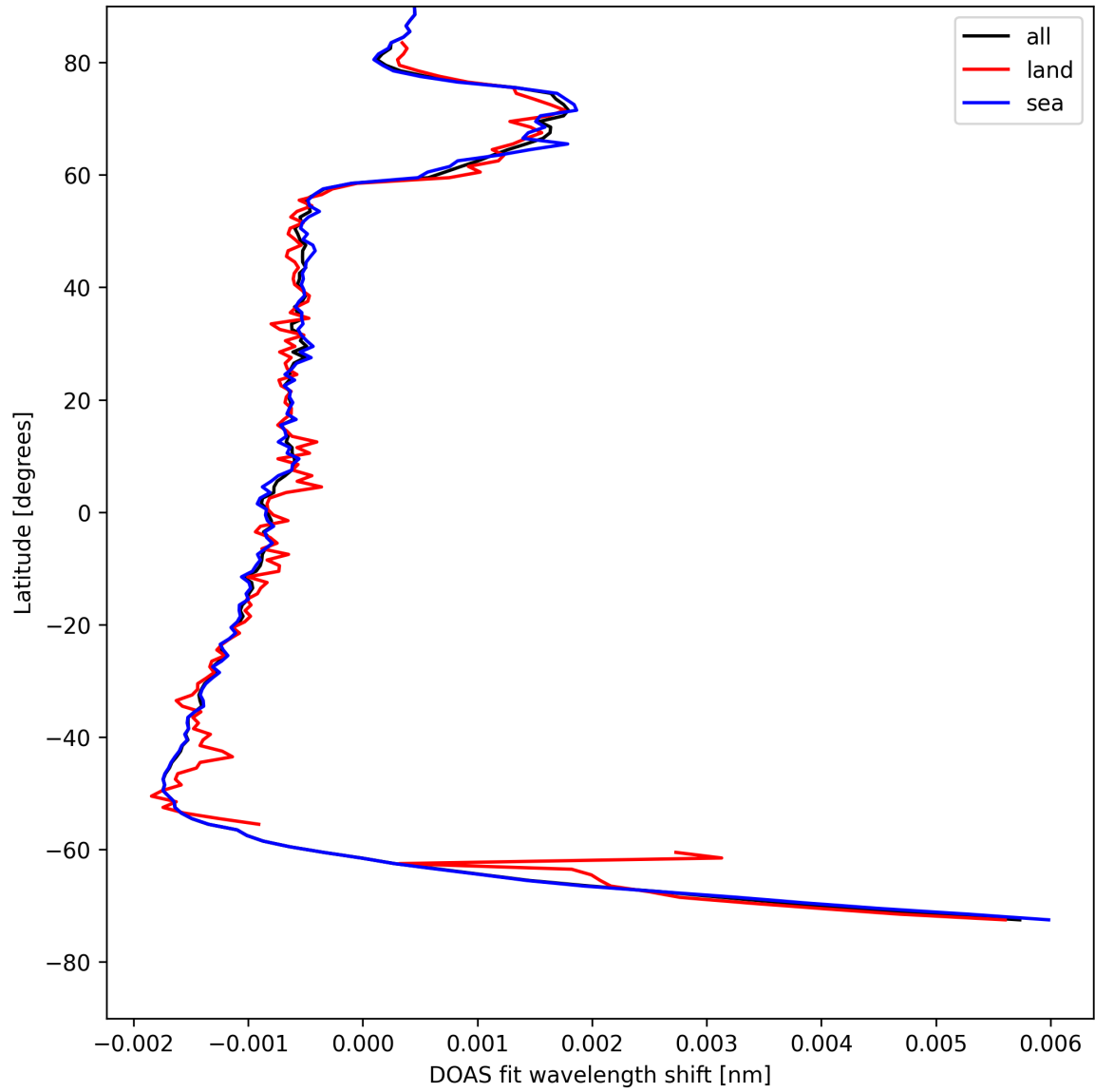
Figure 23: Zonal average of “DOAS fit wavelength shift” for 2025-05-04 to 2025-05-05.
