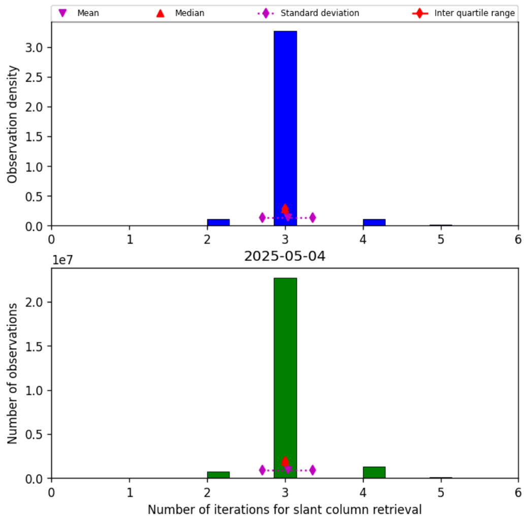
Figure 33: Histogram of “Number of iterations for slant column retrieval” for 2025-05-04 to 2025-05-05
