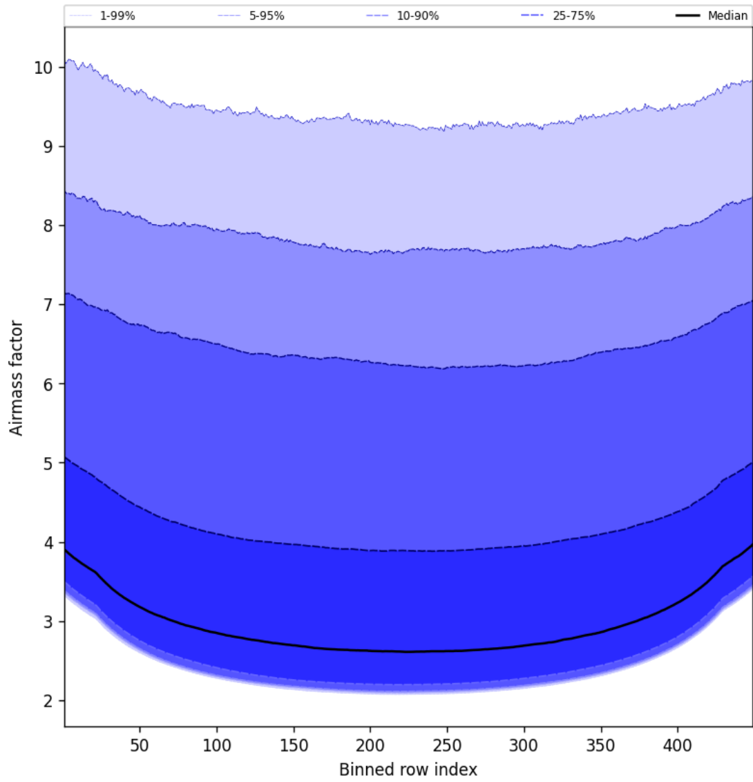
Figure 49: Along track statistics of “Airmass factor” for 2025-05-04 to 2025-05-05
