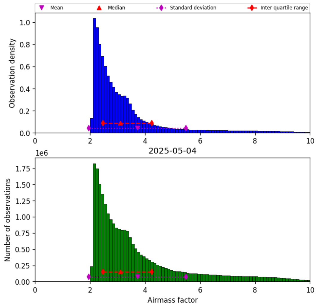
Figure 37: Histogram of “Airmass factor” for 2025-05-04 to 2025-05-05
