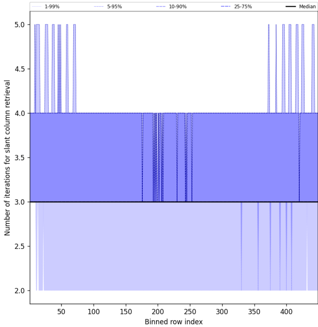
Figure 45: Along track statistics of “Number of iterations for slant column retrieval” for 2025-05-04 to 2025-05-05
