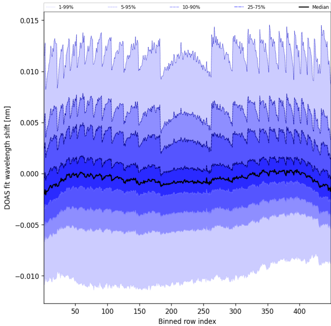
Figure 47: Along track statistics of "DOAS fit wavelength shift" for 2025-05-04 to 2025-05-05
