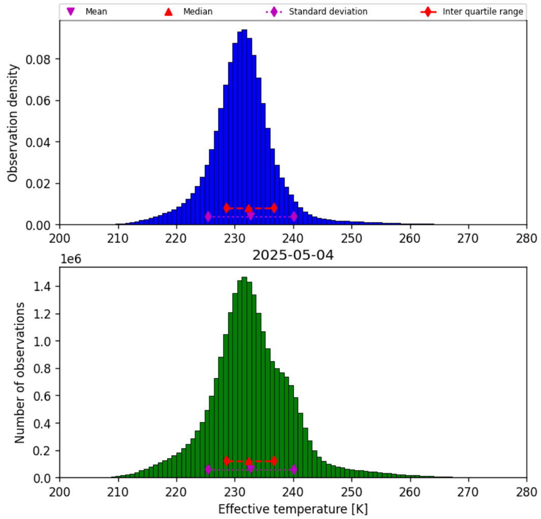
Figure 38: Histogram of “Effective temperature” for 2025-05-04 to 2025-05-05
