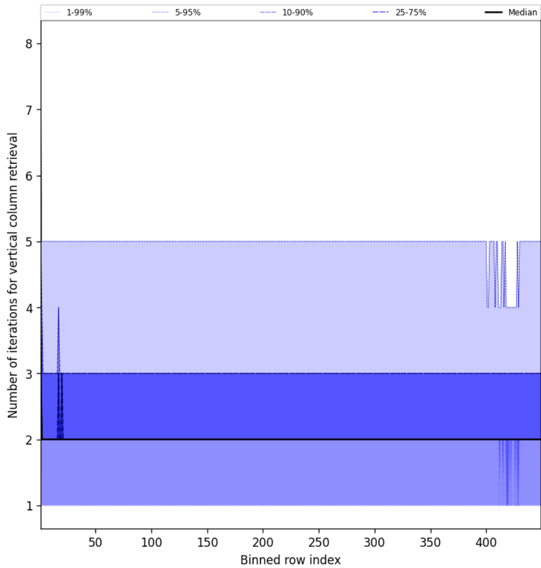
Figure 51: Along track statistics of “Number of iterations for vertical column retrieval” for 2025-05-04 to 2025-05-05
