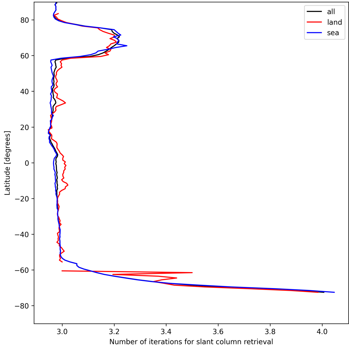
Figure 21: Zonal average of “Number of iterations for slant column retrieval” for 2025-05-04 to 2025-05-05.
