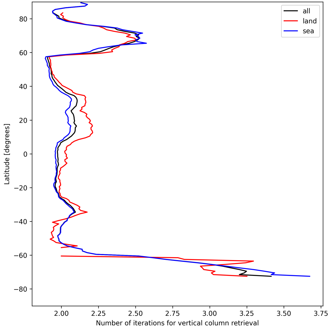
Figure 27: Zonal average of “Number of iterations for vertical column retrieval” for 2025-05-04 to 2025-05-05.
