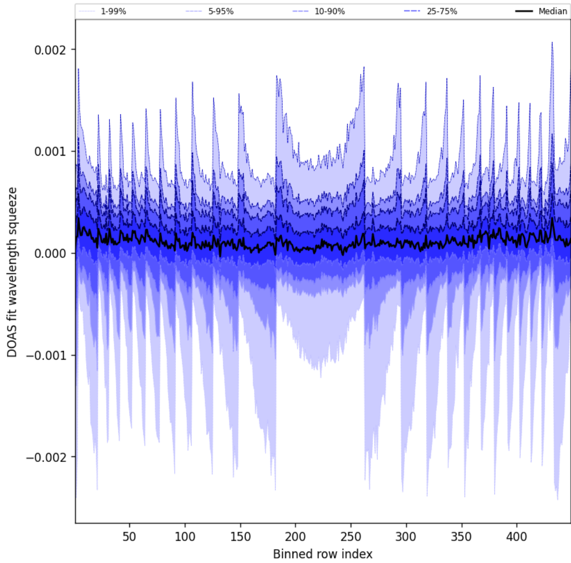
Figure 48: Along track statistics of “DOAS fit wavelength squeeze” for 2025-05-04 to 2025-05-05
