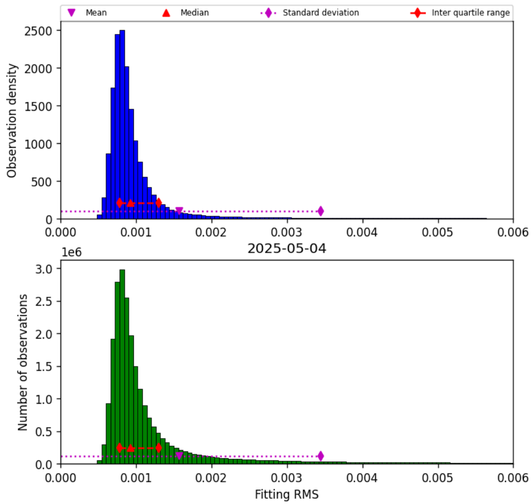
Figure 34: Histogram of “Fitting RMS” for 2025-05-04 to 2025-05-05
