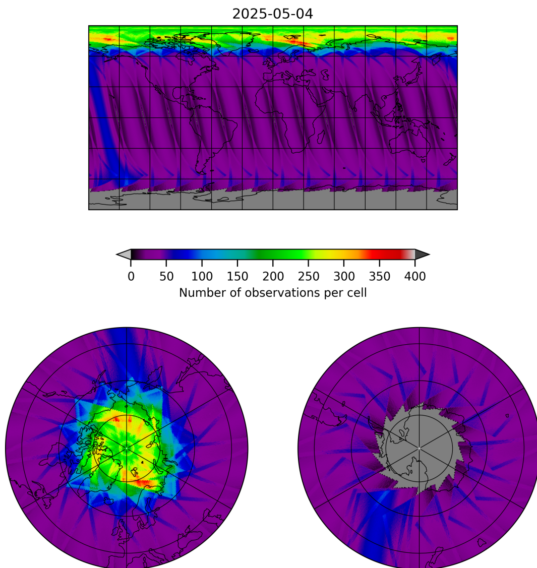
Figure 15: Map of the number of observations for 2025-05-04 to 2025-05-05
