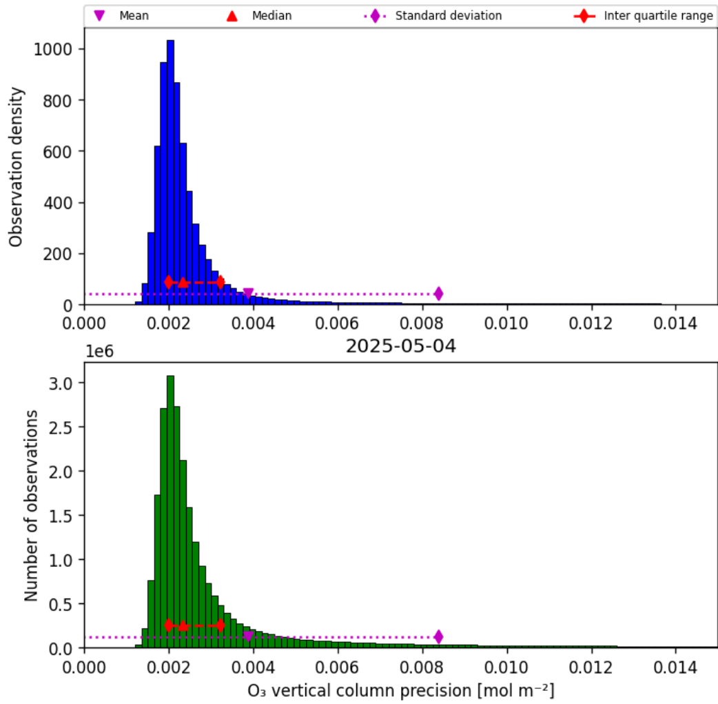
Figure 30: Histogram of “O 3 vertical column precision” for 2025-05-04 to 2025-05-05
