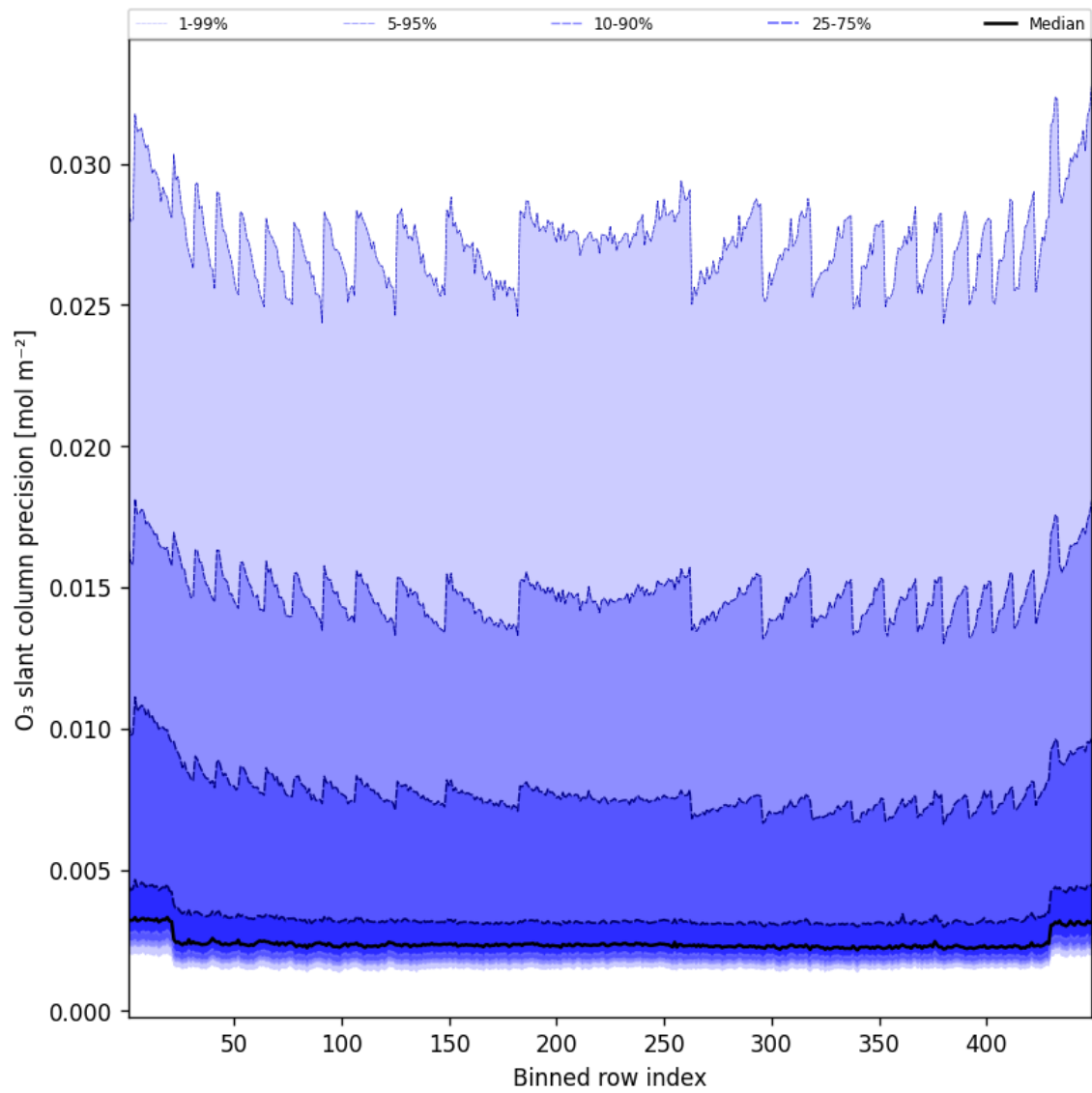
Figure 44: Along track statistics of “O 3 slant column precision” for 2025-05-04 to 2025-05-05
