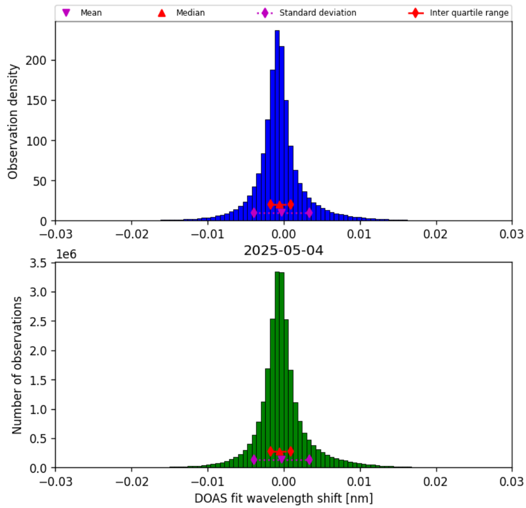
Figure 35: Histogram of “DOAS fit wavelength shift” for 2025-05-04 to 2025-05-05
