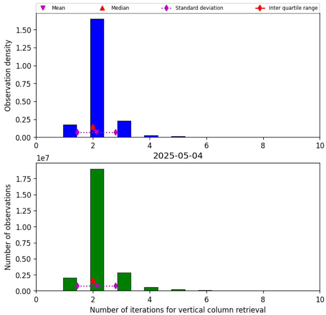
Figure 39: Histogram of “Number of iterations for vertical column retrieval” for 2025-05-04 to 2025-05-05
