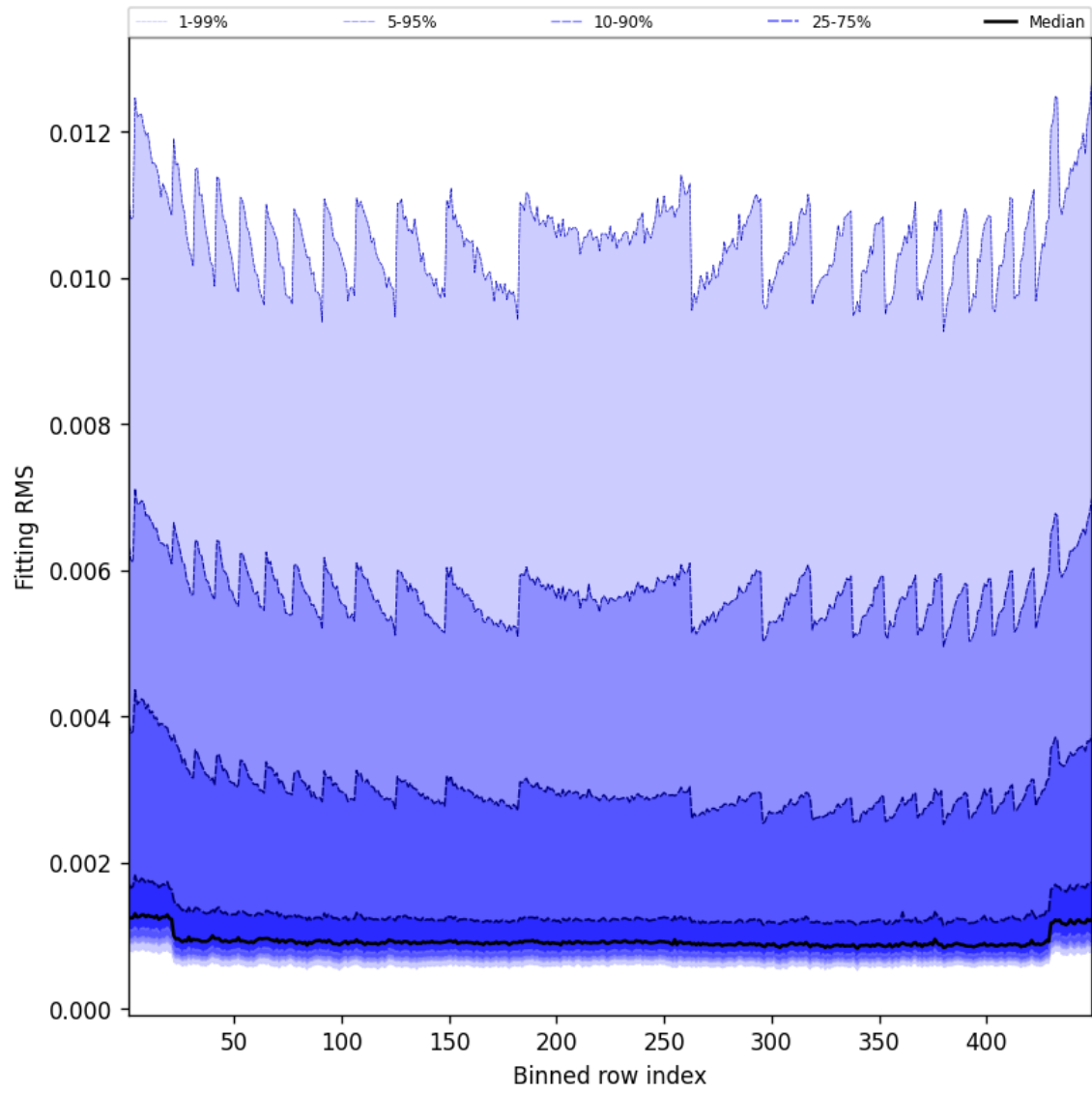
Figure 46: Along track statistics of “Fitting RMS” for 2025-05-04 to 2025-05-05
