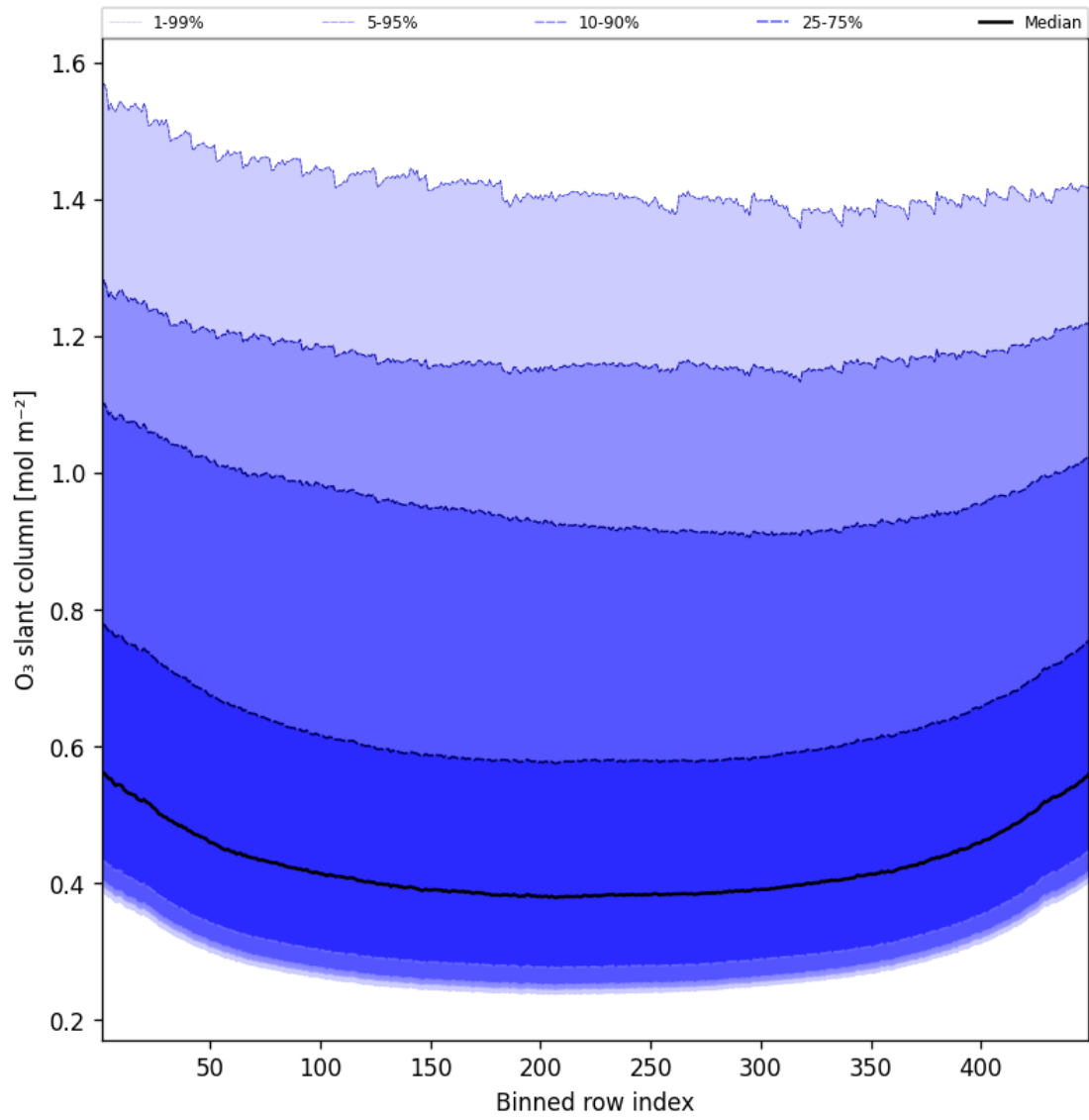
Figure 43: Along track statistics of “O 3 slant column” for 2025-05-04 to 2025-05-05
