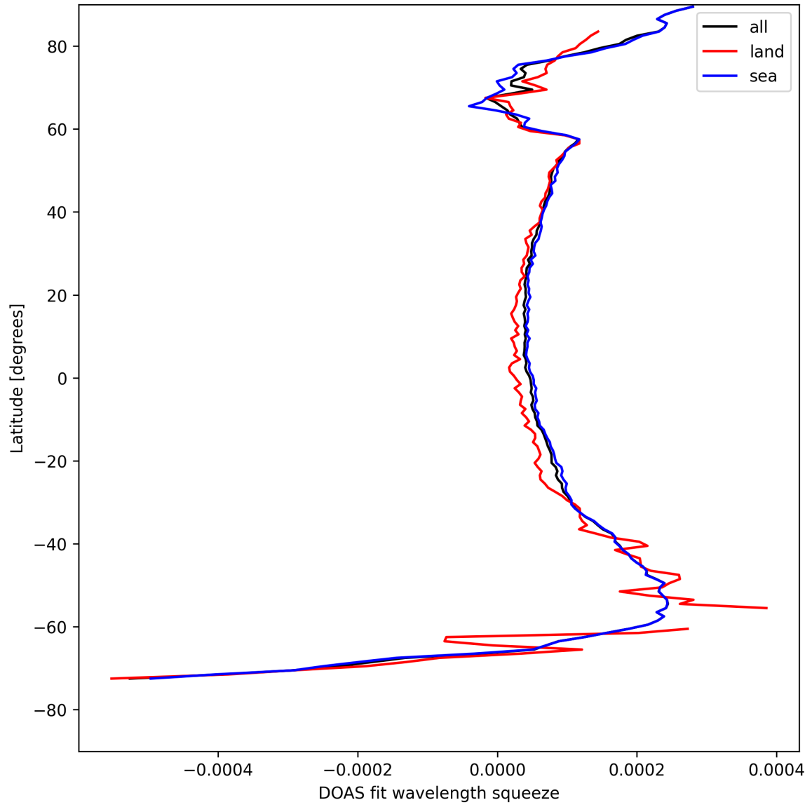
Figure 24: Zonal average of “DOAS fit wavelength squeeze” for 2025-05-04 to 2025-05-05.
