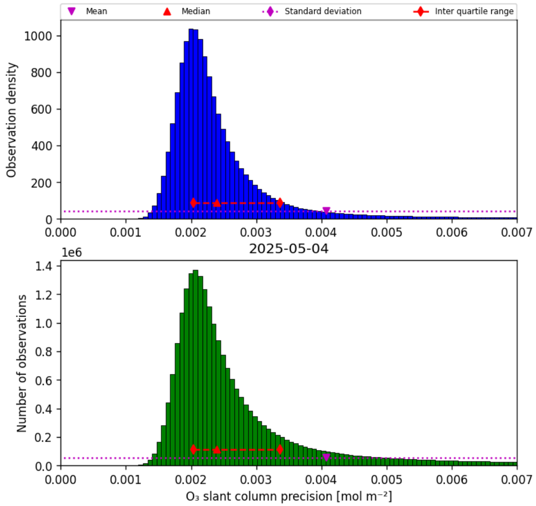
Figure 32: Histogram of “O 3 slant column precision” for 2025-05-04 to 2025-05-05
