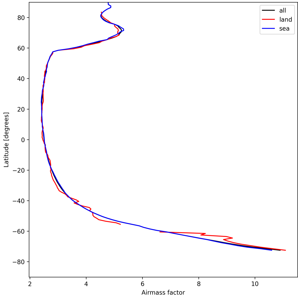
Figure 25: Zonal average of “Airmass factor” for 2025-05-04 to 2025-05-05.
