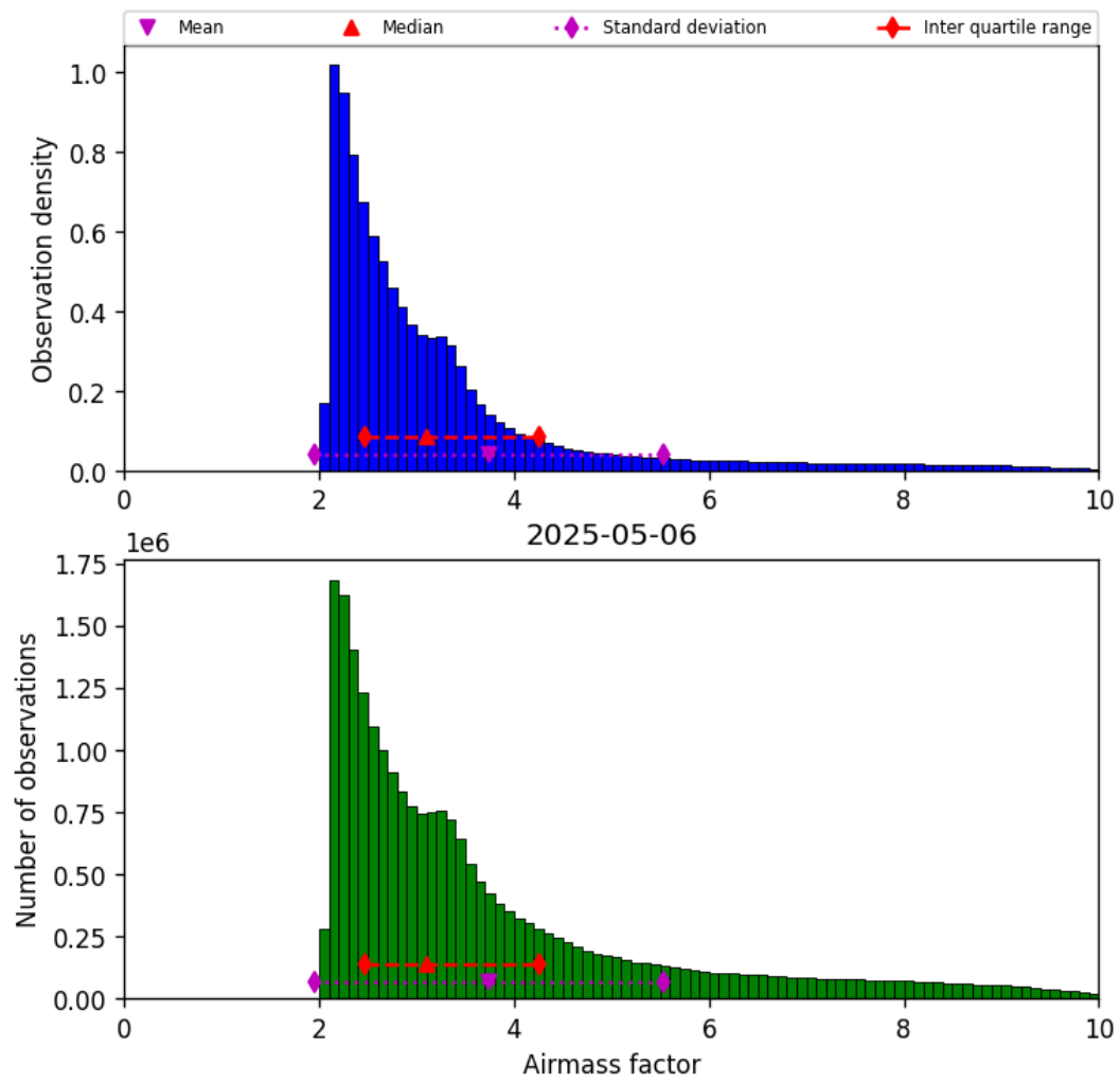
Figure 37: Histogram of “Airmass factor” for 2025-05-06 to 2025-05-07
