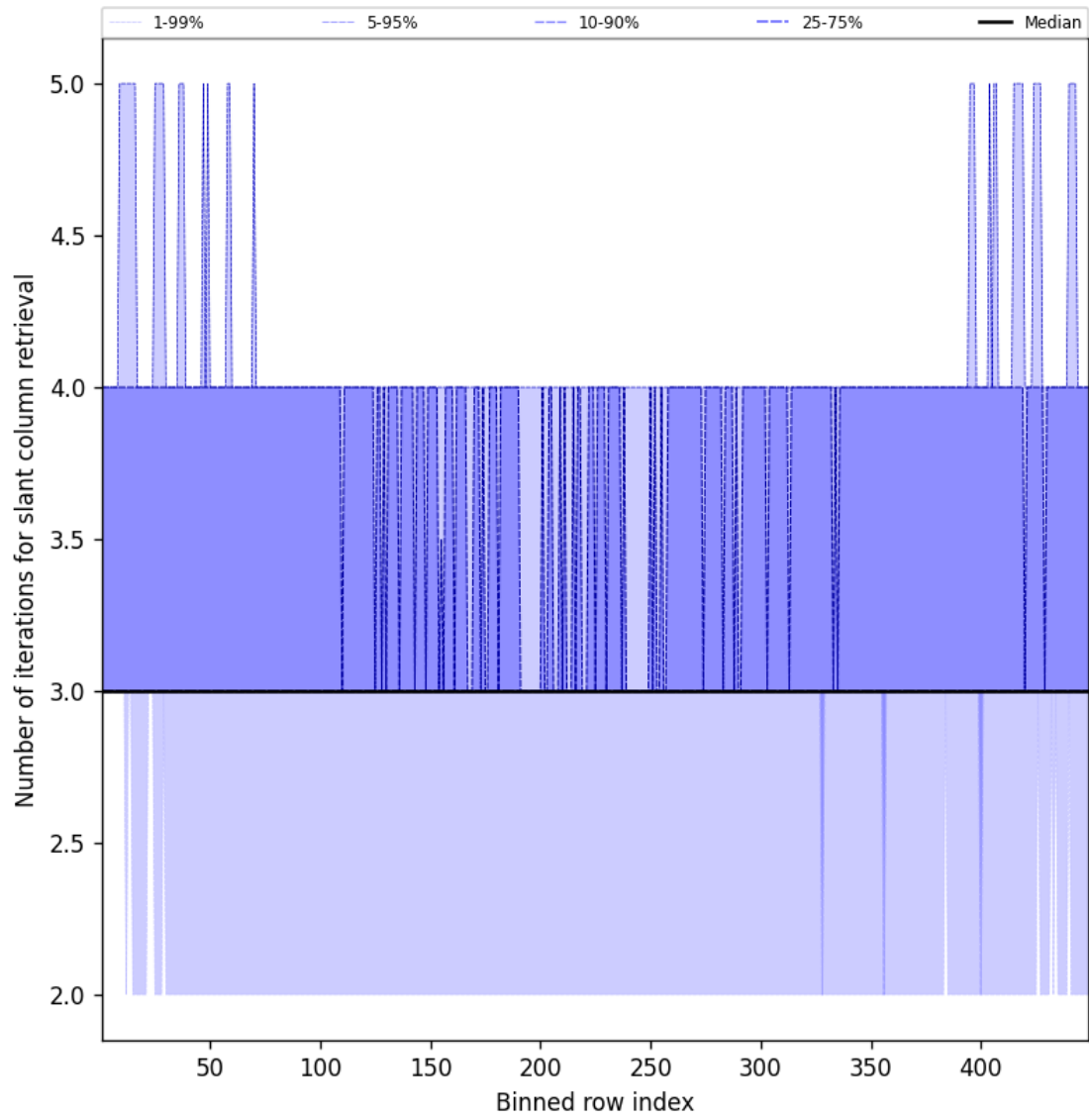
Figure 45: Along track statistics of “Number of iterations for slant column retrieval” for 2025-05-06 to 2025-05-07
