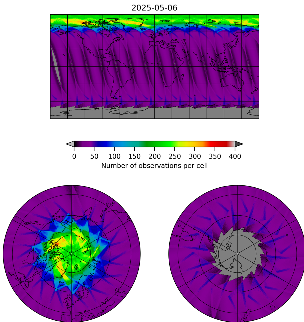
Figure 15: Map of the number of observations for 2025-05-06 to 2025-05-07
