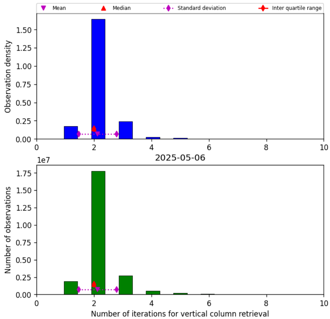
Figure 39: Histogram of “Number of iterations for vertical column retrieval” for 2025-05-06 to 2025-05-07
