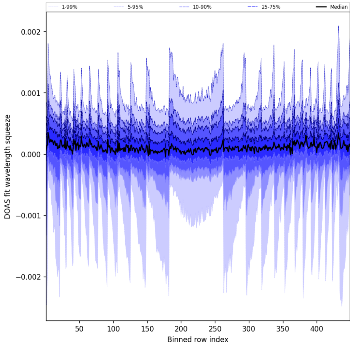
Figure 48: Along track statistics of “DOAS fit wavelength squeeze” for 2025-05-06 to 2025-05-07
