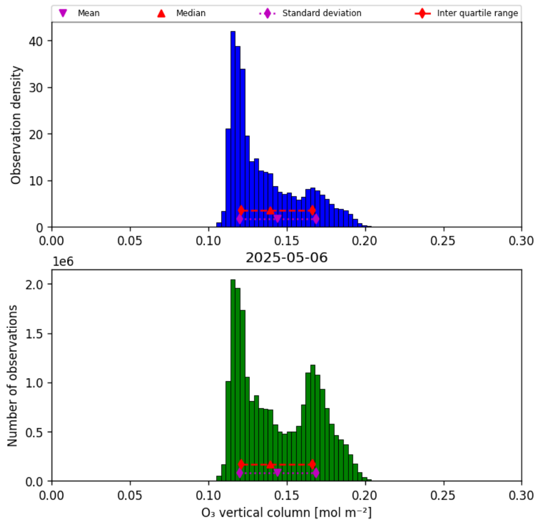
Figure 29: Histogram of “O 3 vertical column” for 2025-05-06 to 2025-05-07
