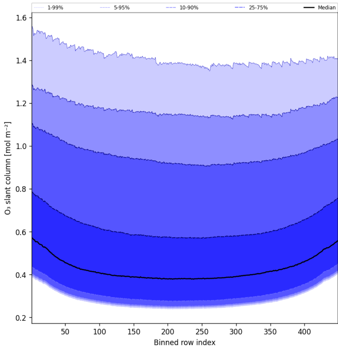
Figure 43: Along track statistics of “O 3 slant column” for 2025-05-06 to 2025-05-07
