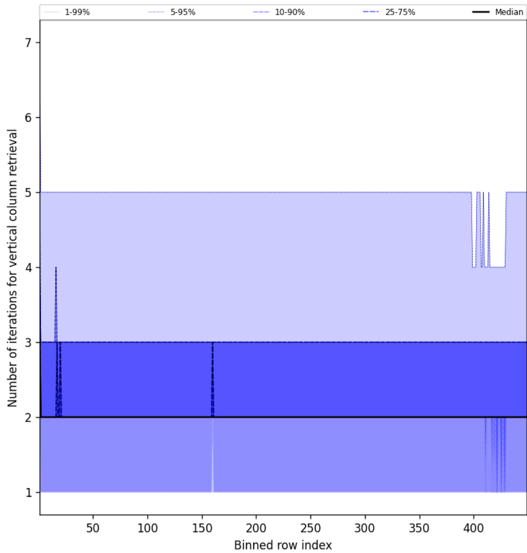
Figure 51: Along track statistics of “Number of iterations for vertical column retrieval” for 2025-05-06 to 2025-05-07
