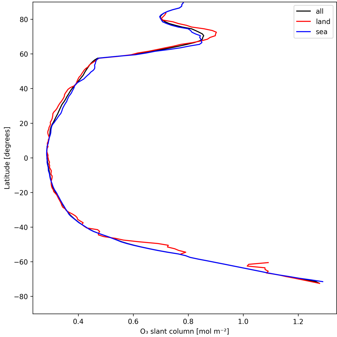
Figure 19: Zonal average of “O 3 slant column” for 2025-05-06 to 2025-05-07.
