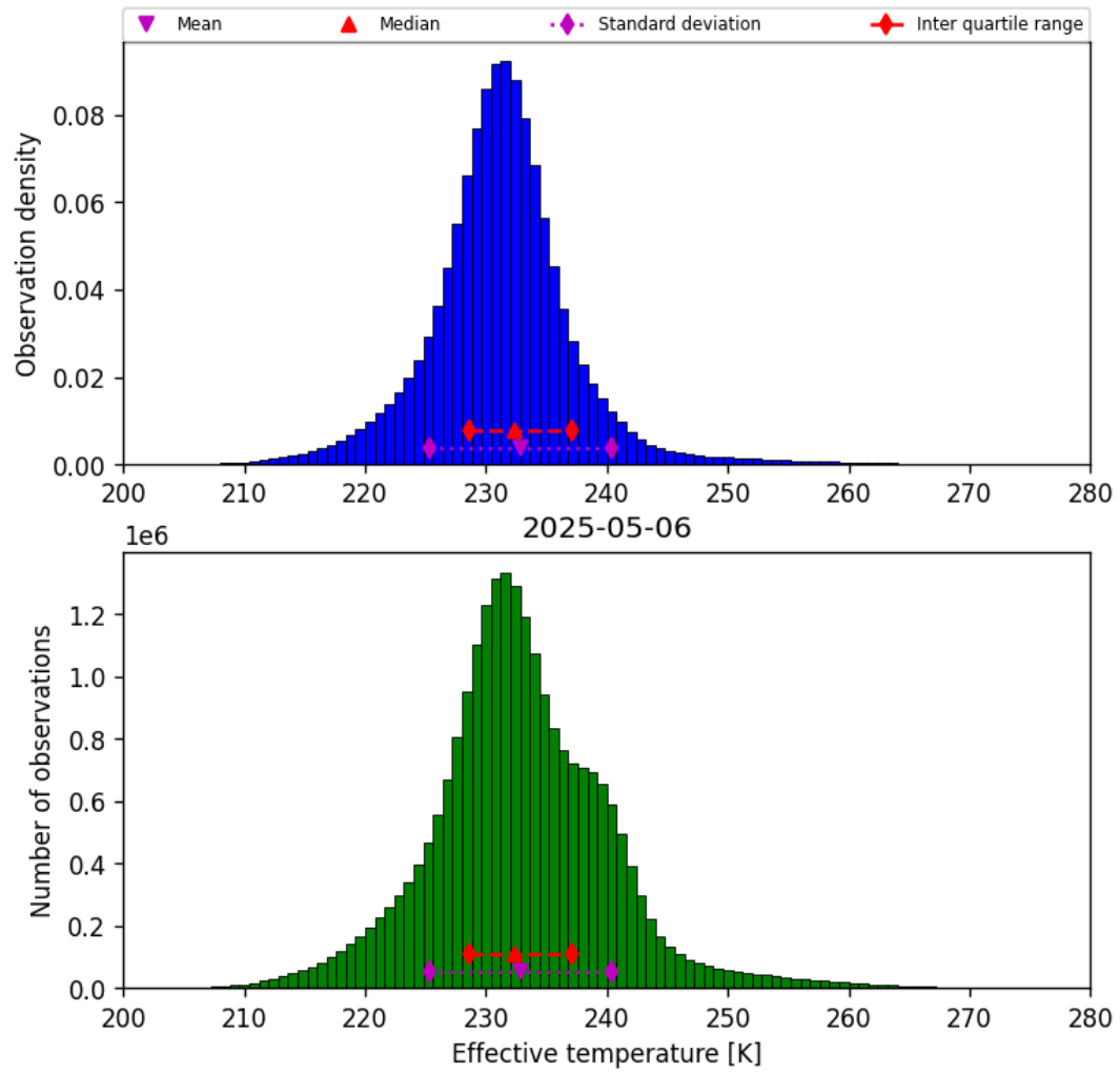
Figure 38: Histogram of “Effective temperature” for 2025-05-06 to 2025-05-07
