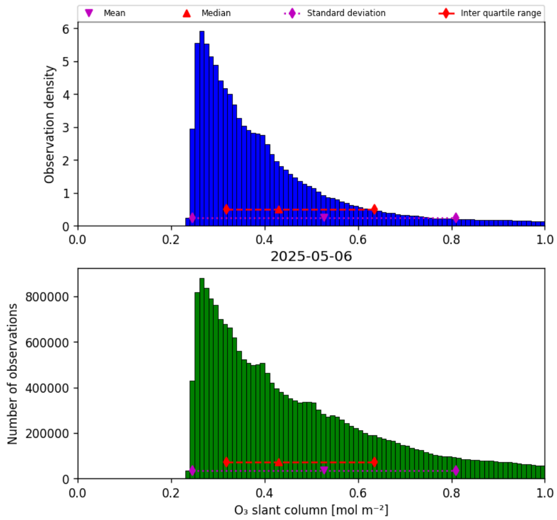
Figure 31: Histogram of “O 3 slant column” for 2025-05-06 to 2025-05-07
