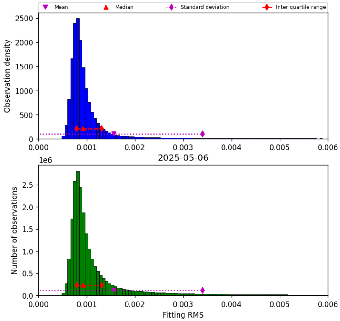
Figure 34: Histogram of “Fitting RMS” for 2025-05-06 to 2025-05-07
