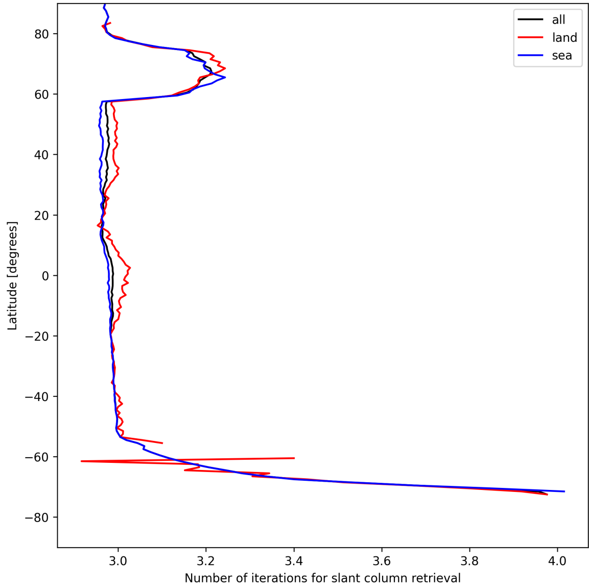
Figure 21: Zonal average of “Number of iterations for slant column retrieval” for 2025-05-06 to 2025-05-07.
