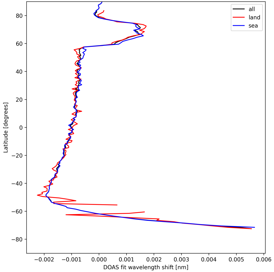
Figure 23: Zonal average of "DOAS fit wavelength shift" for 2025-05-06 to 2025-05-07.
