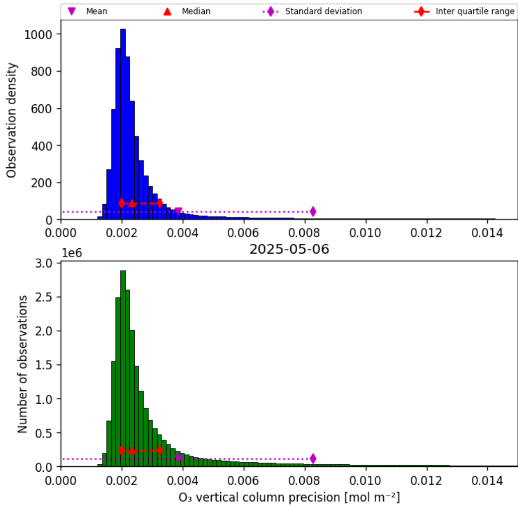
Figure 30: Histogram of “O 3 vertical column precision” for 2025-05-06 to 2025-05-07
