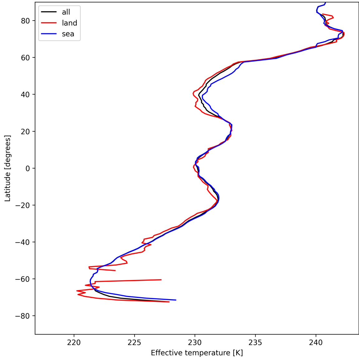
Figure 26: Zonal average of “Effective temperature” for 2025-05-06 to 2025-05-07.
