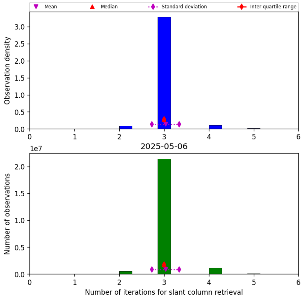
Figure 33: Histogram of “Number of iterations for slant column retrieval” for 2025-05-06 to 2025-05-07
