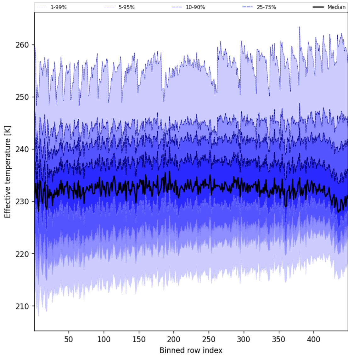
Figure 50: Along track statistics of “Effective temperature” for 2025-05-06 to 2025-05-07
