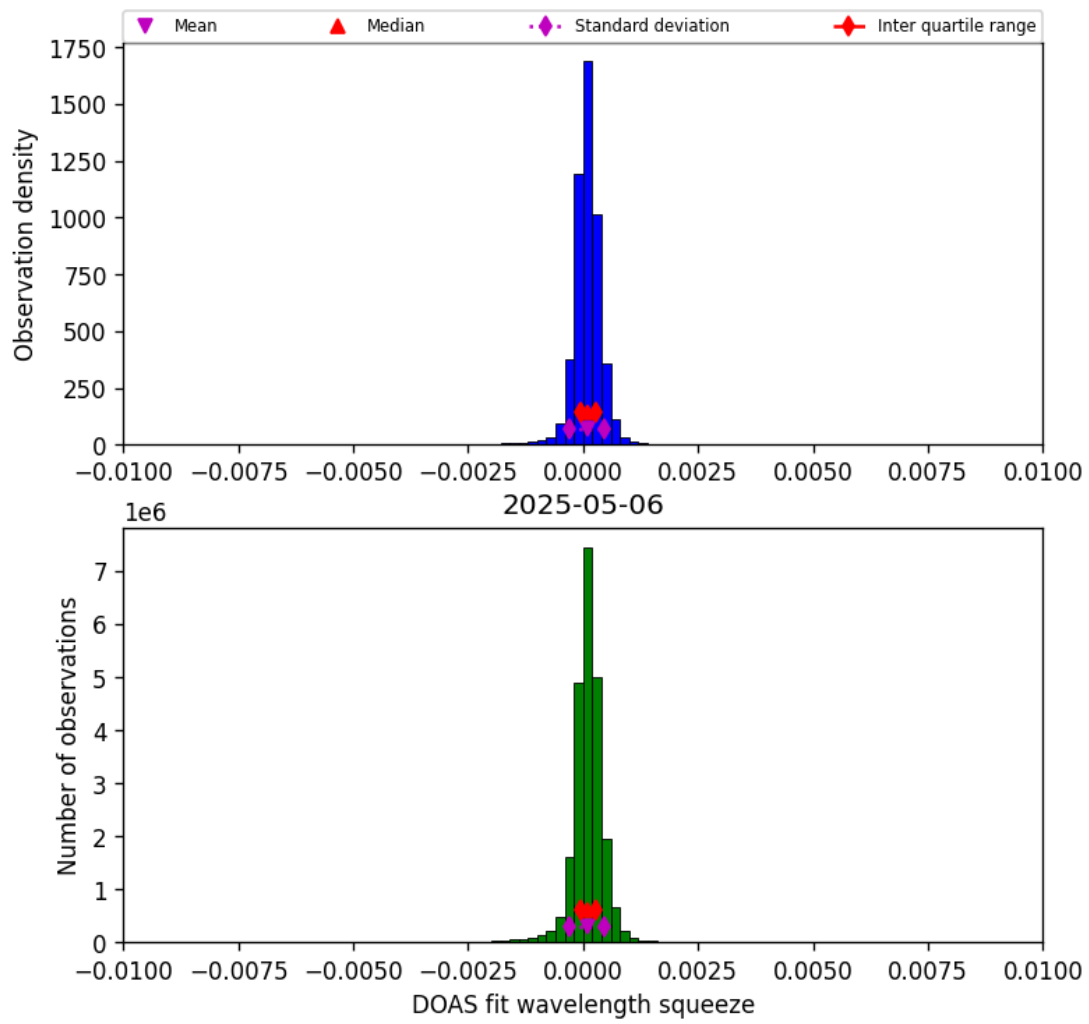
Figure 36: Histogram of “DOAS fit wavelength squeeze” for 2025-05-06 to 2025-05-07
