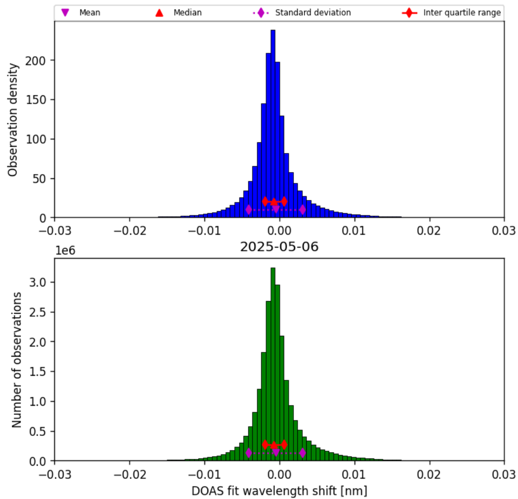
Figure 35: Histogram of “DOAS fit wavelength shift” for 2025-05-06 to 2025-05-07
