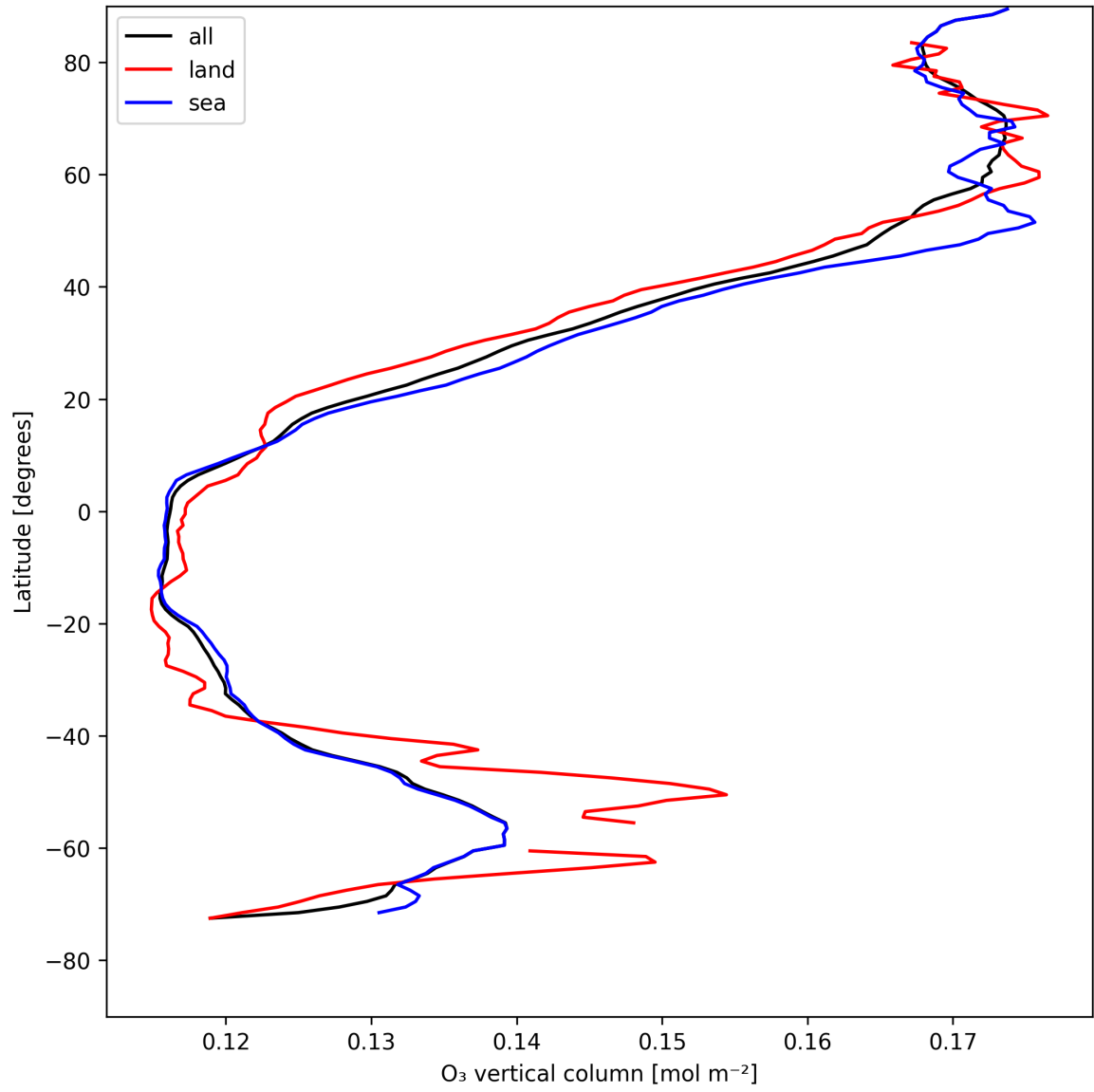
Figure 17: Zonal average of “O 3 vertical column” for 2025-05-06 to 2025-05-07.
