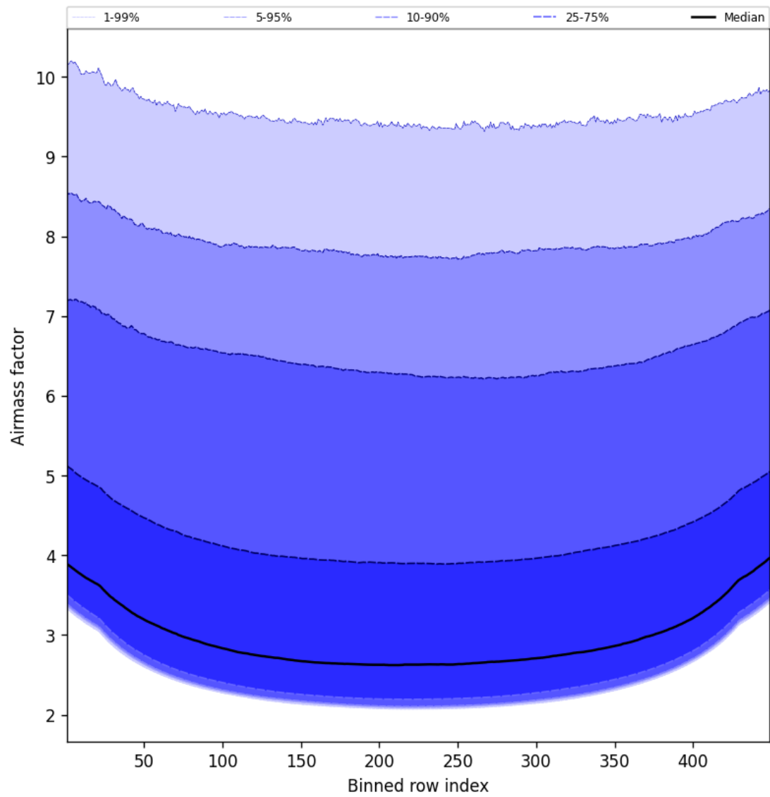
Figure 49: Along track statistics of “Airmass factor” for 2025-05-06 to 2025-05-07
