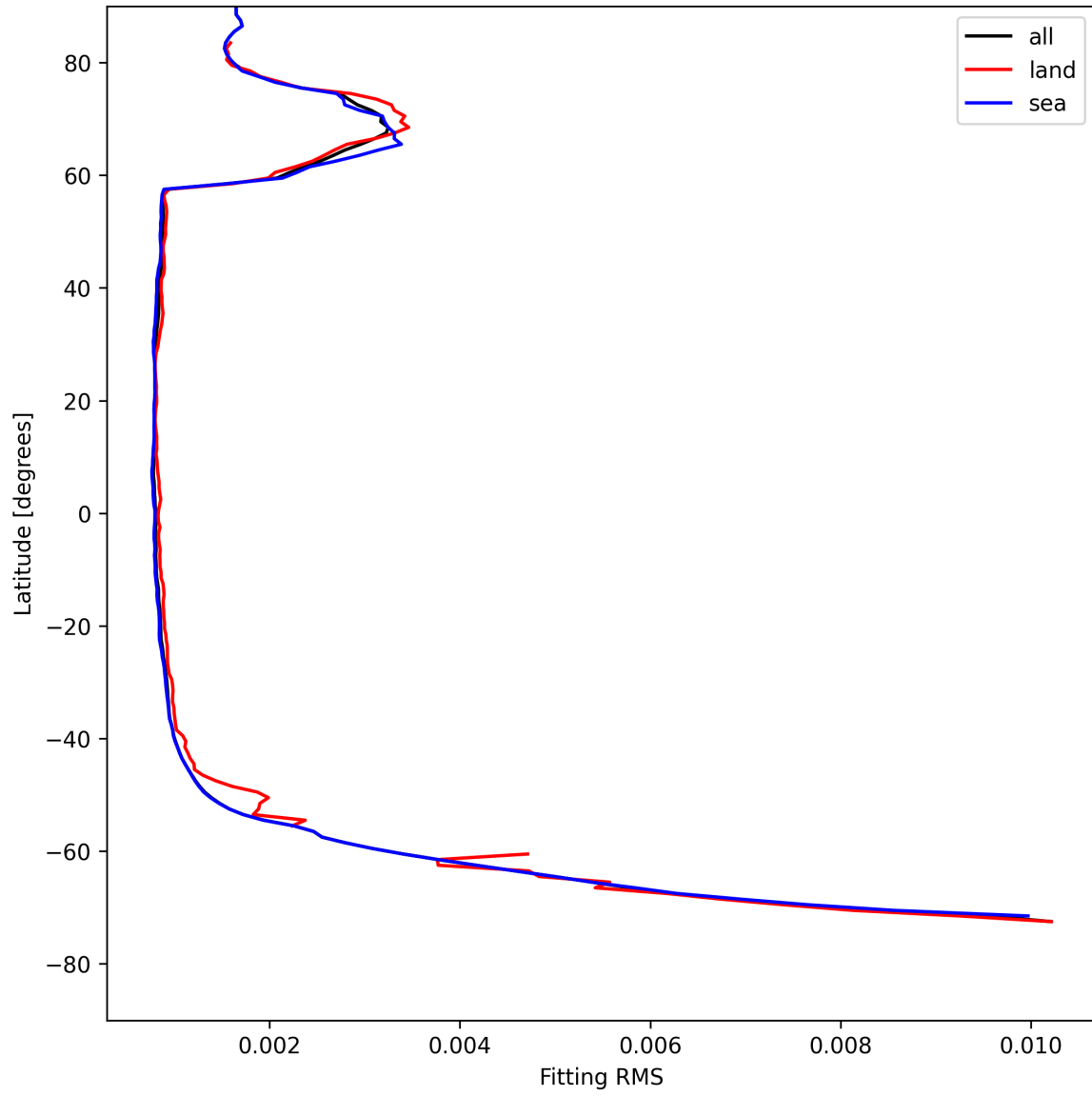
Figure 22: Zonal average of “Fitting RMS” for 2025-05-06 to 2025-05-07.
