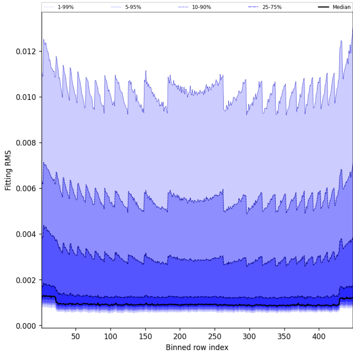
Figure 46: Along track statistics of “Fitting RMS” for 2025-05-06 to 2025-05-07
