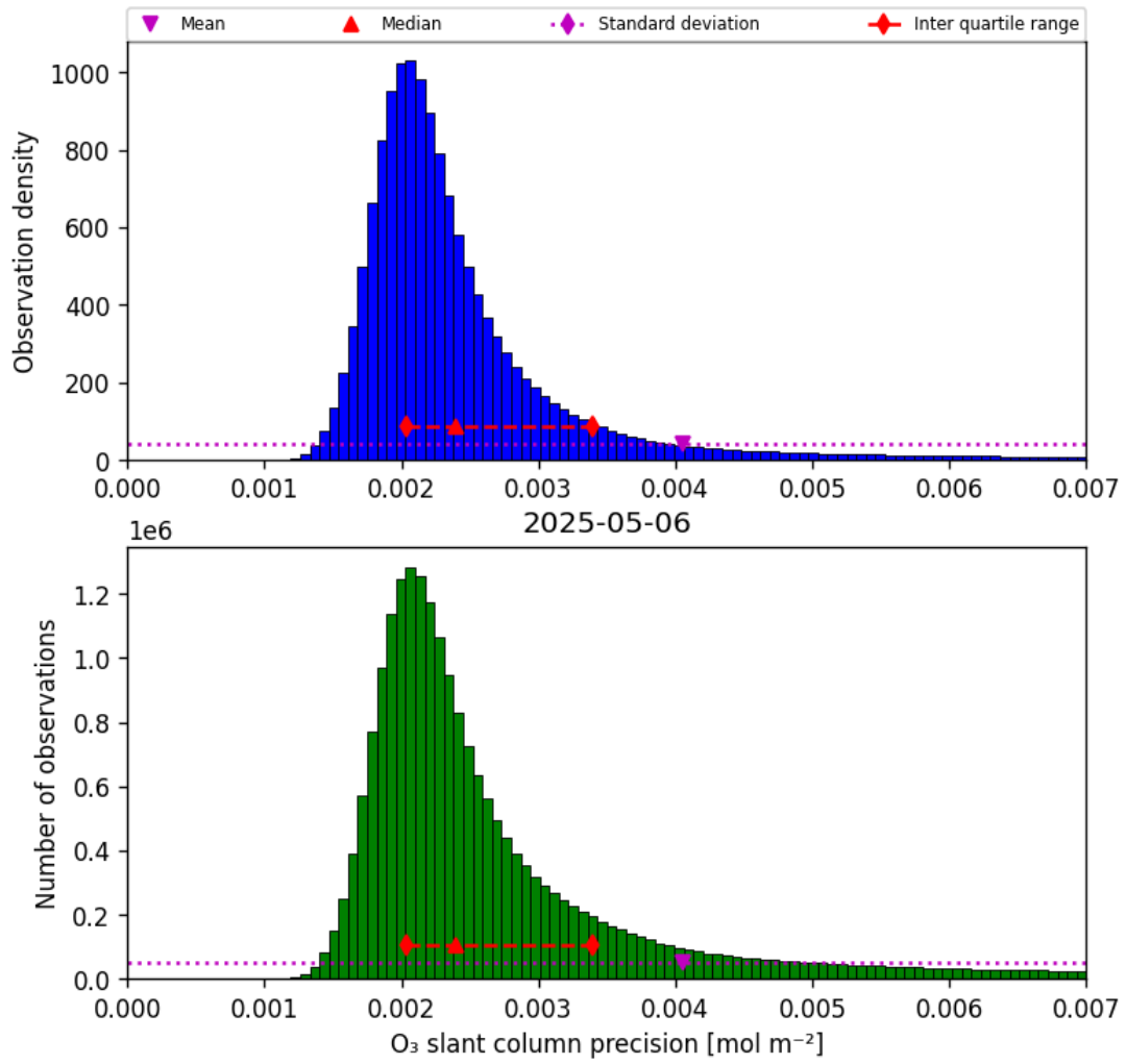
Figure 32: Histogram of “O 3 slant column precision” for 2025-05-06 to 2025-05-07
