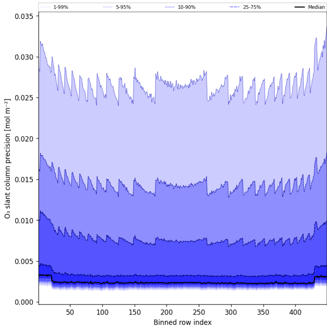
Figure 44: Along track statistics of “O 3 slant column precision” for 2025-05-06 to 2025-05-07
