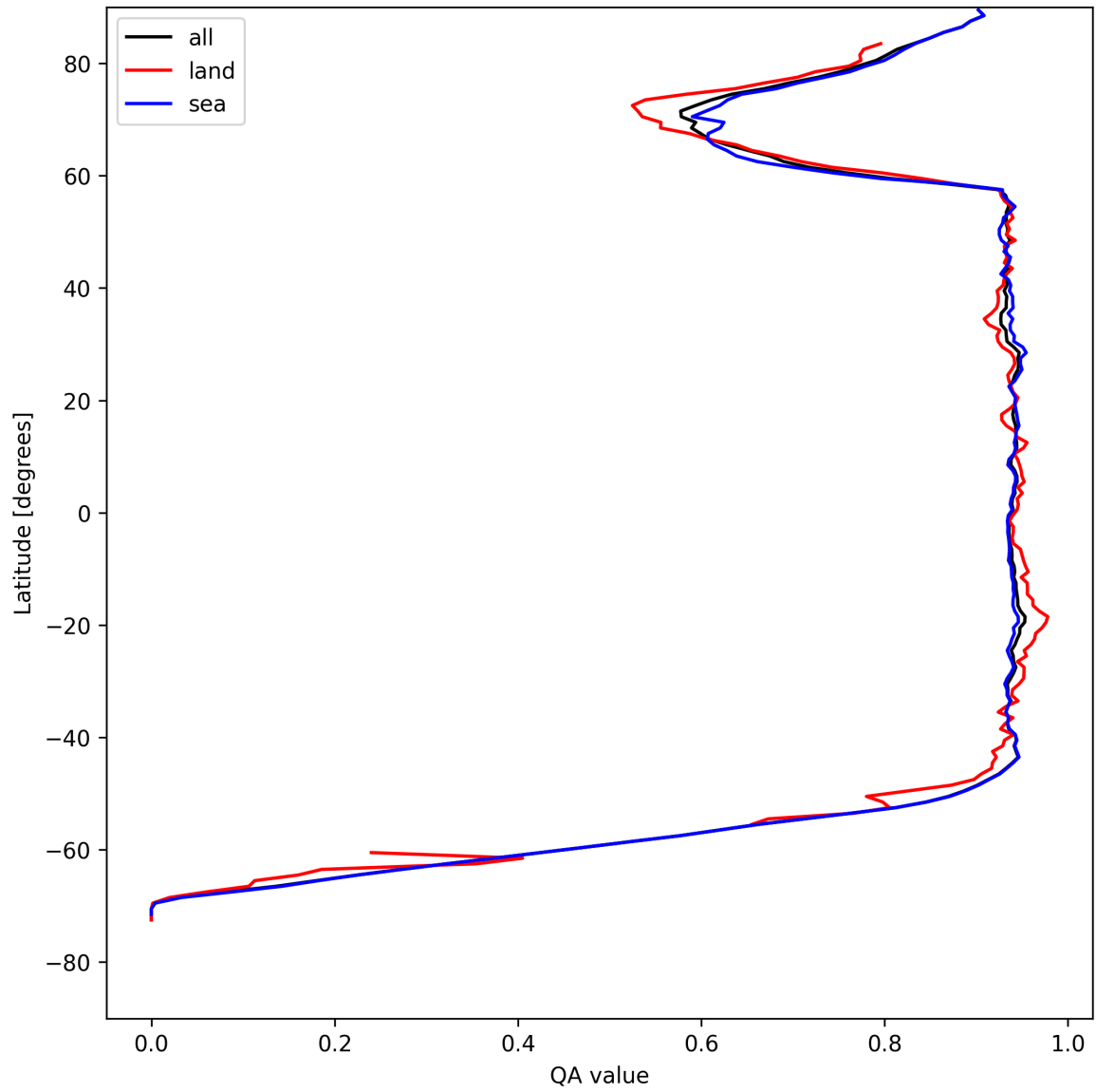
Figure 16: Zonal average of “QA value” for 2025-05-06 to 2025-05-07.
