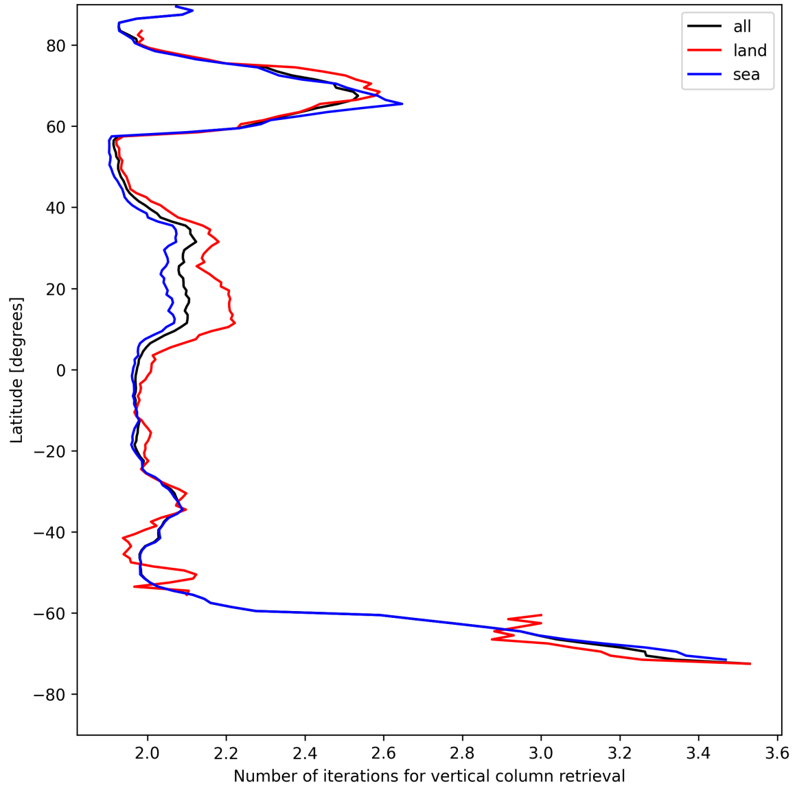
Figure 27: Zonal average of “Number of iterations for vertical column retrieval” for 2025-05-06 to 2025-05-07.
