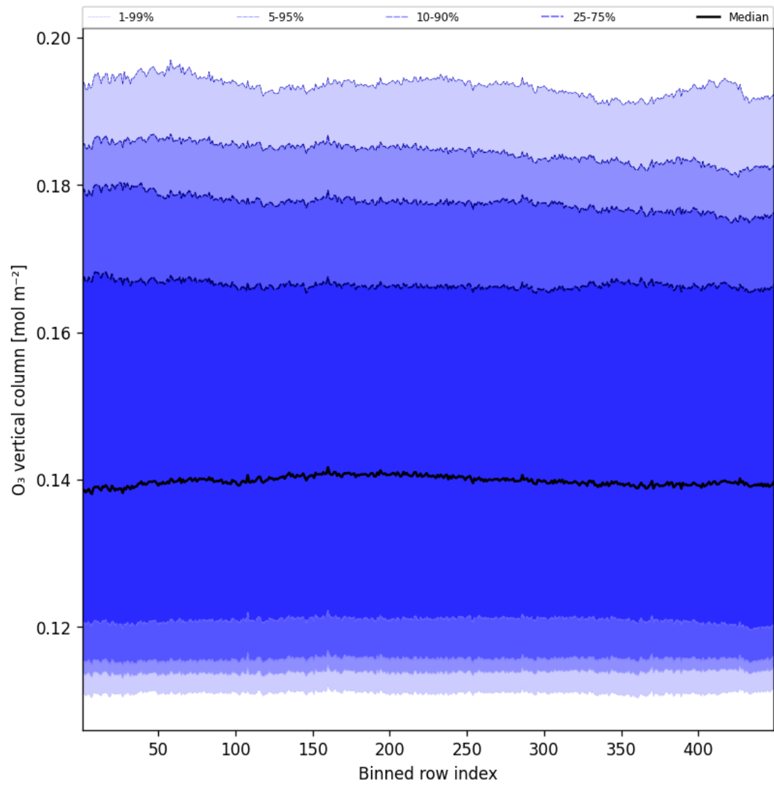
Figure 41: Along track statistics of “O 3 vertical column” for 2025-05-06 to 2025-05-07
