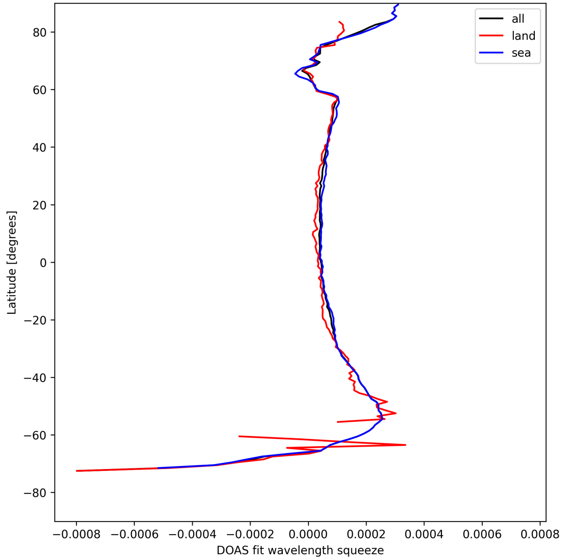
Figure 24: Zonal average of “DOAS fit wavelength squeeze” for 2025-05-06 to 2025-05-07.
