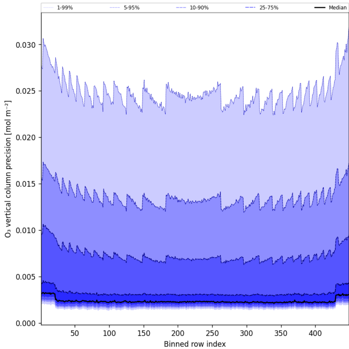
Figure 42: Along track statistics of “O 3 vertical column precision” for 2025-05-06 to 2025-05-07
