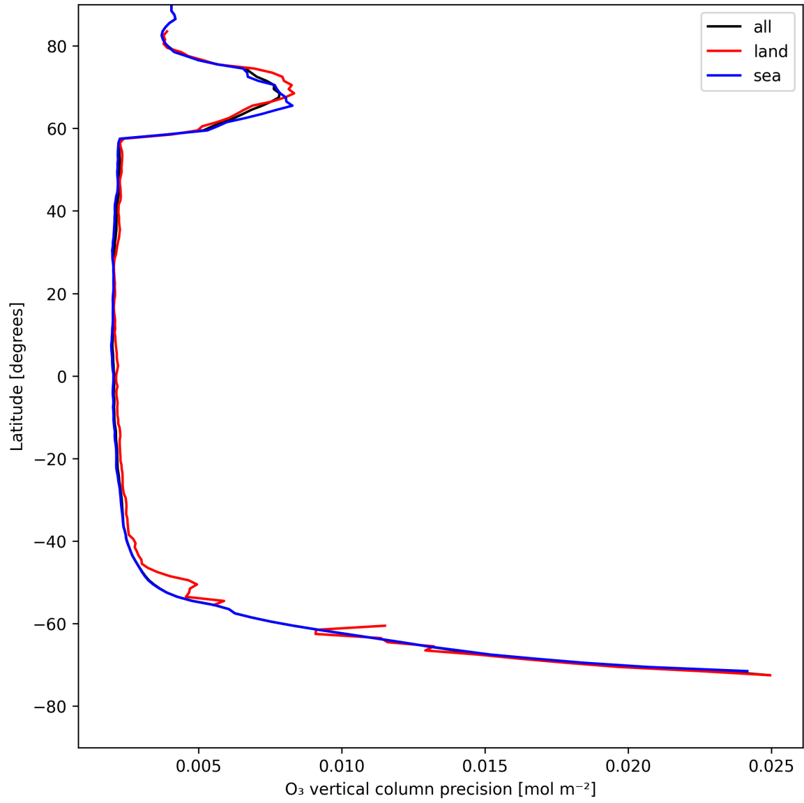
Figure 18: Zonal average of “O 3 vertical column precision” for 2025-05-06 to 2025-05-07.
