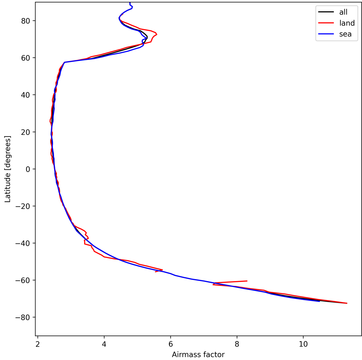
Figure 25: Zonal average of “Airmass factor” for 2025-05-06 to 2025-05-07.
