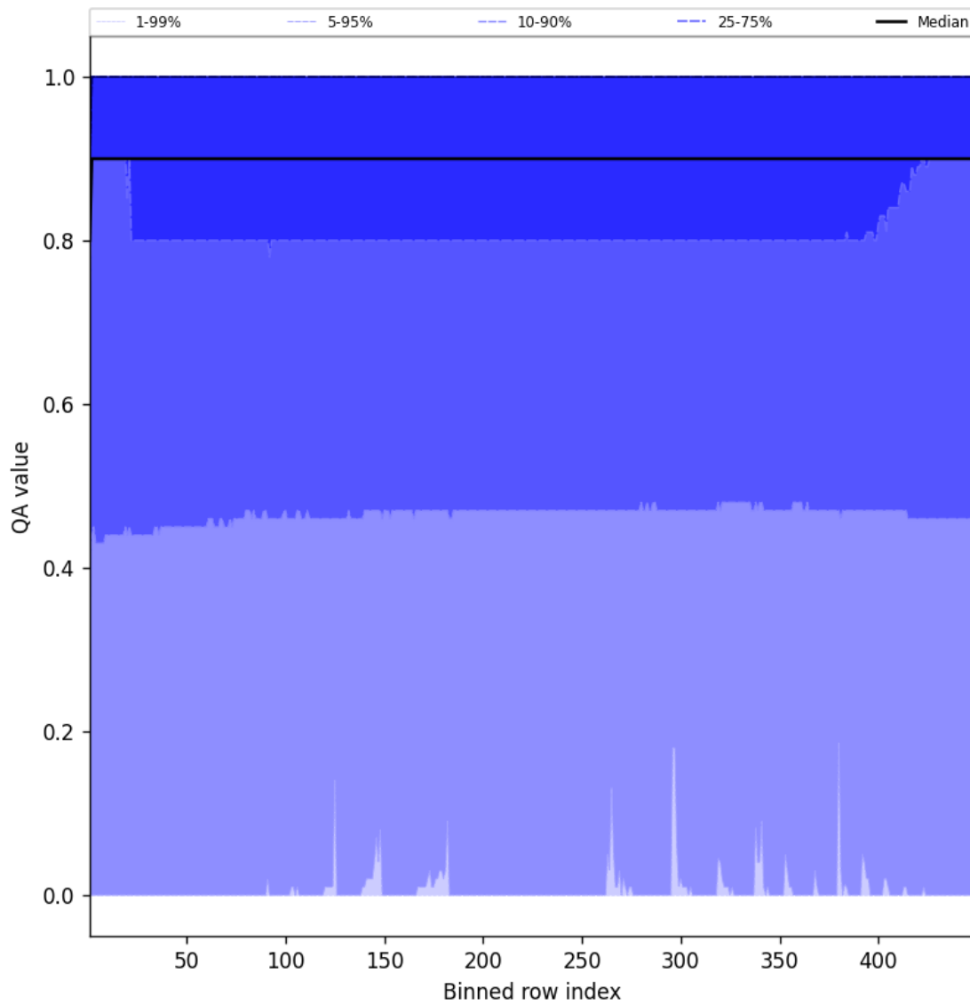
Figure 40: Along track statistics of “QA value” for 2025-05-06 to 2025-05-07
