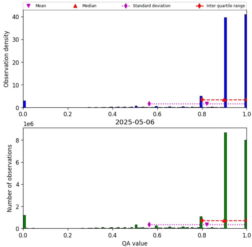
Figure 28: Histogram of “QA value” for 2025-05-06 to 2025-05-07
