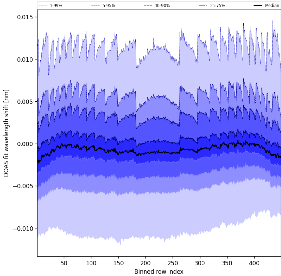
Figure 47: Along track statistics of “DOAS fit wavelength shift” for 2025-05-06 to 2025-05-07
