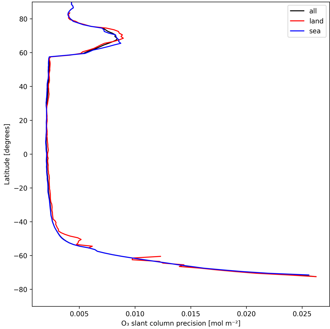
Figure 20: Zonal average of “O 3 slant column precision” for 2025-05-06 to 2025-05-07.
