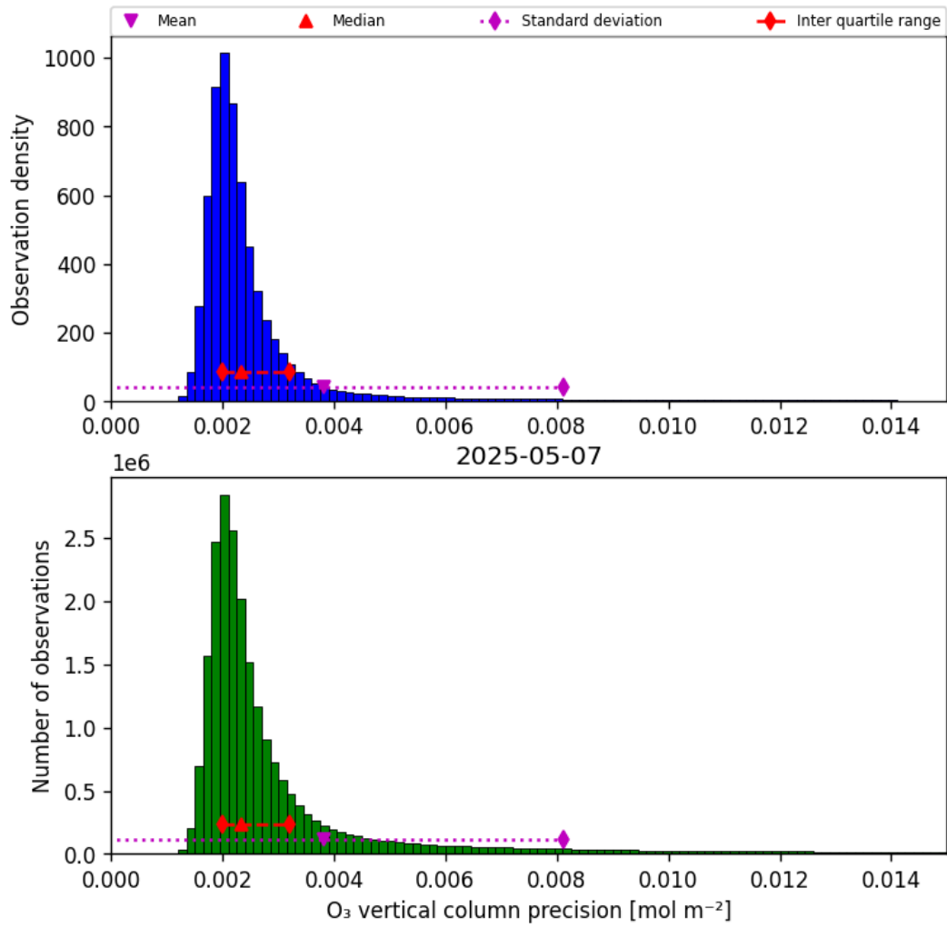
Figure 30: Histogram of “O 3 vertical column precision” for 2025-05-07 to 2025-05-08
