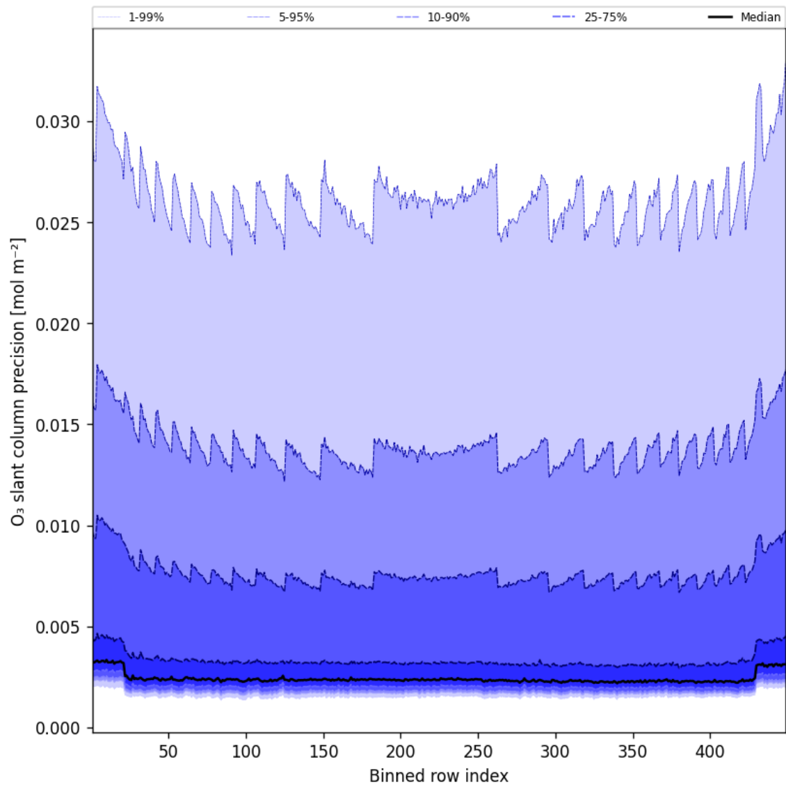
Figure 44: Along track statistics of “O 3 slant column precision” for 2025-05-07 to 2025-05-08
