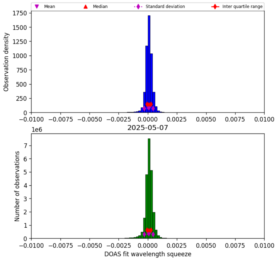
Figure 36: Histogram of “DOAS fit wavelength squeeze” for 2025-05-07 to 2025-05-08
