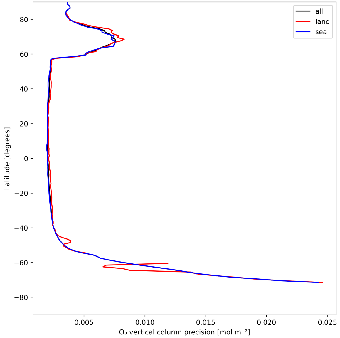
Figure 18: Zonal average of “O 3 vertical column precision” for 2025-05-07 to 2025-05-08.
