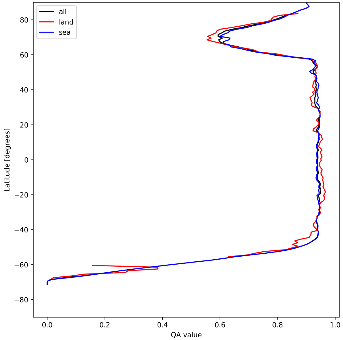
Figure 16: Zonal average of “QA value” for 2025-05-07 to 2025-05-08.
