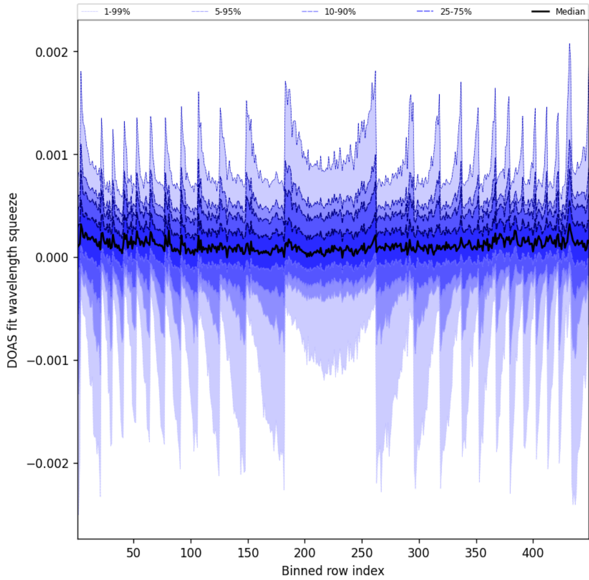
Figure 48: Along track statistics of “DOAS fit wavelength squeeze” for 2025-05-07 to 2025-05-08
