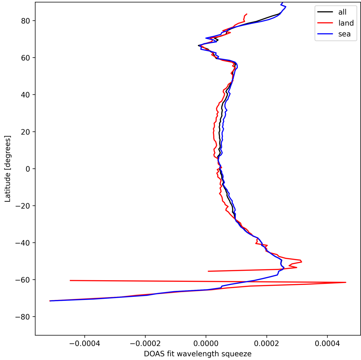
Figure 24: Zonal average of "DOAS fit wavelength squeeze" for 2025-05-07 to 2025-05-08.
