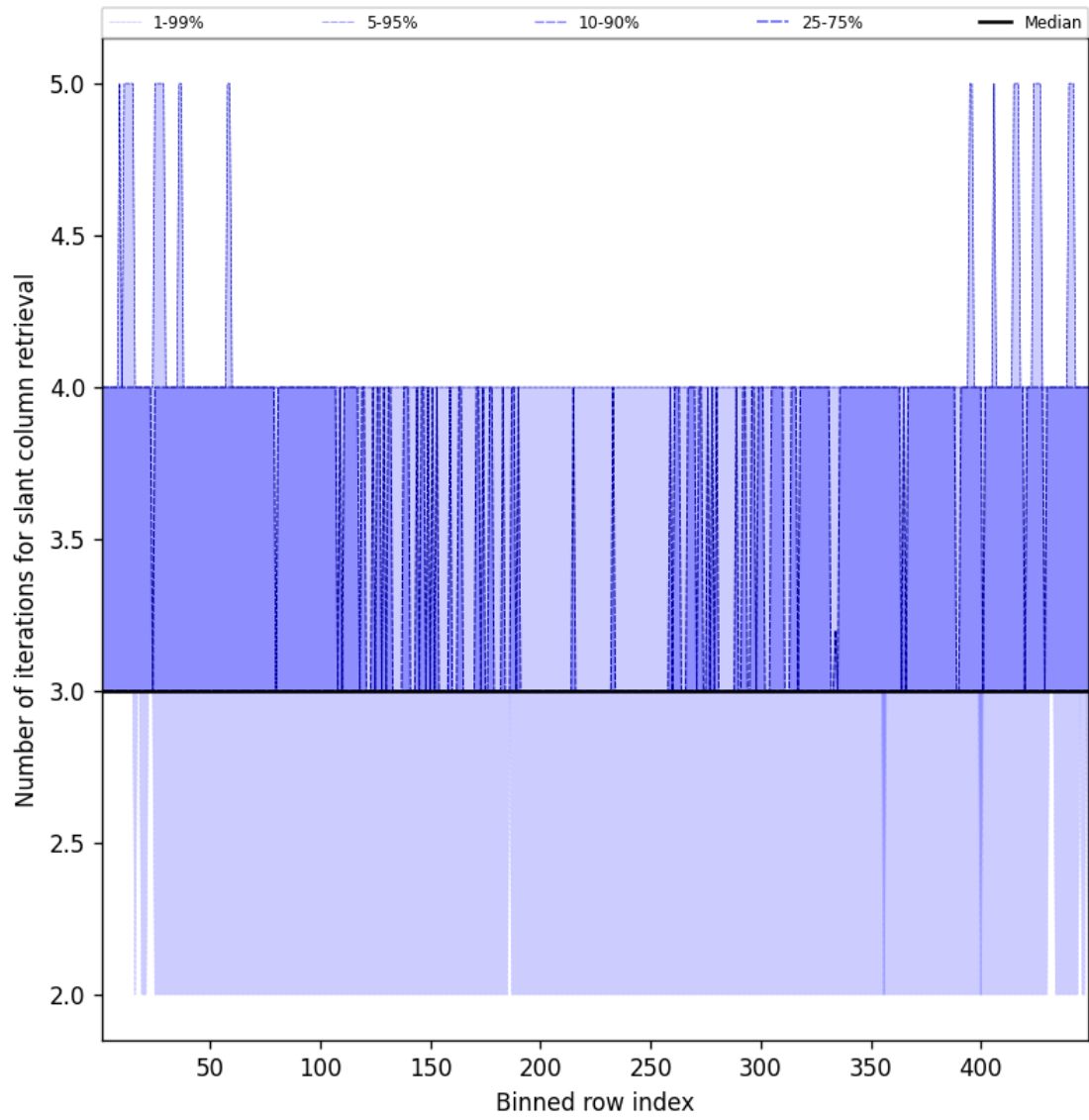
Figure 45: Along track statistics of “Number of iterations for slant column retrieval” for 2025-05-07 to 2025-05-08
