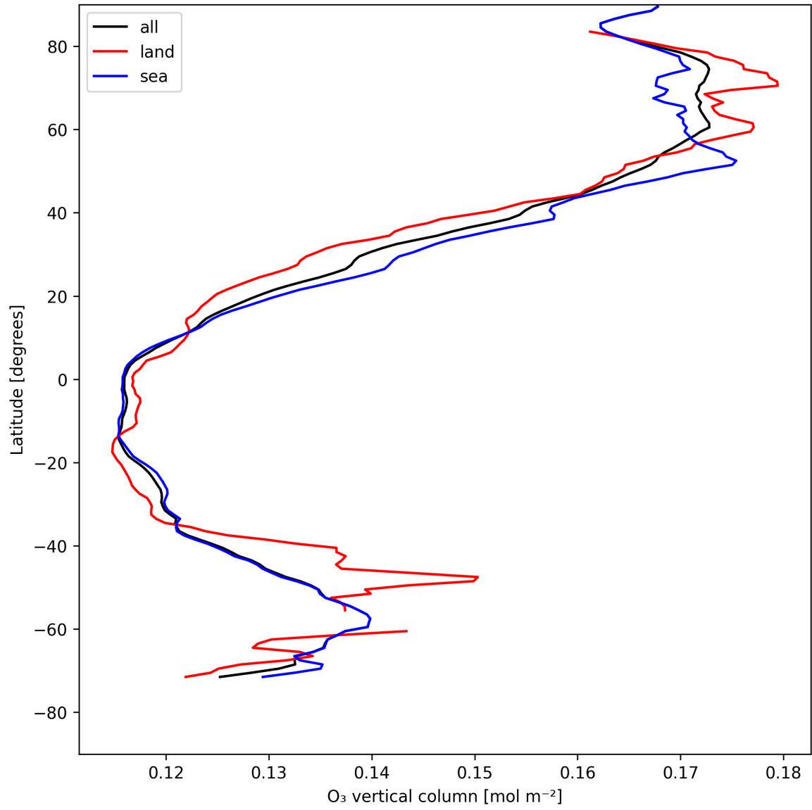
Figure 17: Zonal average of “O 3 vertical column” for 2025-05-07 to 2025-05-08.
