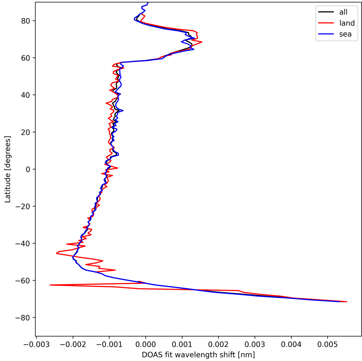
Figure 23: Zonal average of "DOAS fit wavelength shift" for 2025-05-07 to 2025-05-08.
