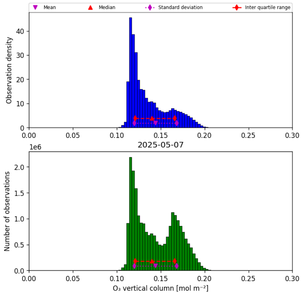
Figure 29: Histogram of “O 3 vertical column” for 2025-05-07 to 2025-05-08
