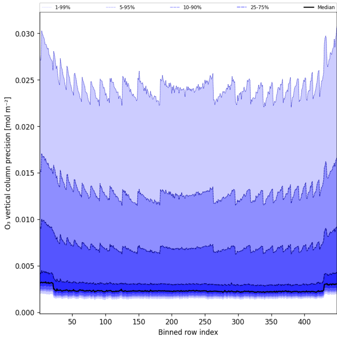
Figure 42: Along track statistics of “O 3 vertical column precision” for 2025-05-07 to 2025-05-08
