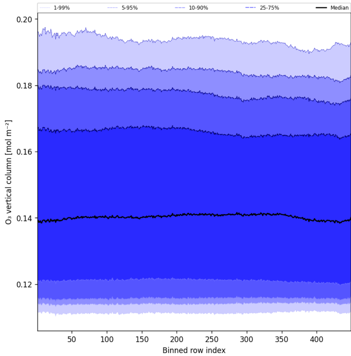
Figure 41: Along track statistics of “ O_3 vertical column” for 2025-05-07 to 2025-05-08
