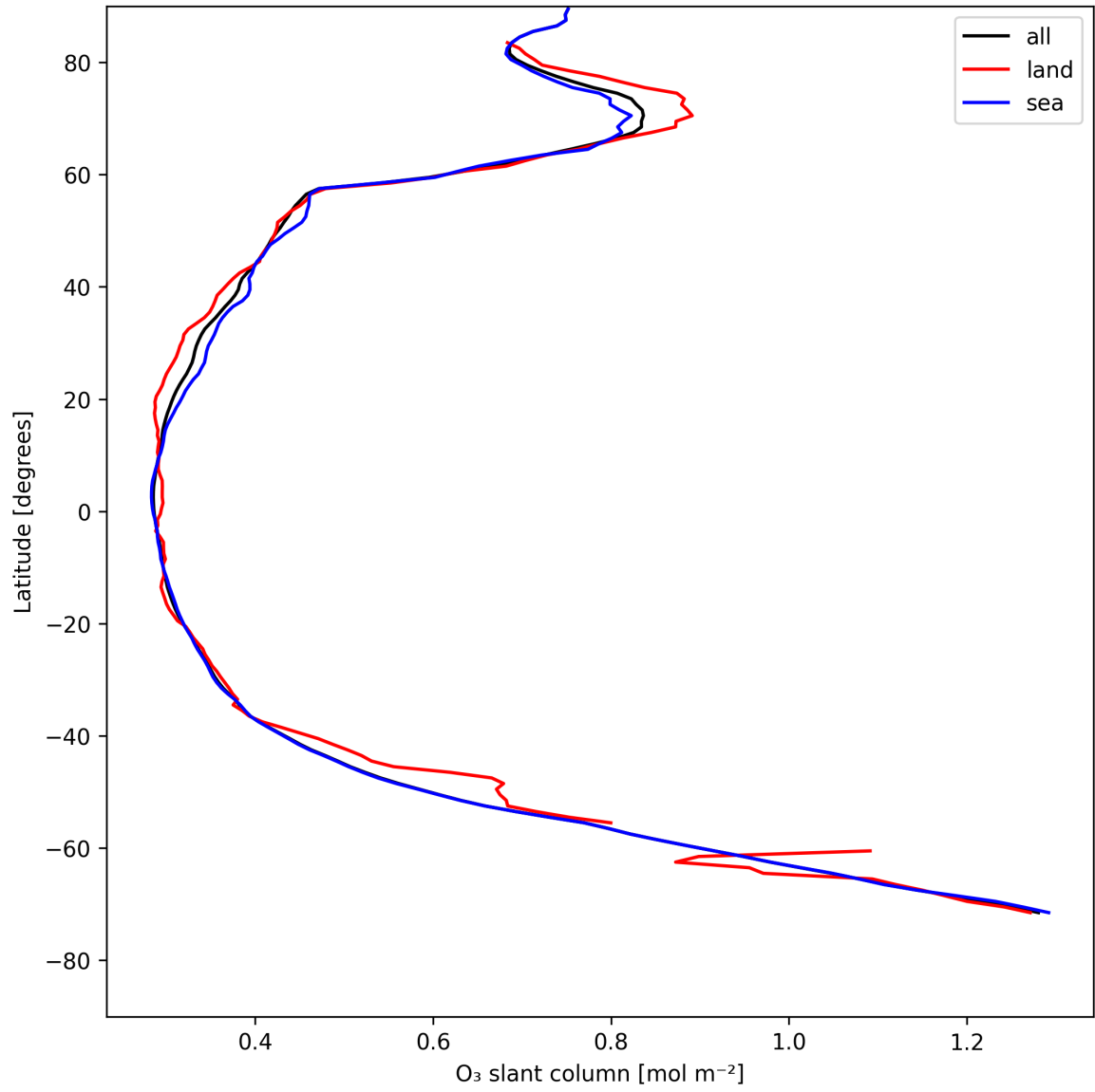
Figure 19: Zonal average of “O 3 slant column” for 2025-05-07 to 2025-05-08.
