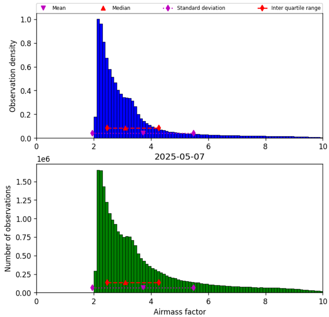
Figure 37: Histogram of “Airmass factor” for 2025-05-07 to 2025-05-08
