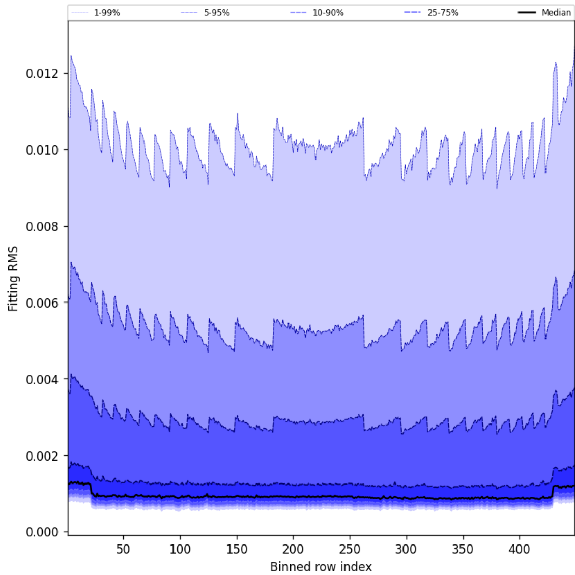
Figure 46: Along track statistics of “Fitting RMS” for 2025-05-07 to 2025-05-08
