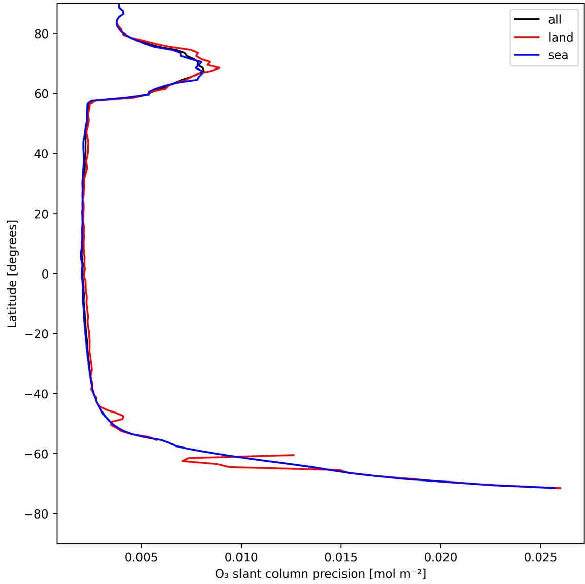
Figure 20: Zonal average of “O 3 slant column precision” for 2025-05-07 to 2025-05-08.
