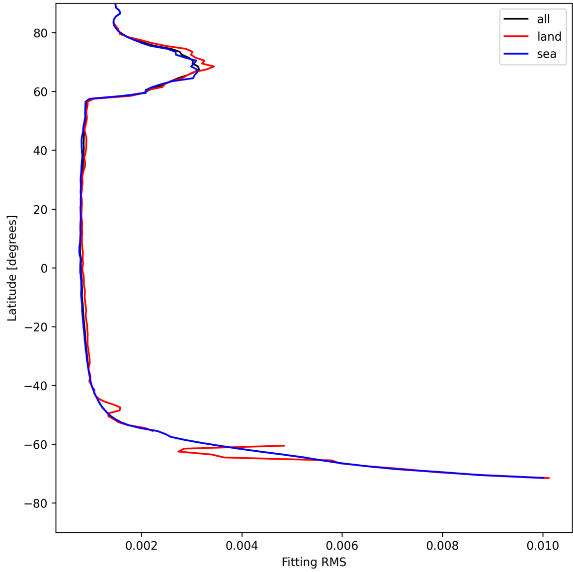
Figure 22: Zonal average of “Fitting RMS” for 2025-05-07 to 2025-05-08.
