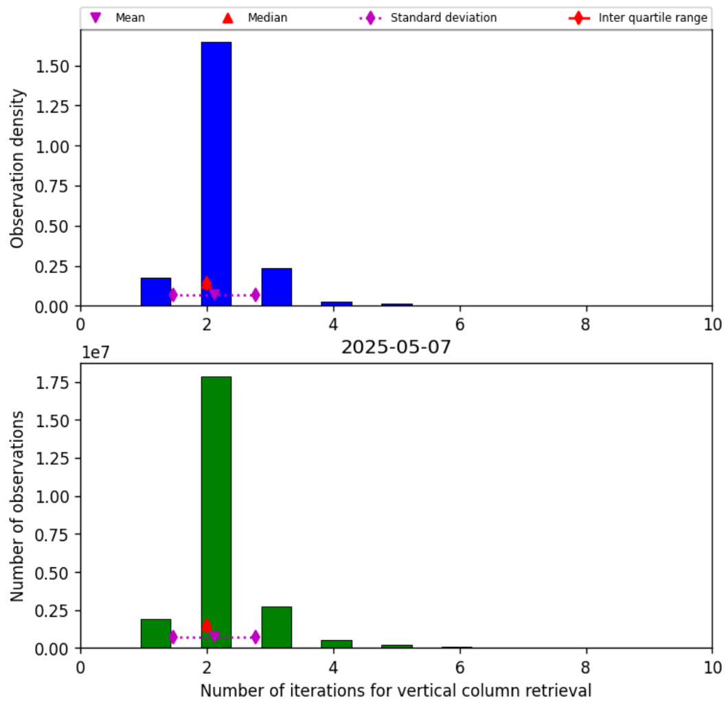
Figure 39: Histogram of “Number of iterations for vertical column retrieval” for 2025-05-07 to 2025-05-08
