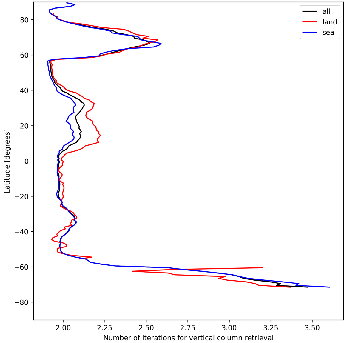
Figure 27: Zonal average of “Number of iterations for vertical column retrieval” for 2025-05-07 to 2025-05-08.
