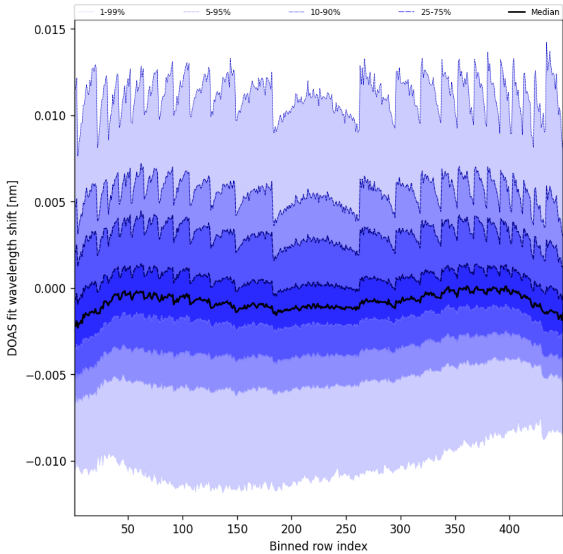
Figure 47: Along track statistics of “DOAS fit wavelength shift” for 2025-05-07 to 2025-05-08
