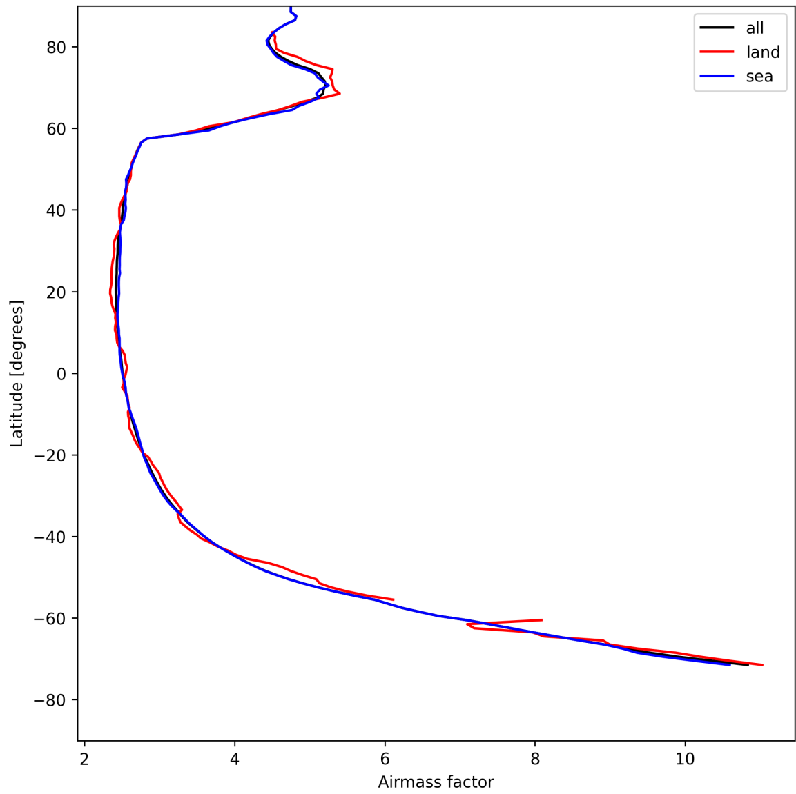
Figure 25: Zonal average of “Airmass factor” for 2025-05-07 to 2025-05-08.
