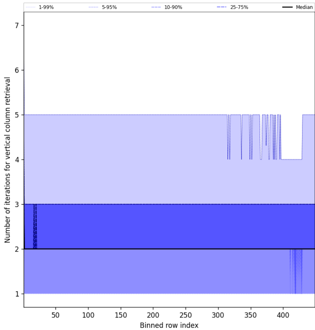
Figure 51: Along track statistics of “Number of iterations for vertical column retrieval” for 2025-05-07 to 2025-05-08
