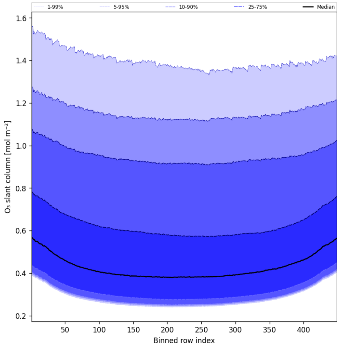
Figure 43: Along track statistics of “O 3 slant column” for 2025-05-07 to 2025-05-08
