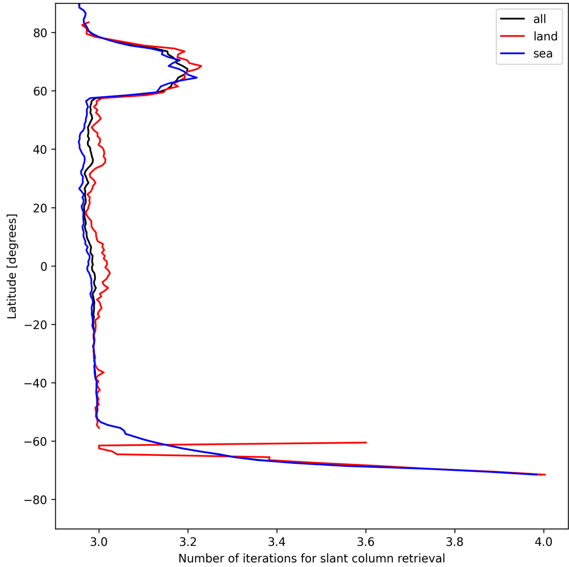
Figure 21: Zonal average of “Number of iterations for slant column retrieval” for 2025-05-07 to 2025-05-08.
