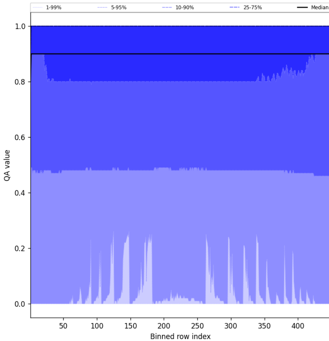
Figure 40: Along track statistics of “QA value” for 2025-05-07 to 2025-05-08
