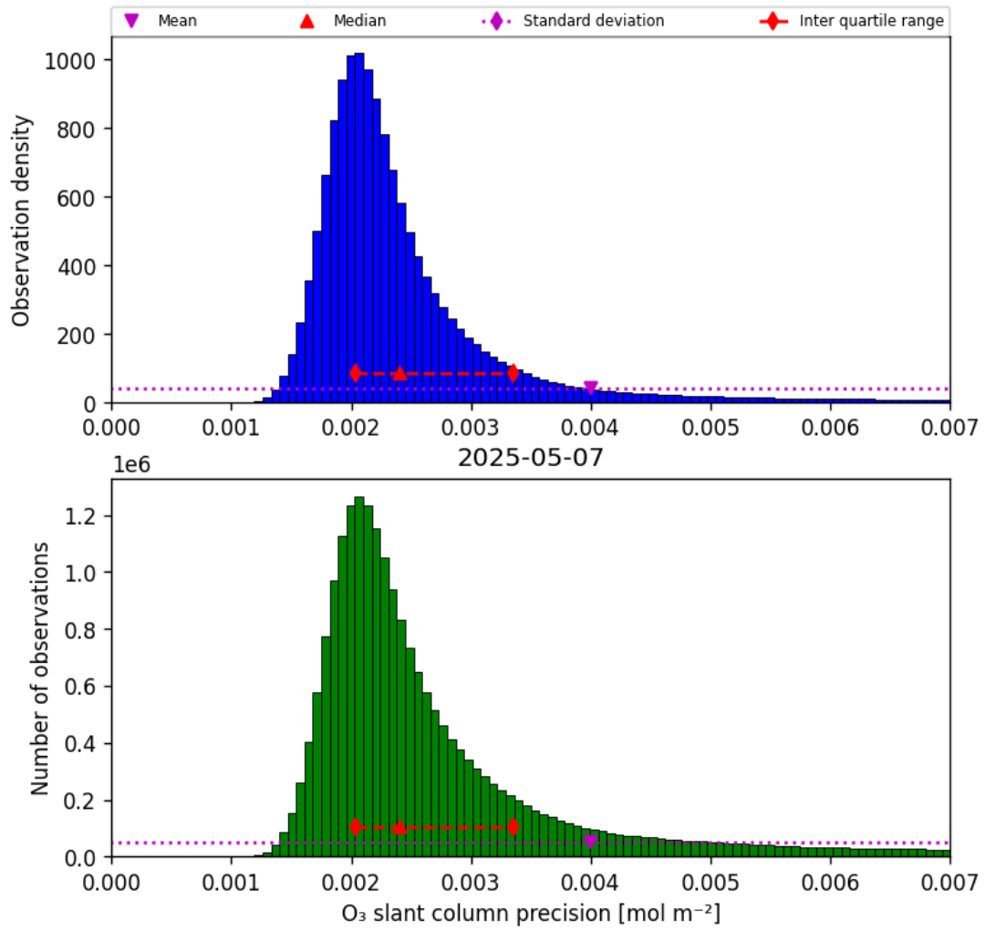
Figure 32: Histogram of “O 3 slant column precision” for 2025-05-07 to 2025-05-08
