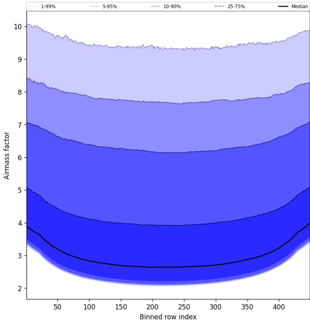
Figure 49: Along track statistics of “Airmass factor” for 2025-05-07 to 2025-05-08
