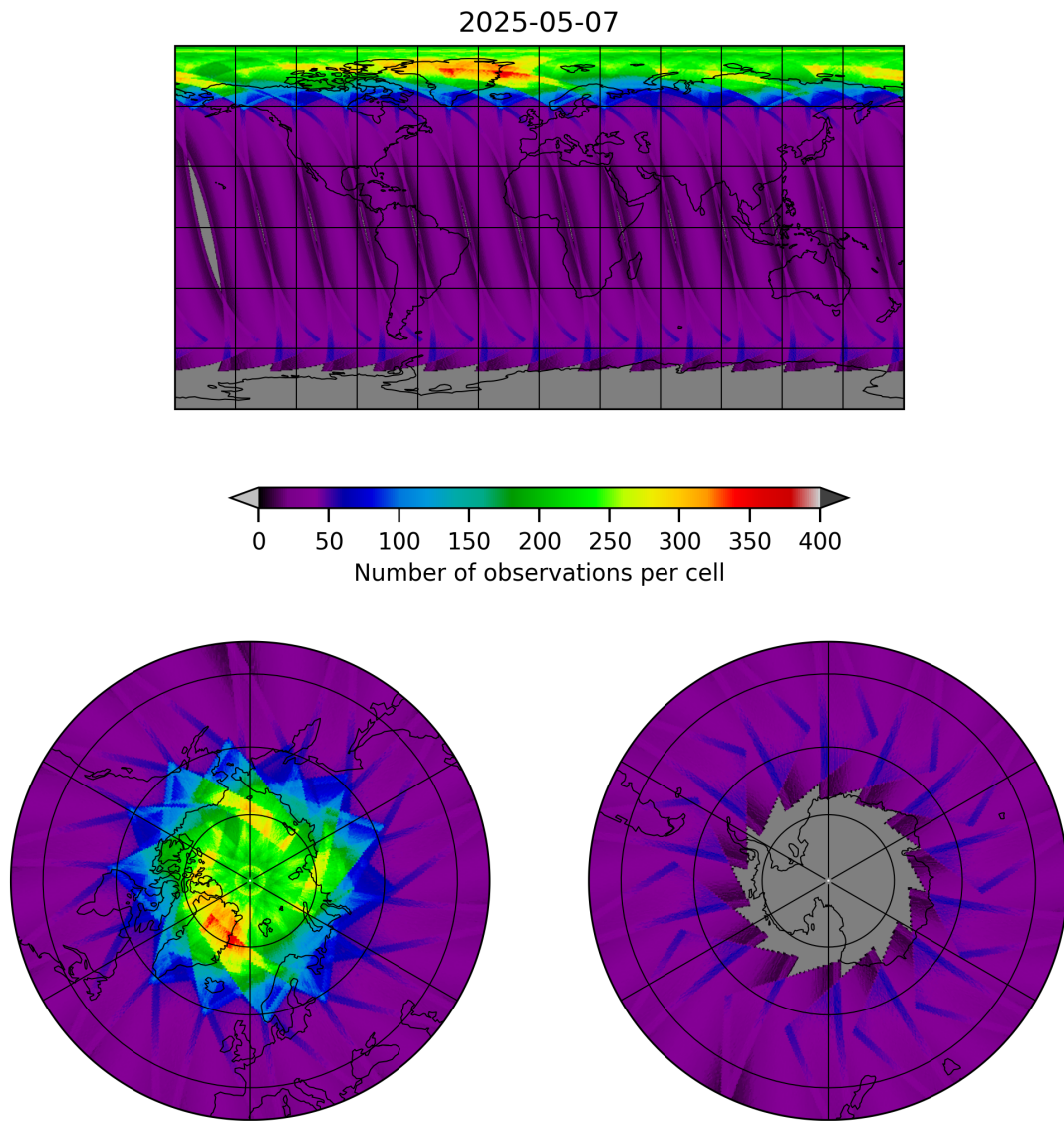
Figure 15: Map of the number of observations for 2025-05-07 to 2025-05-08
