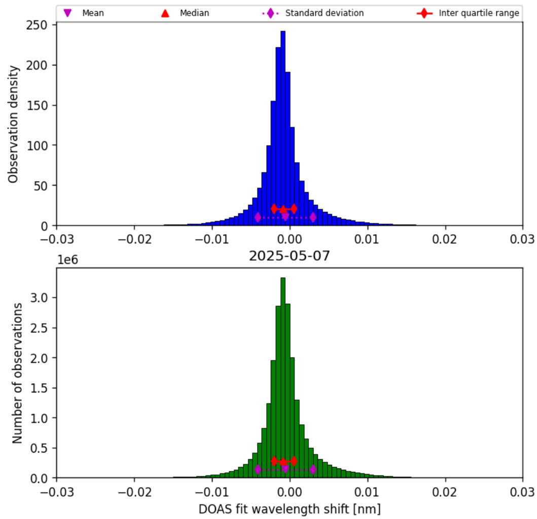
Figure 35: Histogram of “DOAS fit wavelength shift” for 2025-05-07 to 2025-05-08
