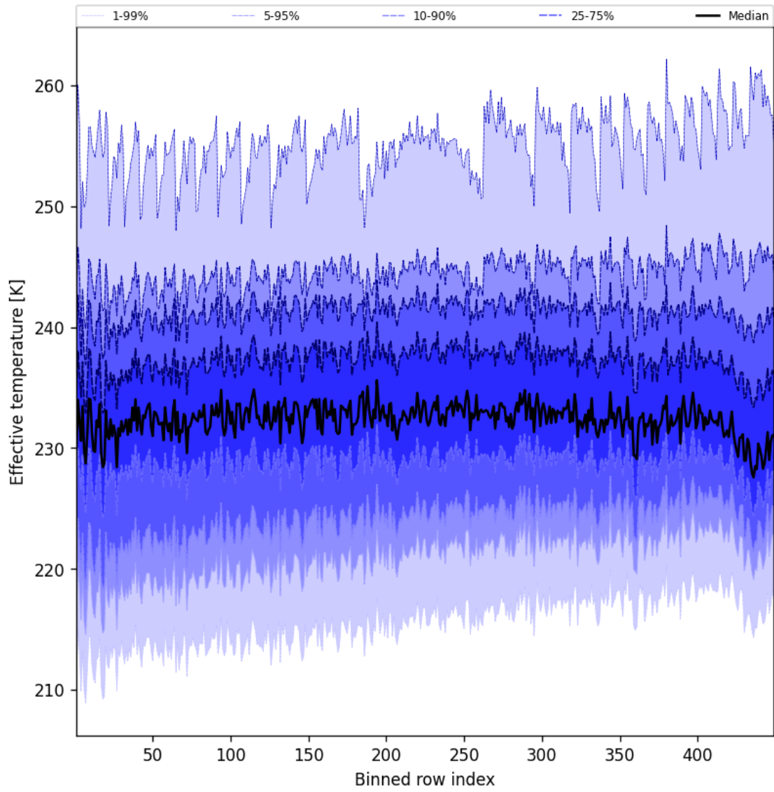
Figure 50: Along track statistics of “Effective temperature” for 2025-05-07 to 2025-05-08
