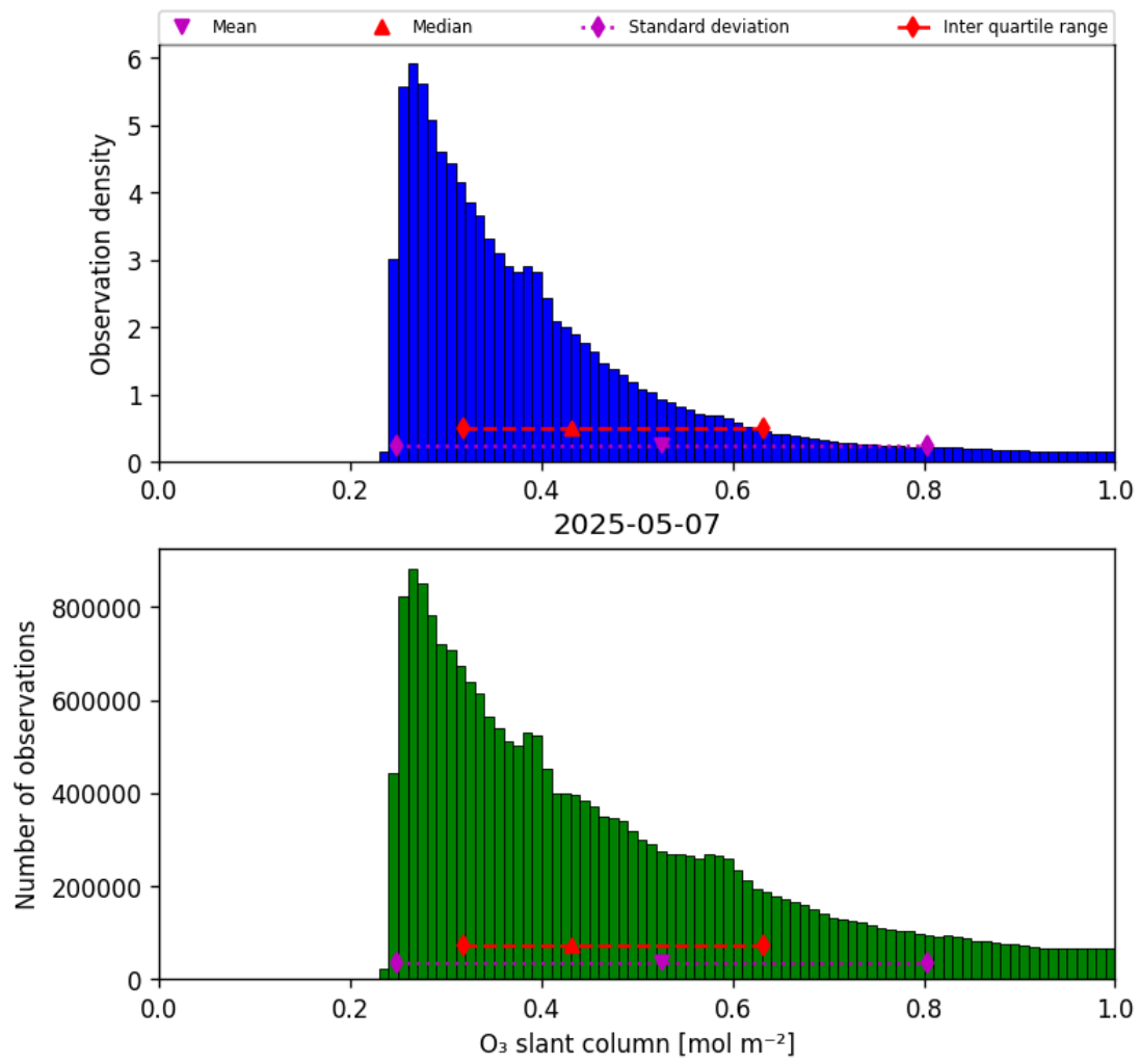
Figure 31: Histogram of “O 3 slant column” for 2025-05-07 to 2025-05-08
