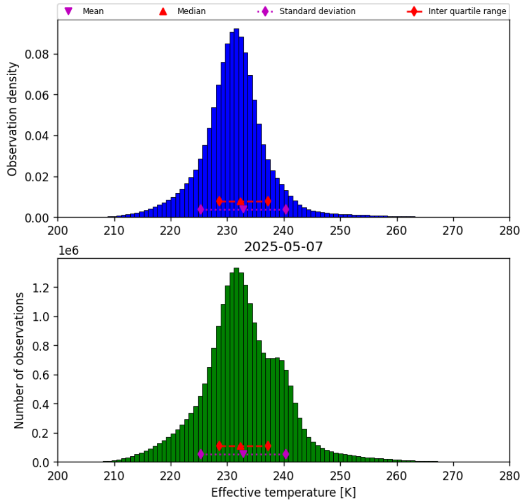
Figure 38: Histogram of “Effective temperature” for 2025-05-07 to 2025-05-08
