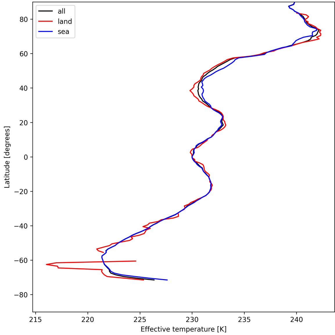
Figure 26: Zonal average of "Effective temperature" for 2025-05-07 to 2025-05-08.
