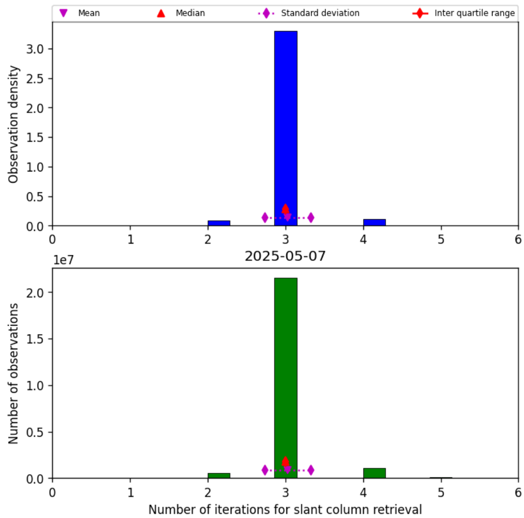
Figure 33: Histogram of “Number of iterations for slant column retrieval” for 2025-05-07 to 2025-05-08
