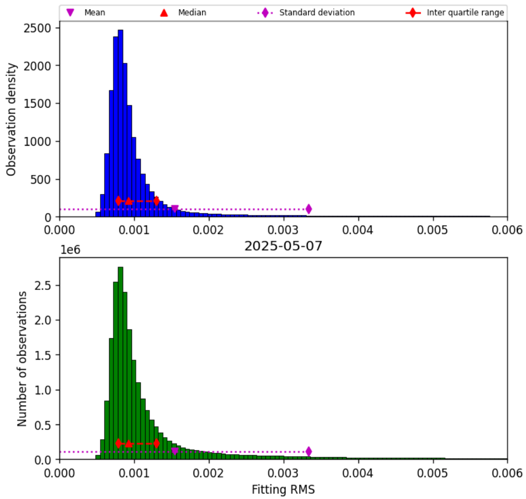
Figure 34: Histogram of “Fitting RMS” for 2025-05-07 to 2025-05-08
