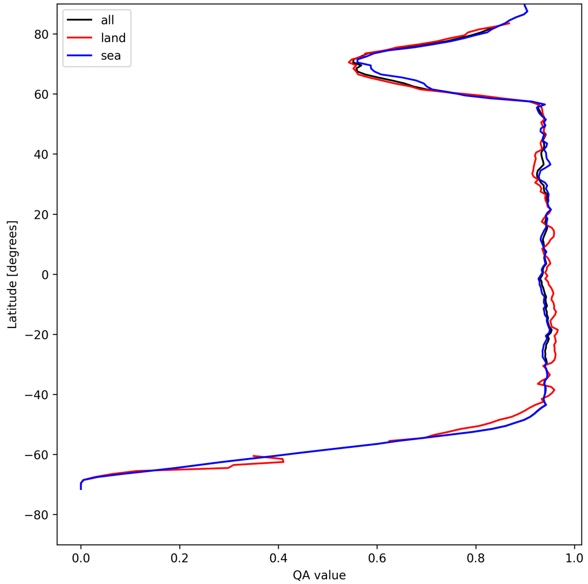
Figure 16: Zonal average of “QA value” for 2025-05-08 to 2025-05-08.
