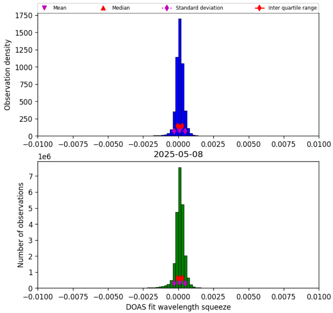
Figure 36: Histogram of “DOAS fit wavelength squeeze” for 2025-05-08 to 2025-05-08
