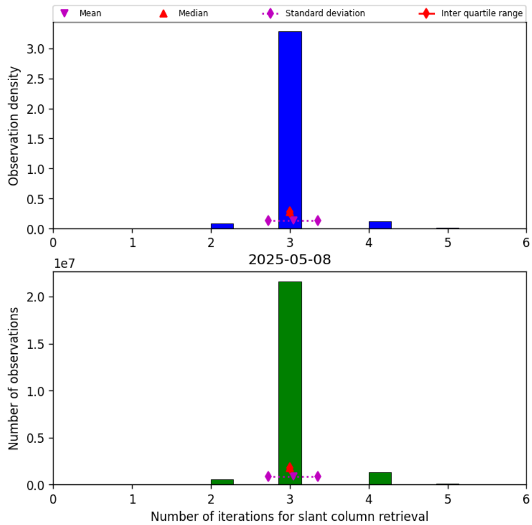
Figure 33: Histogram of “Number of iterations for slant column retrieval” for 2025-05-08 to 2025-05-08
