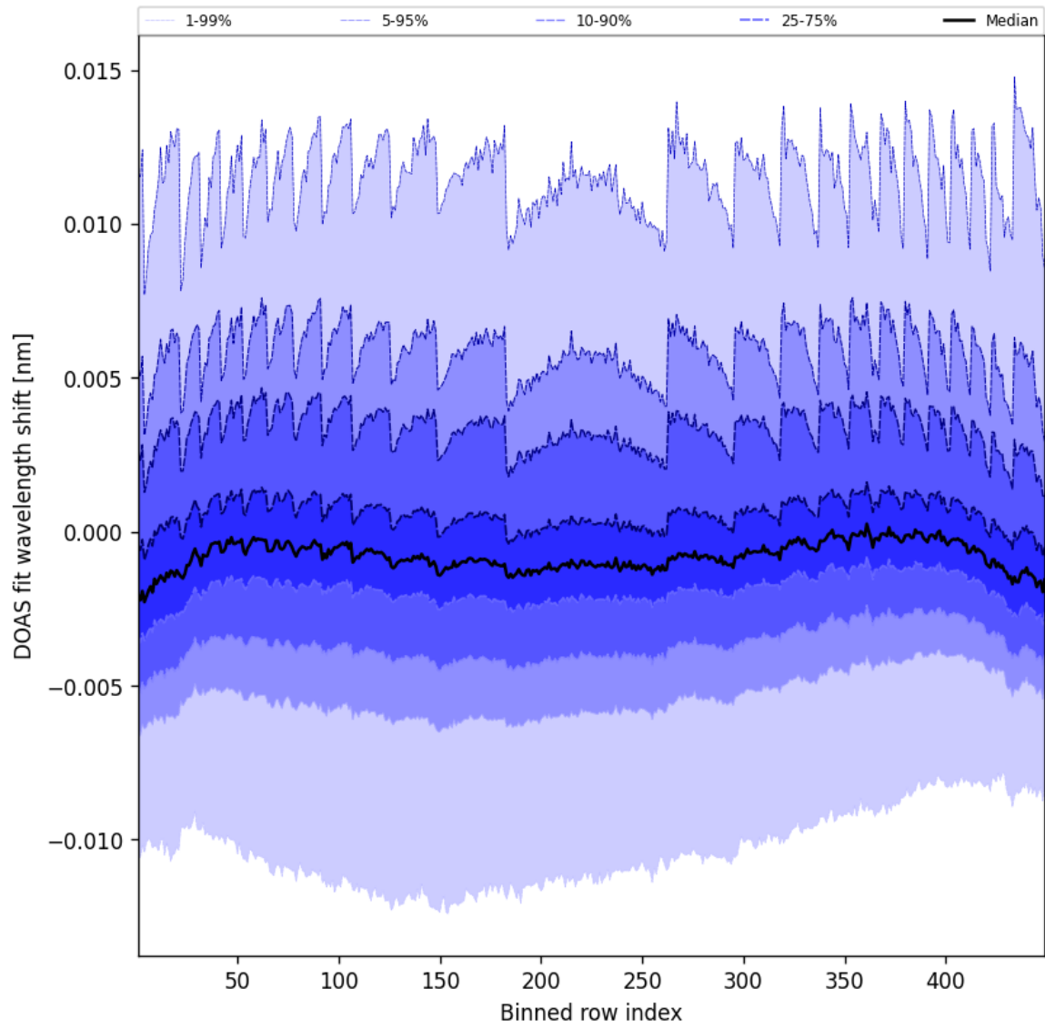
Figure 47: Along track statistics of “DOAS fit wavelength shift” for 2025-05-08 to 2025-05-08
