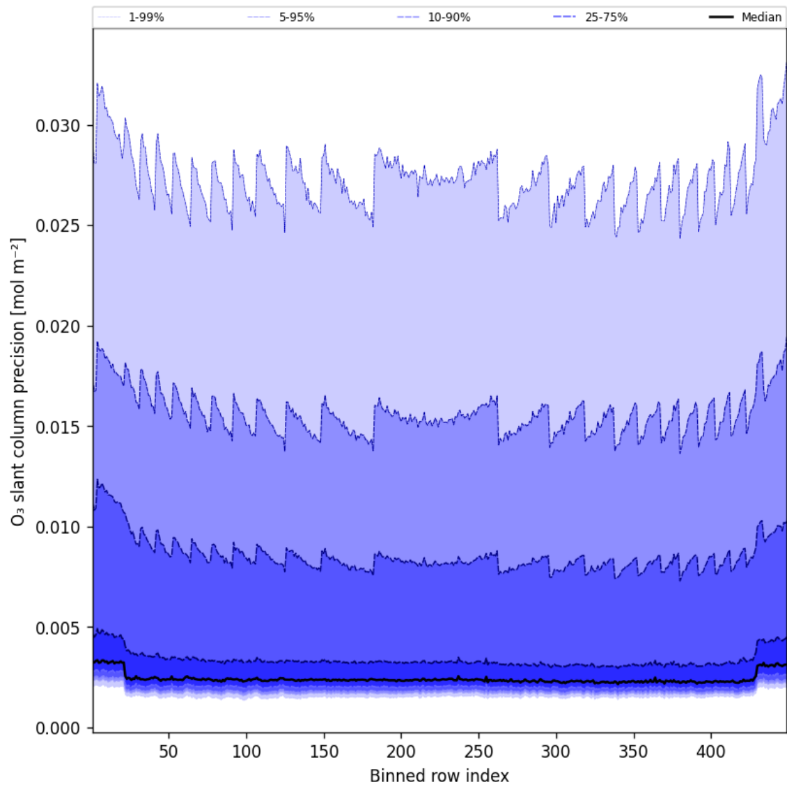
Figure 44: Along track statistics of “O 3 slant column precision” for 2025-05-08 to 2025-05-08
