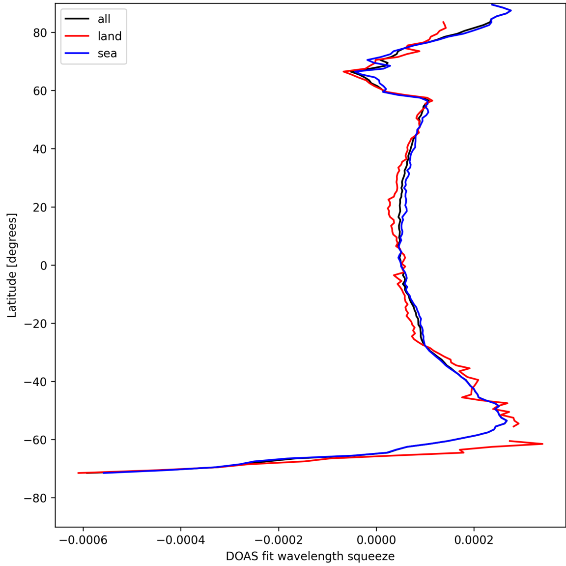
Figure 24: Zonal average of “DOAS fit wavelength squeeze” for 2025-05-08 to 2025-05-08.
