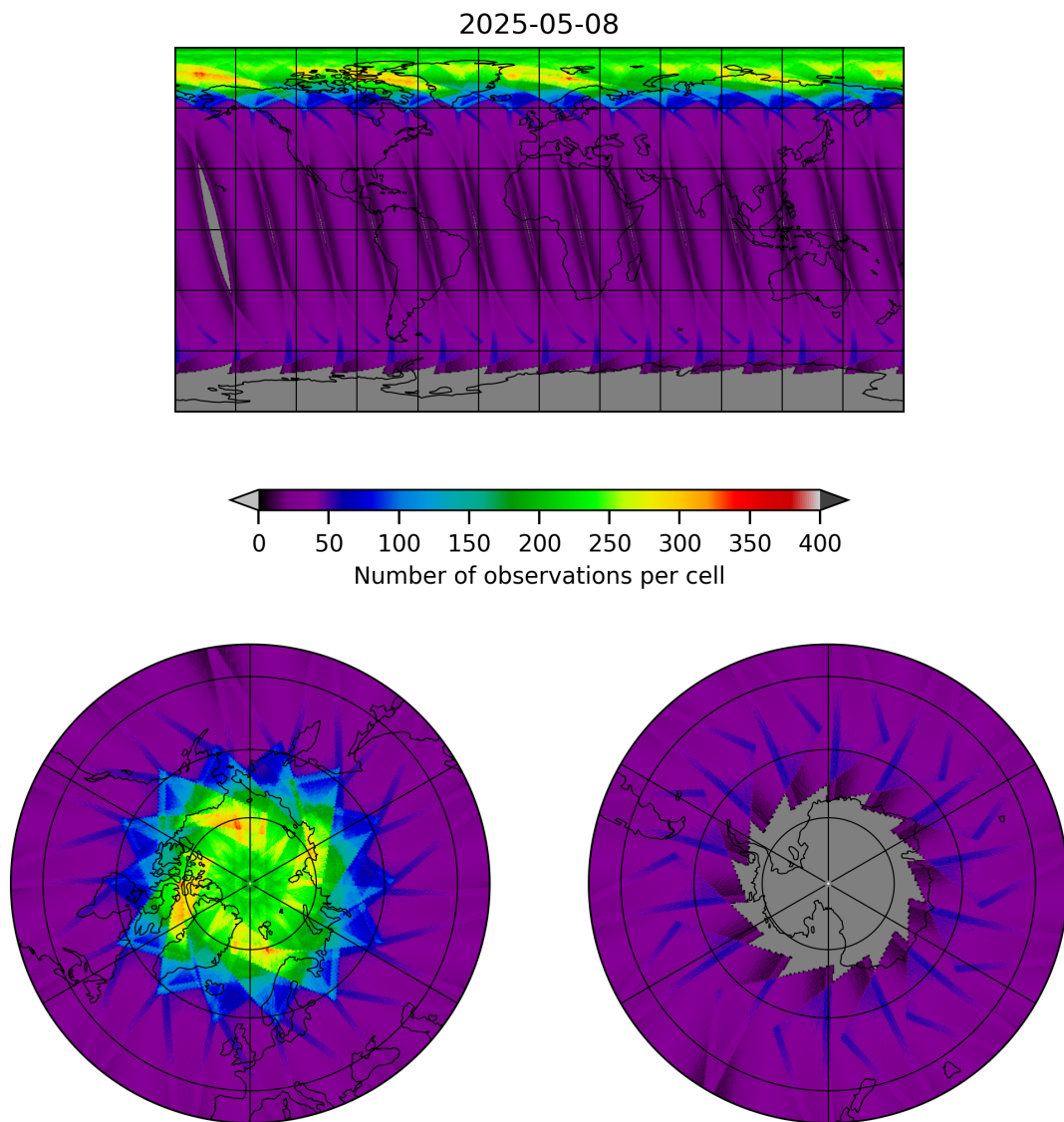
Figure 15: Map of the number of observations for 2025-05-08 to 2025-05-08
