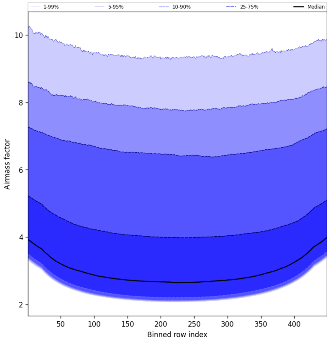
Figure 49: Along track statistics of “Airmass factor” for 2025-05-08 to 2025-05-08
