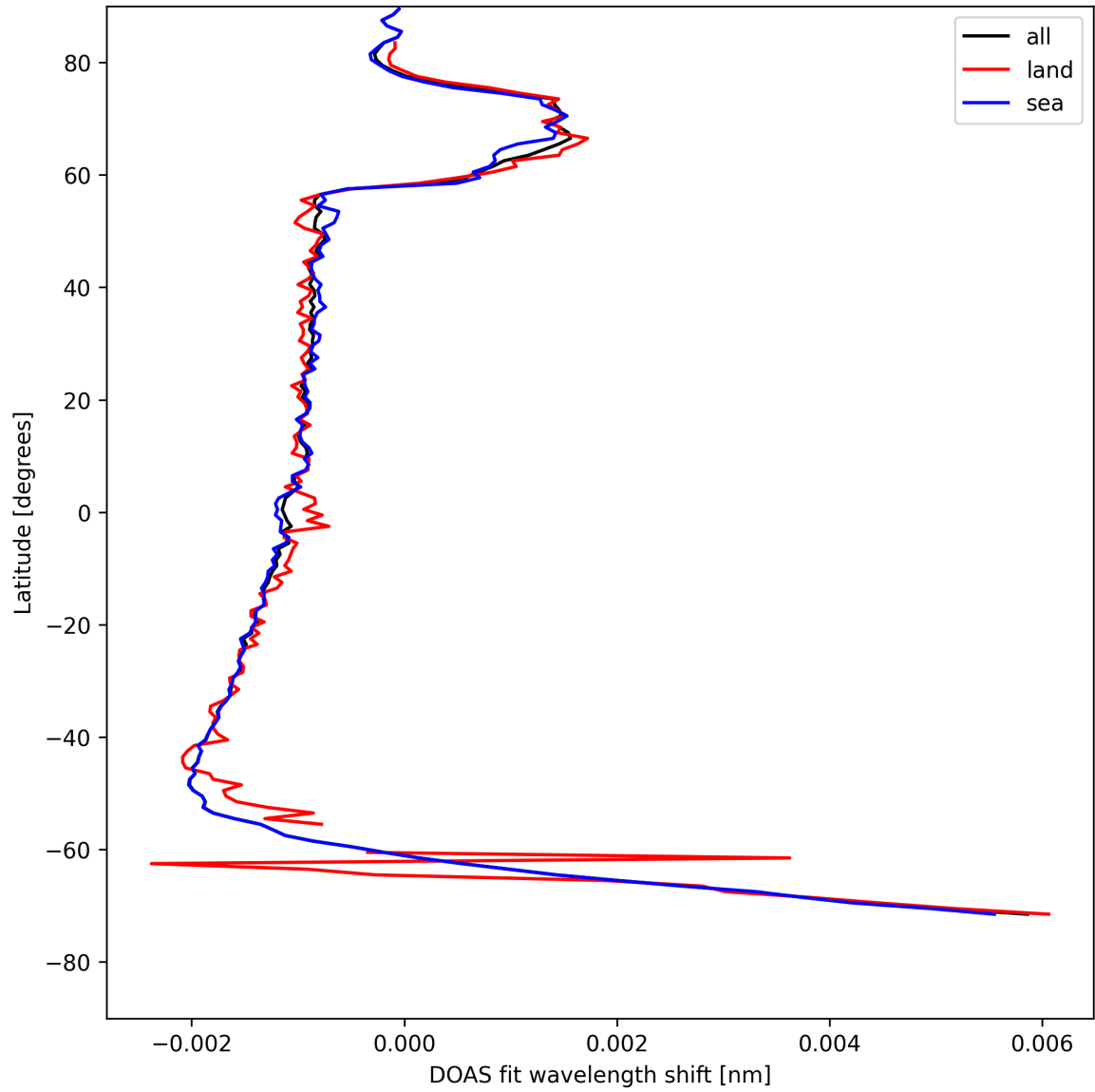
Figure 23: Zonal average of "DOAS fit wavelength shift" for 2025-05-08 to 2025-05-08.
