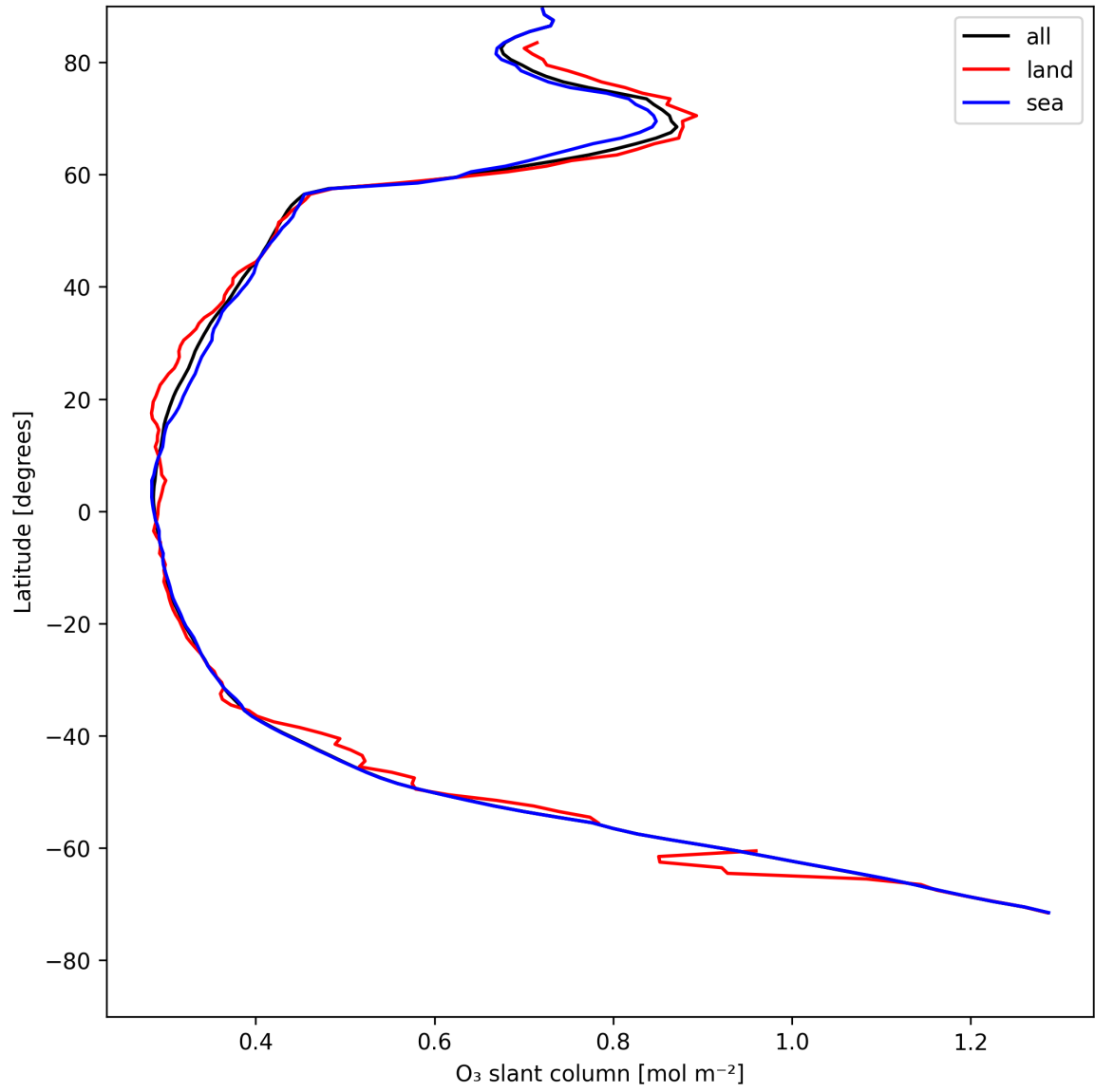
Figure 19: Zonal average of “O 3 slant column” for 2025-05-08 to 2025-05-08.
