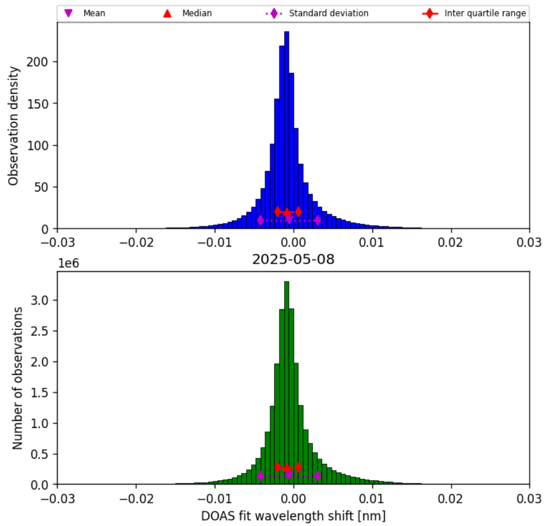
Figure 35: Histogram of “DOAS fit wavelength shift” for 2025-05-08 to 2025-05-08
