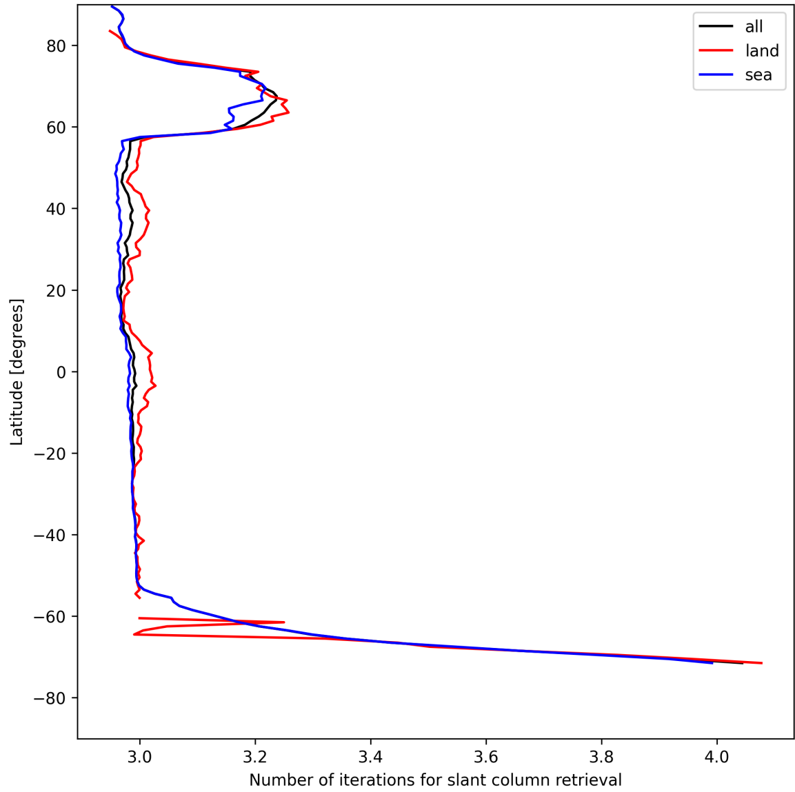
Figure 21: Zonal average of “Number of iterations for slant column retrieval” for 2025-05-08 to 2025-05-08.
