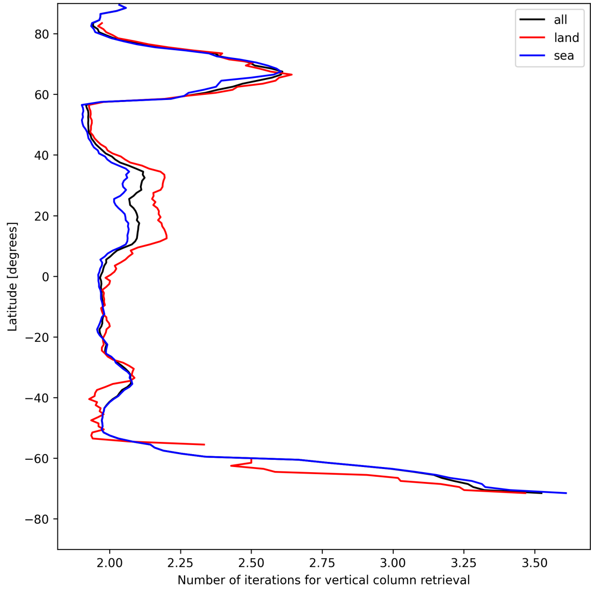
Figure 27: Zonal average of “Number of iterations for vertical column retrieval” for 2025-05-08 to 2025-05-08.
