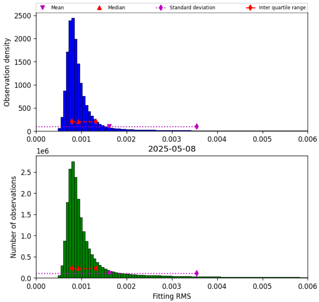
Figure 34: Histogram of “Fitting RMS” for 2025-05-08 to 2025-05-08
