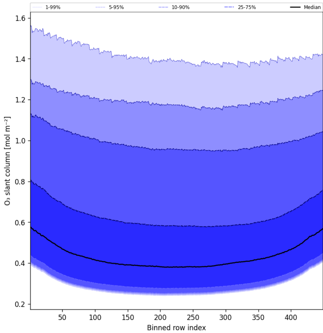
Figure 43: Along track statistics of “O 3 slant column” for 2025-05-08 to 2025-05-08
