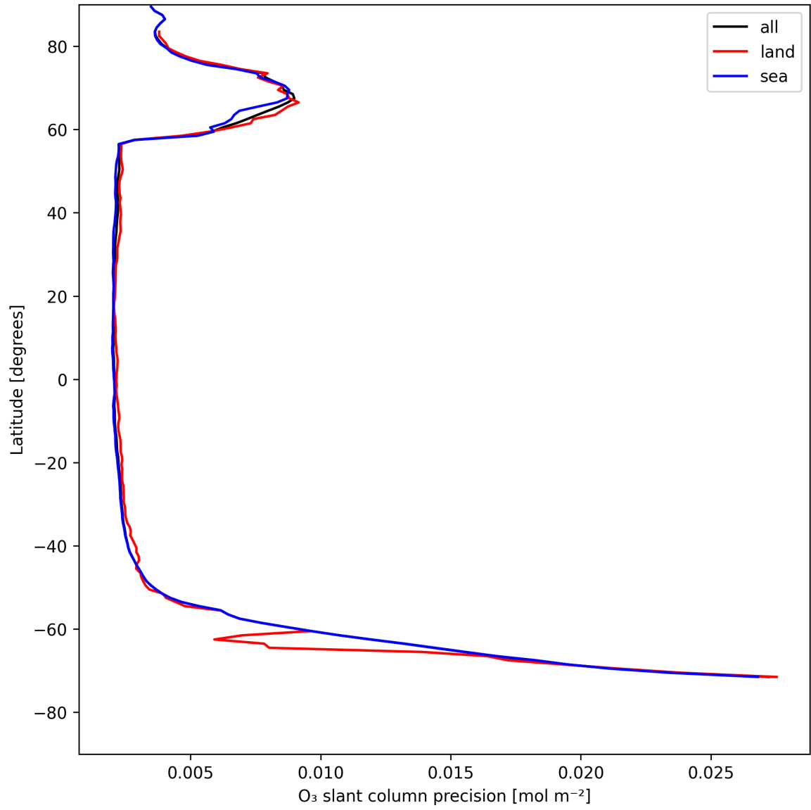
Figure 20: Zonal average of “O 3 slant column precision” for 2025-05-08 to 2025-05-08.
