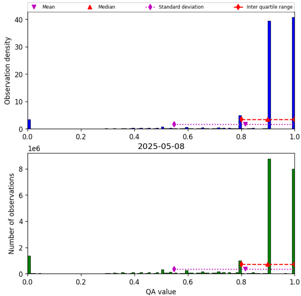
Figure 28: Histogram of “QA value” for 2025-05-08 to 2025-05-08
