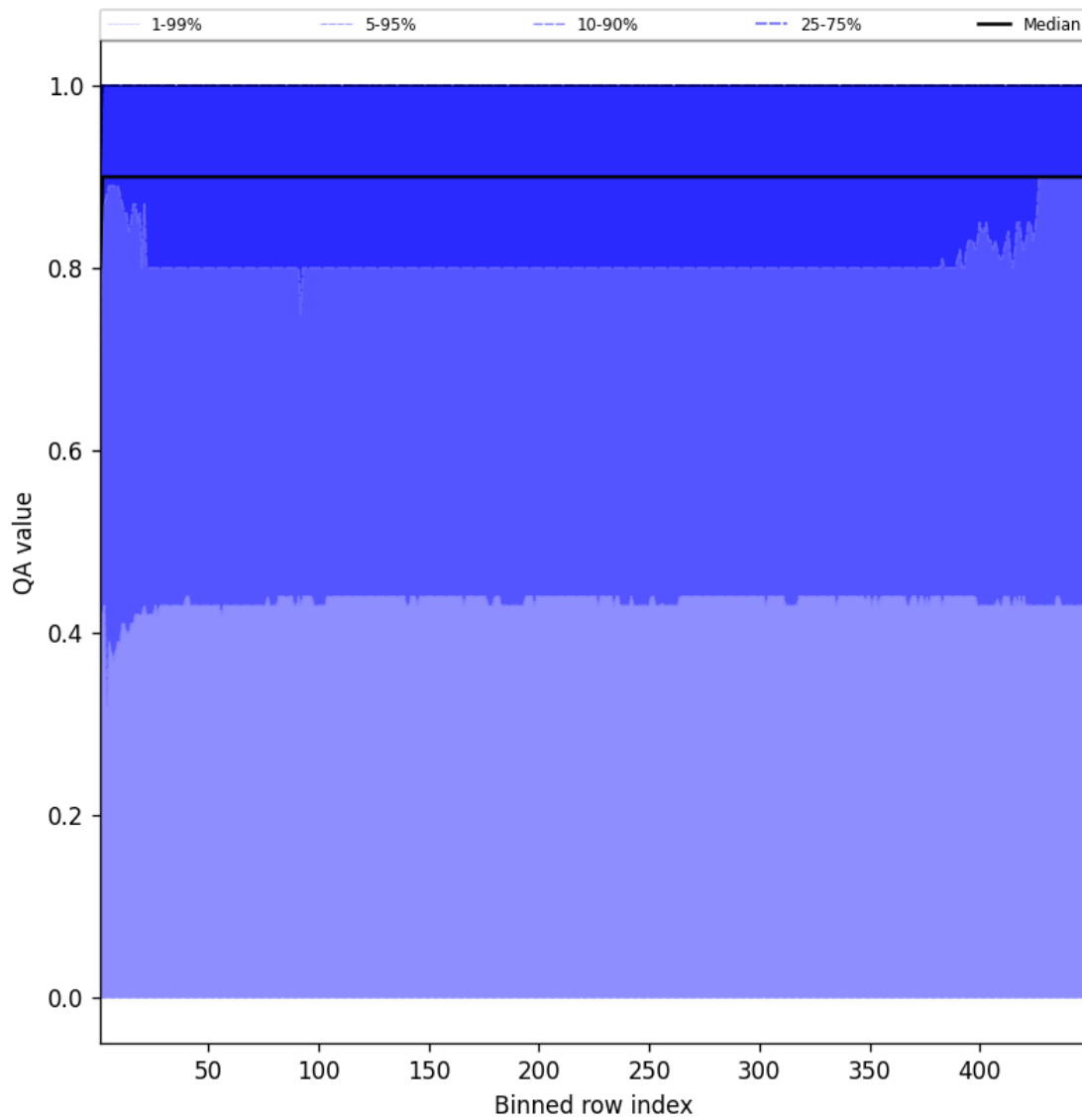
Figure 40: Along track statistics of "QA value" for 2025-05-08 to 2025-05-08
