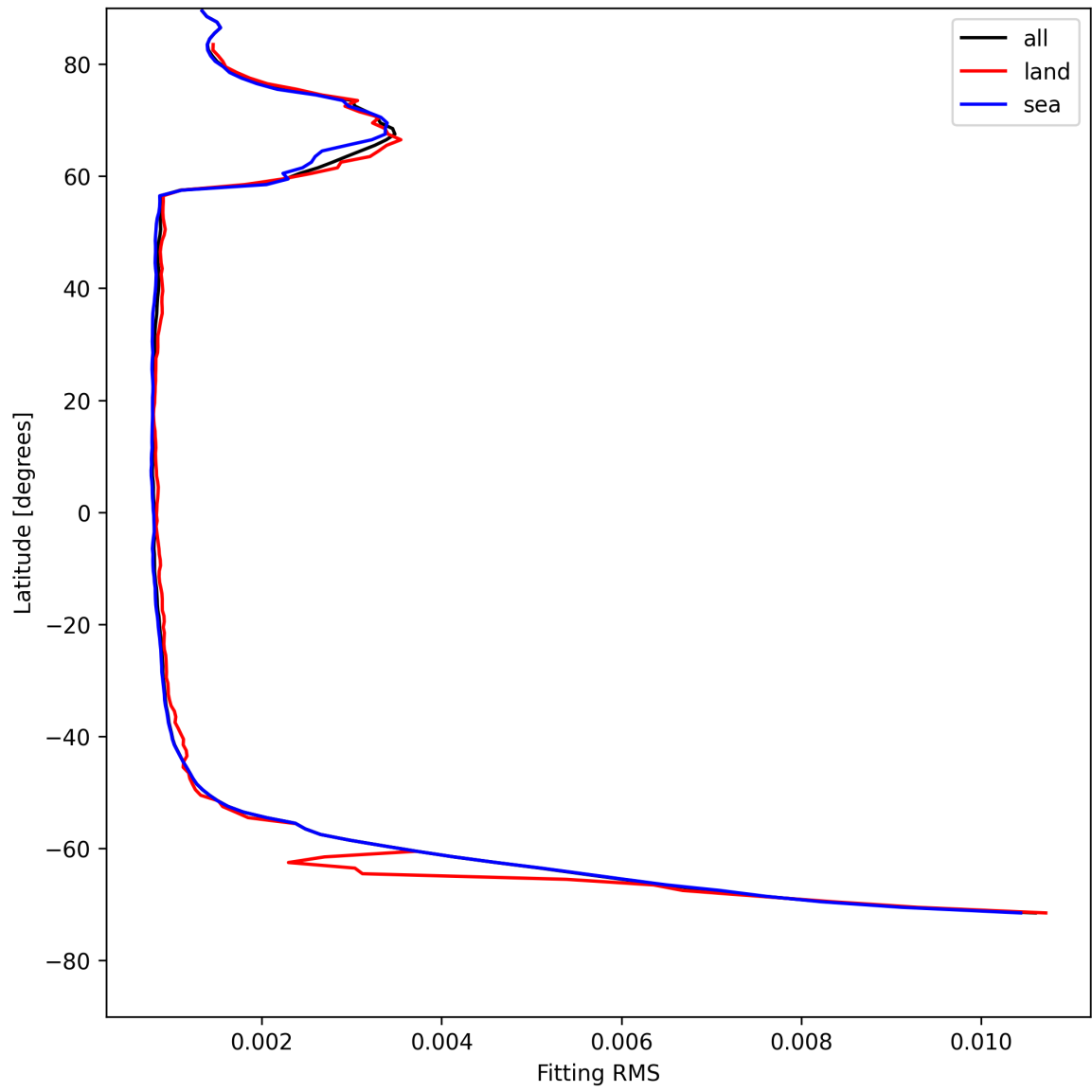
Figure 22: Zonal average of “Fitting RMS” for 2025-05-08 to 2025-05-08.
