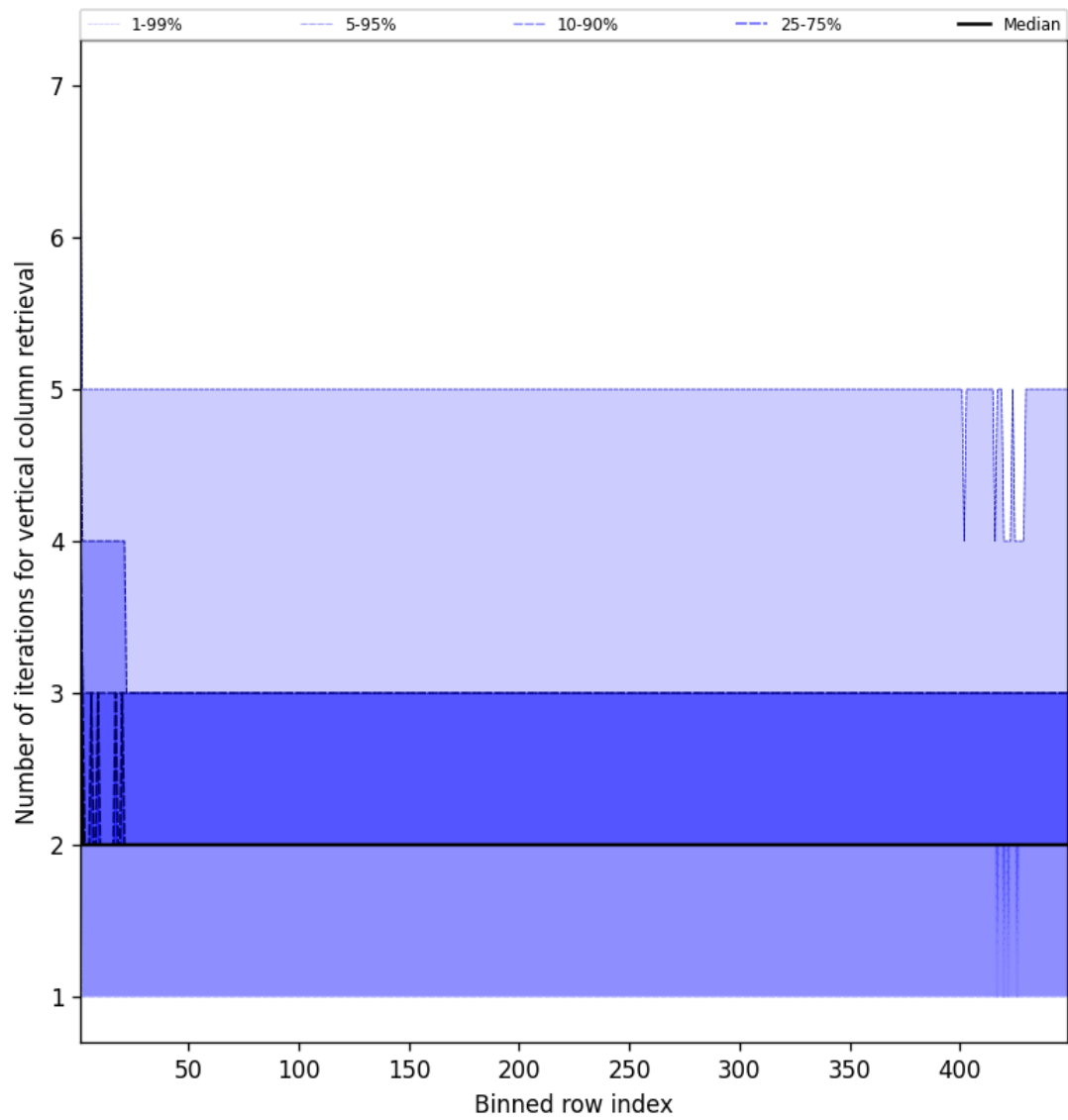
Figure 51: Along track statistics of “Number of iterations for vertical column retrieval” for 2025-05-08 to 2025-05-08
