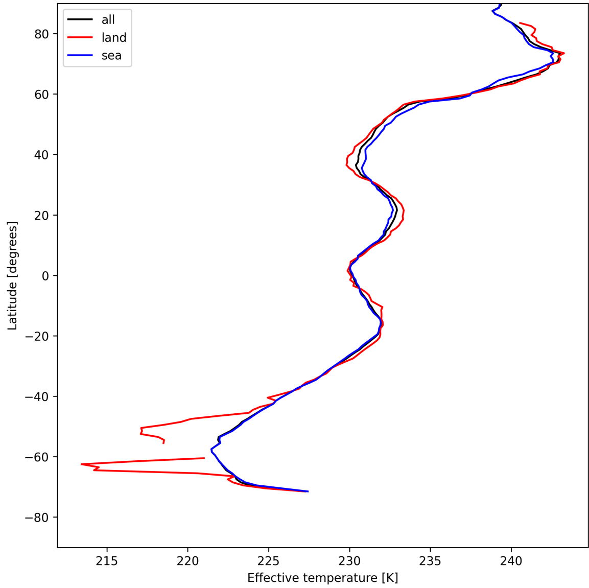
Figure 26: Zonal average of “Effective temperature” for 2025-05-08 to 2025-05-08.
