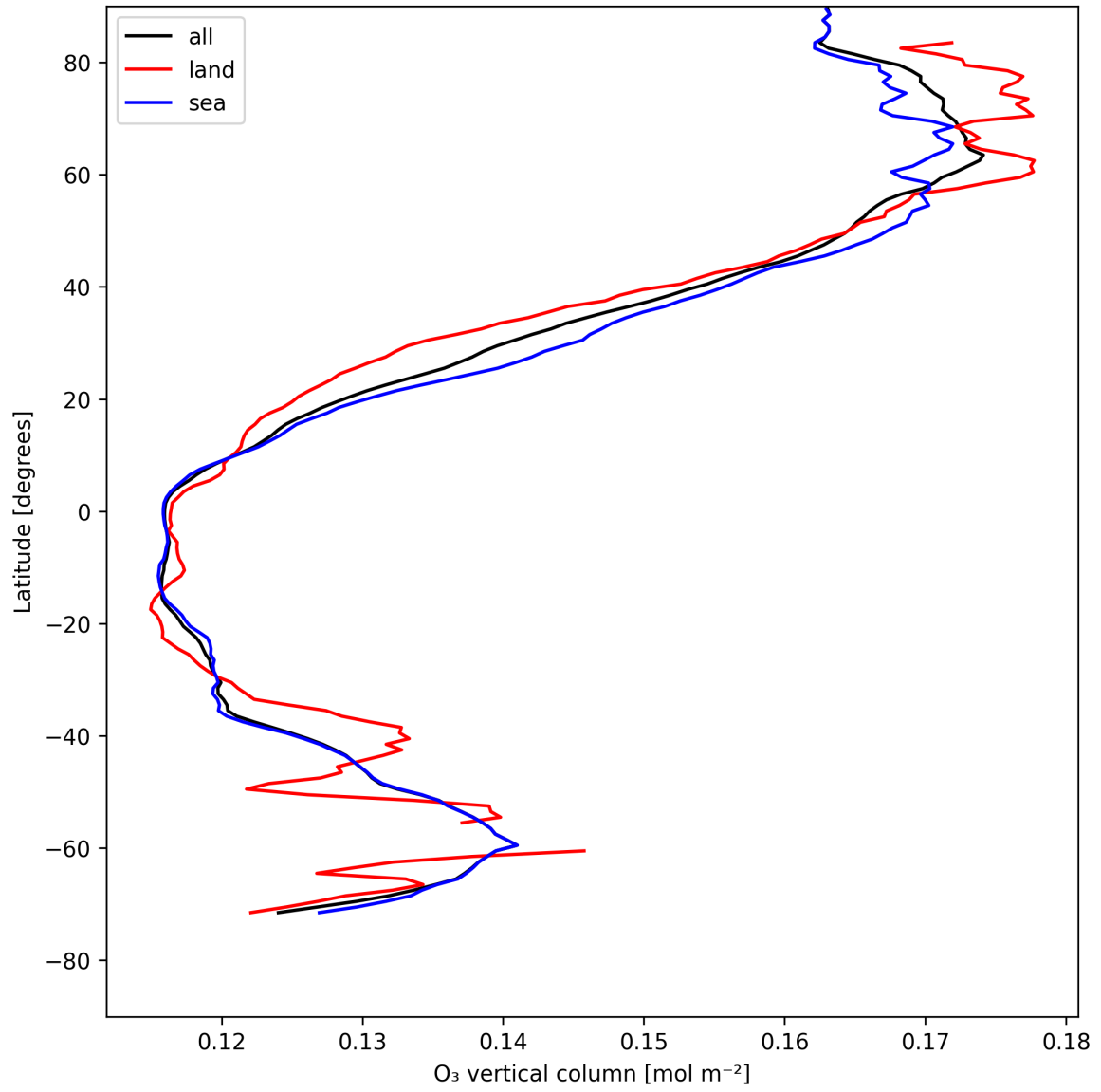
Figure 17: Zonal average of “O 3 vertical column” for 2025-05-08 to 2025-05-08.
