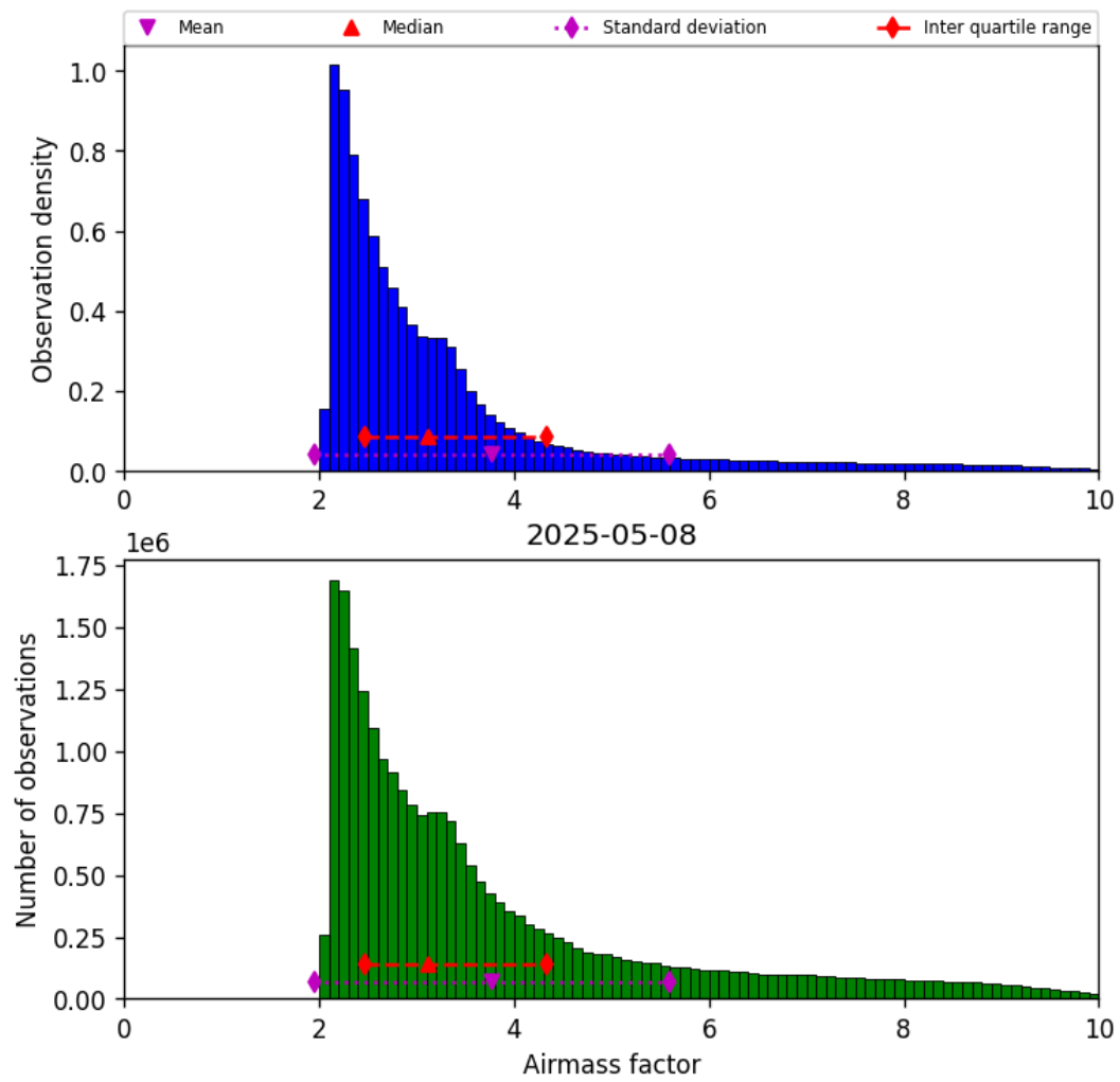
Figure 37: Histogram of “Airmass factor” for 2025-05-08 to 2025-05-08
