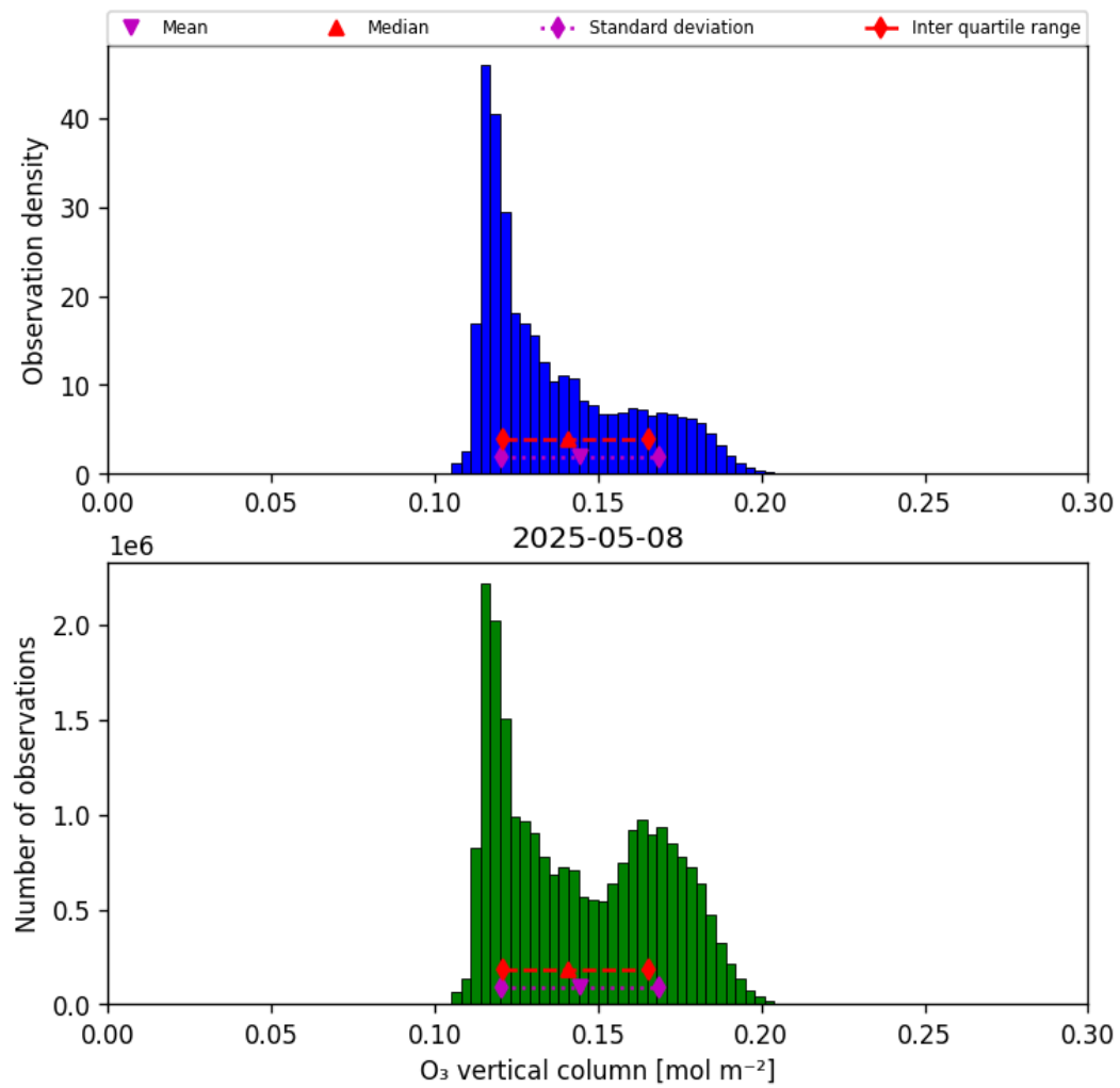
Figure 29: Histogram of “O 3 vertical column” for 2025-05-08 to 2025-05-08
