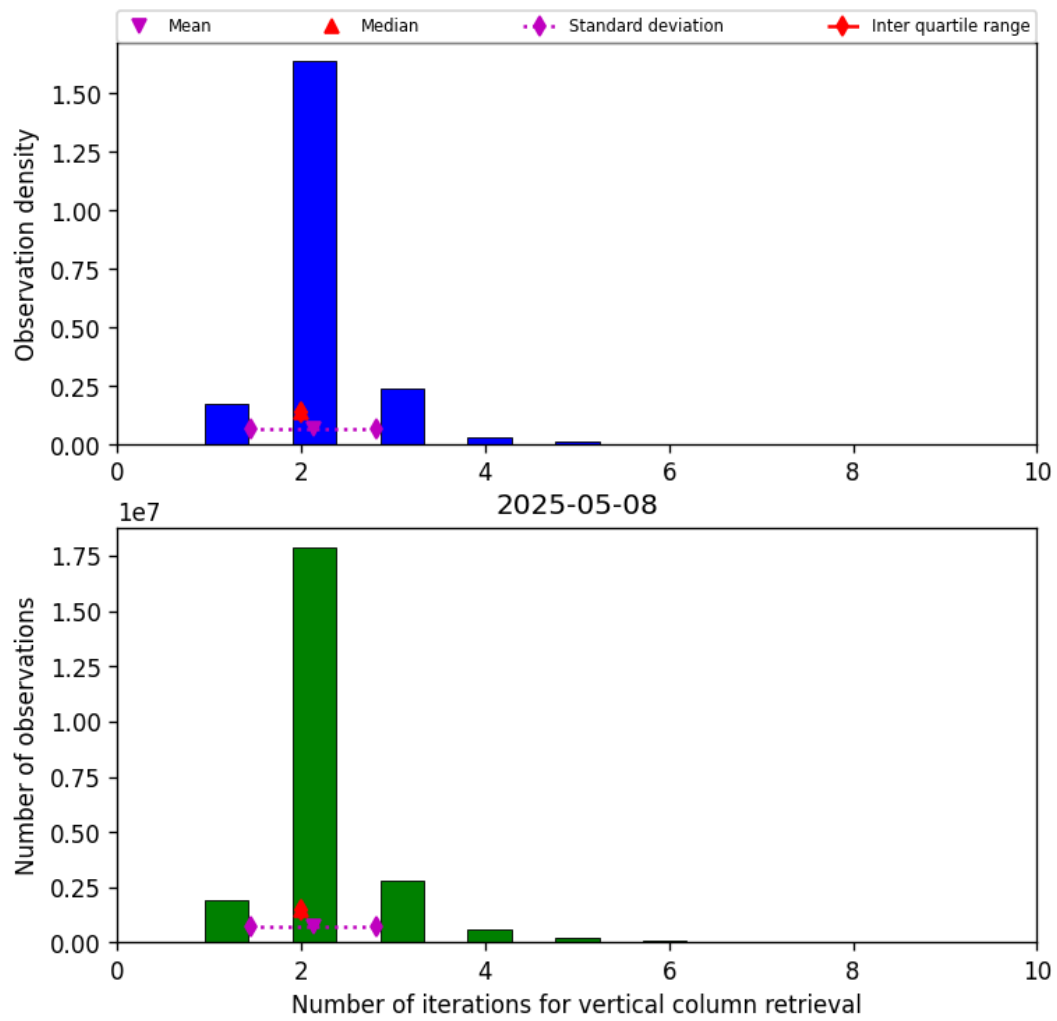
Figure 39: Histogram of “Number of iterations for vertical column retrieval” for 2025-05-08 to 2025-05-08
