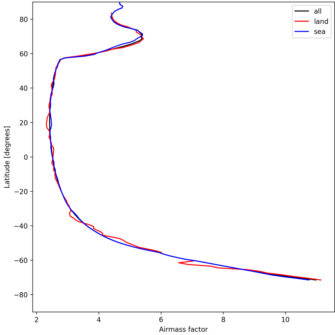
Figure 25: Zonal average of “Airmass factor” for 2025-05-08 to 2025-05-08.
