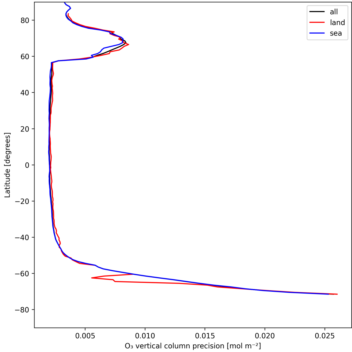
Figure 18: Zonal average of “O 3 vertical column precision” for 2025-05-08 to 2025-05-08.
