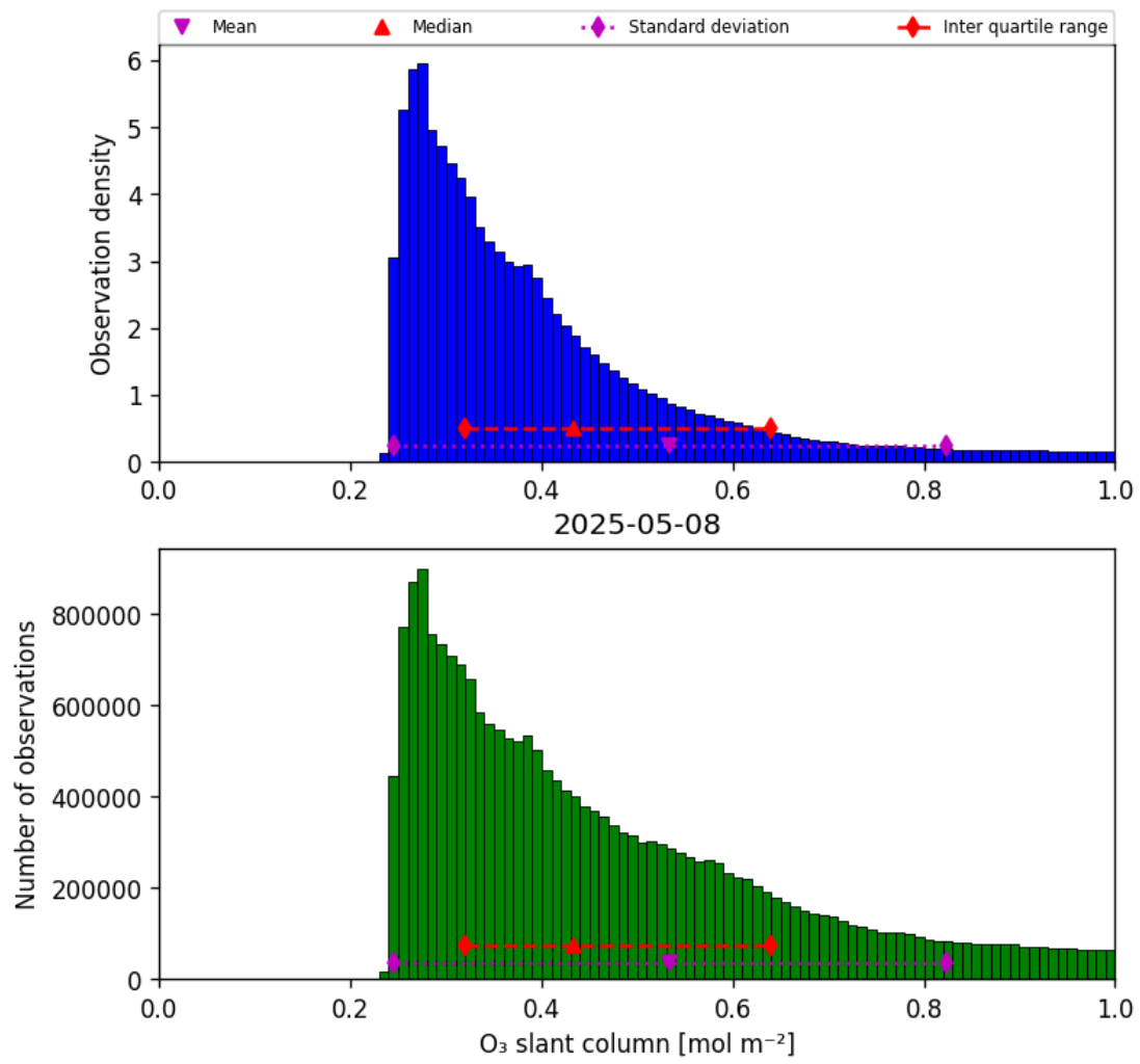
Figure 31: Histogram of “O 3 slant column” for 2025-05-08 to 2025-05-08
