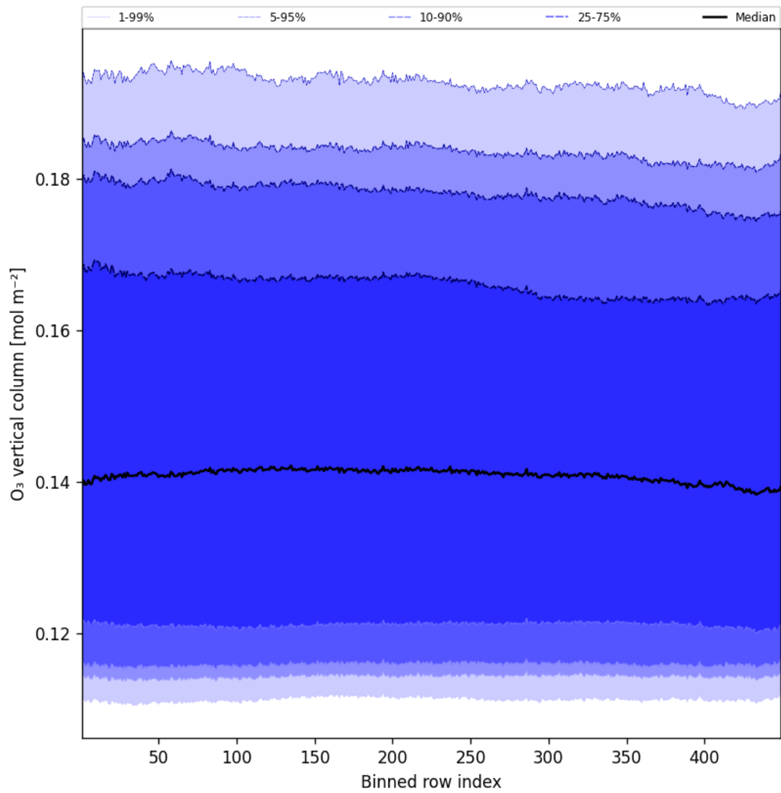
Figure 41: Along track statistics of “O 3 vertical column” for 2025-05-08 to 2025-05-08
