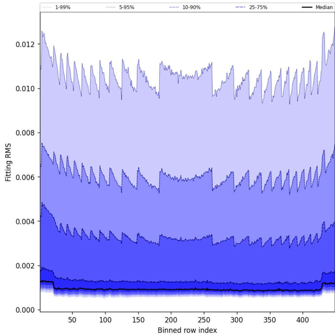
Figure 46: Along track statistics of “Fitting RMS” for 2025-05-08 to 2025-05-08
