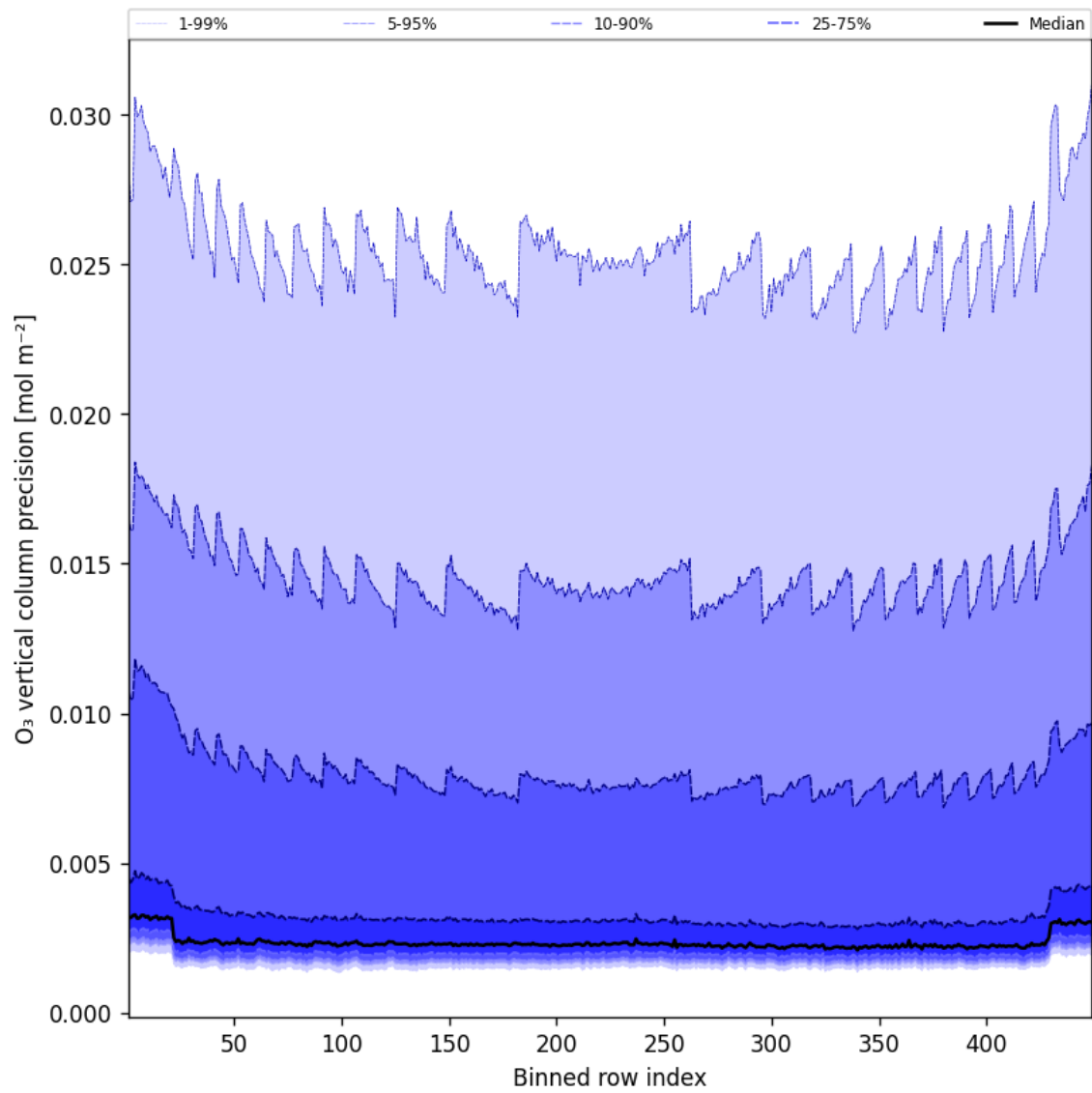
Figure 42: Along track statistics of “O 3 vertical column precision” for 2025-05-08 to 2025-05-08
