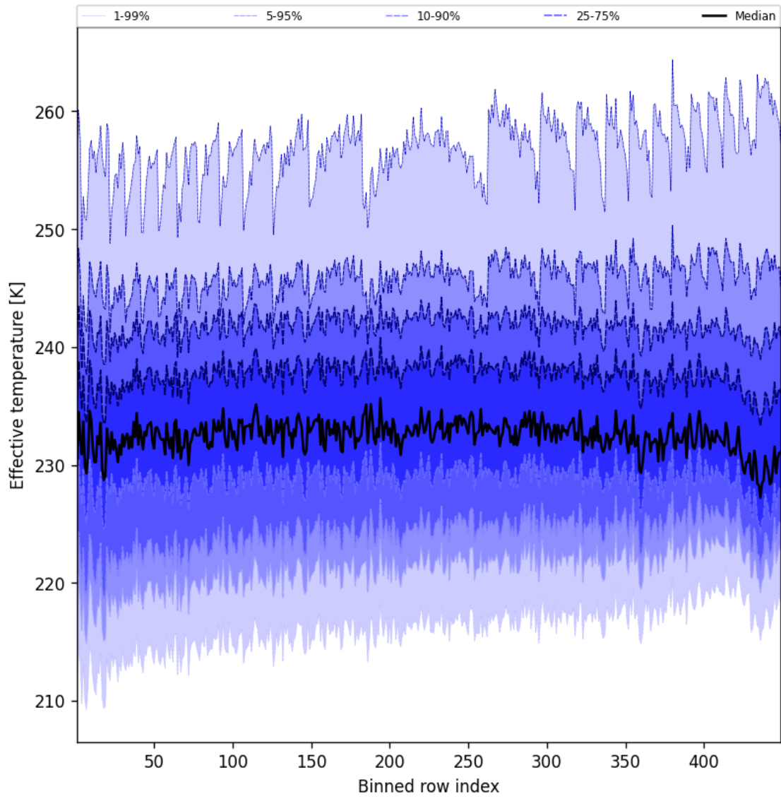
Figure 50: Along track statistics of “Effective temperature” for 2025-05-08 to 2025-05-08
