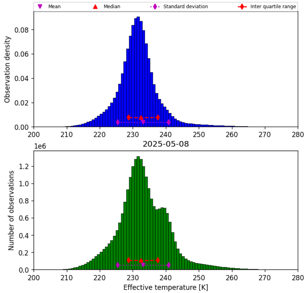
Figure 38: Histogram of “Effective temperature” for 2025-05-08 to 2025-05-08
