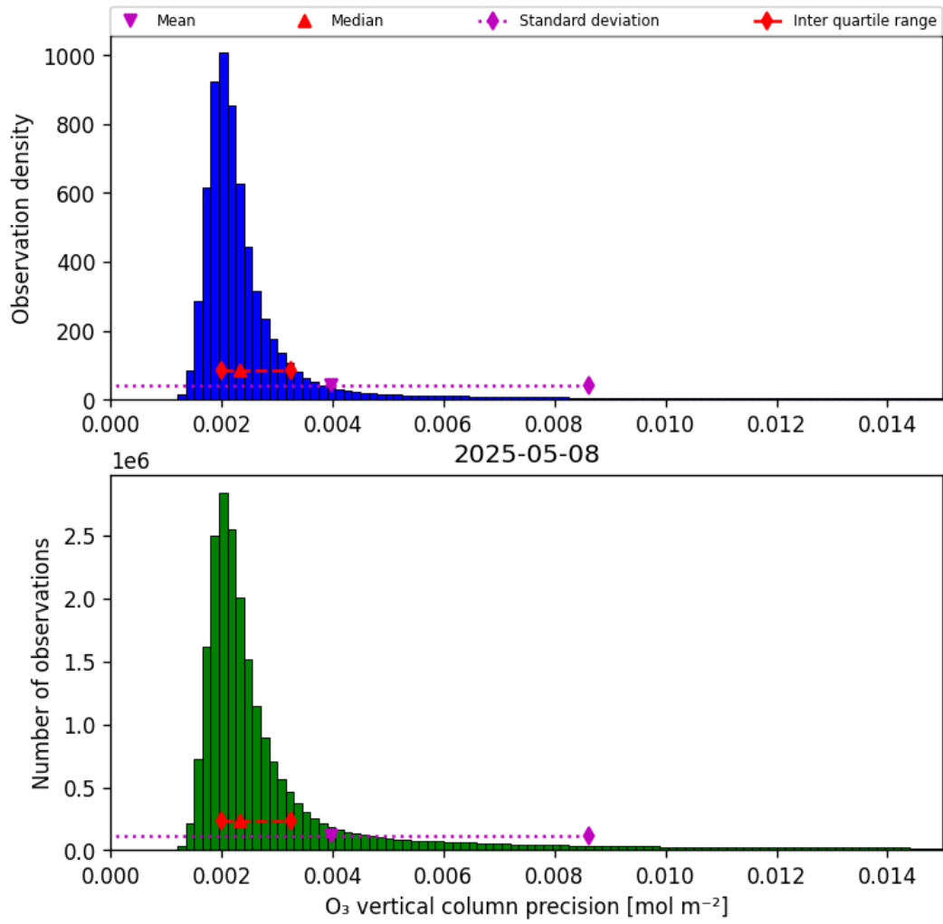
Figure 30: Histogram of “O 3 vertical column precision” for 2025-05-08 to 2025-05-08
