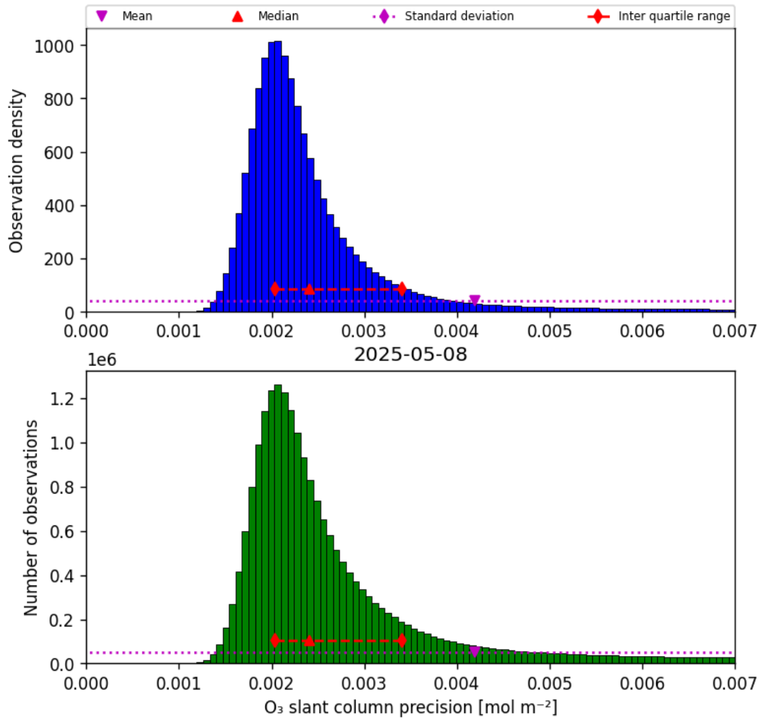
Figure 32: Histogram of “O 3 slant column precision” for 2025-05-08 to 2025-05-08
