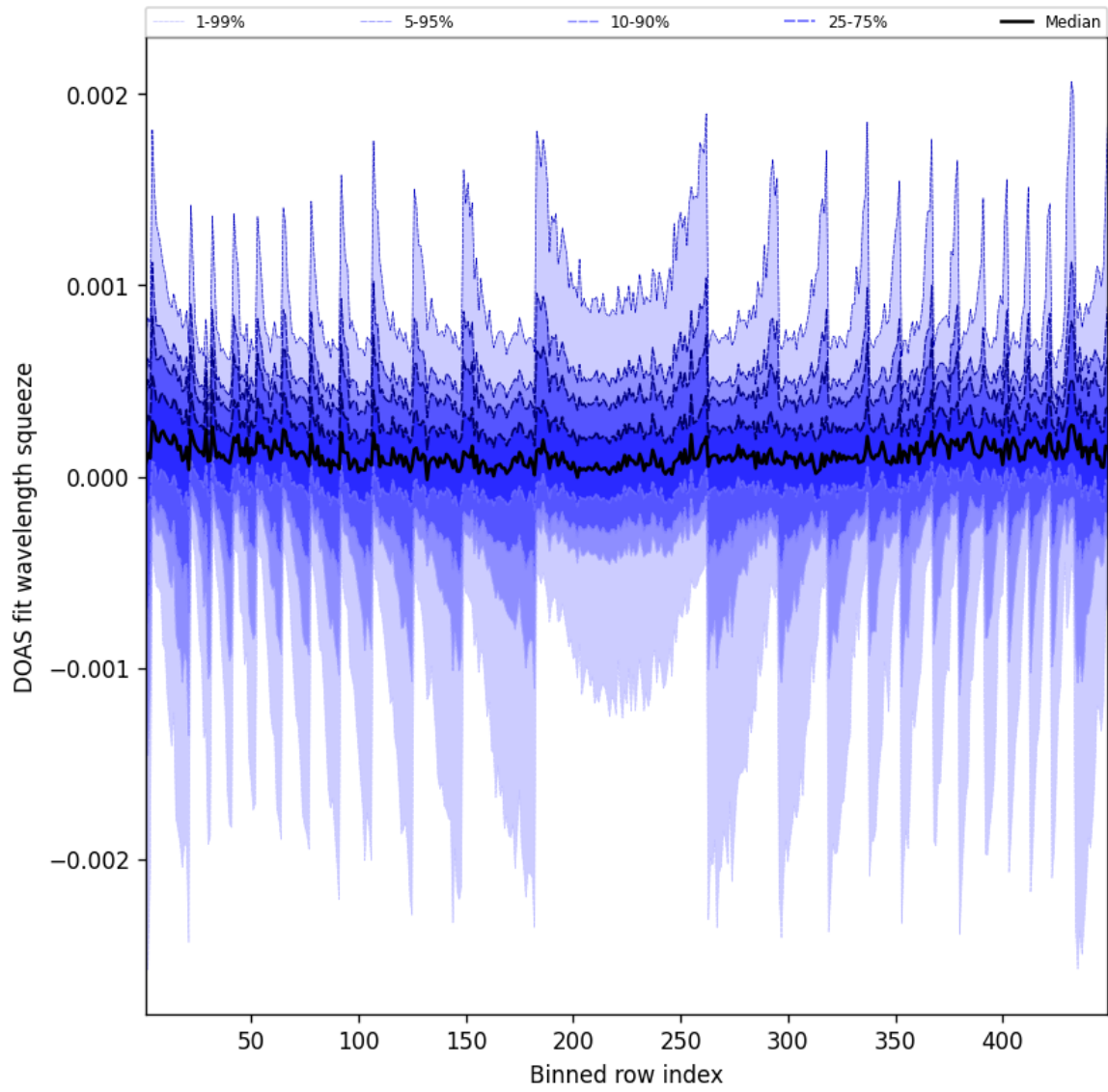
Figure 48: Along track statistics of “DOAS fit wavelength squeeze” for 2025-05-08 to 2025-05-08
