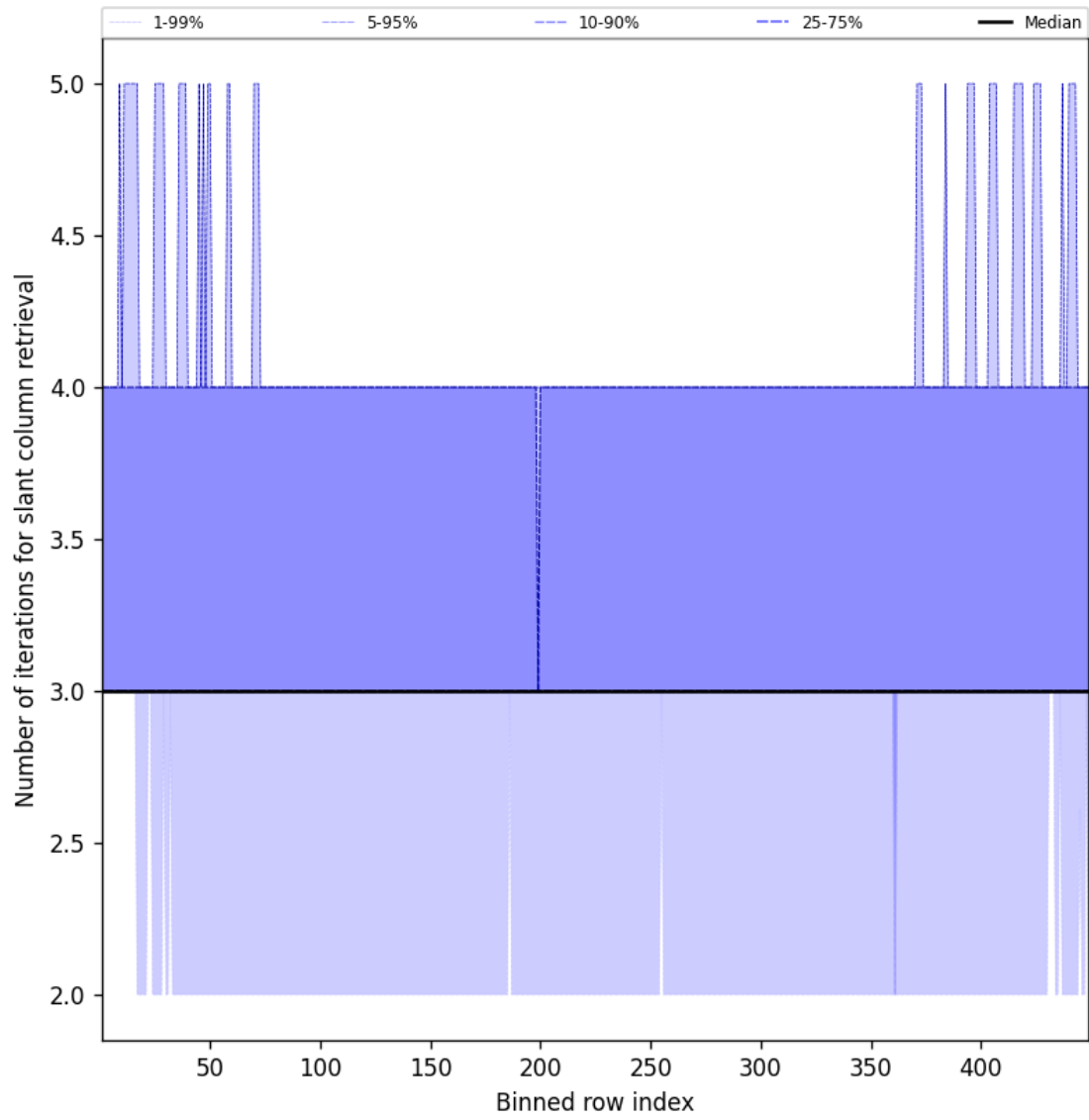
Figure 45: Along track statistics of “Number of iterations for slant column retrieval” for 2025-05-08 to 2025-05-08
