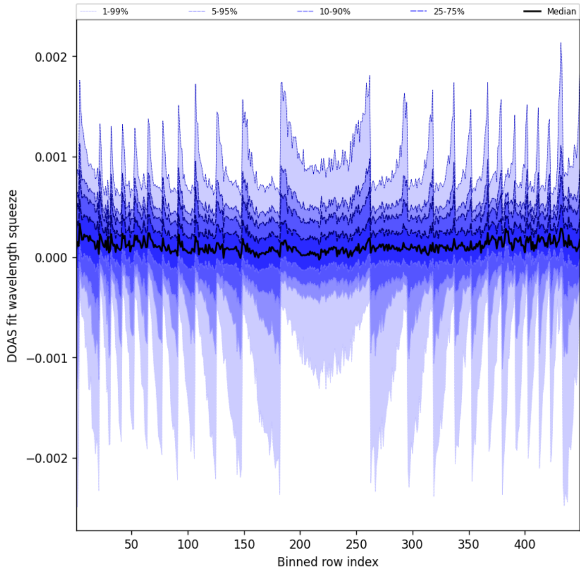
Figure 48: Along track statistics of “DOAS fit wavelength squeeze” for 2025-05-10 to 2025-05-11
