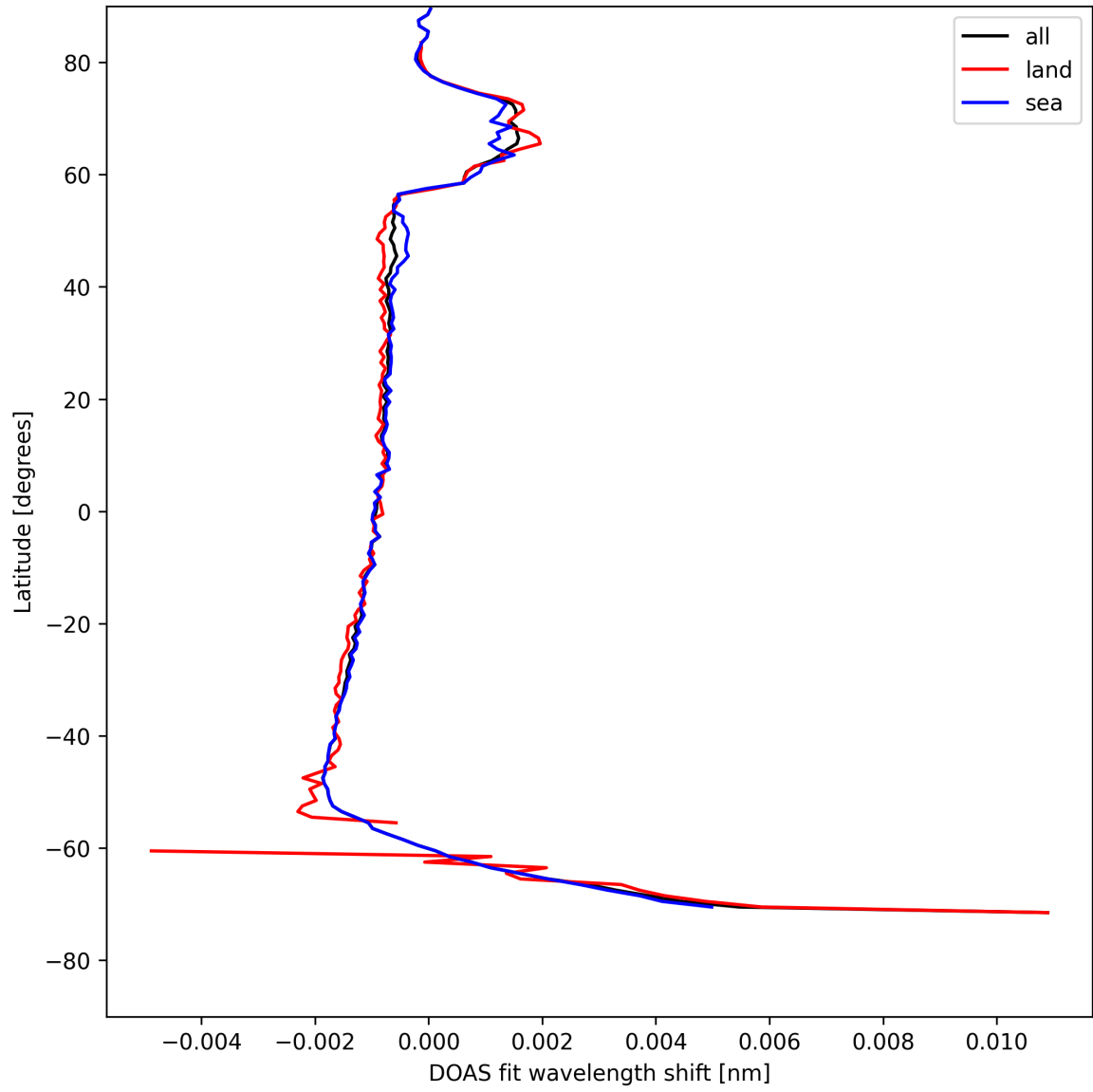
Figure 23: Zonal average of “DOAS fit wavelength shift” for 2025-05-10 to 2025-05-11.
