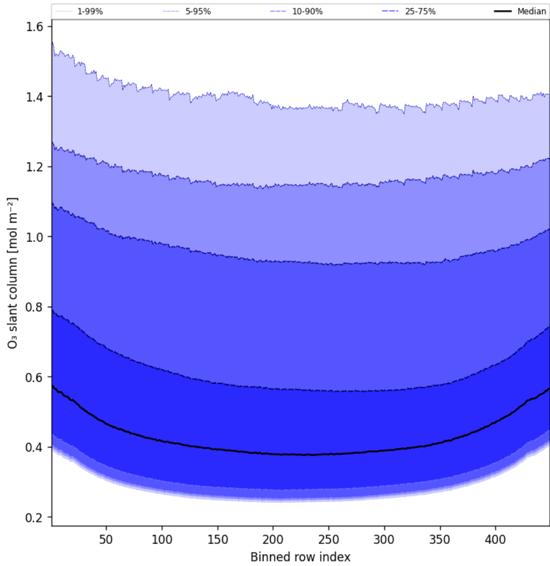
Figure 43: Along track statistics of “O 3 slant column” for 2025-05-10 to 2025-05-11
