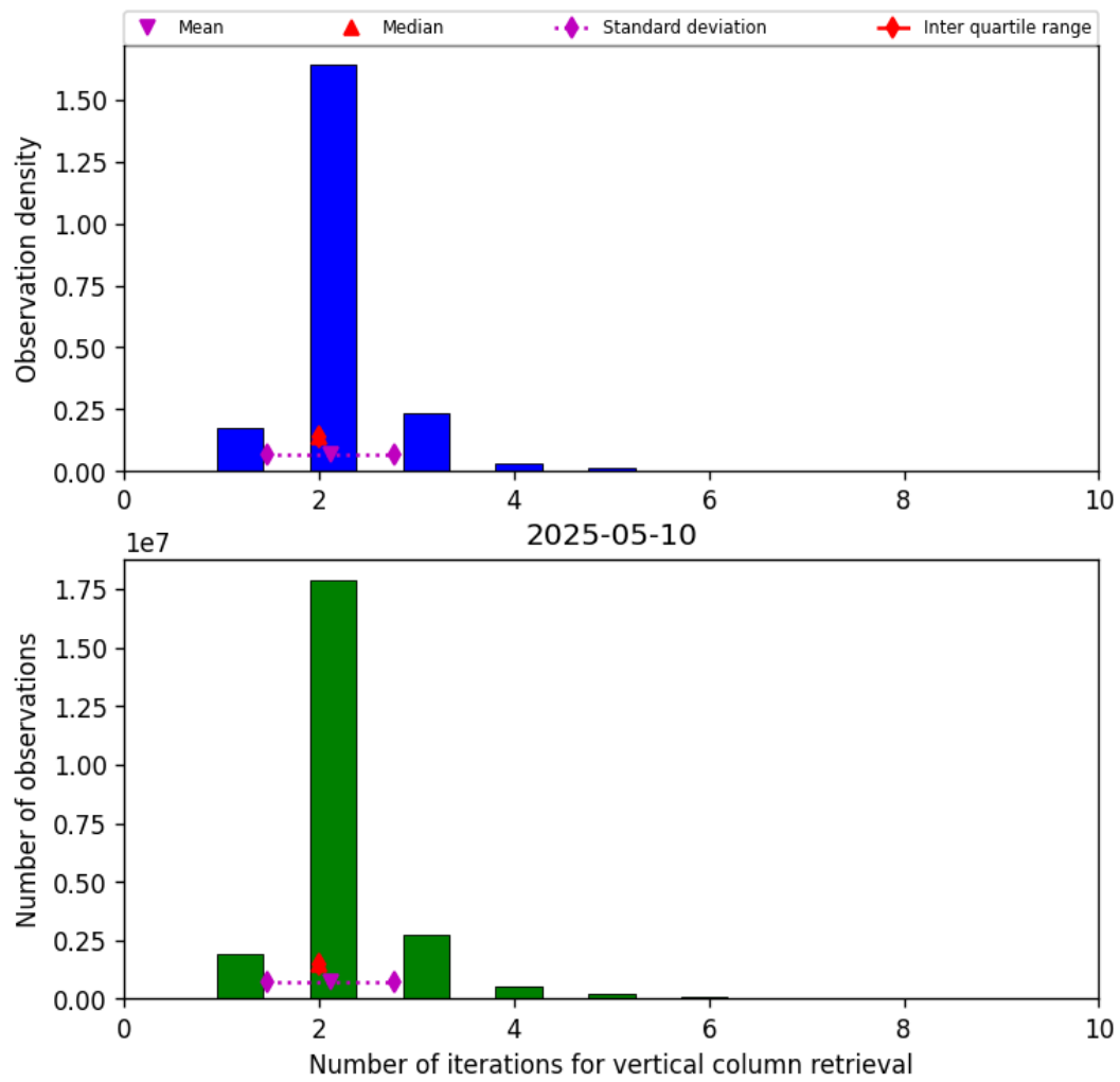
Figure 39: Histogram of “Number of iterations for vertical column retrieval” for 2025-05-10 to 2025-05-11
