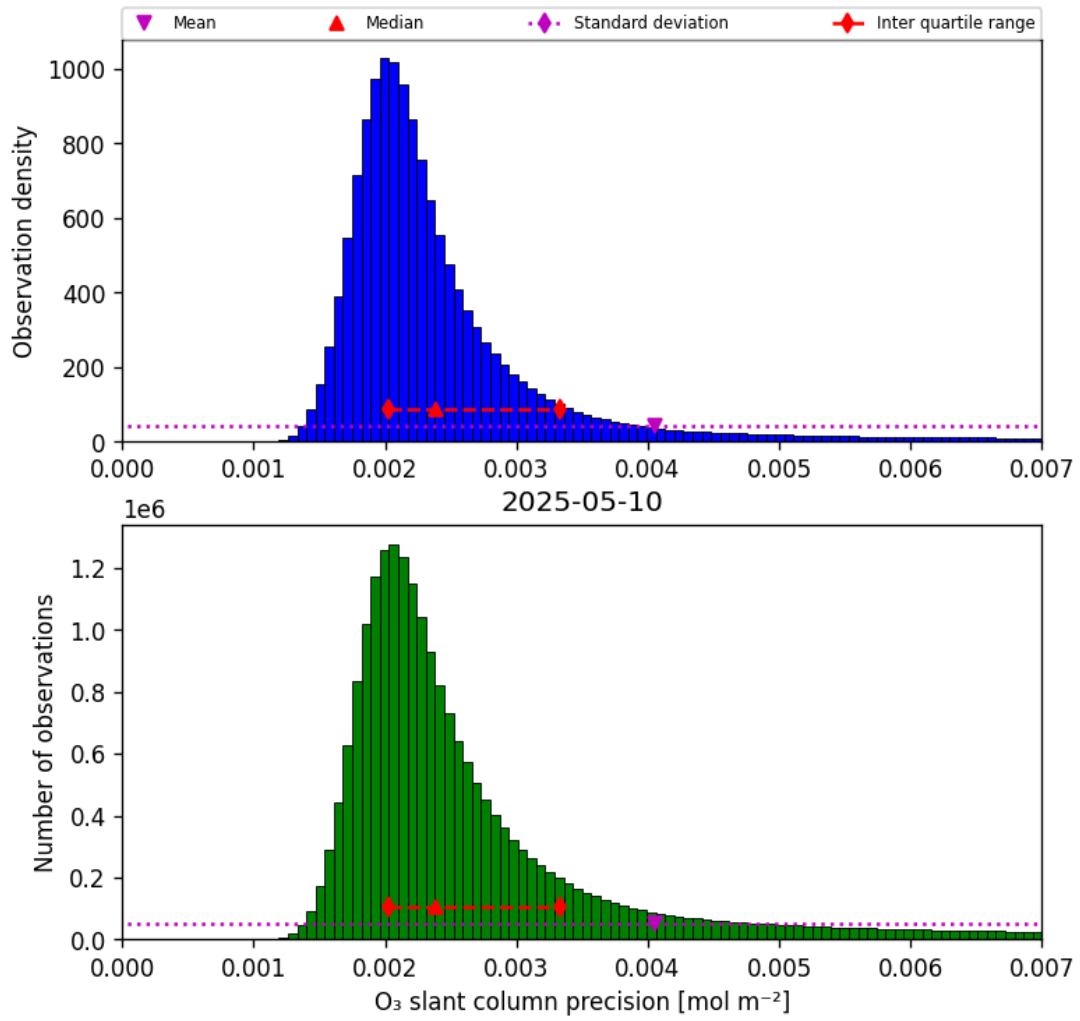
Figure 32: Histogram of “O 3 slant column precision” for 2025-05-10 to 2025-05-11
