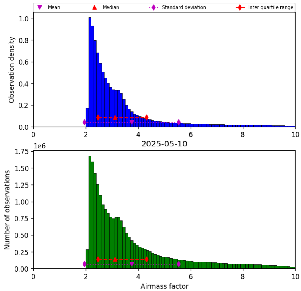
Figure 37: Histogram of “Airmass factor” for 2025-05-10 to 2025-05-11
