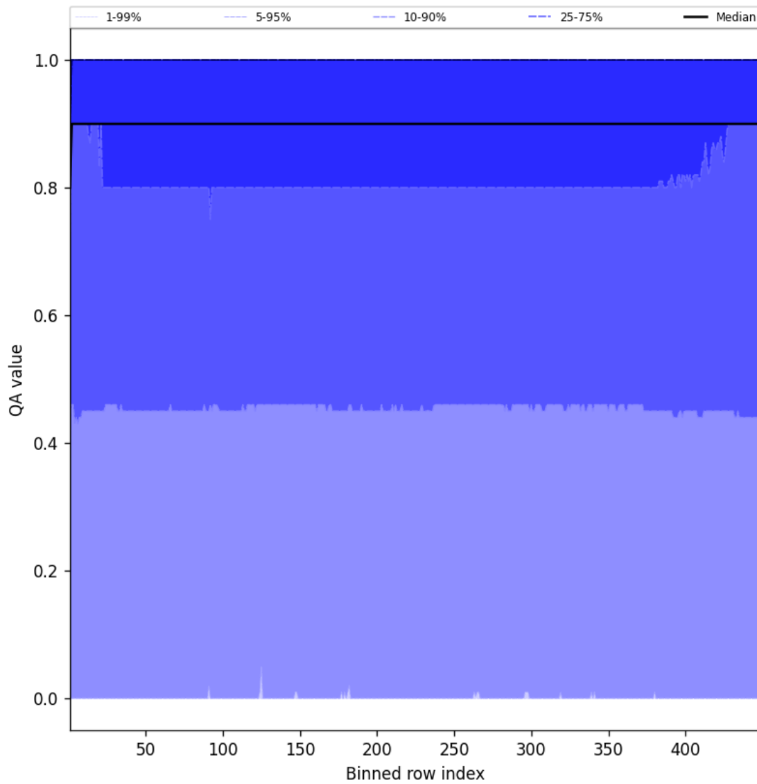
Figure 40: Along track statistics of “QA value” for 2025-05-10 to 2025-05-11
