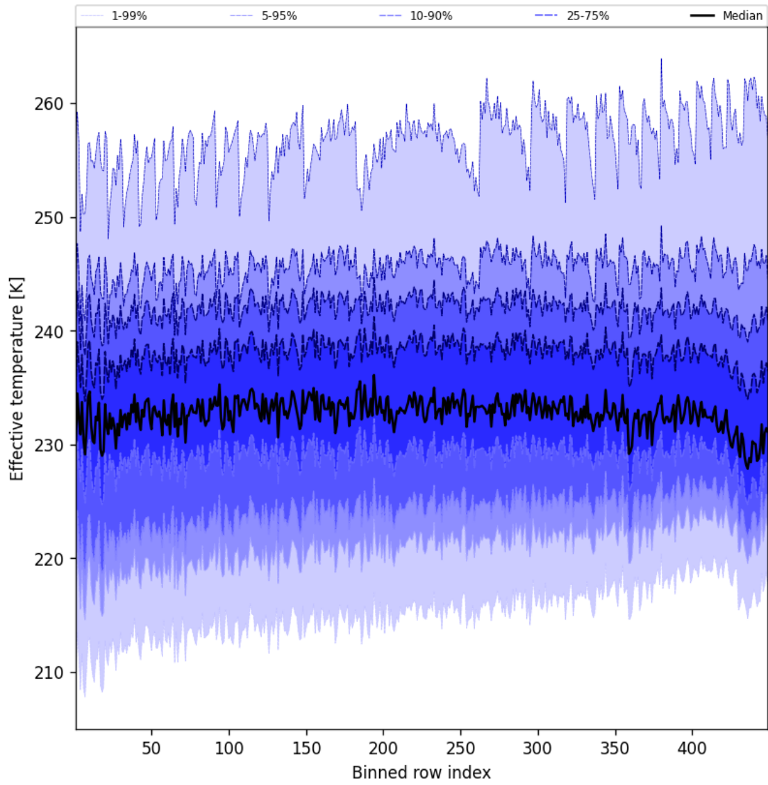
Figure 50: Along track statistics of "Effective temperature" for 2025-05-10 to 2025-05-11
