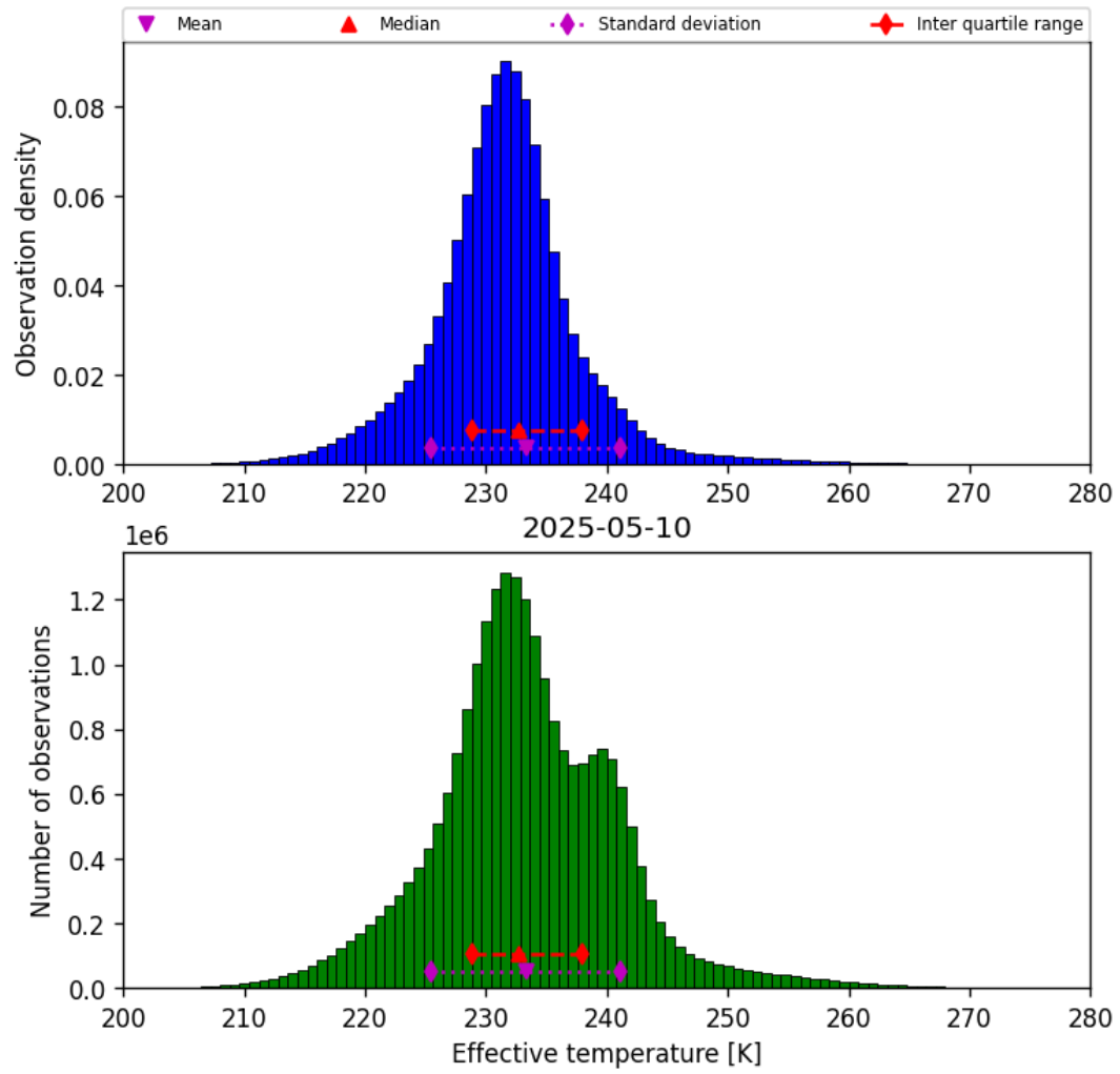
Figure 38: Histogram of “Effective temperature” for 2025-05-10 to 2025-05-11
