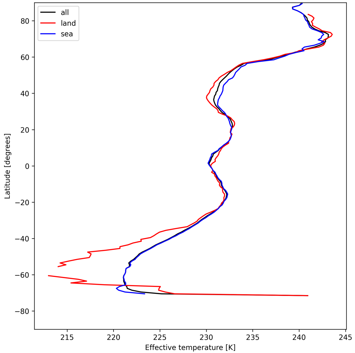
Figure 26: Zonal average of “Effective temperature” for 2025-05-10 to 2025-05-11.
