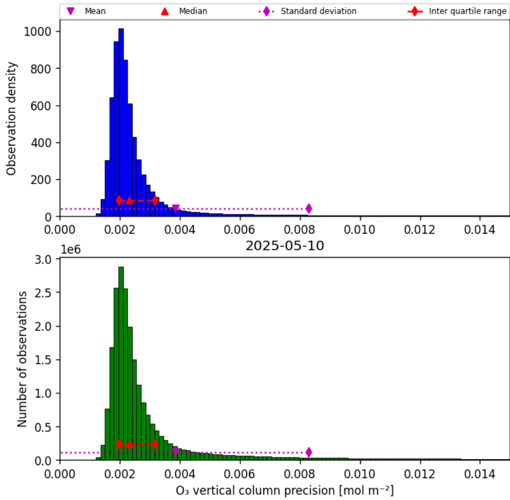
Figure 30: Histogram of “O 3 vertical column precision” for 2025-05-10 to 2025-05-11
