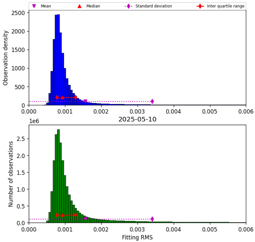
Figure 34: Histogram of “Fitting RMS” for 2025-05-10 to 2025-05-11
