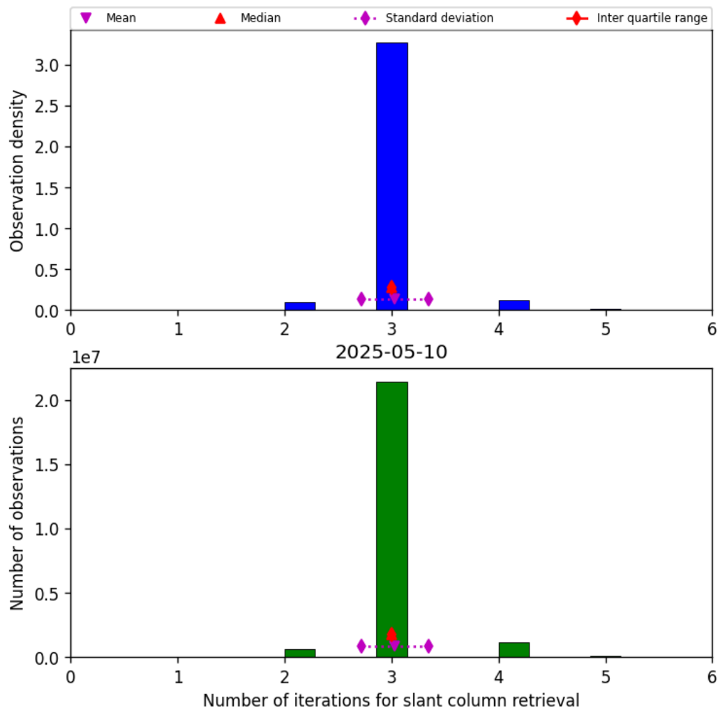
Figure 33: Histogram of “Number of iterations for slant column retrieval” for 2025-05-10 to 2025-05-11
