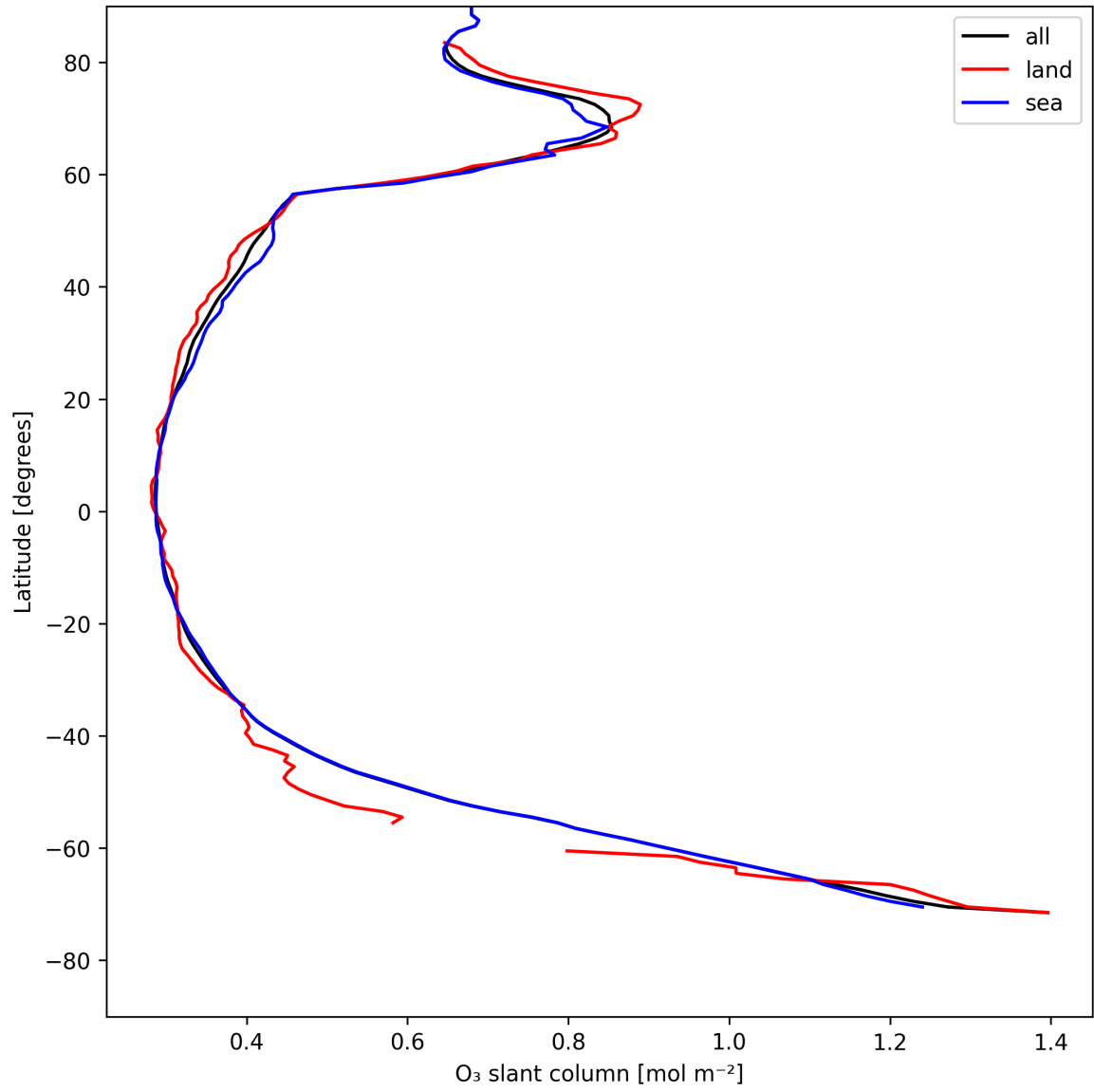
Figure 19: Zonal average of “O 3 slant column” for 2025-05-10 to 2025-05-11.
