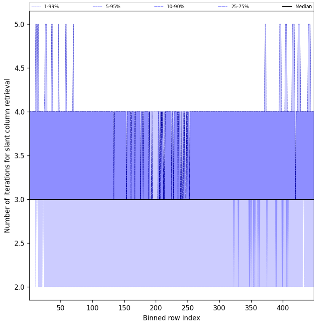
Figure 45: Along track statistics of “Number of iterations for slant column retrieval” for 2025-05-10 to 2025-05-11
