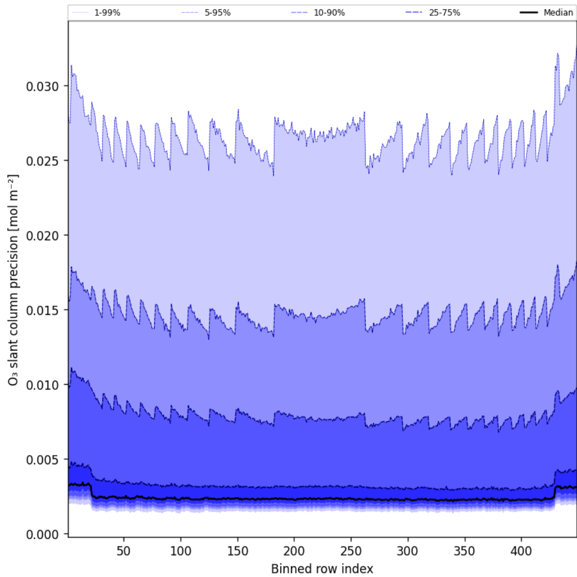
Figure 44: Along track statistics of “O 3 slant column precision” for 2025-05-10 to 2025-05-11
