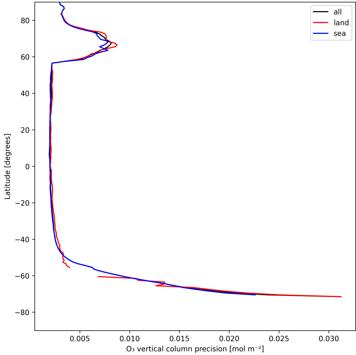
Figure 18: Zonal average of “O 3 vertical column precision” for 2025-05-10 to 2025-05-11.
