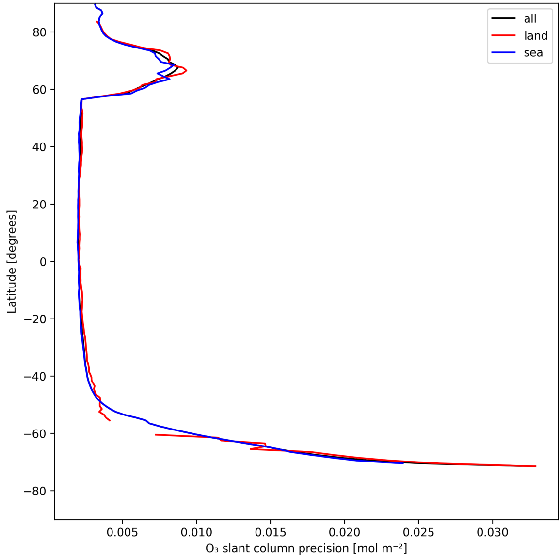
Figure 20: Zonal average of "O 3 slant column precision" for 2025-05-10 to 2025-05-11.
