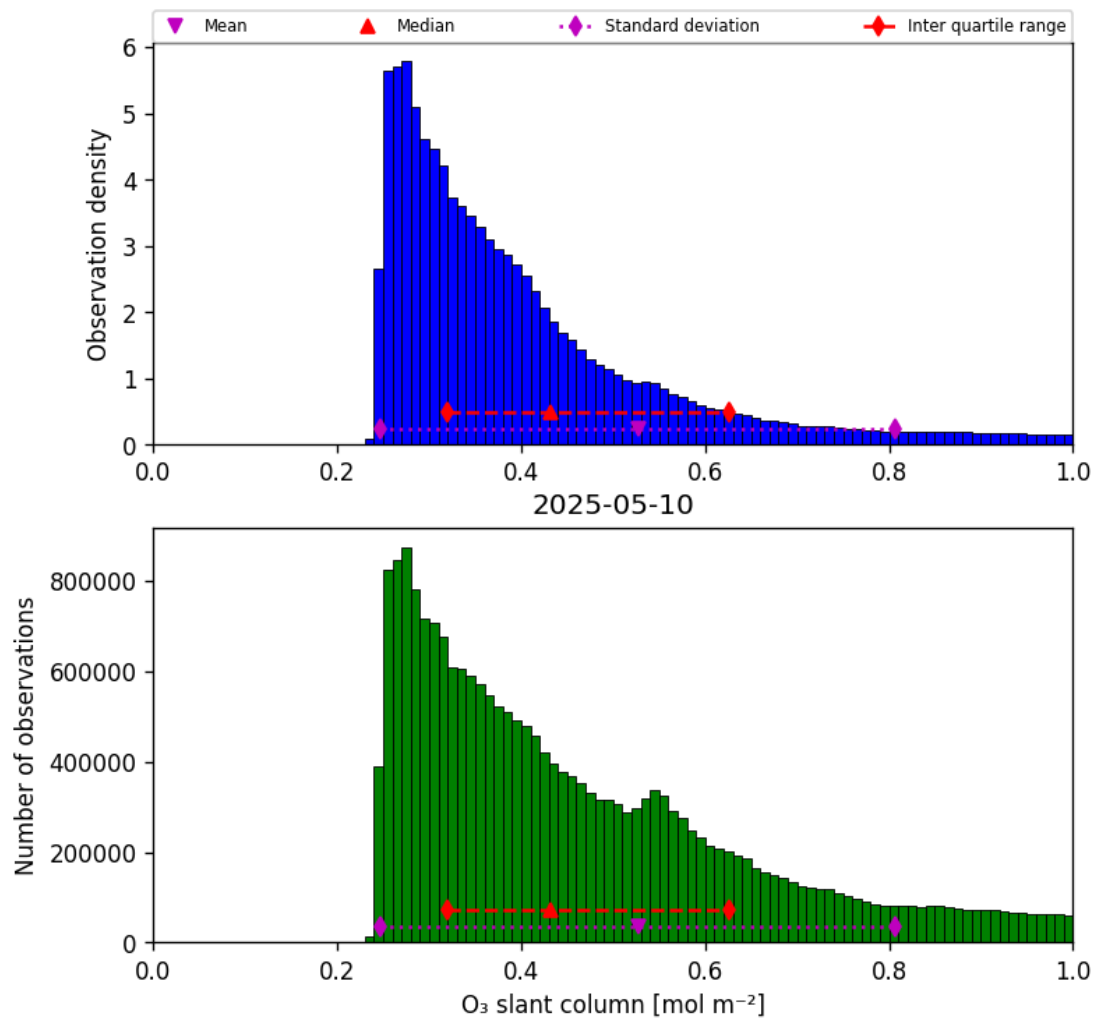
Figure 31: Histogram of “O 3 slant column” for 2025-05-10 to 2025-05-11
