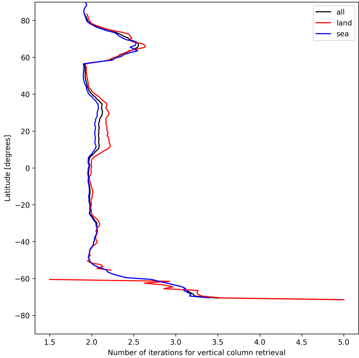
Figure 27: Zonal average of “Number of iterations for vertical column retrieval” for 2025-05-10 to 2025-05-11.
