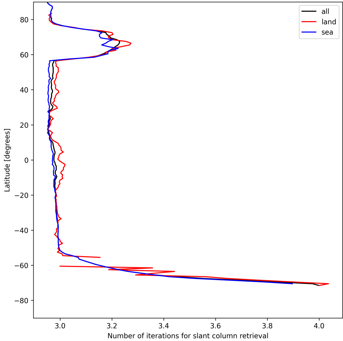
Figure 21: Zonal average of “Number of iterations for slant column retrieval” for 2025-05-10 to 2025-05-11.
