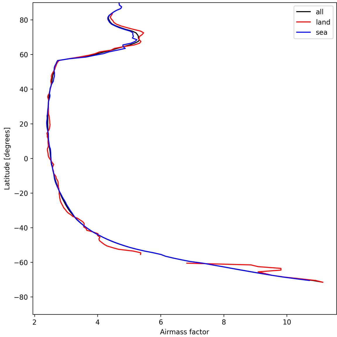
Figure 25: Zonal average of “Airmass factor” for 2025-05-10 to 2025-05-11.
