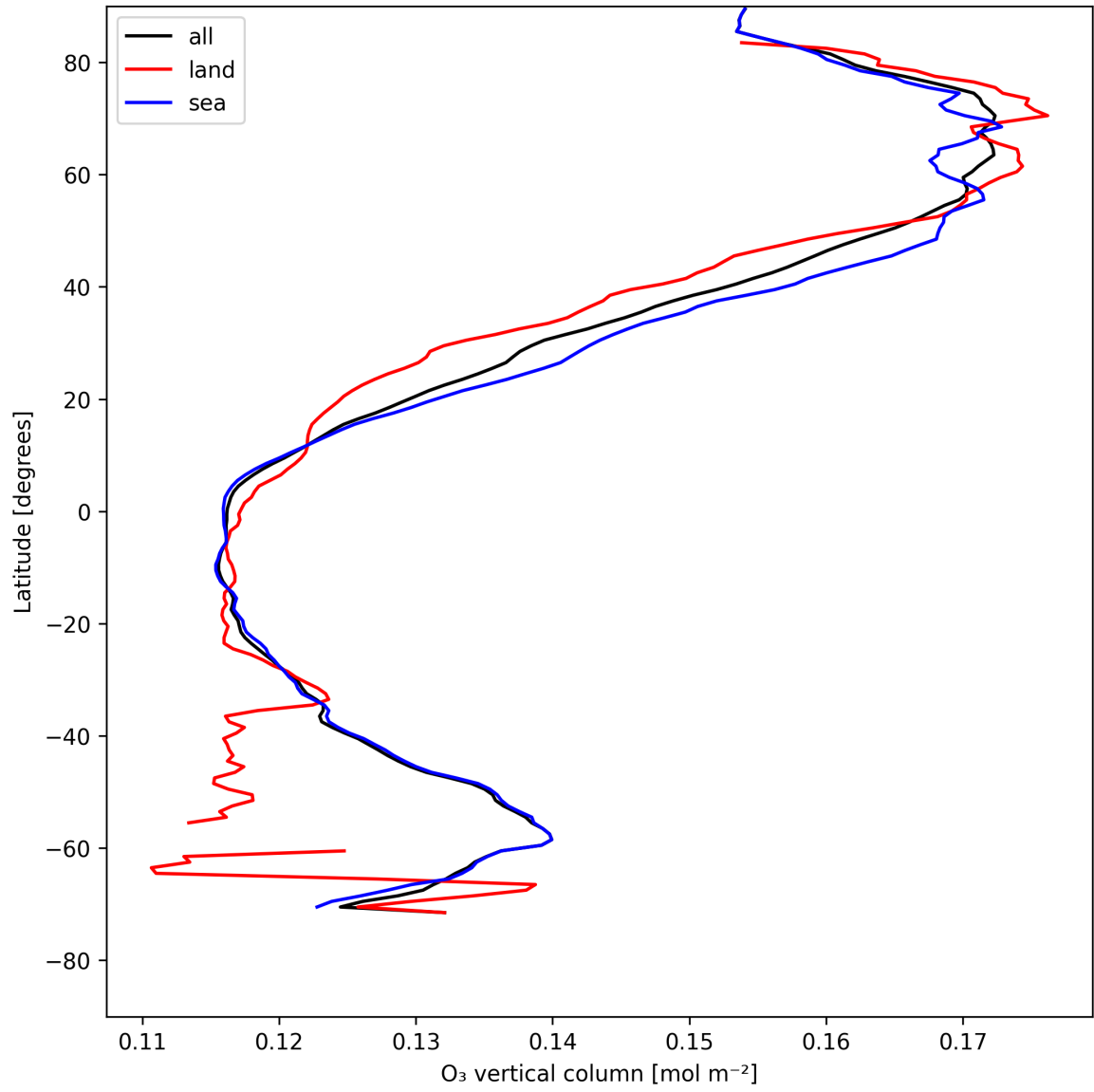
Figure 17: Zonal average of “O 3 vertical column” for 2025-05-10 to 2025-05-11.
