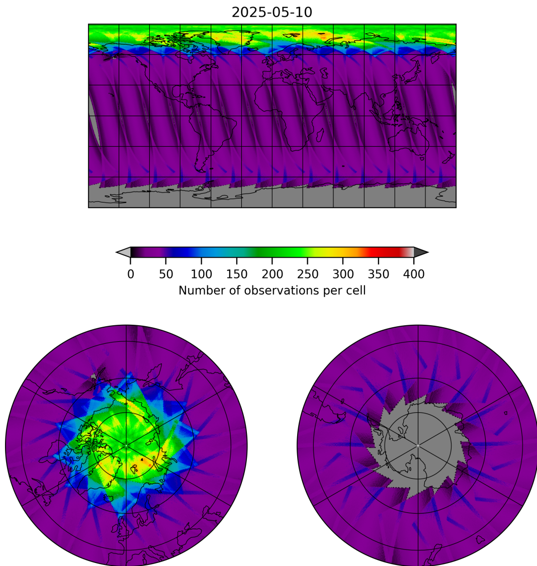
Figure 15: Map of the number of observations for 2025-05-10 to 2025-05-11
