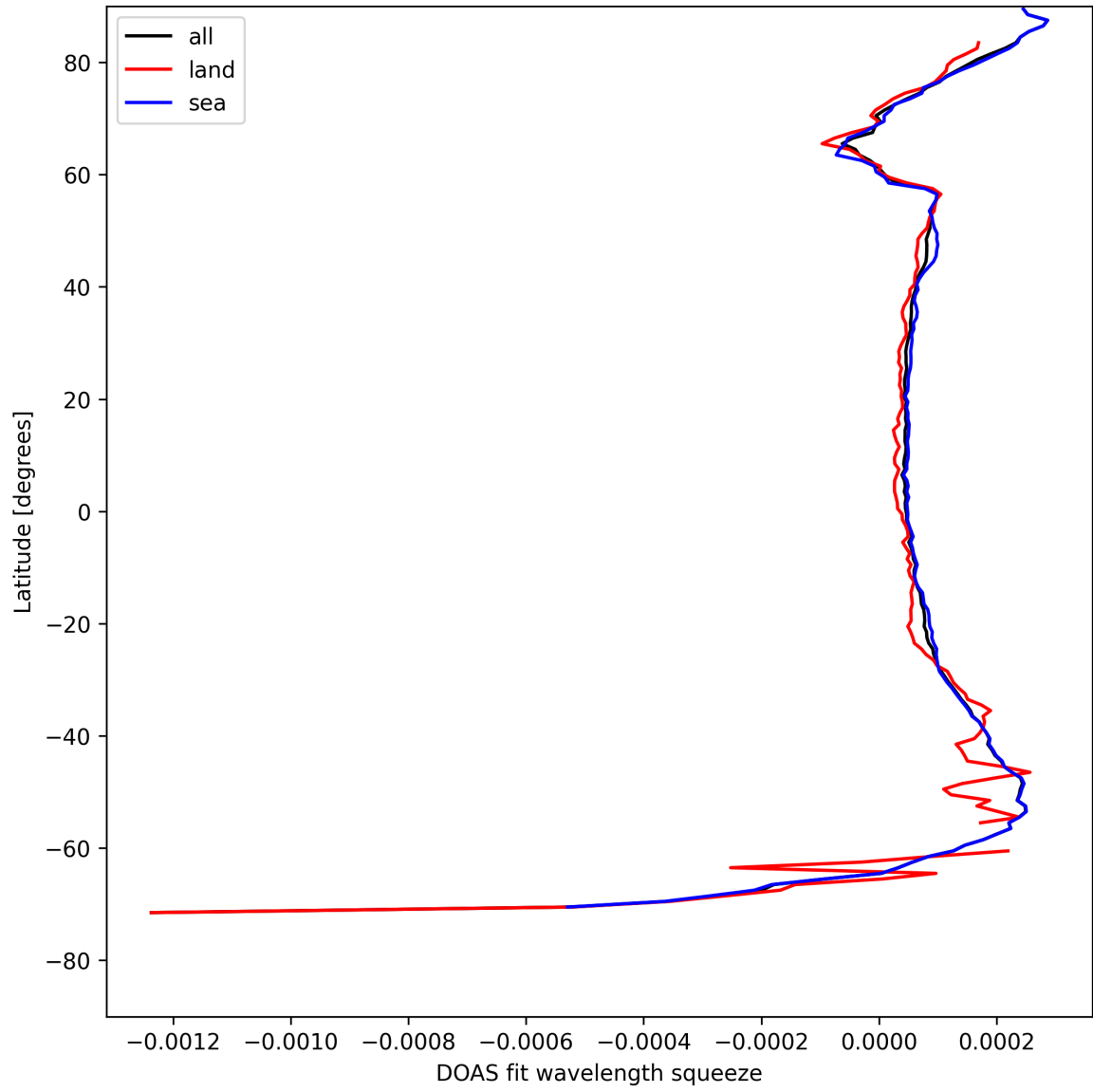
Figure 24: Zonal average of “DOAS fit wavelength squeeze” for 2025-05-10 to 2025-05-11.
