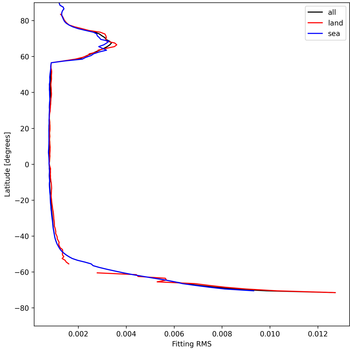
Figure 22: Zonal average of “Fitting RMS” for 2025-05-10 to 2025-05-11.
