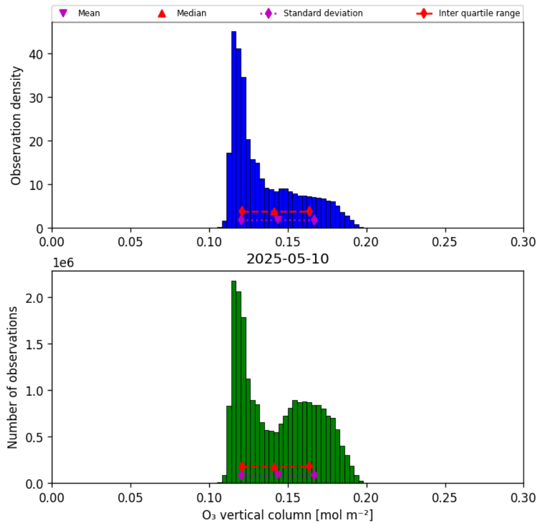
Figure 29: Histogram of “O 3 vertical column” for 2025-05-10 to 2025-05-11
