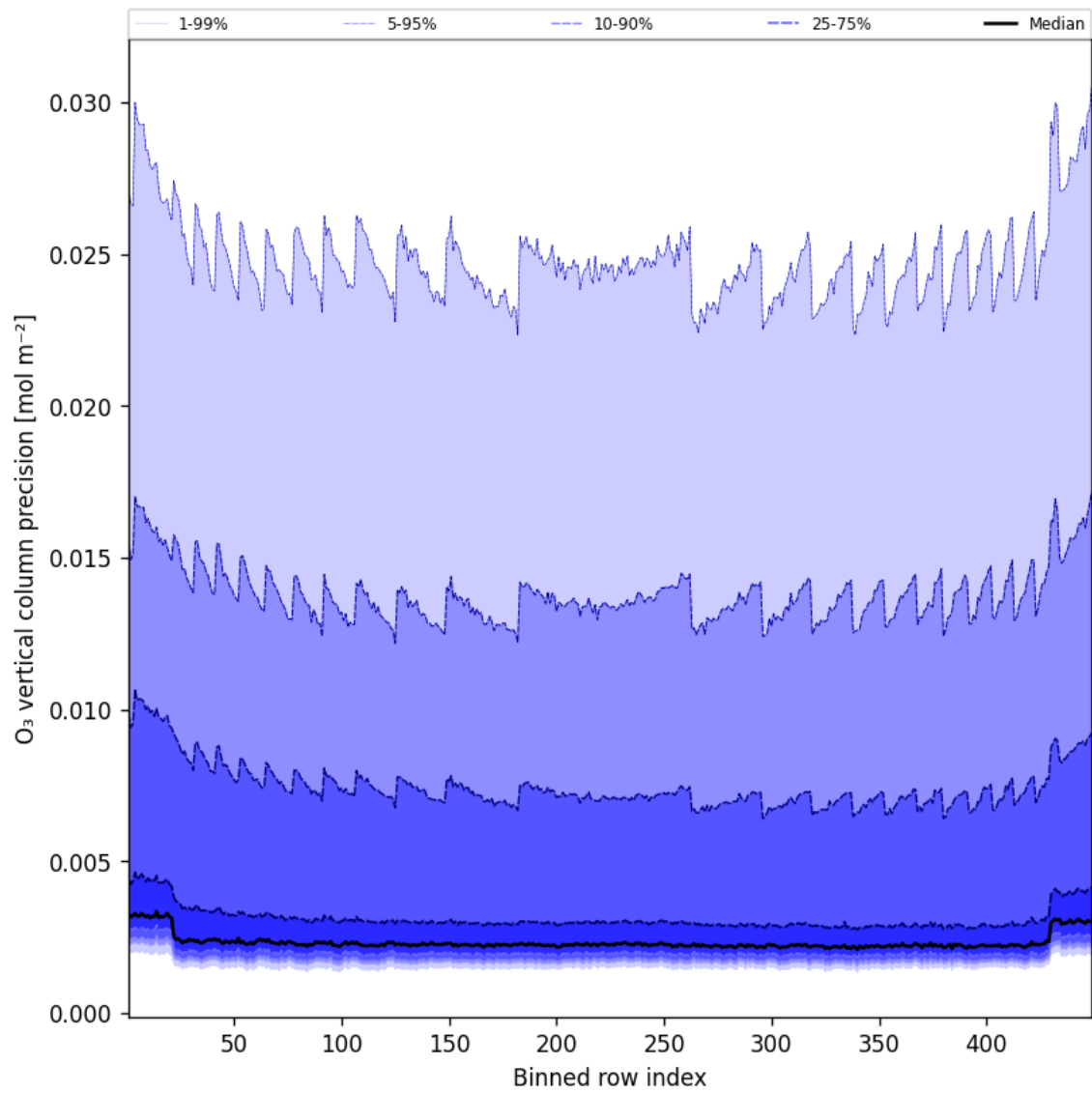
Figure 42: Along track statistics of “O 3 vertical column precision” for 2025-05-10 to 2025-05-11
