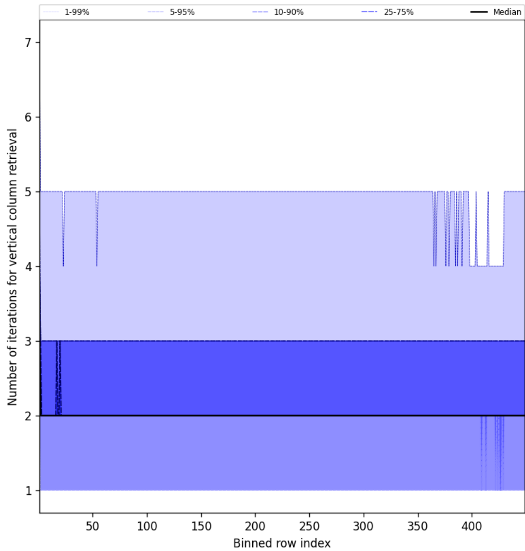
Figure 51: Along track statistics of “Number of iterations for vertical column retrieval” for 2025-05-10 to 2025-05-11
