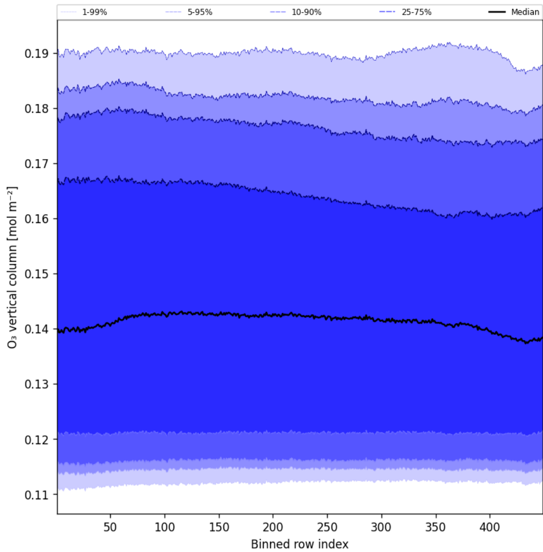
Figure 41: Along track statistics of “O 3 vertical column” for 2025-05-10 to 2025-05-11
