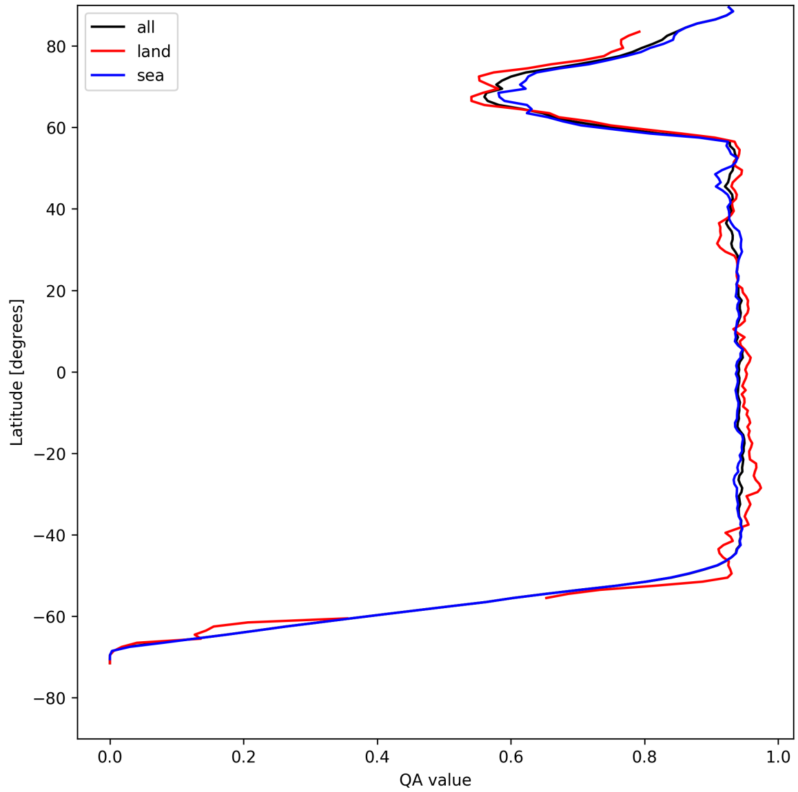
Figure 16: Zonal average of “QA value” for 2025-05-10 to 2025-05-11.
