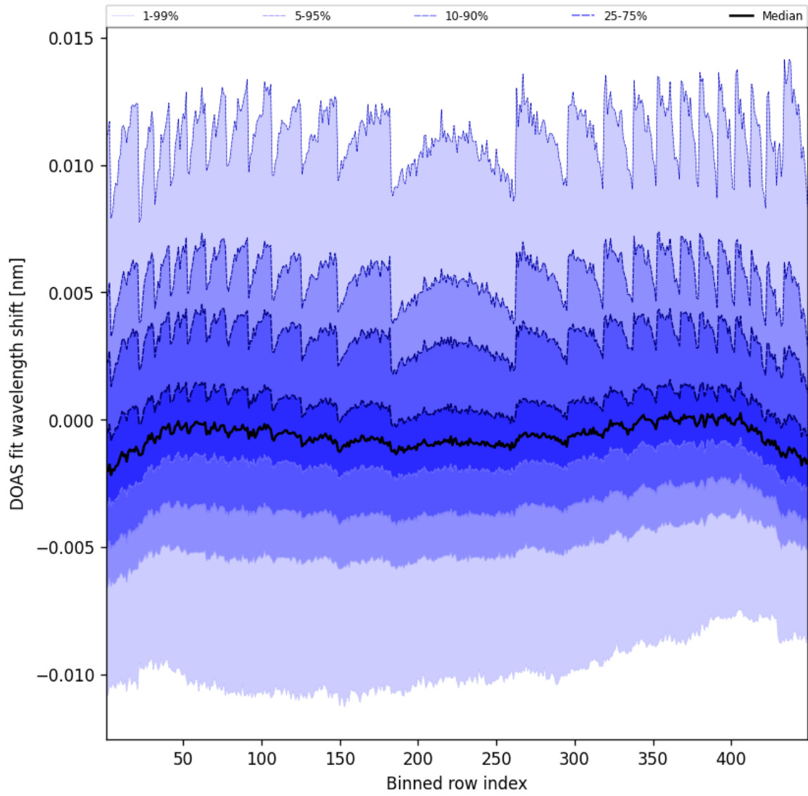
Figure 47: Along track statistics of “DOAS fit wavelength shift” for 2025-05-10 to 2025-05-11
