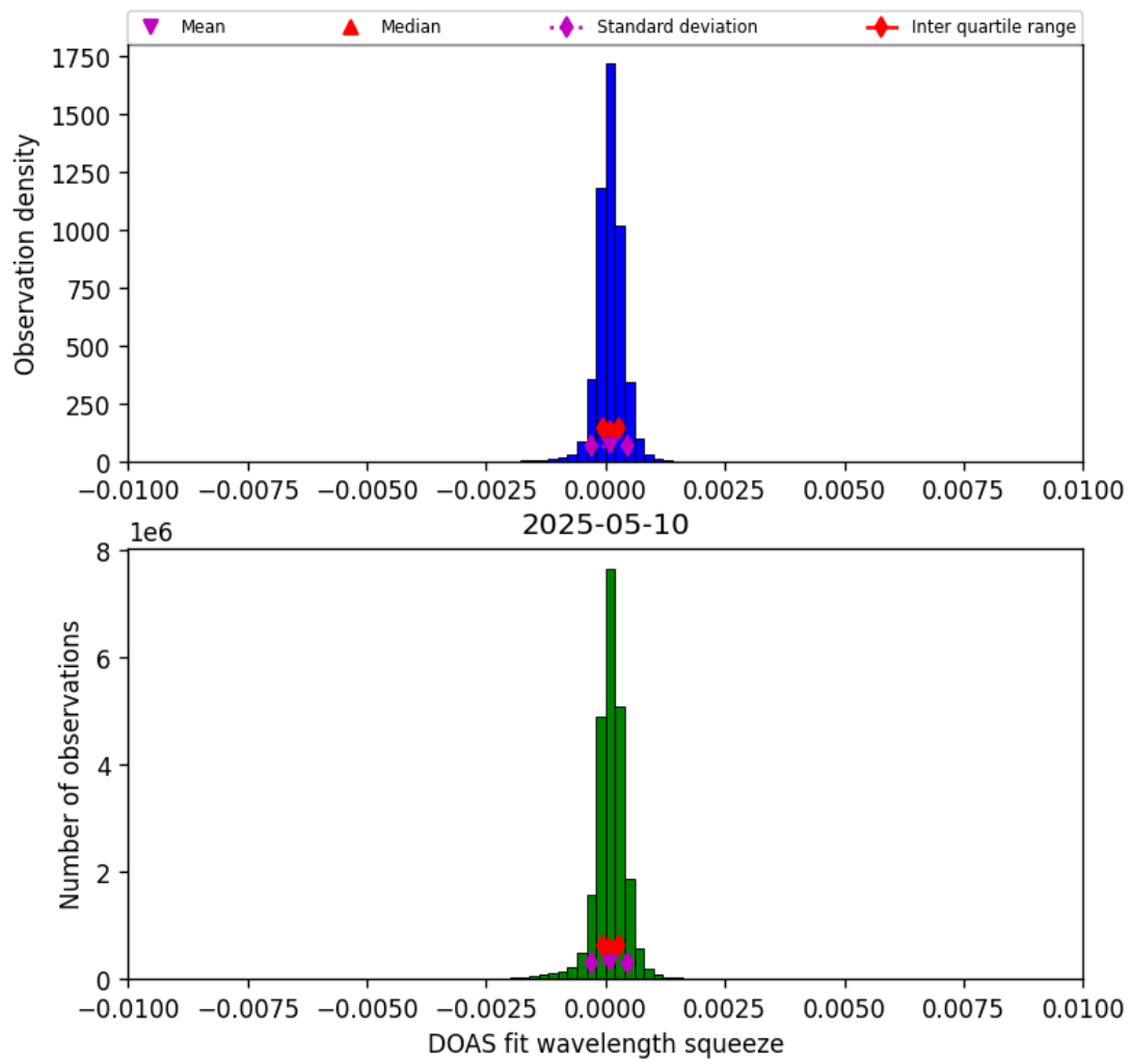
Figure 36: Histogram of “DOAS fit wavelength squeeze” for 2025-05-10 to 2025-05-11
