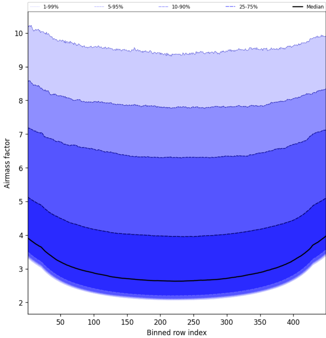
Figure 49: Along track statistics of “Airmass factor” for 2025-05-10 to 2025-05-11
