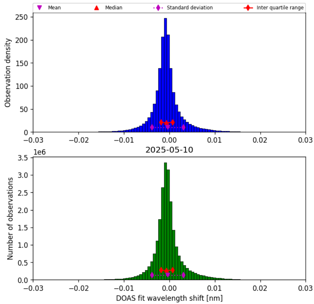
Figure 35: Histogram of “DOAS fit wavelength shift” for 2025-05-10 to 2025-05-11
