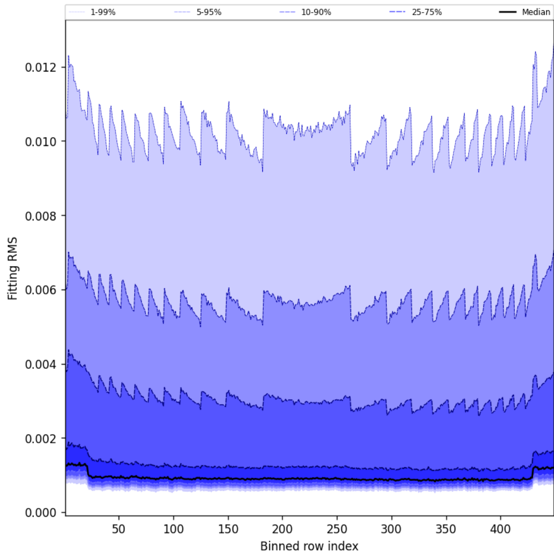
Figure 46: Along track statistics of “Fitting RMS” for 2025-05-10 to 2025-05-11
