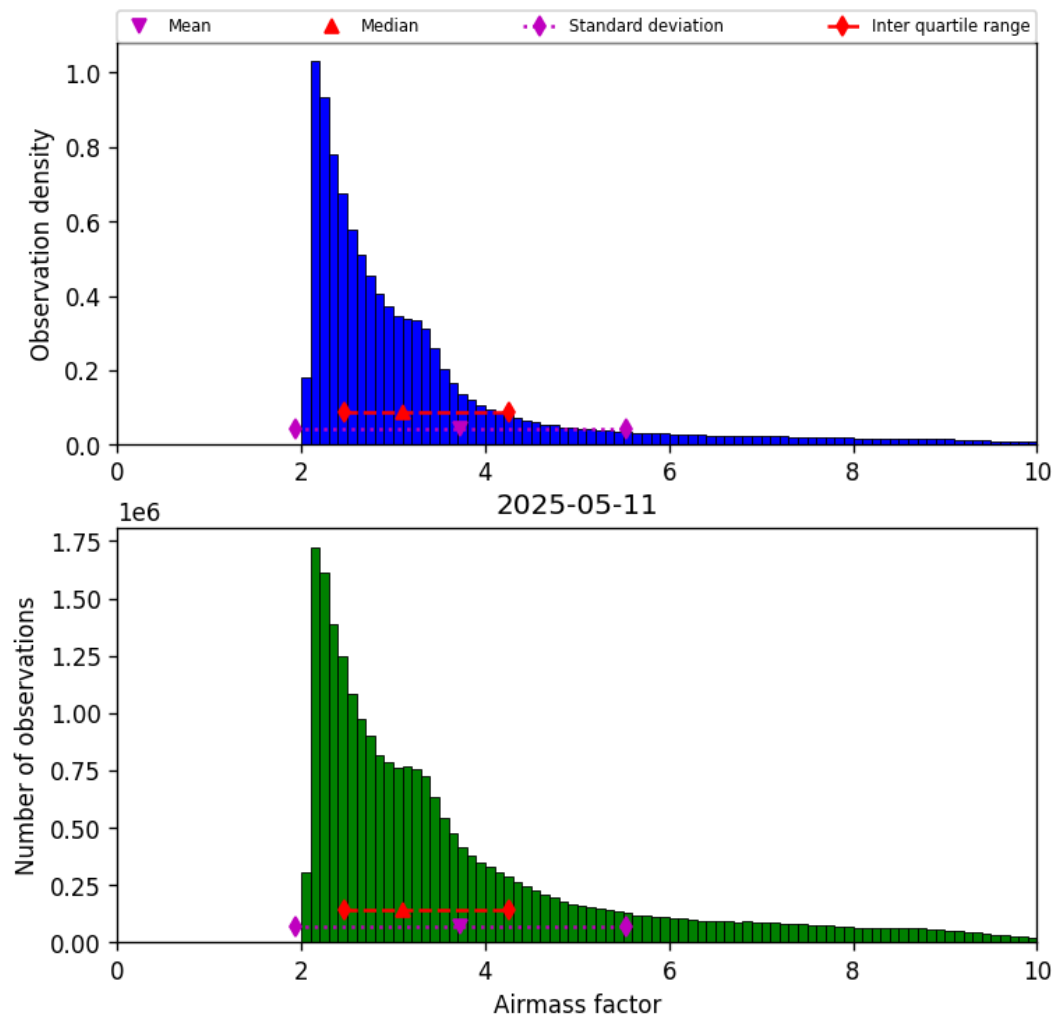
Figure 37: Histogram of “Airmass factor” for 2025-05-11 to 2025-05-12
