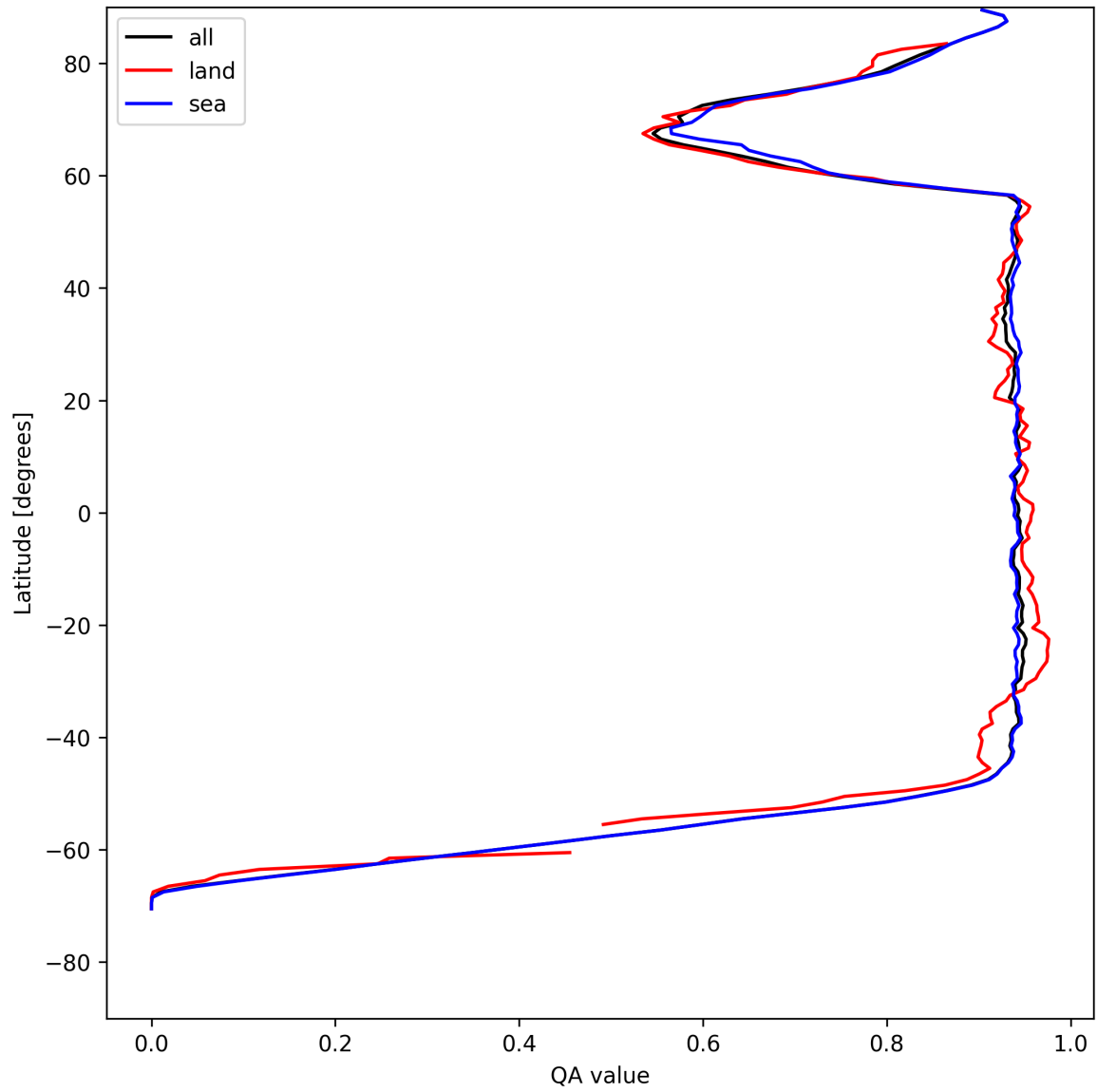
Figure 16: Zonal average of “QA value” for 2025-05-11 to 2025-05-12.
