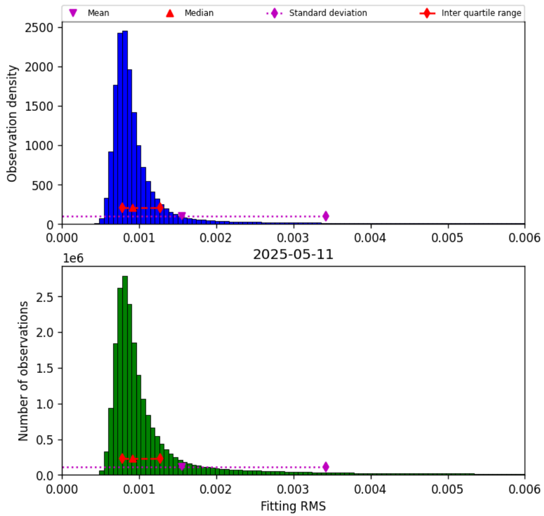
Figure 34: Histogram of “Fitting RMS” for 2025-05-11 to 2025-05-12
