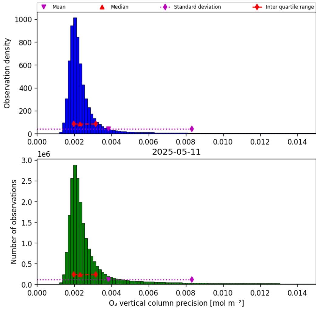
Figure 30: Histogram of “O 3 vertical column precision” for 2025-05-11 to 2025-05-12
