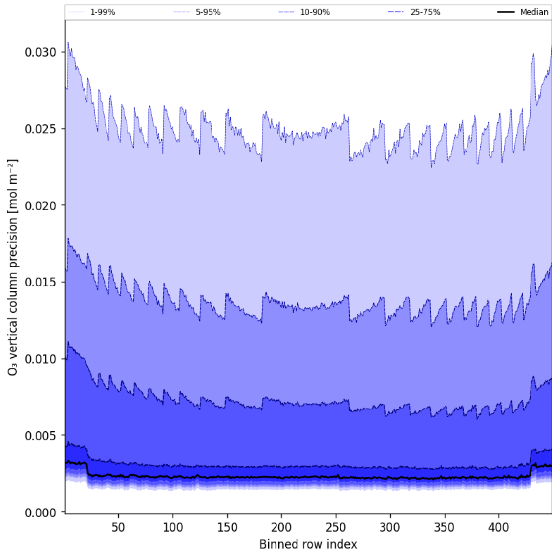
Figure 42: Along track statistics of “O 3 vertical column precision” for 2025-05-11 to 2025-05-12
