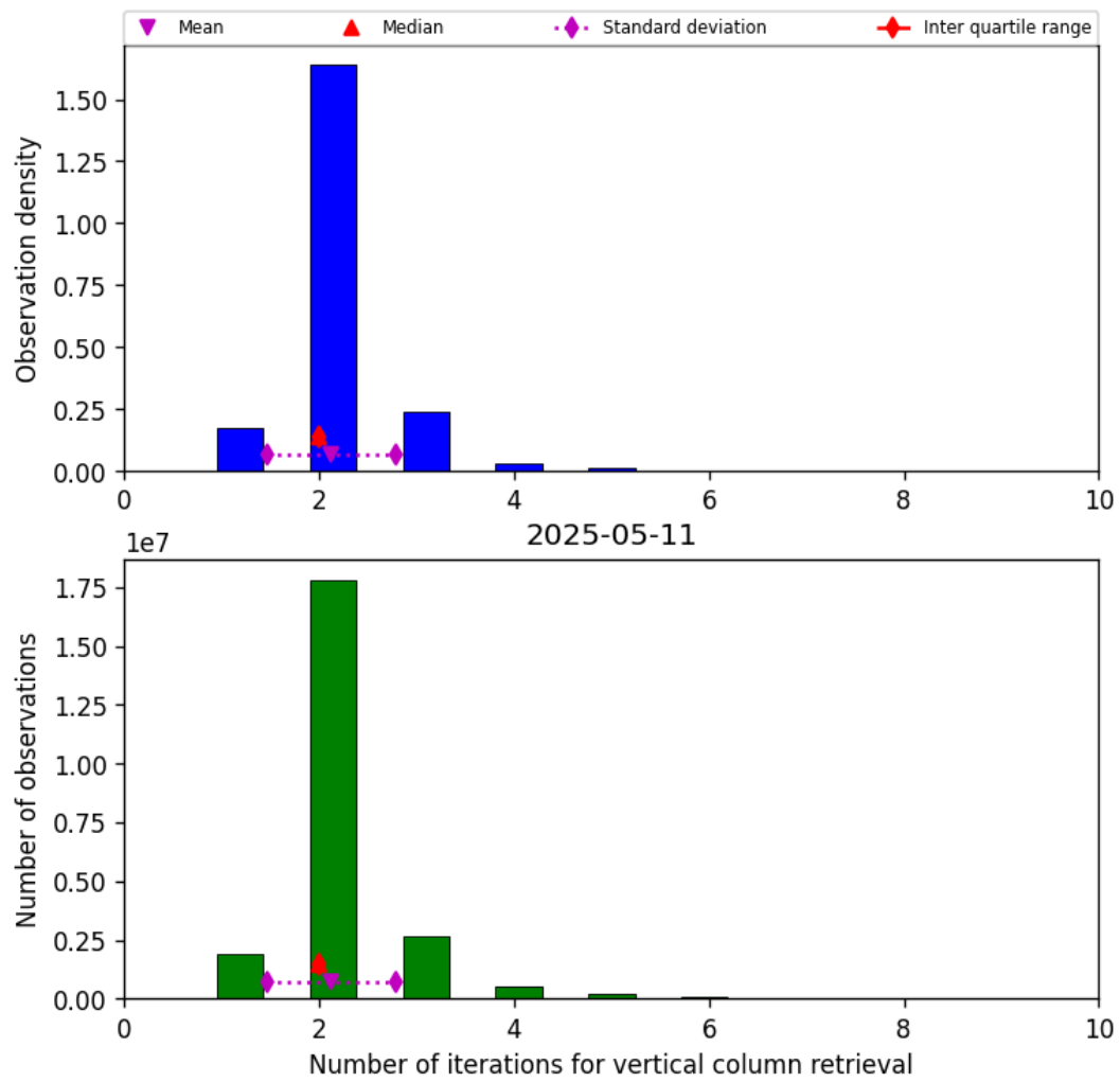
Figure 39: Histogram of “Number of iterations for vertical column retrieval” for 2025-05-11 to 2025-05-12
