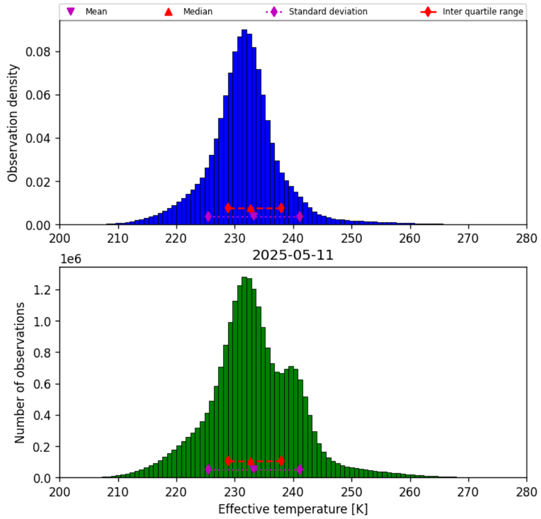
Figure 38: Histogram of “Effective temperature” for 2025-05-11 to 2025-05-12
