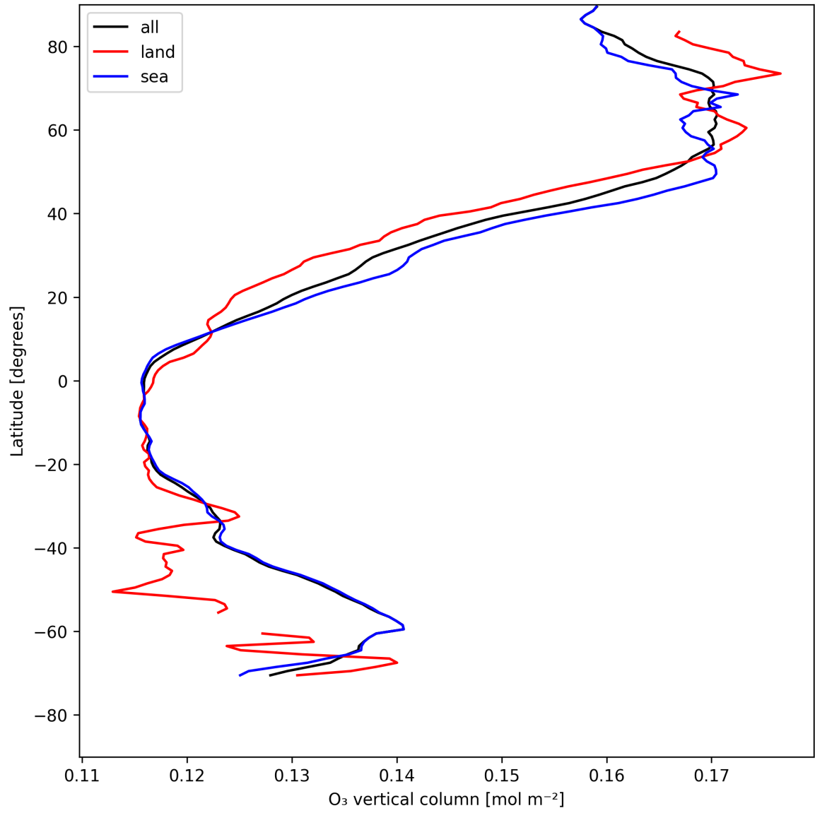
Figure 17: Zonal average of “O 3 vertical column” for 2025-05-11 to 2025-05-12.
