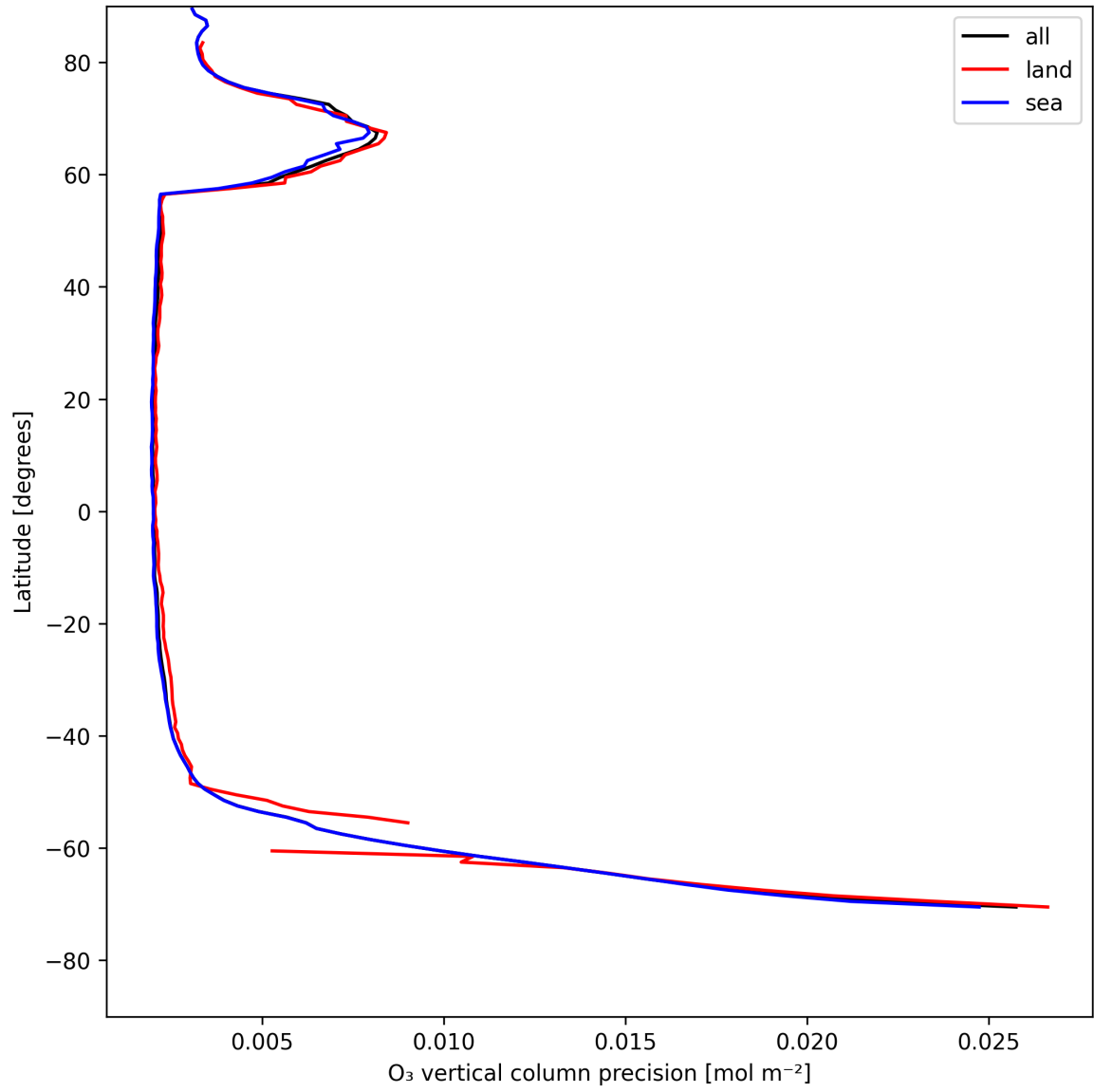
Figure 18: Zonal average of “O 3 vertical column precision” for 2025-05-11 to 2025-05-12.
