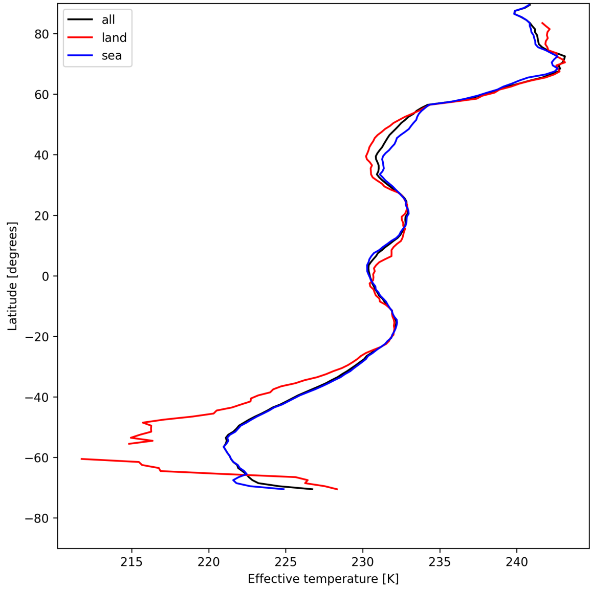
Figure 26: Zonal average of "Effective temperature" for 2025-05-11 to 2025-05-12.
