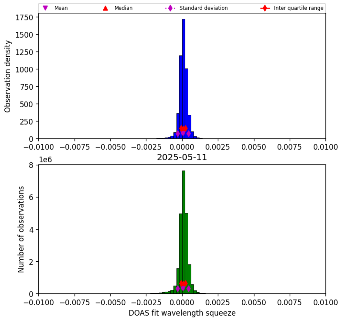
Figure 36: Histogram of “DOAS fit wavelength squeeze” for 2025-05-11 to 2025-05-12
