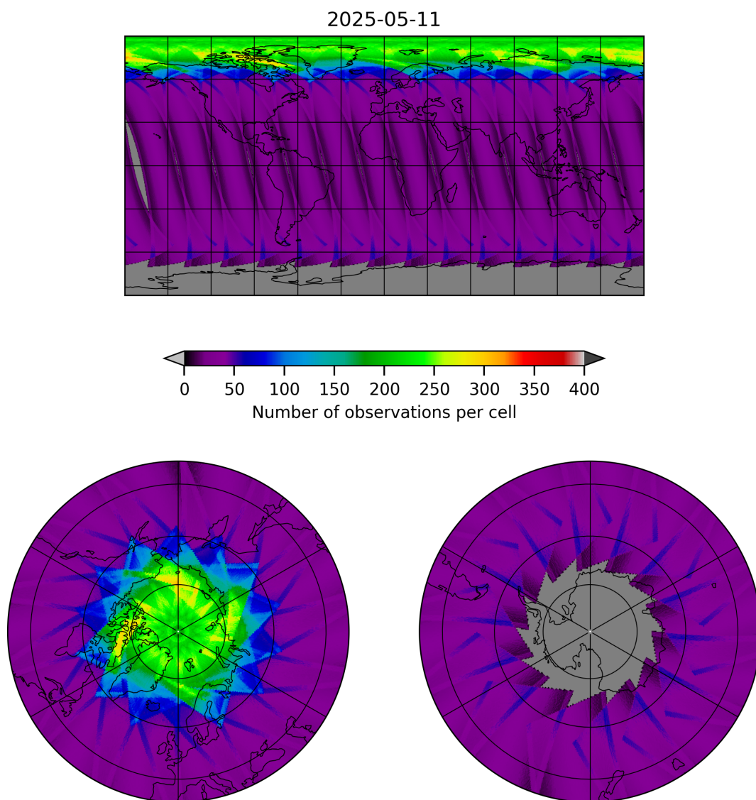
Figure 15: Map of the number of observations for 2025-05-11 to 2025-05-12
