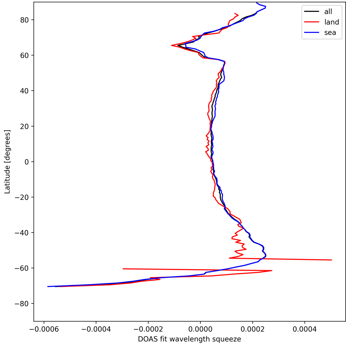
Figure 24: Zonal average of “DOAS fit wavelength squeeze” for 2025-05-11 to 2025-05-12.
