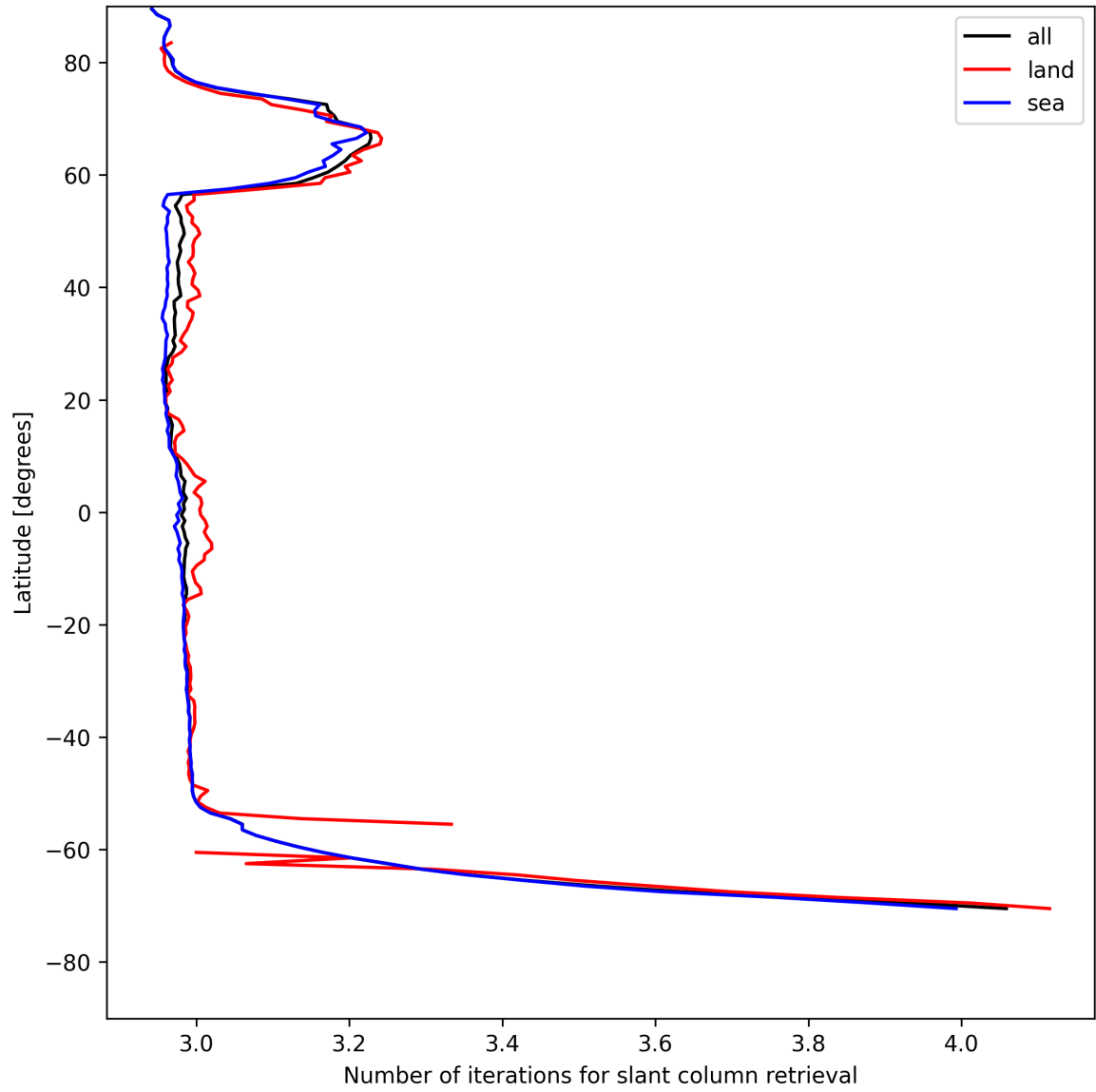
Figure 21: Zonal average of “Number of iterations for slant column retrieval” for 2025-05-11 to 2025-05-12.
