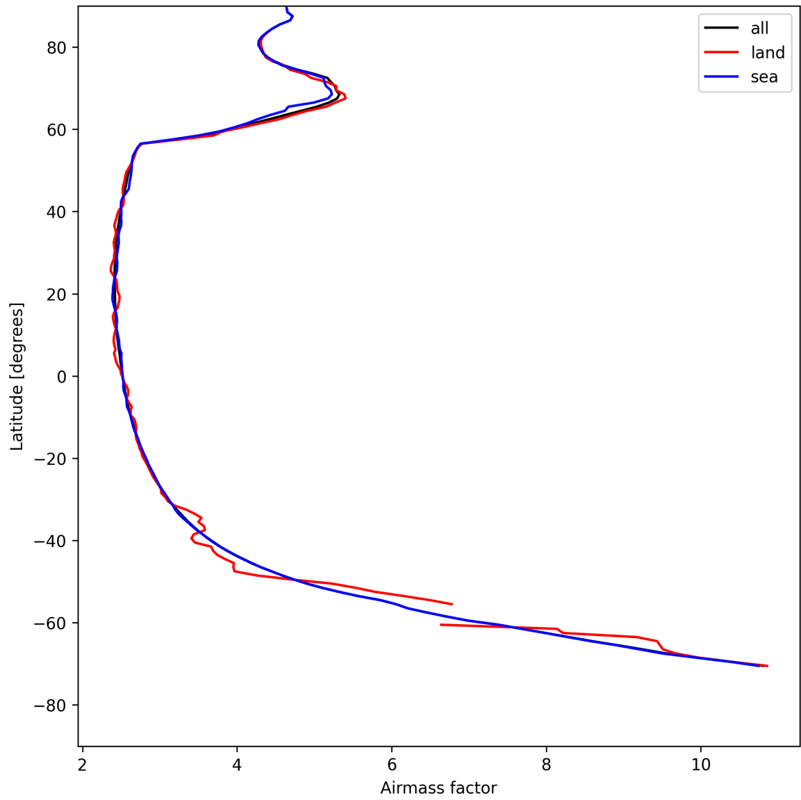
Figure 25: Zonal average of “Airmass factor” for 2025-05-11 to 2025-05-12.
