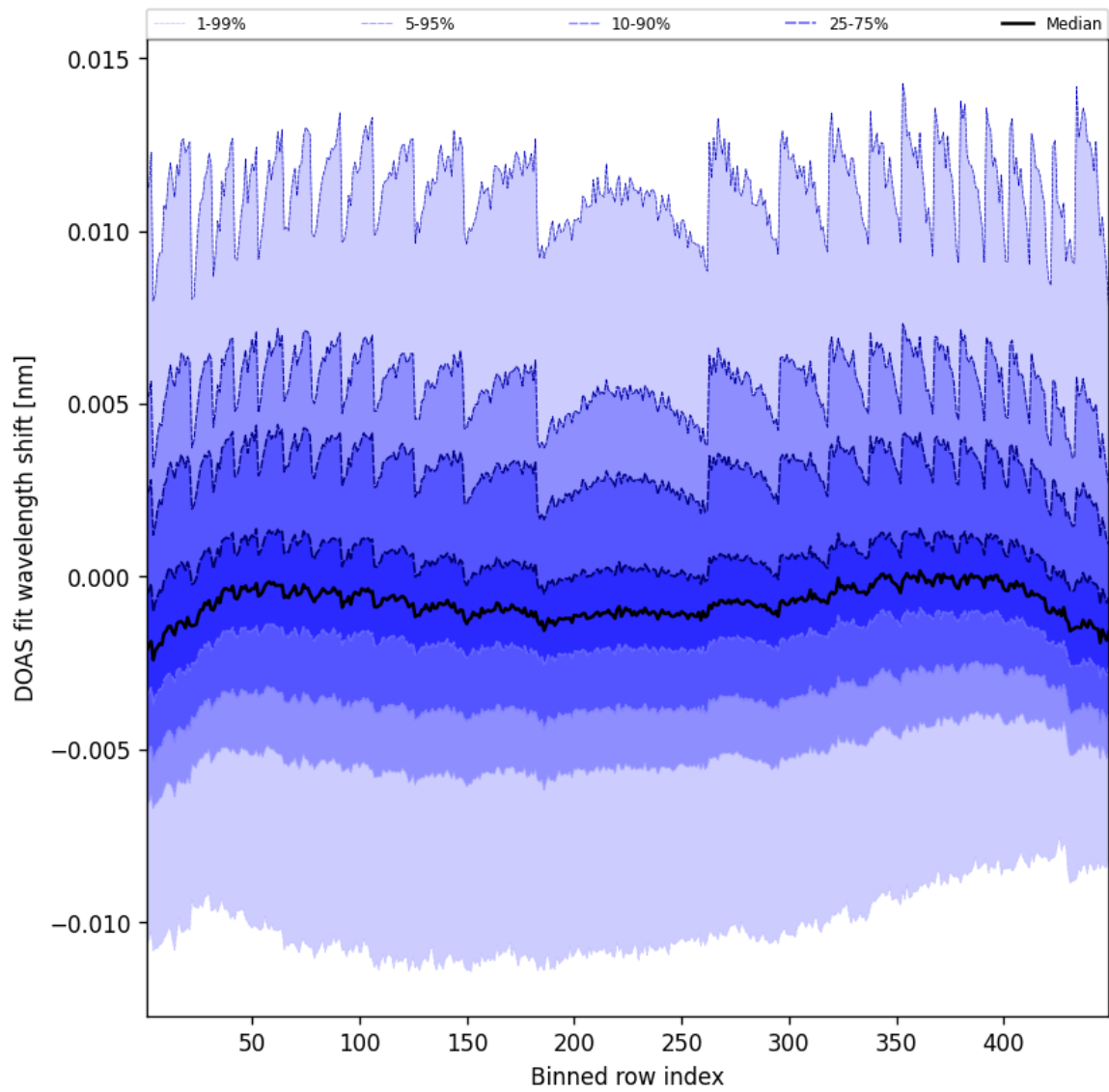
Figure 47: Along track statistics of “DOAS fit wavelength shift” for 2025-05-11 to 2025-05-12
