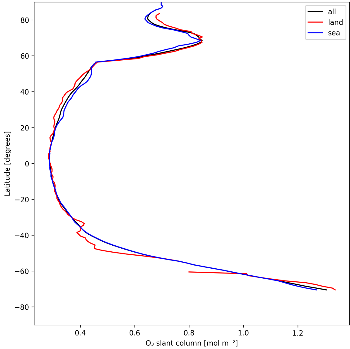
Figure 19: Zonal average of “O 3 slant column” for 2025-05-11 to 2025-05-12.
