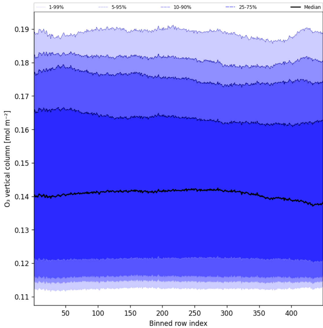
Figure 41: Along track statistics of “O 3 vertical column” for 2025-05-11 to 2025-05-12
