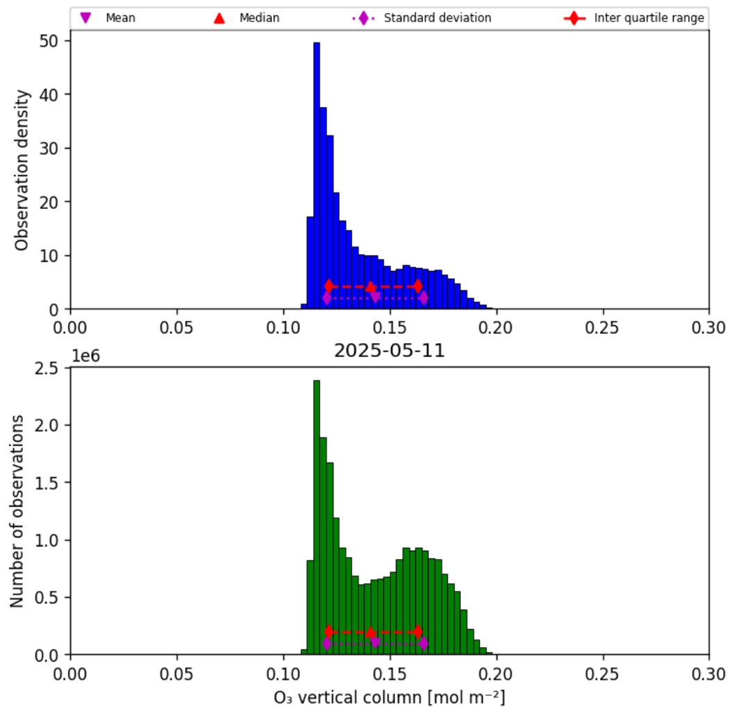
Figure 29: Histogram of “O 3 vertical column” for 2025-05-11 to 2025-05-12
