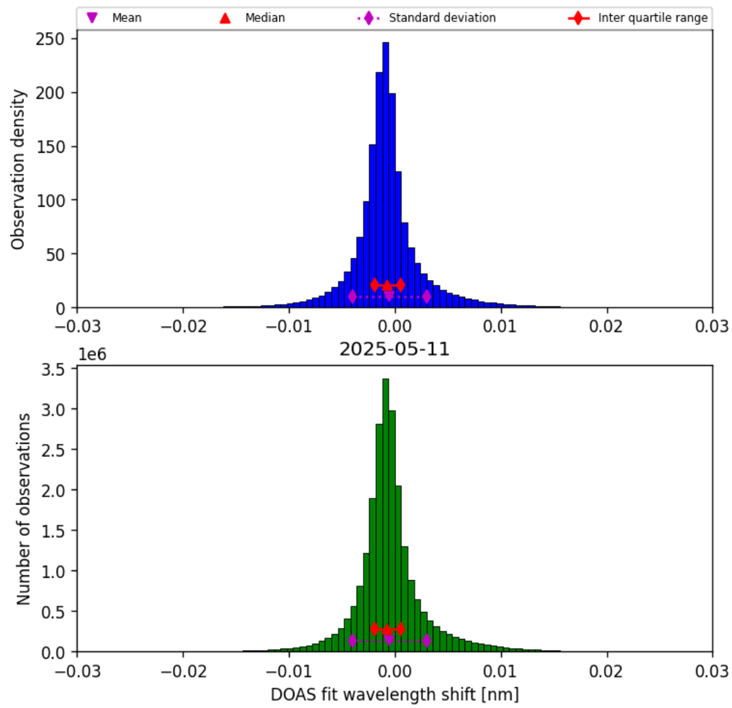
Figure 35: Histogram of “DOAS fit wavelength shift” for 2025-05-11 to 2025-05-12
