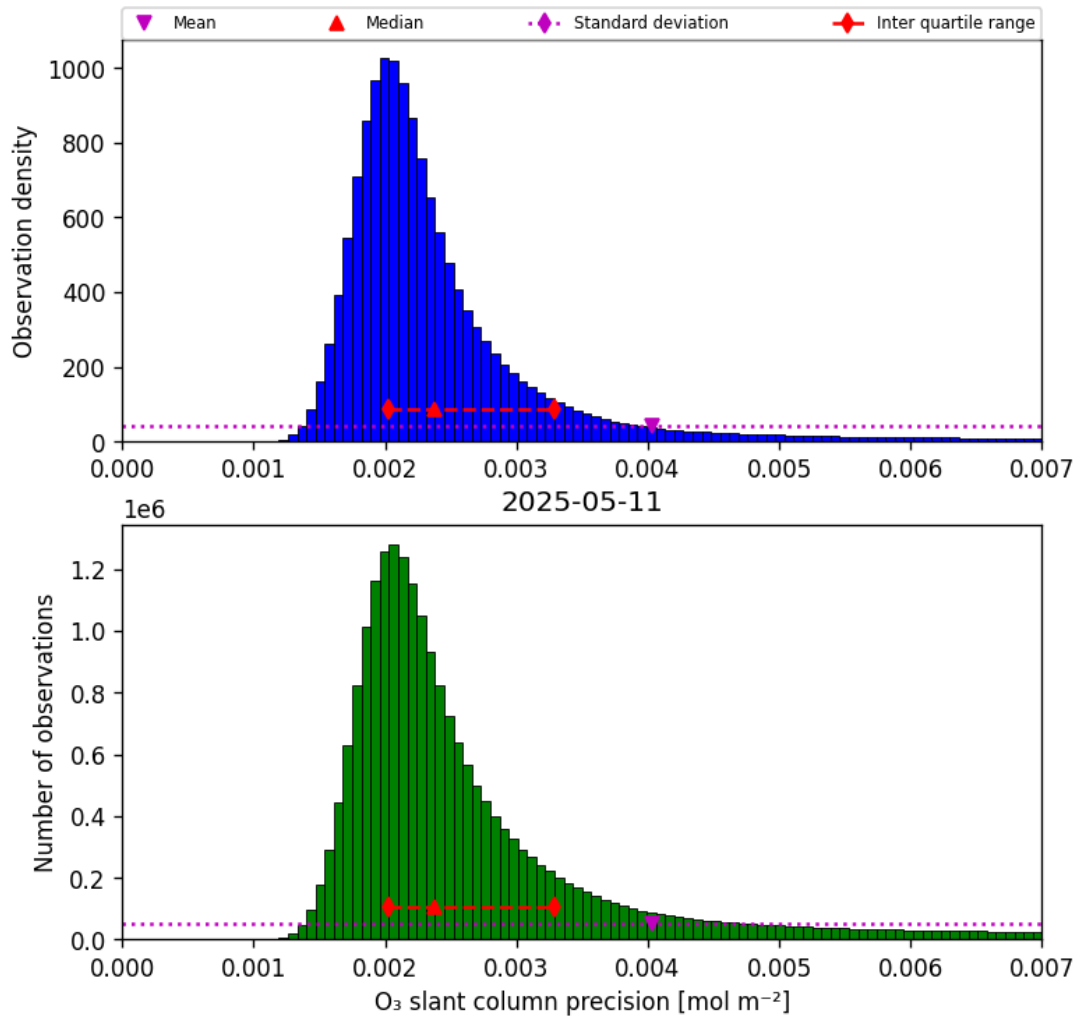
Figure 32: Histogram of “O 3 slant column precision” for 2025-05-11 to 2025-05-12
