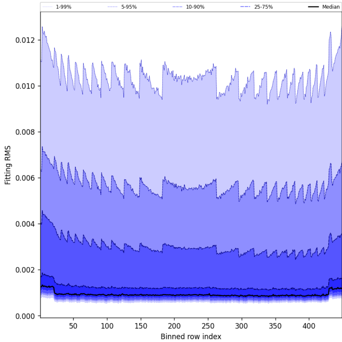
Figure 46: Along track statistics of “Fitting RMS” for 2025-05-11 to 2025-05-12
