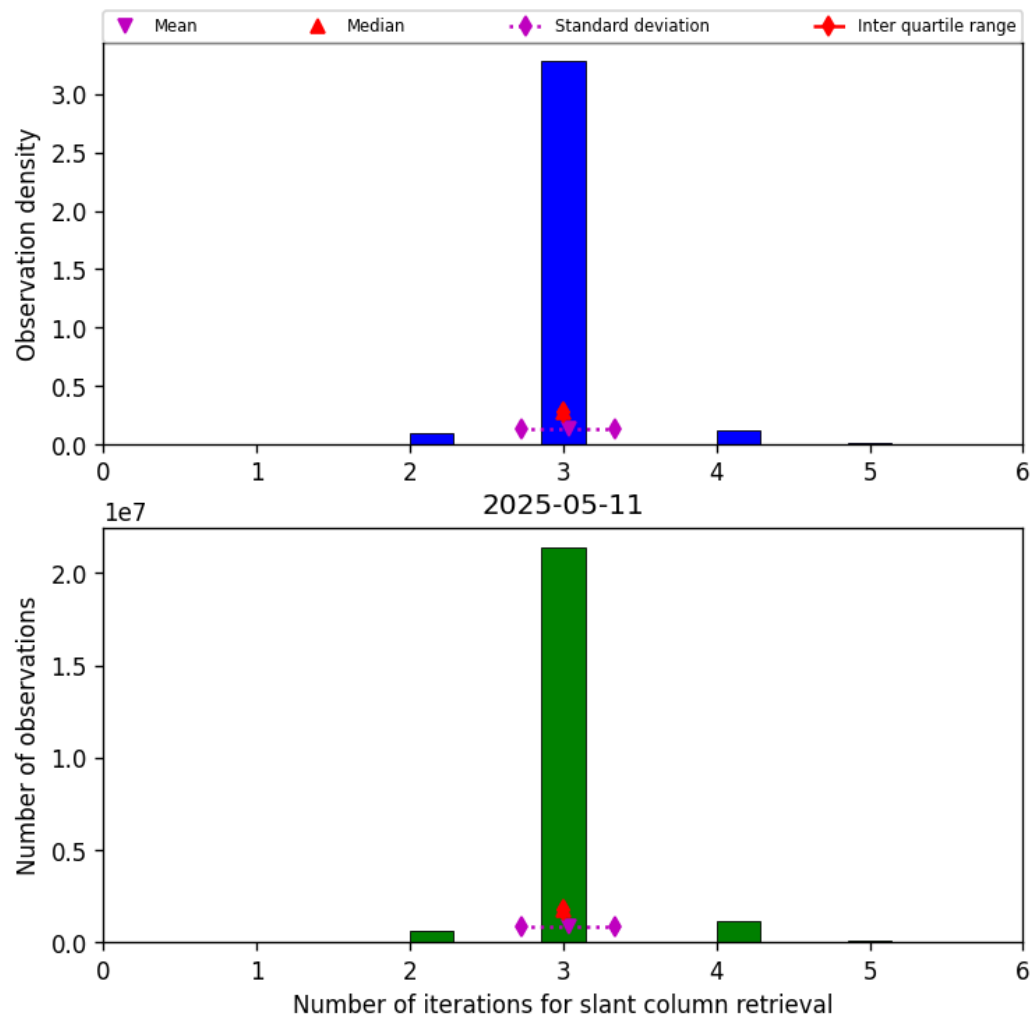
Figure 33: Histogram of “Number of iterations for slant column retrieval” for 2025-05-11 to 2025-05-12
