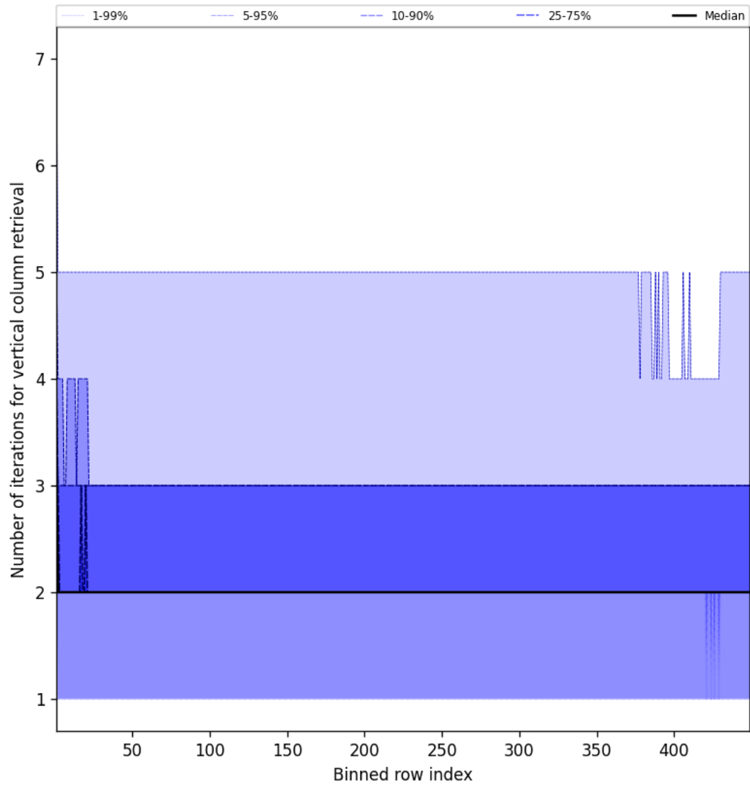
Figure 51: Along track statistics of “Number of iterations for vertical column retrieval” for 2025-05-11 to 2025-05-12
