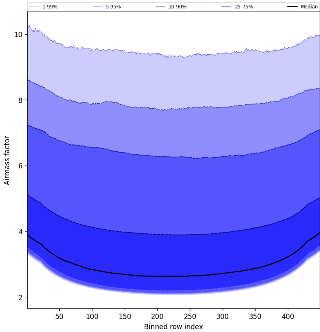
Figure 49: Along track statistics of “Airmass factor” for 2025-05-11 to 2025-05-12
