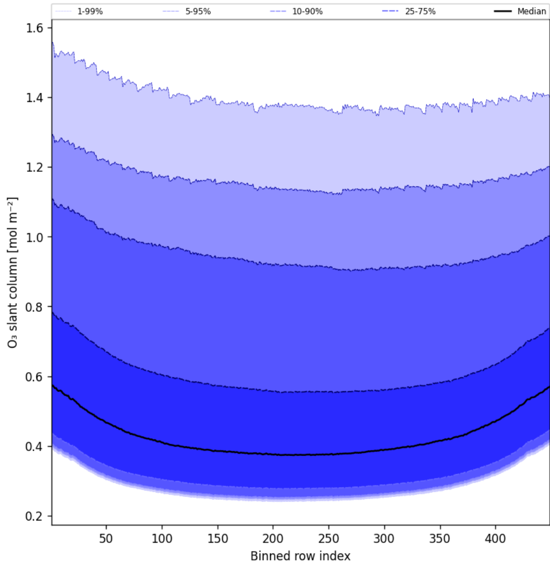
Figure 43: Along track statistics of “O 3 slant column” for 2025-05-11 to 2025-05-12
