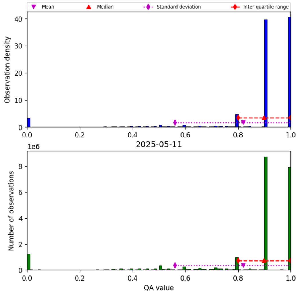
Figure 28: Histogram of “QA value” for 2025-05-11 to 2025-05-12
