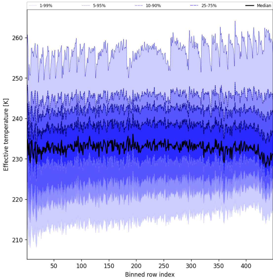
Figure 50: Along track statistics of “Effective temperature” for 2025-05-11 to 2025-05-12
