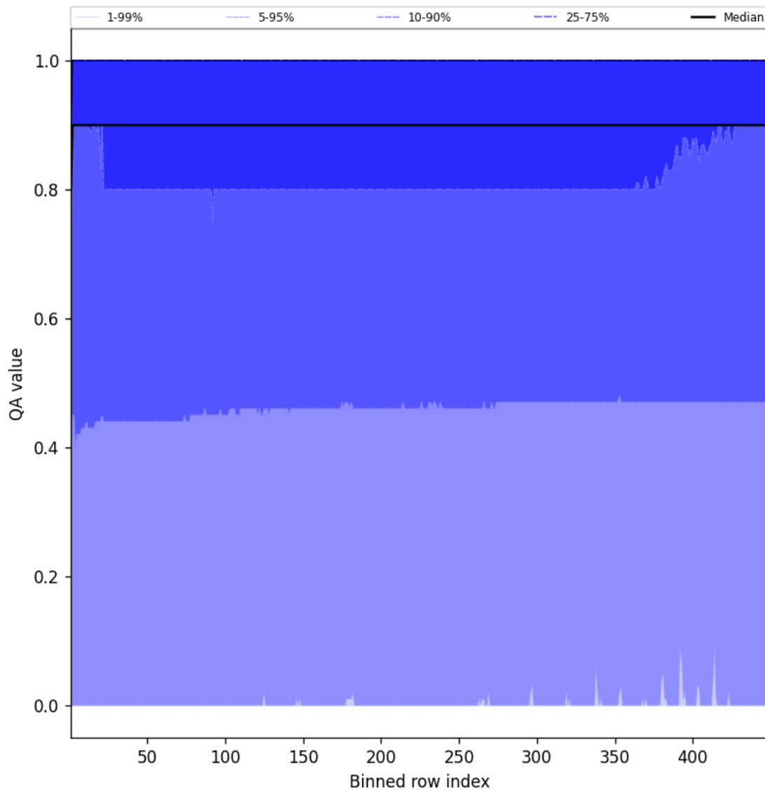
Figure 40: Along track statistics of “QA value” for 2025-05-11 to 2025-05-12
