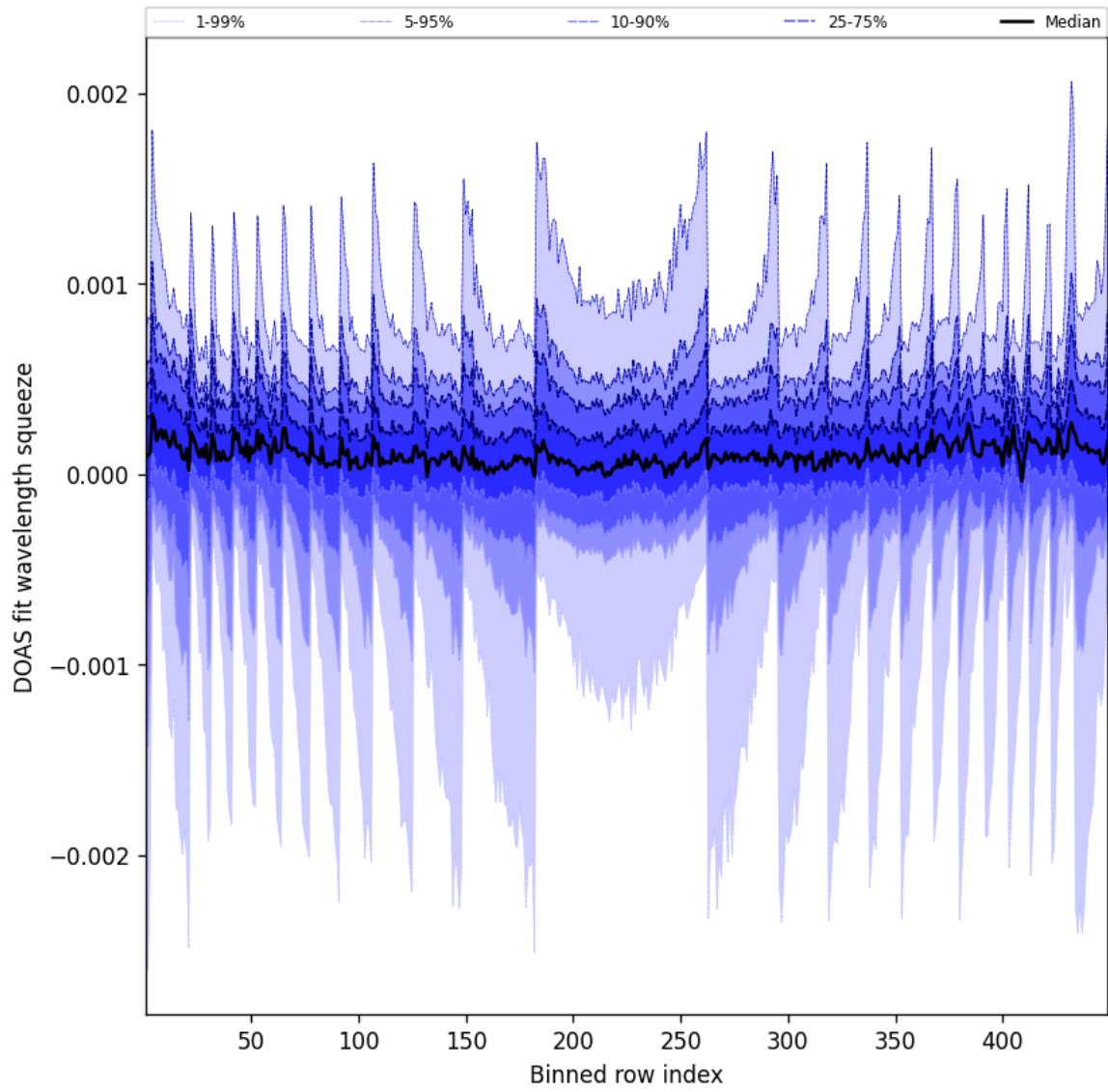
Figure 48: Along track statistics of “DOAS fit wavelength squeeze” for 2025-05-11 to 2025-05-12
