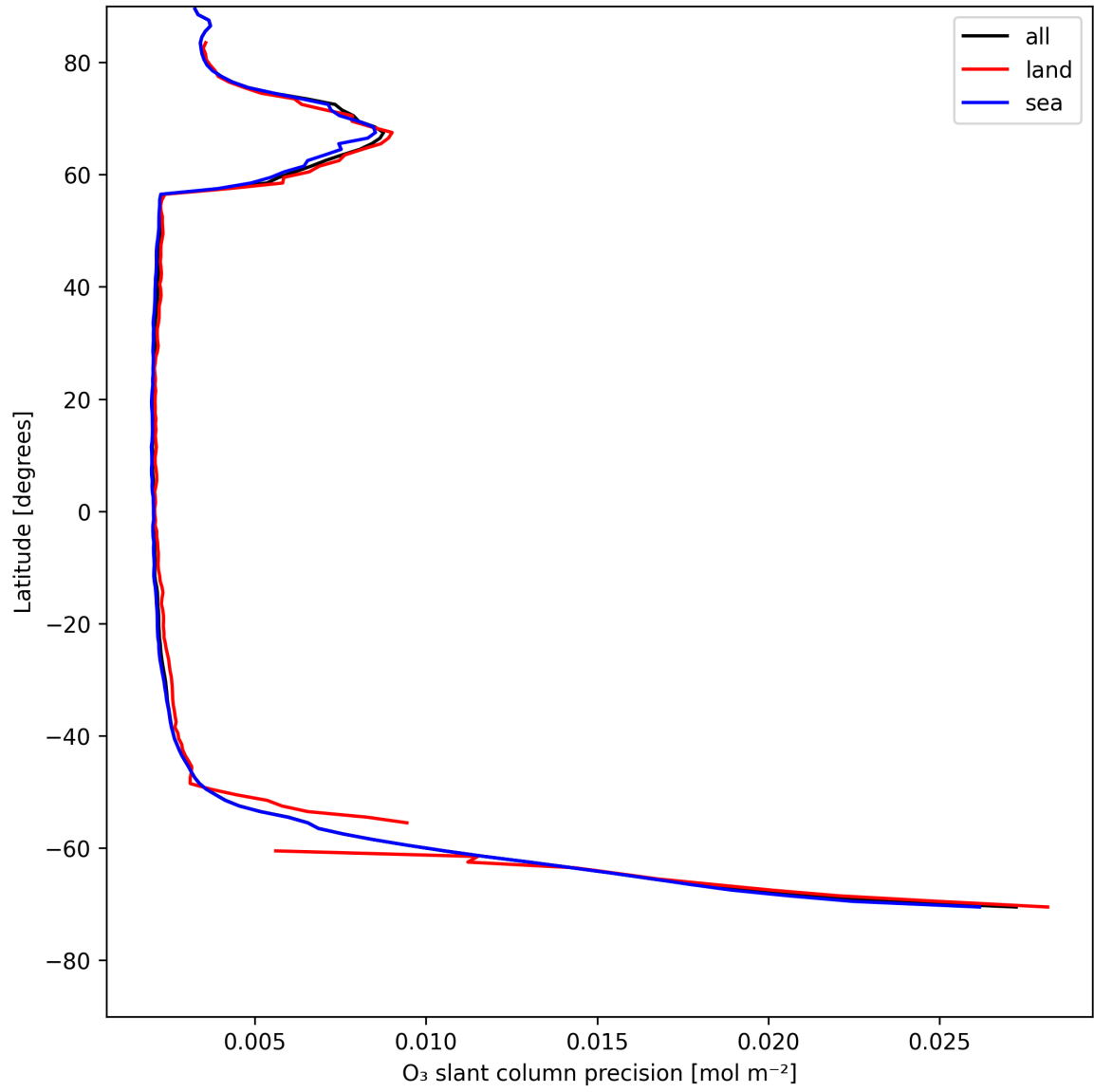
Figure 20: Zonal average of “O 3 slant column precision” for 2025-05-11 to 2025-05-12.
