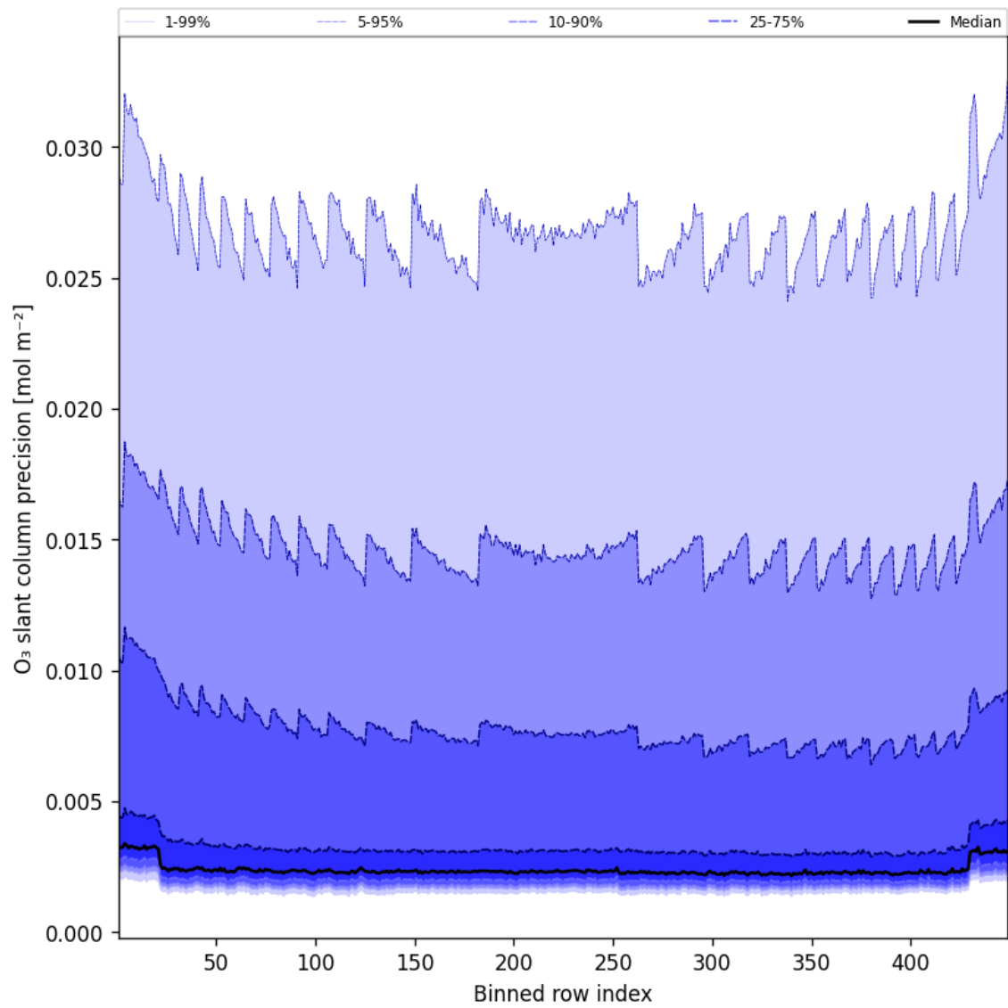
Figure 44: Along track statistics of “O 3 slant column precision” for 2025-05-11 to 2025-05-12
