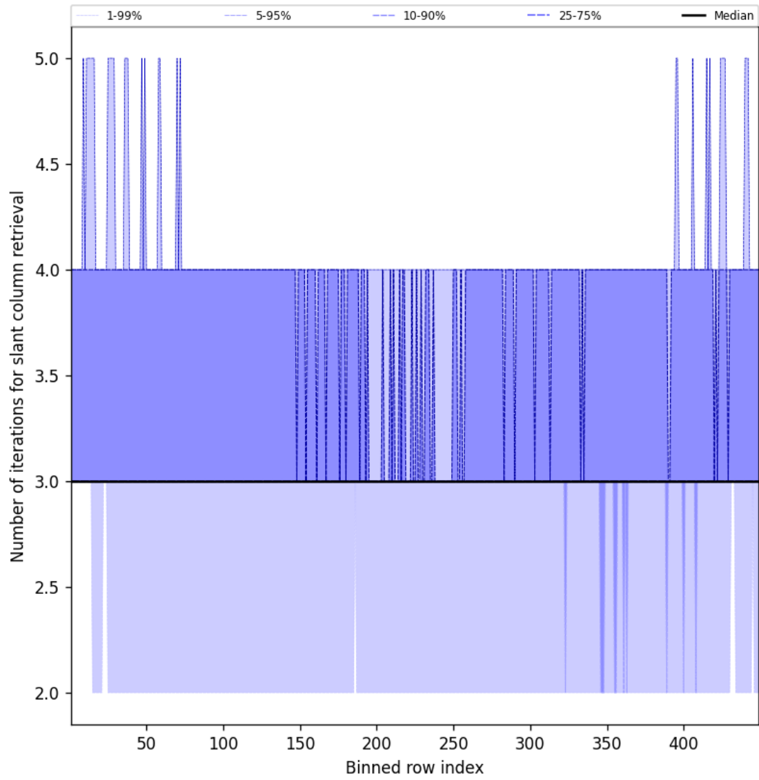
Figure 45: Along track statistics of “Number of iterations for slant column retrieval” for 2025-05-11 to 2025-05-12
