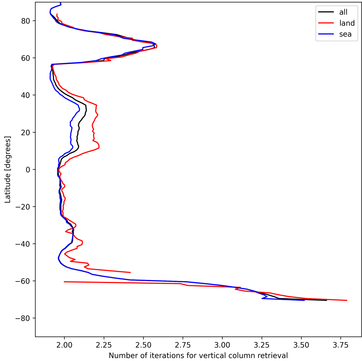
Figure 27: Zonal average of “Number of iterations for vertical column retrieval” for 2025-05-11 to 2025-05-12.
