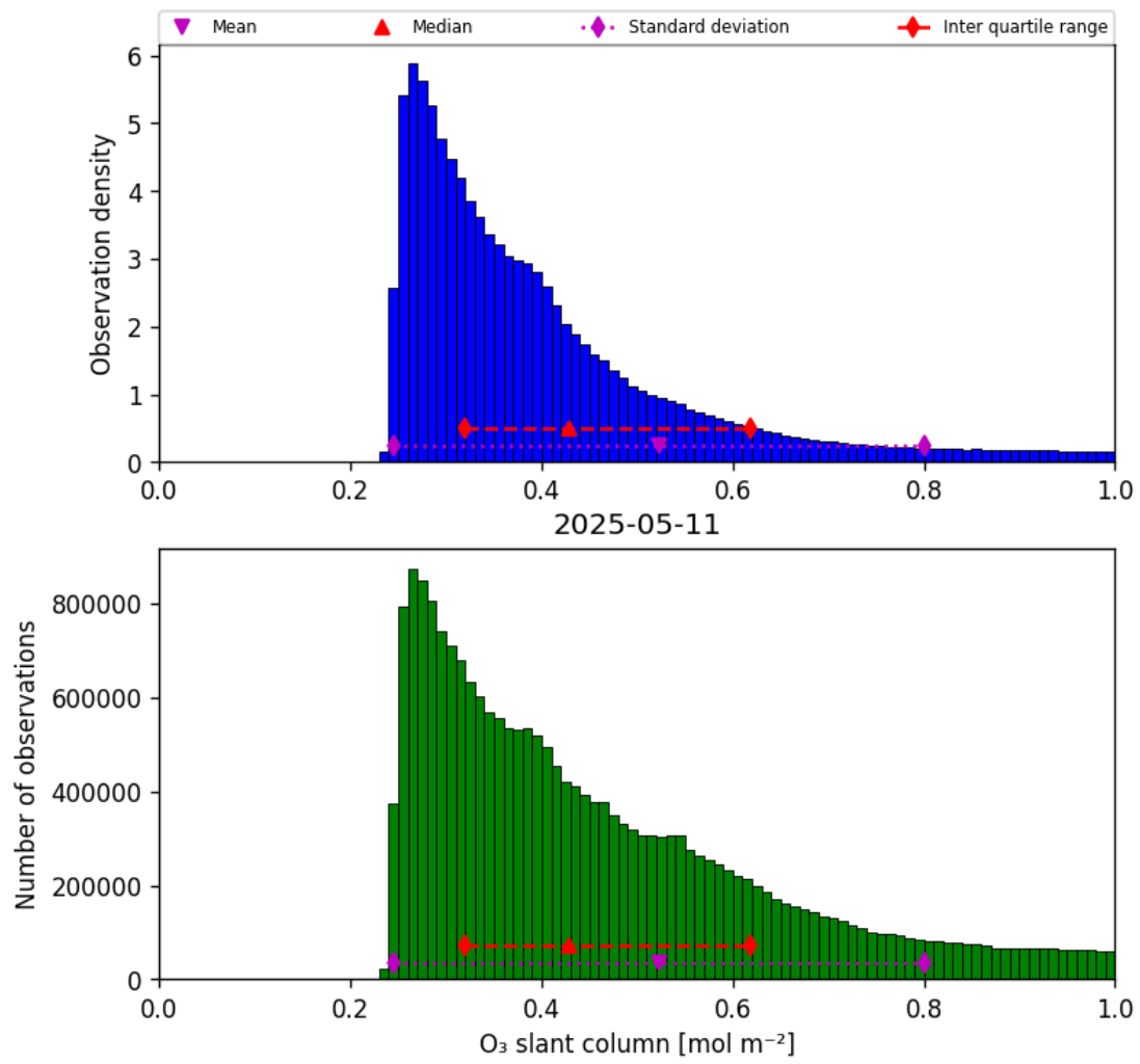
Figure 31: Histogram of “O 3 slant column” for 2025-05-11 to 2025-05-12
