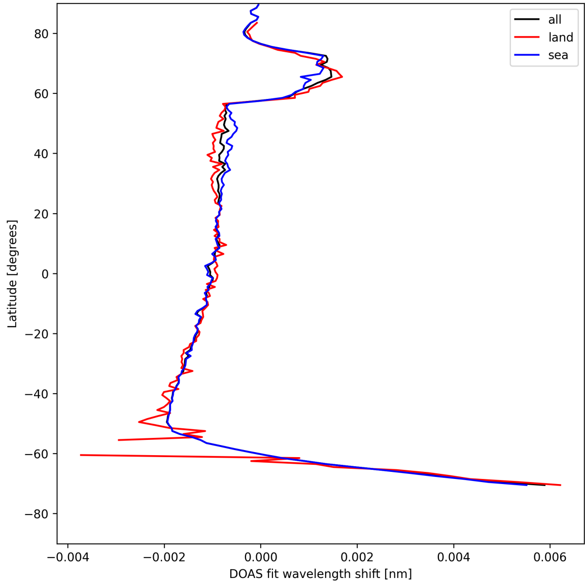
Figure 23: Zonal average of “DOAS fit wavelength shift” for 2025-05-11 to 2025-05-12.
