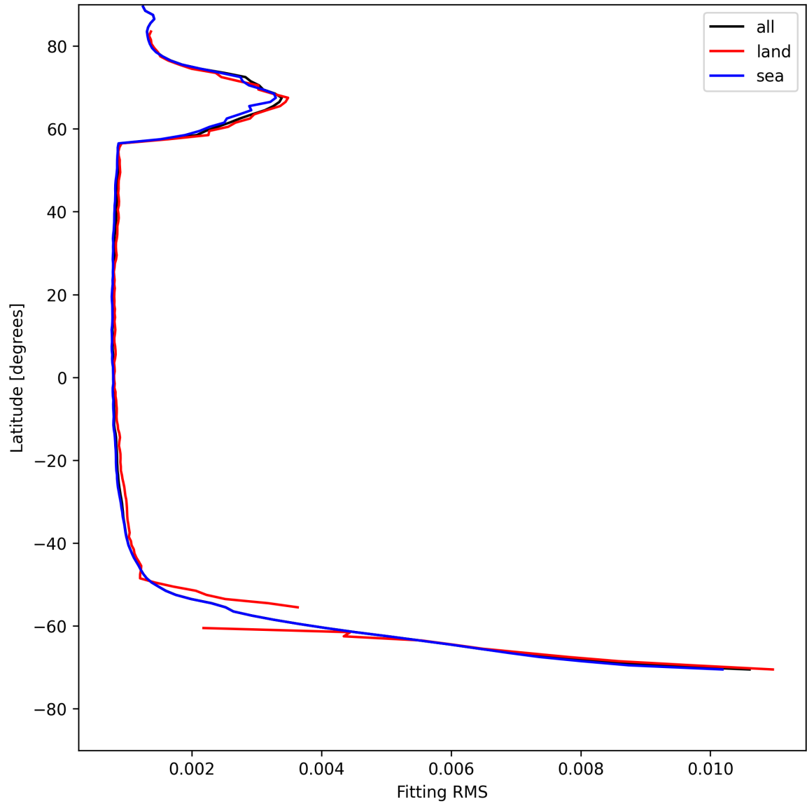
Figure 22: Zonal average of “Fitting RMS” for 2025-05-11 to 2025-05-12.
