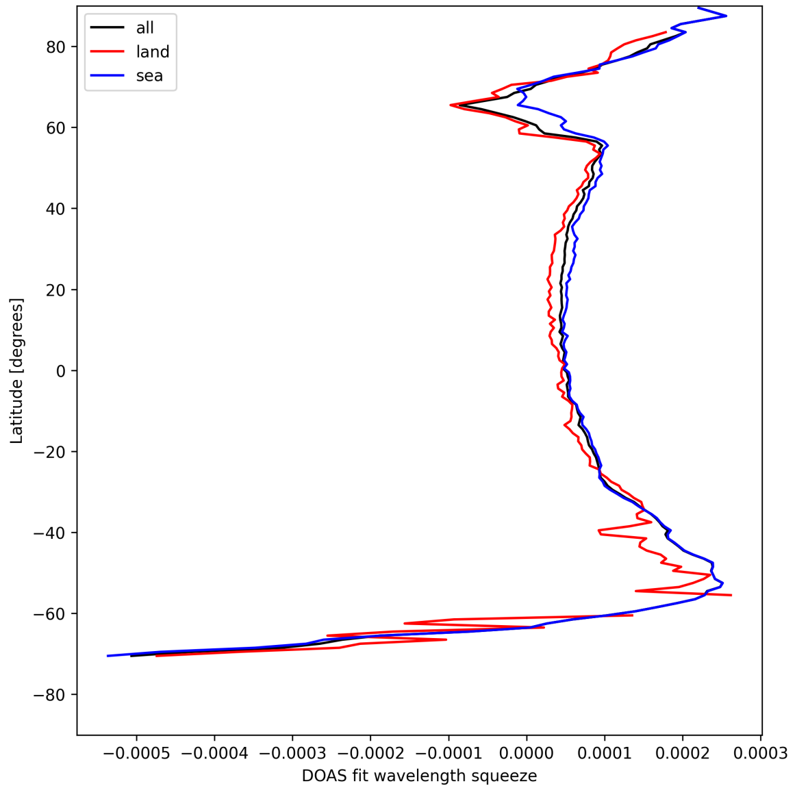
Figure 24: Zonal average of “DOAS fit wavelength squeeze” for 2025-05-12 to 2025-05-13.
