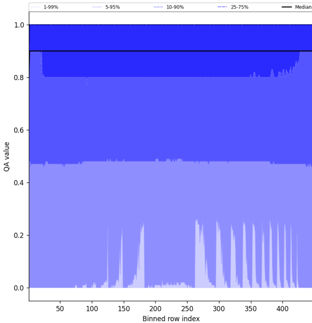
Figure 40: Along track statistics of “QA value” for 2025-05-12 to 2025-05-13
