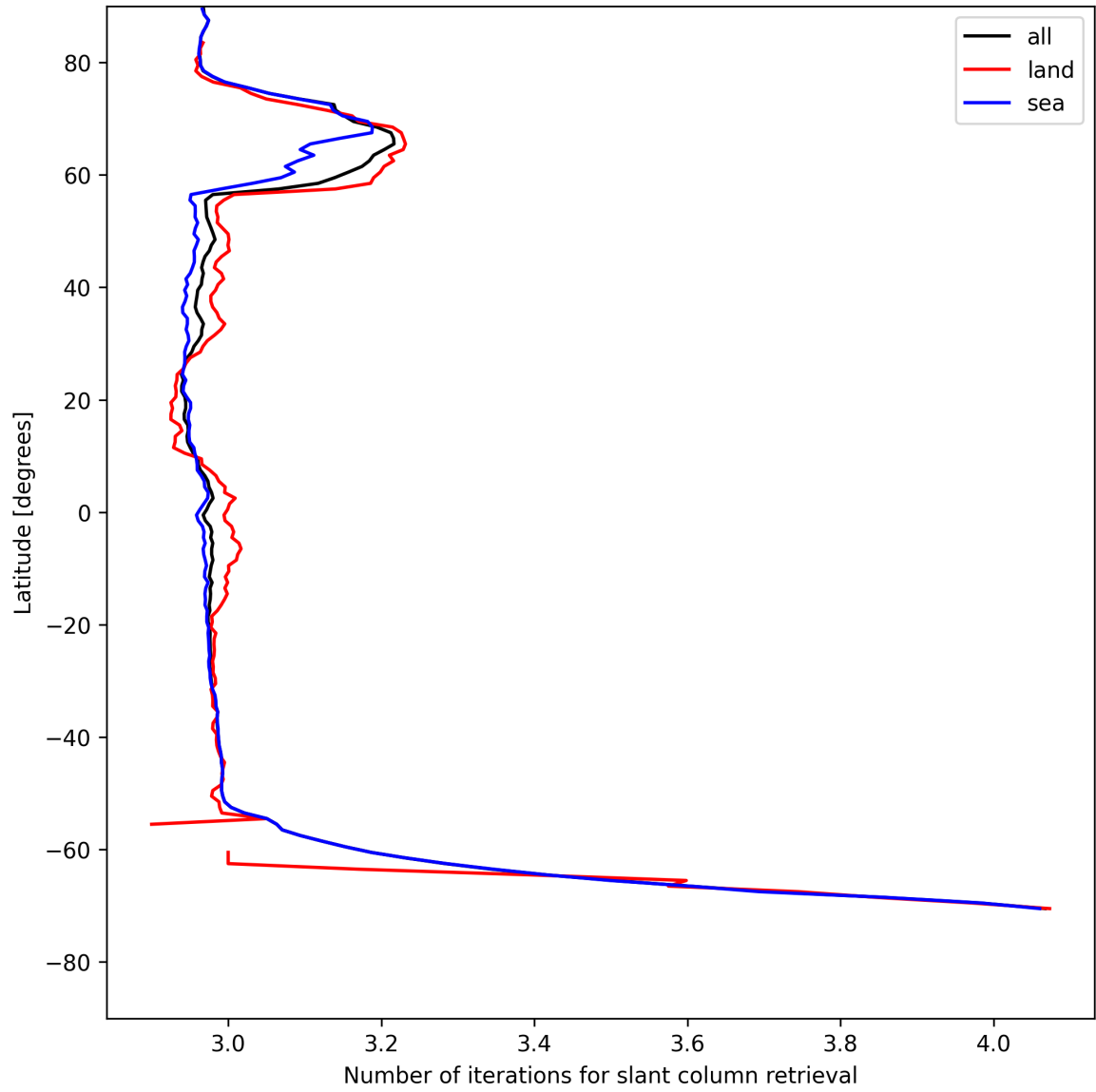
Figure 21: Zonal average of “Number of iterations for slant column retrieval” for 2025-05-12 to 2025-05-13.
