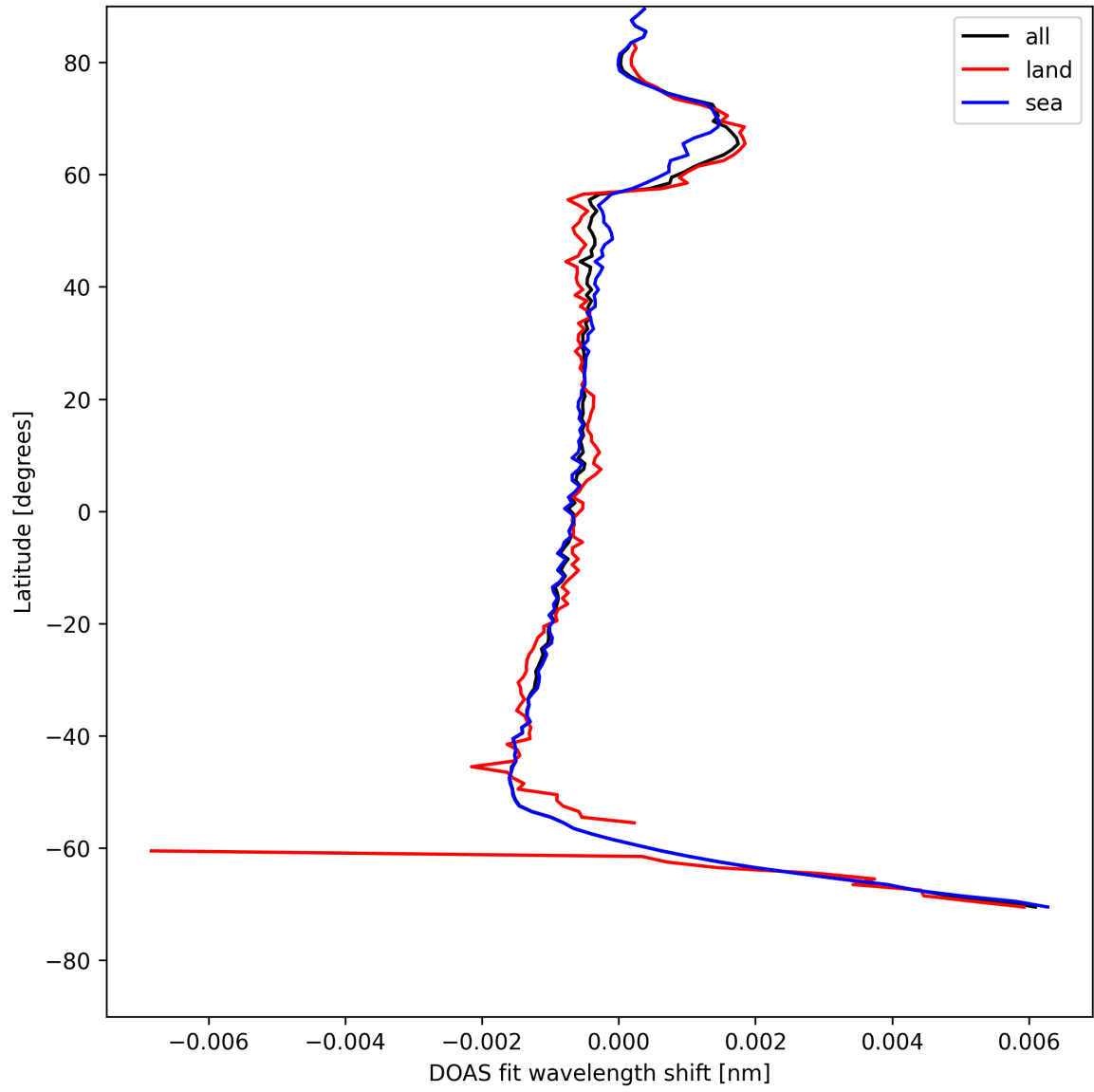
Figure 23: Zonal average of “DOAS fit wavelength shift” for 2025-05-12 to 2025-05-13.
