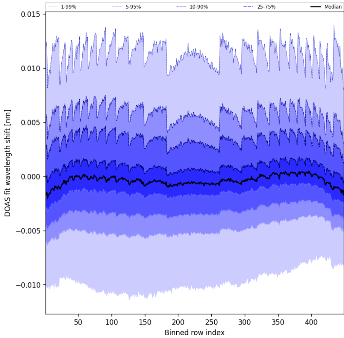
Figure 47: Along track statistics of "DOAS fit wavelength shift" for 2025-05-12 to 2025-05-13
