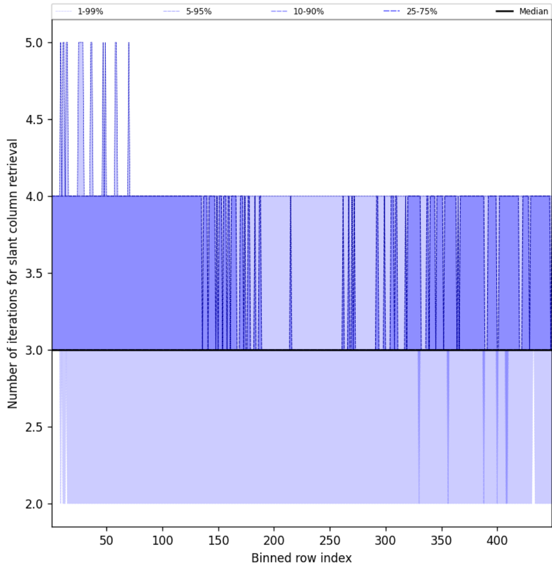
Figure 45: Along track statistics of “Number of iterations for slant column retrieval” for 2025-05-12 to 2025-05-13
