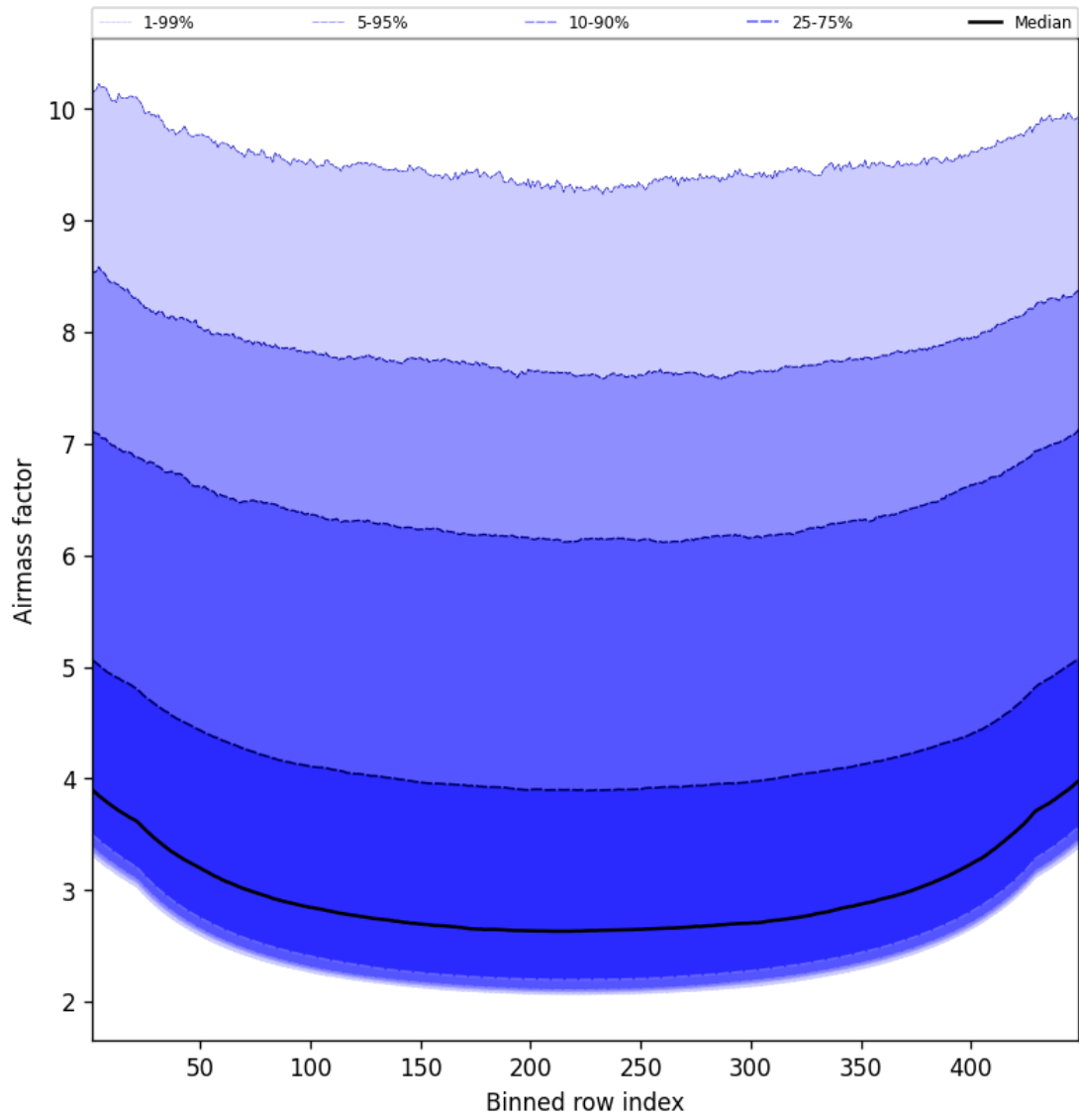
Figure 49: Along track statistics of “Airmass factor” for 2025-05-12 to 2025-05-13
