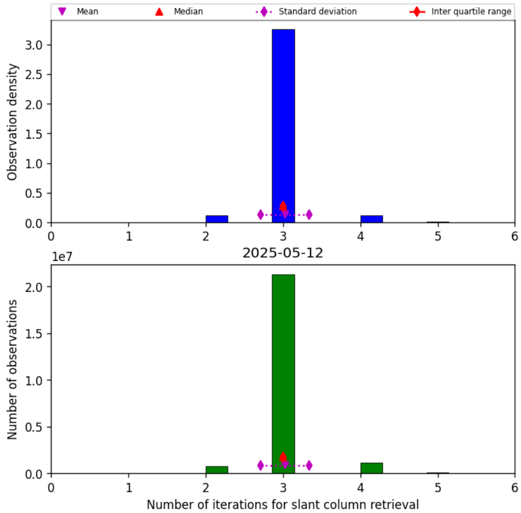
Figure 33: Histogram of “Number of iterations for slant column retrieval” for 2025-05-12 to 2025-05-13
