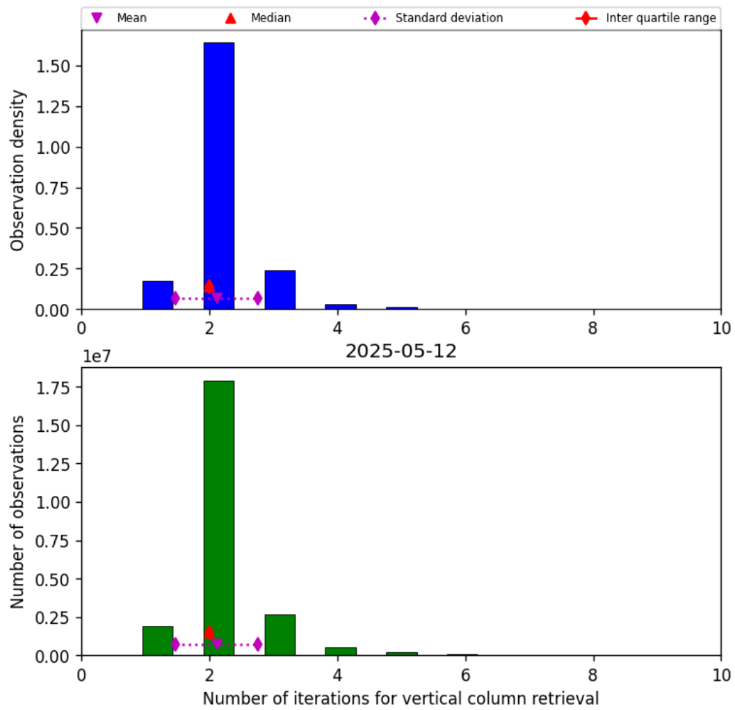
Figure 39: Histogram of “Number of iterations for vertical column retrieval” for 2025-05-12 to 2025-05-13
