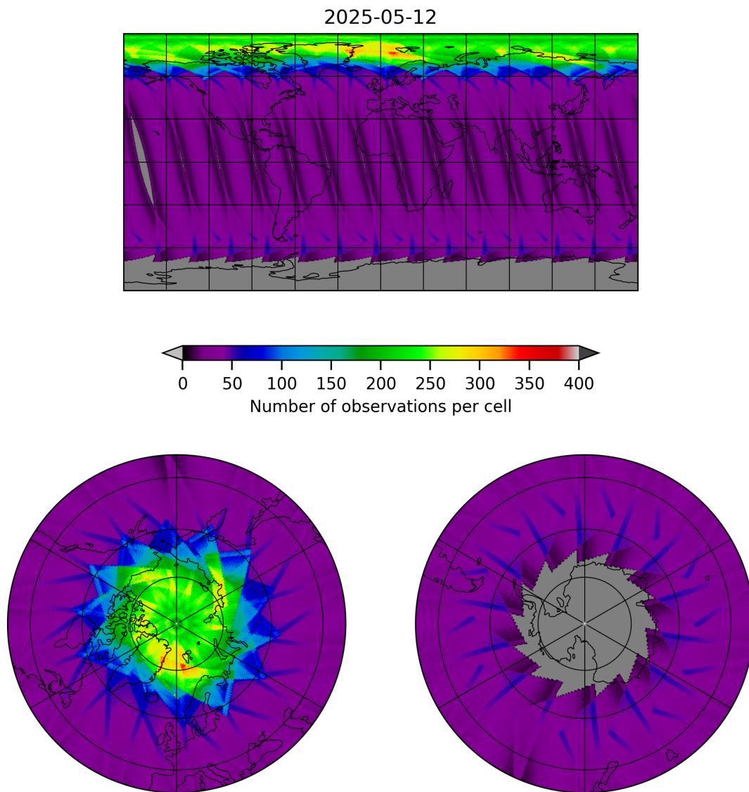
Figure 15: Map of the number of observations for 2025-05-12 to 2025-05-13
