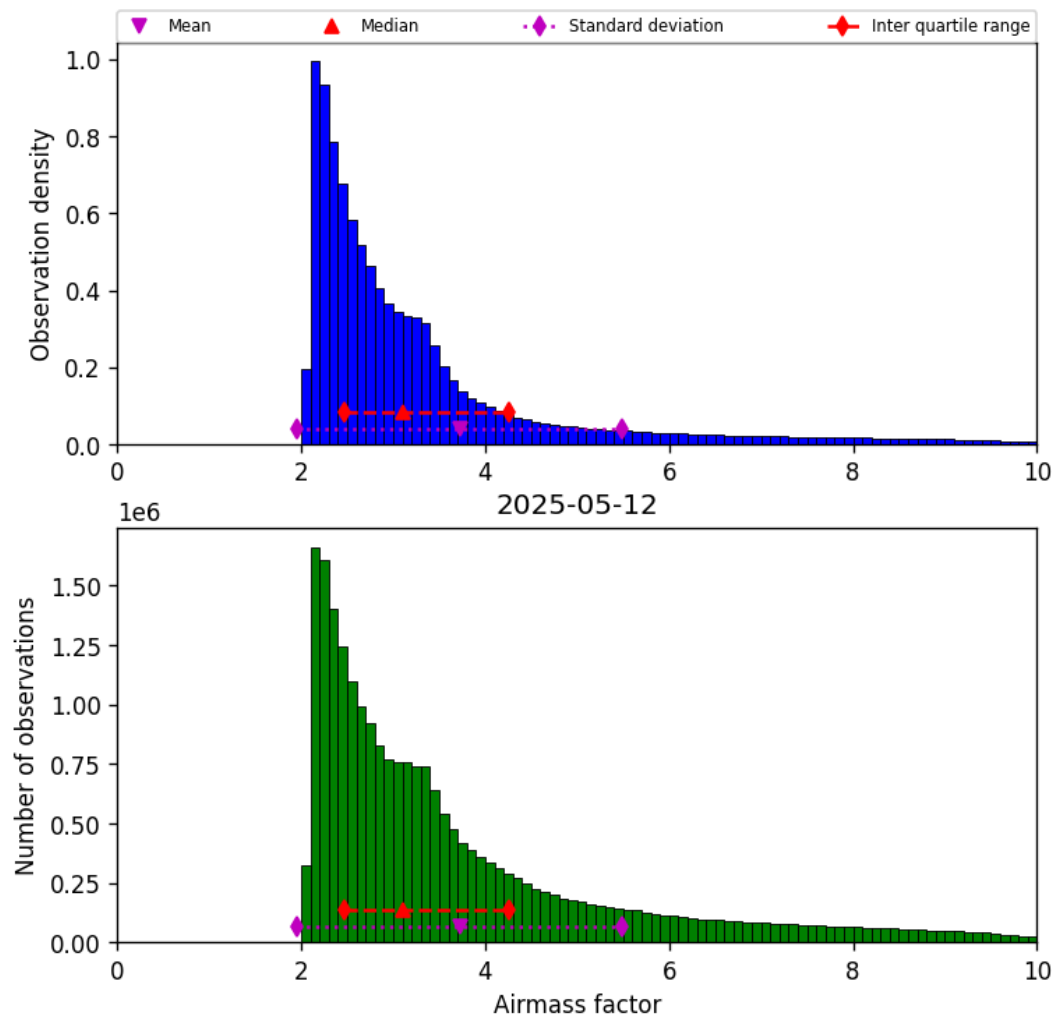
Figure 37: Histogram of “Airmass factor” for 2025-05-12 to 2025-05-13
