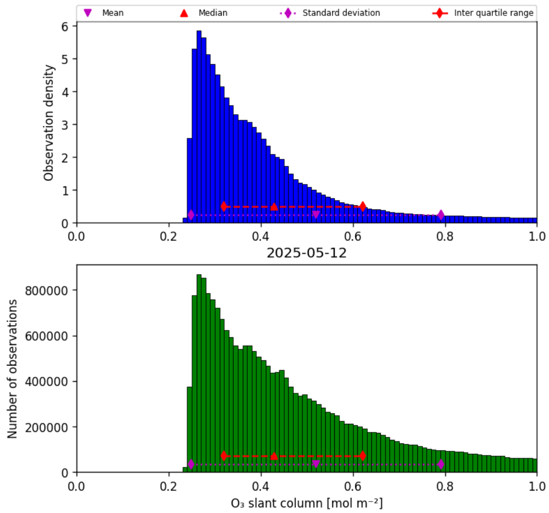
Figure 31: Histogram of “O 3 slant column” for 2025-05-12 to 2025-05-13
