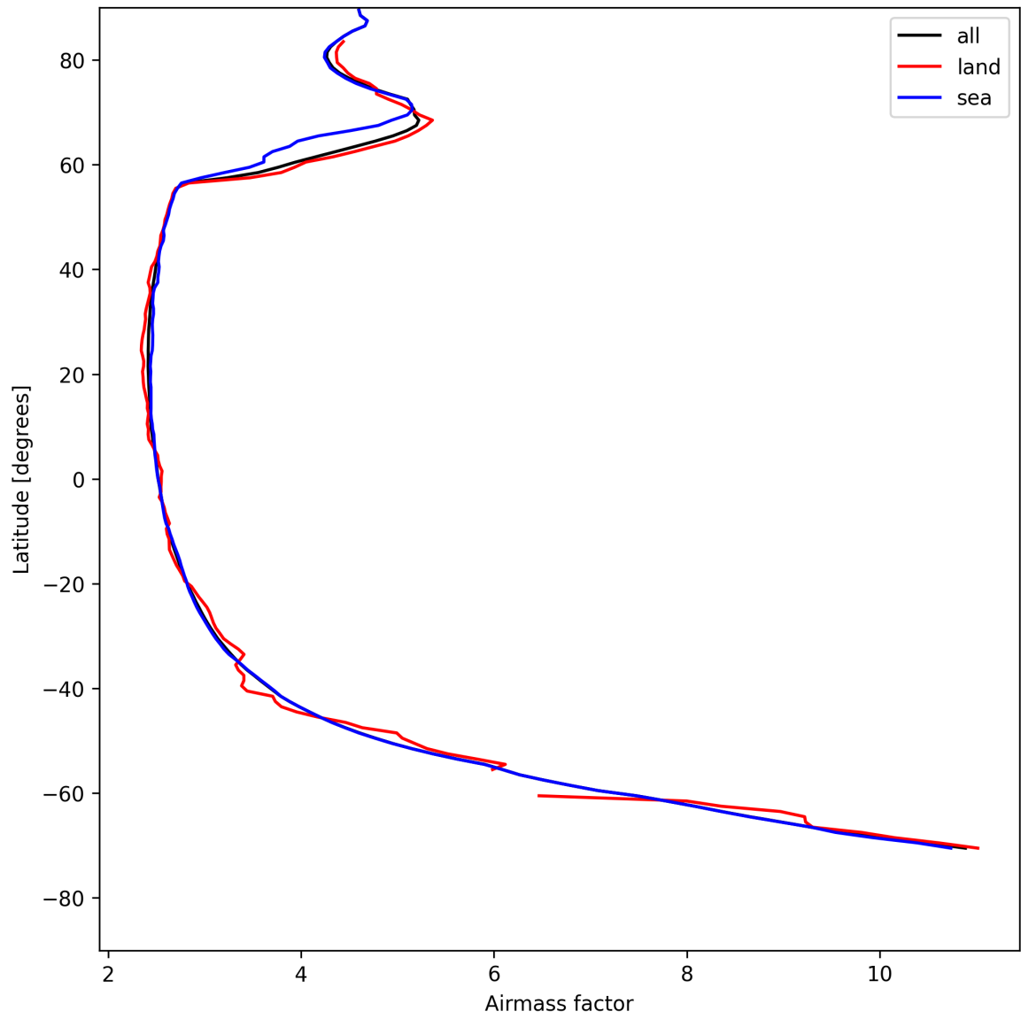
Figure 25: Zonal average of “Airmass factor” for 2025-05-12 to 2025-05-13.
