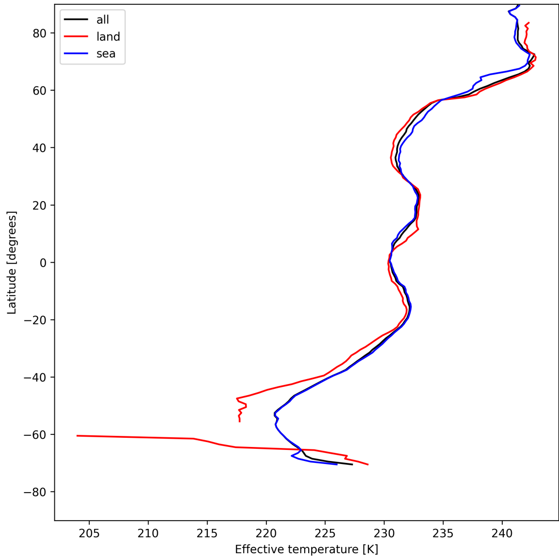
Figure 26: Zonal average of "Effective temperature" for 2025-05-12 to 2025-05-13.
