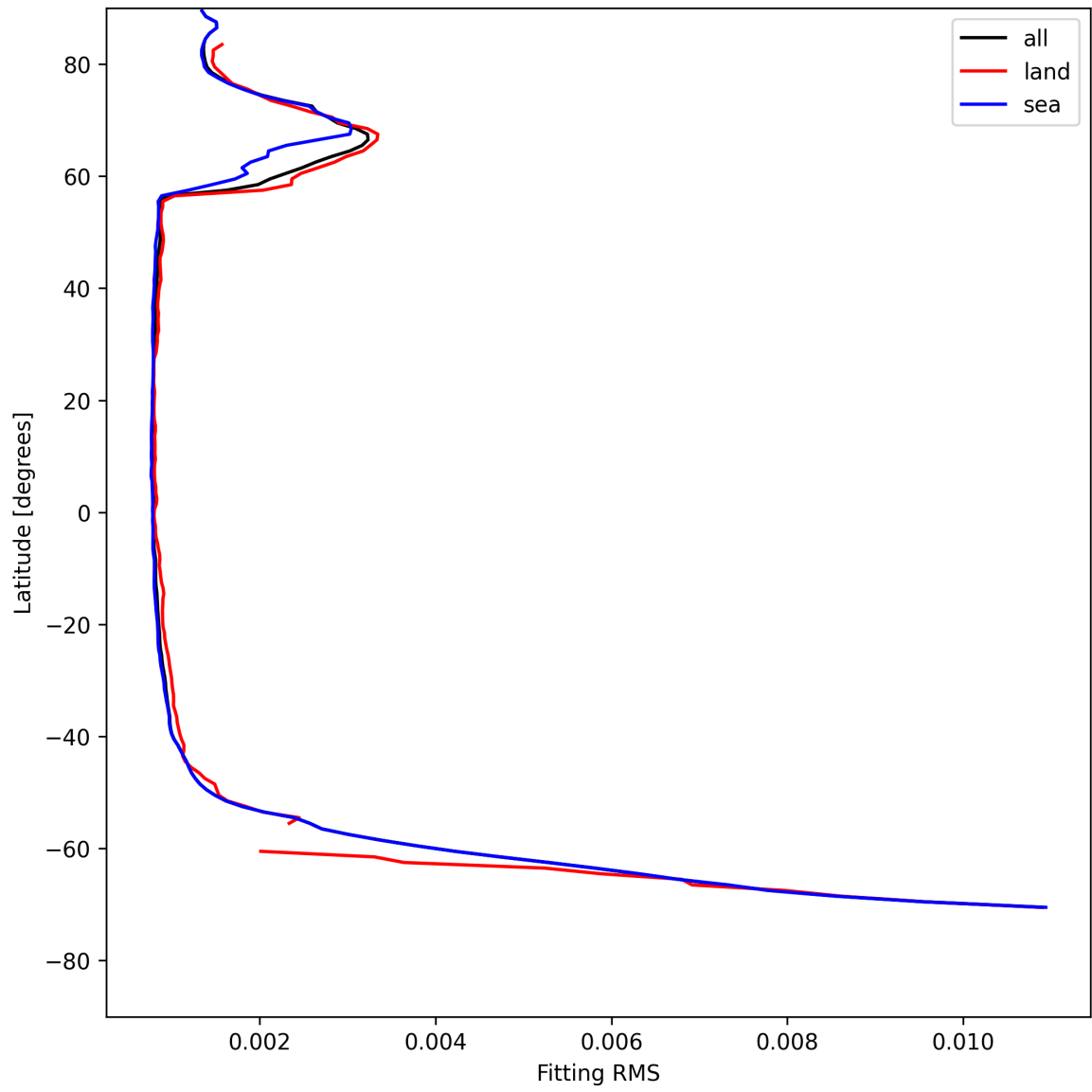
Figure 22: Zonal average of “Fitting RMS” for 2025-05-12 to 2025-05-13.
