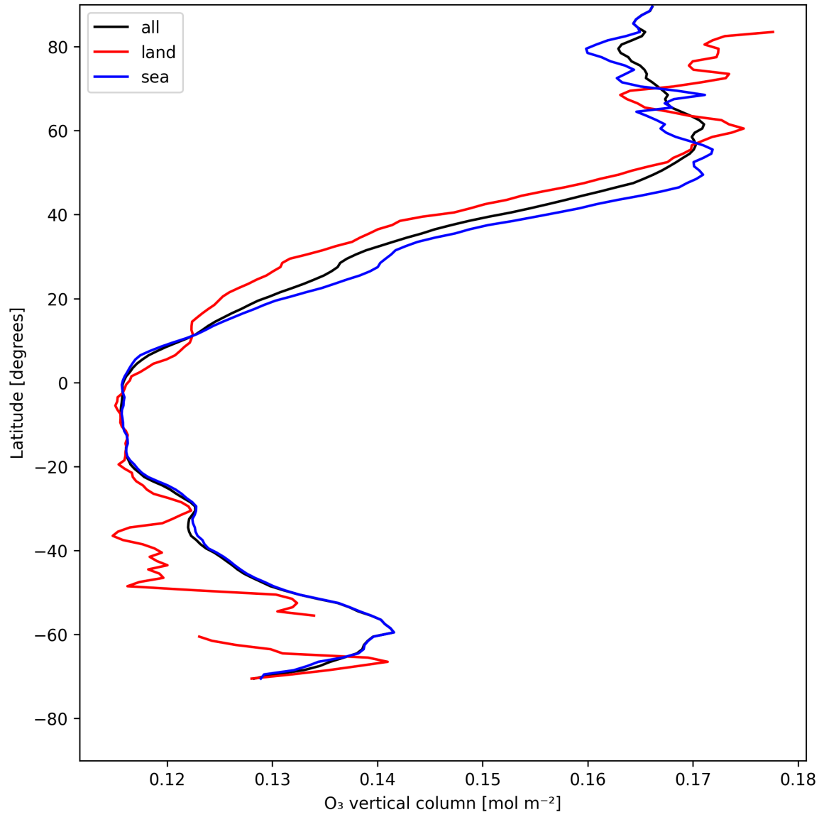
Figure 17: Zonal average of “O 3 vertical column” for 2025-05-12 to 2025-05-13.
