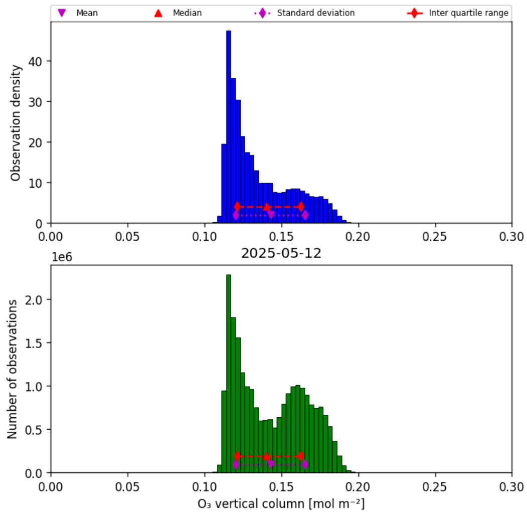
Figure 29: Histogram of “O 3 vertical column” for 2025-05-12 to 2025-05-13
