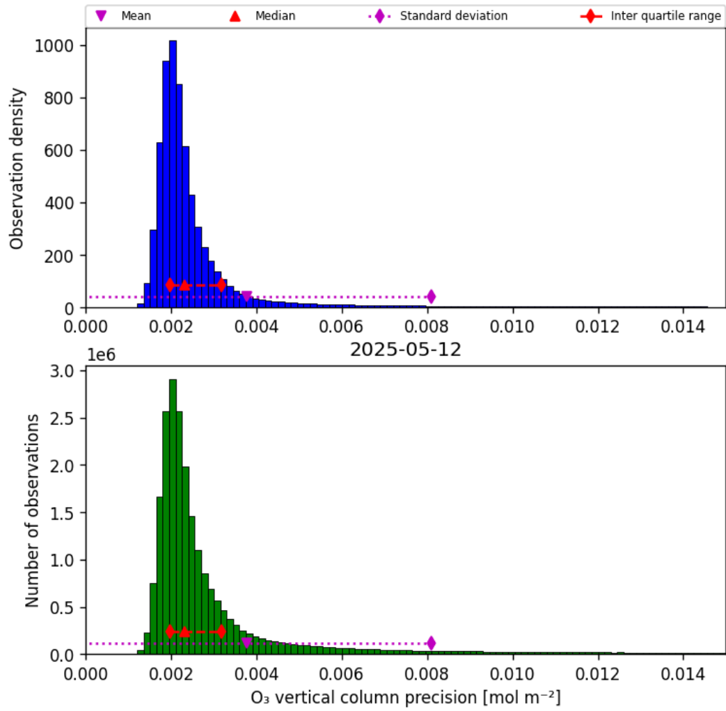
Figure 30: Histogram of “O 3 vertical column precision” for 2025-05-12 to 2025-05-13
