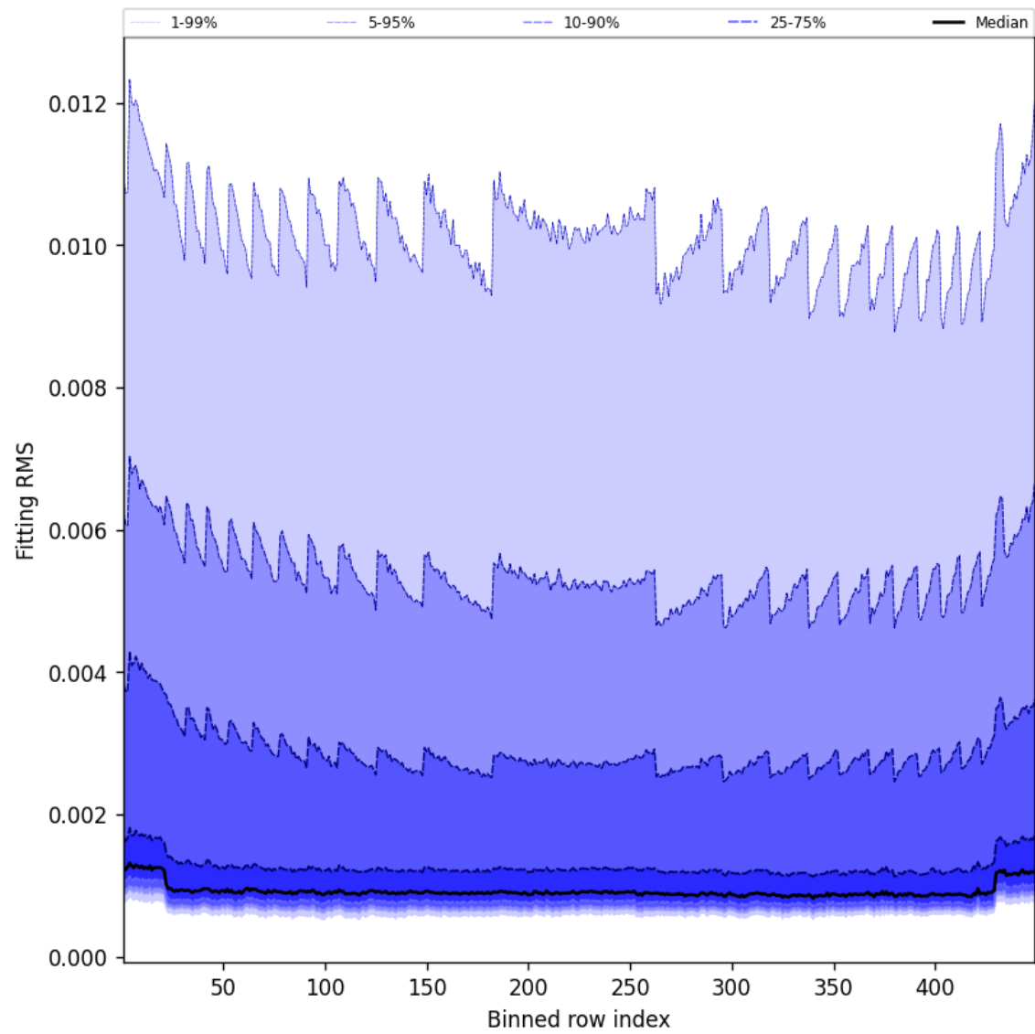
Figure 46: Along track statistics of “Fitting RMS” for 2025-05-12 to 2025-05-13
