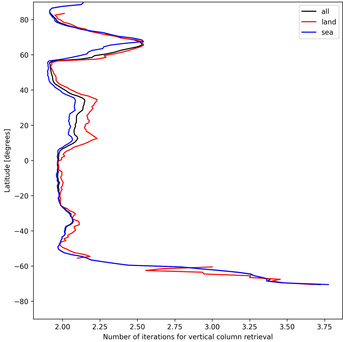
Figure 27: Zonal average of “Number of iterations for vertical column retrieval” for 2025-05-12 to 2025-05-13.
