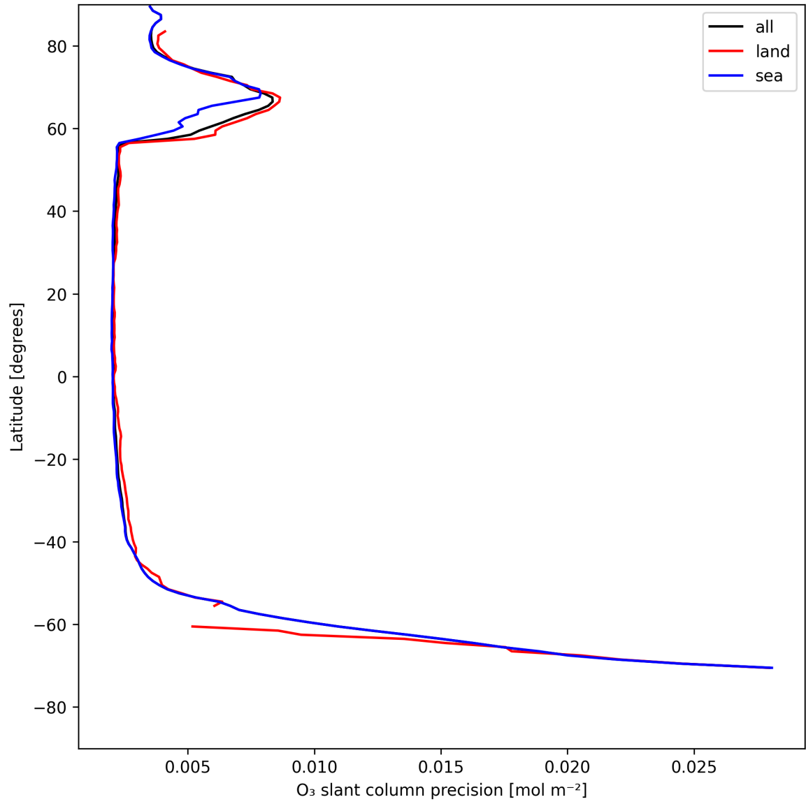
Figure 20: Zonal average of "O 3 slant column precision" for 2025-05-12 to 2025-05-13.
