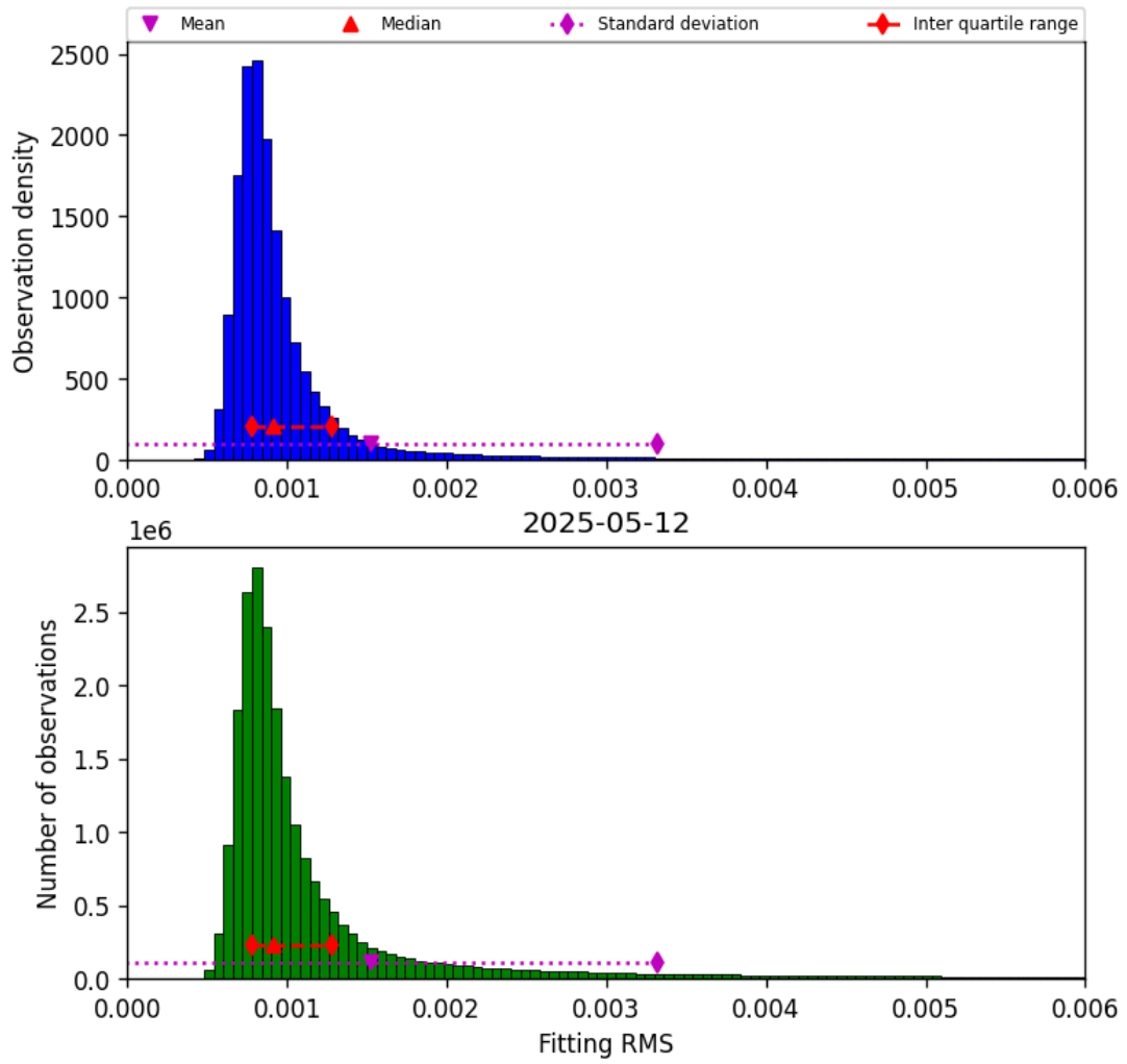
Figure 34: Histogram of “Fitting RMS” for 2025-05-12 to 2025-05-13
