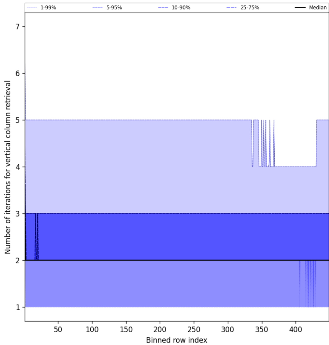
Figure 51: Along track statistics of “Number of iterations for vertical column retrieval” for 2025-05-12 to 2025-05-13
