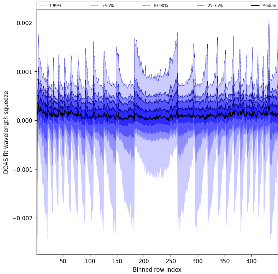
Figure 48: Along track statistics of “DOAS fit wavelength squeeze” for 2025-05-12 to 2025-05-13
