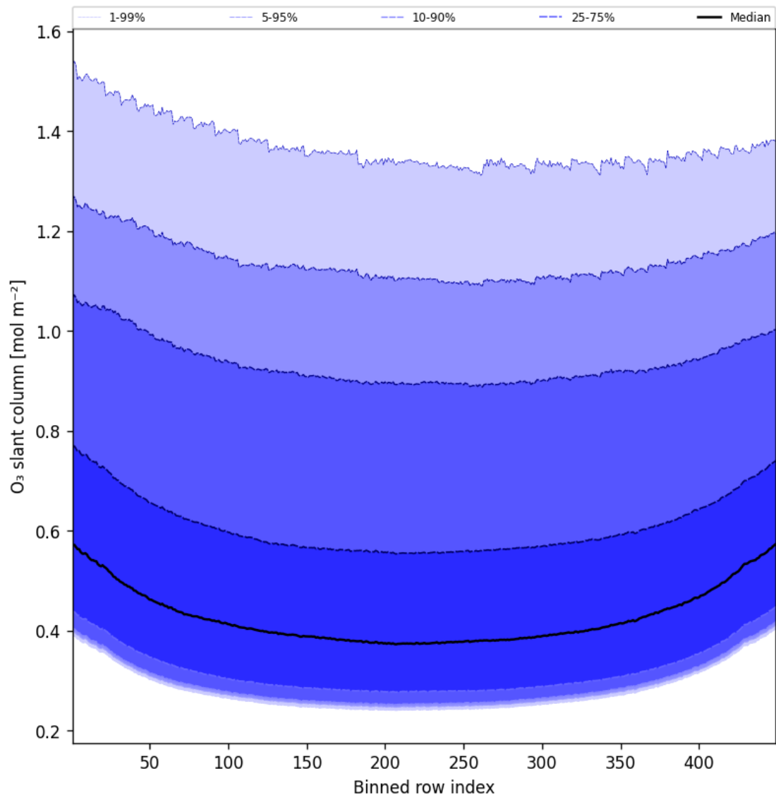
Figure 43: Along track statistics of “O 3 slant column” for 2025-05-12 to 2025-05-13
