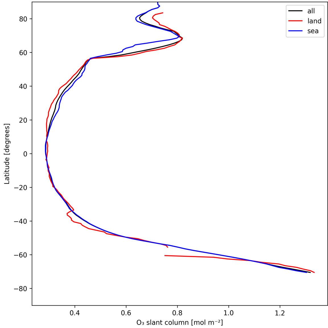
Figure 19: Zonal average of “O 3 slant column” for 2025-05-12 to 2025-05-13.
