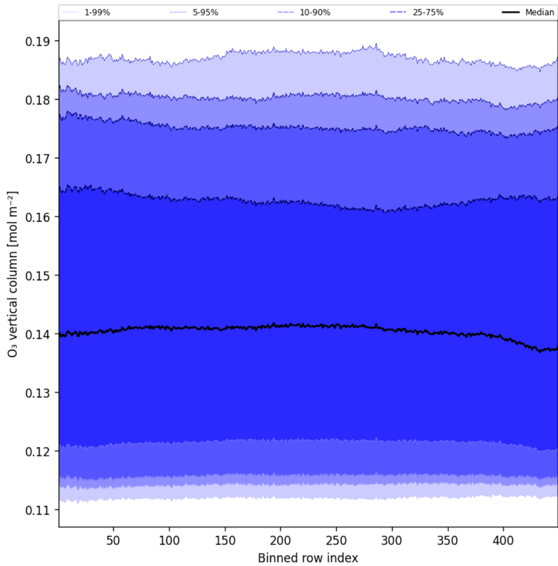
Figure 41: Along track statistics of “ O_3 vertical column” for 2025-05-12 to 2025-05-13
