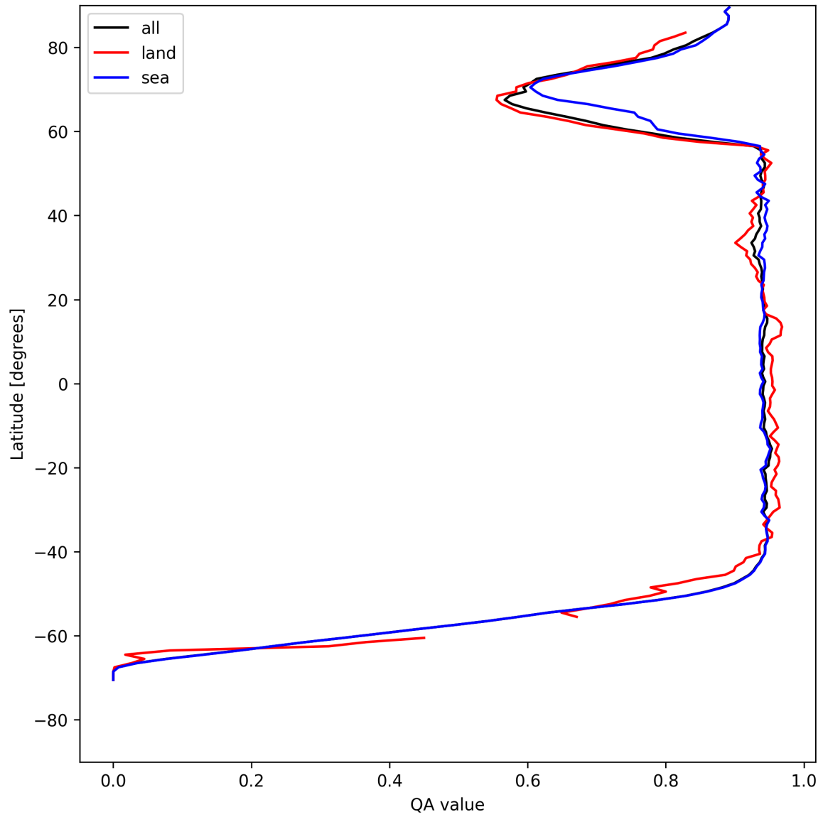
Figure 16: Zonal average of “QA value” for 2025-05-12 to 2025-05-13.
