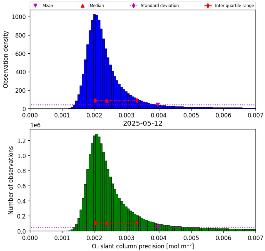
Figure 32: Histogram of “O 3 slant column precision” for 2025-05-12 to 2025-05-13
