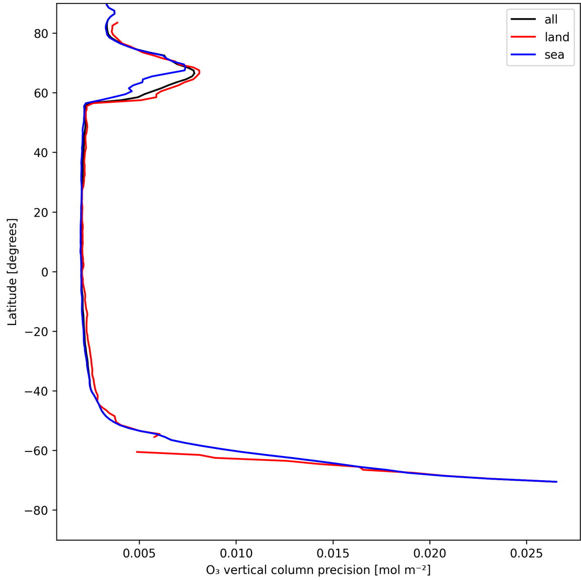
Figure 18: Zonal average of “O 3 vertical column precision” for 2025-05-12 to 2025-05-13.
