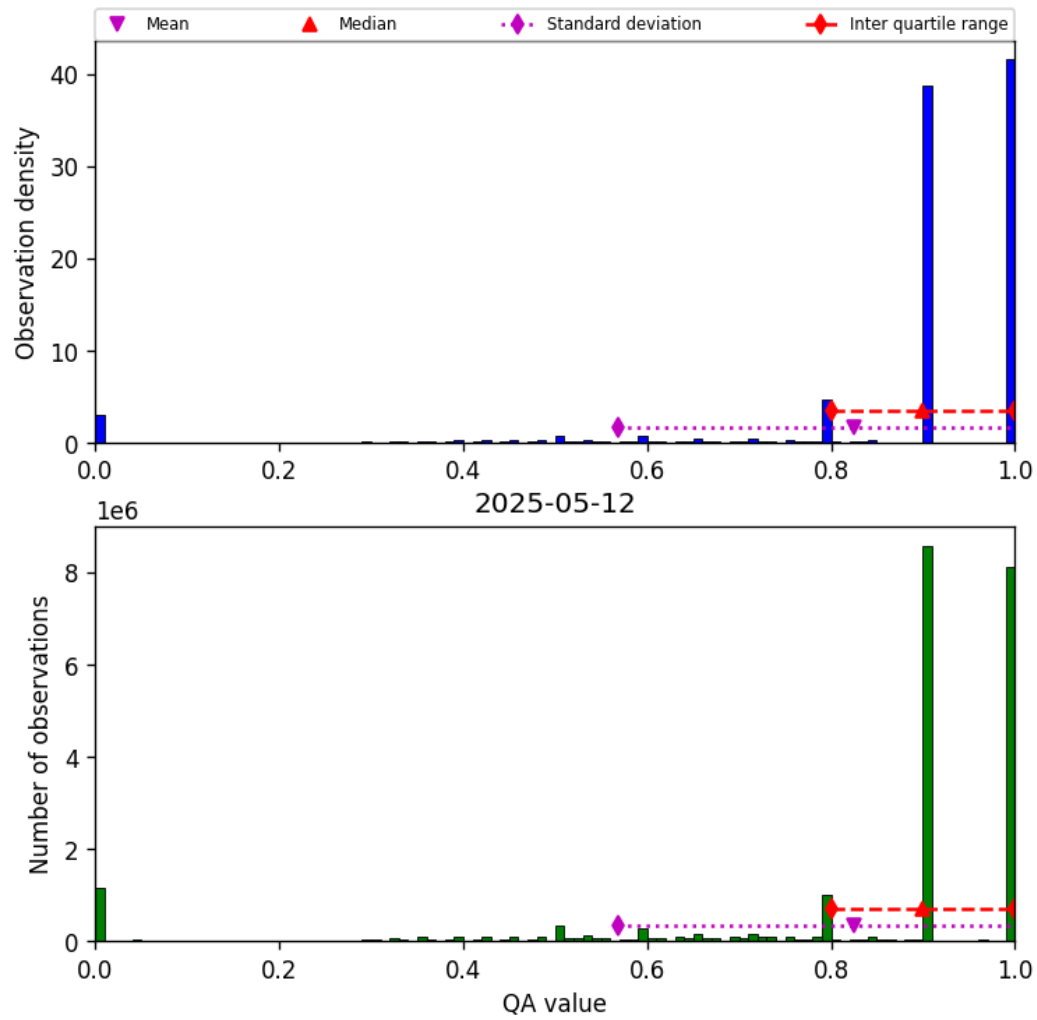
Figure 28: Histogram of “QA value” for 2025-05-12 to 2025-05-13
