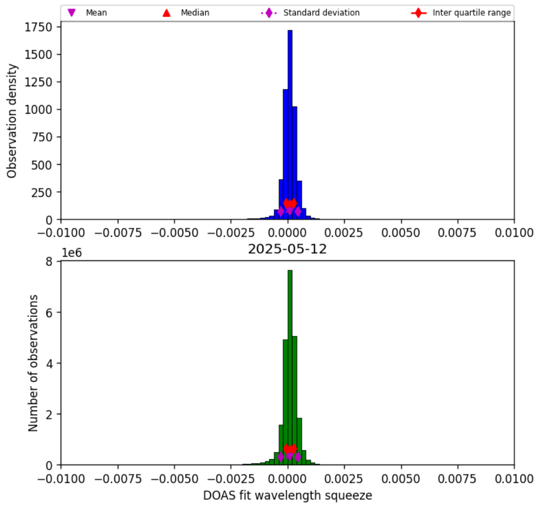
Figure 36: Histogram of “DOAS fit wavelength squeeze” for 2025-05-12 to 2025-05-13
