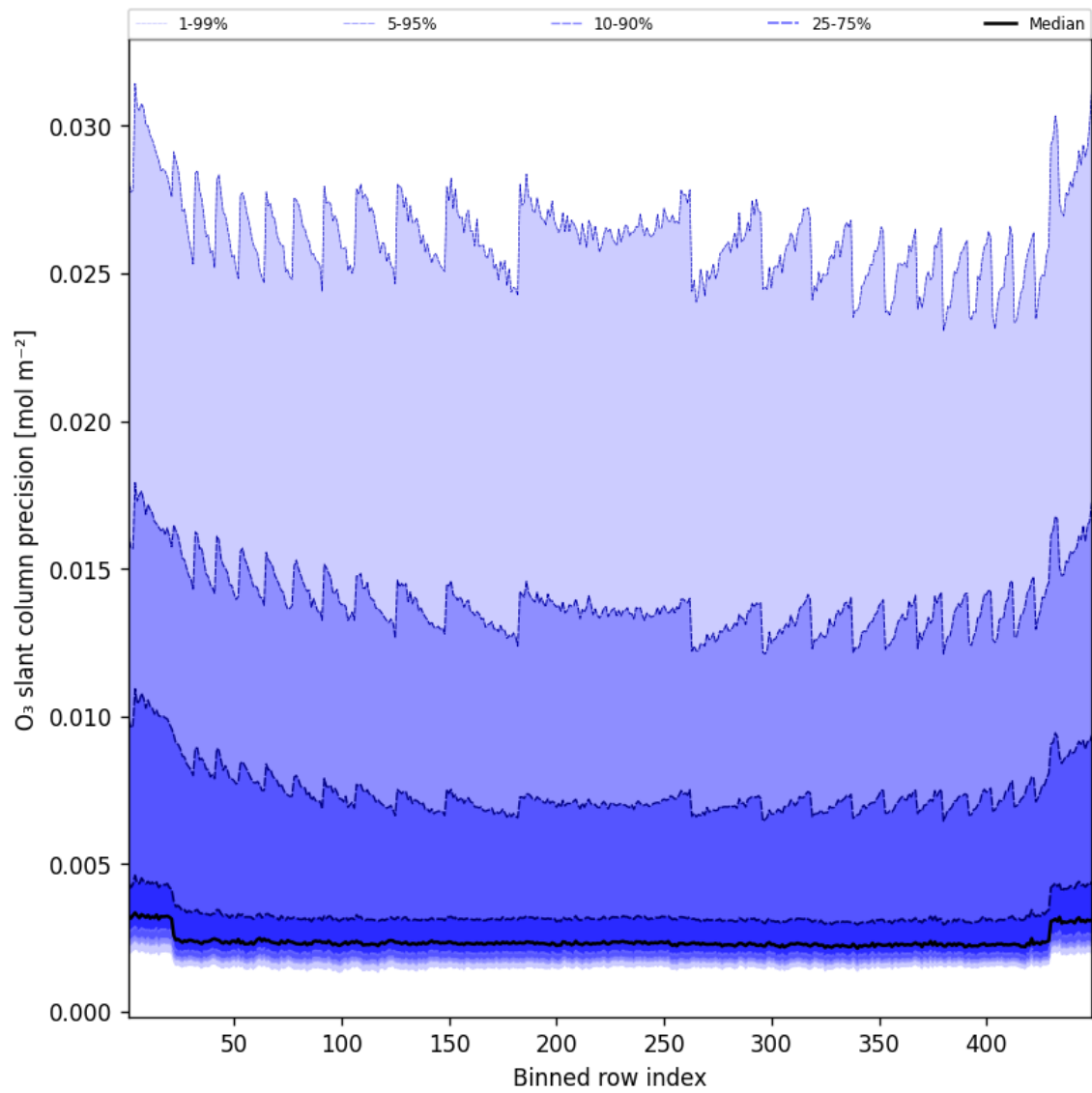
Figure 44: Along track statistics of “O 3 slant column precision” for 2025-05-12 to 2025-05-13
