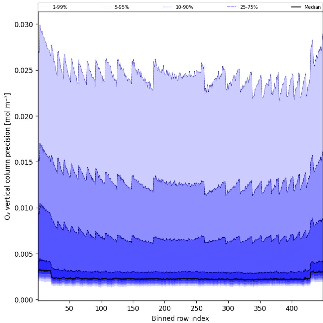
Figure 42: Along track statistics of “O 3 vertical column precision” for 2025-05-12 to 2025-05-13
