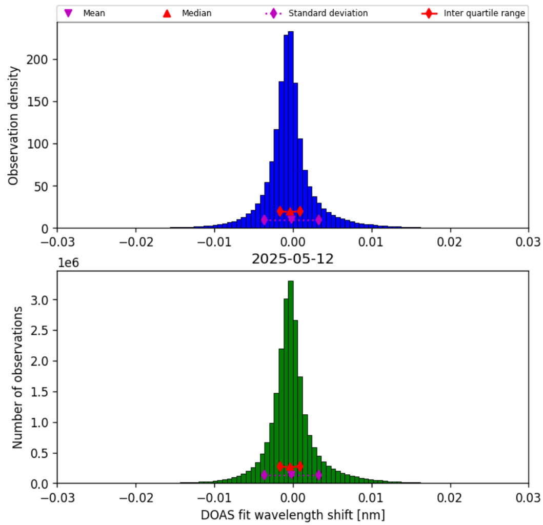
Figure 35: Histogram of “DOAS fit wavelength shift” for 2025-05-12 to 2025-05-13
