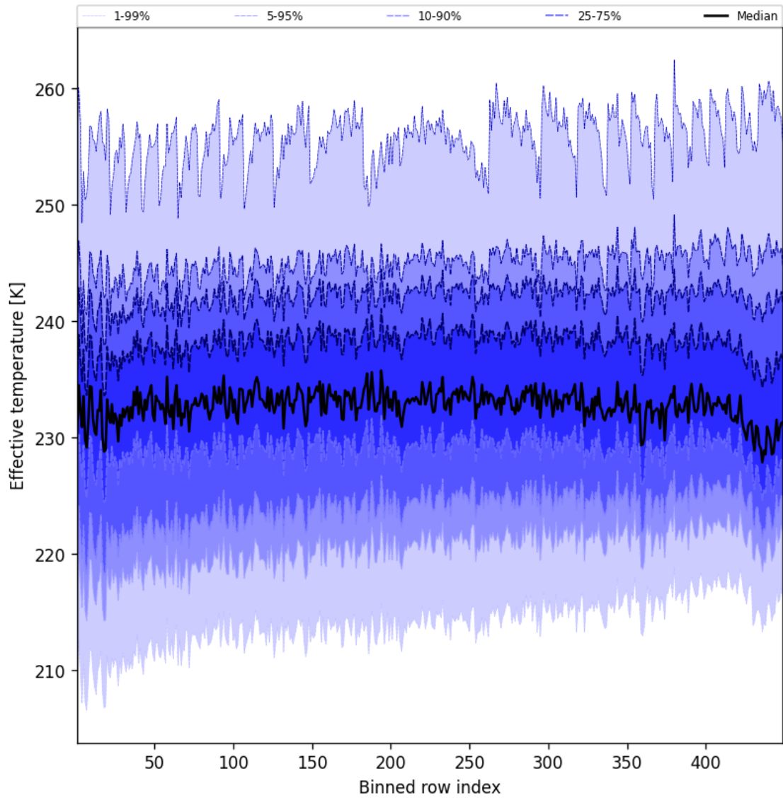
Figure 50: Along track statistics of “Effective temperature” for 2025-05-12 to 2025-05-13
