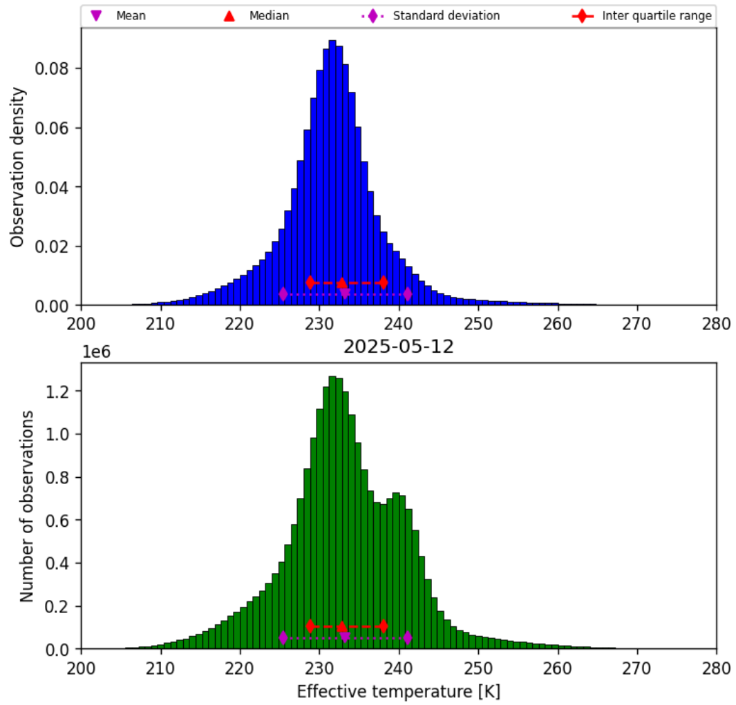
Figure 38: Histogram of “Effective temperature” for 2025-05-12 to 2025-05-13
