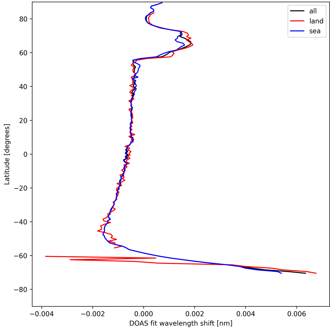
Figure 23: Zonal average of “DOAS fit wavelength shift” for 2025-05-13 to 2025-05-13.
