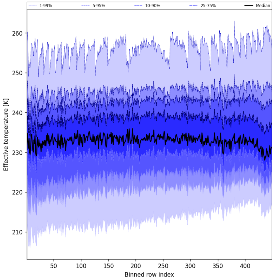
Figure 50: Along track statistics of “Effective temperature” for 2025-05-13 to 2025-05-13
