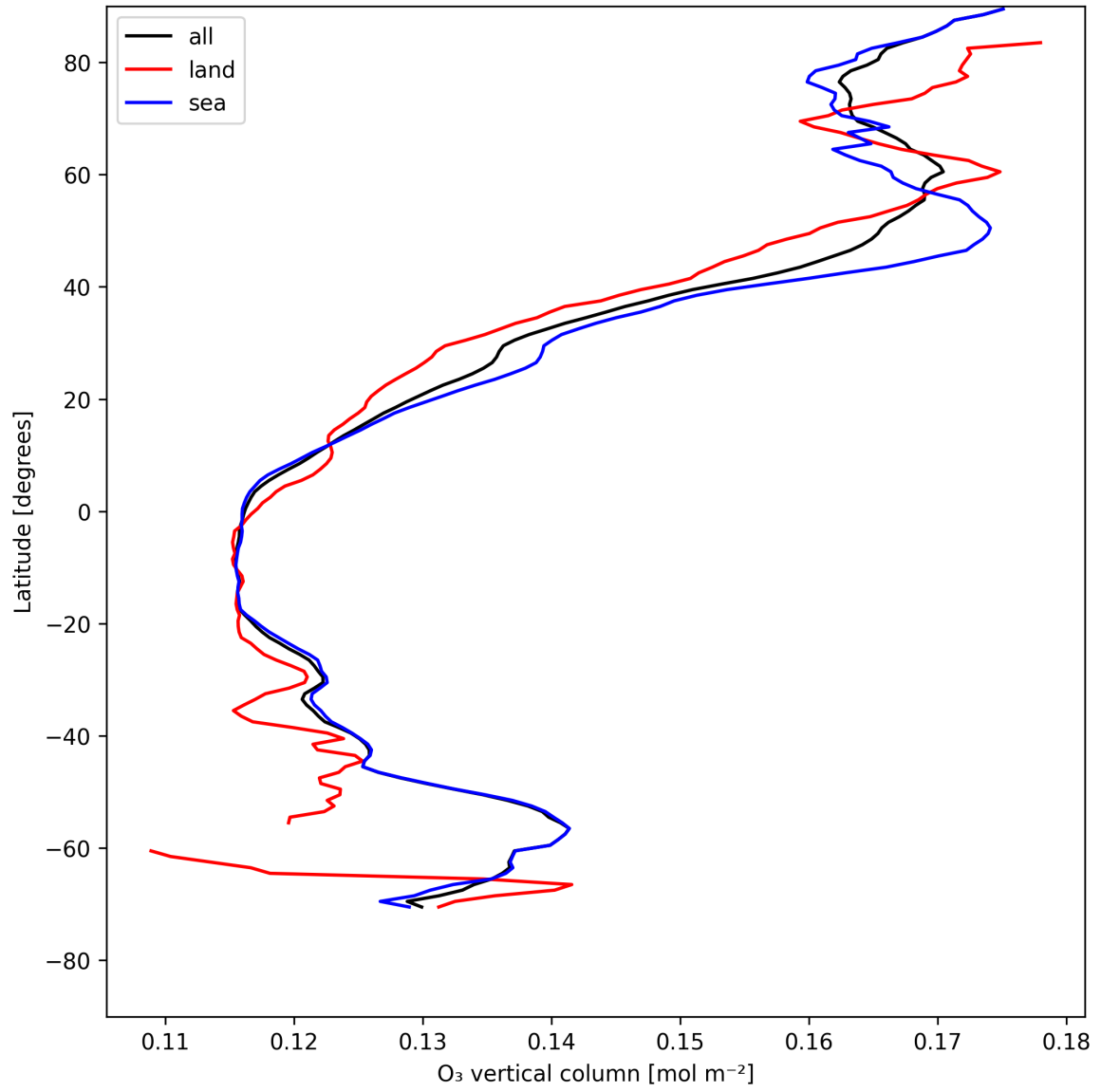
Figure 17: Zonal average of “O 3 vertical column” for 2025-05-13 to 2025-05-13.
