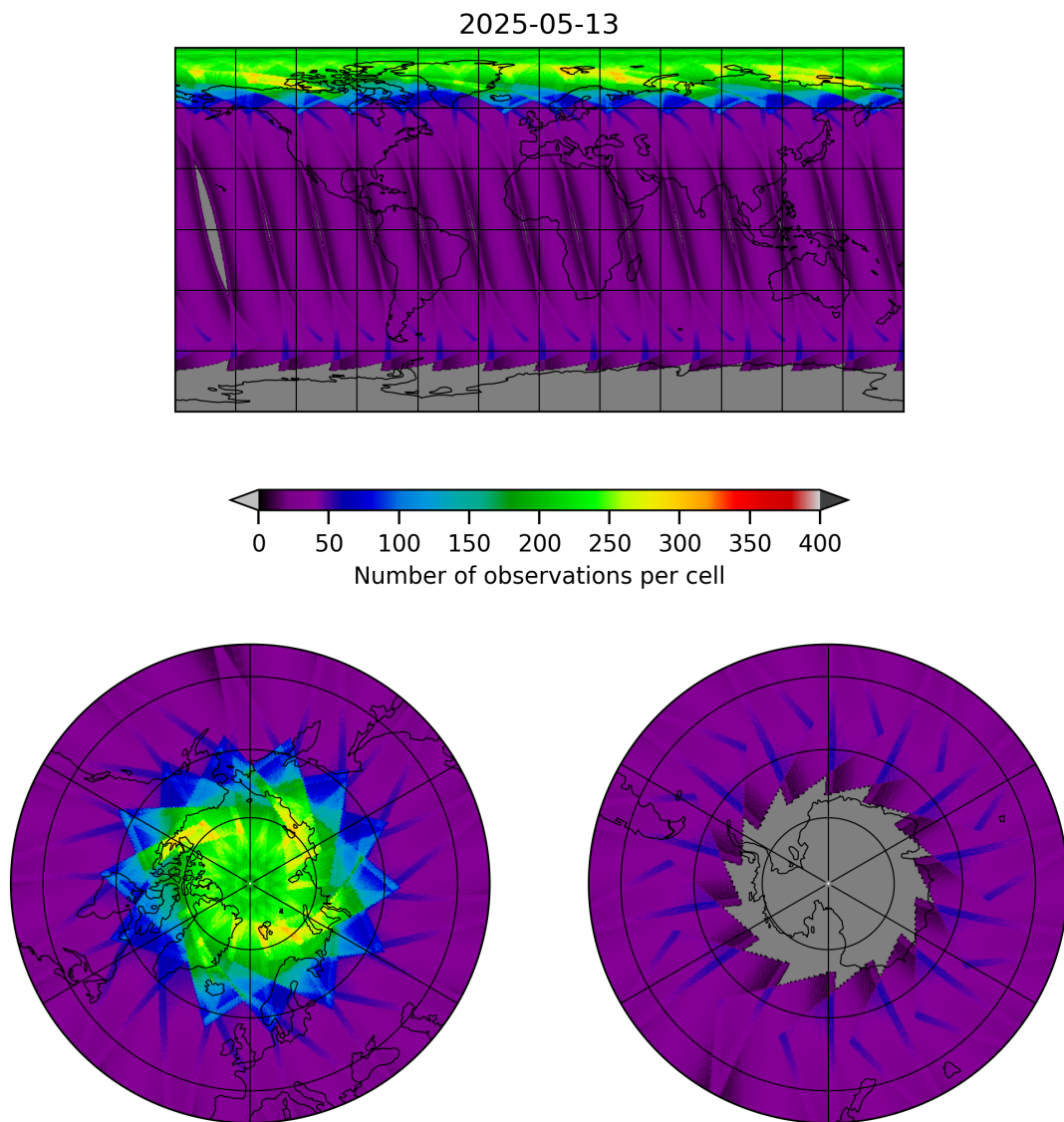
Figure 15: Map of the number of observations for 2025-05-13 to 2025-05-13
