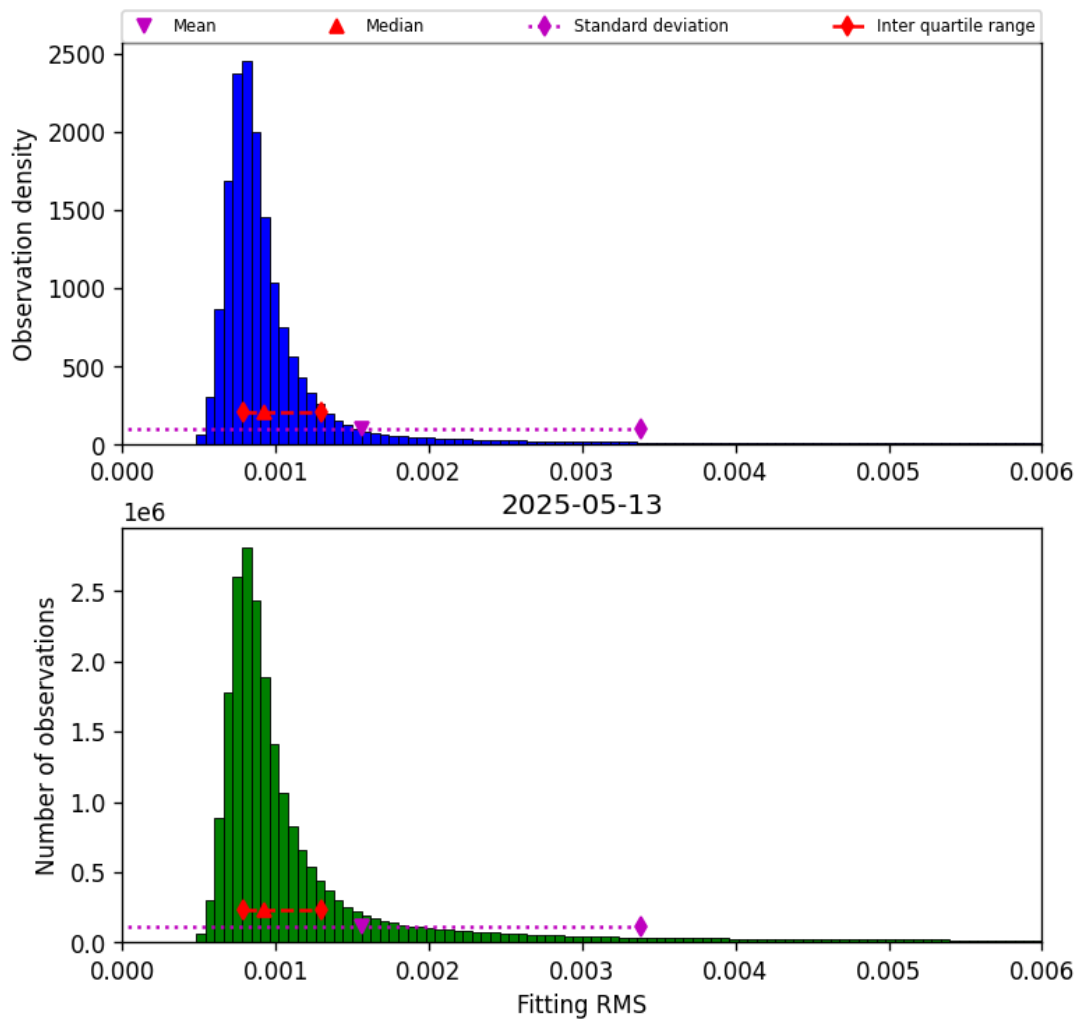
Figure 34: Histogram of “Fitting RMS” for 2025-05-13 to 2025-05-13
