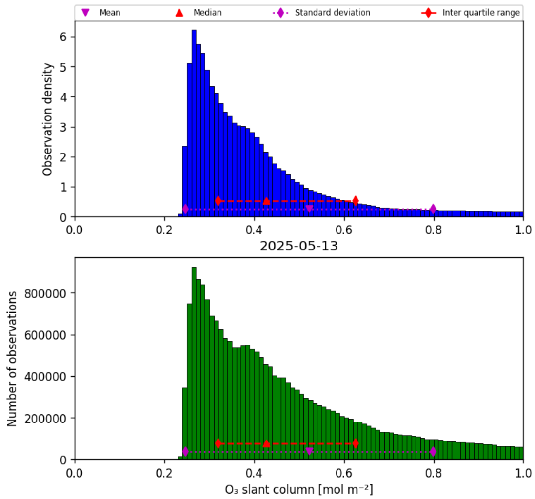
Figure 31: Histogram of “O 3 slant column” for 2025-05-13 to 2025-05-13
