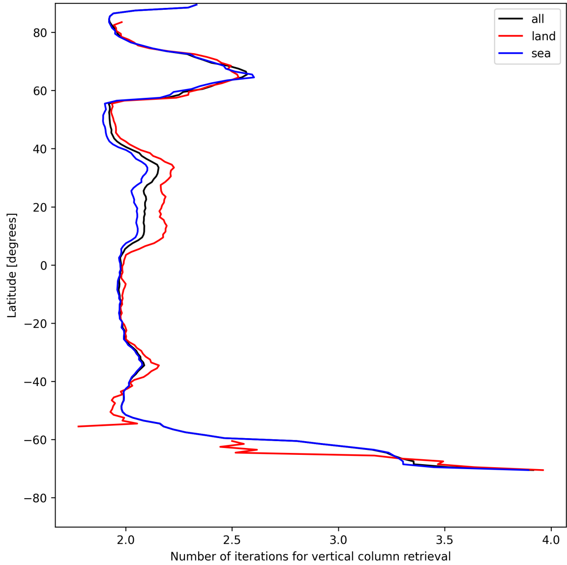
Figure 27: Zonal average of “Number of iterations for vertical column retrieval” for 2025-05-13 to 2025-05-13.
