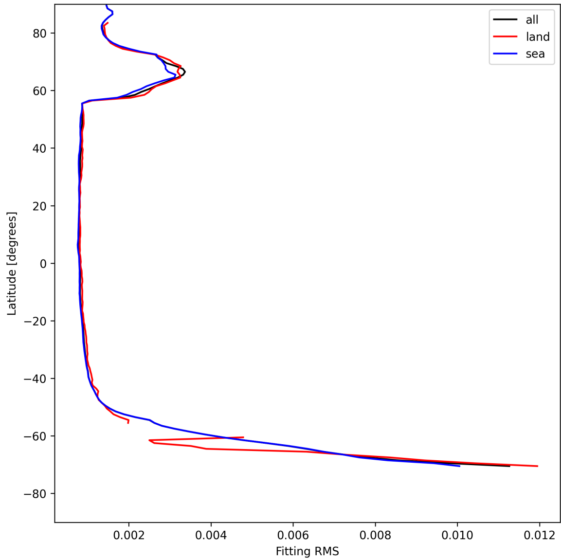
Figure 22: Zonal average of “Fitting RMS” for 2025-05-13 to 2025-05-13.
