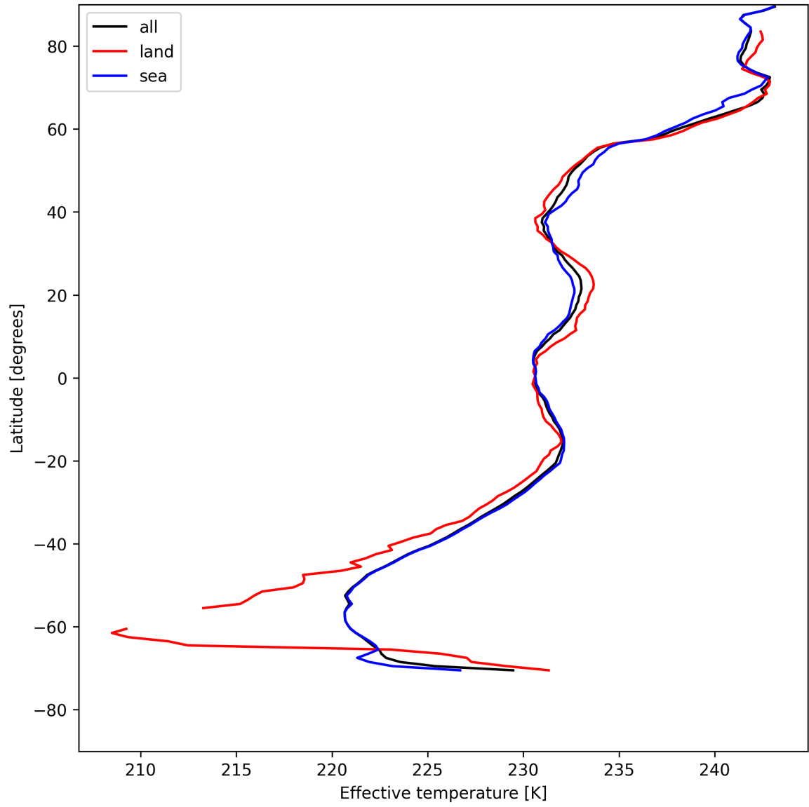
Figure 26: Zonal average of "Effective temperature" for 2025-05-13 to 2025-05-13.
