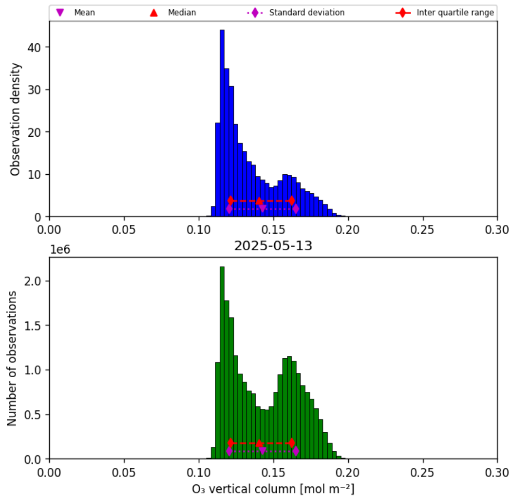
Figure 29: Histogram of “O 3 vertical column” for 2025-05-13 to 2025-05-13
