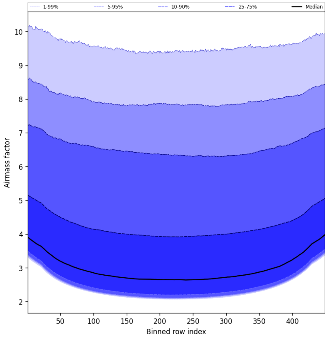
Figure 49: Along track statistics of “Airmass factor” for 2025-05-13 to 2025-05-13
