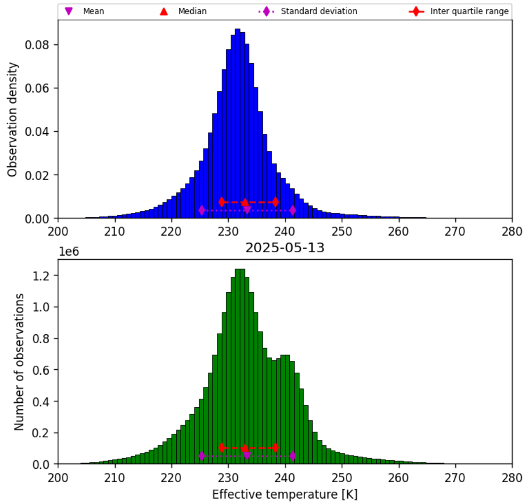
Figure 38: Histogram of “Effective temperature” for 2025-05-13 to 2025-05-13
