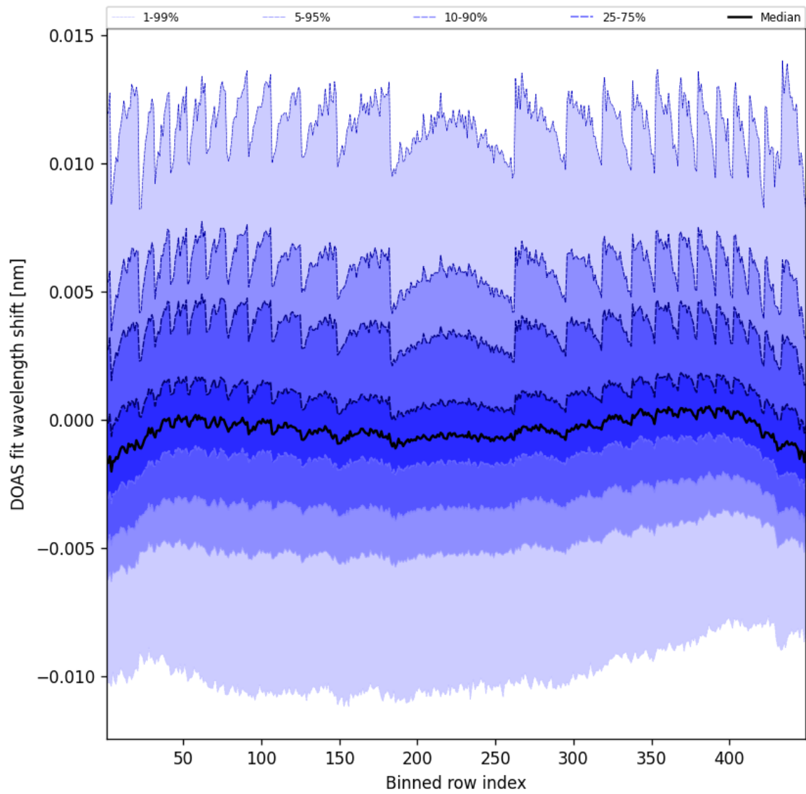
Figure 47: Along track statistics of “DOAS fit wavelength shift” for 2025-05-13 to 2025-05-13
