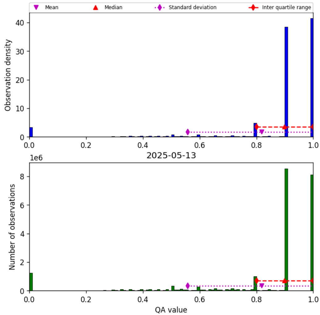
Figure 28: Histogram of “QA value” for 2025-05-13 to 2025-05-13
