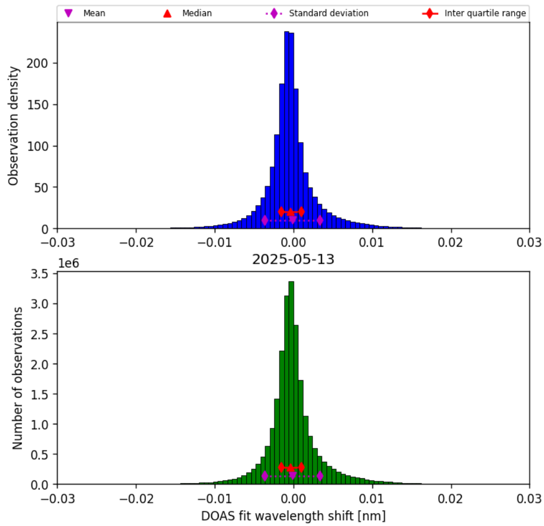
Figure 35: Histogram of “DOAS fit wavelength shift” for 2025-05-13 to 2025-05-13
