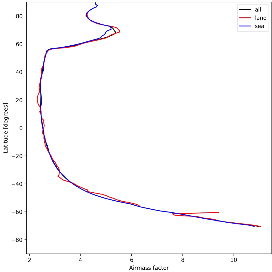
Figure 25: Zonal average of “Airmass factor” for 2025-05-13 to 2025-05-13.
