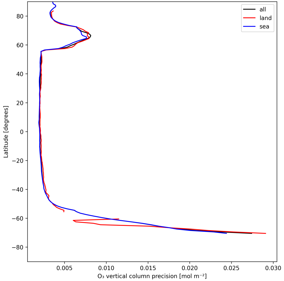
Figure 18: Zonal average of “O 3 vertical column precision” for 2025-05-13 to 2025-05-13.
