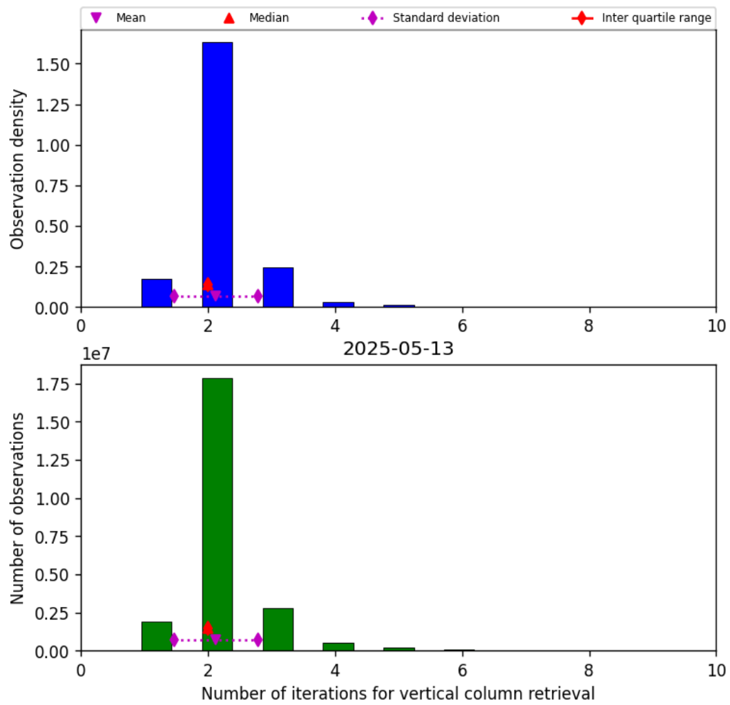
Figure 39: Histogram of “Number of iterations for vertical column retrieval” for 2025-05-13 to 2025-05-13
