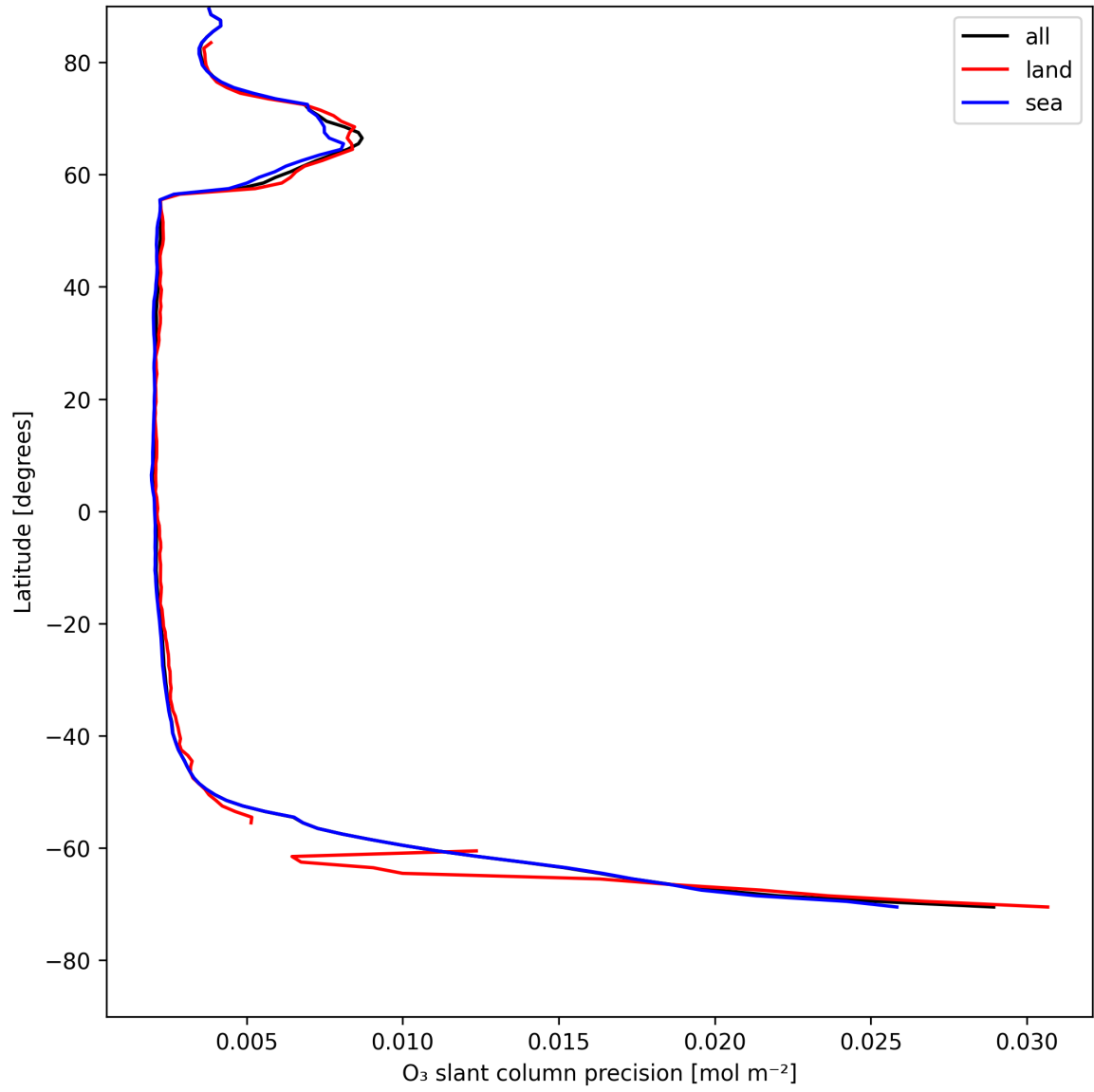
Figure 20: Zonal average of “O 3 slant column precision” for 2025-05-13 to 2025-05-13.
