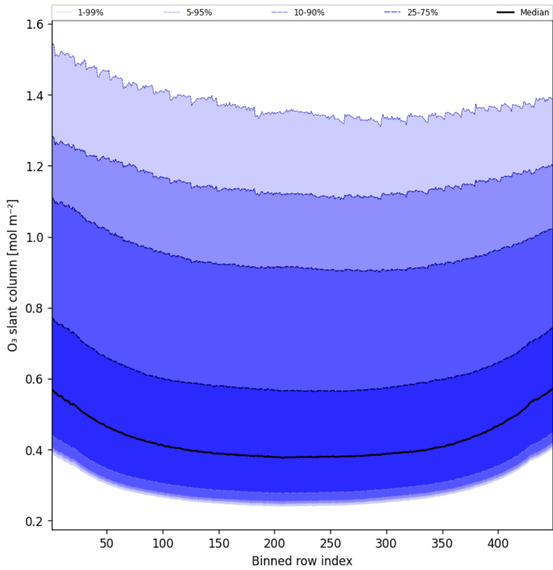
Figure 43: Along track statistics of “O 3 slant column” for 2025-05-13 to 2025-05-13
