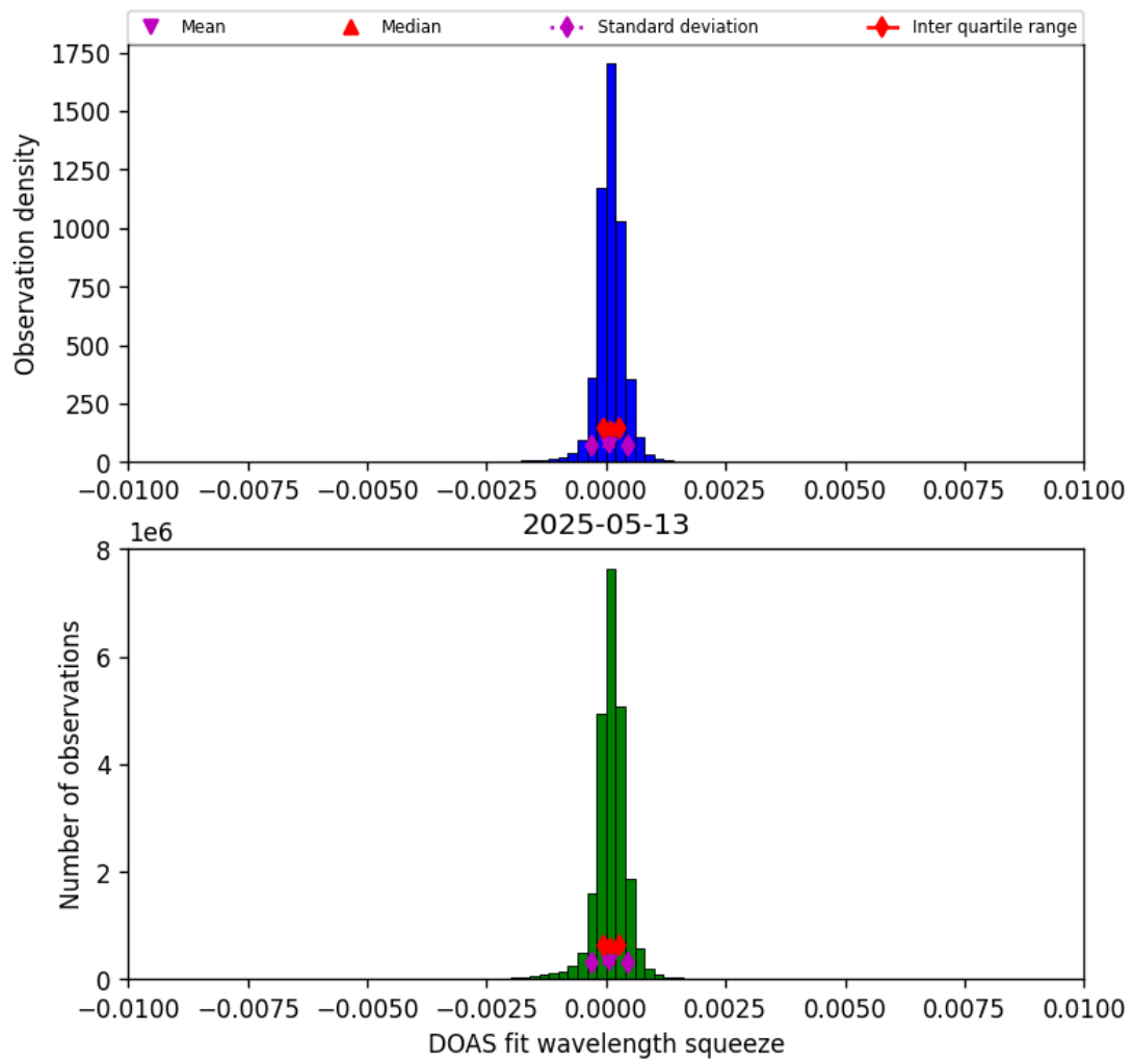
Figure 36: Histogram of “DOAS fit wavelength squeeze” for 2025-05-13 to 2025-05-13
