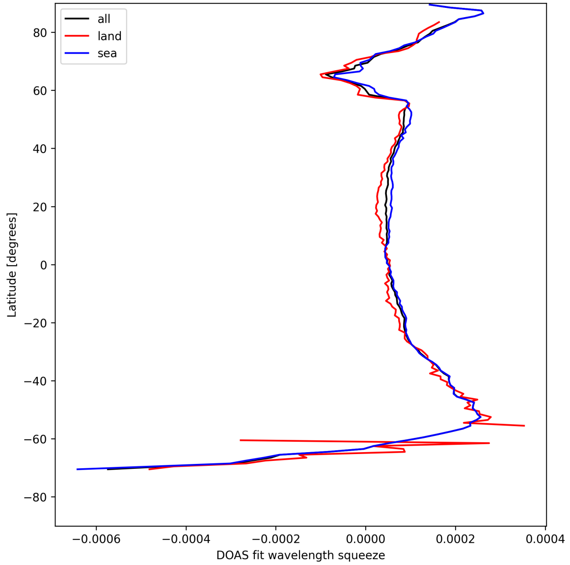
Figure 24: Zonal average of “DOAS fit wavelength squeeze” for 2025-05-13 to 2025-05-13.
