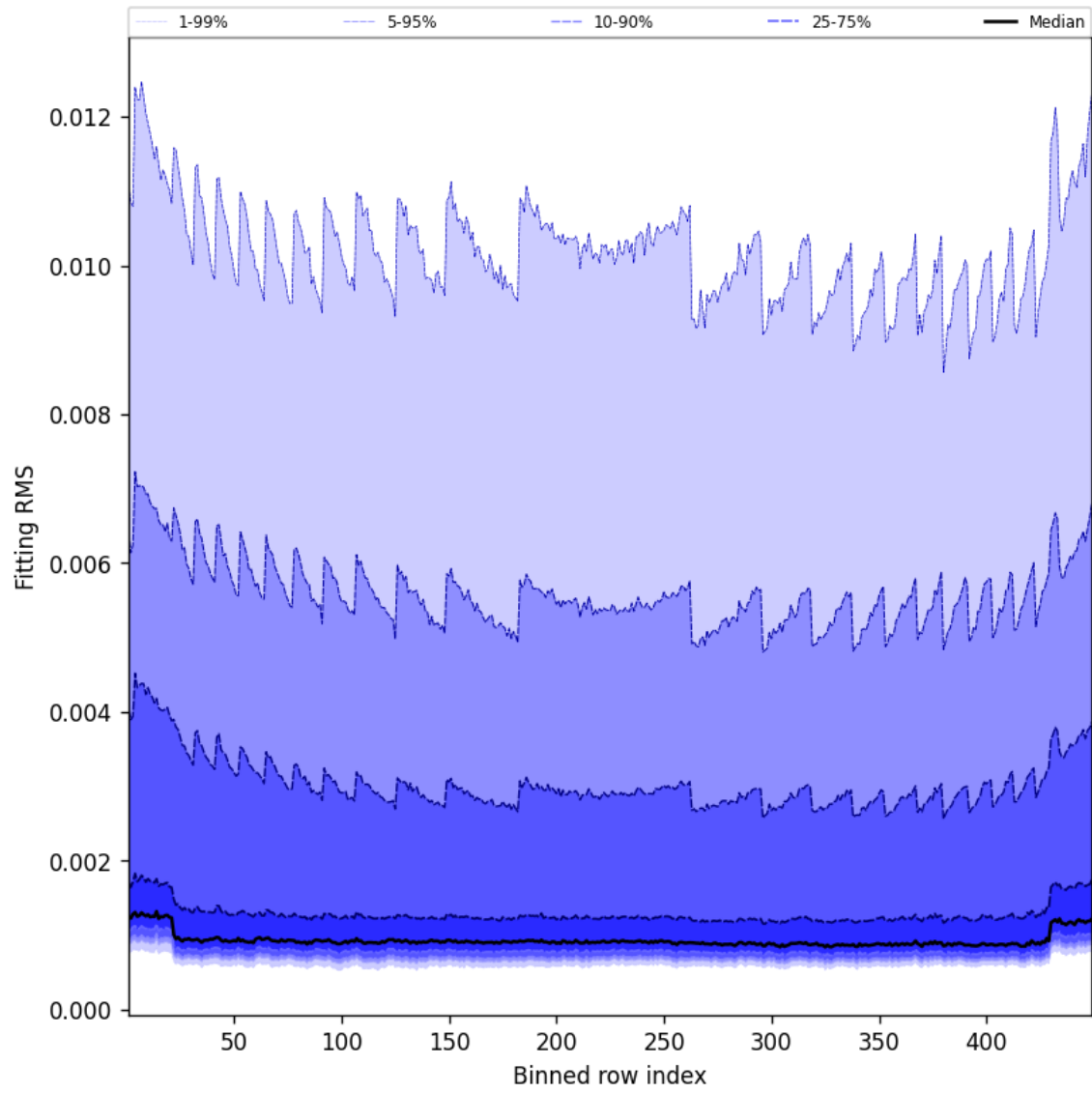
Figure 46: Along track statistics of “Fitting RMS” for 2025-05-13 to 2025-05-13
