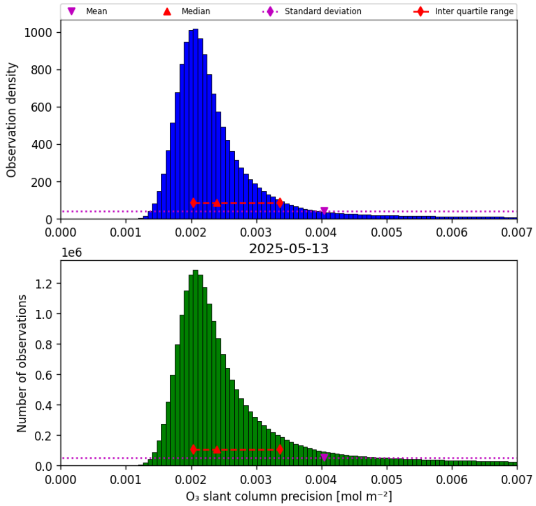
Figure 32: Histogram of "O 3 slant column precision" for 2025-05-13 to 2025-05-13
