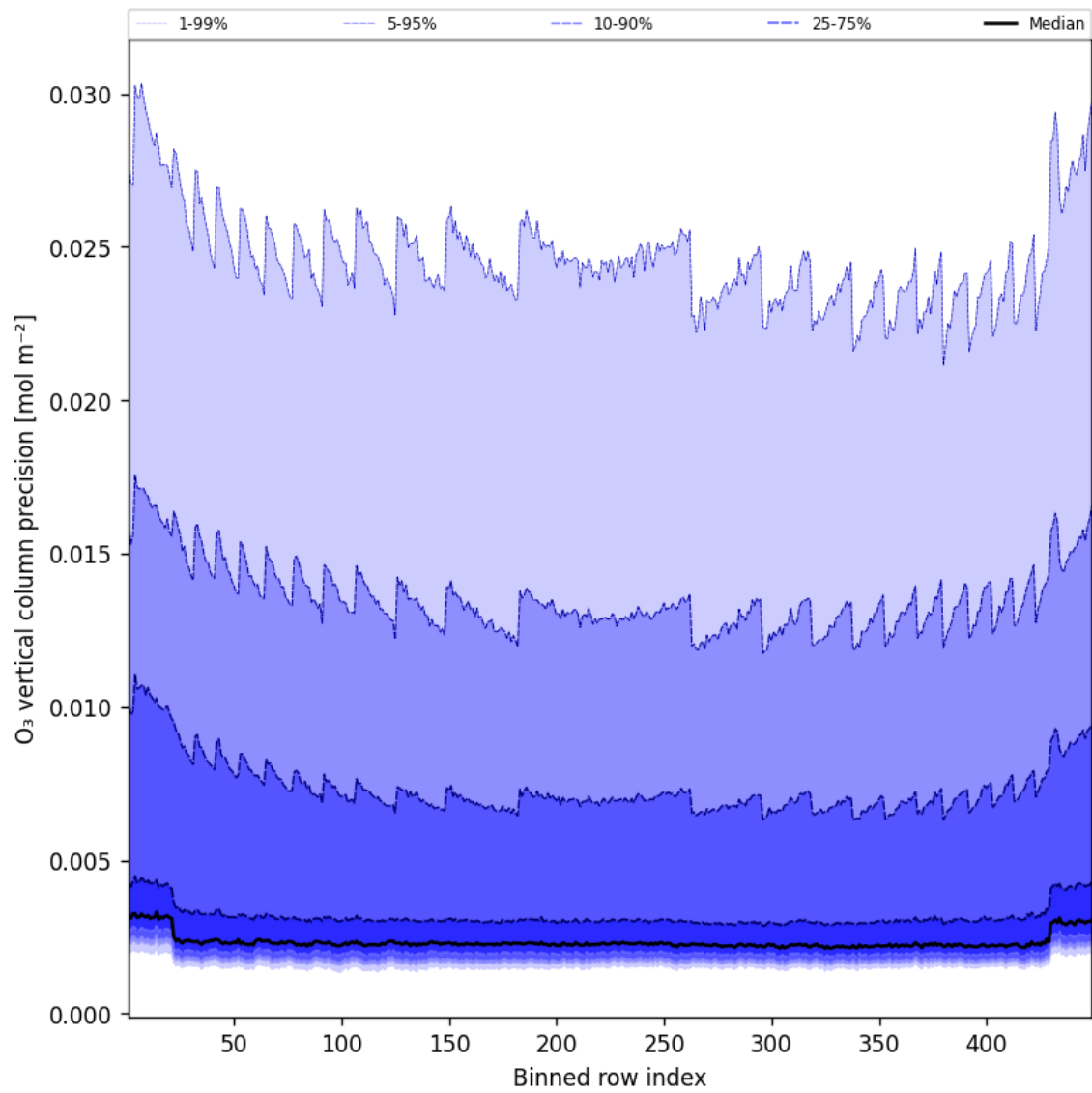
Figure 42: Along track statistics of “O 3 vertical column precision” for 2025-05-13 to 2025-05-13
