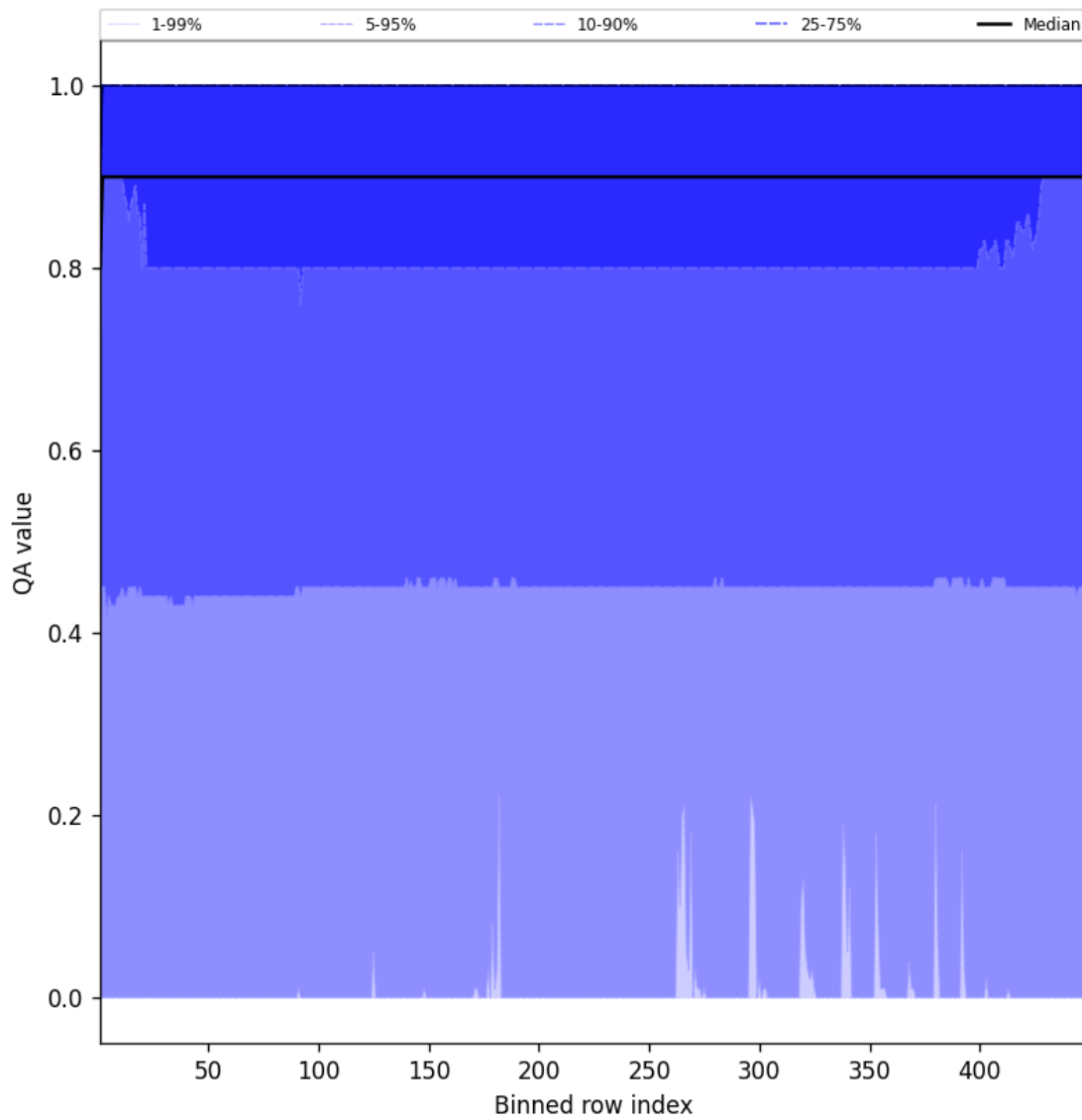
Figure 40: Along track statistics of “QA value” for 2025-05-13 to 2025-05-13
