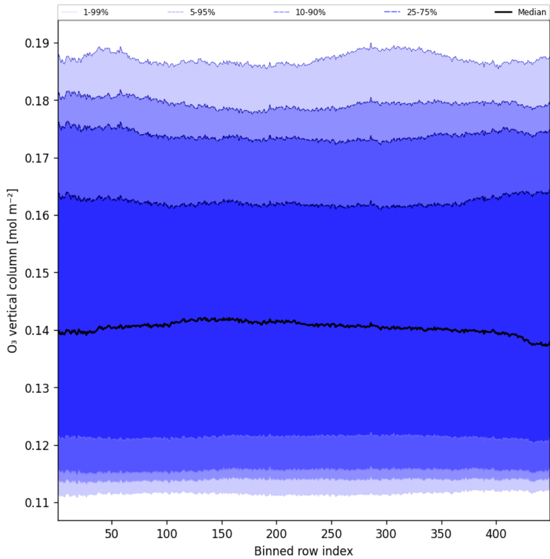
Figure 41: Along track statistics of “ O_3 vertical column” for 2025-05-13 to 2025-05-13
