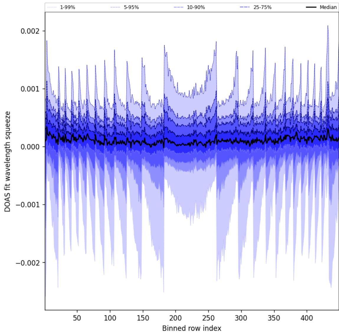
Figure 48: Along track statistics of “DOAS fit wavelength squeeze” for 2025-05-13 to 2025-05-13
