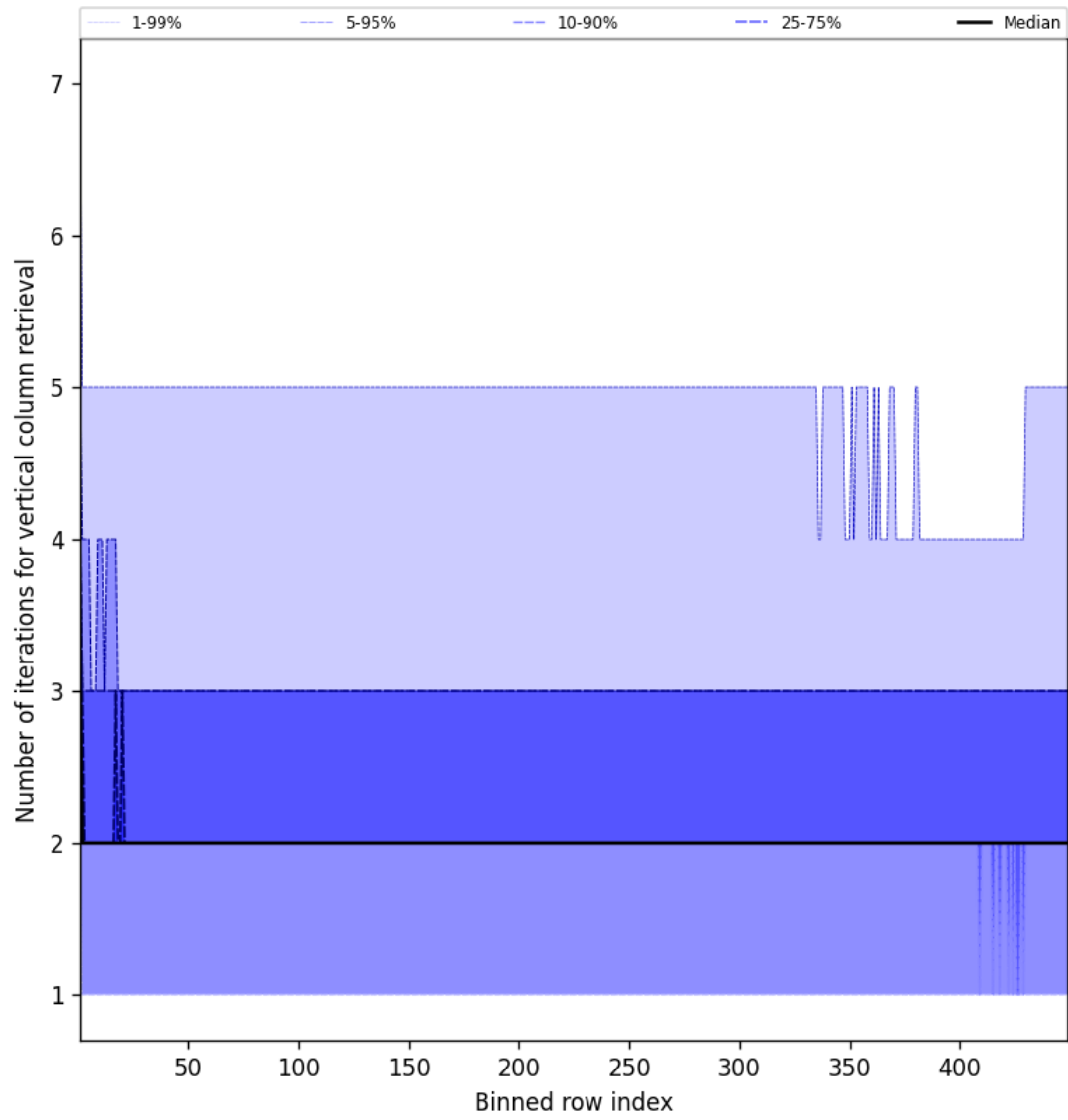
Figure 51: Along track statistics of “Number of iterations for vertical column retrieval” for 2025-05-13 to 2025-05-13
