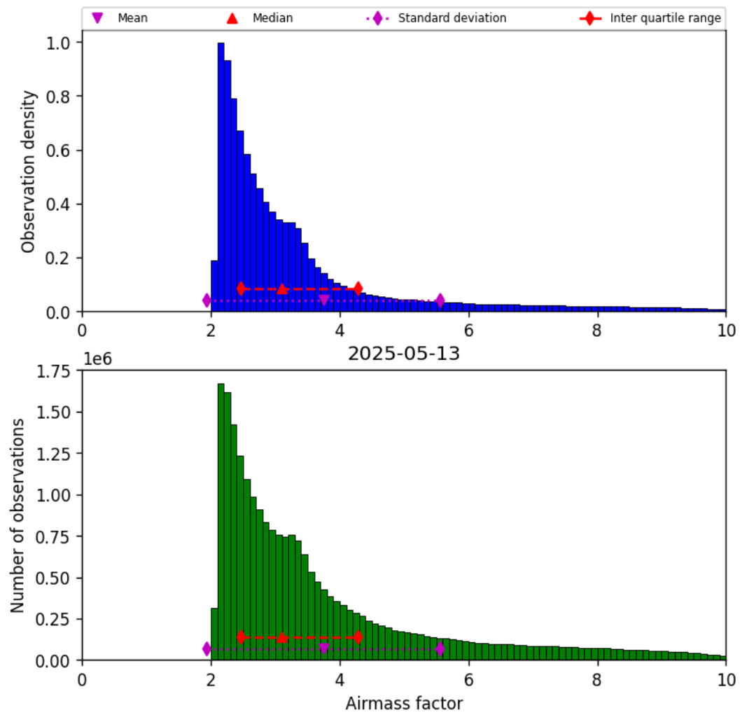
Figure 37: Histogram of “Airmass factor” for 2025-05-13 to 2025-05-13
