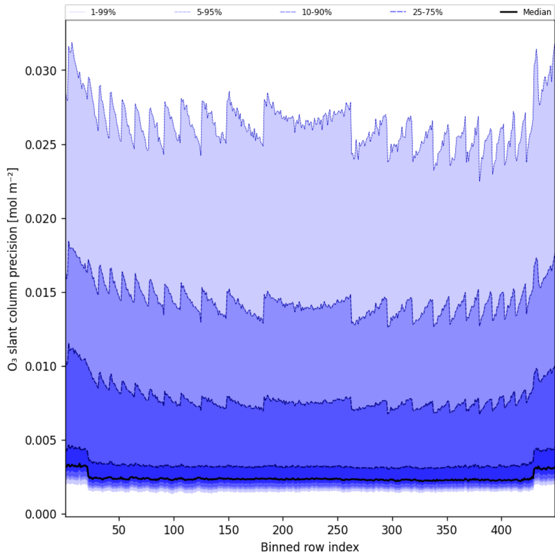
Figure 44: Along track statistics of “O 3 slant column precision” for 2025-05-13 to 2025-05-13
