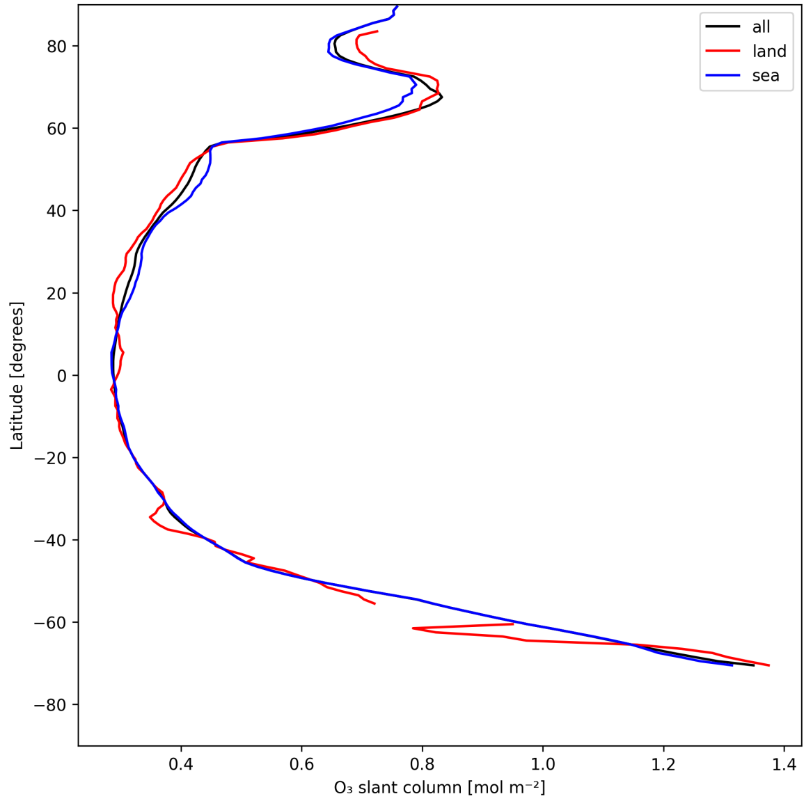
Figure 19: Zonal average of “O 3 slant column” for 2025-05-13 to 2025-05-13.
