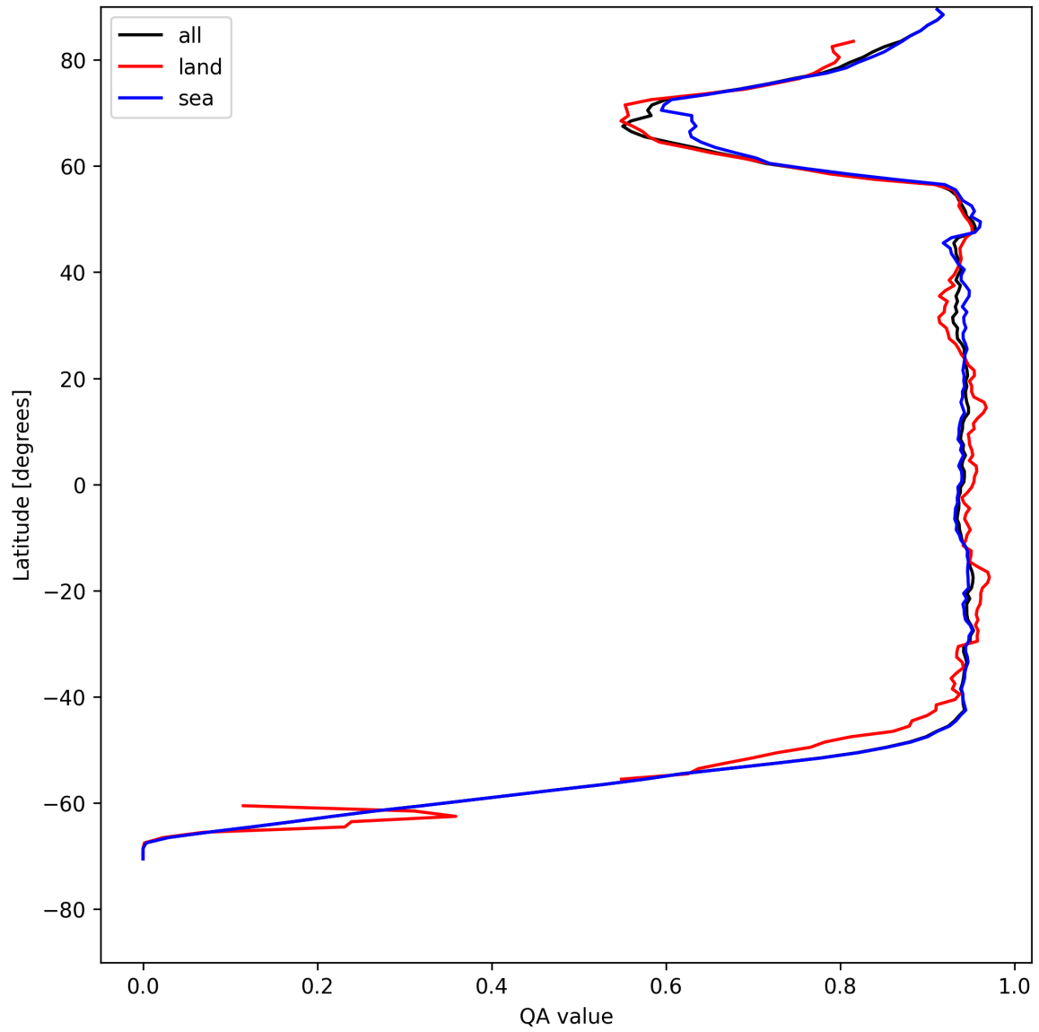
Figure 16: Zonal average of “QA value” for 2025-05-13 to 2025-05-13.
