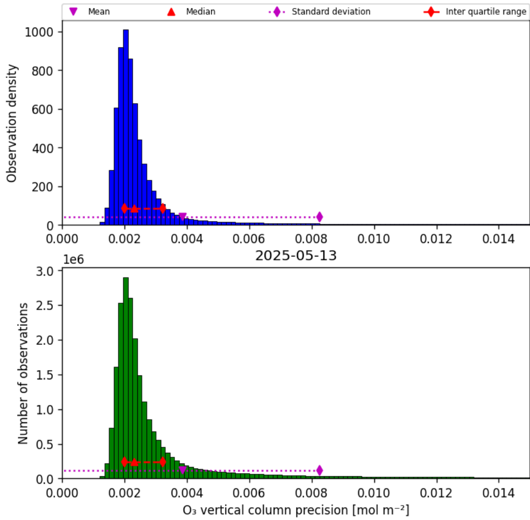
Figure 30: Histogram of “O 3 vertical column precision” for 2025-05-13 to 2025-05-13
