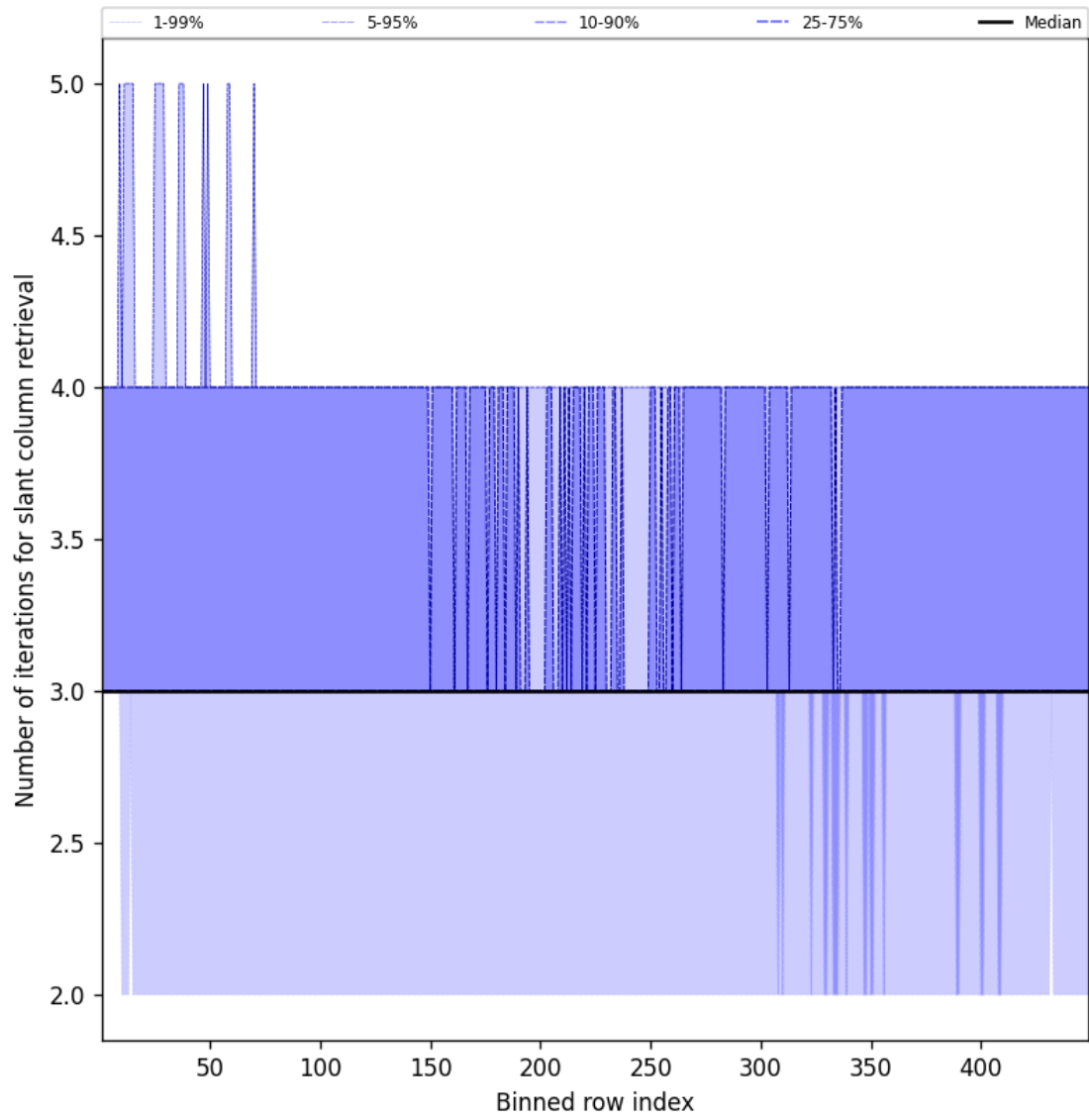
Figure 45: Along track statistics of “Number of iterations for slant column retrieval” for 2025-05-13 to 2025-05-13
