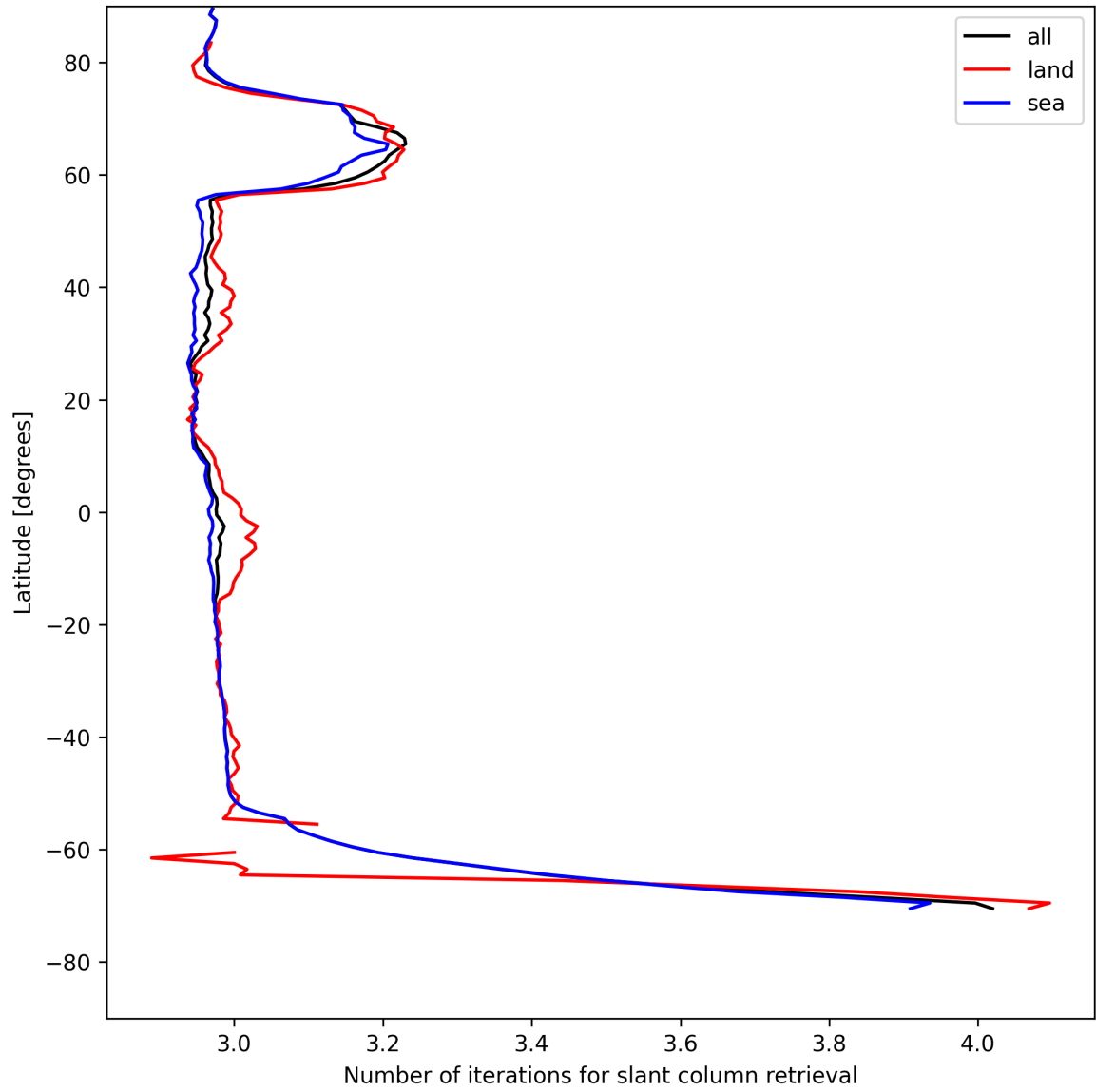
Figure 21: Zonal average of “Number of iterations for slant column retrieval” for 2025-05-13 to 2025-05-13.
