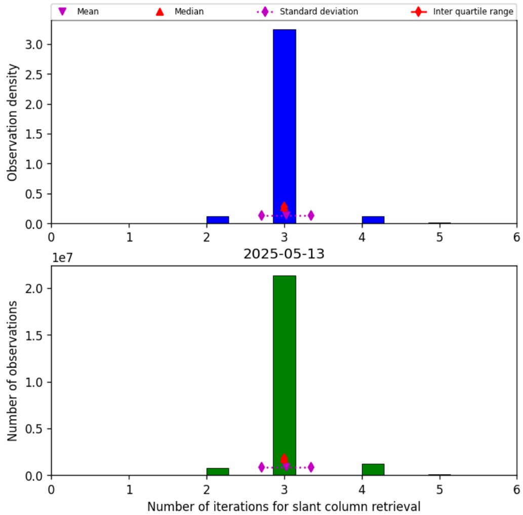
Figure 33: Histogram of “Number of iterations for slant column retrieval” for 2025-05-13 to 2025-05-13
