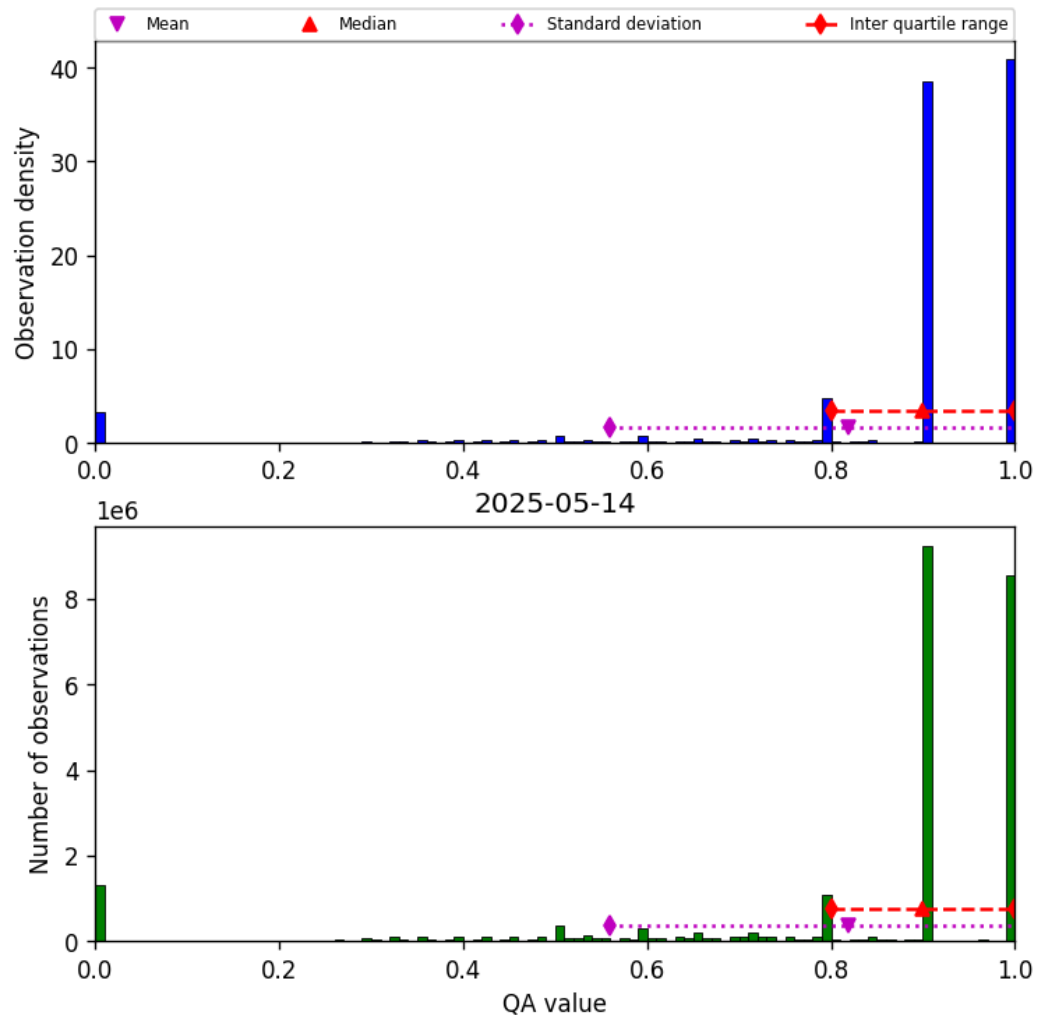
Figure 28: Histogram of “QA value” for 2025-05-14 to 2025-05-15
