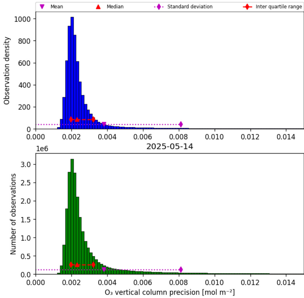
Figure 30: Histogram of “O 3 vertical column precision” for 2025-05-14 to 2025-05-15
