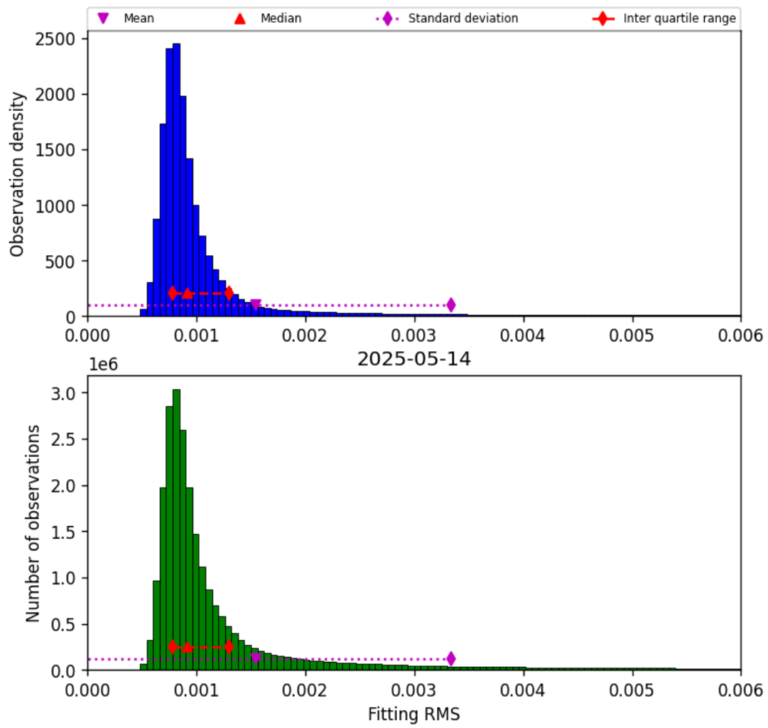
Figure 34: Histogram of “Fitting RMS” for 2025-05-14 to 2025-05-15
