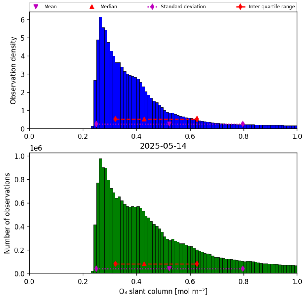
Figure 31: Histogram of “O 3 slant column” for 2025-05-14 to 2025-05-15
