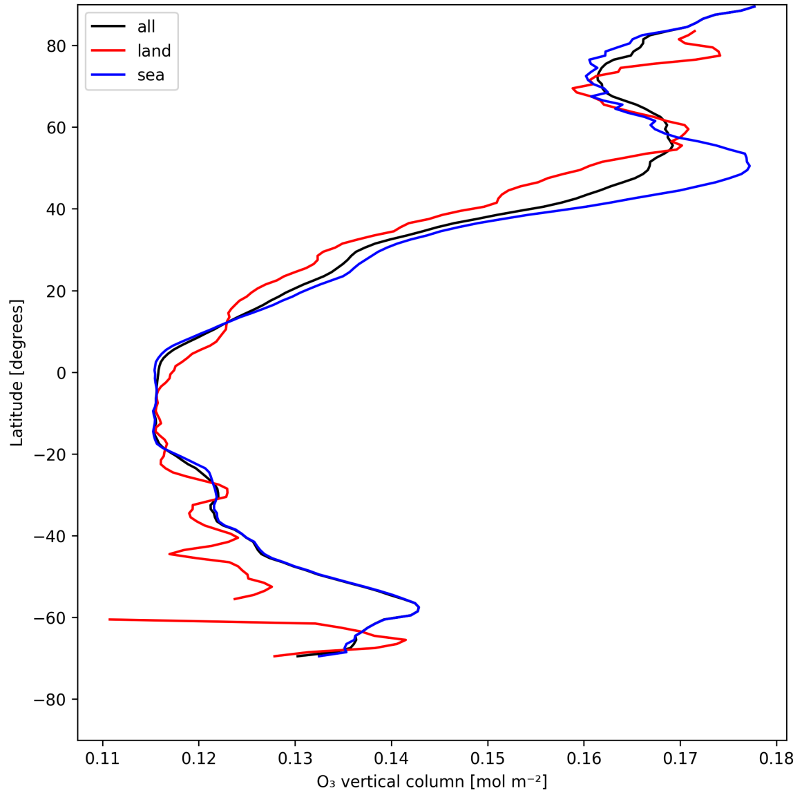
Figure 17: Zonal average of “O 3 vertical column” for 2025-05-14 to 2025-05-15.
