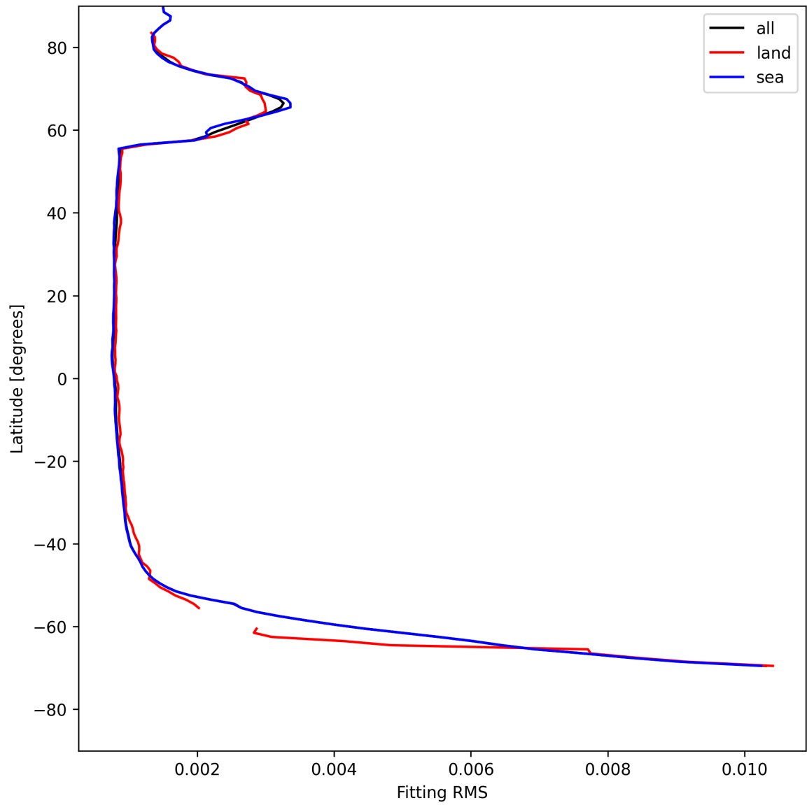
Figure 22: Zonal average of “Fitting RMS” for 2025-05-14 to 2025-05-15.
