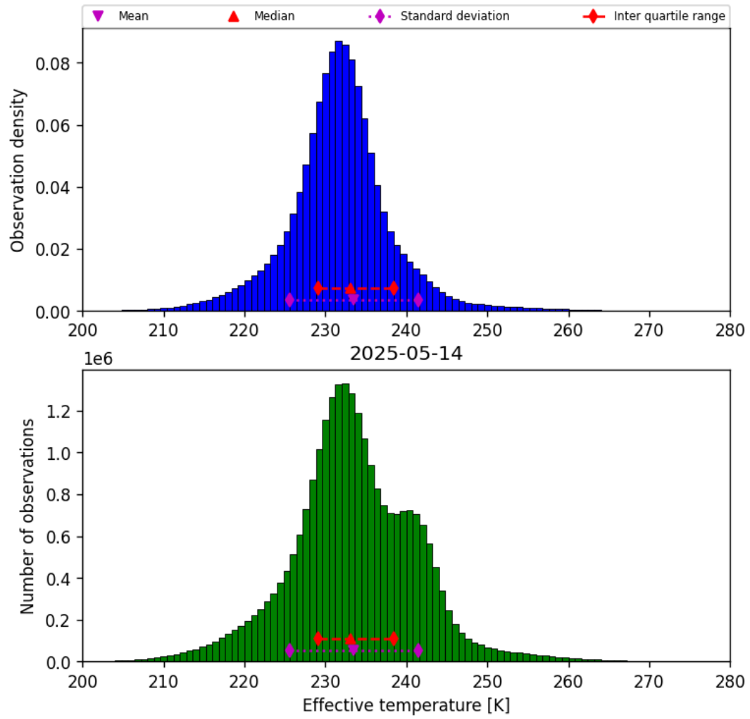
Figure 38: Histogram of “Effective temperature” for 2025-05-14 to 2025-05-15
