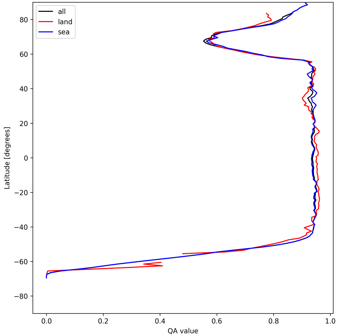
Figure 16: Zonal average of “QA value” for 2025-05-14 to 2025-05-15.
