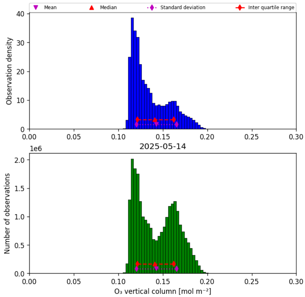
Figure 29: Histogram of “O 3 vertical column” for 2025-05-14 to 2025-05-15
