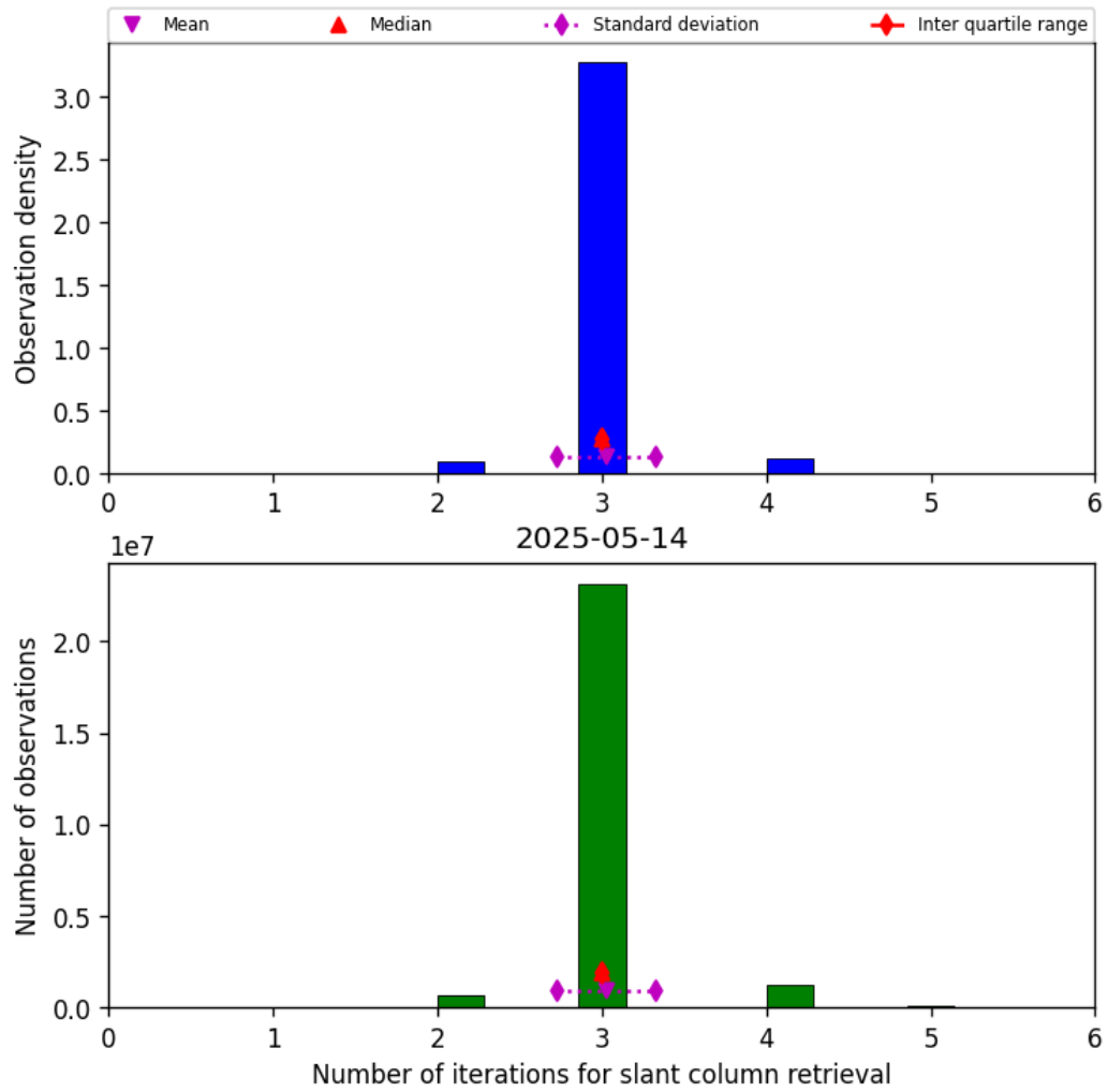
Figure 33: Histogram of “Number of iterations for slant column retrieval” for 2025-05-14 to 2025-05-15
