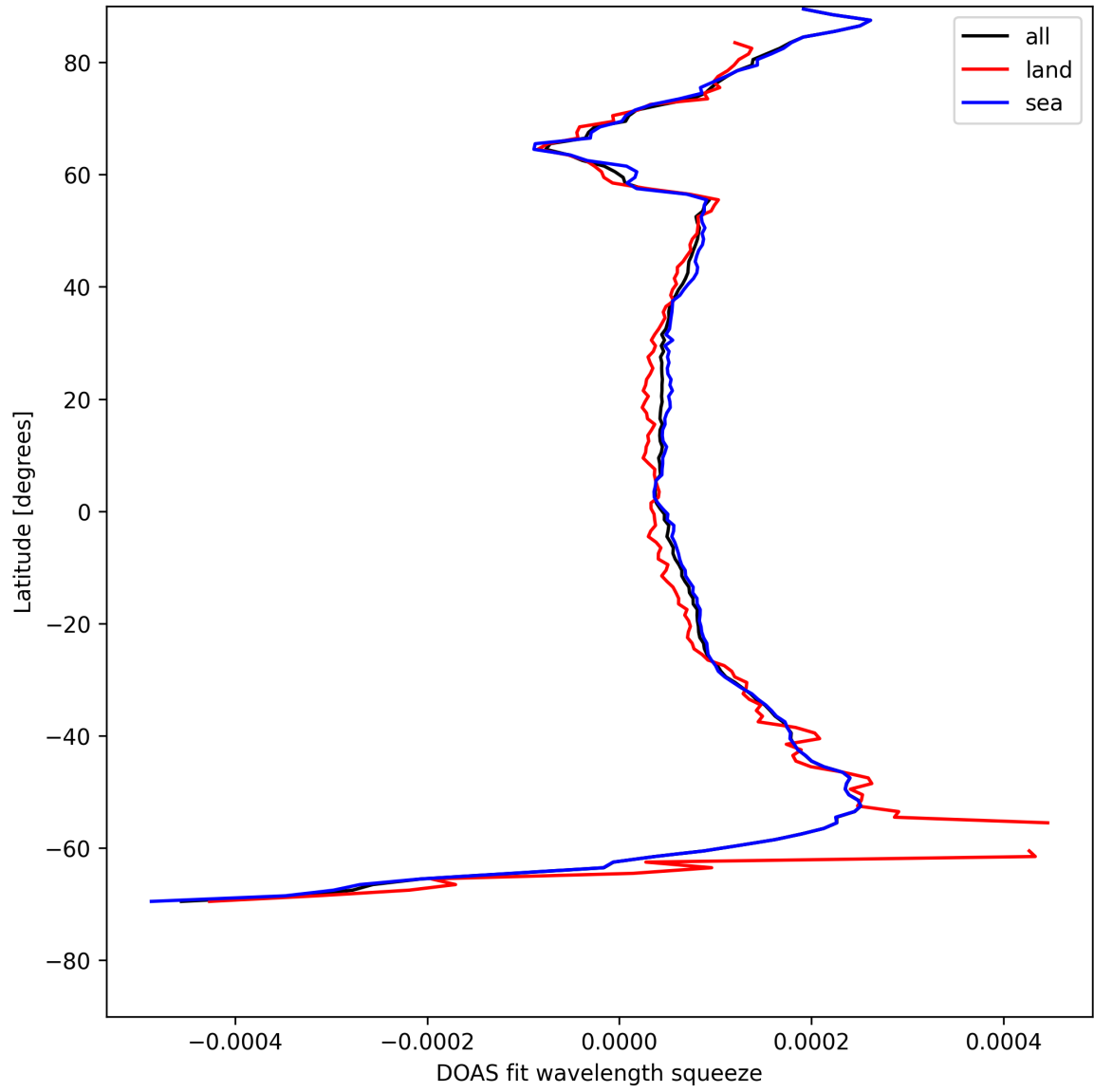
Figure 24: Zonal average of “DOAS fit wavelength squeeze” for 2025-05-14 to 2025-05-15.
