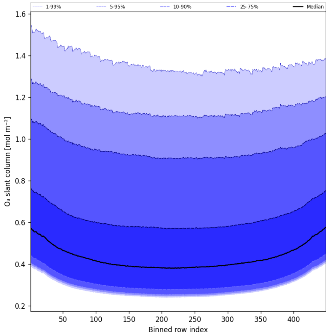
Figure 43: Along track statistics of “O 3 slant column” for 2025-05-14 to 2025-05-15
