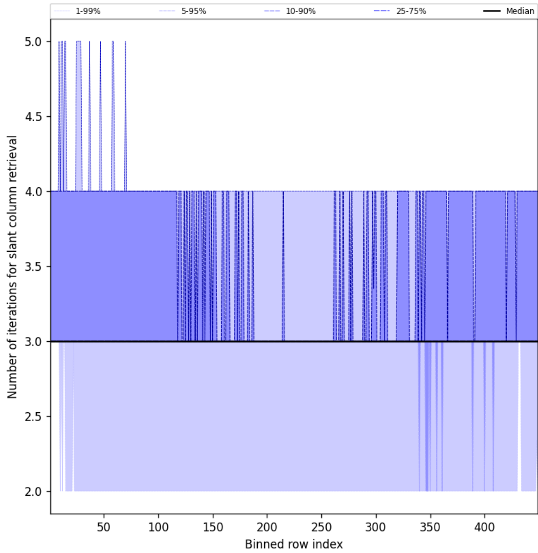
Figure 45: Along track statistics of “Number of iterations for slant column retrieval” for 2025-05-14 to 2025-05-15
