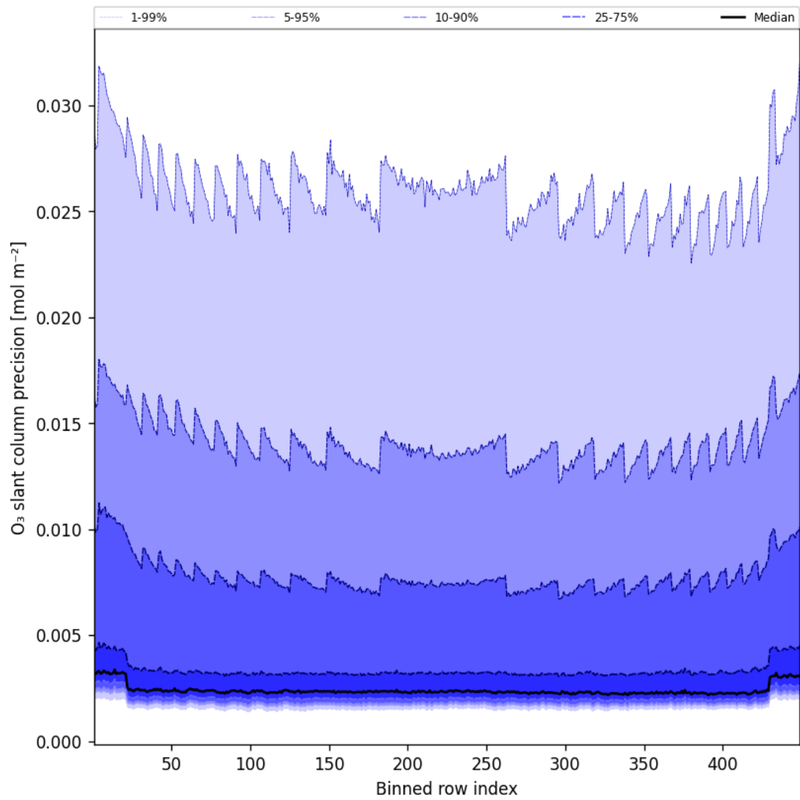
Figure 44: Along track statistics of “O 3 slant column precision” for 2025-05-14 to 2025-05-15
