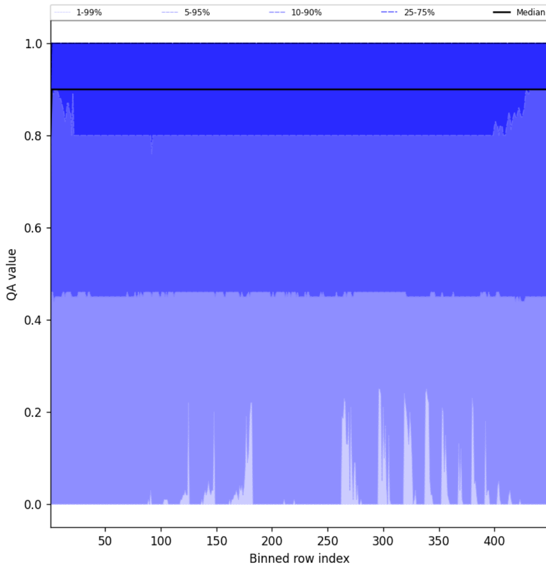
Figure 40: Along track statistics of “QA value” for 2025-05-14 to 2025-05-15
