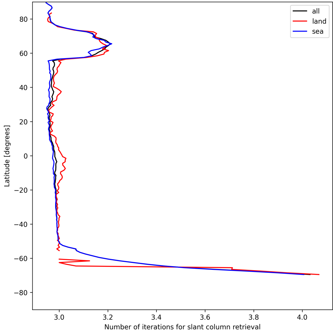
Figure 21: Zonal average of “Number of iterations for slant column retrieval” for 2025-05-14 to 2025-05-15.
