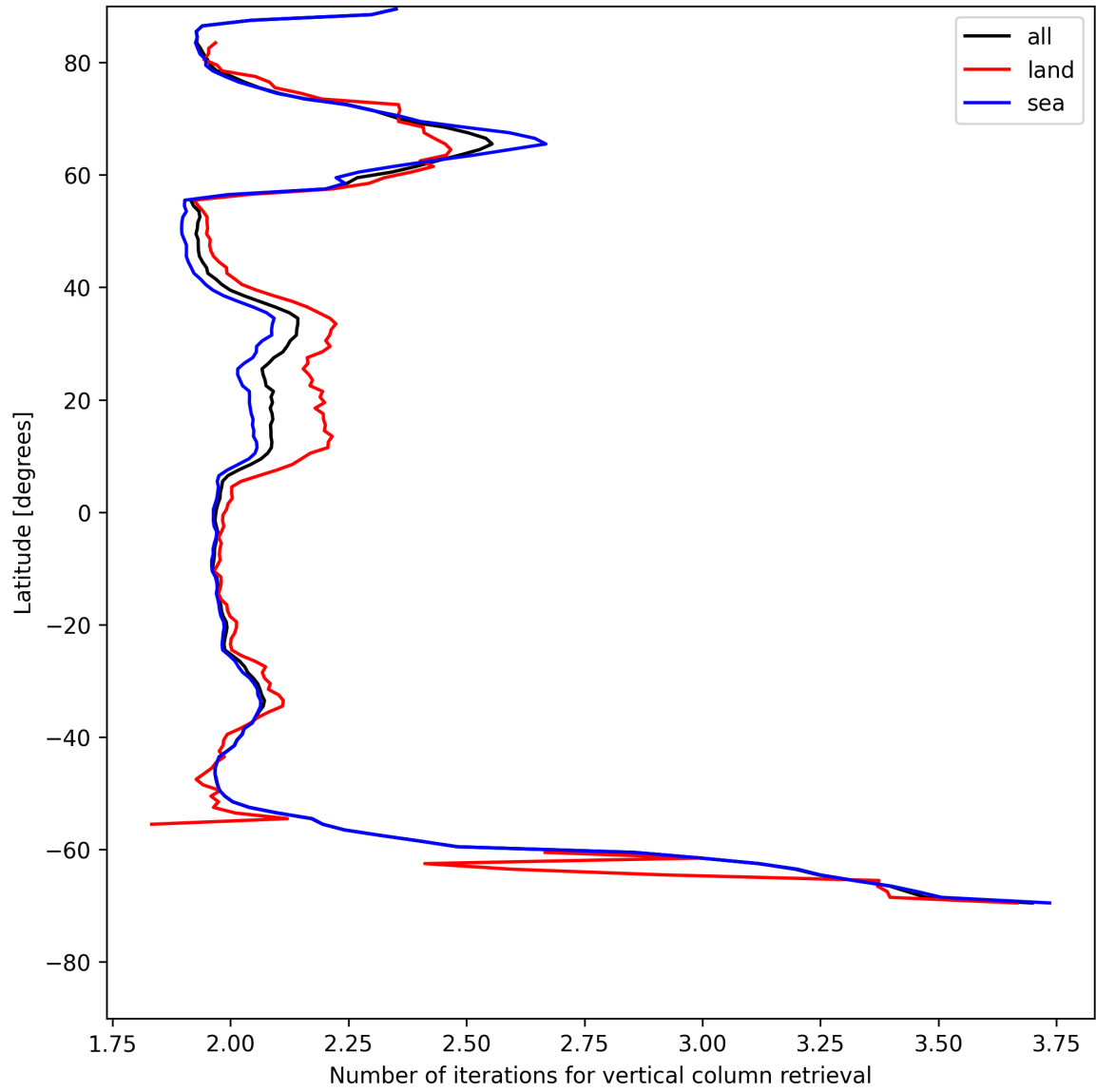
Figure 27: Zonal average of “Number of iterations for vertical column retrieval” for 2025-05-14 to 2025-05-15.
