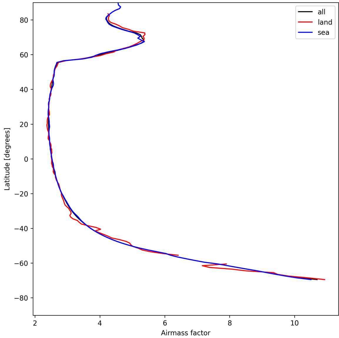
Figure 25: Zonal average of “Airmass factor” for 2025-05-14 to 2025-05-15.
