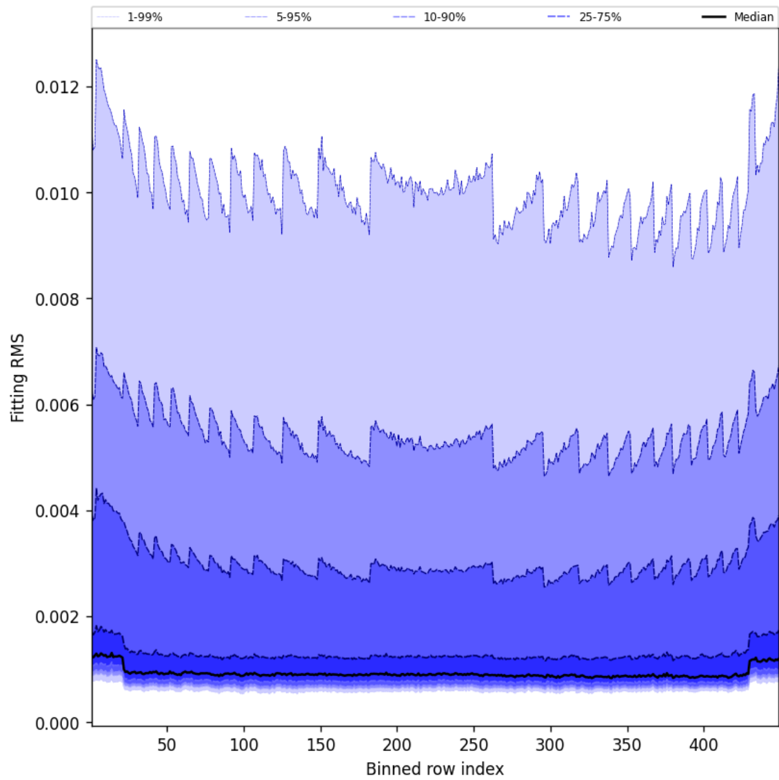
Figure 46: Along track statistics of “Fitting RMS” for 2025-05-14 to 2025-05-15
