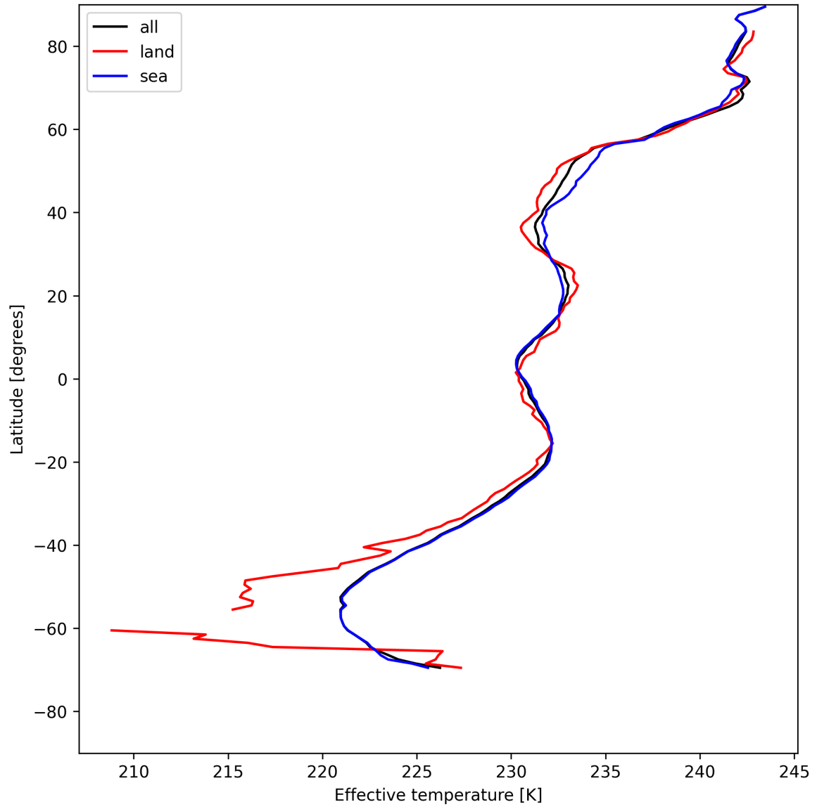
Figure 26: Zonal average of “Effective temperature” for 2025-05-14 to 2025-05-15.
