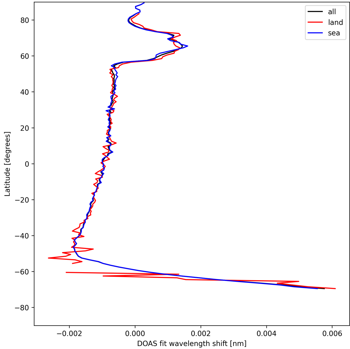
Figure 23: Zonal average of “DOAS fit wavelength shift” for 2025-05-14 to 2025-05-15.
