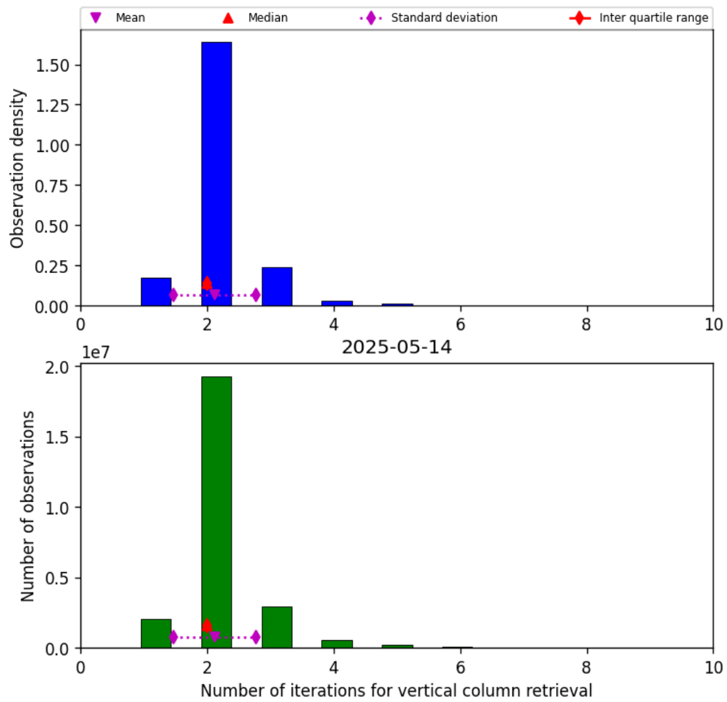
Figure 39: Histogram of “Number of iterations for vertical column retrieval” for 2025-05-14 to 2025-05-15
