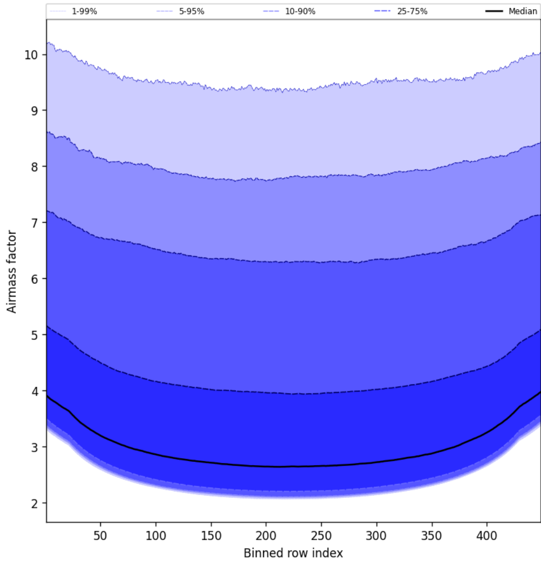
Figure 49: Along track statistics of “Airmass factor” for 2025-05-14 to 2025-05-15
