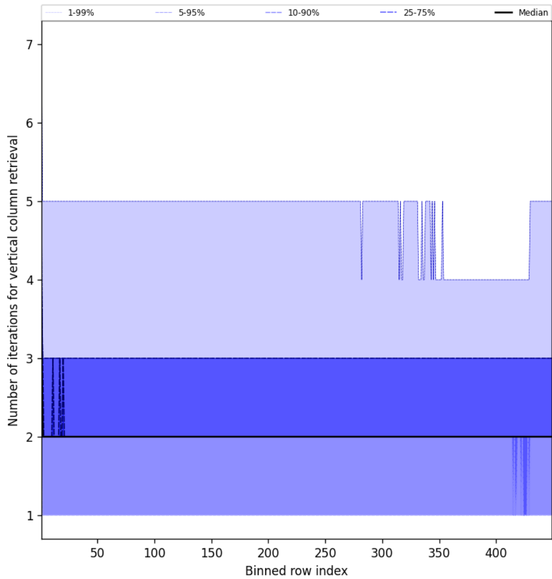
Figure 51: Along track statistics of “Number of iterations for vertical column retrieval” for 2025-05-14 to 2025-05-15
