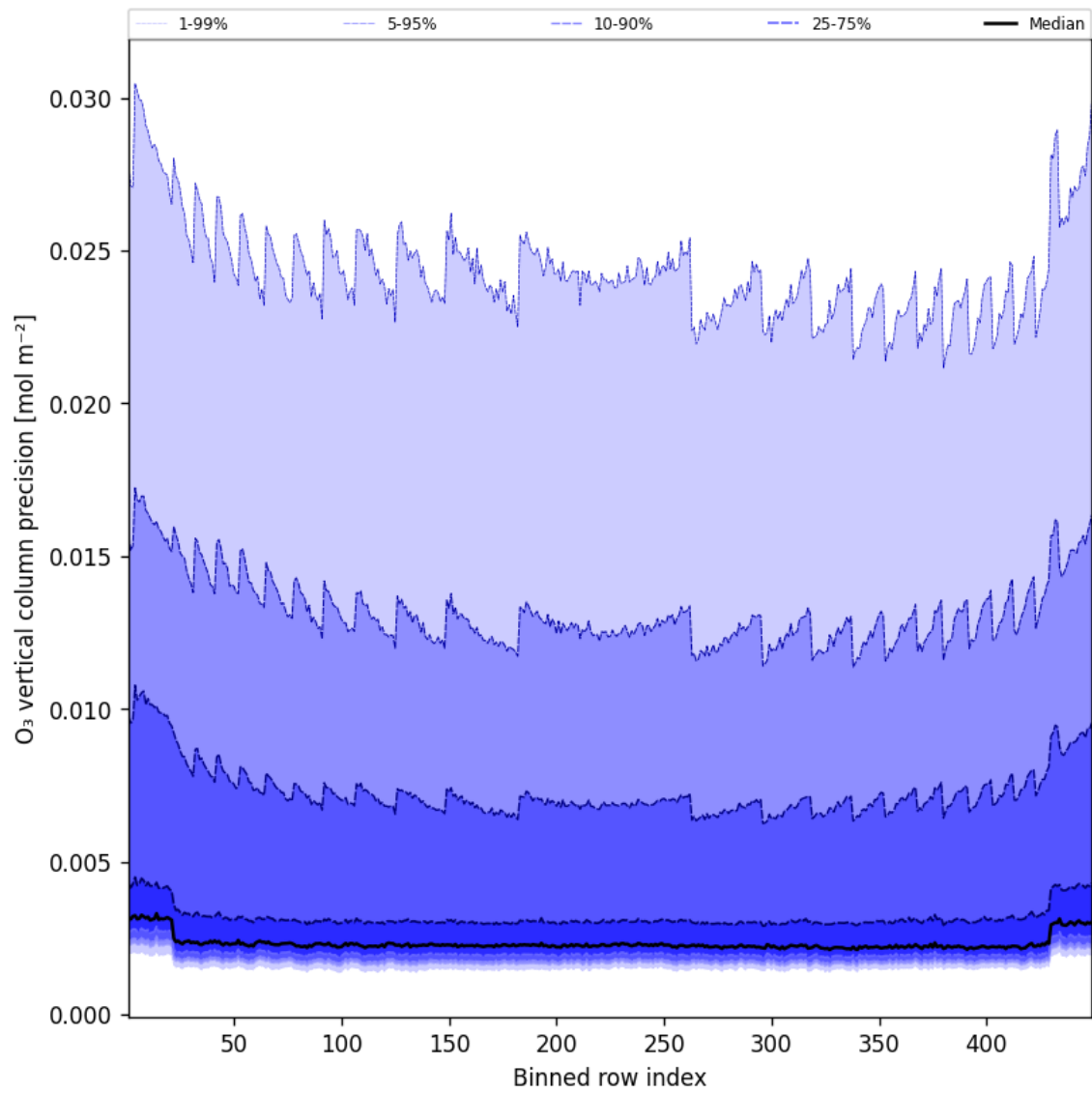
Figure 42: Along track statistics of “O 3 vertical column precision” for 2025-05-14 to 2025-05-15
