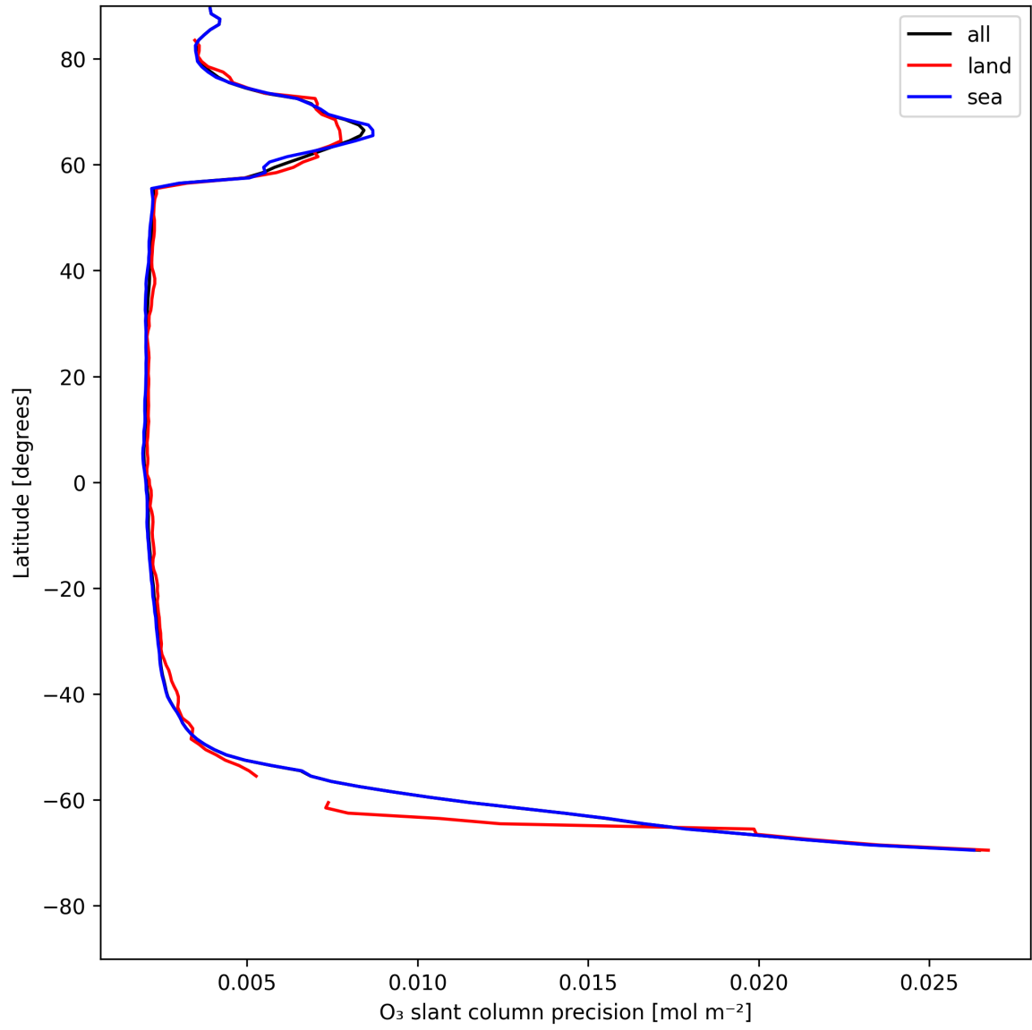
Figure 20: Zonal average of “O 3 slant column precision” for 2025-05-14 to 2025-05-15.
