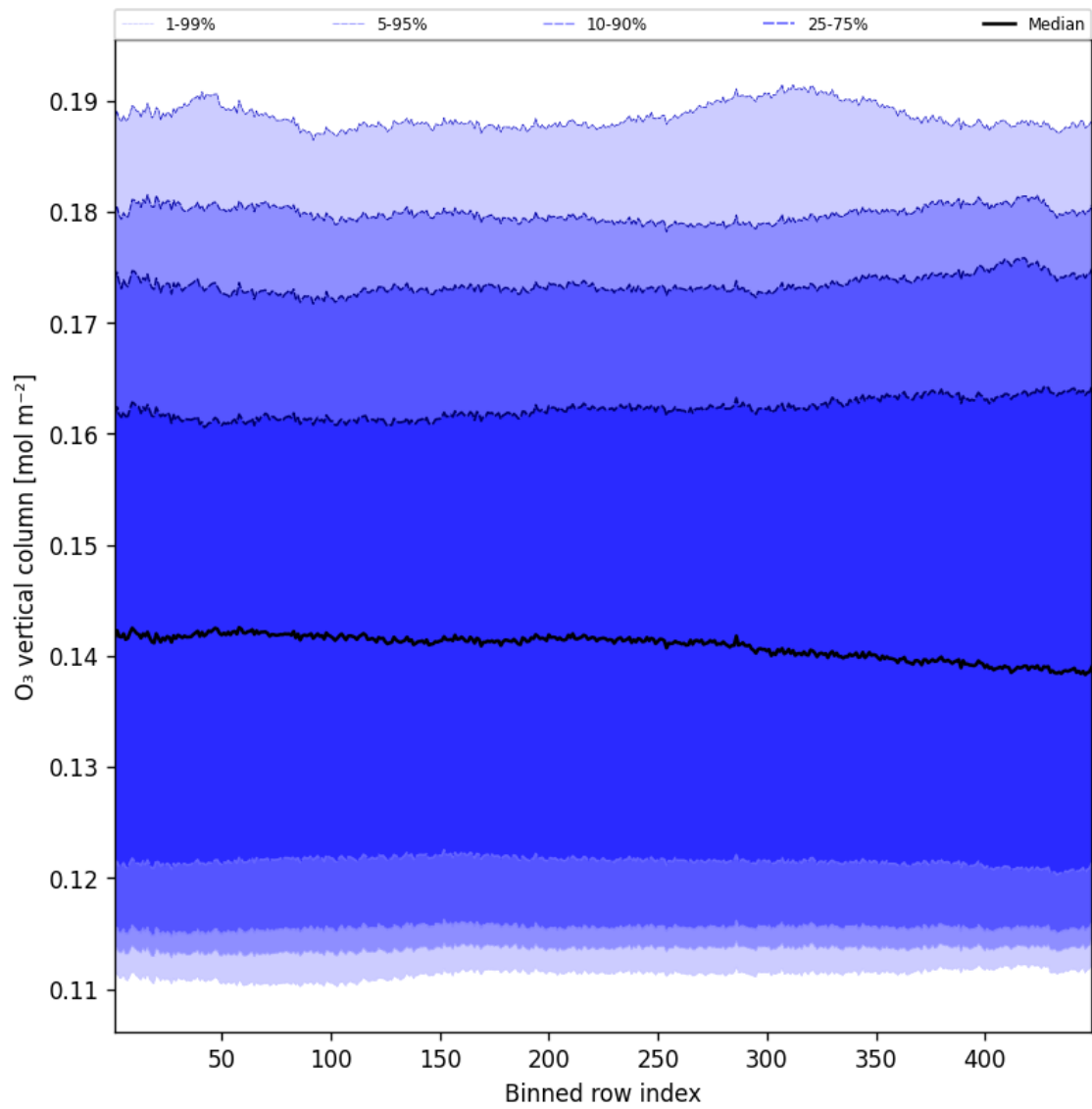
Figure 41: Along track statistics of “O 3 vertical column” for 2025-05-14 to 2025-05-15
