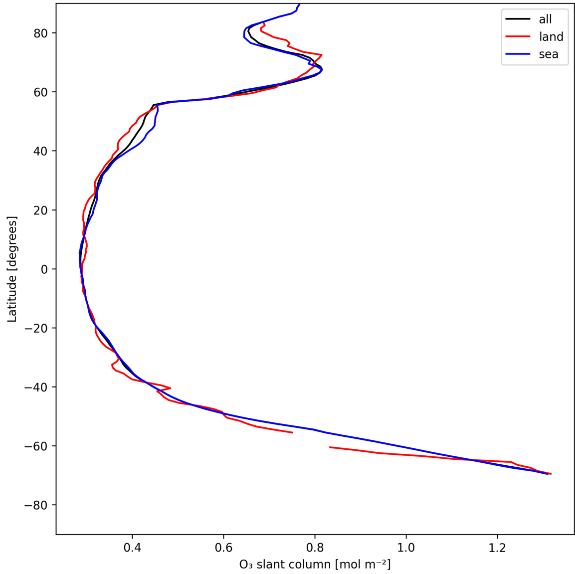
Figure 19: Zonal average of “O 3 slant column” for 2025-05-14 to 2025-05-15.
