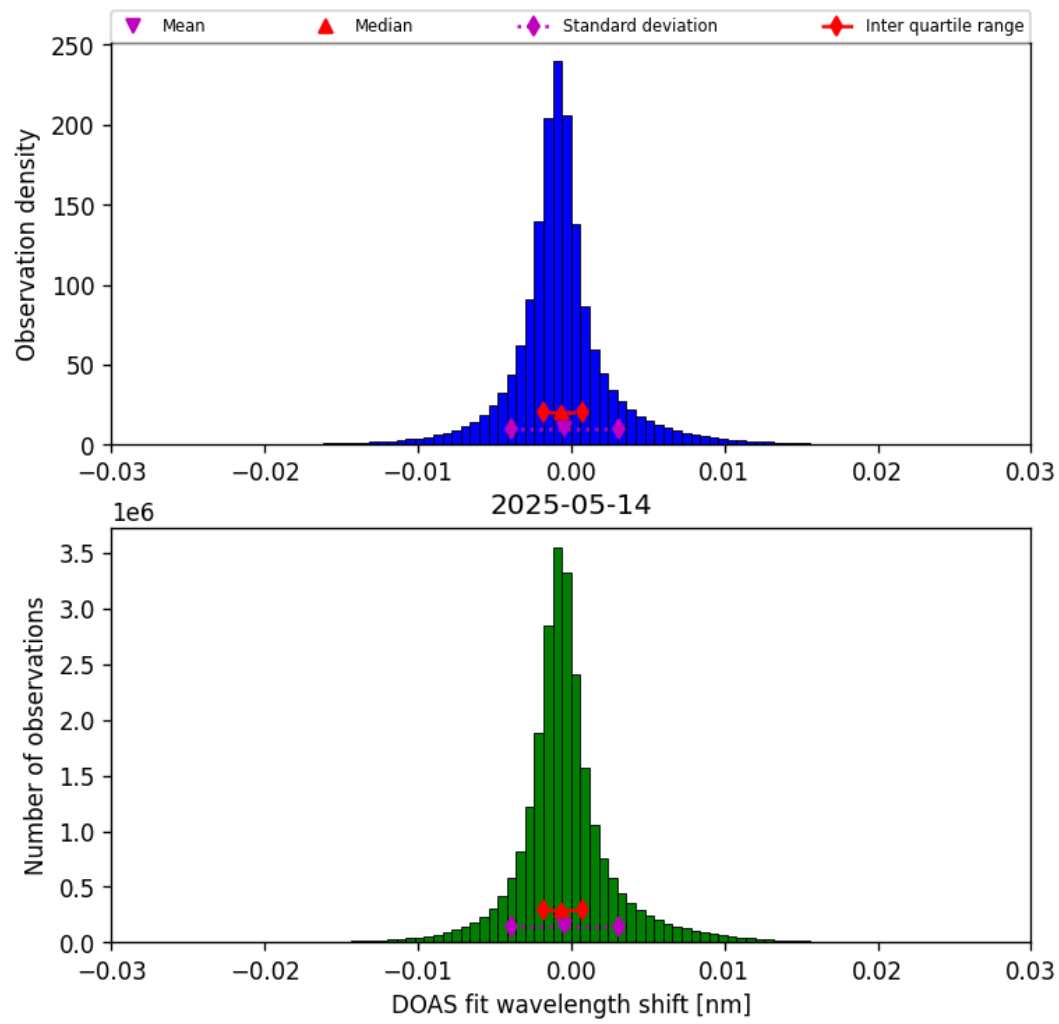
Figure 35: Histogram of “DOAS fit wavelength shift” for 2025-05-14 to 2025-05-15
