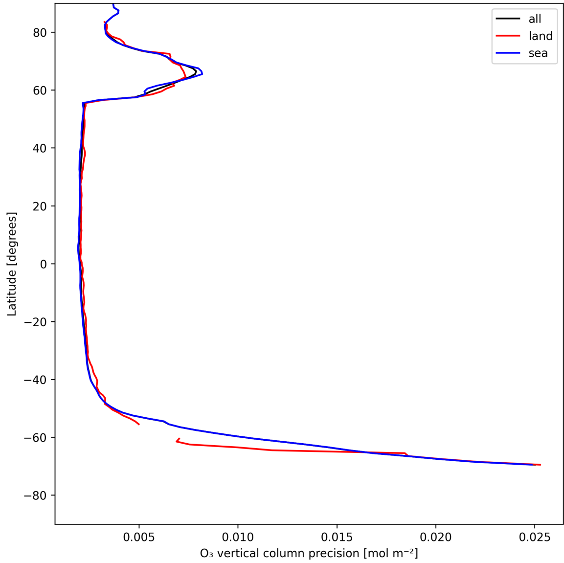
Figure 18: Zonal average of “O 3 vertical column precision” for 2025-05-14 to 2025-05-15.
