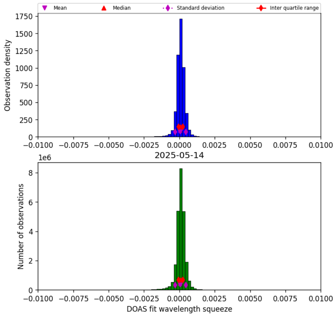
Figure 36: Histogram of “DOAS fit wavelength squeeze” for 2025-05-14 to 2025-05-15
