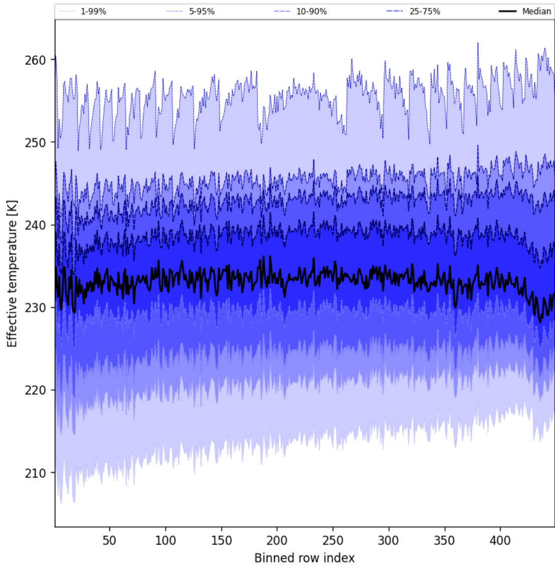
Figure 50: Along track statistics of “Effective temperature” for 2025-05-14 to 2025-05-15
