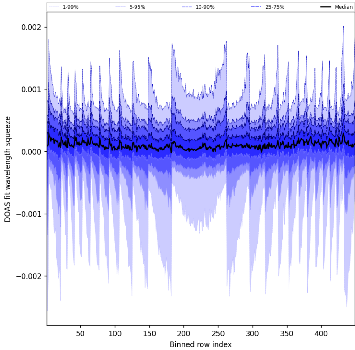
Figure 48: Along track statistics of “DOAS fit wavelength squeeze” for 2025-05-14 to 2025-05-15
