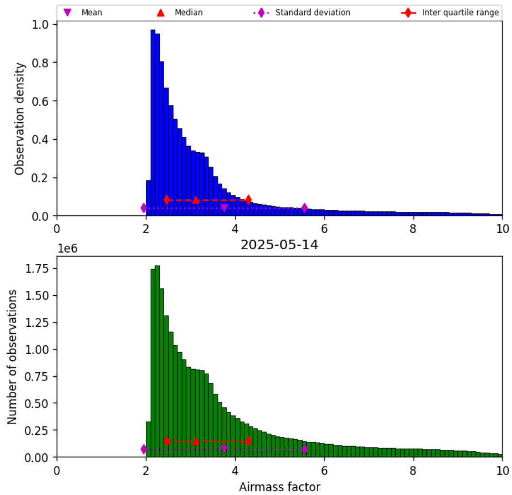
Figure 37: Histogram of “Airmass factor” for 2025-05-14 to 2025-05-15
