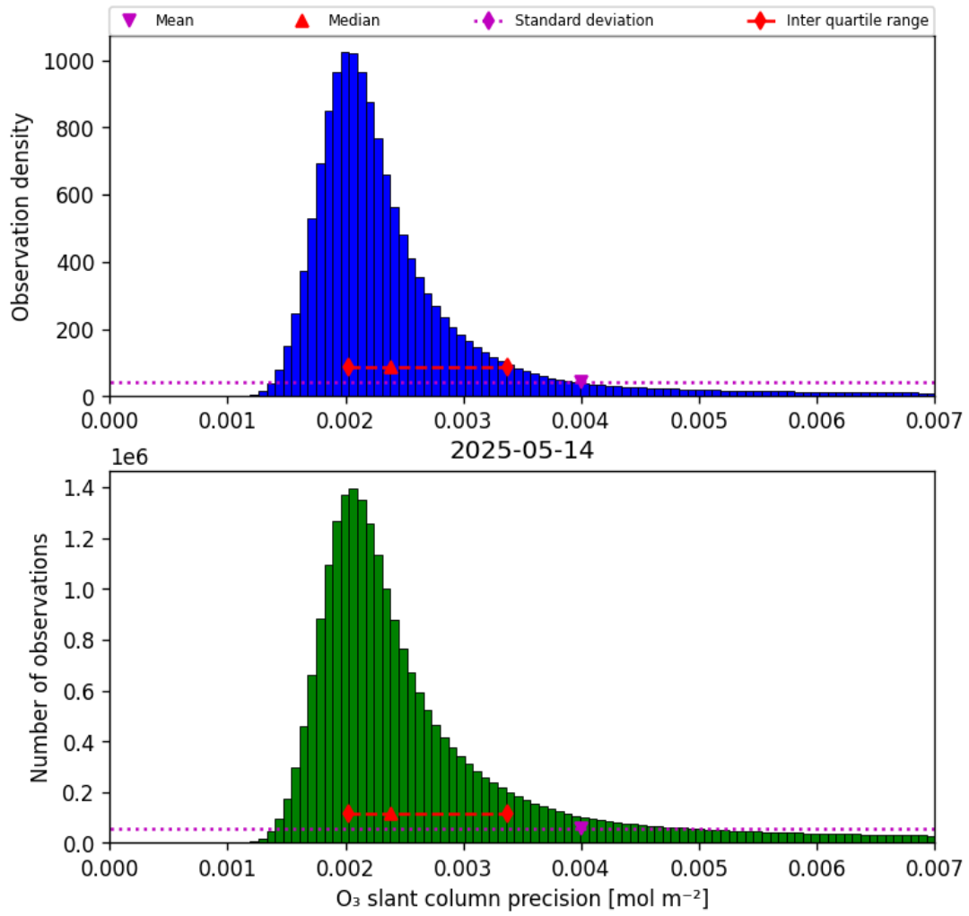
Figure 32: Histogram of “O 3 slant column precision” for 2025-05-14 to 2025-05-15
