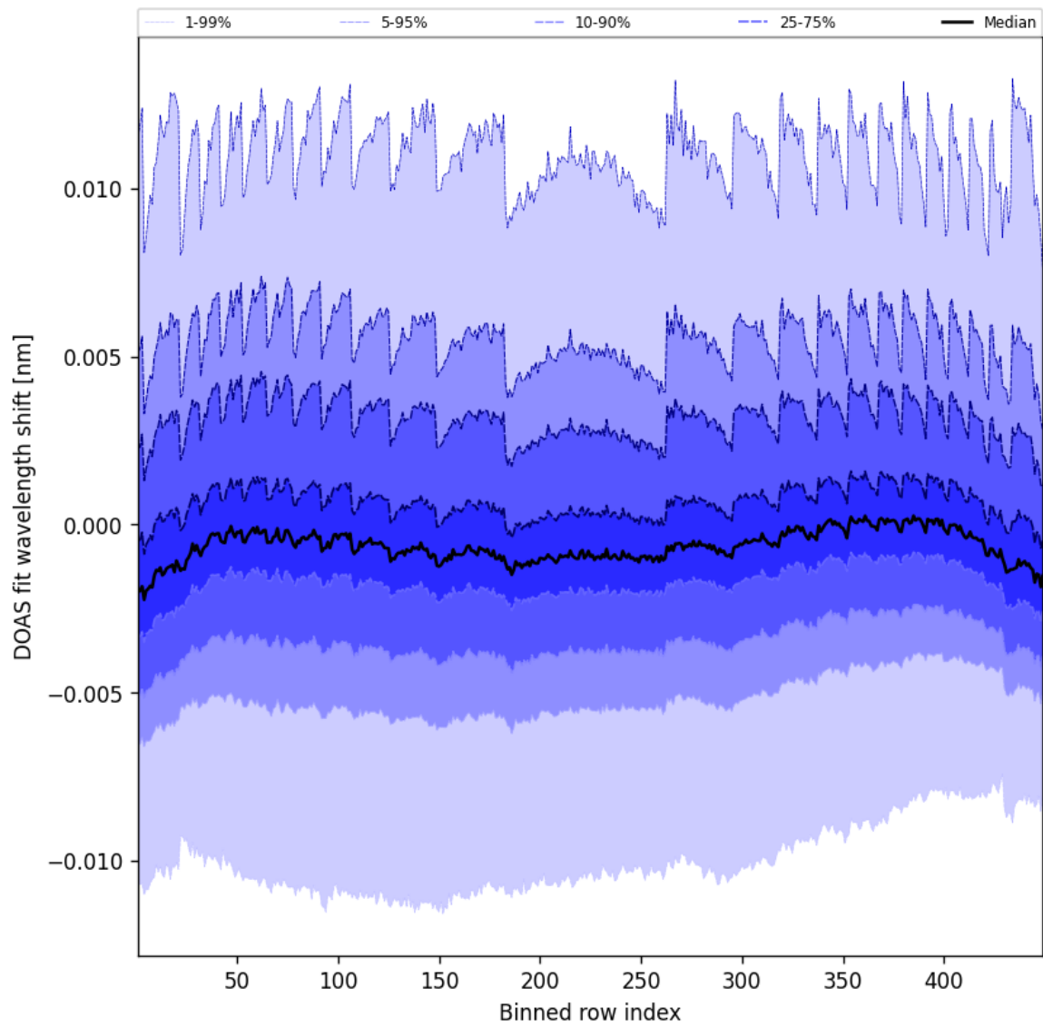
Figure 47: Along track statistics of “DOAS fit wavelength shift” for 2025-05-14 to 2025-05-15
