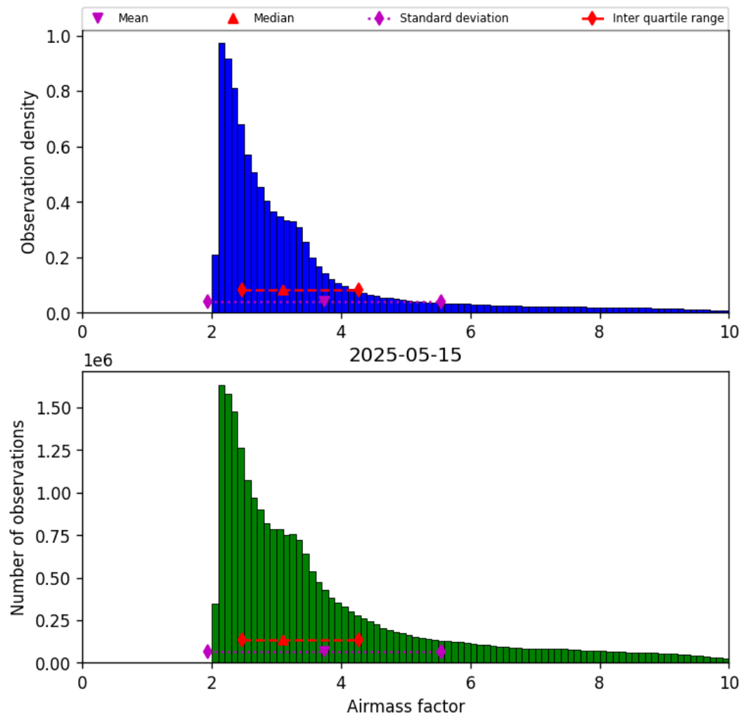
Figure 37: Histogram of “Airmass factor” for 2025-05-15 to 2025-05-16
