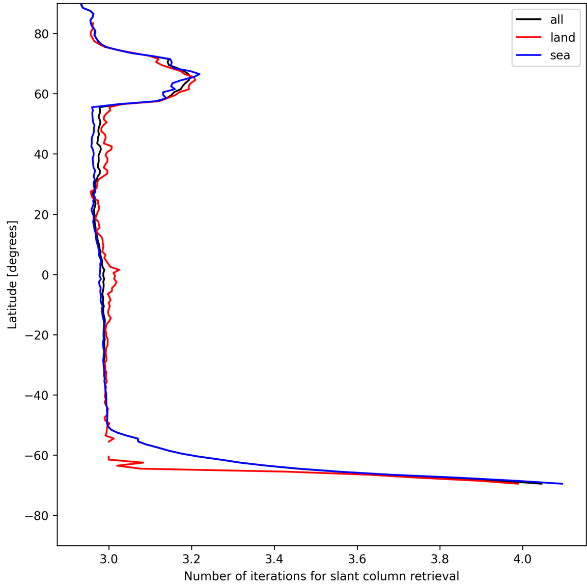
Figure 21: Zonal average of “Number of iterations for slant column retrieval” for 2025-05-15 to 2025-05-16.
