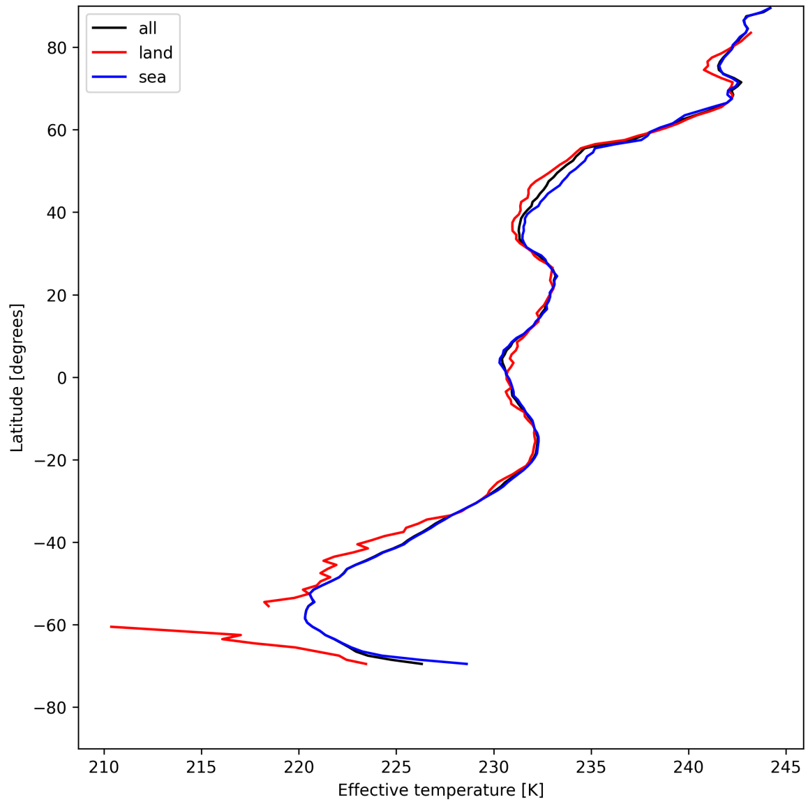
Figure 26: Zonal average of "Effective temperature" for 2025-05-15 to 2025-05-16.
