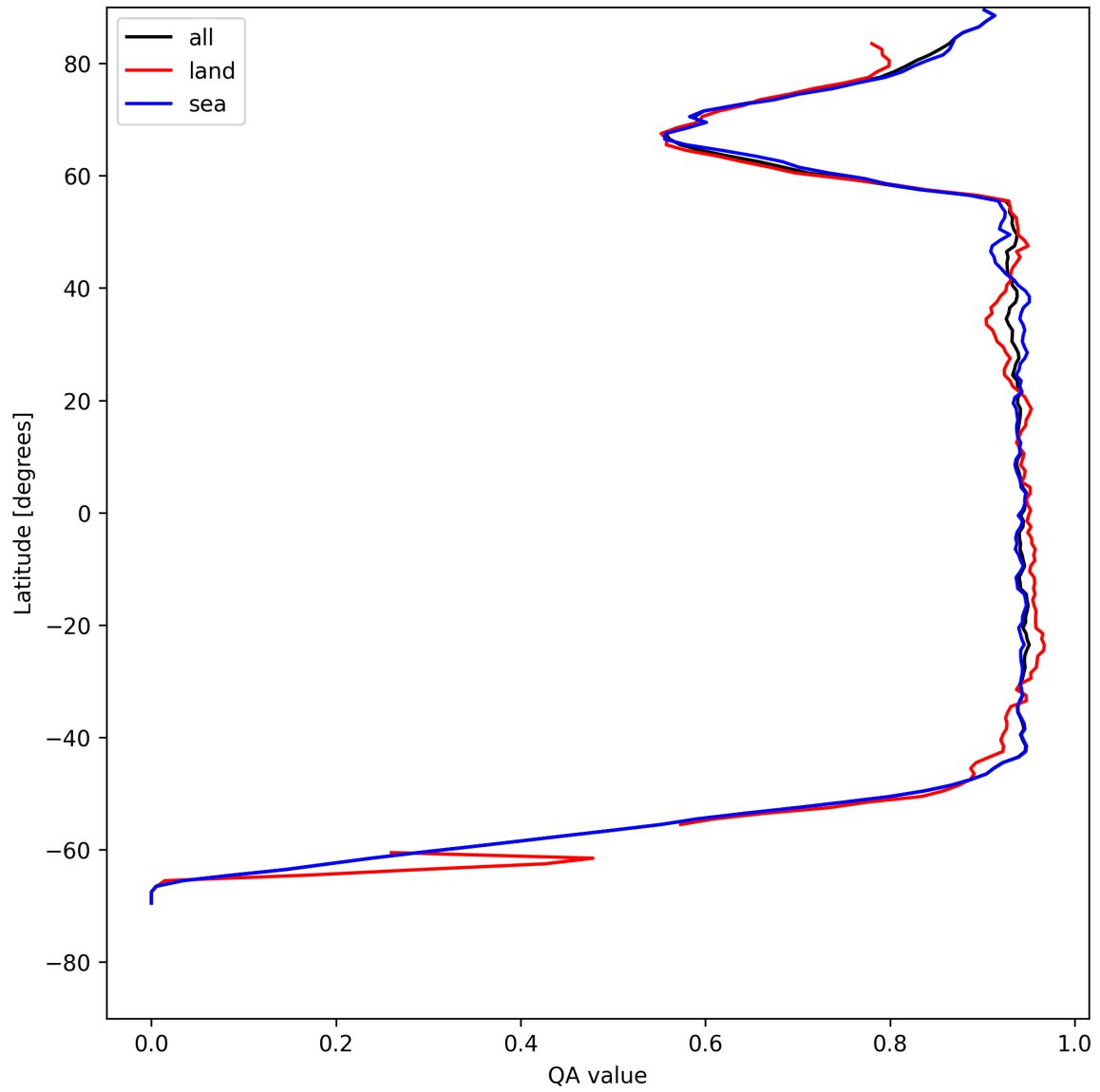
Figure 16: Zonal average of “QA value” for 2025-05-15 to 2025-05-16.
