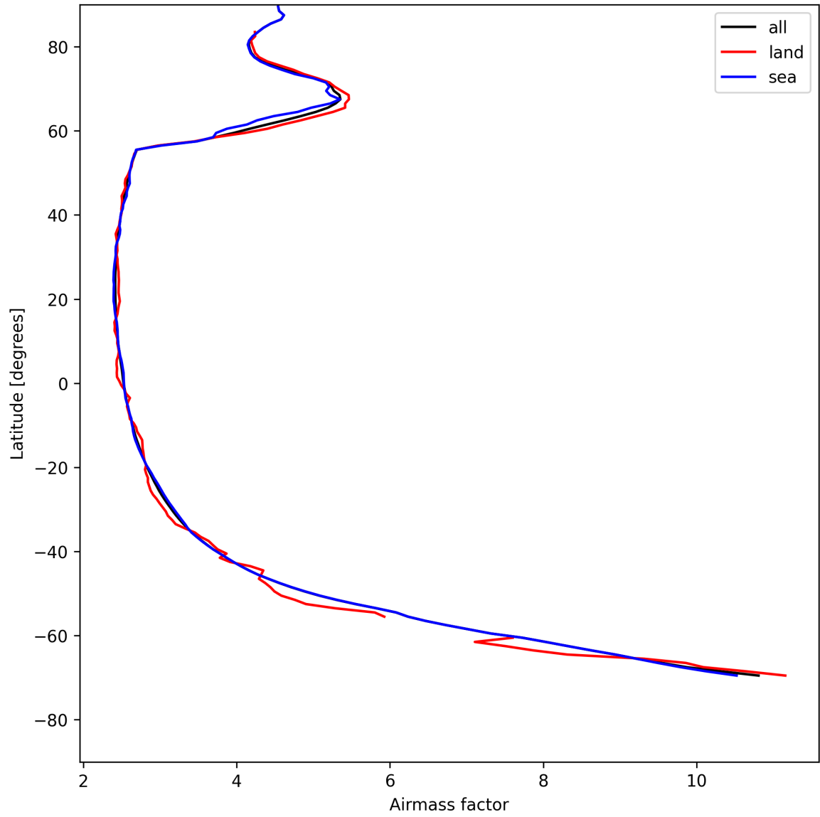
Figure 25: Zonal average of “Airmass factor” for 2025-05-15 to 2025-05-16.
