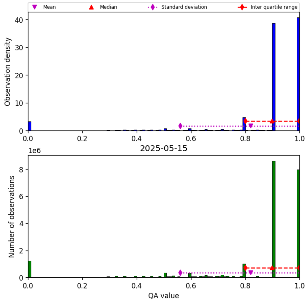
Figure 28: Histogram of “QA value” for 2025-05-15 to 2025-05-16
