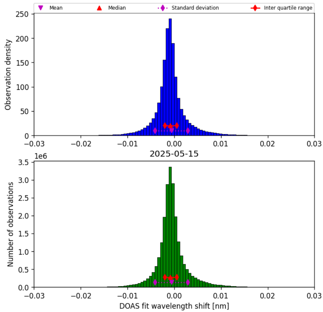
Figure 35: Histogram of “DOAS fit wavelength shift” for 2025-05-15 to 2025-05-16
