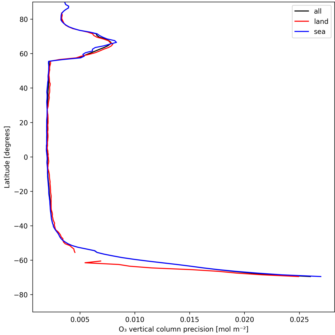
Figure 18: Zonal average of “O 3 vertical column precision” for 2025-05-15 to 2025-05-16.
