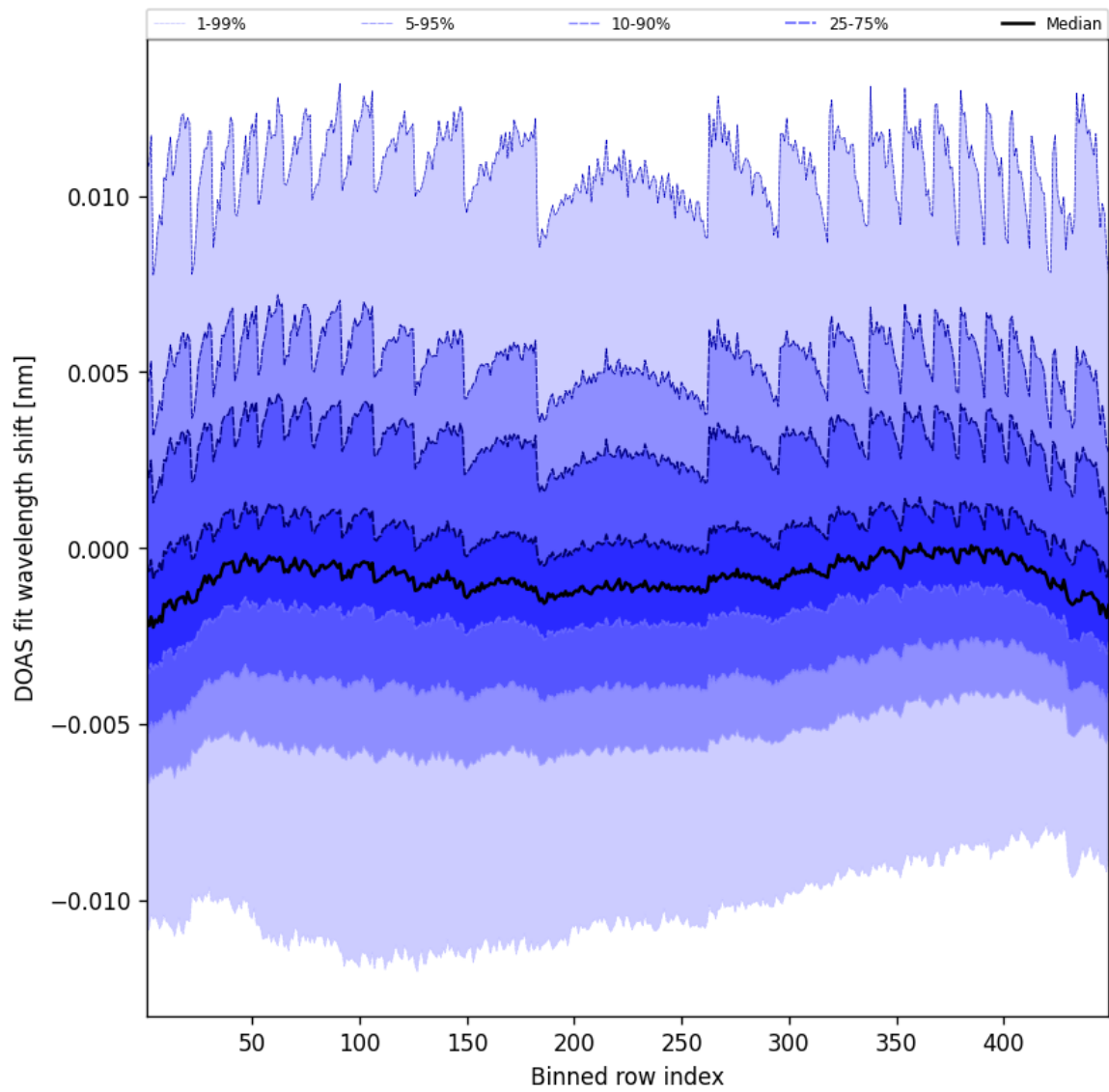
Figure 47: Along track statistics of “DOAS fit wavelength shift” for 2025-05-15 to 2025-05-16
