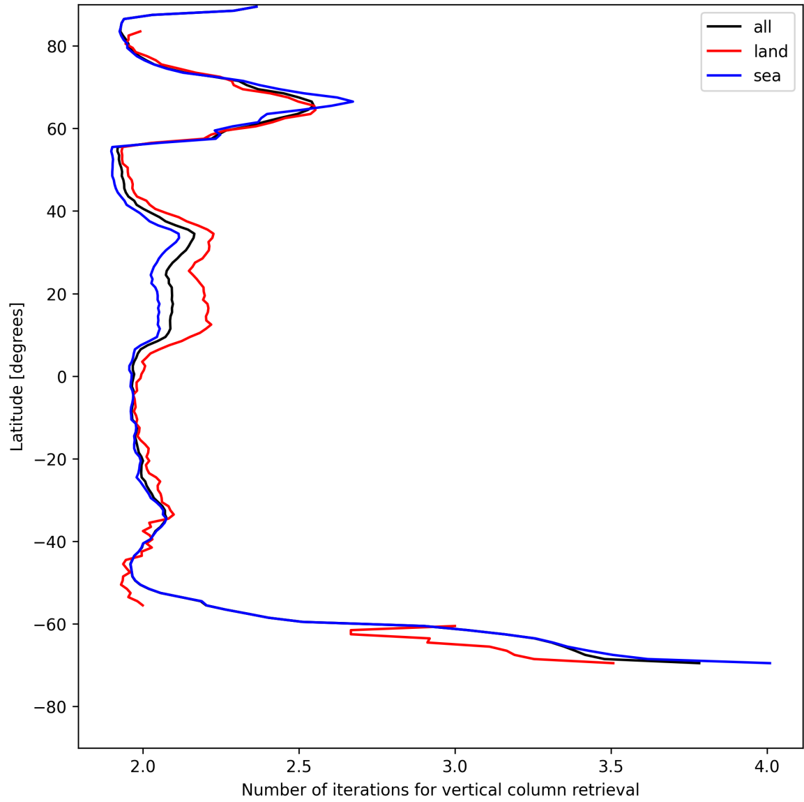
Figure 27: Zonal average of “Number of iterations for vertical column retrieval” for 2025-05-15 to 2025-05-16.
