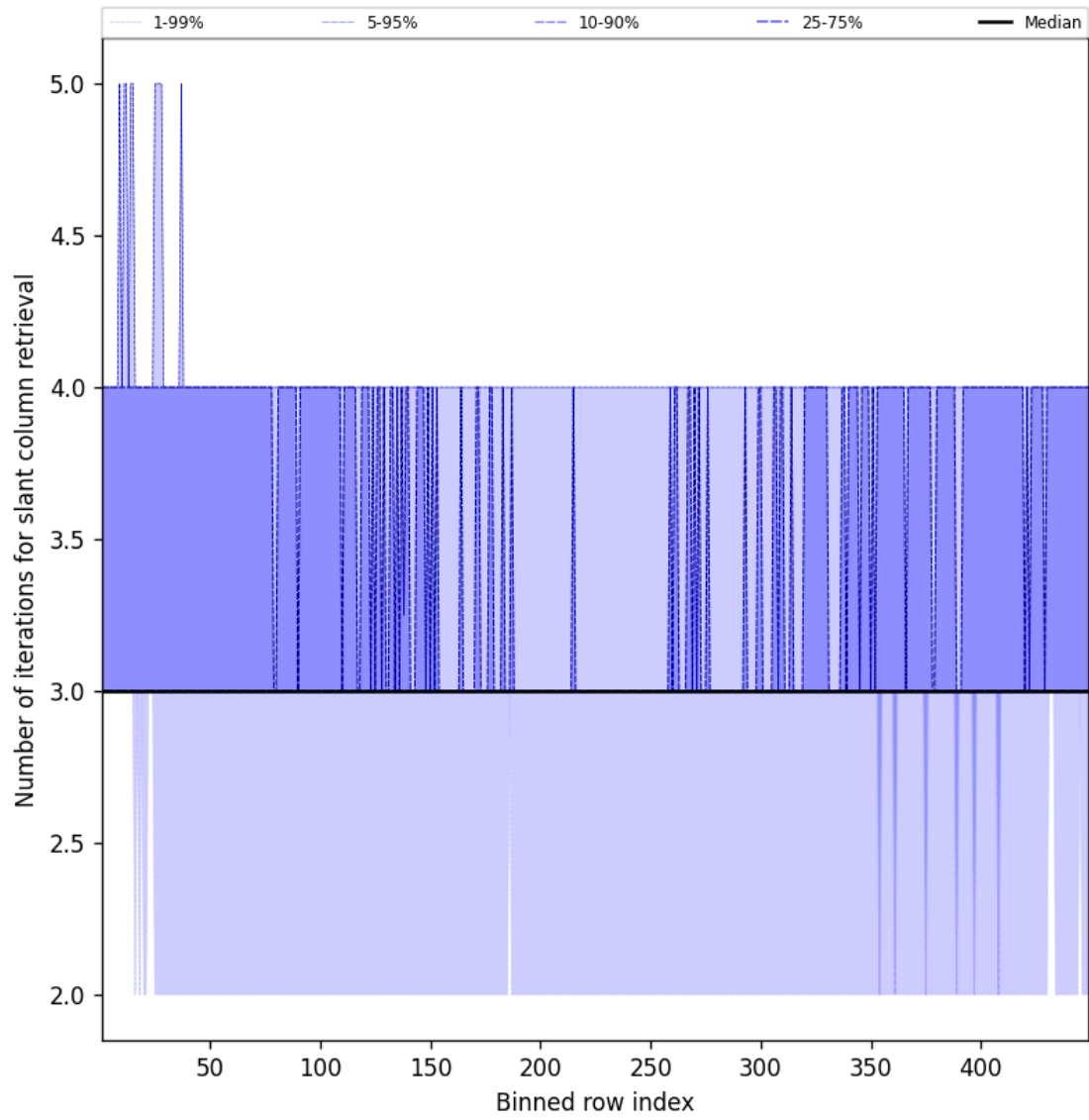
Figure 45: Along track statistics of “Number of iterations for slant column retrieval” for 2025-05-15 to 2025-05-16
