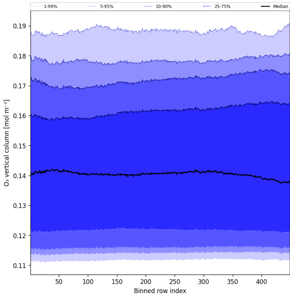
Figure 41: Along track statistics of “ \text{O}_3 vertical column” for 2025-05-15 to 2025-05-16
