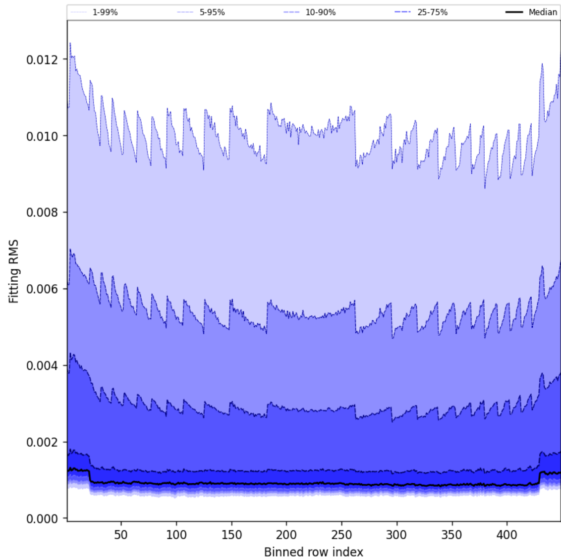
Figure 46: Along track statistics of “Fitting RMS” for 2025-05-15 to 2025-05-16
