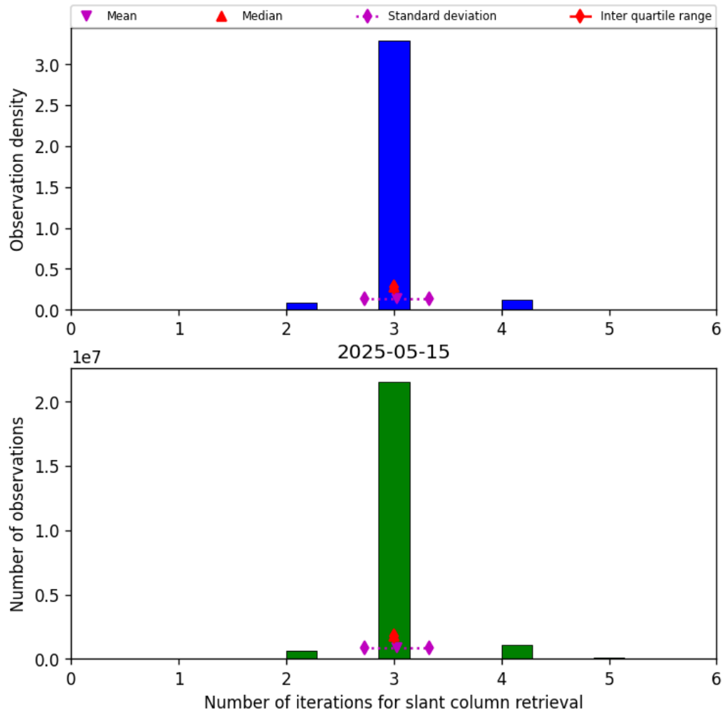
Figure 33: Histogram of “Number of iterations for slant column retrieval” for 2025-05-15 to 2025-05-16
