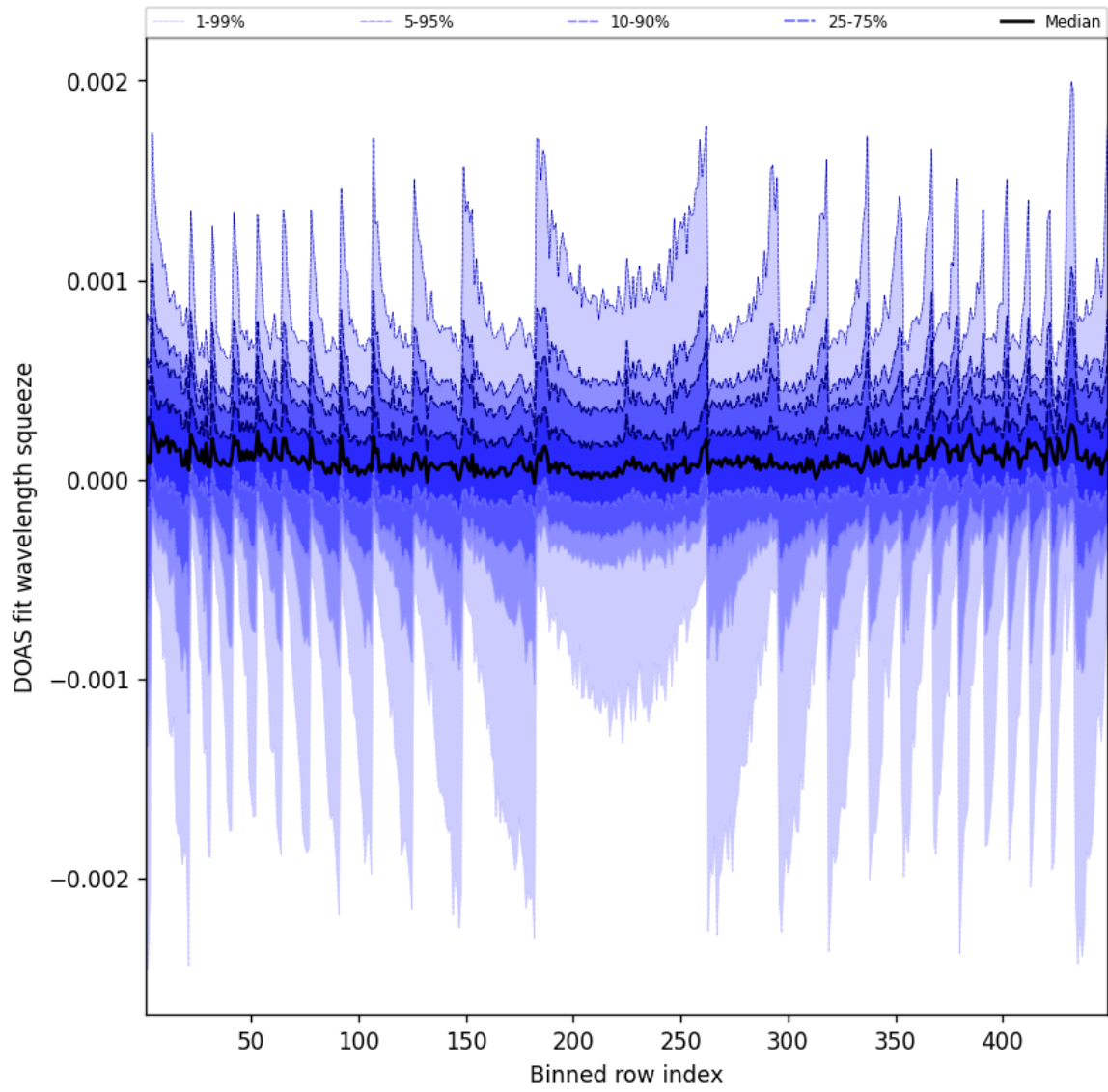
Figure 48: Along track statistics of “DOAS fit wavelength squeeze” for 2025-05-15 to 2025-05-16
