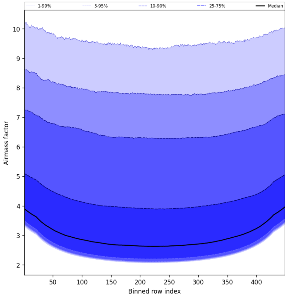
Figure 49: Along track statistics of “Airmass factor” for 2025-05-15 to 2025-05-16
