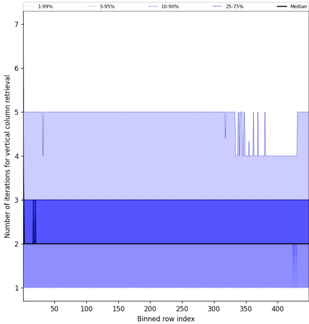
Figure 51: Along track statistics of “Number of iterations for vertical column retrieval” for 2025-05-15 to 2025-05-16
