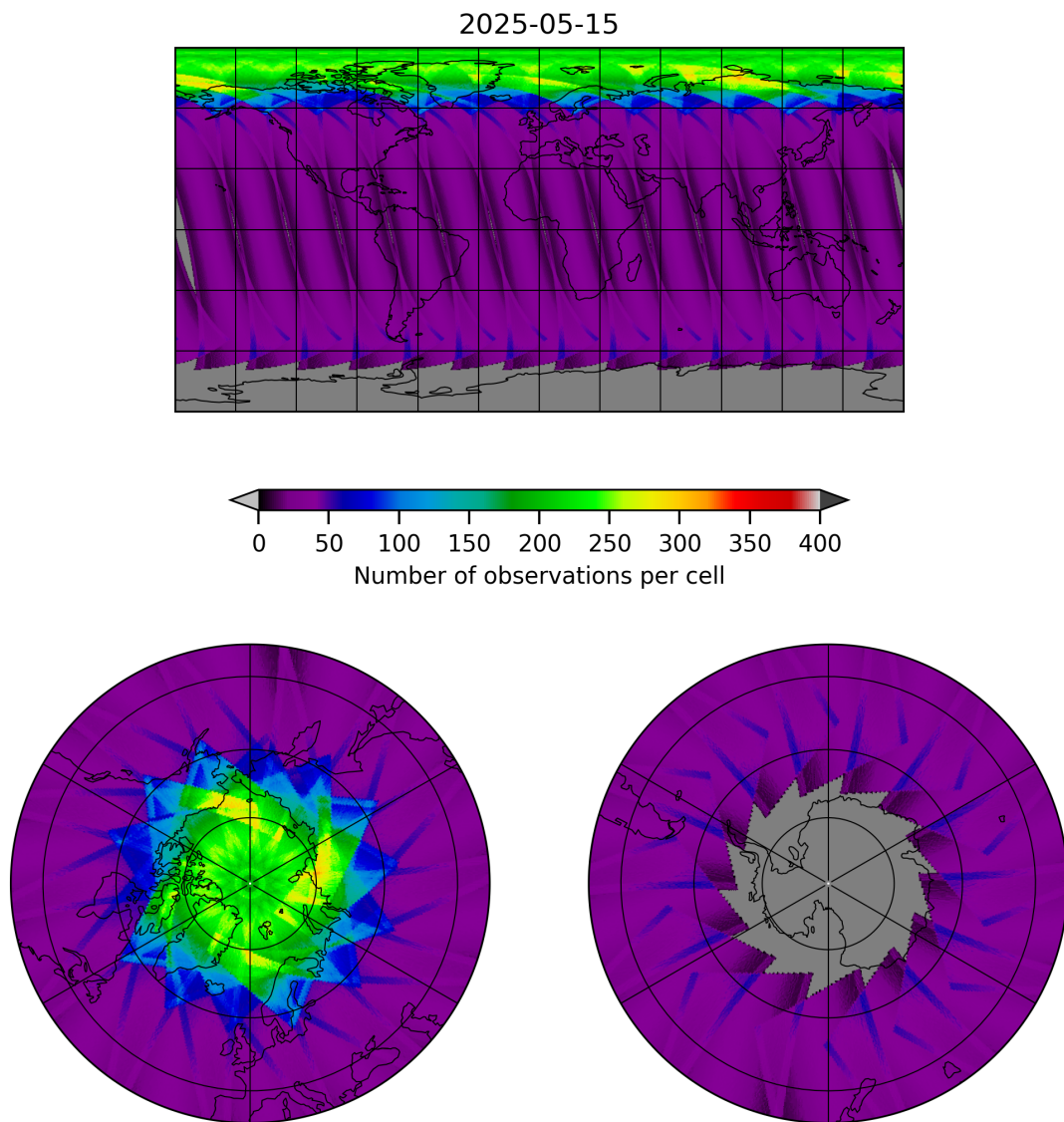
Figure 15: Map of the number of observations for 2025-05-15 to 2025-05-16
