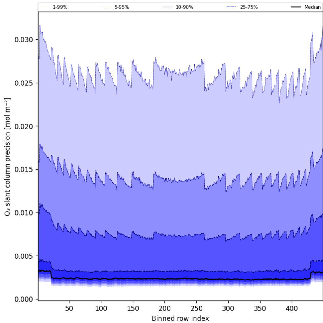
Figure 44: Along track statistics of “O 3 slant column precision” for 2025-05-15 to 2025-05-16
