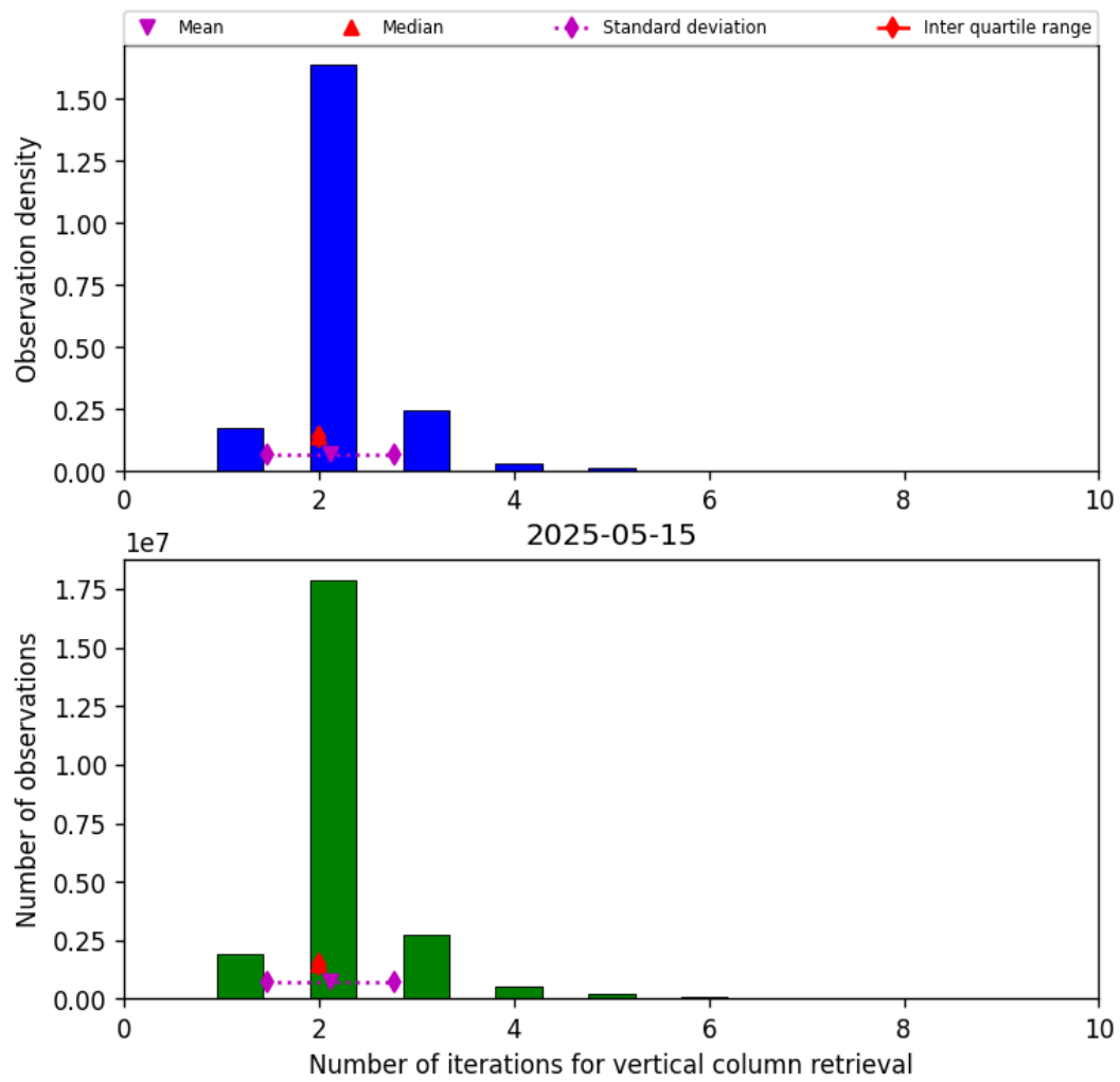
Figure 39: Histogram of “Number of iterations for vertical column retrieval” for 2025-05-15 to 2025-05-16
