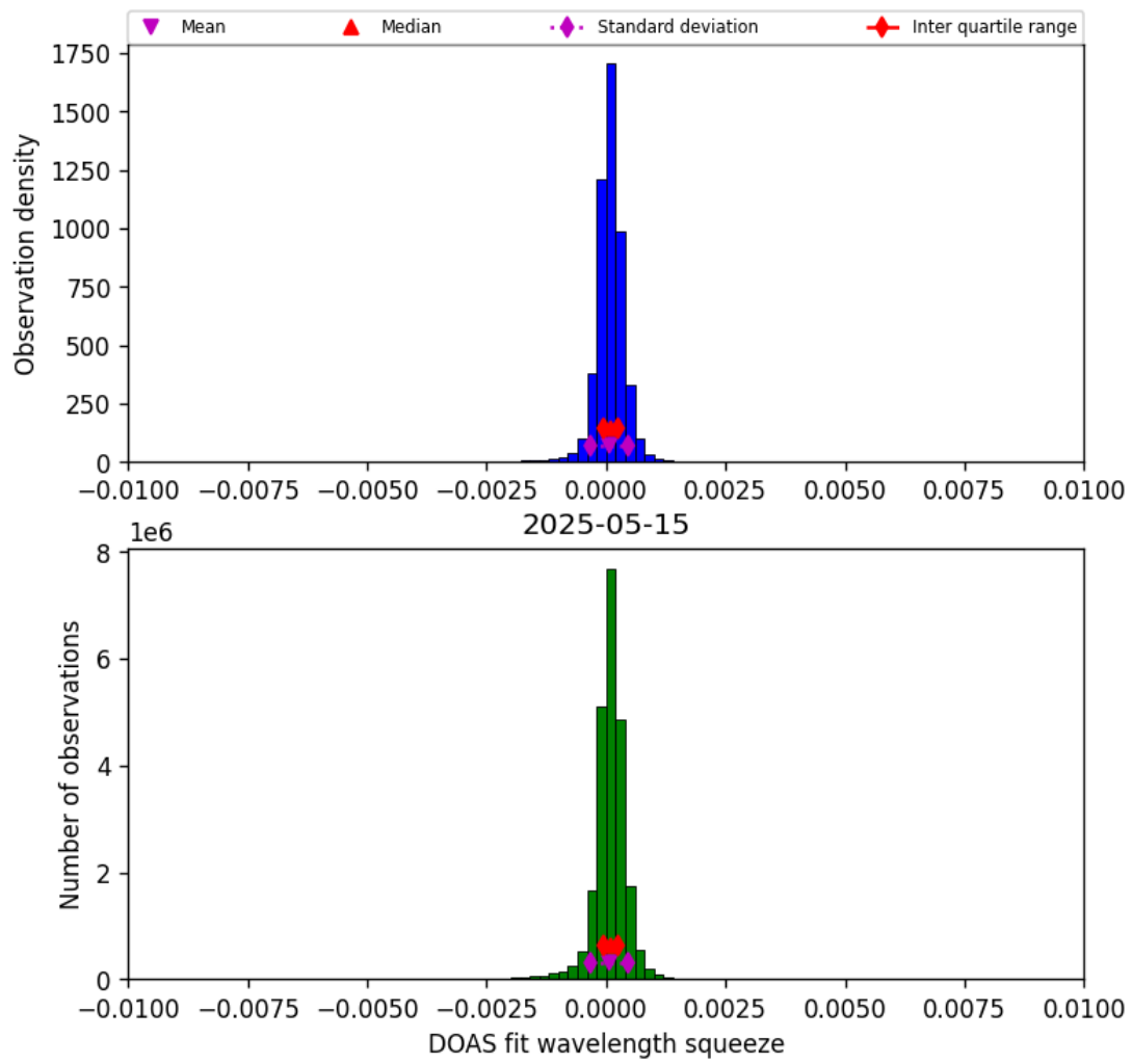
Figure 36: Histogram of “DOAS fit wavelength squeeze” for 2025-05-15 to 2025-05-16
