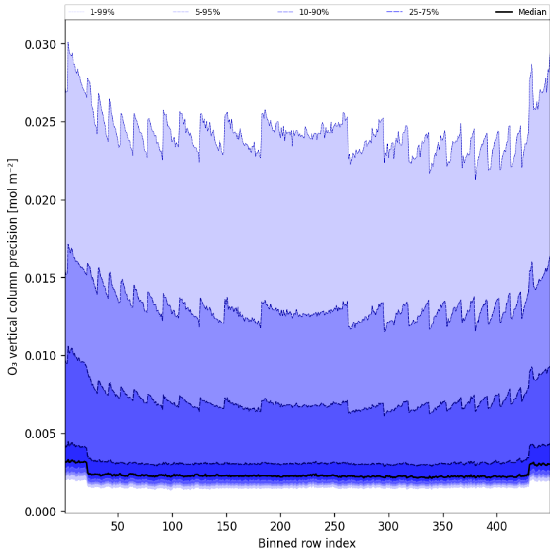
Figure 42: Along track statistics of “O 3 vertical column precision” for 2025-05-15 to 2025-05-16
