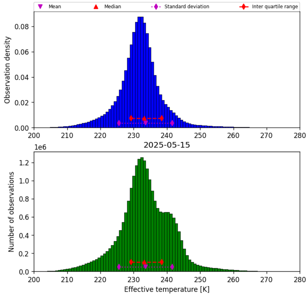
Figure 38: Histogram of “Effective temperature” for 2025-05-15 to 2025-05-16
