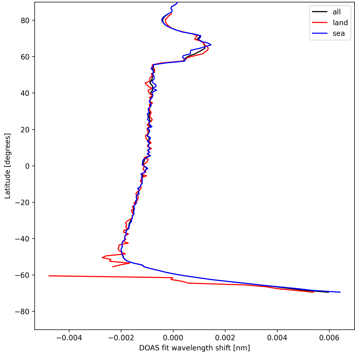
Figure 23: Zonal average of “DOAS fit wavelength shift” for 2025-05-15 to 2025-05-16.
