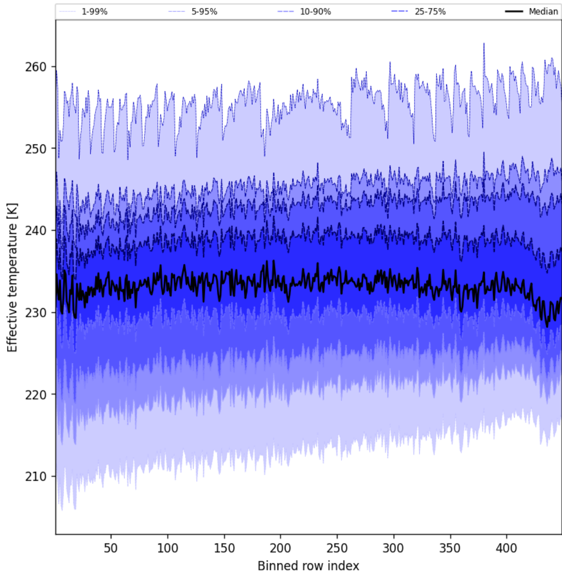
Figure 50: Along track statistics of “Effective temperature” for 2025-05-15 to 2025-05-16
