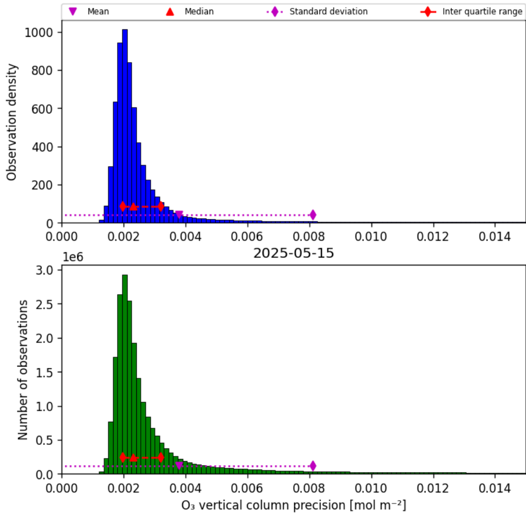
Figure 30: Histogram of “O 3 vertical column precision” for 2025-05-15 to 2025-05-16
