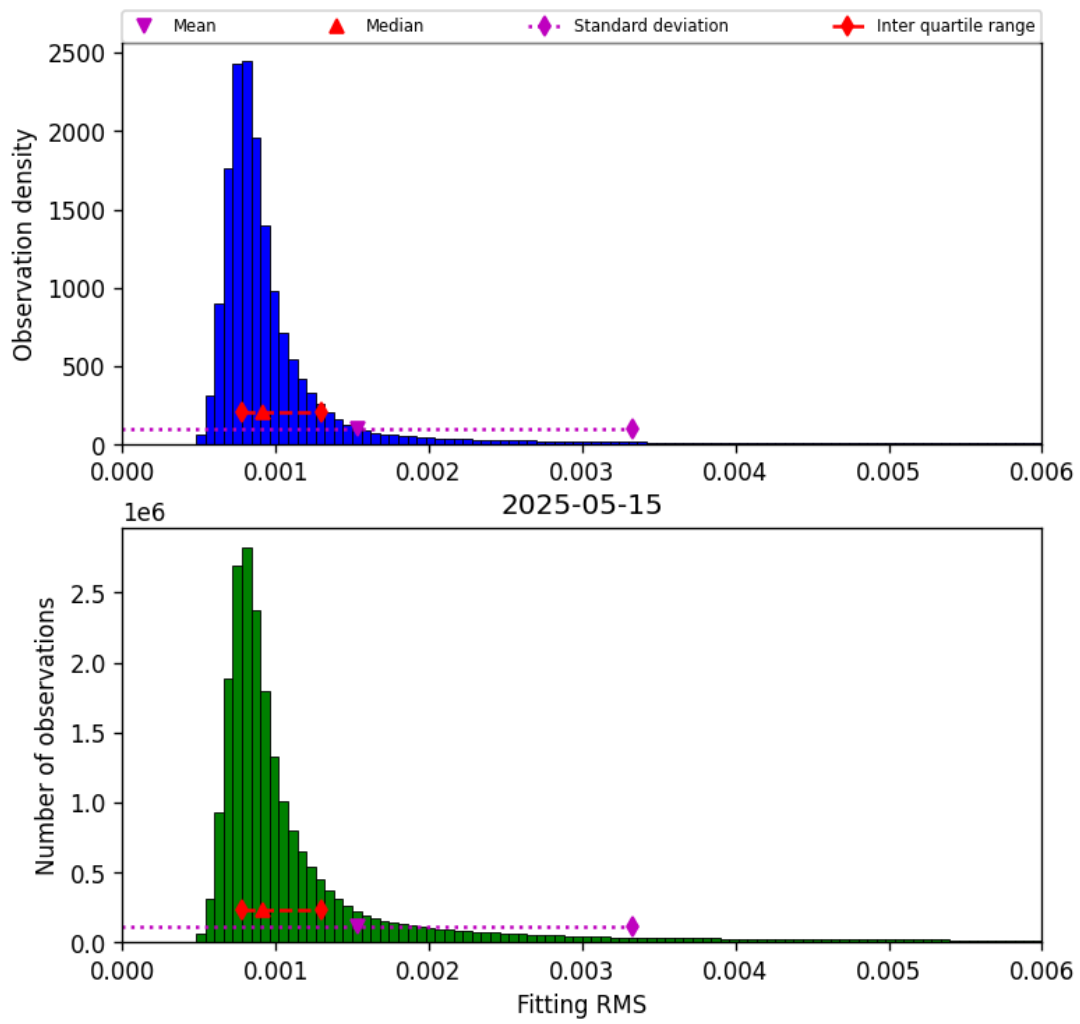
Figure 34: Histogram of “Fitting RMS” for 2025-05-15 to 2025-05-16
