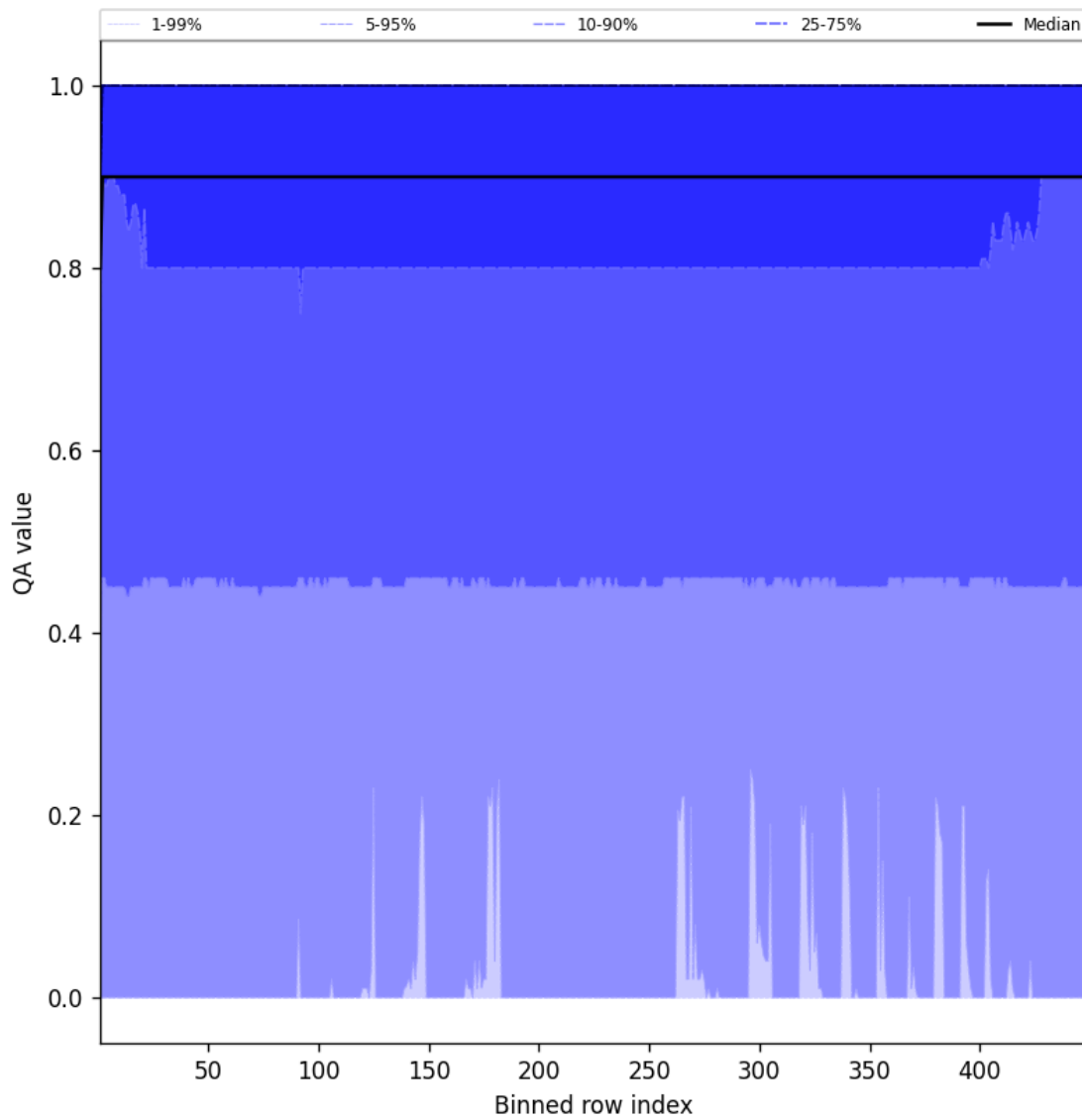
Figure 40: Along track statistics of “QA value” for 2025-05-15 to 2025-05-16
