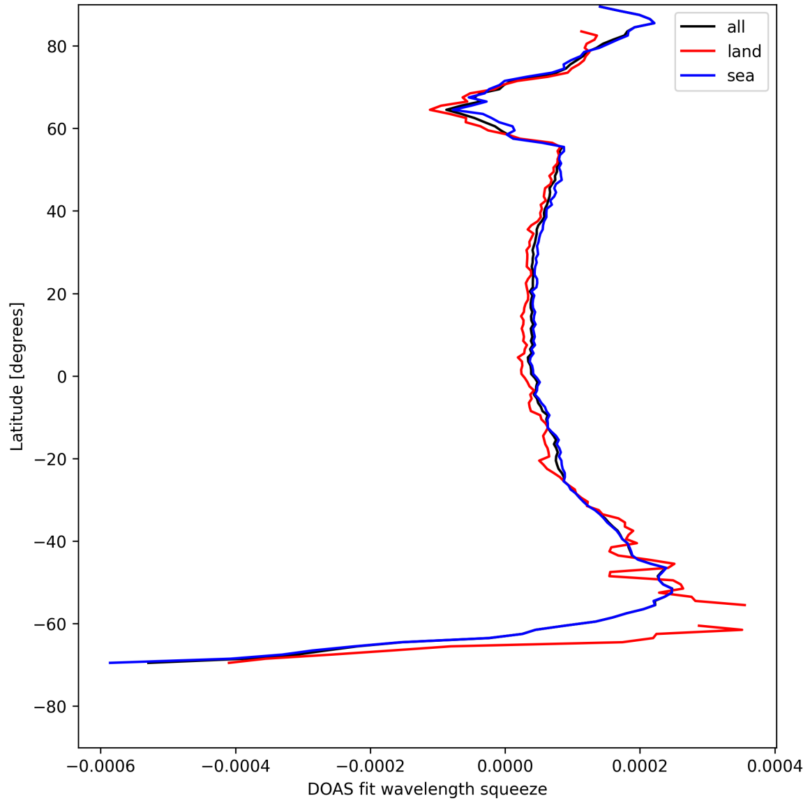
Figure 24: Zonal average of “DOAS fit wavelength squeeze” for 2025-05-15 to 2025-05-16.
