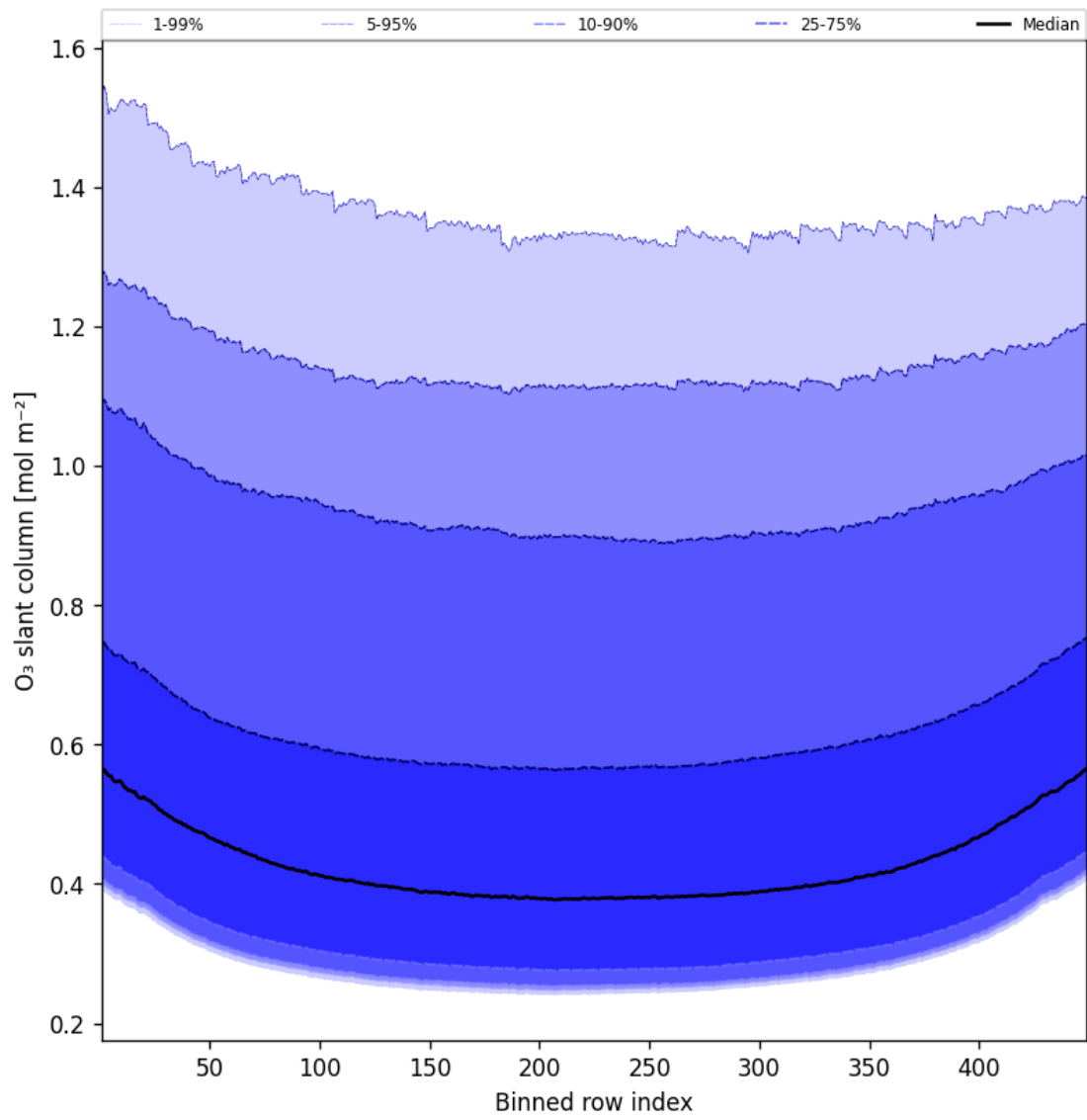
Figure 43: Along track statistics of “O 3 slant column” for 2025-05-15 to 2025-05-16
