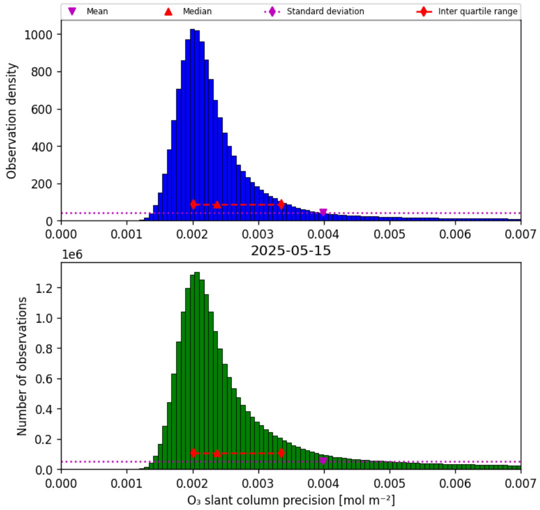
Figure 32: Histogram of “O 3 slant column precision” for 2025-05-15 to 2025-05-16
