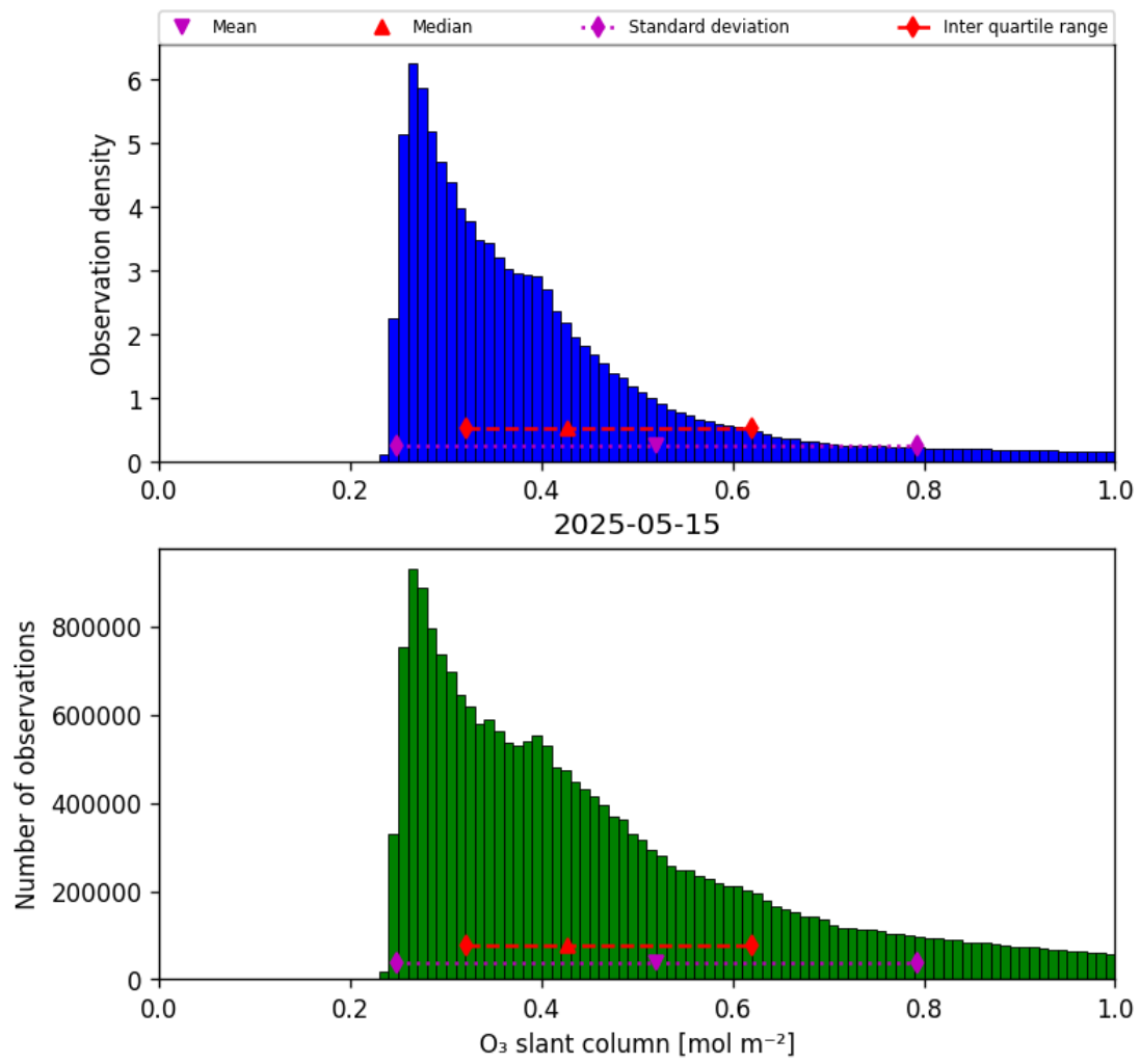
Figure 31: Histogram of “O 3 slant column” for 2025-05-15 to 2025-05-16
