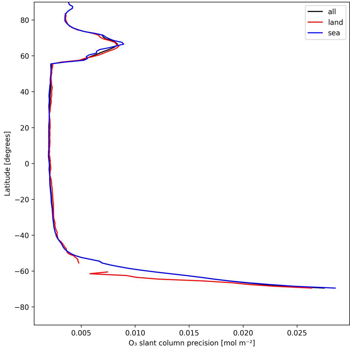
Figure 20: Zonal average of “O 3 slant column precision” for 2025-05-15 to 2025-05-16.
