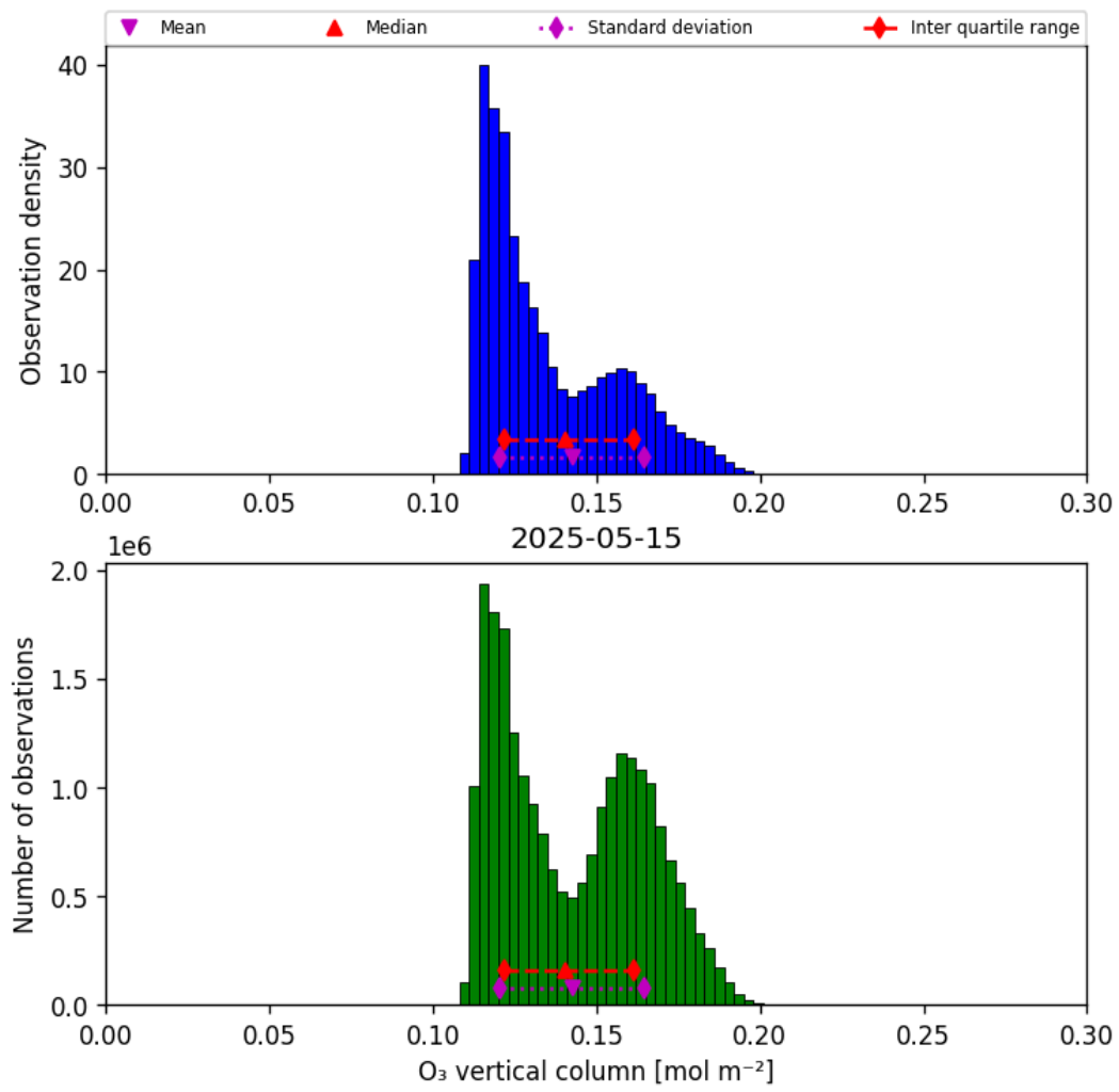
Figure 29: Histogram of “O 3 vertical column” for 2025-05-15 to 2025-05-16
