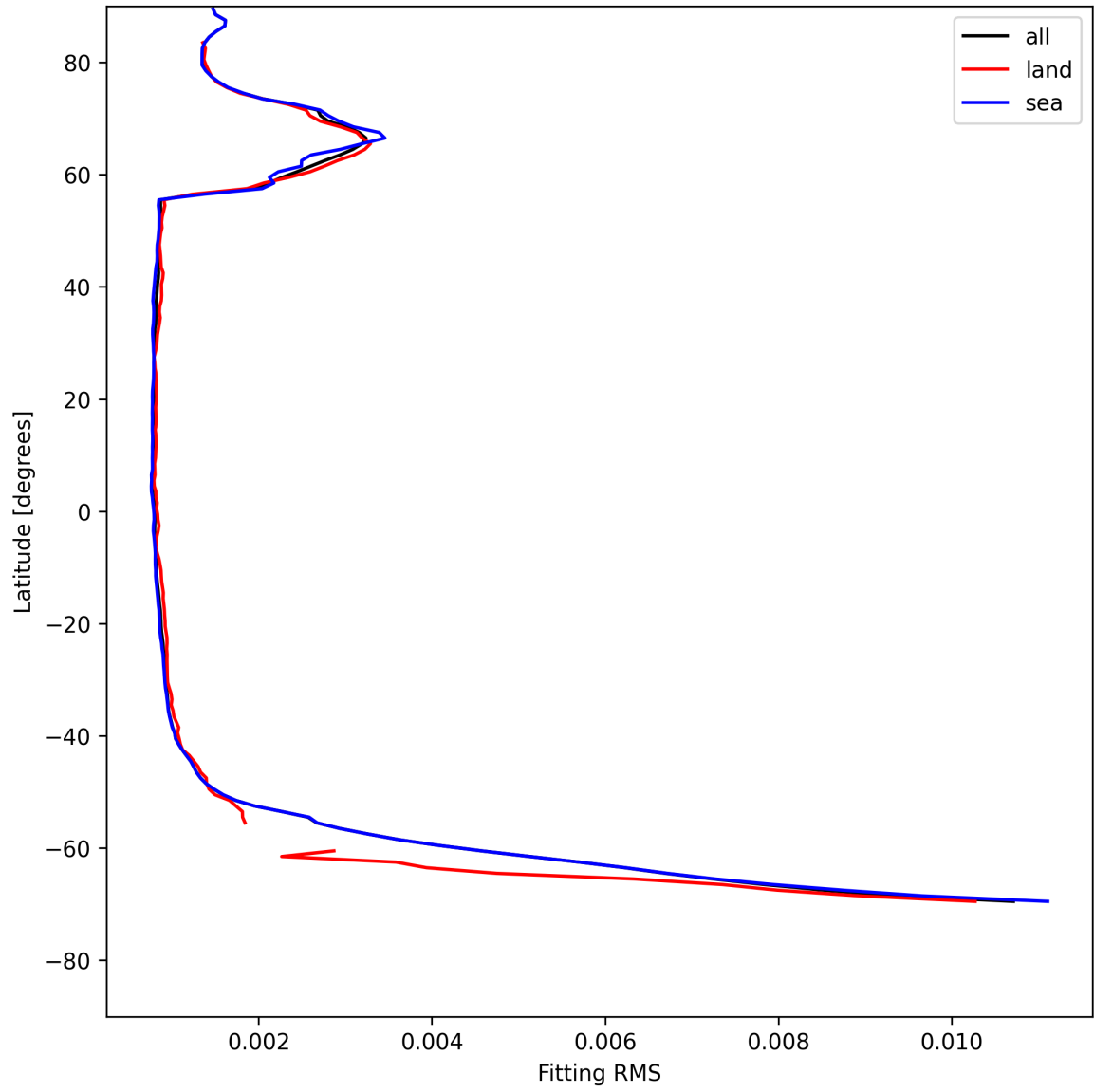
Figure 22: Zonal average of “Fitting RMS” for 2025-05-15 to 2025-05-16.
