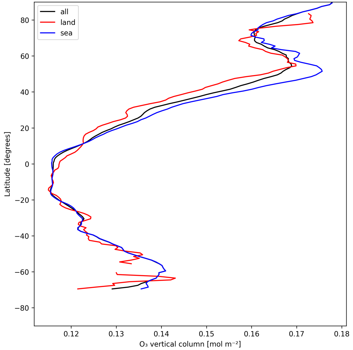
Figure 17: Zonal average of “O 3 vertical column” for 2025-05-15 to 2025-05-16.
