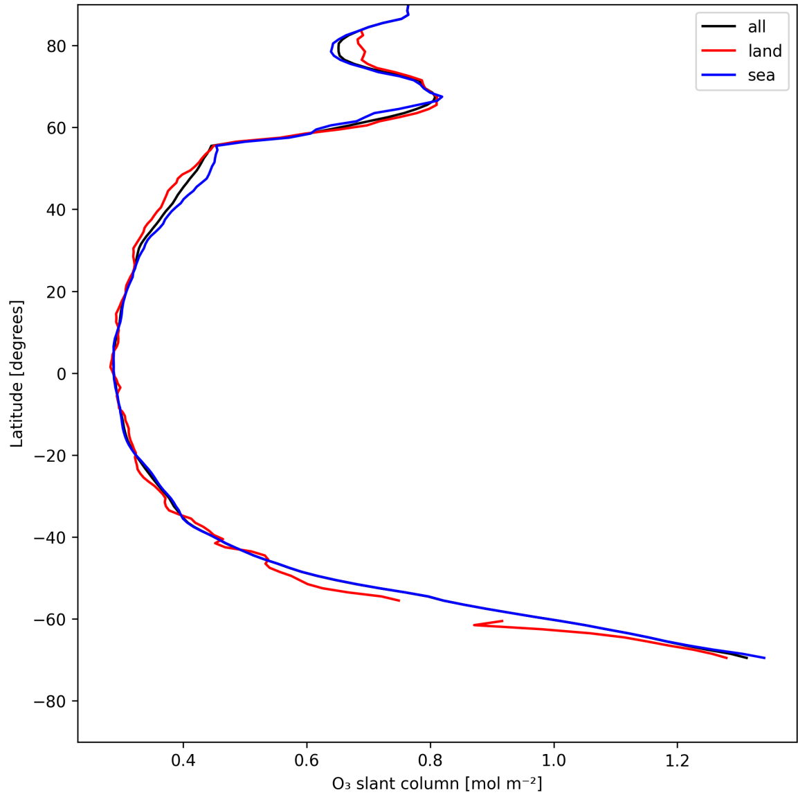
Figure 19: Zonal average of “O 3 slant column” for 2025-05-15 to 2025-05-16.
