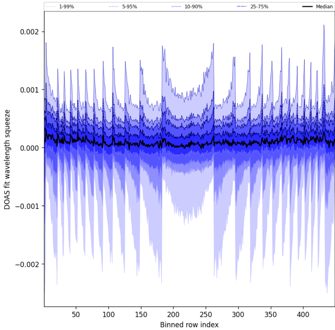
Figure 48: Along track statistics of “DOAS fit wavelength squeeze” for 2025-05-16 to 2025-05-17
