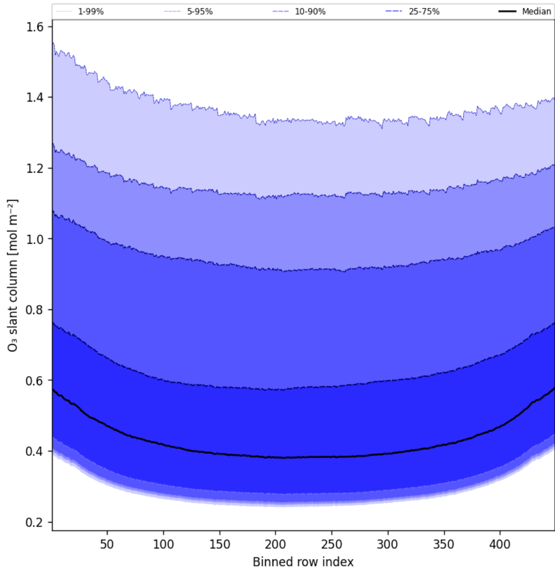
Figure 43: Along track statistics of “O 3 slant column” for 2025-05-16 to 2025-05-17
