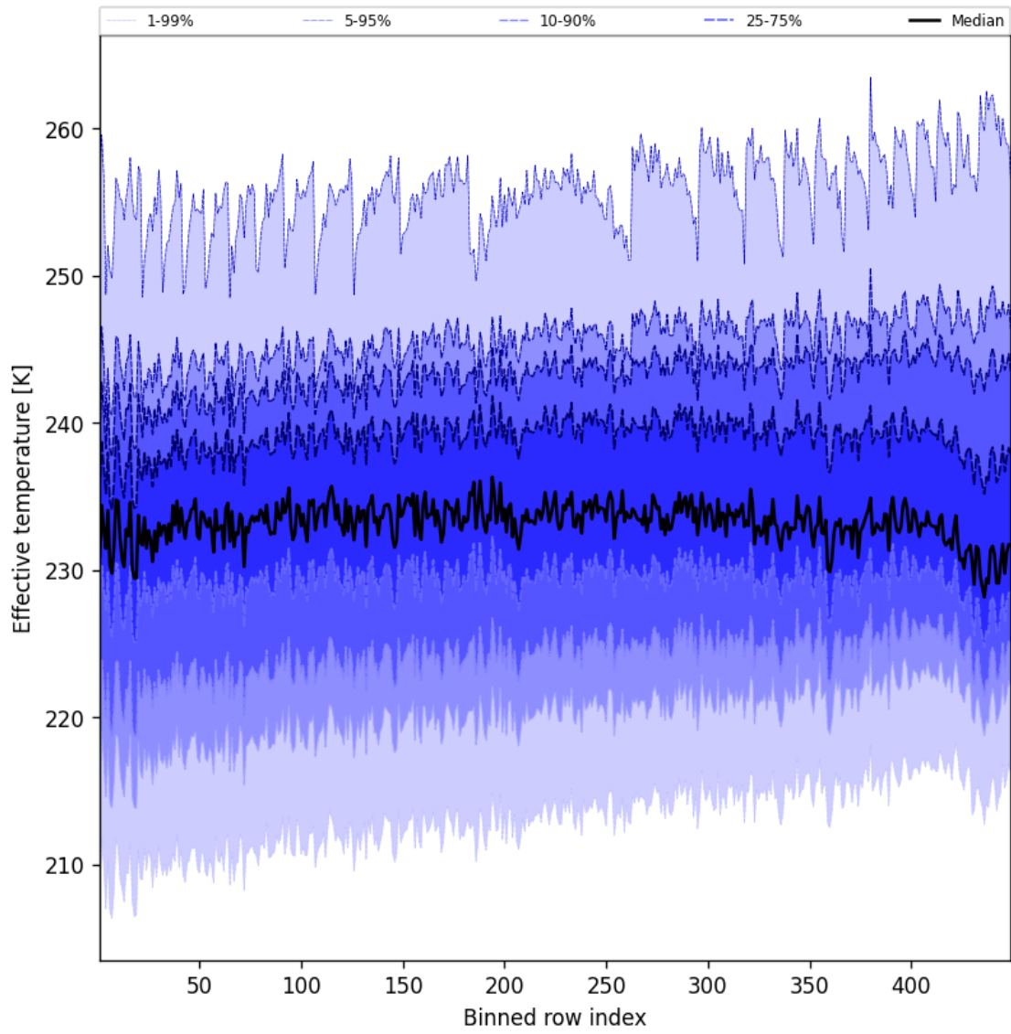
Figure 50: Along track statistics of “Effective temperature” for 2025-05-16 to 2025-05-17
