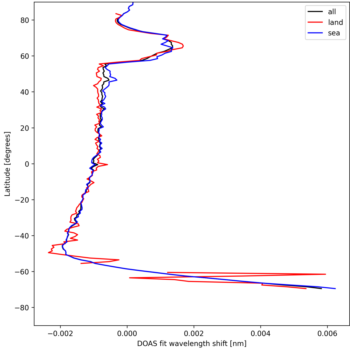
Figure 23: Zonal average of “DOAS fit wavelength shift” for 2025-05-16 to 2025-05-17.
