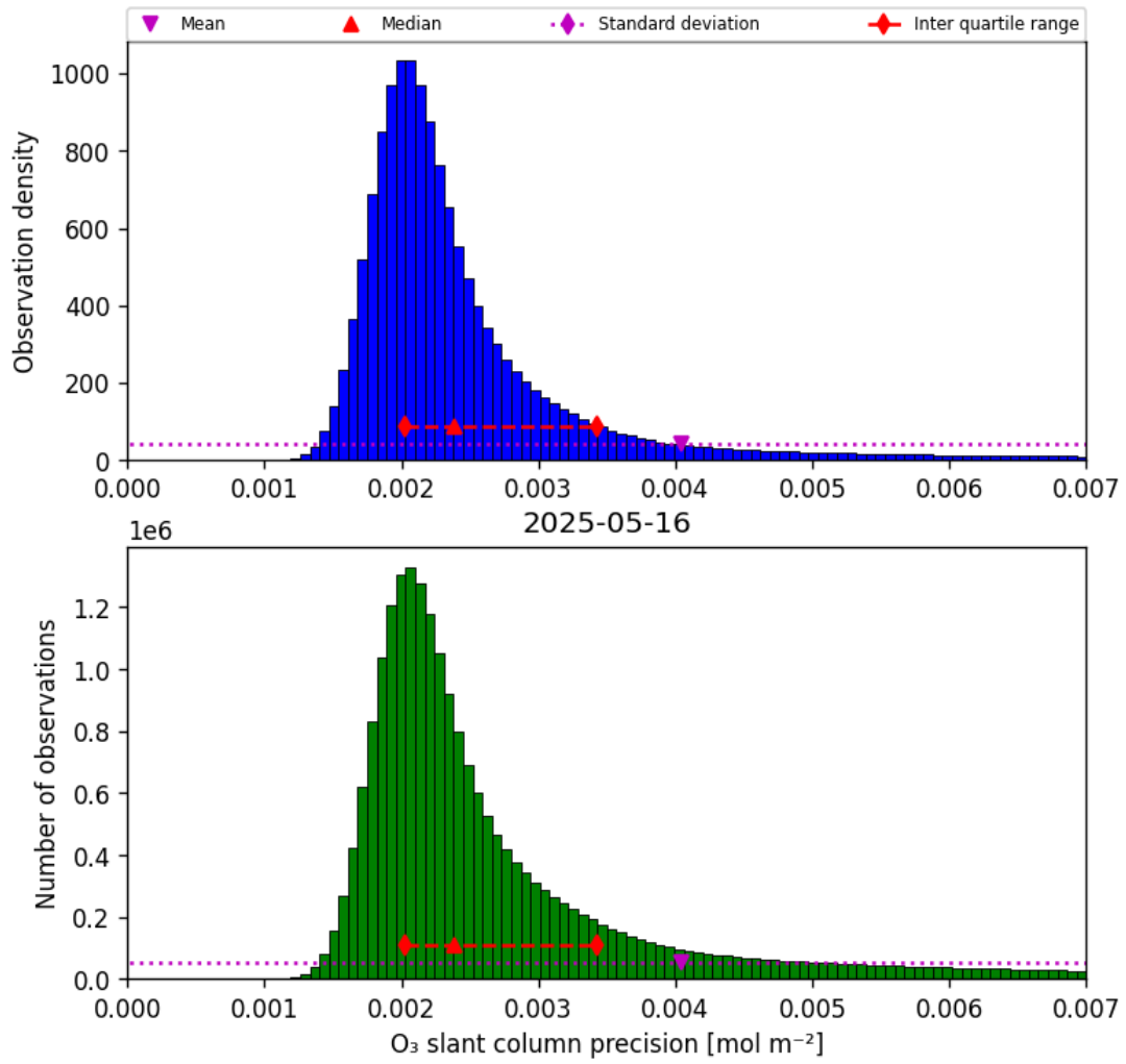
Figure 32: Histogram of “O 3 slant column precision” for 2025-05-16 to 2025-05-17
