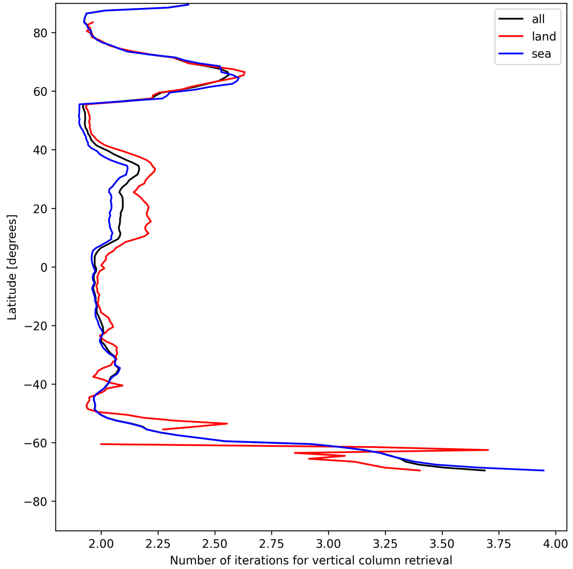
Figure 27: Zonal average of “Number of iterations for vertical column retrieval” for 2025-05-16 to 2025-05-17.
