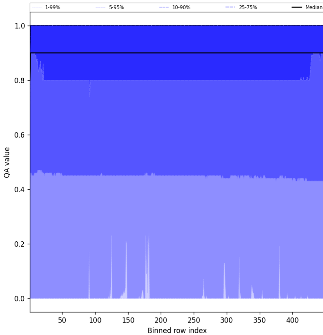
Figure 40: Along track statistics of “QA value” for 2025-05-16 to 2025-05-17
