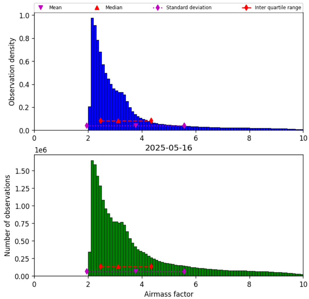
Figure 37: Histogram of “Airmass factor” for 2025-05-16 to 2025-05-17
