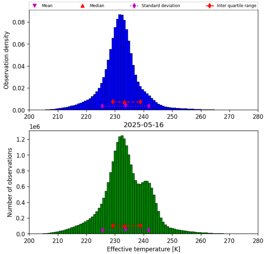
Figure 38: Histogram of “Effective temperature” for 2025-05-16 to 2025-05-17
