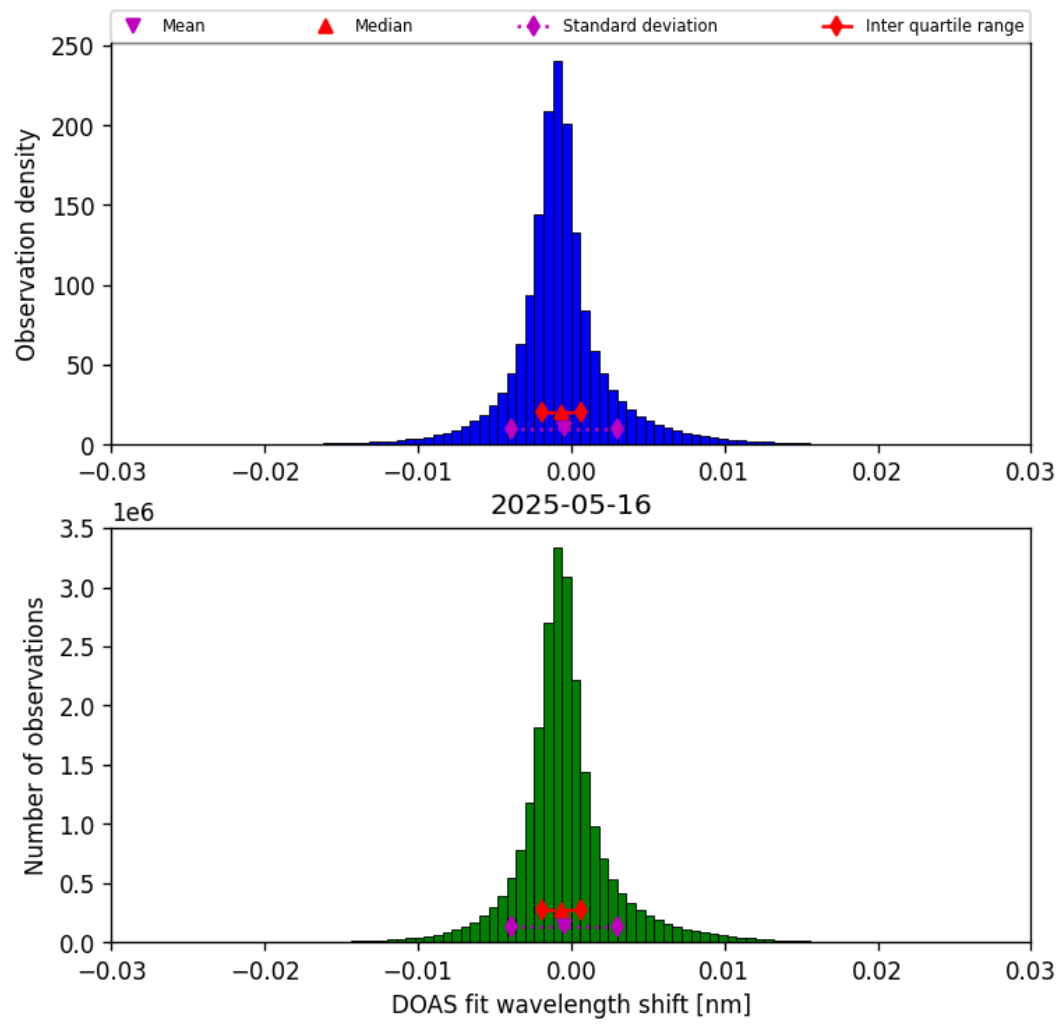
Figure 35: Histogram of “DOAS fit wavelength shift” for 2025-05-16 to 2025-05-17
