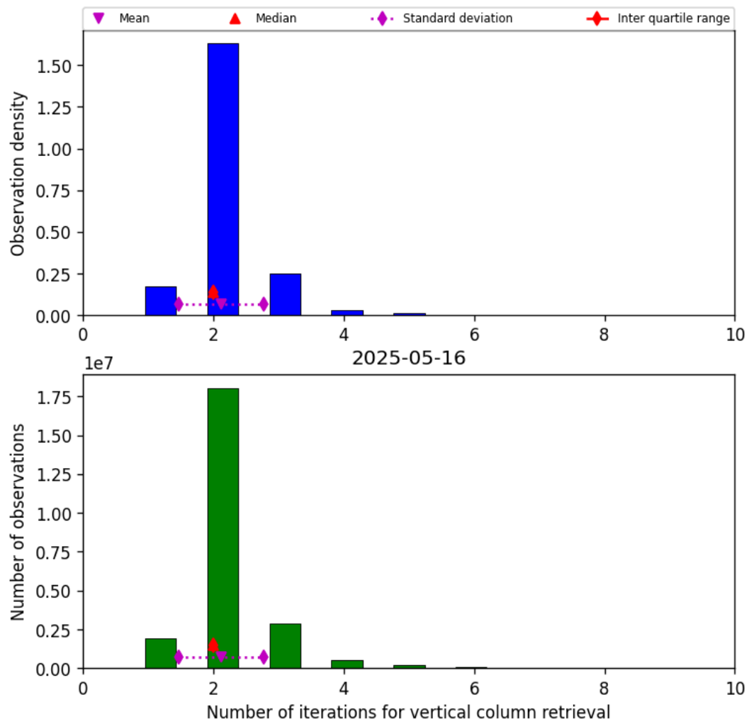
Figure 39: Histogram of “Number of iterations for vertical column retrieval” for 2025-05-16 to 2025-05-17
