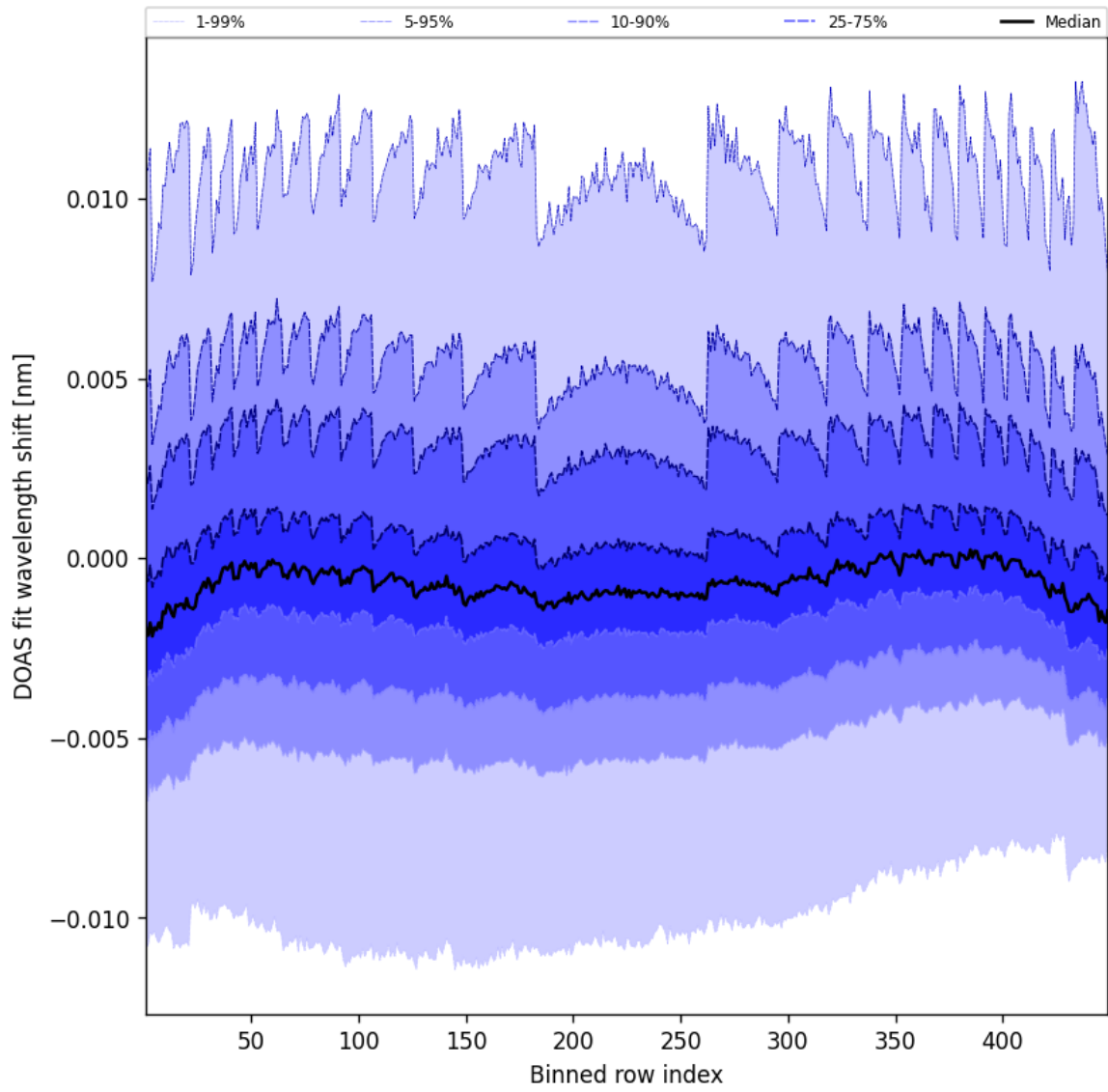
Figure 47: Along track statistics of “DOAS fit wavelength shift” for 2025-05-16 to 2025-05-17
