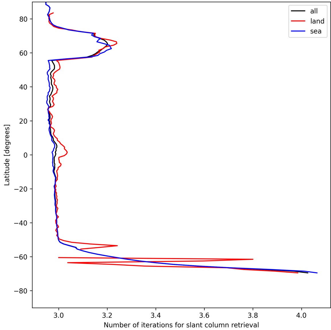
Figure 21: Zonal average of “Number of iterations for slant column retrieval” for 2025-05-16 to 2025-05-17.
