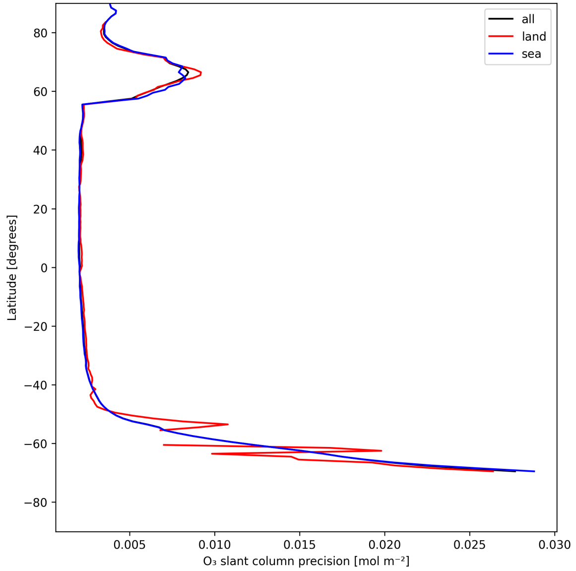
Figure 20: Zonal average of “O 3 slant column precision” for 2025-05-16 to 2025-05-17.
