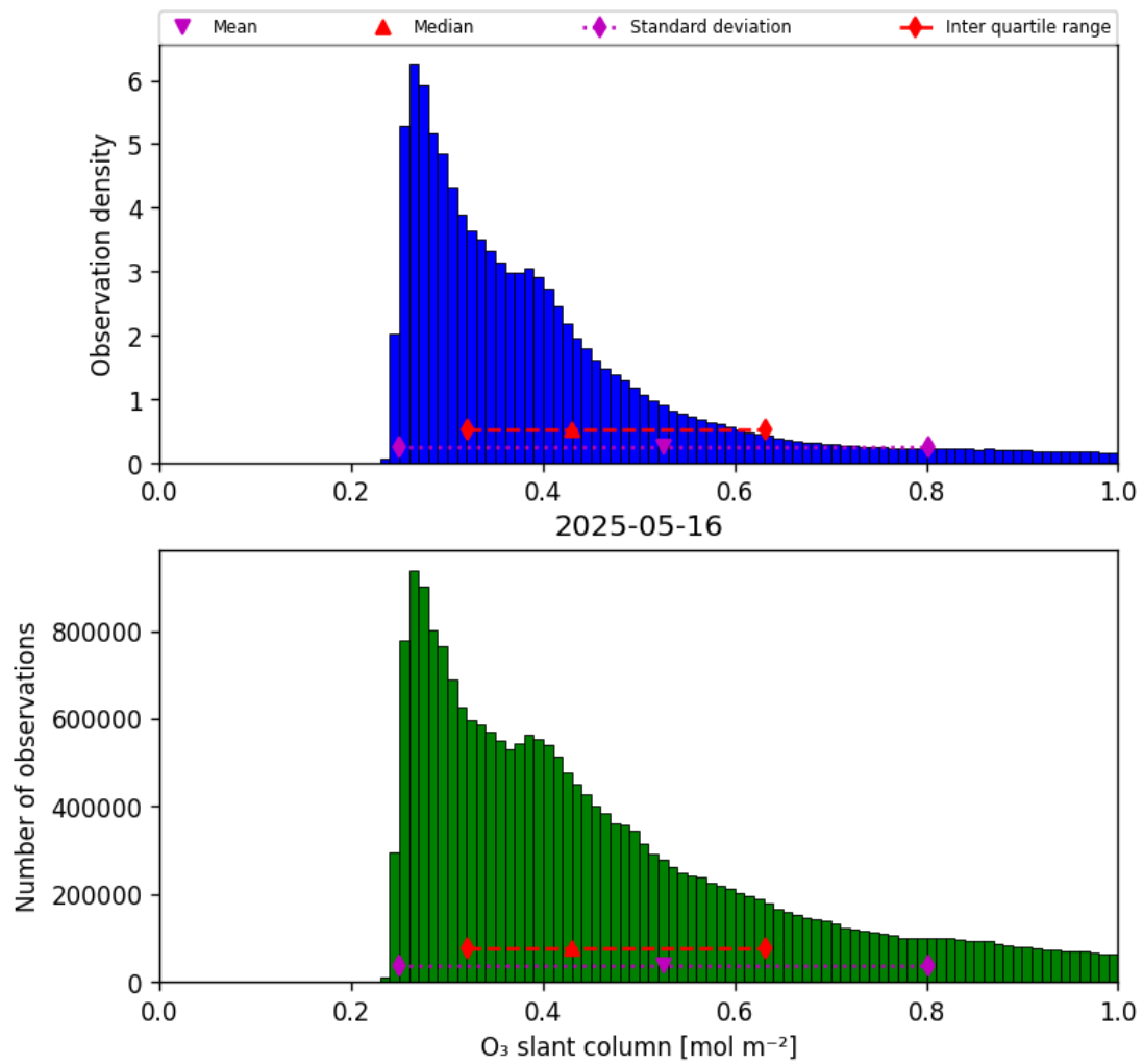
Figure 31: Histogram of “O 3 slant column” for 2025-05-16 to 2025-05-17
