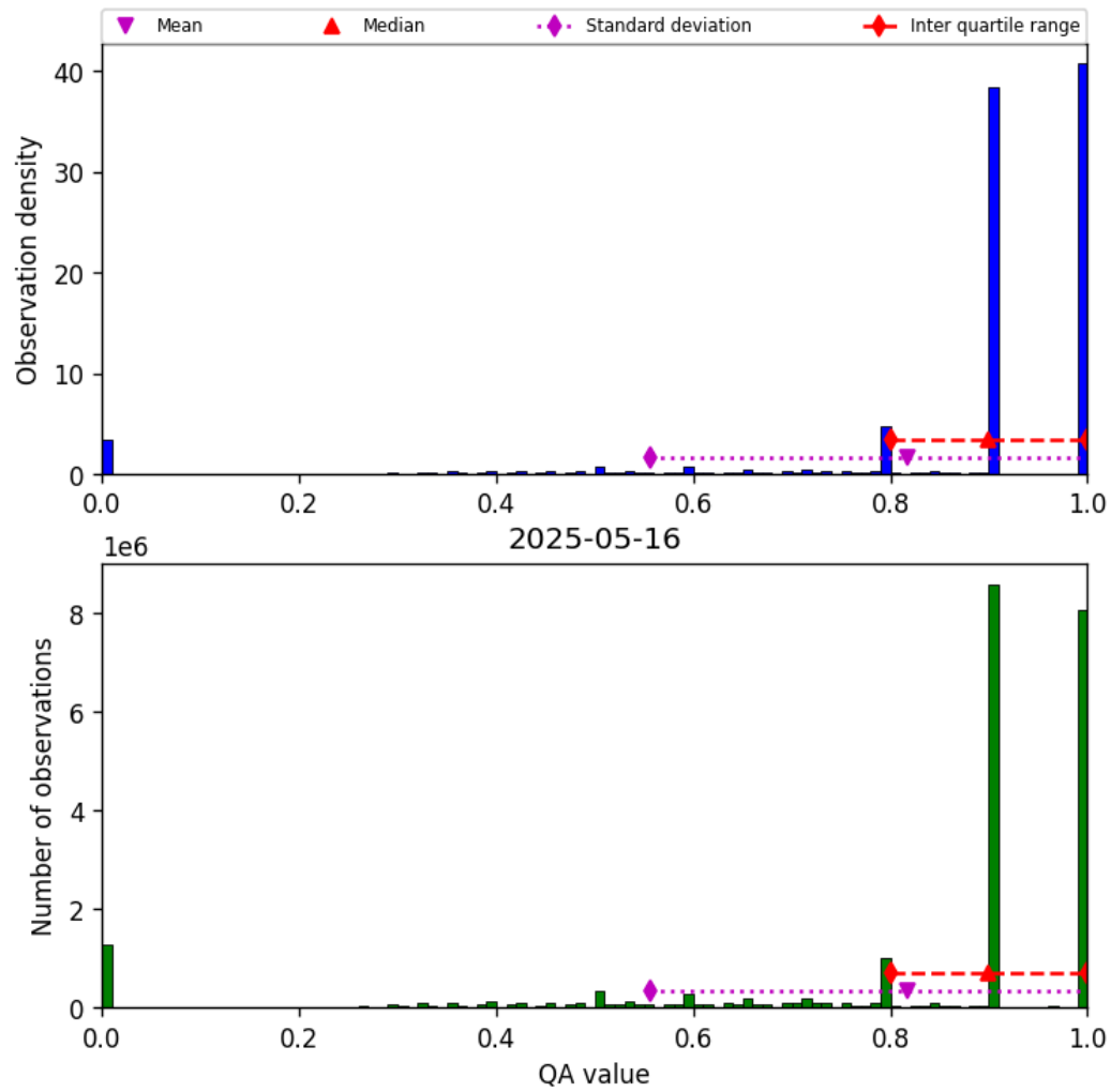
Figure 28: Histogram of “QA value” for 2025-05-16 to 2025-05-17
