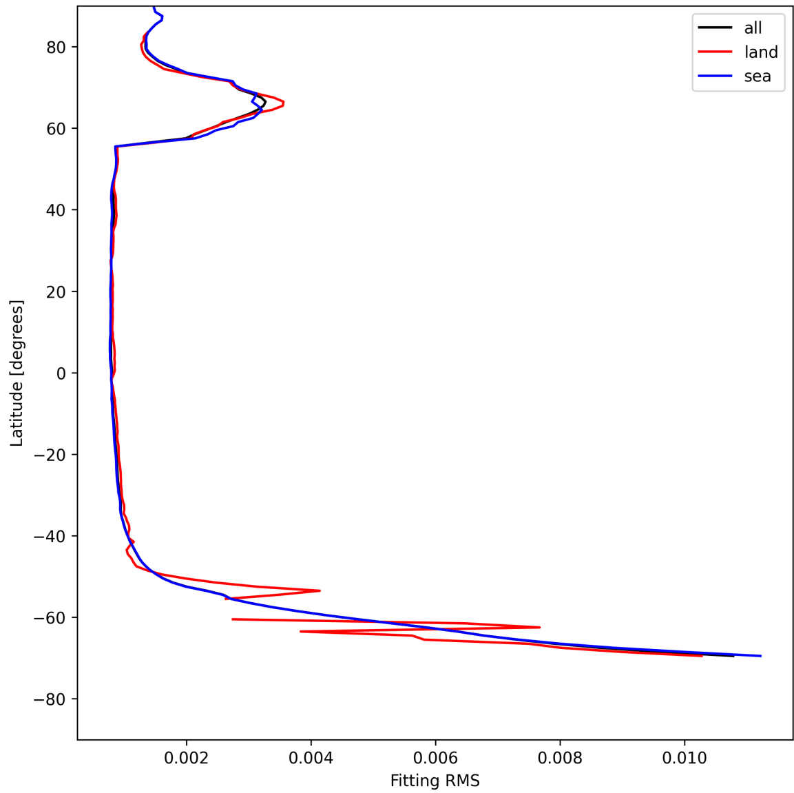
Figure 22: Zonal average of “Fitting RMS” for 2025-05-16 to 2025-05-17.
