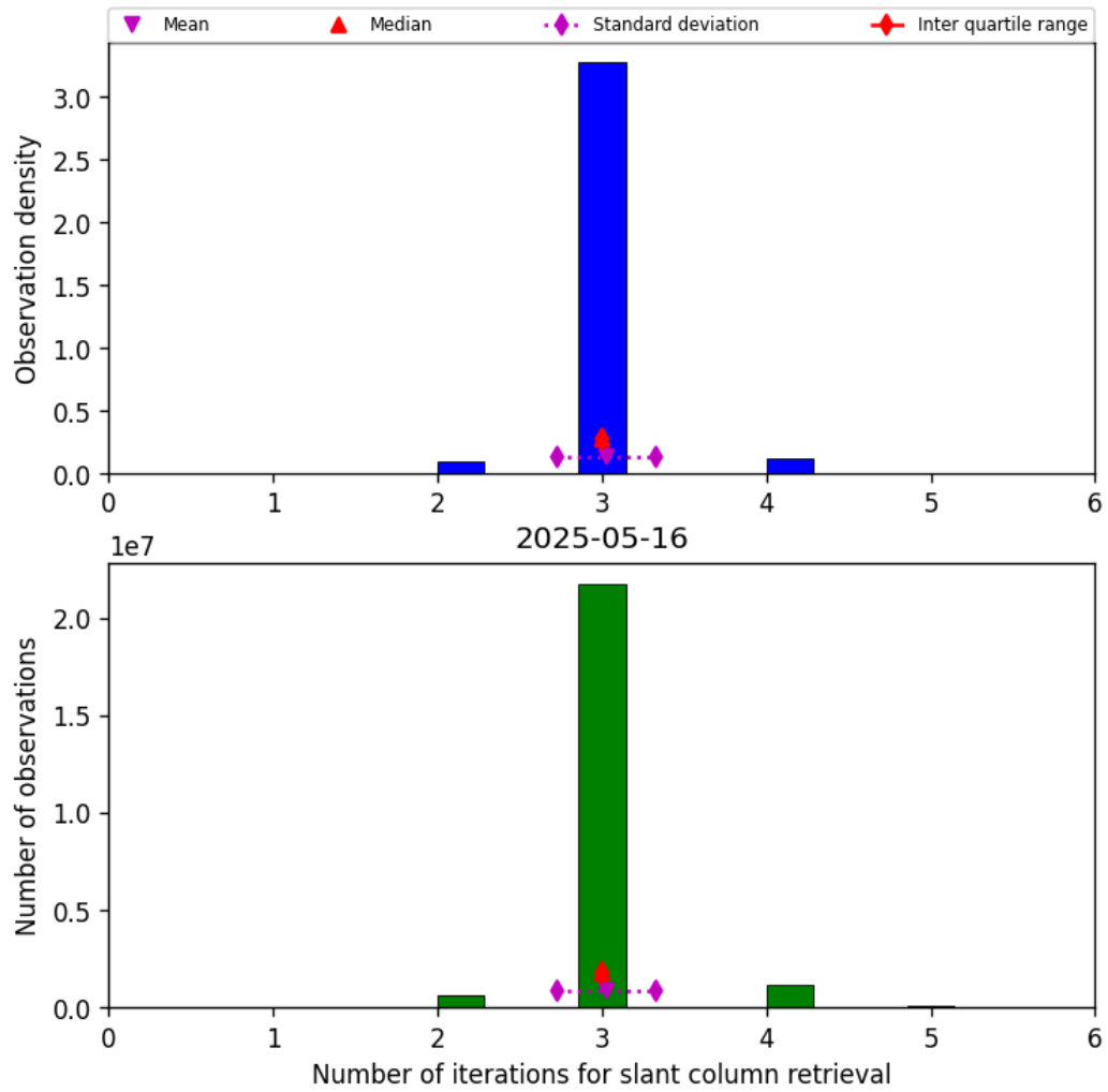
Figure 33: Histogram of “Number of iterations for slant column retrieval” for 2025-05-16 to 2025-05-17
