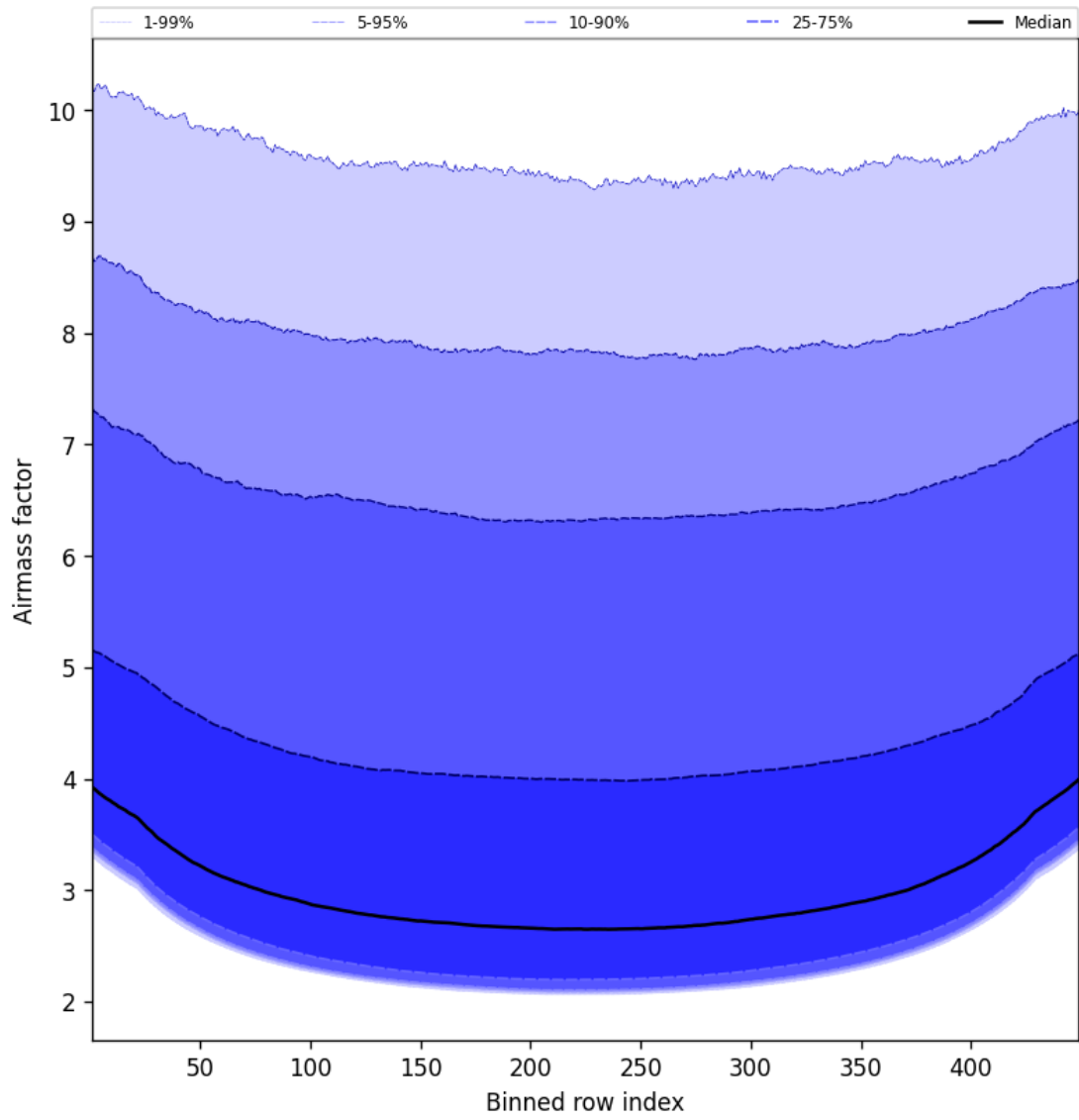
Figure 49: Along track statistics of “Airmass factor” for 2025-05-16 to 2025-05-17
