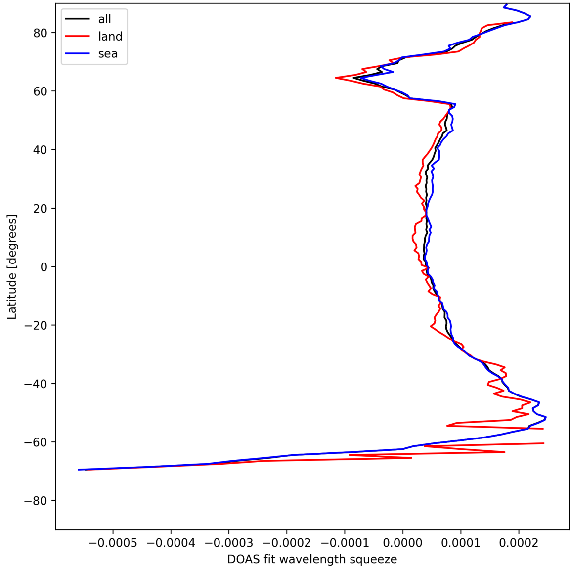
Figure 24: Zonal average of “DOAS fit wavelength squeeze” for 2025-05-16 to 2025-05-17.
