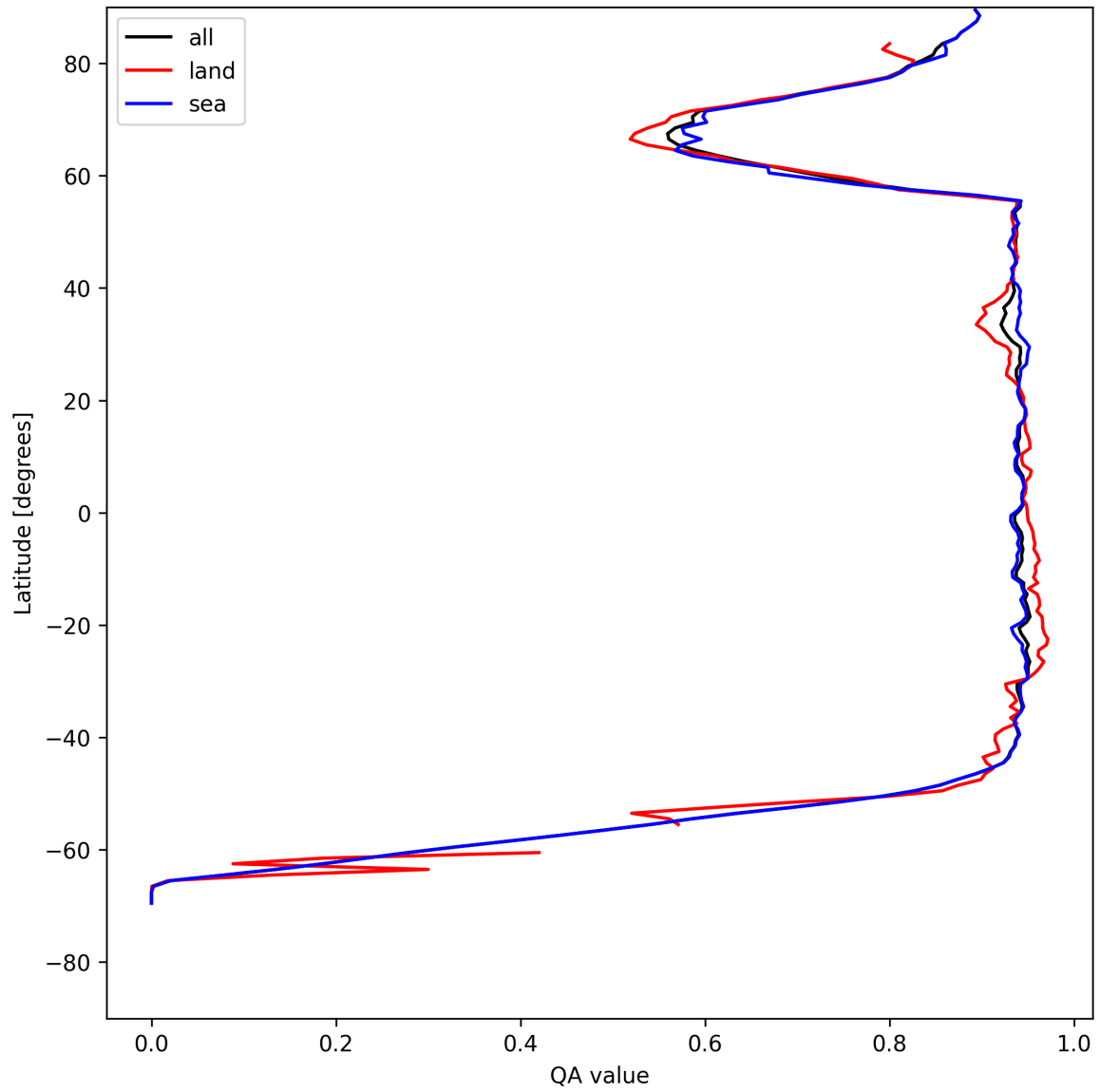
Figure 16: Zonal average of “QA value” for 2025-05-16 to 2025-05-17.
