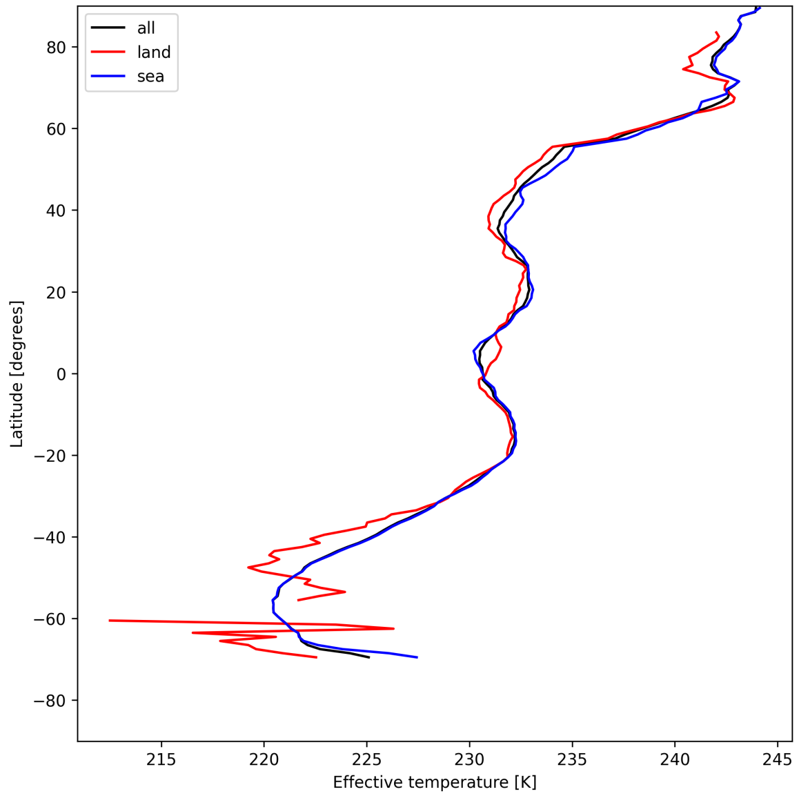
Figure 26: Zonal average of “Effective temperature” for 2025-05-16 to 2025-05-17.
