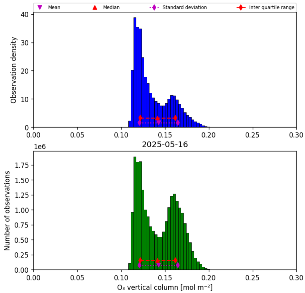
Figure 29: Histogram of “O 3 vertical column” for 2025-05-16 to 2025-05-17
