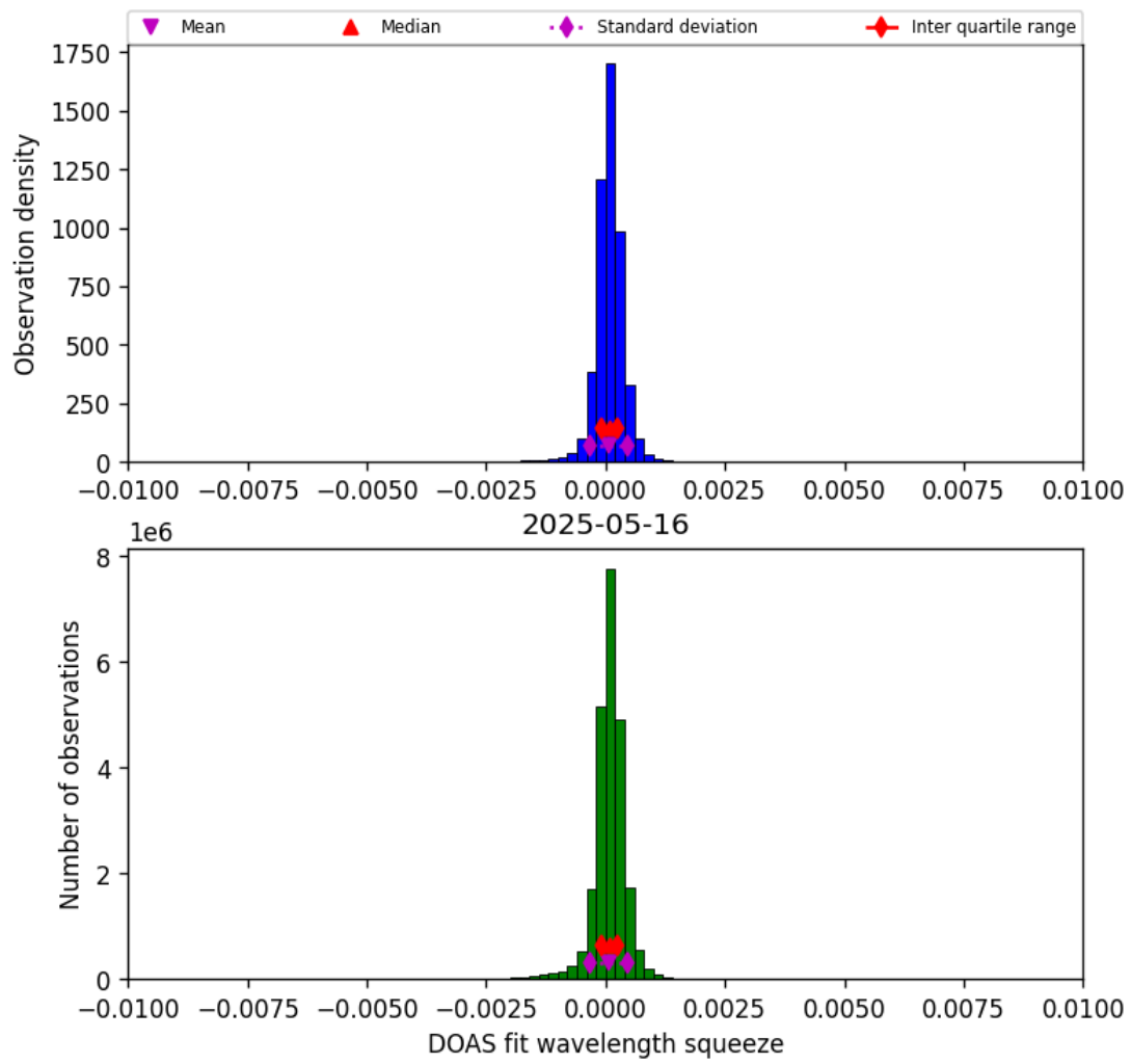
Figure 36: Histogram of “DOAS fit wavelength squeeze” for 2025-05-16 to 2025-05-17
