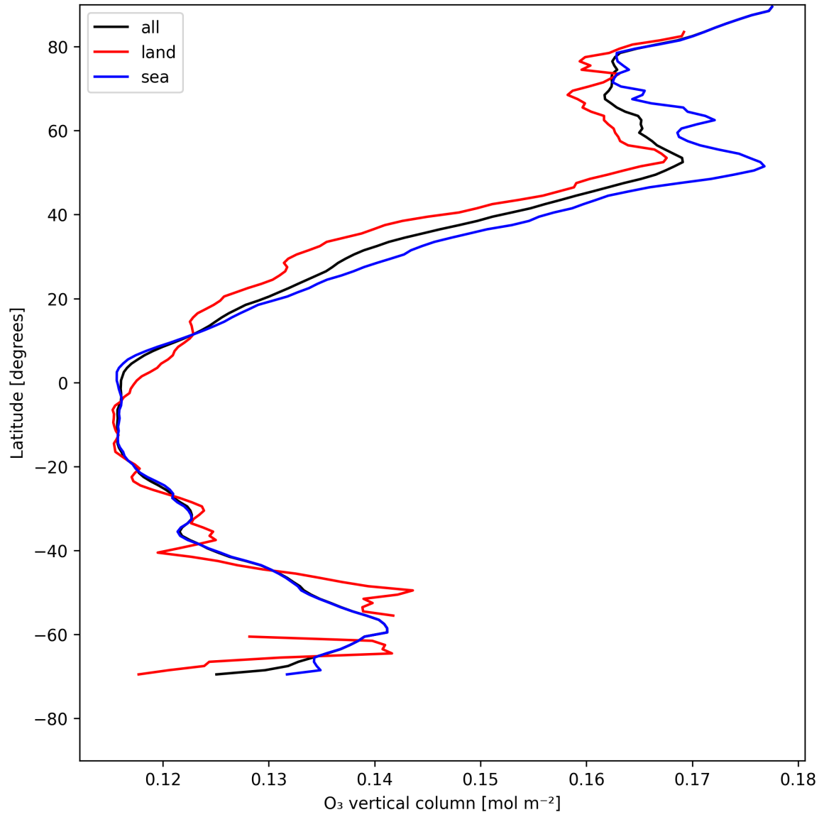
Figure 17: Zonal average of “O 3 vertical column” for 2025-05-16 to 2025-05-17.
