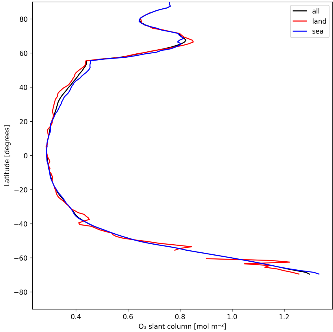
Figure 19: Zonal average of “O 3 slant column” for 2025-05-16 to 2025-05-17.
