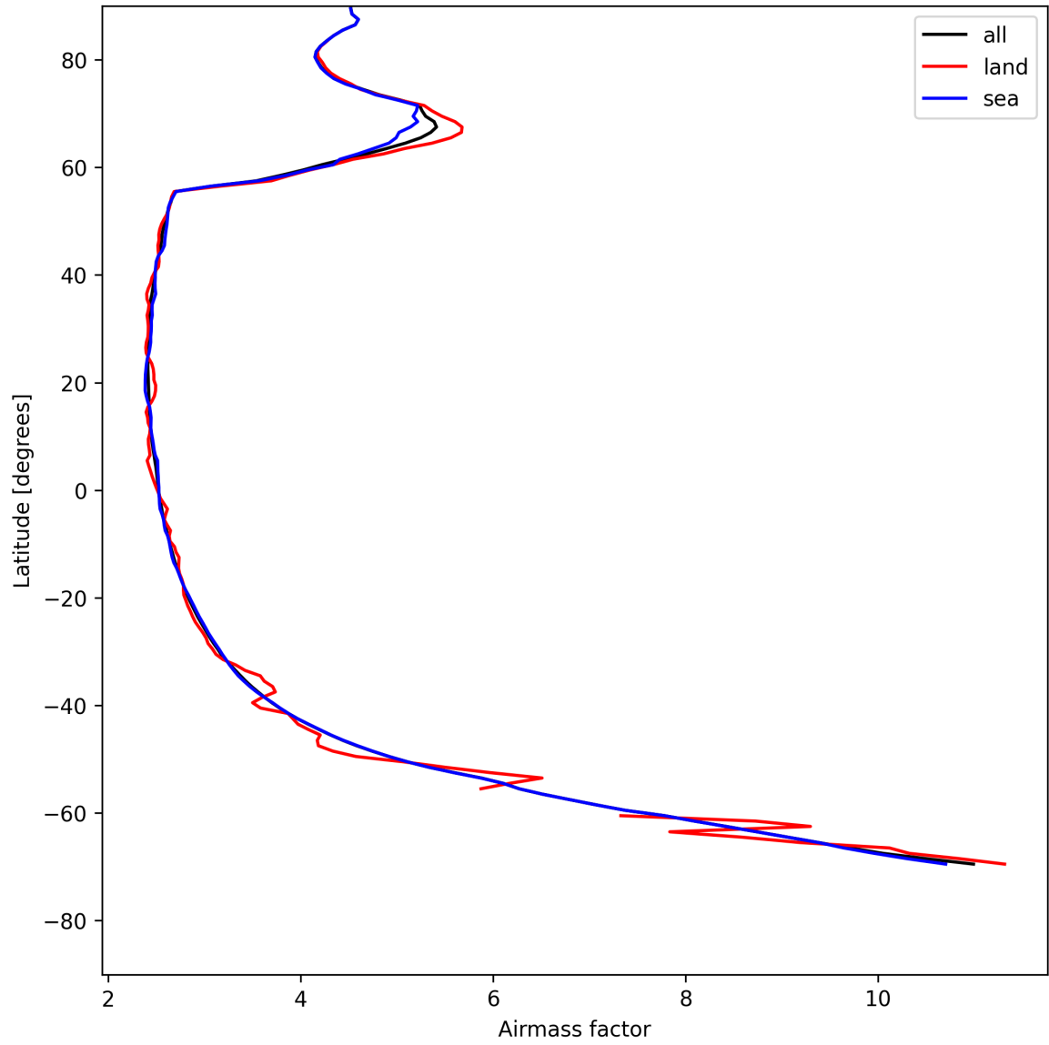
Figure 25: Zonal average of “Airmass factor” for 2025-05-16 to 2025-05-17.
