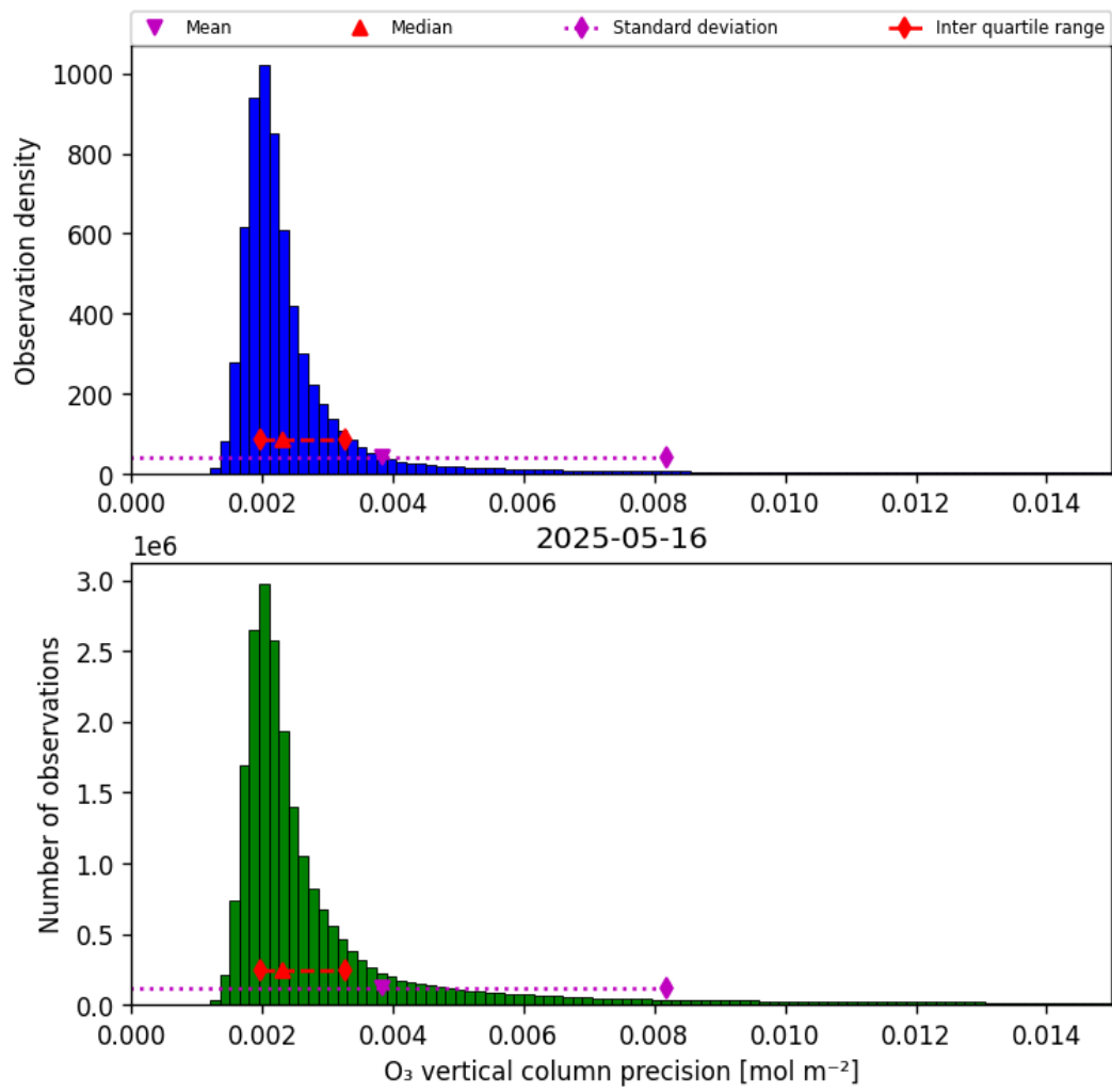
Figure 30: Histogram of “O 3 vertical column precision” for 2025-05-16 to 2025-05-17
