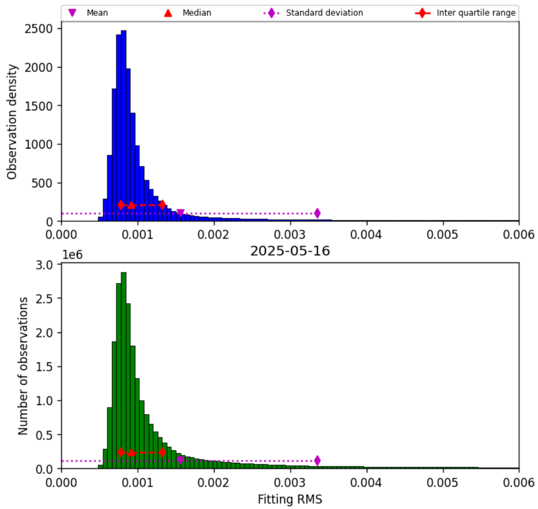
Figure 34: Histogram of “Fitting RMS” for 2025-05-16 to 2025-05-17
