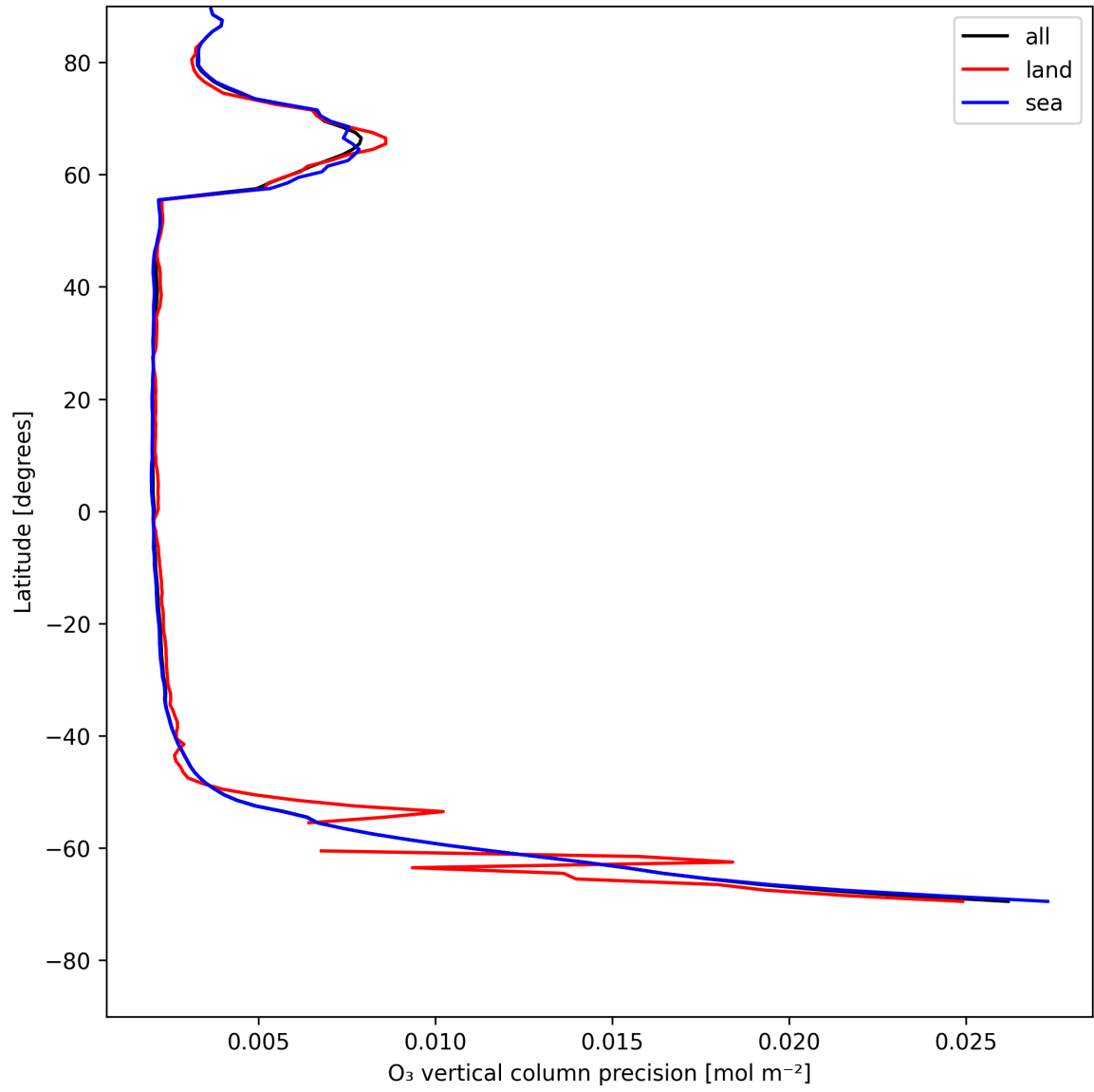
Figure 18: Zonal average of “O 3 vertical column precision” for 2025-05-16 to 2025-05-17.
