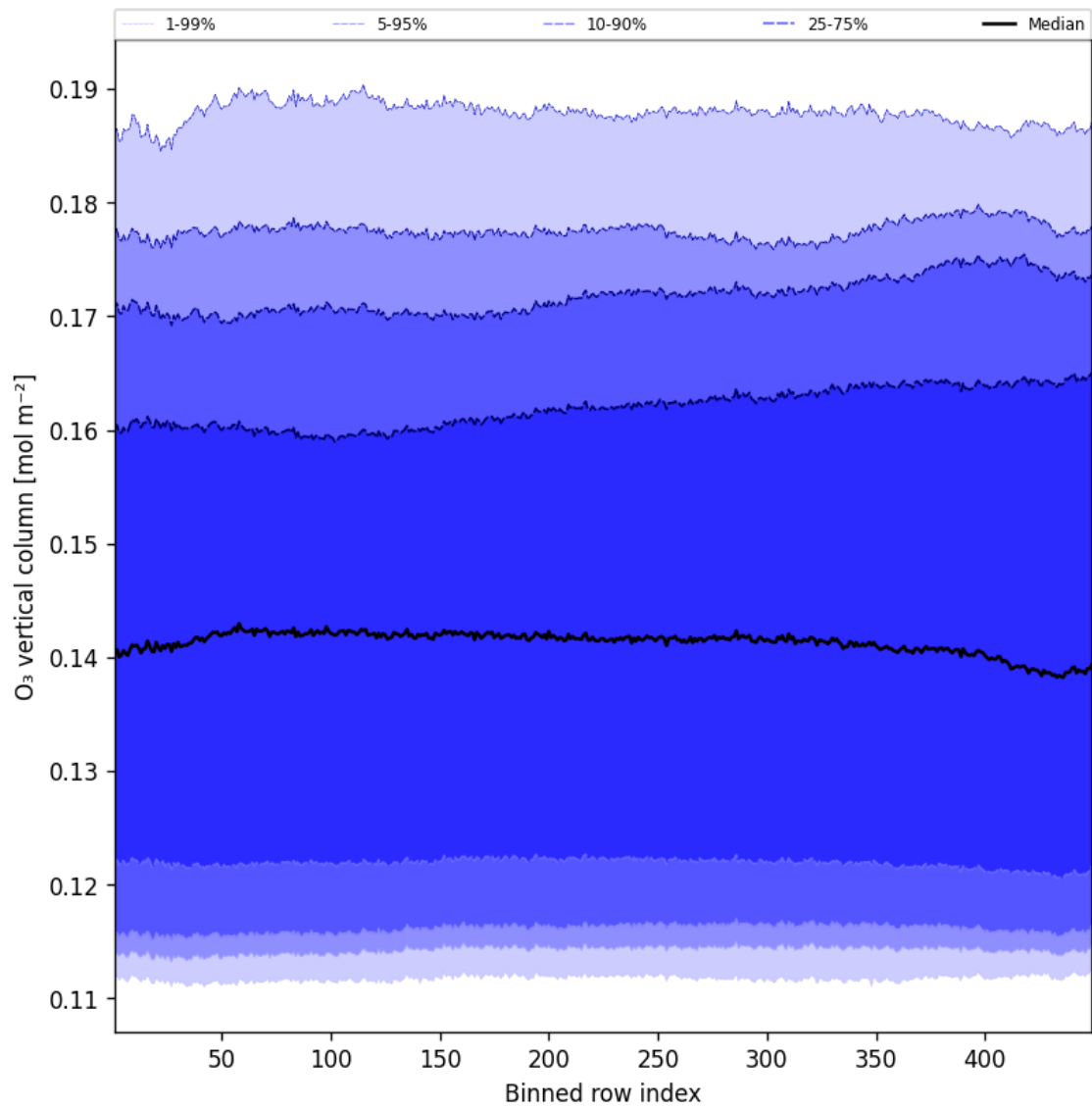
Figure 41: Along track statistics of “ O_3 vertical column” for 2025-05-16 to 2025-05-17
