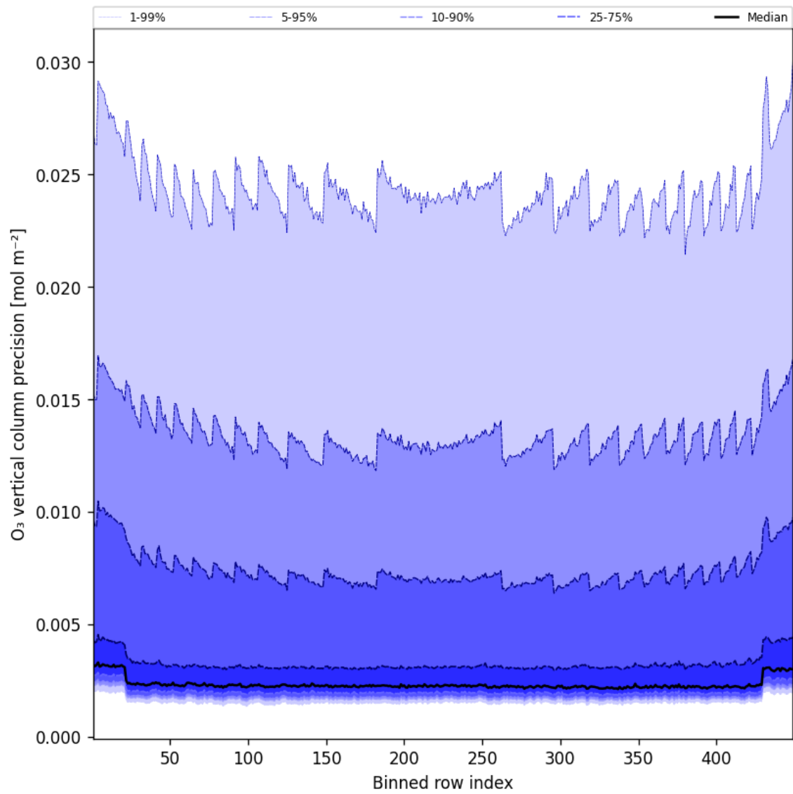
Figure 42: Along track statistics of “O 3 vertical column precision” for 2025-05-16 to 2025-05-17
