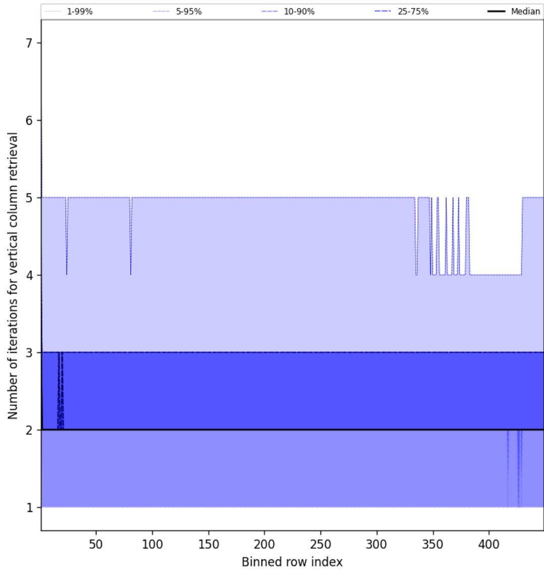
Figure 51: Along track statistics of “Number of iterations for vertical column retrieval” for 2025-05-16 to 2025-05-17
