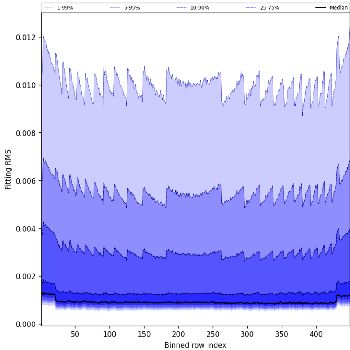
Figure 46: Along track statistics of “Fitting RMS” for 2025-05-16 to 2025-05-17
