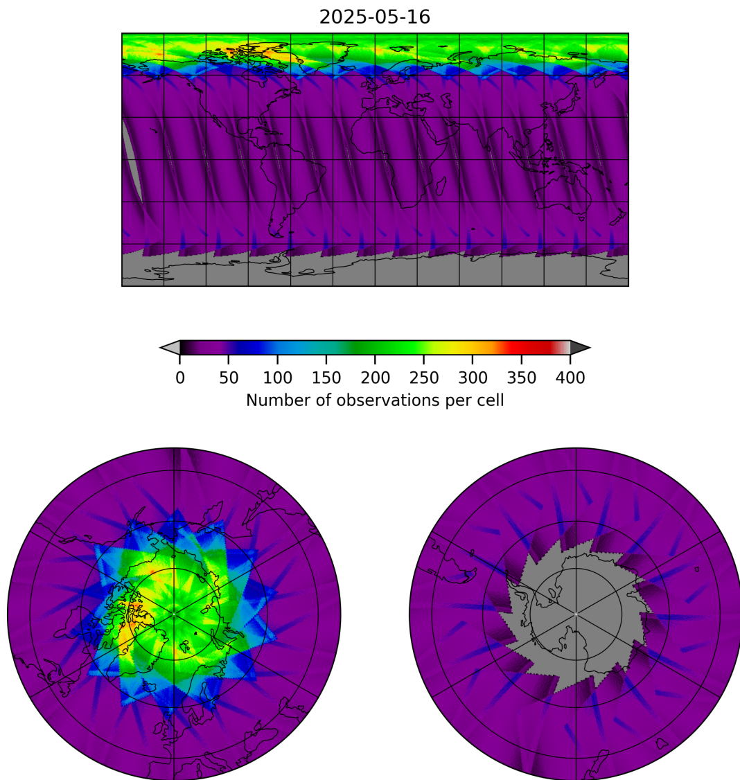
Figure 15: Map of the number of observations for 2025-05-16 to 2025-05-17
