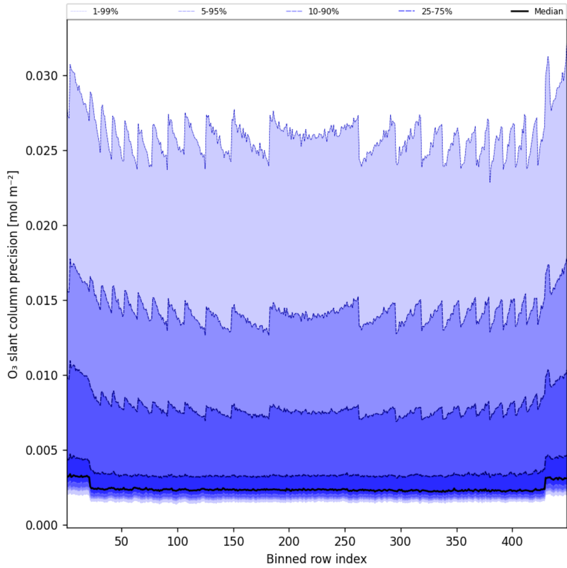
Figure 44: Along track statistics of “O 3 slant column precision” for 2025-05-16 to 2025-05-17
