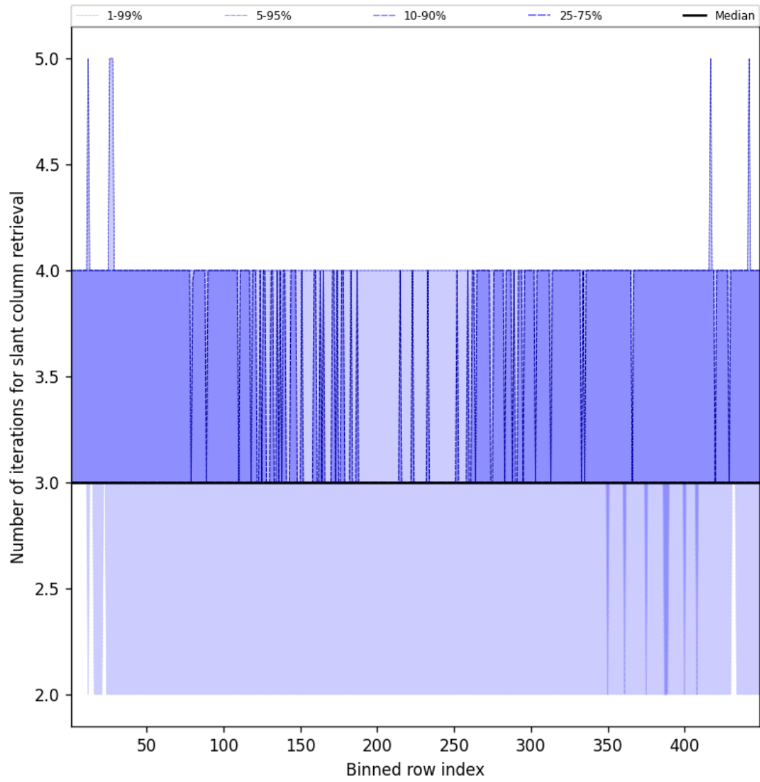
Figure 45: Along track statistics of “Number of iterations for slant column retrieval” for 2025-05-16 to 2025-05-17
