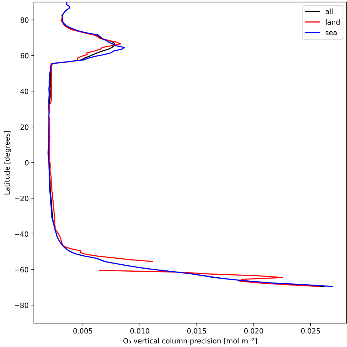
Figure 18: Zonal average of “O 3 vertical column precision” for 2025-05-17 to 2025-05-18.
