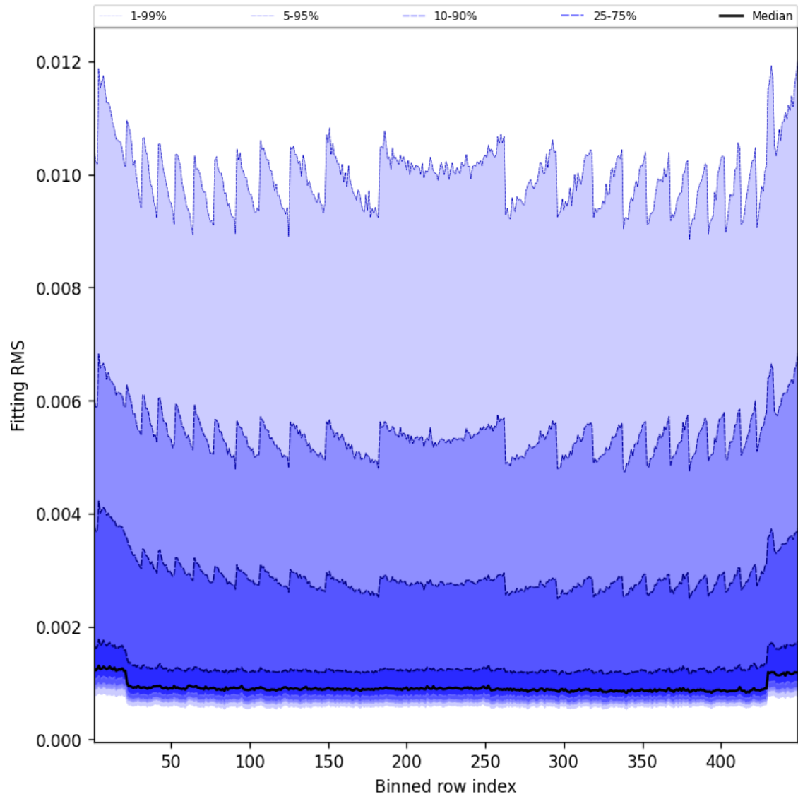
Figure 46: Along track statistics of “Fitting RMS” for 2025-05-17 to 2025-05-18
