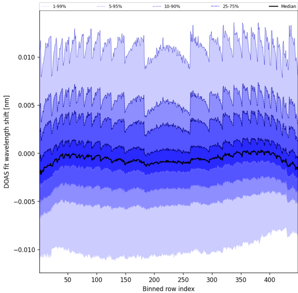
Figure 47: Along track statistics of “DOAS fit wavelength shift” for 2025-05-17 to 2025-05-18
