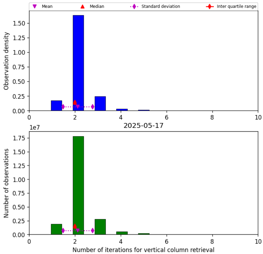
Figure 39: Histogram of “Number of iterations for vertical column retrieval” for 2025-05-17 to 2025-05-18
