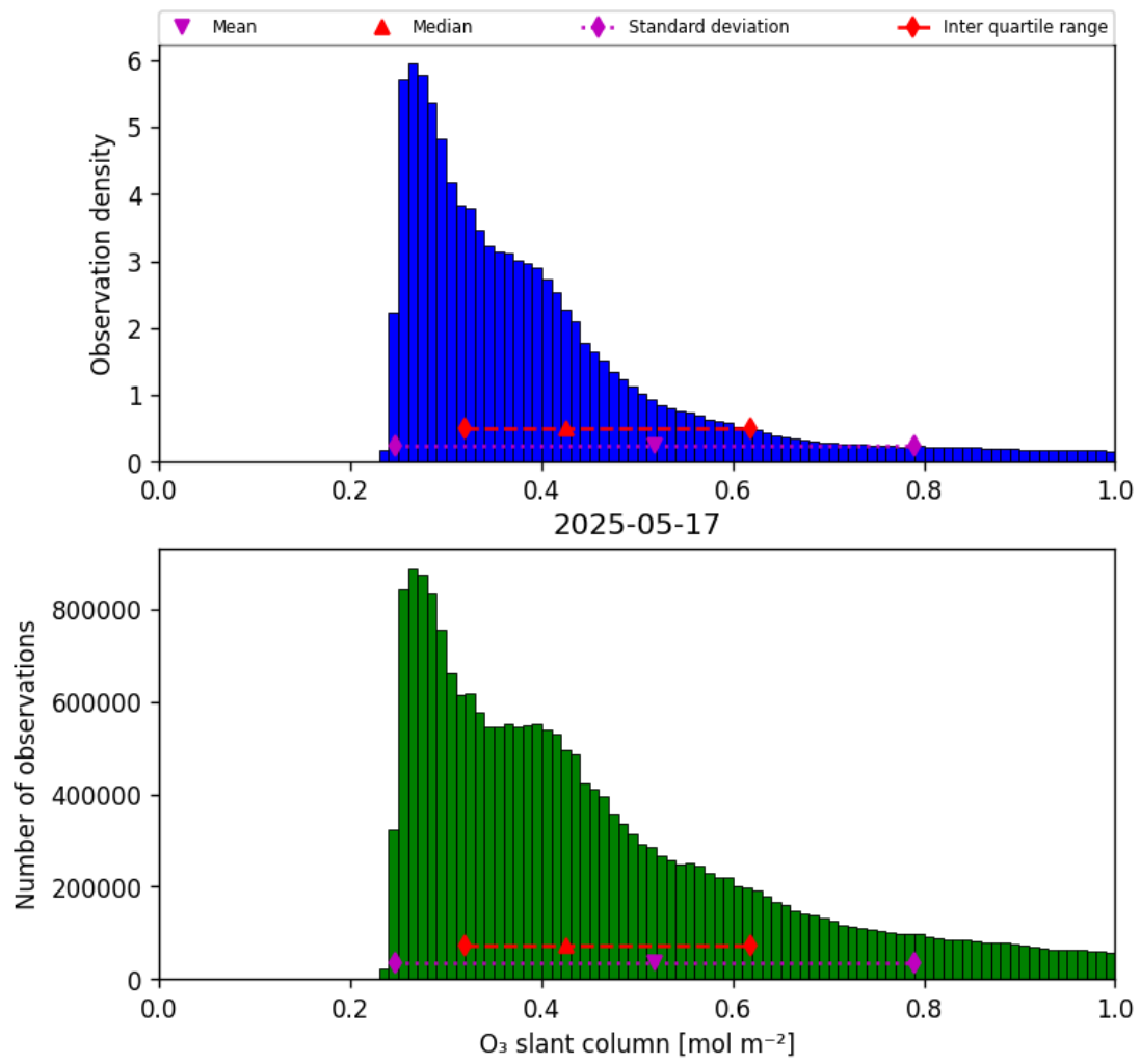
Figure 31: Histogram of “O 3 slant column” for 2025-05-17 to 2025-05-18
