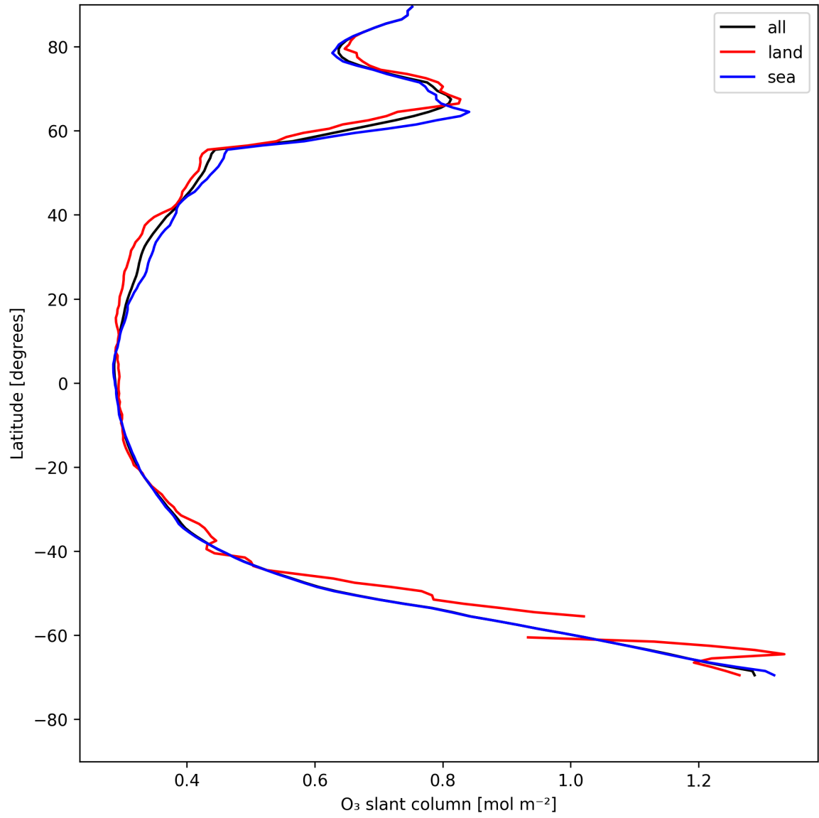
Figure 19: Zonal average of “O 3 slant column” for 2025-05-17 to 2025-05-18.
