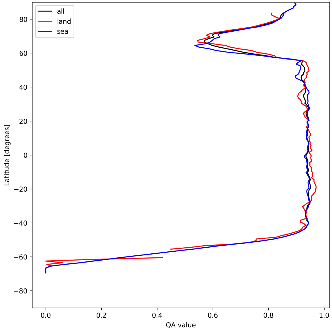
Figure 16: Zonal average of “QA value” for 2025-05-17 to 2025-05-18.
