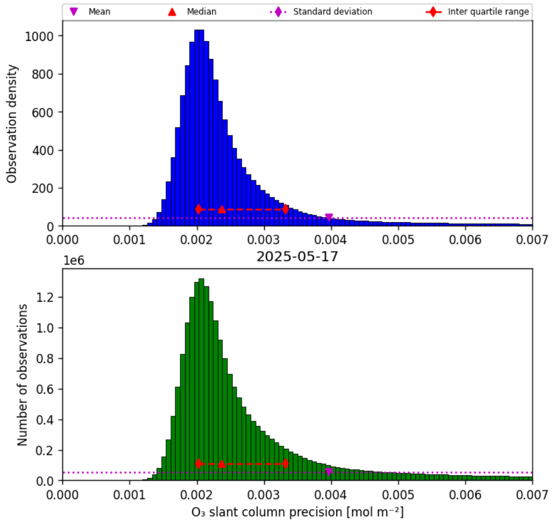
Figure 32: Histogram of “O 3 slant column precision” for 2025-05-17 to 2025-05-18
