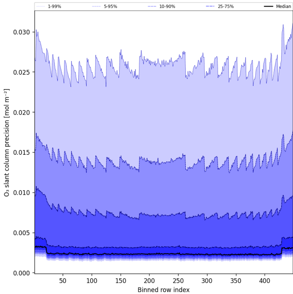
Figure 44: Along track statistics of “O 3 slant column precision” for 2025-05-17 to 2025-05-18
