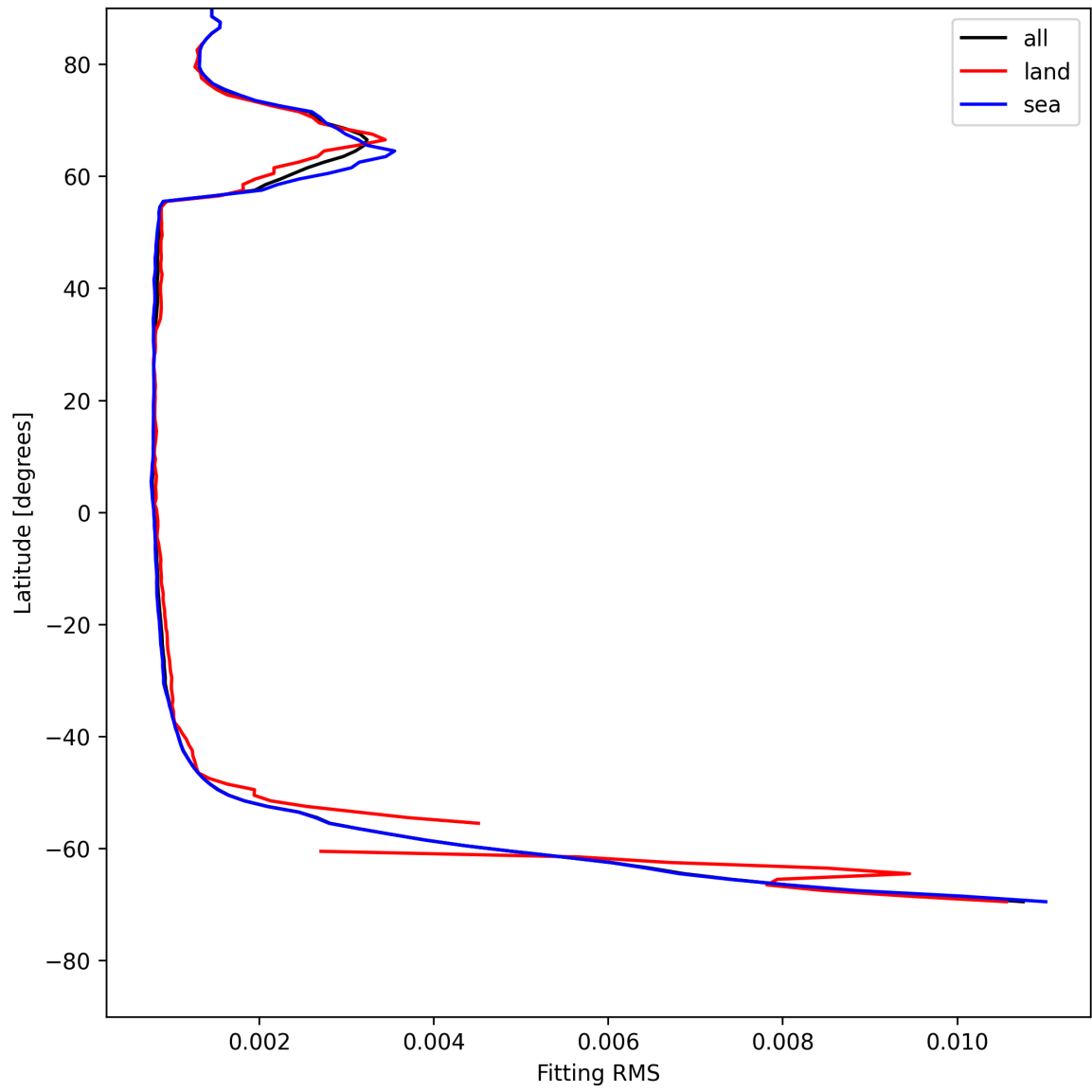
Figure 22: Zonal average of “Fitting RMS” for 2025-05-17 to 2025-05-18.
