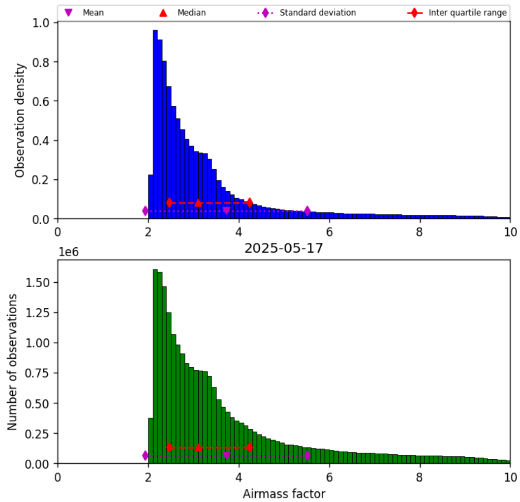
Figure 37: Histogram of “Airmass factor” for 2025-05-17 to 2025-05-18
