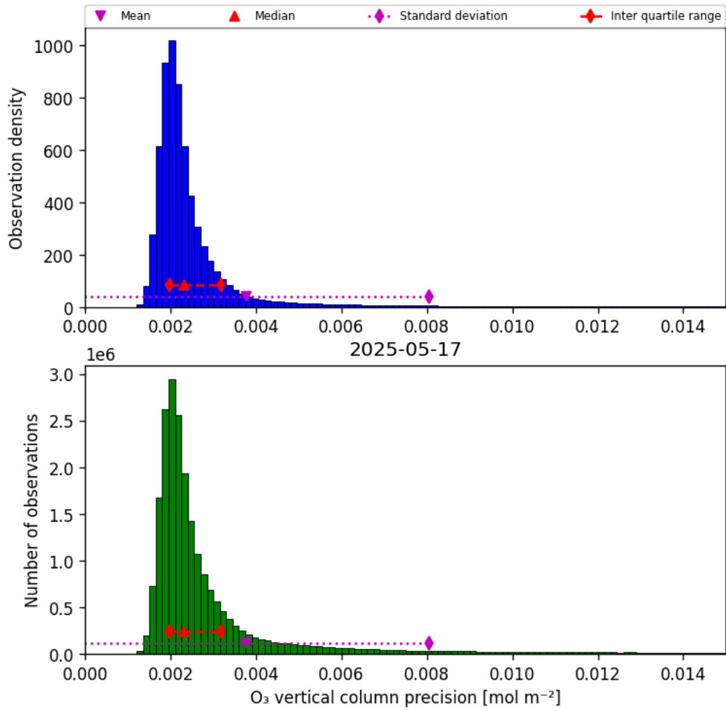
Figure 30: Histogram of “O 3 vertical column precision” for 2025-05-17 to 2025-05-18
