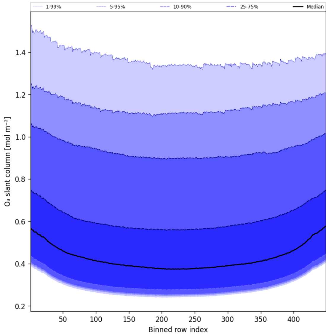
Figure 43: Along track statistics of “O 3 slant column” for 2025-05-17 to 2025-05-18
