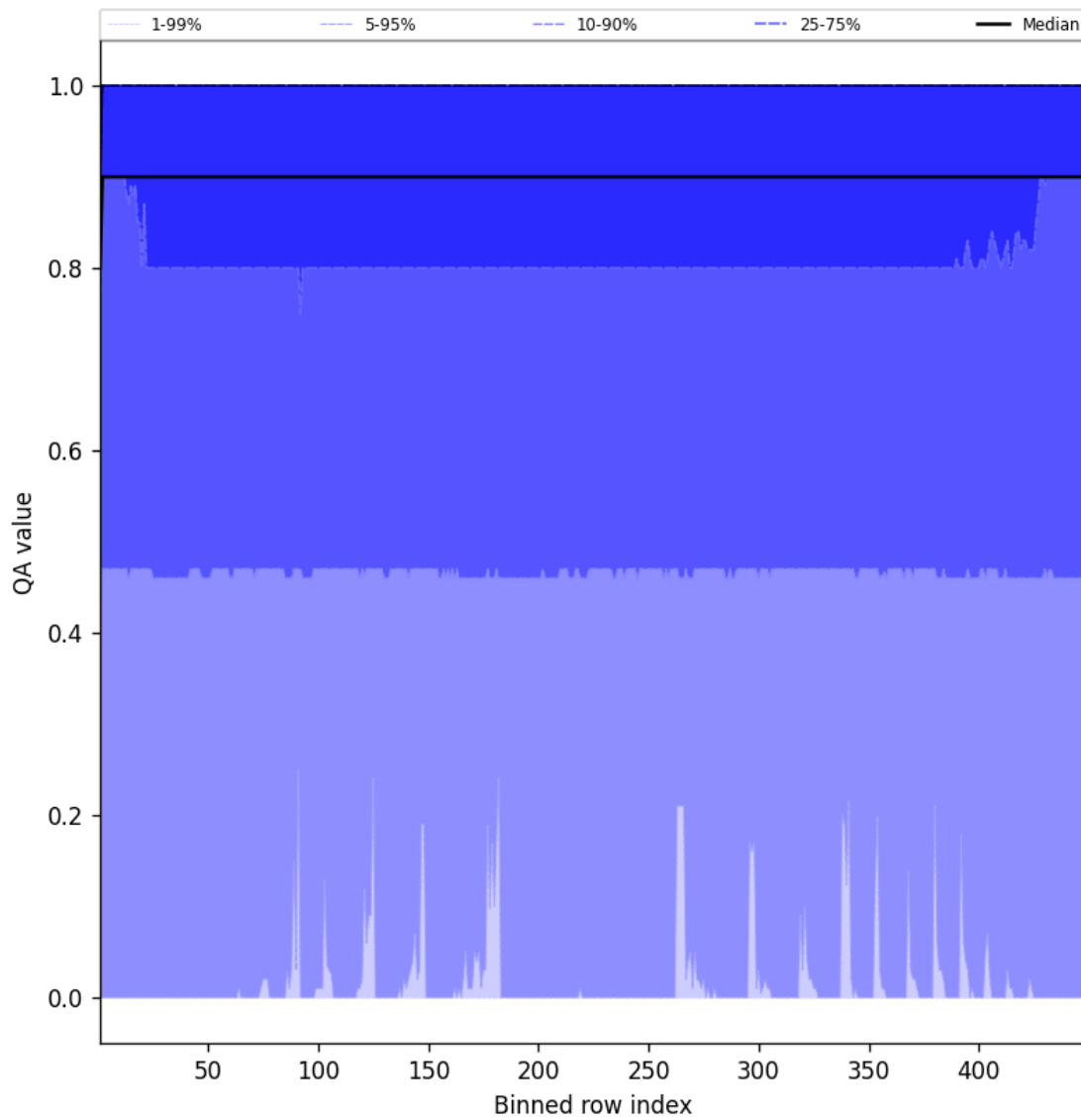
Figure 40: Along track statistics of “QA value” for 2025-05-17 to 2025-05-18
