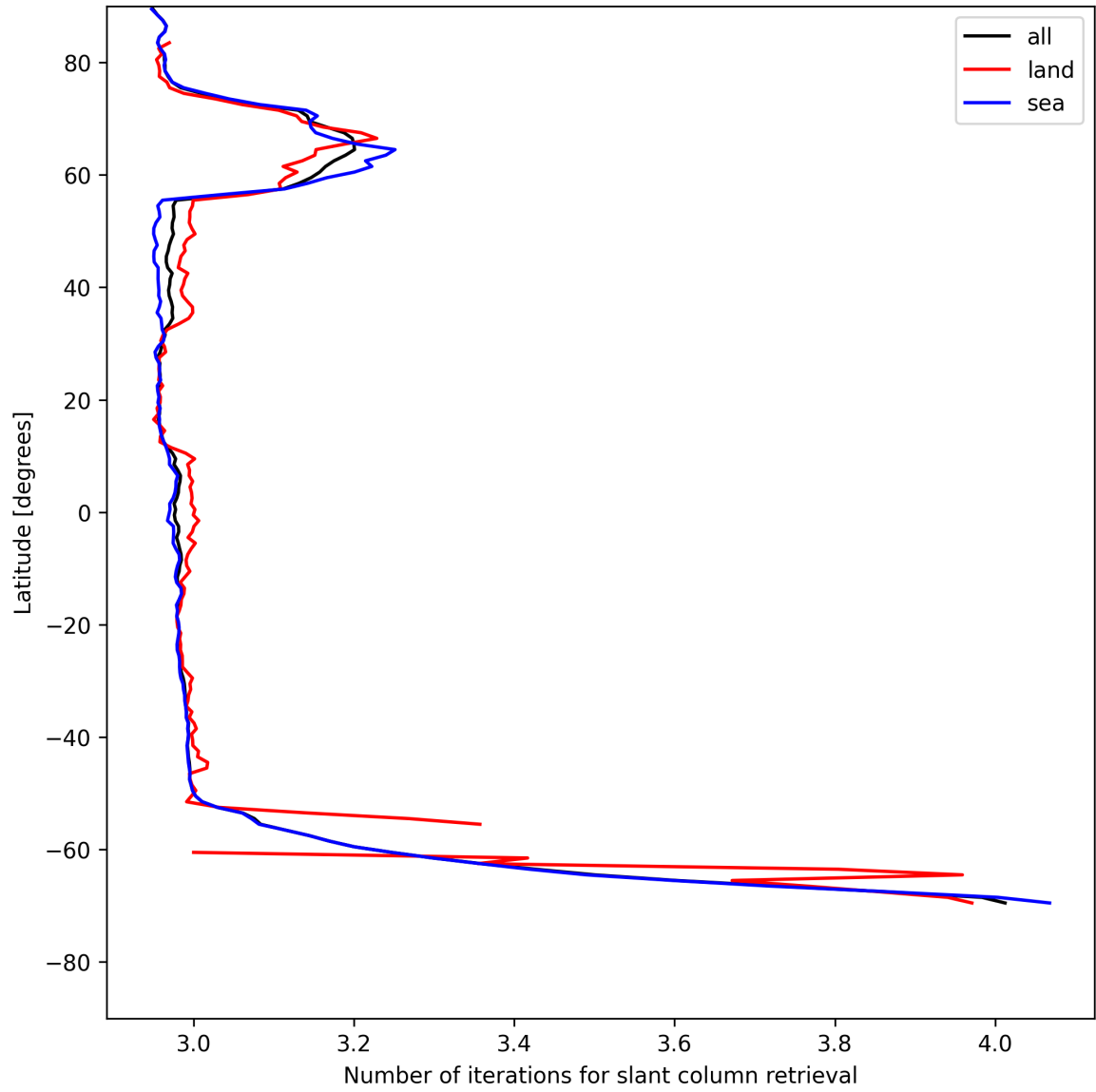
Figure 21: Zonal average of “Number of iterations for slant column retrieval” for 2025-05-17 to 2025-05-18.
