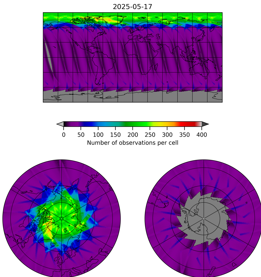
Figure 15: Map of the number of observations for 2025-05-17 to 2025-05-18
