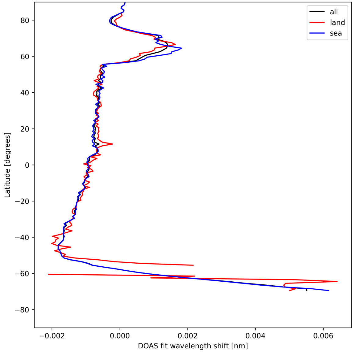
Figure 23: Zonal average of “DOAS fit wavelength shift” for 2025-05-17 to 2025-05-18.
