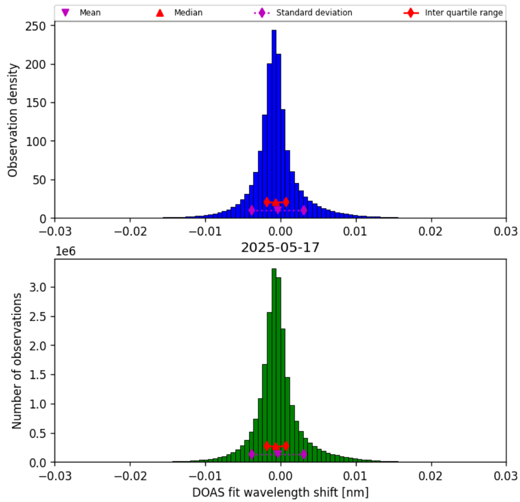
Figure 35: Histogram of “DOAS fit wavelength shift” for 2025-05-17 to 2025-05-18
