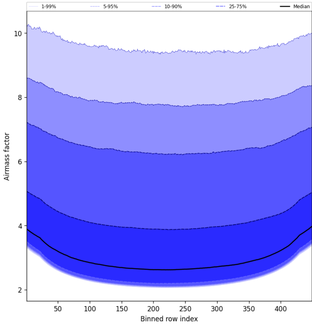
Figure 49: Along track statistics of “Airmass factor” for 2025-05-17 to 2025-05-18
