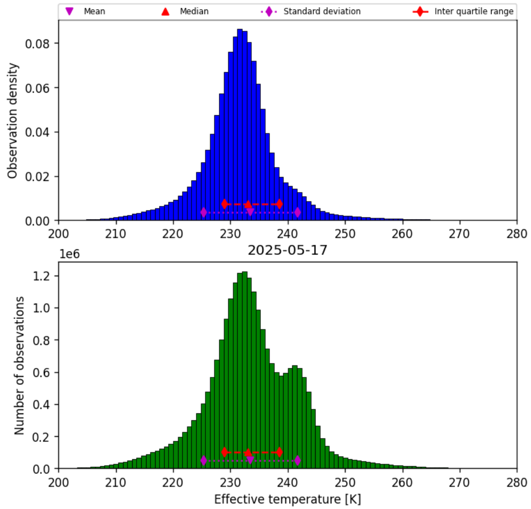
Figure 38: Histogram of “Effective temperature” for 2025-05-17 to 2025-05-18
