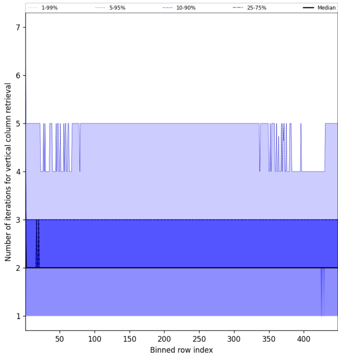
Figure 51: Along track statistics of “Number of iterations for vertical column retrieval” for 2025-05-17 to 2025-05-18
