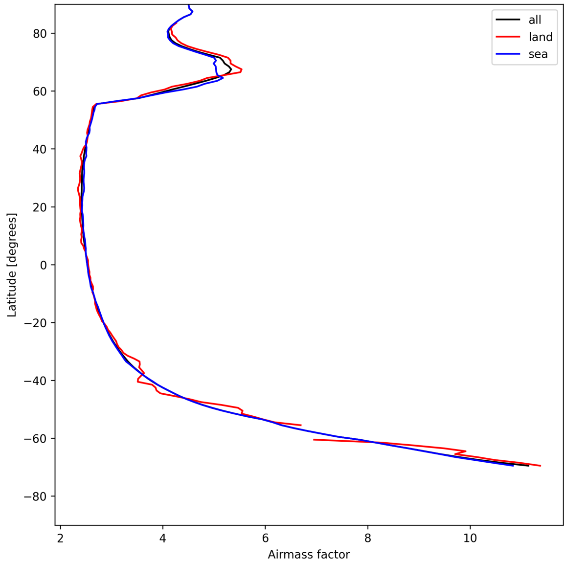
Figure 25: Zonal average of “Airmass factor” for 2025-05-17 to 2025-05-18.
