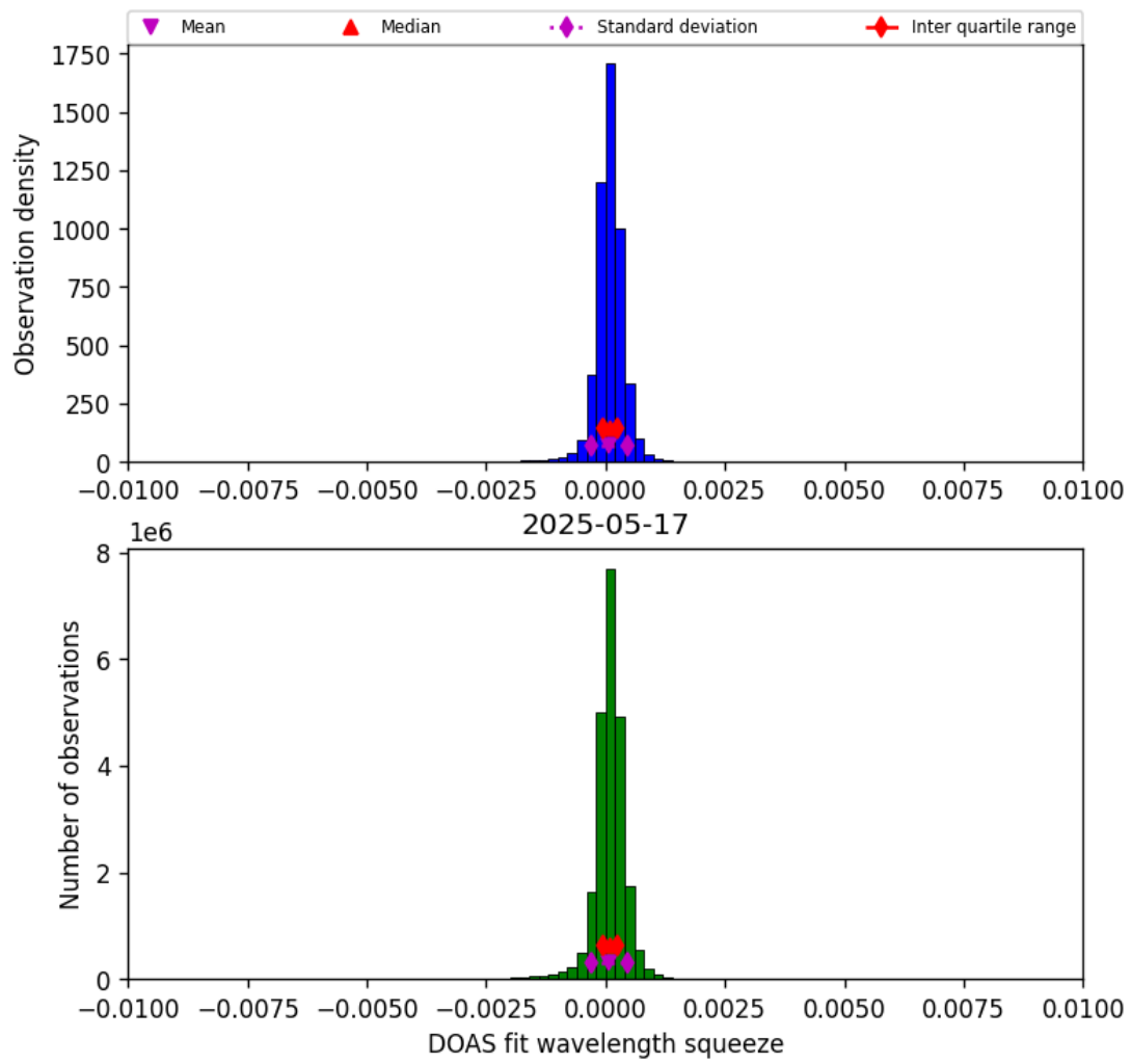
Figure 36: Histogram of “DOAS fit wavelength squeeze” for 2025-05-17 to 2025-05-18
