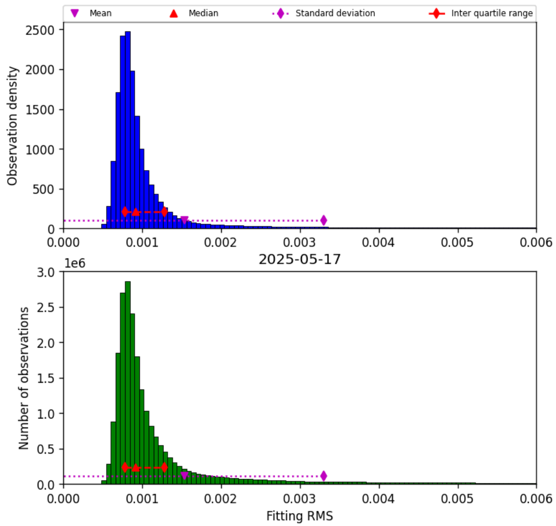
Figure 34: Histogram of “Fitting RMS” for 2025-05-17 to 2025-05-18
