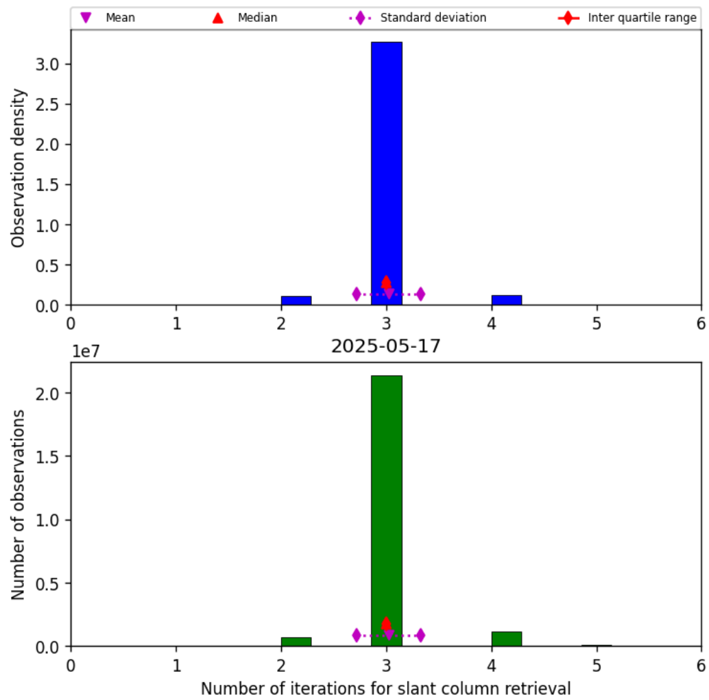
Figure 33: Histogram of “Number of iterations for slant column retrieval” for 2025-05-17 to 2025-05-18
