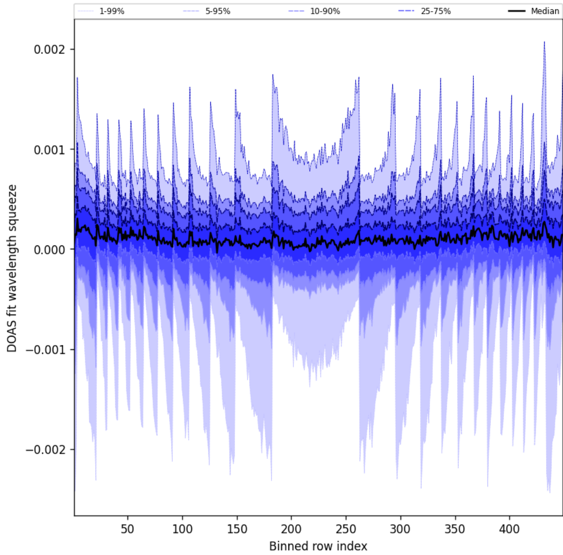
Figure 48: Along track statistics of “DOAS fit wavelength squeeze” for 2025-05-17 to 2025-05-18
