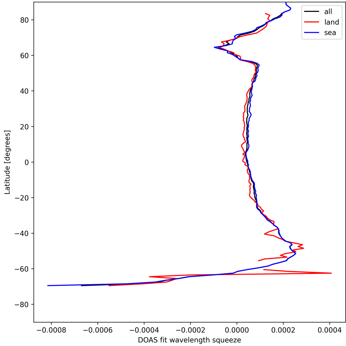
Figure 24: Zonal average of “DOAS fit wavelength squeeze” for 2025-05-17 to 2025-05-18.
