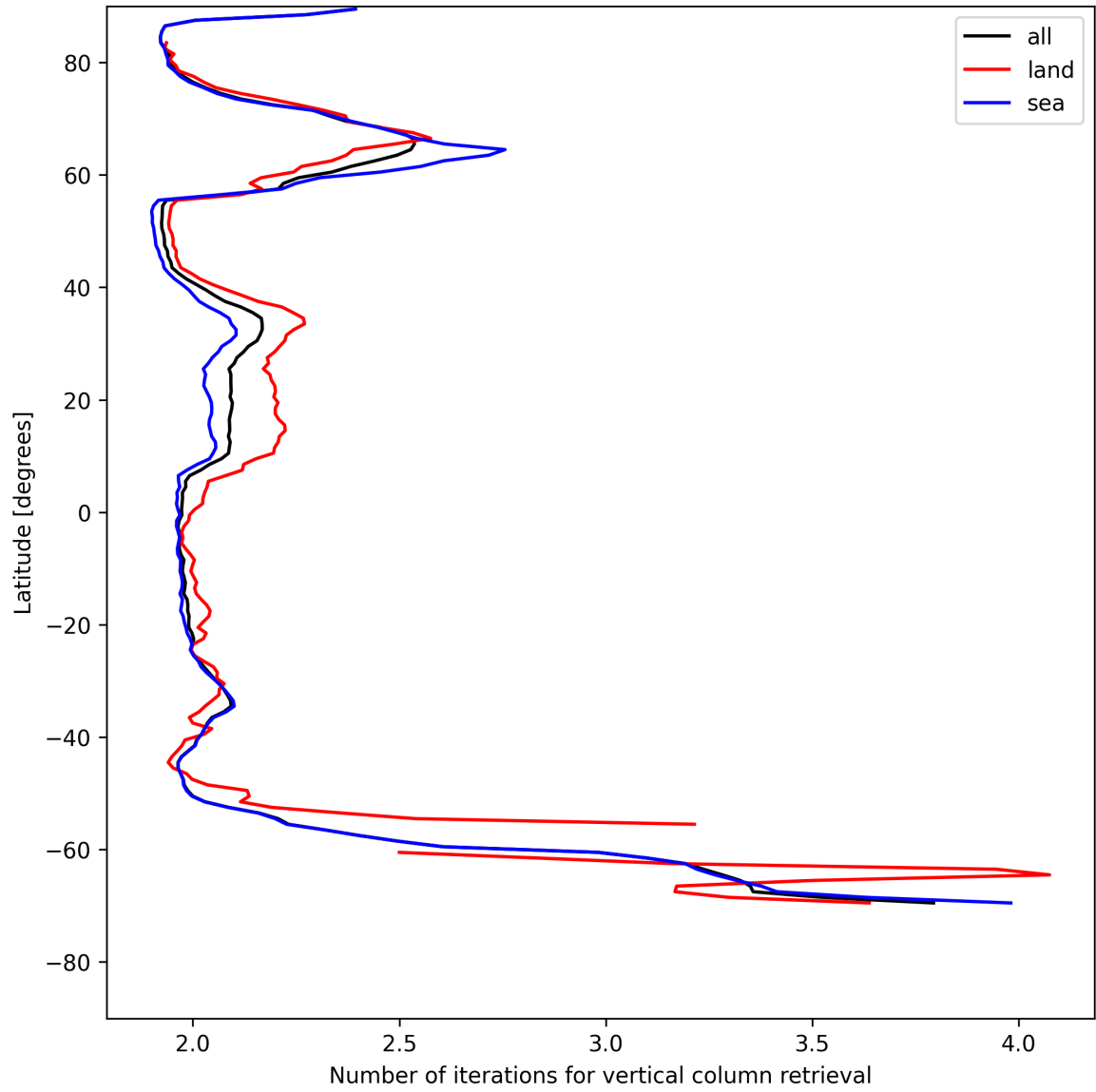
Figure 27: Zonal average of “Number of iterations for vertical column retrieval” for 2025-05-17 to 2025-05-18.
