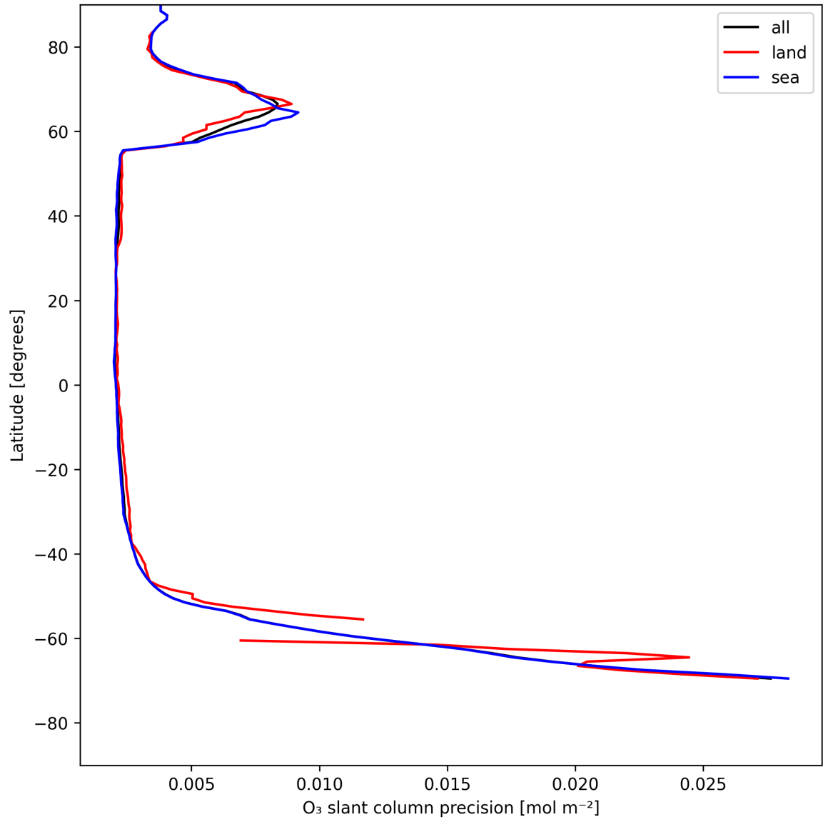
Figure 20: Zonal average of "O 3 slant column precision" for 2025-05-17 to 2025-05-18.
