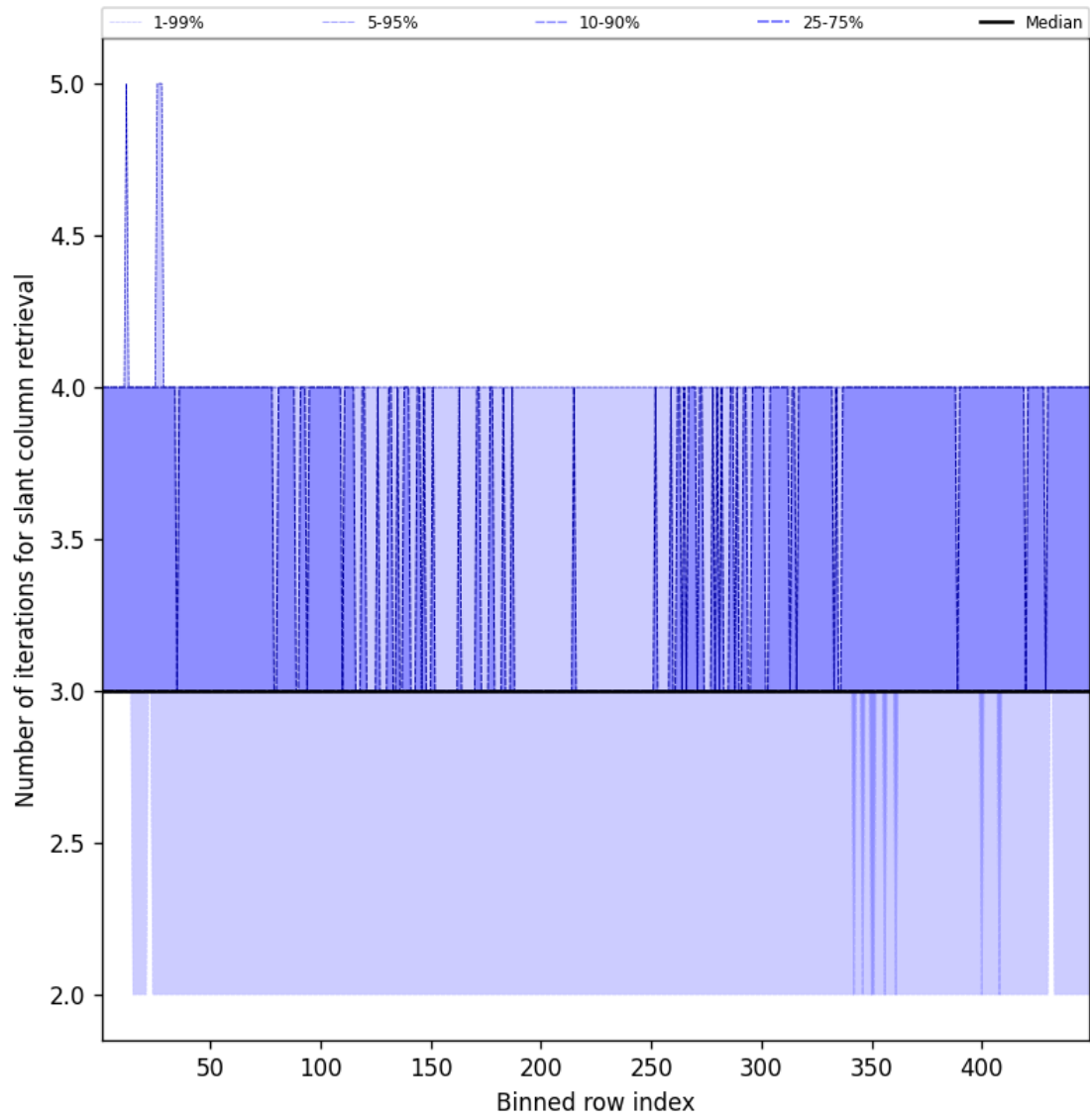
Figure 45: Along track statistics of “Number of iterations for slant column retrieval” for 2025-05-17 to 2025-05-18
