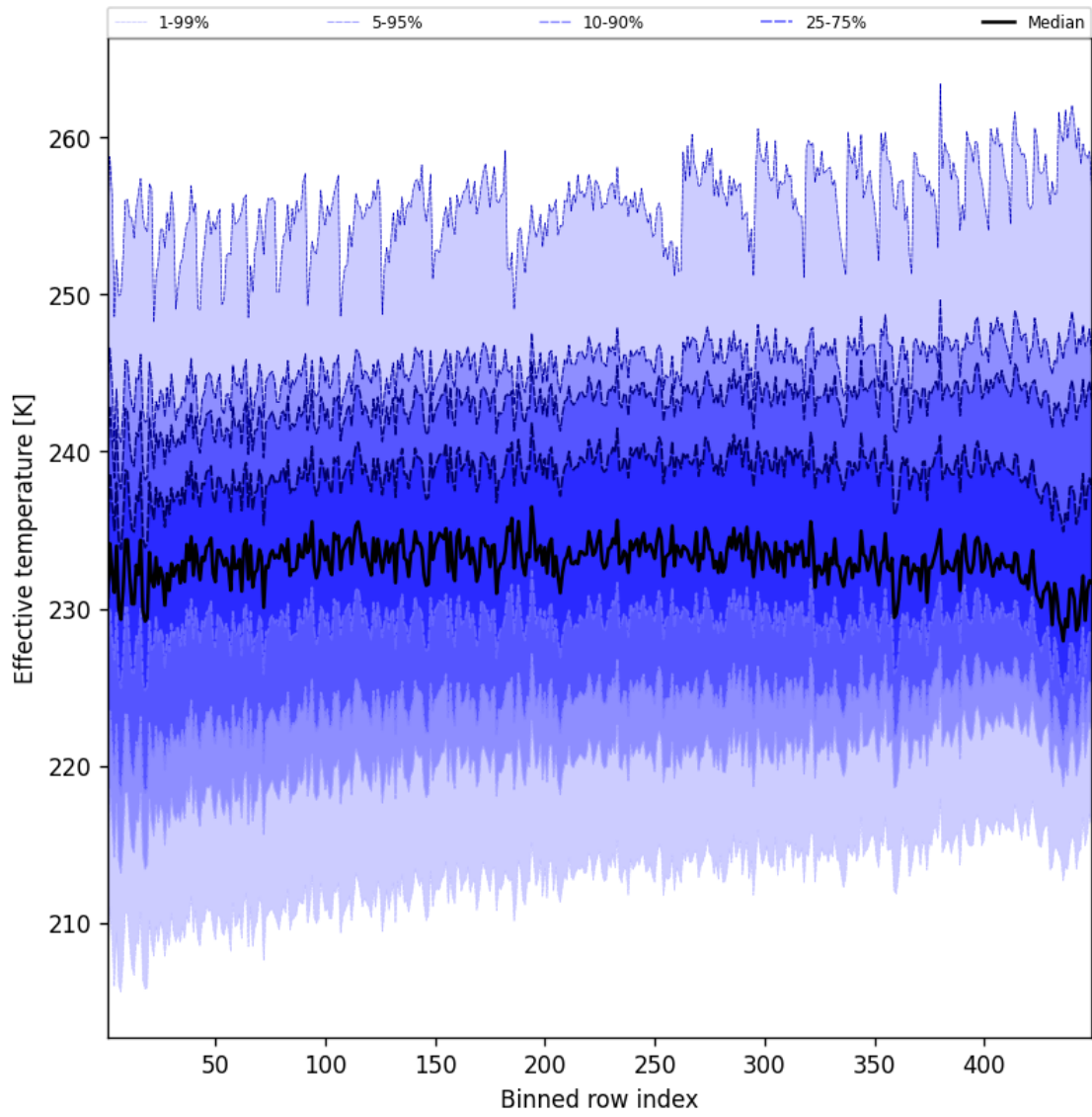
Figure 50: Along track statistics of “Effective temperature” for 2025-05-17 to 2025-05-18
