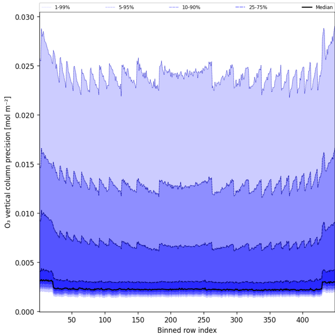
Figure 42: Along track statistics of “O 3 vertical column precision” for 2025-05-17 to 2025-05-18
