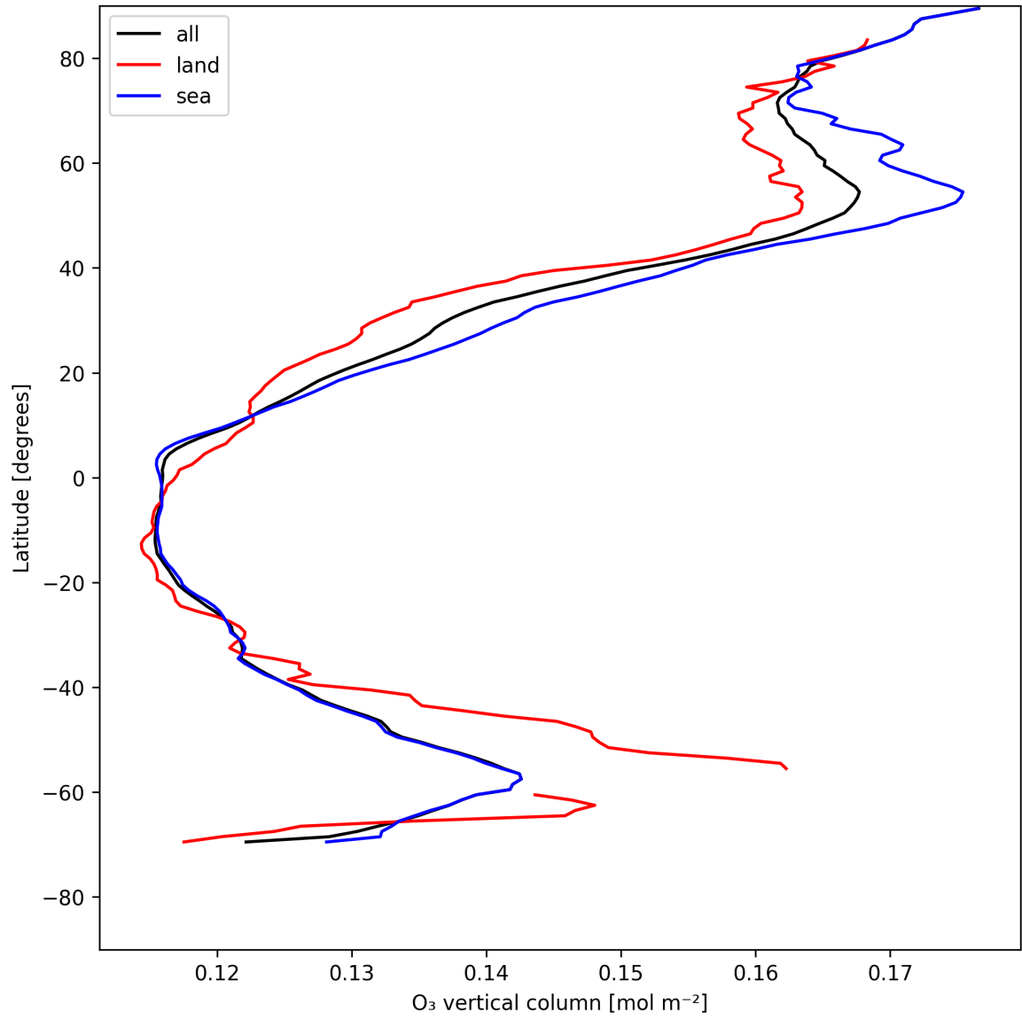
Figure 17: Zonal average of “O 3 vertical column” for 2025-05-17 to 2025-05-18.
