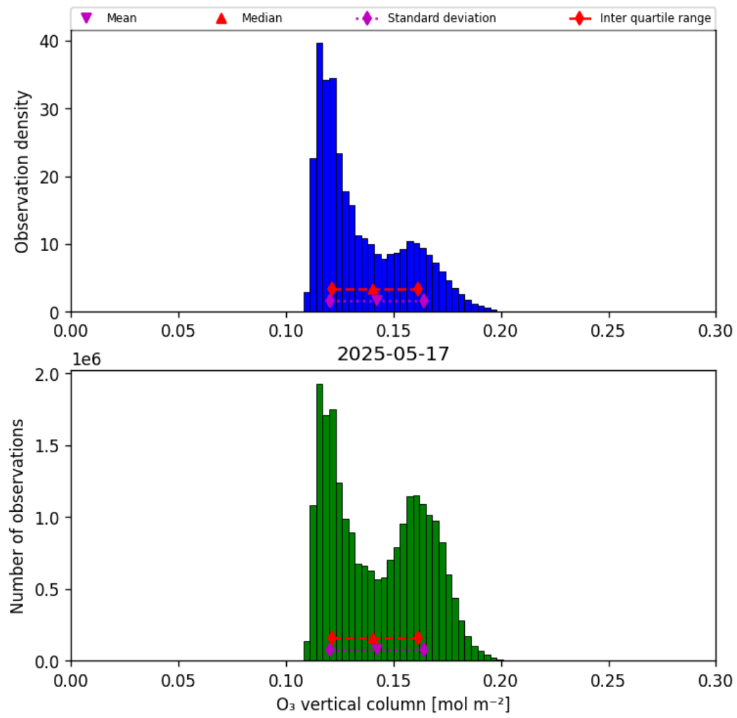
Figure 29: Histogram of “O 3 vertical column” for 2025-05-17 to 2025-05-18
