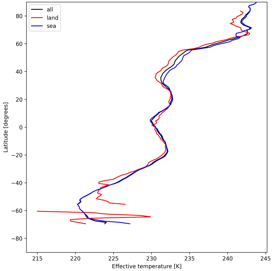
Figure 26: Zonal average of "Effective temperature" for 2025-05-17 to 2025-05-18.
