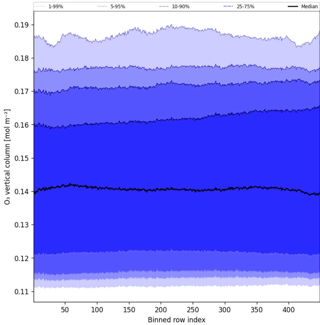
Figure 41: Along track statistics of “ \text{O}_3 vertical column” for 2025-05-17 to 2025-05-18
