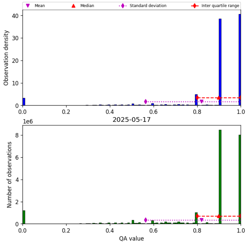
Figure 28: Histogram of “QA value” for 2025-05-17 to 2025-05-18
