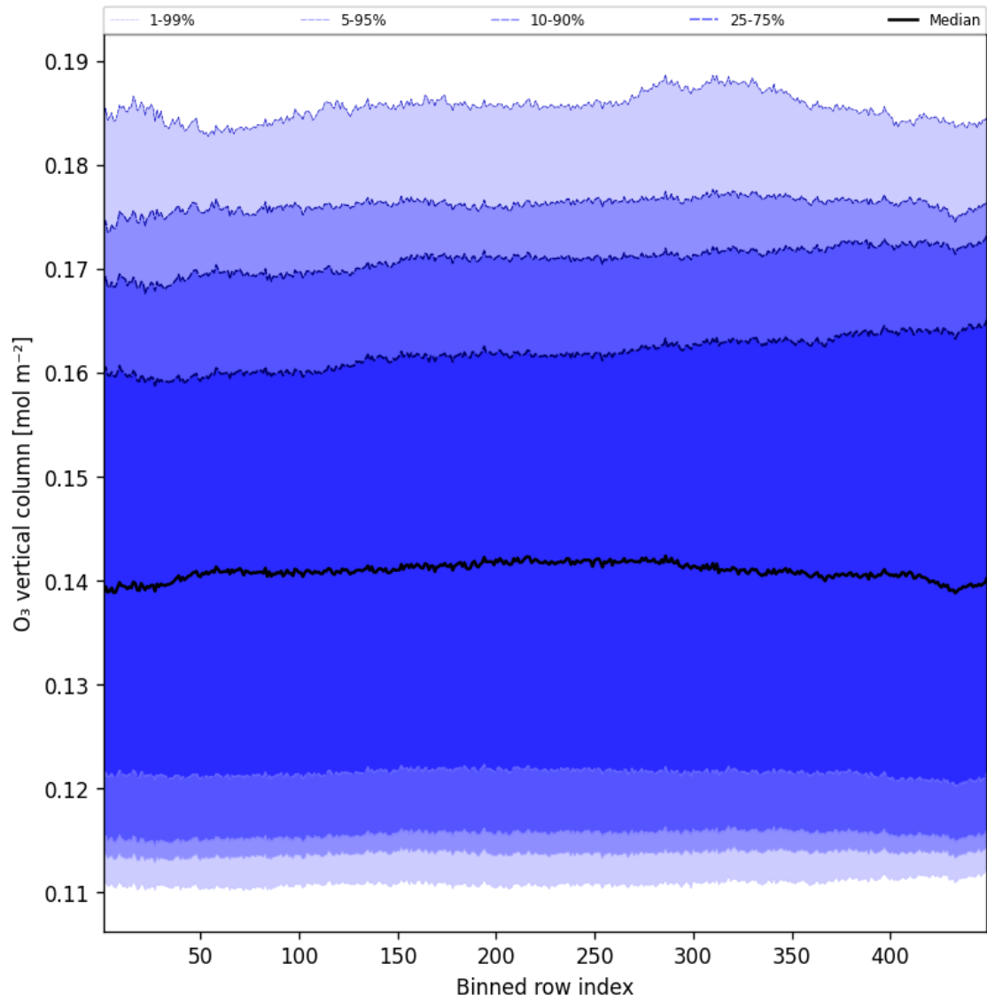
Figure 41: Along track statistics of “O 3 vertical column” for 2025-05-18 to 2025-05-19
