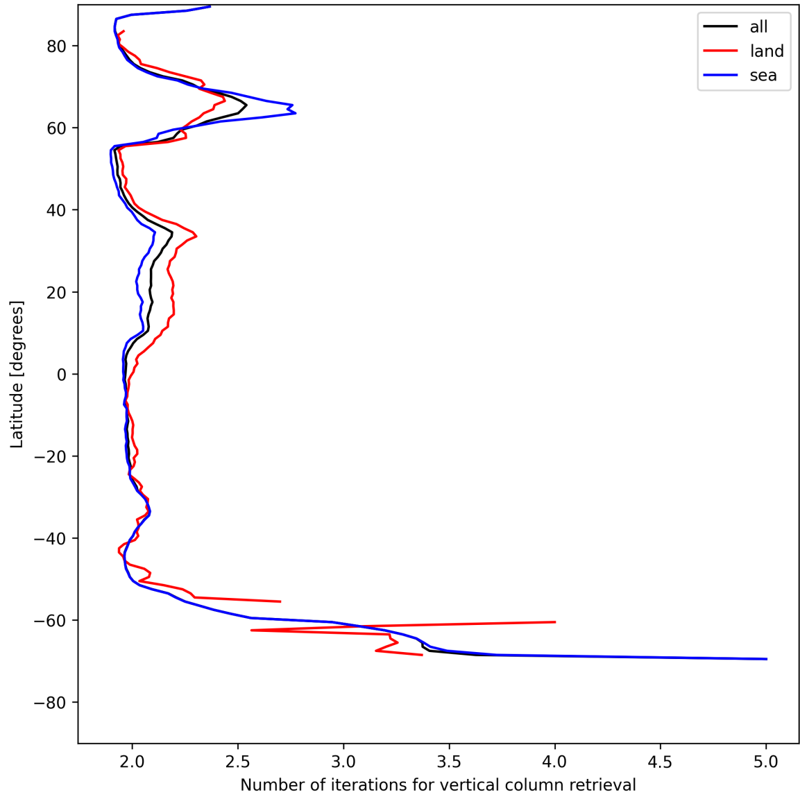
Figure 27: Zonal average of “Number of iterations for vertical column retrieval” for 2025-05-18 to 2025-05-19.
