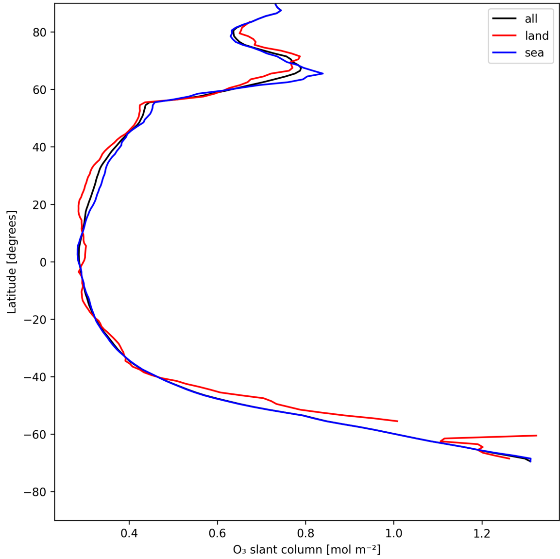
Figure 19: Zonal average of “O 3 slant column” for 2025-05-18 to 2025-05-19.
