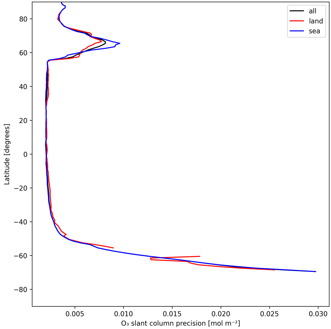
Figure 20: Zonal average of “O 3 slant column precision” for 2025-05-18 to 2025-05-19.
