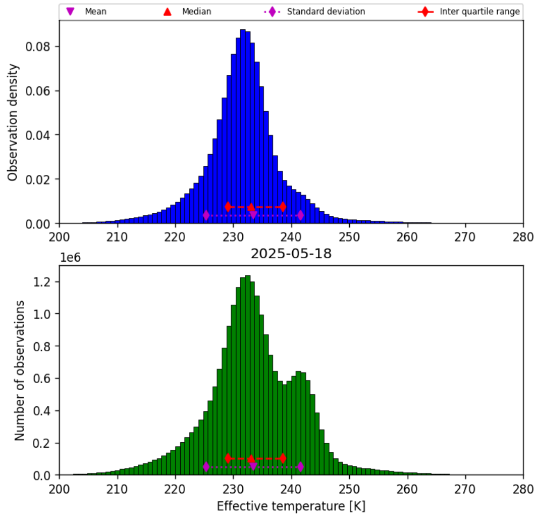
Figure 38: Histogram of “Effective temperature” for 2025-05-18 to 2025-05-19
