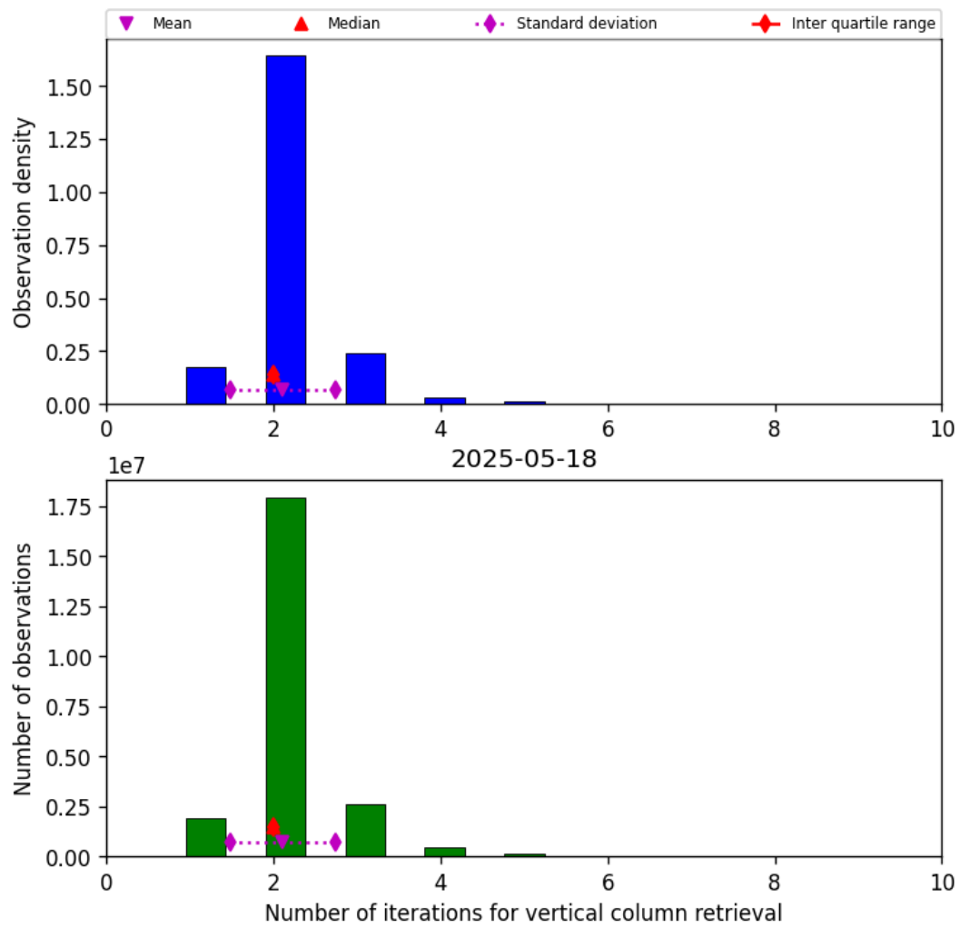
Figure 39: Histogram of “Number of iterations for vertical column retrieval” for 2025-05-18 to 2025-05-19
