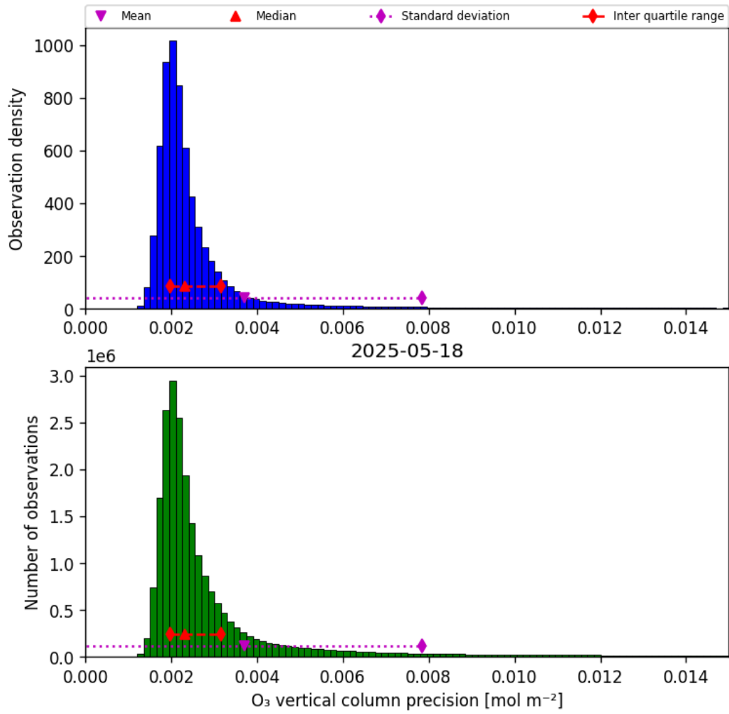
Figure 30: Histogram of “O 3 vertical column precision” for 2025-05-18 to 2025-05-19
