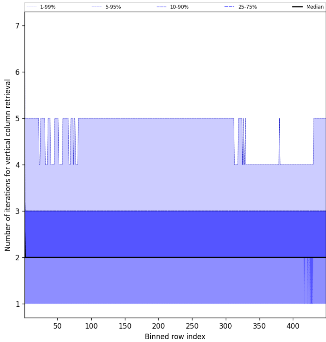
Figure 51: Along track statistics of “Number of iterations for vertical column retrieval” for 2025-05-18 to 2025-05-19
