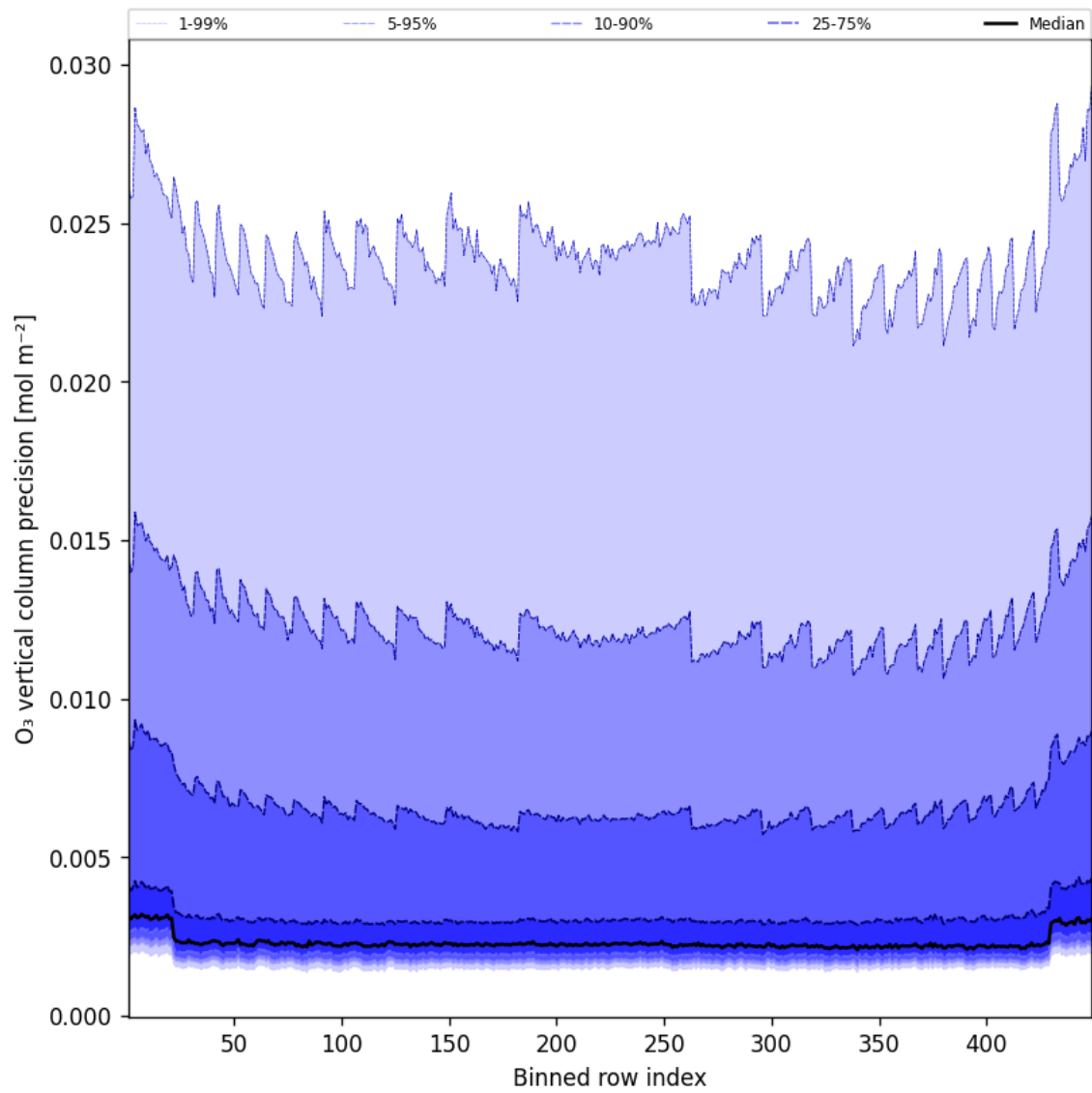
Figure 42: Along track statistics of “O 3 vertical column precision” for 2025-05-18 to 2025-05-19
