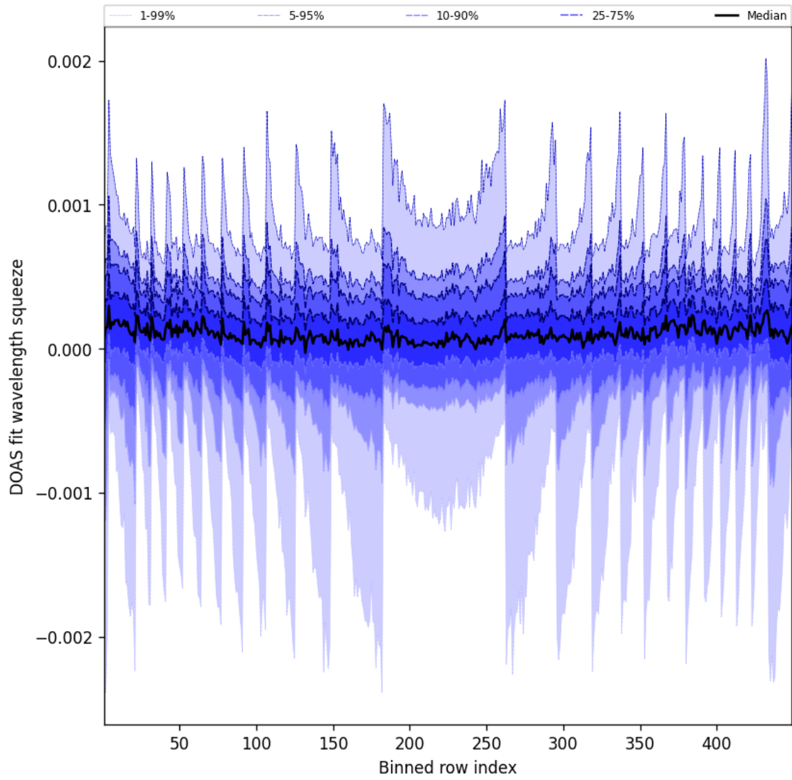
Figure 48: Along track statistics of “DOAS fit wavelength squeeze” for 2025-05-18 to 2025-05-19
