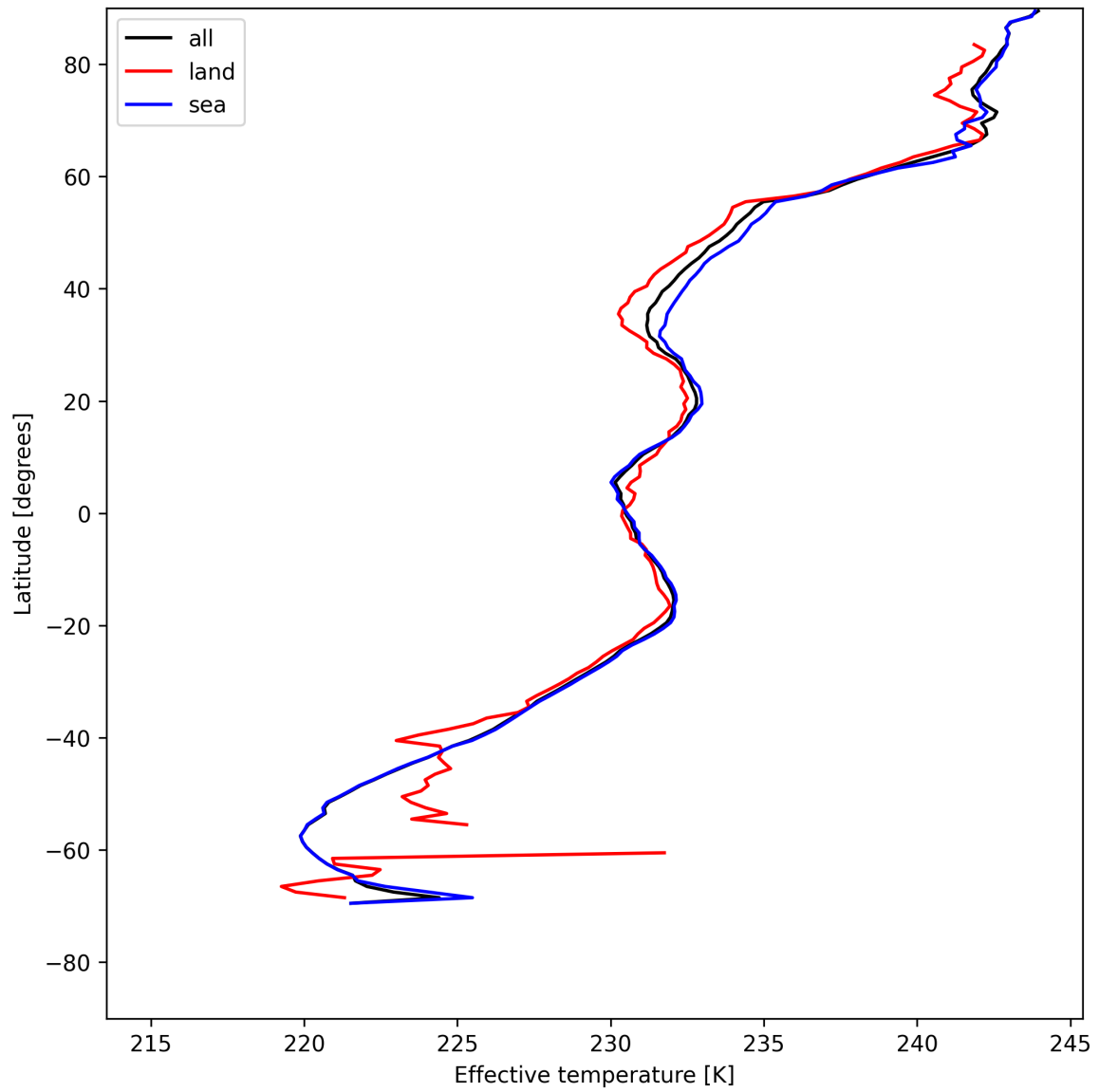
Figure 26: Zonal average of "Effective temperature" for 2025-05-18 to 2025-05-19.
