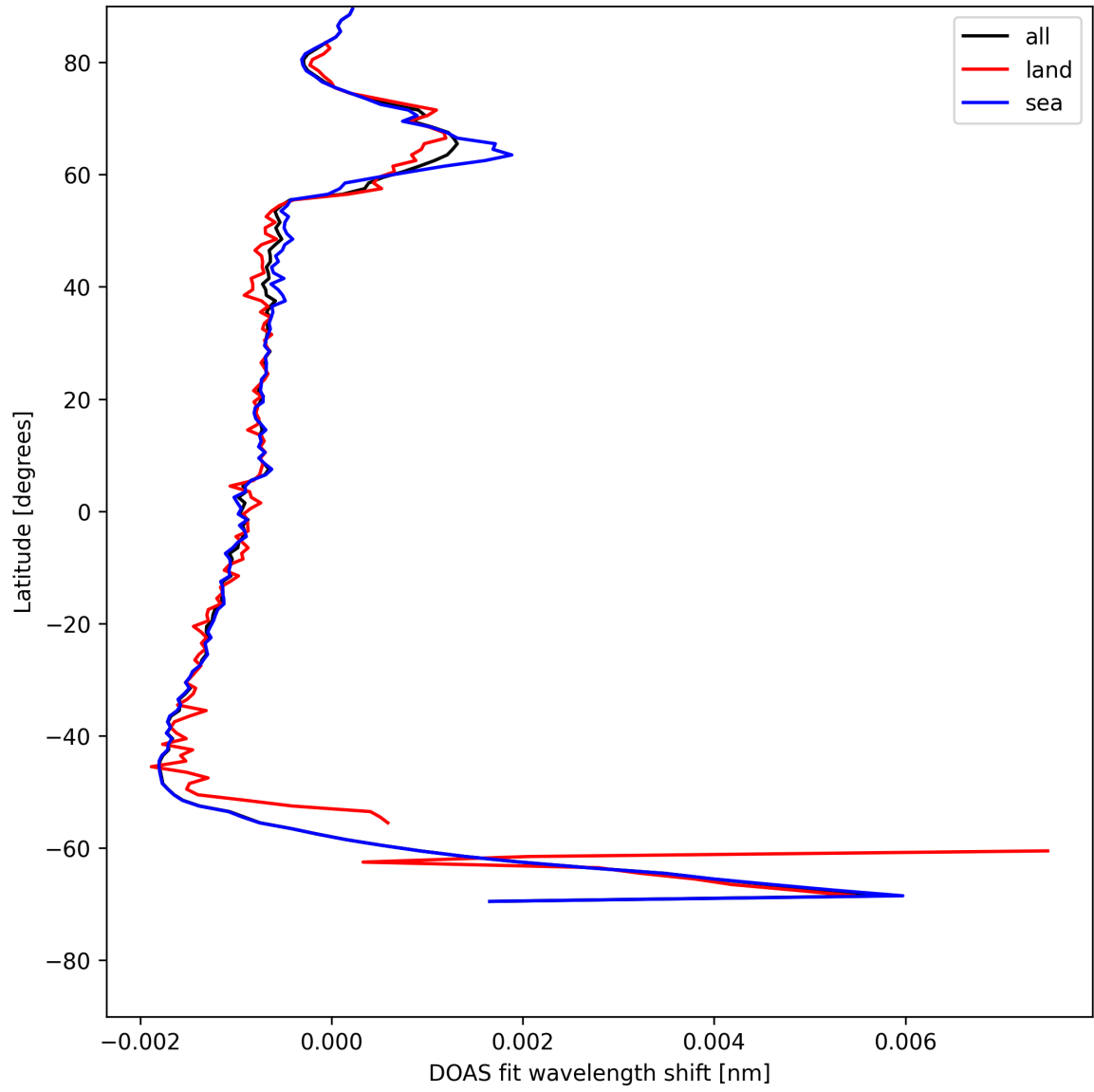
Figure 23: Zonal average of "DOAS fit wavelength shift" for 2025-05-18 to 2025-05-19.
