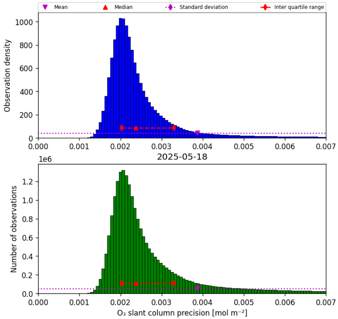
Figure 32: Histogram of “O 3 slant column precision” for 2025-05-18 to 2025-05-19
