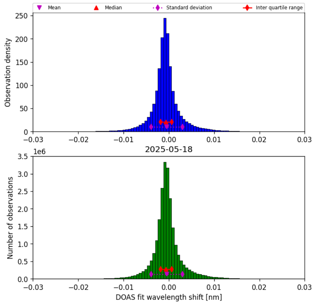
Figure 35: Histogram of “DOAS fit wavelength shift” for 2025-05-18 to 2025-05-19
