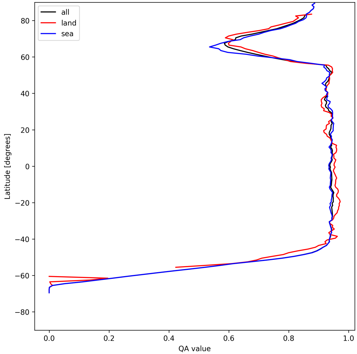
Figure 16: Zonal average of “QA value” for 2025-05-18 to 2025-05-19.
