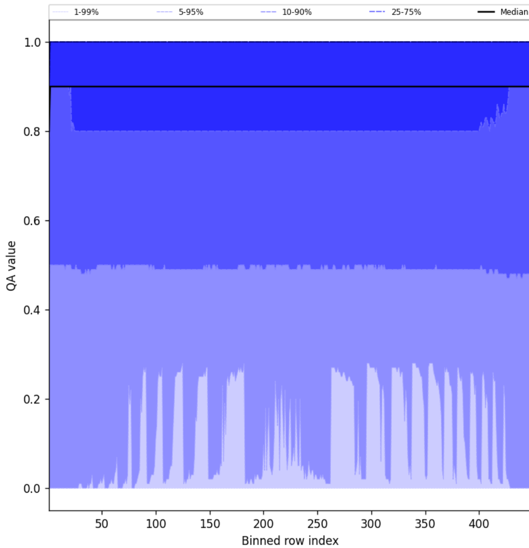
Figure 40: Along track statistics of “QA value” for 2025-05-18 to 2025-05-19
