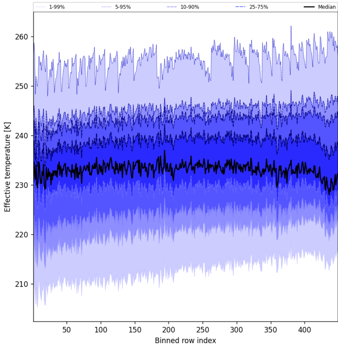
Figure 50: Along track statistics of “Effective temperature” for 2025-05-18 to 2025-05-19
