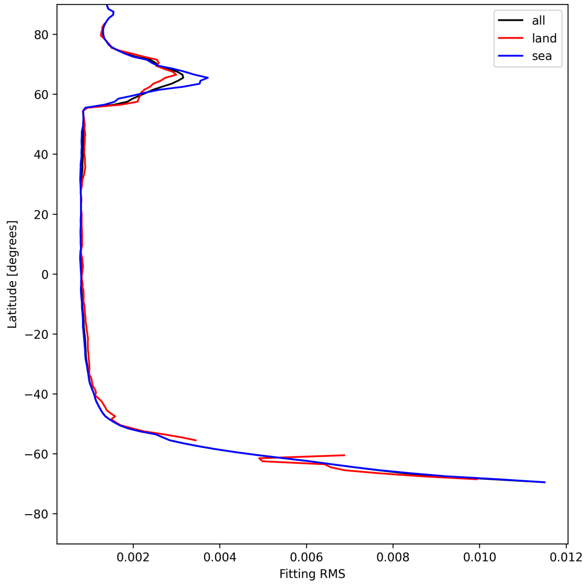
Figure 22: Zonal average of “Fitting RMS” for 2025-05-18 to 2025-05-19.
