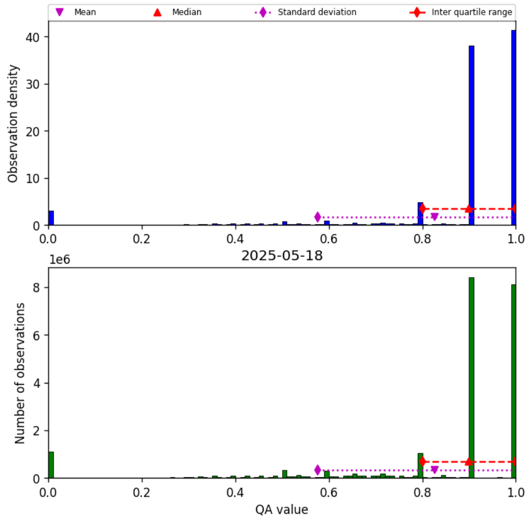
Figure 28: Histogram of “QA value” for 2025-05-18 to 2025-05-19
