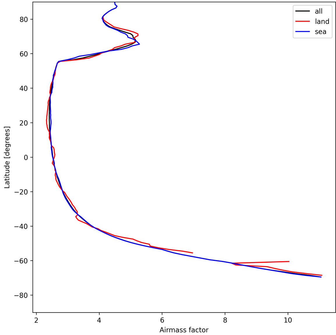
Figure 25: Zonal average of “Airmass factor” for 2025-05-18 to 2025-05-19.
