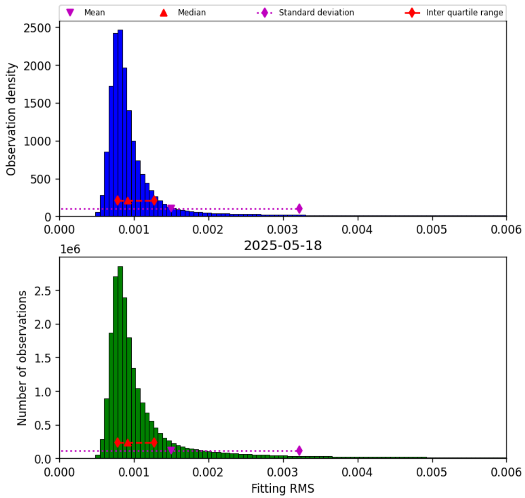
Figure 34: Histogram of “Fitting RMS” for 2025-05-18 to 2025-05-19
