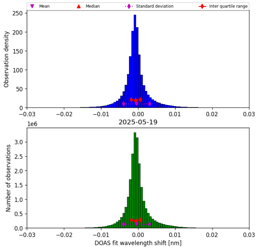
Figure 35: Histogram of “DOAS fit wavelength shift” for 2025-05-19 to 2025-05-19
