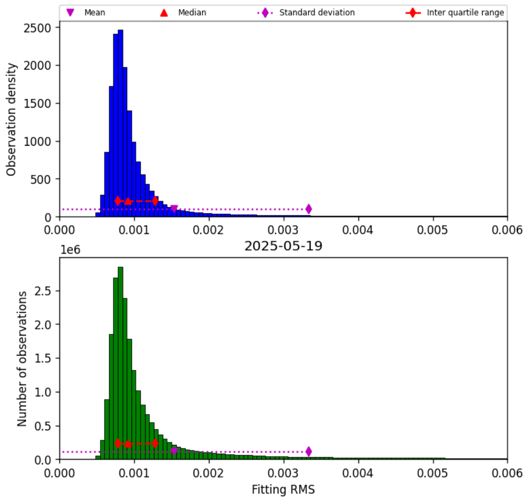
Figure 34: Histogram of “Fitting RMS” for 2025-05-19 to 2025-05-19
