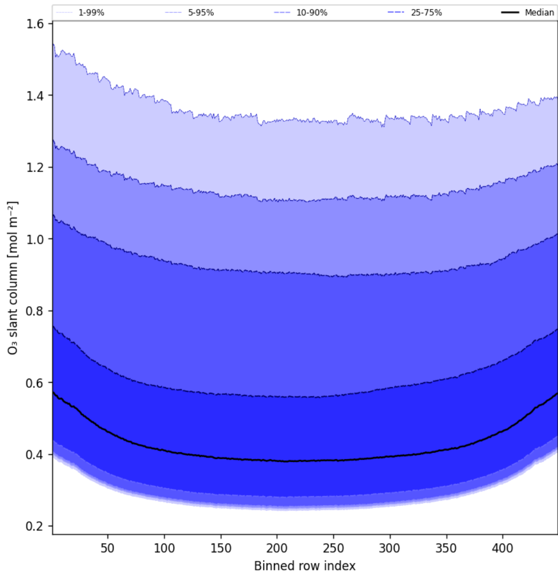
Figure 43: Along track statistics of “O 3 slant column” for 2025-05-19 to 2025-05-19
