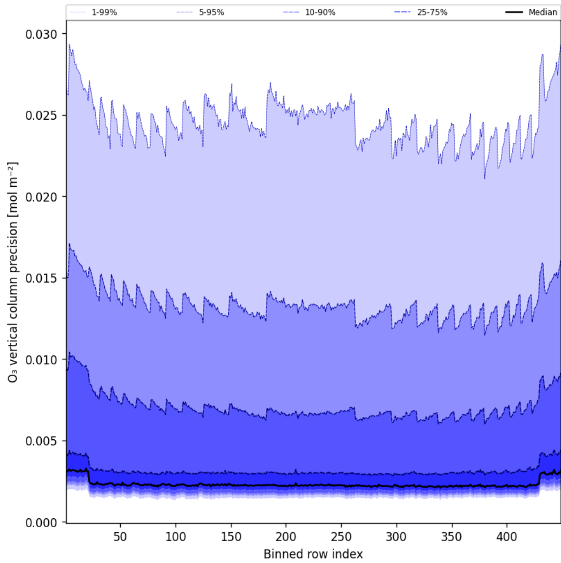
Figure 42: Along track statistics of “O 3 vertical column precision” for 2025-05-19 to 2025-05-19
