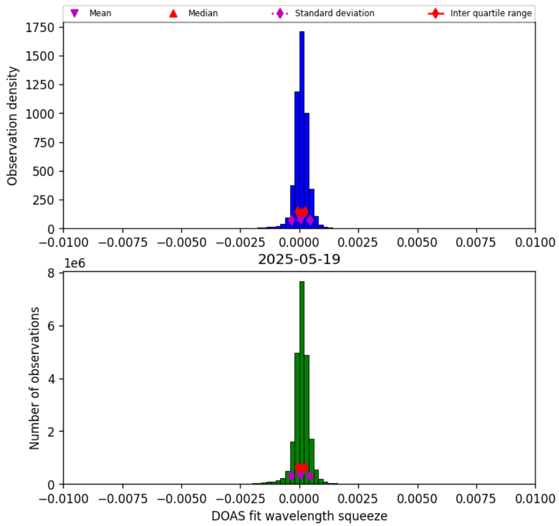
Figure 36: Histogram of “DOAS fit wavelength squeeze” for 2025-05-19 to 2025-05-19
