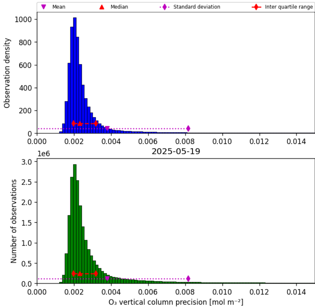
Figure 30: Histogram of “O 3 vertical column precision” for 2025-05-19 to 2025-05-19
