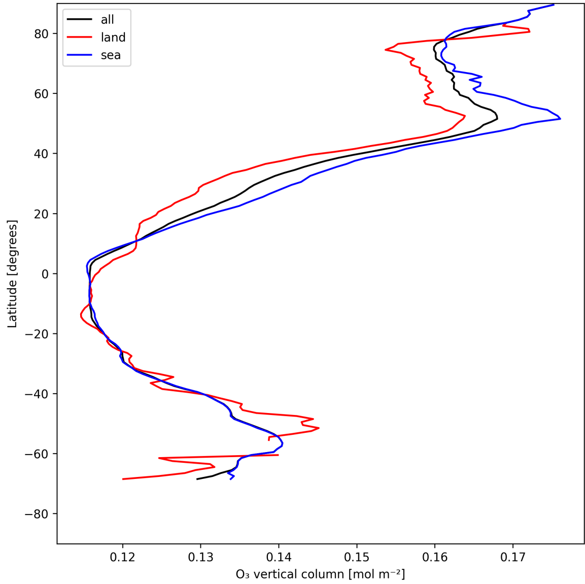
Figure 17: Zonal average of “O 3 vertical column” for 2025-05-19 to 2025-05-19.
