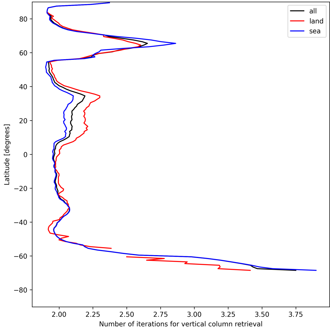
Figure 27: Zonal average of “Number of iterations for vertical column retrieval” for 2025-05-19 to 2025-05-19.
