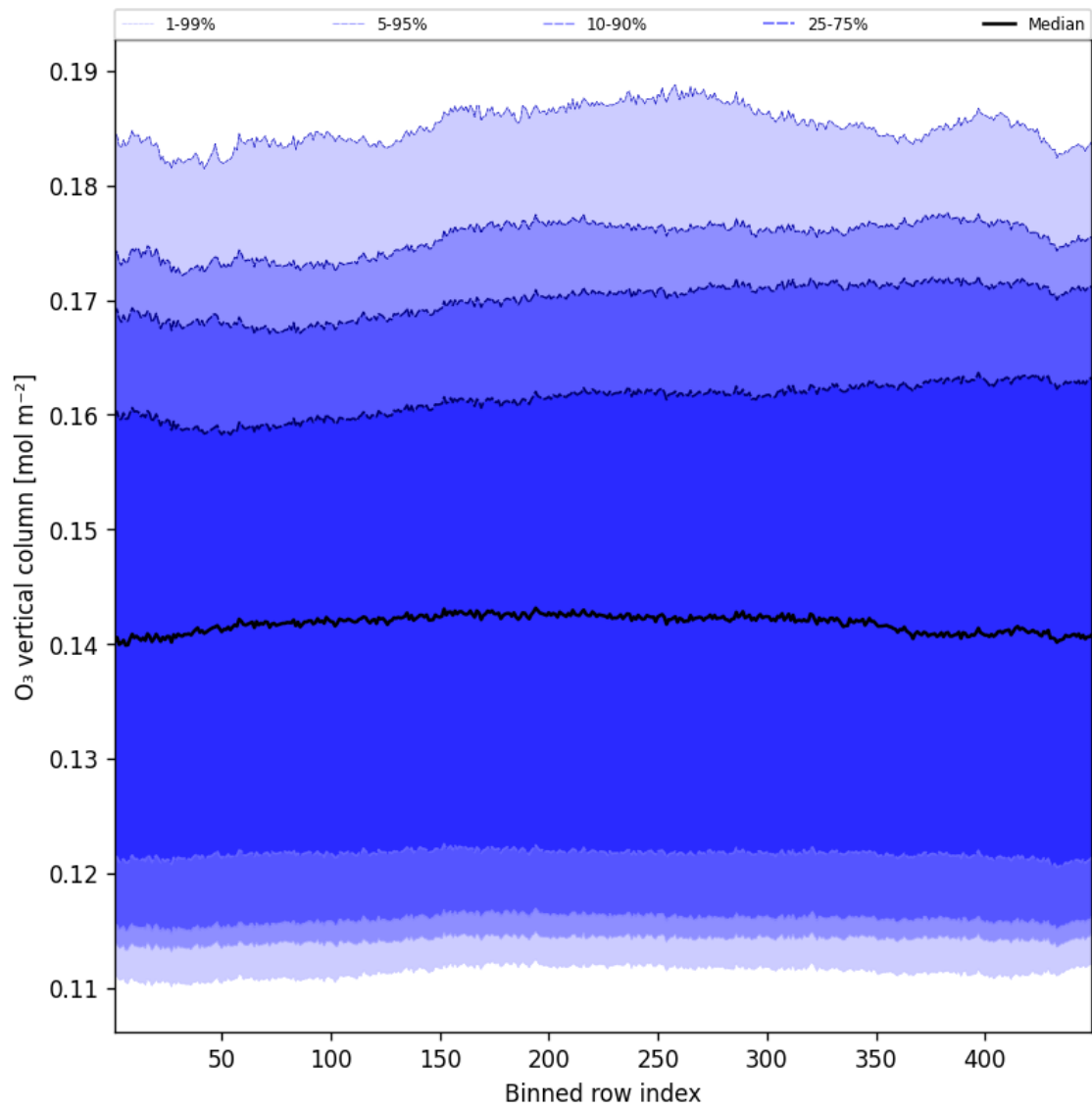
Figure 41: Along track statistics of “O 3 vertical column” for 2025-05-19 to 2025-05-19
