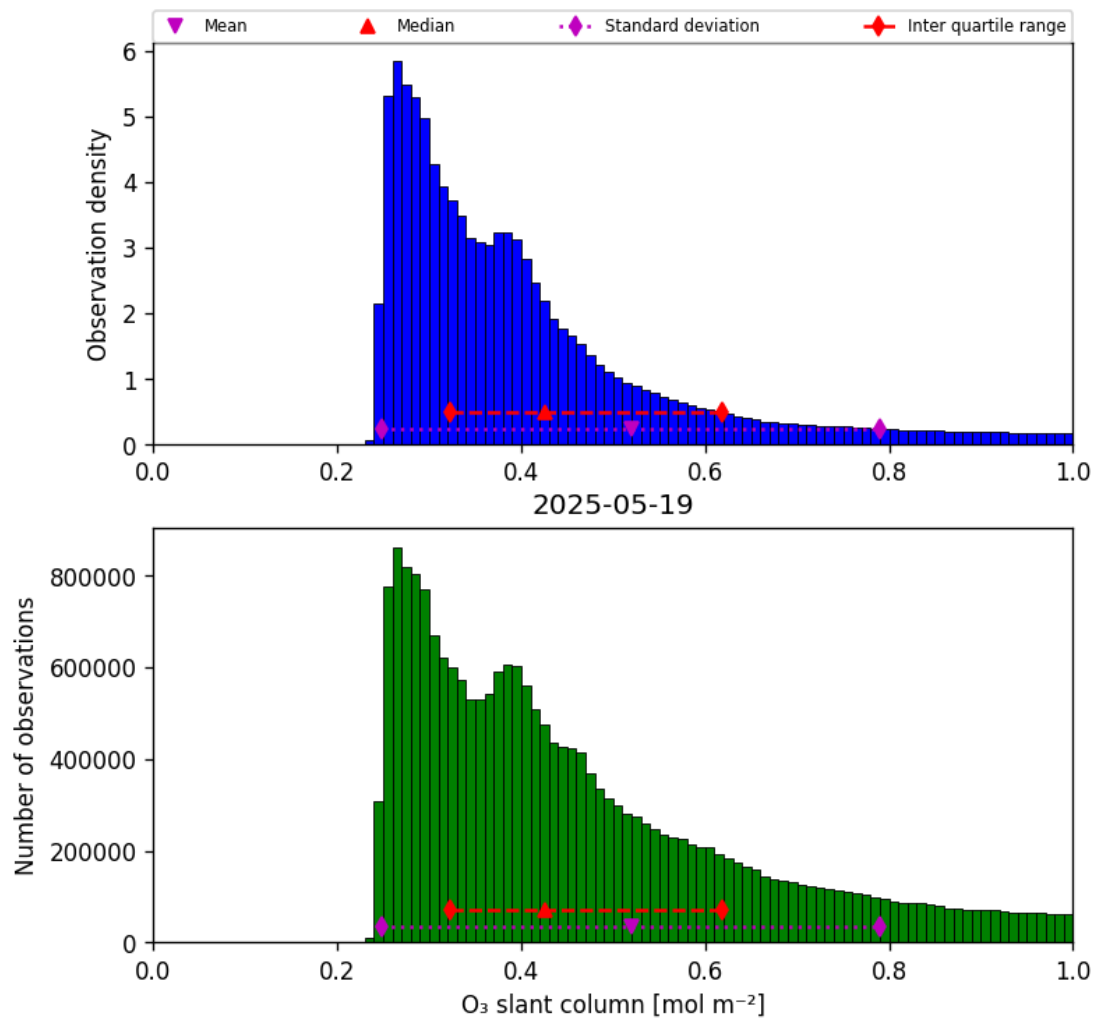
Figure 31: Histogram of “O 3 slant column” for 2025-05-19 to 2025-05-19
