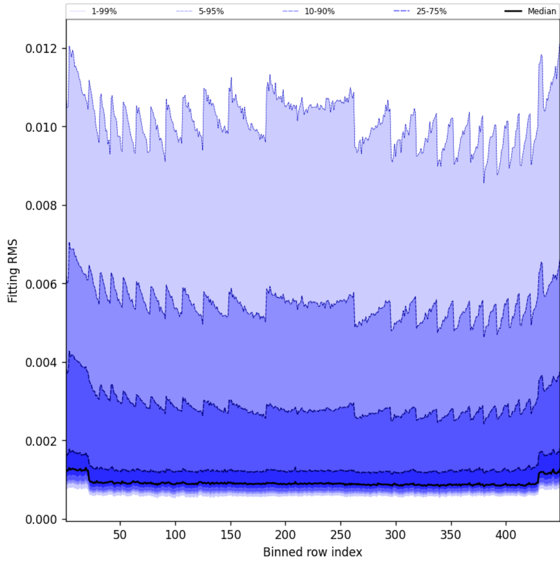
Figure 46: Along track statistics of “Fitting RMS” for 2025-05-19 to 2025-05-19
