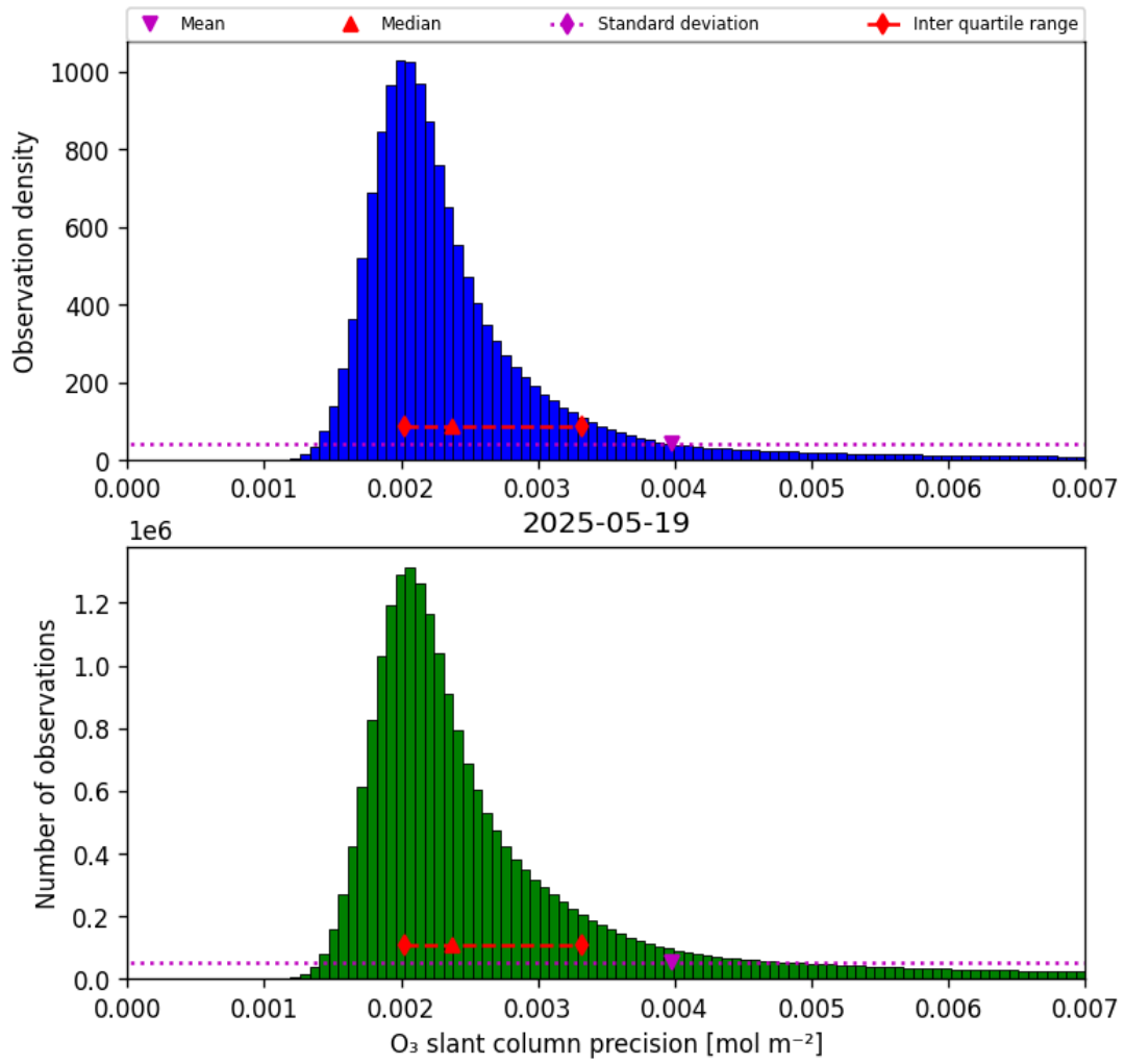
Figure 32: Histogram of “O 3 slant column precision” for 2025-05-19 to 2025-05-19
