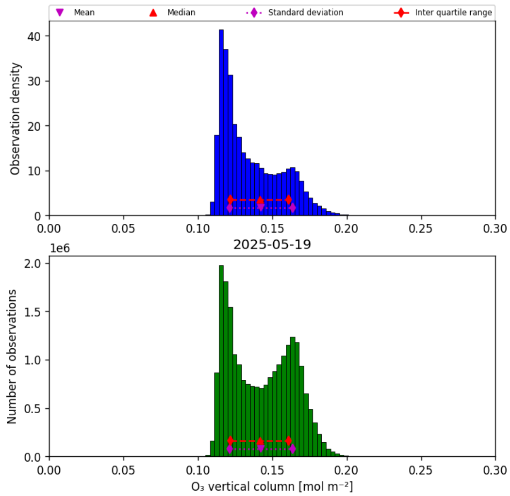
Figure 29: Histogram of “O 3 vertical column” for 2025-05-19 to 2025-05-19
