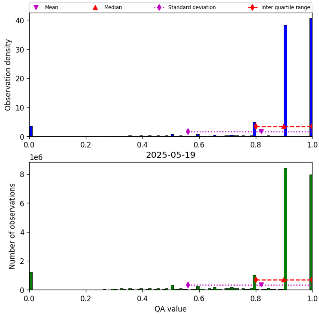
Figure 28: Histogram of “QA value” for 2025-05-19 to 2025-05-19
