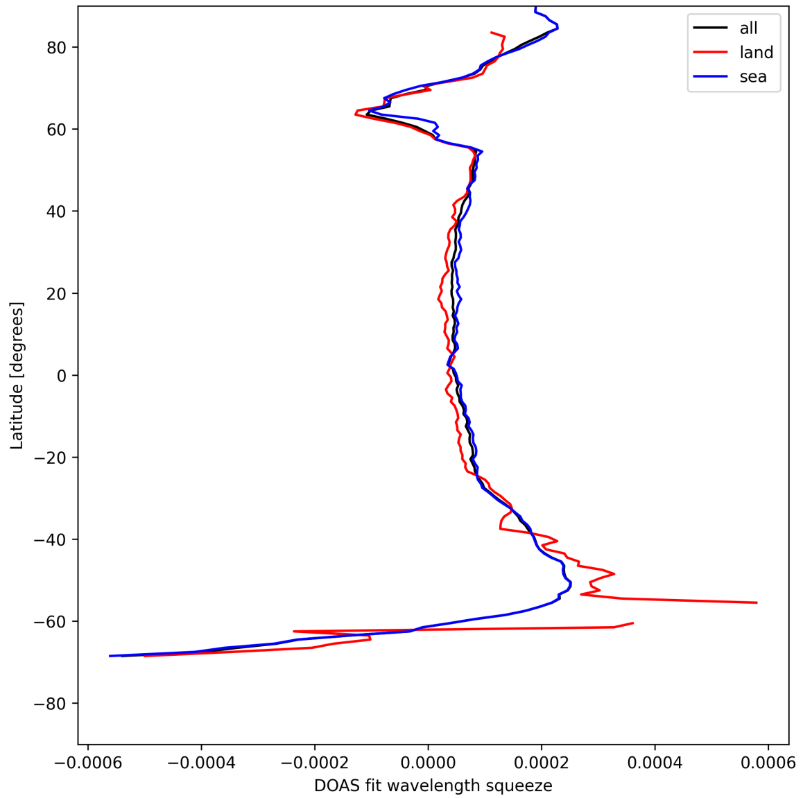
Figure 24: Zonal average of “DOAS fit wavelength squeeze” for 2025-05-19 to 2025-05-19.
