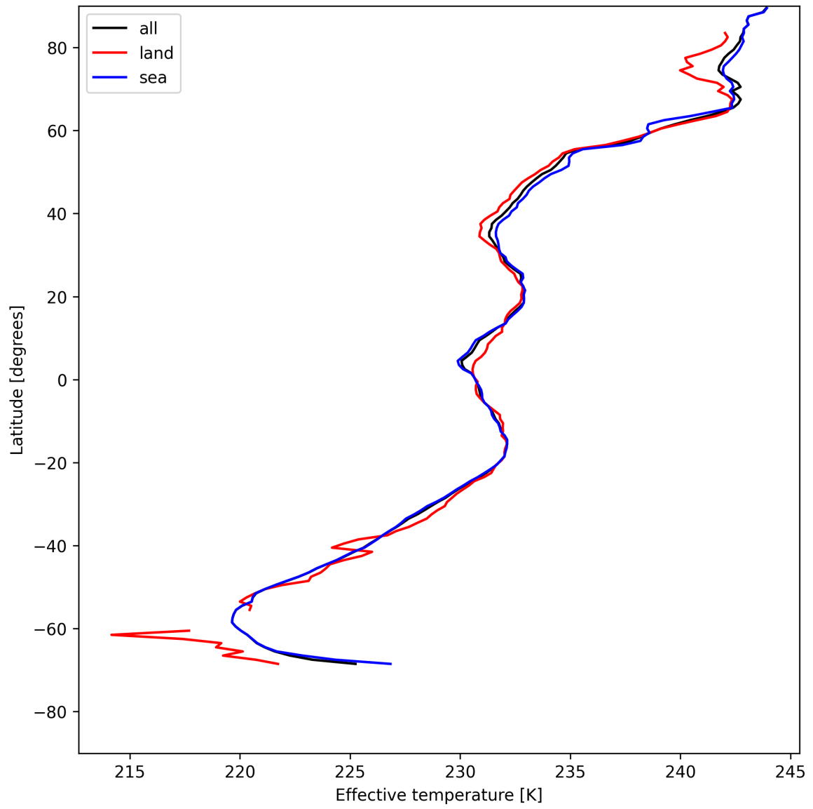
Figure 26: Zonal average of “Effective temperature” for 2025-05-19 to 2025-05-19.
