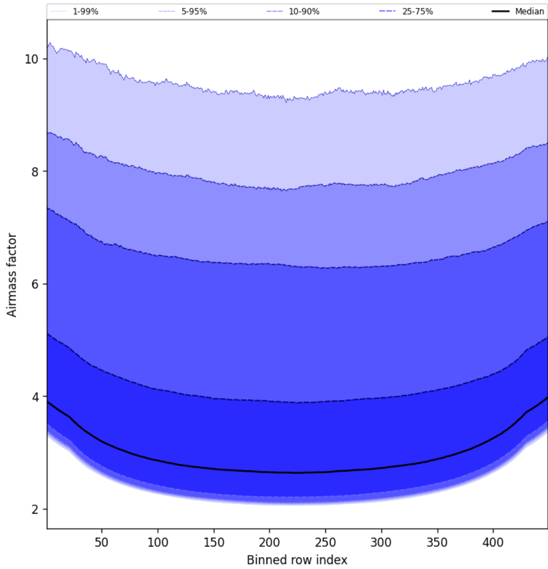
Figure 49: Along track statistics of “Airmass factor” for 2025-05-19 to 2025-05-19
