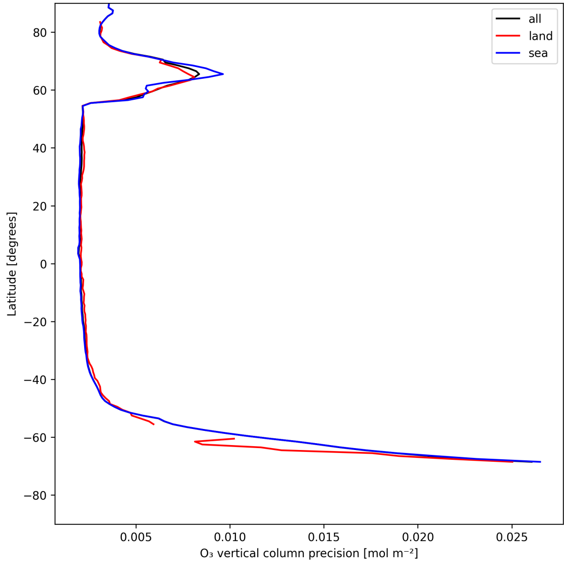
Figure 18: Zonal average of “O 3 vertical column precision” for 2025-05-19 to 2025-05-19.
