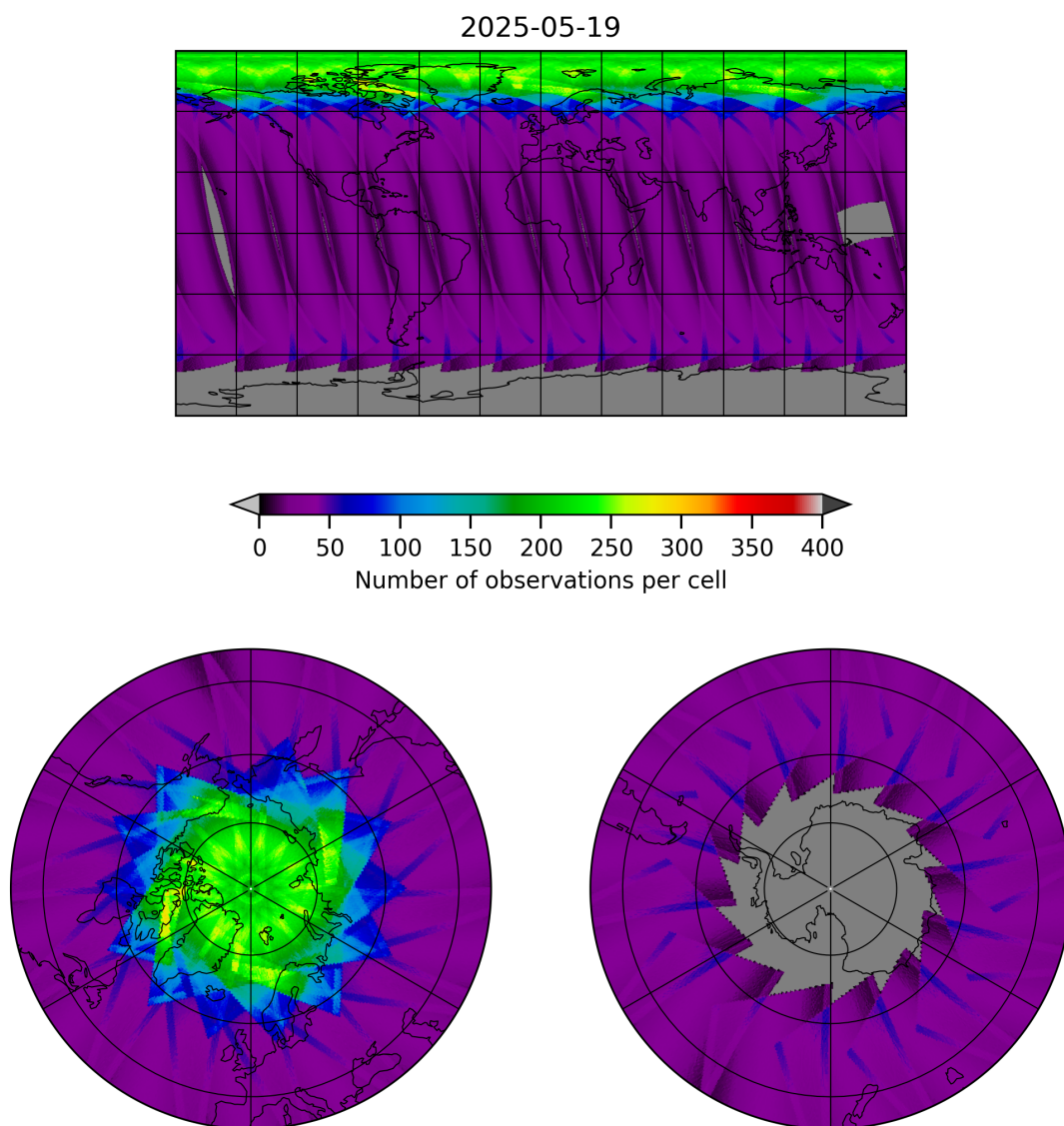
Figure 15: Map of the number of observations for 2025-05-19 to 2025-05-19
