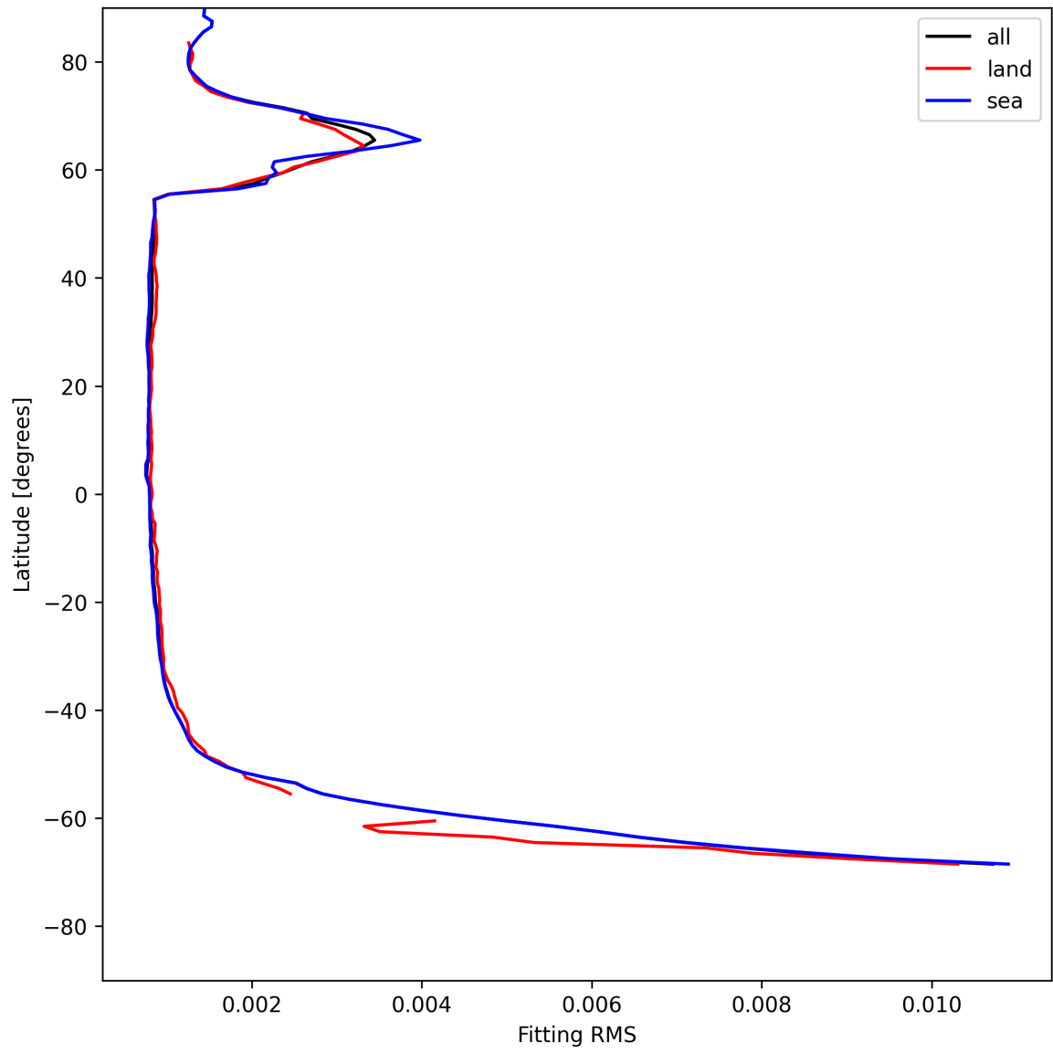
Figure 22: Zonal average of “Fitting RMS” for 2025-05-19 to 2025-05-19.
