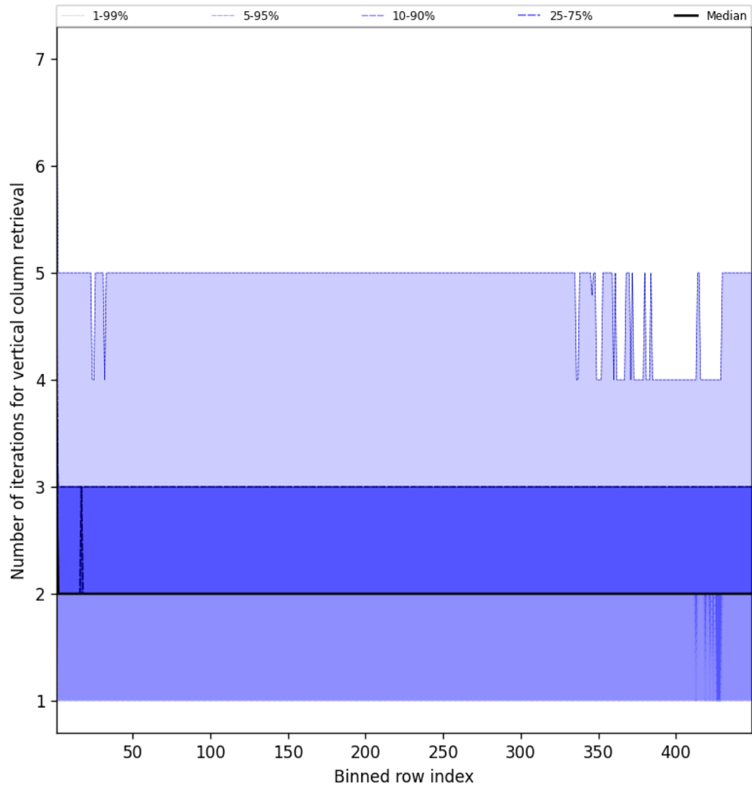
Figure 51: Along track statistics of “Number of iterations for vertical column retrieval” for 2025-05-19 to 2025-05-19
