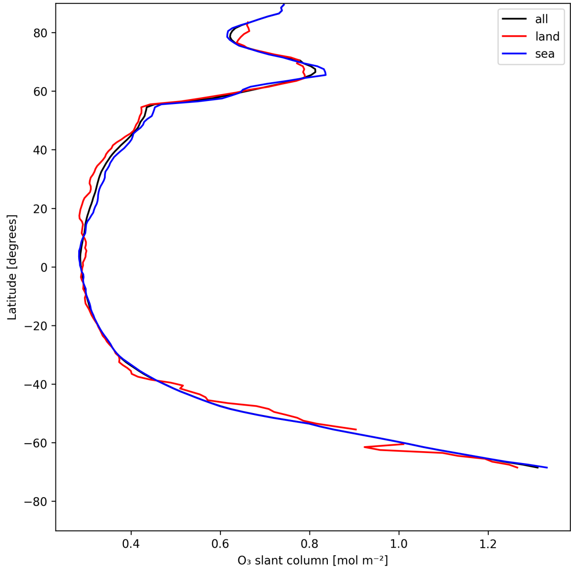
Figure 19: Zonal average of “O 3 slant column” for 2025-05-19 to 2025-05-19.
