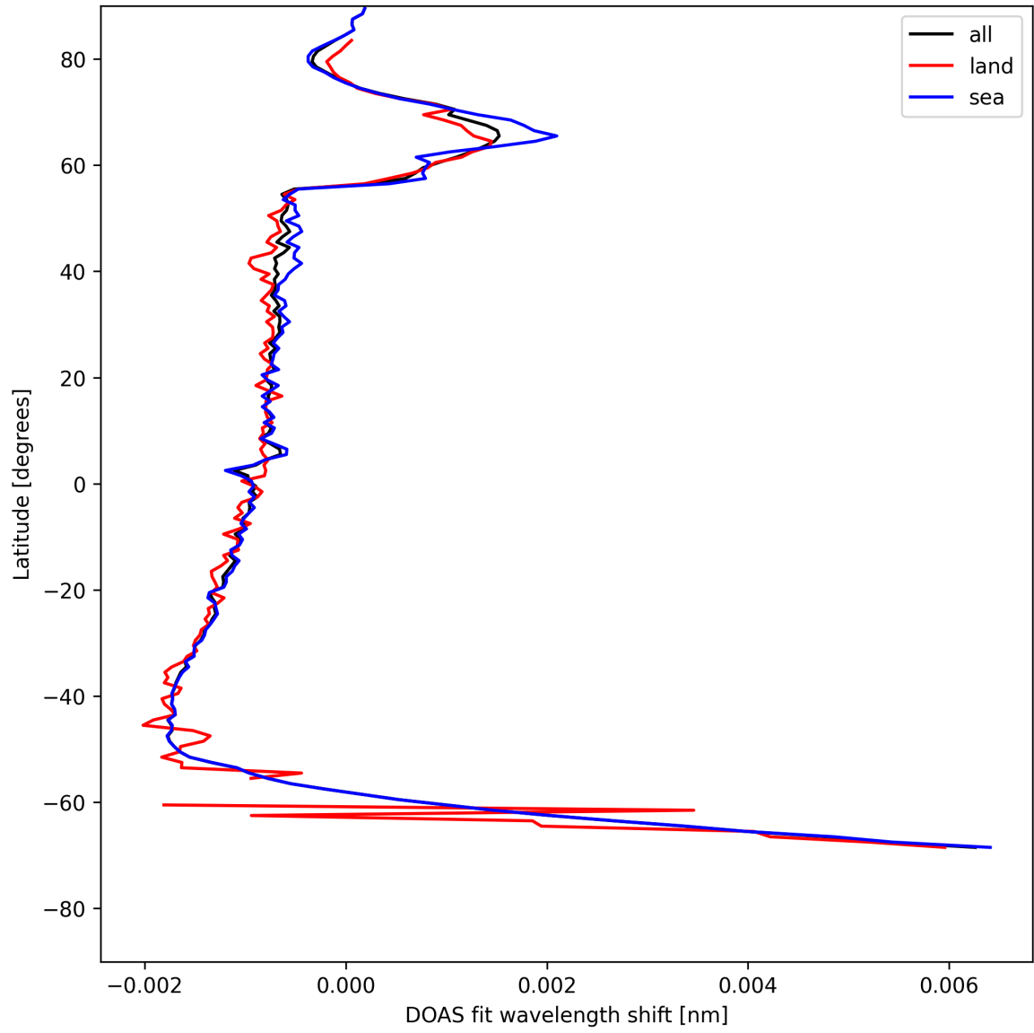
Figure 23: Zonal average of “DOAS fit wavelength shift” for 2025-05-19 to 2025-05-19.
