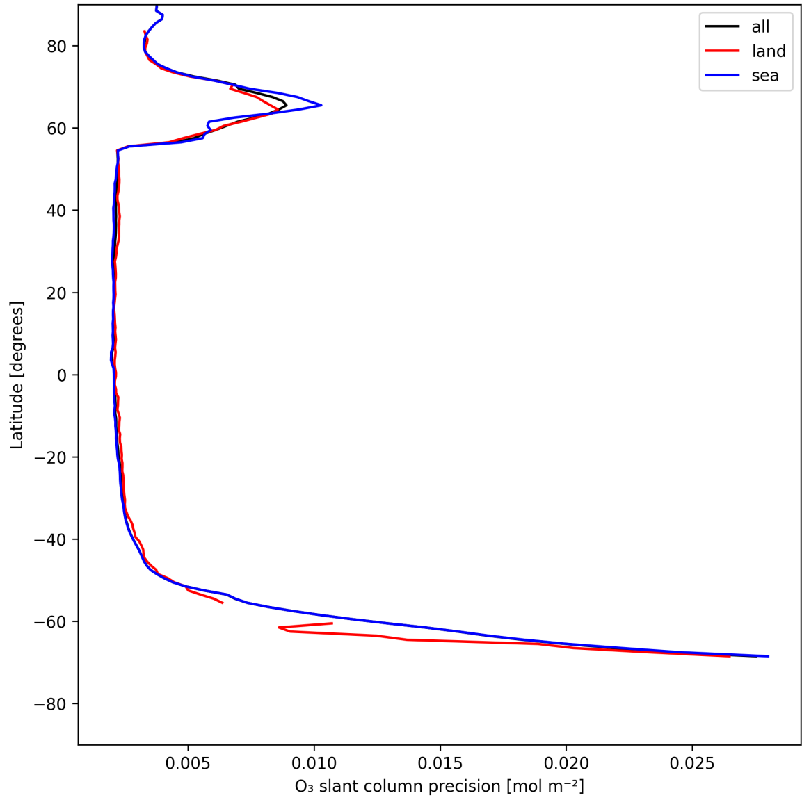
Figure 20: Zonal average of “O 3 slant column precision” for 2025-05-19 to 2025-05-19.
