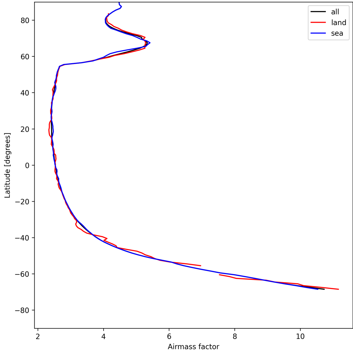
Figure 25: Zonal average of “Airmass factor” for 2025-05-19 to 2025-05-19.
