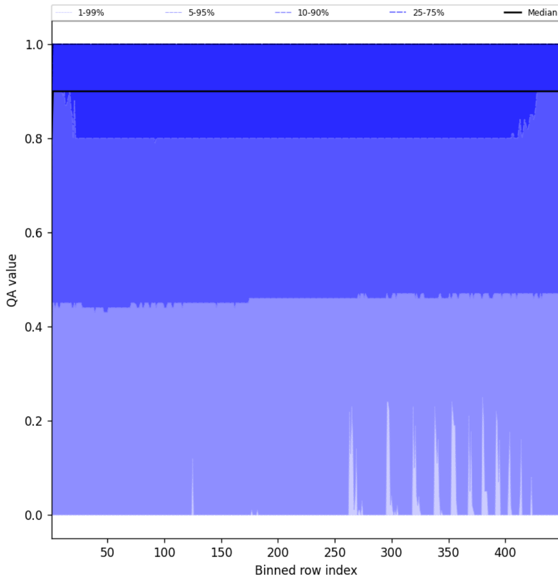
Figure 40: Along track statistics of “QA value” for 2025-05-19 to 2025-05-19
