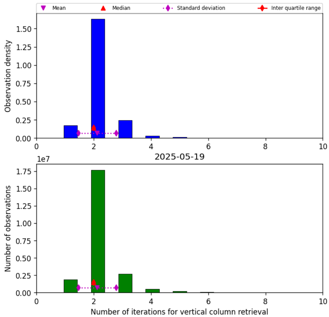
Figure 39: Histogram of “Number of iterations for vertical column retrieval” for 2025-05-19 to 2025-05-19
