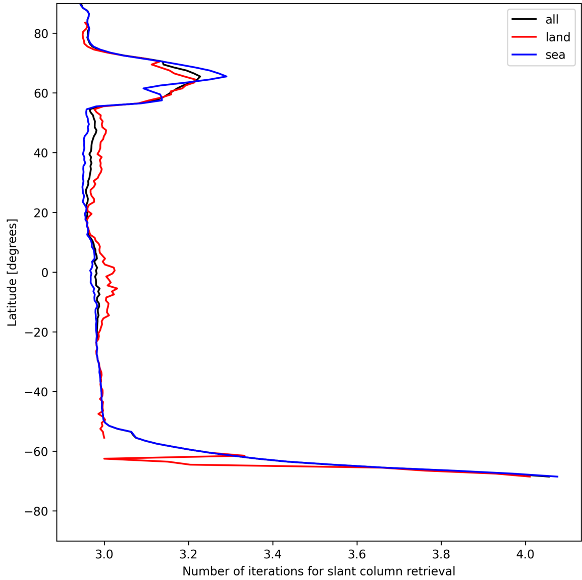
Figure 21: Zonal average of “Number of iterations for slant column retrieval” for 2025-05-19 to 2025-05-19.
