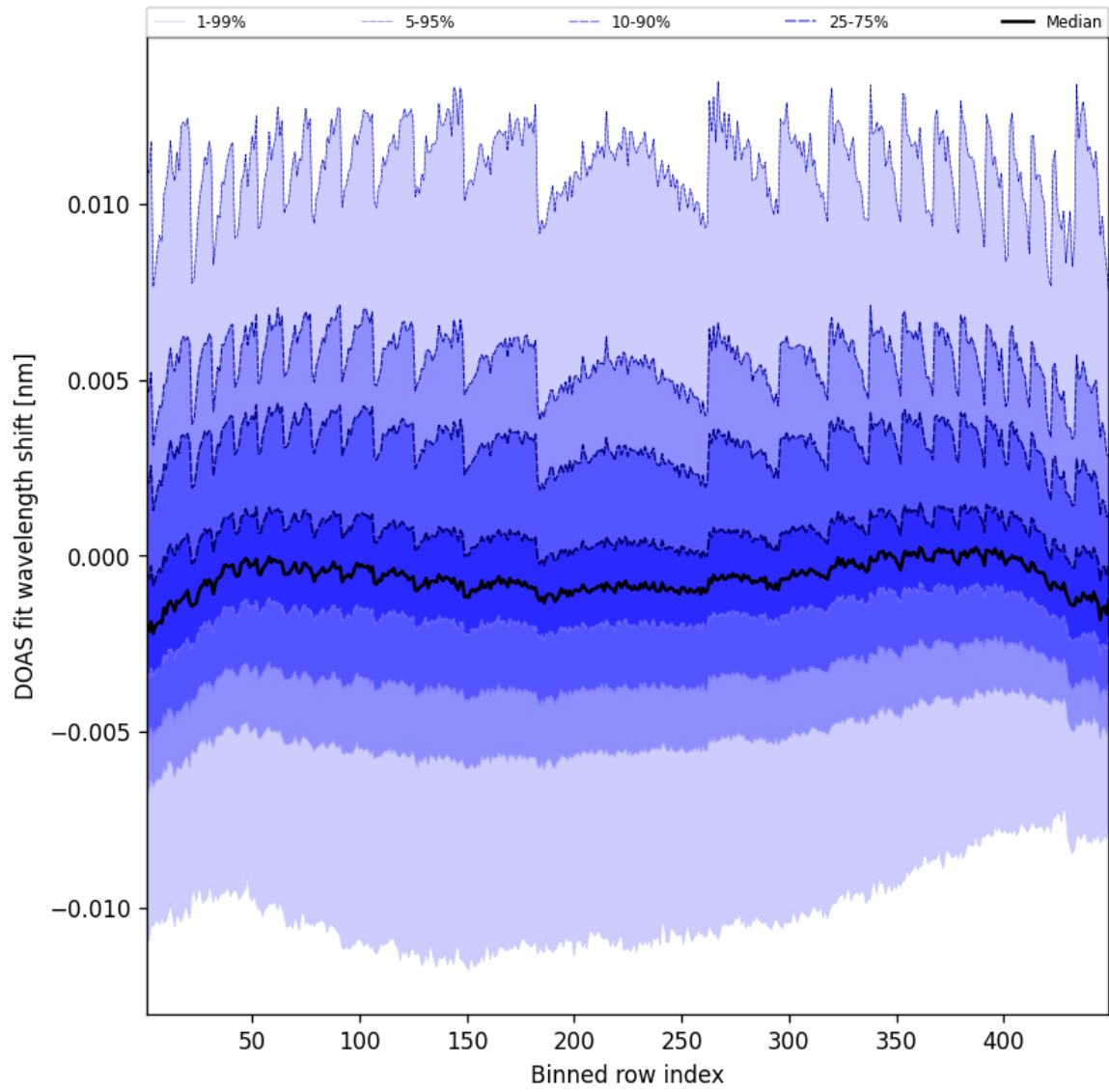
Figure 47: Along track statistics of “DOAS fit wavelength shift” for 2025-05-19 to 2025-05-19
