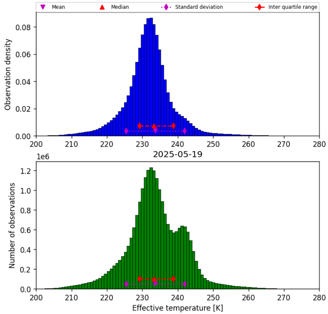
Figure 38: Histogram of “Effective temperature” for 2025-05-19 to 2025-05-19
