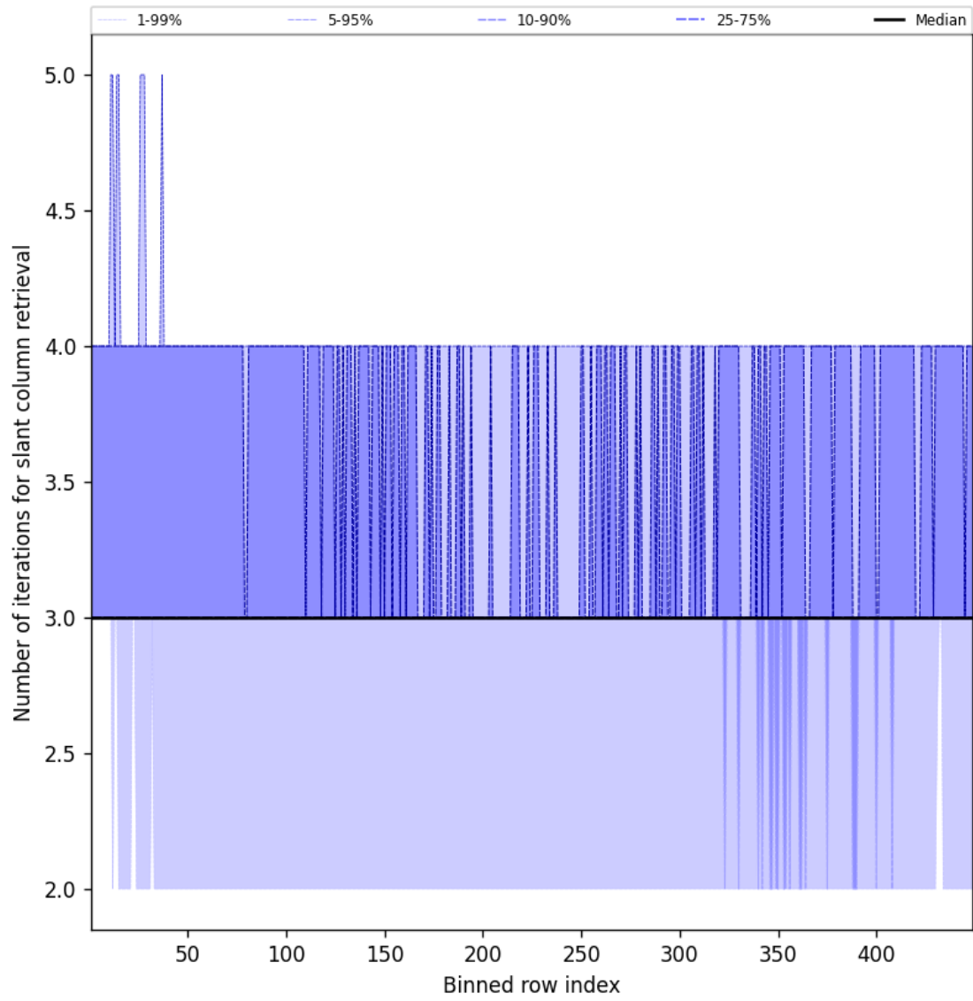
Figure 45: Along track statistics of “Number of iterations for slant column retrieval” for 2025-05-19 to 2025-05-19
