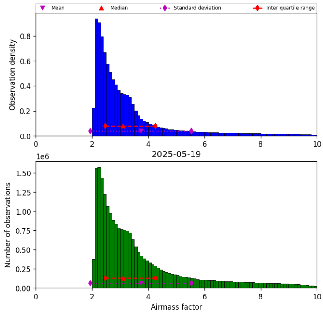
Figure 37: Histogram of “Airmass factor” for 2025-05-19 to 2025-05-19
