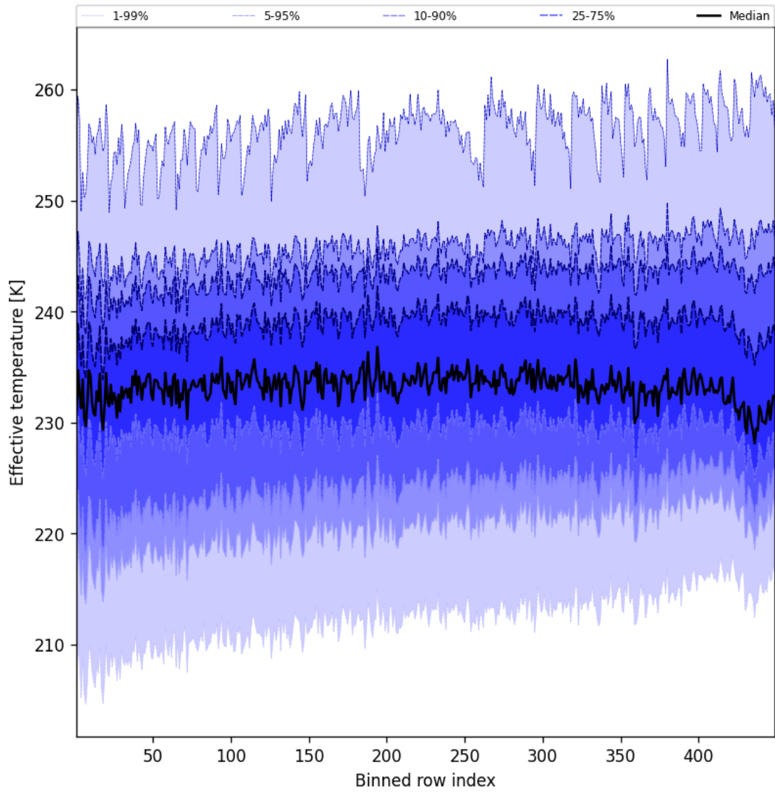
Figure 50: Along track statistics of “Effective temperature” for 2025-05-19 to 2025-05-19
