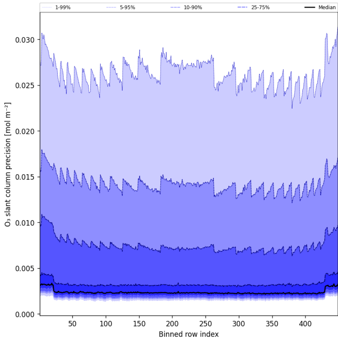
Figure 44: Along track statistics of “O 3 slant column precision” for 2025-05-19 to 2025-05-19
