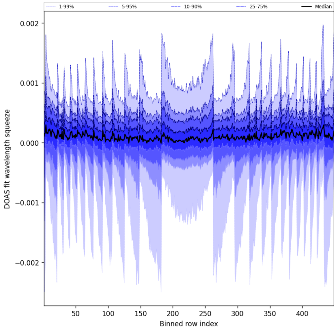
Figure 48: Along track statistics of “DOAS fit wavelength squeeze” for 2025-05-19 to 2025-05-19
