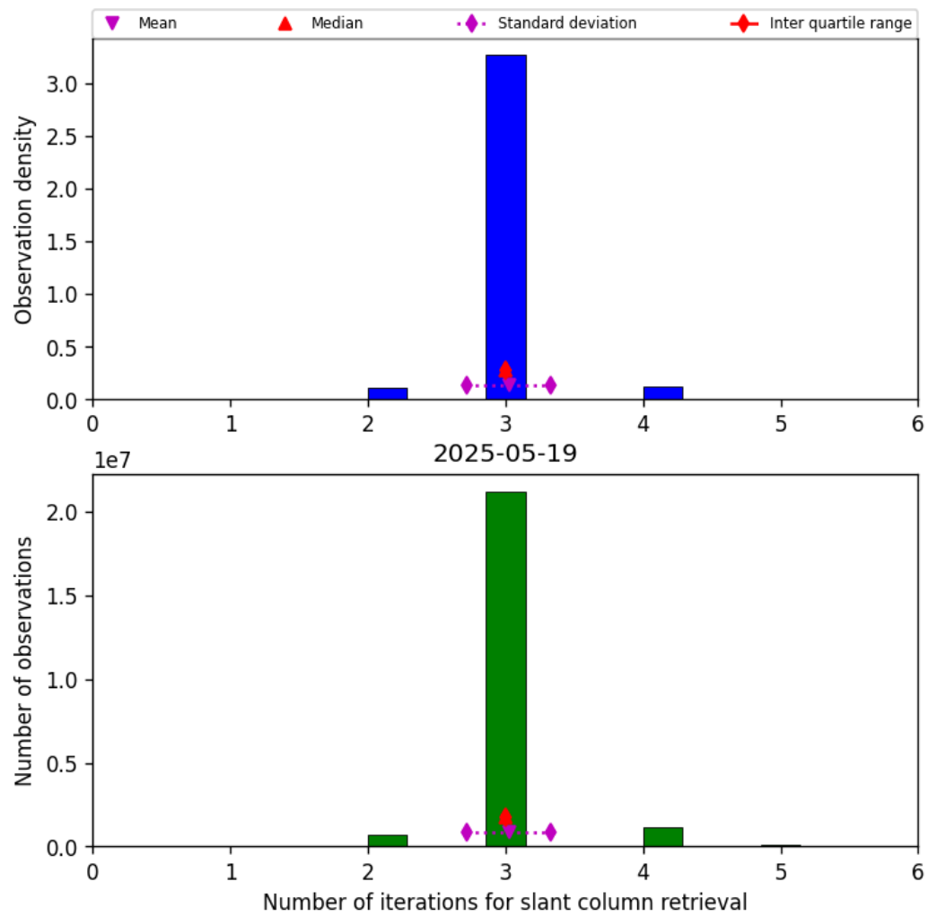
Figure 33: Histogram of “Number of iterations for slant column retrieval” for 2025-05-19 to 2025-05-19
