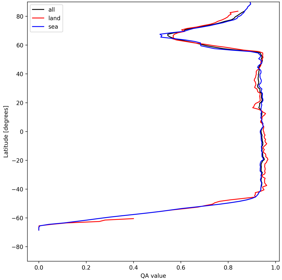
Figure 16: Zonal average of “QA value” for 2025-05-19 to 2025-05-19.
