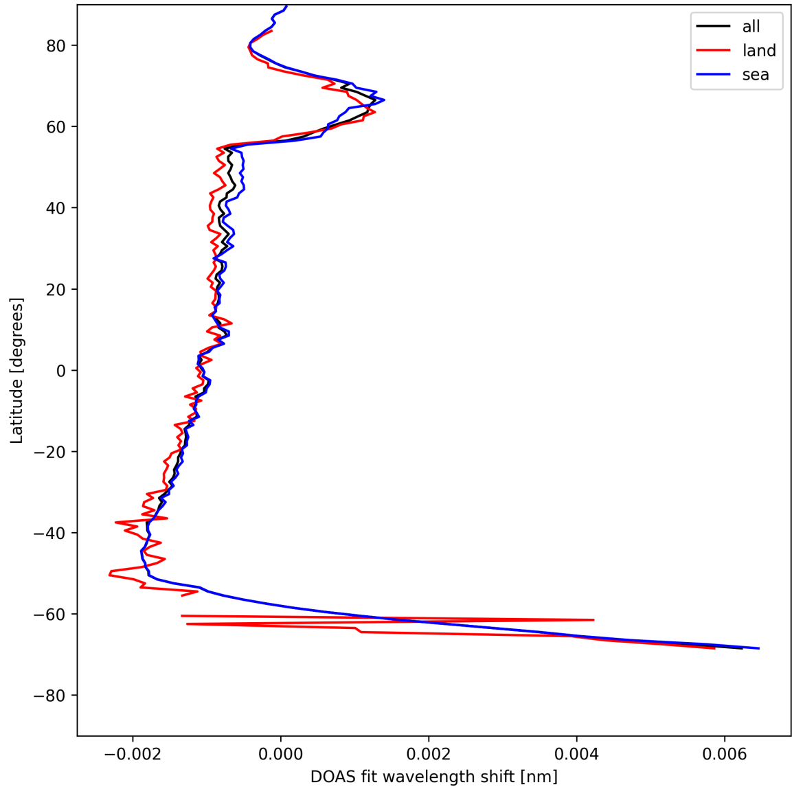
Figure 23: Zonal average of “DOAS fit wavelength shift” for 2025-05-20 to 2025-05-21.
