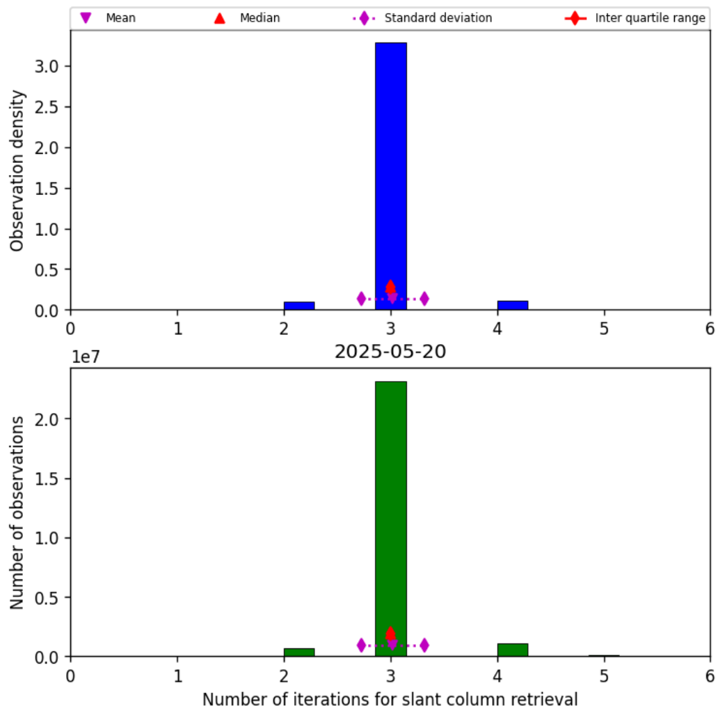
Figure 33: Histogram of “Number of iterations for slant column retrieval” for 2025-05-20 to 2025-05-21
