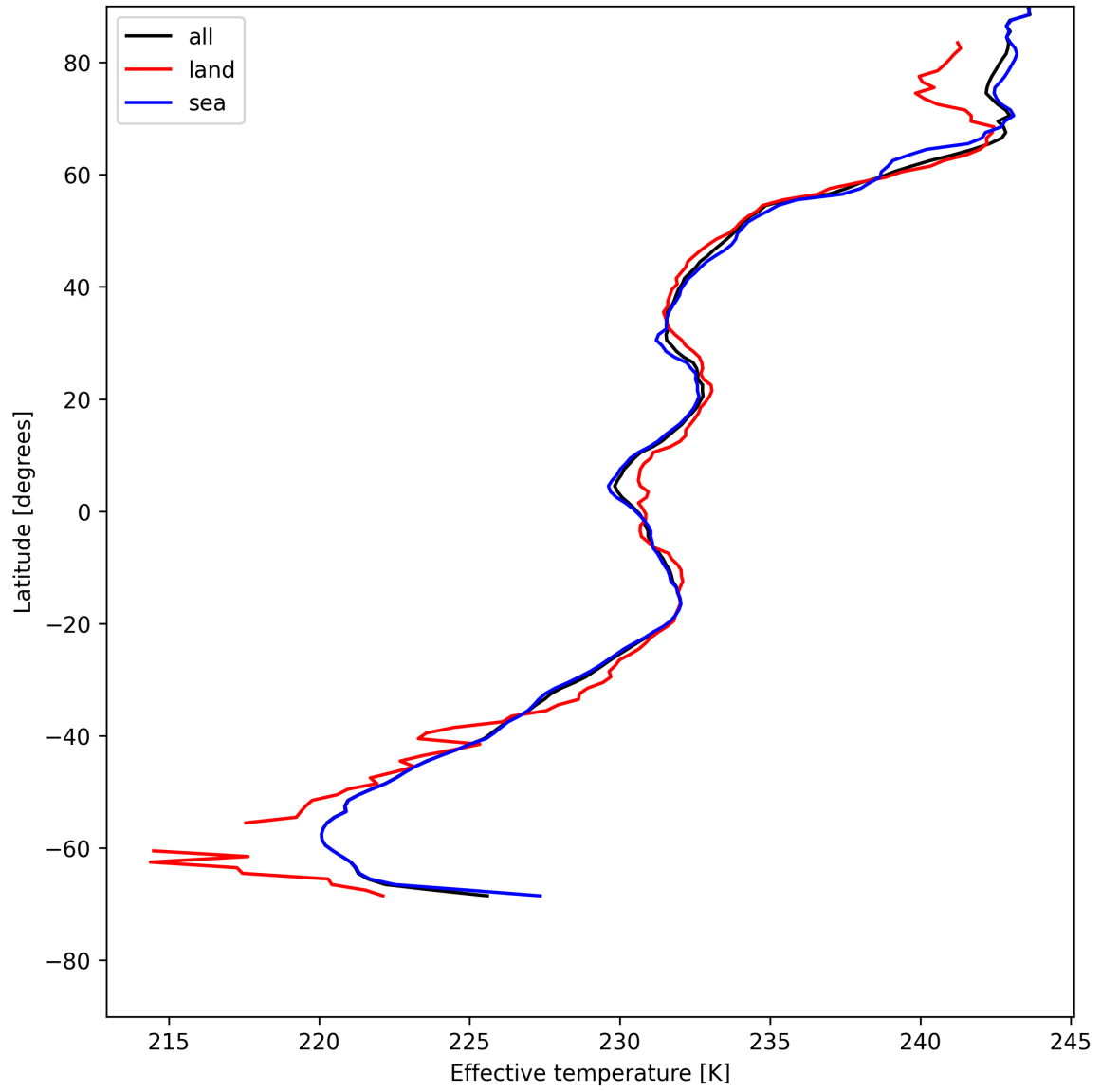
Figure 26: Zonal average of “Effective temperature” for 2025-05-20 to 2025-05-21.
