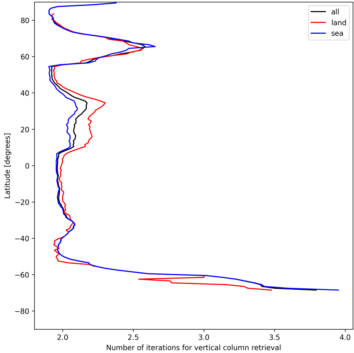
Figure 27: Zonal average of “Number of iterations for vertical column retrieval” for 2025-05-20 to 2025-05-21.
