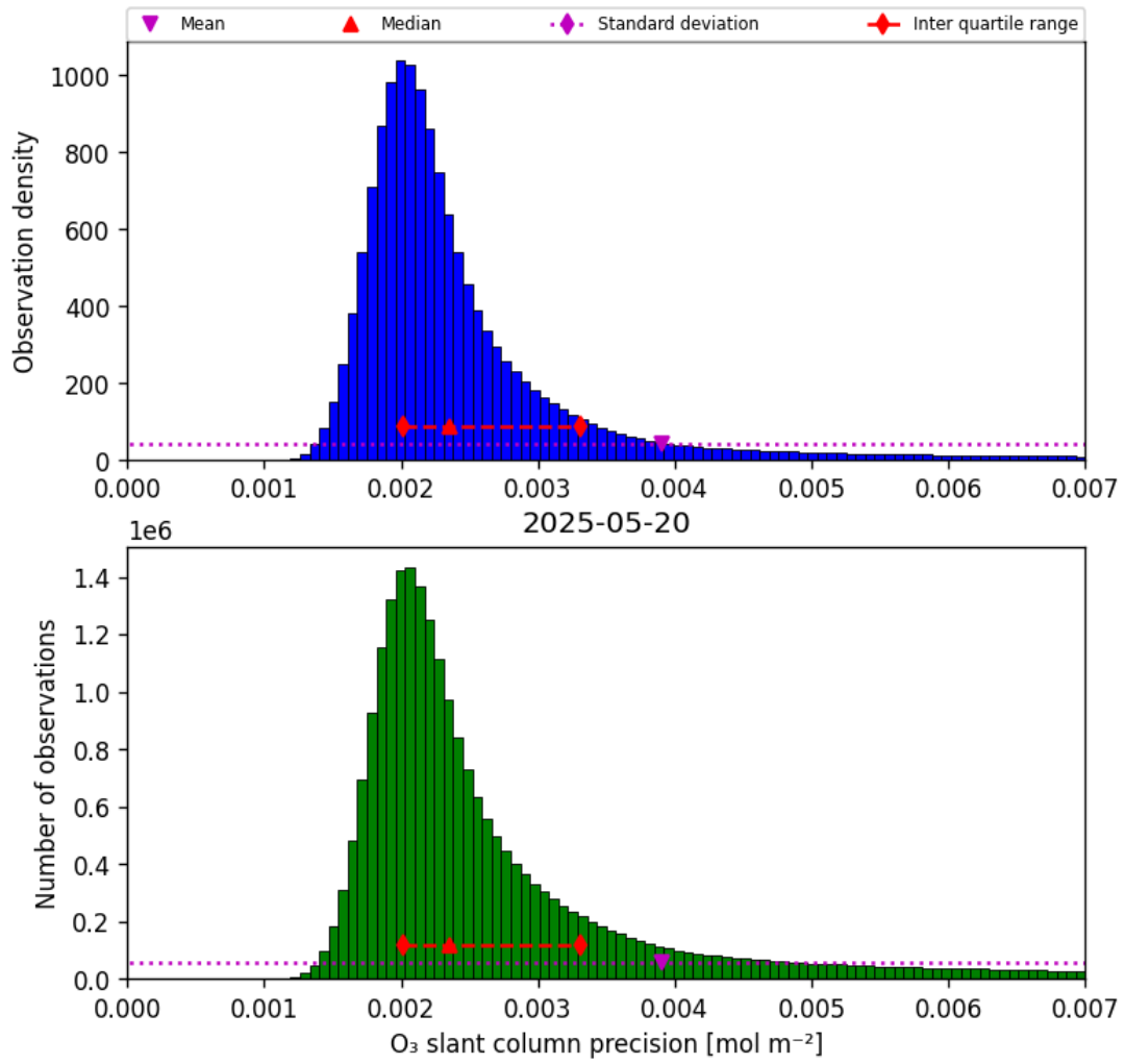
Figure 32: Histogram of “O 3 slant column precision” for 2025-05-20 to 2025-05-21
