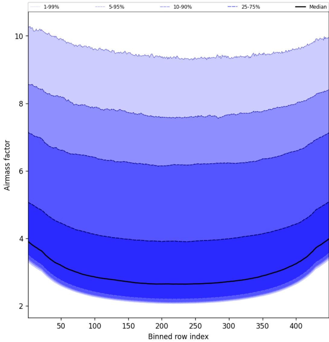
Figure 49: Along track statistics of “Airmass factor” for 2025-05-20 to 2025-05-21
