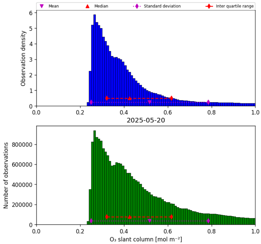
Figure 31: Histogram of “O 3 slant column” for 2025-05-20 to 2025-05-21
