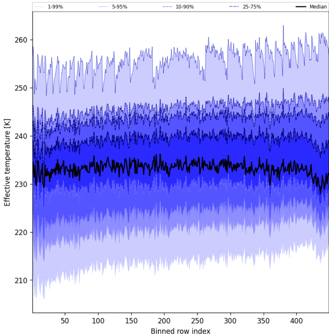
Figure 50: Along track statistics of “Effective temperature” for 2025-05-20 to 2025-05-21
