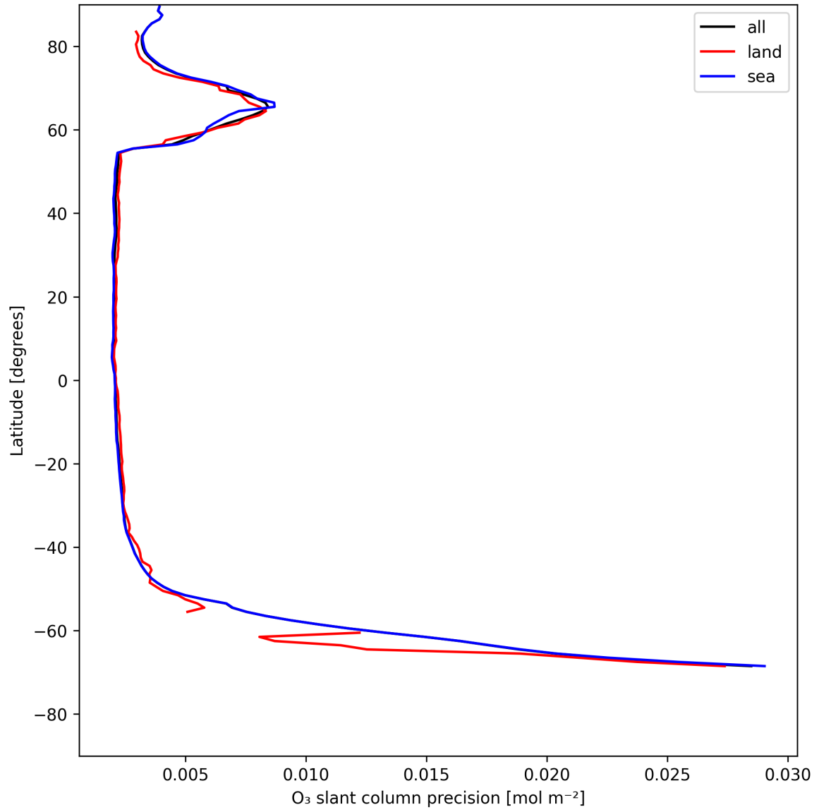
Figure 20: Zonal average of “O 3 slant column precision” for 2025-05-20 to 2025-05-21.
