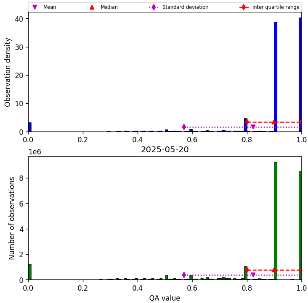
Figure 28: Histogram of “QA value” for 2025-05-20 to 2025-05-21
