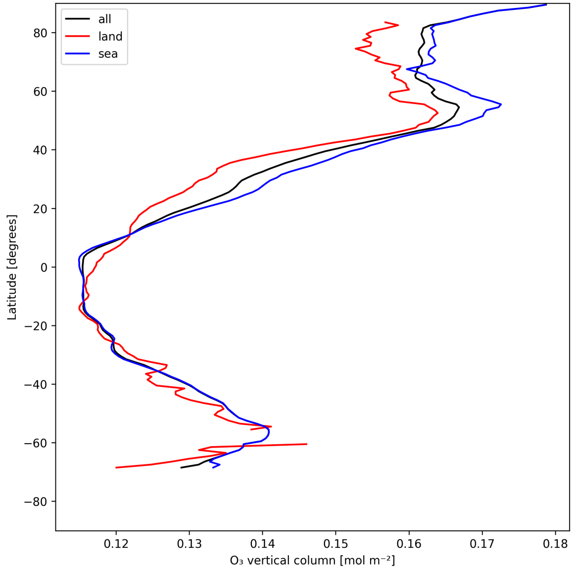
Figure 17: Zonal average of “O 3 vertical column” for 2025-05-20 to 2025-05-21.
