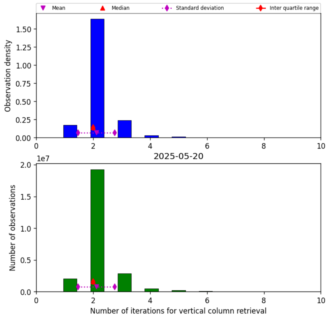
Figure 39: Histogram of “Number of iterations for vertical column retrieval” for 2025-05-20 to 2025-05-21
