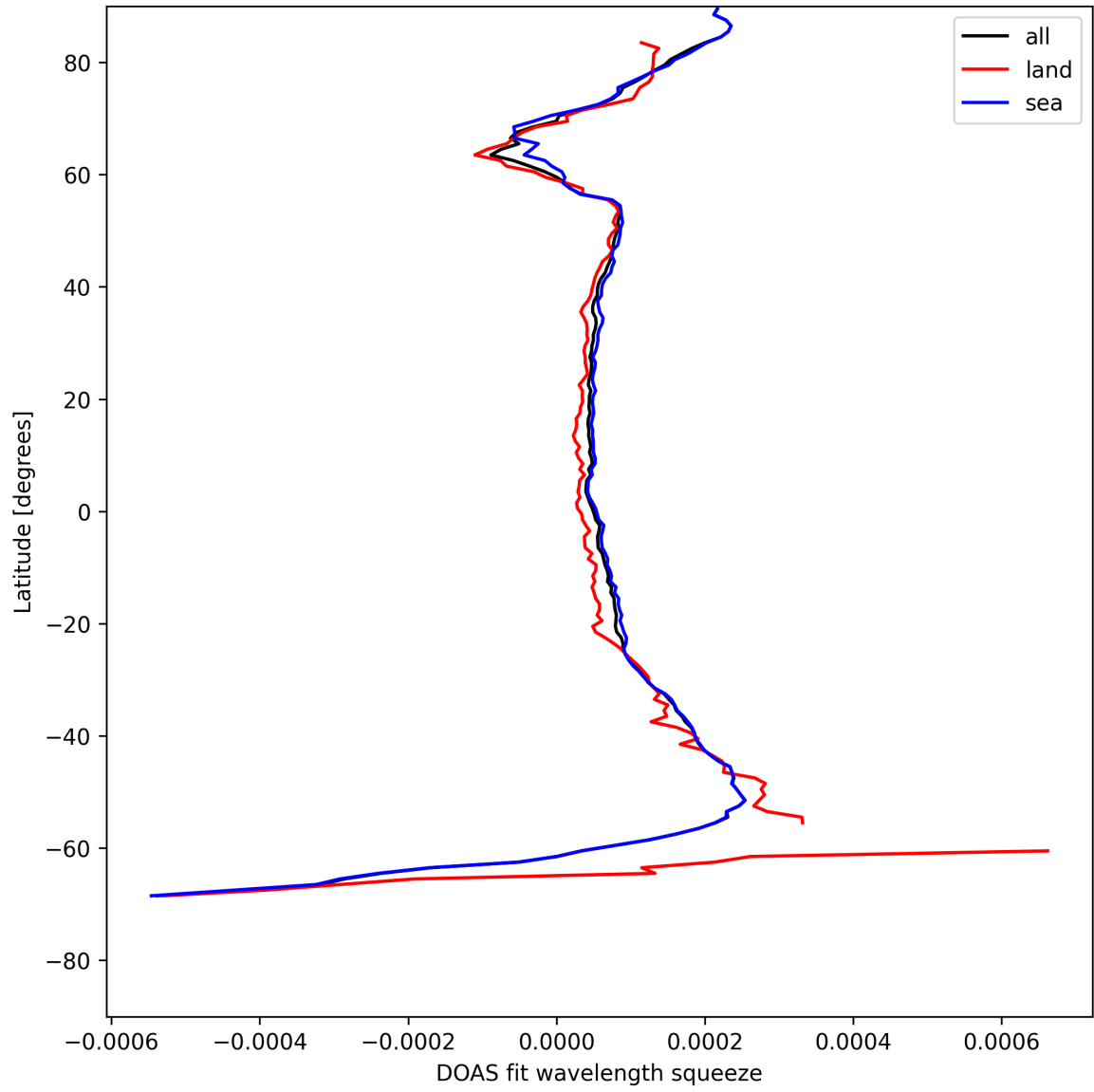
Figure 24: Zonal average of “DOAS fit wavelength squeeze” for 2025-05-20 to 2025-05-21.
