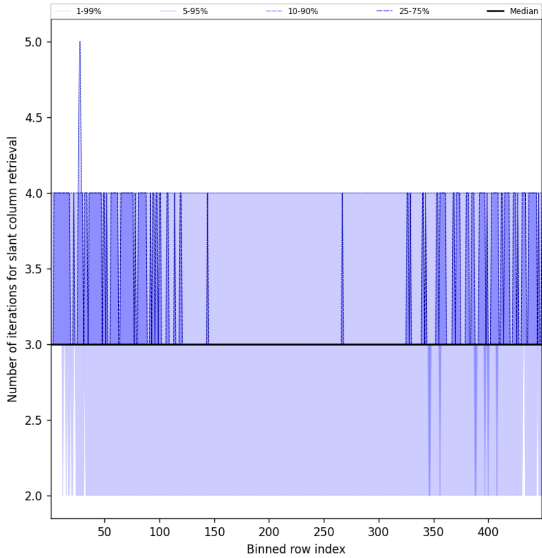
Figure 45: Along track statistics of “Number of iterations for slant column retrieval” for 2025-05-20 to 2025-05-21
