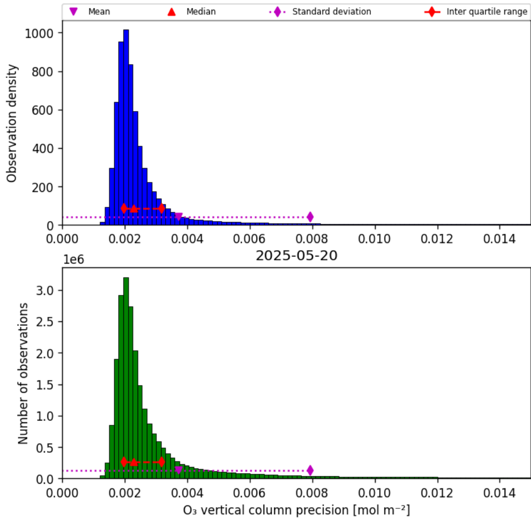
Figure 30: Histogram of “O 3 vertical column precision” for 2025-05-20 to 2025-05-21
