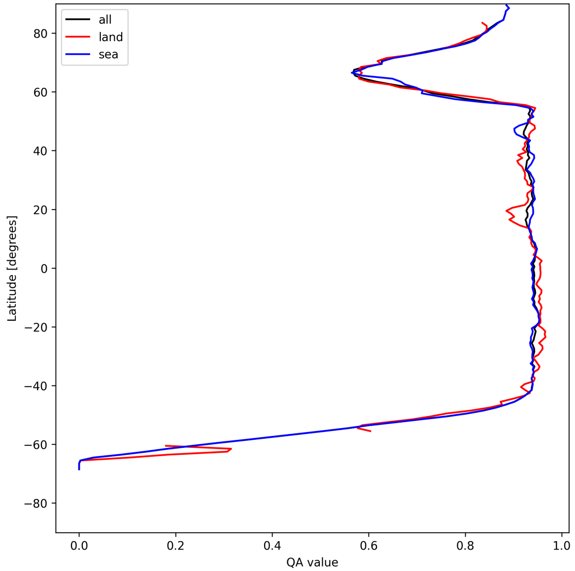
Figure 16: Zonal average of “QA value” for 2025-05-20 to 2025-05-21.
