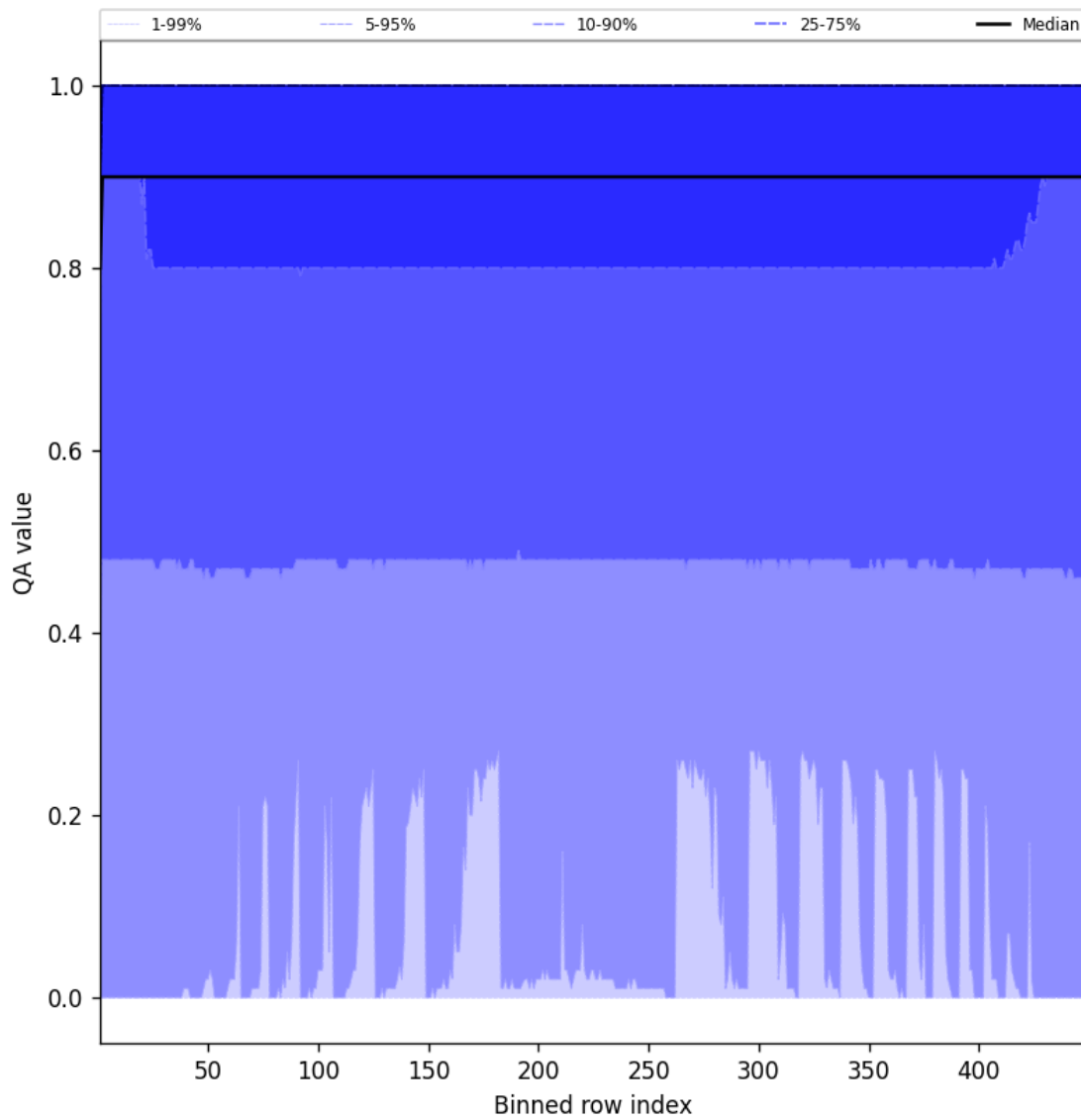
Figure 40: Along track statistics of “QA value” for 2025-05-20 to 2025-05-21
