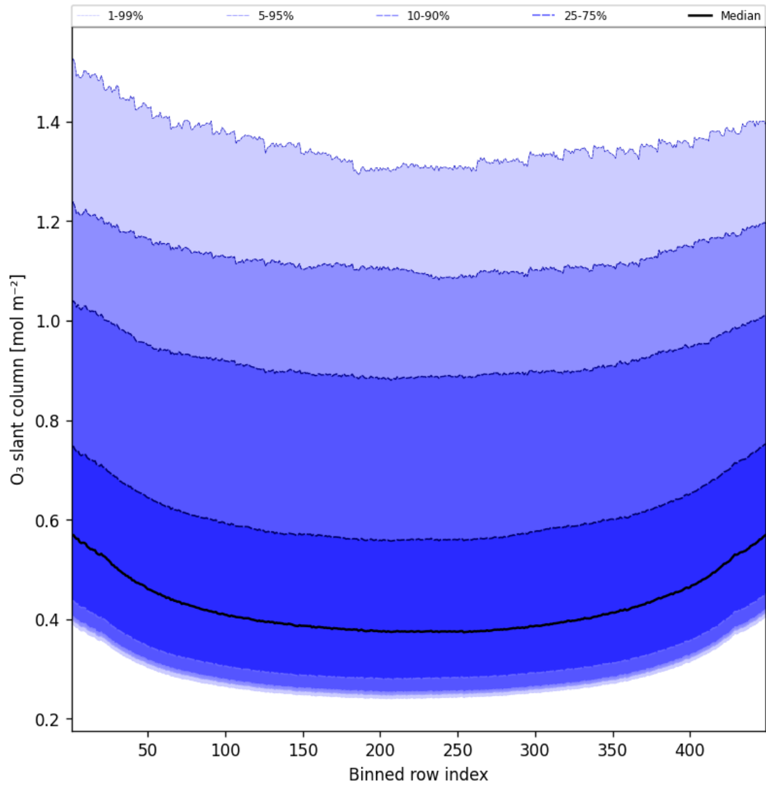
Figure 43: Along track statistics of “O 3 slant column” for 2025-05-20 to 2025-05-21
