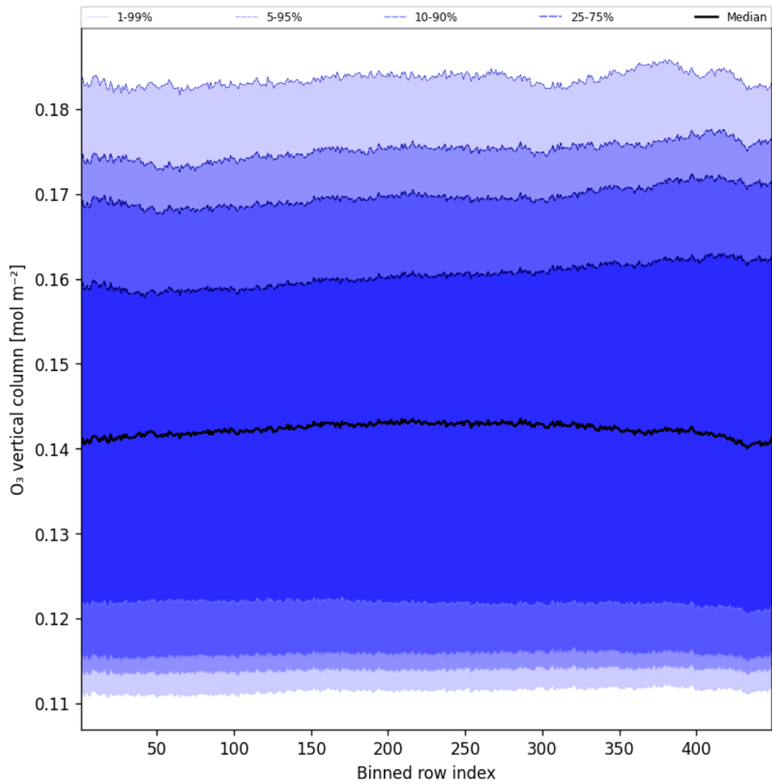
Figure 41: Along track statistics of “O 3 vertical column” for 2025-05-20 to 2025-05-21
