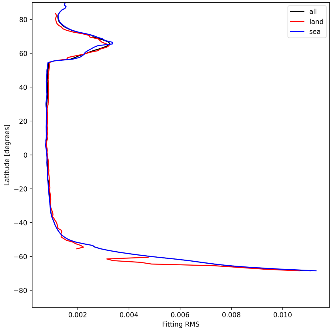
Figure 22: Zonal average of “Fitting RMS” for 2025-05-20 to 2025-05-21.
