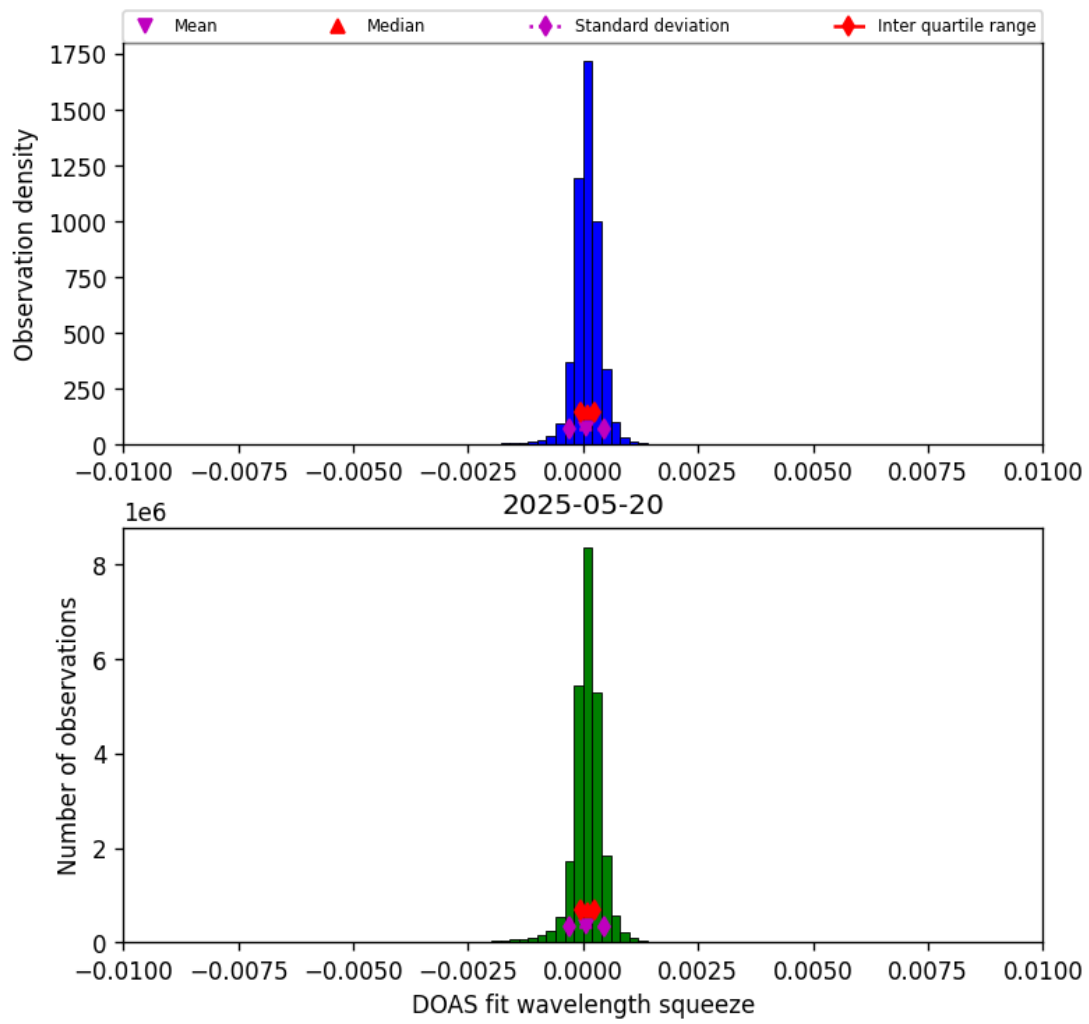
Figure 36: Histogram of “DOAS fit wavelength squeeze” for 2025-05-20 to 2025-05-21
