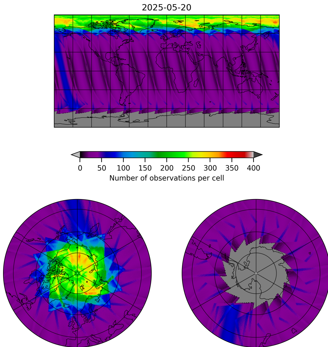
Figure 15: Map of the number of observations for 2025-05-20 to 2025-05-21
