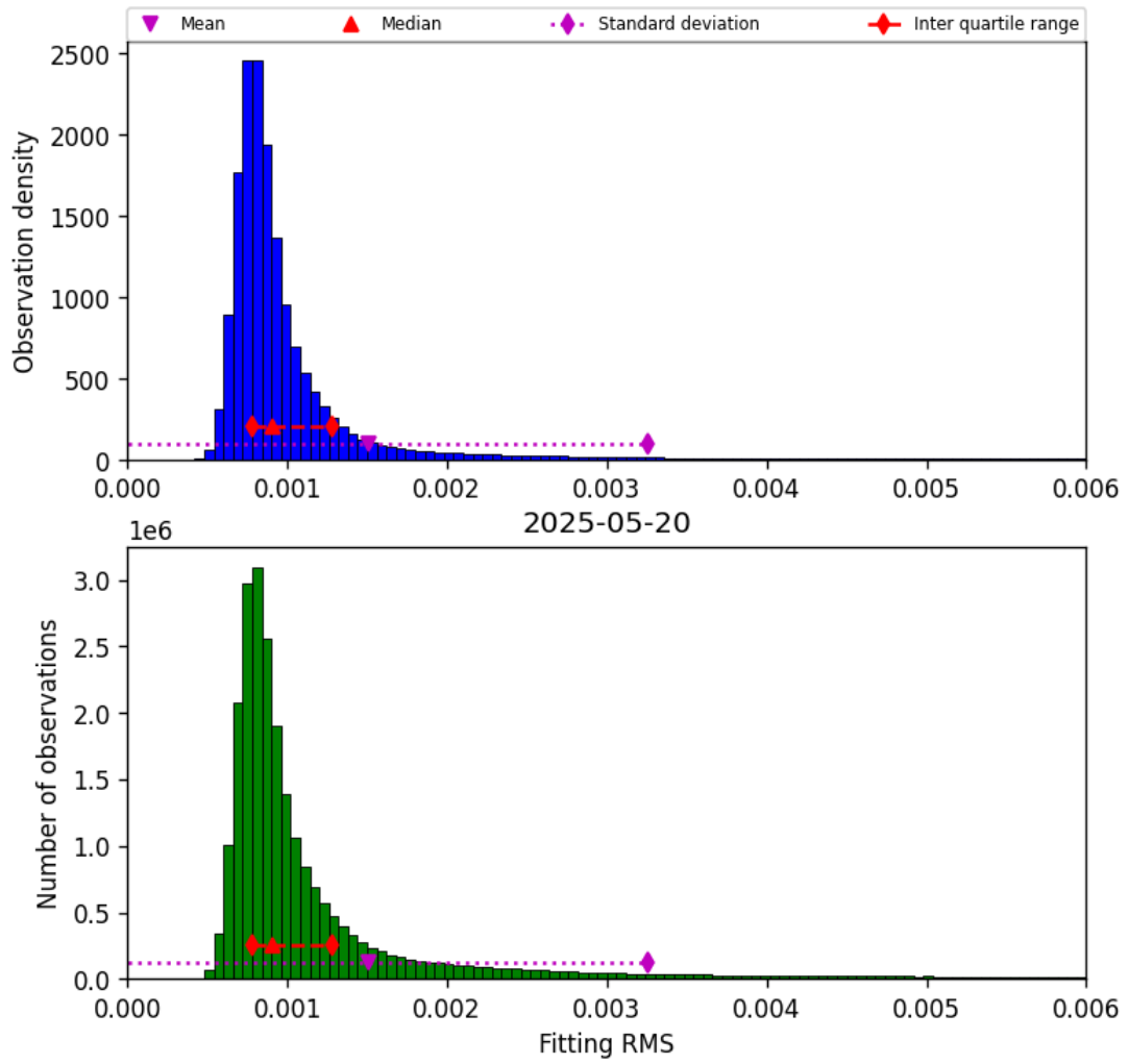
Figure 34: Histogram of “Fitting RMS” for 2025-05-20 to 2025-05-21
