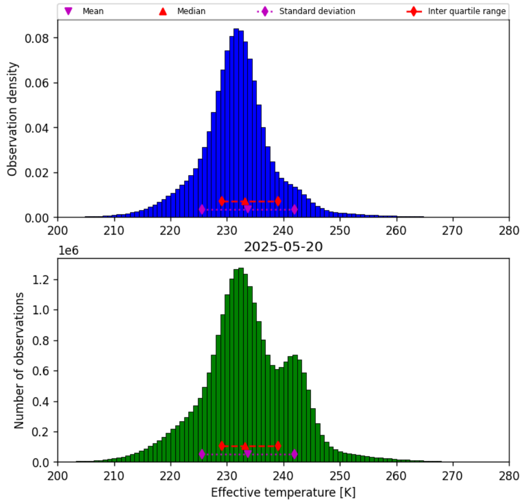
Figure 38: Histogram of “Effective temperature” for 2025-05-20 to 2025-05-21
