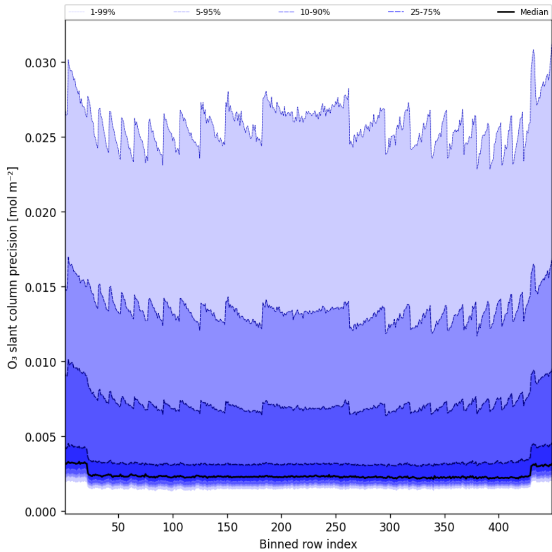
Figure 44: Along track statistics of “O 3 slant column precision” for 2025-05-20 to 2025-05-21
