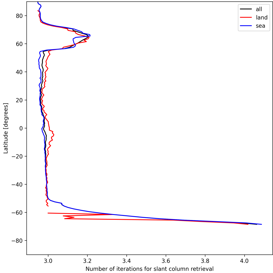
Figure 21: Zonal average of “Number of iterations for slant column retrieval” for 2025-05-20 to 2025-05-21.
