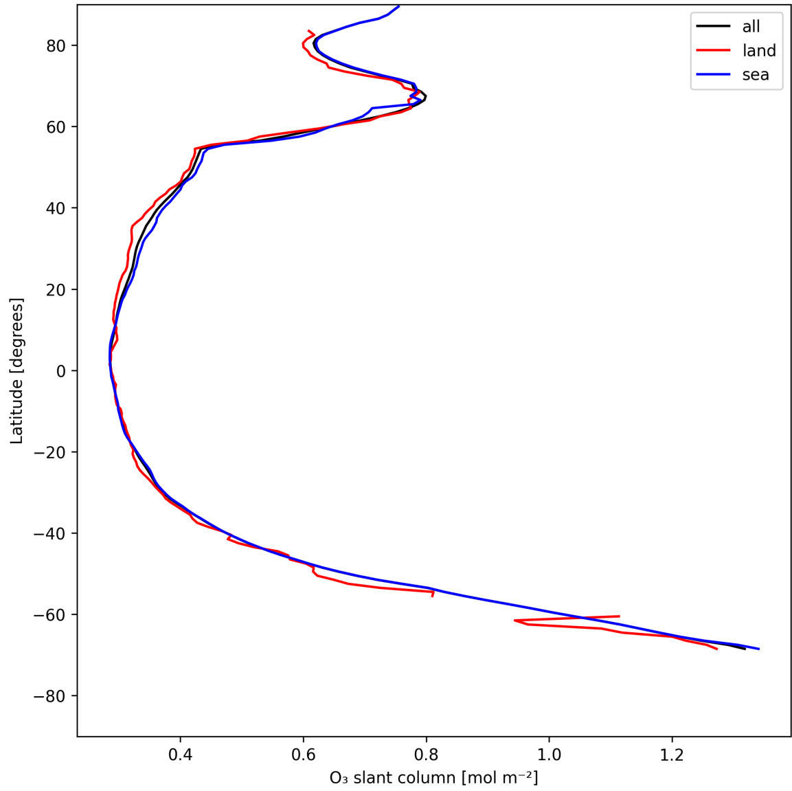
Figure 19: Zonal average of “O 3 slant column” for 2025-05-20 to 2025-05-21.
