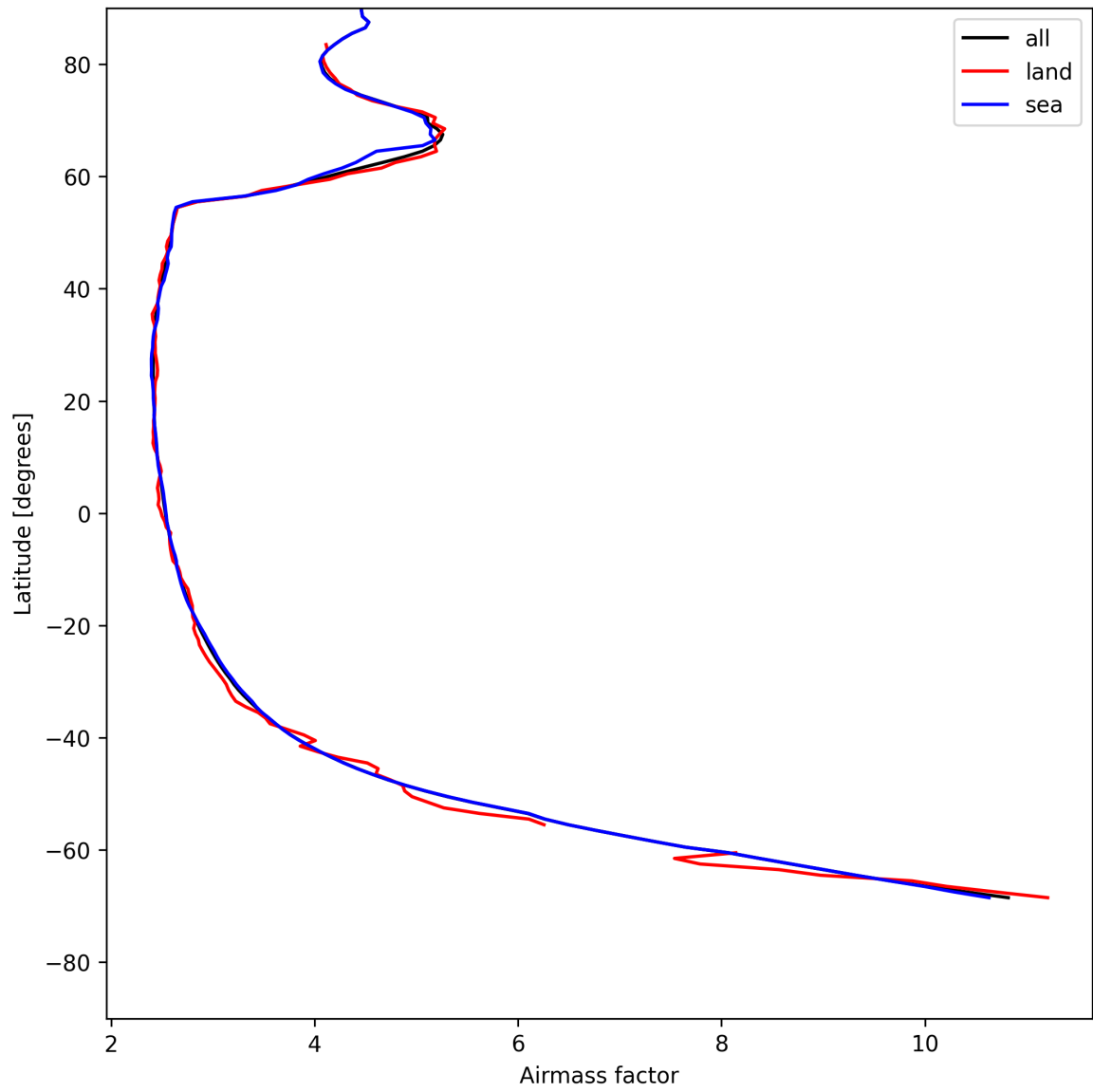
Figure 25: Zonal average of “Airmass factor” for 2025-05-20 to 2025-05-21.
