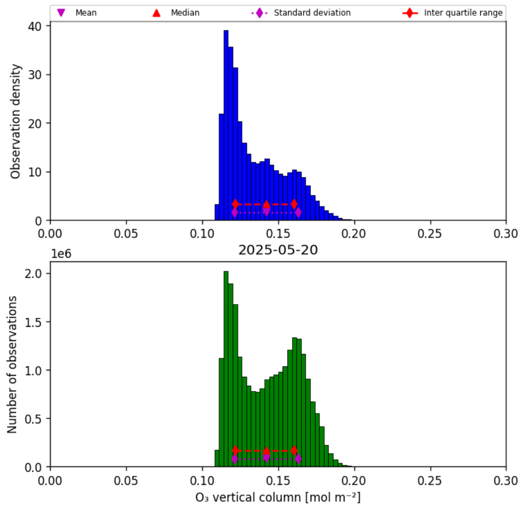
Figure 29: Histogram of “O 3 vertical column” for 2025-05-20 to 2025-05-21
