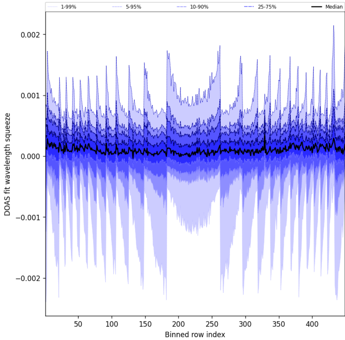
Figure 48: Along track statistics of “DOAS fit wavelength squeeze” for 2025-05-20 to 2025-05-21
