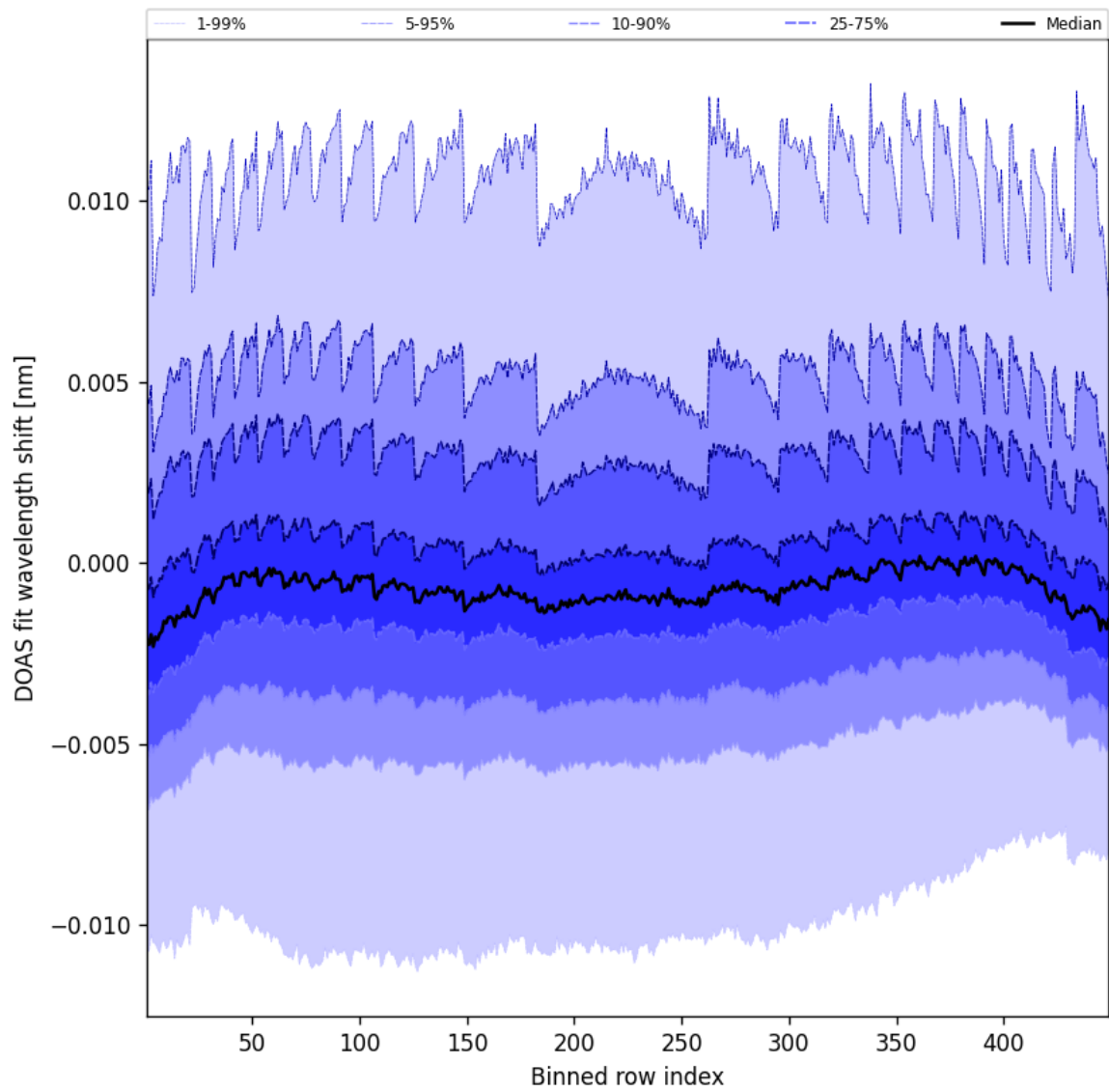
Figure 47: Along track statistics of “DOAS fit wavelength shift” for 2025-05-20 to 2025-05-21
