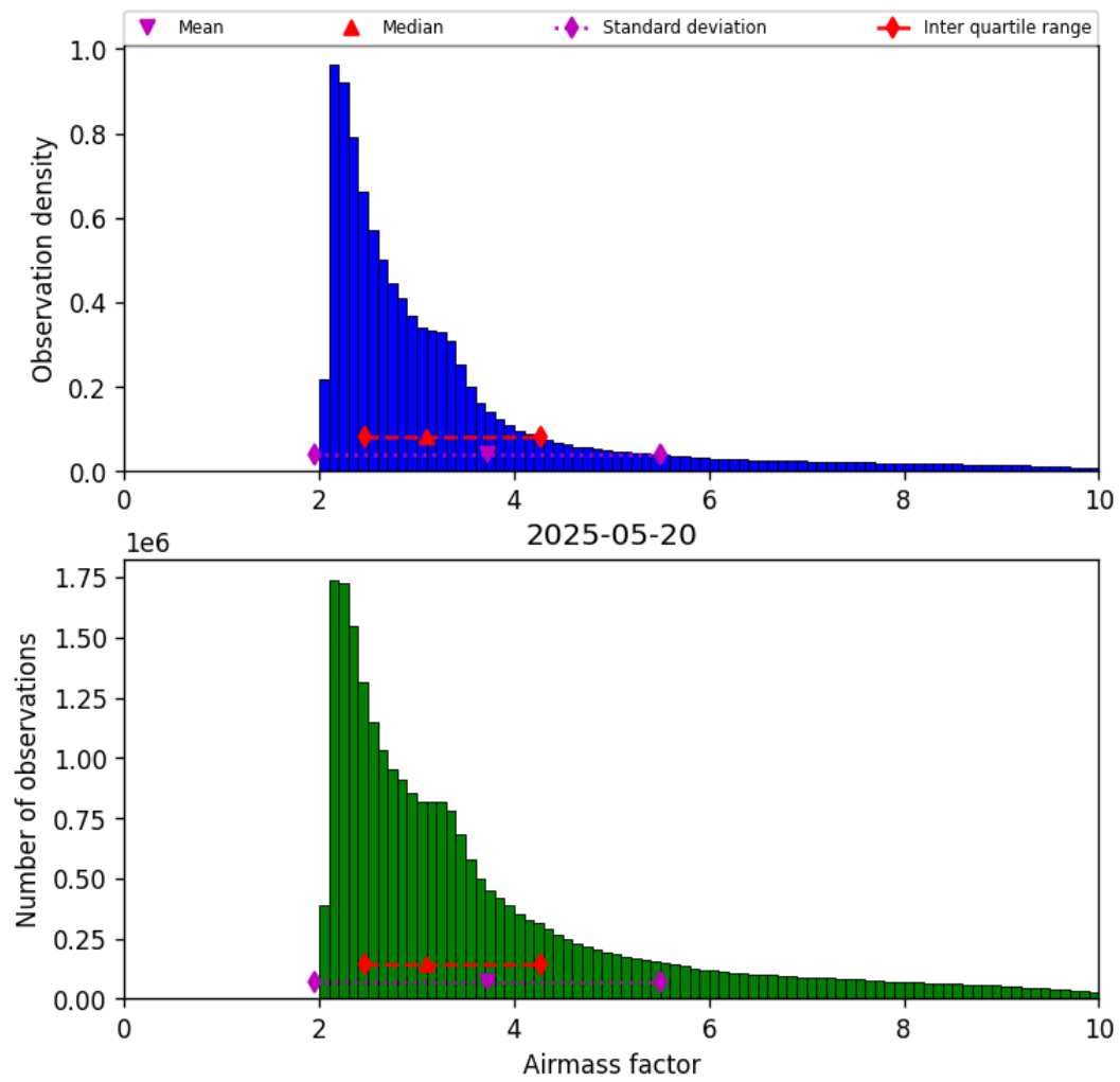
Figure 37: Histogram of “Airmass factor” for 2025-05-20 to 2025-05-21
