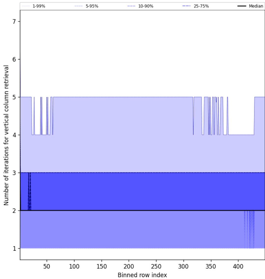
Figure 51: Along track statistics of “Number of iterations for vertical column retrieval” for 2025-05-20 to 2025-05-21
