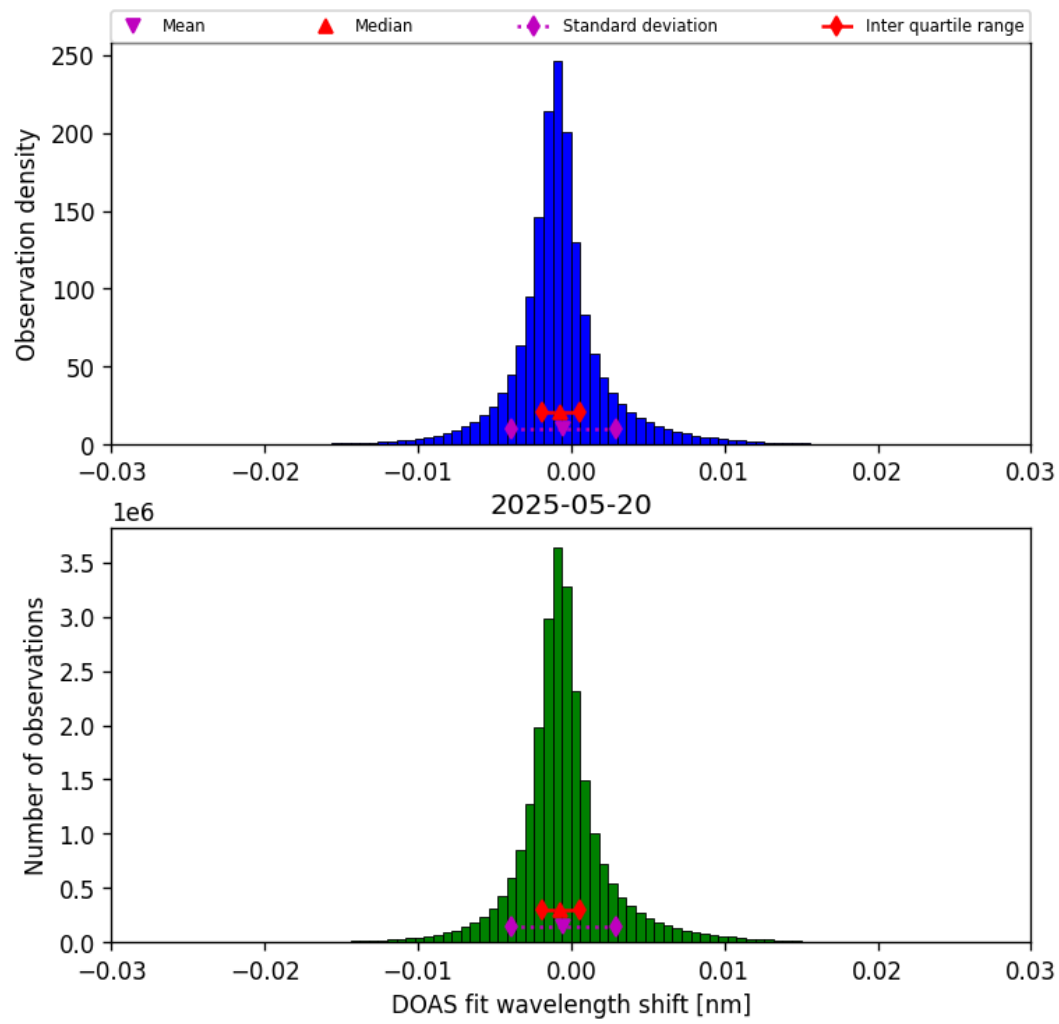
Figure 35: Histogram of “DOAS fit wavelength shift” for 2025-05-20 to 2025-05-21
