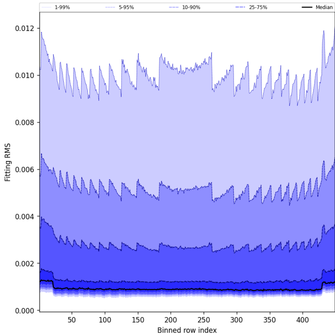
Figure 46: Along track statistics of “Fitting RMS” for 2025-05-20 to 2025-05-21
