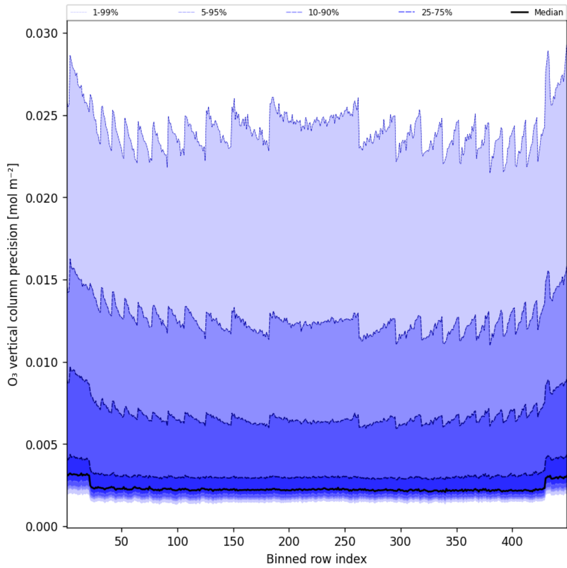
Figure 42: Along track statistics of “O 3 vertical column precision” for 2025-05-20 to 2025-05-21
