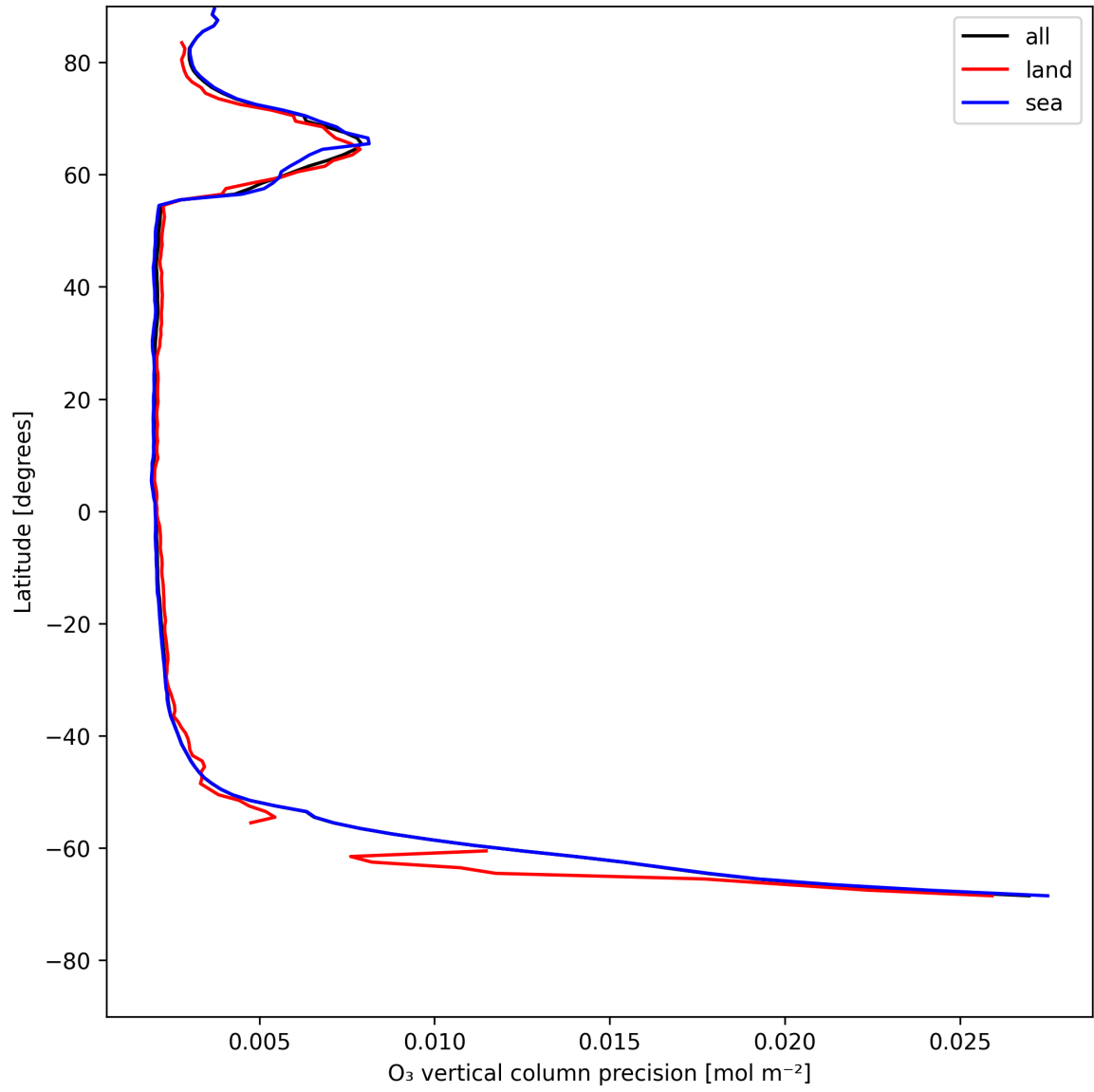
Figure 18: Zonal average of “O 3 vertical column precision” for 2025-05-20 to 2025-05-21.
