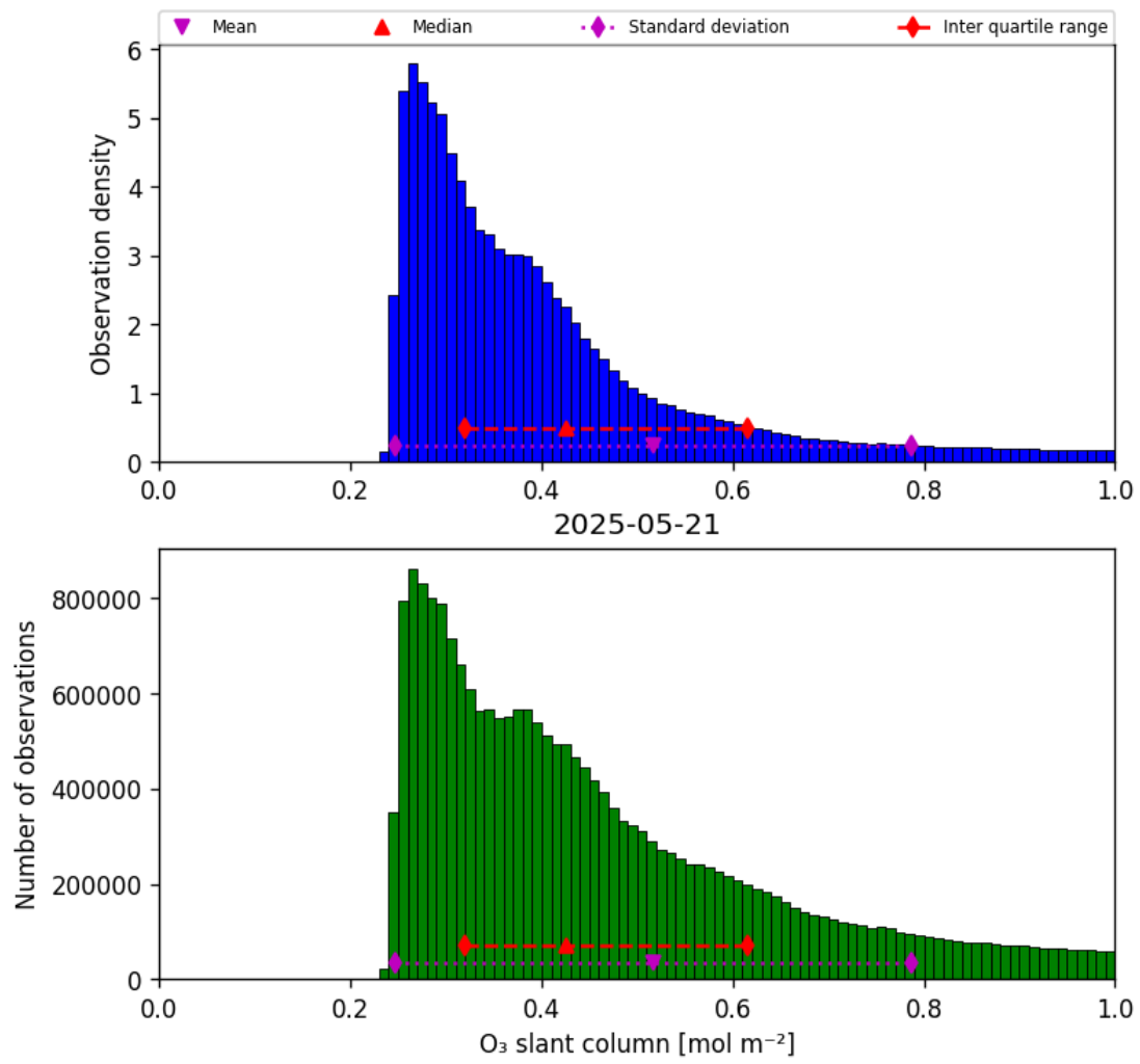
Figure 31: Histogram of “O 3 slant column” for 2025-05-21 to 2025-05-22
