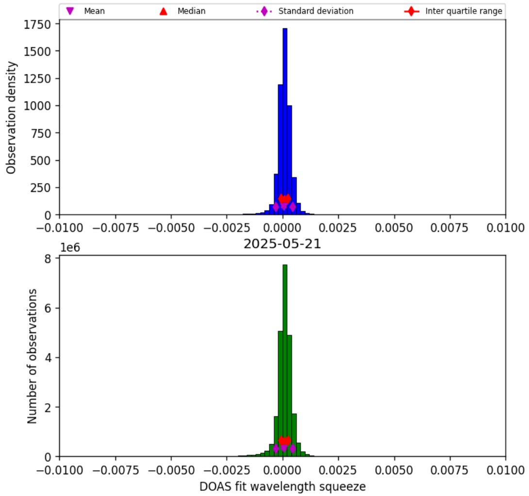
Figure 36: Histogram of “DOAS fit wavelength squeeze” for 2025-05-21 to 2025-05-22
