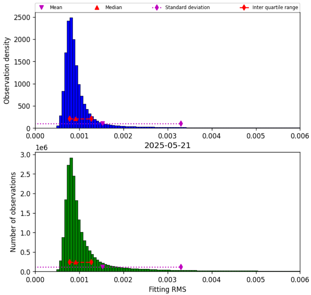
Figure 34: Histogram of “Fitting RMS” for 2025-05-21 to 2025-05-22
