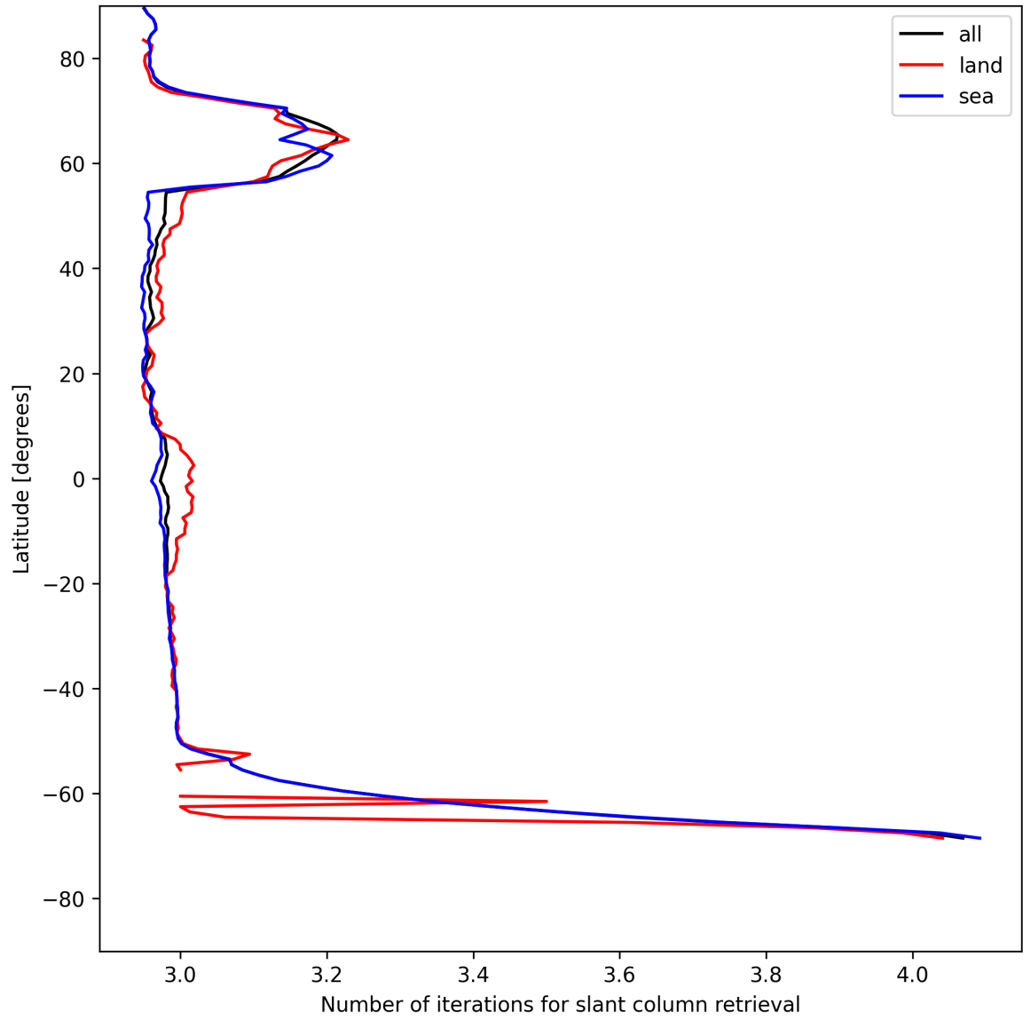
Figure 21: Zonal average of “Number of iterations for slant column retrieval” for 2025-05-21 to 2025-05-22.
