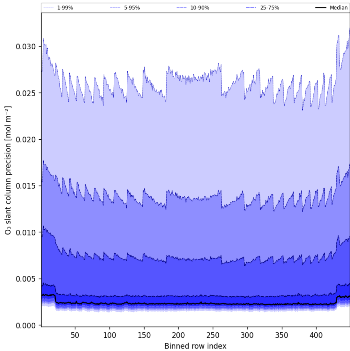
Figure 44: Along track statistics of “O 3 slant column precision” for 2025-05-21 to 2025-05-22
