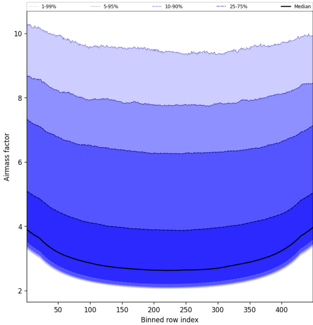
Figure 49: Along track statistics of “Airmass factor” for 2025-05-21 to 2025-05-22
