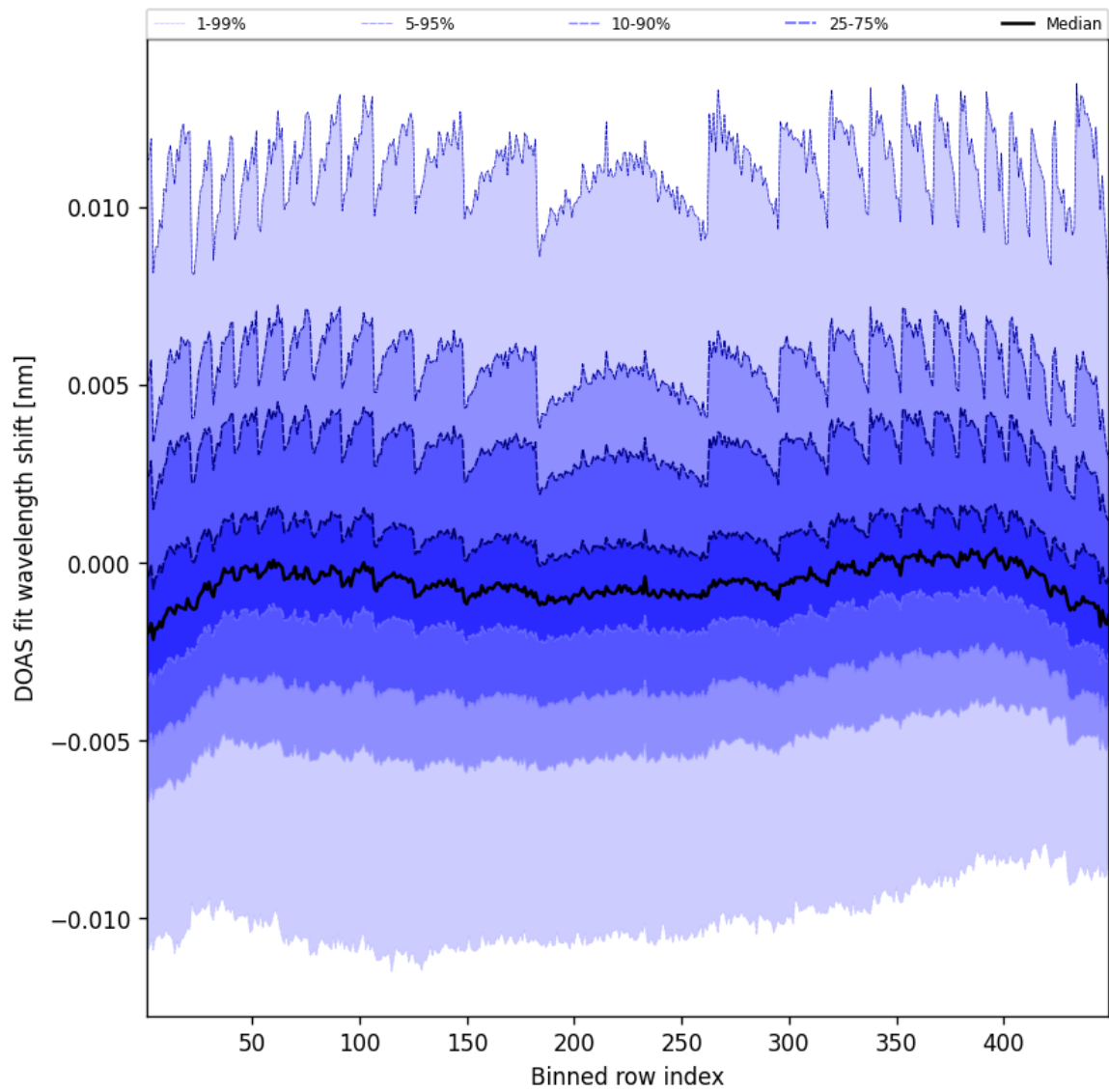
Figure 47: Along track statistics of “DOAS fit wavelength shift” for 2025-05-21 to 2025-05-22
