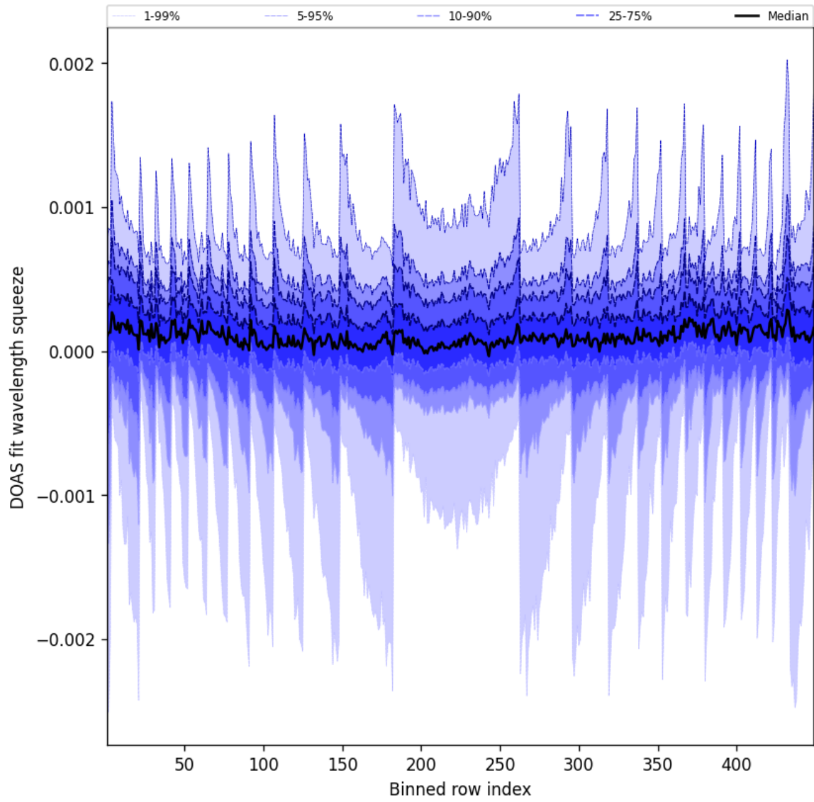
Figure 48: Along track statistics of “DOAS fit wavelength squeeze” for 2025-05-21 to 2025-05-22
