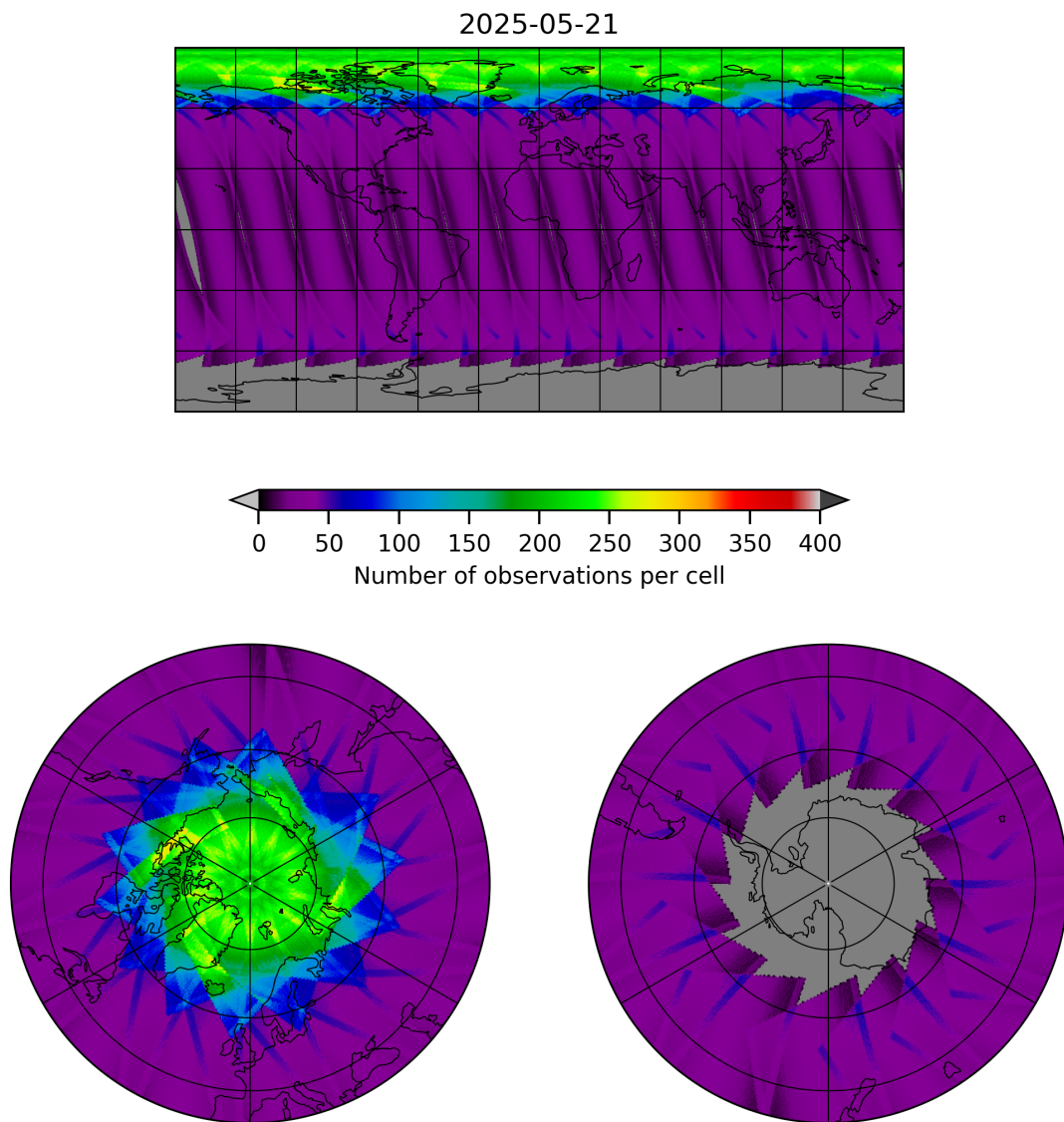
Figure 15: Map of the number of observations for 2025-05-21 to 2025-05-22
