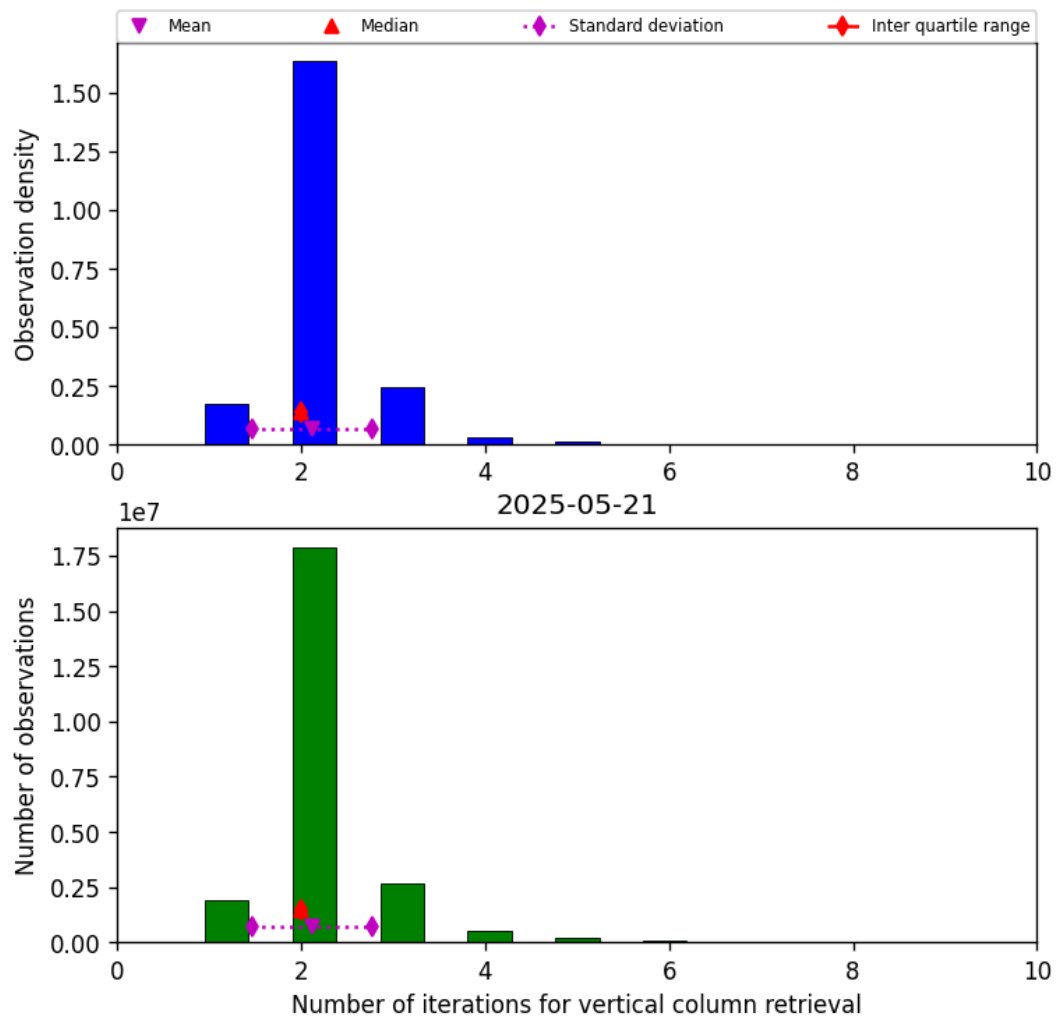
Figure 39: Histogram of “Number of iterations for vertical column retrieval” for 2025-05-21 to 2025-05-22
