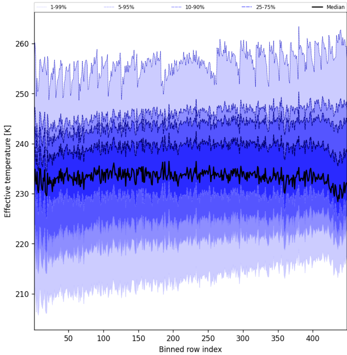
Figure 50: Along track statistics of “Effective temperature” for 2025-05-21 to 2025-05-22
