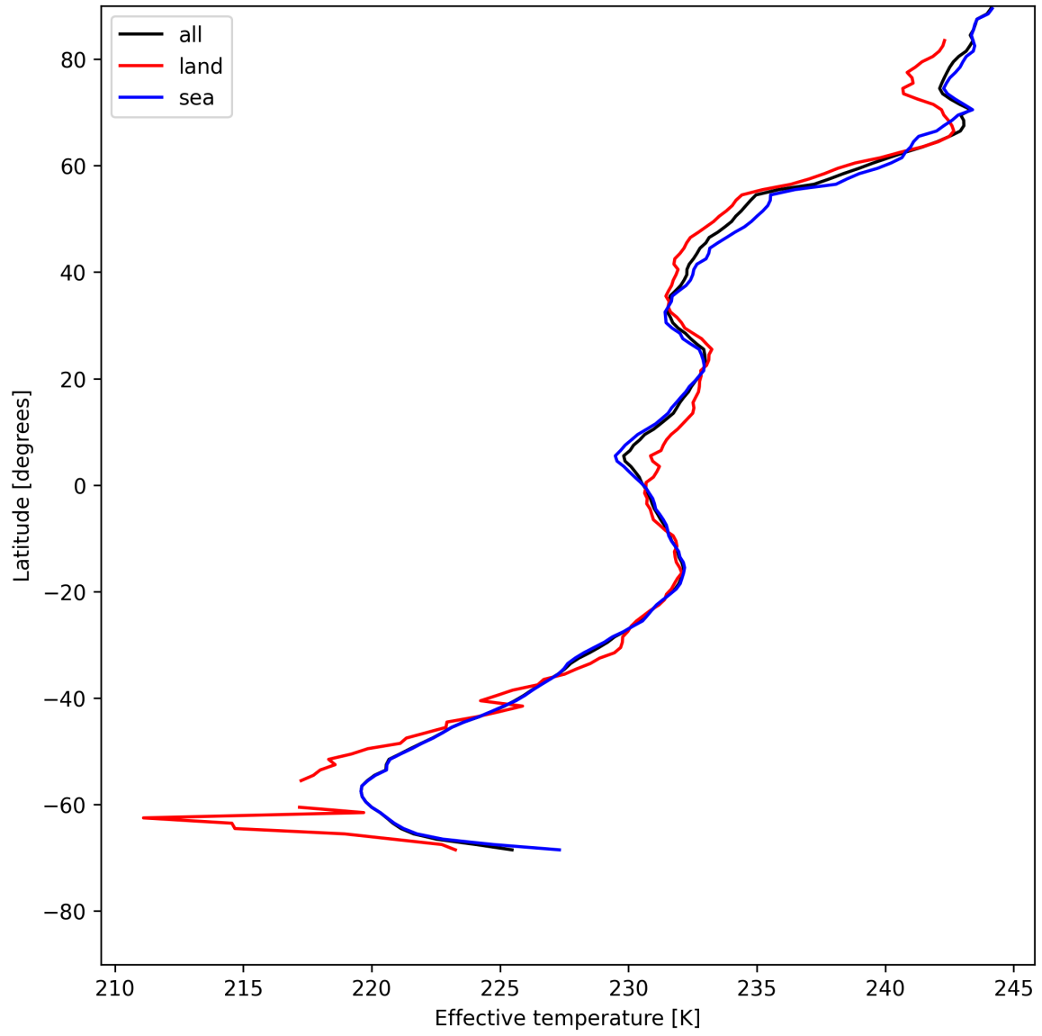
Figure 26: Zonal average of "Effective temperature" for 2025-05-21 to 2025-05-22.
