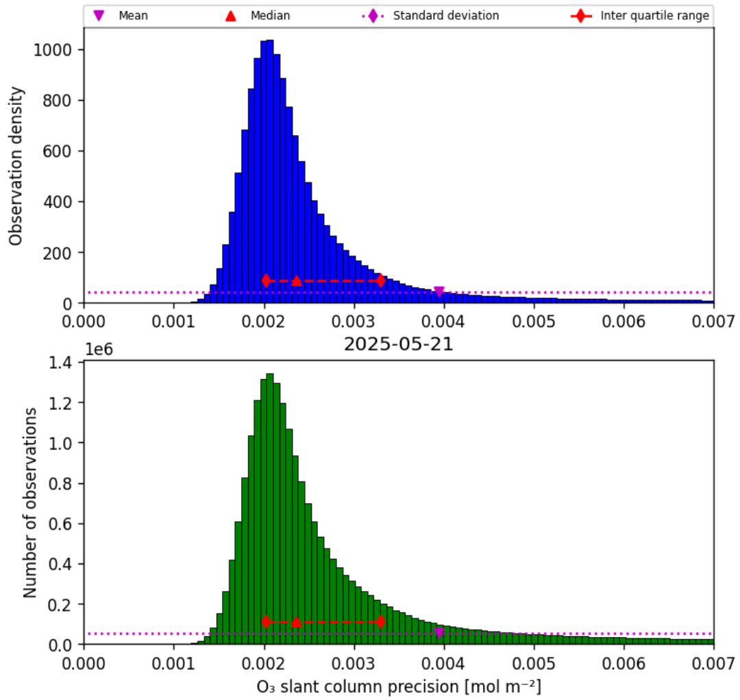
Figure 32: Histogram of “O 3 slant column precision” for 2025-05-21 to 2025-05-22
