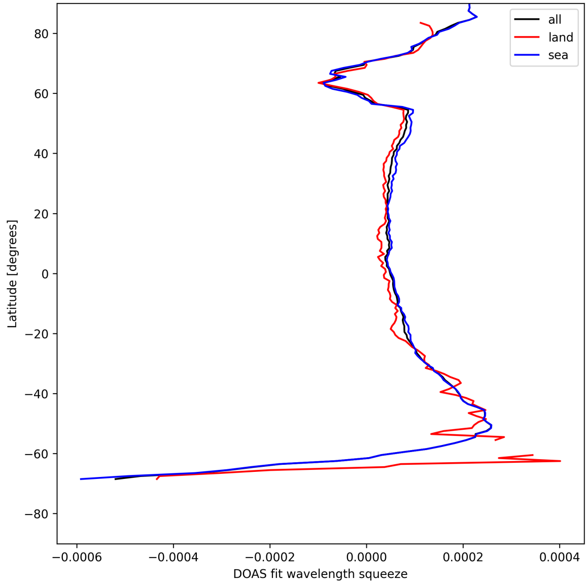
Figure 24: Zonal average of “DOAS fit wavelength squeeze” for 2025-05-21 to 2025-05-22.
