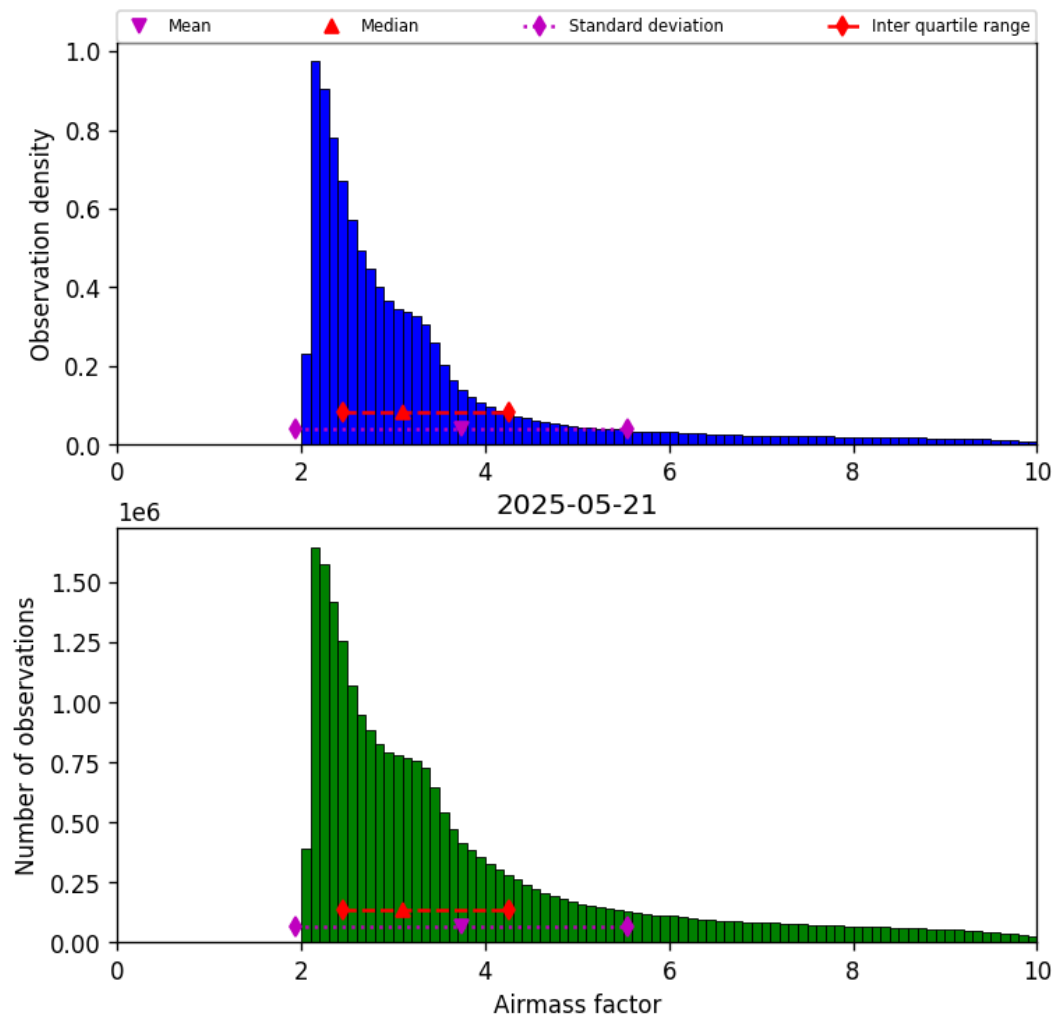
Figure 37: Histogram of “Airmass factor” for 2025-05-21 to 2025-05-22
