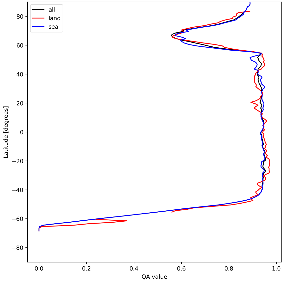
Figure 16: Zonal average of “QA value” for 2025-05-21 to 2025-05-22.
