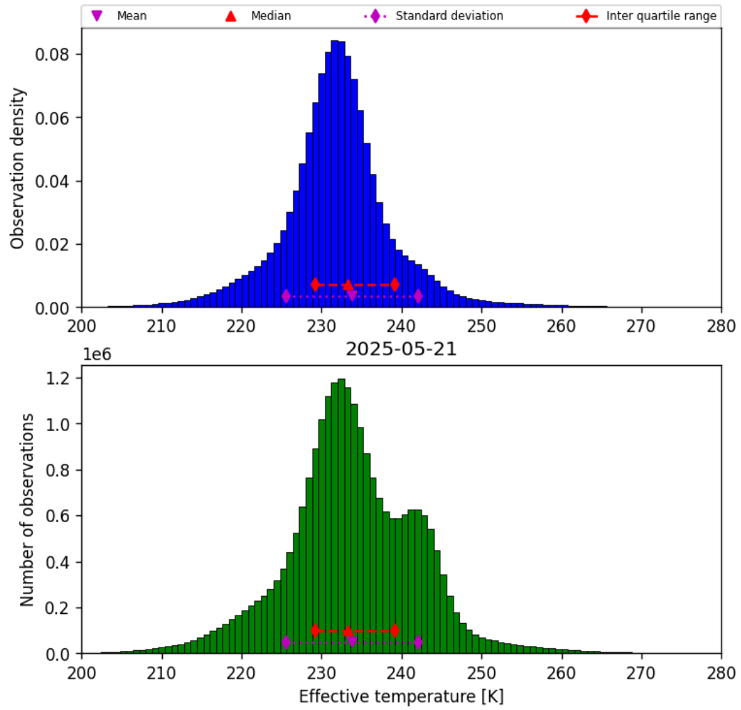
Figure 38: Histogram of “Effective temperature” for 2025-05-21 to 2025-05-22
