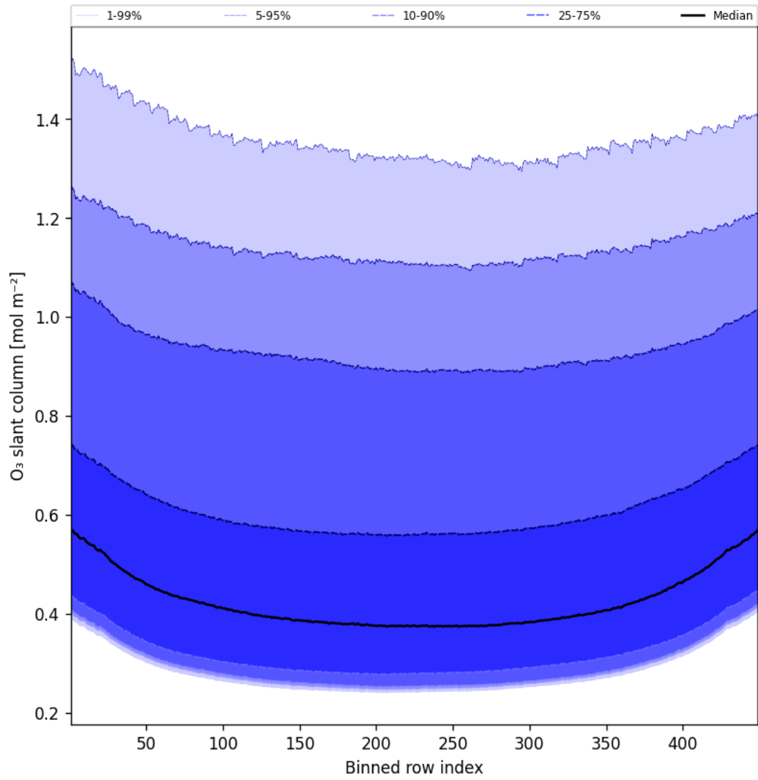
Figure 43: Along track statistics of “O 3 slant column” for 2025-05-21 to 2025-05-22
