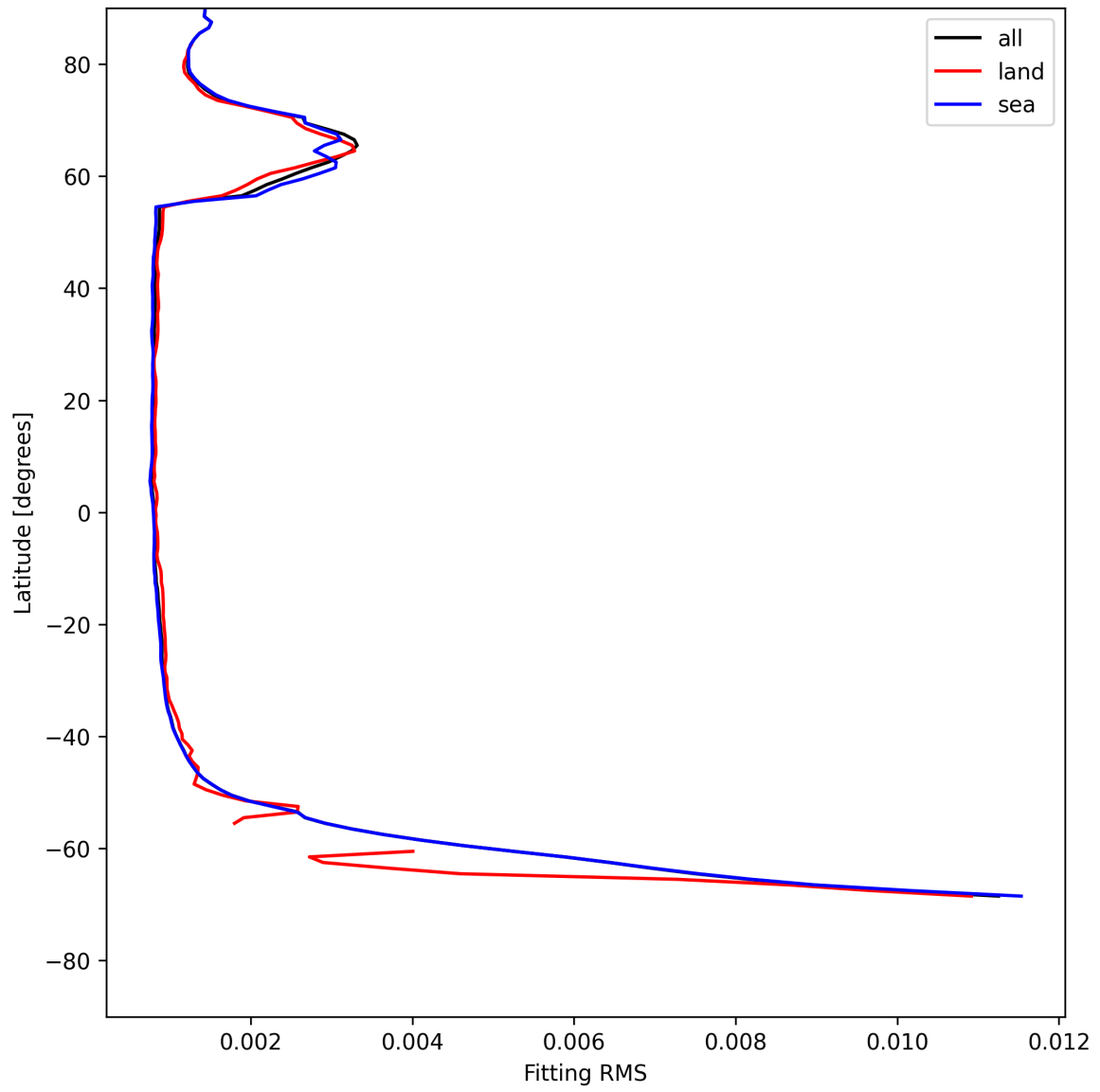
Figure 22: Zonal average of “Fitting RMS” for 2025-05-21 to 2025-05-22.
