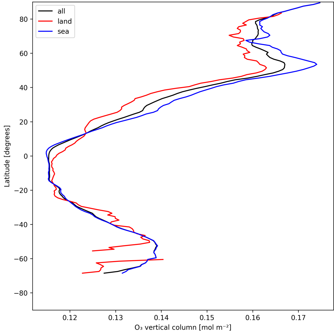
Figure 17: Zonal average of “O 3 vertical column” for 2025-05-21 to 2025-05-22.
