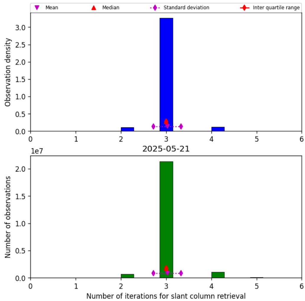
Figure 33: Histogram of “Number of iterations for slant column retrieval” for 2025-05-21 to 2025-05-22
