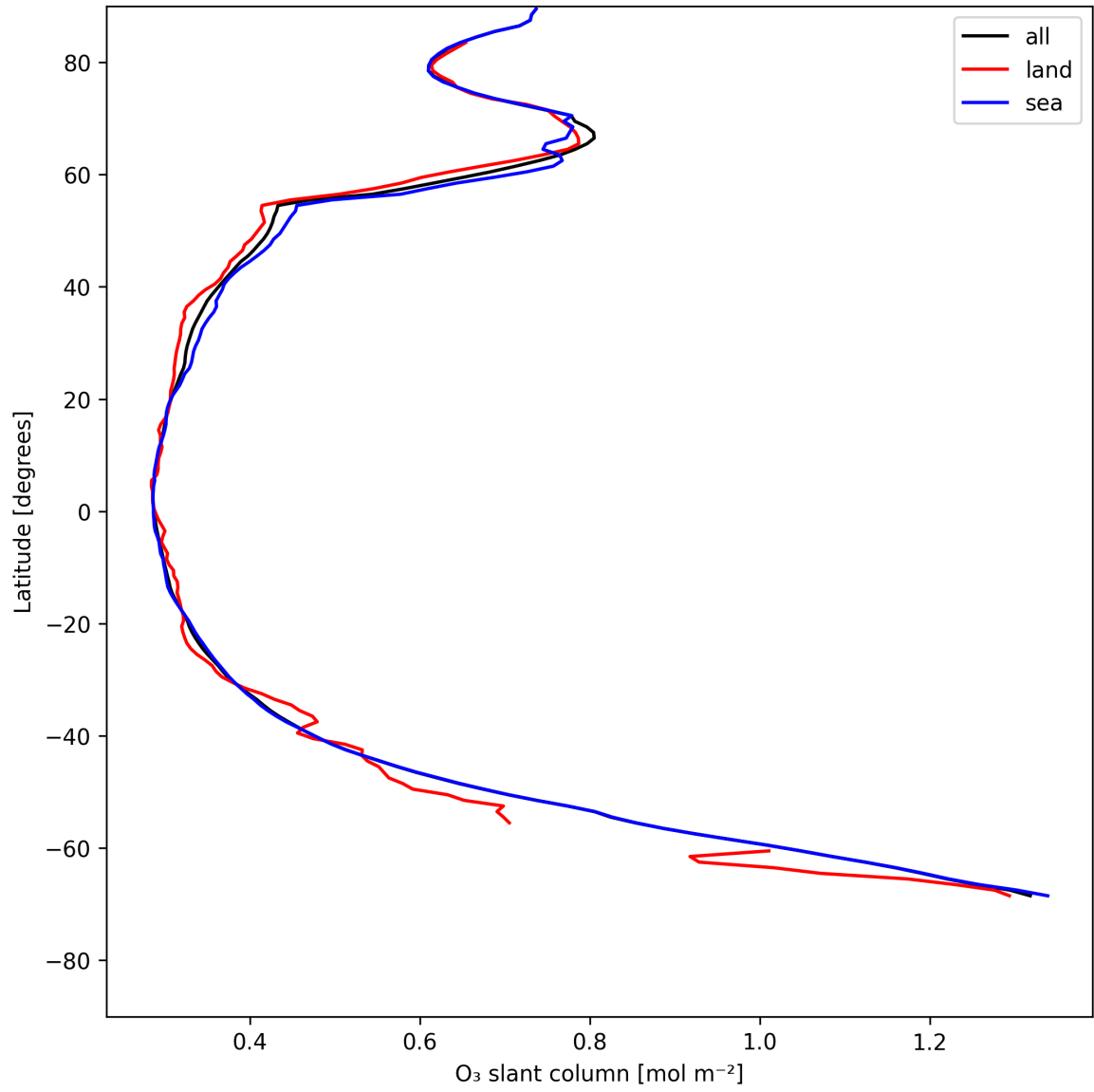
Figure 19: Zonal average of “O 3 slant column” for 2025-05-21 to 2025-05-22.
