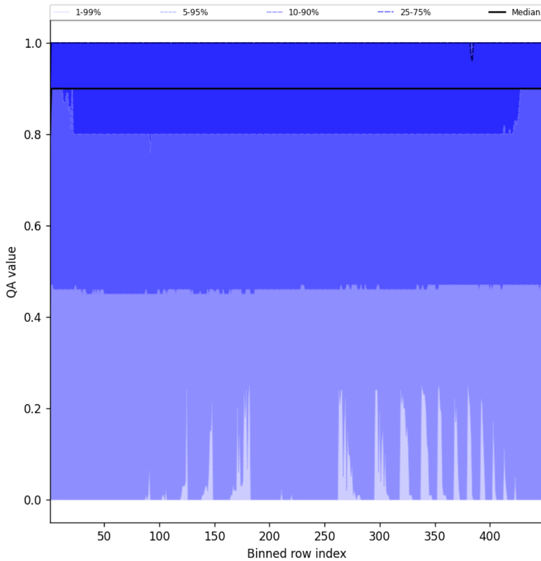
Figure 40: Along track statistics of “QA value” for 2025-05-21 to 2025-05-22
