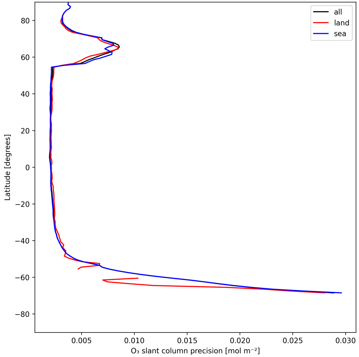
Figure 20: Zonal average of “O 3 slant column precision” for 2025-05-21 to 2025-05-22.
