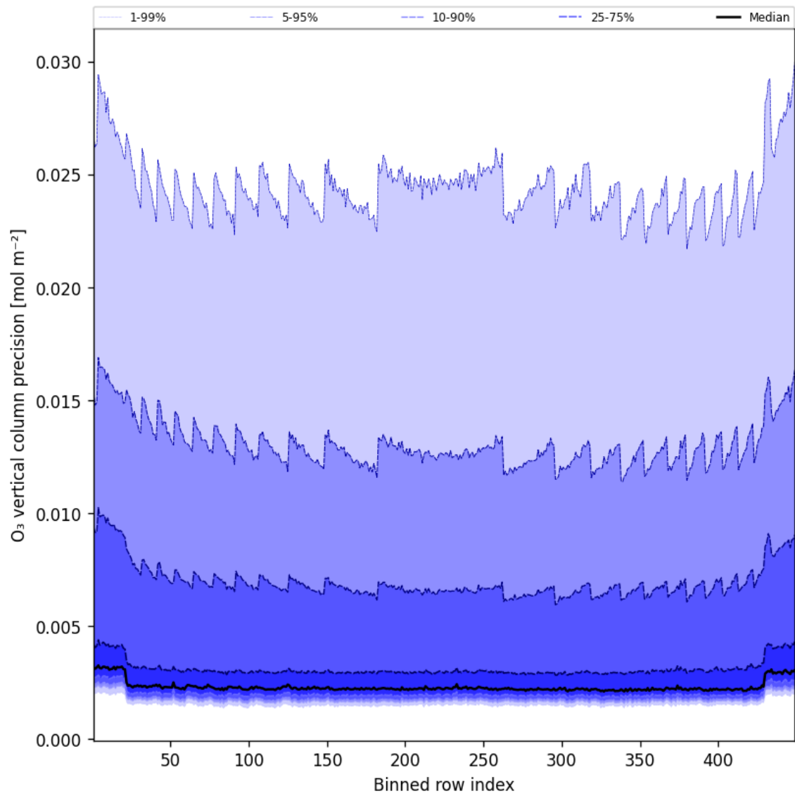
Figure 42: Along track statistics of “O 3 vertical column precision” for 2025-05-21 to 2025-05-22
