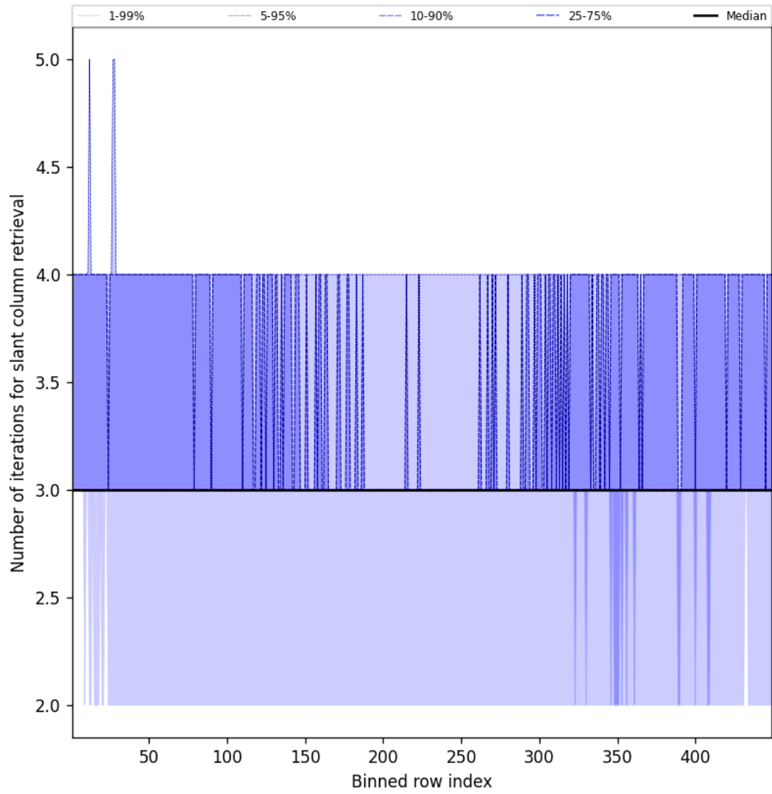
Figure 45: Along track statistics of “Number of iterations for slant column retrieval” for 2025-05-21 to 2025-05-22
