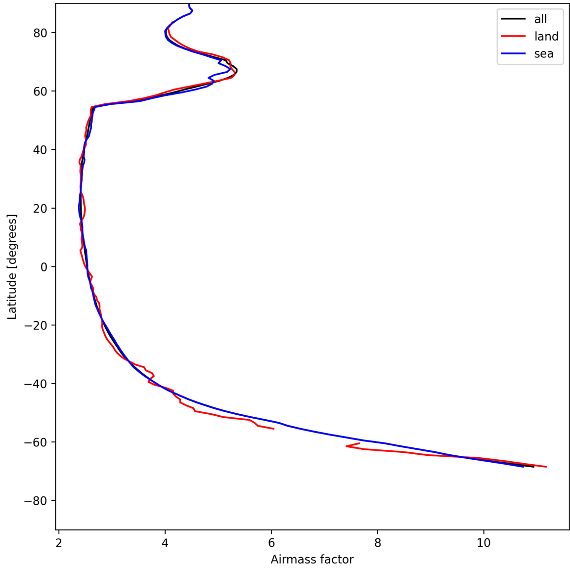
Figure 25: Zonal average of “Airmass factor” for 2025-05-21 to 2025-05-22.
