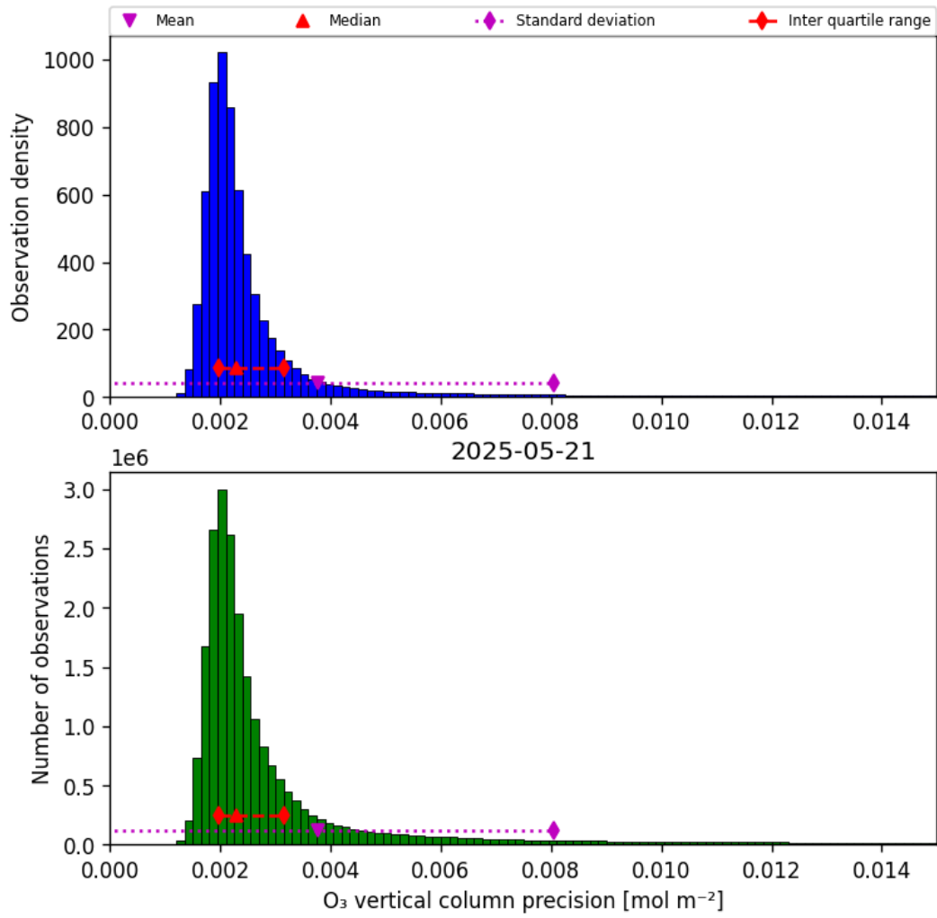
Figure 30: Histogram of “O 3 vertical column precision” for 2025-05-21 to 2025-05-22
