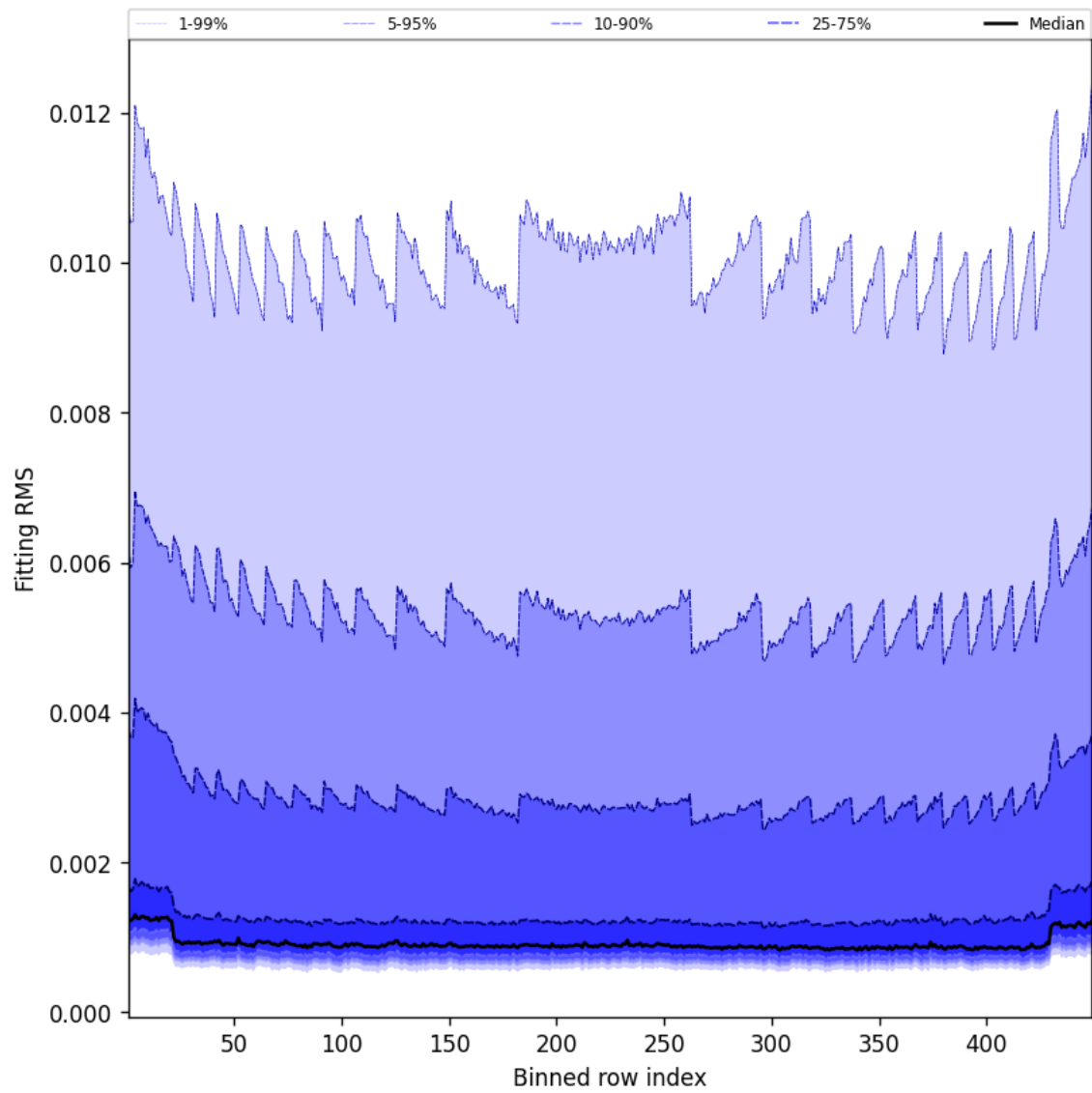
Figure 46: Along track statistics of “Fitting RMS” for 2025-05-21 to 2025-05-22
