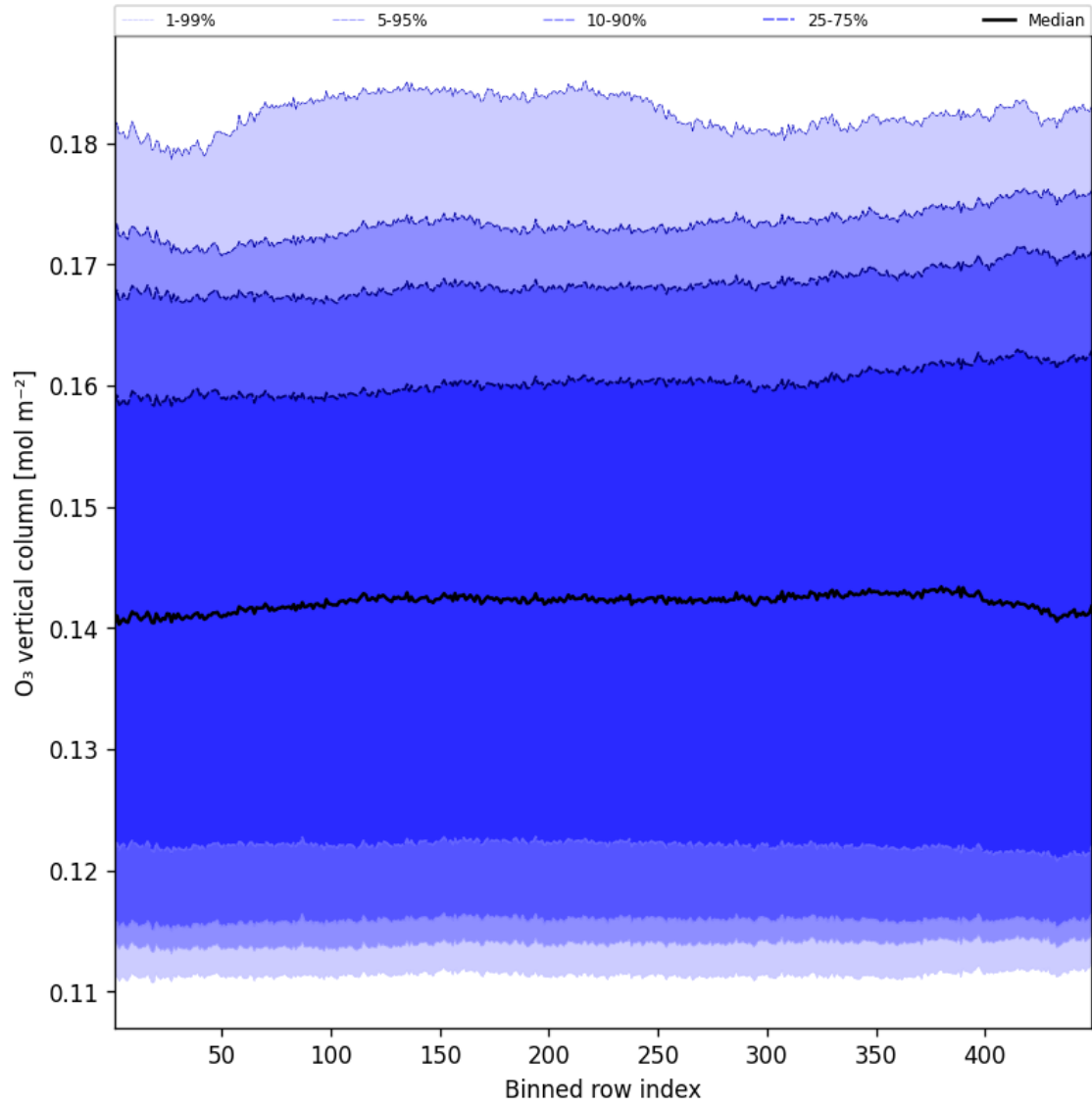
Figure 41: Along track statistics of “O 3 vertical column” for 2025-05-21 to 2025-05-22
