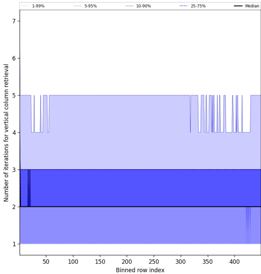
Figure 51: Along track statistics of “Number of iterations for vertical column retrieval” for 2025-05-21 to 2025-05-22
