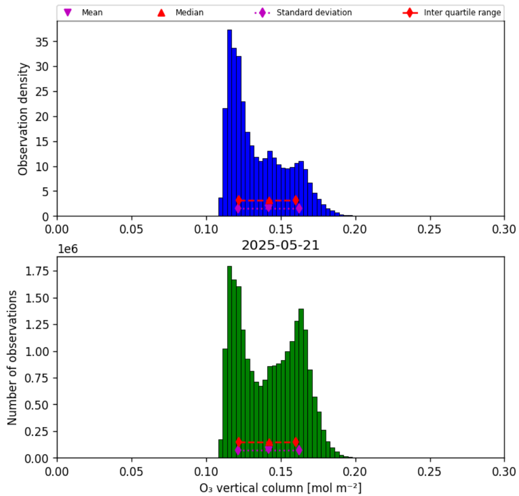
Figure 29: Histogram of “O 3 vertical column” for 2025-05-21 to 2025-05-22
