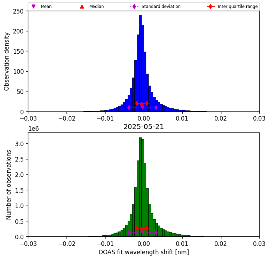
Figure 35: Histogram of “DOAS fit wavelength shift” for 2025-05-21 to 2025-05-22
