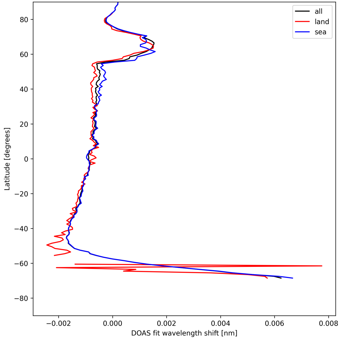
Figure 23: Zonal average of “DOAS fit wavelength shift” for 2025-05-21 to 2025-05-22.
