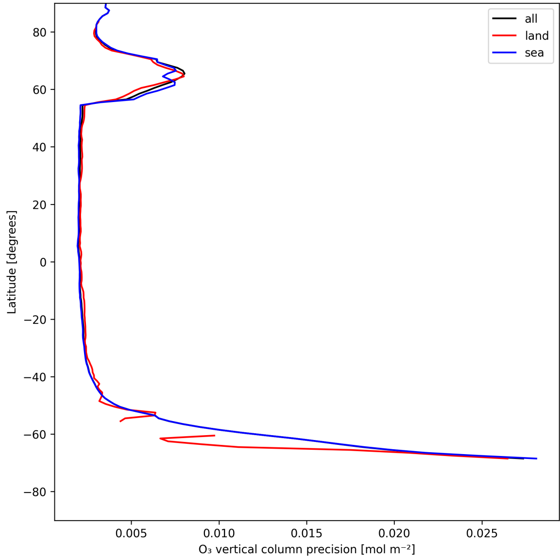
Figure 18: Zonal average of “O 3 vertical column precision” for 2025-05-21 to 2025-05-22.
