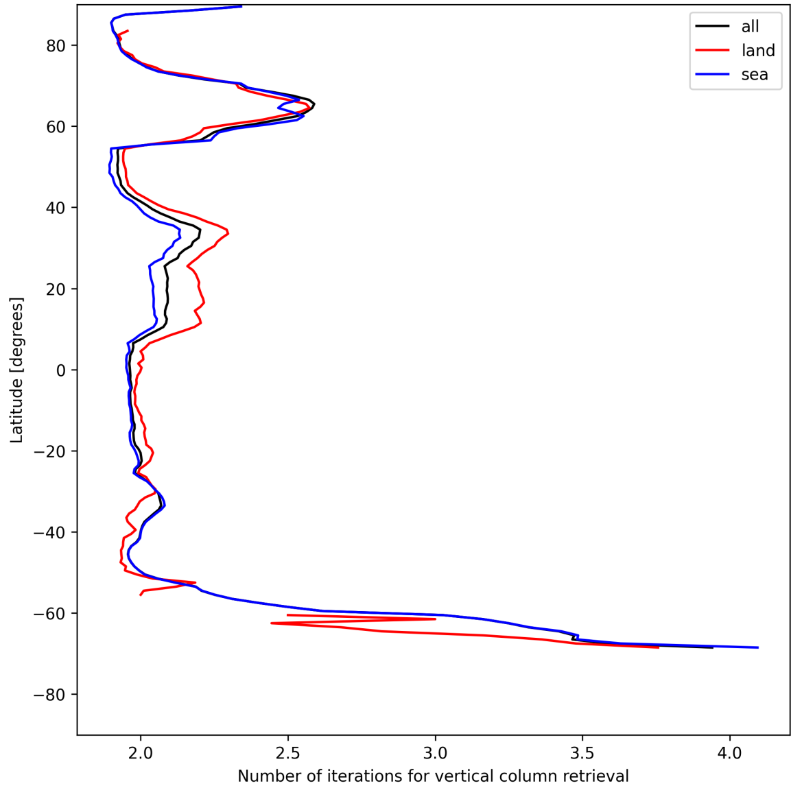
Figure 27: Zonal average of “Number of iterations for vertical column retrieval” for 2025-05-21 to 2025-05-22.
