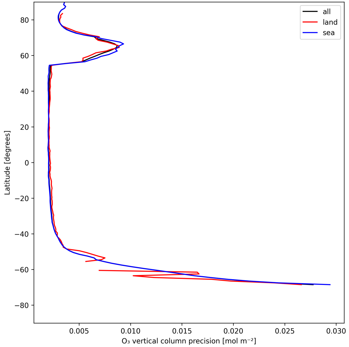
Figure 18: Zonal average of “O 3 vertical column precision” for 2025-05-22 to 2025-05-23.
