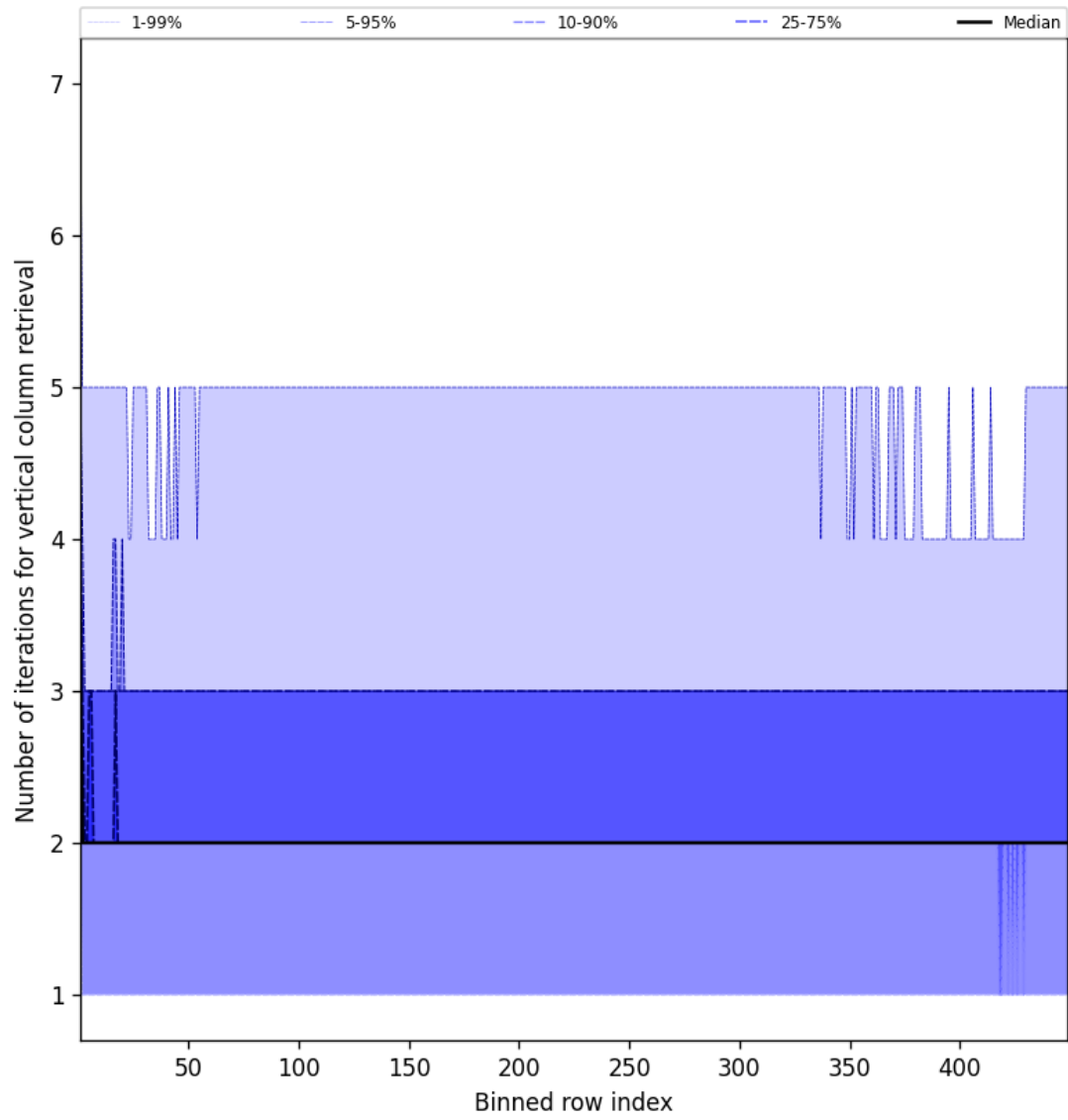
Figure 51: Along track statistics of “Number of iterations for vertical column retrieval” for 2025-05-22 to 2025-05-23
