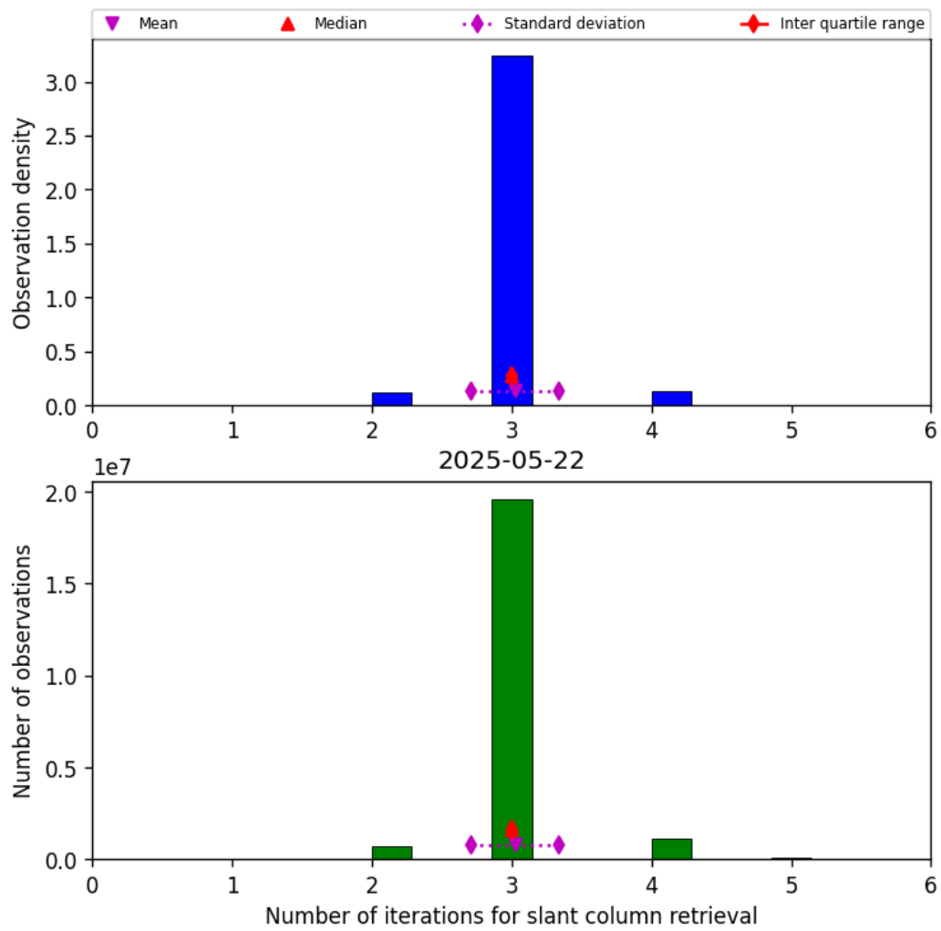
Figure 33: Histogram of “Number of iterations for slant column retrieval” for 2025-05-22 to 2025-05-23
