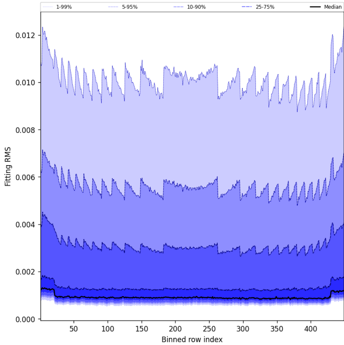
Figure 46: Along track statistics of “Fitting RMS” for 2025-05-22 to 2025-05-23
