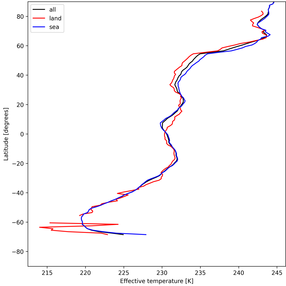
Figure 26: Zonal average of “Effective temperature” for 2025-05-22 to 2025-05-23.
