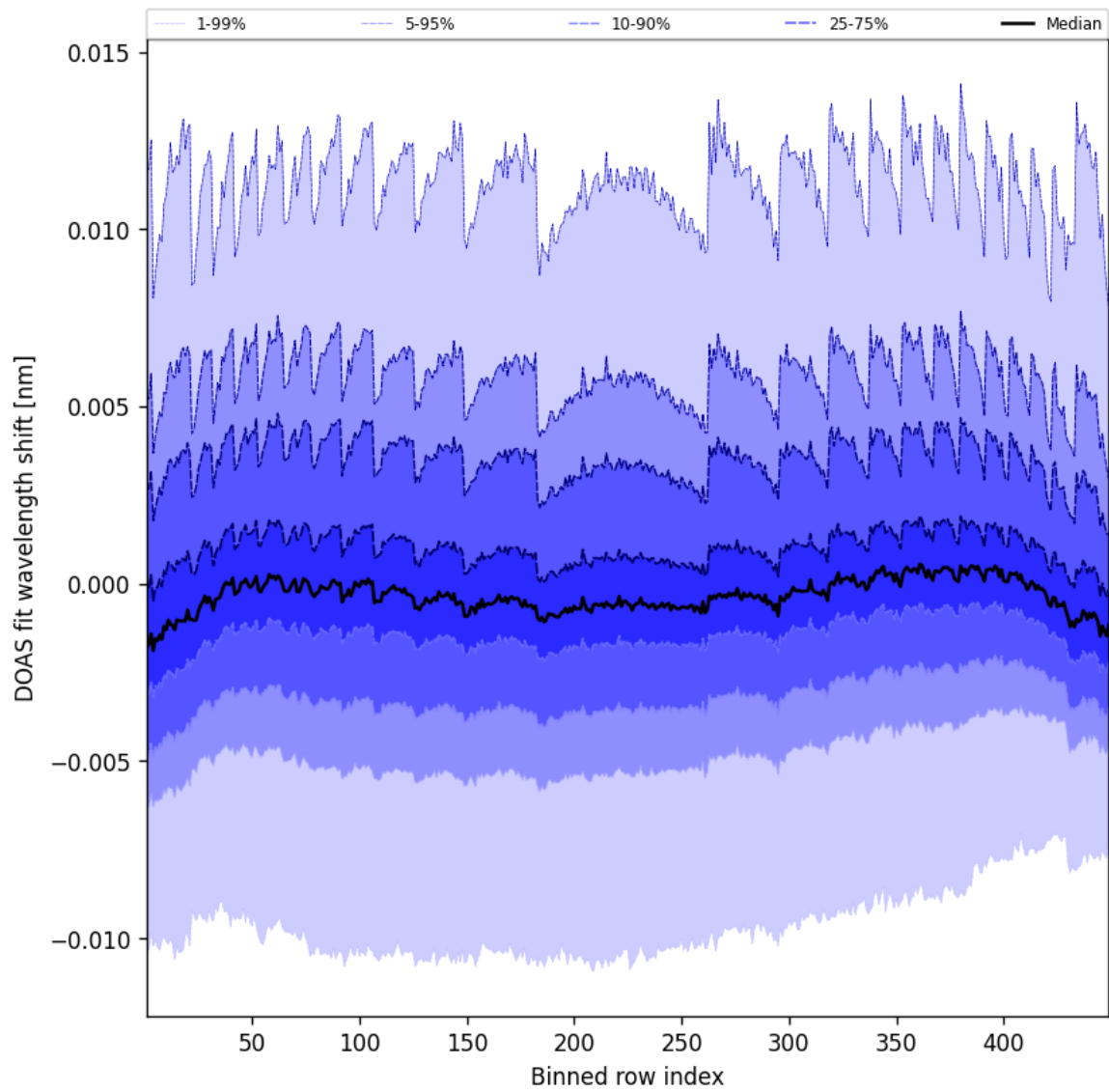
Figure 47: Along track statistics of “DOAS fit wavelength shift” for 2025-05-22 to 2025-05-23
