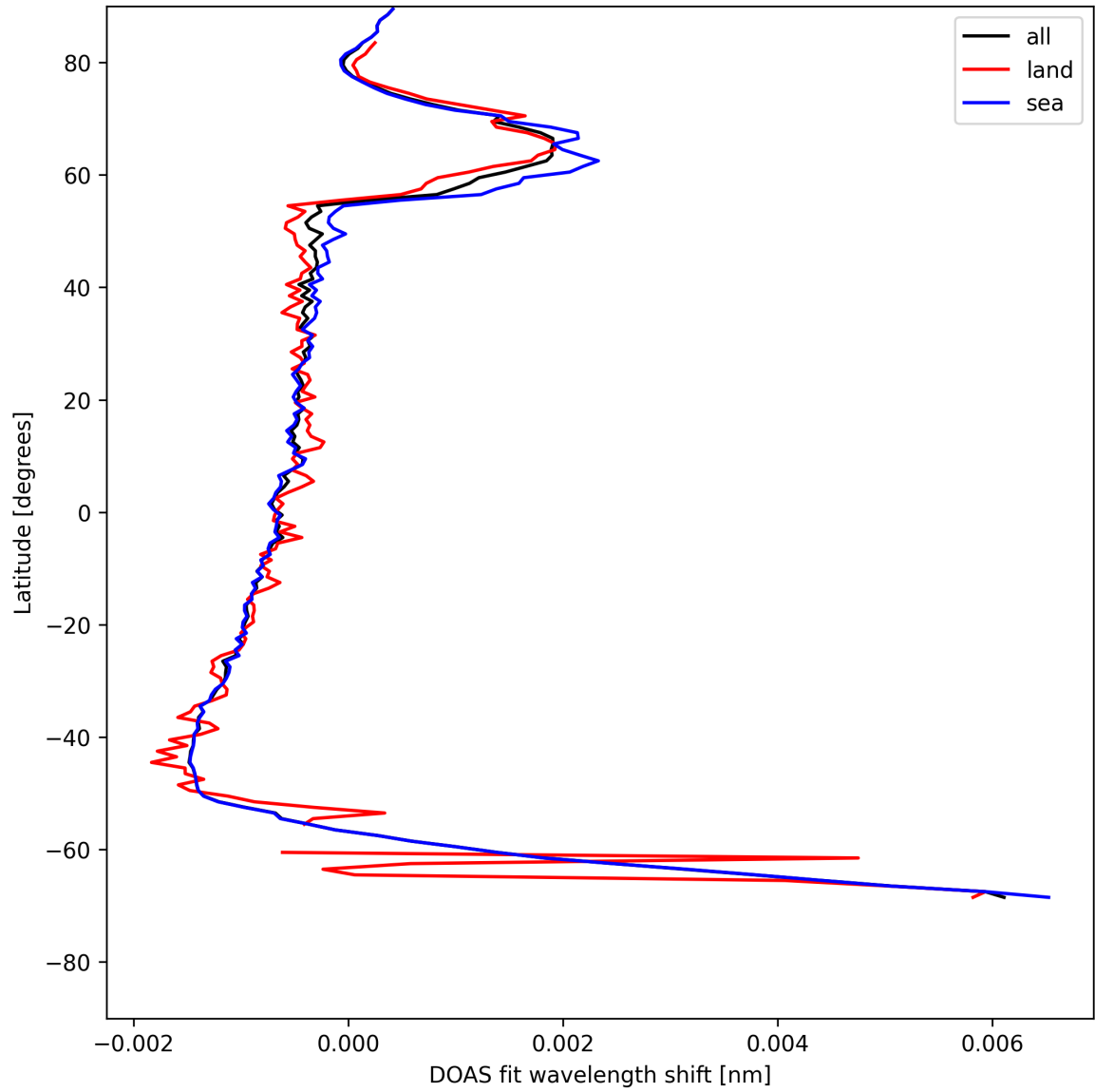
Figure 23: Zonal average of "DOAS fit wavelength shift" for 2025-05-22 to 2025-05-23.
