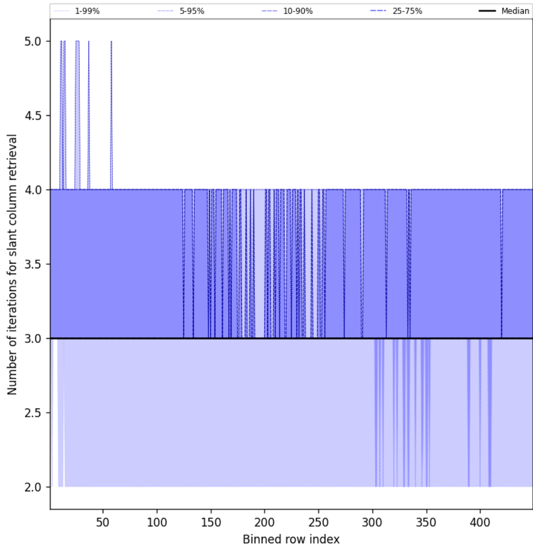
Figure 45: Along track statistics of “Number of iterations for slant column retrieval” for 2025-05-22 to 2025-05-23
