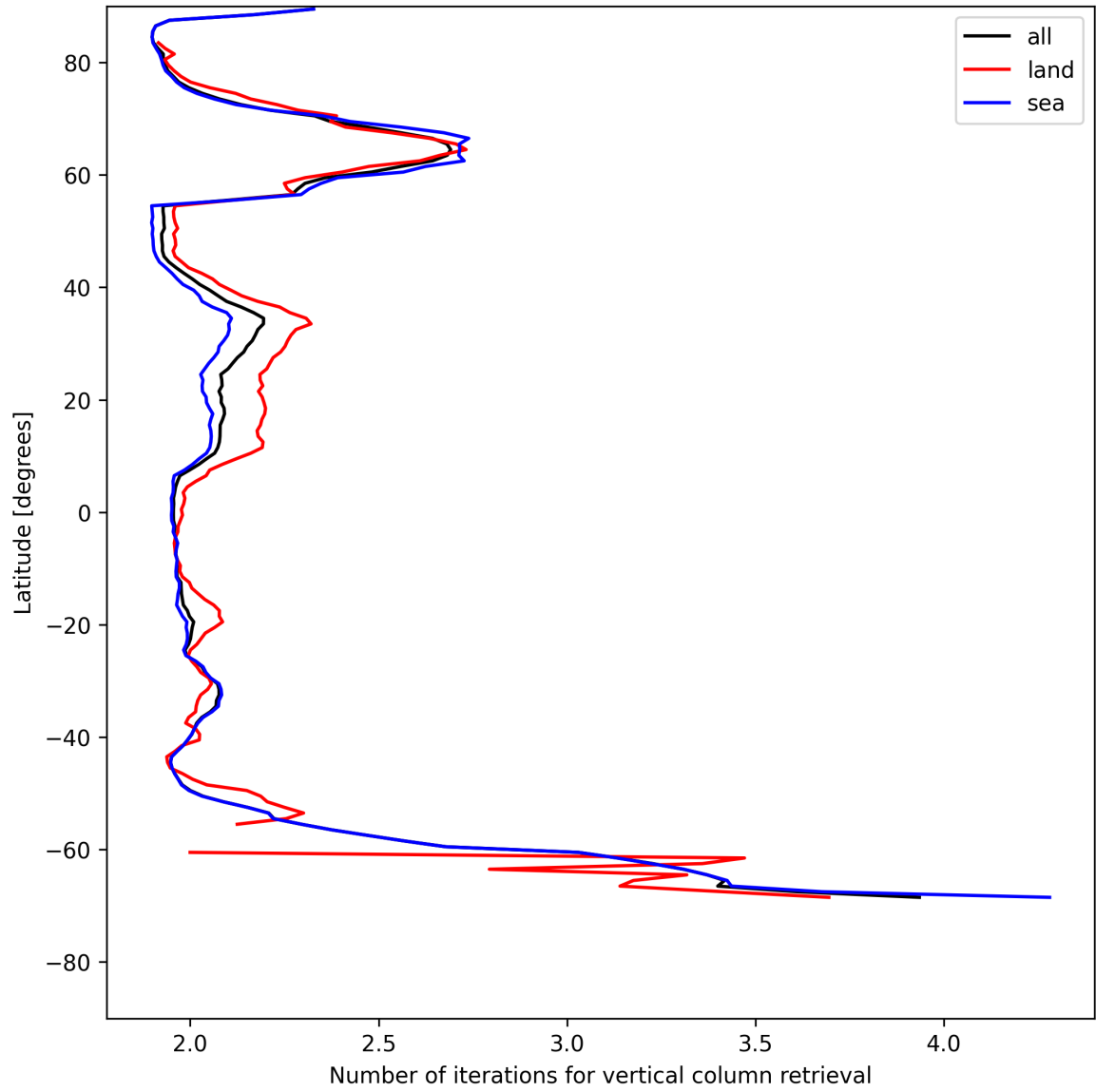
Figure 27: Zonal average of “Number of iterations for vertical column retrieval” for 2025-05-22 to 2025-05-23.
