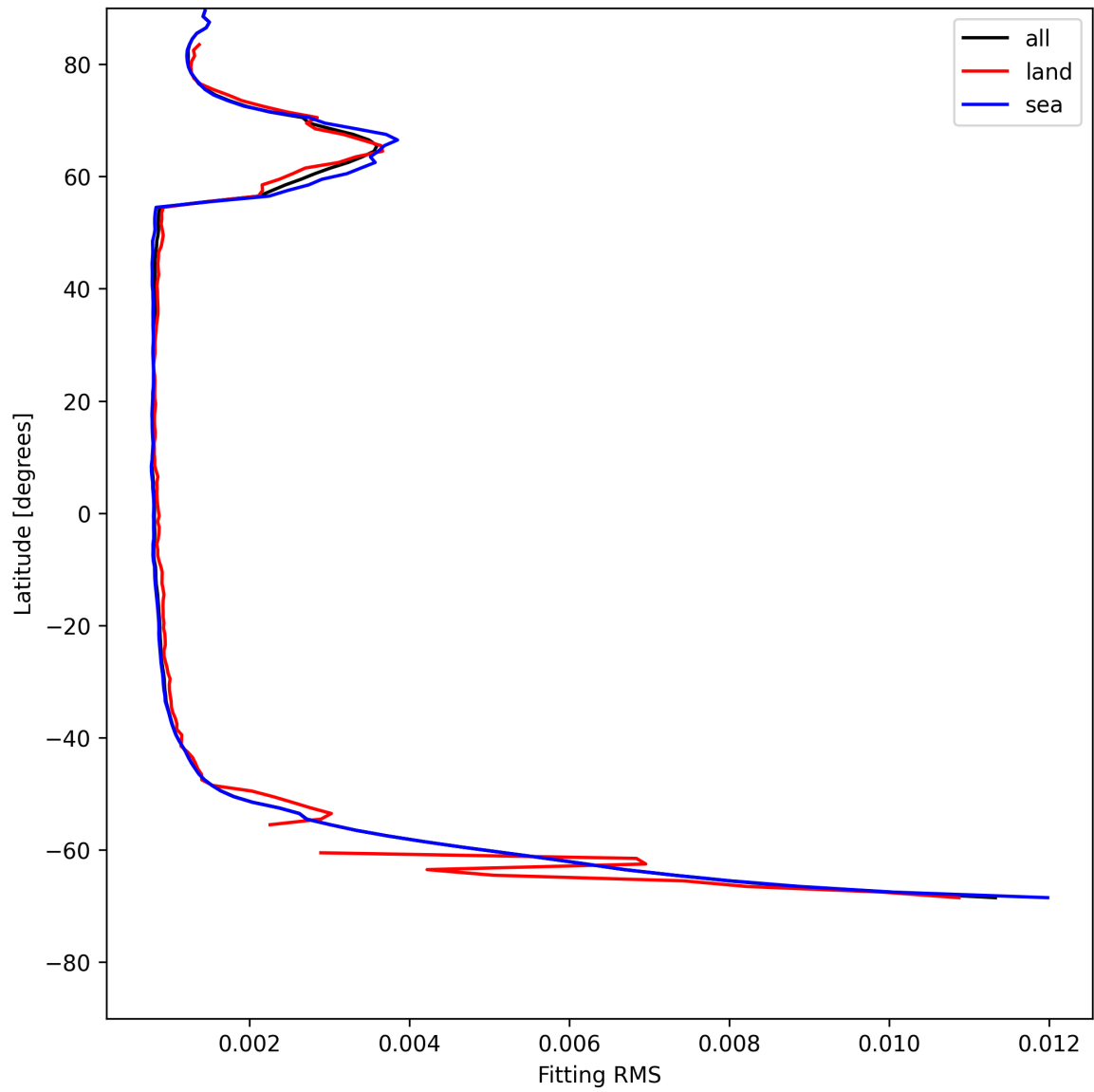
Figure 22: Zonal average of “Fitting RMS” for 2025-05-22 to 2025-05-23.
