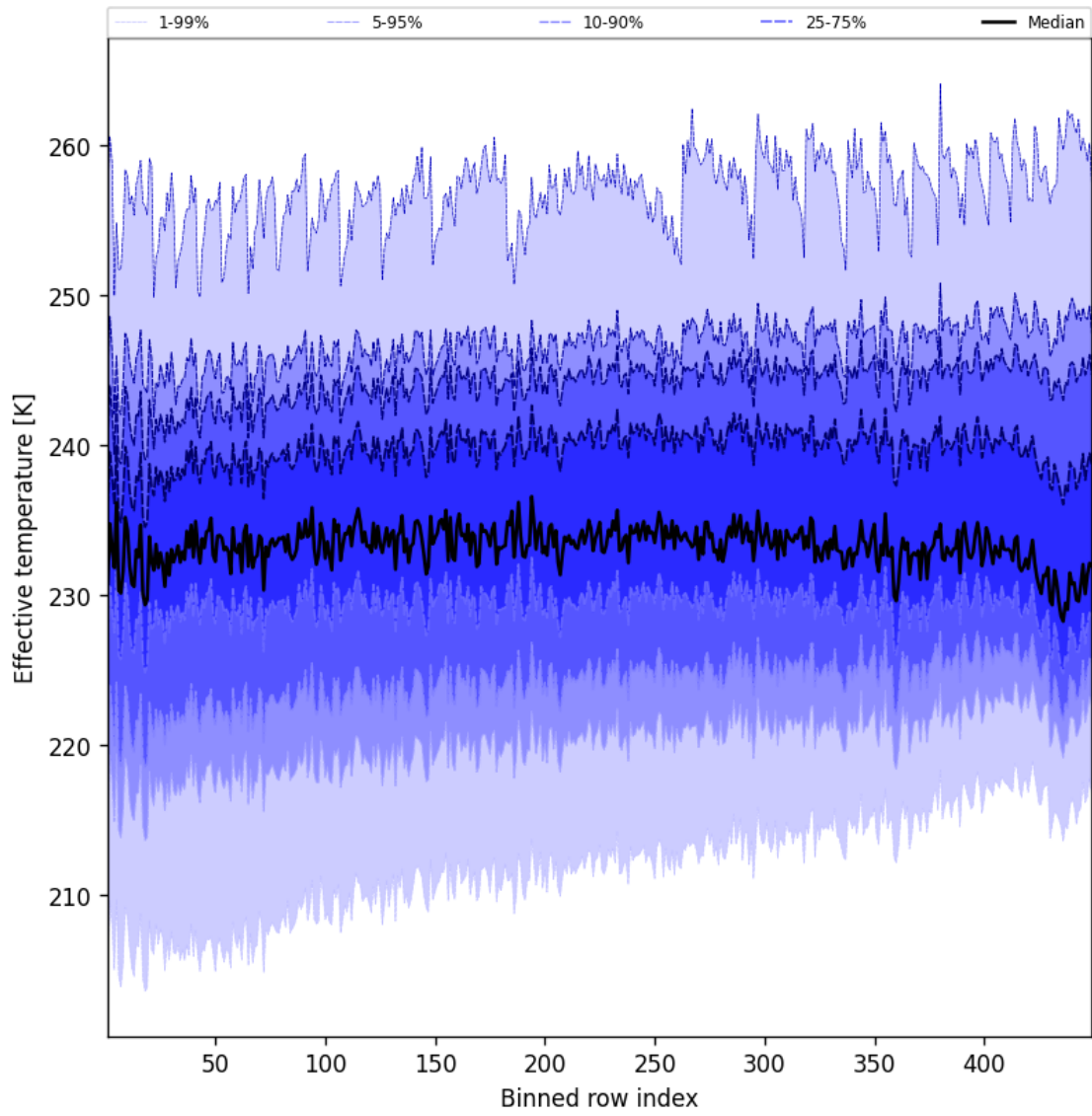
Figure 50: Along track statistics of “Effective temperature” for 2025-05-22 to 2025-05-23
