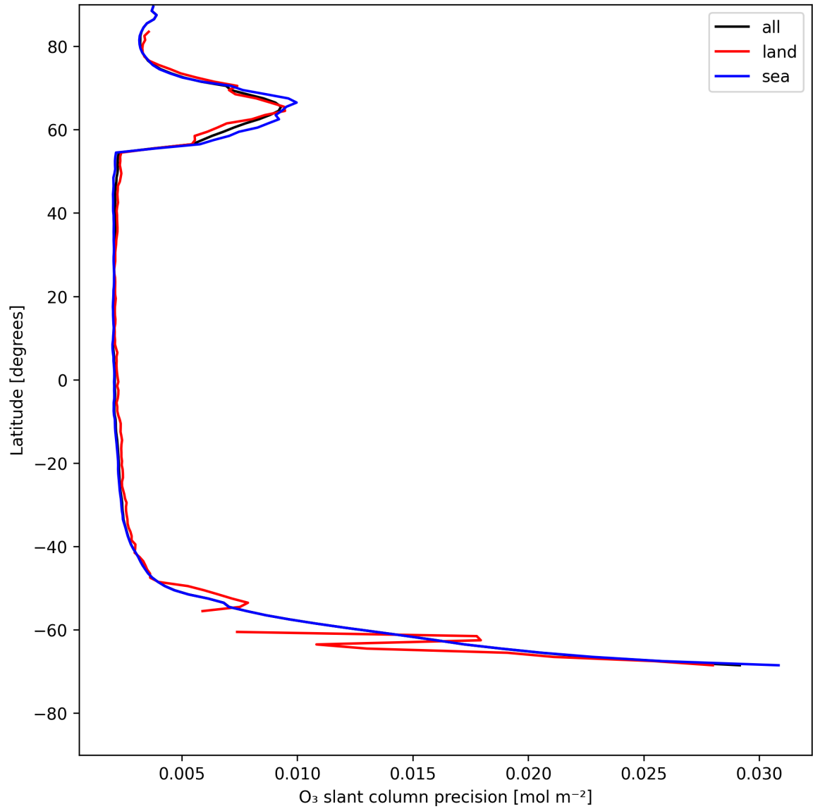
Figure 20: Zonal average of "O 3 slant column precision" for 2025-05-22 to 2025-05-23.
