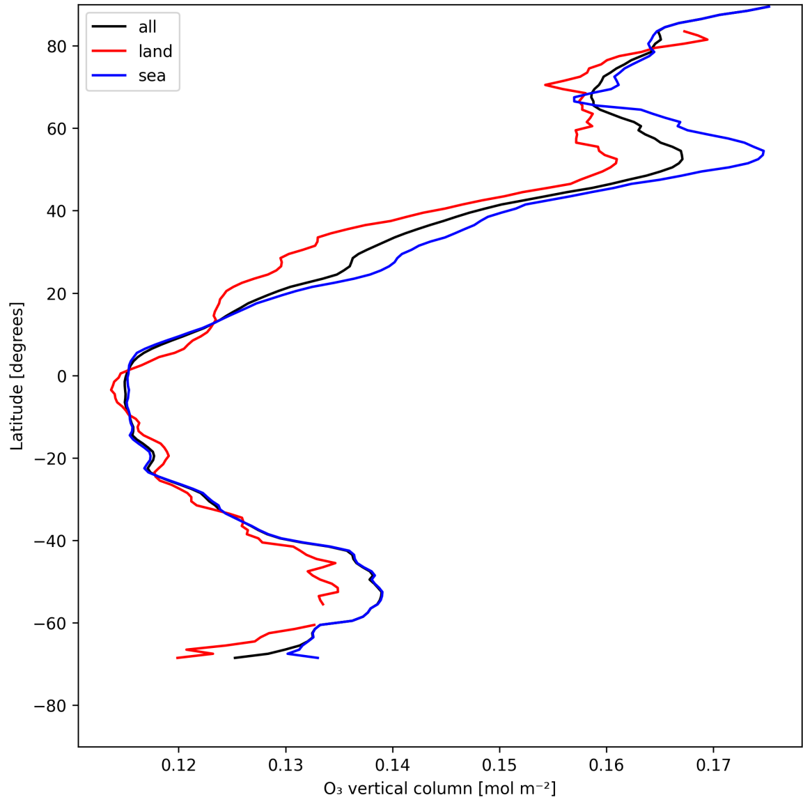
Figure 17: Zonal average of “O 3 vertical column” for 2025-05-22 to 2025-05-23.
