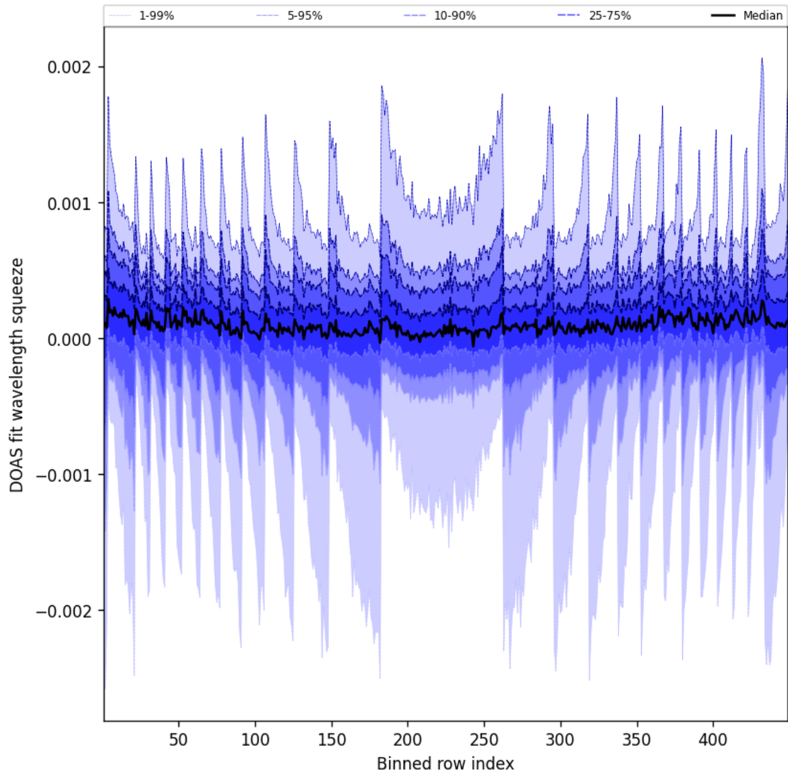
Figure 48: Along track statistics of “DOAS fit wavelength squeeze” for 2025-05-22 to 2025-05-23
