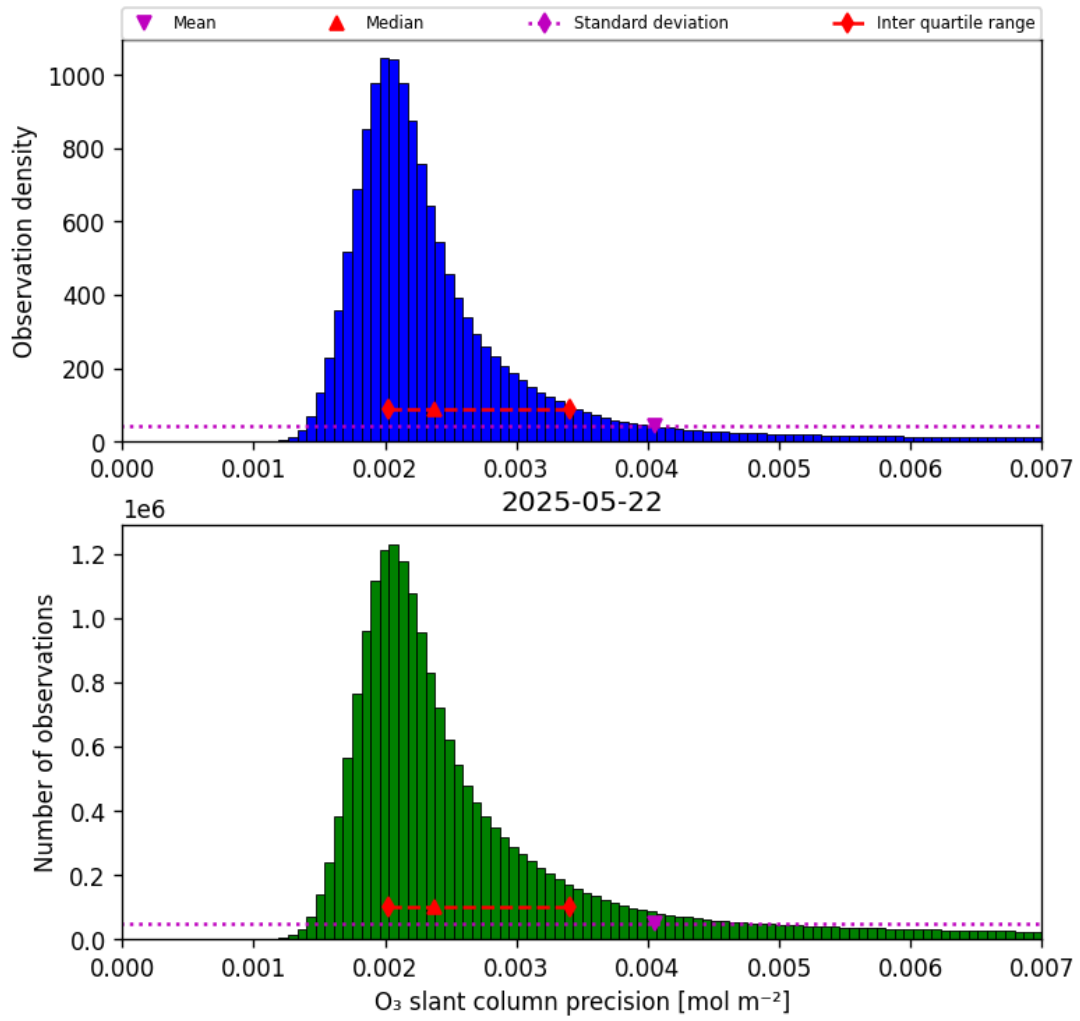
Figure 32: Histogram of “O 3 slant column precision” for 2025-05-22 to 2025-05-23
