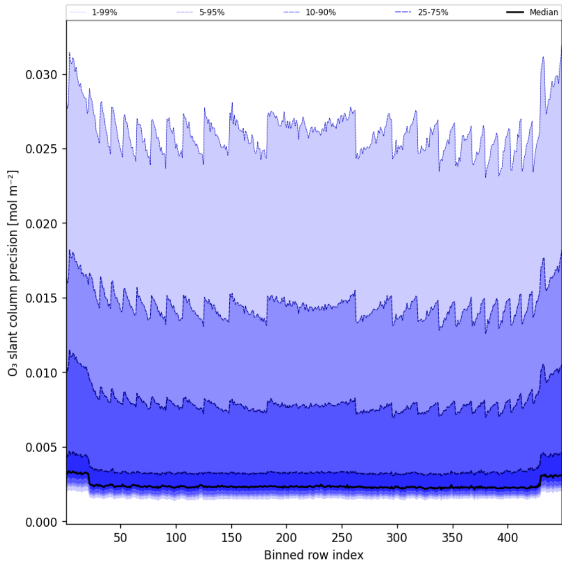
Figure 44: Along track statistics of “O 3 slant column precision” for 2025-05-22 to 2025-05-23
