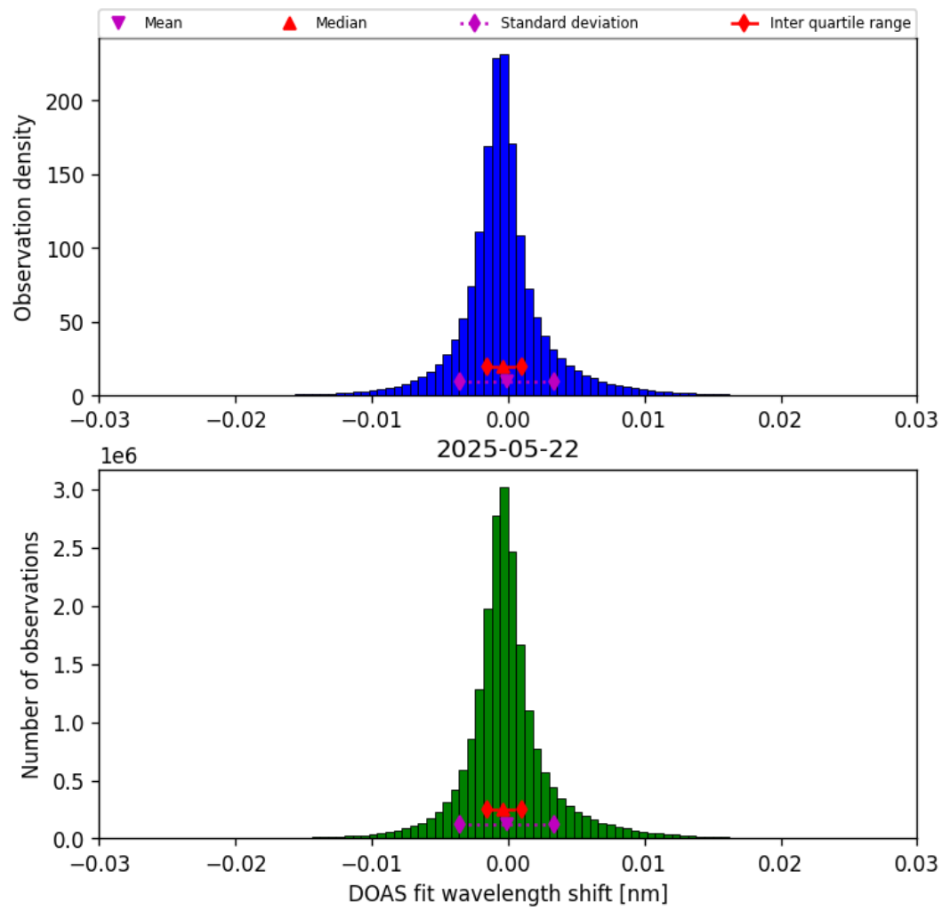
Figure 35: Histogram of “DOAS fit wavelength shift” for 2025-05-22 to 2025-05-23
