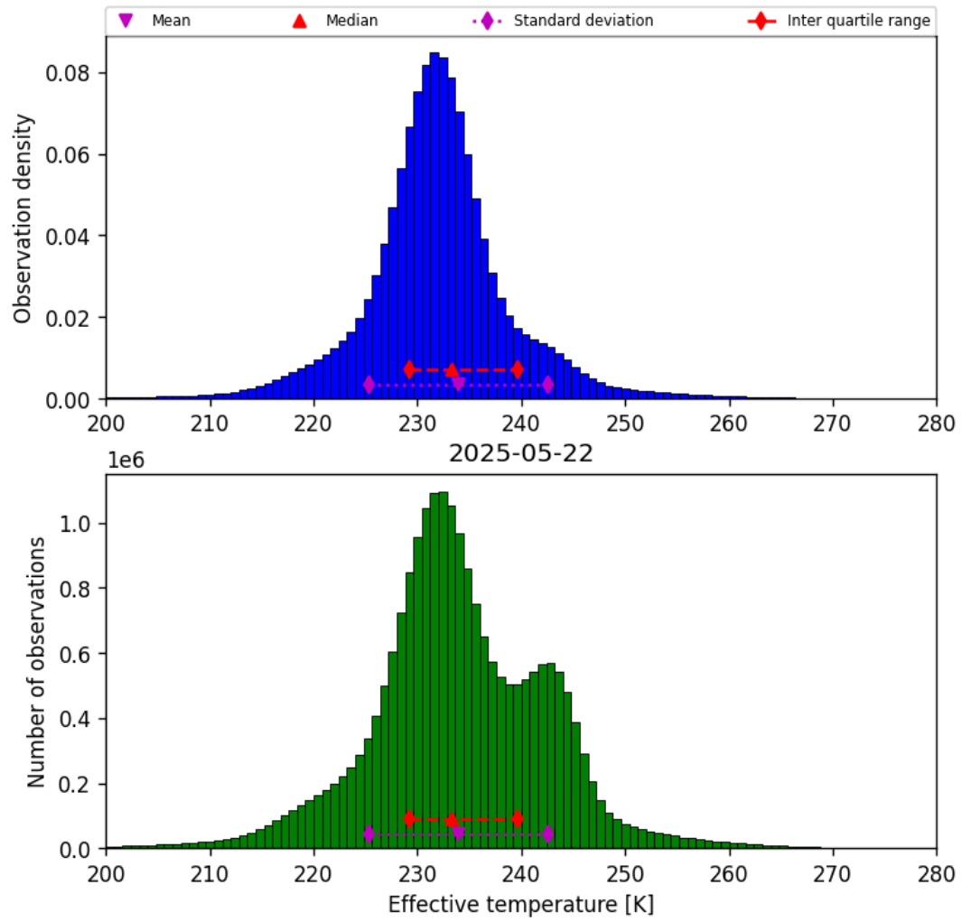
Figure 38: Histogram of “Effective temperature” for 2025-05-22 to 2025-05-23
