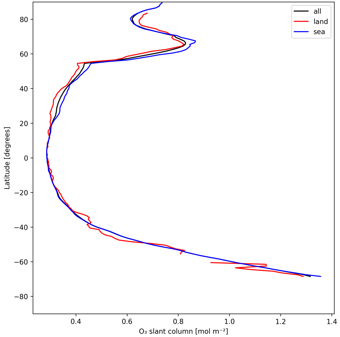
Figure 19: Zonal average of “O 3 slant column” for 2025-05-22 to 2025-05-23.
