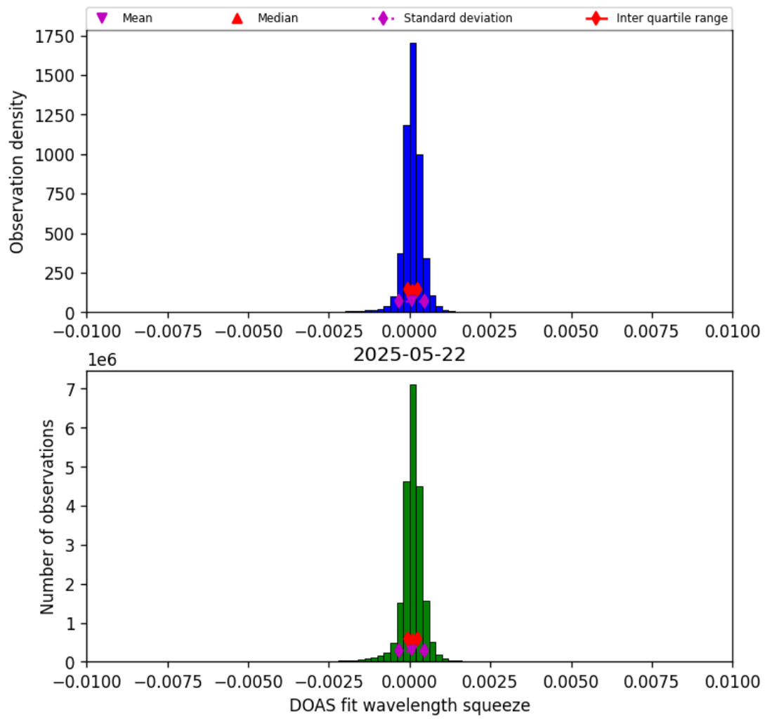
Figure 36: Histogram of “DOAS fit wavelength squeeze” for 2025-05-22 to 2025-05-23
