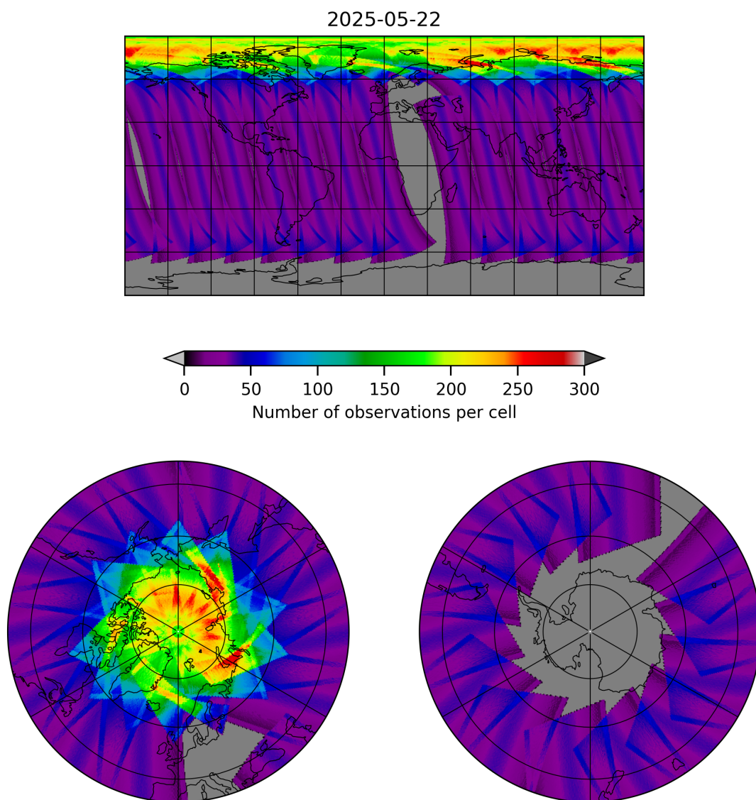
Figure 15: Map of the number of observations for 2025-05-22 to 2025-05-23
