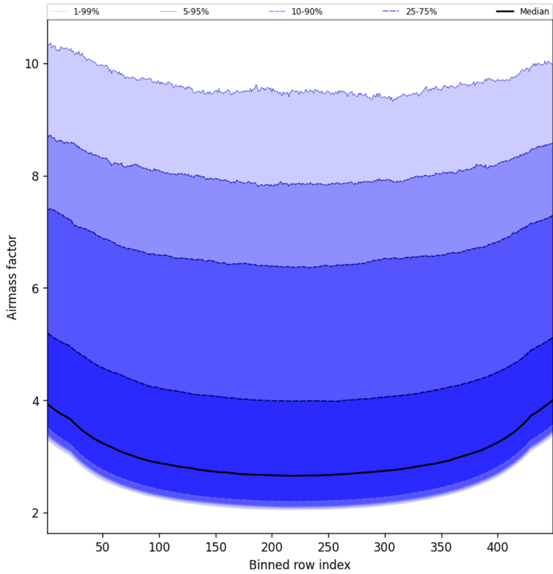
Figure 49: Along track statistics of “Airmass factor” for 2025-05-22 to 2025-05-23
