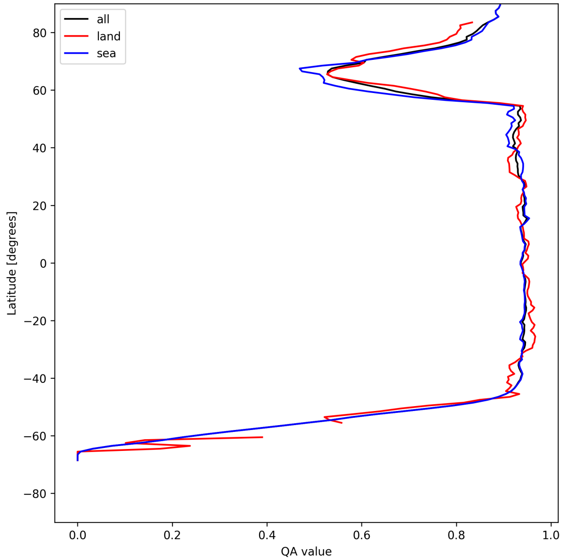
Figure 16: Zonal average of “QA value” for 2025-05-22 to 2025-05-23.
