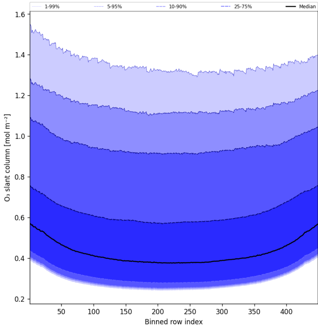
Figure 43: Along track statistics of “O 3 slant column” for 2025-05-22 to 2025-05-23
