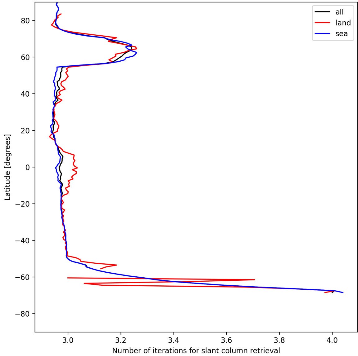
Figure 21: Zonal average of “Number of iterations for slant column retrieval” for 2025-05-22 to 2025-05-23.
