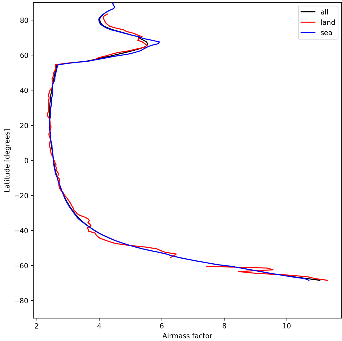
Figure 25: Zonal average of “Airmass factor” for 2025-05-22 to 2025-05-23.
