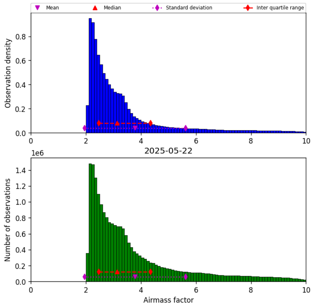
Figure 37: Histogram of “Airmass factor” for 2025-05-22 to 2025-05-23
