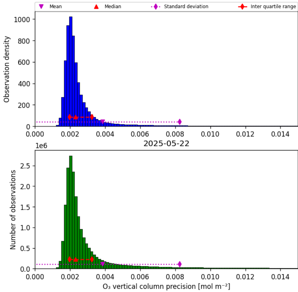
Figure 30: Histogram of “O 3 vertical column precision” for 2025-05-22 to 2025-05-23
