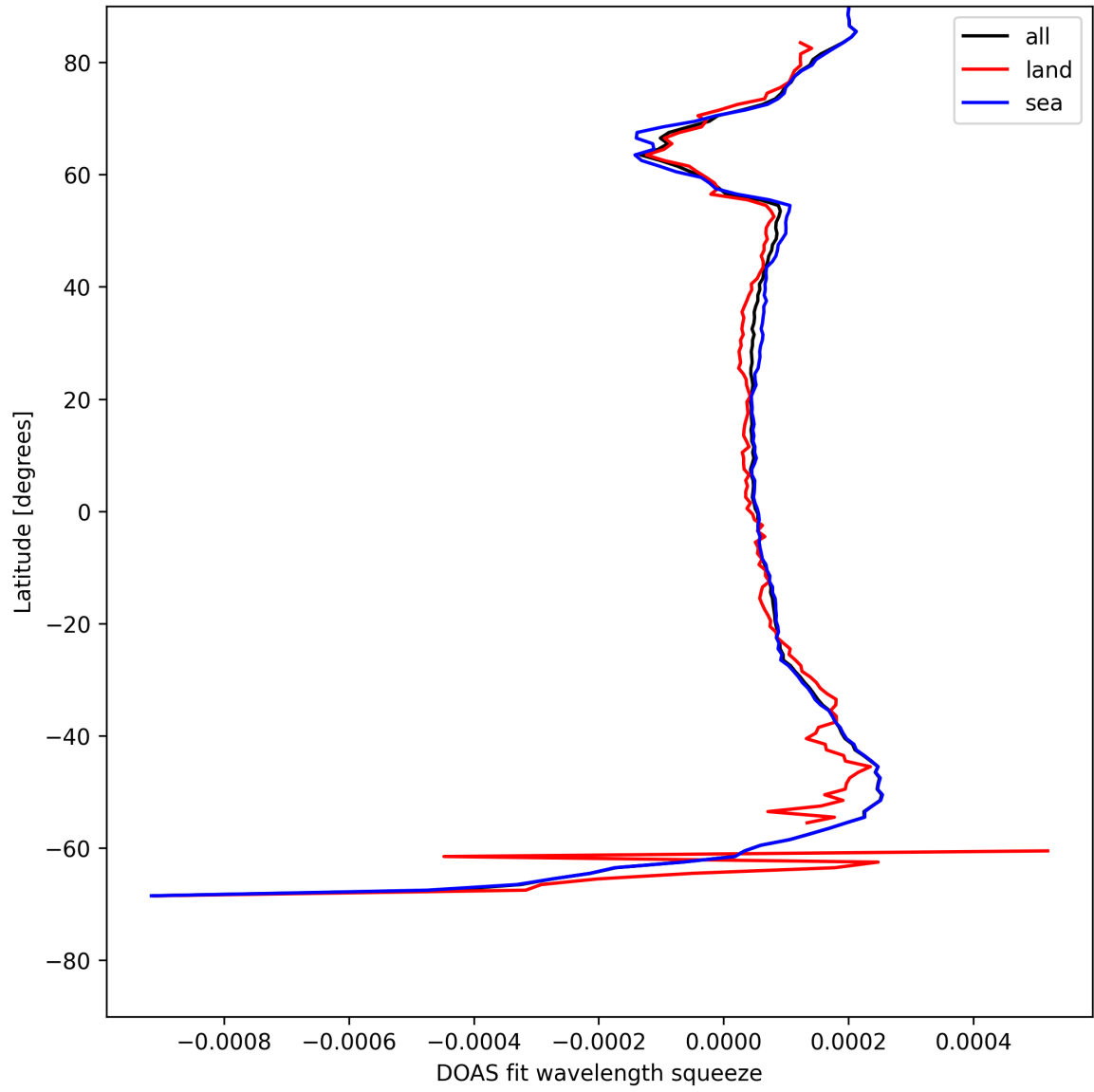
Figure 24: Zonal average of “DOAS fit wavelength squeeze” for 2025-05-22 to 2025-05-23.
