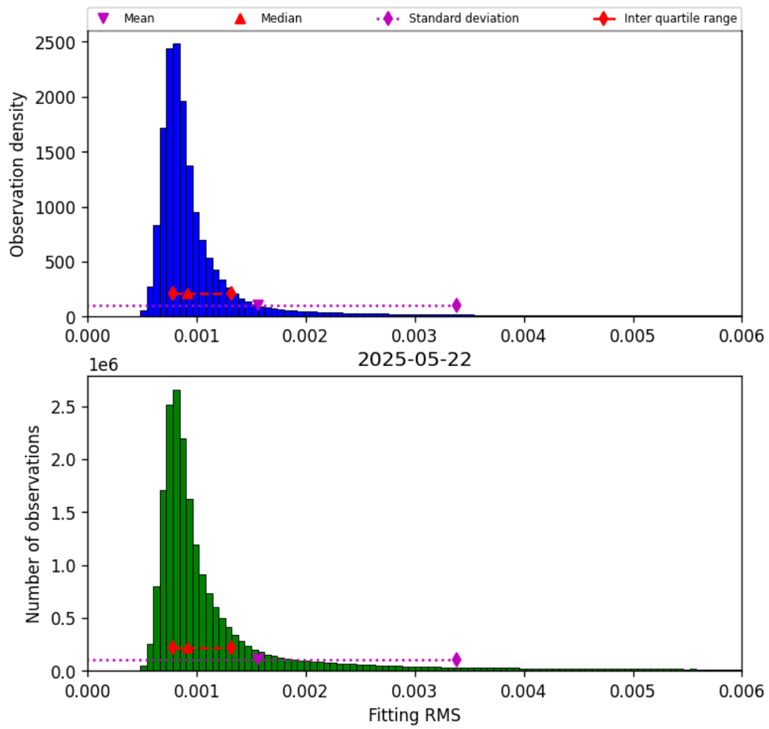
Figure 34: Histogram of “Fitting RMS” for 2025-05-22 to 2025-05-23
