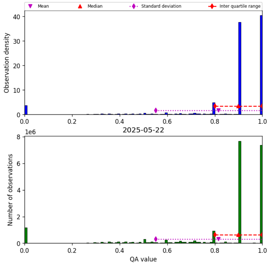
Figure 28: Histogram of “QA value” for 2025-05-22 to 2025-05-23
