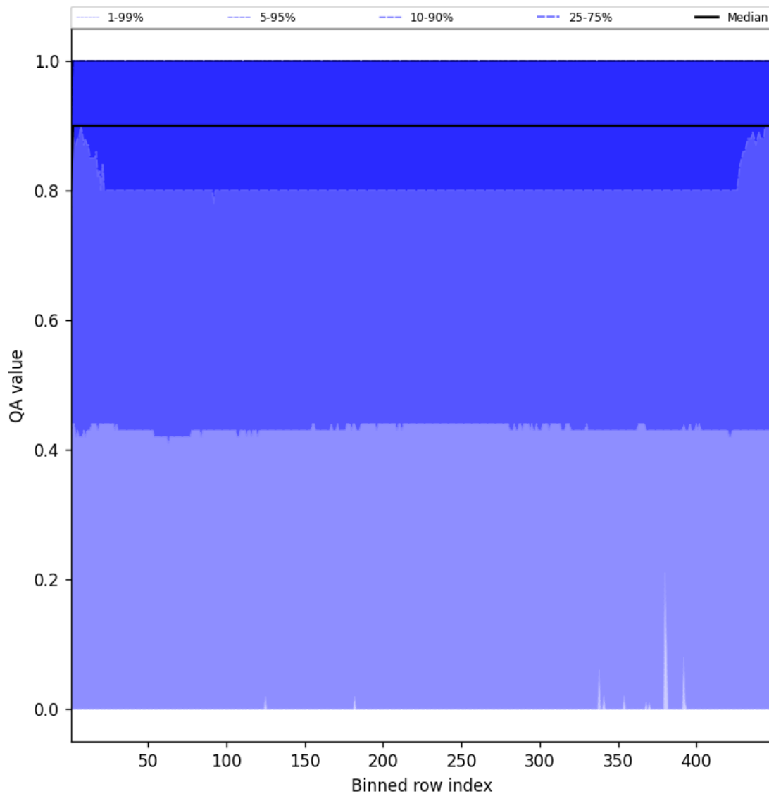
Figure 40: Along track statistics of “QA value” for 2025-05-22 to 2025-05-23
