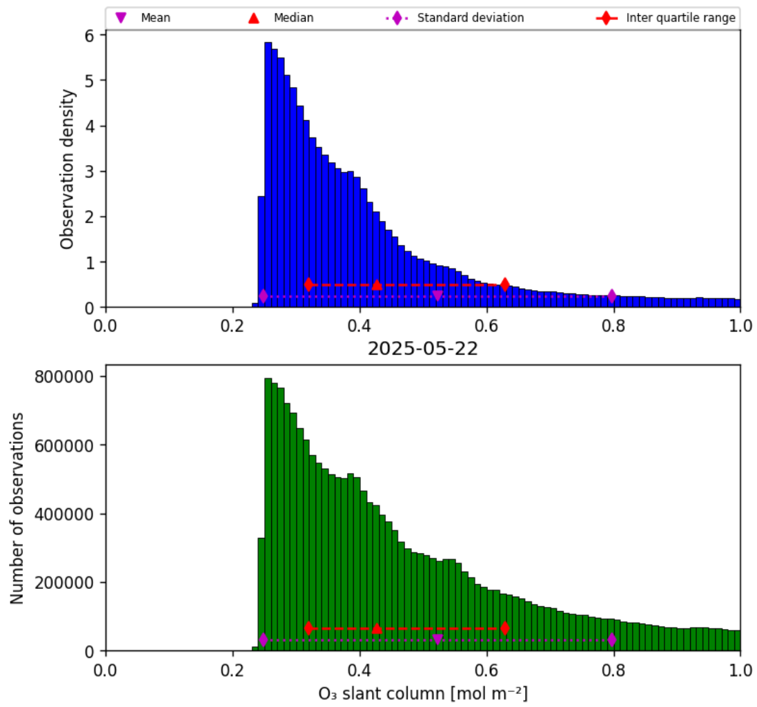
Figure 31: Histogram of “O 3 slant column” for 2025-05-22 to 2025-05-23
