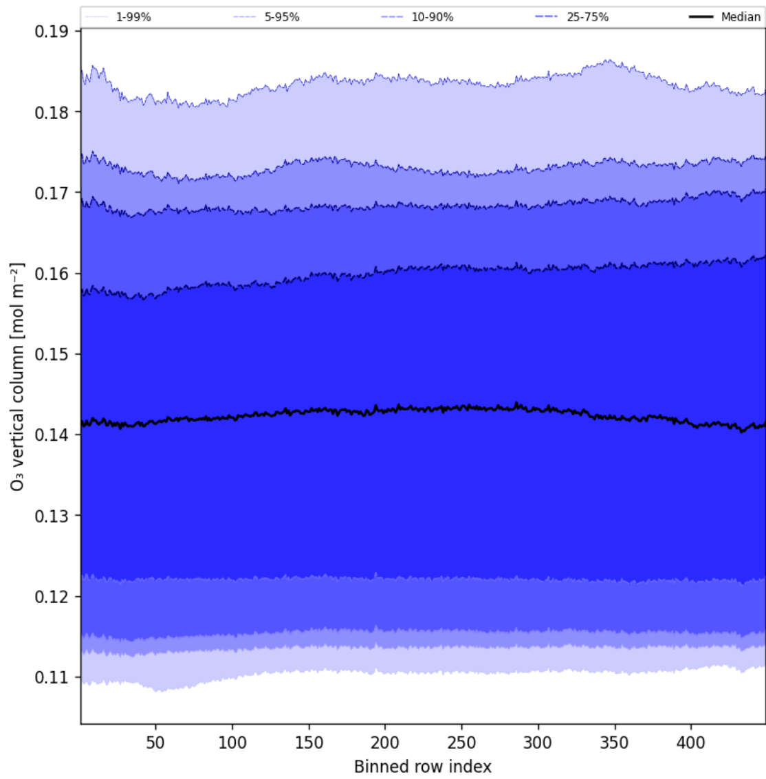
Figure 41: Along track statistics of “O 3 vertical column” for 2025-05-22 to 2025-05-23
