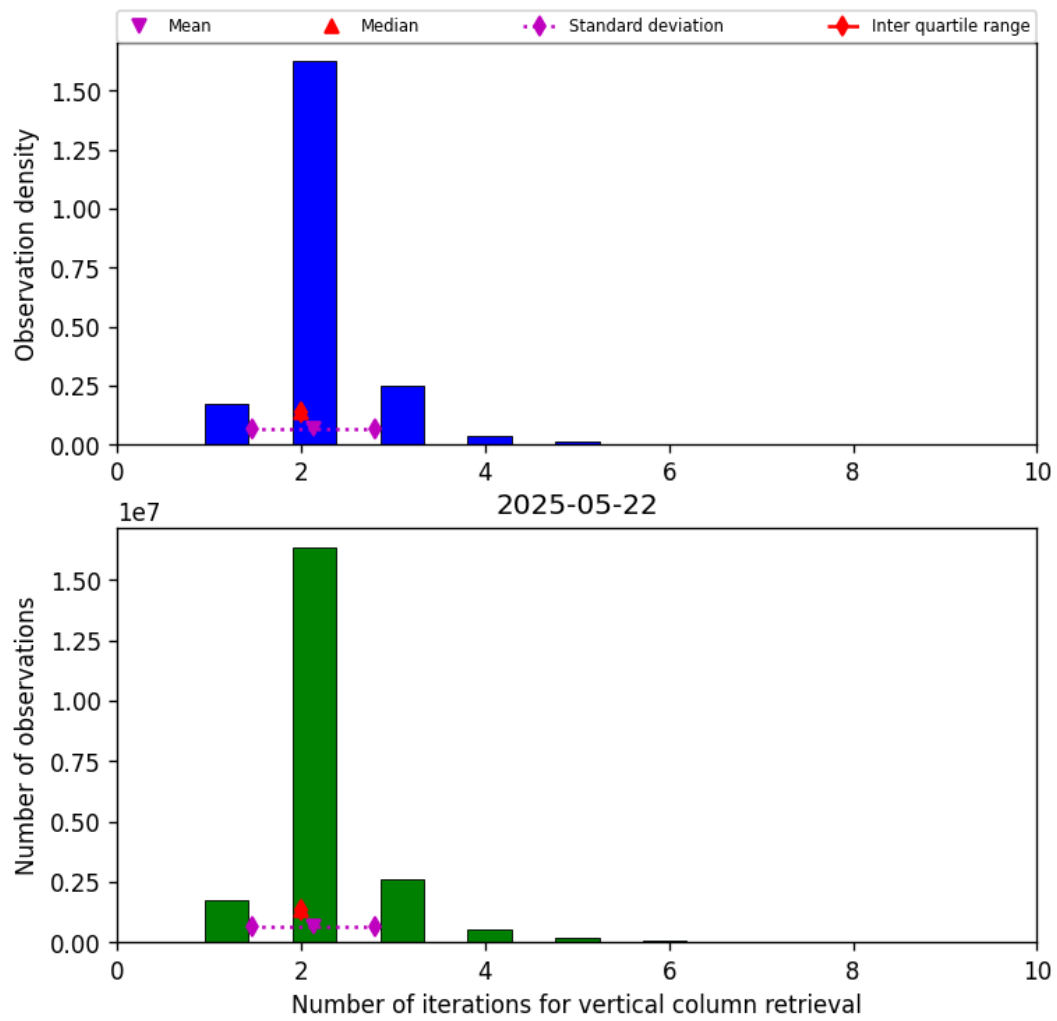
Figure 39: Histogram of “Number of iterations for vertical column retrieval” for 2025-05-22 to 2025-05-23
