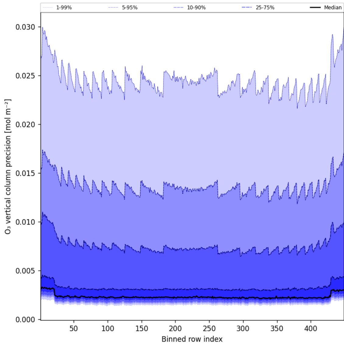
Figure 42: Along track statistics of “O 3 vertical column precision” for 2025-05-22 to 2025-05-23
