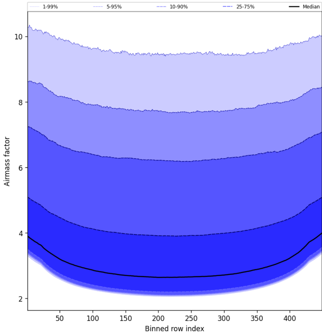
Figure 49: Along track statistics of “Airmass factor” for 2025-05-23 to 2025-05-24
