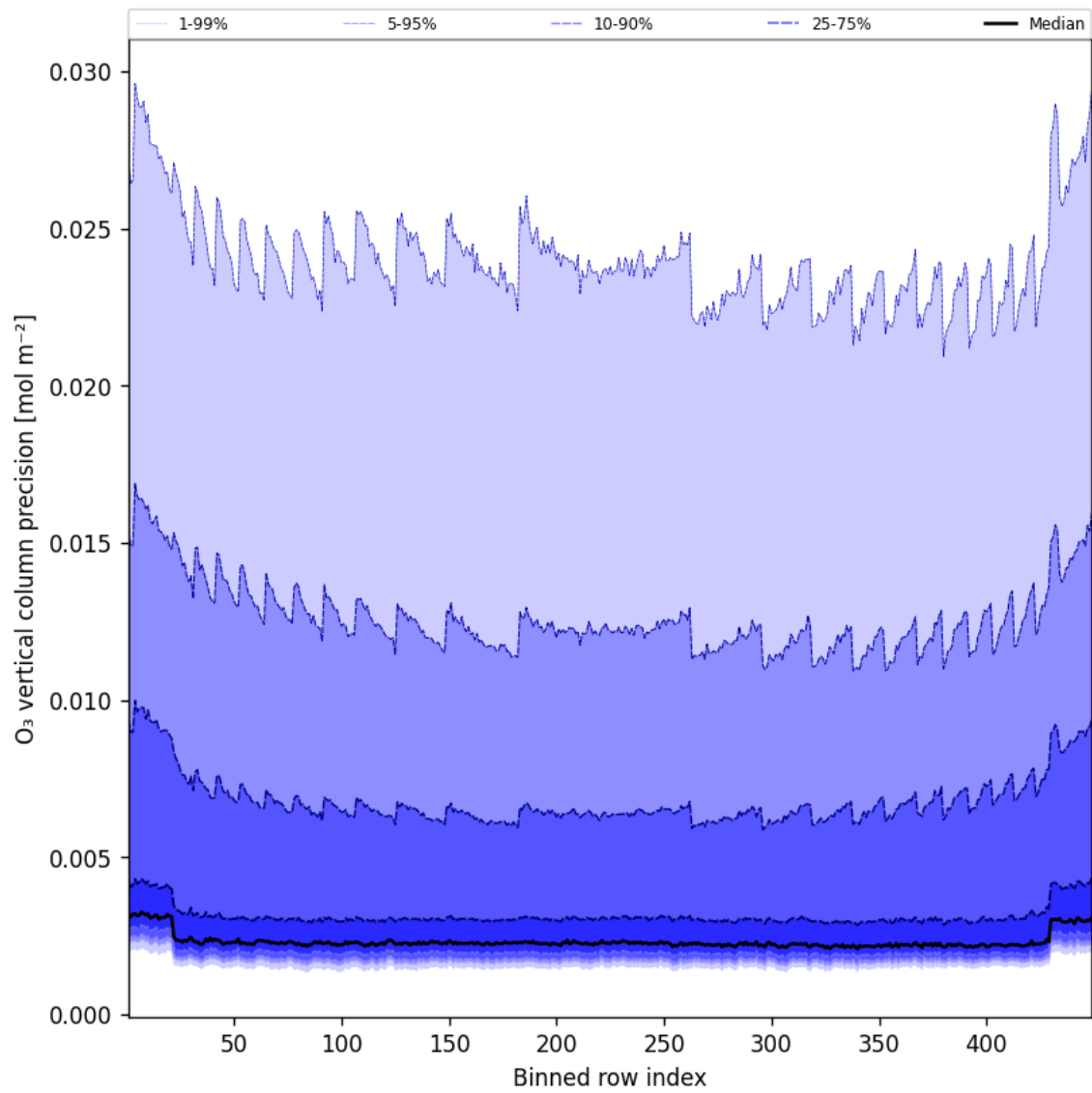
Figure 42: Along track statistics of “O 3 vertical column precision” for 2025-05-23 to 2025-05-24
