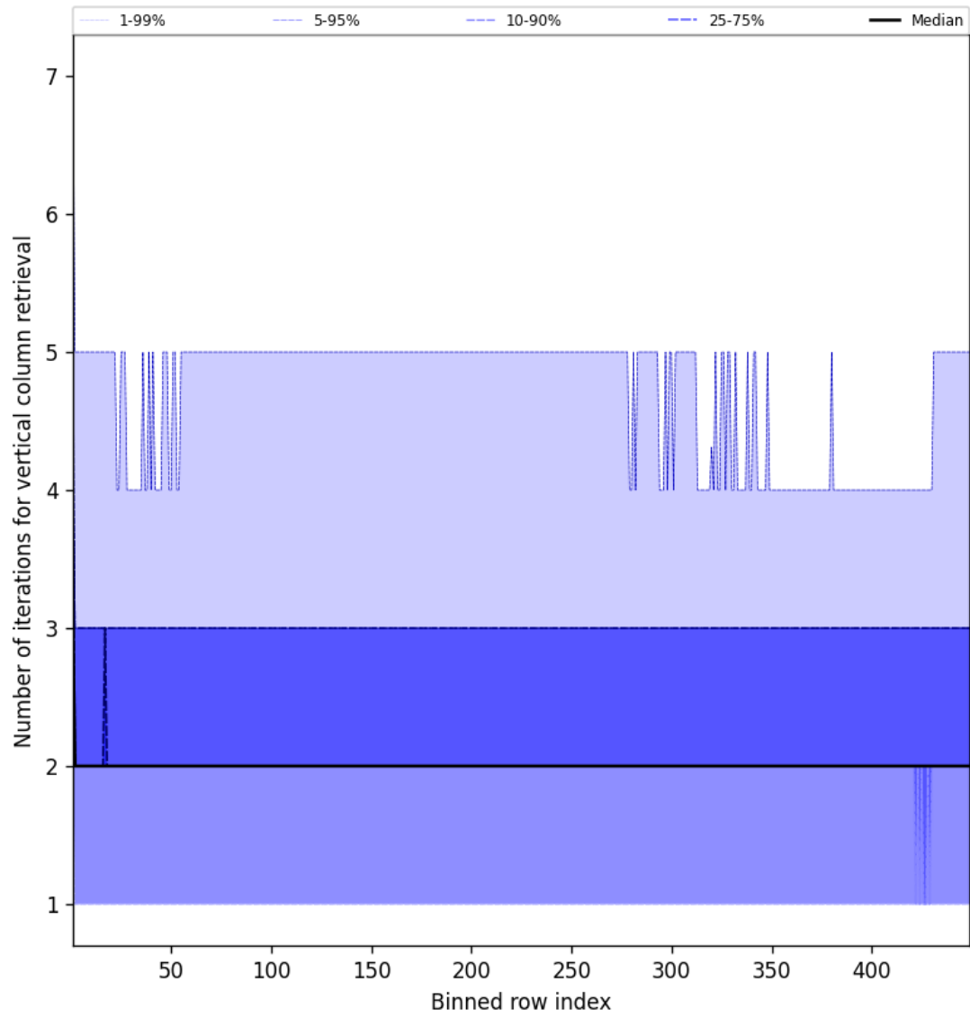
Figure 51: Along track statistics of “Number of iterations for vertical column retrieval” for 2025-05-23 to 2025-05-24
