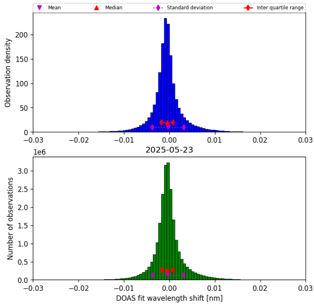
Figure 35: Histogram of “DOAS fit wavelength shift” for 2025-05-23 to 2025-05-24
