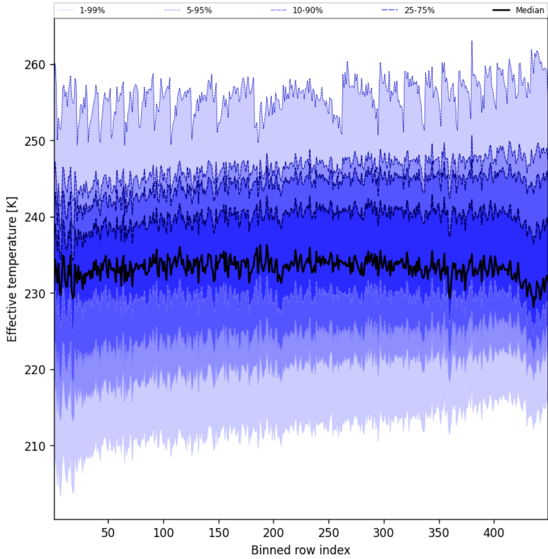
Figure 50: Along track statistics of “Effective temperature” for 2025-05-23 to 2025-05-24
