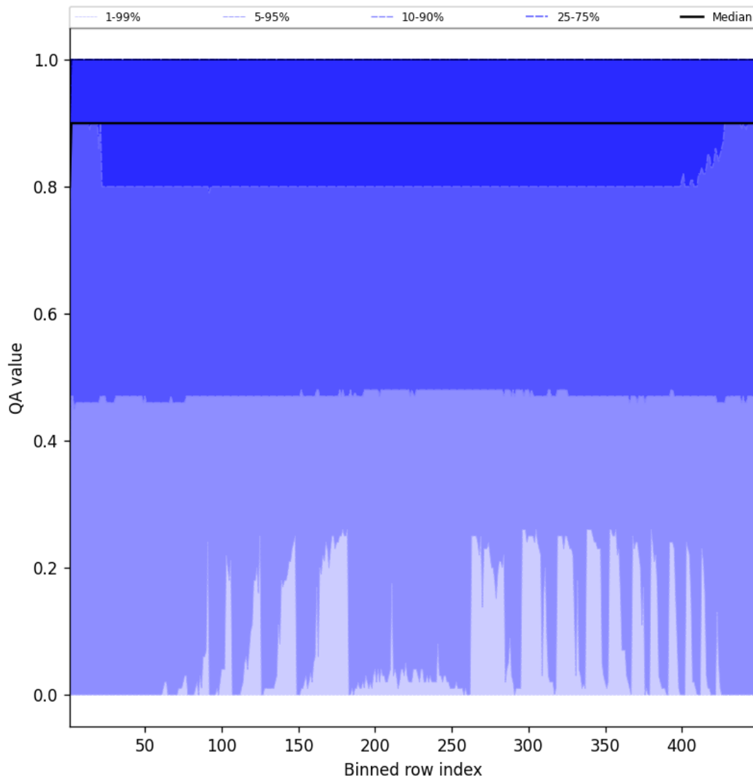
Figure 40: Along track statistics of “QA value” for 2025-05-23 to 2025-05-24
