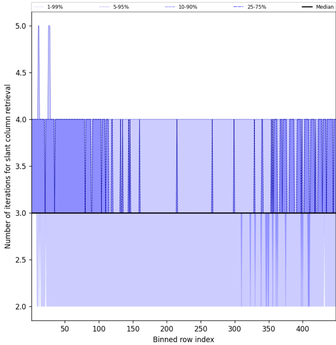
Figure 45: Along track statistics of “Number of iterations for slant column retrieval” for 2025-05-23 to 2025-05-24
