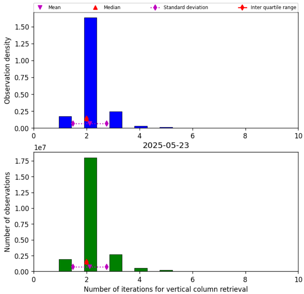
Figure 39: Histogram of “Number of iterations for vertical column retrieval” for 2025-05-23 to 2025-05-24
