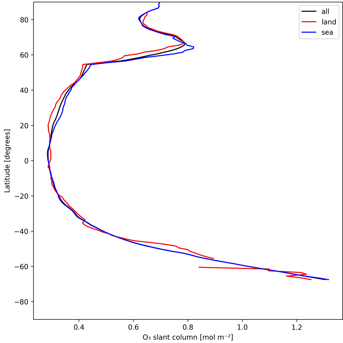
Figure 19: Zonal average of “O 3 slant column” for 2025-05-23 to 2025-05-24.
