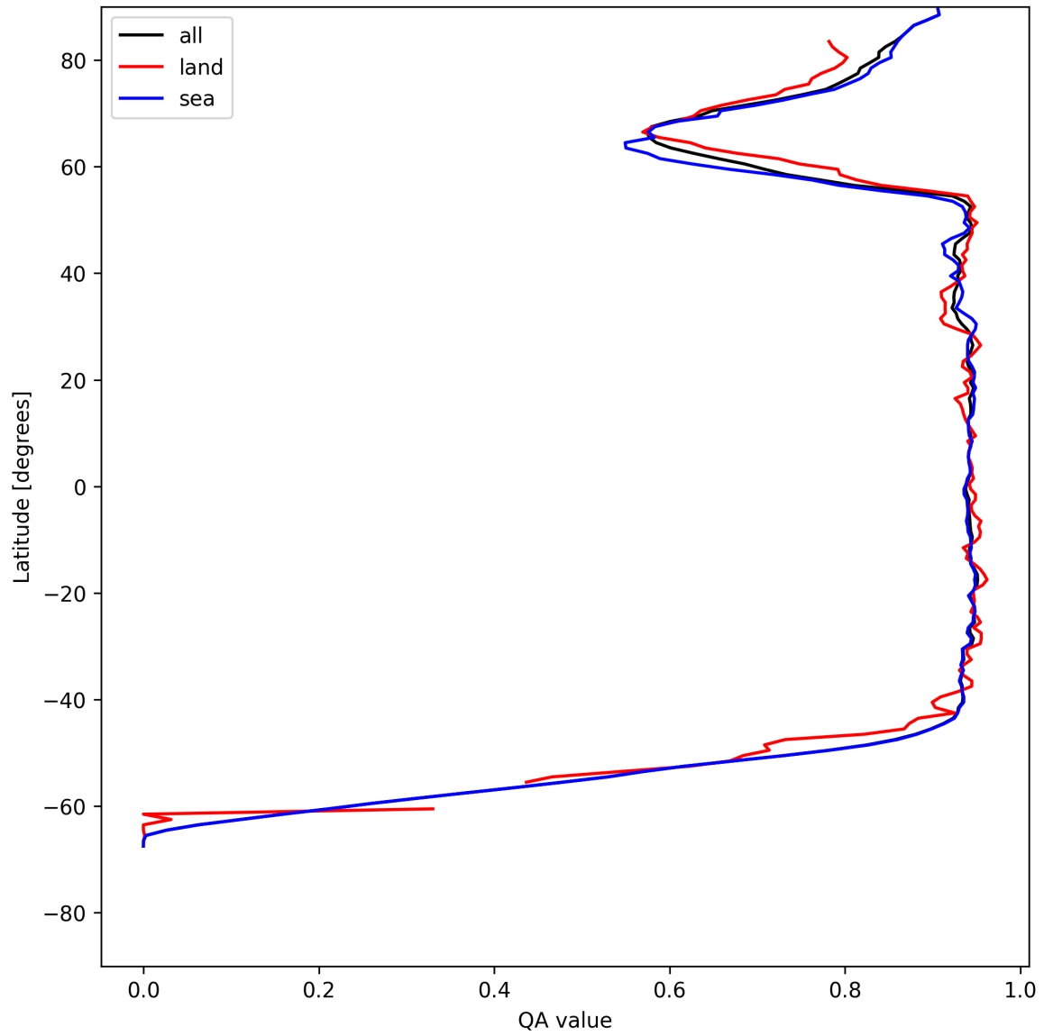
Figure 16: Zonal average of “QA value” for 2025-05-23 to 2025-05-24.
