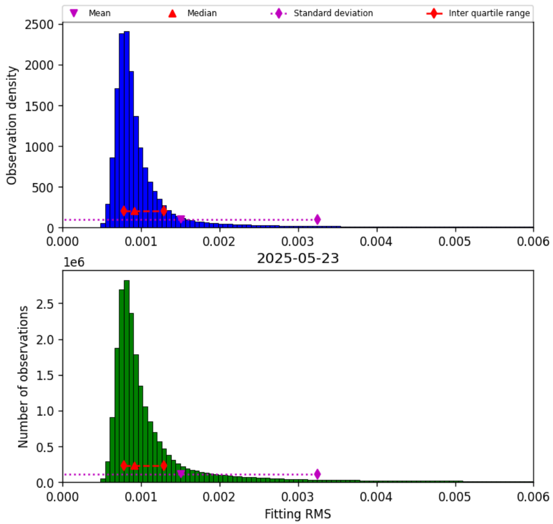
Figure 34: Histogram of “Fitting RMS” for 2025-05-23 to 2025-05-24
