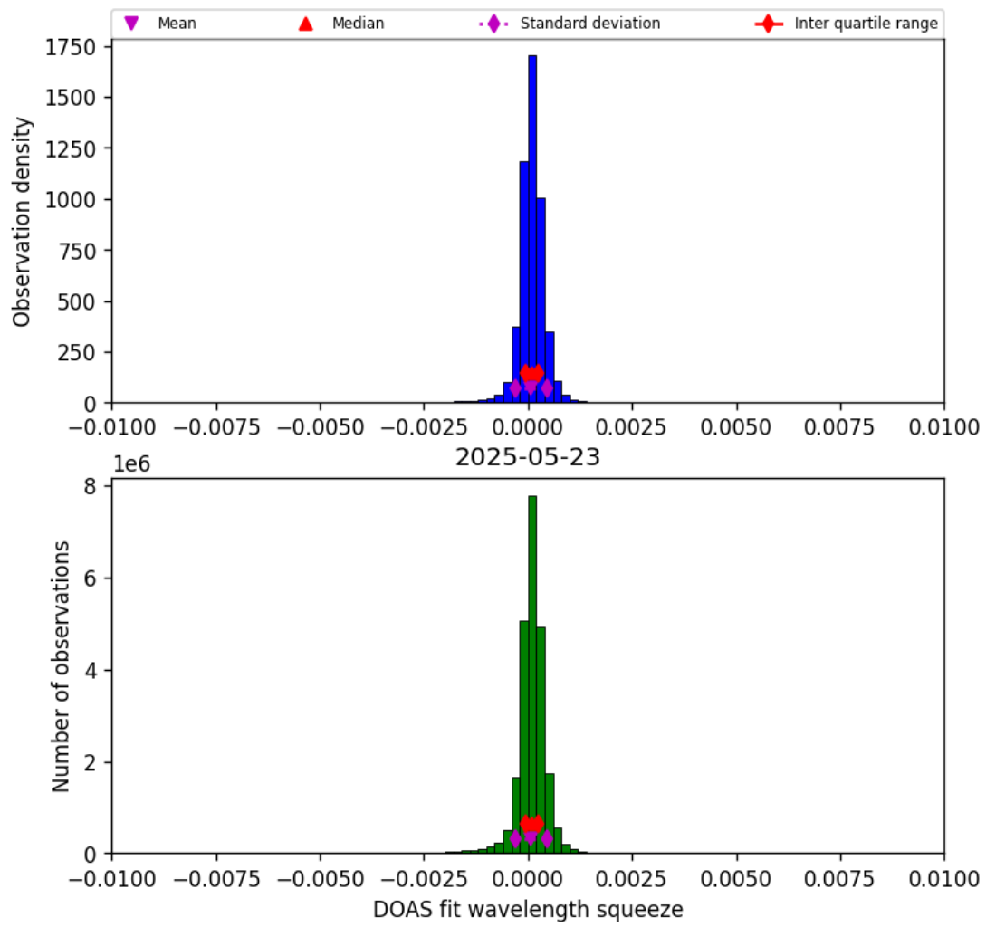
Figure 36: Histogram of “DOAS fit wavelength squeeze” for 2025-05-23 to 2025-05-24
