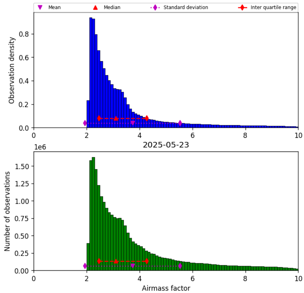
Figure 37: Histogram of “Airmass factor” for 2025-05-23 to 2025-05-24
