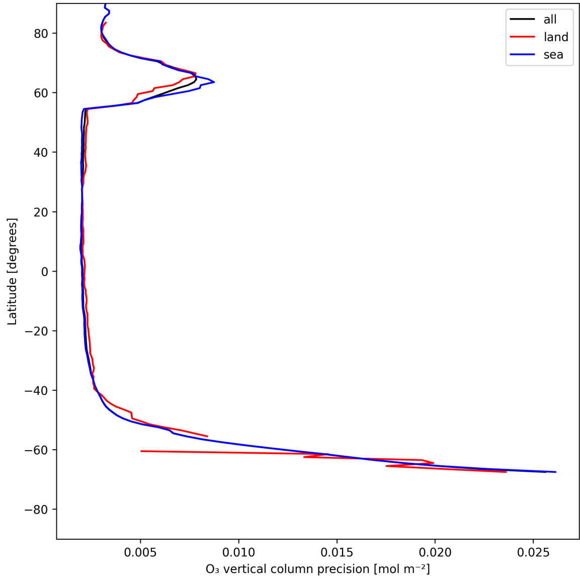
Figure 18: Zonal average of “O 3 vertical column precision” for 2025-05-23 to 2025-05-24.
