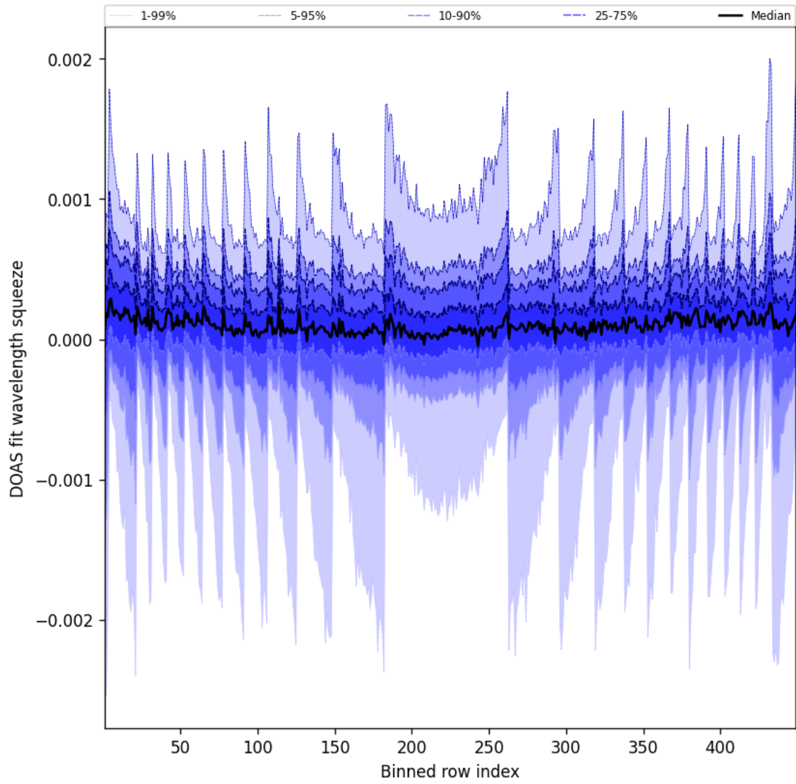
Figure 48: Along track statistics of “DOAS fit wavelength squeeze” for 2025-05-23 to 2025-05-24
