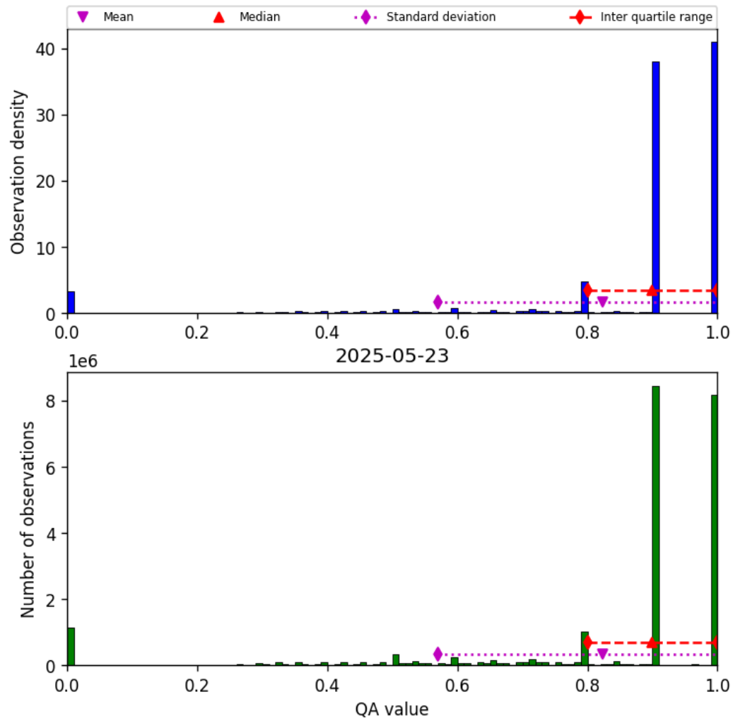
Figure 28: Histogram of “QA value” for 2025-05-23 to 2025-05-24
