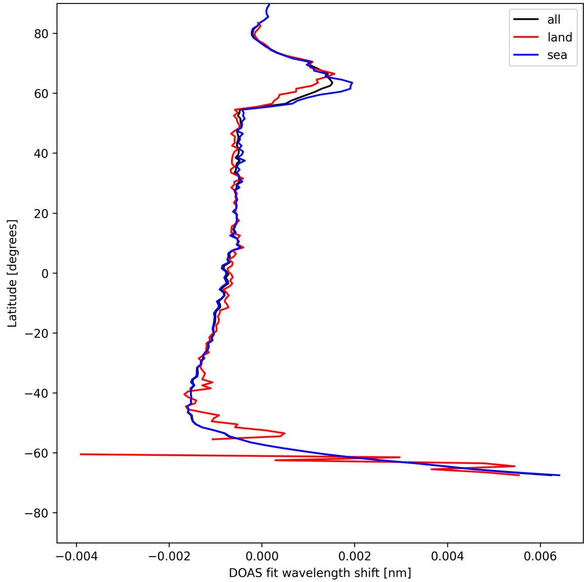
Figure 23: Zonal average of “DOAS fit wavelength shift” for 2025-05-23 to 2025-05-24.
