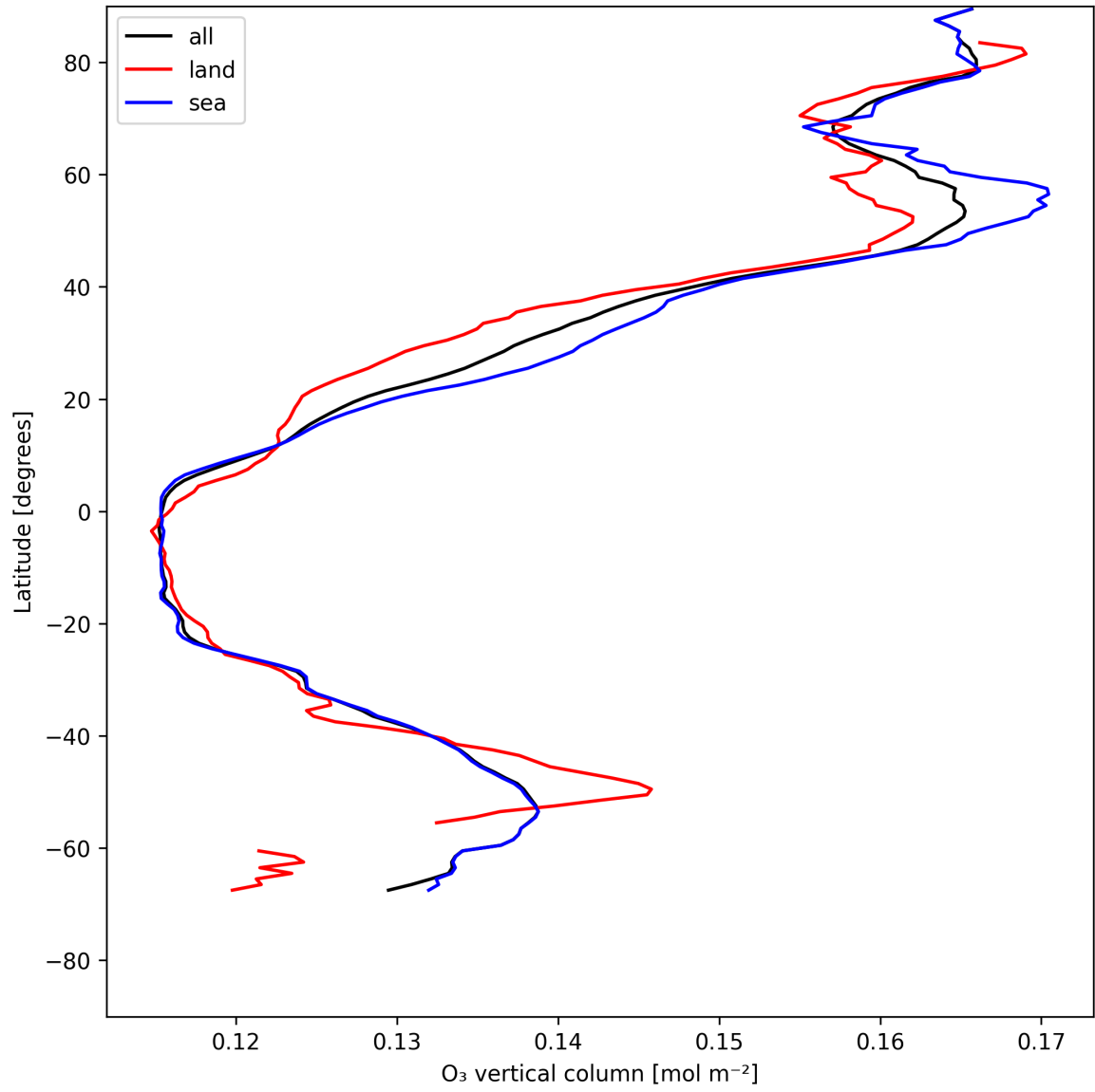
Figure 17: Zonal average of “O 3 vertical column” for 2025-05-23 to 2025-05-24.
