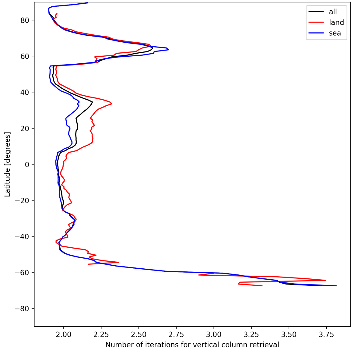
Figure 27: Zonal average of “Number of iterations for vertical column retrieval” for 2025-05-23 to 2025-05-24.
