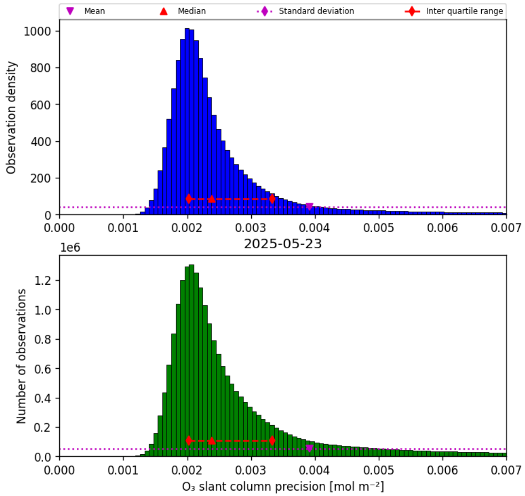
Figure 32: Histogram of “O 3 slant column precision” for 2025-05-23 to 2025-05-24
