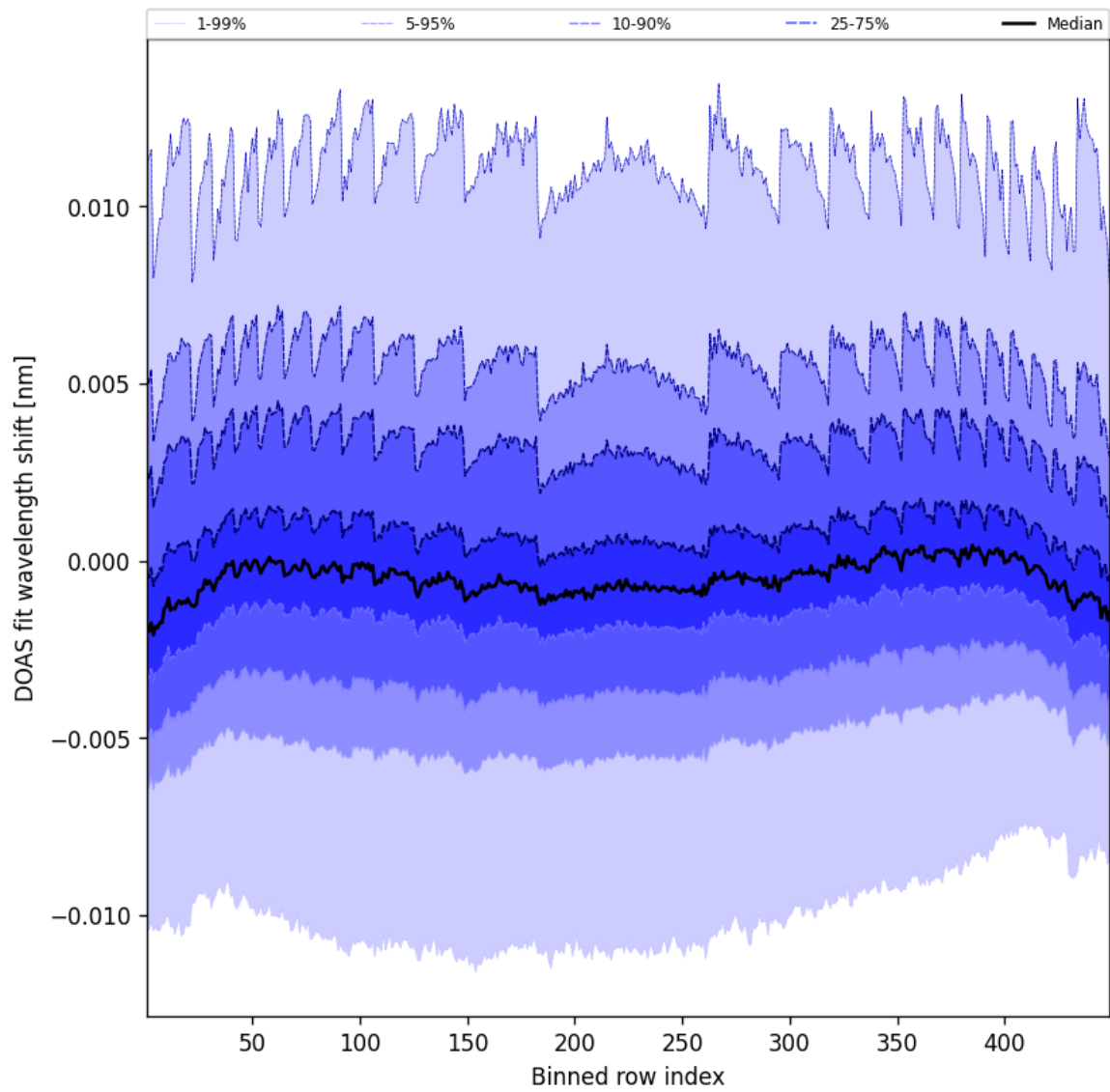
Figure 47: Along track statistics of “DOAS fit wavelength shift” for 2025-05-23 to 2025-05-24
