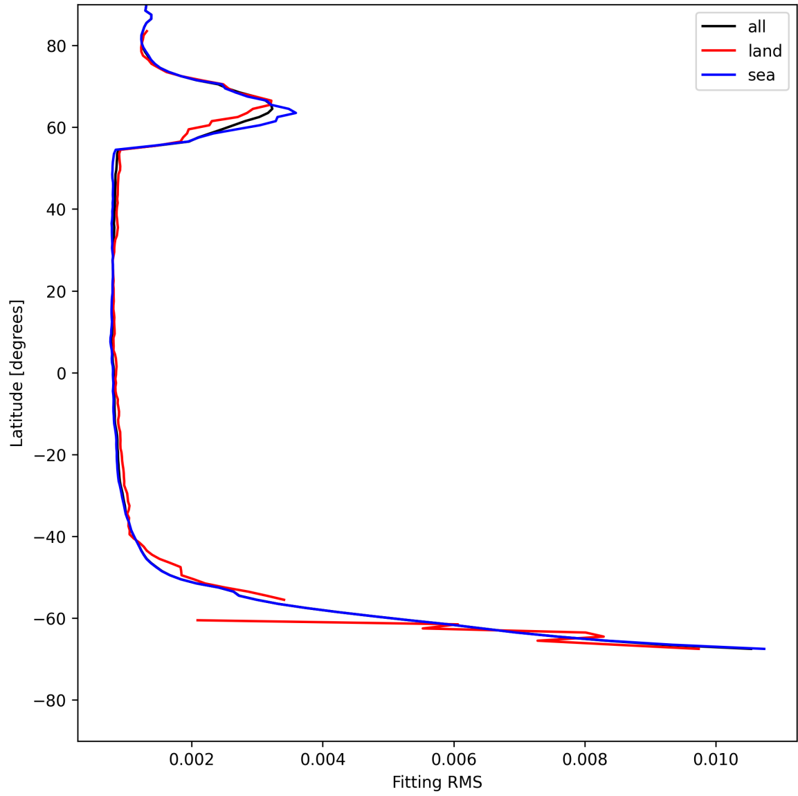
Figure 22: Zonal average of “Fitting RMS” for 2025-05-23 to 2025-05-24.
