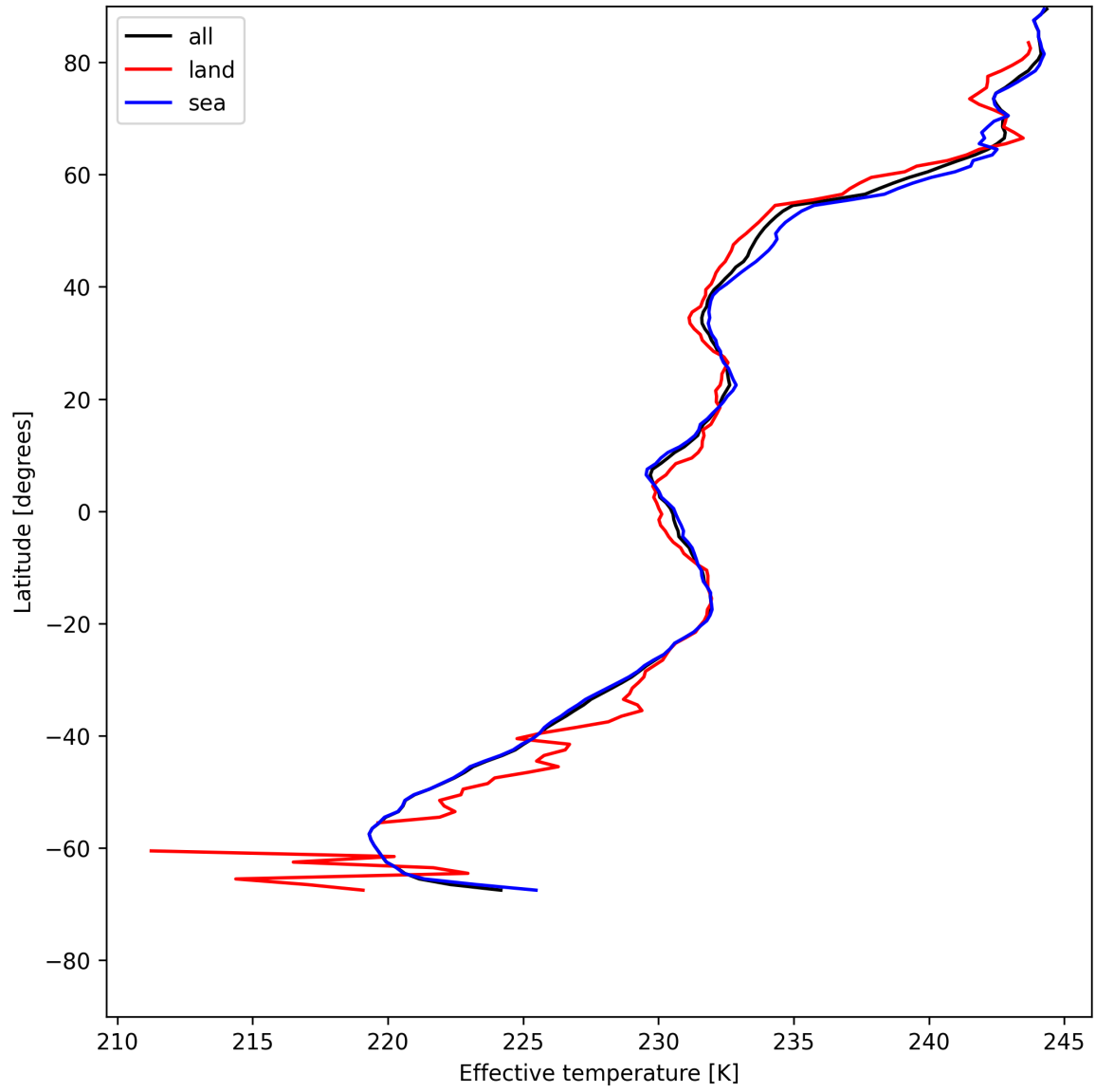
Figure 26: Zonal average of "Effective temperature" for 2025-05-23 to 2025-05-24.
