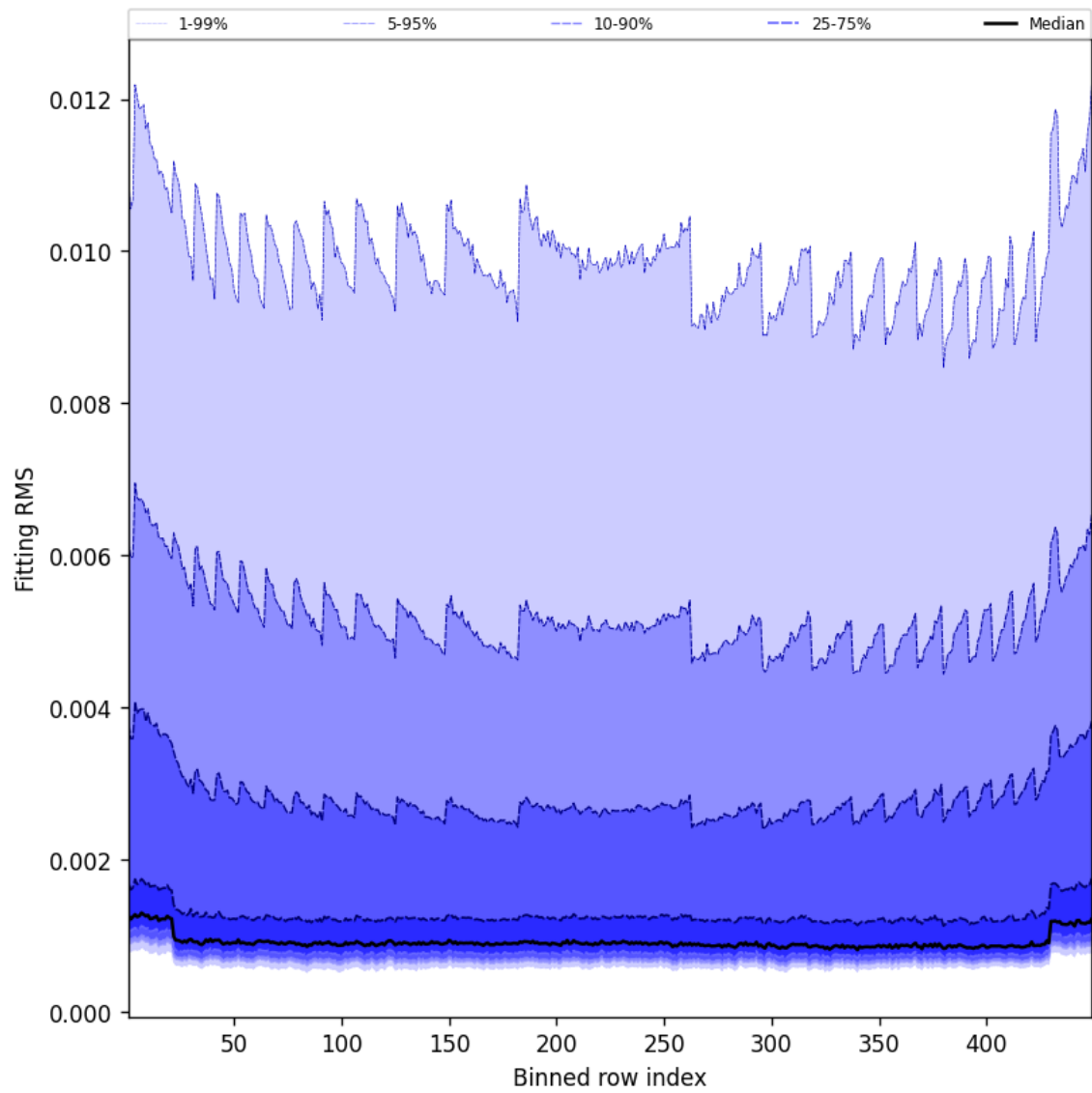
Figure 46: Along track statistics of “Fitting RMS” for 2025-05-23 to 2025-05-24
