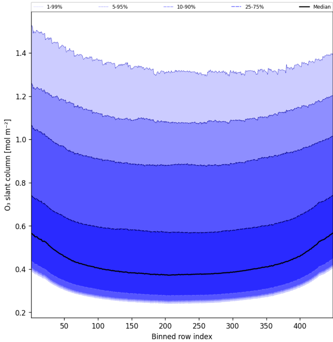
Figure 43: Along track statistics of “O 3 slant column” for 2025-05-23 to 2025-05-24
