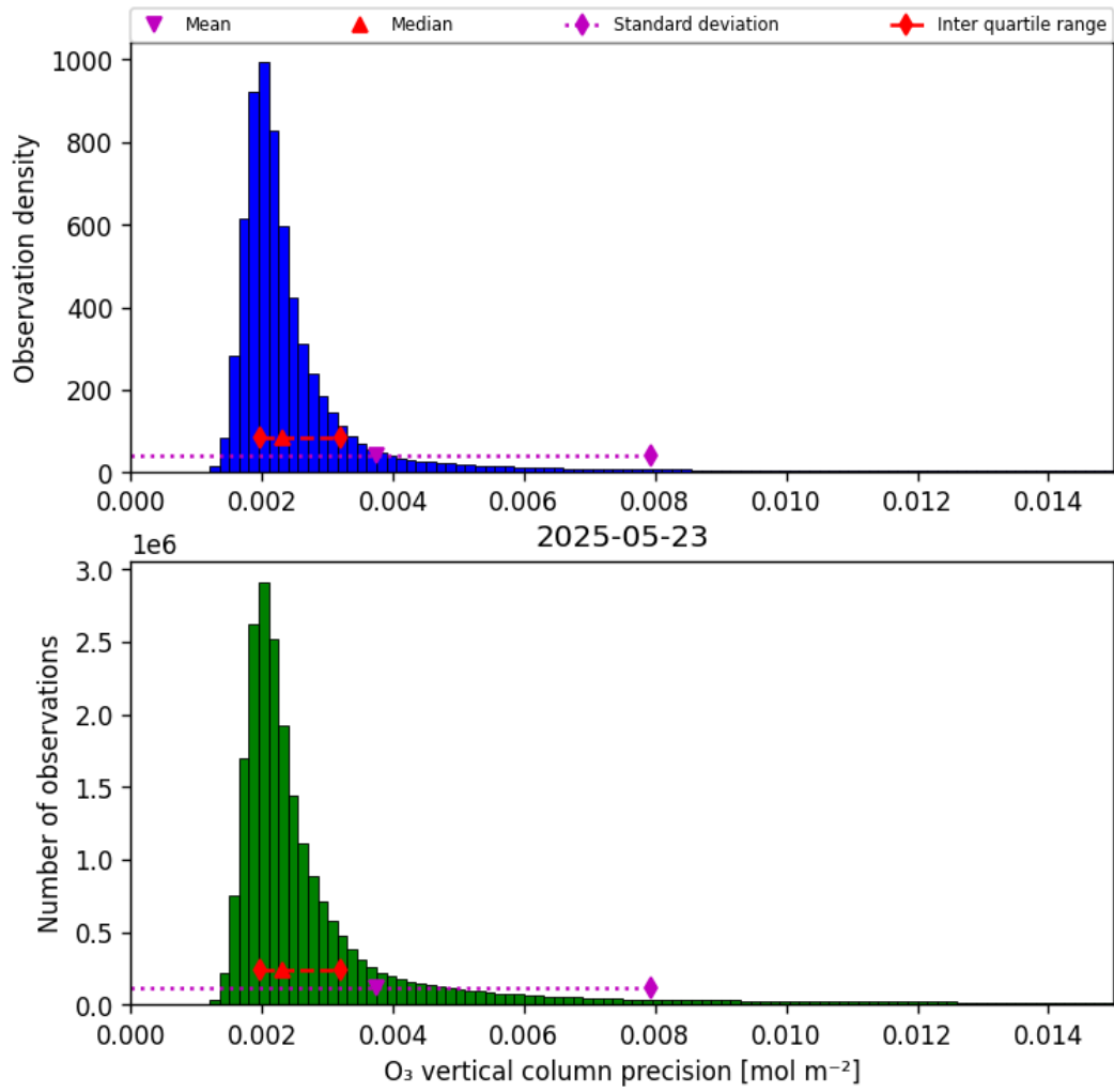
Figure 30: Histogram of “O 3 vertical column precision” for 2025-05-23 to 2025-05-24
