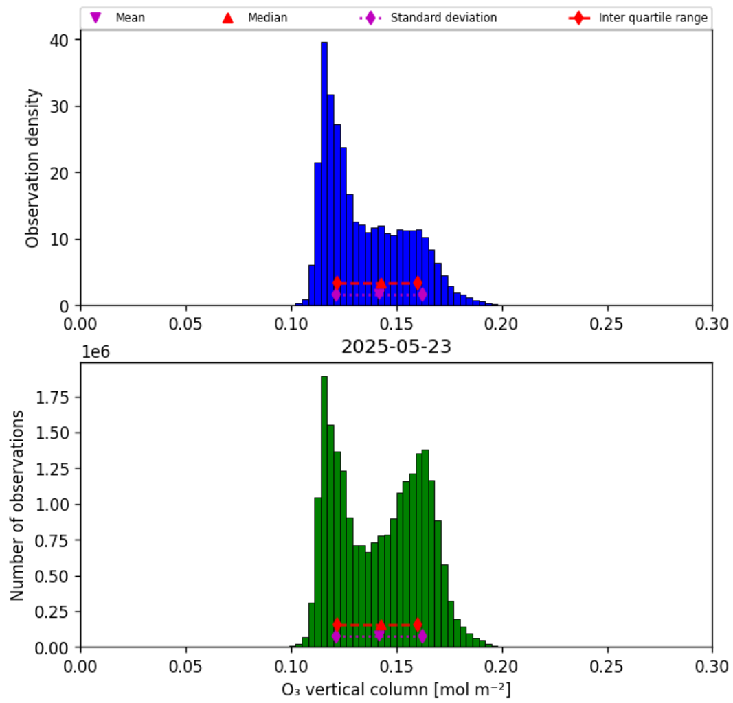
Figure 29: Histogram of “O 3 vertical column” for 2025-05-23 to 2025-05-24
