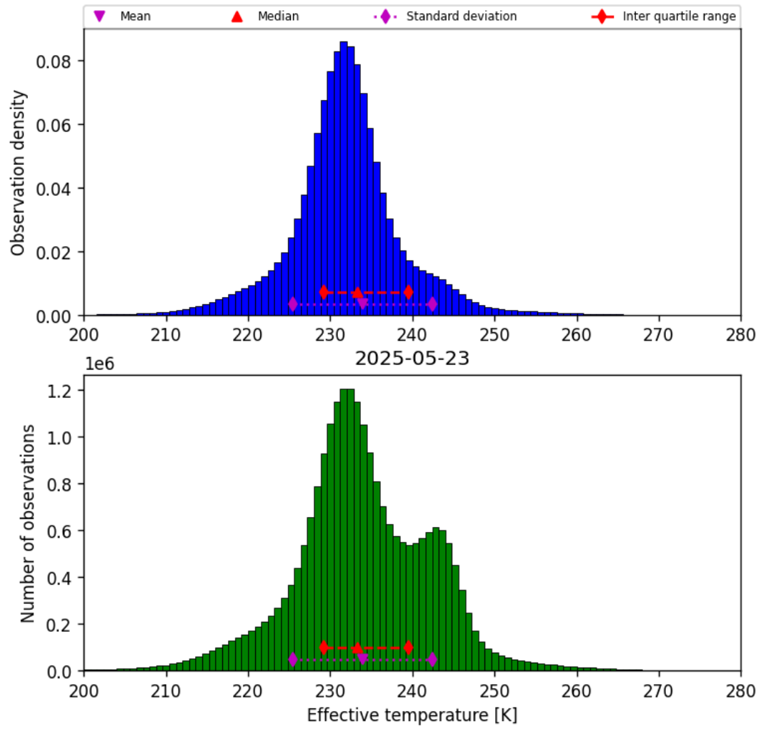
Figure 38: Histogram of “Effective temperature” for 2025-05-23 to 2025-05-24
