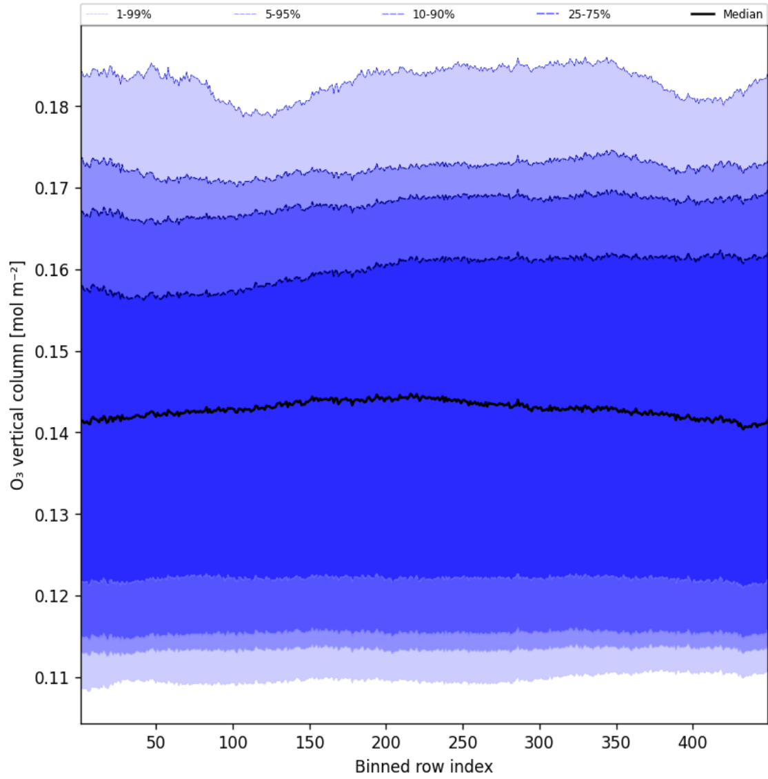
Figure 41: Along track statistics of “O 3 vertical column” for 2025-05-23 to 2025-05-24
