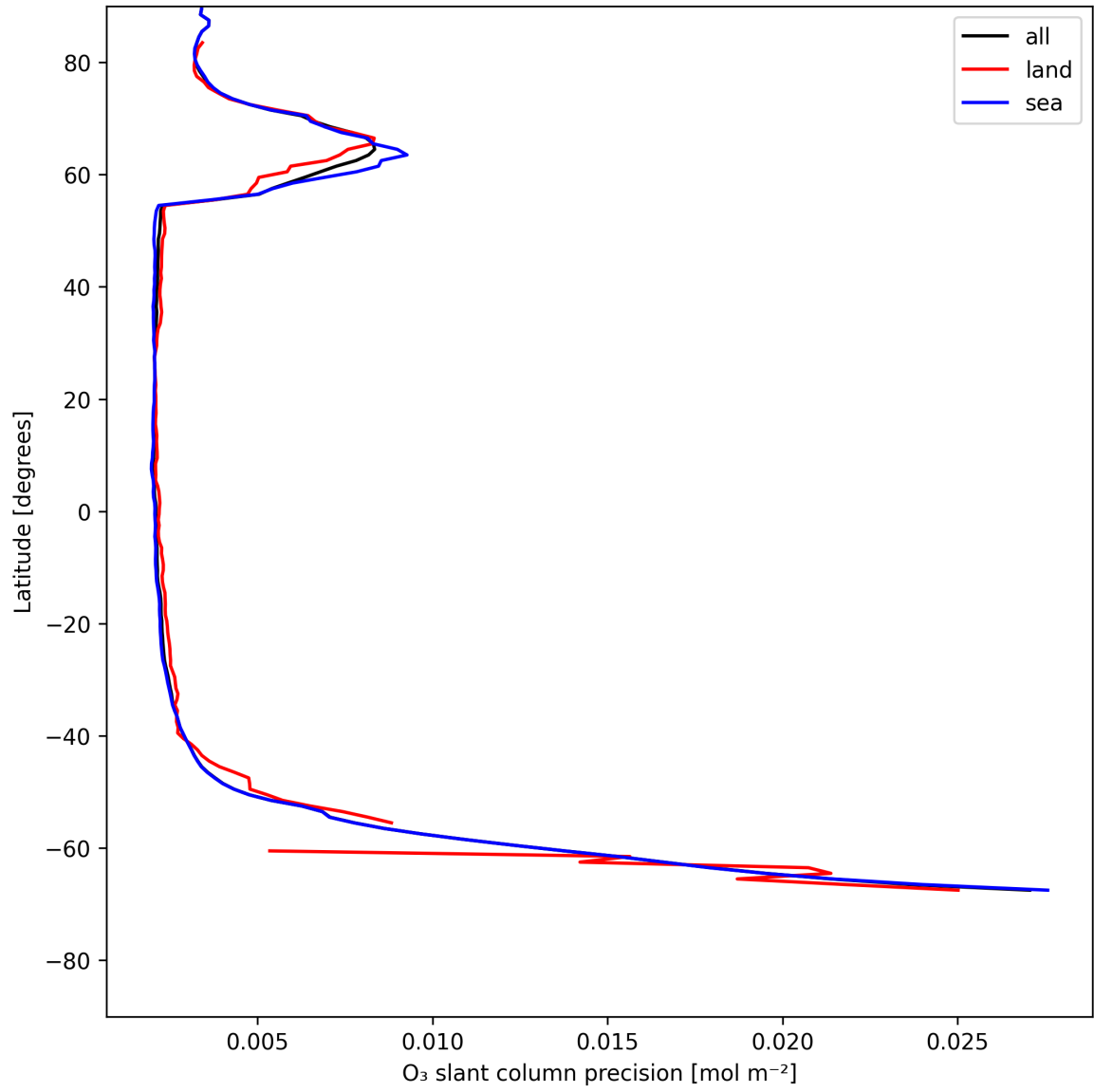
Figure 20: Zonal average of “O 3 slant column precision” for 2025-05-23 to 2025-05-24.
