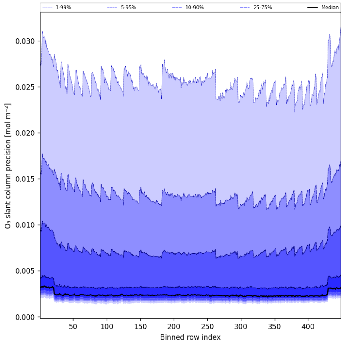
Figure 44: Along track statistics of “O 3 slant column precision” for 2025-05-23 to 2025-05-24
