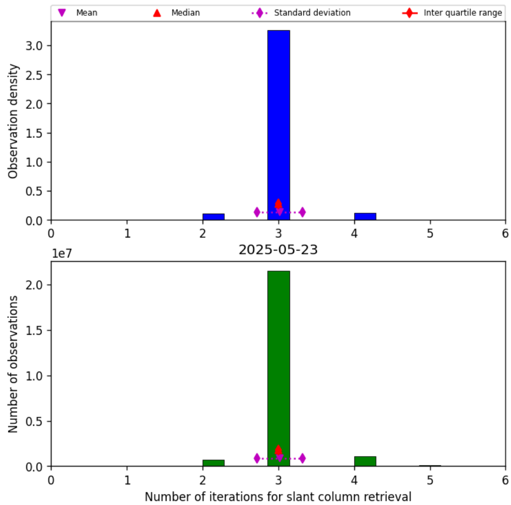
Figure 33: Histogram of “Number of iterations for slant column retrieval” for 2025-05-23 to 2025-05-24
