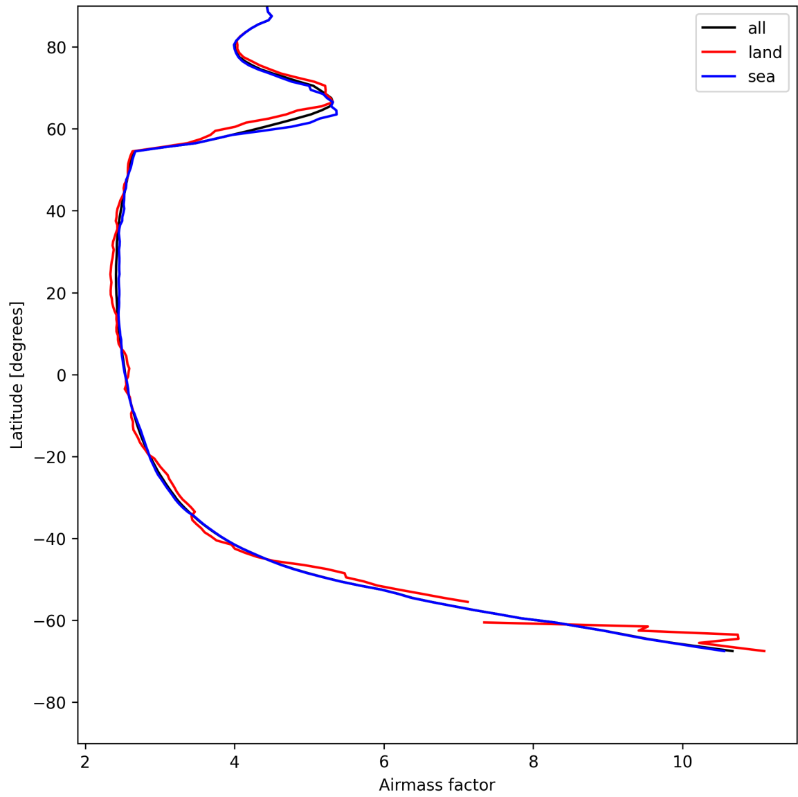
Figure 25: Zonal average of “Airmass factor” for 2025-05-23 to 2025-05-24.
