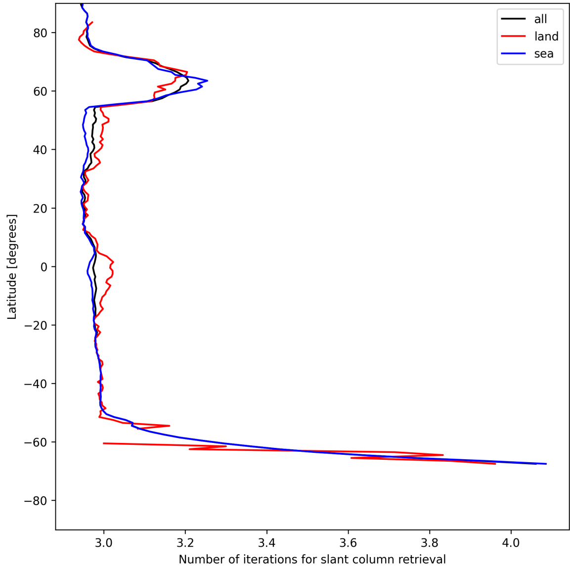
Figure 21: Zonal average of “Number of iterations for slant column retrieval” for 2025-05-23 to 2025-05-24.
