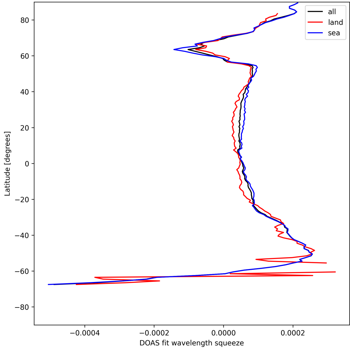
Figure 24: Zonal average of “DOAS fit wavelength squeeze” for 2025-05-23 to 2025-05-24.
