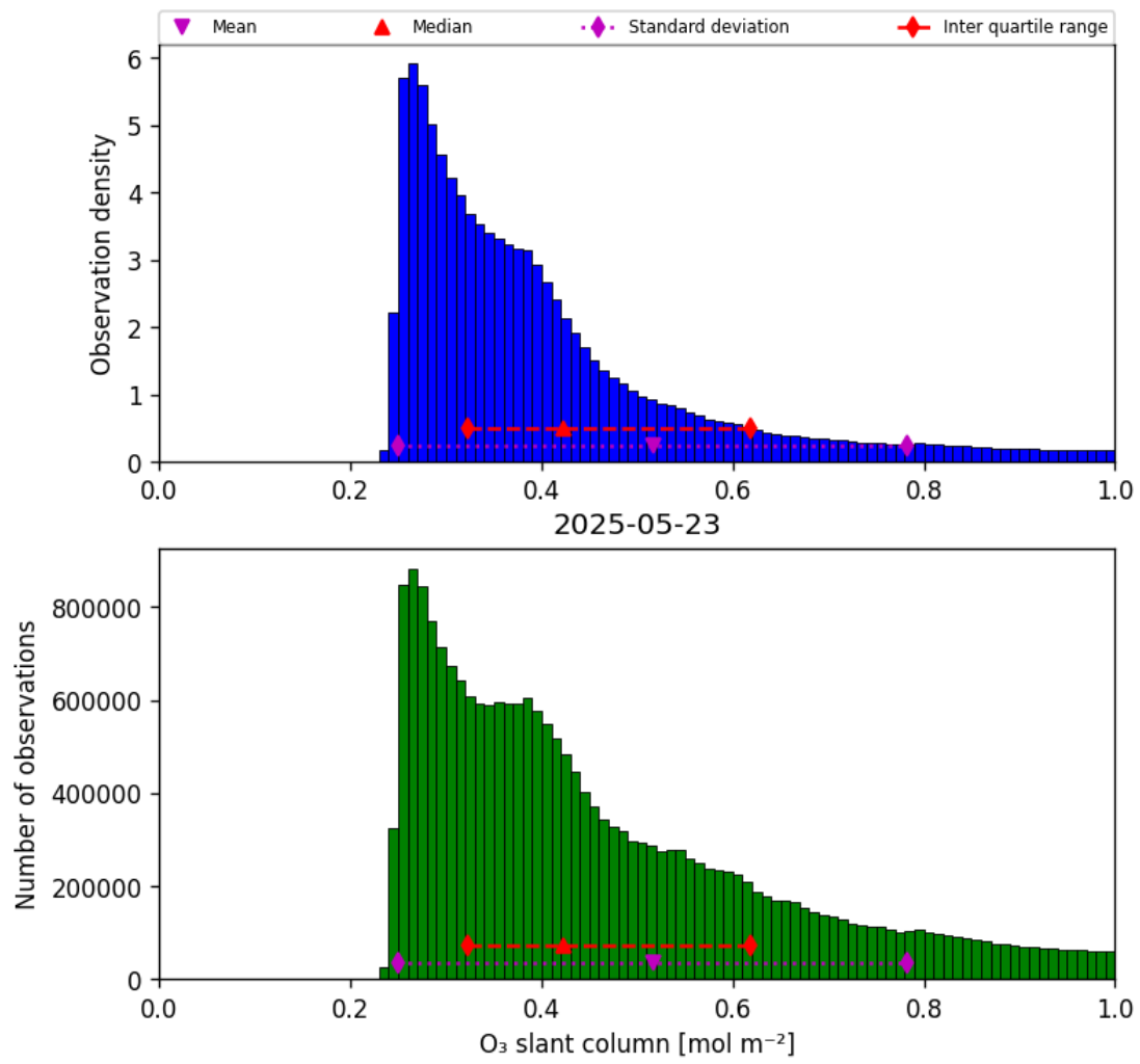
Figure 31: Histogram of “O 3 slant column” for 2025-05-23 to 2025-05-24
