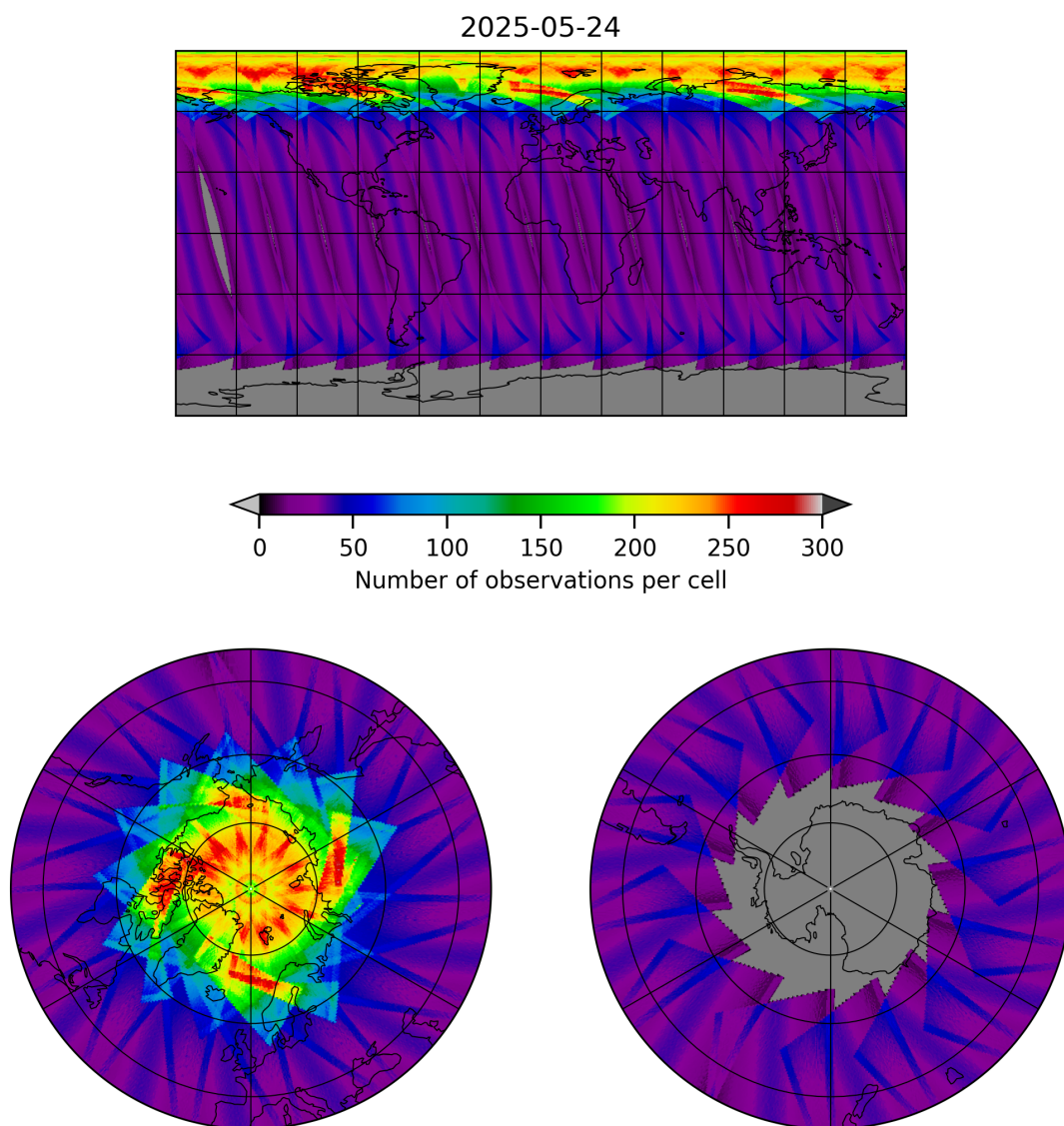
Figure 15: Map of the number of observations for 2025-05-24 to 2025-05-24
