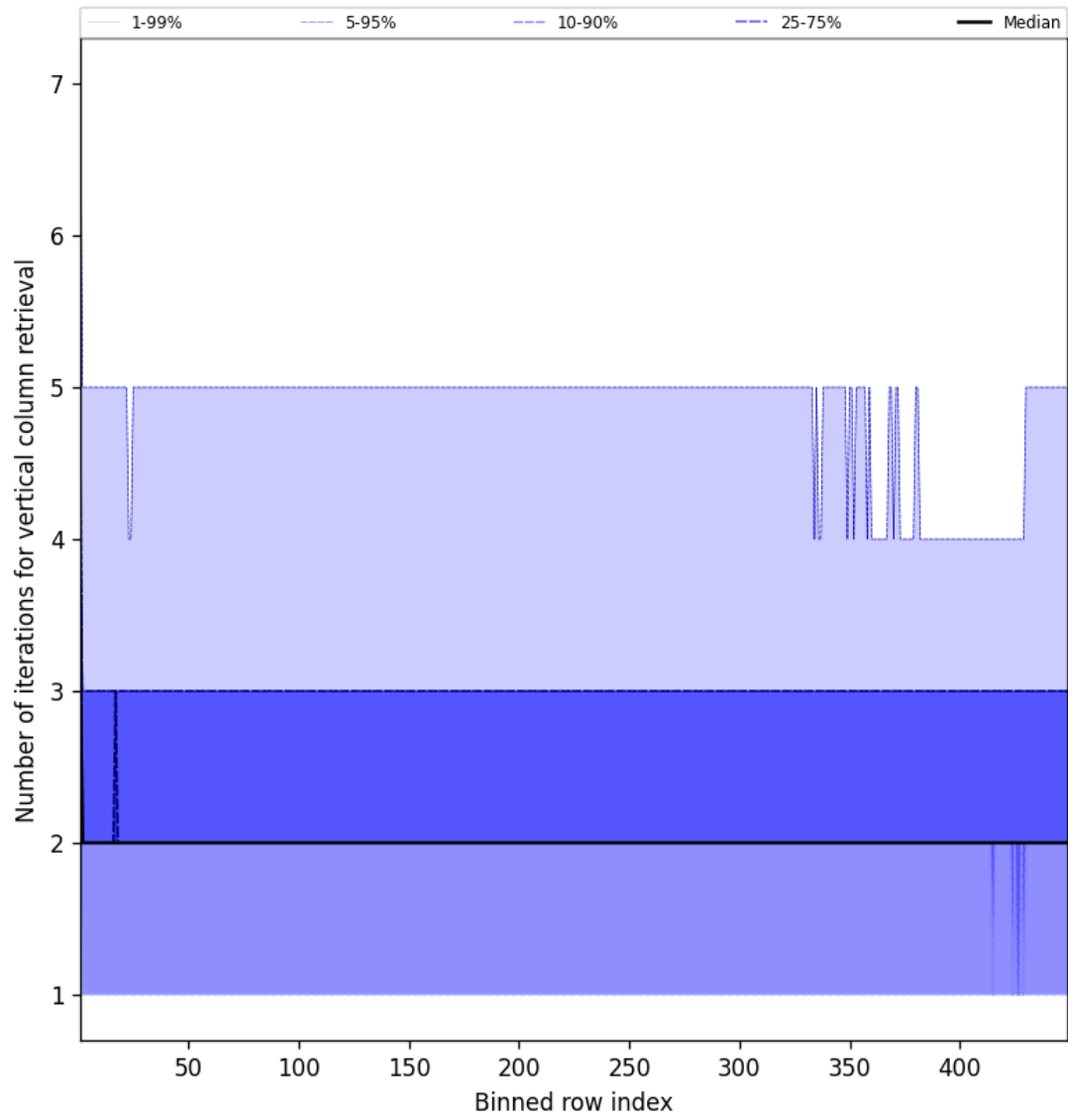
Figure 51: Along track statistics of “Number of iterations for vertical column retrieval” for 2025-05-24 to 2025-05-24
