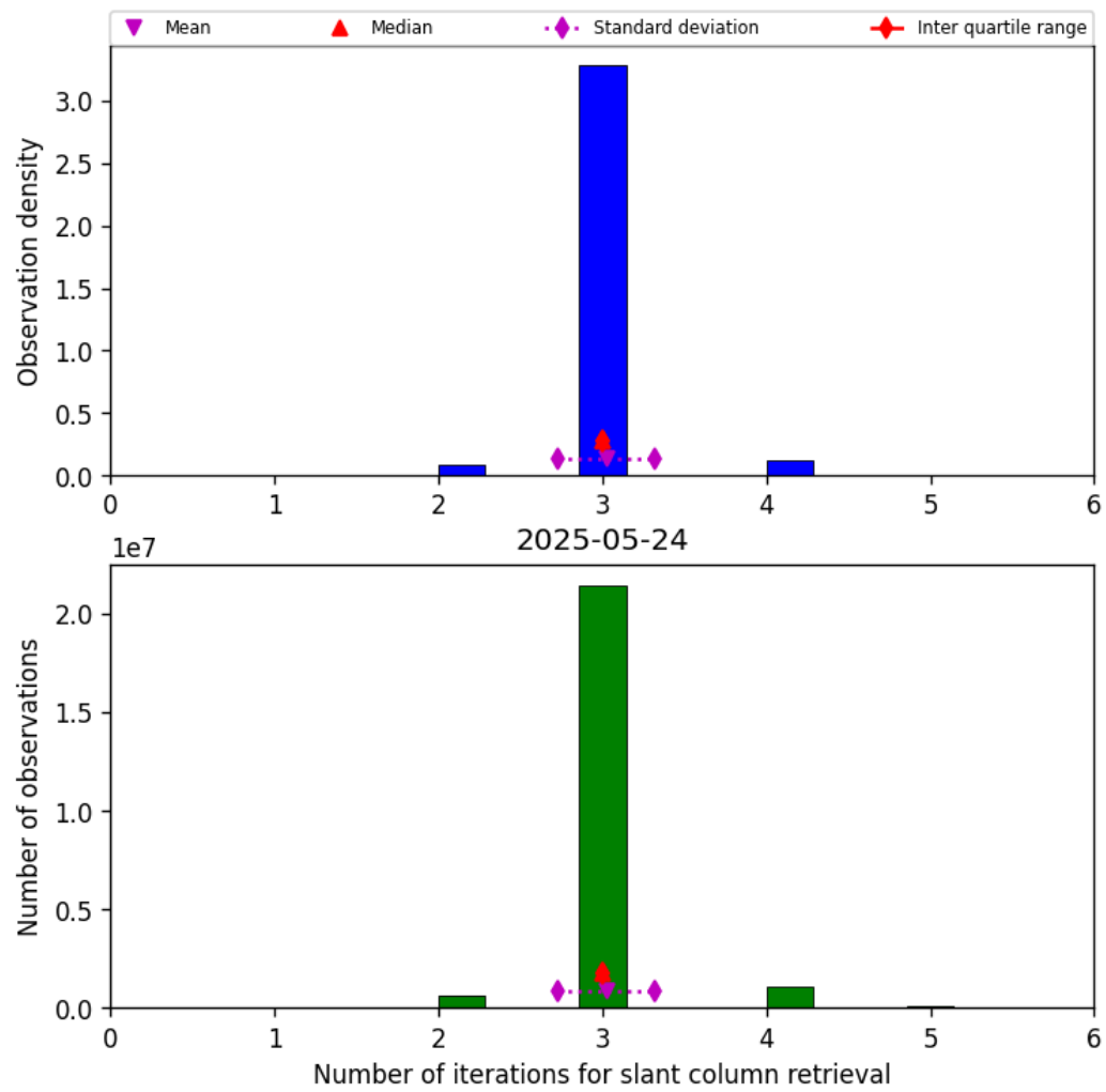
Figure 33: Histogram of “Number of iterations for slant column retrieval” for 2025-05-24 to 2025-05-24
