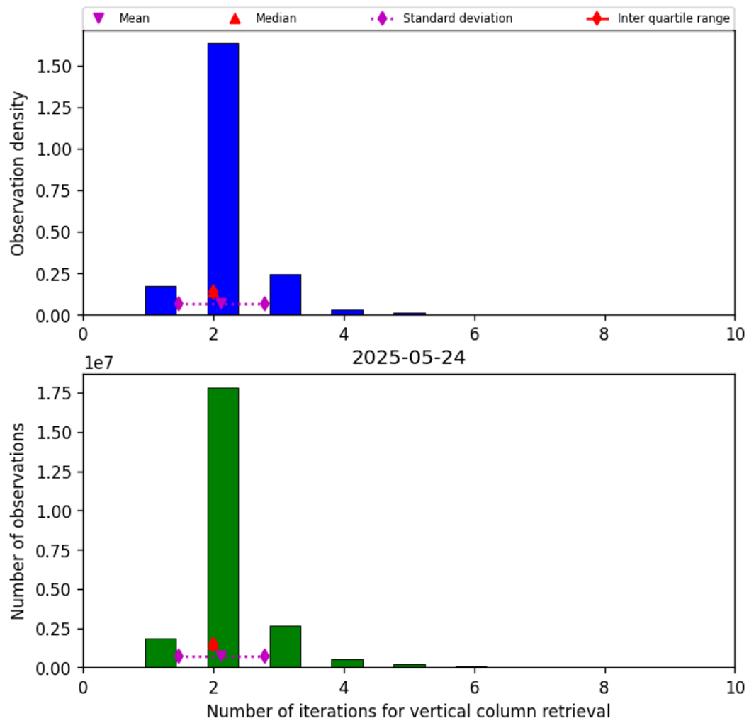
Figure 39: Histogram of “Number of iterations for vertical column retrieval” for 2025-05-24 to 2025-05-24
