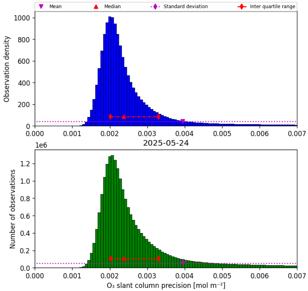
Figure 32: Histogram of “O 3 slant column precision” for 2025-05-24 to 2025-05-24
