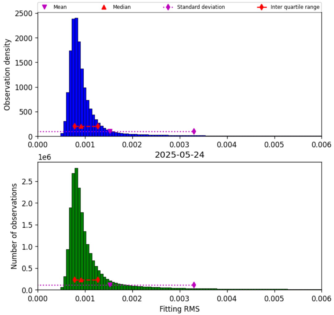
Figure 34: Histogram of “Fitting RMS” for 2025-05-24 to 2025-05-24
