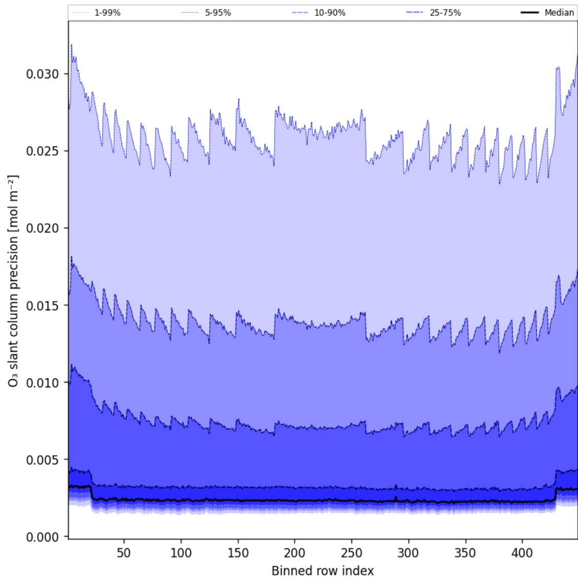
Figure 44: Along track statistics of “O 3 slant column precision” for 2025-05-24 to 2025-05-24
