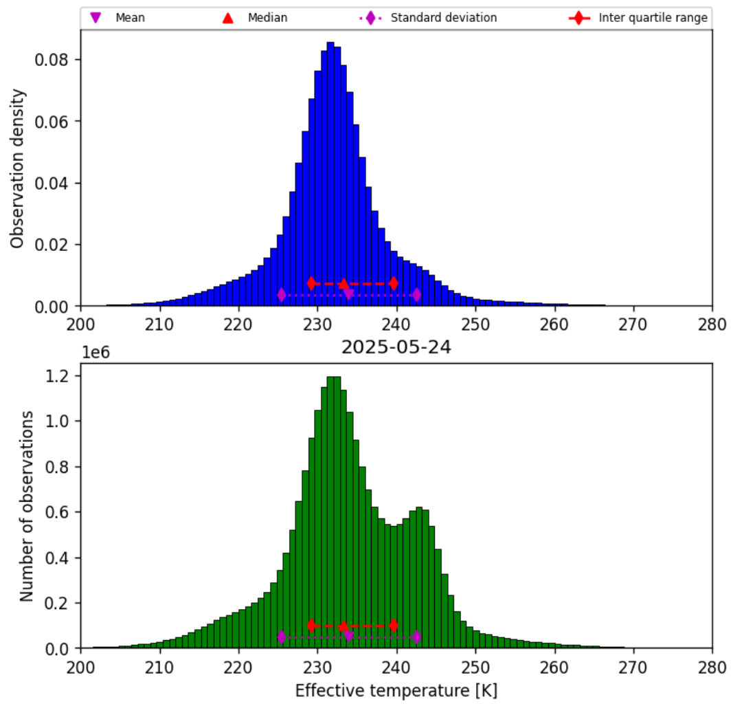
Figure 38: Histogram of “Effective temperature” for 2025-05-24 to 2025-05-24
