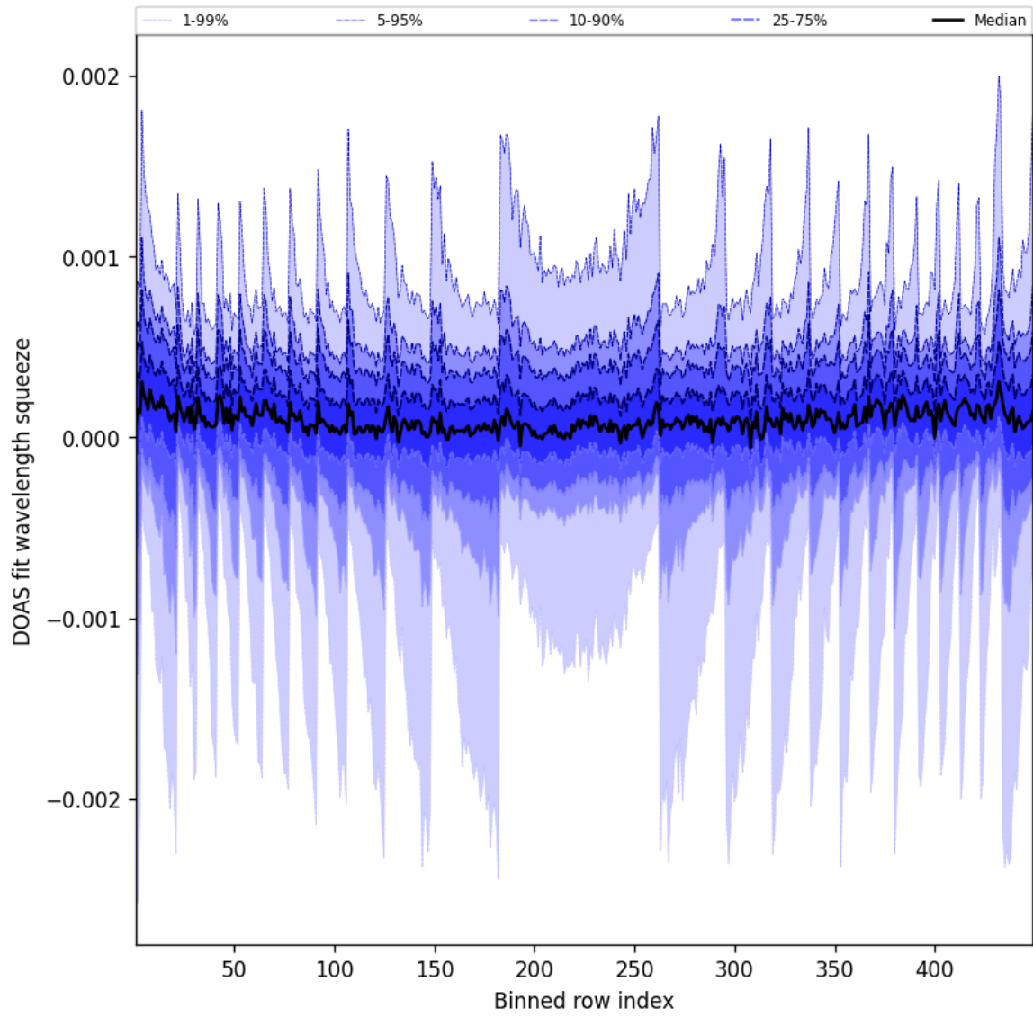
Figure 48: Along track statistics of “DOAS fit wavelength squeeze” for 2025-05-24 to 2025-05-24
