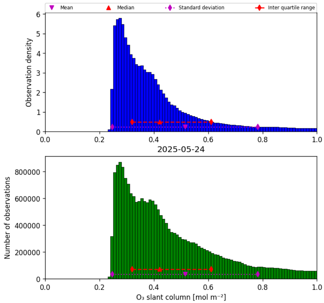
Figure 31: Histogram of “O 3 slant column” for 2025-05-24 to 2025-05-24
