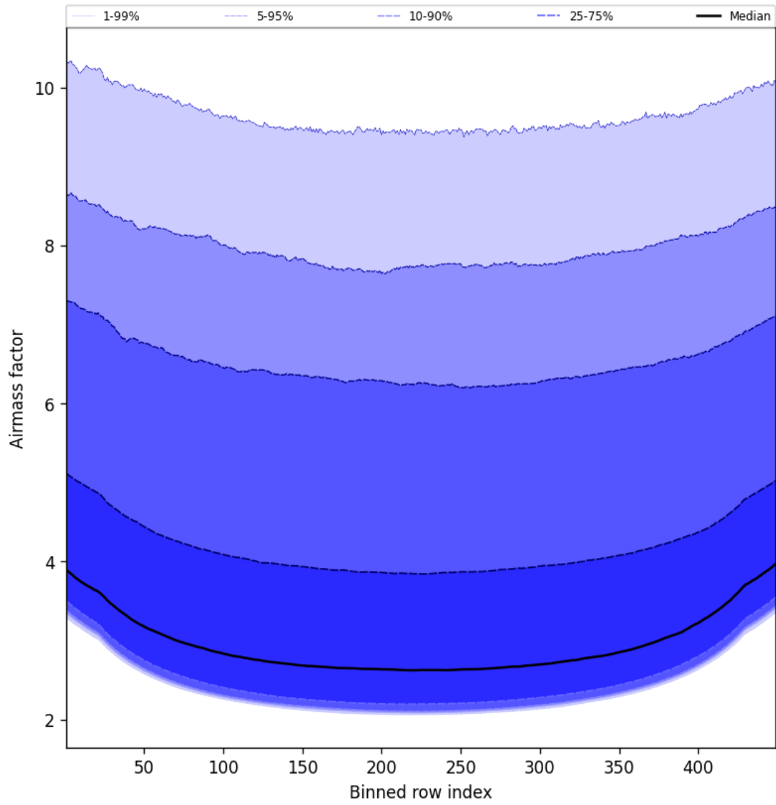
Figure 49: Along track statistics of “Airmass factor” for 2025-05-24 to 2025-05-24
