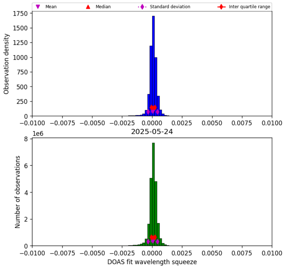
Figure 36: Histogram of “DOAS fit wavelength squeeze” for 2025-05-24 to 2025-05-24
