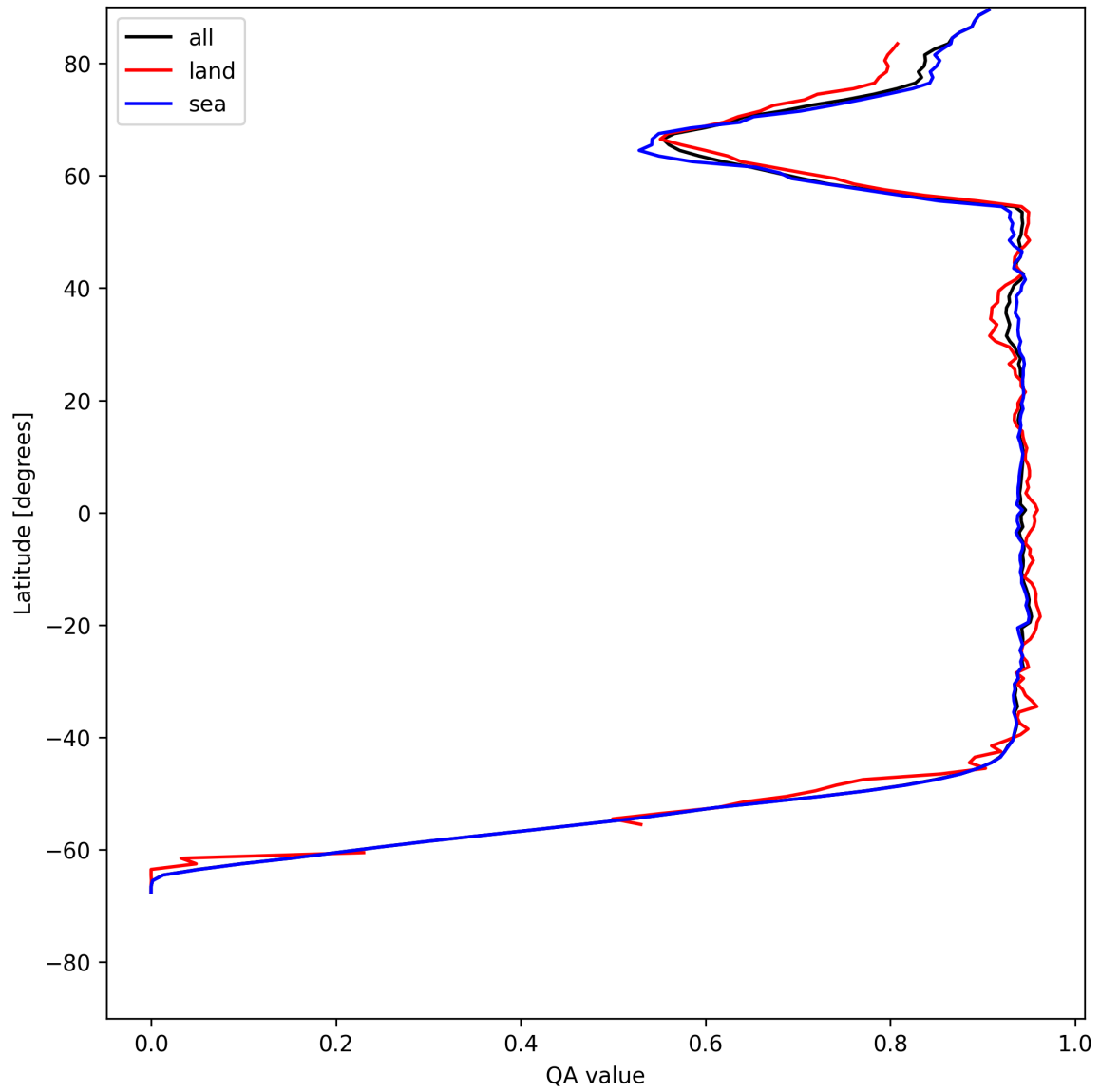
Figure 16: Zonal average of “QA value” for 2025-05-24 to 2025-05-24.
