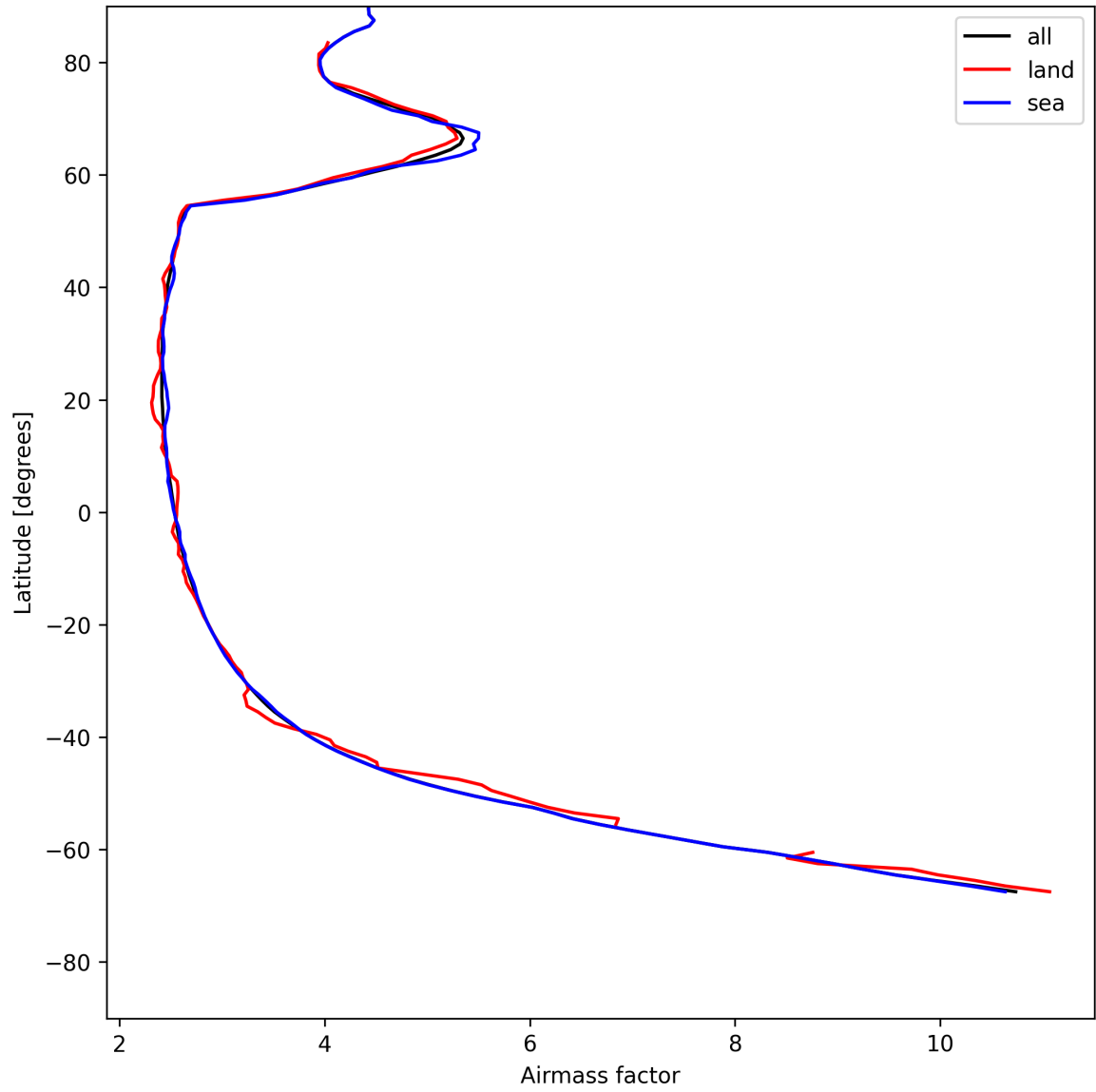
Figure 25: Zonal average of “Airmass factor” for 2025-05-24 to 2025-05-24.
