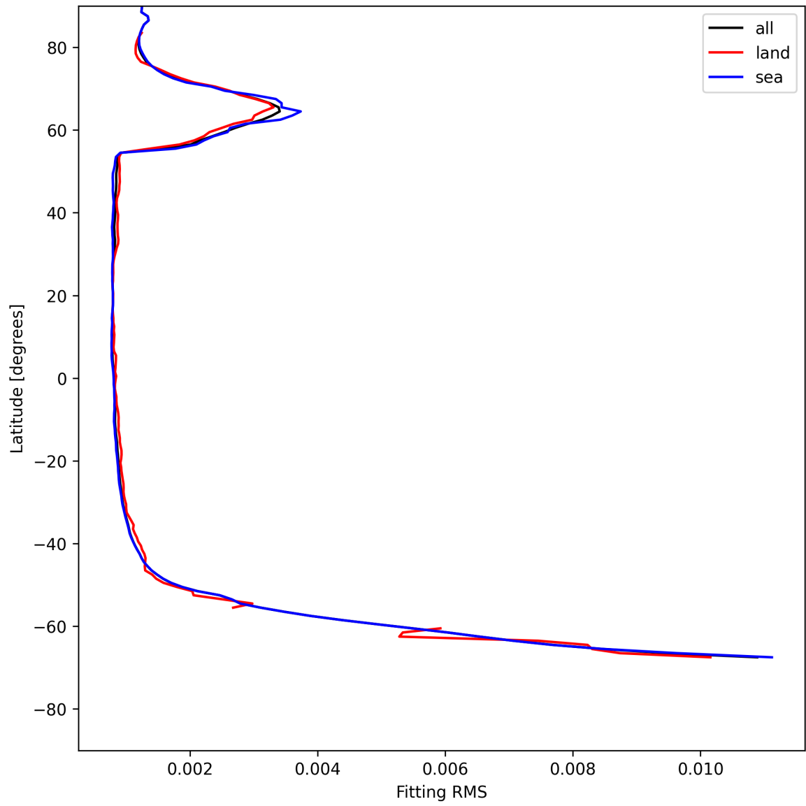
Figure 22: Zonal average of “Fitting RMS” for 2025-05-24 to 2025-05-24.
