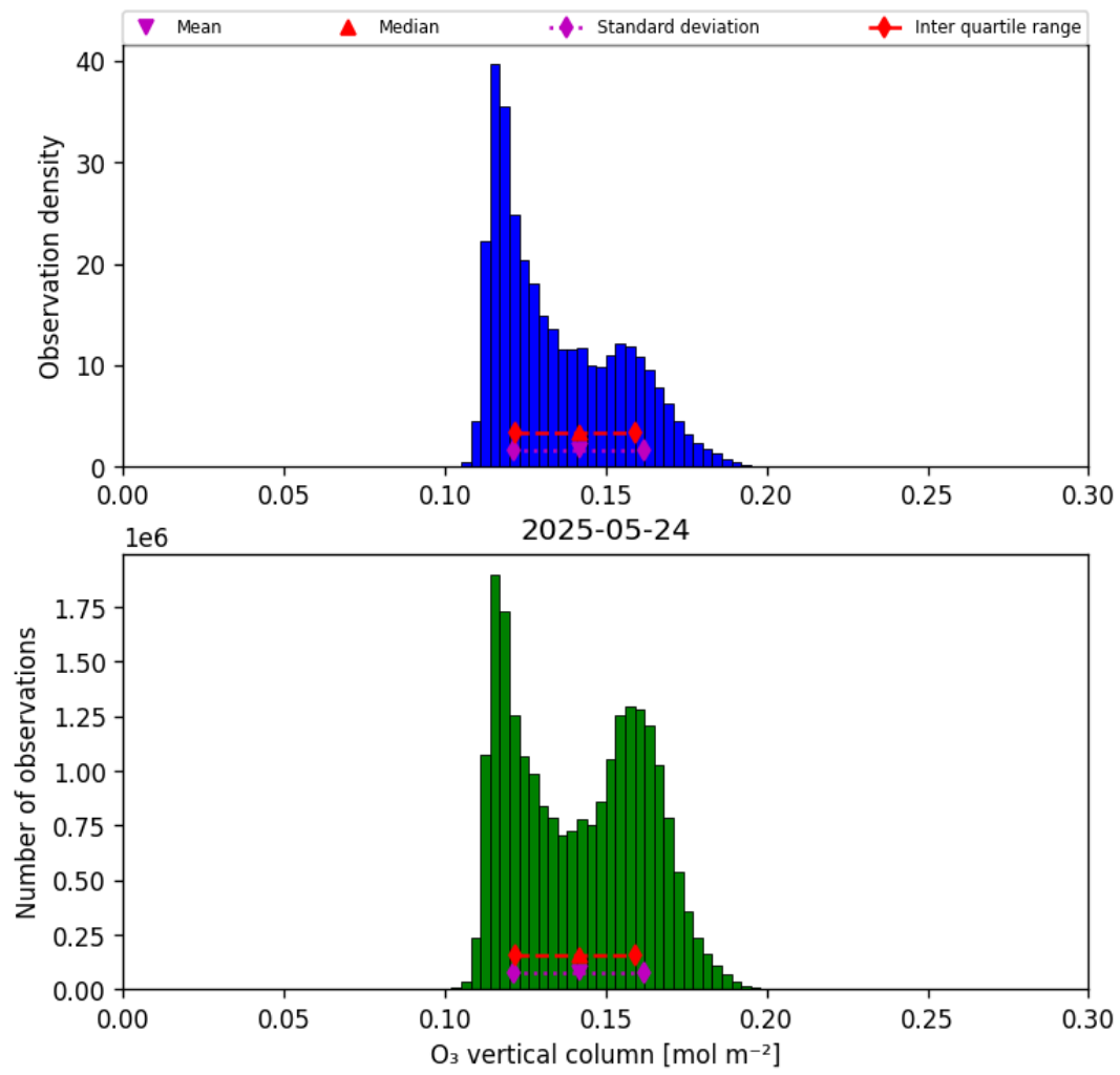
Figure 29: Histogram of “O 3 vertical column” for 2025-05-24 to 2025-05-24
