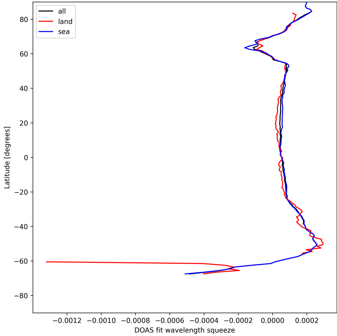
Figure 24: Zonal average of “DOAS fit wavelength squeeze” for 2025-05-24 to 2025-05-24.
