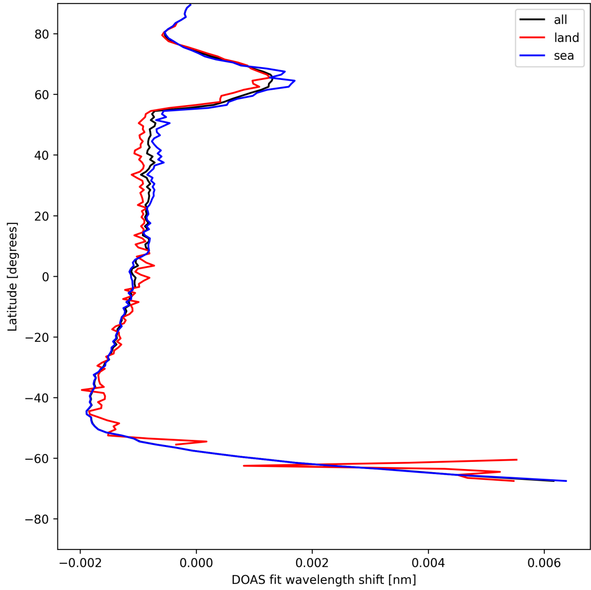
Figure 23: Zonal average of “DOAS fit wavelength shift” for 2025-05-24 to 2025-05-24.
