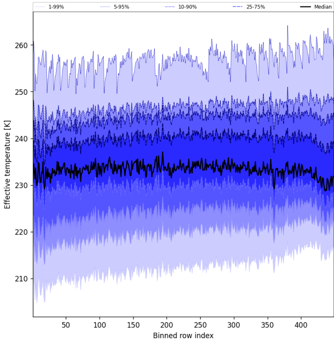
Figure 50: Along track statistics of “Effective temperature” for 2025-05-24 to 2025-05-24
