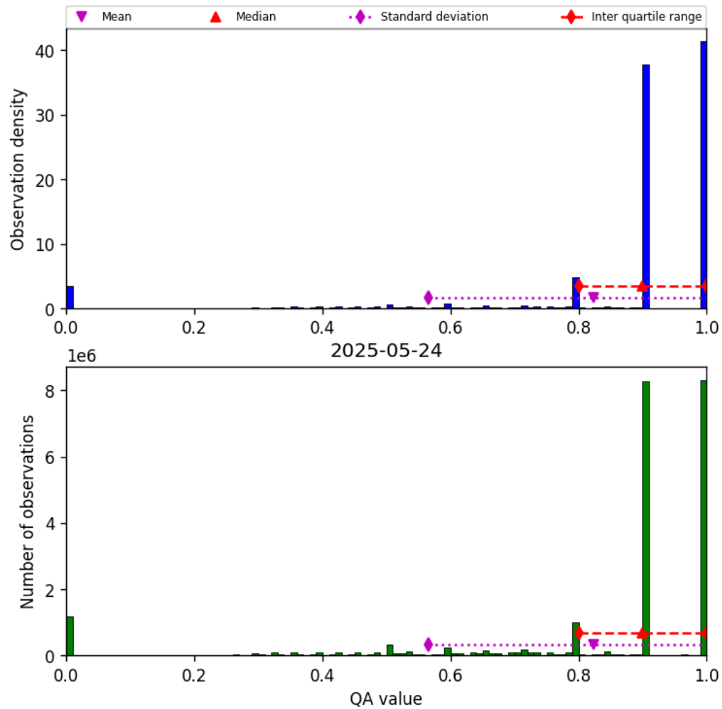
Figure 28: Histogram of “QA value” for 2025-05-24 to 2025-05-24
