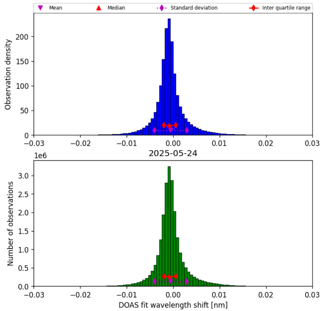
Figure 35: Histogram of “DOAS fit wavelength shift” for 2025-05-24 to 2025-05-24
