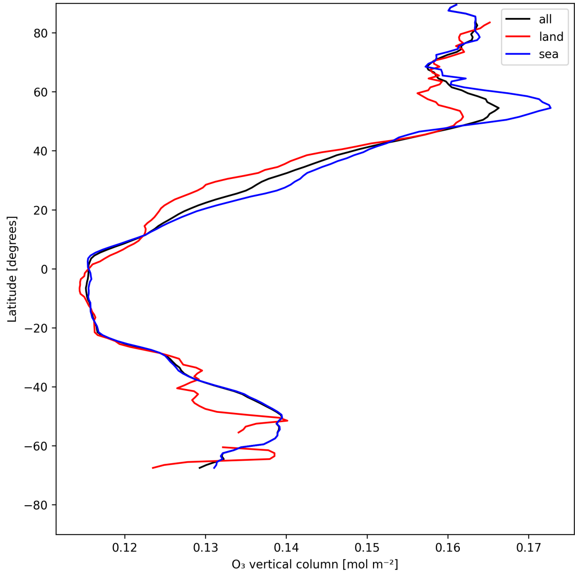
Figure 17: Zonal average of “O 3 vertical column” for 2025-05-24 to 2025-05-24.
