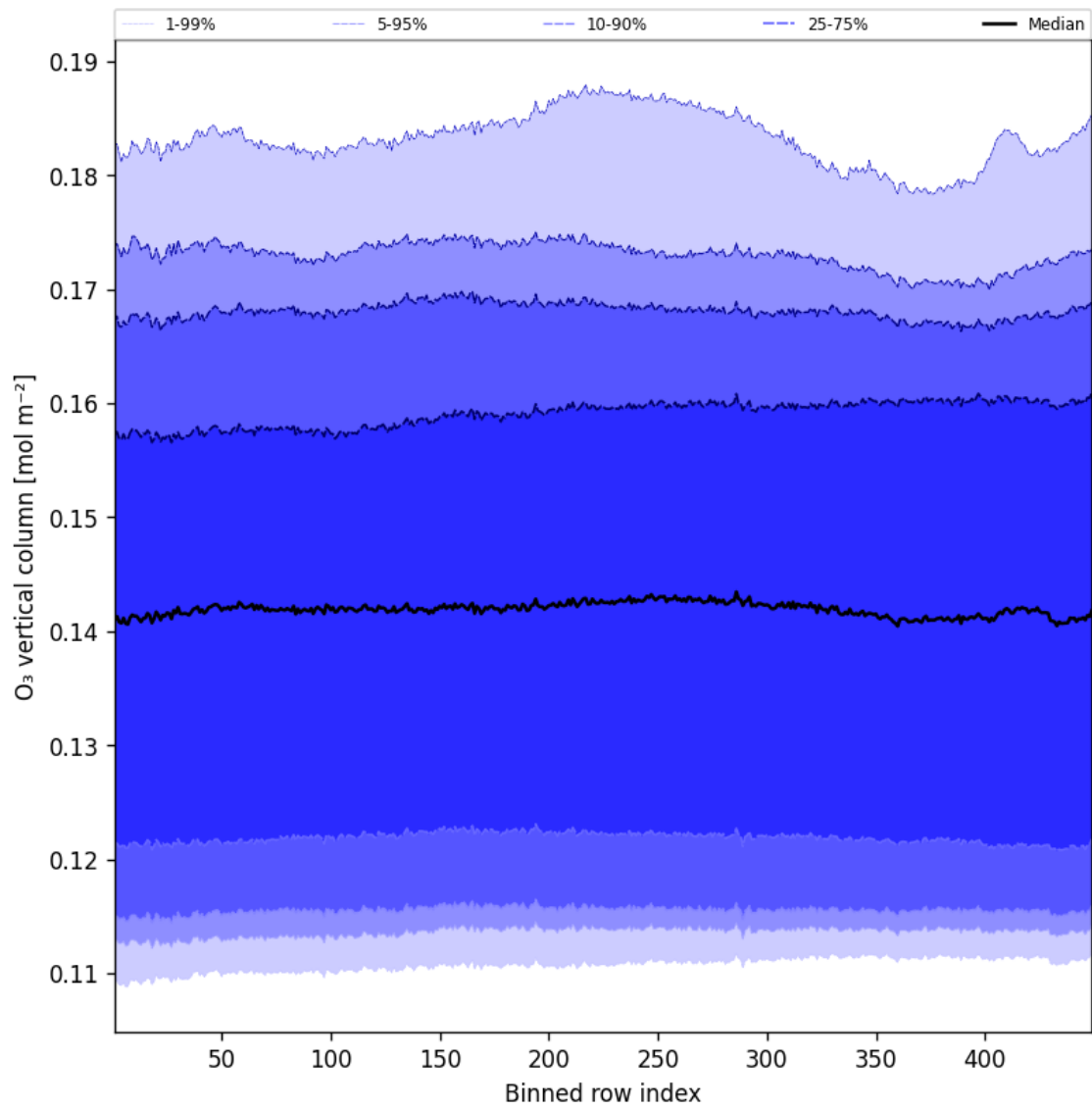
Figure 41: Along track statistics of “O 3 vertical column” for 2025-05-24 to 2025-05-24
