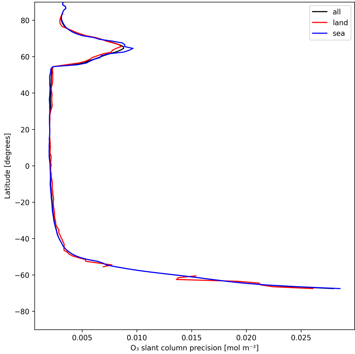
Figure 20: Zonal average of “O 3 slant column precision” for 2025-05-24 to 2025-05-24.
