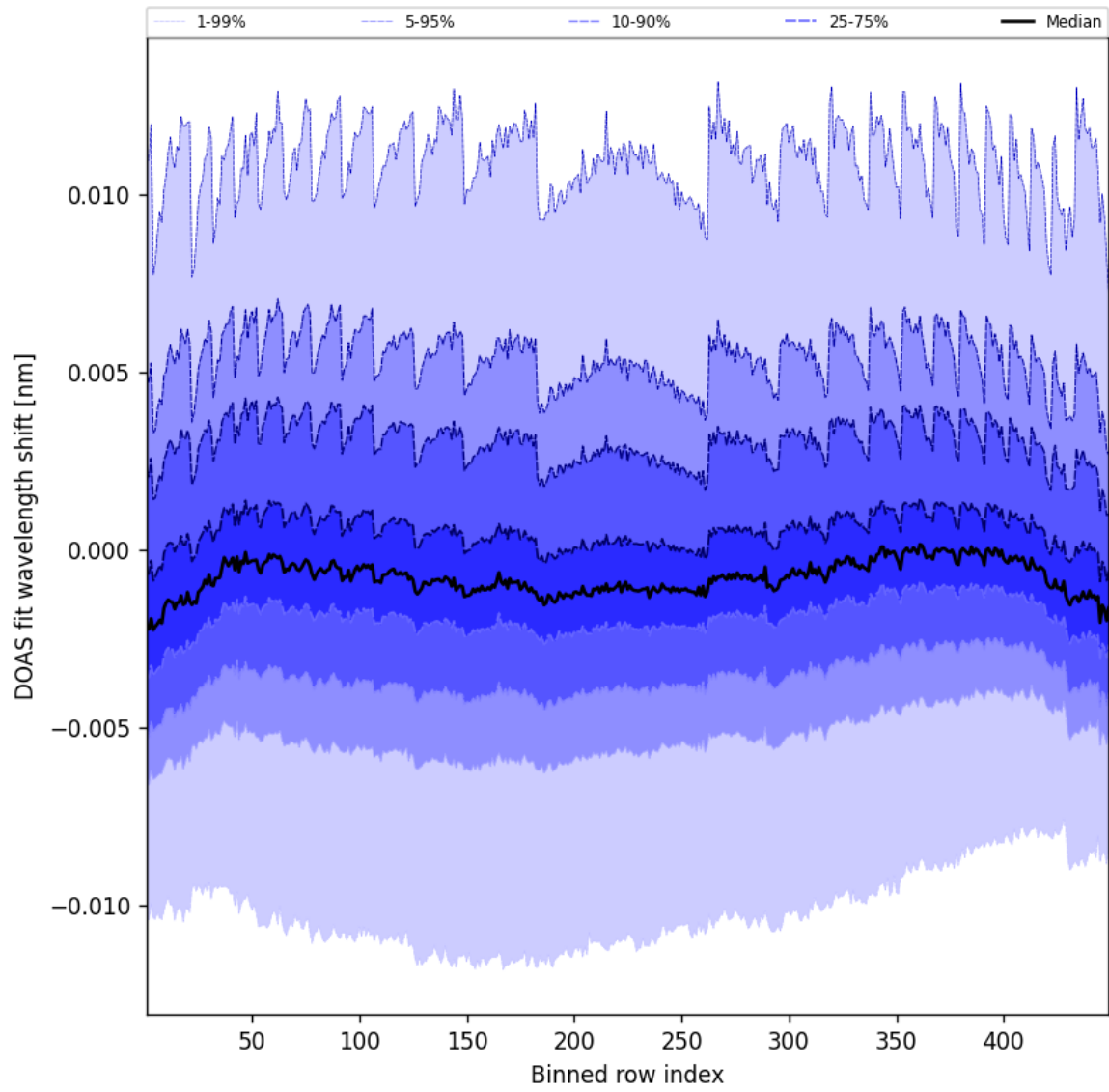
Figure 47: Along track statistics of “DOAS fit wavelength shift” for 2025-05-24 to 2025-05-24
