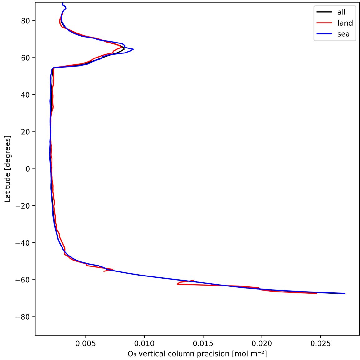
Figure 18: Zonal average of “O 3 vertical column precision” for 2025-05-24 to 2025-05-24.
