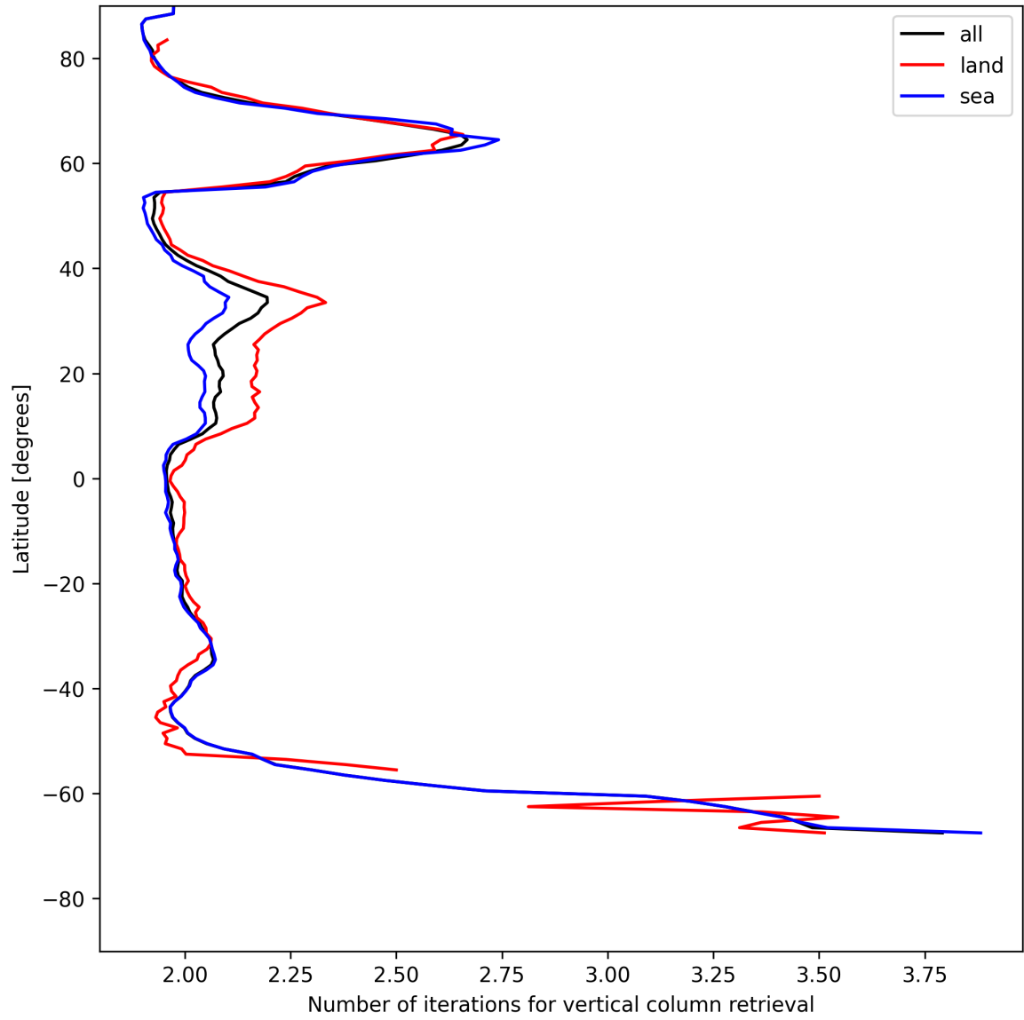
Figure 27: Zonal average of “Number of iterations for vertical column retrieval” for 2025-05-24 to 2025-05-24.
