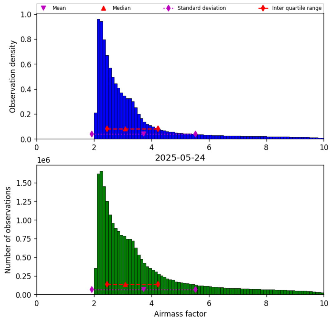
Figure 37: Histogram of “Airmass factor” for 2025-05-24 to 2025-05-24
