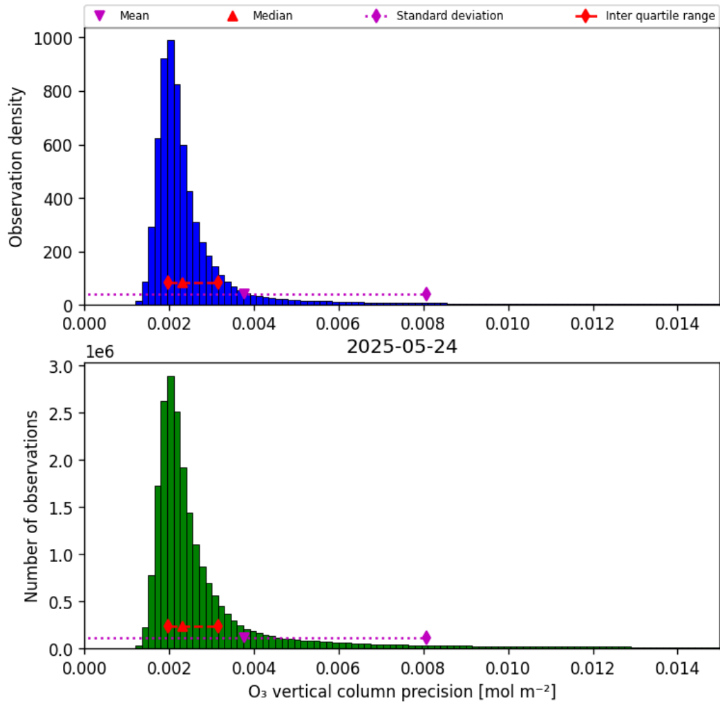
Figure 30: Histogram of “O 3 vertical column precision” for 2025-05-24 to 2025-05-24
