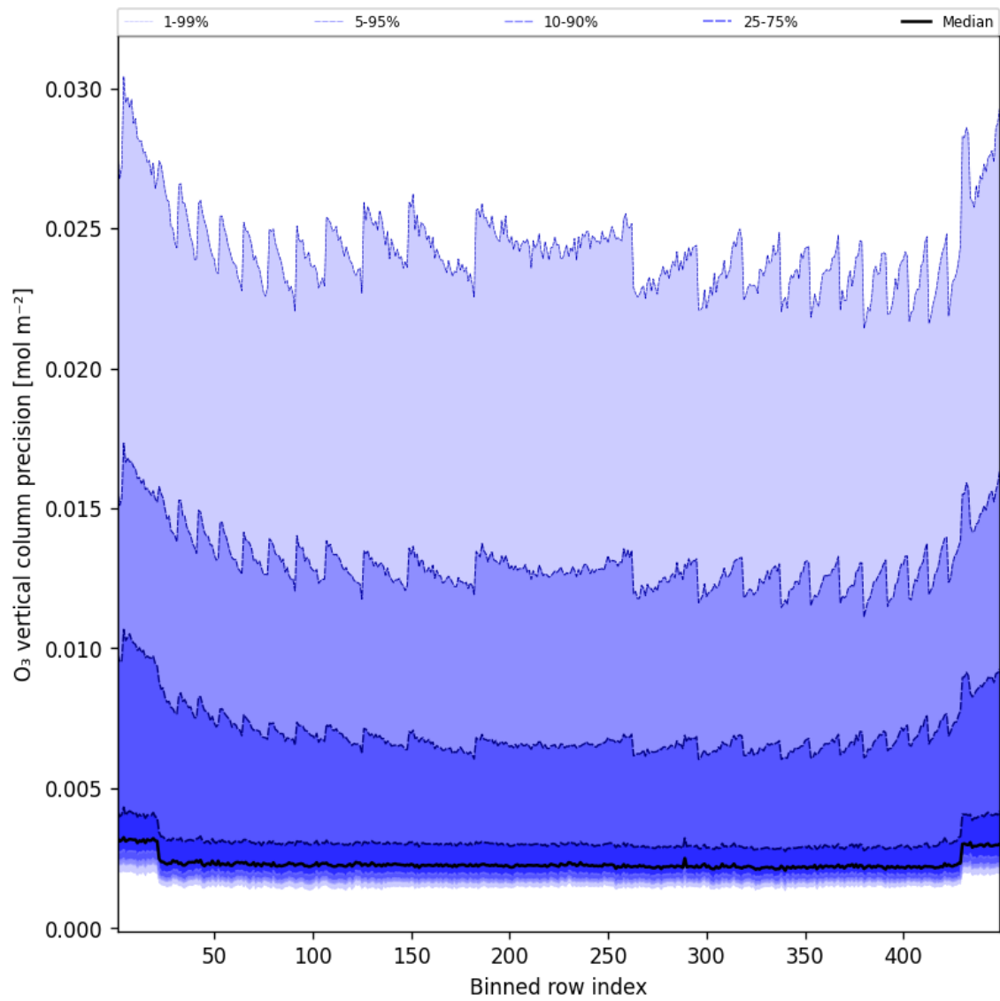
Figure 42: Along track statistics of “O 3 vertical column precision” for 2025-05-24 to 2025-05-24
