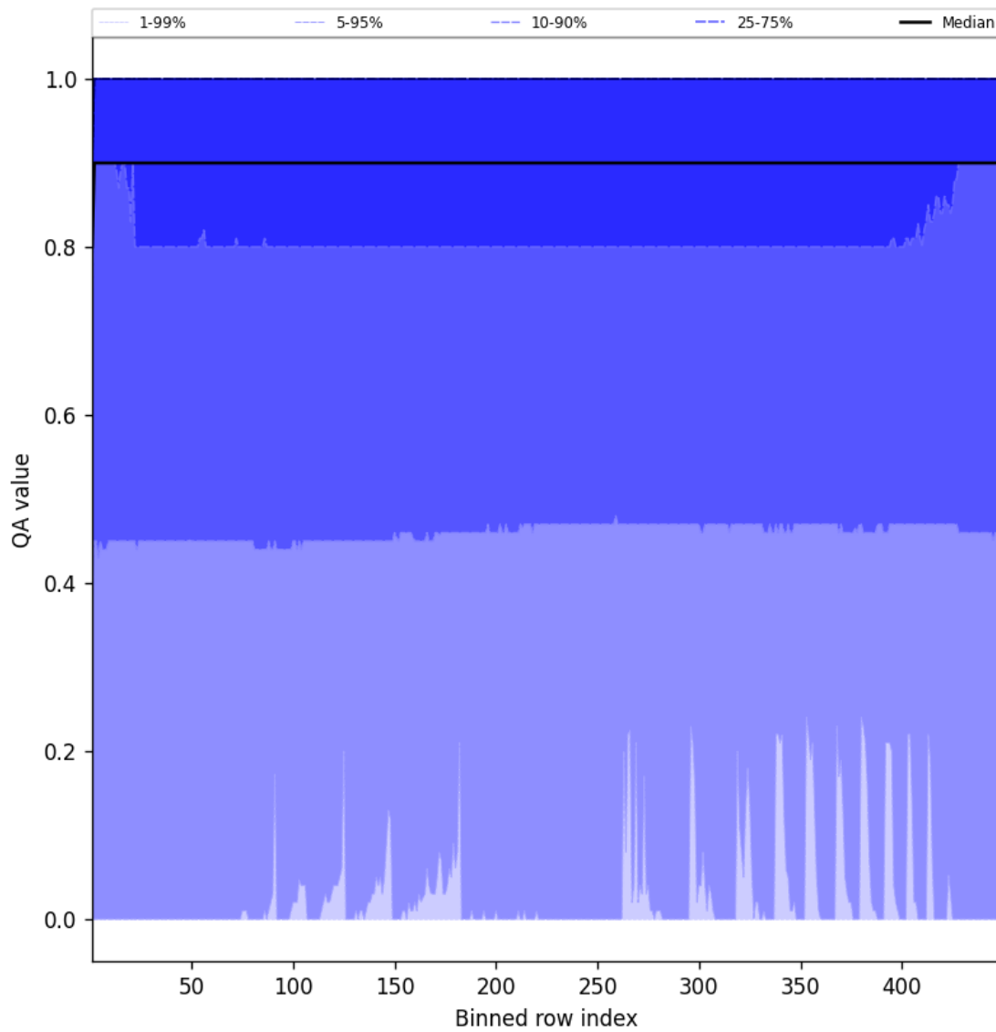
Figure 40: Along track statistics of “QA value” for 2025-05-24 to 2025-05-24
