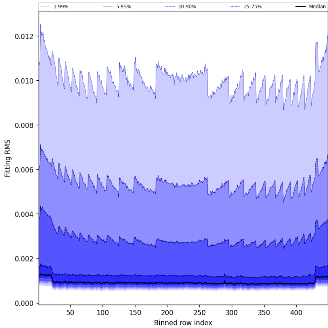
Figure 46: Along track statistics of “Fitting RMS” for 2025-05-24 to 2025-05-24
