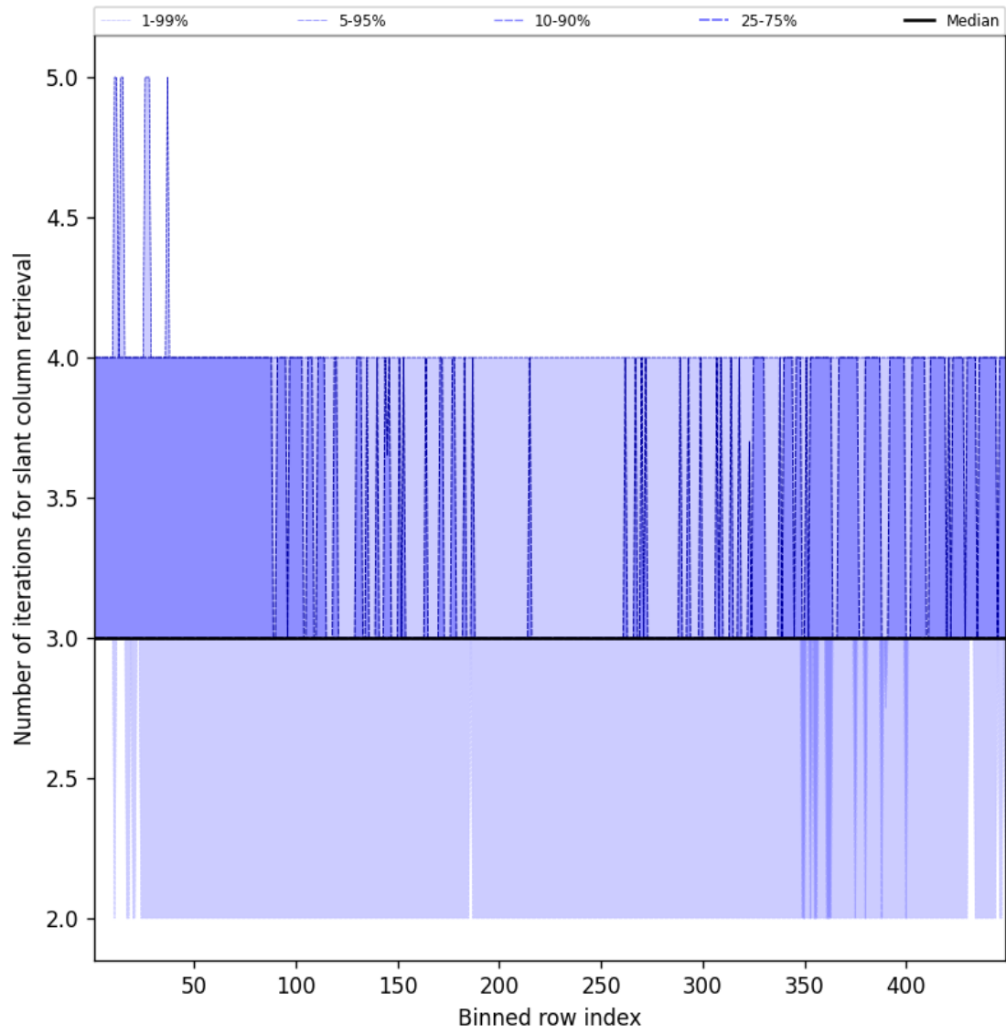
Figure 45: Along track statistics of “Number of iterations for slant column retrieval” for 2025-05-24 to 2025-05-24
