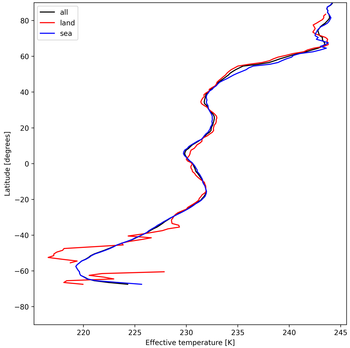
Figure 26: Zonal average of “Effective temperature” for 2025-05-24 to 2025-05-24.
