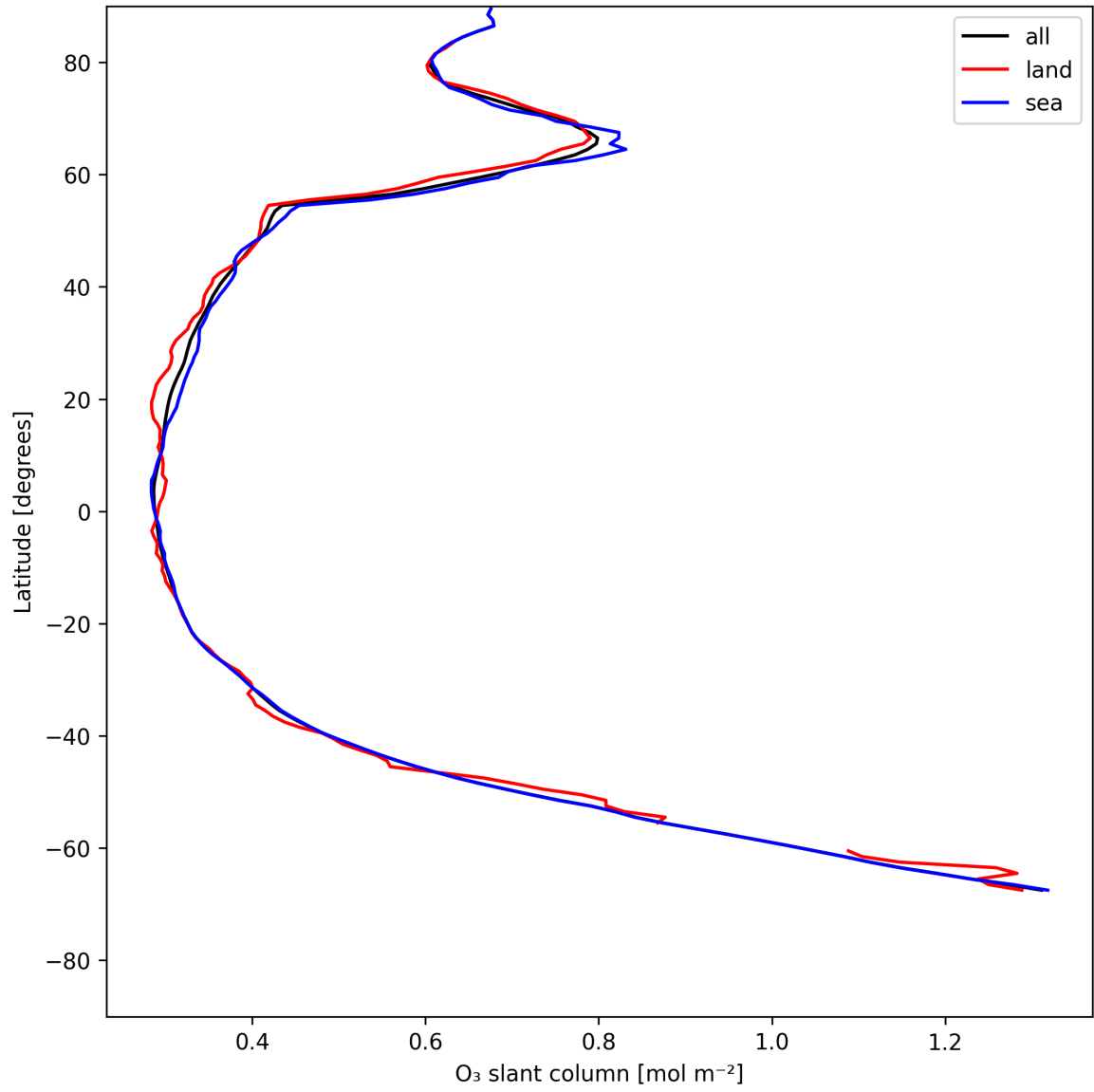
Figure 19: Zonal average of “O 3 slant column” for 2025-05-24 to 2025-05-24.
