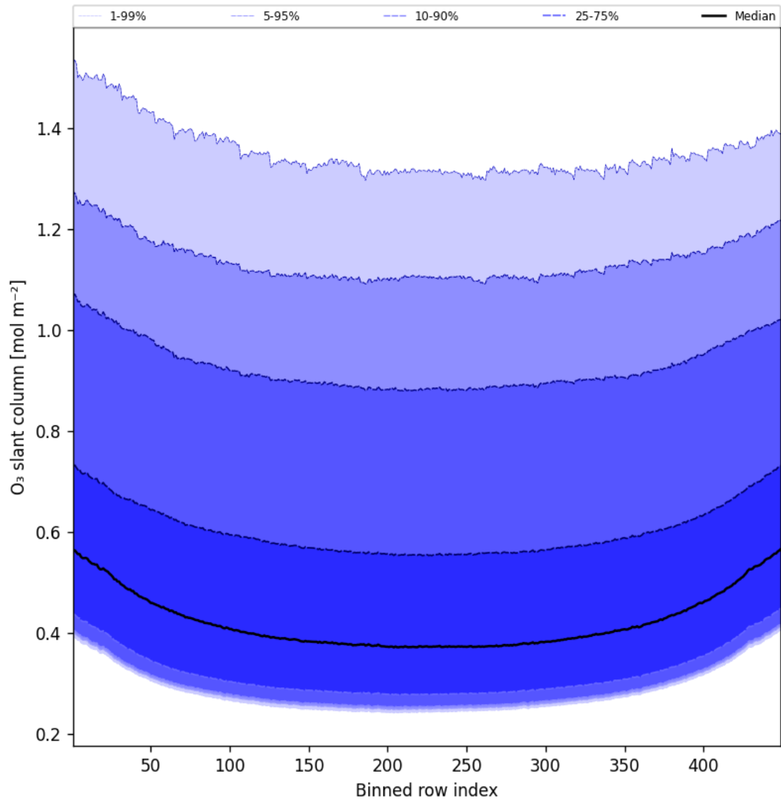
Figure 43: Along track statistics of “O 3 slant column” for 2025-05-24 to 2025-05-24
