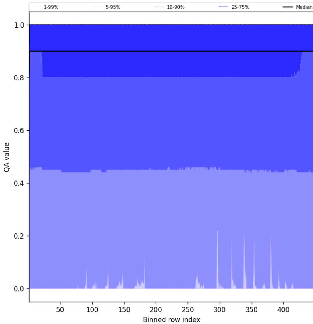
Figure 40: Along track statistics of “QA value” for 2025-05-25 to 2025-05-26
