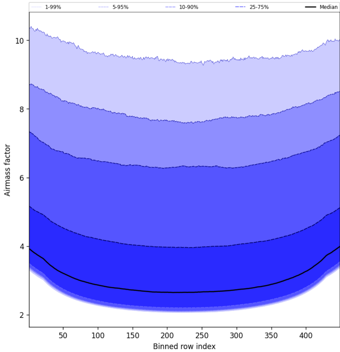
Figure 49: Along track statistics of “Airmass factor” for 2025-05-25 to 2025-05-26
