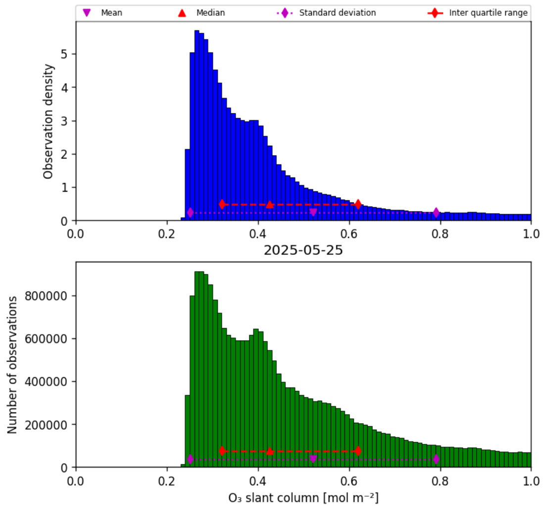
Figure 31: Histogram of “O 3 slant column” for 2025-05-25 to 2025-05-26
