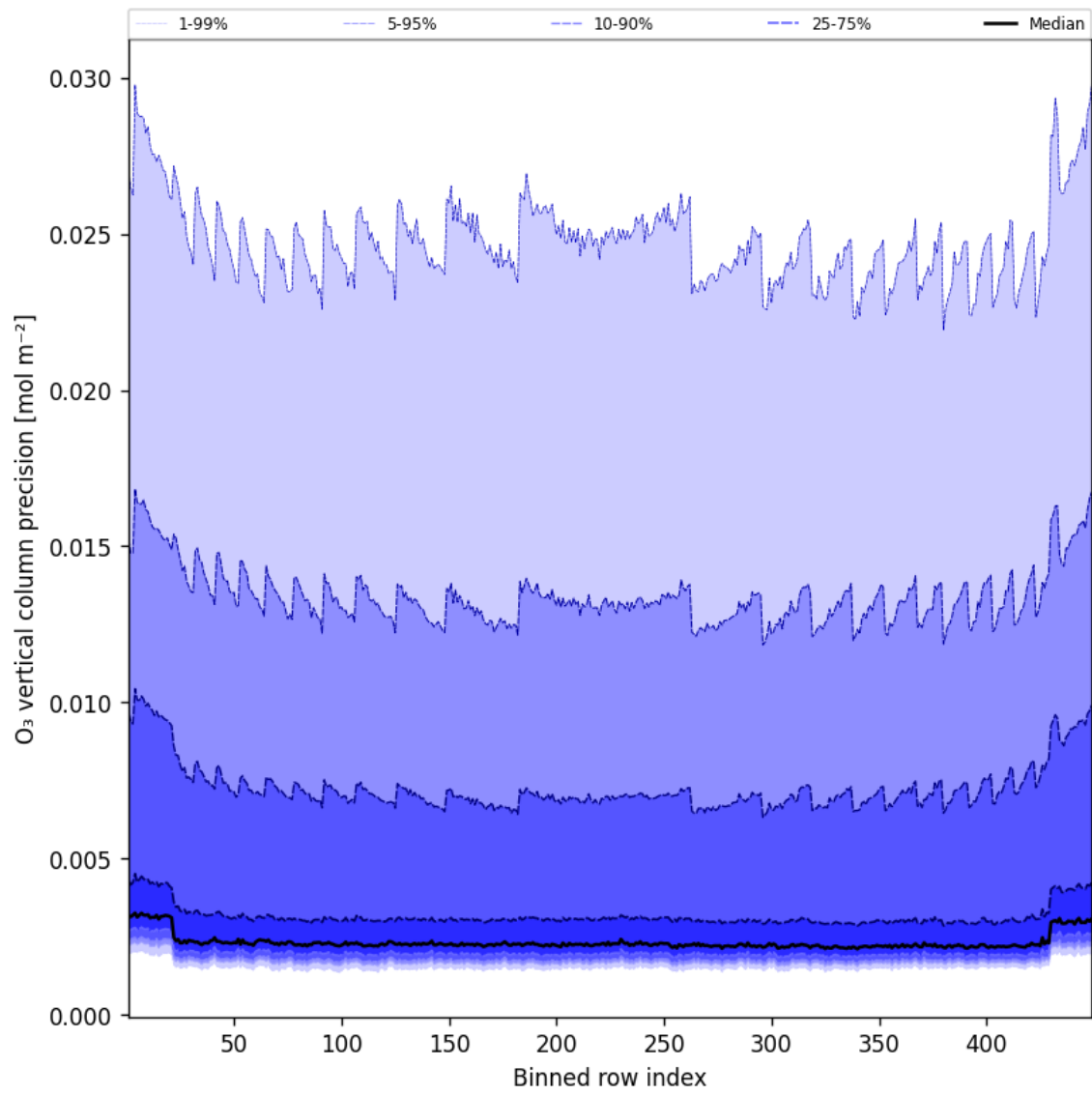
Figure 42: Along track statistics of “O 3 vertical column precision” for 2025-05-25 to 2025-05-26
