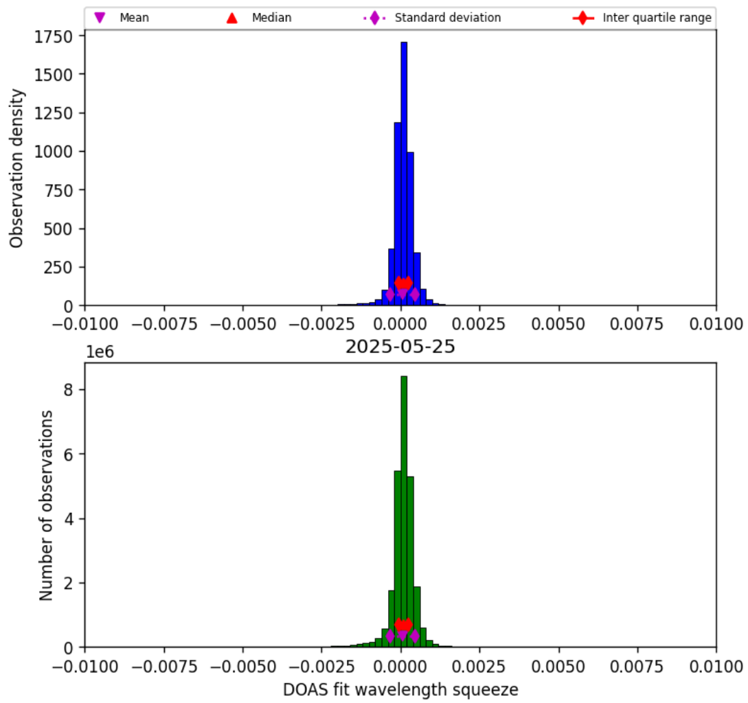
Figure 36: Histogram of “DOAS fit wavelength squeeze” for 2025-05-25 to 2025-05-26
