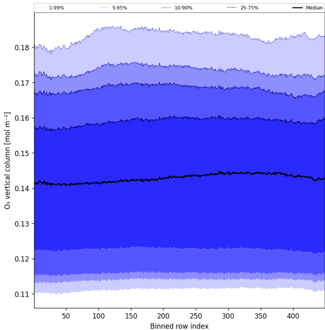
Figure 41: Along track statistics of “O 3 vertical column” for 2025-05-25 to 2025-05-26
