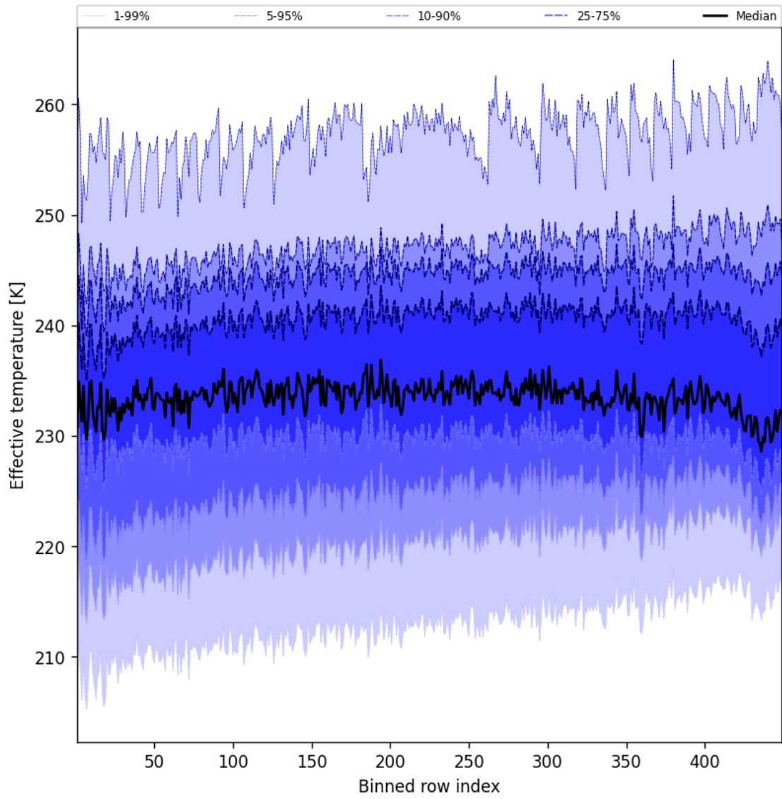
Figure 50: Along track statistics of "Effective temperature" for 2025-05-25 to 2025-05-26
