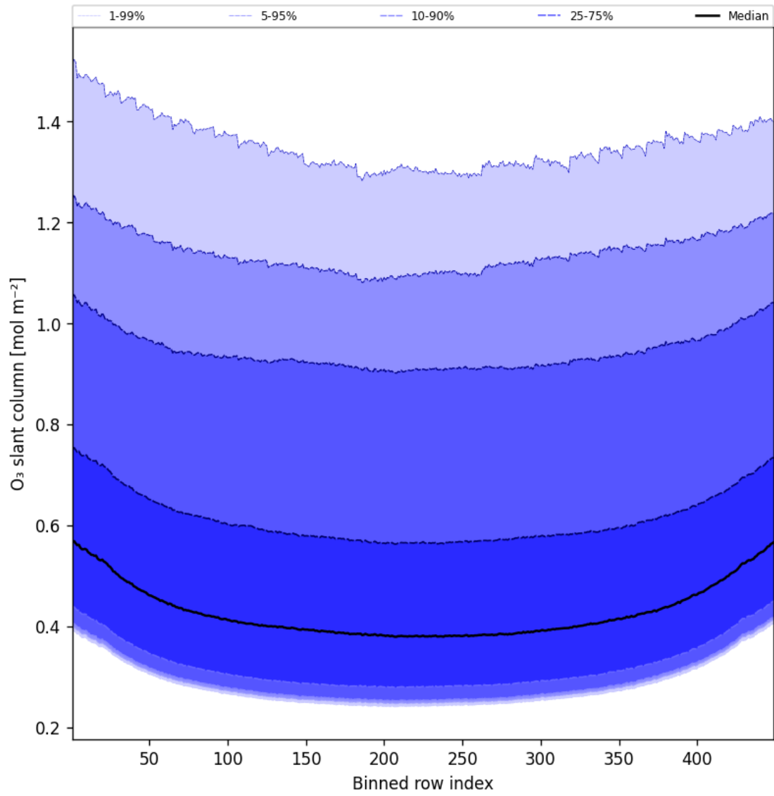
Figure 43: Along track statistics of “O 3 slant column” for 2025-05-25 to 2025-05-26
