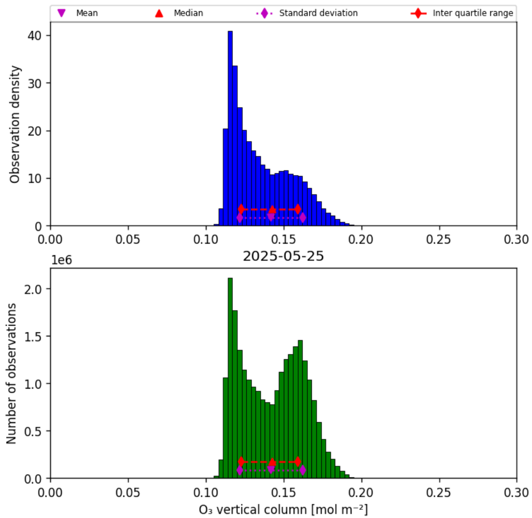
Figure 29: Histogram of “O 3 vertical column” for 2025-05-25 to 2025-05-26
