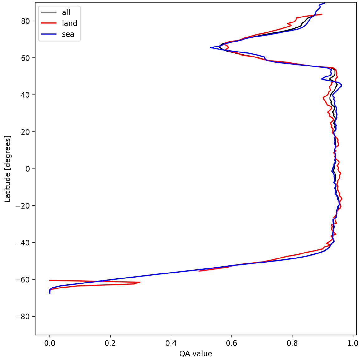
Figure 16: Zonal average of “QA value” for 2025-05-25 to 2025-05-26.
