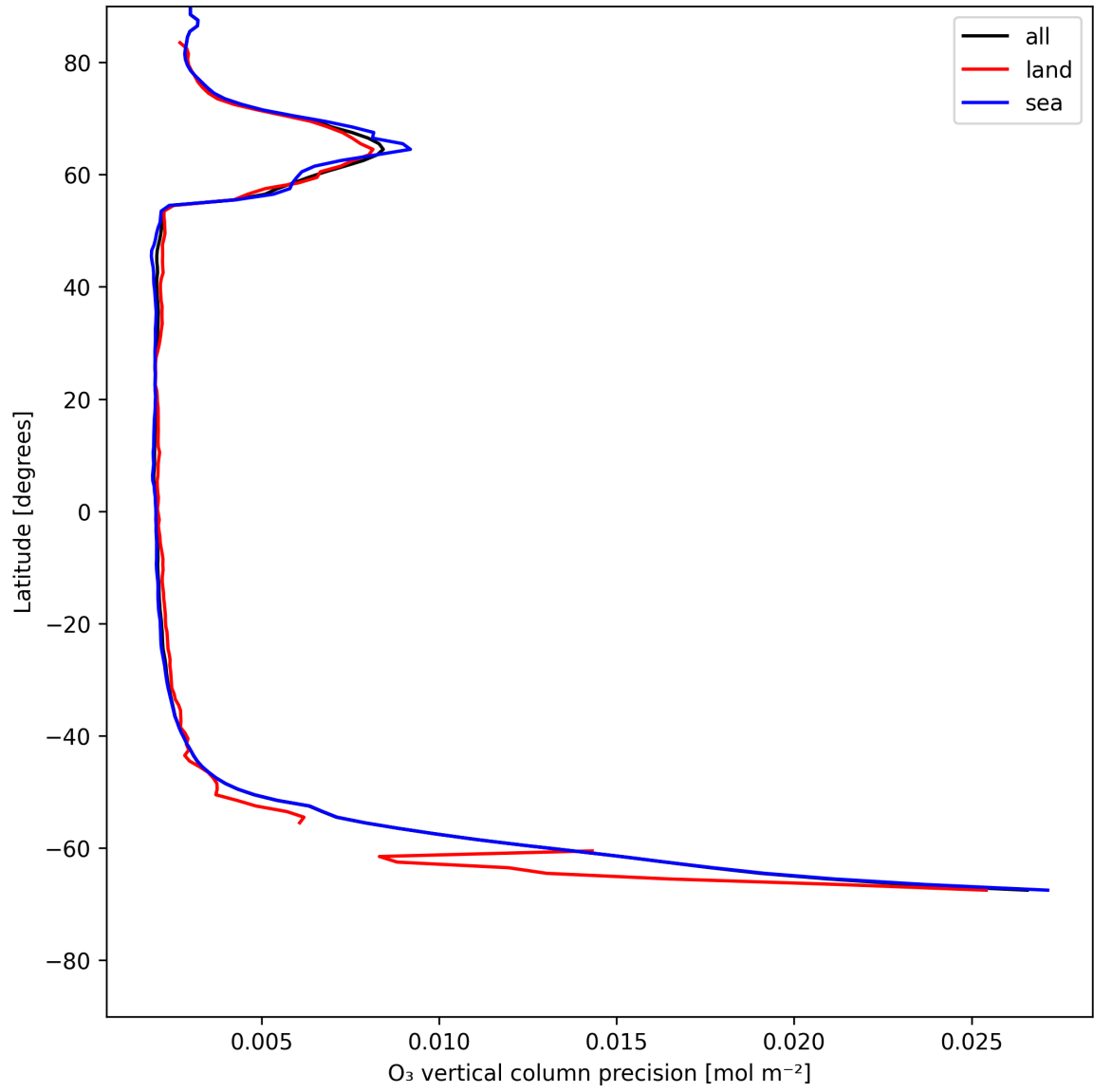
Figure 18: Zonal average of “O 3 vertical column precision” for 2025-05-25 to 2025-05-26.
