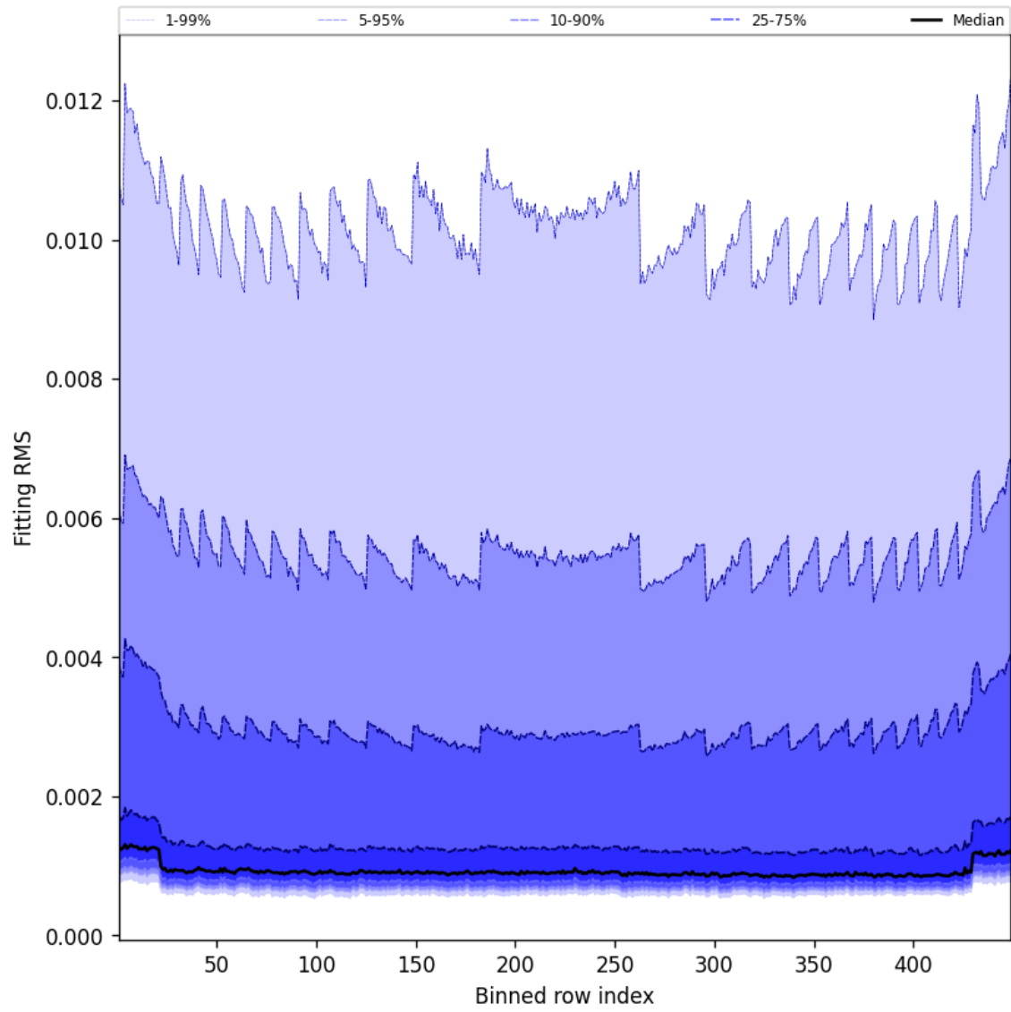
Figure 46: Along track statistics of “Fitting RMS” for 2025-05-25 to 2025-05-26
