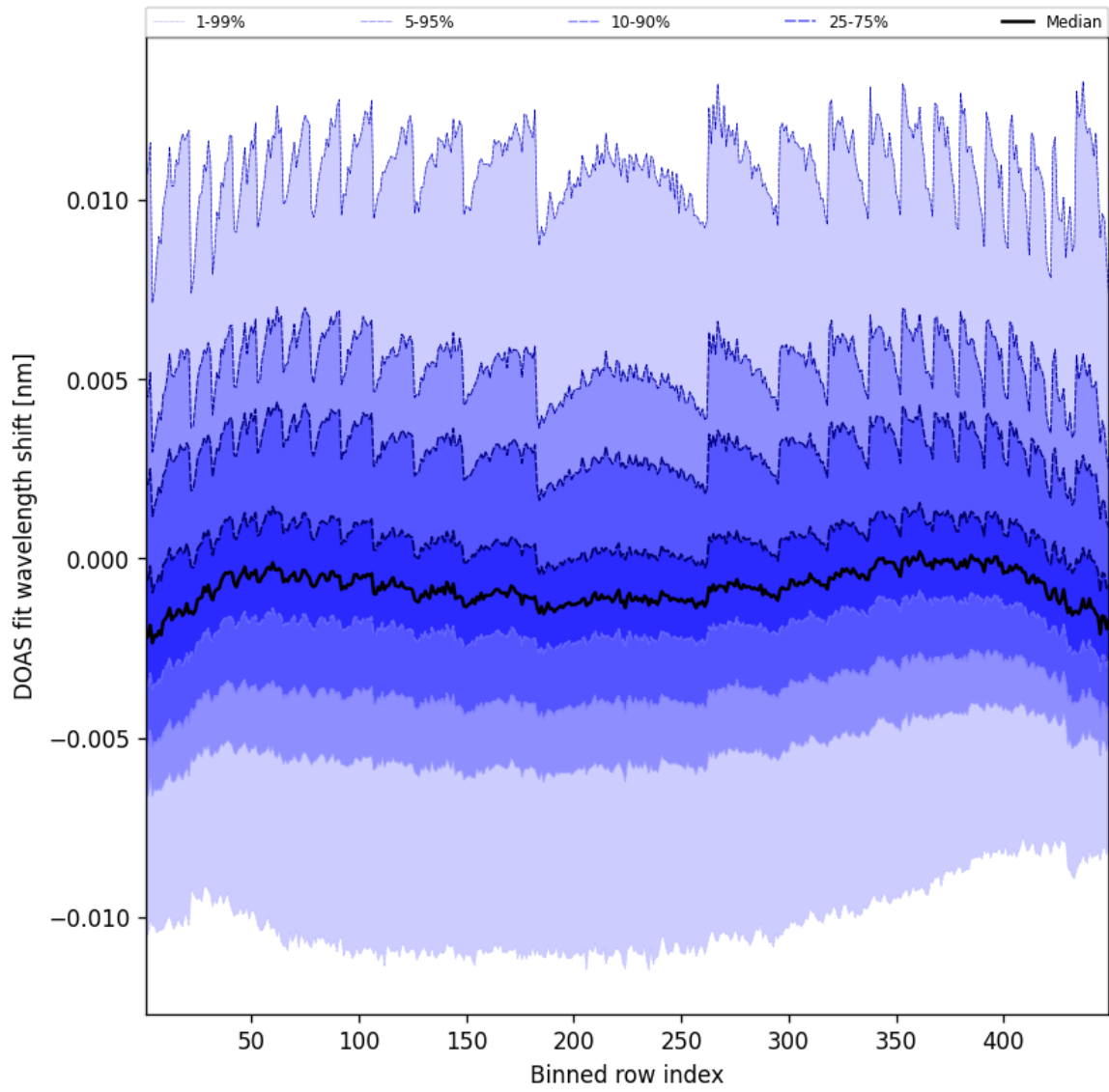
Figure 47: Along track statistics of “DOAS fit wavelength shift” for 2025-05-25 to 2025-05-26
