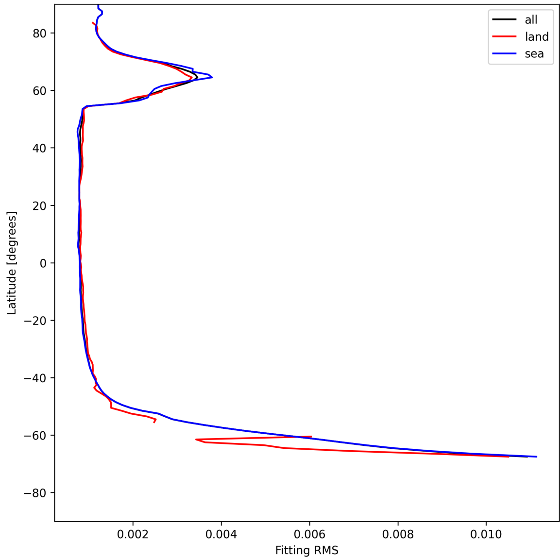
Figure 22: Zonal average of “Fitting RMS” for 2025-05-25 to 2025-05-26.
