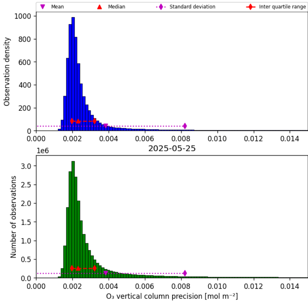
Figure 30: Histogram of “O 3 vertical column precision” for 2025-05-25 to 2025-05-26
