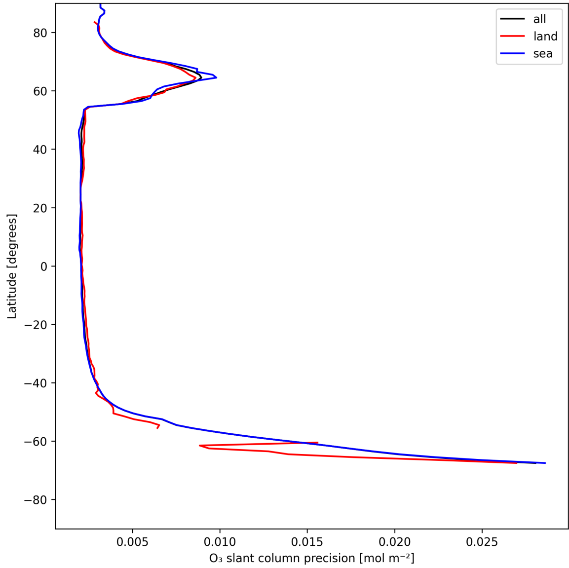
Figure 20: Zonal average of “O 3 slant column precision” for 2025-05-25 to 2025-05-26.
