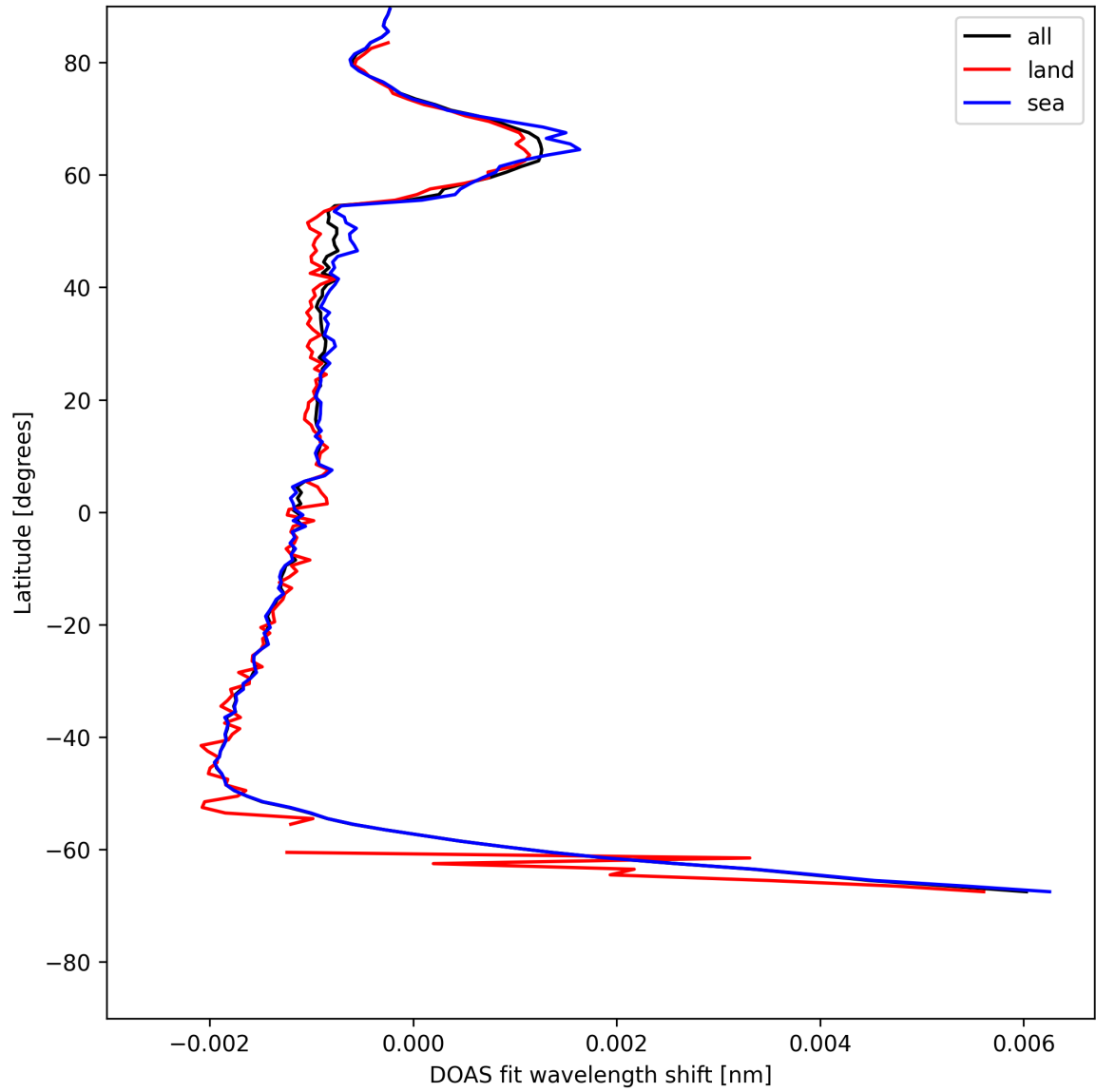
Figure 23: Zonal average of “DOAS fit wavelength shift” for 2025-05-25 to 2025-05-26.
