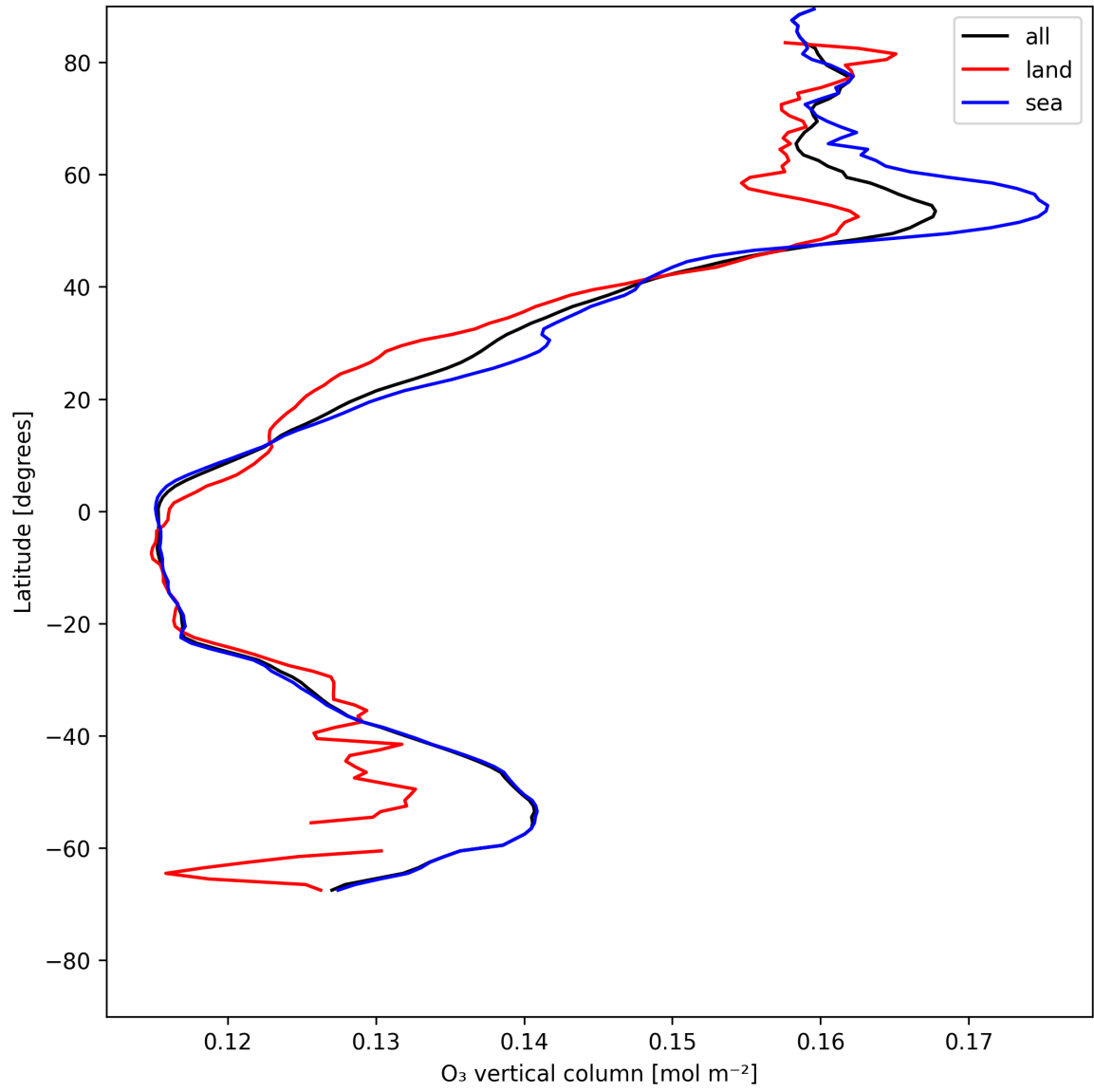
Figure 17: Zonal average of “O 3 vertical column” for 2025-05-25 to 2025-05-26.
