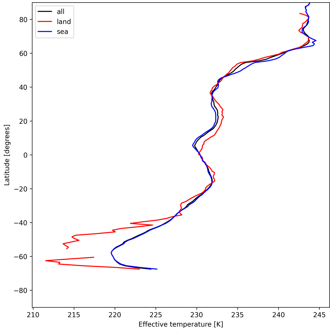
Figure 26: Zonal average of "Effective temperature" for 2025-05-25 to 2025-05-26.
