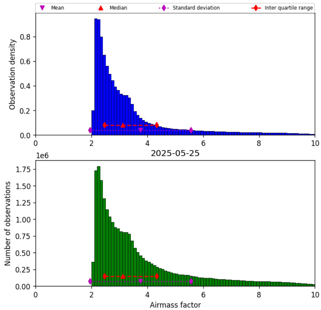
Figure 37: Histogram of “Airmass factor” for 2025-05-25 to 2025-05-26
