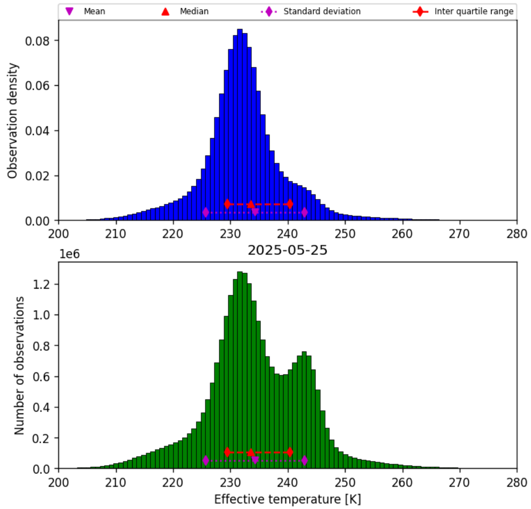
Figure 38: Histogram of “Effective temperature” for 2025-05-25 to 2025-05-26
