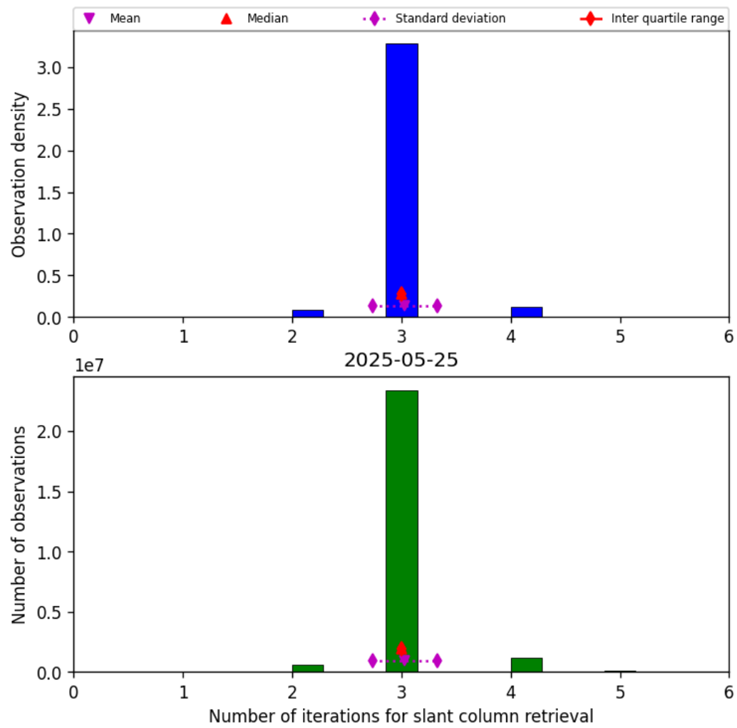
Figure 33: Histogram of “Number of iterations for slant column retrieval” for 2025-05-25 to 2025-05-26
