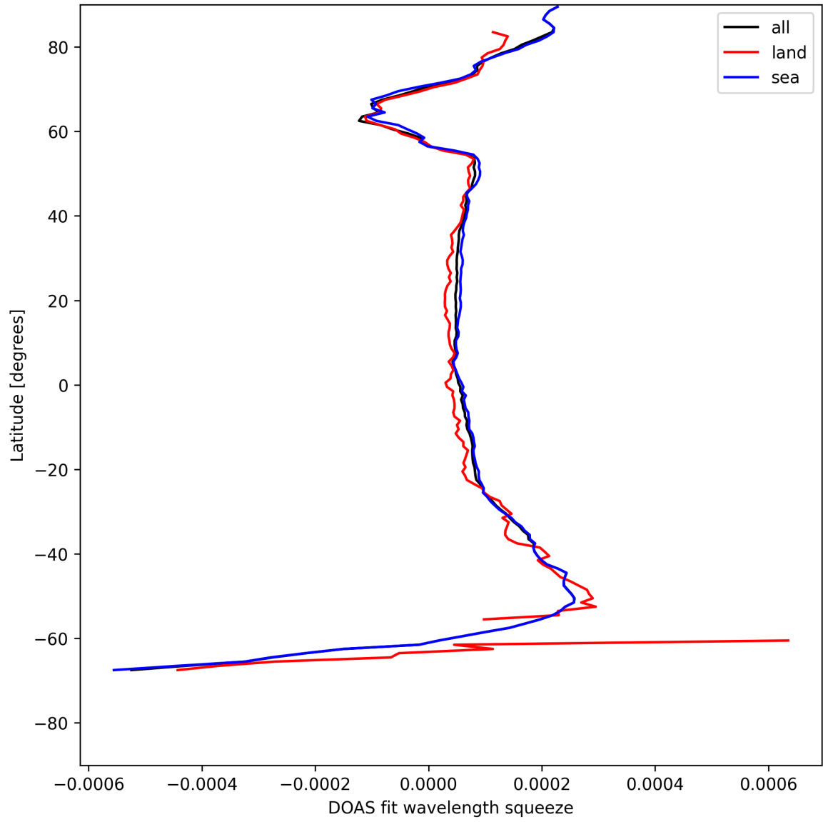
Figure 24: Zonal average of “DOAS fit wavelength squeeze” for 2025-05-25 to 2025-05-26.
