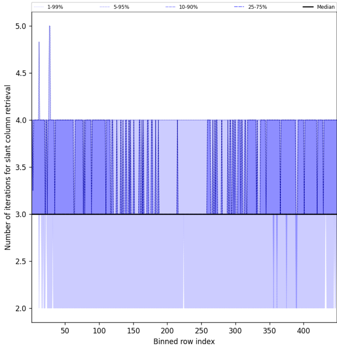
Figure 45: Along track statistics of “Number of iterations for slant column retrieval” for 2025-05-25 to 2025-05-26
