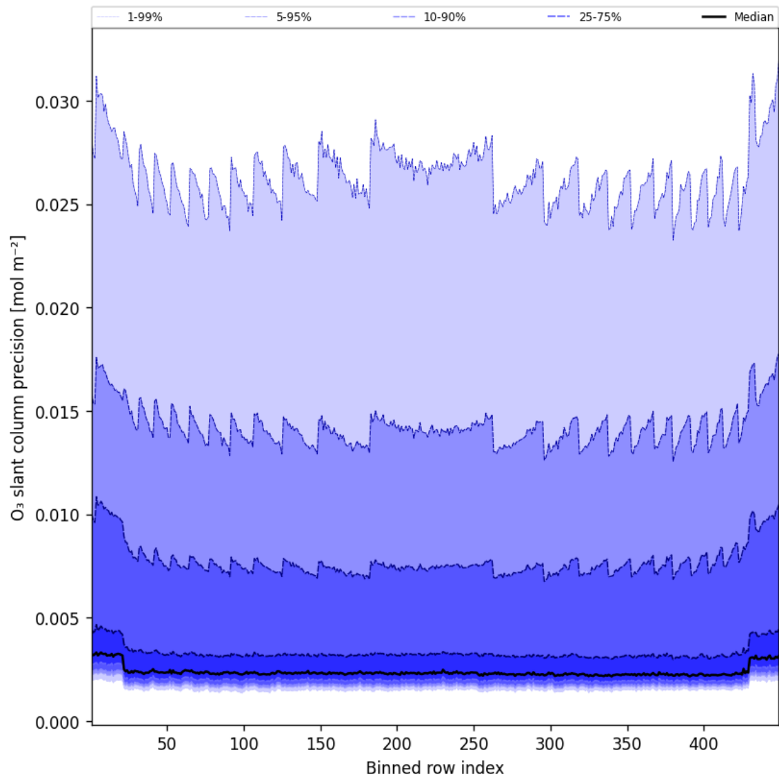
Figure 44: Along track statistics of “O 3 slant column precision” for 2025-05-25 to 2025-05-26
