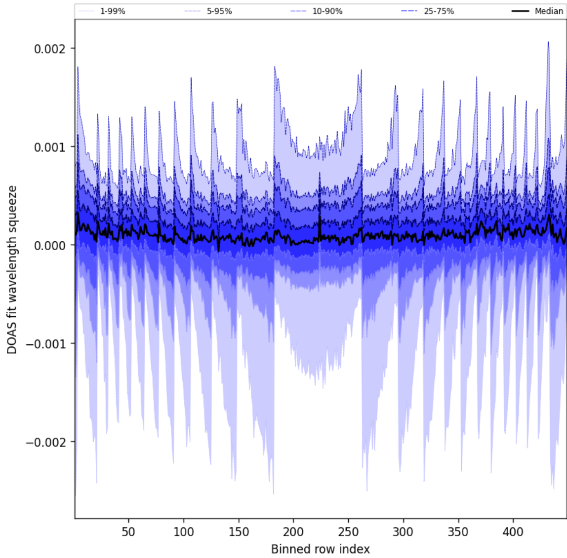
Figure 48: Along track statistics of “DOAS fit wavelength squeeze” for 2025-05-25 to 2025-05-26
