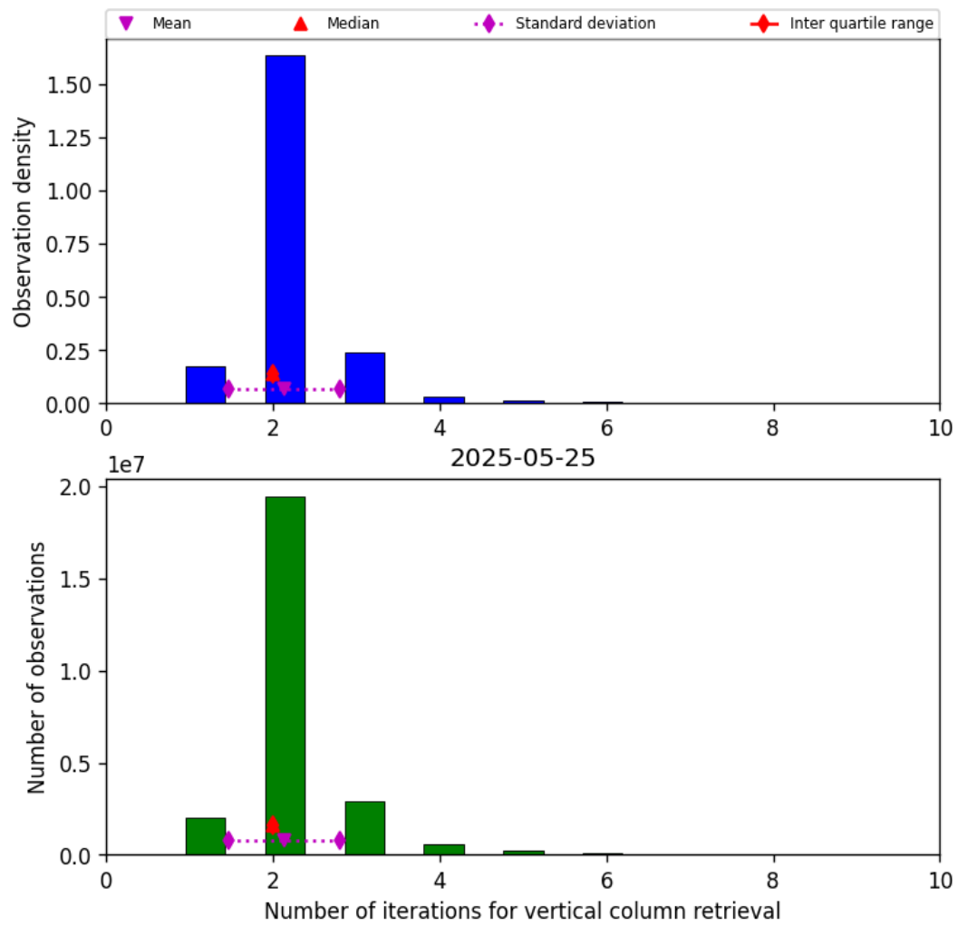
Figure 39: Histogram of “Number of iterations for vertical column retrieval” for 2025-05-25 to 2025-05-26
