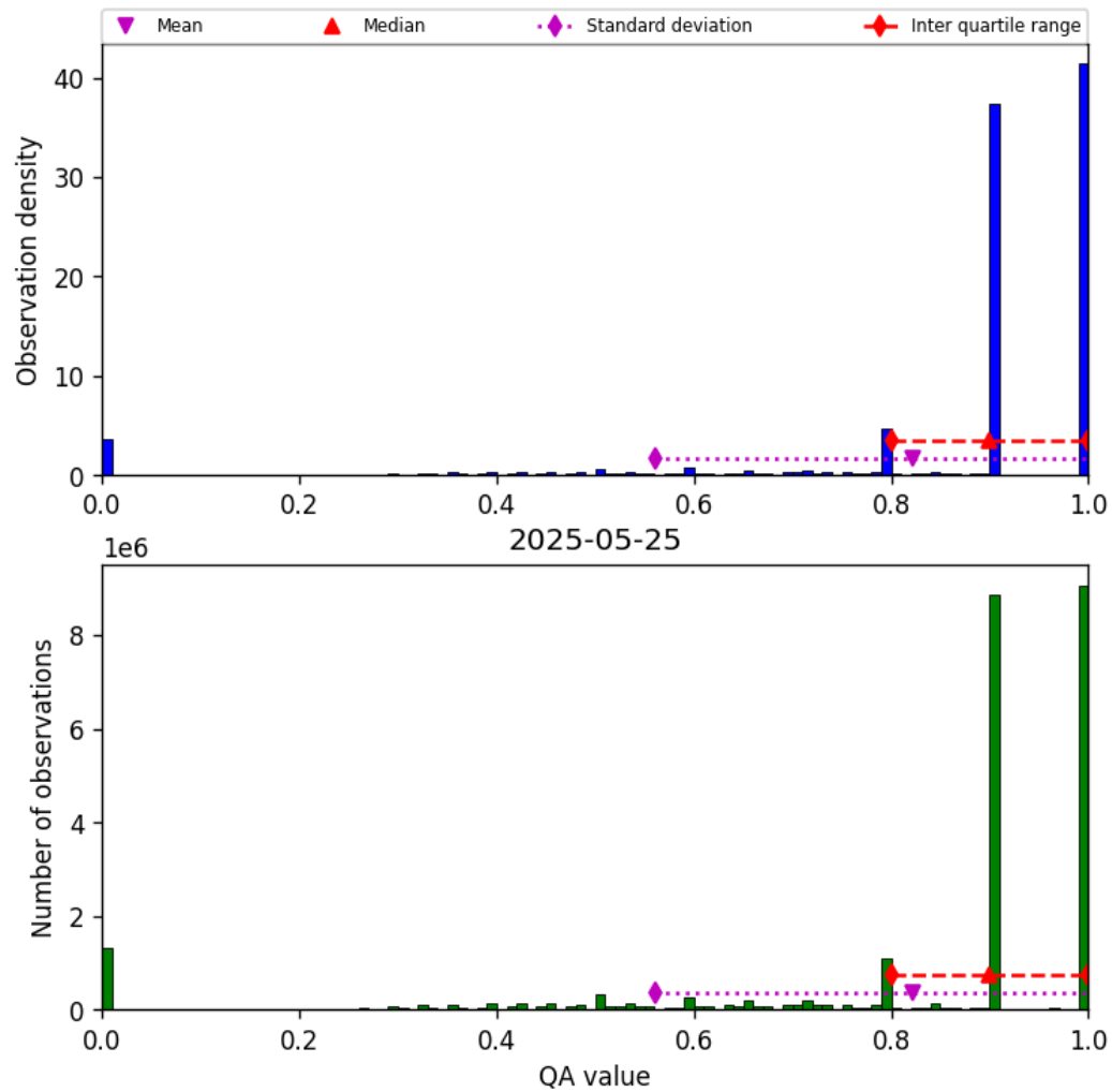
Figure 28: Histogram of “QA value” for 2025-05-25 to 2025-05-26
