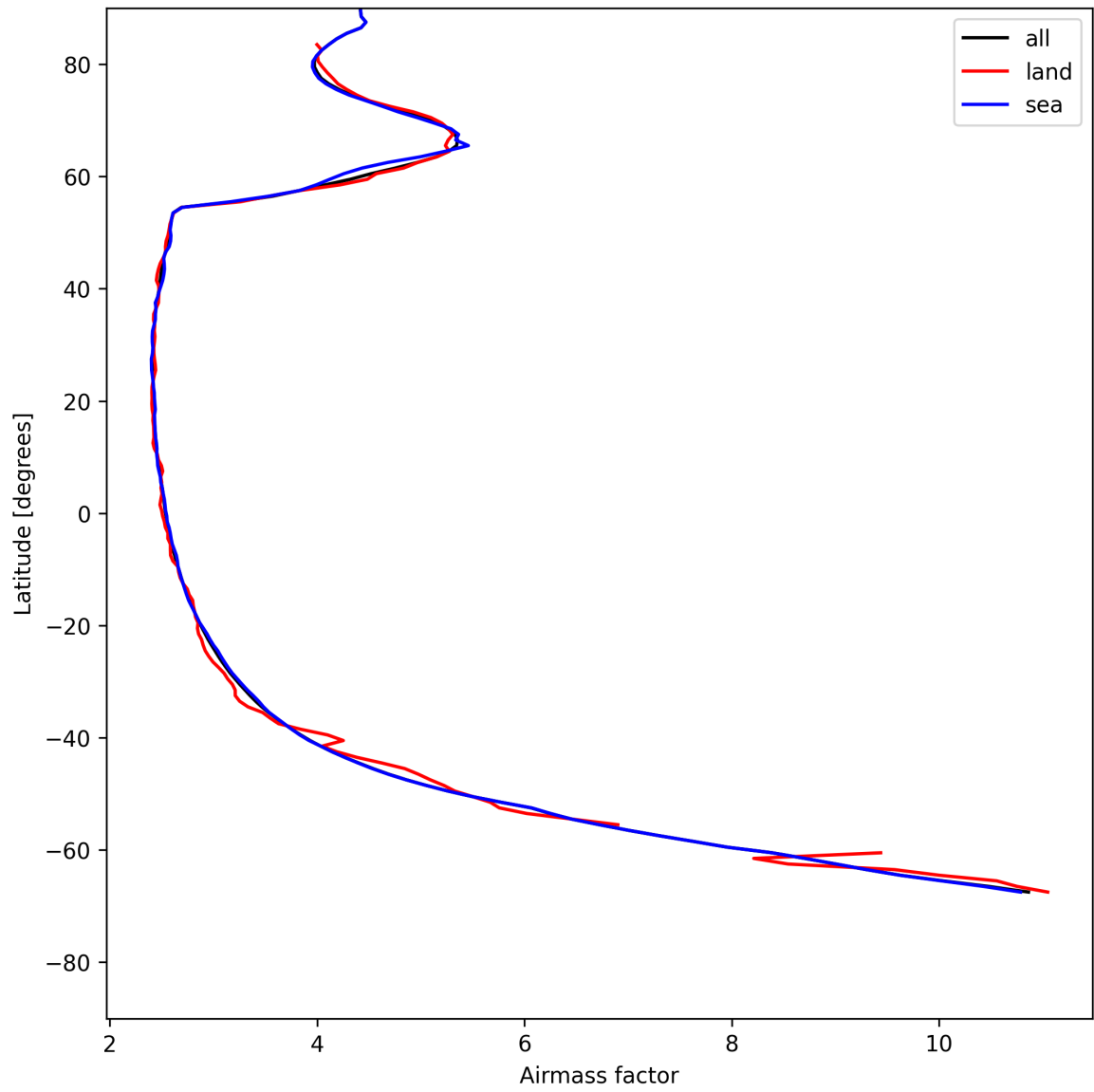
Figure 25: Zonal average of “Airmass factor” for 2025-05-25 to 2025-05-26.
