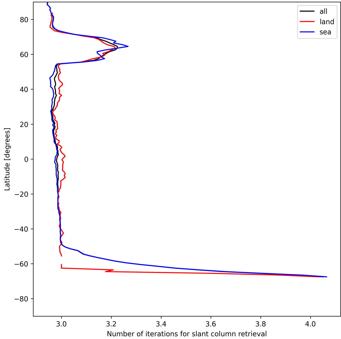
Figure 21: Zonal average of “Number of iterations for slant column retrieval” for 2025-05-25 to 2025-05-26.
