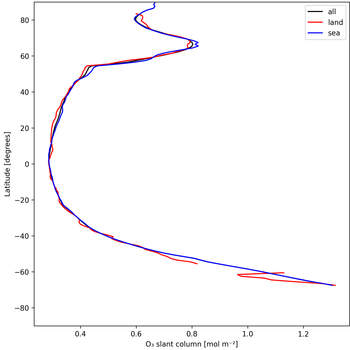
Figure 19: Zonal average of “O 3 slant column” for 2025-05-25 to 2025-05-26.
