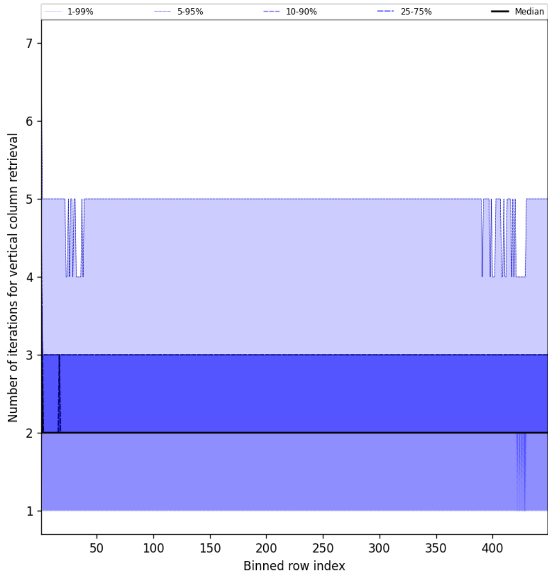
Figure 51: Along track statistics of “Number of iterations for vertical column retrieval” for 2025-05-25 to 2025-05-26
