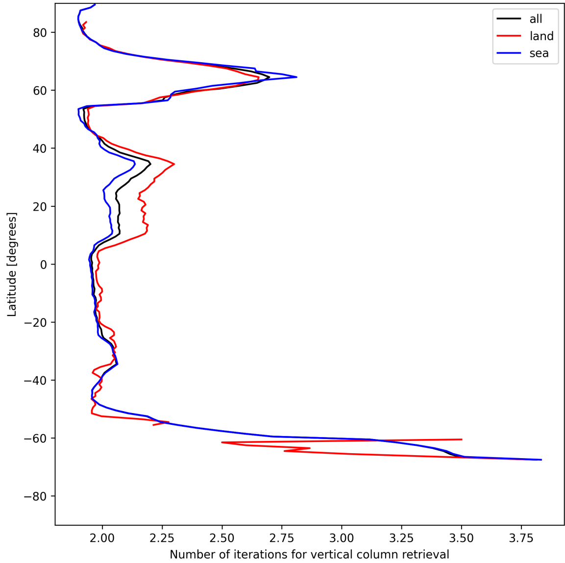
Figure 27: Zonal average of “Number of iterations for vertical column retrieval” for 2025-05-25 to 2025-05-26.
