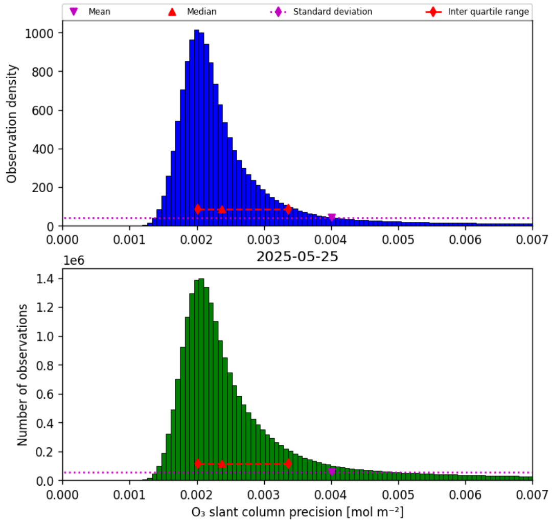
Figure 32: Histogram of “O 3 slant column precision” for 2025-05-25 to 2025-05-26
