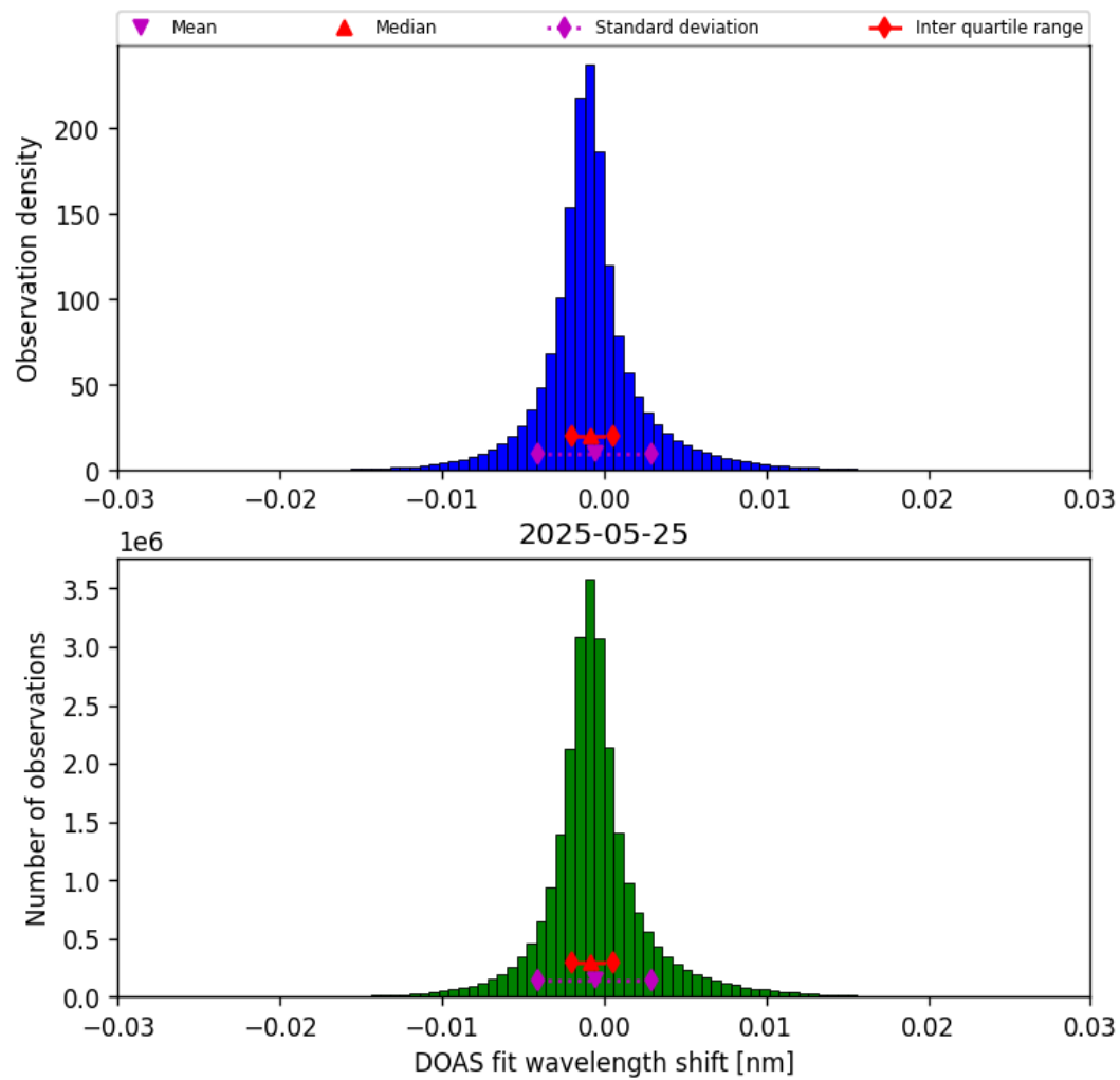
Figure 35: Histogram of “DOAS fit wavelength shift” for 2025-05-25 to 2025-05-26
