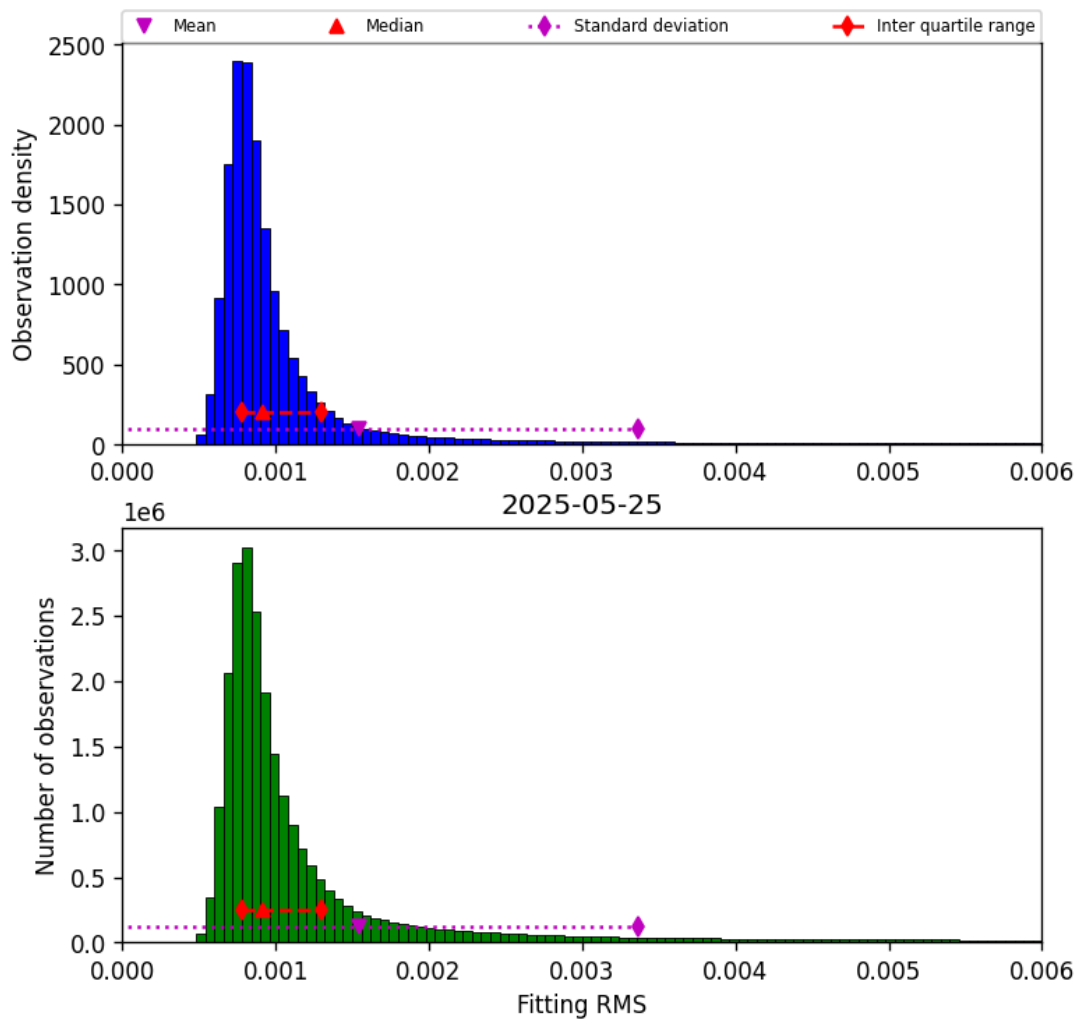
Figure 34: Histogram of “Fitting RMS” for 2025-05-25 to 2025-05-26
