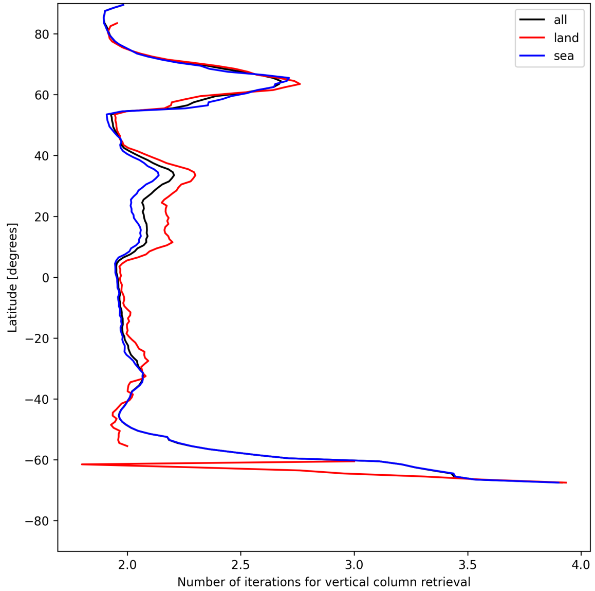
Figure 27: Zonal average of “Number of iterations for vertical column retrieval” for 2025-05-26 to 2025-05-27.
