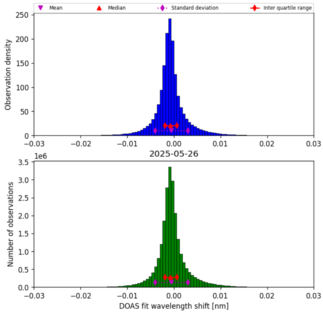
Figure 35: Histogram of “DOAS fit wavelength shift” for 2025-05-26 to 2025-05-27
