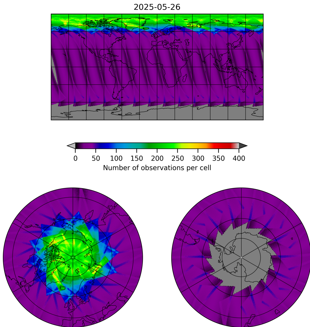
Figure 15: Map of the number of observations for 2025-05-26 to 2025-05-27
