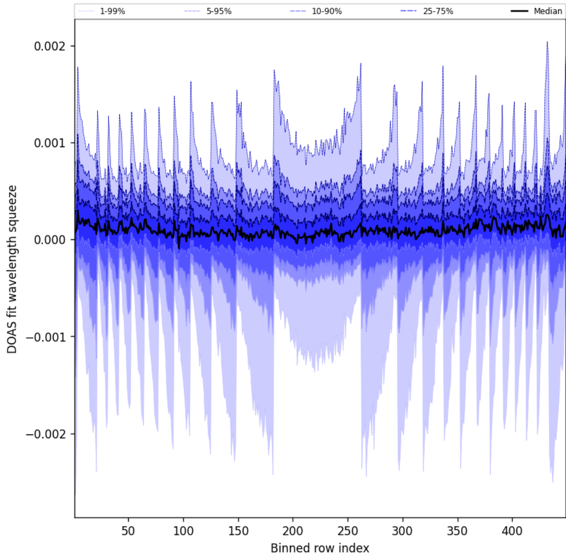
Figure 48: Along track statistics of “DOAS fit wavelength squeeze” for 2025-05-26 to 2025-05-27
