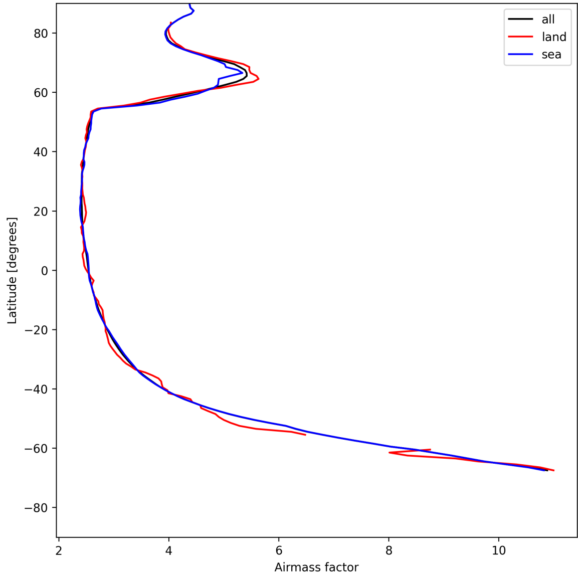
Figure 25: Zonal average of “Airmass factor” for 2025-05-26 to 2025-05-27.
