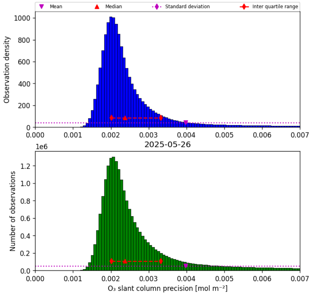
Figure 32: Histogram of “O 3 slant column precision” for 2025-05-26 to 2025-05-27
