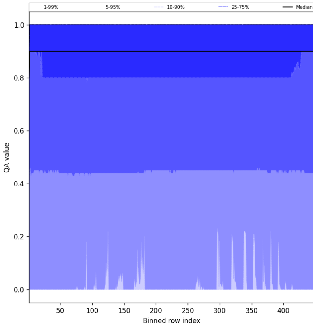
Figure 40: Along track statistics of “QA value” for 2025-05-26 to 2025-05-27
