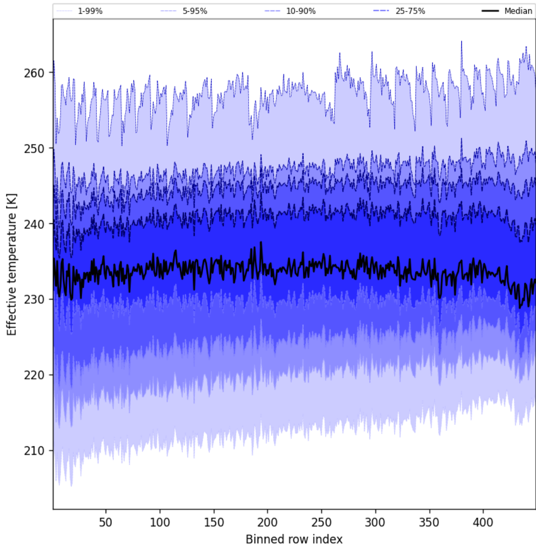
Figure 50: Along track statistics of “Effective temperature” for 2025-05-26 to 2025-05-27
