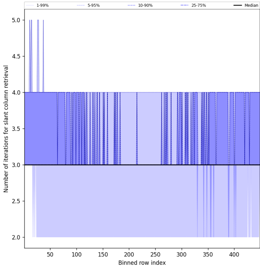
Figure 45: Along track statistics of “Number of iterations for slant column retrieval” for 2025-05-26 to 2025-05-27
