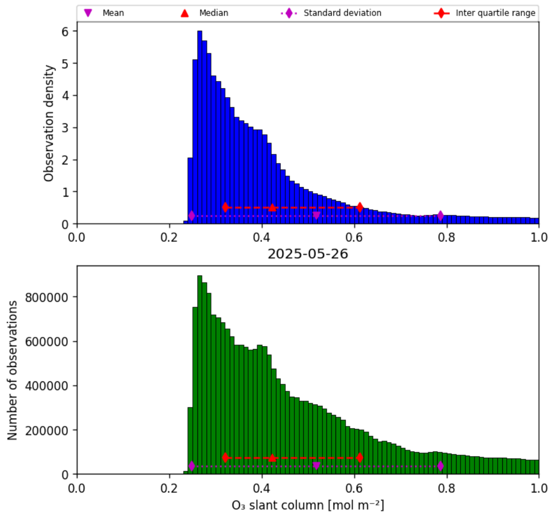
Figure 31: Histogram of “O 3 slant column” for 2025-05-26 to 2025-05-27
