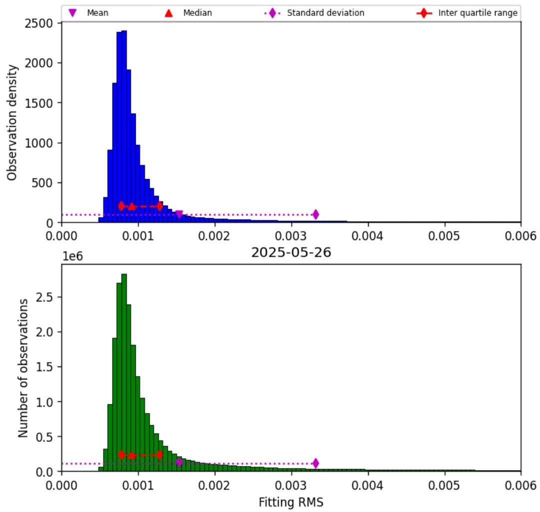
Figure 34: Histogram of “Fitting RMS” for 2025-05-26 to 2025-05-27
