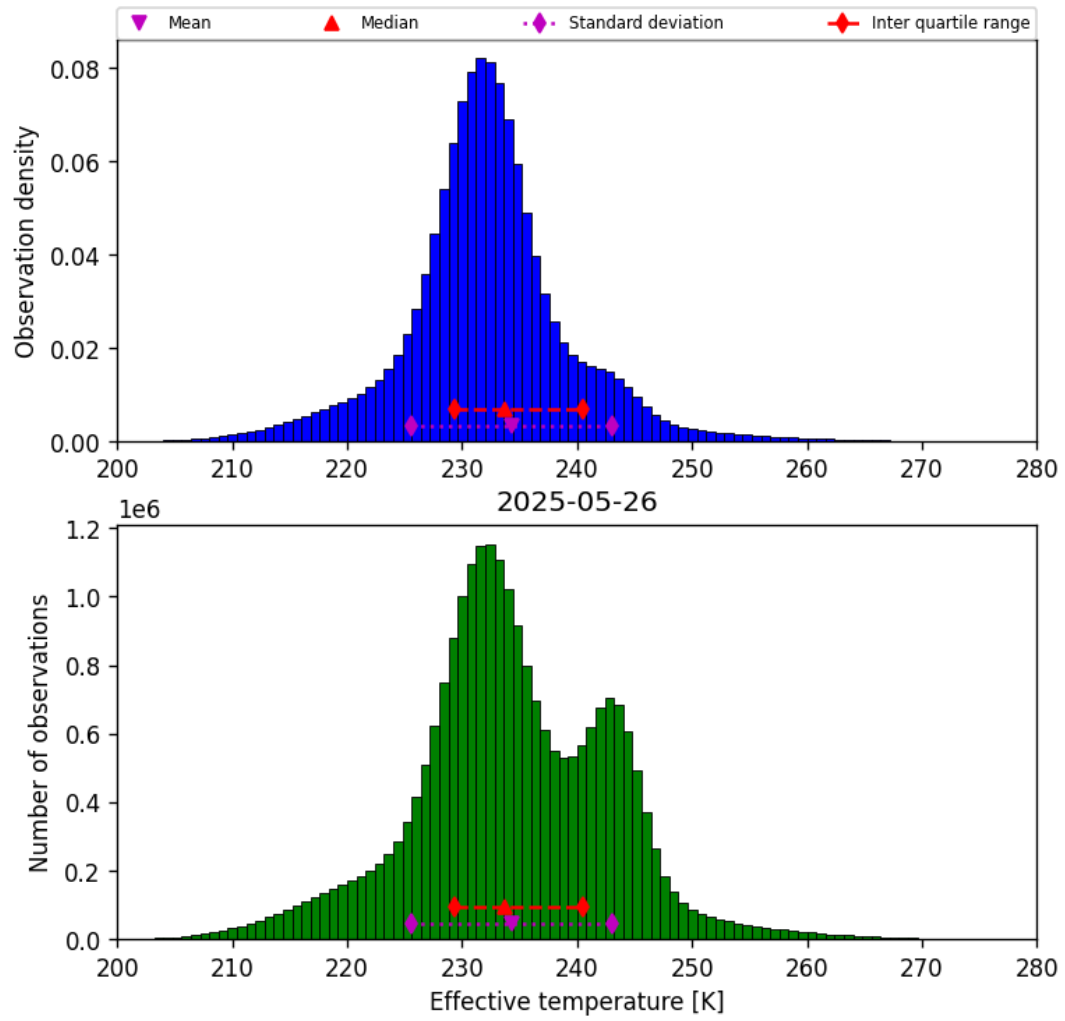
Figure 38: Histogram of “Effective temperature” for 2025-05-26 to 2025-05-27
