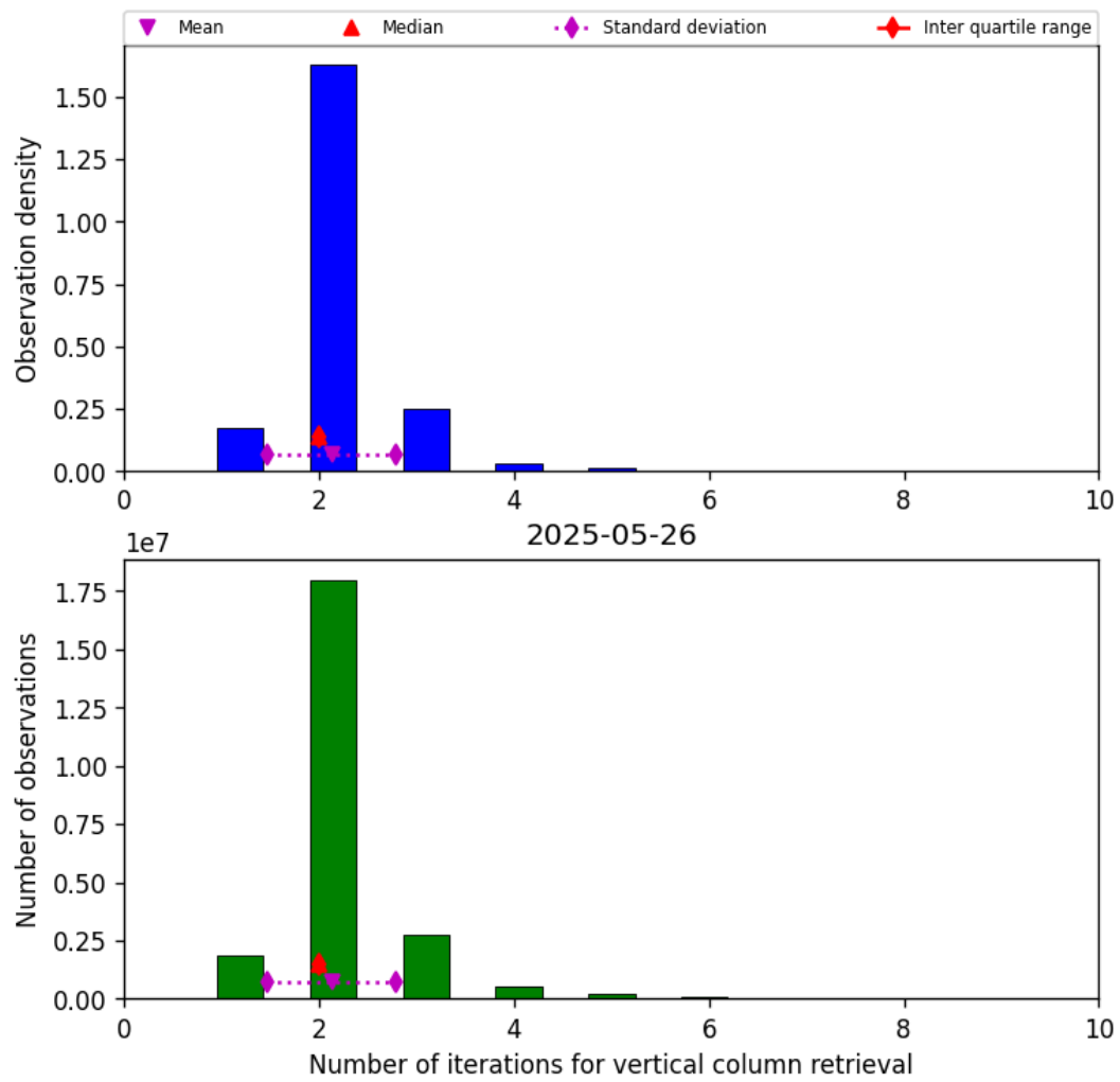
Figure 39: Histogram of “Number of iterations for vertical column retrieval” for 2025-05-26 to 2025-05-27
