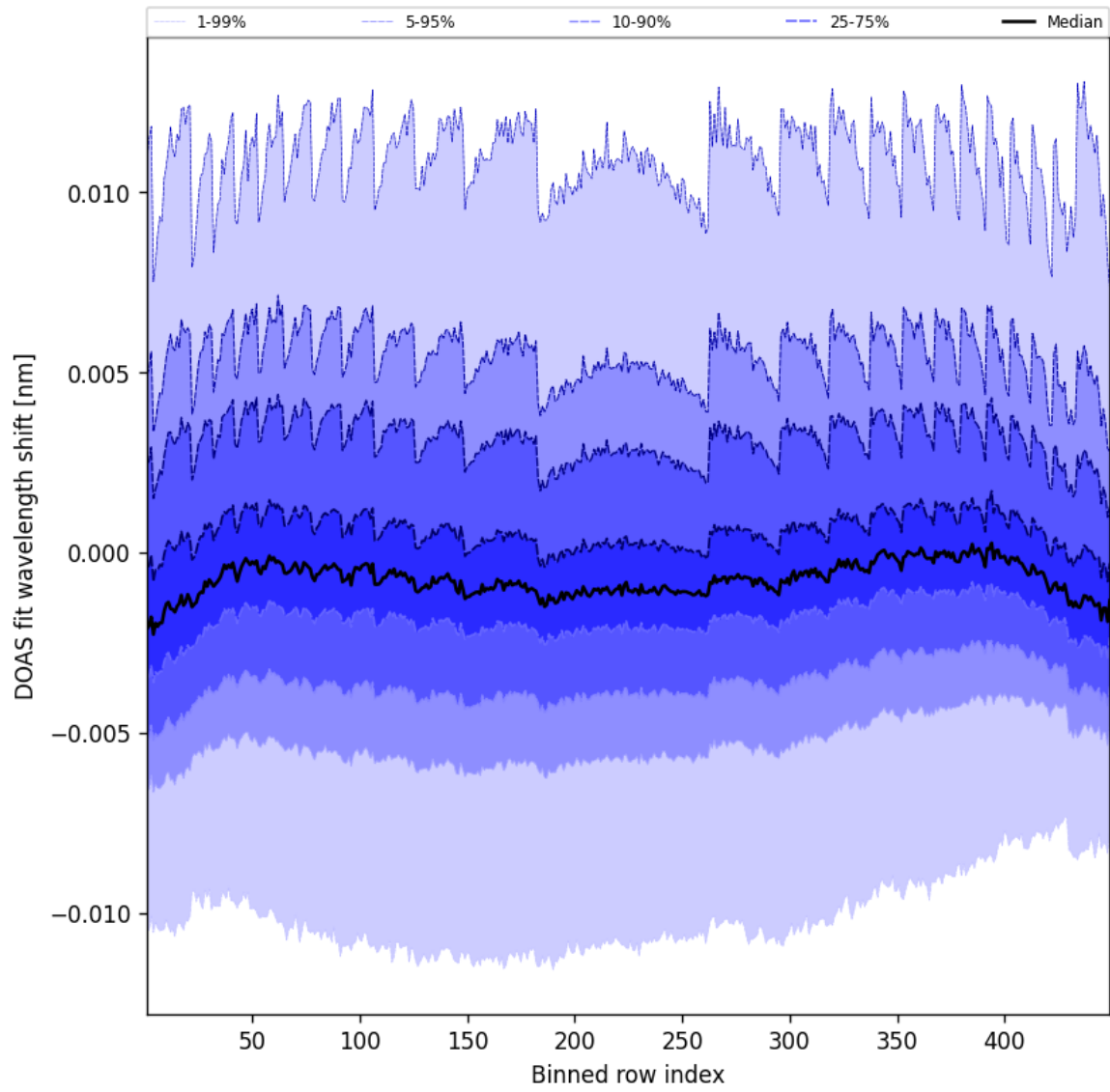
Figure 47: Along track statistics of “DOAS fit wavelength shift” for 2025-05-26 to 2025-05-27
