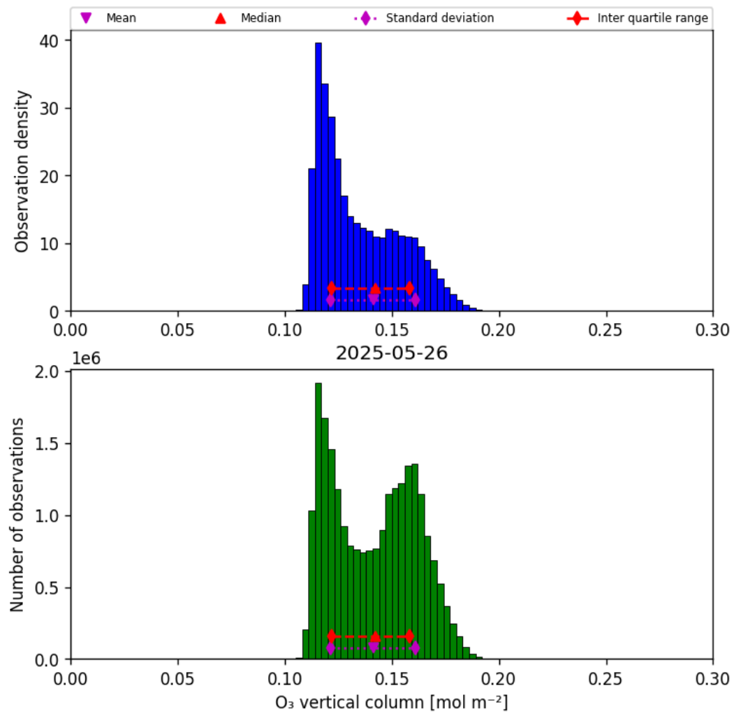
Figure 29: Histogram of “O 3 vertical column” for 2025-05-26 to 2025-05-27
