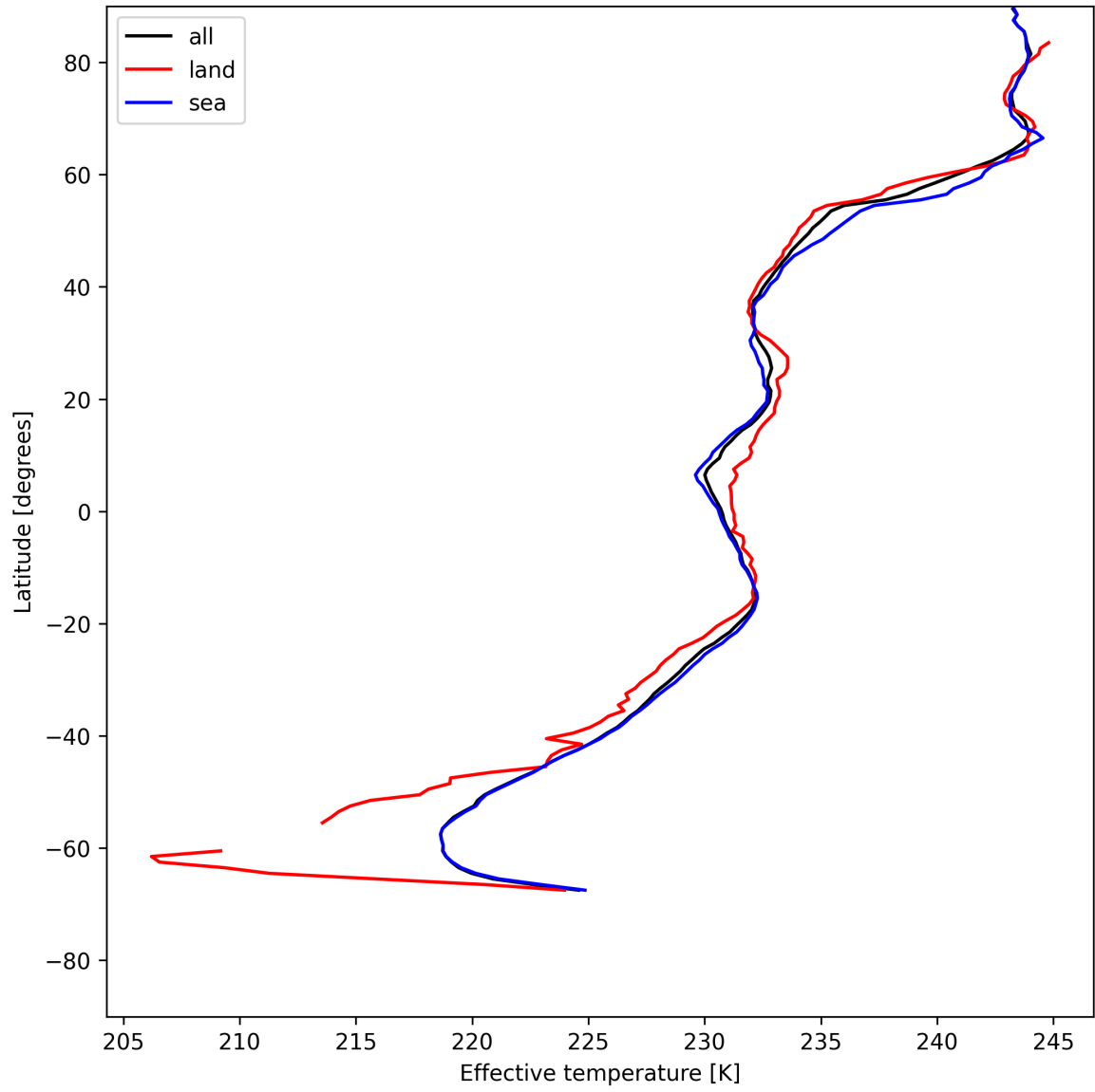
Figure 26: Zonal average of “Effective temperature” for 2025-05-26 to 2025-05-27.
