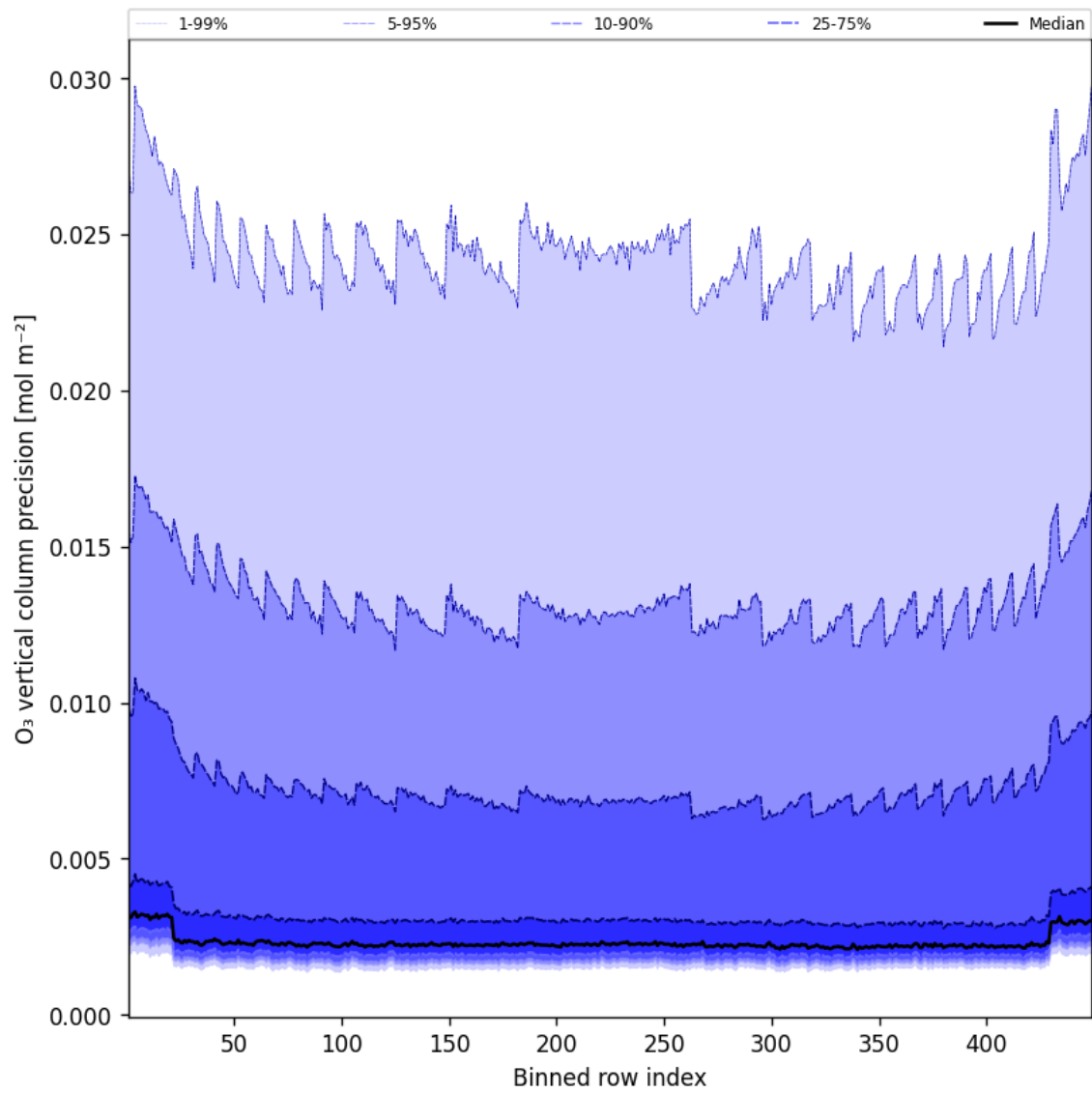
Figure 42: Along track statistics of “O 3 vertical column precision” for 2025-05-26 to 2025-05-27
