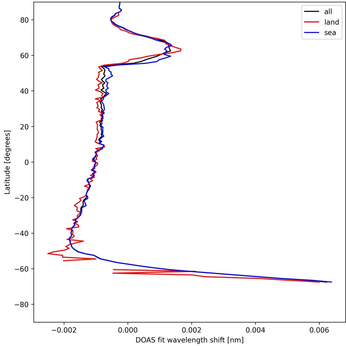
Figure 23: Zonal average of “DOAS fit wavelength shift” for 2025-05-26 to 2025-05-27.
