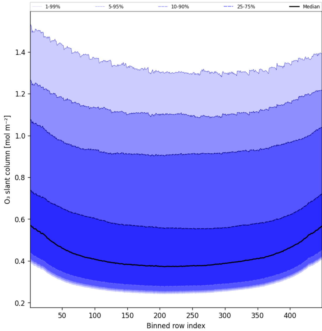
Figure 43: Along track statistics of “O 3 slant column” for 2025-05-26 to 2025-05-27
