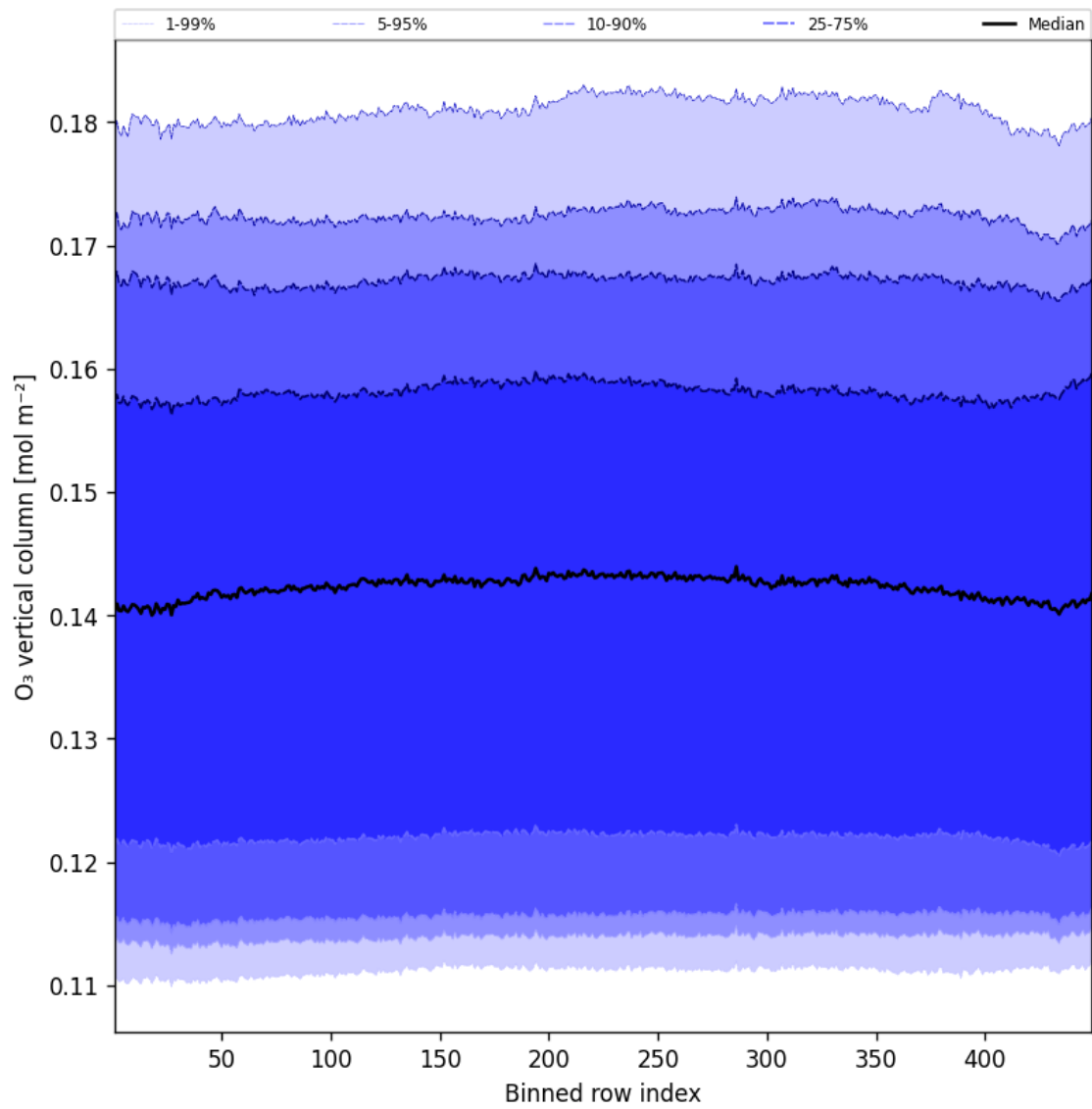
Figure 41: Along track statistics of “O 3 vertical column” for 2025-05-26 to 2025-05-27
