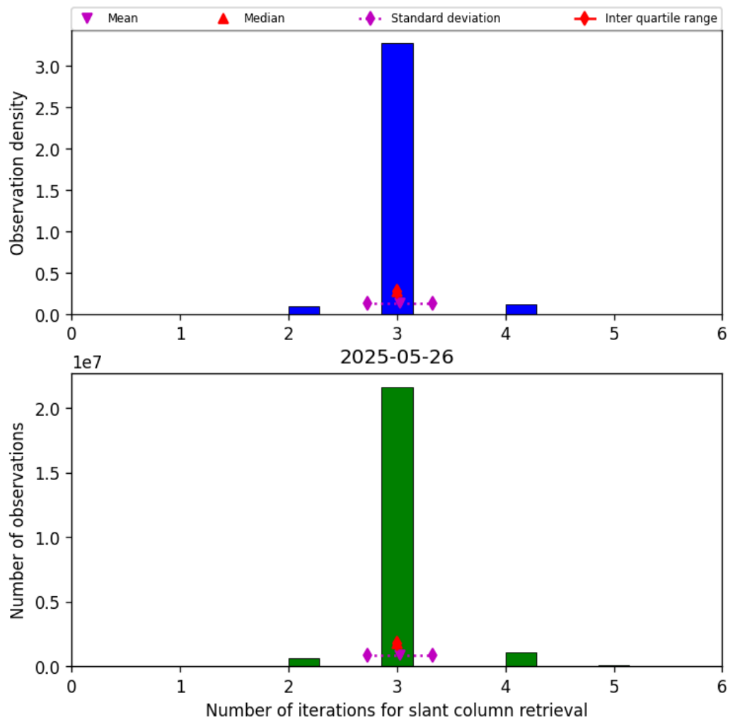
Figure 33: Histogram of “Number of iterations for slant column retrieval” for 2025-05-26 to 2025-05-27
