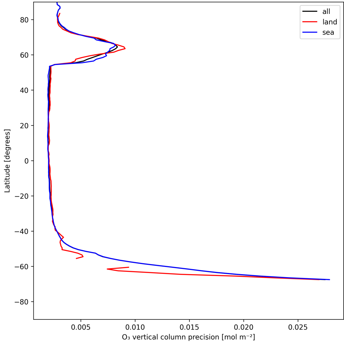
Figure 18: Zonal average of “O 3 vertical column precision” for 2025-05-26 to 2025-05-27.
