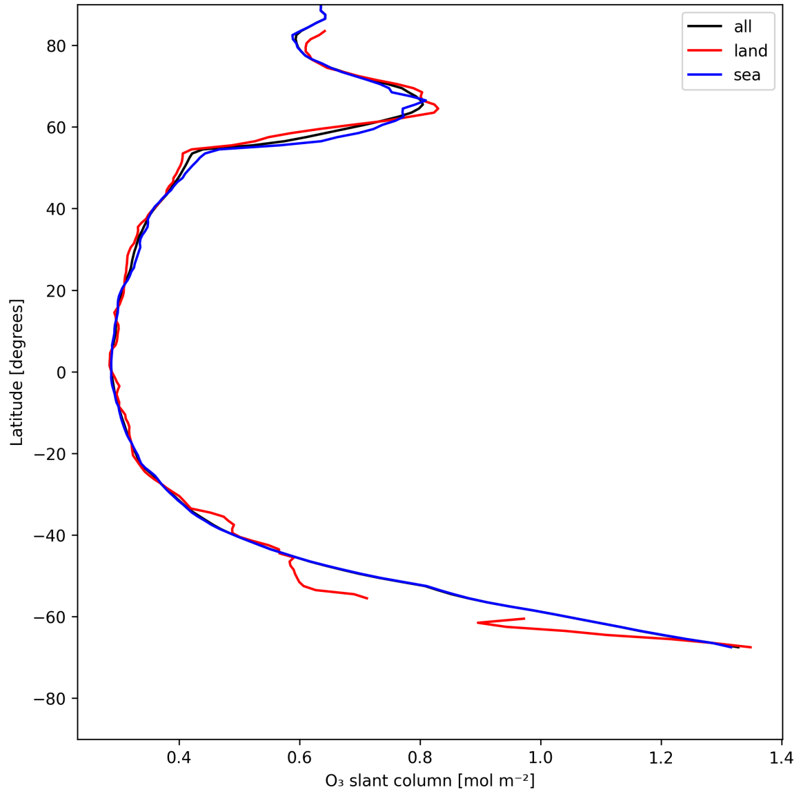
Figure 19: Zonal average of “O 3 slant column” for 2025-05-26 to 2025-05-27.
