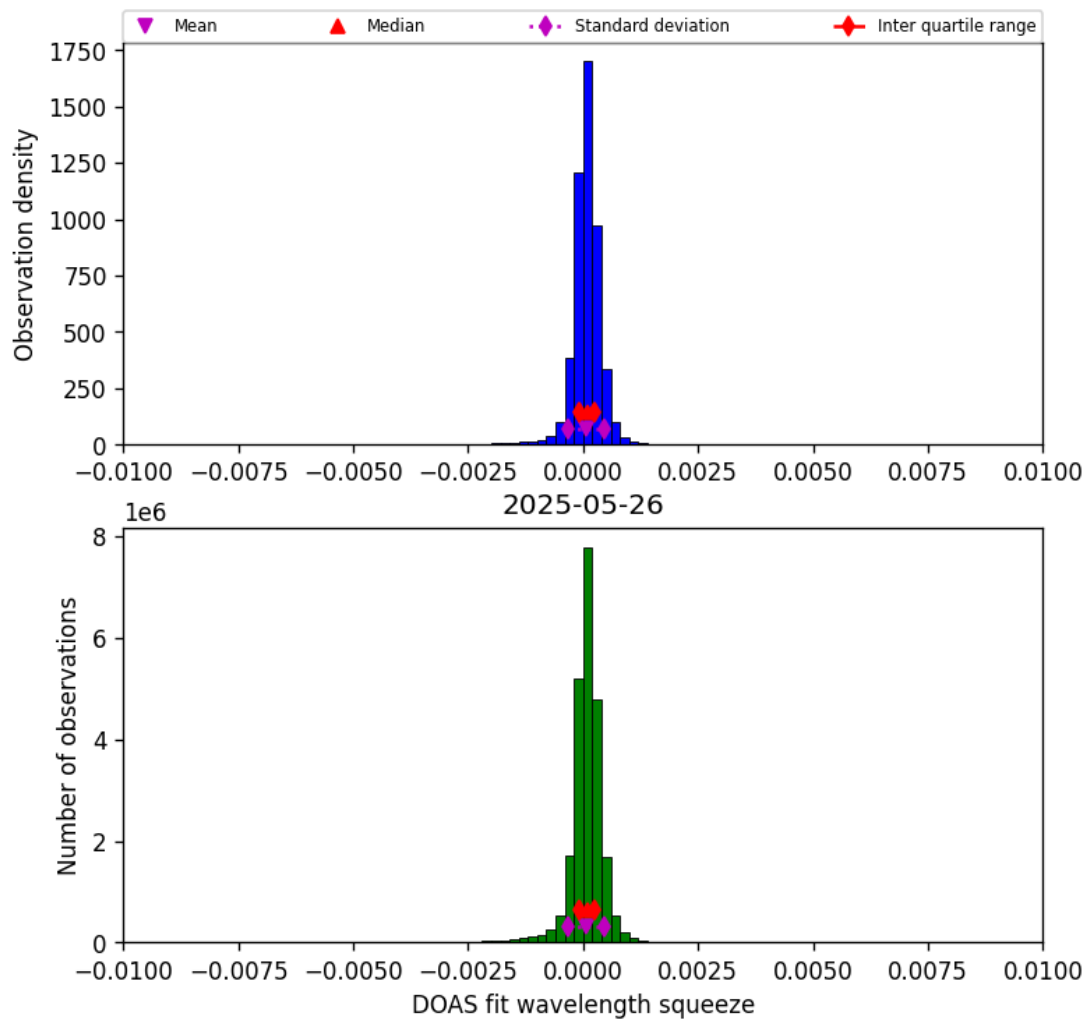
Figure 36: Histogram of “DOAS fit wavelength squeeze” for 2025-05-26 to 2025-05-27
