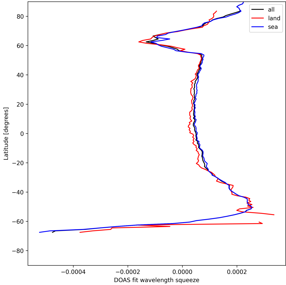
Figure 24: Zonal average of “DOAS fit wavelength squeeze” for 2025-05-26 to 2025-05-27.
