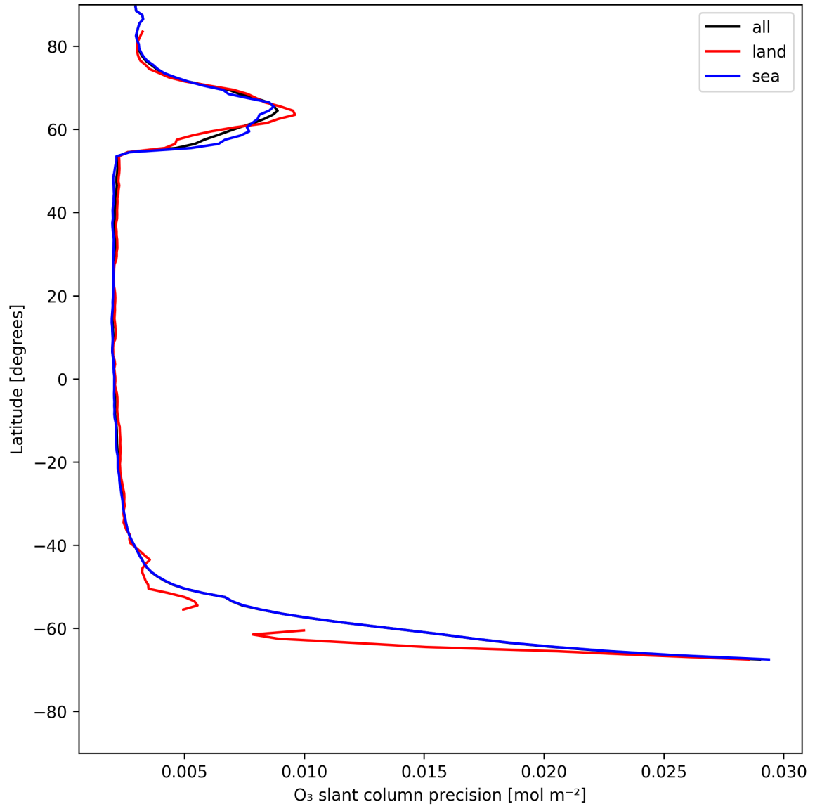
Figure 20: Zonal average of "O 3 slant column precision" for 2025-05-26 to 2025-05-27.
