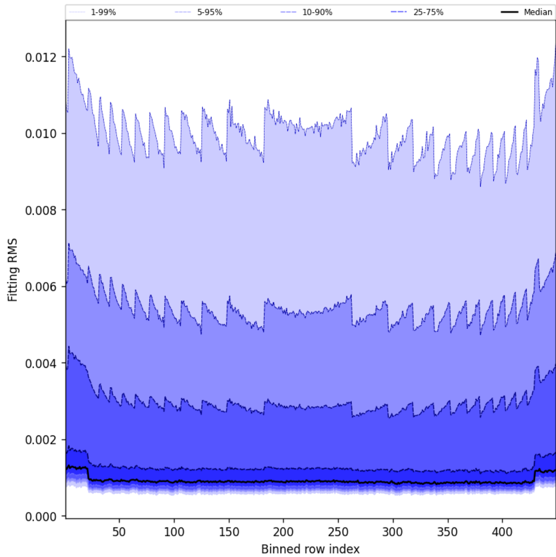
Figure 46: Along track statistics of “Fitting RMS” for 2025-05-26 to 2025-05-27
