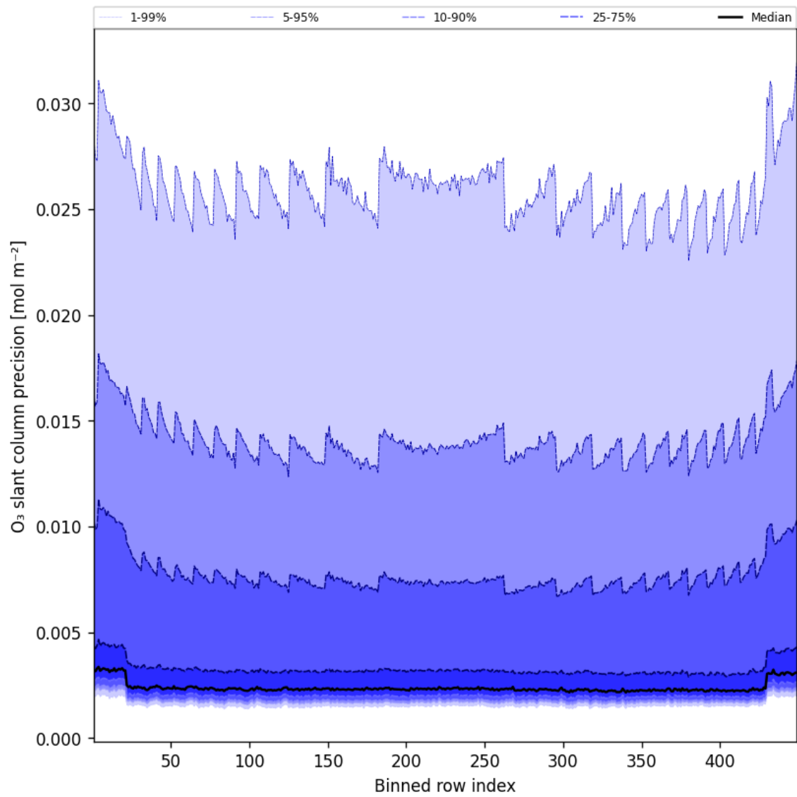
Figure 44: Along track statistics of “O 3 slant column precision” for 2025-05-26 to 2025-05-27
