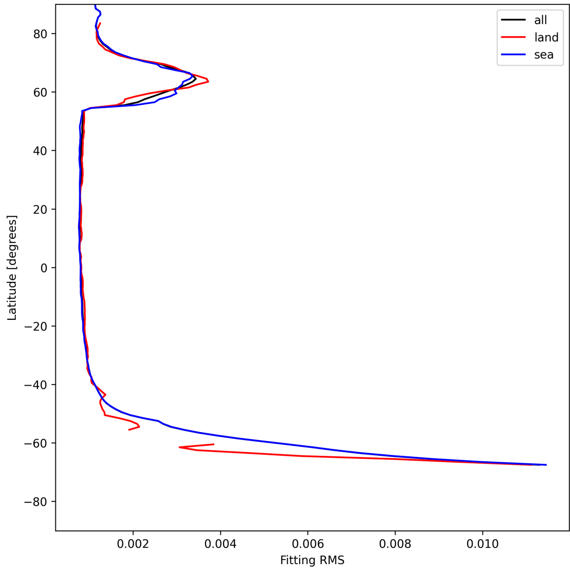
Figure 22: Zonal average of “Fitting RMS” for 2025-05-26 to 2025-05-27.
