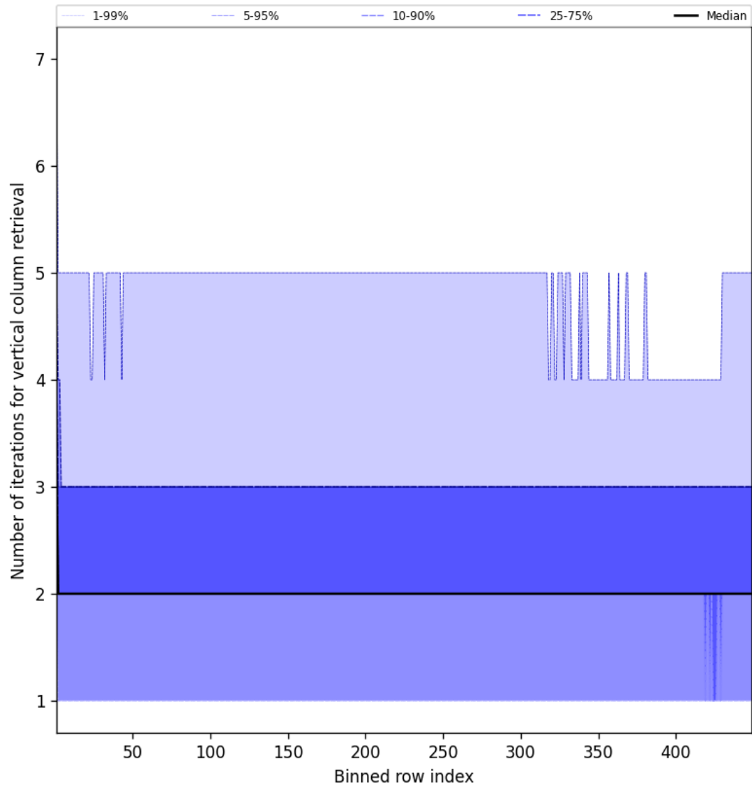
Figure 51: Along track statistics of “Number of iterations for vertical column retrieval” for 2025-05-26 to 2025-05-27
