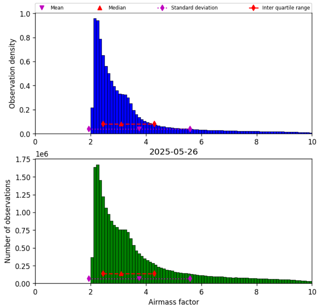
Figure 37: Histogram of “Airmass factor” for 2025-05-26 to 2025-05-27
