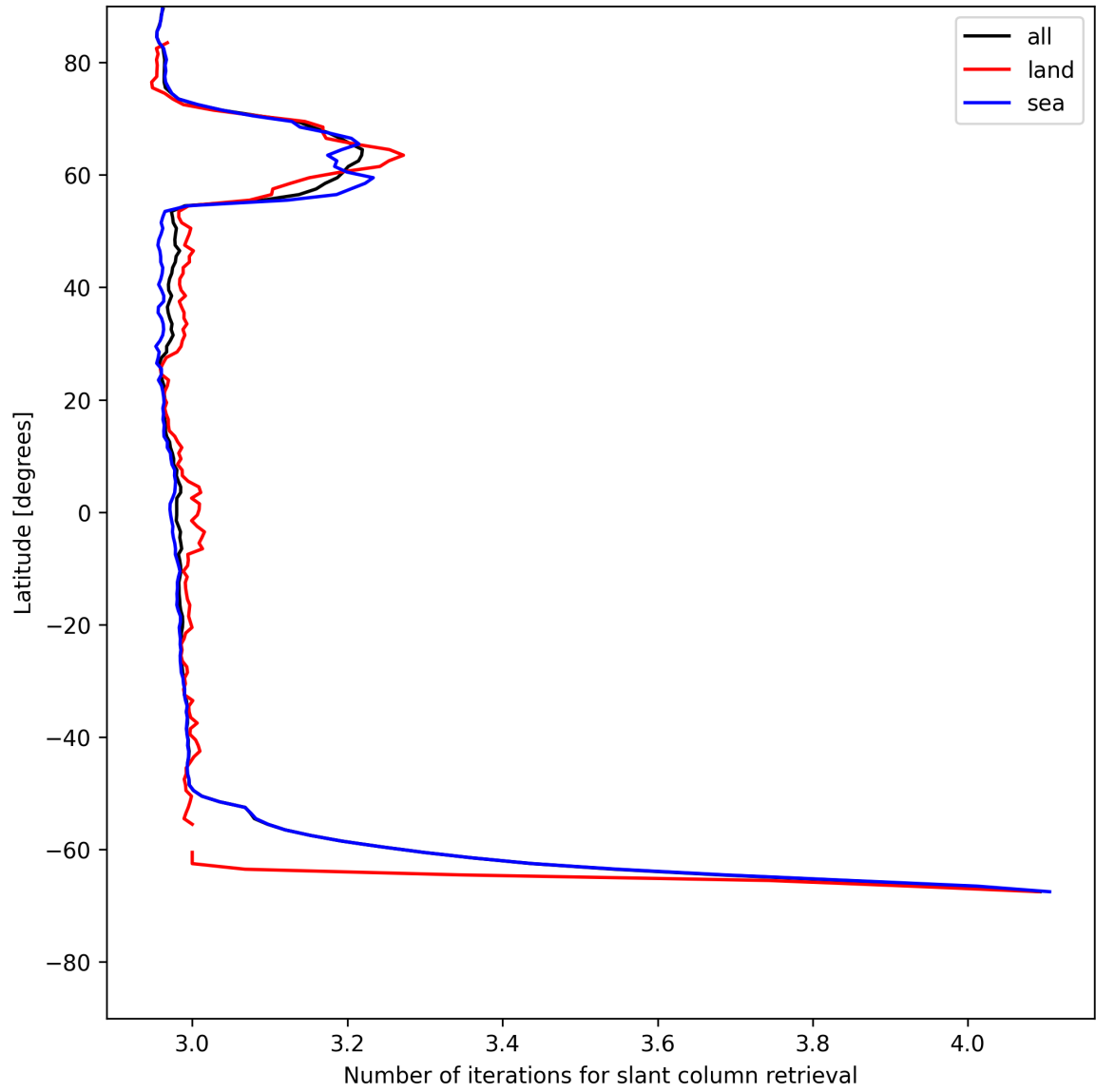
Figure 21: Zonal average of “Number of iterations for slant column retrieval” for 2025-05-26 to 2025-05-27.
