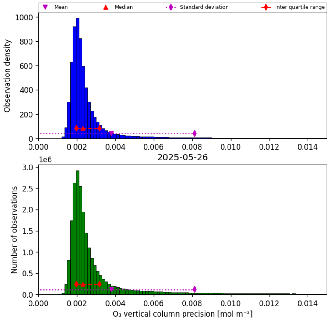
Figure 30: Histogram of “O 3 vertical column precision” for 2025-05-26 to 2025-05-27
