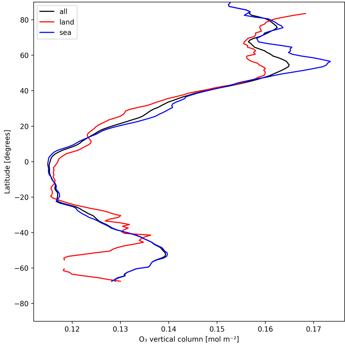
Figure 17: Zonal average of “O 3 vertical column” for 2025-05-26 to 2025-05-27.
