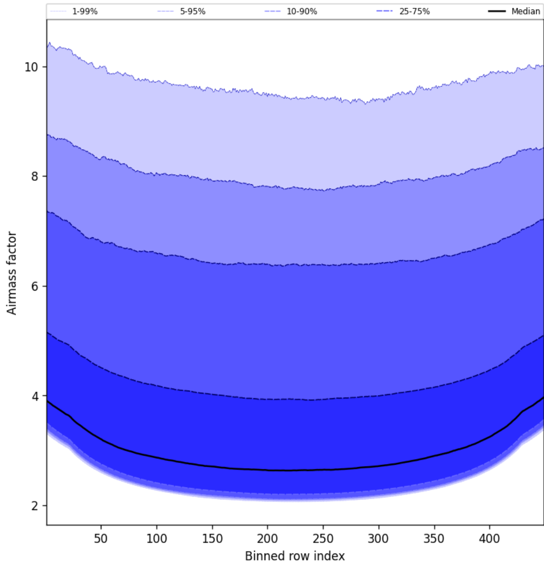
Figure 49: Along track statistics of “Airmass factor” for 2025-05-26 to 2025-05-27
