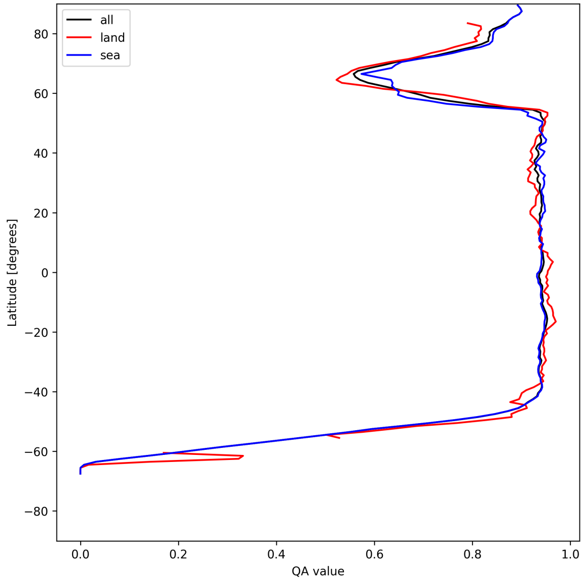
Figure 16: Zonal average of “QA value” for 2025-05-26 to 2025-05-27.
