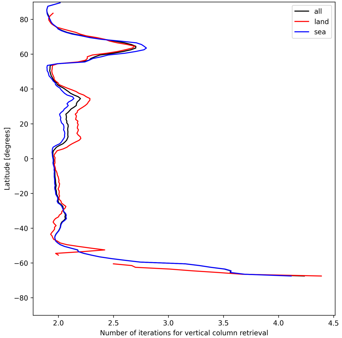
Figure 27: Zonal average of “Number of iterations for vertical column retrieval” for 2025-05-27 to 2025-05-28.
