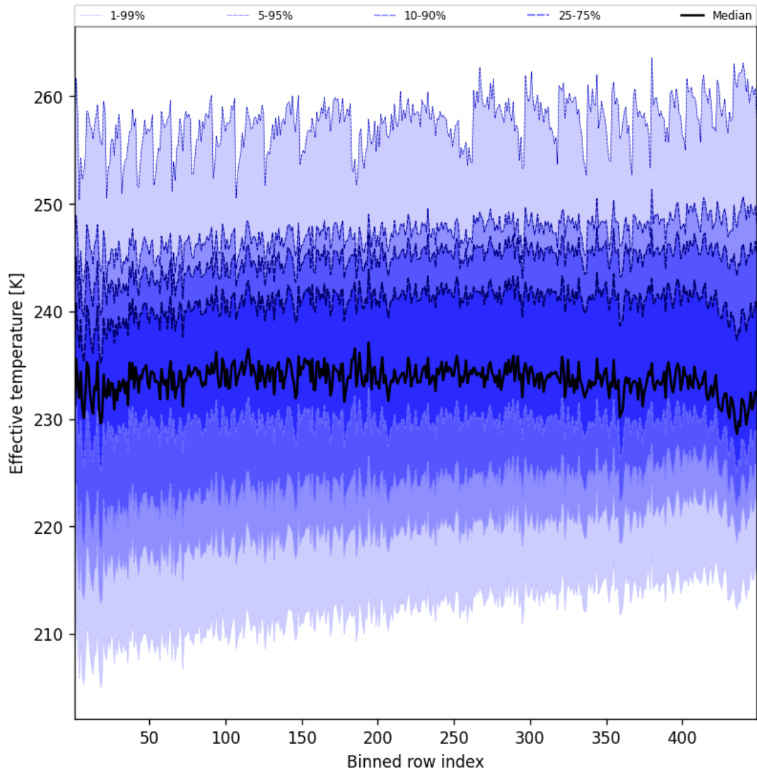
Figure 50: Along track statistics of “Effective temperature” for 2025-05-27 to 2025-05-28
