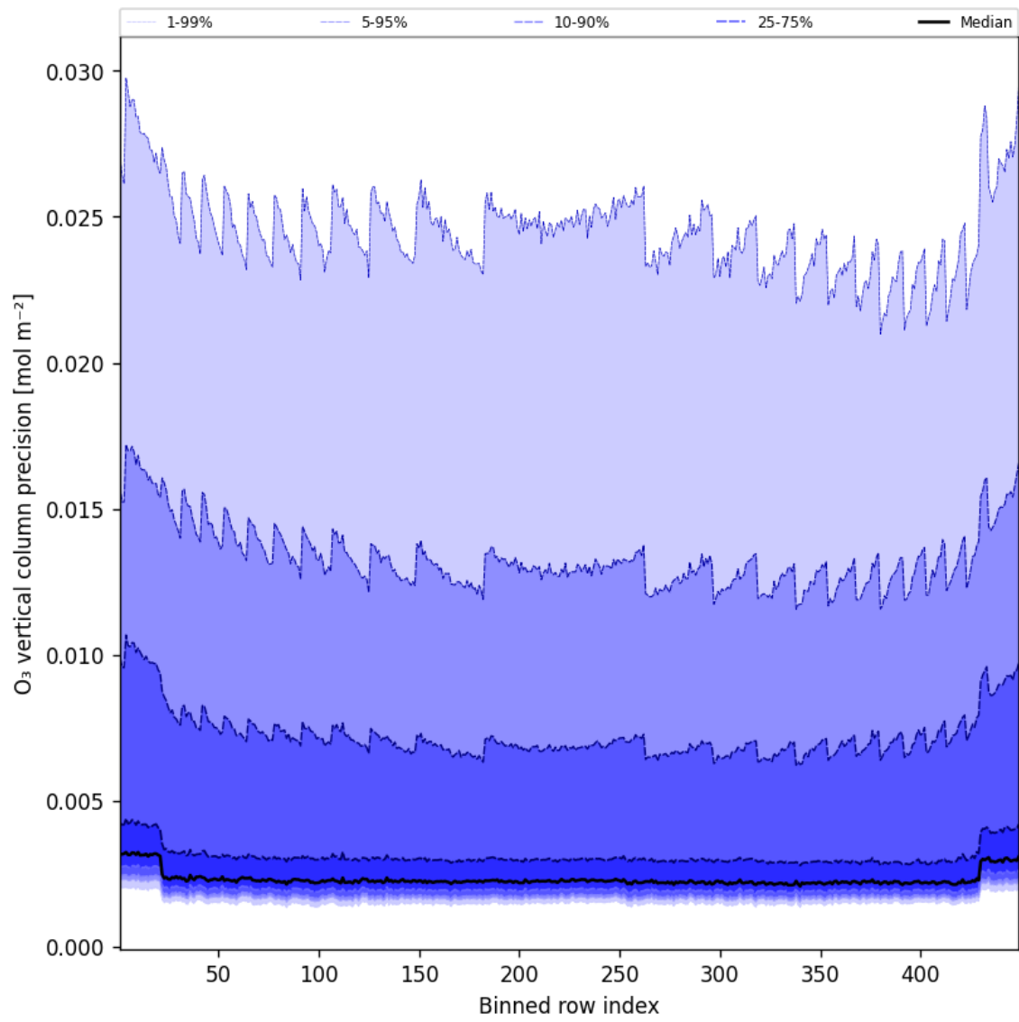
Figure 42: Along track statistics of “O 3 vertical column precision” for 2025-05-27 to 2025-05-28
