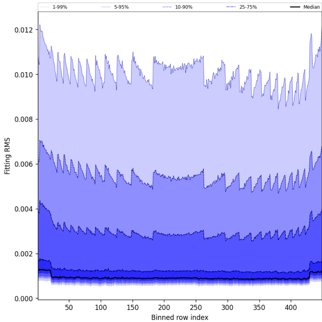
Figure 46: Along track statistics of “Fitting RMS” for 2025-05-27 to 2025-05-28
