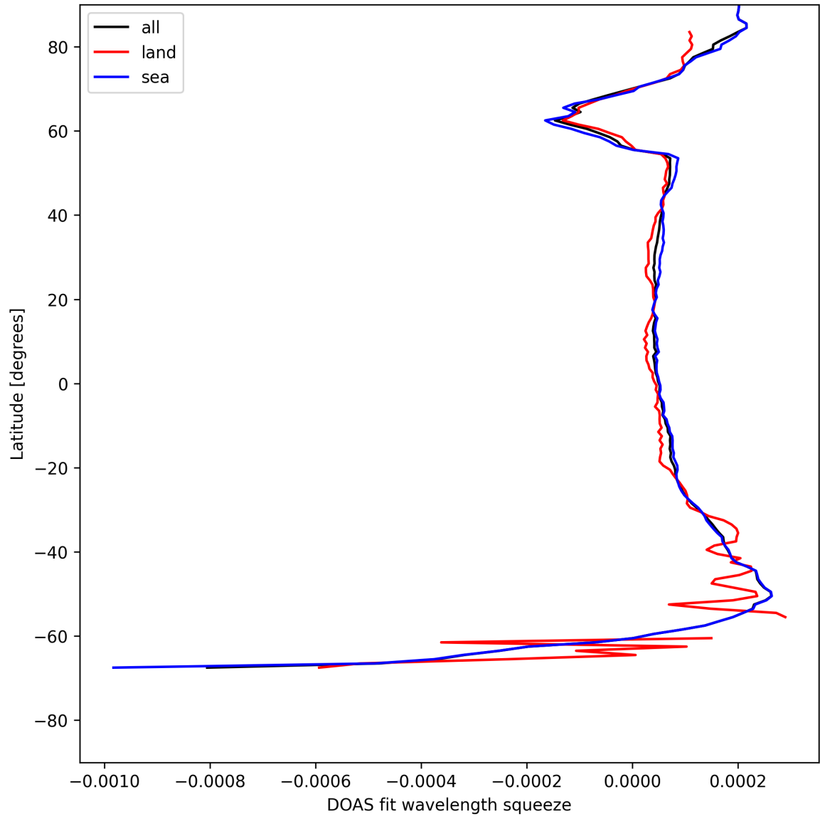
Figure 24: Zonal average of “DOAS fit wavelength squeeze” for 2025-05-27 to 2025-05-28.
