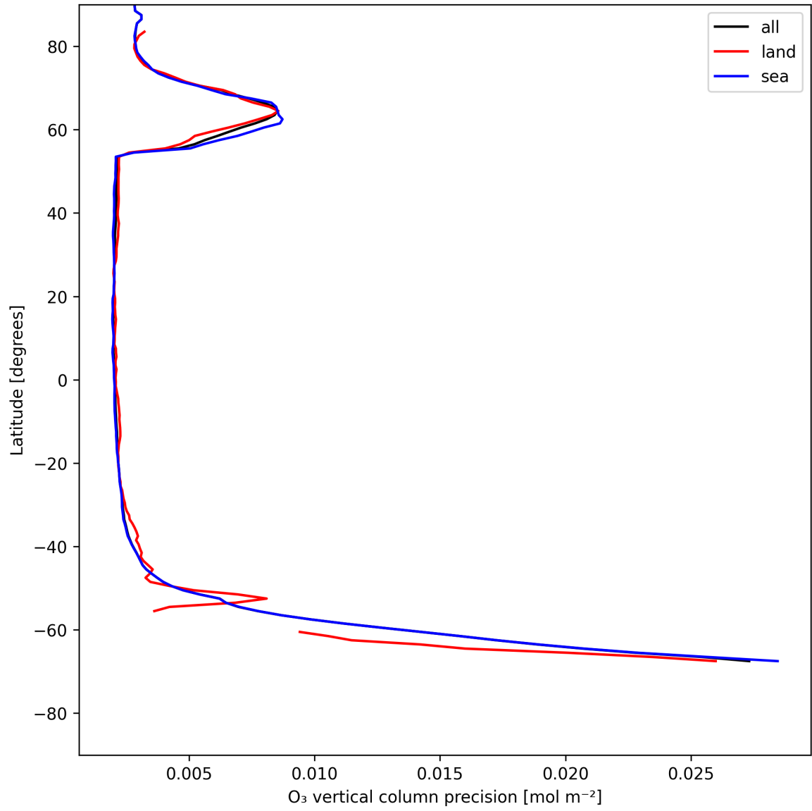
Figure 18: Zonal average of “O 3 vertical column precision” for 2025-05-27 to 2025-05-28.
