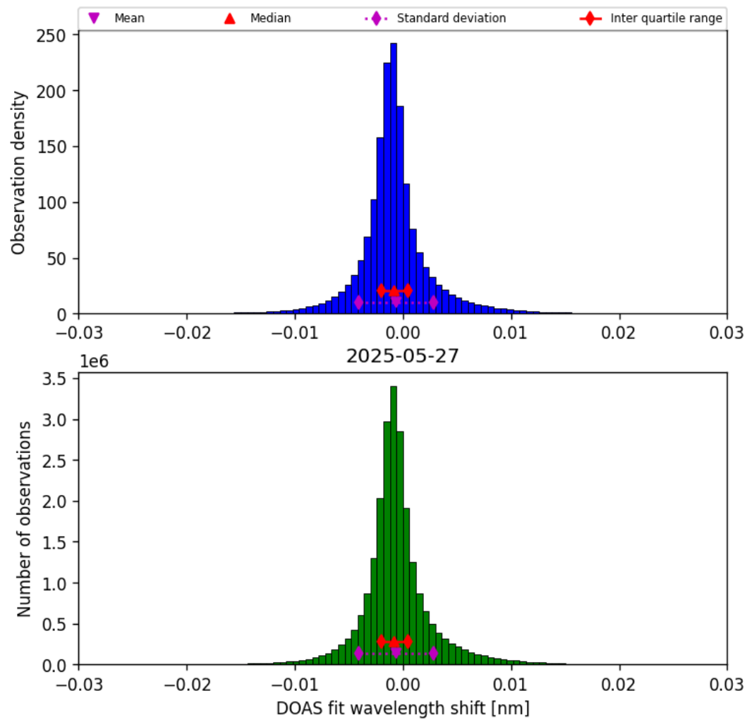
Figure 35: Histogram of “DOAS fit wavelength shift” for 2025-05-27 to 2025-05-28
