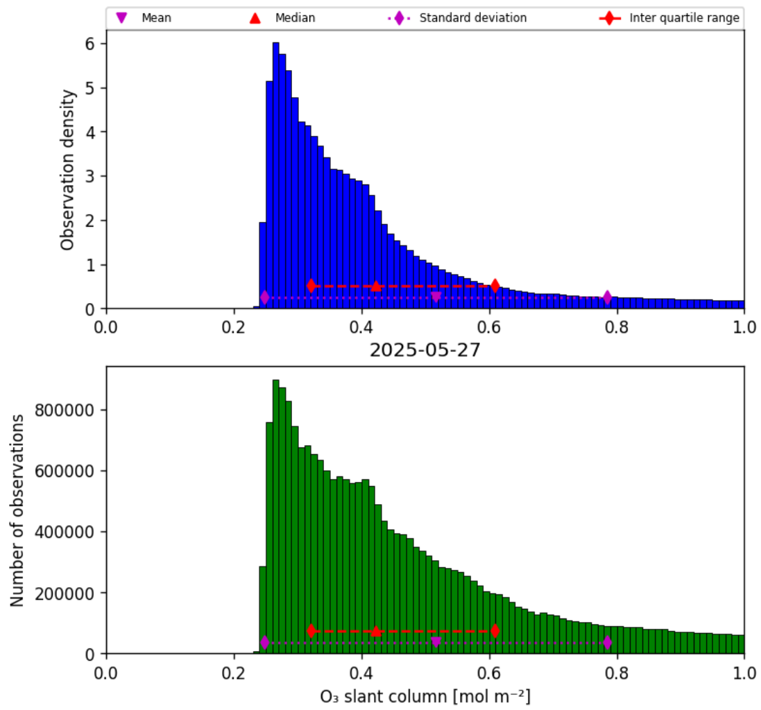
Figure 31: Histogram of “O 3 slant column” for 2025-05-27 to 2025-05-28
