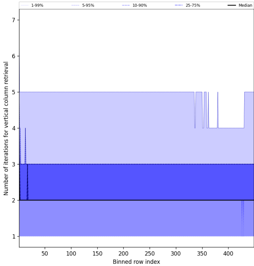
Figure 51: Along track statistics of “Number of iterations for vertical column retrieval” for 2025-05-27 to 2025-05-28
