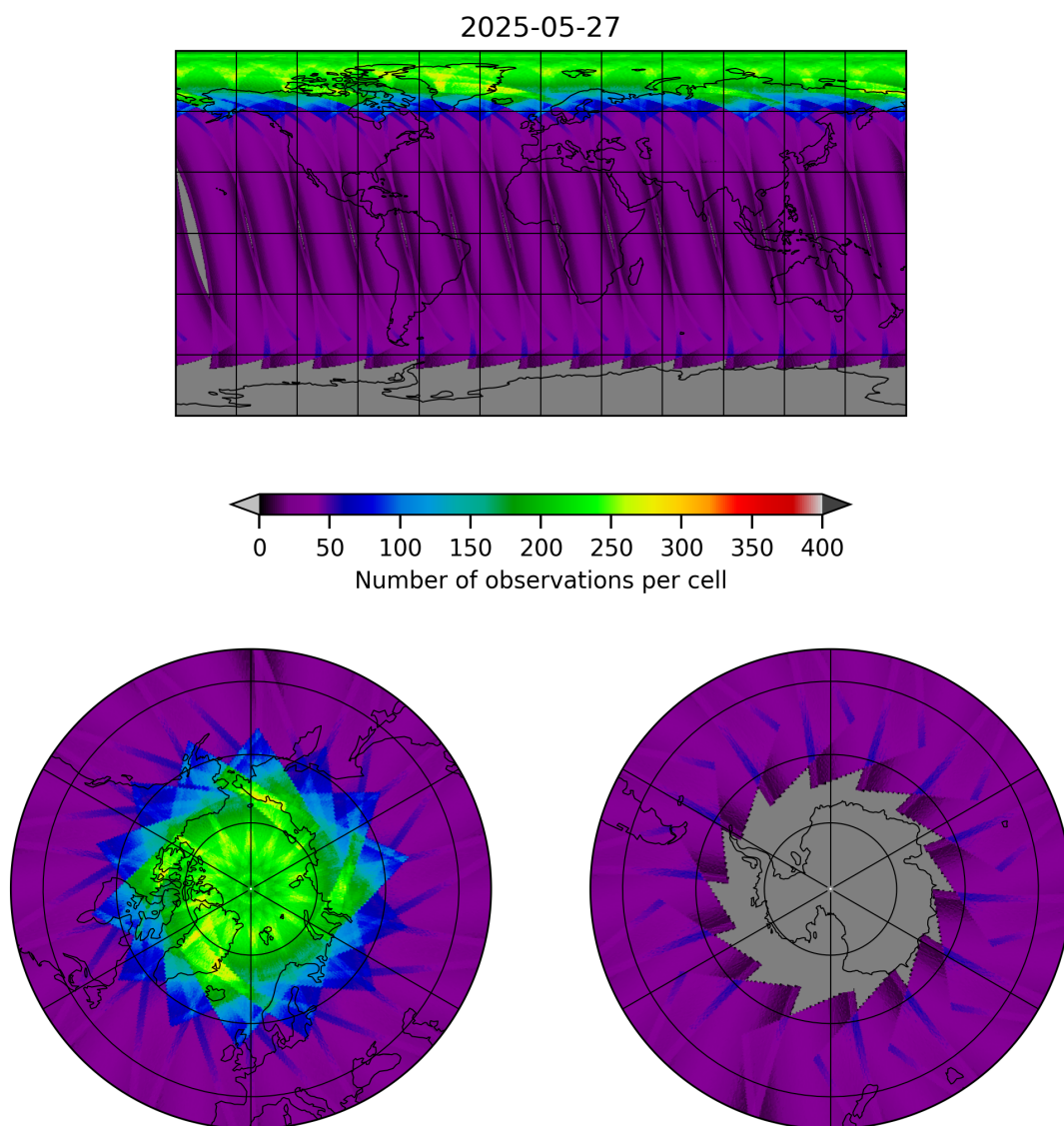
Figure 15: Map of the number of observations for 2025-05-27 to 2025-05-28
