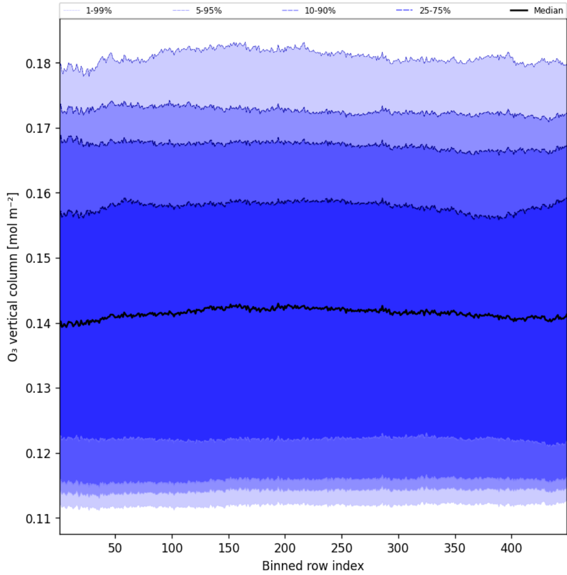
Figure 41: Along track statistics of “O 3 vertical column” for 2025-05-27 to 2025-05-28
