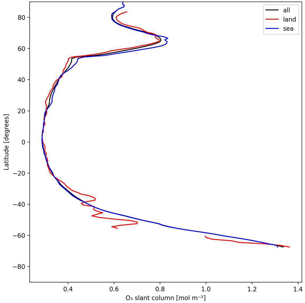
Figure 19: Zonal average of “O 3 slant column” for 2025-05-27 to 2025-05-28.
