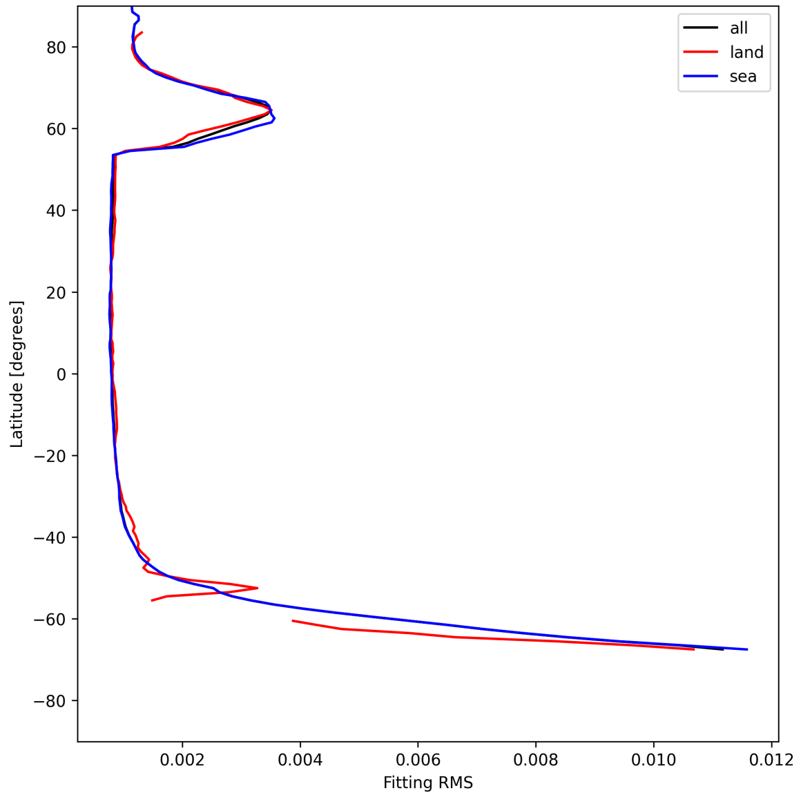
Figure 22: Zonal average of “Fitting RMS” for 2025-05-27 to 2025-05-28.
