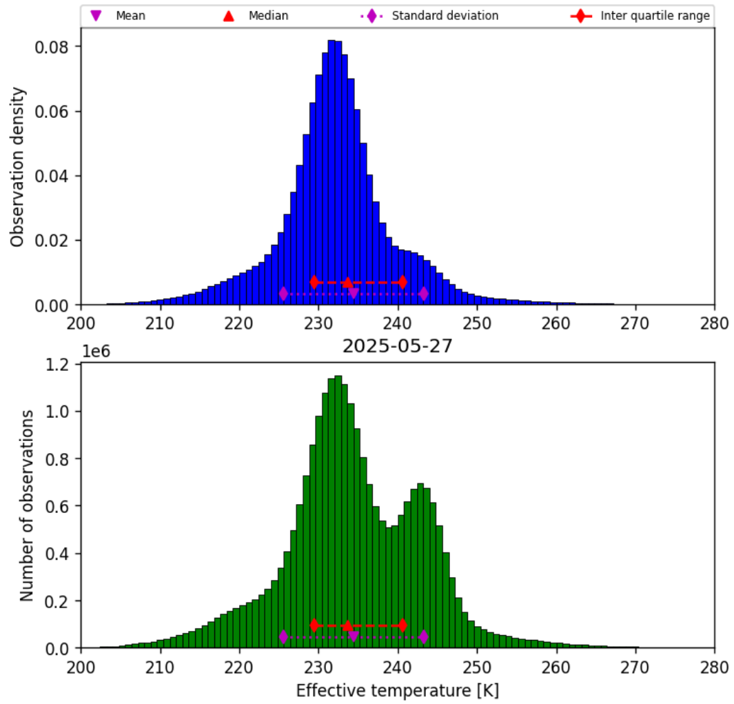
Figure 38: Histogram of “Effective temperature” for 2025-05-27 to 2025-05-28
