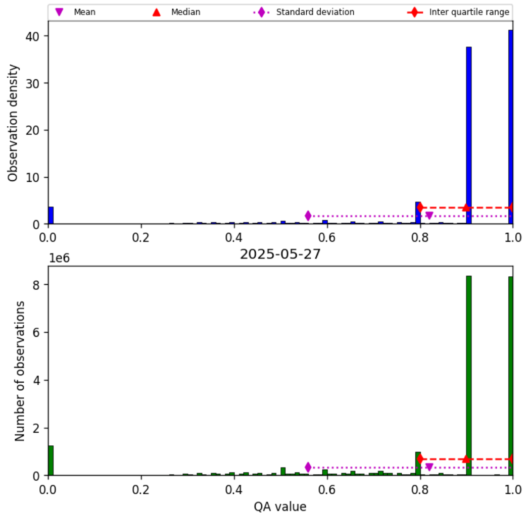
Figure 28: Histogram of “QA value” for 2025-05-27 to 2025-05-28
