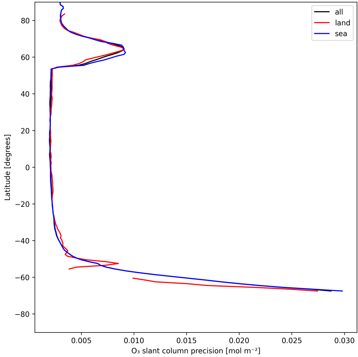
Figure 20: Zonal average of “O 3 slant column precision” for 2025-05-27 to 2025-05-28.
