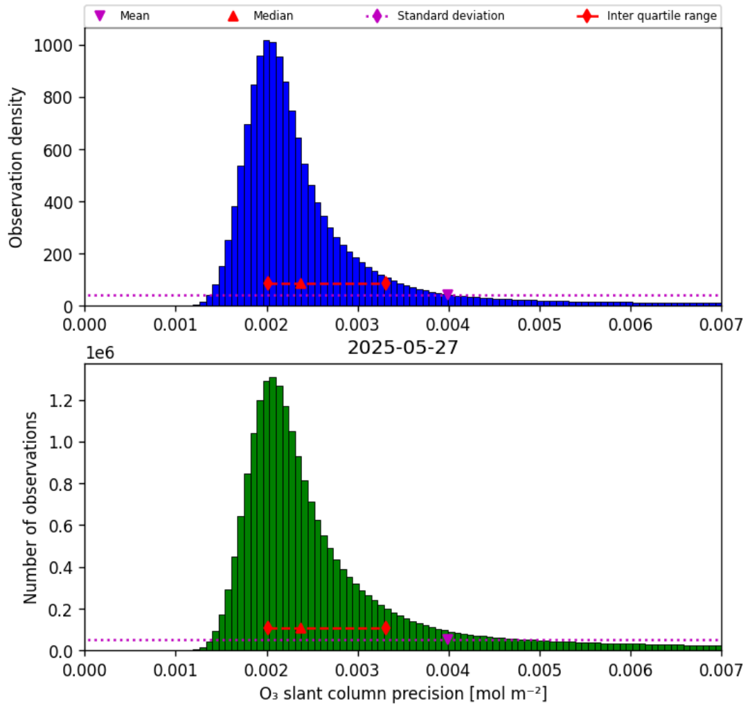
Figure 32: Histogram of “O 3 slant column precision” for 2025-05-27 to 2025-05-28
