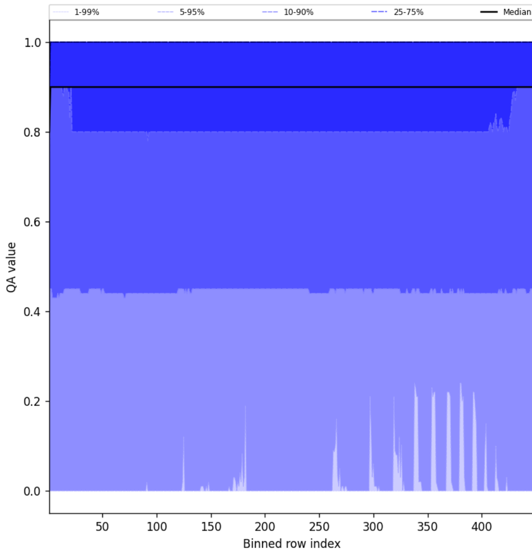
Figure 40: Along track statistics of “QA value” for 2025-05-27 to 2025-05-28
