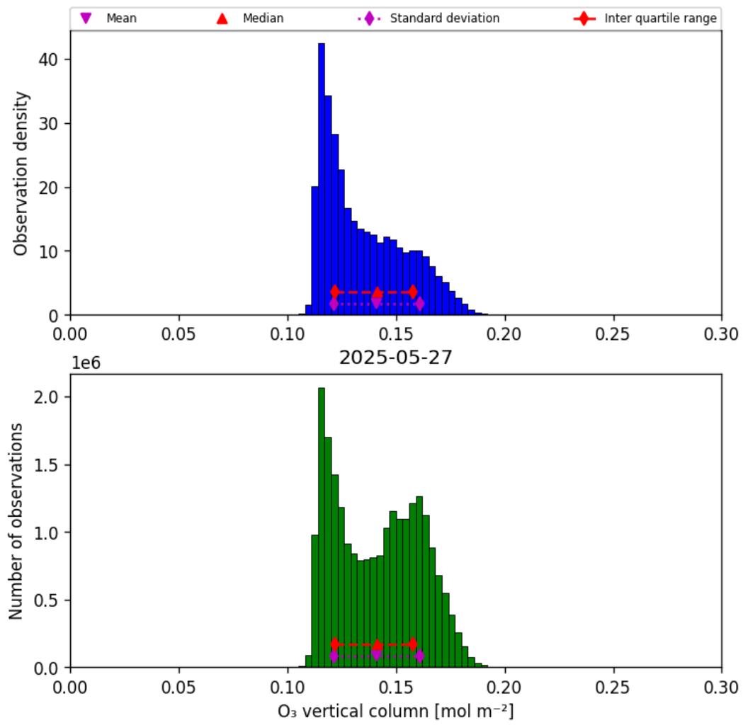
Figure 29: Histogram of “O 3 vertical column” for 2025-05-27 to 2025-05-28
