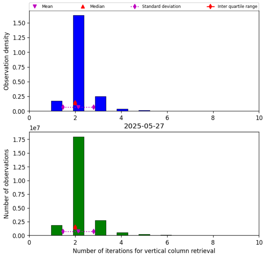
Figure 39: Histogram of “Number of iterations for vertical column retrieval” for 2025-05-27 to 2025-05-28
