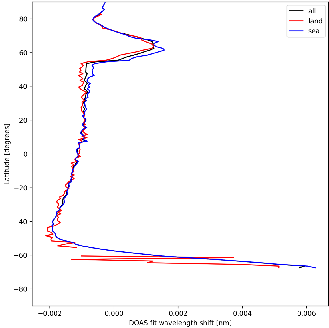
Figure 23: Zonal average of “DOAS fit wavelength shift” for 2025-05-27 to 2025-05-28.
