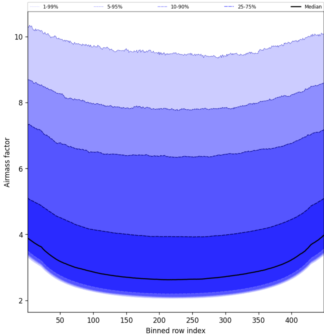
Figure 49: Along track statistics of “Airmass factor” for 2025-05-27 to 2025-05-28
