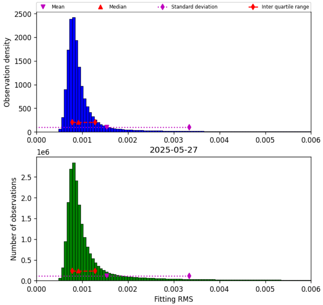
Figure 34: Histogram of “Fitting RMS” for 2025-05-27 to 2025-05-28
