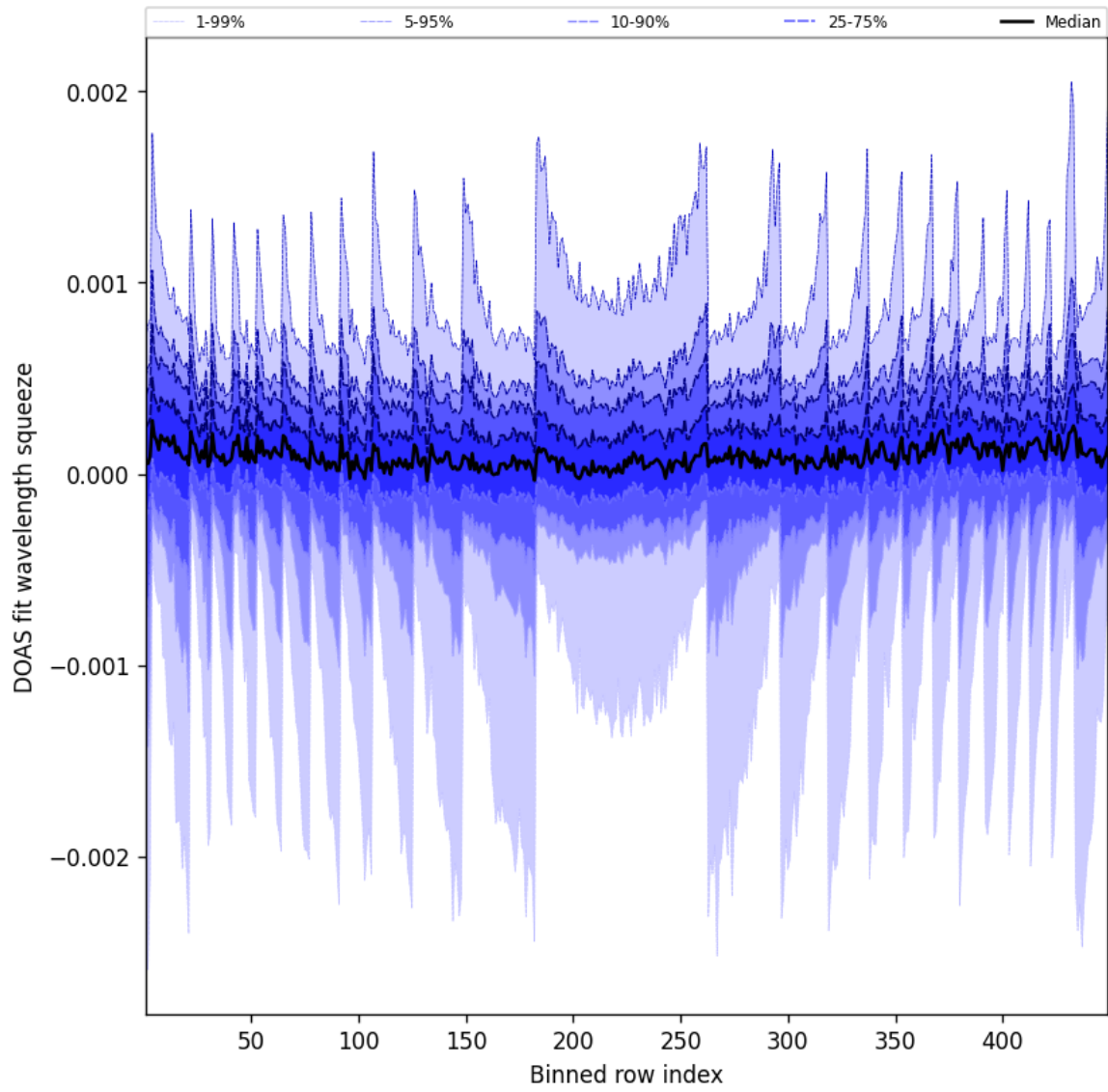
Figure 48: Along track statistics of “DOAS fit wavelength squeeze” for 2025-05-27 to 2025-05-28
