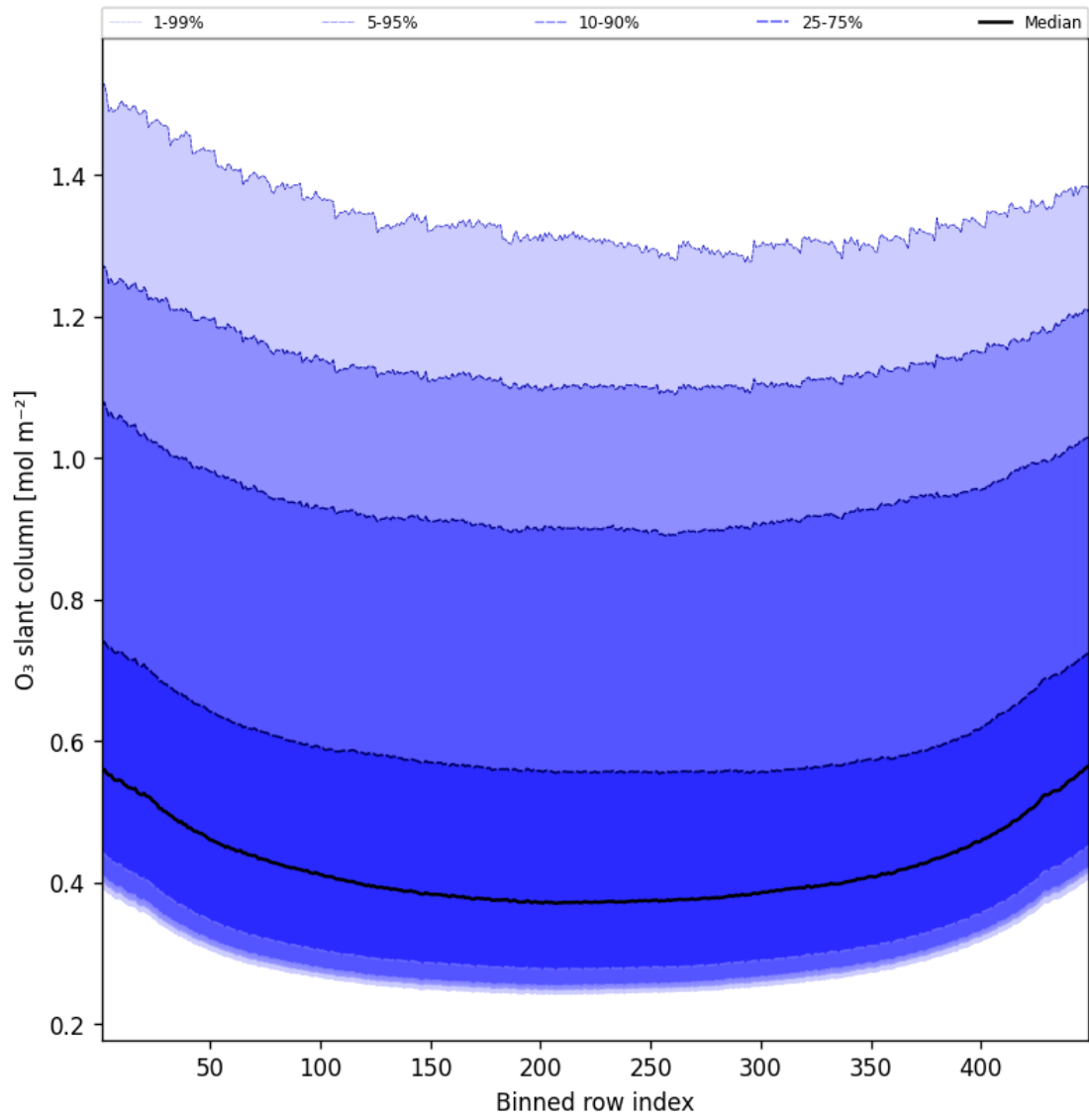
Figure 43: Along track statistics of “O 3 slant column” for 2025-05-27 to 2025-05-28
