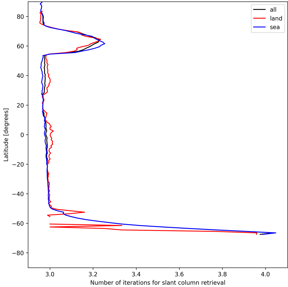
Figure 21: Zonal average of “Number of iterations for slant column retrieval” for 2025-05-27 to 2025-05-28.
