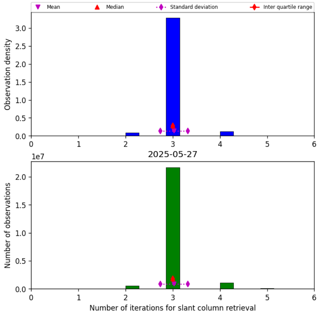
Figure 33: Histogram of “Number of iterations for slant column retrieval” for 2025-05-27 to 2025-05-28
