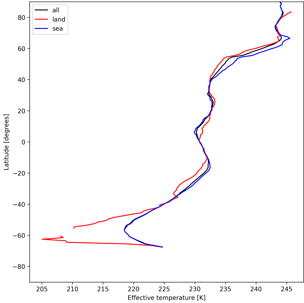
Figure 26: Zonal average of “Effective temperature” for 2025-05-27 to 2025-05-28.
