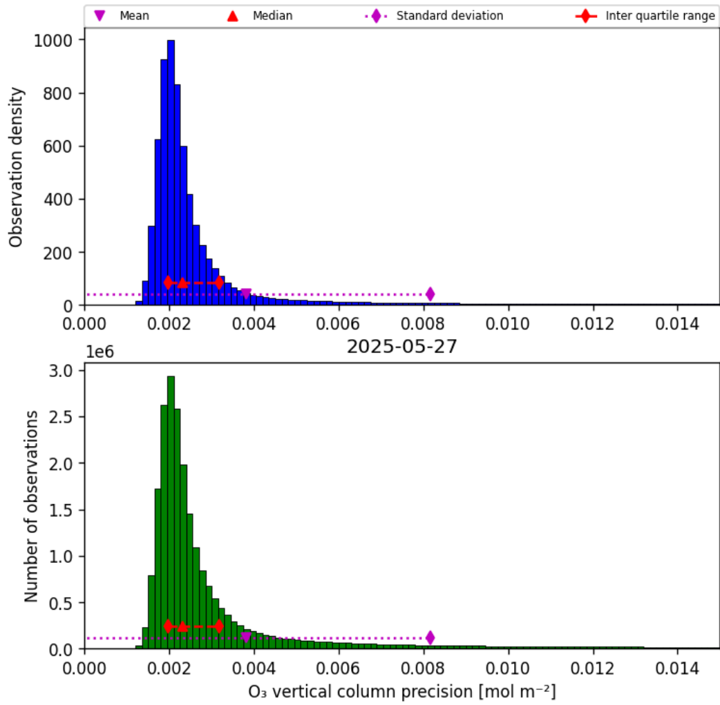
Figure 30: Histogram of “O 3 vertical column precision” for 2025-05-27 to 2025-05-28
