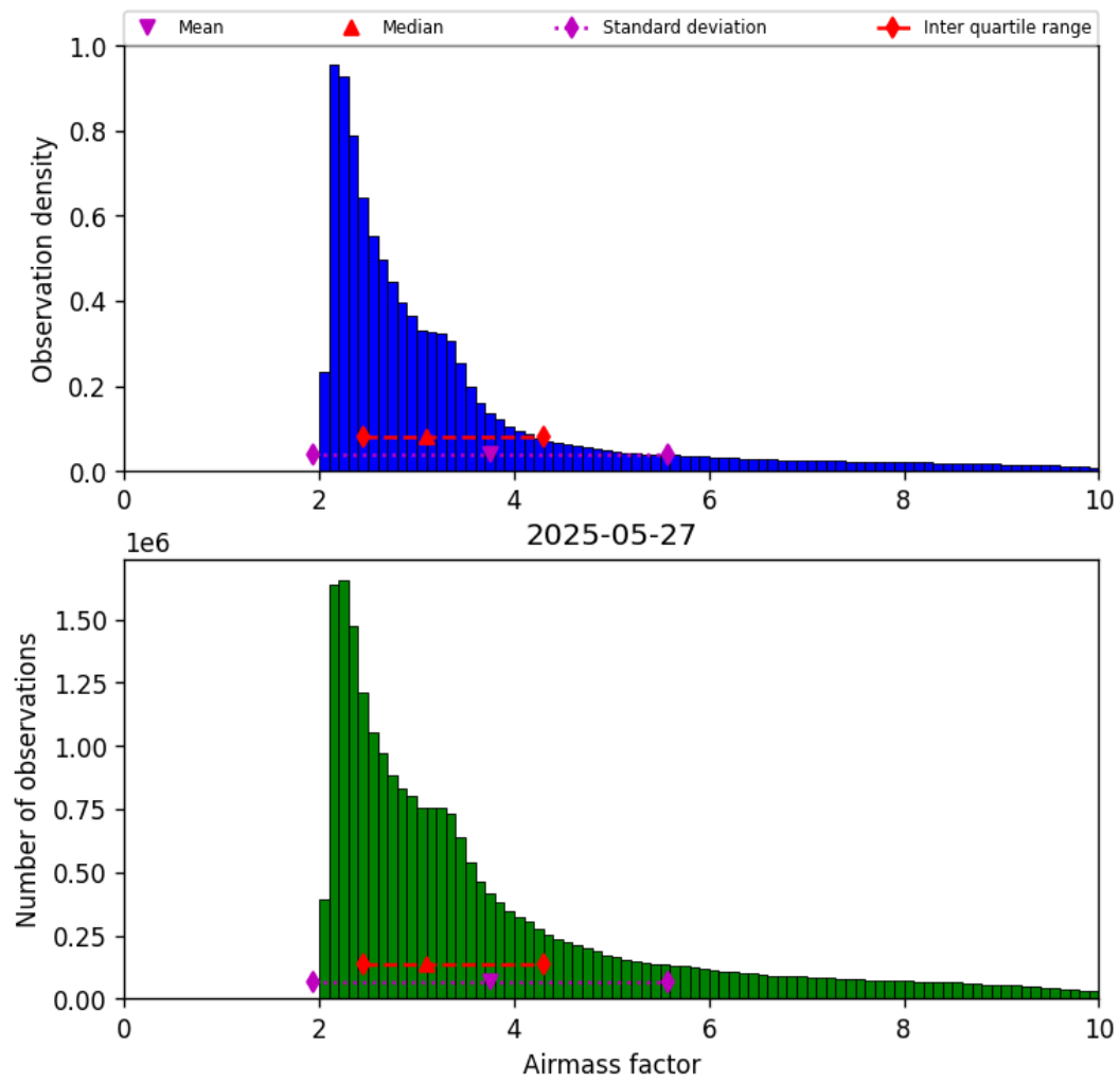
Figure 37: Histogram of “Airmass factor” for 2025-05-27 to 2025-05-28
