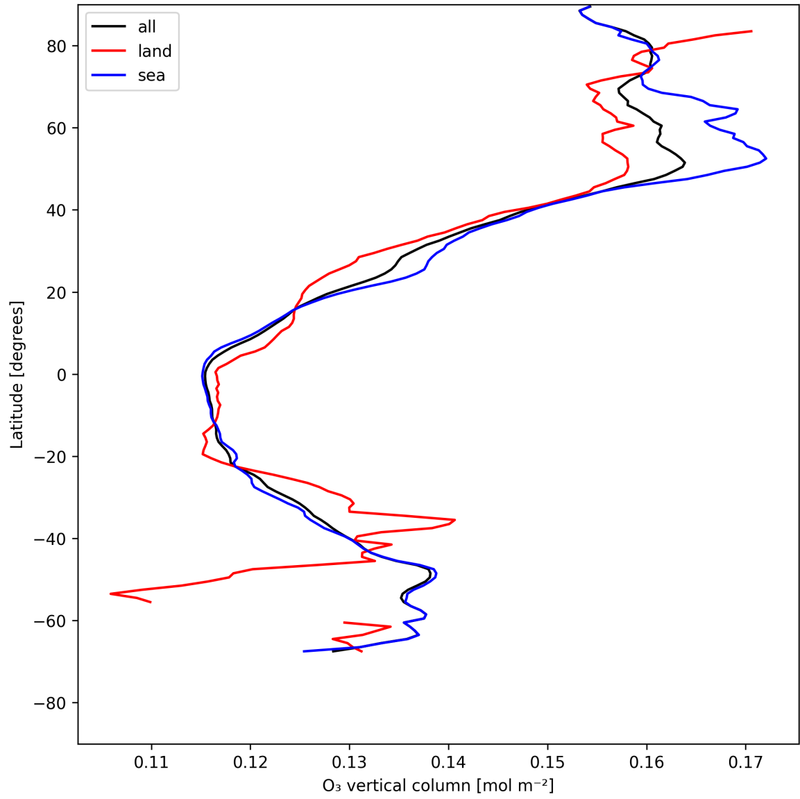
Figure 17: Zonal average of “O 3 vertical column” for 2025-05-27 to 2025-05-28.
