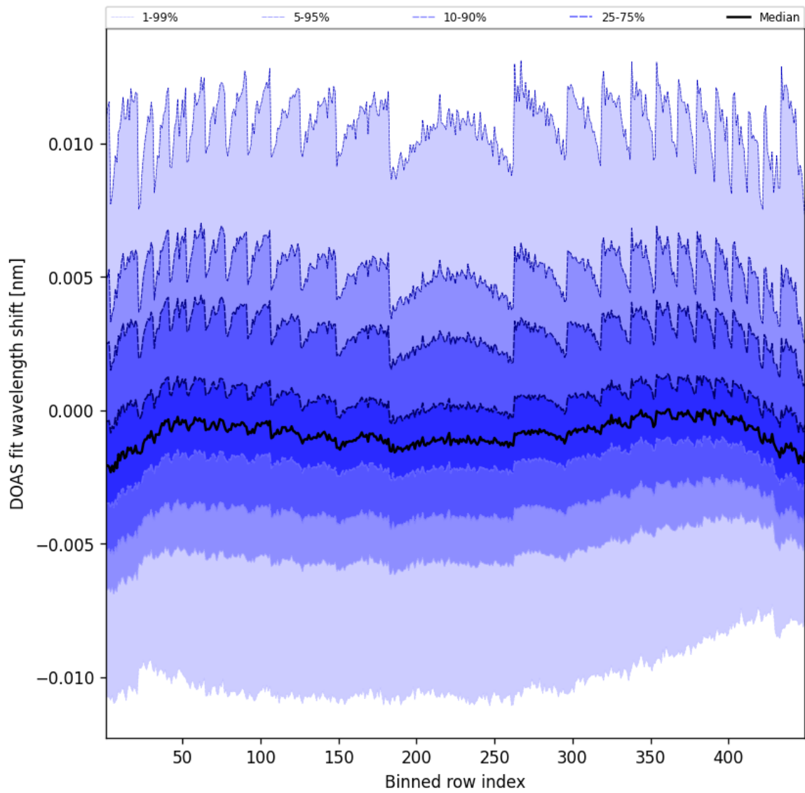
Figure 47: Along track statistics of “DOAS fit wavelength shift” for 2025-05-27 to 2025-05-28
