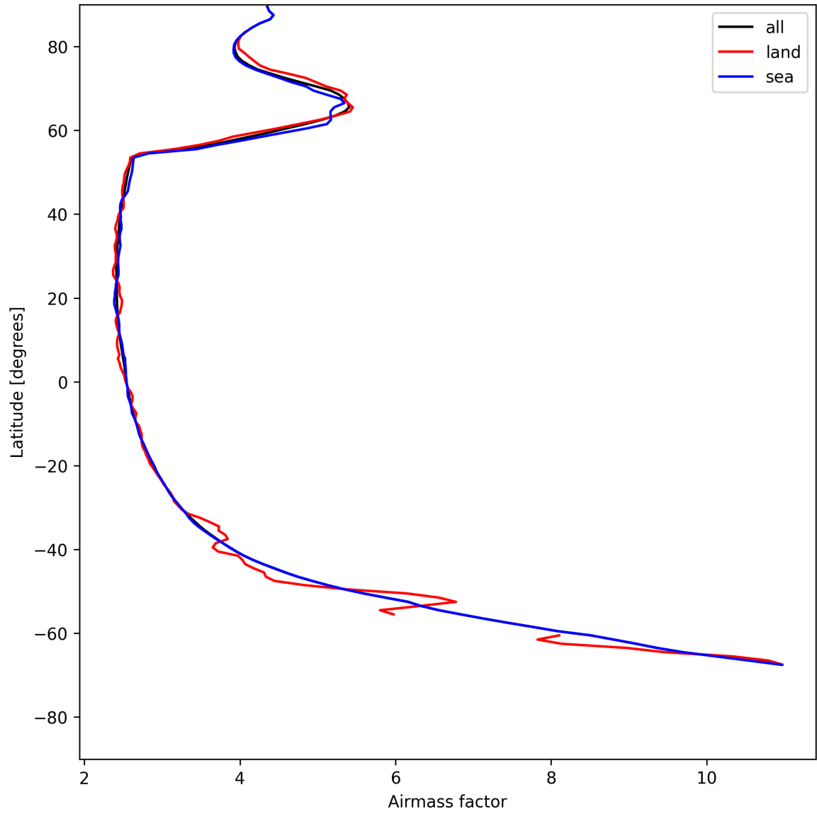
Figure 25: Zonal average of “Airmass factor” for 2025-05-27 to 2025-05-28.
