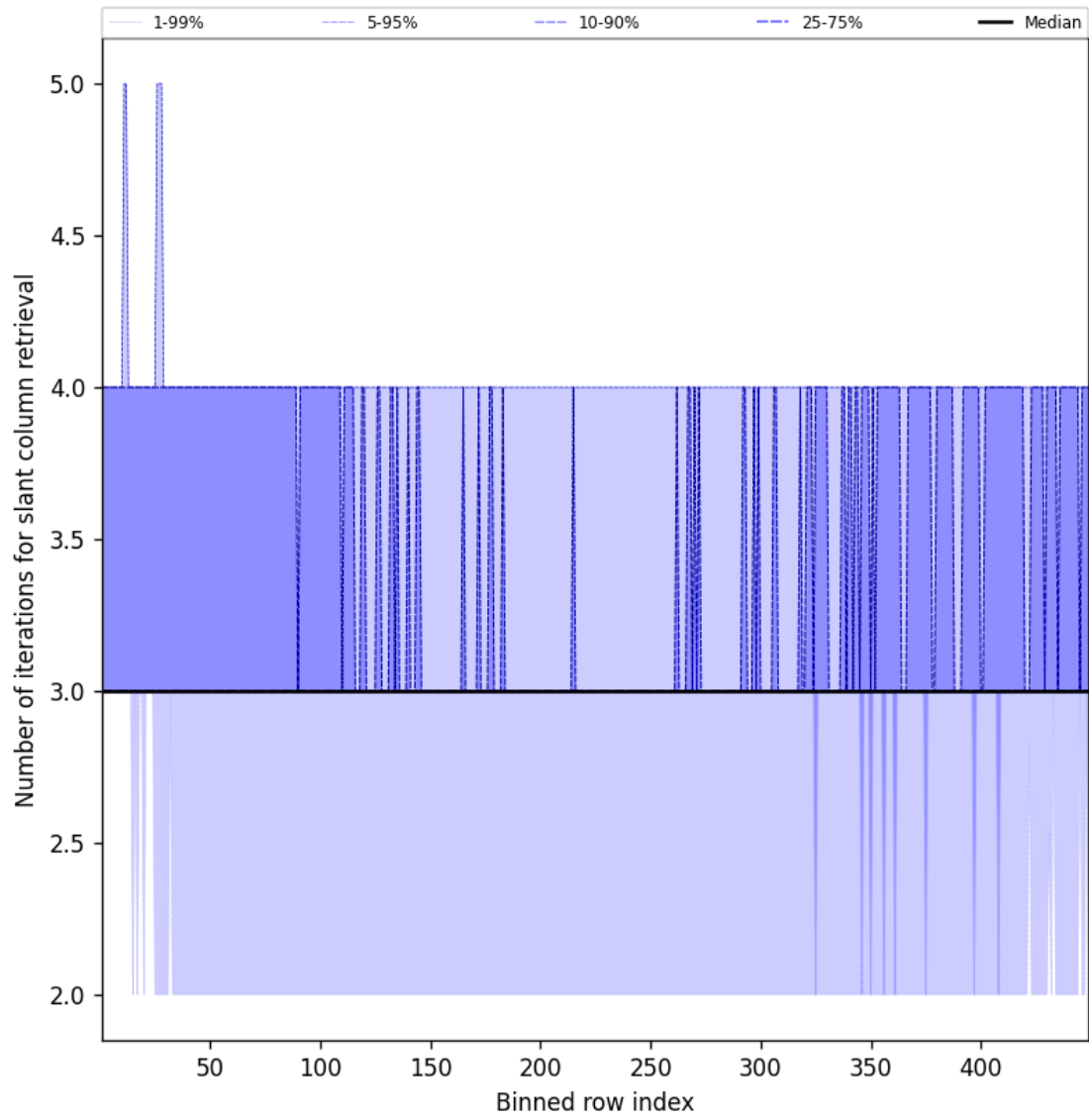
Figure 45: Along track statistics of “Number of iterations for slant column retrieval” for 2025-05-27 to 2025-05-28
