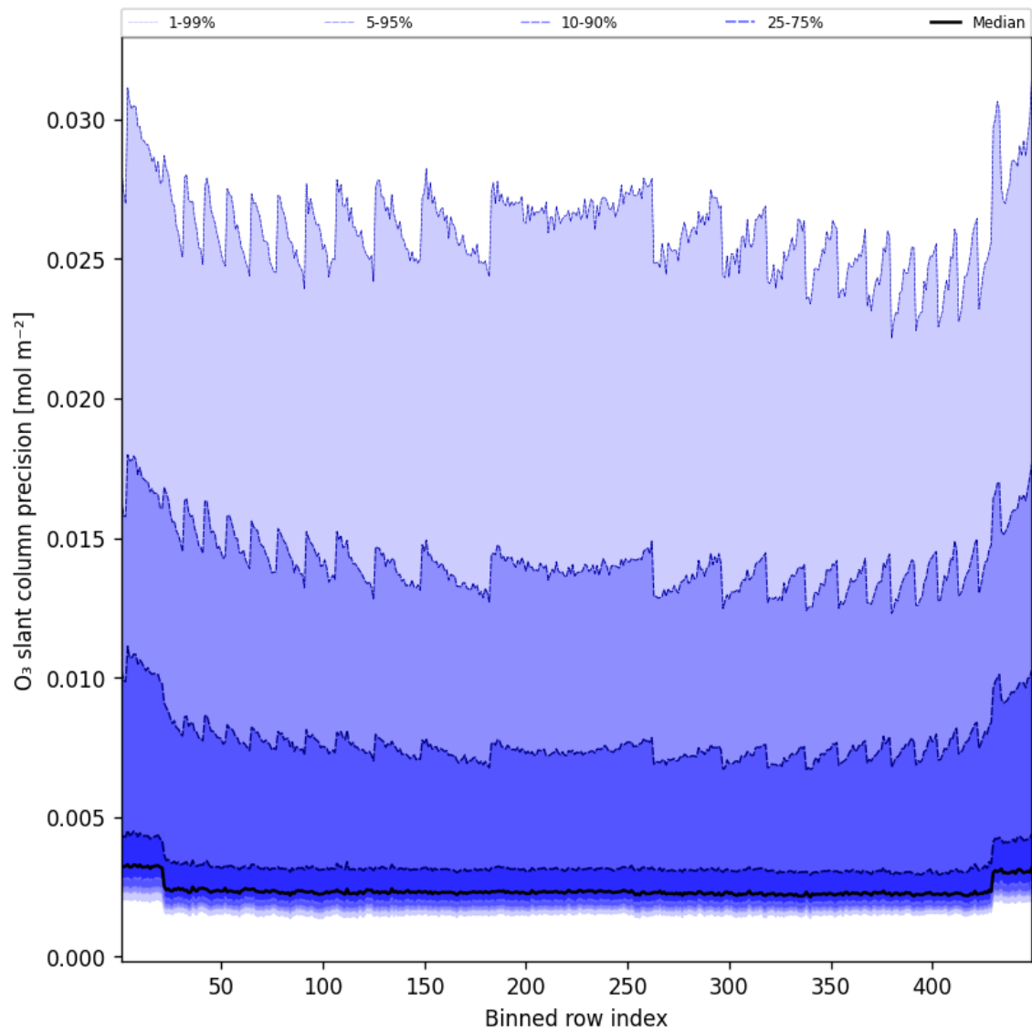
Figure 44: Along track statistics of “O 3 slant column precision” for 2025-05-27 to 2025-05-28
