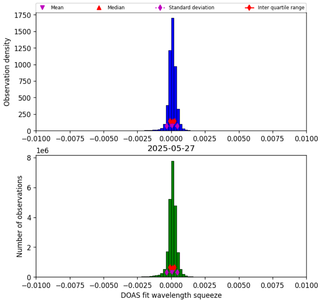
Figure 36: Histogram of “DOAS fit wavelength squeeze” for 2025-05-27 to 2025-05-28
