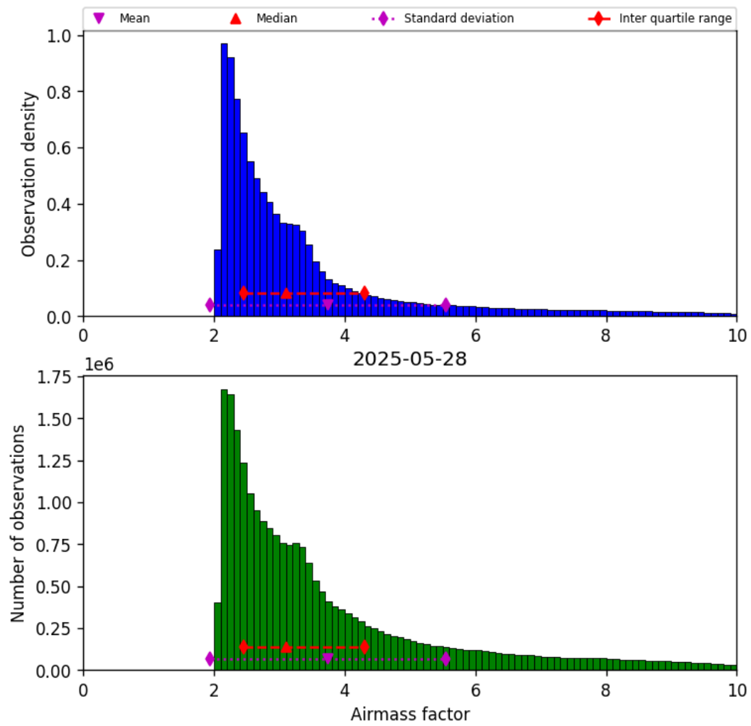
Figure 37: Histogram of “Airmass factor” for 2025-05-28 to 2025-05-29
