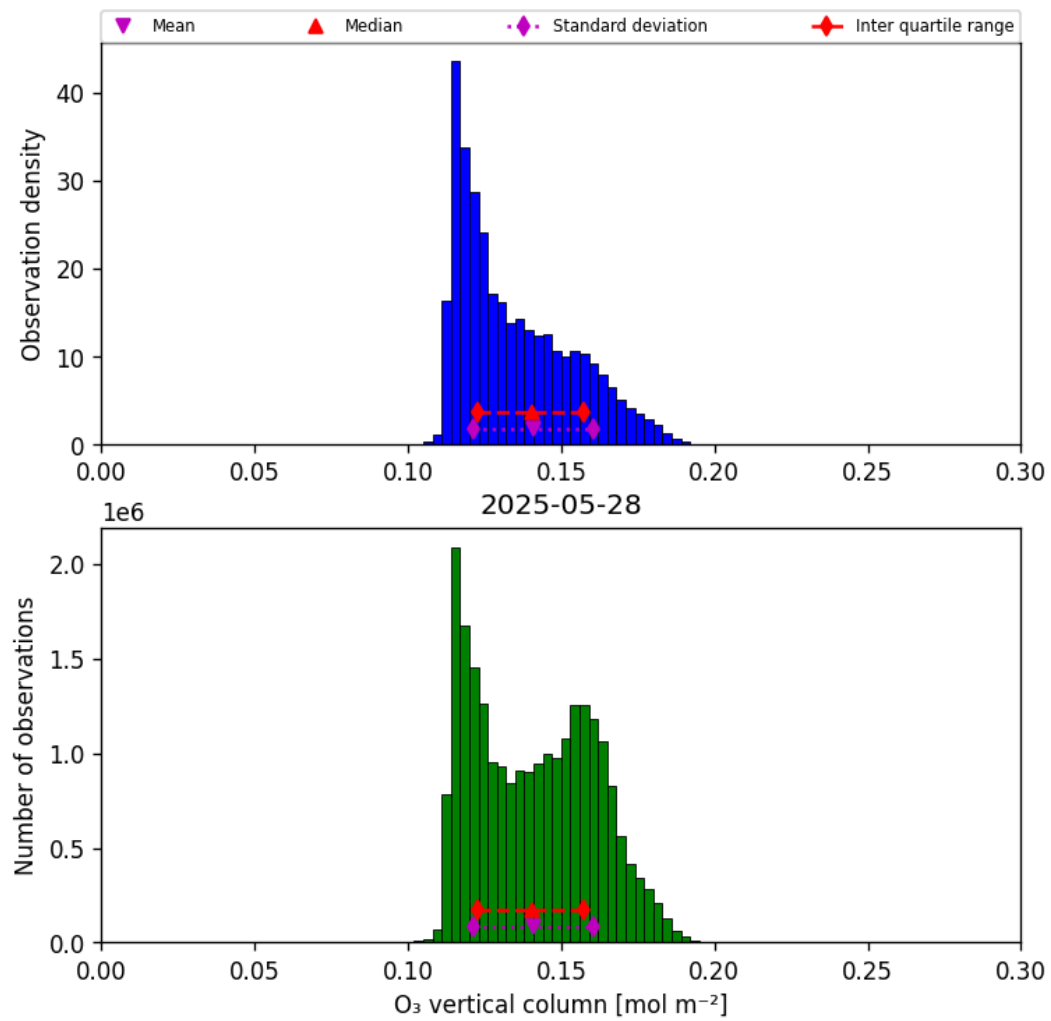
Figure 29: Histogram of “O 3 vertical column” for 2025-05-28 to 2025-05-29
