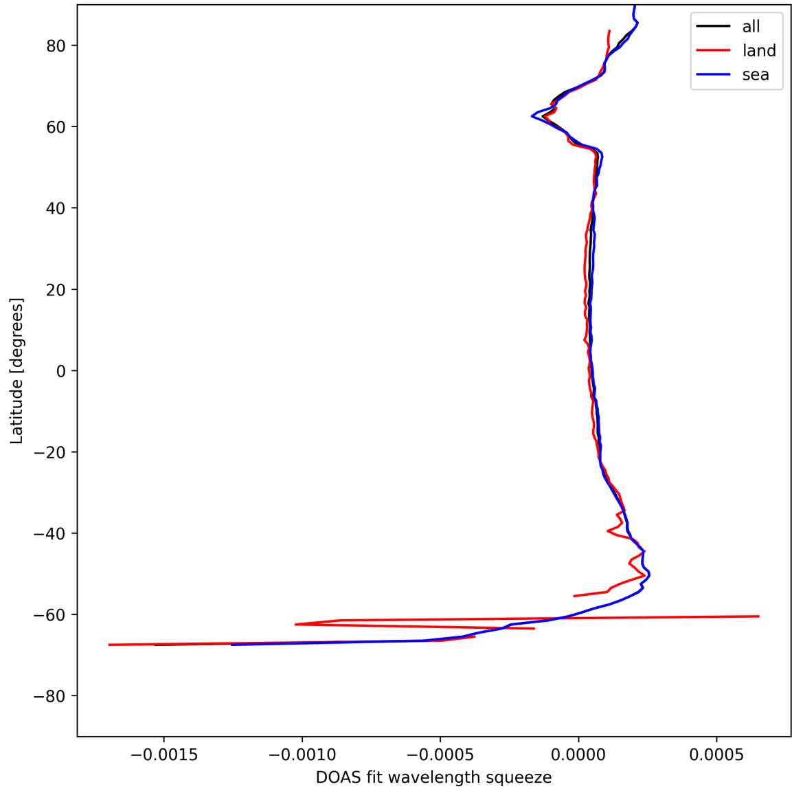
Figure 24: Zonal average of “DOAS fit wavelength squeeze” for 2025-05-28 to 2025-05-29.
