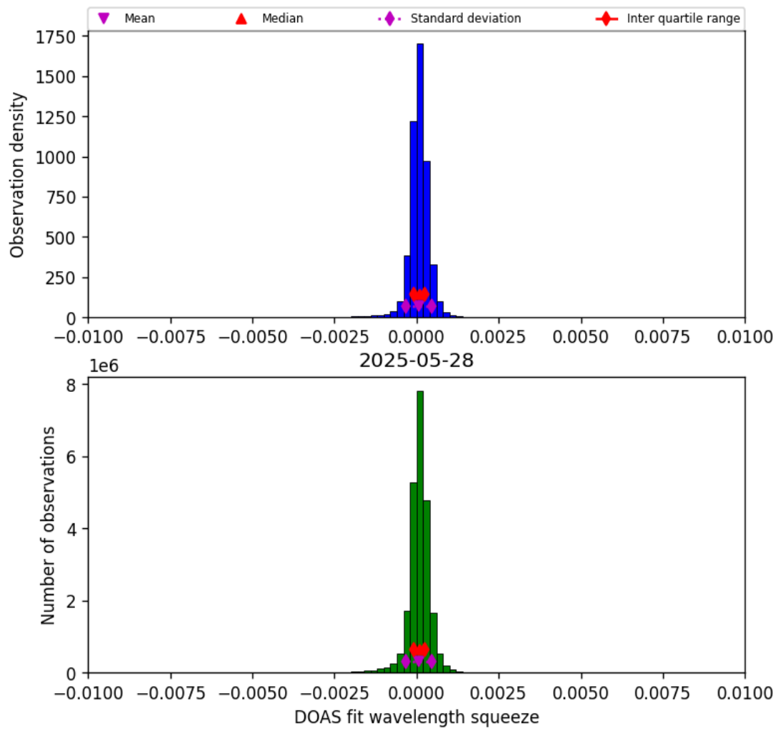
Figure 36: Histogram of “DOAS fit wavelength squeeze” for 2025-05-28 to 2025-05-29
