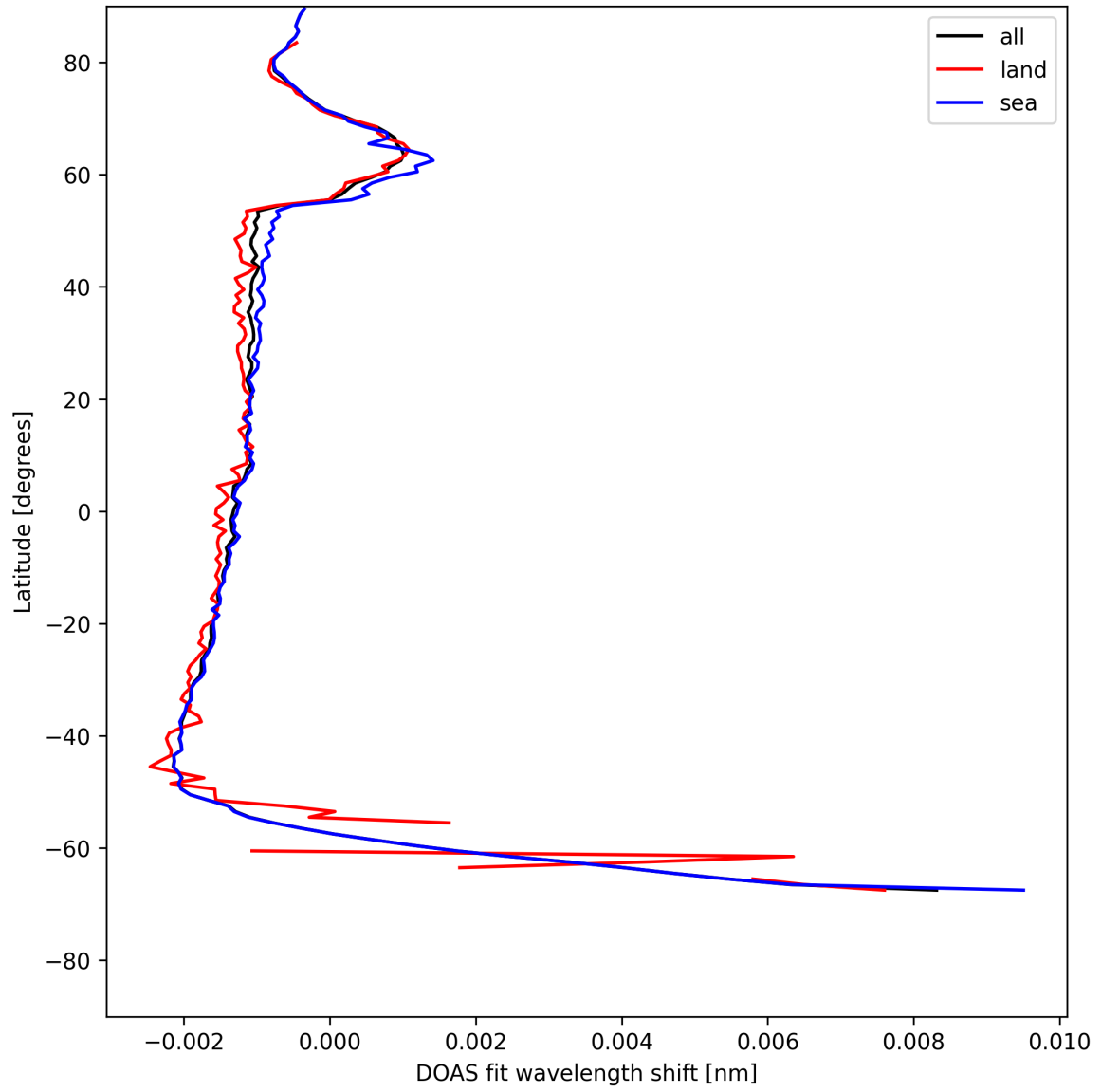
Figure 23: Zonal average of “DOAS fit wavelength shift” for 2025-05-28 to 2025-05-29.
