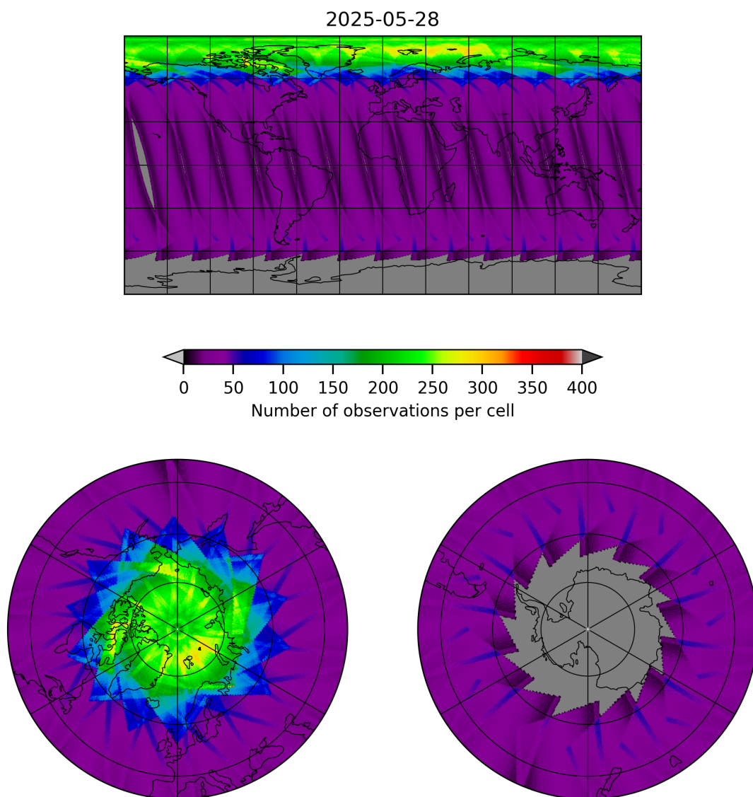
Figure 15: Map of the number of observations for 2025-05-28 to 2025-05-29
