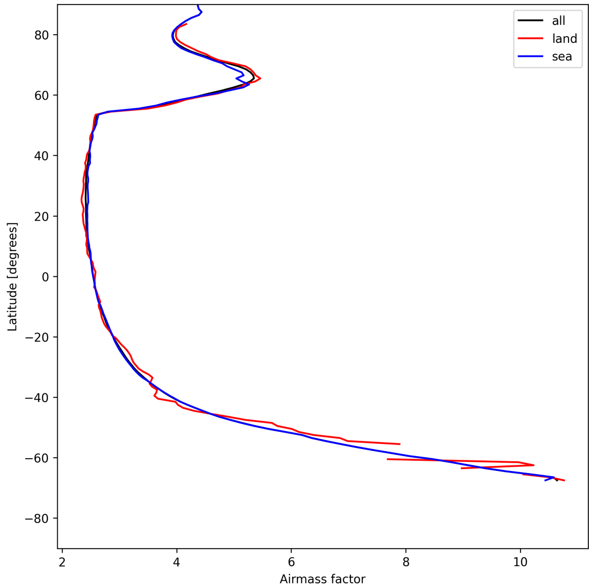
Figure 25: Zonal average of “Airmass factor” for 2025-05-28 to 2025-05-29.
