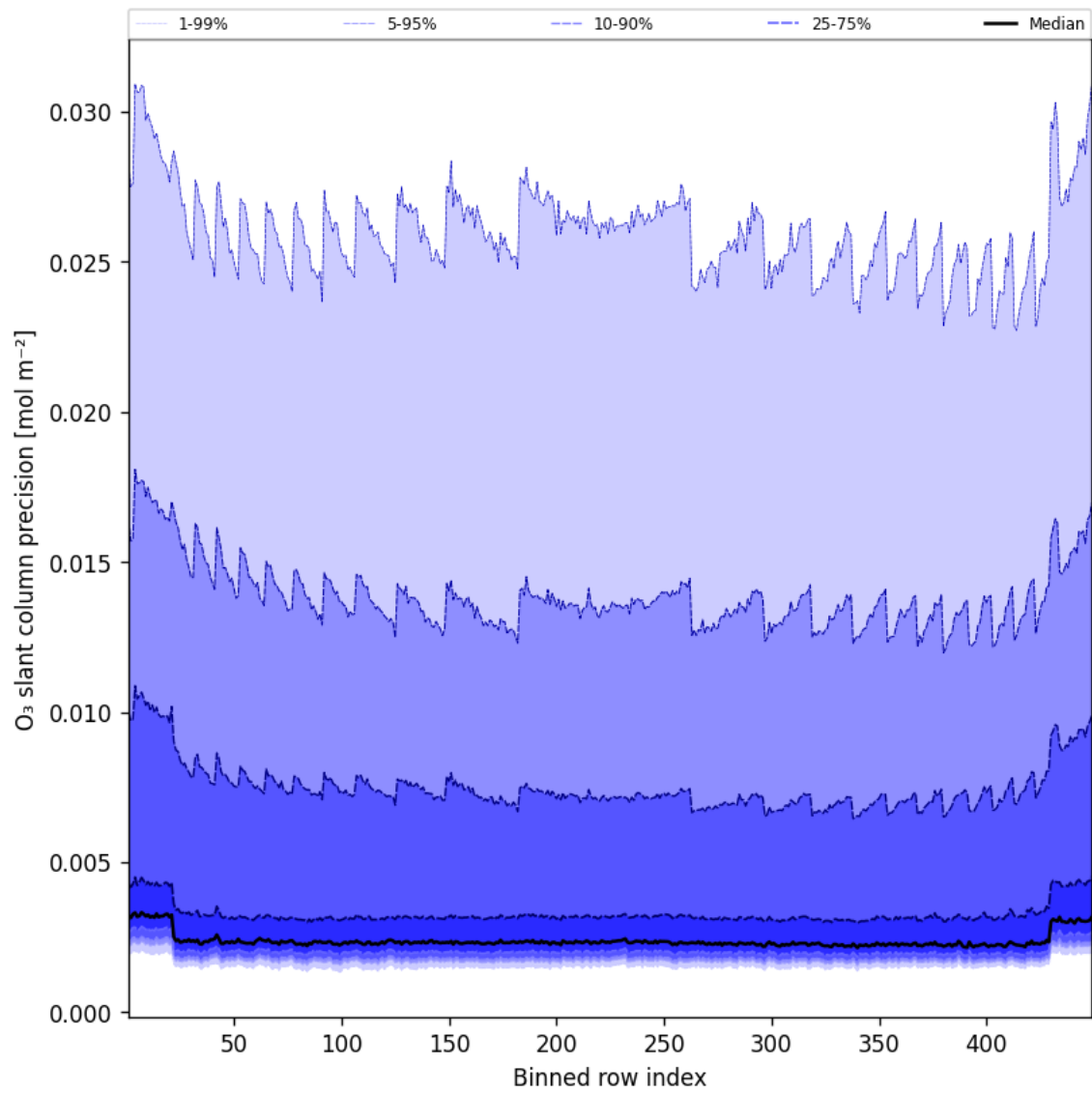
Figure 44: Along track statistics of “O 3 slant column precision” for 2025-05-28 to 2025-05-29
