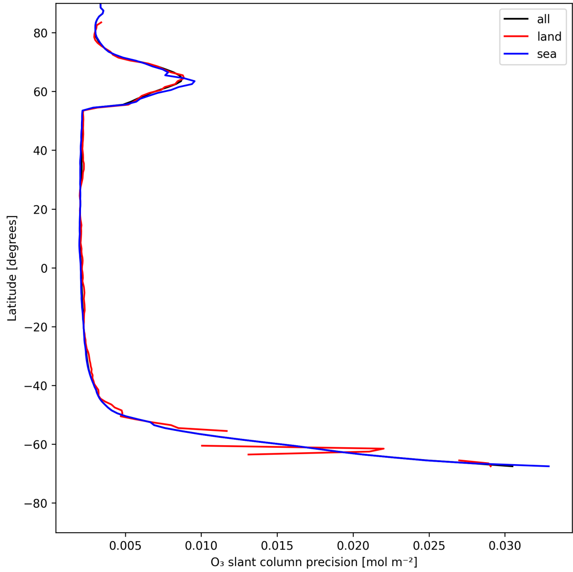
Figure 20: Zonal average of “O 3 slant column precision” for 2025-05-28 to 2025-05-29.
