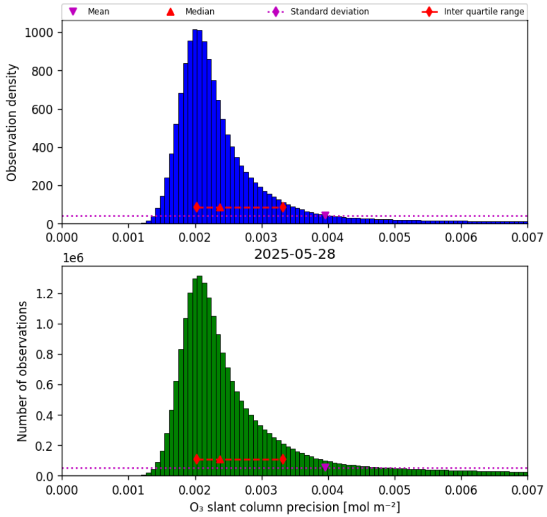
Figure 32: Histogram of “O 3 slant column precision” for 2025-05-28 to 2025-05-29
