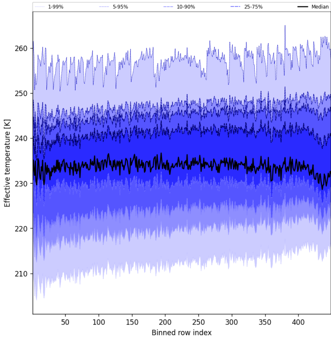
Figure 50: Along track statistics of “Effective temperature” for 2025-05-28 to 2025-05-29
