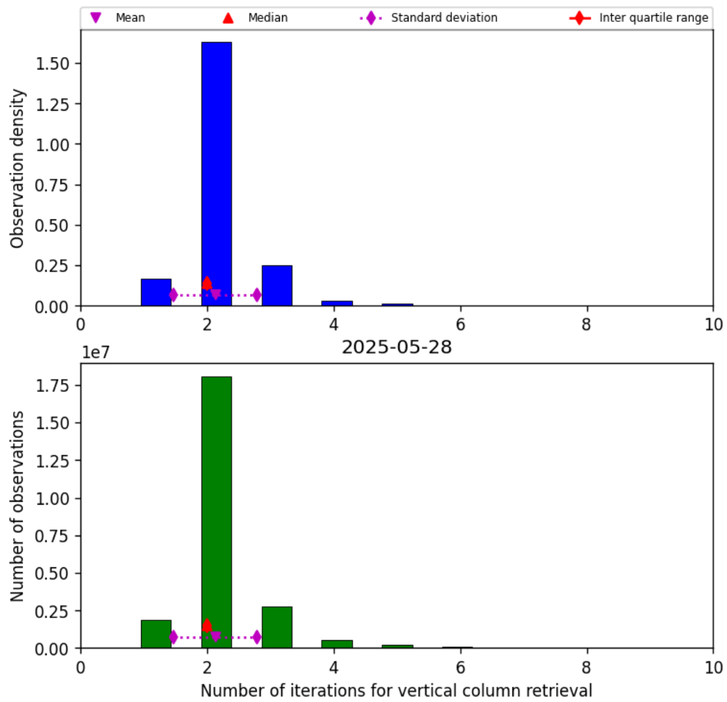
Figure 39: Histogram of “Number of iterations for vertical column retrieval” for 2025-05-28 to 2025-05-29
