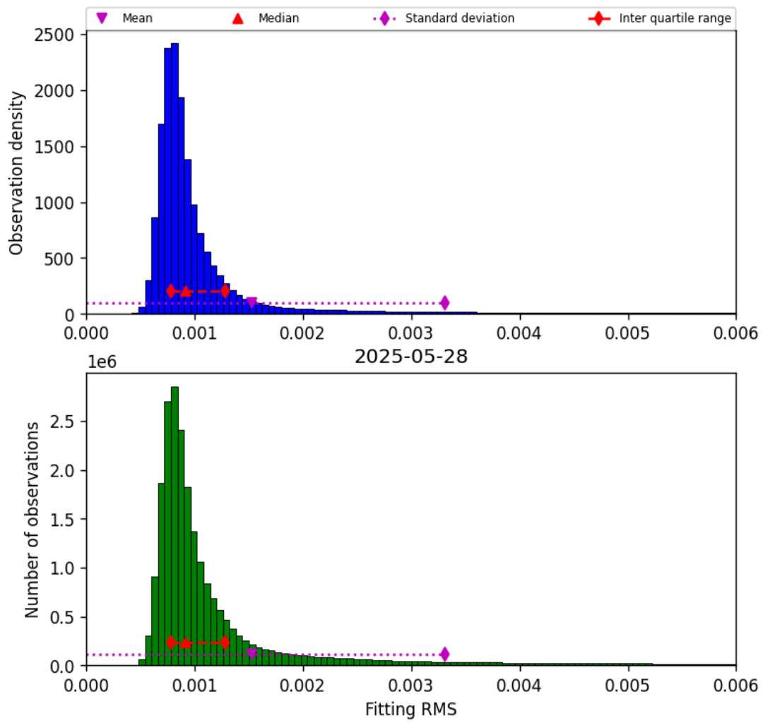
Figure 34: Histogram of “Fitting RMS” for 2025-05-28 to 2025-05-29
