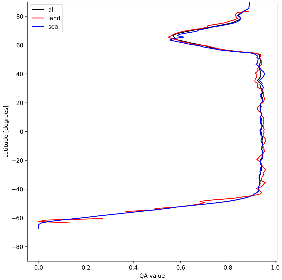
Figure 16: Zonal average of “QA value” for 2025-05-28 to 2025-05-29.
