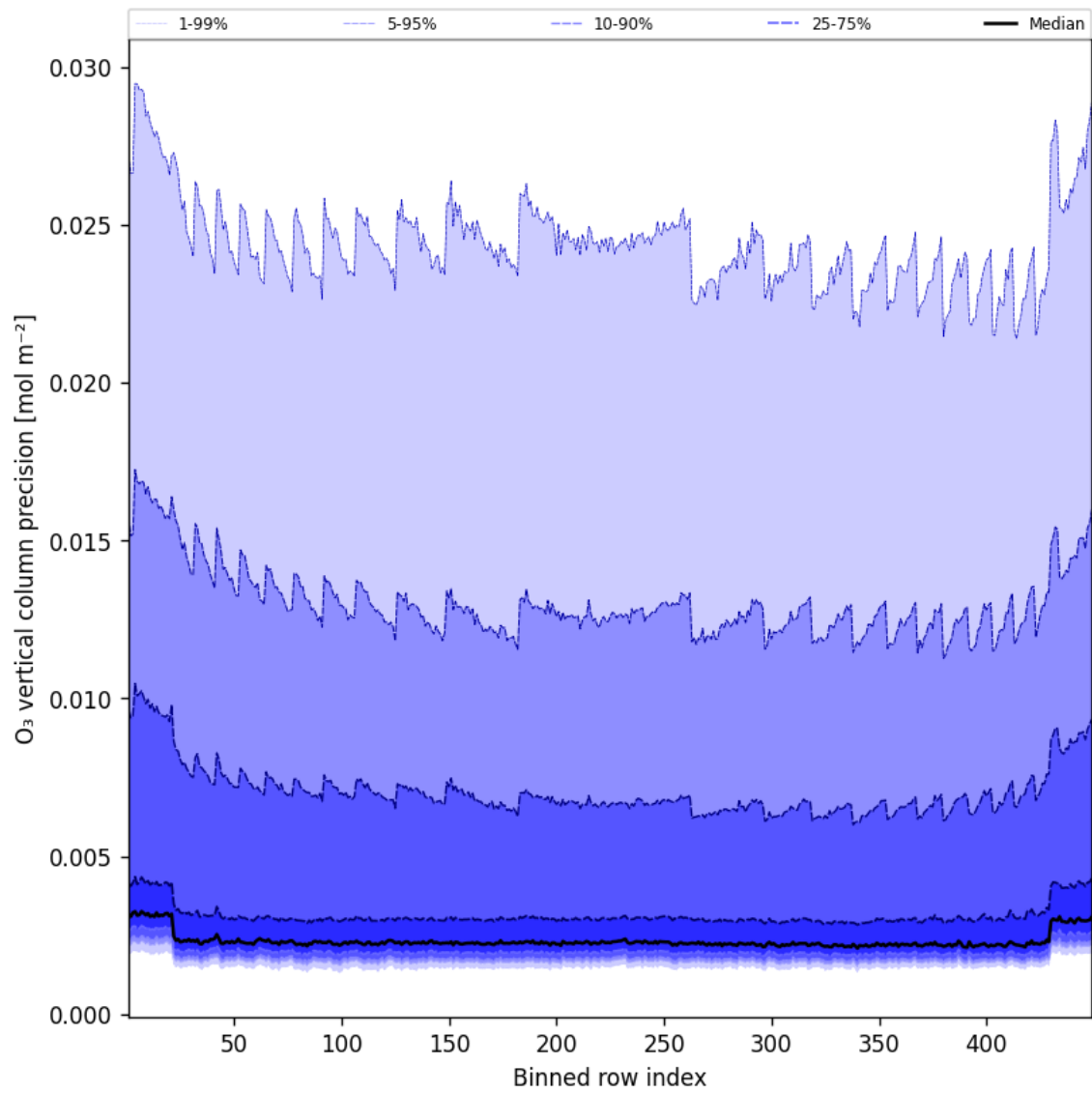
Figure 42: Along track statistics of “O 3 vertical column precision” for 2025-05-28 to 2025-05-29
