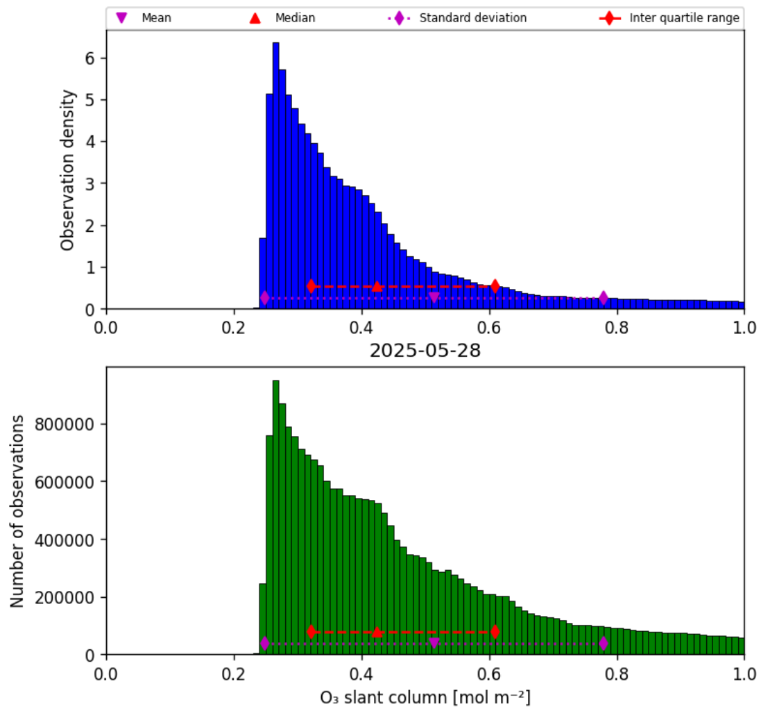
Figure 31: Histogram of “O 3 slant column” for 2025-05-28 to 2025-05-29
