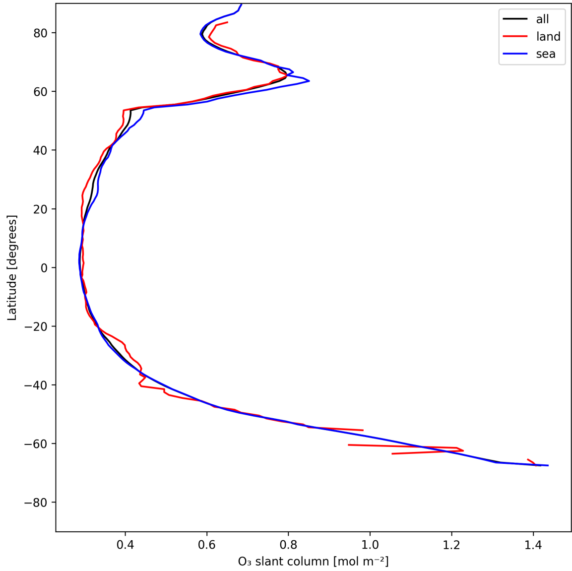
Figure 19: Zonal average of “O 3 slant column” for 2025-05-28 to 2025-05-29.
