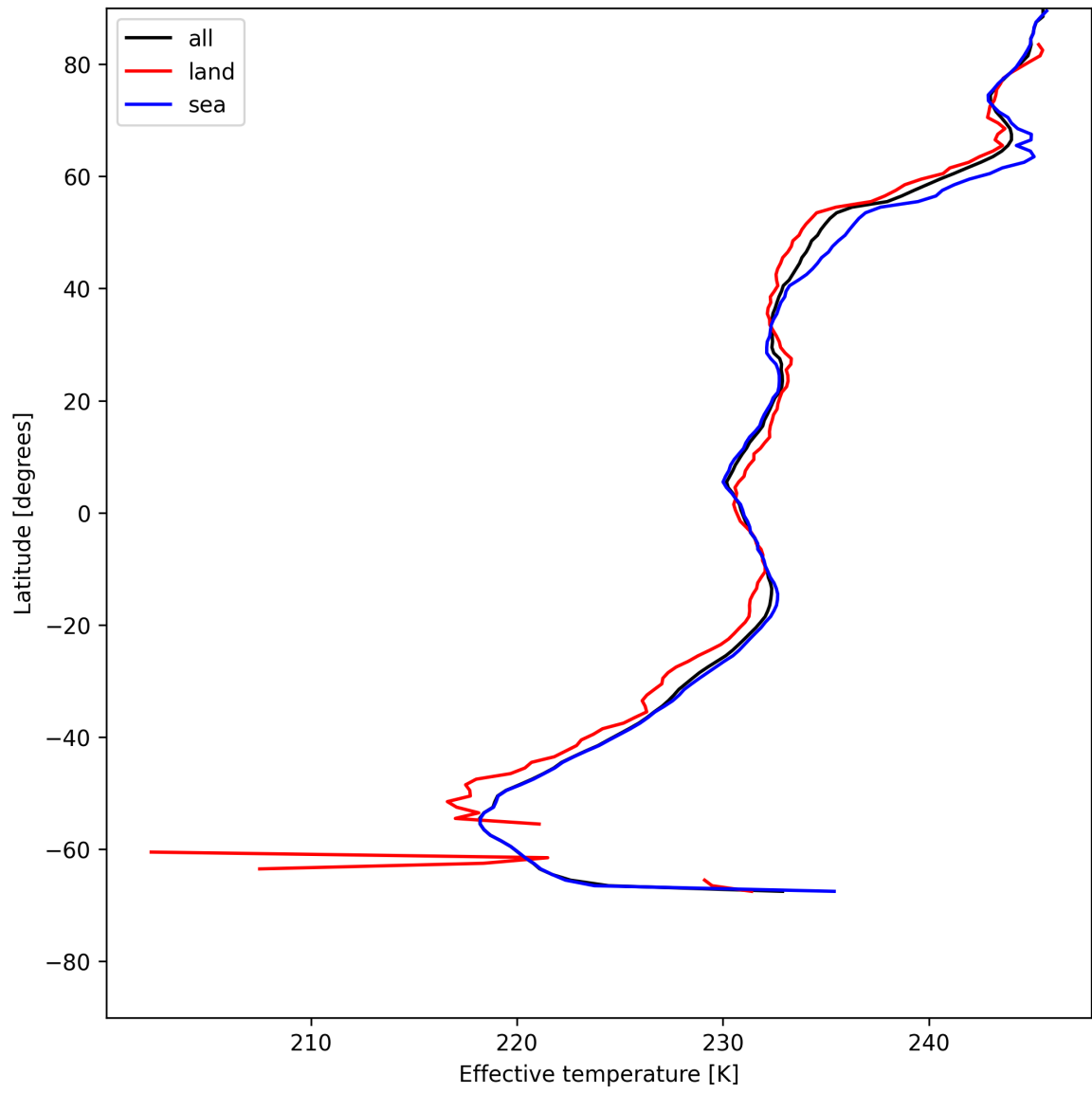
Figure 26: Zonal average of "Effective temperature" for 2025-05-28 to 2025-05-29.
