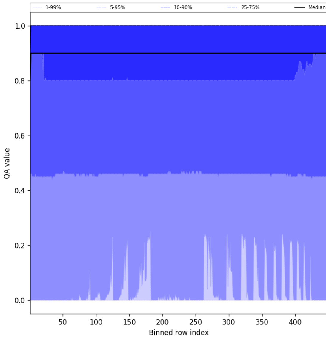
Figure 40: Along track statistics of “QA value” for 2025-05-28 to 2025-05-29
