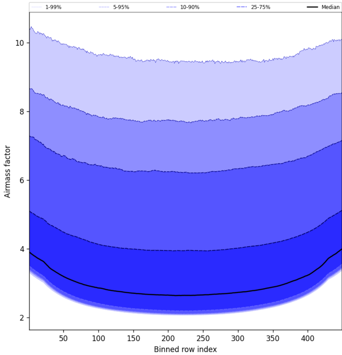
Figure 49: Along track statistics of “Airmass factor” for 2025-05-28 to 2025-05-29
