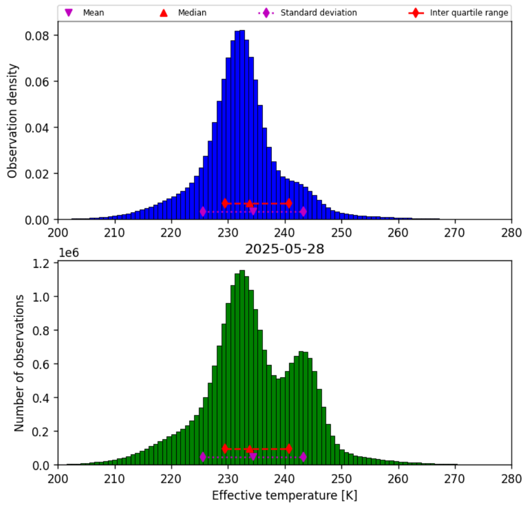
Figure 38: Histogram of “Effective temperature” for 2025-05-28 to 2025-05-29
