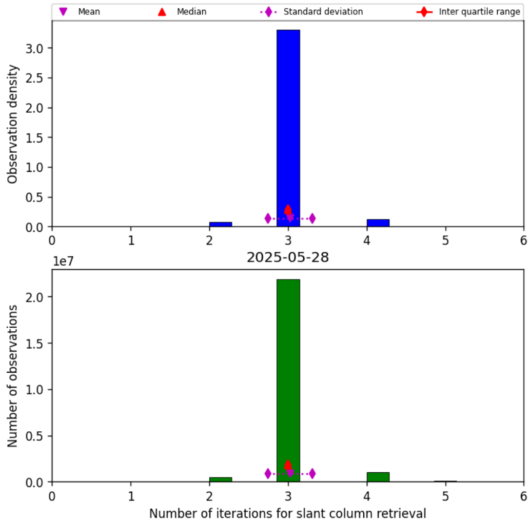
Figure 33: Histogram of “Number of iterations for slant column retrieval” for 2025-05-28 to 2025-05-29
