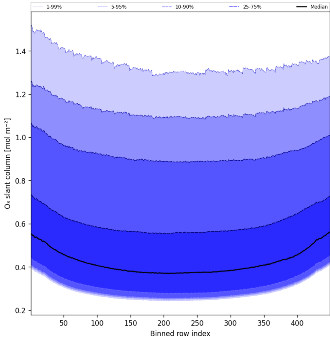
Figure 43: Along track statistics of “O 3 slant column” for 2025-05-28 to 2025-05-29
