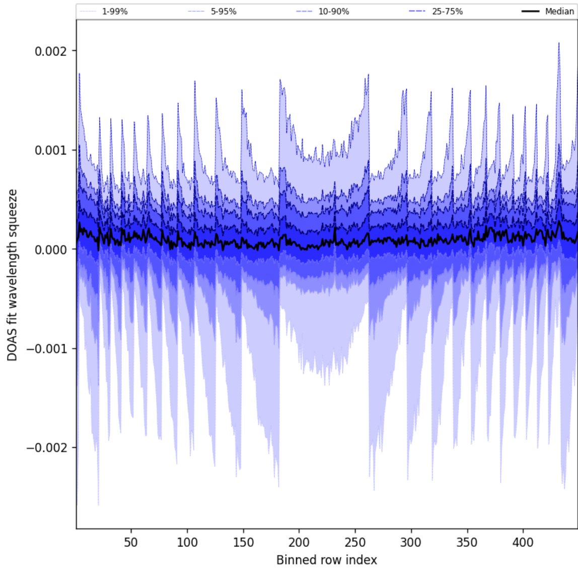
Figure 48: Along track statistics of “DOAS fit wavelength squeeze” for 2025-05-28 to 2025-05-29
