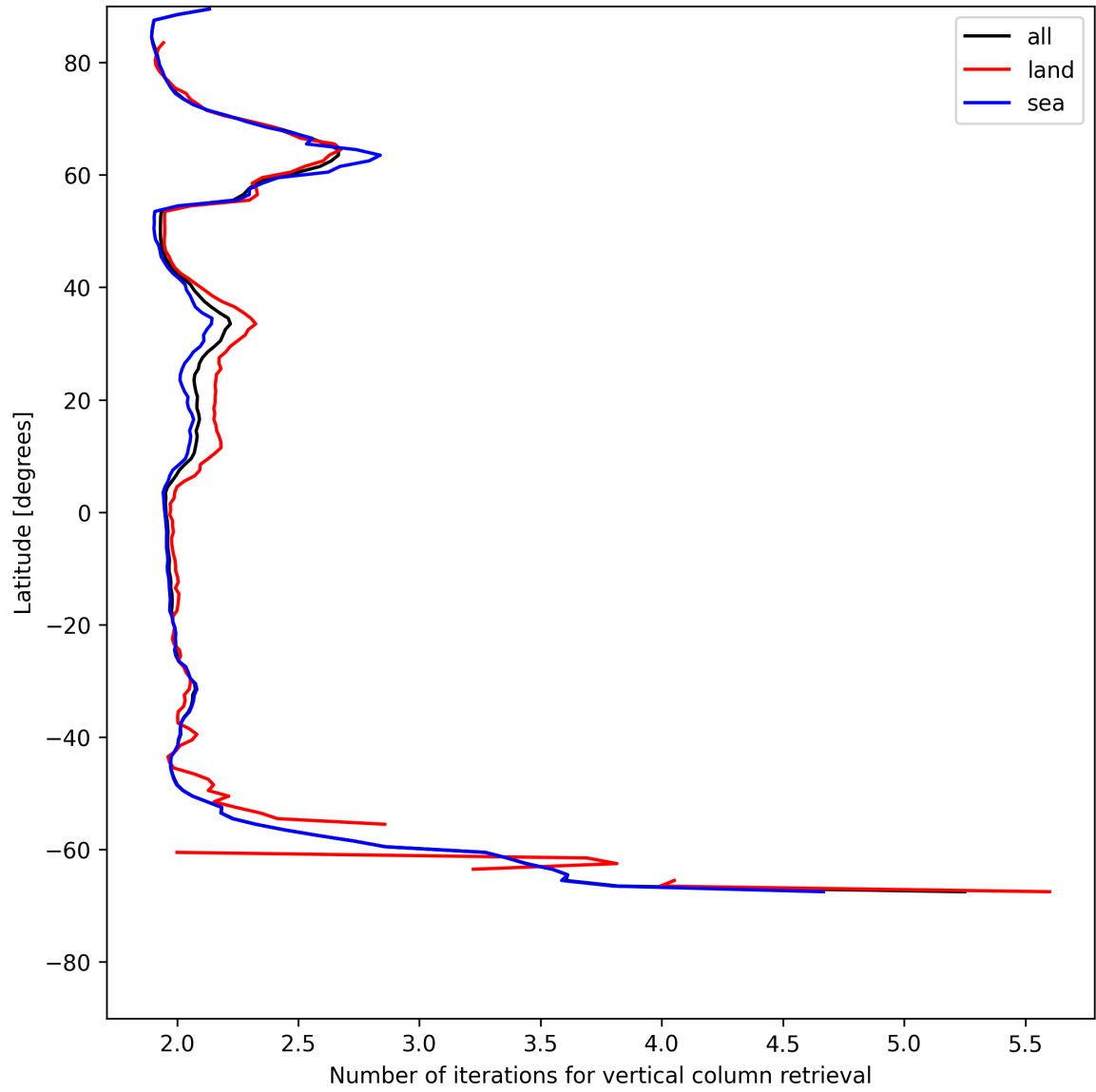
Figure 27: Zonal average of “Number of iterations for vertical column retrieval” for 2025-05-28 to 2025-05-29.
