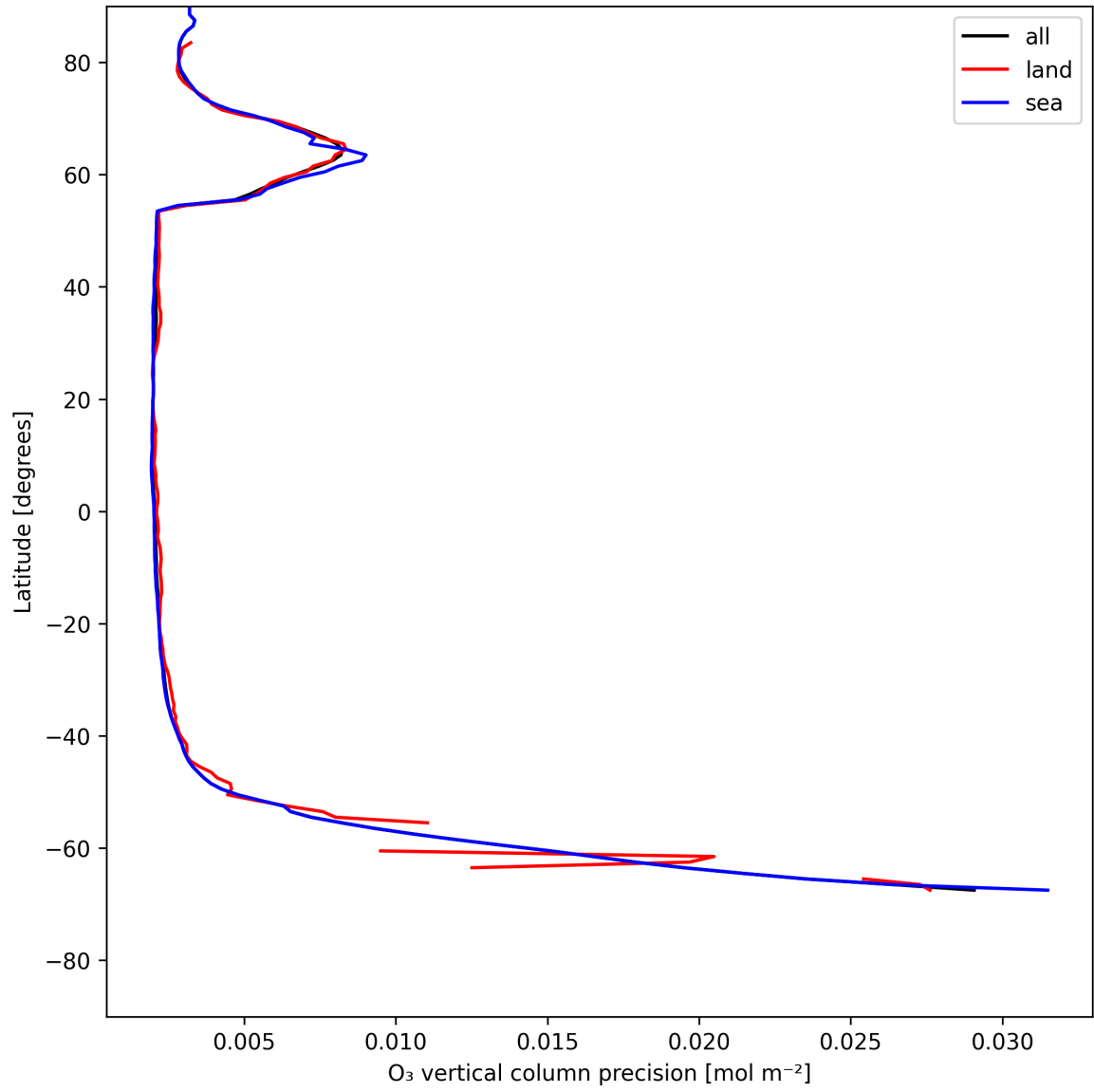
Figure 18: Zonal average of “O 3 vertical column precision” for 2025-05-28 to 2025-05-29.
