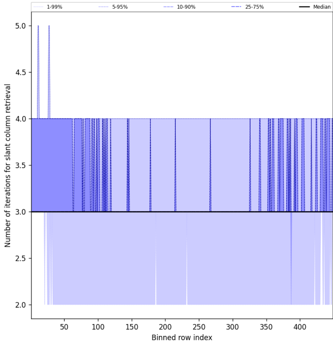
Figure 45: Along track statistics of “Number of iterations for slant column retrieval” for 2025-05-28 to 2025-05-29
