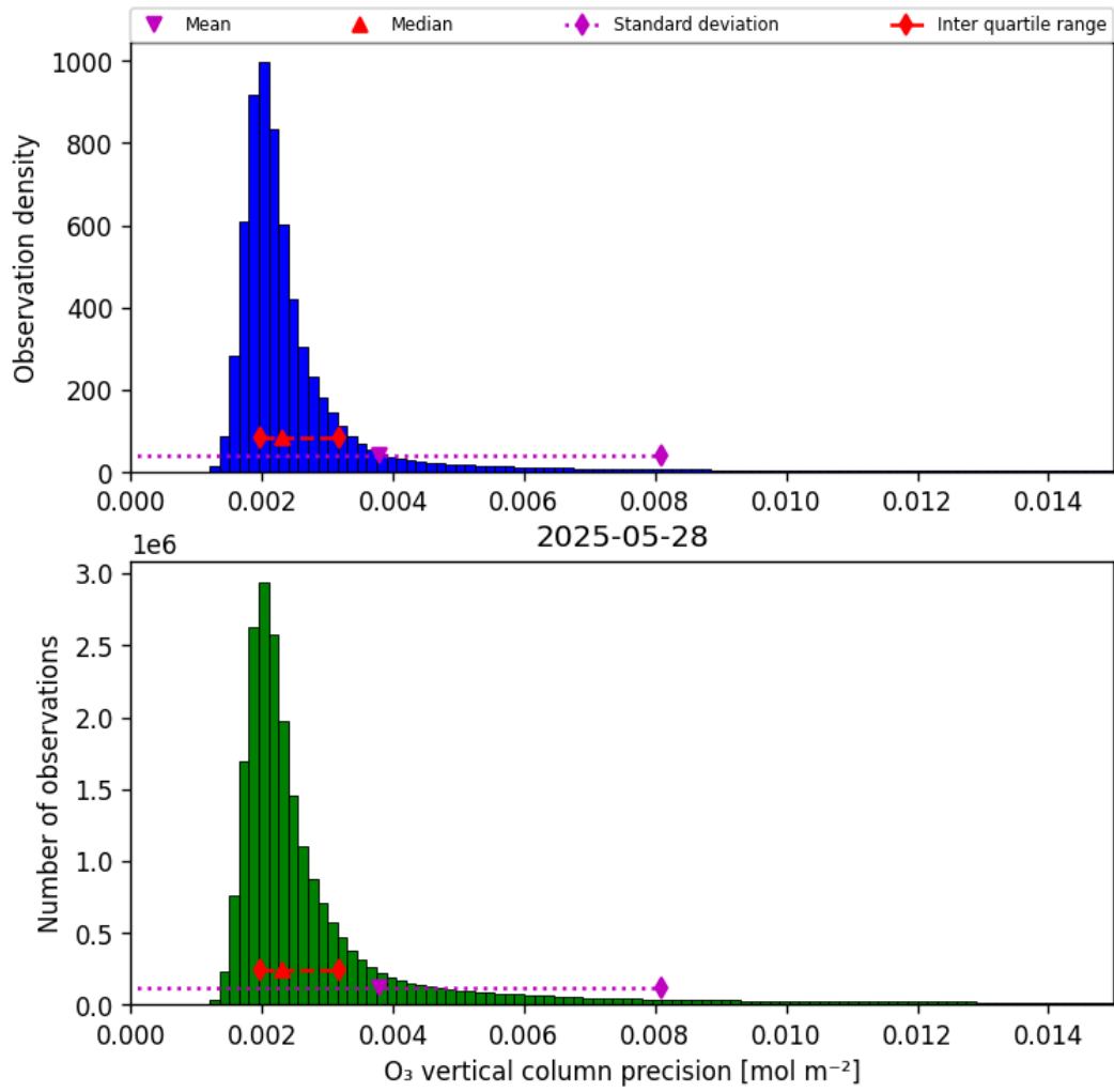
Figure 30: Histogram of “O 3 vertical column precision” for 2025-05-28 to 2025-05-29
