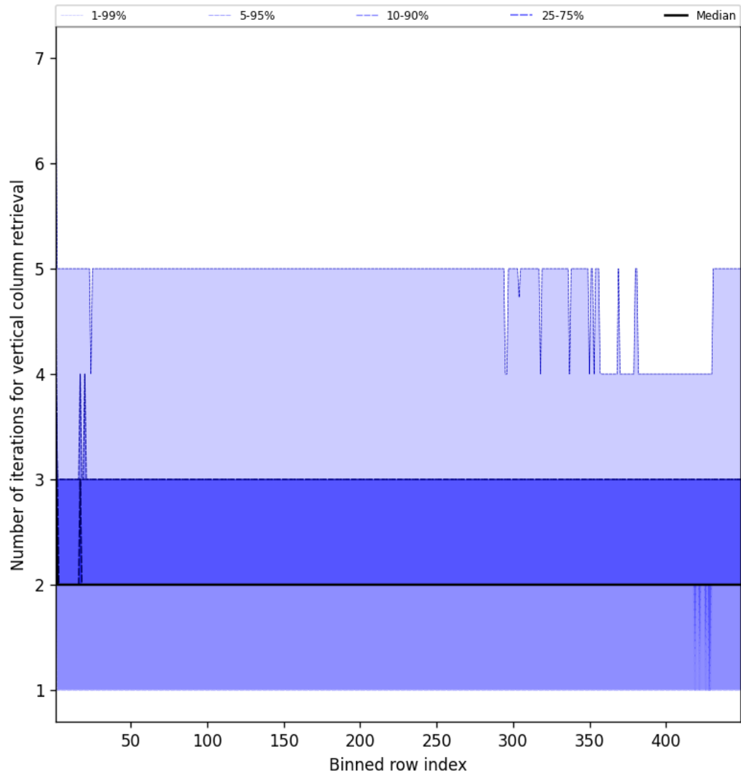
Figure 51: Along track statistics of “Number of iterations for vertical column retrieval” for 2025-05-28 to 2025-05-29
