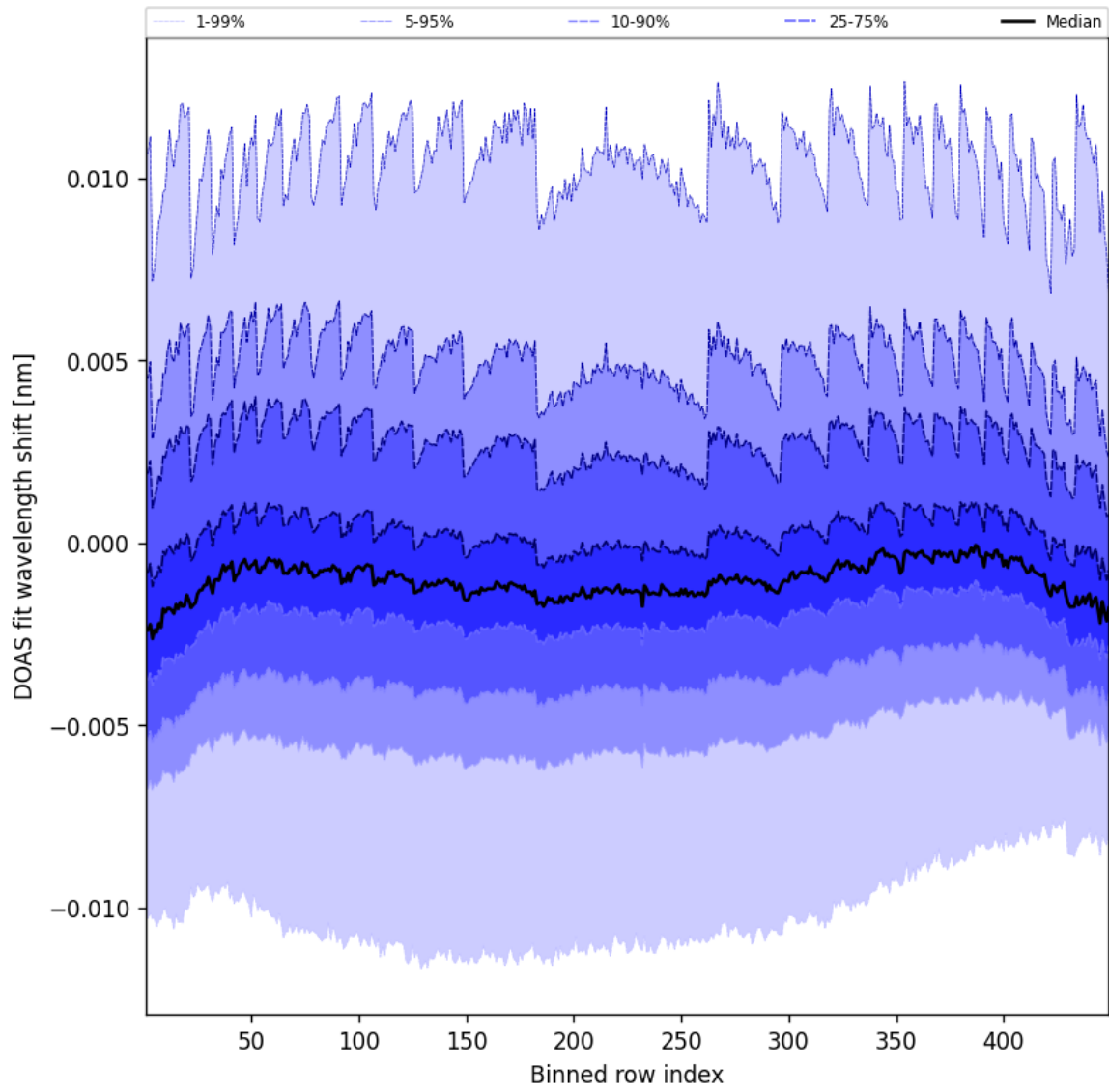
Figure 47: Along track statistics of “DOAS fit wavelength shift” for 2025-05-28 to 2025-05-29
