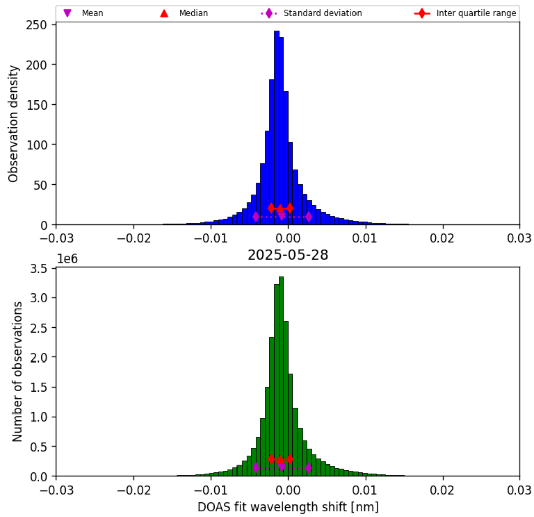
Figure 35: Histogram of “DOAS fit wavelength shift” for 2025-05-28 to 2025-05-29
