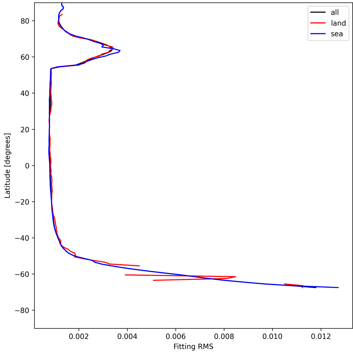
Figure 22: Zonal average of “Fitting RMS” for 2025-05-28 to 2025-05-29.
