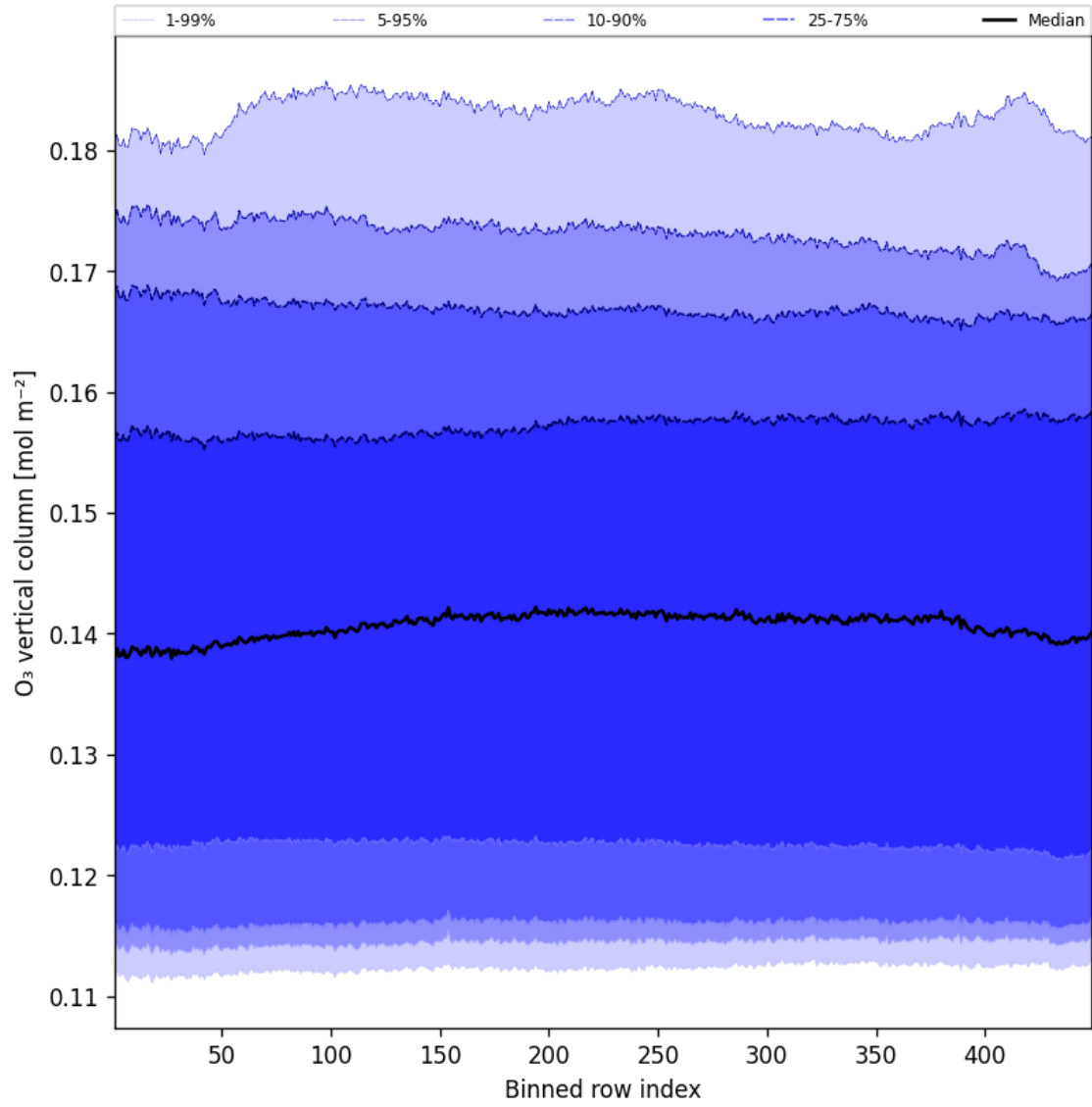
Figure 41: Along track statistics of “O 3 vertical column” for 2025-05-28 to 2025-05-29
