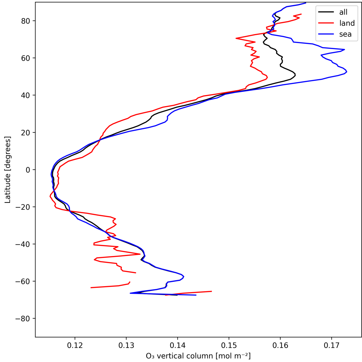
Figure 17: Zonal average of “O 3 vertical column” for 2025-05-28 to 2025-05-29.
