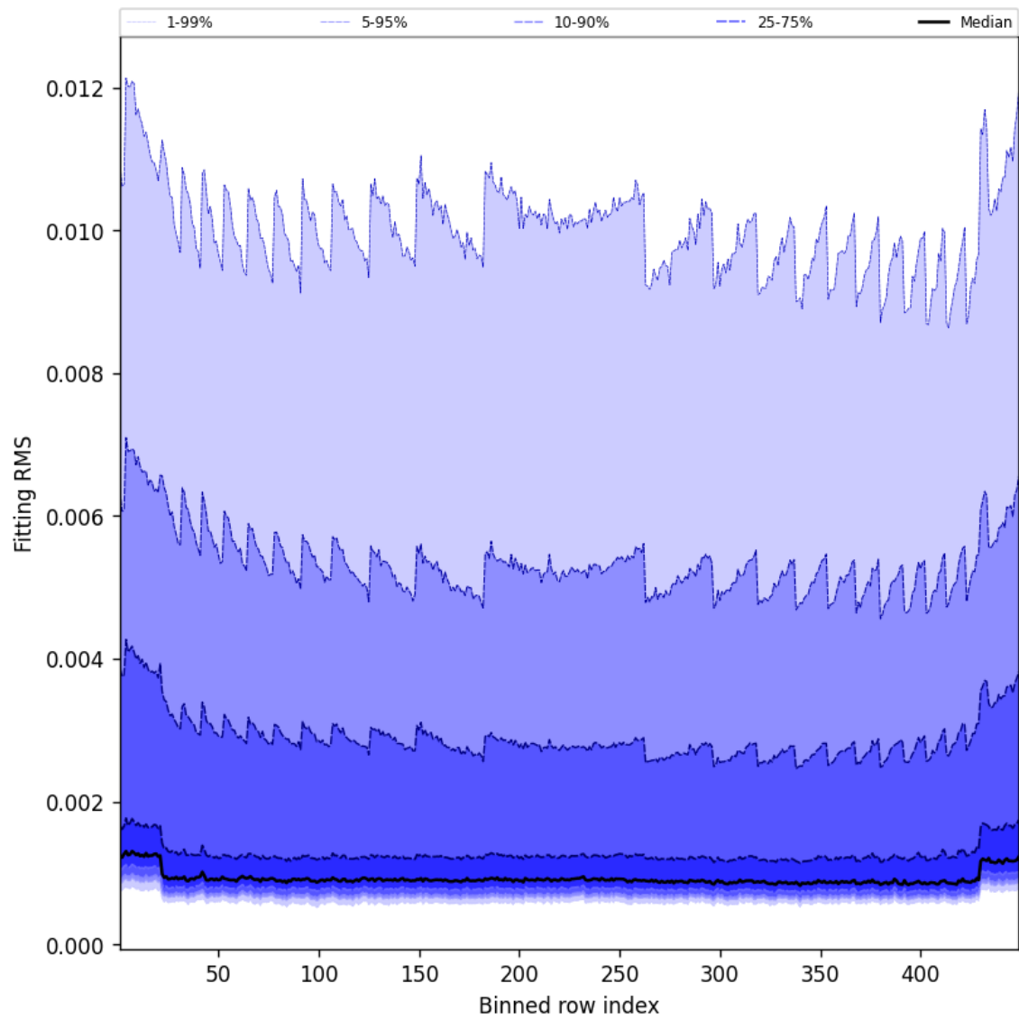
Figure 46: Along track statistics of “Fitting RMS” for 2025-05-28 to 2025-05-29
