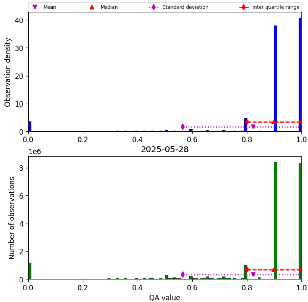
Figure 28: Histogram of “QA value” for 2025-05-28 to 2025-05-29
