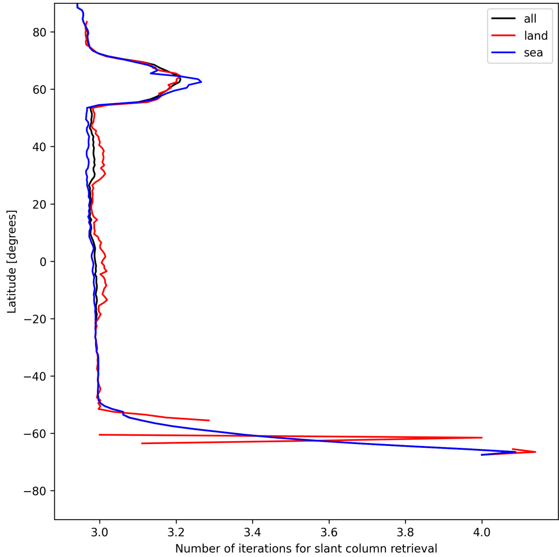
Figure 21: Zonal average of “Number of iterations for slant column retrieval” for 2025-05-28 to 2025-05-29.
