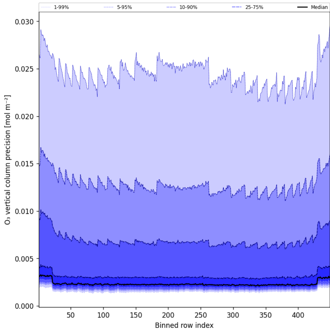
Figure 42: Along track statistics of “O 3 vertical column precision” for 2025-05-29 to 2025-05-29
