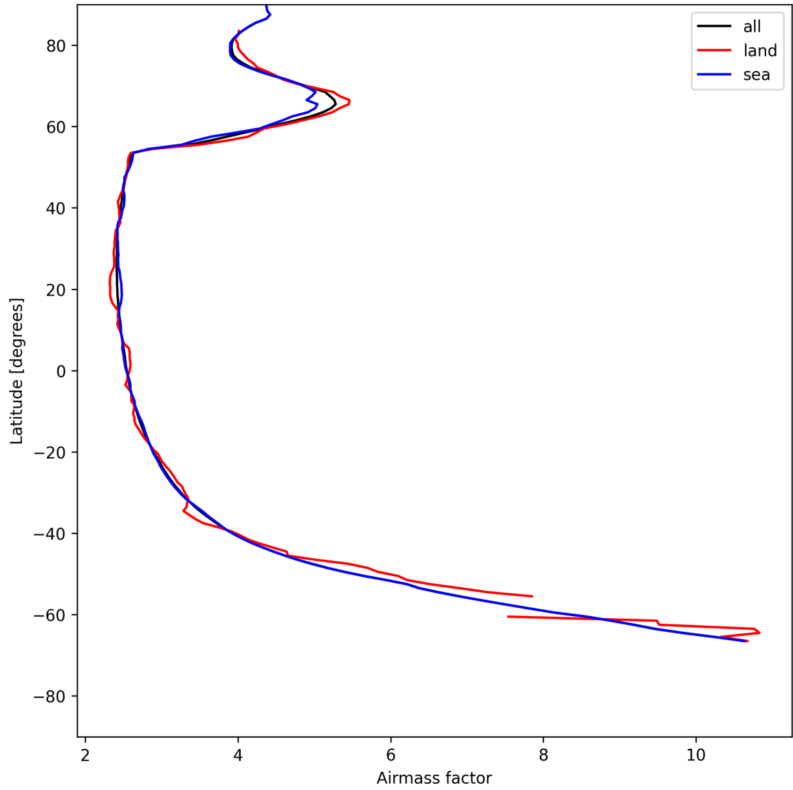
Figure 25: Zonal average of “Airmass factor” for 2025-05-29 to 2025-05-29.
