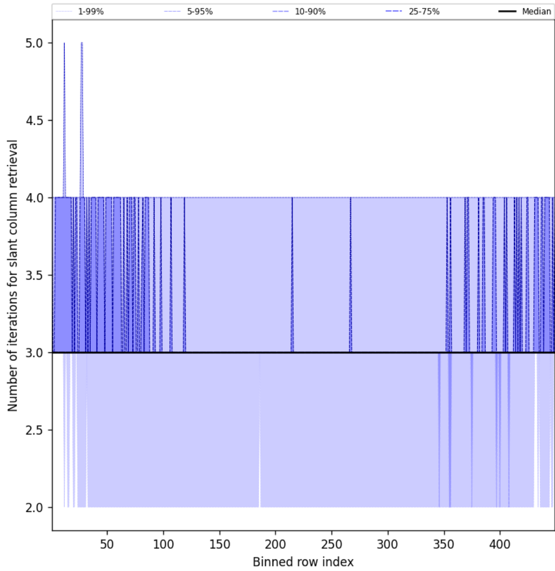
Figure 45: Along track statistics of “Number of iterations for slant column retrieval” for 2025-05-29 to 2025-05-29
