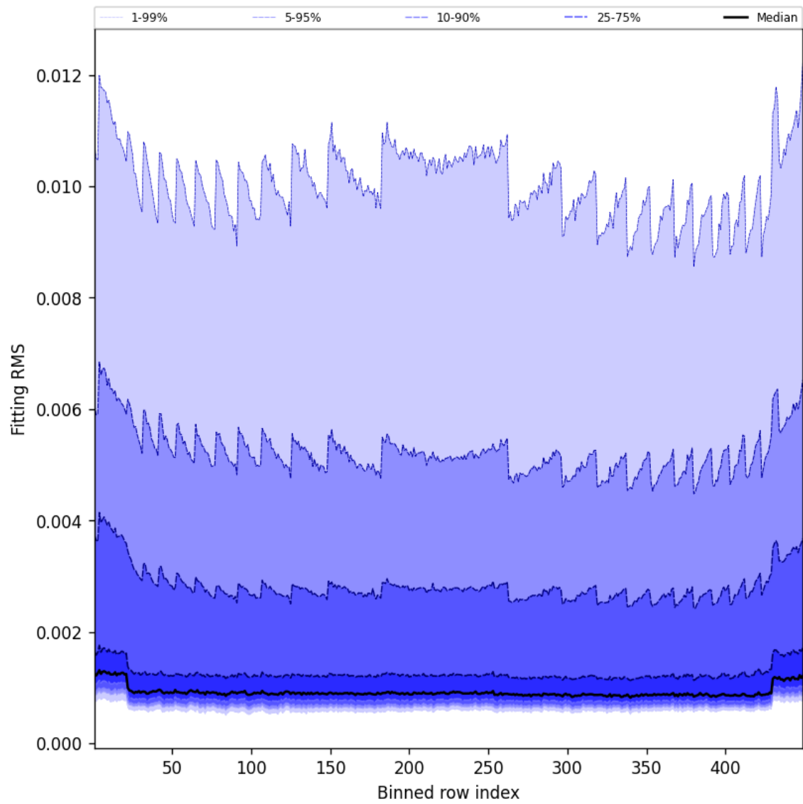
Figure 46: Along track statistics of “Fitting RMS” for 2025-05-29 to 2025-05-29
