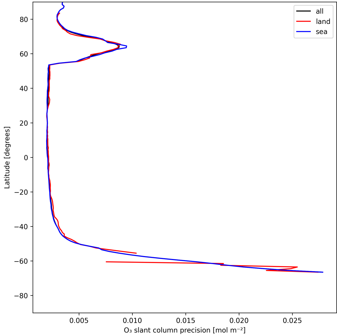
Figure 20: Zonal average of “O 3 slant column precision” for 2025-05-29 to 2025-05-29.
