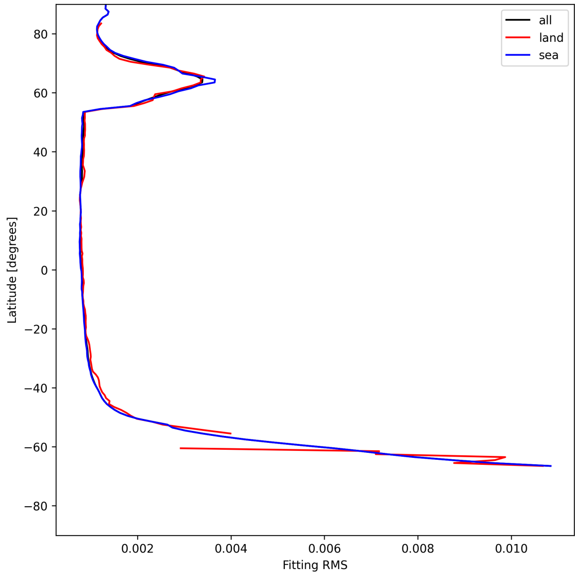
Figure 22: Zonal average of “Fitting RMS” for 2025-05-29 to 2025-05-29.
