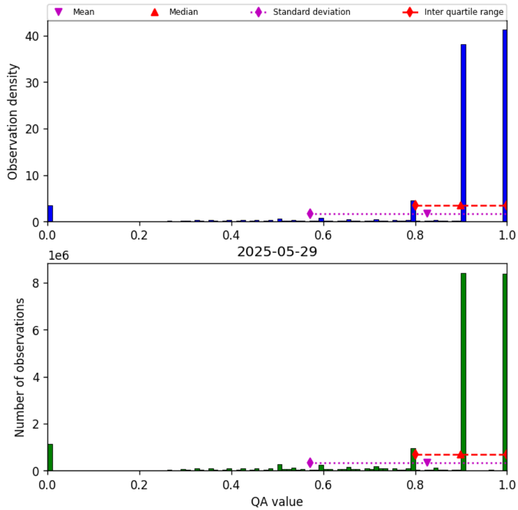
Figure 28: Histogram of “QA value” for 2025-05-29 to 2025-05-29
