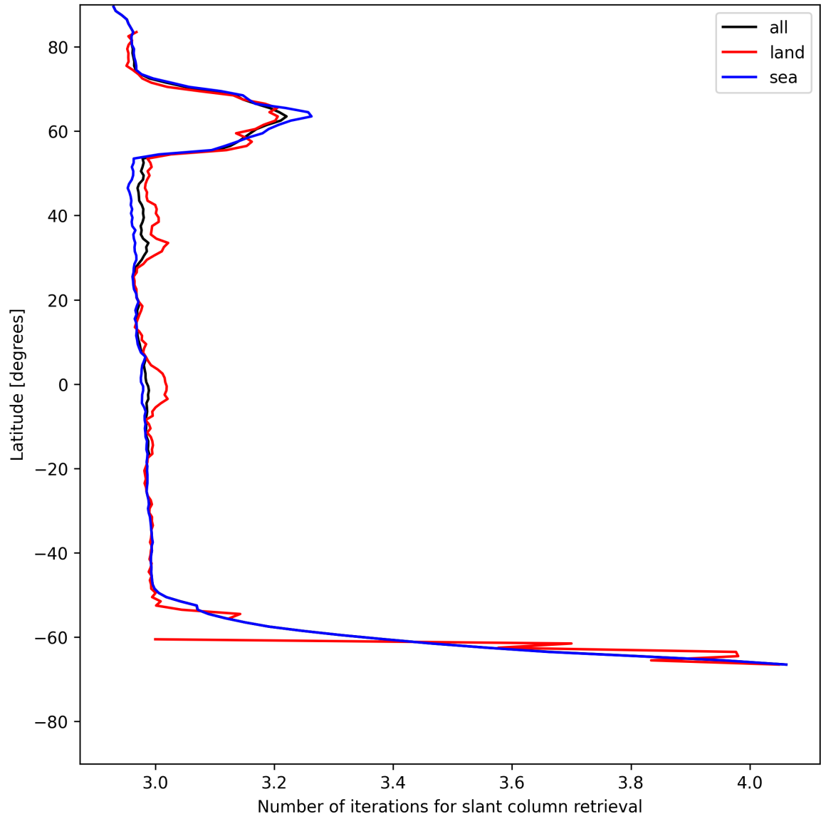
Figure 21: Zonal average of “Number of iterations for slant column retrieval” for 2025-05-29 to 2025-05-29.
