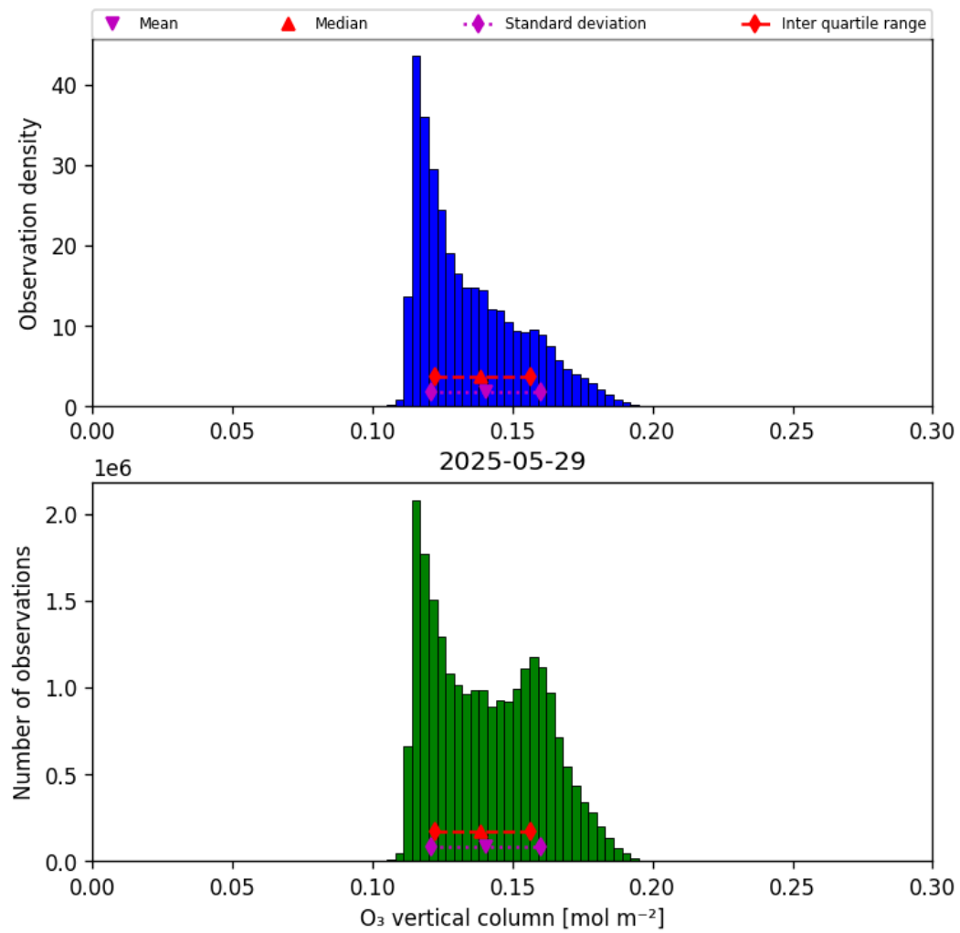
Figure 29: Histogram of “O 3 vertical column” for 2025-05-29 to 2025-05-29
