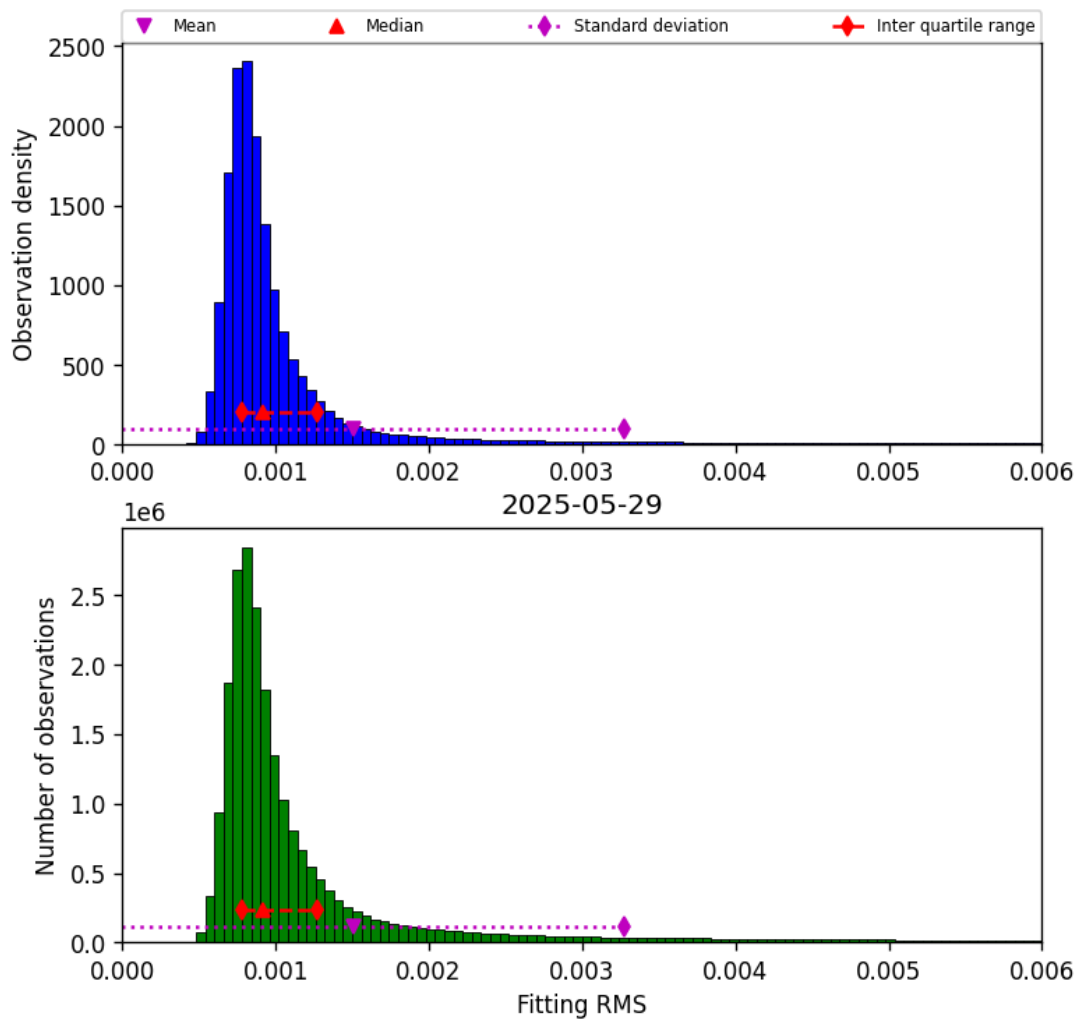
Figure 34: Histogram of “Fitting RMS” for 2025-05-29 to 2025-05-29
