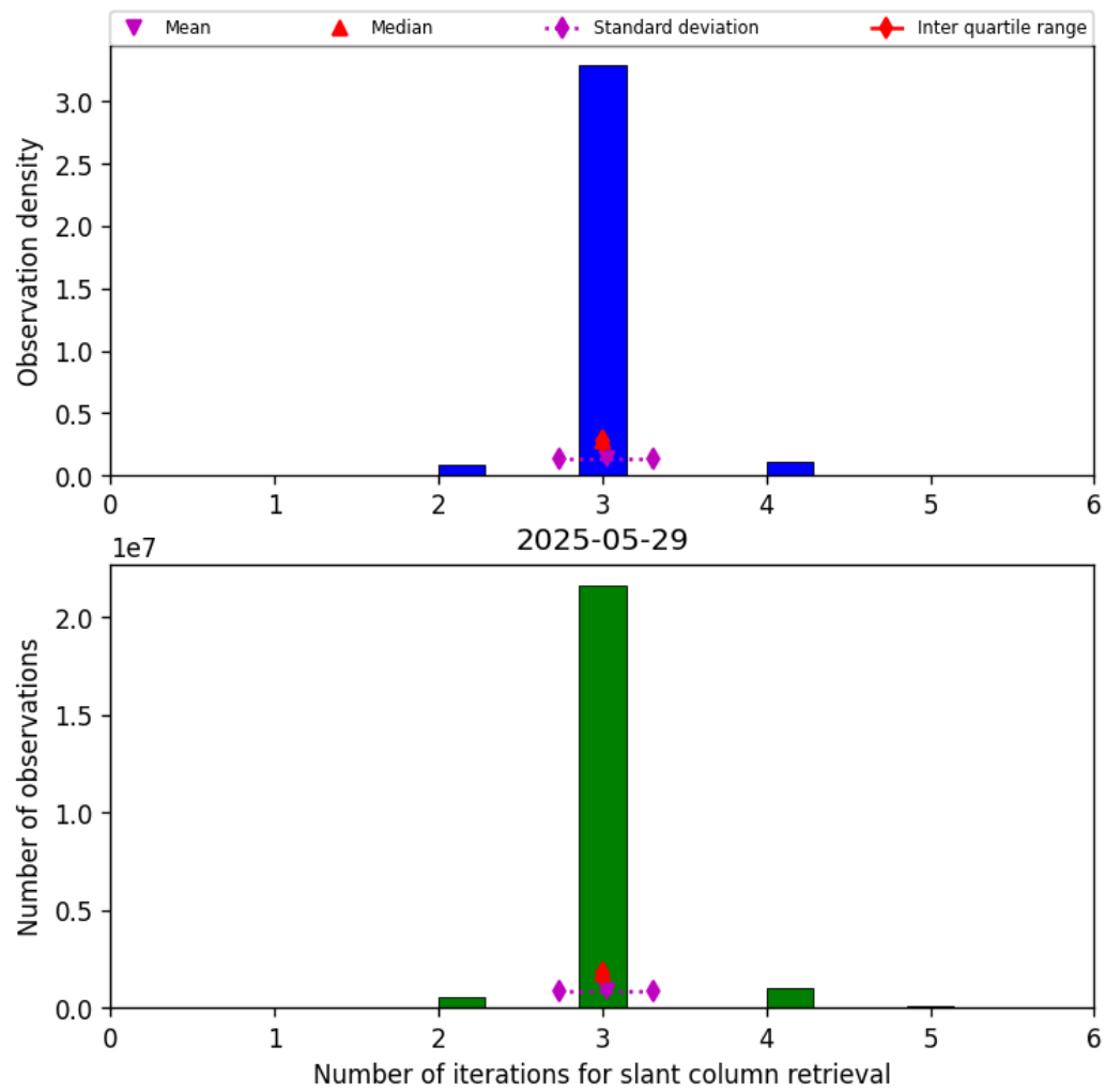
Figure 33: Histogram of “Number of iterations for slant column retrieval” for 2025-05-29 to 2025-05-29
