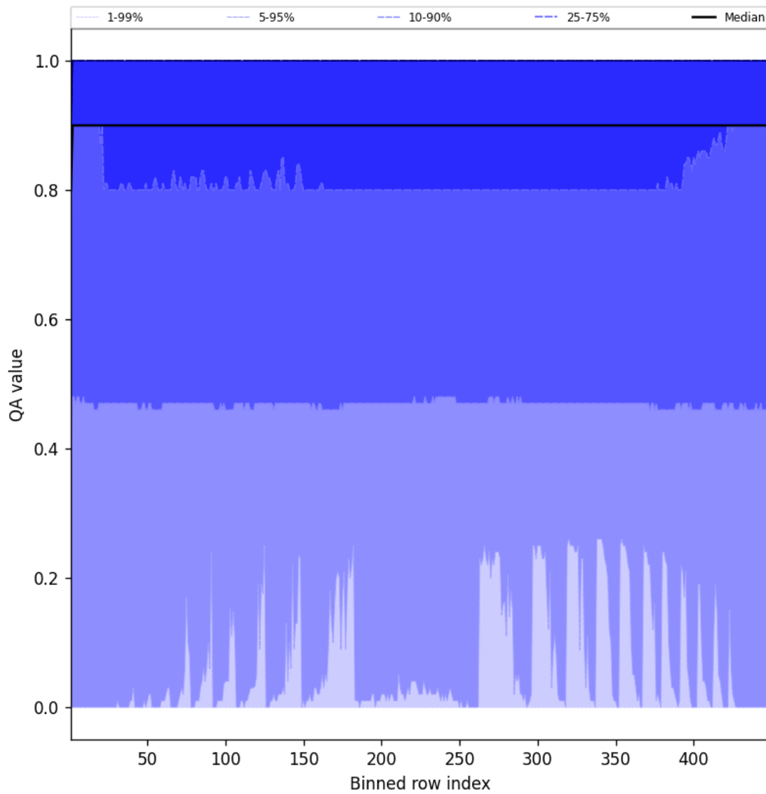
Figure 40: Along track statistics of “QA value” for 2025-05-29 to 2025-05-29
