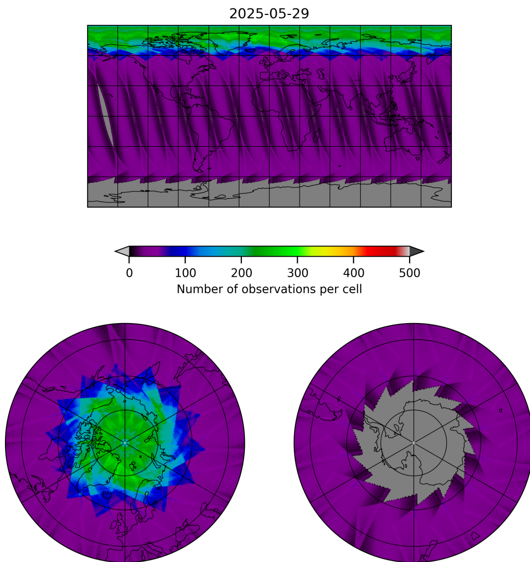
Figure 15: Map of the number of observations for 2025-05-29 to 2025-05-29
