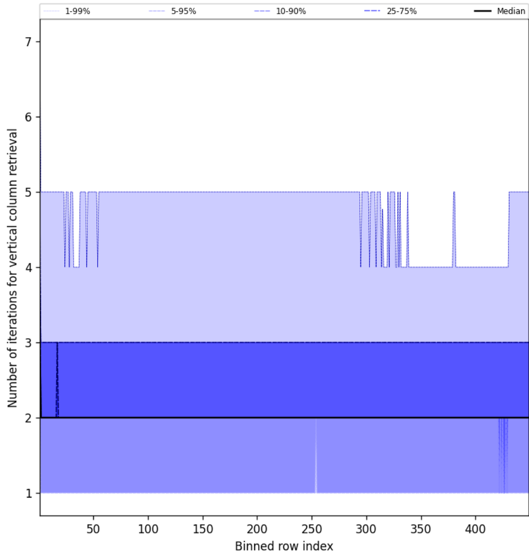
Figure 51: Along track statistics of “Number of iterations for vertical column retrieval” for 2025-05-29 to 2025-05-29
