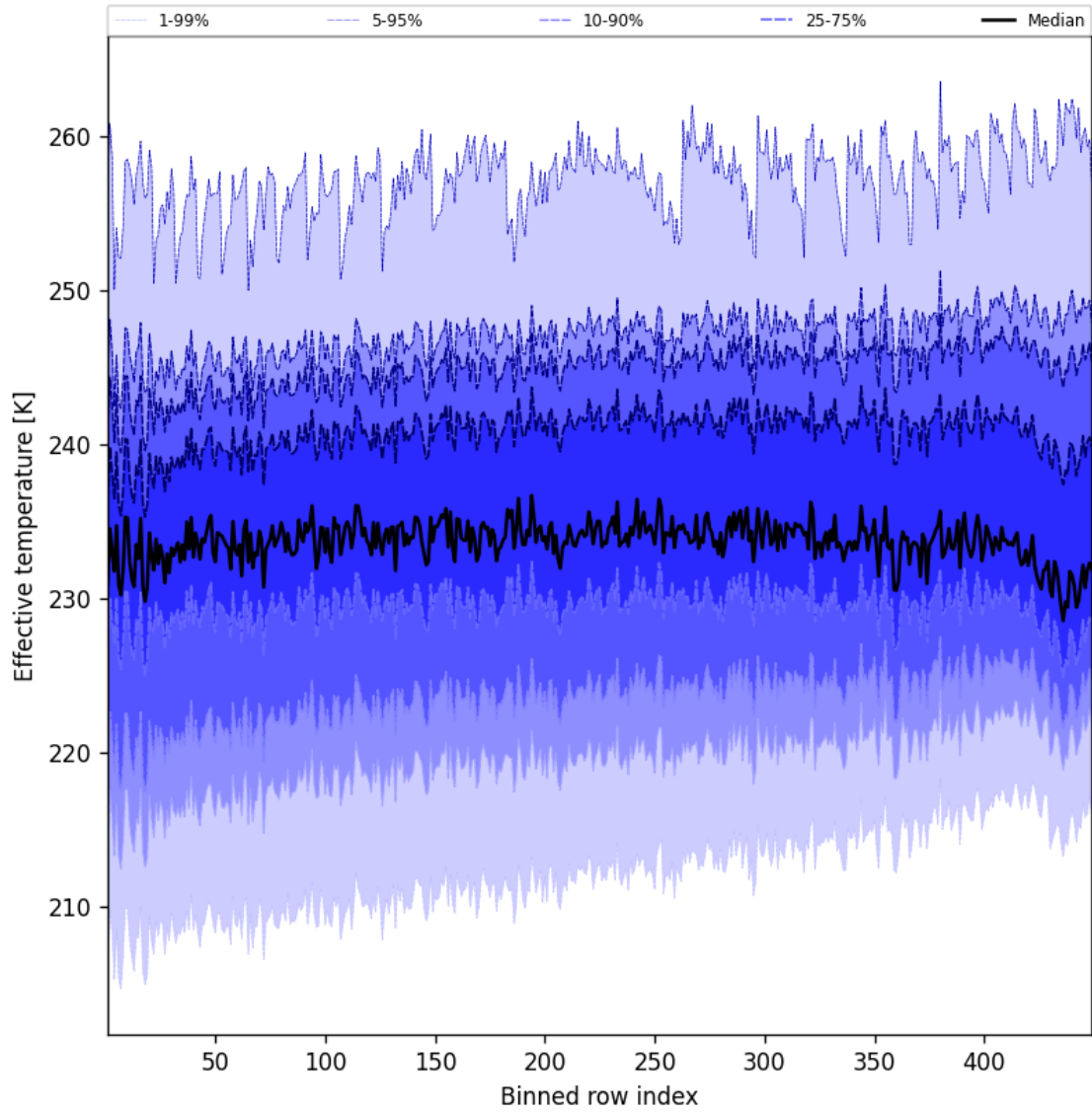
Figure 50: Along track statistics of “Effective temperature” for 2025-05-29 to 2025-05-29
