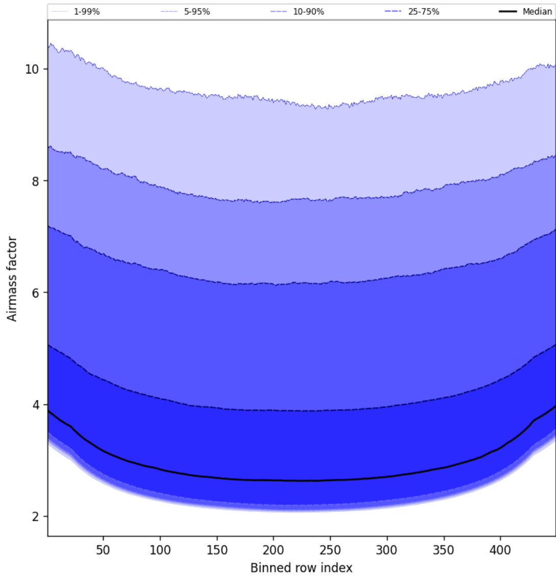
Figure 49: Along track statistics of “Airmass factor” for 2025-05-29 to 2025-05-29
