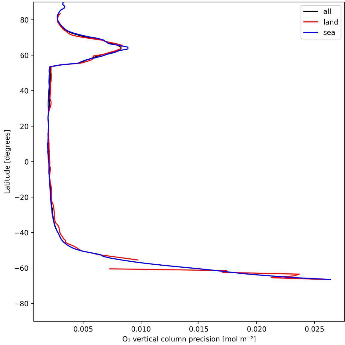
Figure 18: Zonal average of “O 3 vertical column precision” for 2025-05-29 to 2025-05-29.
