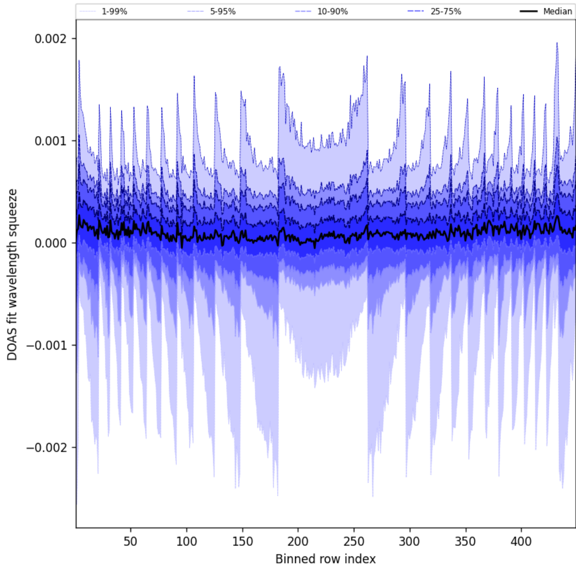
Figure 48: Along track statistics of “DOAS fit wavelength squeeze” for 2025-05-29 to 2025-05-29
