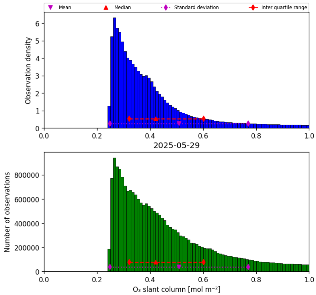
Figure 31: Histogram of “O 3 slant column” for 2025-05-29 to 2025-05-29
