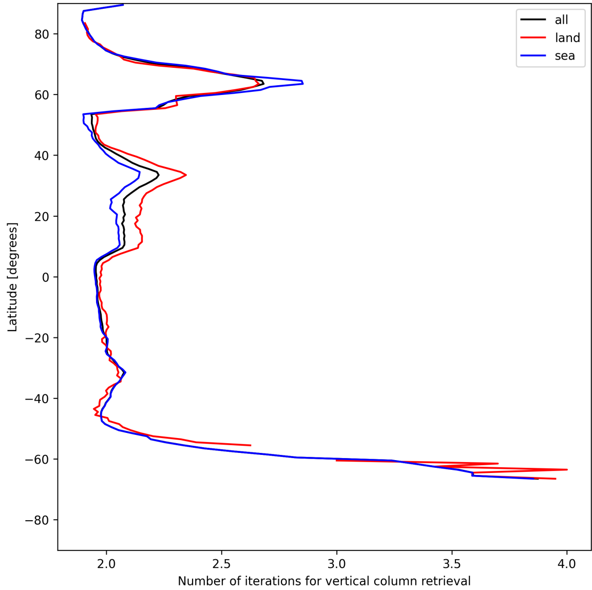
Figure 27: Zonal average of “Number of iterations for vertical column retrieval” for 2025-05-29 to 2025-05-29.
