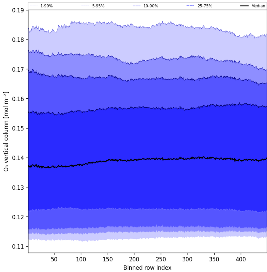
Figure 41: Along track statistics of “O 3 vertical column” for 2025-05-29 to 2025-05-29
