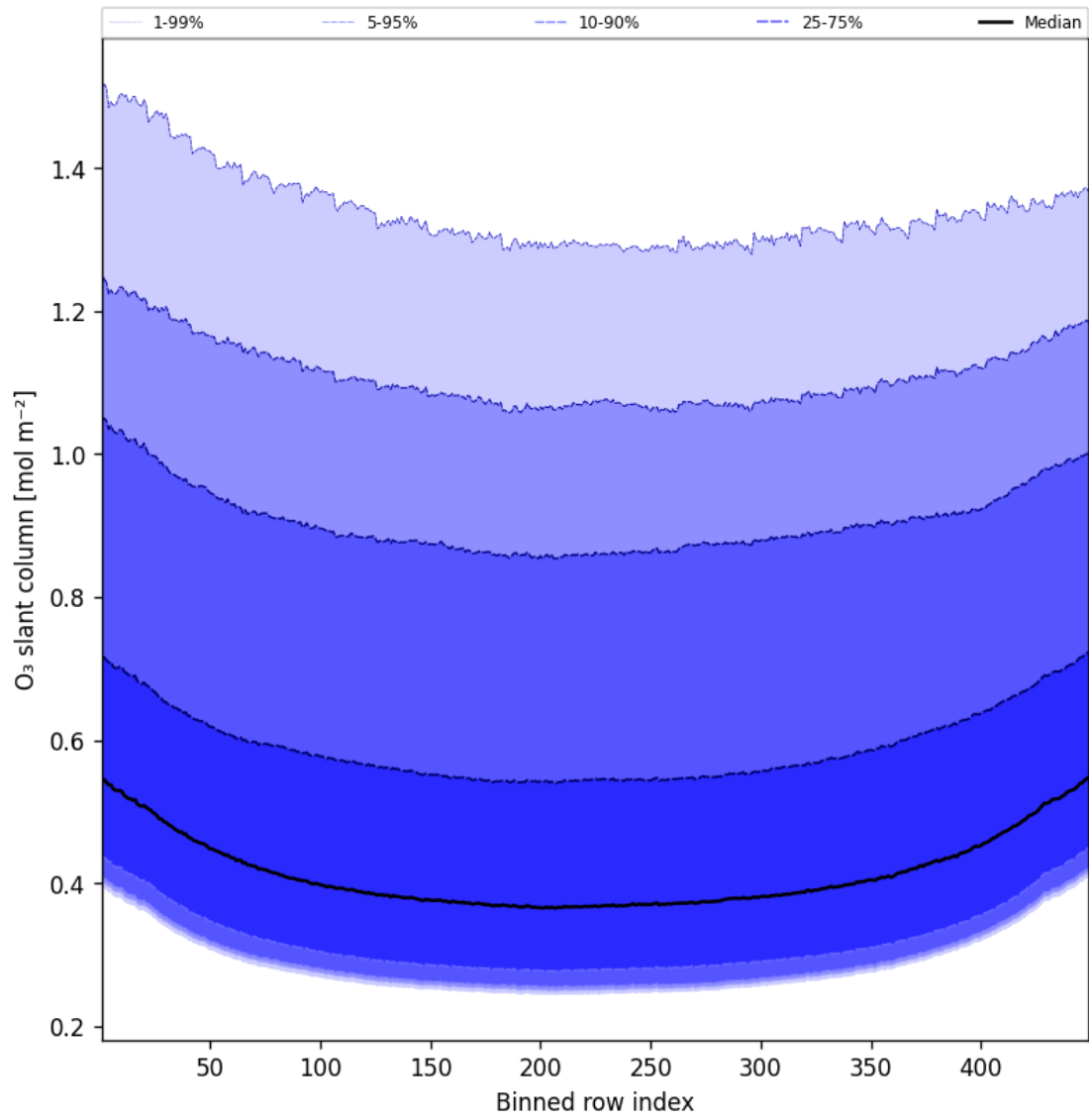
Figure 43: Along track statistics of “O 3 slant column” for 2025-05-29 to 2025-05-29
