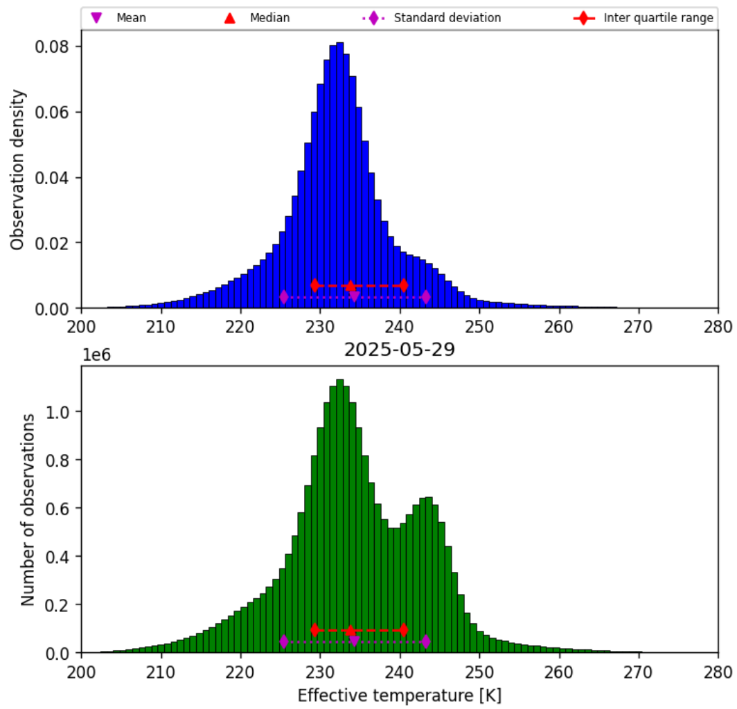
Figure 38: Histogram of “Effective temperature” for 2025-05-29 to 2025-05-29
