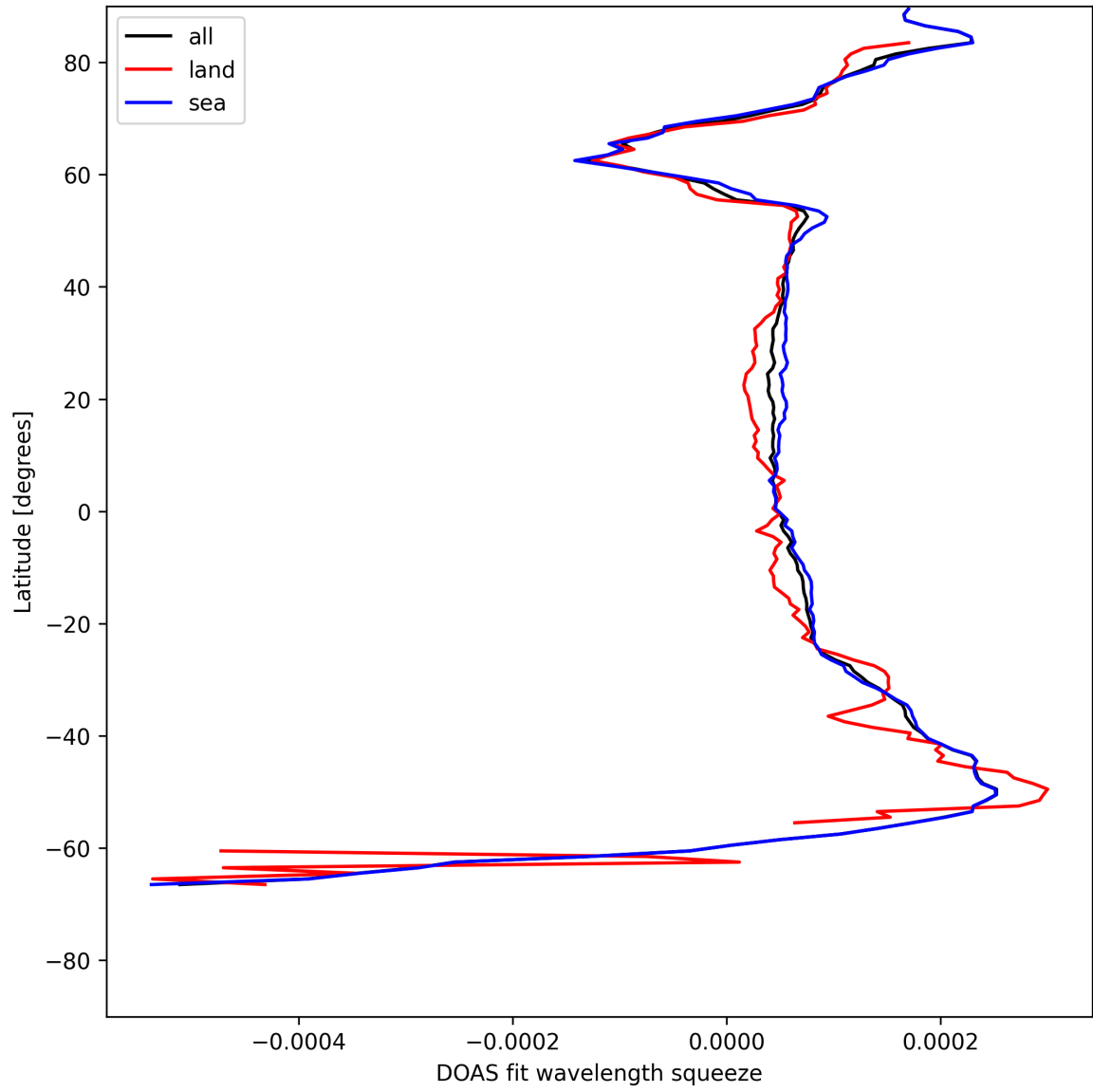
Figure 24: Zonal average of “DOAS fit wavelength squeeze” for 2025-05-29 to 2025-05-29.
