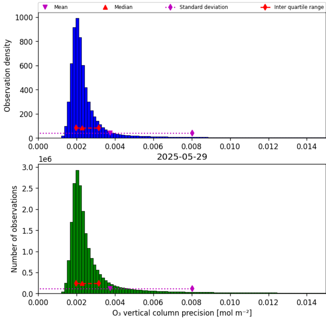
Figure 30: Histogram of “O 3 vertical column precision” for 2025-05-29 to 2025-05-29
