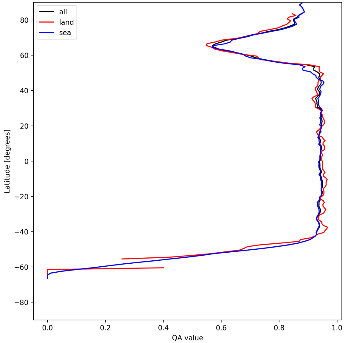
Figure 16: Zonal average of “QA value” for 2025-05-29 to 2025-05-29.
