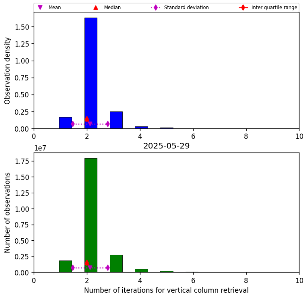
Figure 39: Histogram of “Number of iterations for vertical column retrieval” for 2025-05-29 to 2025-05-29
