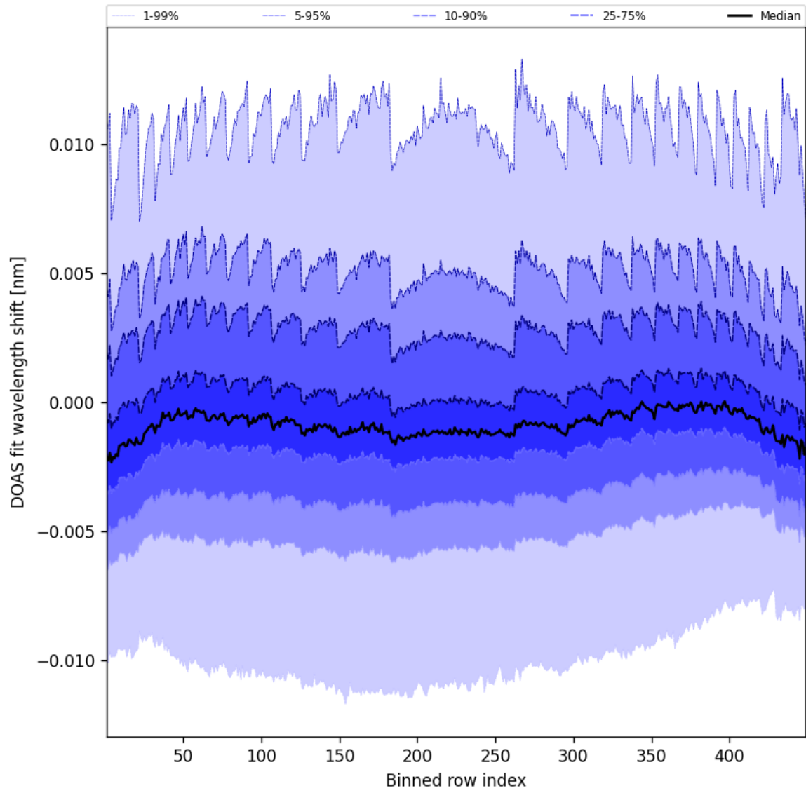
Figure 47: Along track statistics of “DOAS fit wavelength shift” for 2025-05-29 to 2025-05-29
