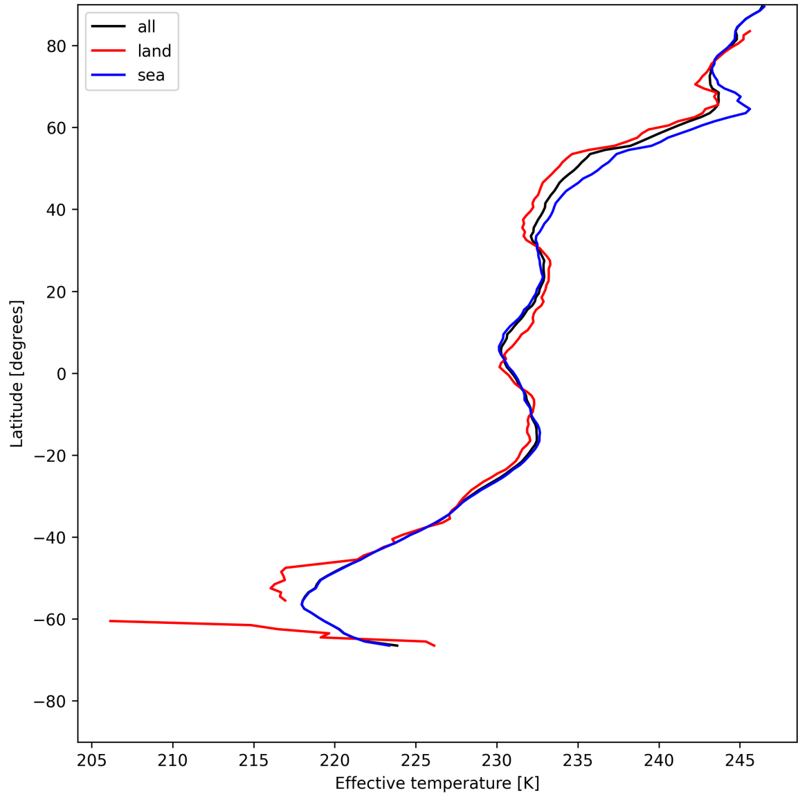
Figure 26: Zonal average of “Effective temperature” for 2025-05-29 to 2025-05-29.
