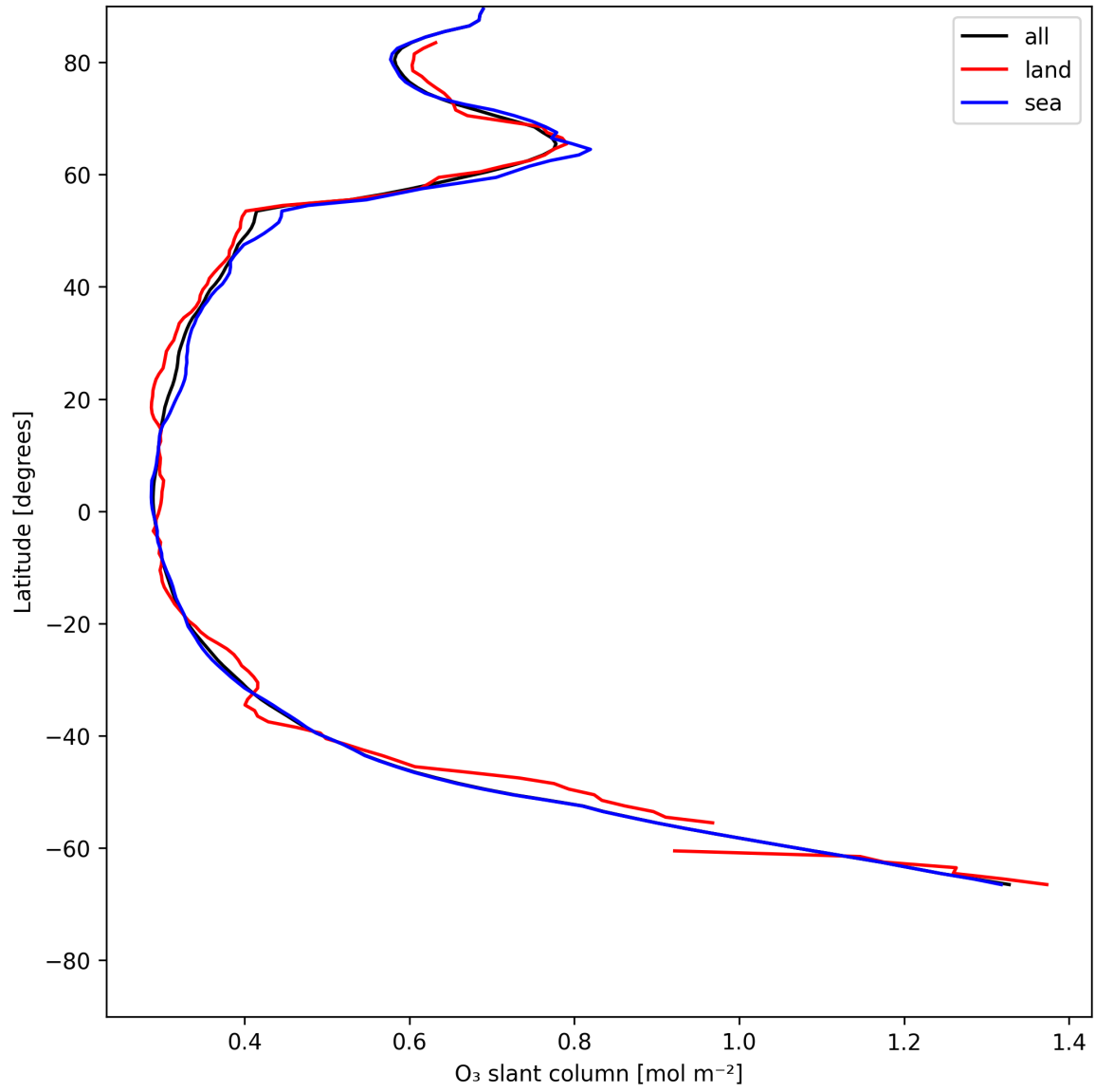
Figure 19: Zonal average of “O 3 slant column” for 2025-05-29 to 2025-05-29.
