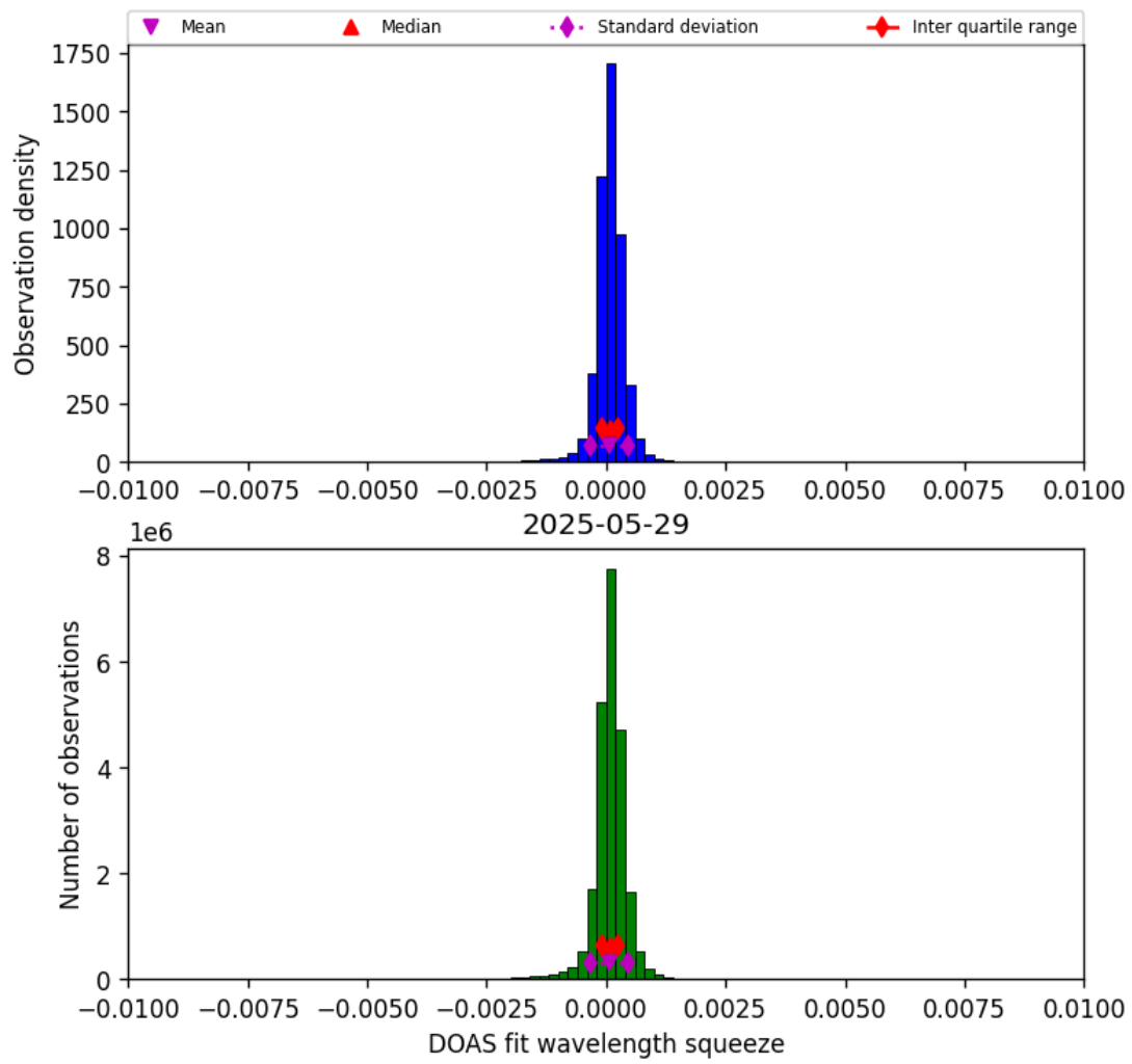
Figure 36: Histogram of “DOAS fit wavelength squeeze” for 2025-05-29 to 2025-05-29
