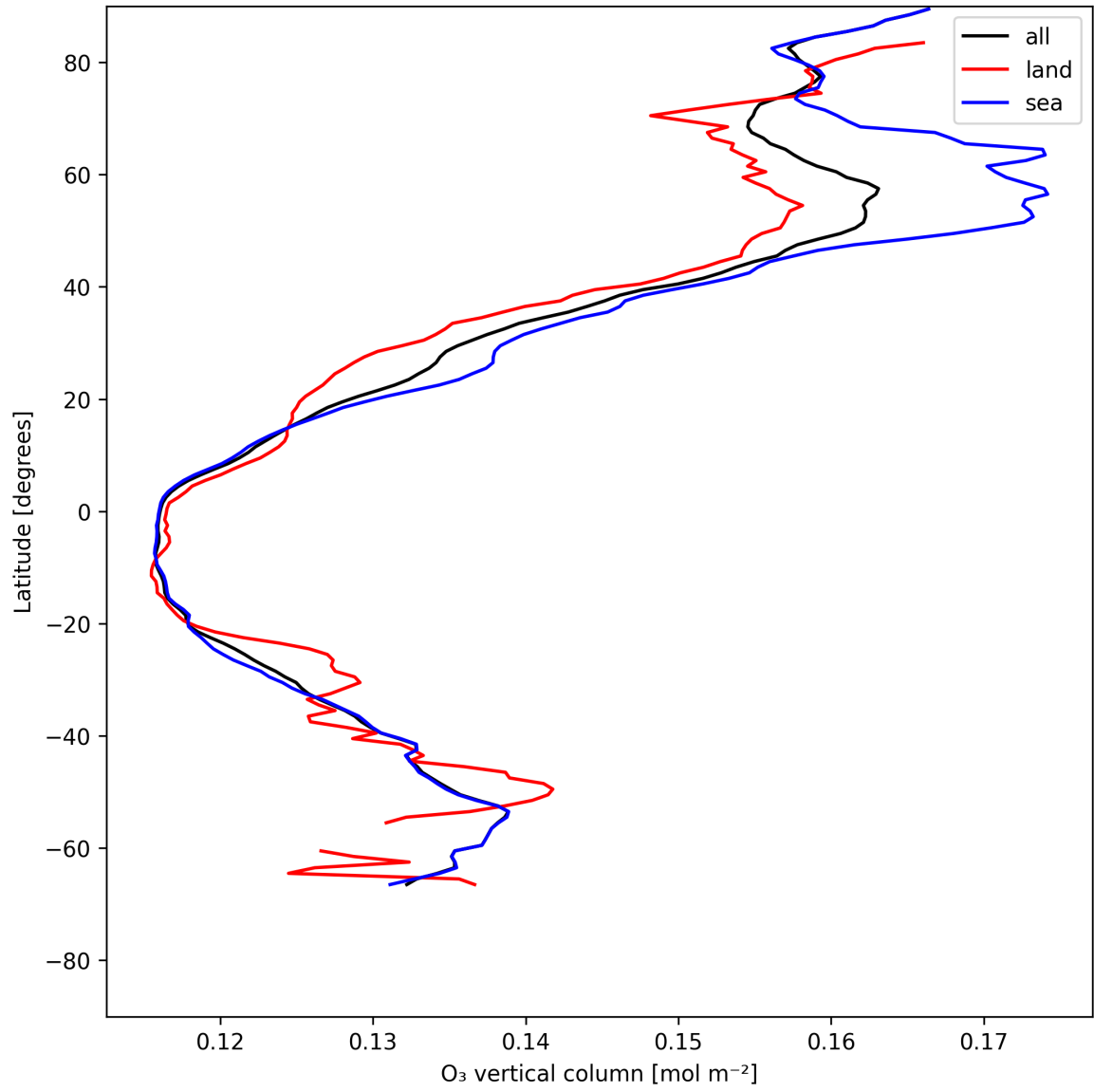
Figure 17: Zonal average of “O 3 vertical column” for 2025-05-29 to 2025-05-29.
