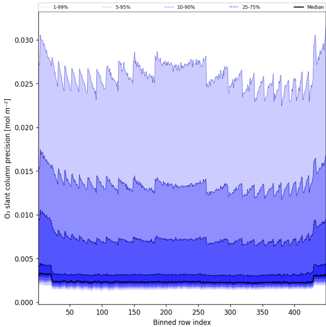
Figure 44: Along track statistics of “O 3 slant column precision” for 2025-05-29 to 2025-05-29
