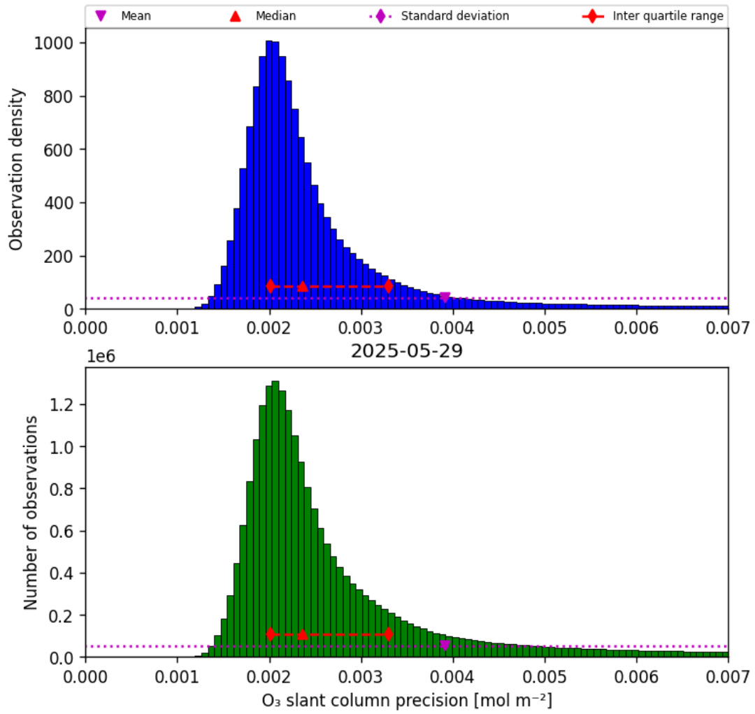
Figure 32: Histogram of “O 3 slant column precision” for 2025-05-29 to 2025-05-29
