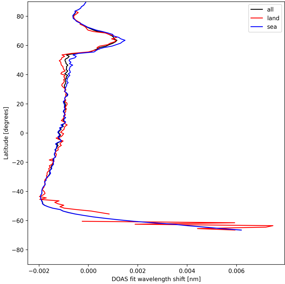
Figure 23: Zonal average of “DOAS fit wavelength shift” for 2025-05-29 to 2025-05-29.
