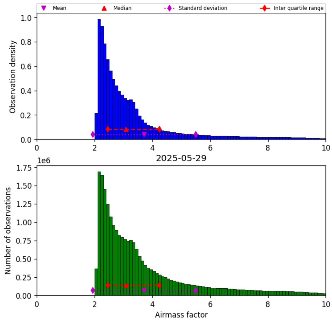
Figure 37: Histogram of “Airmass factor” for 2025-05-29 to 2025-05-29
