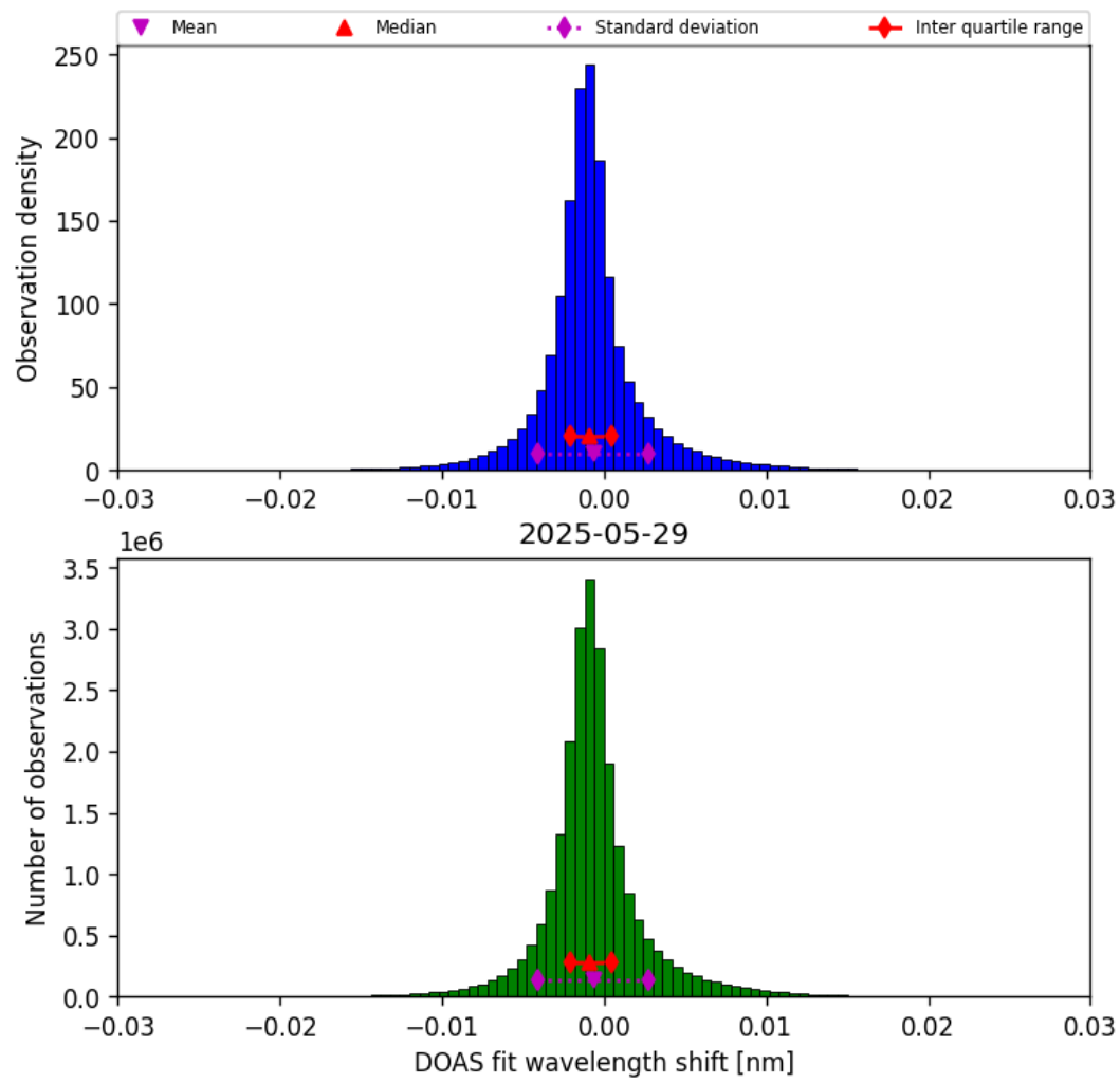
Figure 35: Histogram of “DOAS fit wavelength shift” for 2025-05-29 to 2025-05-29
