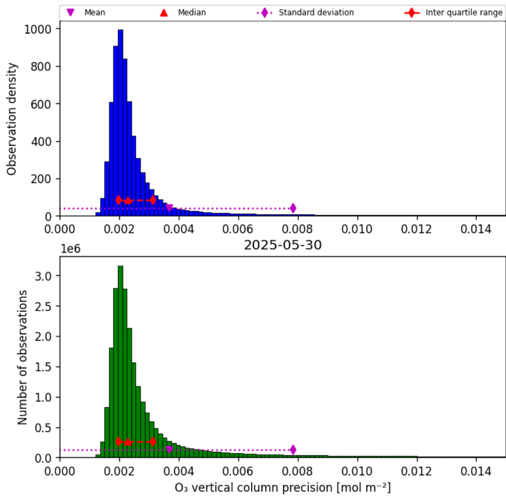
Figure 30: Histogram of “O 3 vertical column precision” for 2025-05-30 to 2025-05-31
