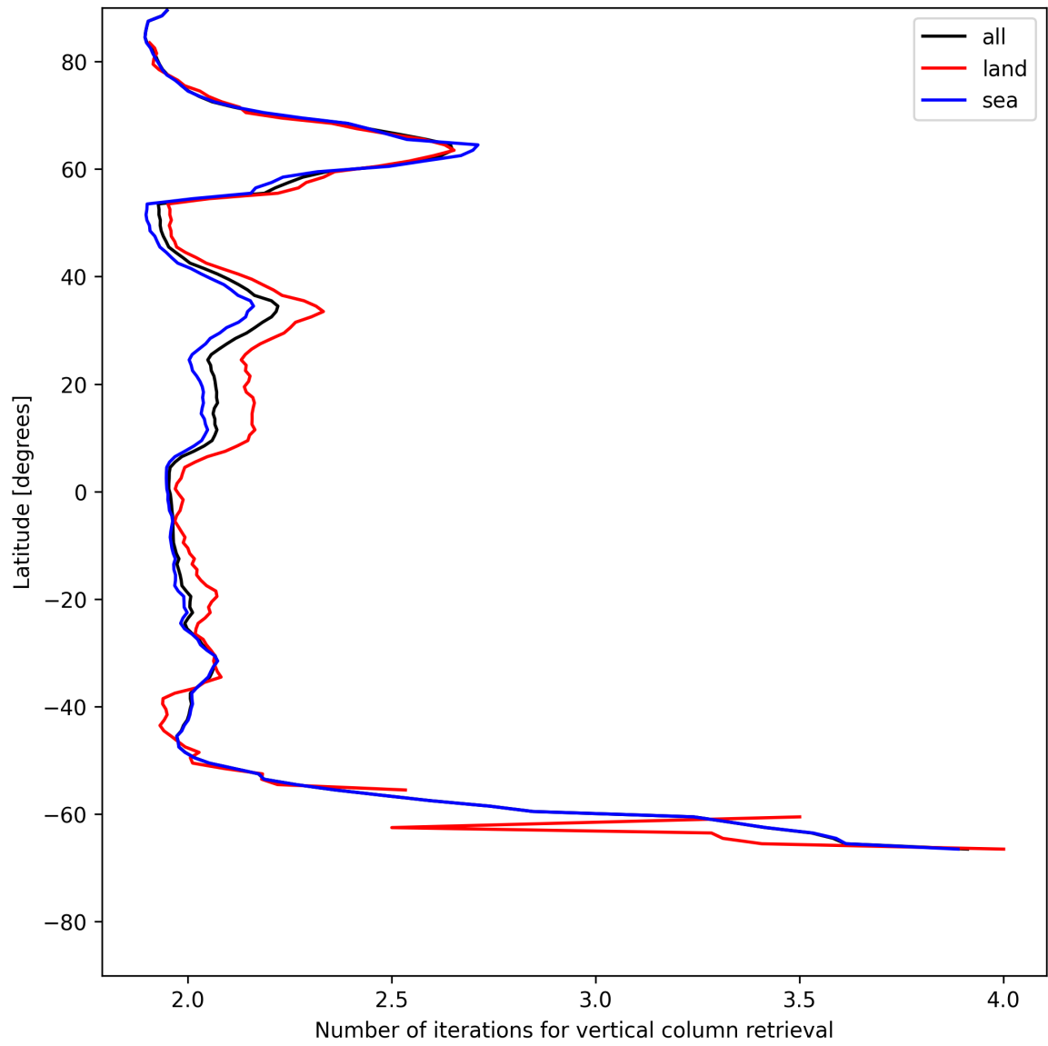
Figure 27: Zonal average of “Number of iterations for vertical column retrieval” for 2025-05-30 to 2025-05-31.
