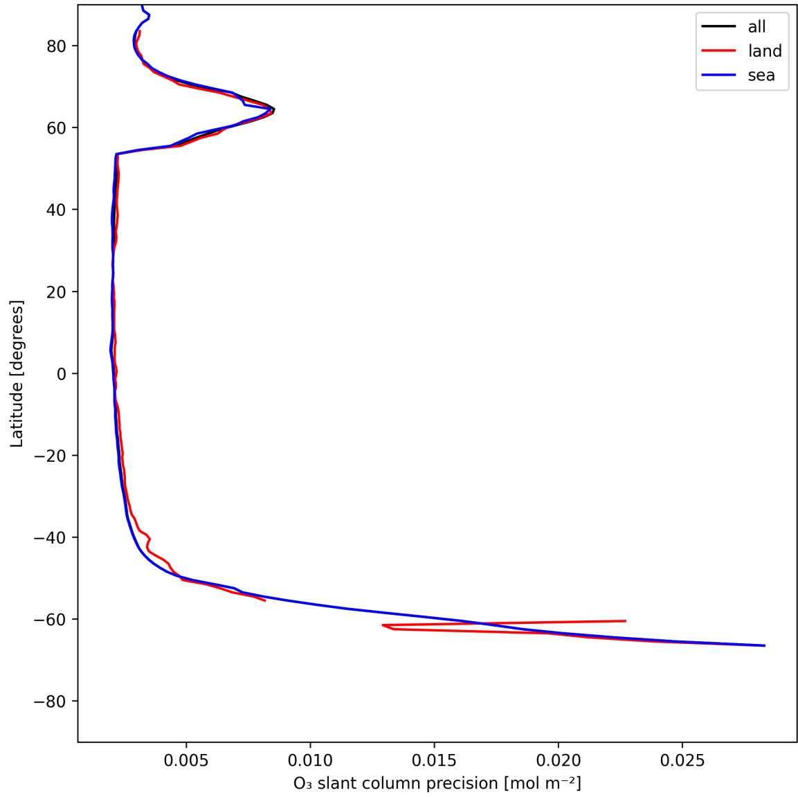
Figure 20: Zonal average of “O 3 slant column precision” for 2025-05-30 to 2025-05-31.
