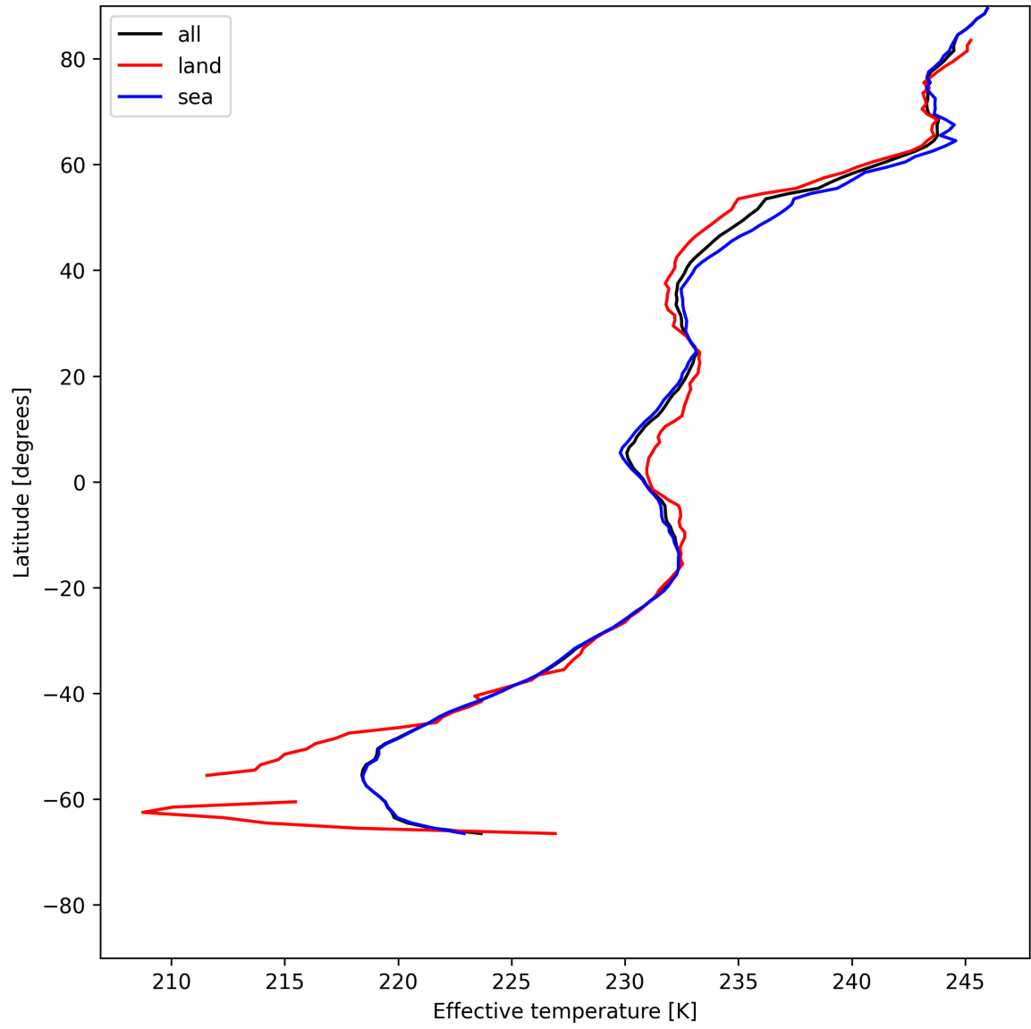
Figure 26: Zonal average of “Effective temperature” for 2025-05-30 to 2025-05-31.
