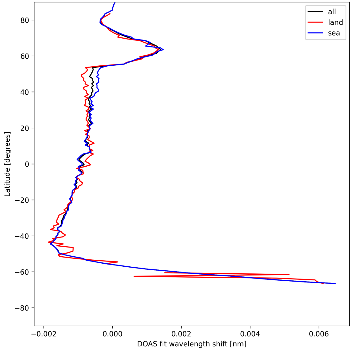
Figure 23: Zonal average of "DOAS fit wavelength shift" for 2025-05-30 to 2025-05-31.
