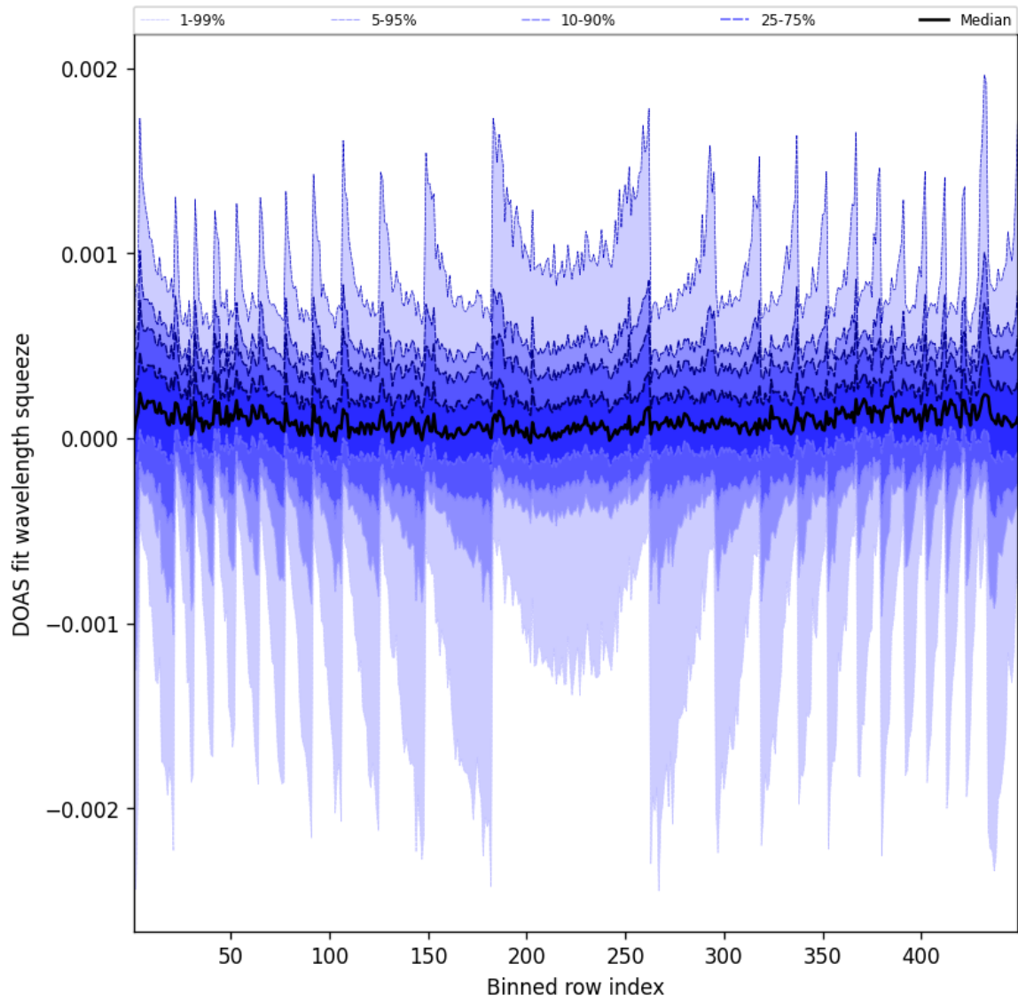
Figure 48: Along track statistics of “DOAS fit wavelength squeeze” for 2025-05-30 to 2025-05-31
