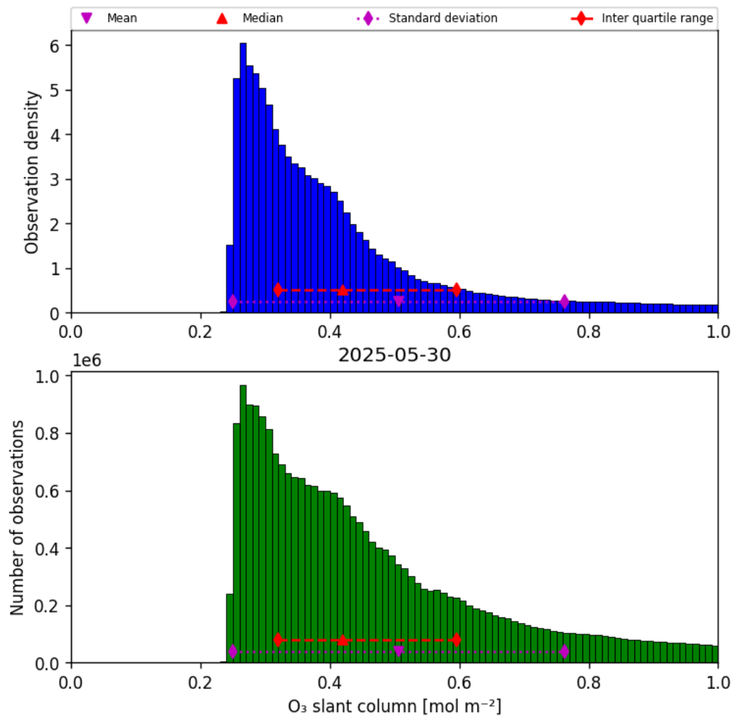
Figure 31: Histogram of “O 3 slant column” for 2025-05-30 to 2025-05-31
