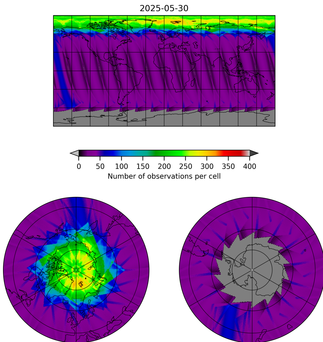
Figure 15: Map of the number of observations for 2025-05-30 to 2025-05-31
