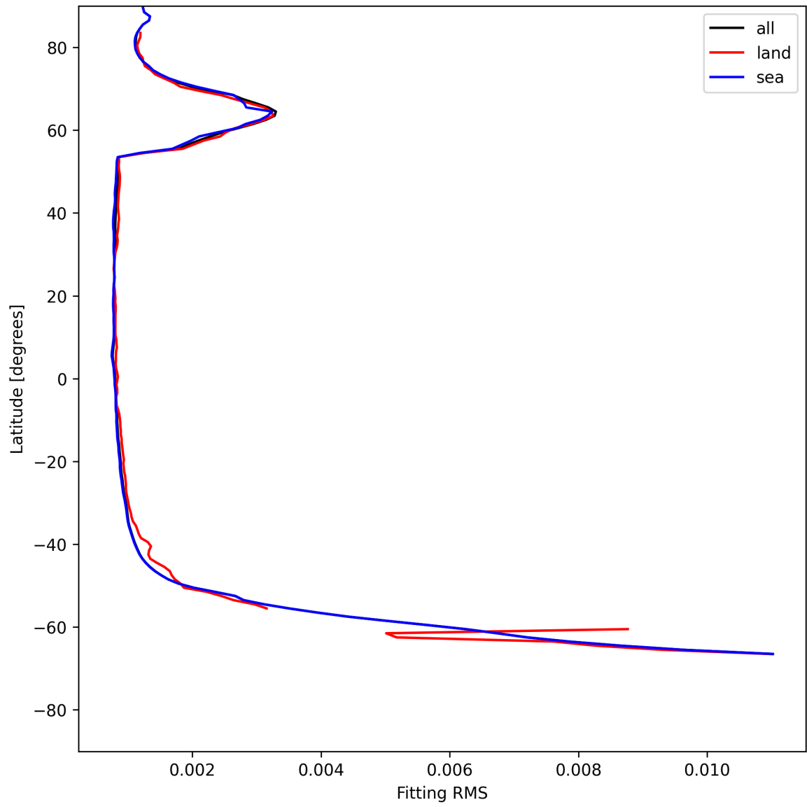
Figure 22: Zonal average of “Fitting RMS” for 2025-05-30 to 2025-05-31.
