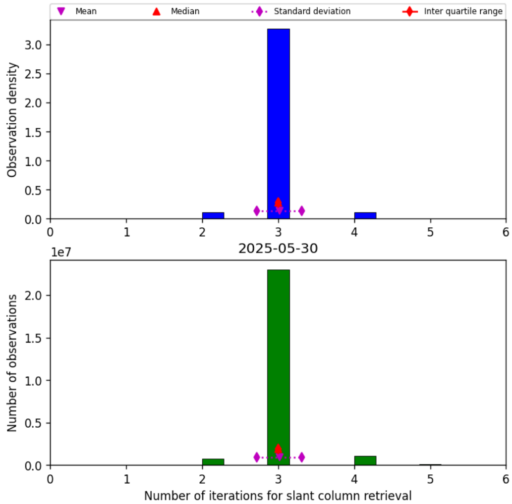
Figure 33: Histogram of “Number of iterations for slant column retrieval” for 2025-05-30 to 2025-05-31
