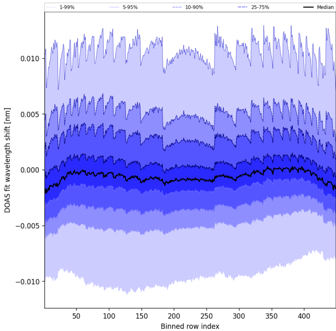
Figure 47: Along track statistics of “DOAS fit wavelength shift” for 2025-05-30 to 2025-05-31
