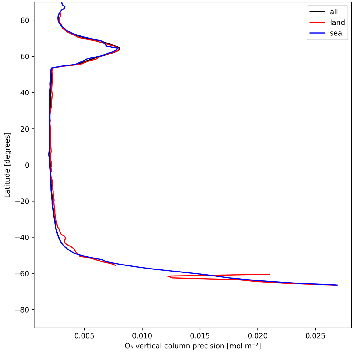
Figure 18: Zonal average of “O 3 vertical column precision” for 2025-05-30 to 2025-05-31.
