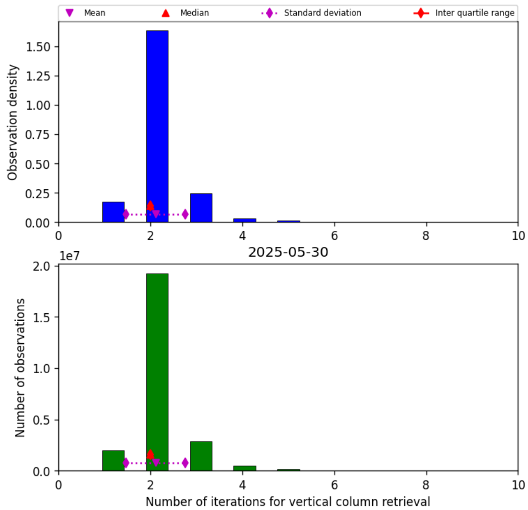
Figure 39: Histogram of “Number of iterations for vertical column retrieval” for 2025-05-30 to 2025-05-31
