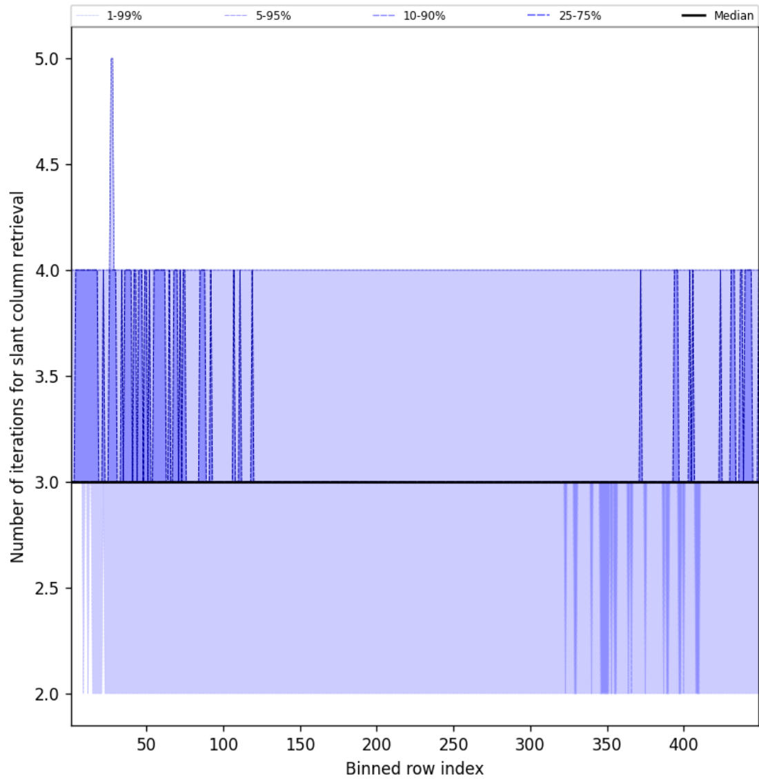
Figure 45: Along track statistics of “Number of iterations for slant column retrieval” for 2025-05-30 to 2025-05-31
