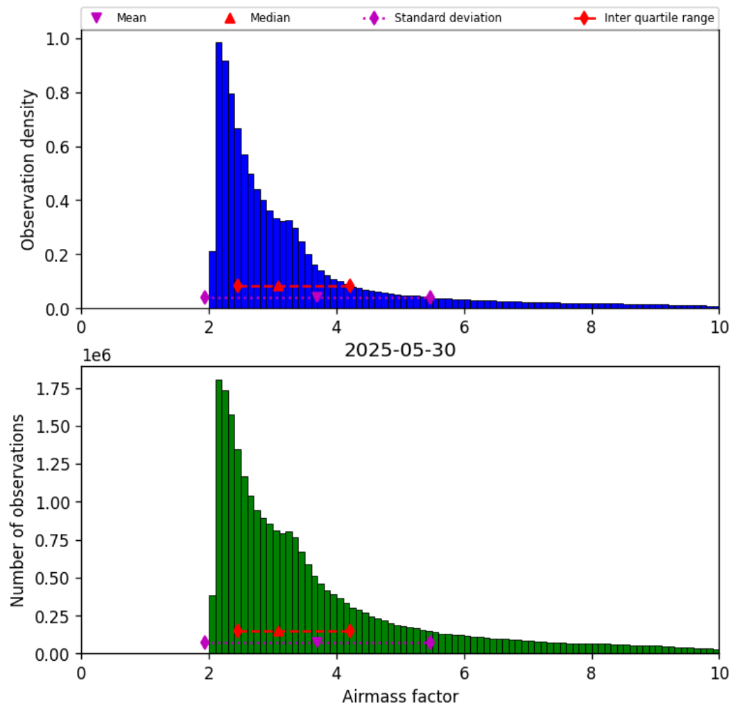
Figure 37: Histogram of “Airmass factor” for 2025-05-30 to 2025-05-31
