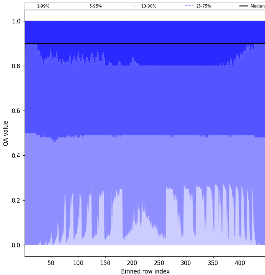
Figure 40: Along track statistics of “QA value” for 2025-05-30 to 2025-05-31
