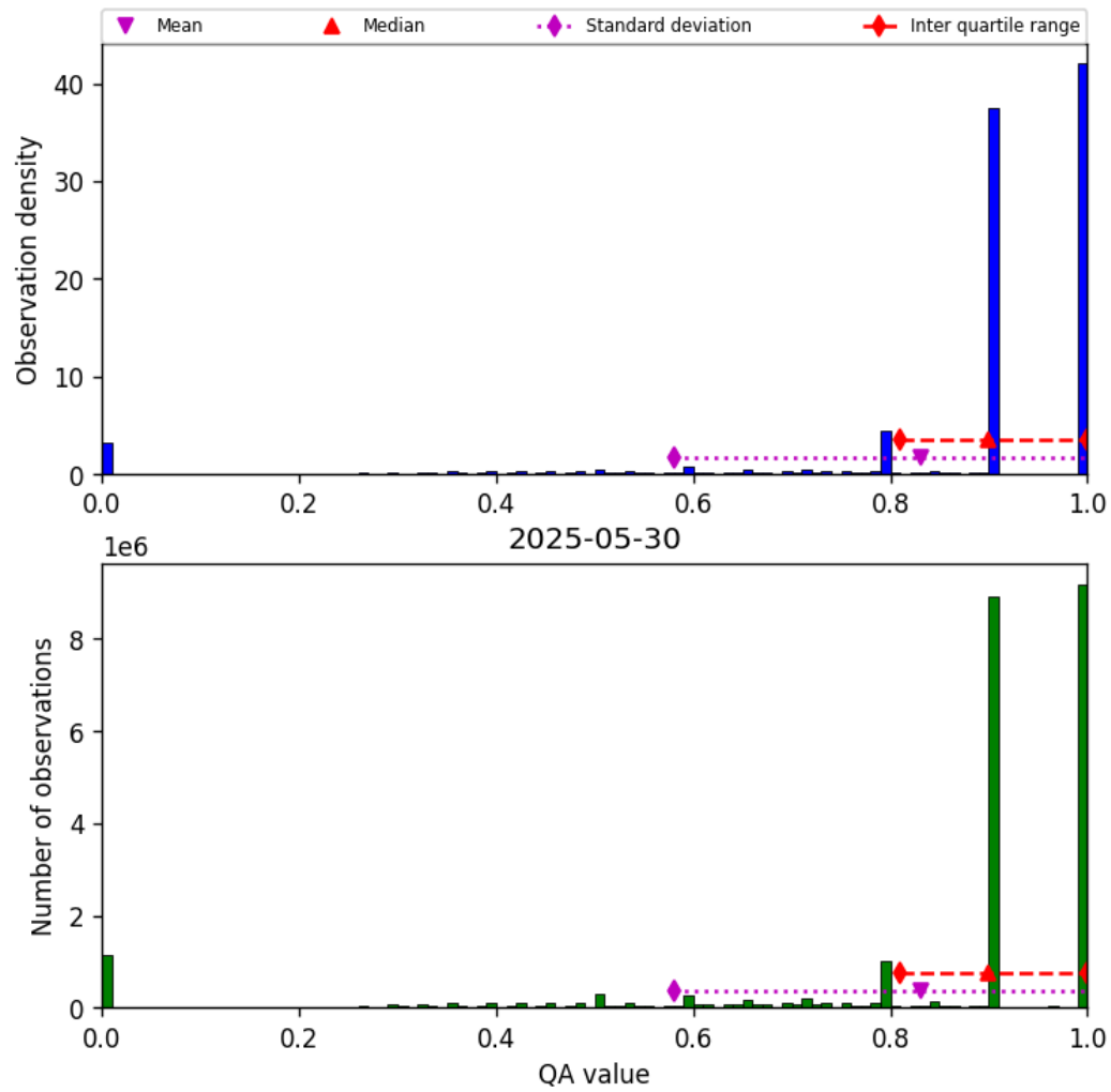
Figure 28: Histogram of “QA value” for 2025-05-30 to 2025-05-31
