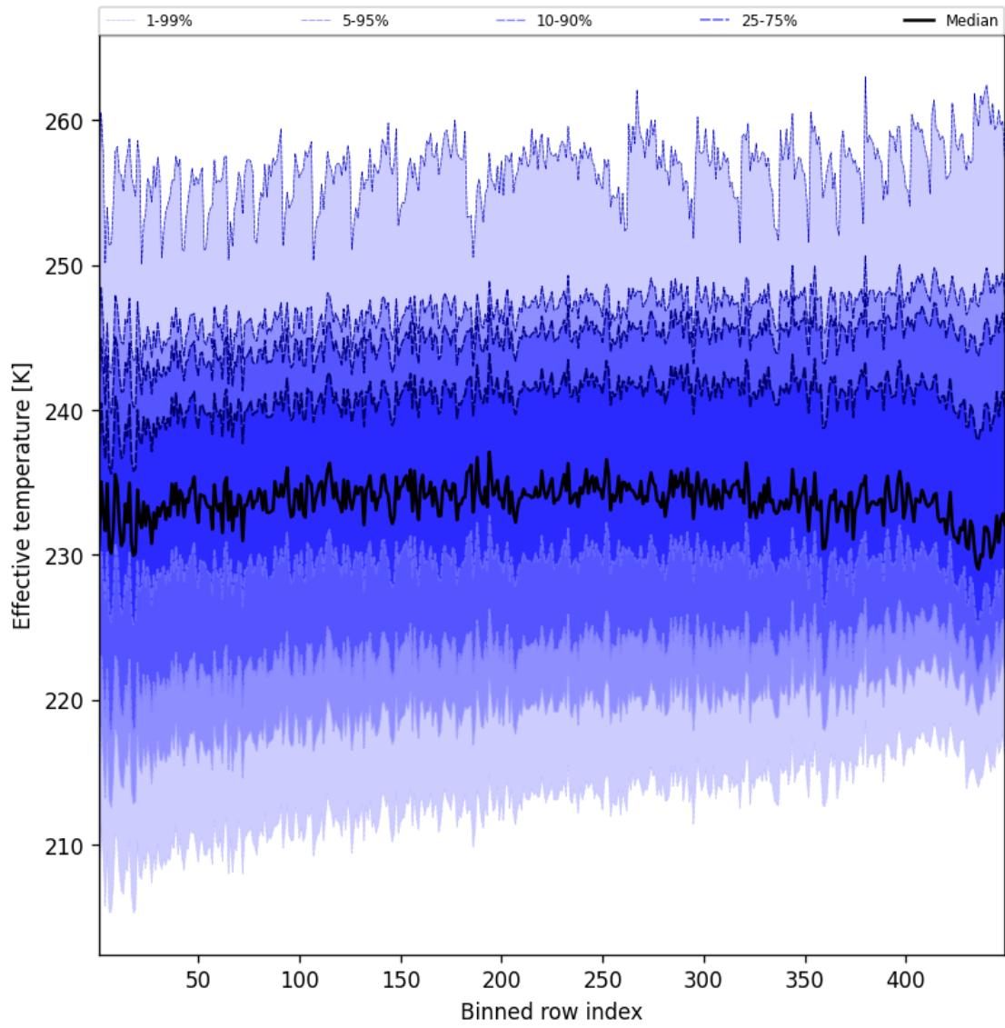
Figure 50: Along track statistics of “Effective temperature” for 2025-05-30 to 2025-05-31
