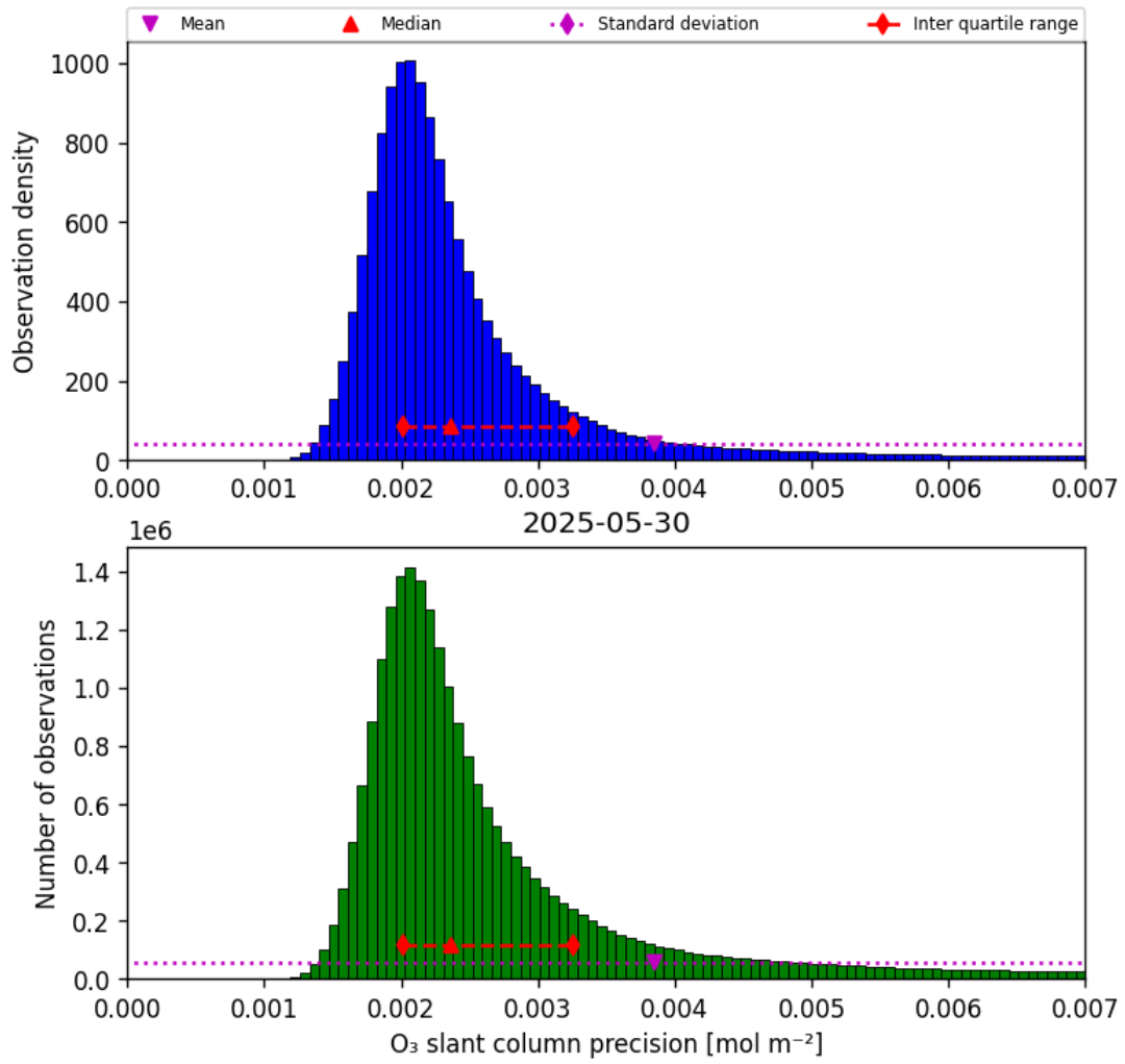
Figure 32: Histogram of “O 3 slant column precision” for 2025-05-30 to 2025-05-31
