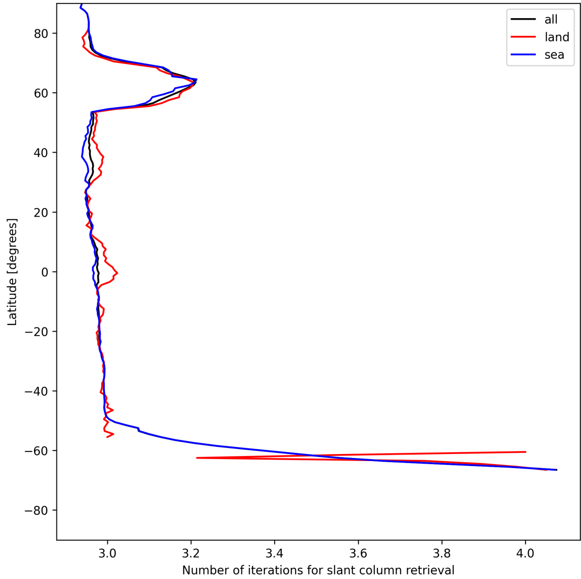
Figure 21: Zonal average of “Number of iterations for slant column retrieval” for 2025-05-30 to 2025-05-31.
