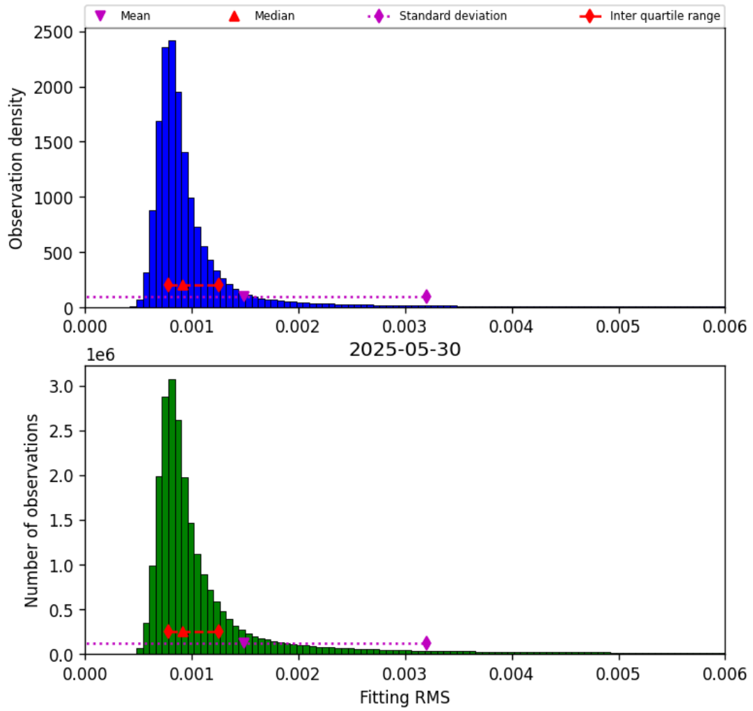
Figure 34: Histogram of “Fitting RMS” for 2025-05-30 to 2025-05-31
