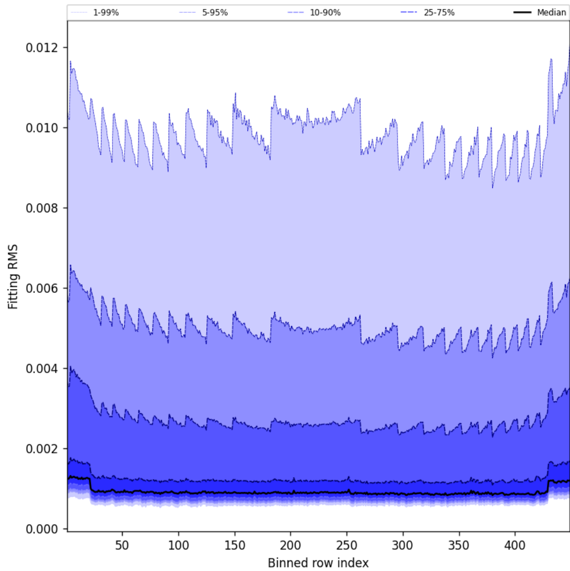
Figure 46: Along track statistics of “Fitting RMS” for 2025-05-30 to 2025-05-31
