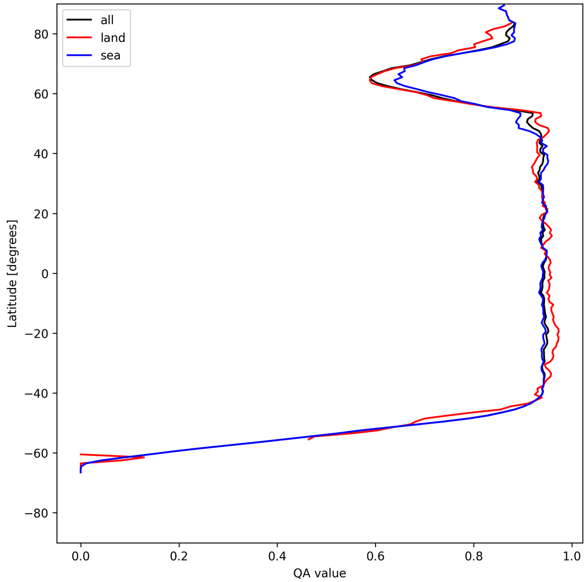
Figure 16: Zonal average of “QA value” for 2025-05-30 to 2025-05-31.
