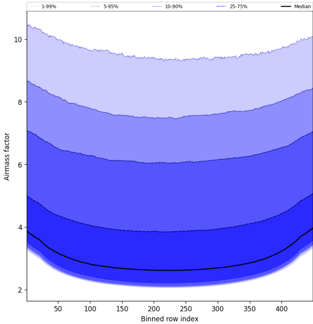
Figure 49: Along track statistics of “Airmass factor” for 2025-05-30 to 2025-05-31
