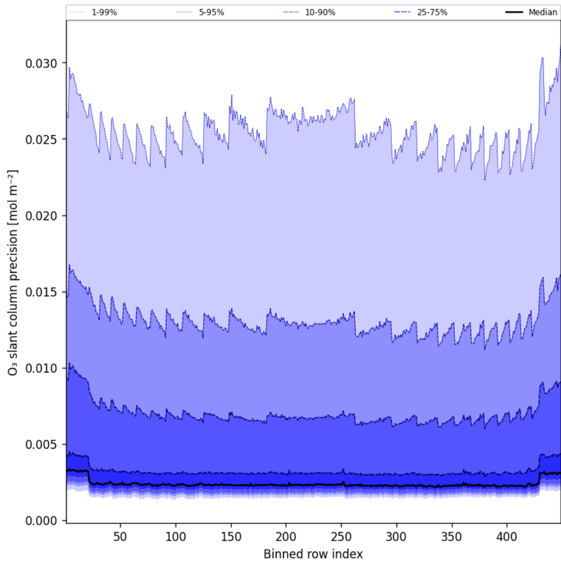
Figure 44: Along track statistics of “O 3 slant column precision” for 2025-05-30 to 2025-05-31
