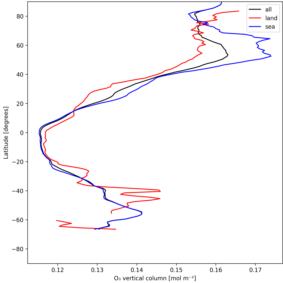
Figure 17: Zonal average of “O 3 vertical column” for 2025-05-30 to 2025-05-31.
