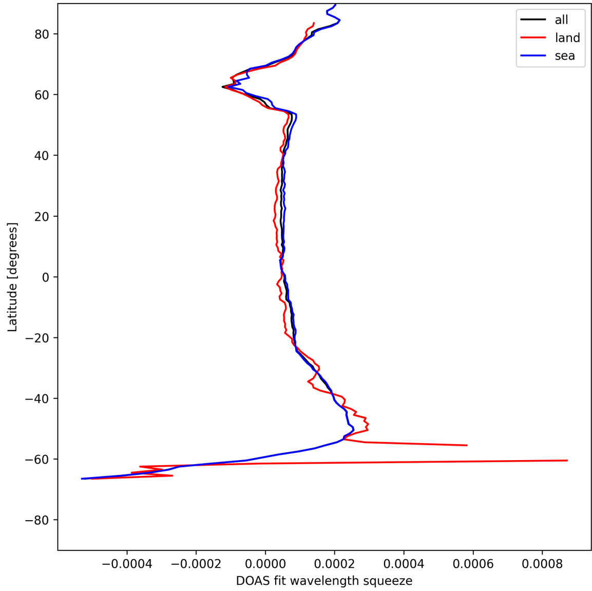
Figure 24: Zonal average of “DOAS fit wavelength squeeze” for 2025-05-30 to 2025-05-31.
