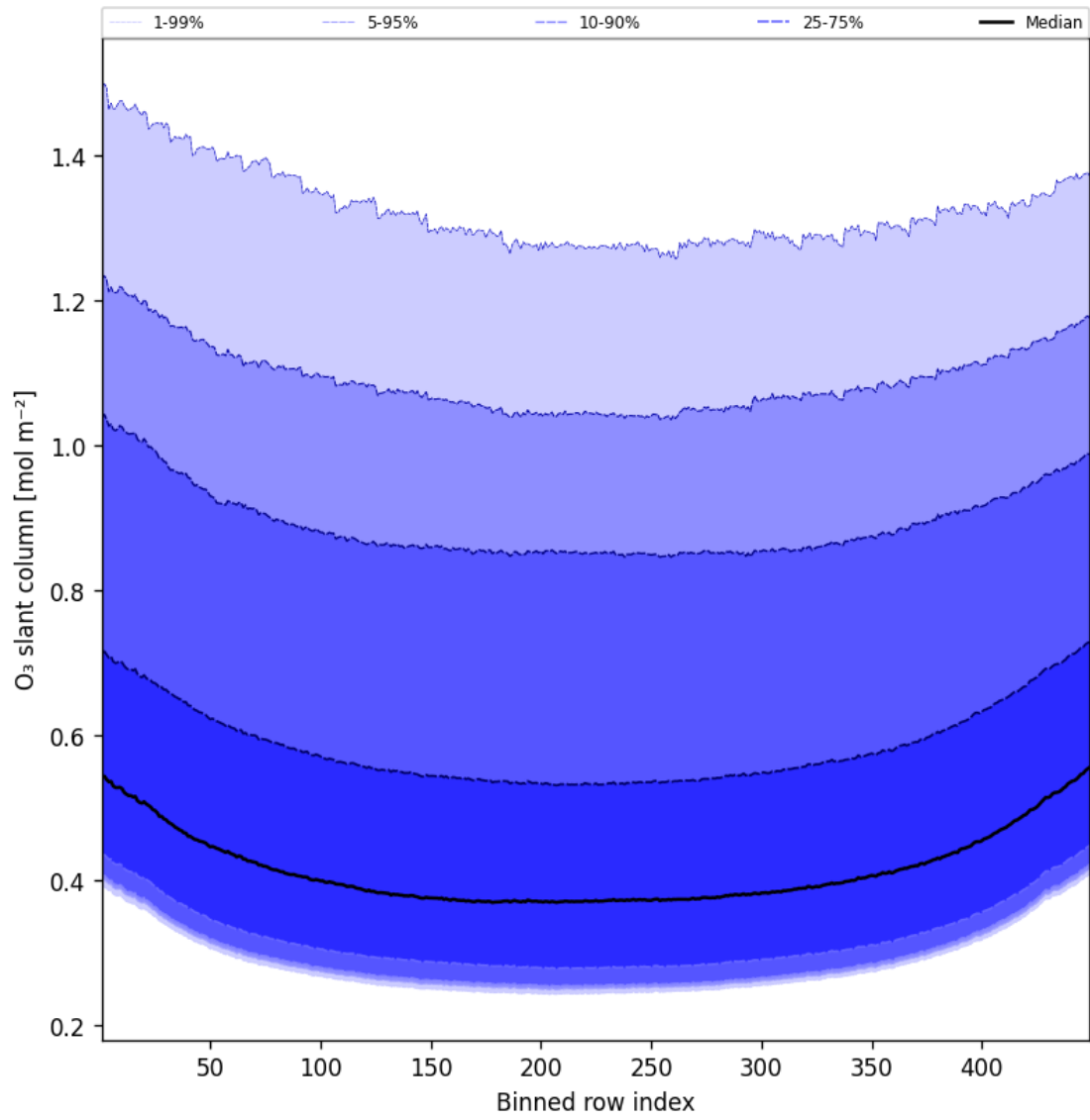
Figure 43: Along track statistics of “O 3 slant column” for 2025-05-30 to 2025-05-31
