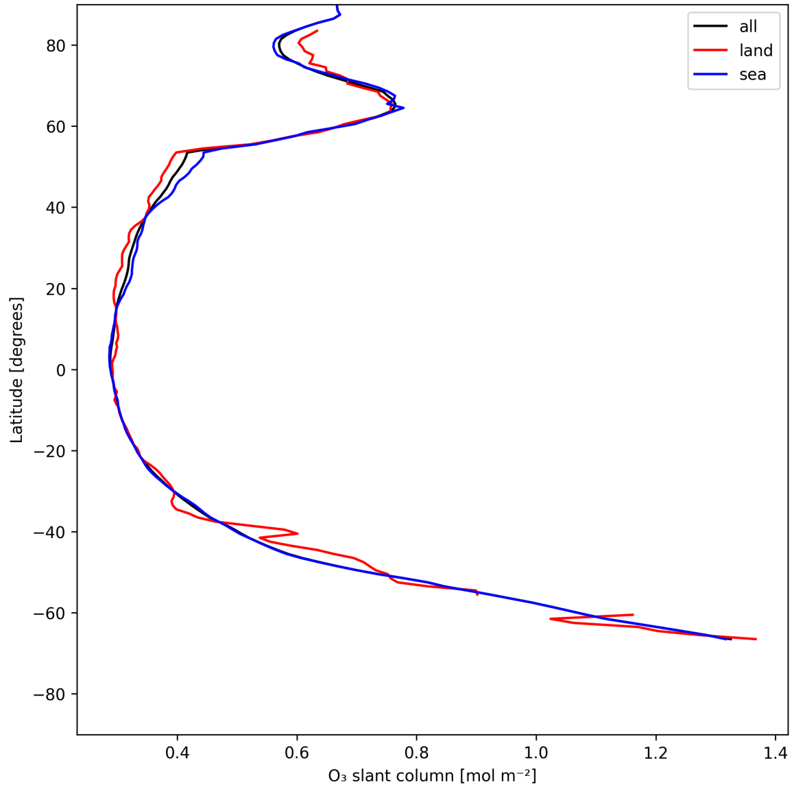
Figure 19: Zonal average of “O 3 slant column” for 2025-05-30 to 2025-05-31.
