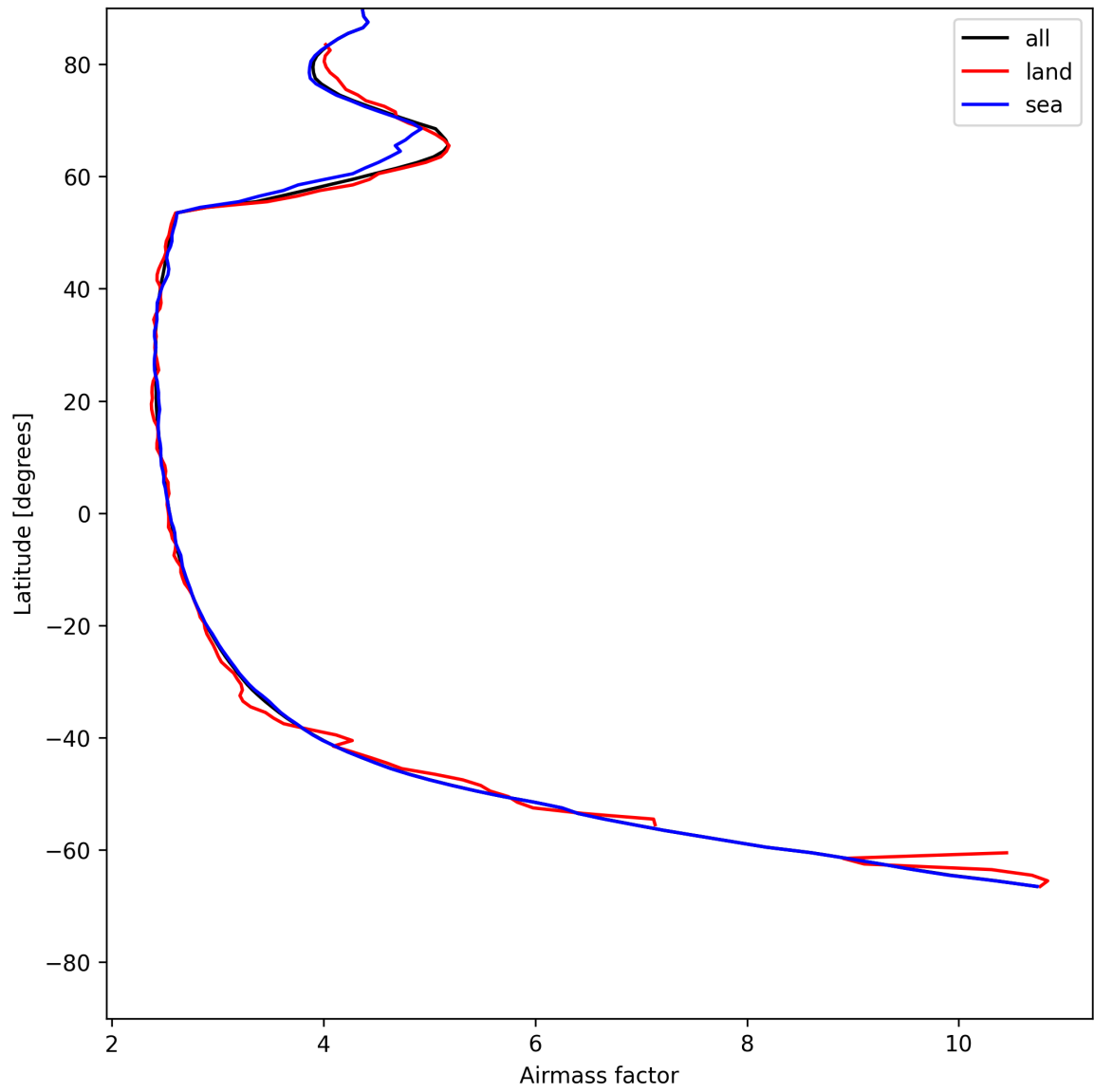
Figure 25: Zonal average of “Airmass factor” for 2025-05-30 to 2025-05-31.
