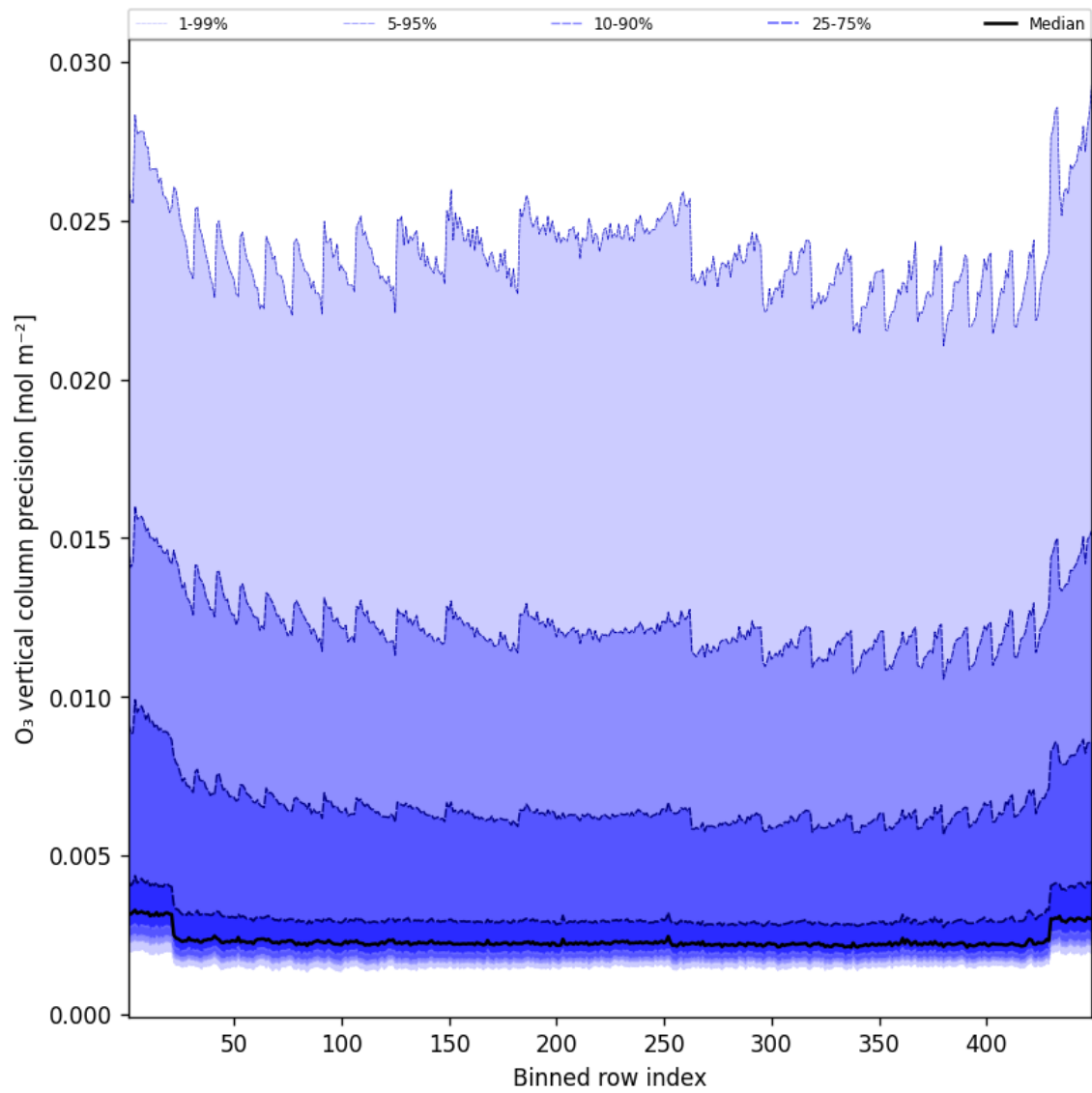
Figure 42: Along track statistics of “O 3 vertical column precision” for 2025-05-30 to 2025-05-31
