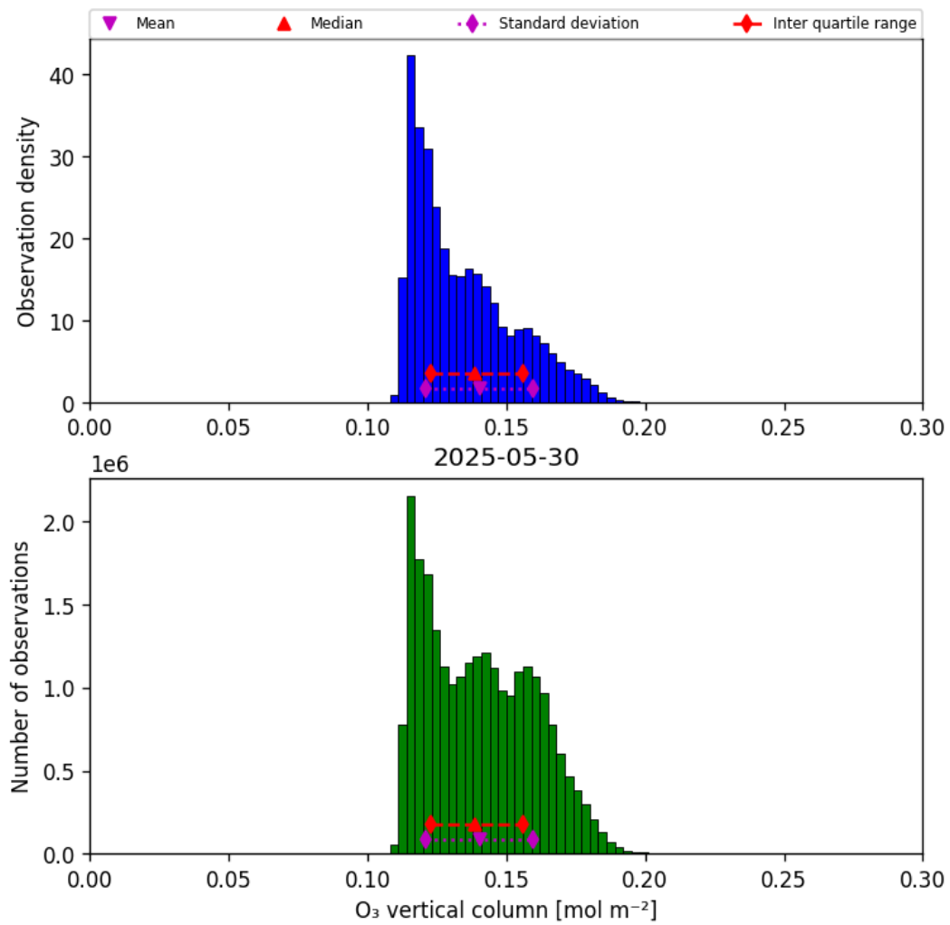
Figure 29: Histogram of “O 3 vertical column” for 2025-05-30 to 2025-05-31
