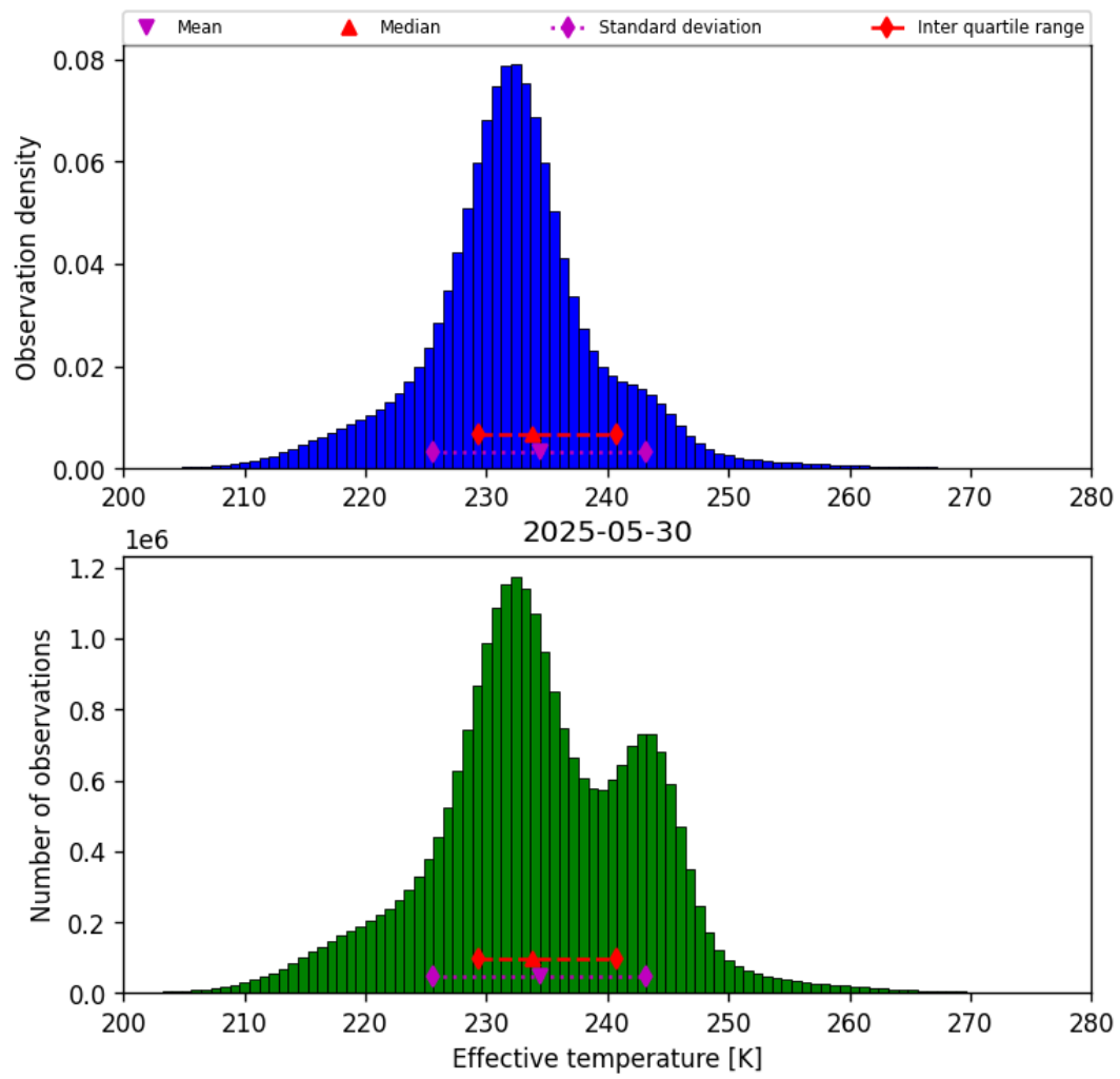
Figure 38: Histogram of “Effective temperature” for 2025-05-30 to 2025-05-31
