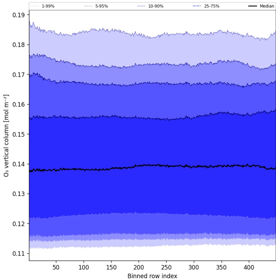
Figure 41: Along track statistics of “O 3 vertical column” for 2025-05-30 to 2025-05-31
