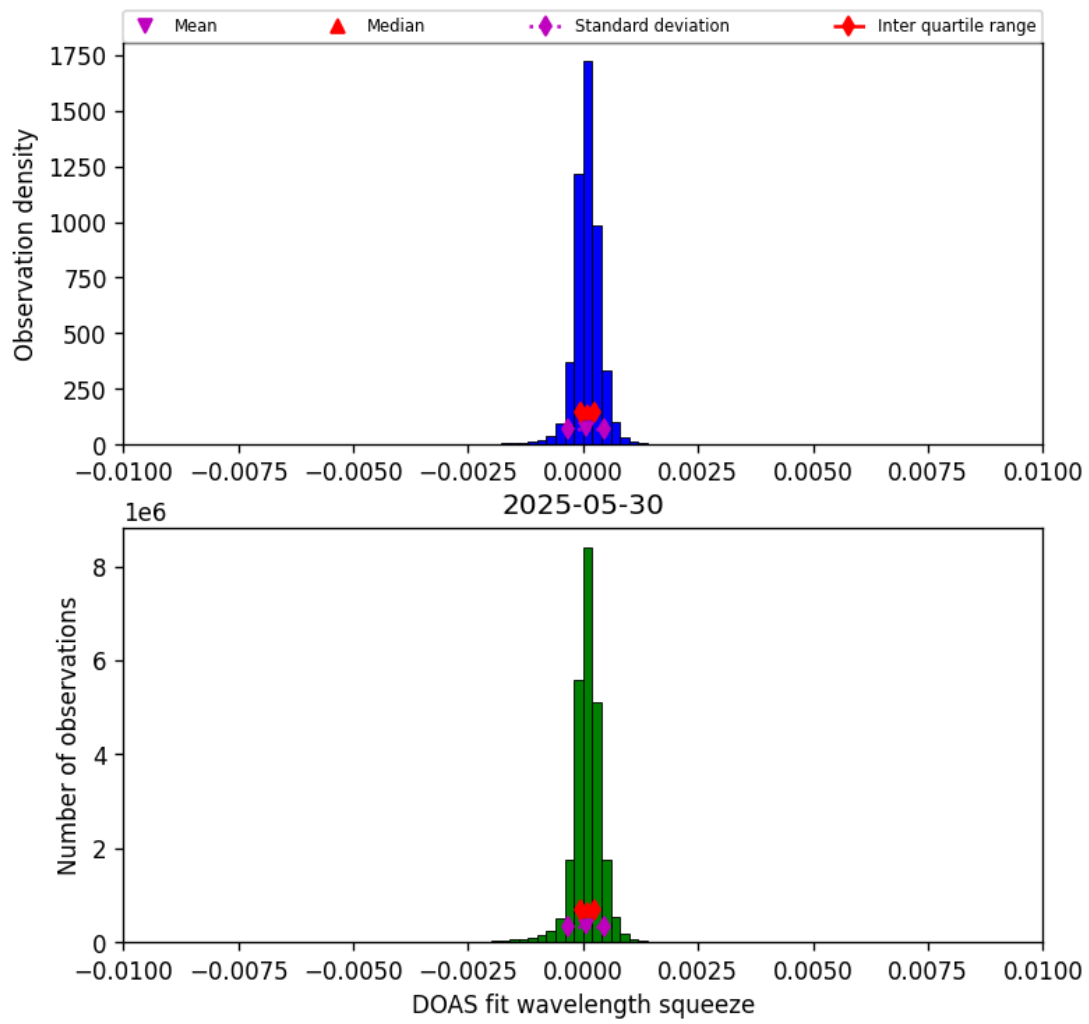
Figure 36: Histogram of “DOAS fit wavelength squeeze” for 2025-05-30 to 2025-05-31
