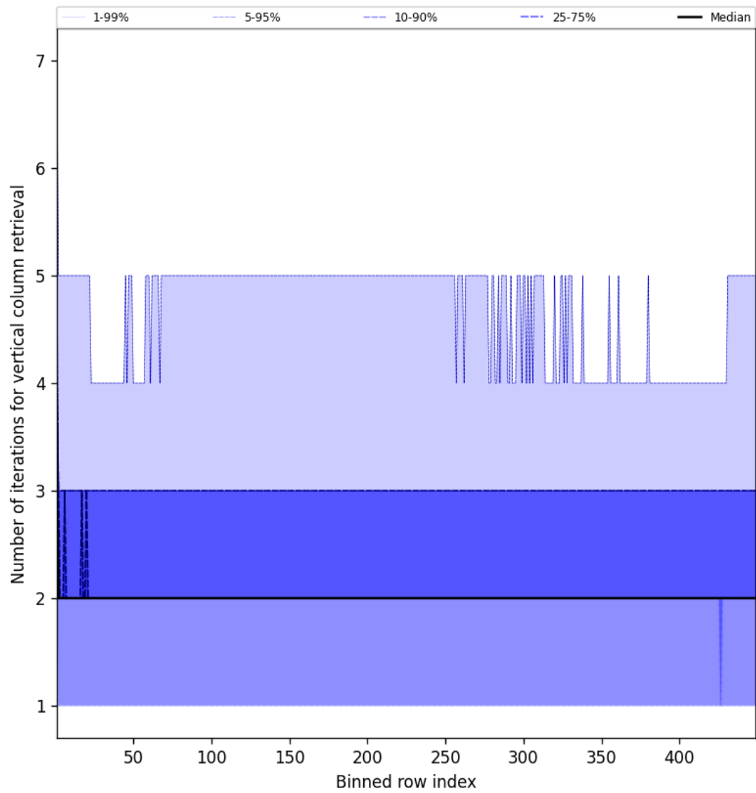
Figure 51: Along track statistics of “Number of iterations for vertical column retrieval” for 2025-05-30 to 2025-05-31
