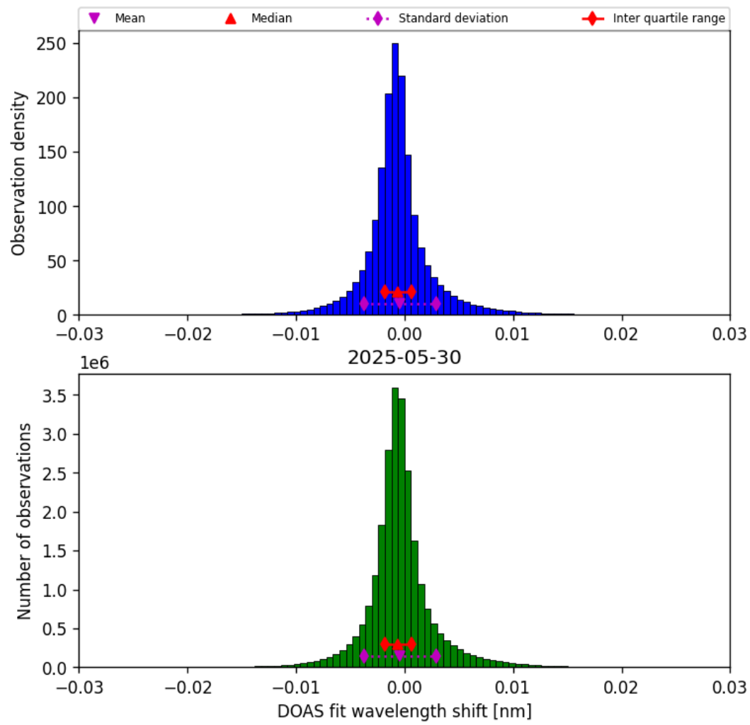
Figure 35: Histogram of “DOAS fit wavelength shift” for 2025-05-30 to 2025-05-31
