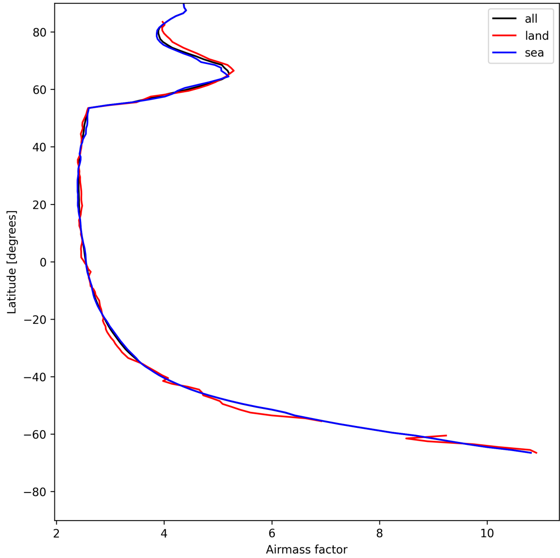
Figure 25: Zonal average of “Airmass factor” for 2025-05-31 to 2025-06-01.
