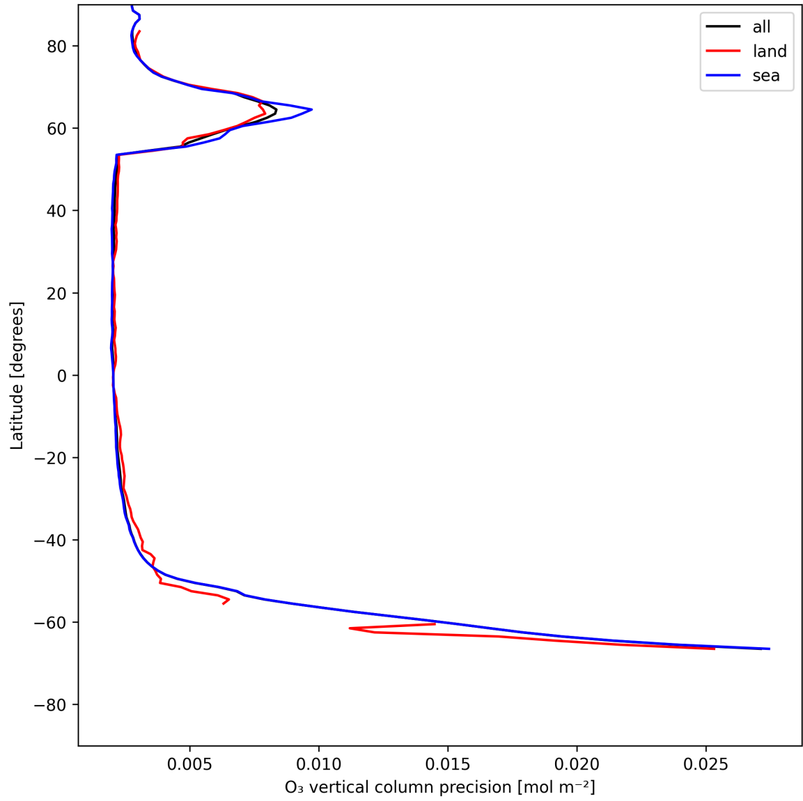
Figure 18: Zonal average of “O 3 vertical column precision” for 2025-05-31 to 2025-06-01.
