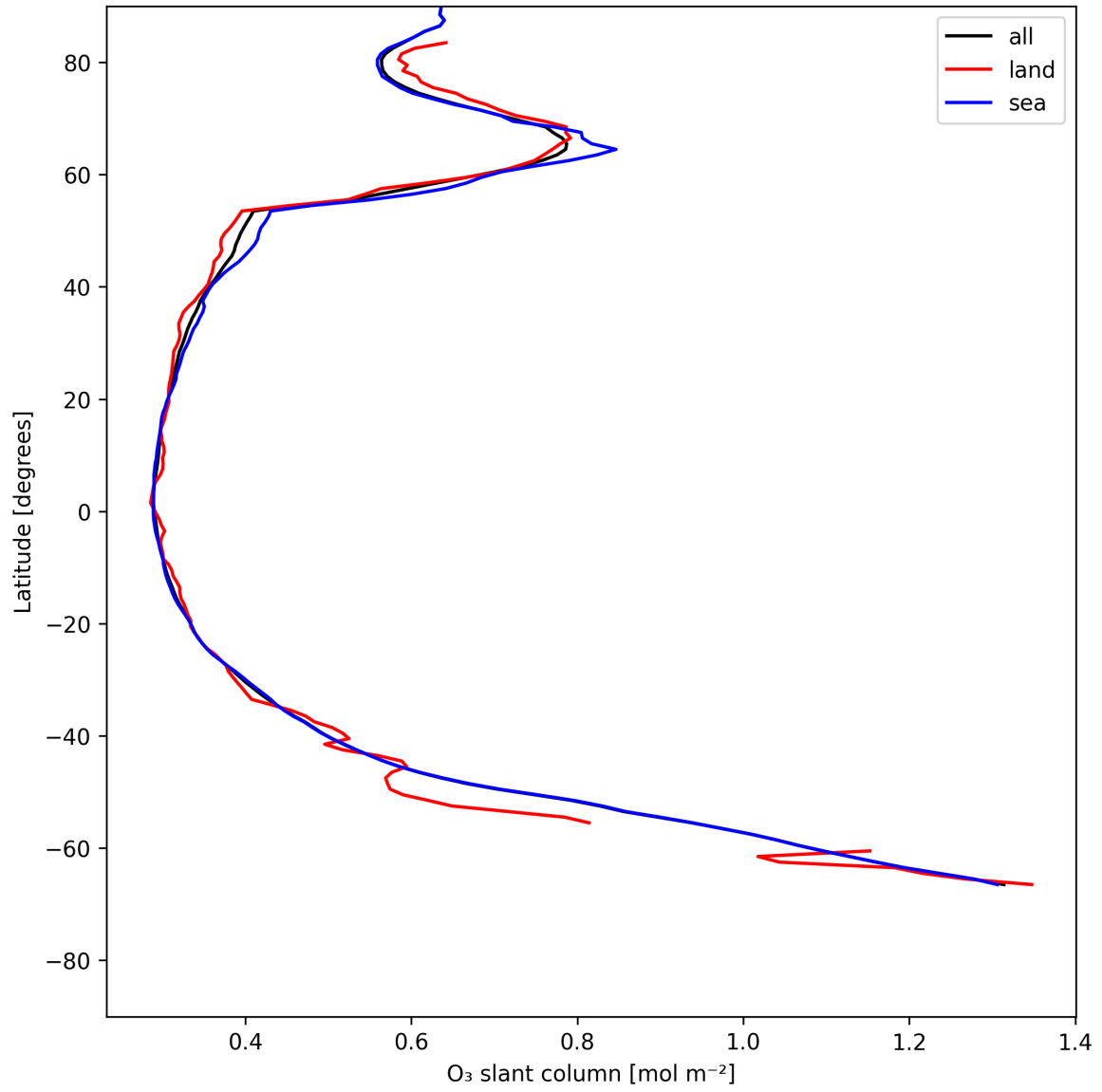
Figure 19: Zonal average of “O 3 slant column” for 2025-05-31 to 2025-06-01.
