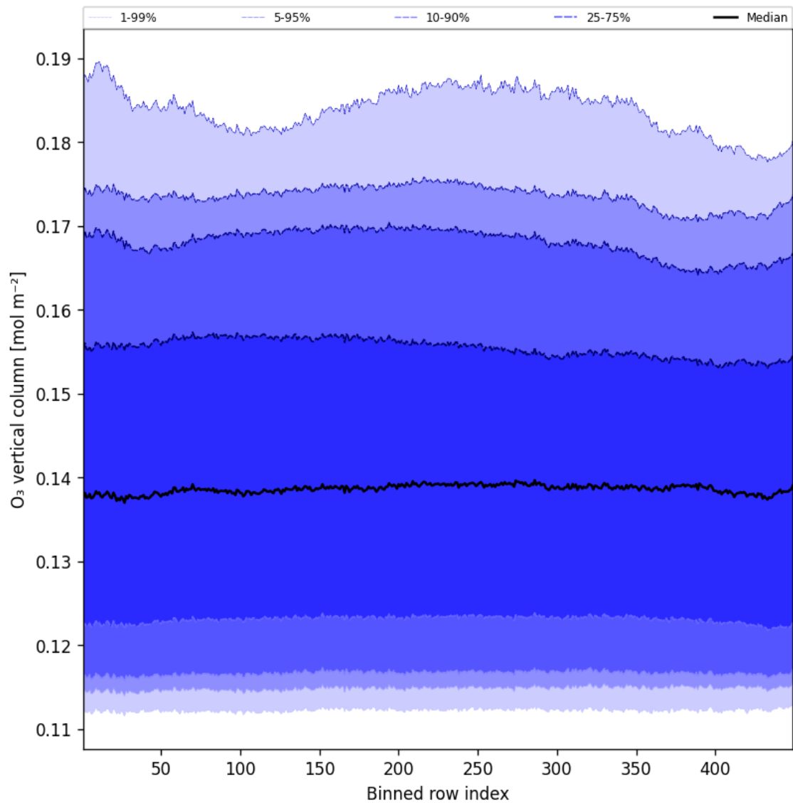
Figure 41: Along track statistics of “ \text{O}_3 vertical column” for 2025-05-31 to 2025-06-01
