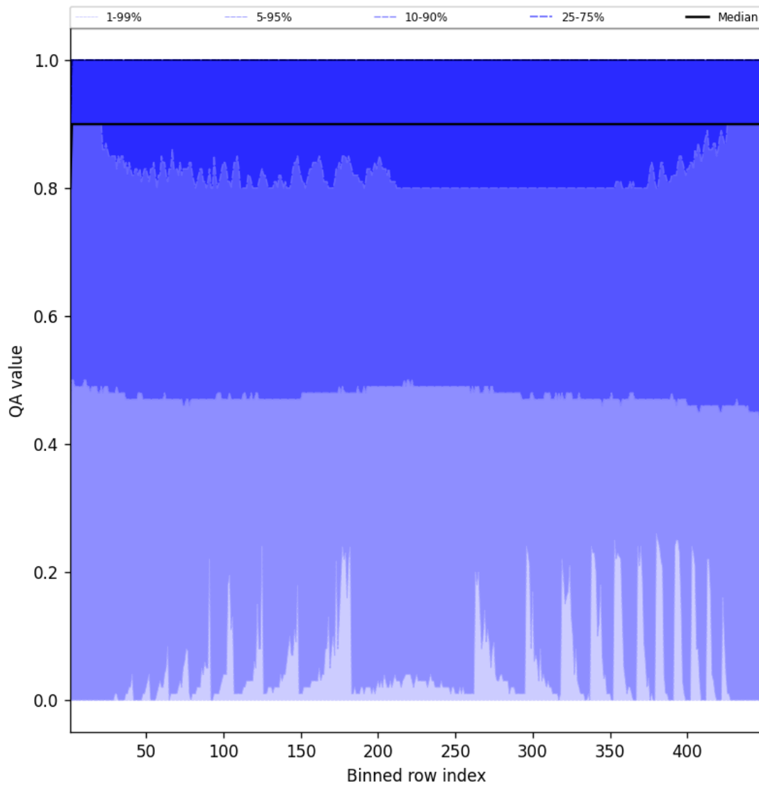
Figure 40: Along track statistics of “QA value” for 2025-05-31 to 2025-06-01
