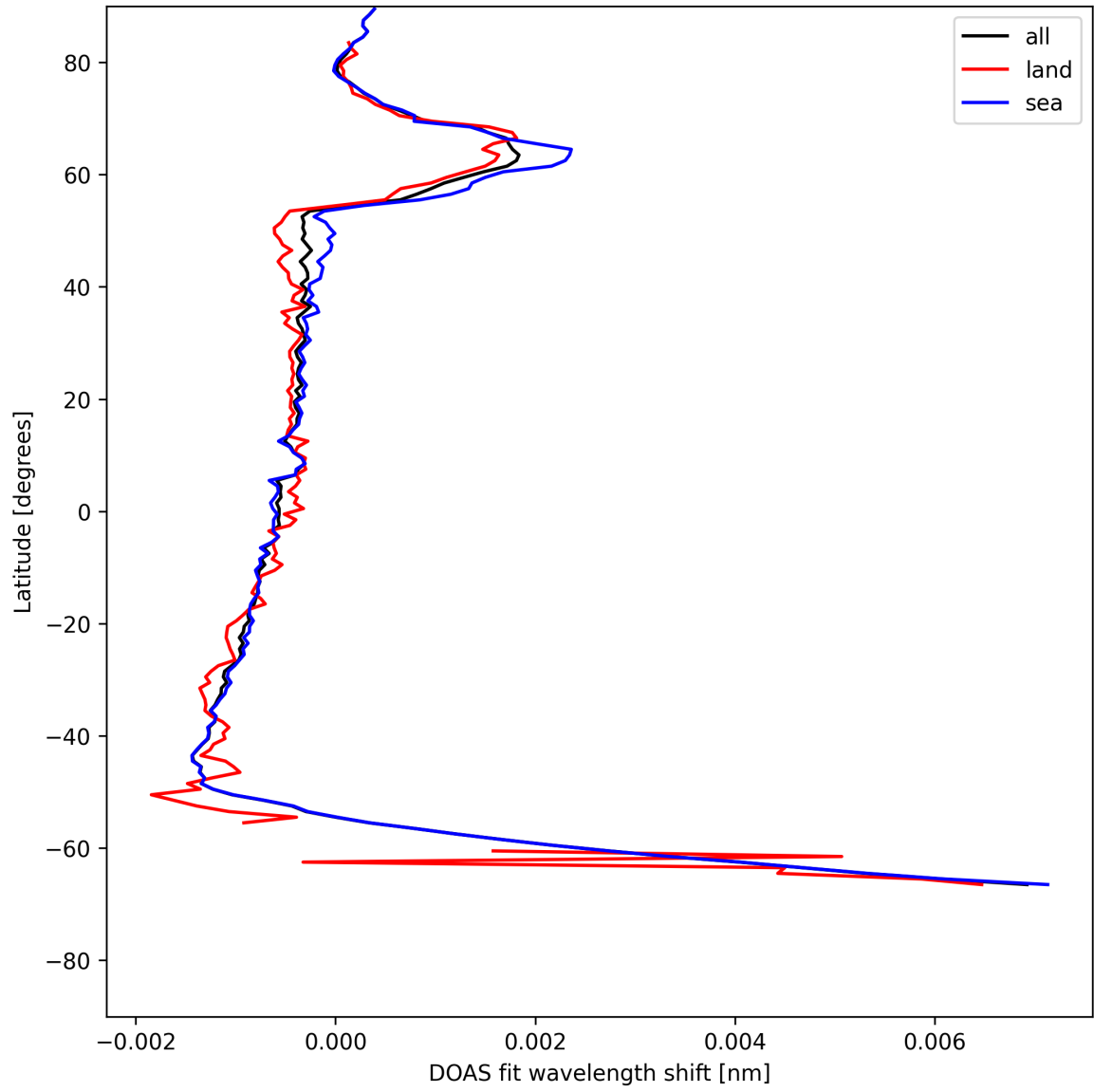
Figure 23: Zonal average of "DOAS fit wavelength shift" for 2025-05-31 to 2025-06-01.
