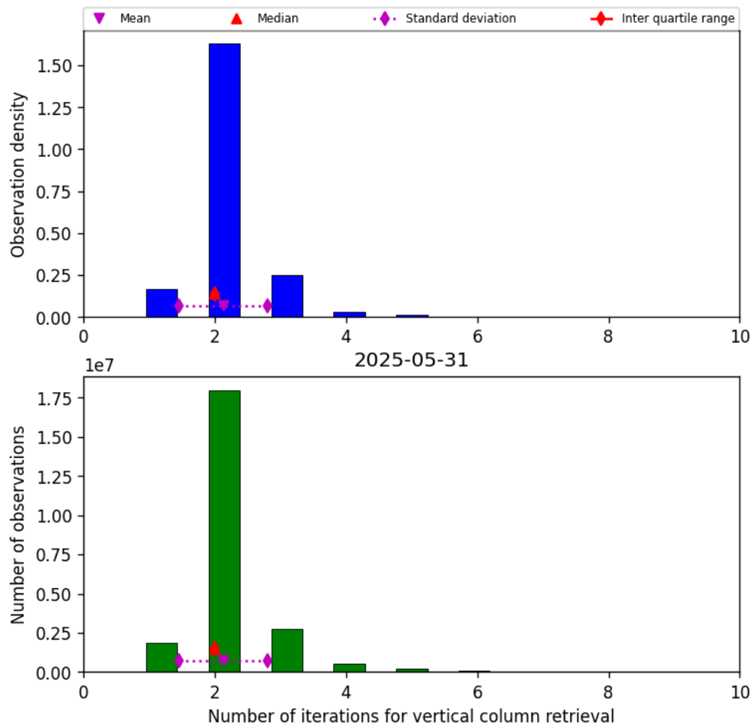
Figure 39: Histogram of “Number of iterations for vertical column retrieval” for 2025-05-31 to 2025-06-01
