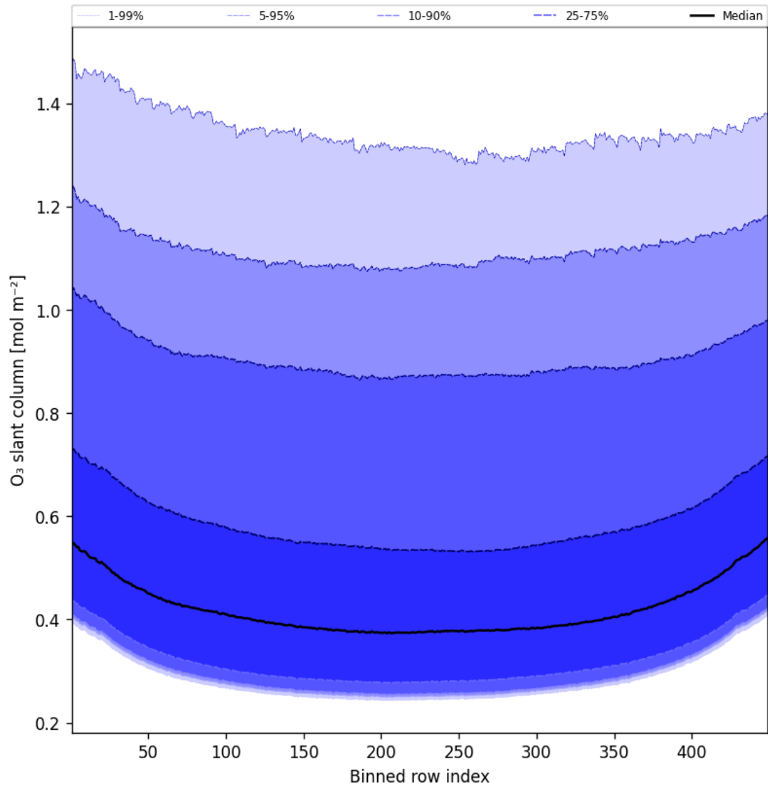
Figure 43: Along track statistics of “O 3 slant column” for 2025-05-31 to 2025-06-01
