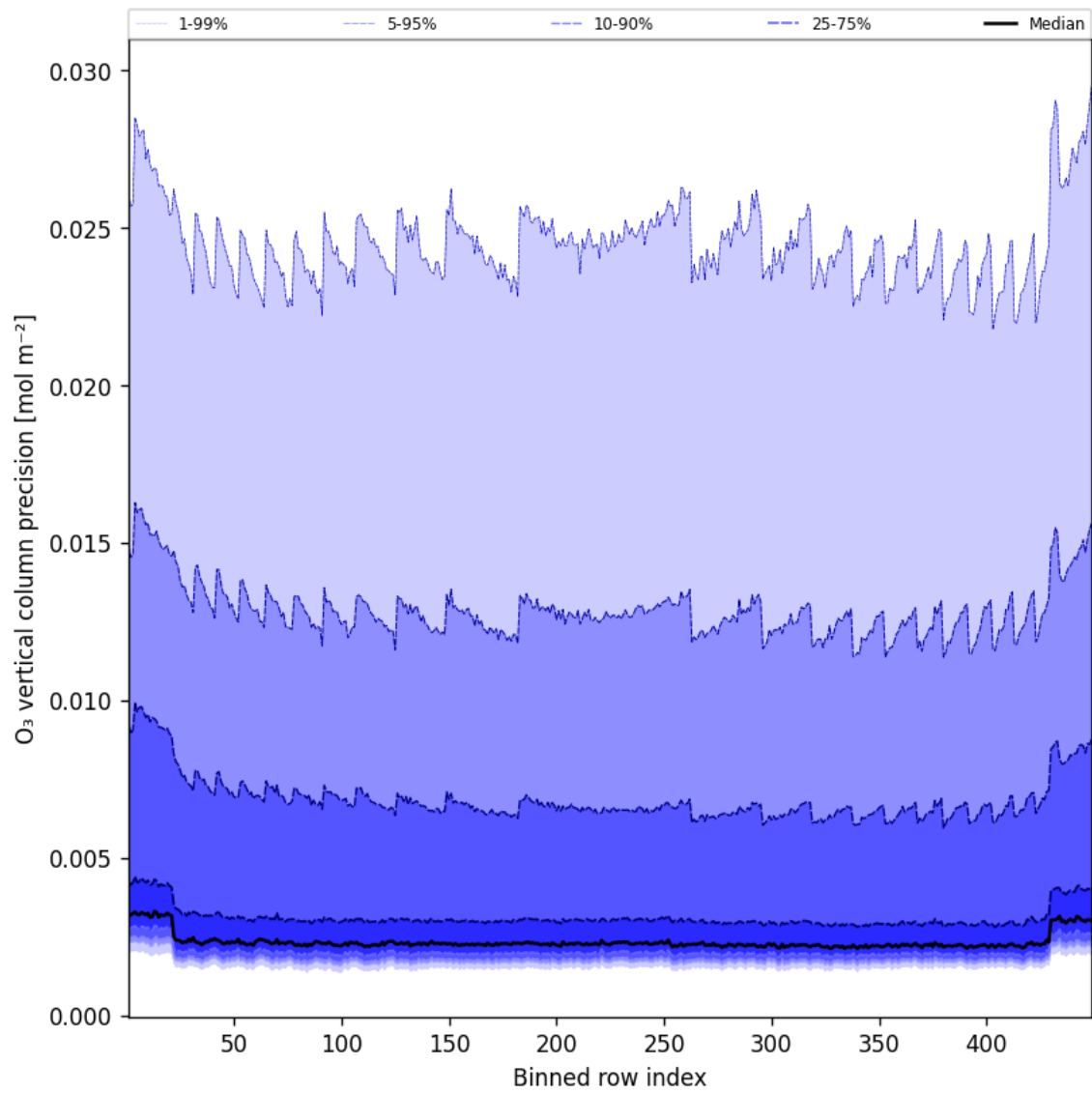
Figure 42: Along track statistics of “O 3 vertical column precision” for 2025-05-31 to 2025-06-01
