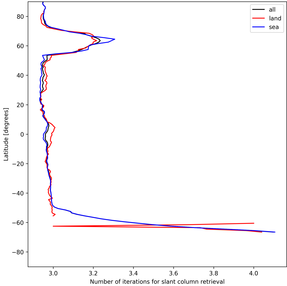
Figure 21: Zonal average of “Number of iterations for slant column retrieval” for 2025-05-31 to 2025-06-01.
