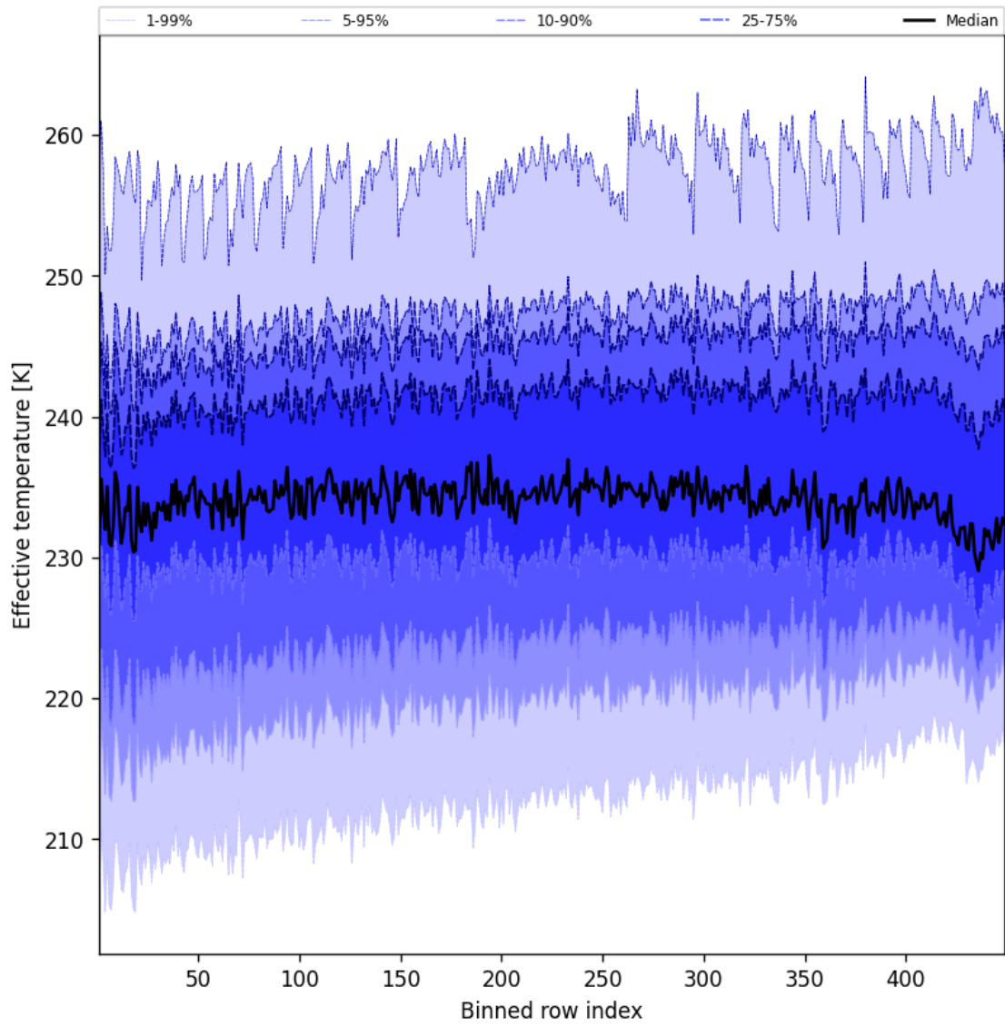
Figure 50: Along track statistics of “Effective temperature” for 2025-05-31 to 2025-06-01
