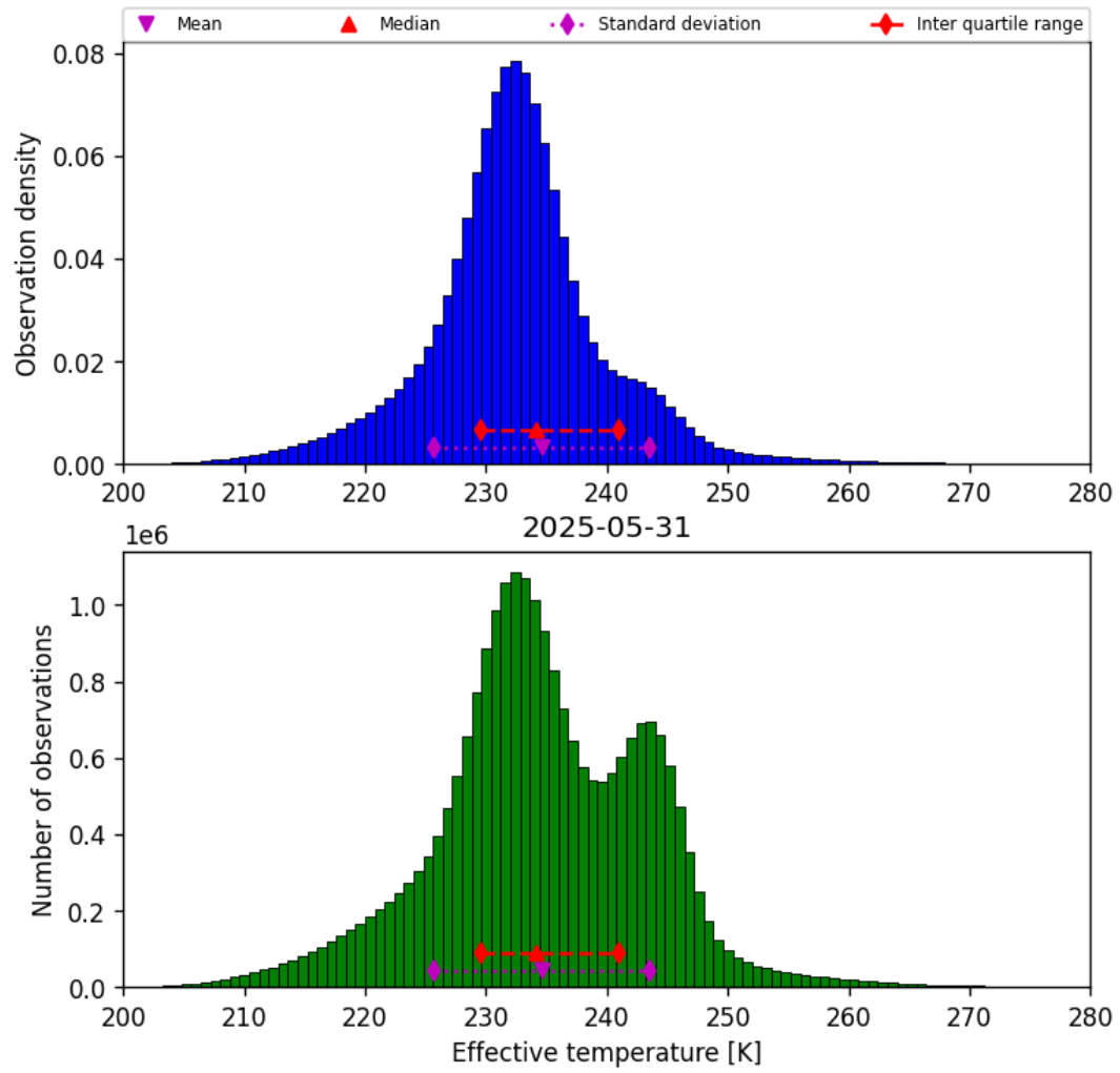
Figure 38: Histogram of “Effective temperature” for 2025-05-31 to 2025-06-01
