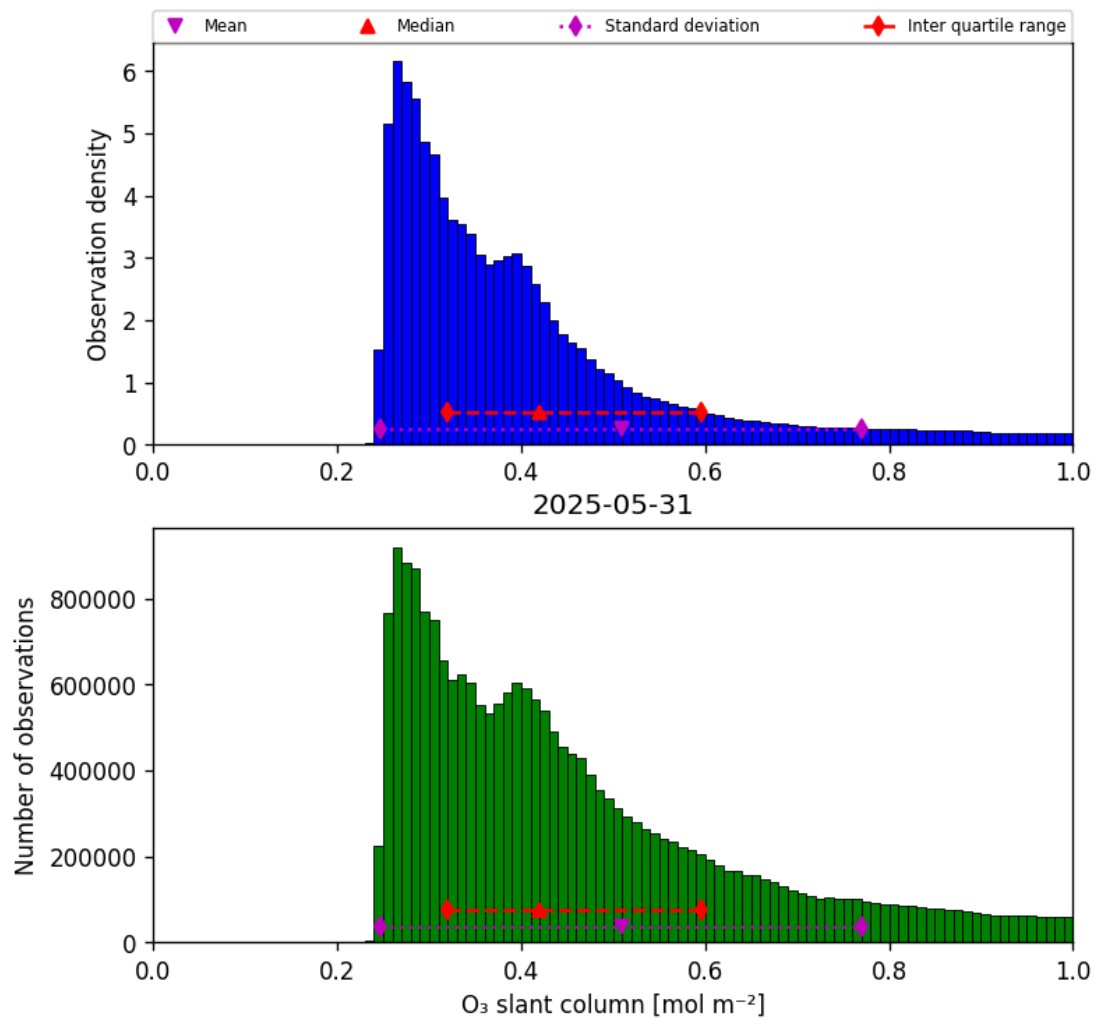
Figure 31: Histogram of “O 3 slant column” for 2025-05-31 to 2025-06-01
