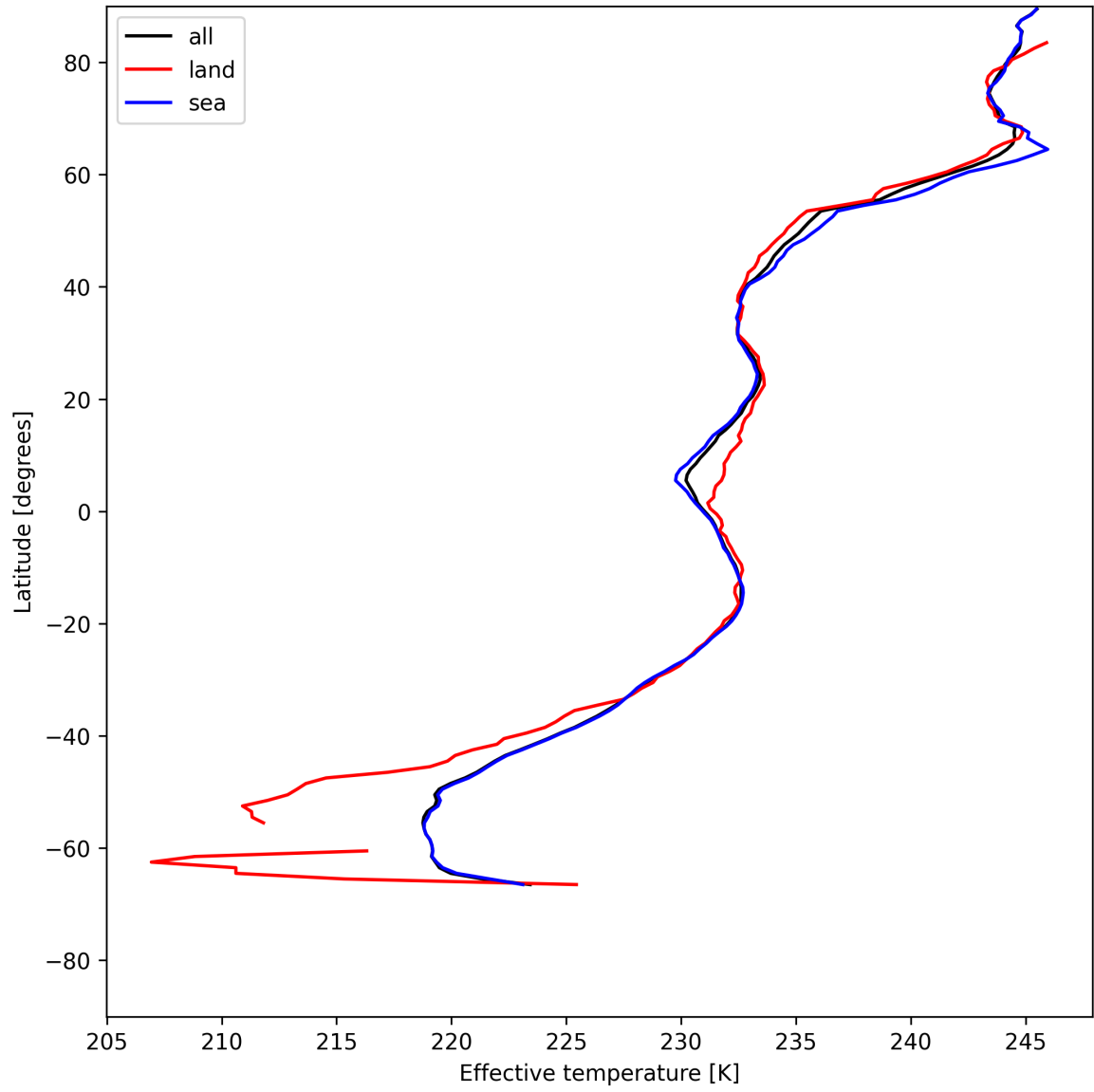
Figure 26: Zonal average of “Effective temperature” for 2025-05-31 to 2025-06-01.
