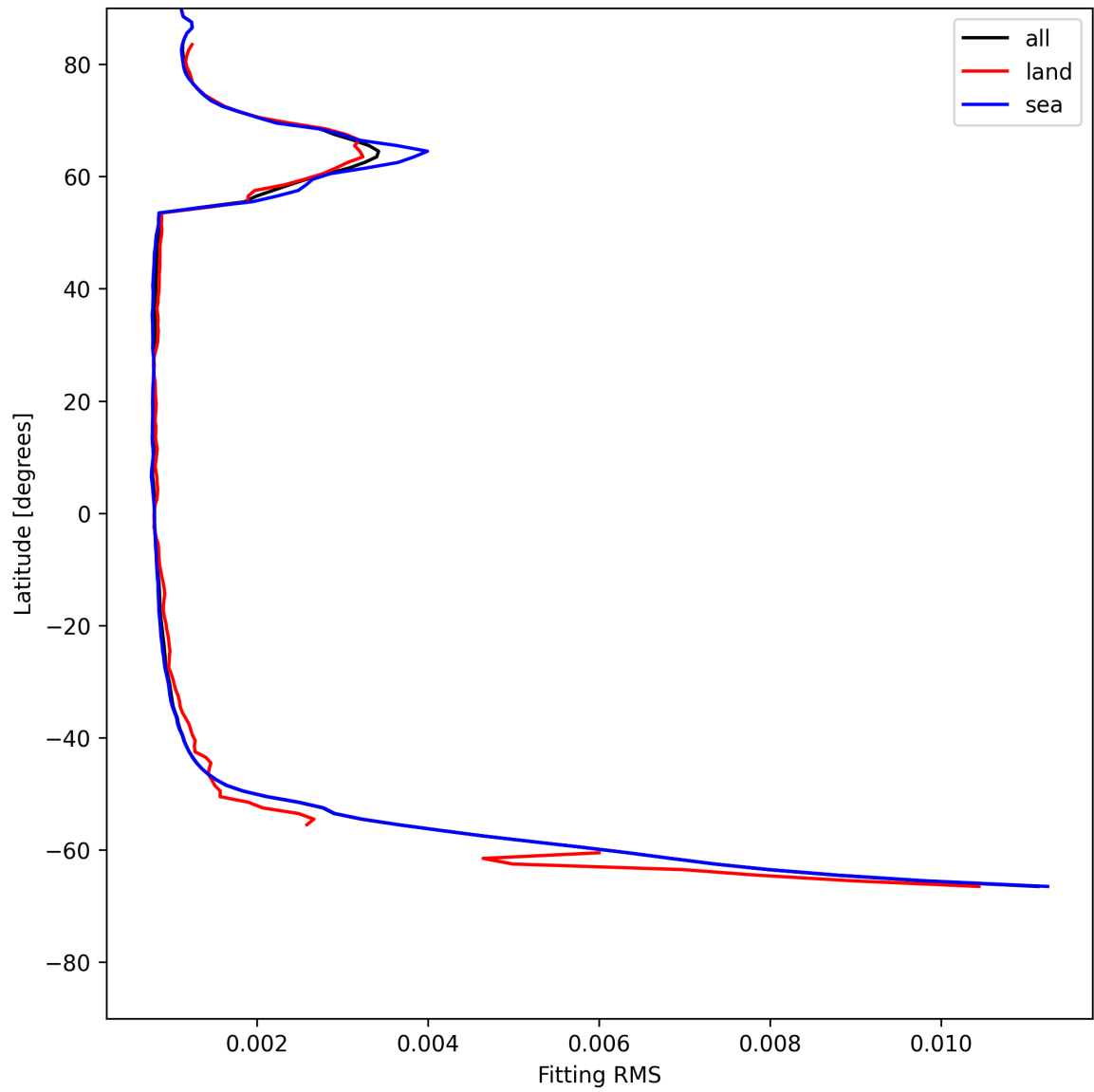
Figure 22: Zonal average of “Fitting RMS” for 2025-05-31 to 2025-06-01.
