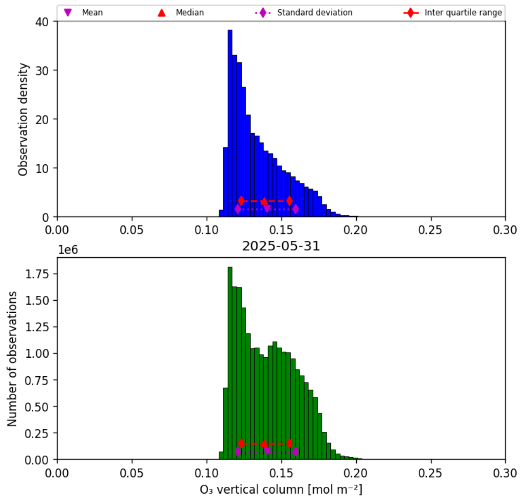
Figure 29: Histogram of “O 3 vertical column” for 2025-05-31 to 2025-06-01
