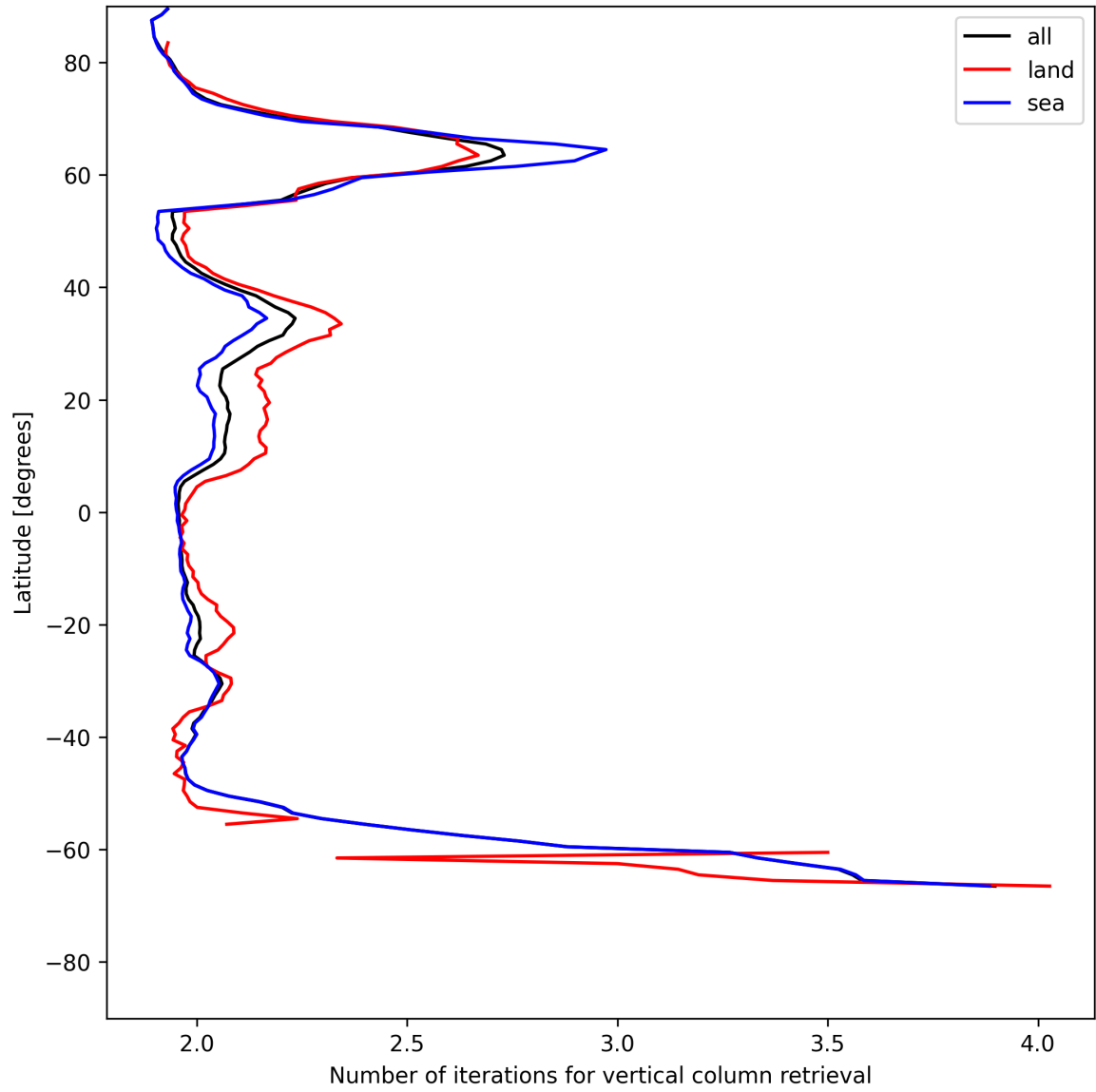
Figure 27: Zonal average of “Number of iterations for vertical column retrieval” for 2025-05-31 to 2025-06-01.
