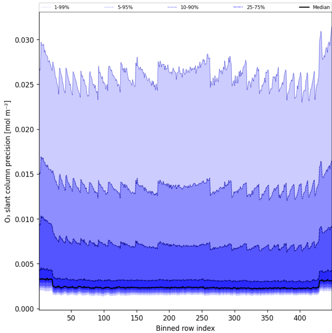
Figure 44: Along track statistics of “O 3 slant column precision” for 2025-05-31 to 2025-06-01
