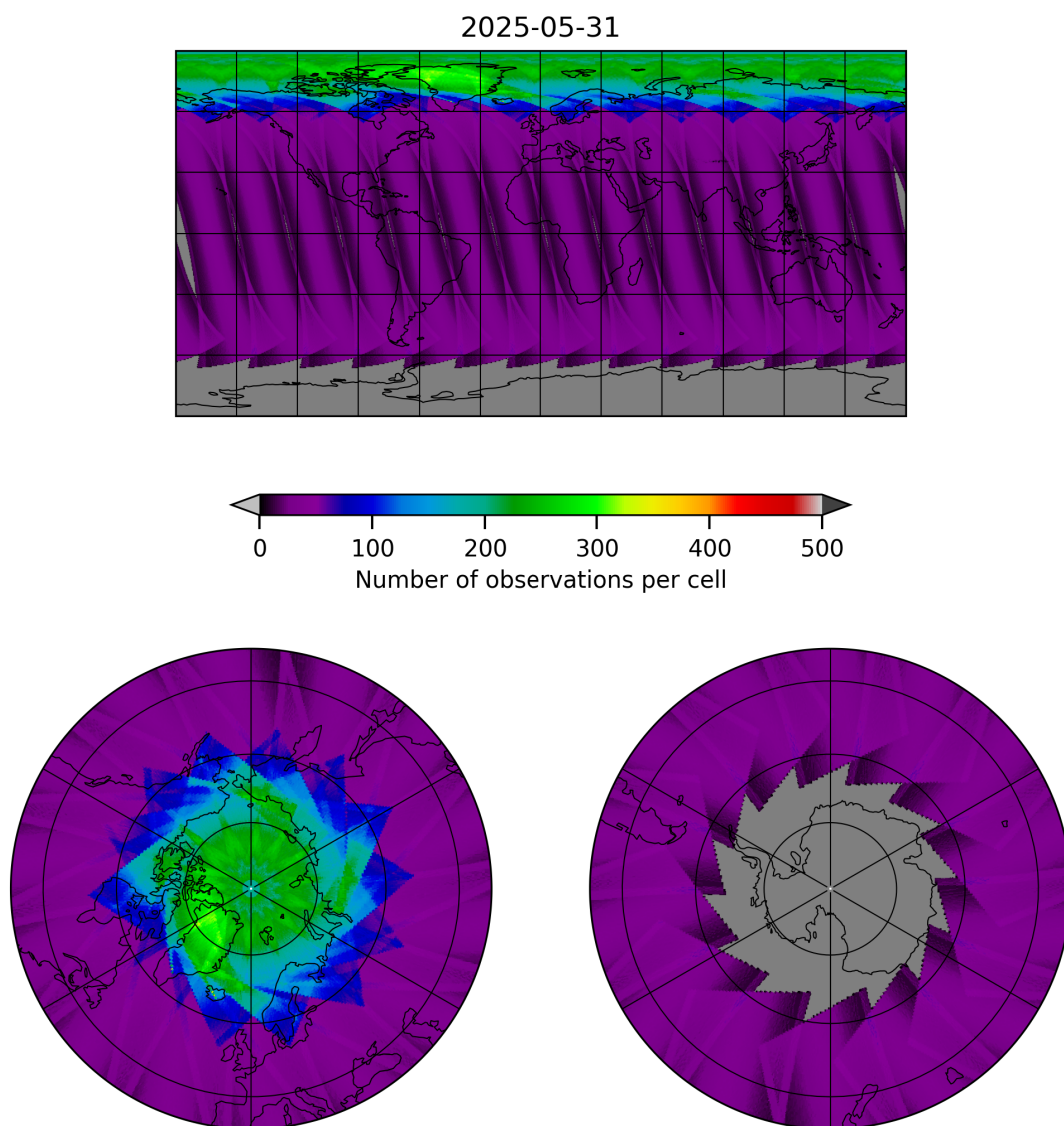
Figure 15: Map of the number of observations for 2025-05-31 to 2025-06-01
