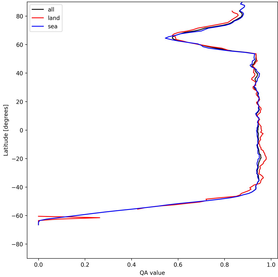
Figure 16: Zonal average of “QA value” for 2025-05-31 to 2025-06-01.
