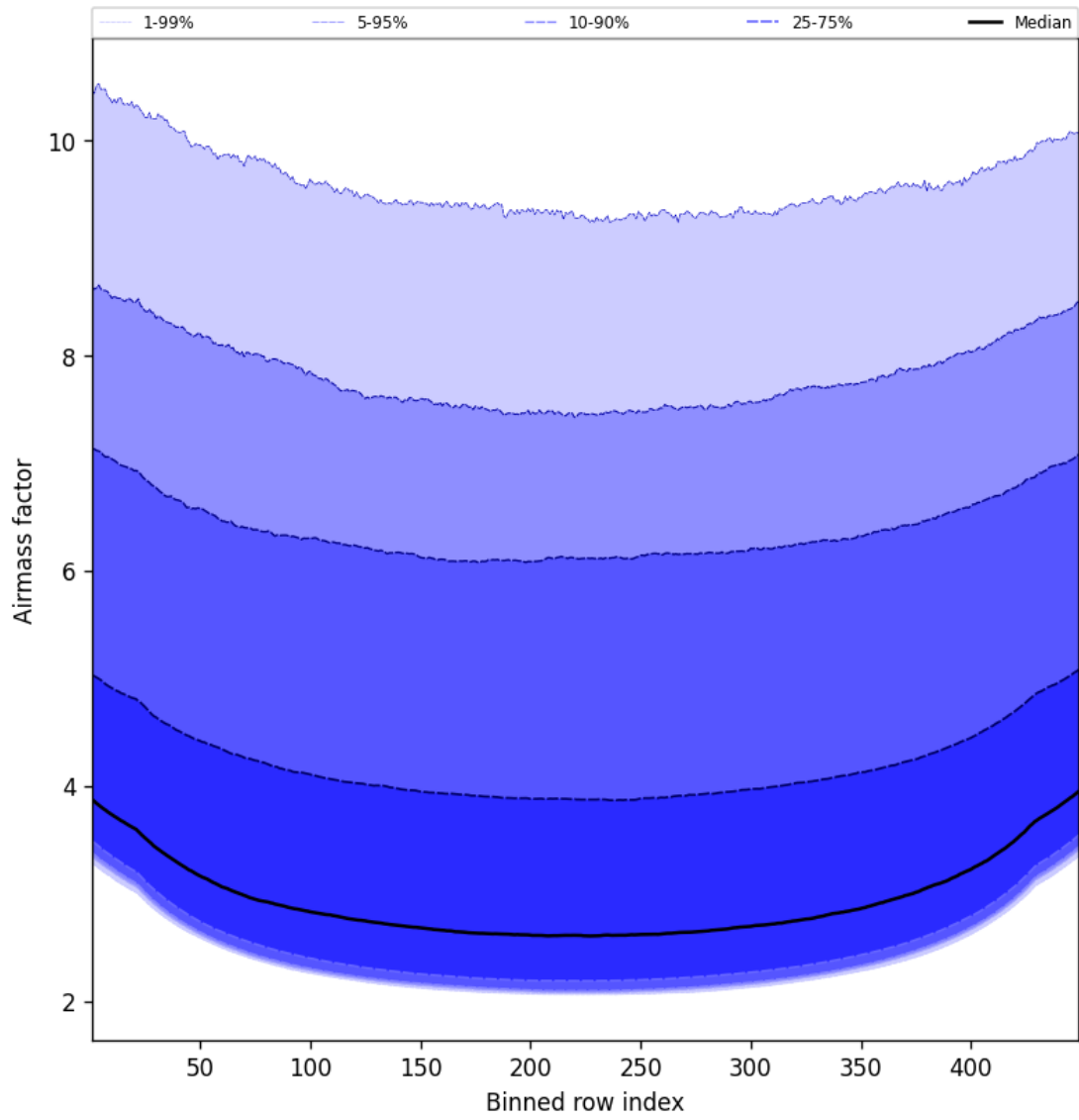
Figure 49: Along track statistics of “Airmass factor” for 2025-05-31 to 2025-06-01
