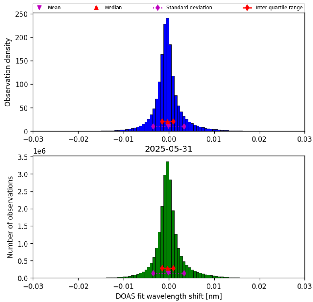
Figure 35: Histogram of “DOAS fit wavelength shift” for 2025-05-31 to 2025-06-01
