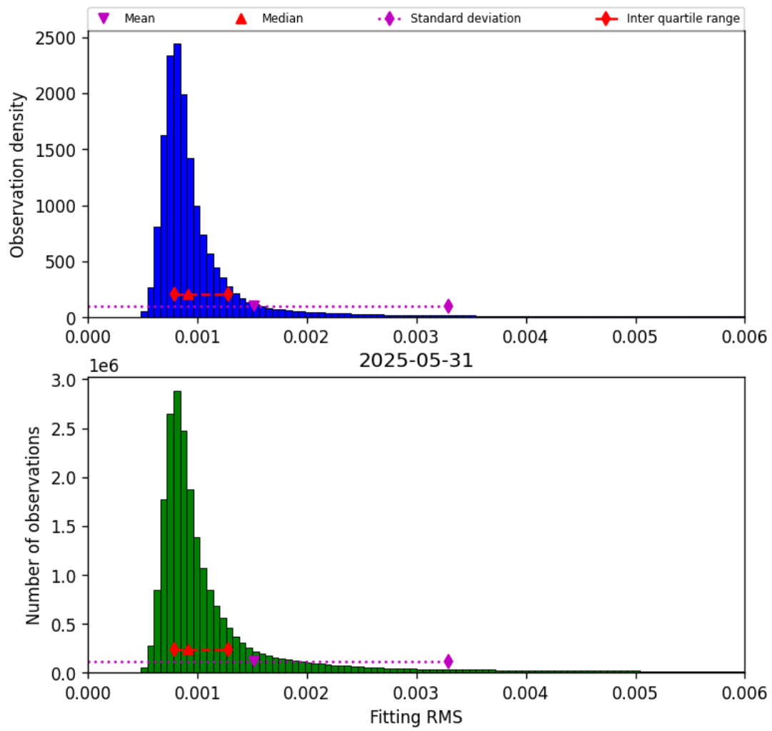
Figure 34: Histogram of “Fitting RMS” for 2025-05-31 to 2025-06-01
