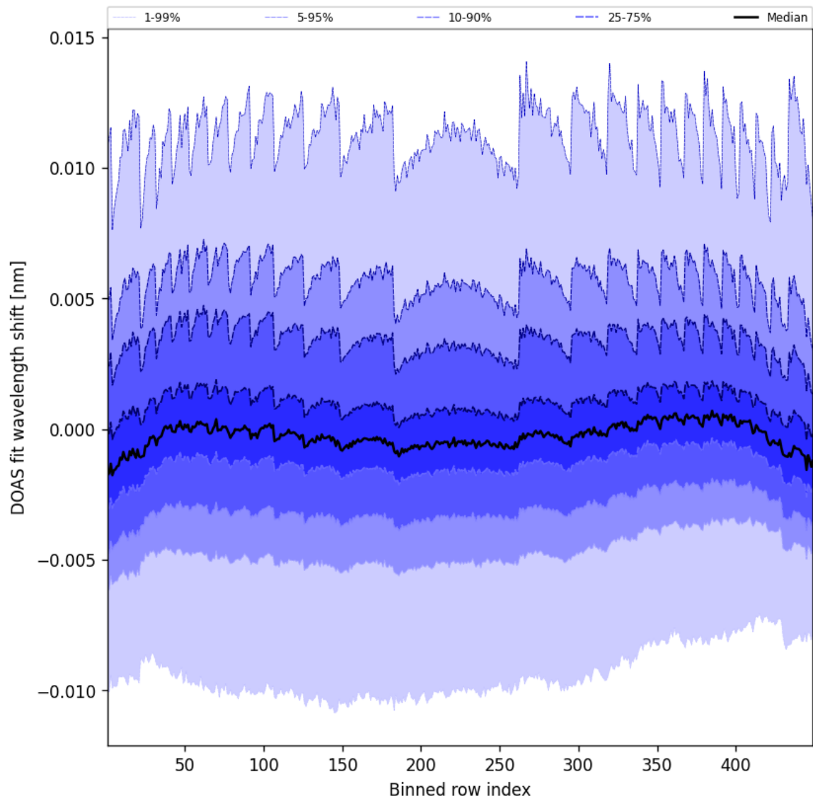
Figure 47: Along track statistics of “DOAS fit wavelength shift” for 2025-05-31 to 2025-06-01
