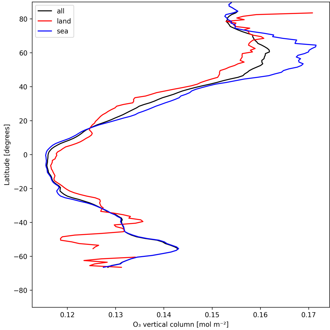
Figure 17: Zonal average of “O 3 vertical column” for 2025-05-31 to 2025-06-01.
