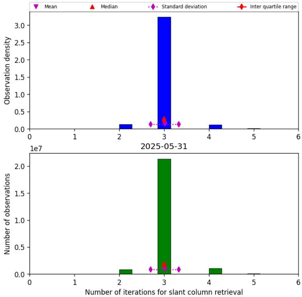
Figure 33: Histogram of “Number of iterations for slant column retrieval” for 2025-05-31 to 2025-06-01
