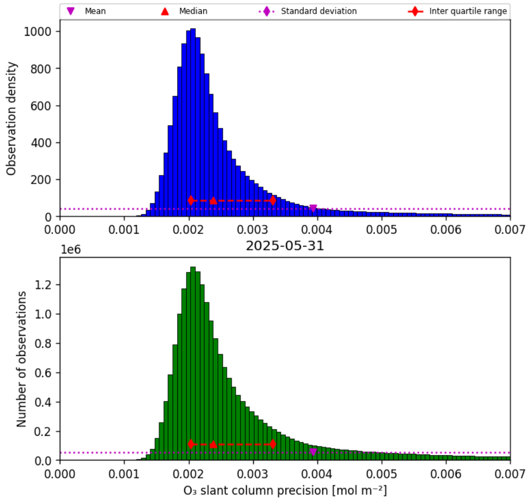
Figure 32: Histogram of “O 3 slant column precision” for 2025-05-31 to 2025-06-01
