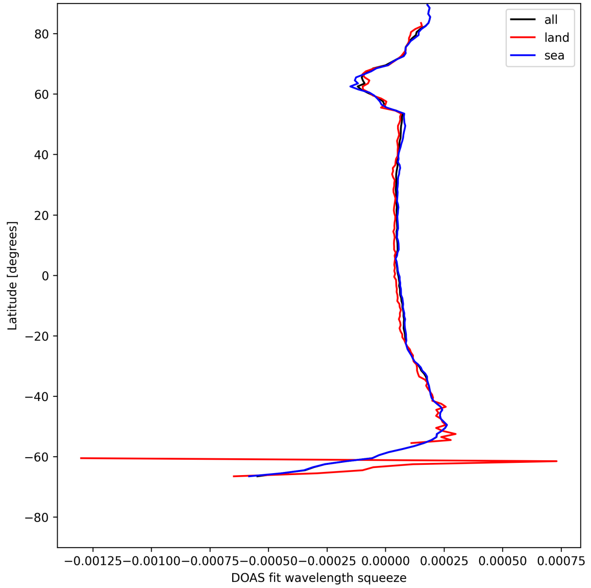
Figure 24: Zonal average of “DOAS fit wavelength squeeze” for 2025-05-31 to 2025-06-01.
