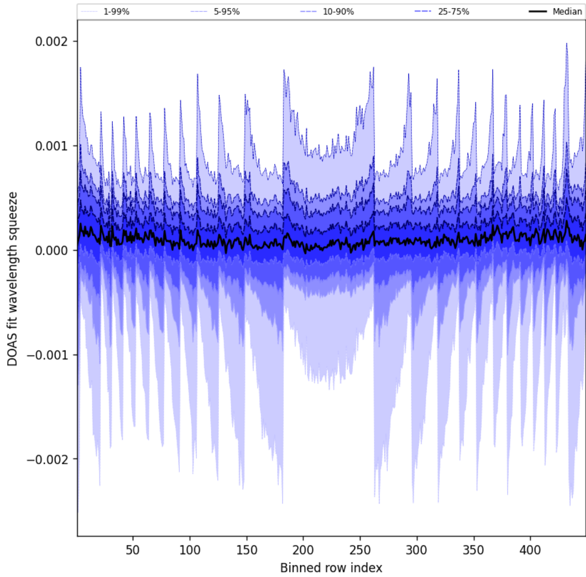
Figure 48: Along track statistics of “DOAS fit wavelength squeeze” for 2025-05-31 to 2025-06-01
