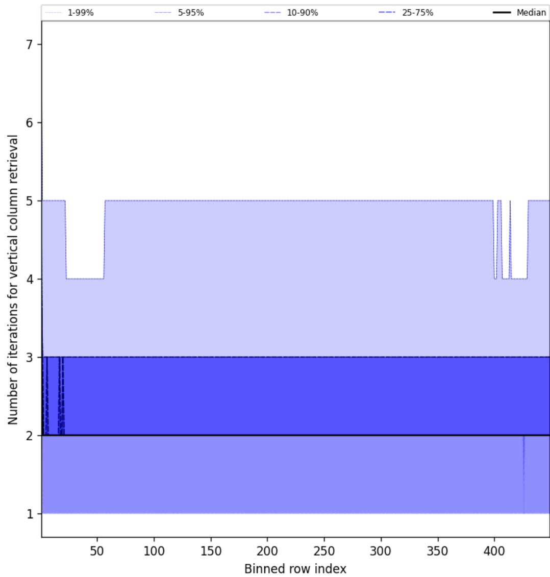
Figure 51: Along track statistics of “Number of iterations for vertical column retrieval” for 2025-05-31 to 2025-06-01
