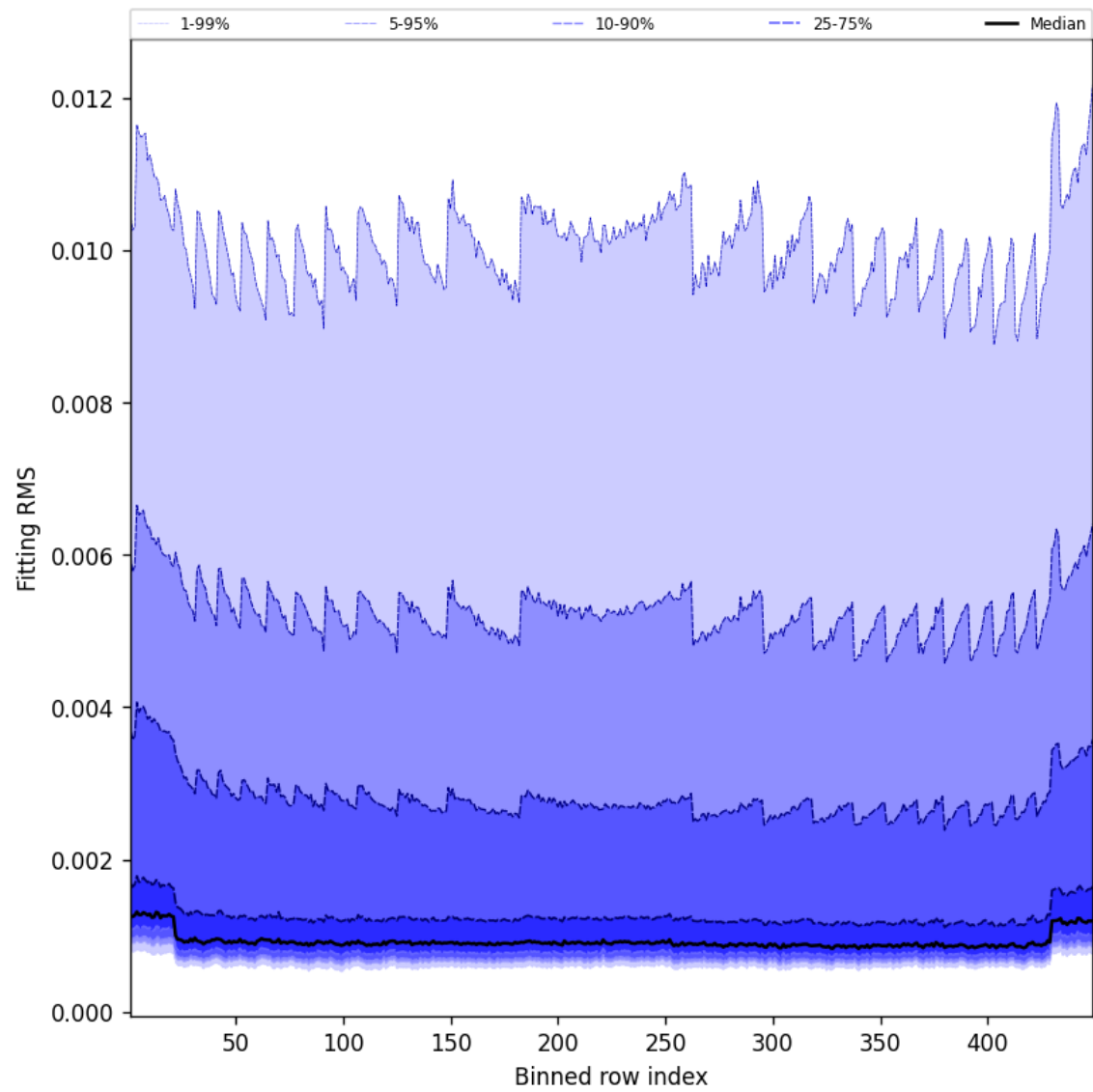
Figure 46: Along track statistics of “Fitting RMS” for 2025-05-31 to 2025-06-01
