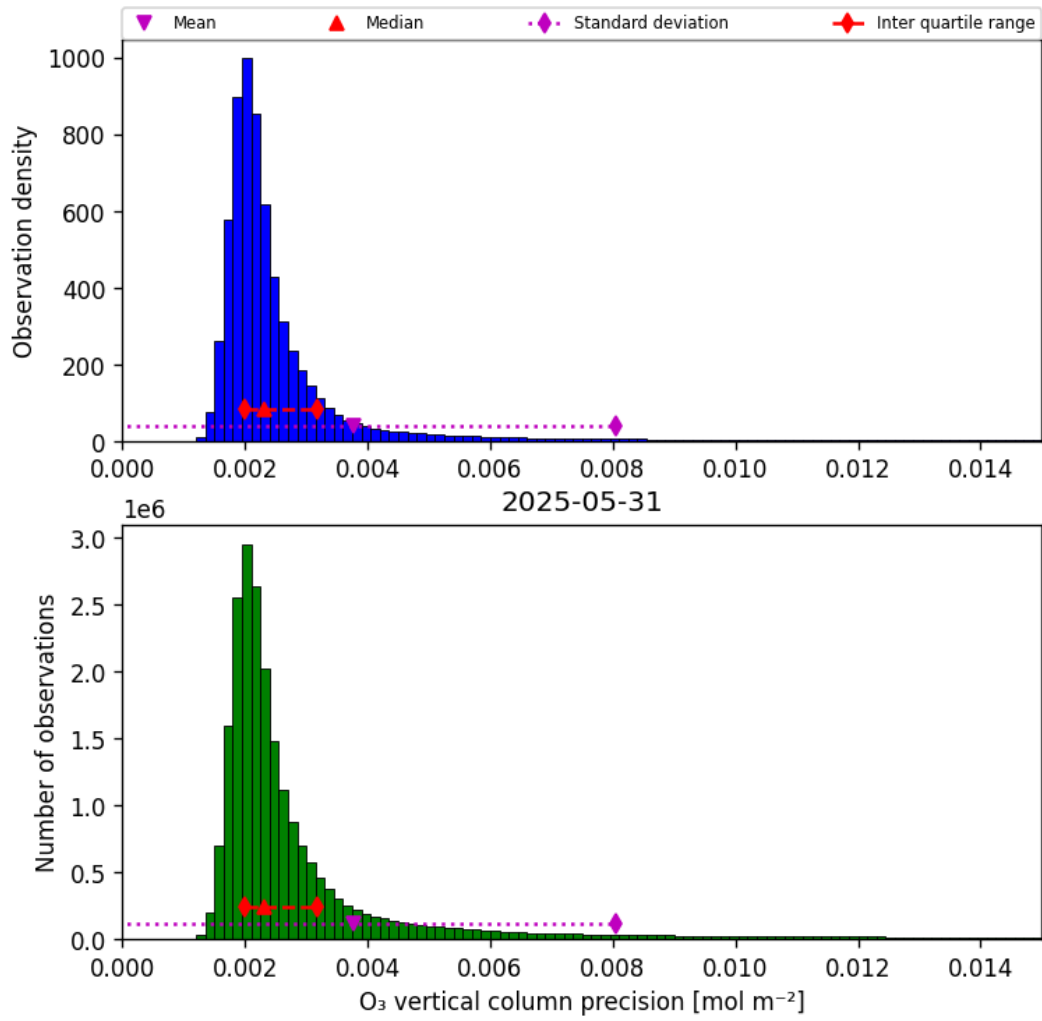
Figure 30: Histogram of “O 3 vertical column precision” for 2025-05-31 to 2025-06-01
