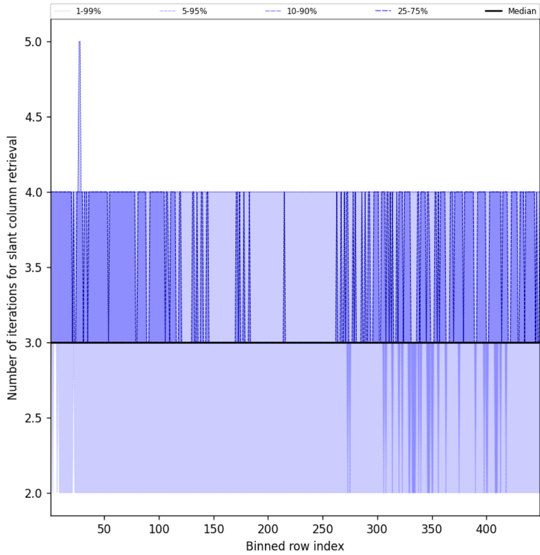
Figure 45: Along track statistics of “Number of iterations for slant column retrieval” for 2025-05-31 to 2025-06-01
