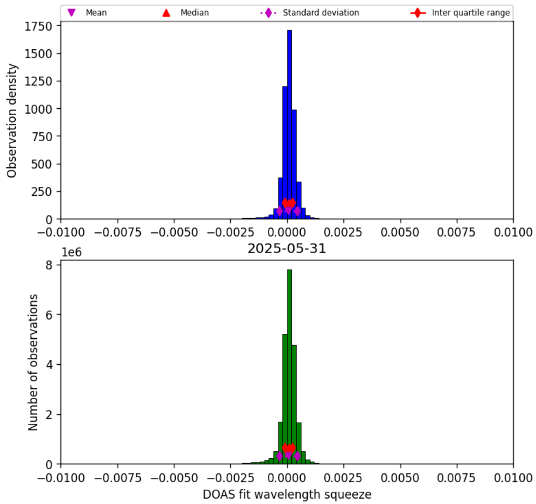
Figure 36: Histogram of “DOAS fit wavelength squeeze” for 2025-05-31 to 2025-06-01
