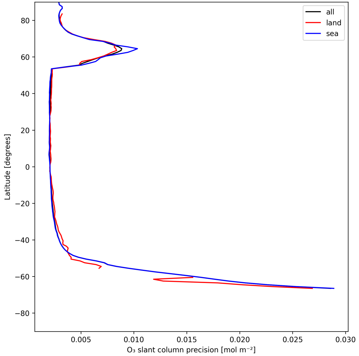
Figure 20: Zonal average of “O 3 slant column precision” for 2025-05-31 to 2025-06-01.
