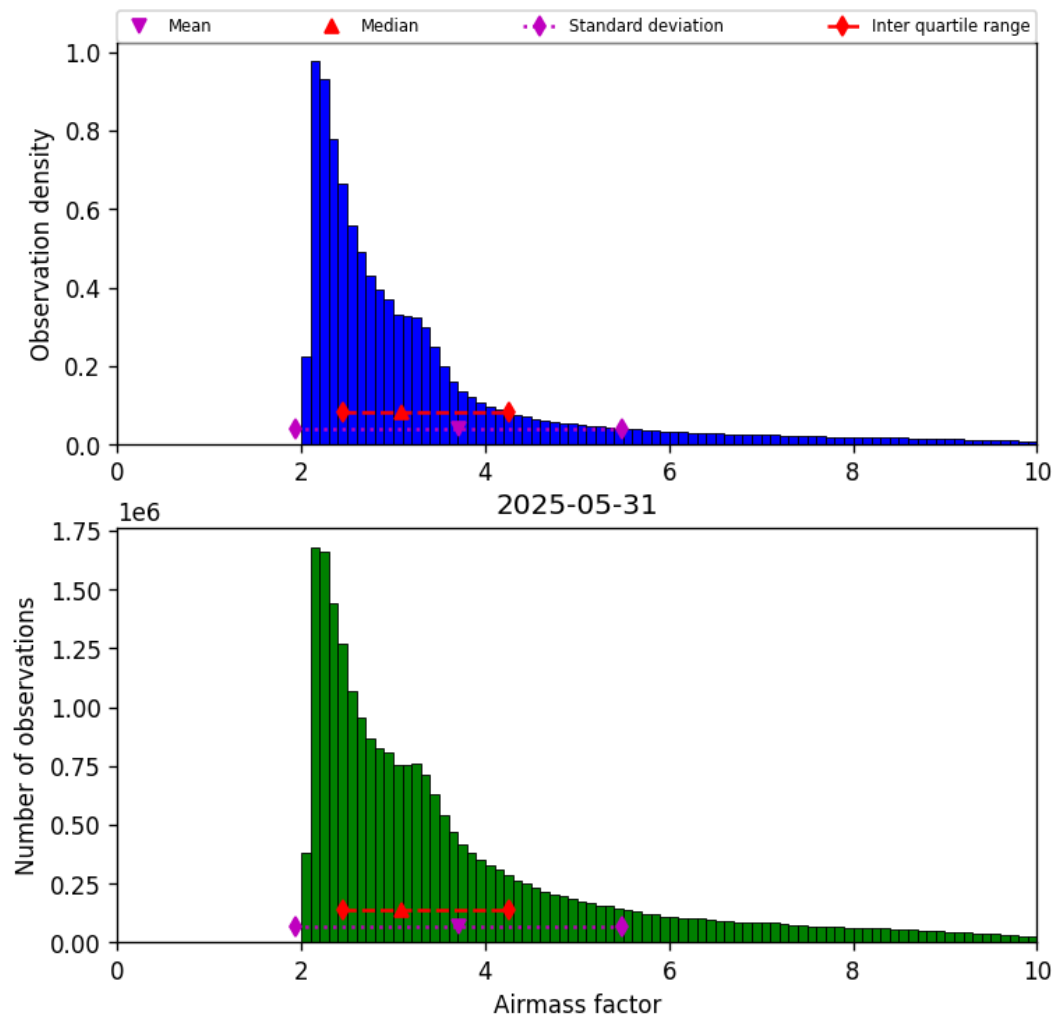
Figure 37: Histogram of “Airmass factor” for 2025-05-31 to 2025-06-01
