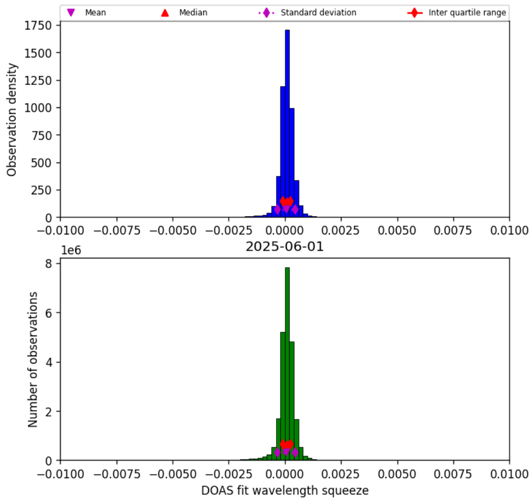
Figure 36: Histogram of “DOAS fit wavelength squeeze” for 2025-06-01 to 2025-06-02
