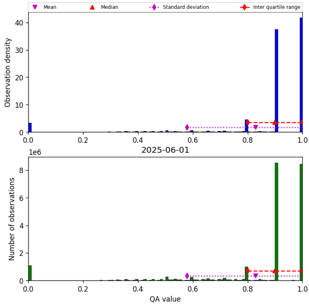
Figure 28: Histogram of “QA value” for 2025-06-01 to 2025-06-02
