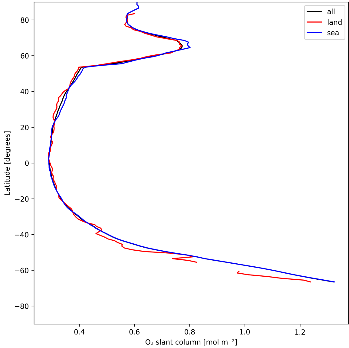
Figure 19: Zonal average of “O 3 slant column” for 2025-06-01 to 2025-06-02.
