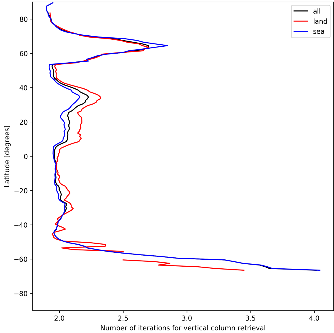
Figure 27: Zonal average of “Number of iterations for vertical column retrieval” for 2025-06-01 to 2025-06-02.
