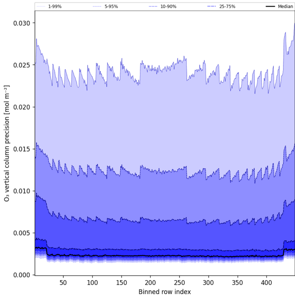
Figure 42: Along track statistics of “O 3 vertical column precision” for 2025-06-01 to 2025-06-02
