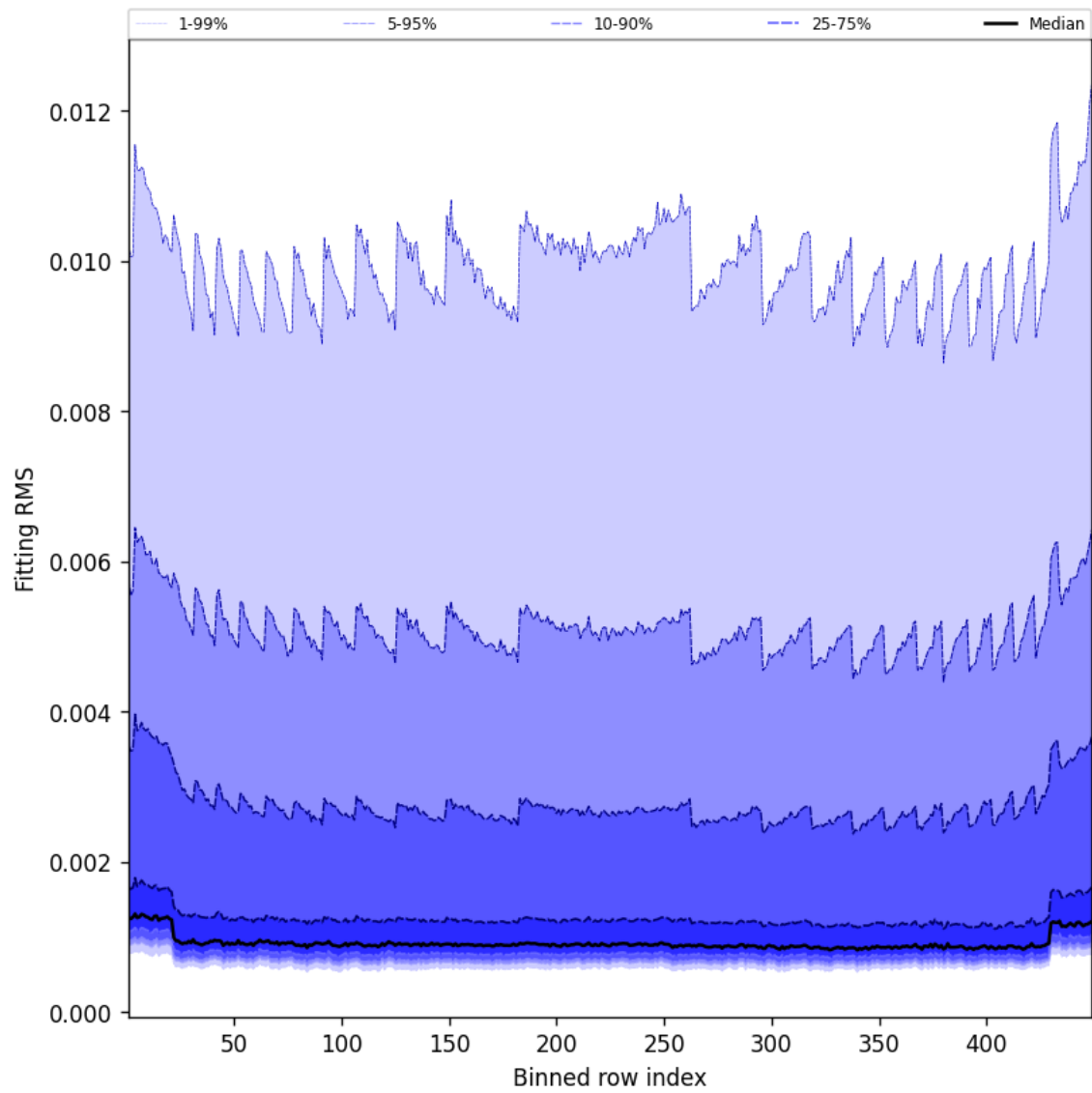
Figure 46: Along track statistics of “Fitting RMS” for 2025-06-01 to 2025-06-02
