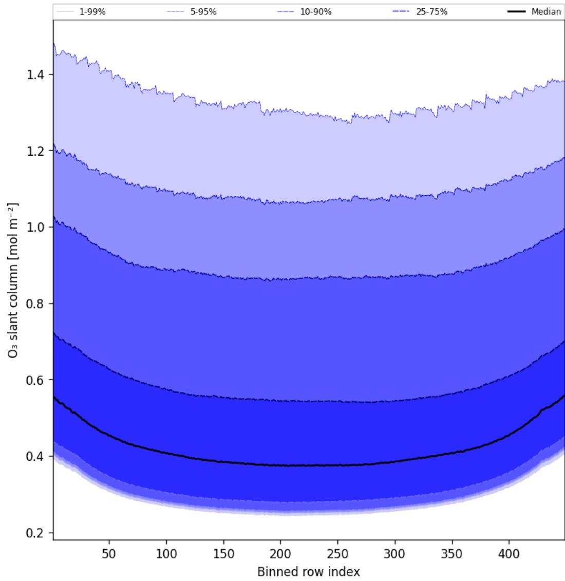
Figure 43: Along track statistics of “O 3 slant column” for 2025-06-01 to 2025-06-02
