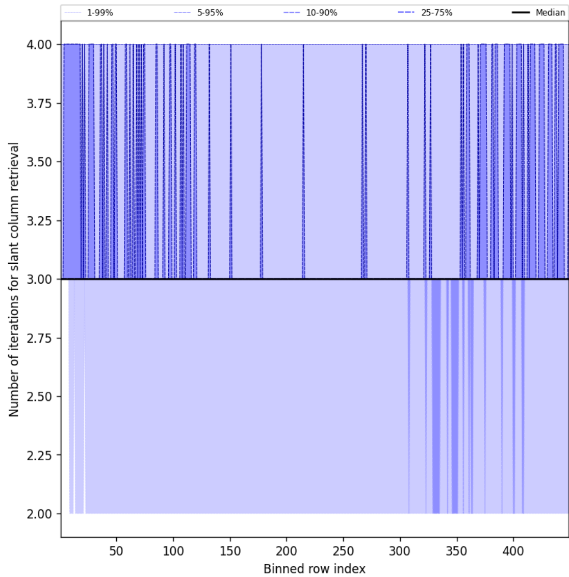
Figure 45: Along track statistics of “Number of iterations for slant column retrieval” for 2025-06-01 to 2025-06-02
