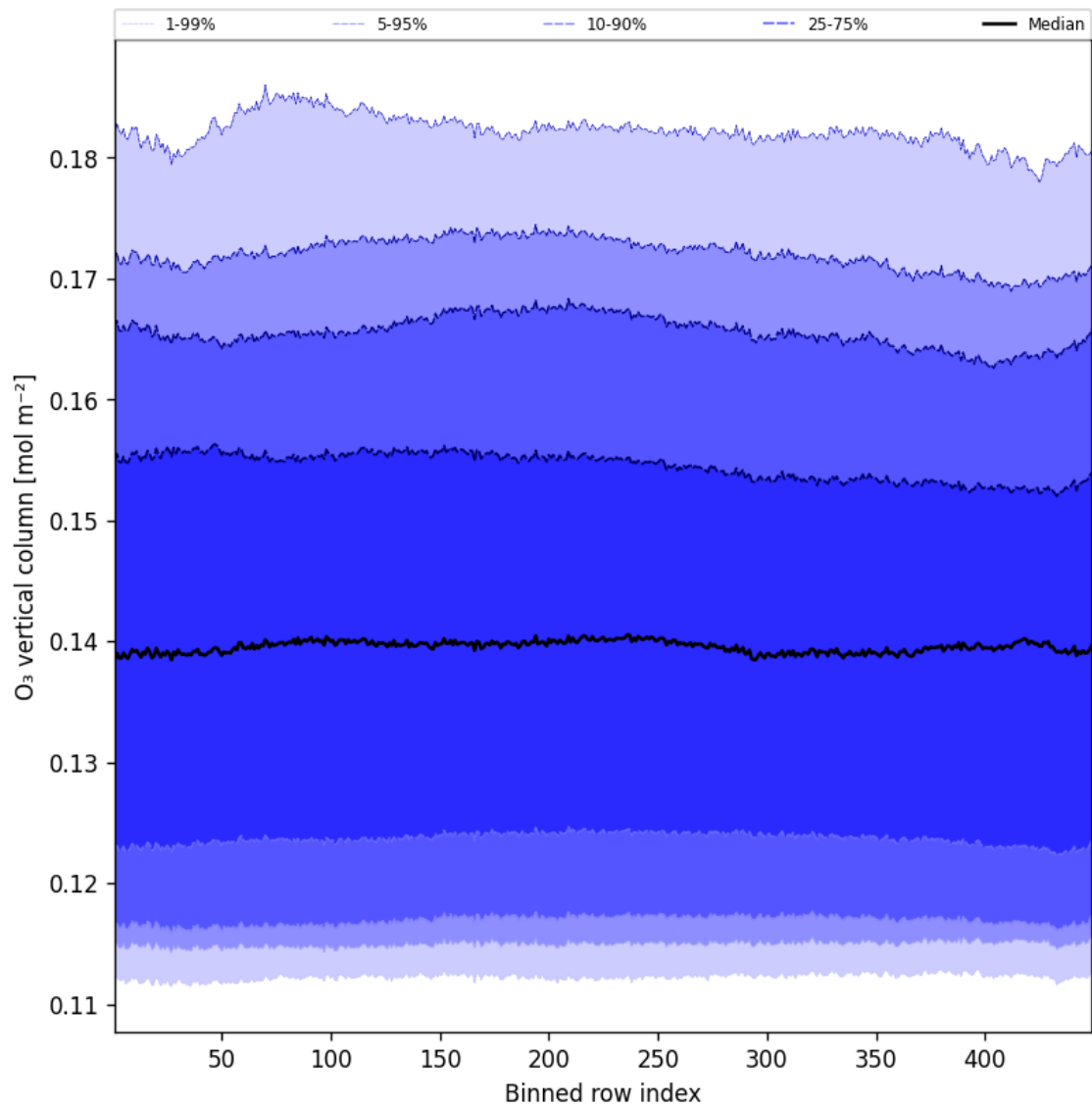
Figure 41: Along track statistics of “ \text{O}_3 vertical column” for 2025-06-01 to 2025-06-02
