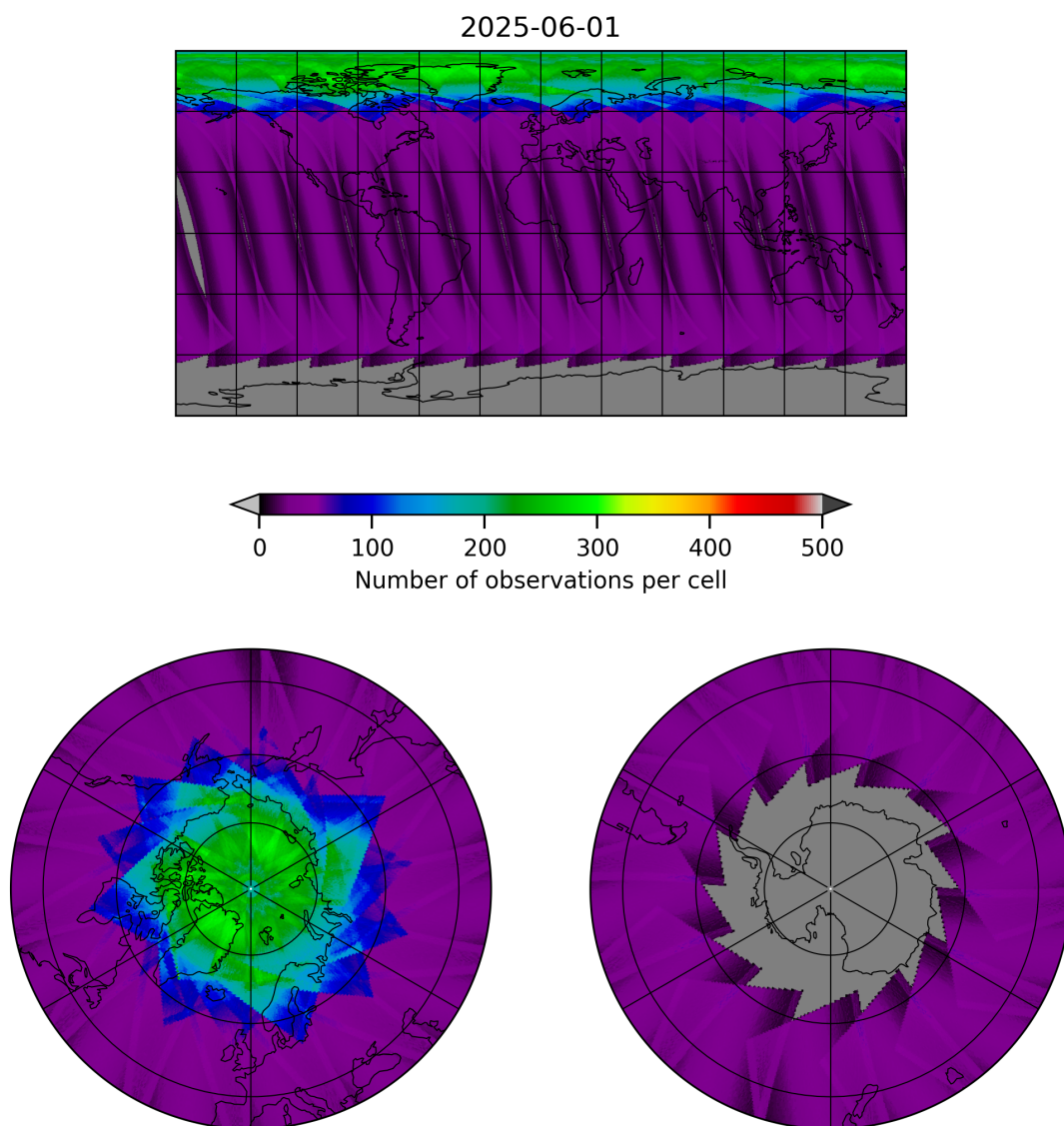
Figure 15: Map of the number of observations for 2025-06-01 to 2025-06-02
