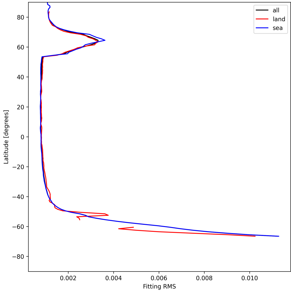
Figure 22: Zonal average of “Fitting RMS” for 2025-06-01 to 2025-06-02.
