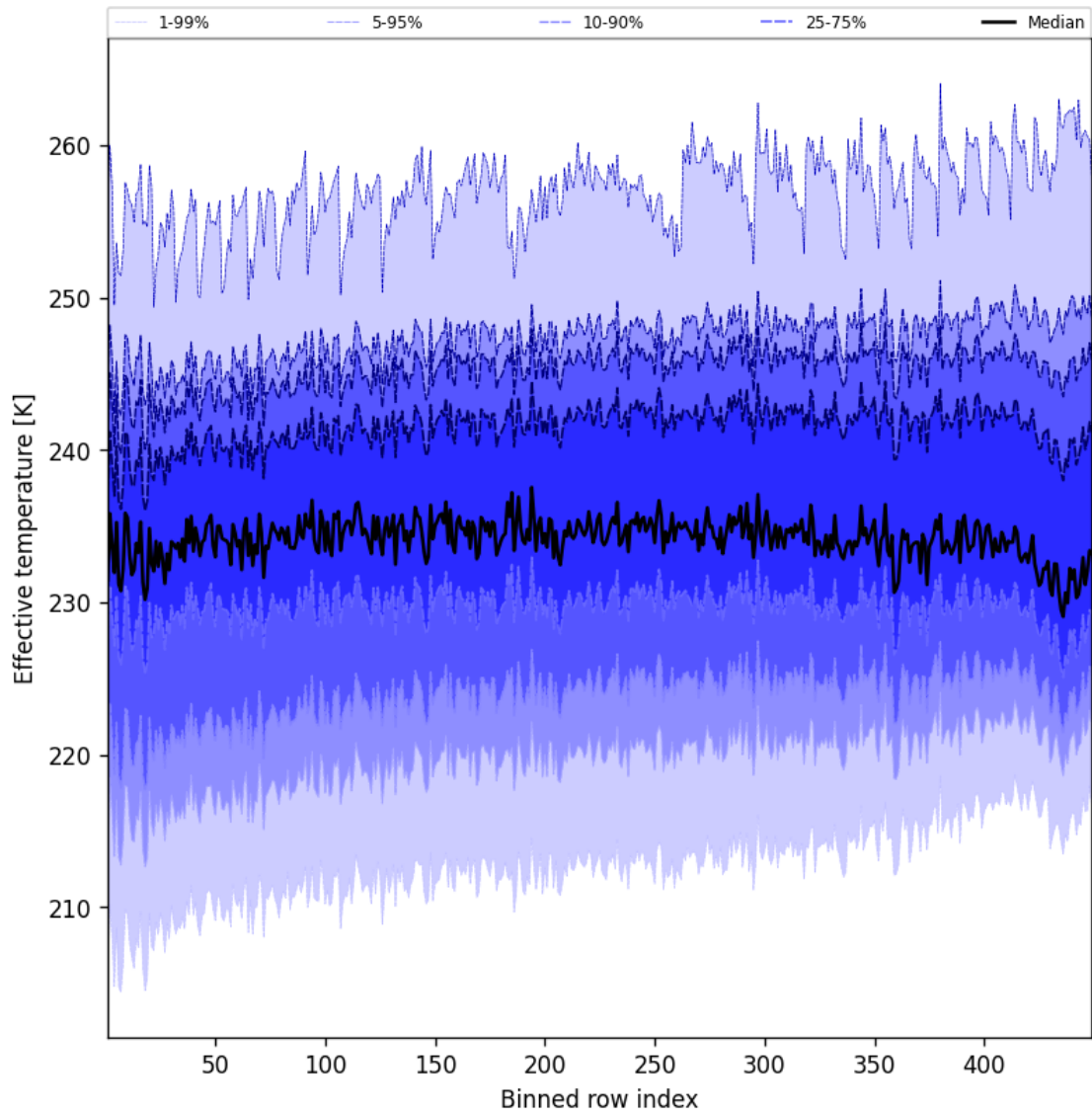
Figure 50: Along track statistics of “Effective temperature” for 2025-06-01 to 2025-06-02
