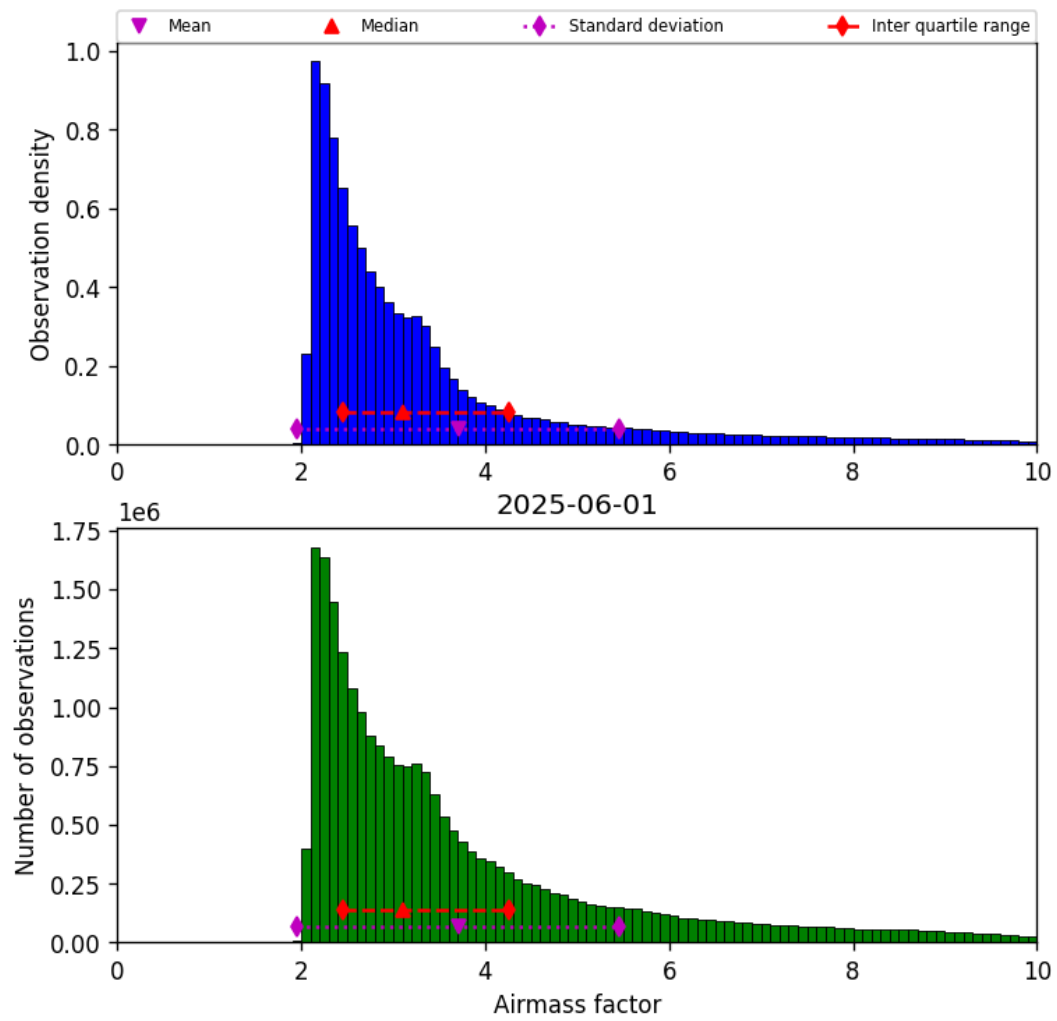
Figure 37: Histogram of “Airmass factor” for 2025-06-01 to 2025-06-02
