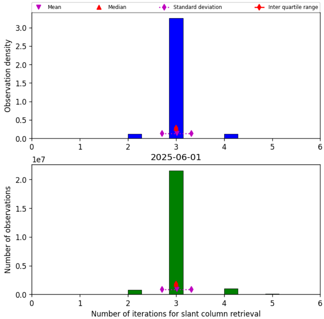
Figure 33: Histogram of “Number of iterations for slant column retrieval” for 2025-06-01 to 2025-06-02
