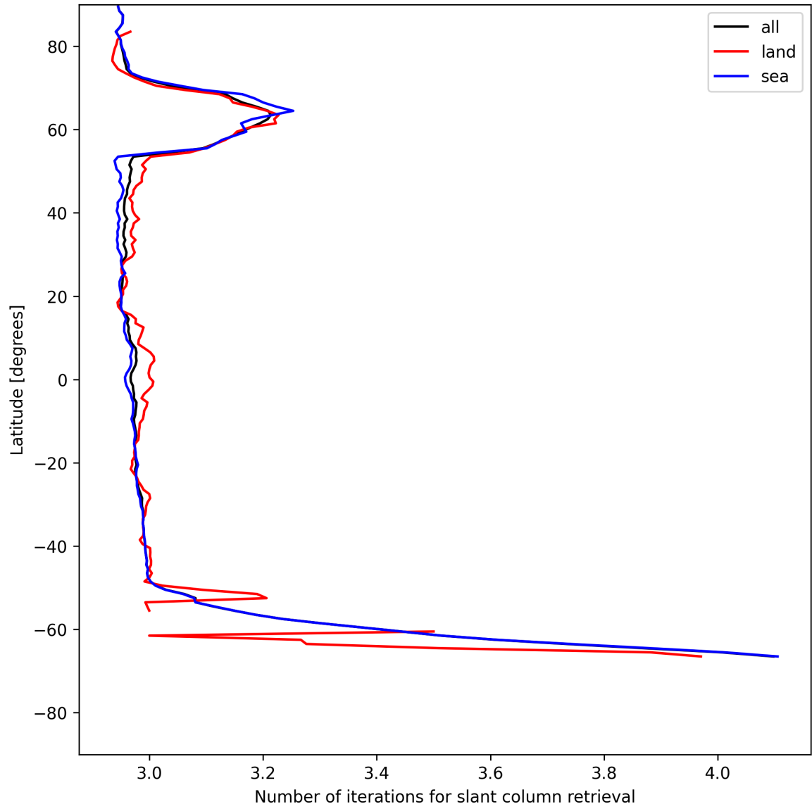
Figure 21: Zonal average of “Number of iterations for slant column retrieval” for 2025-06-01 to 2025-06-02.
