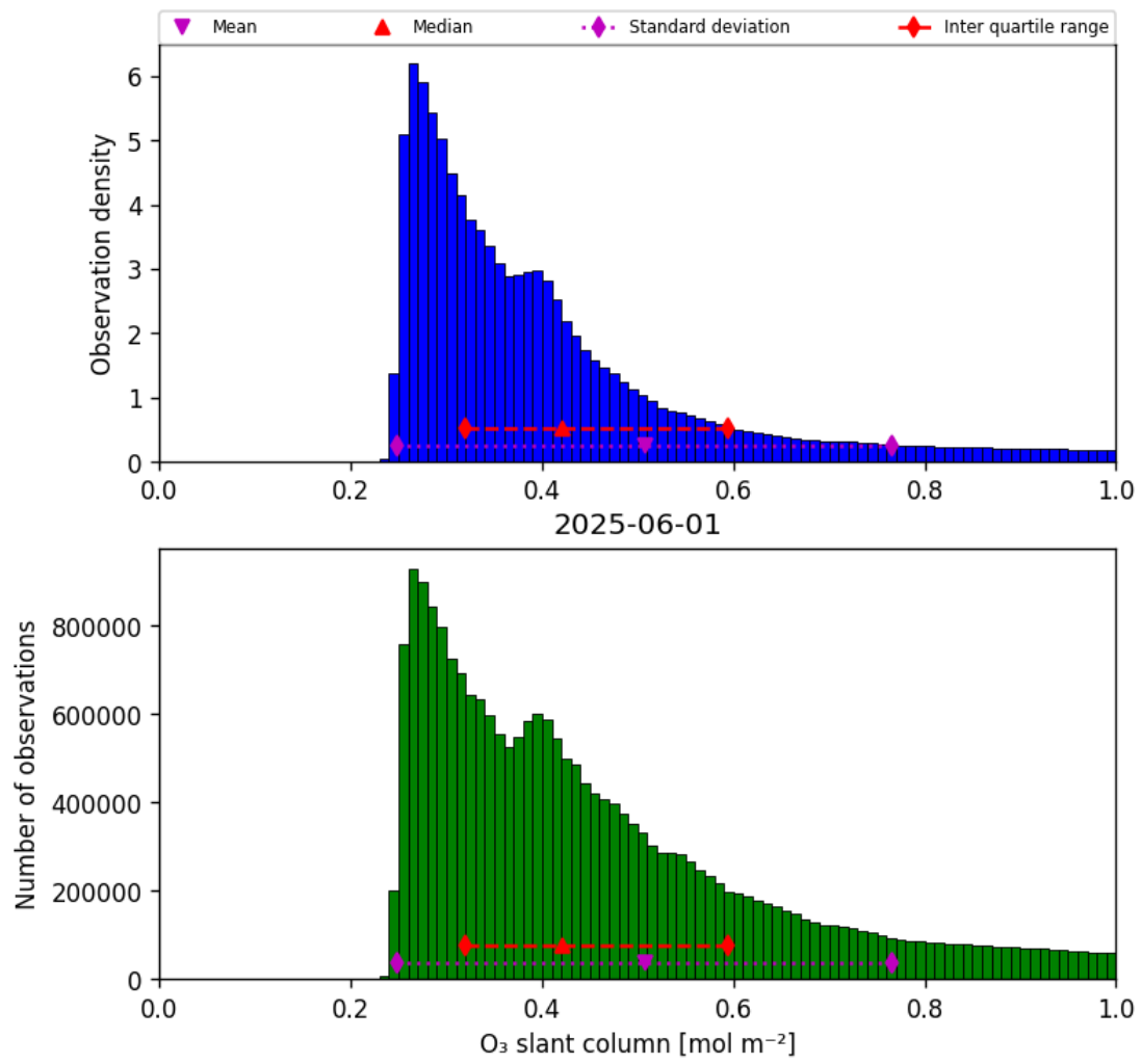
Figure 31: Histogram of “O 3 slant column” for 2025-06-01 to 2025-06-02
