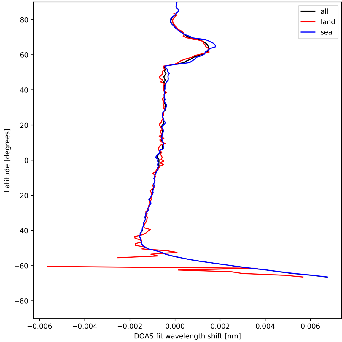
Figure 23: Zonal average of “DOAS fit wavelength shift” for 2025-06-01 to 2025-06-02.
