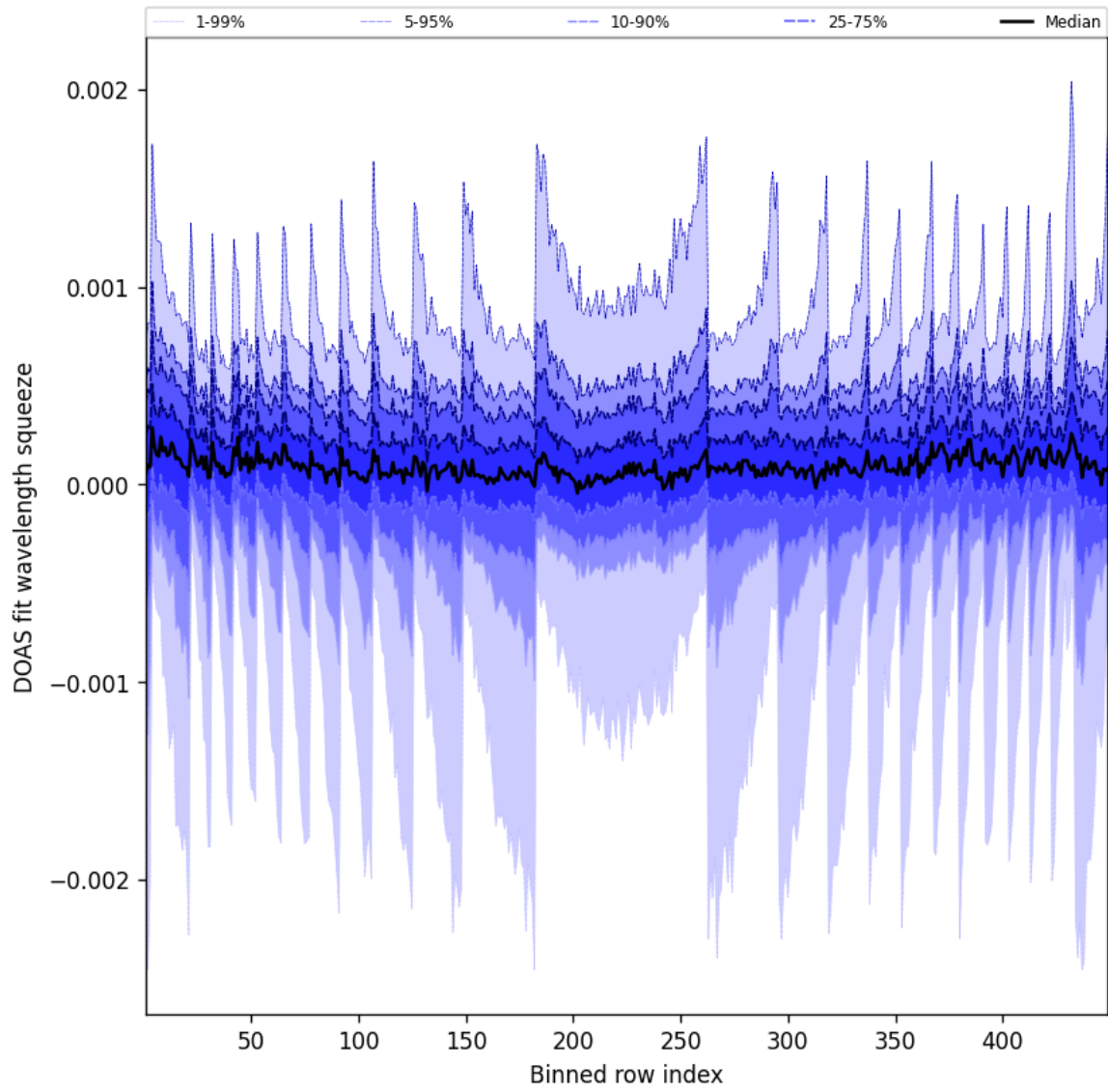
Figure 48: Along track statistics of “DOAS fit wavelength squeeze” for 2025-06-01 to 2025-06-02
