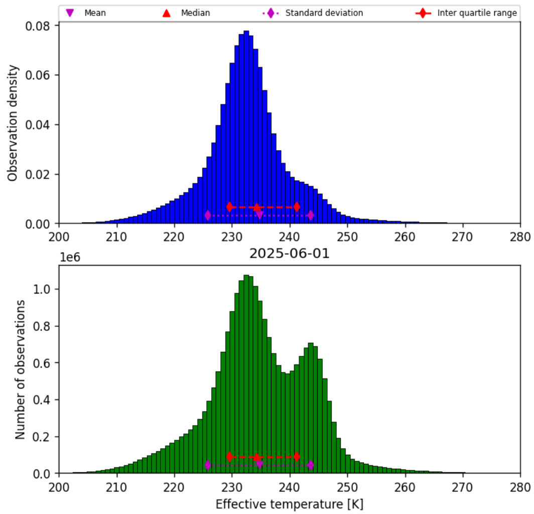
Figure 38: Histogram of “Effective temperature” for 2025-06-01 to 2025-06-02
