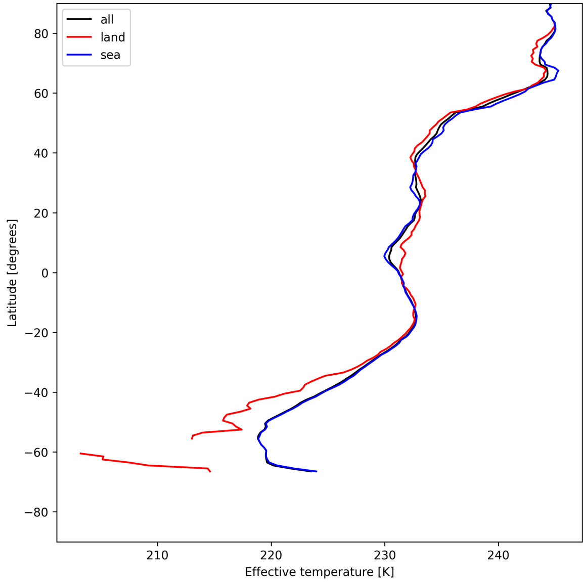
Figure 26: Zonal average of "Effective temperature" for 2025-06-01 to 2025-06-02.
