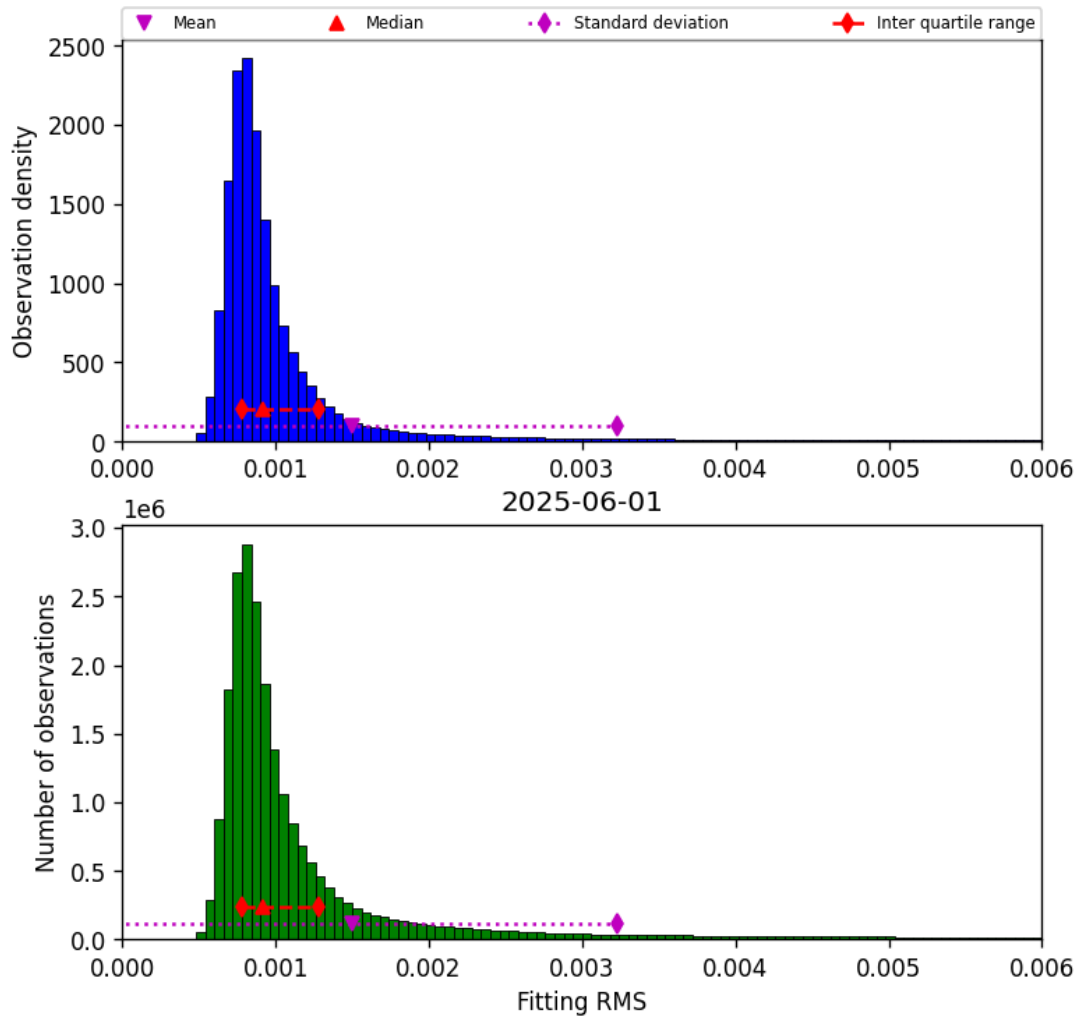
Figure 34: Histogram of “Fitting RMS” for 2025-06-01 to 2025-06-02
