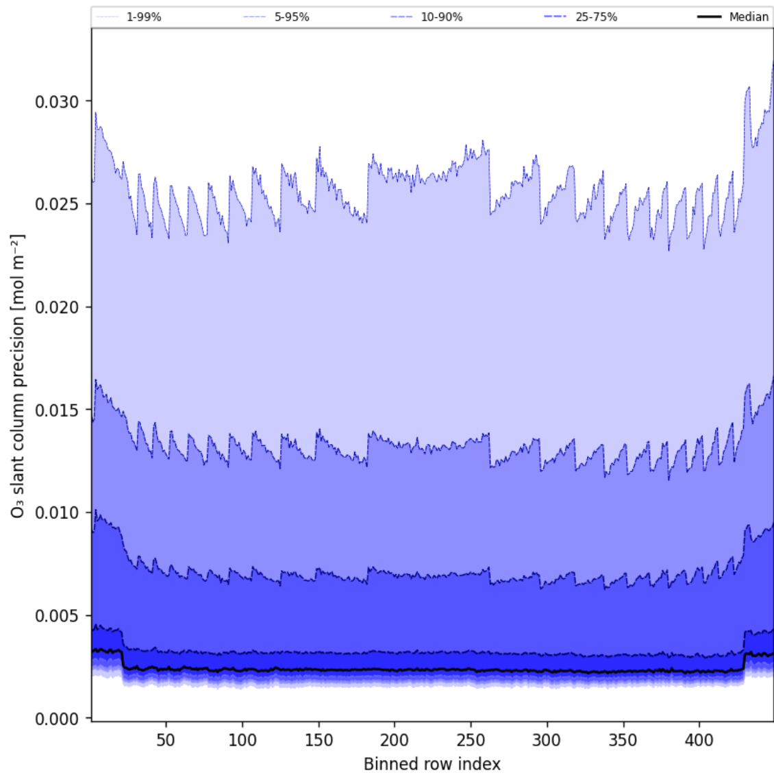
Figure 44: Along track statistics of “O 3 slant column precision” for 2025-06-01 to 2025-06-02
