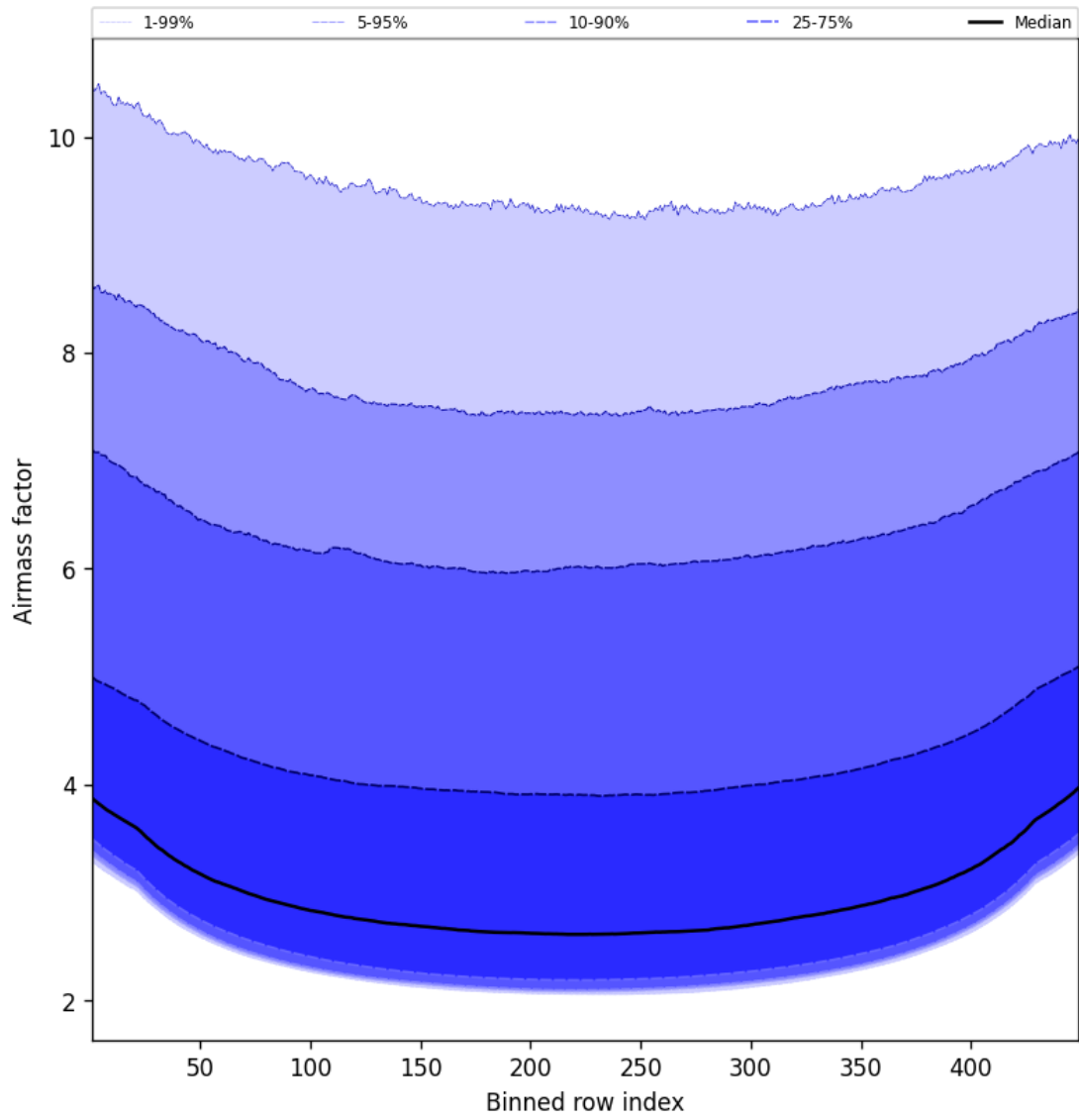
Figure 49: Along track statistics of “Airmass factor” for 2025-06-01 to 2025-06-02
