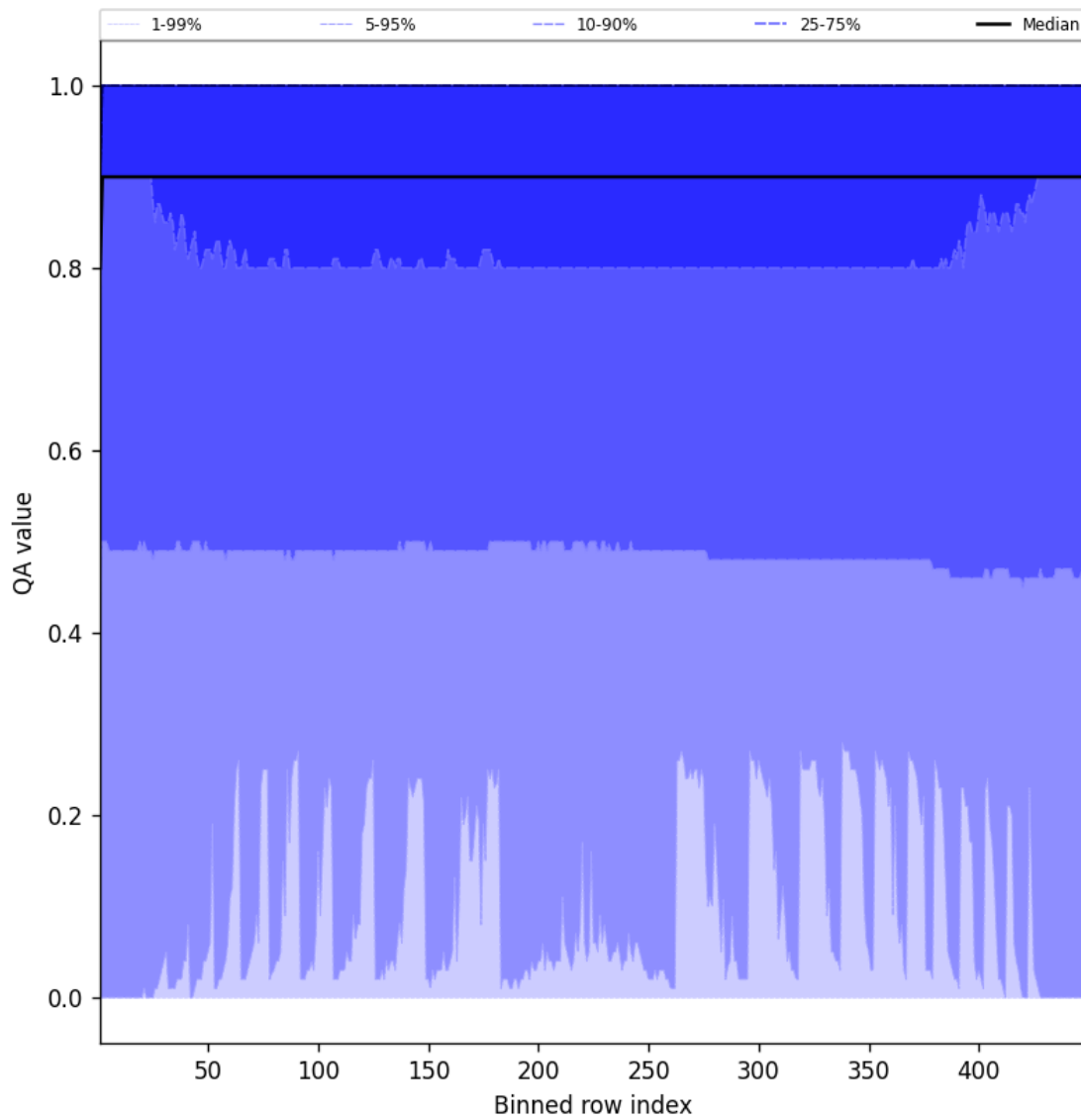
Figure 40: Along track statistics of “QA value” for 2025-06-01 to 2025-06-02
