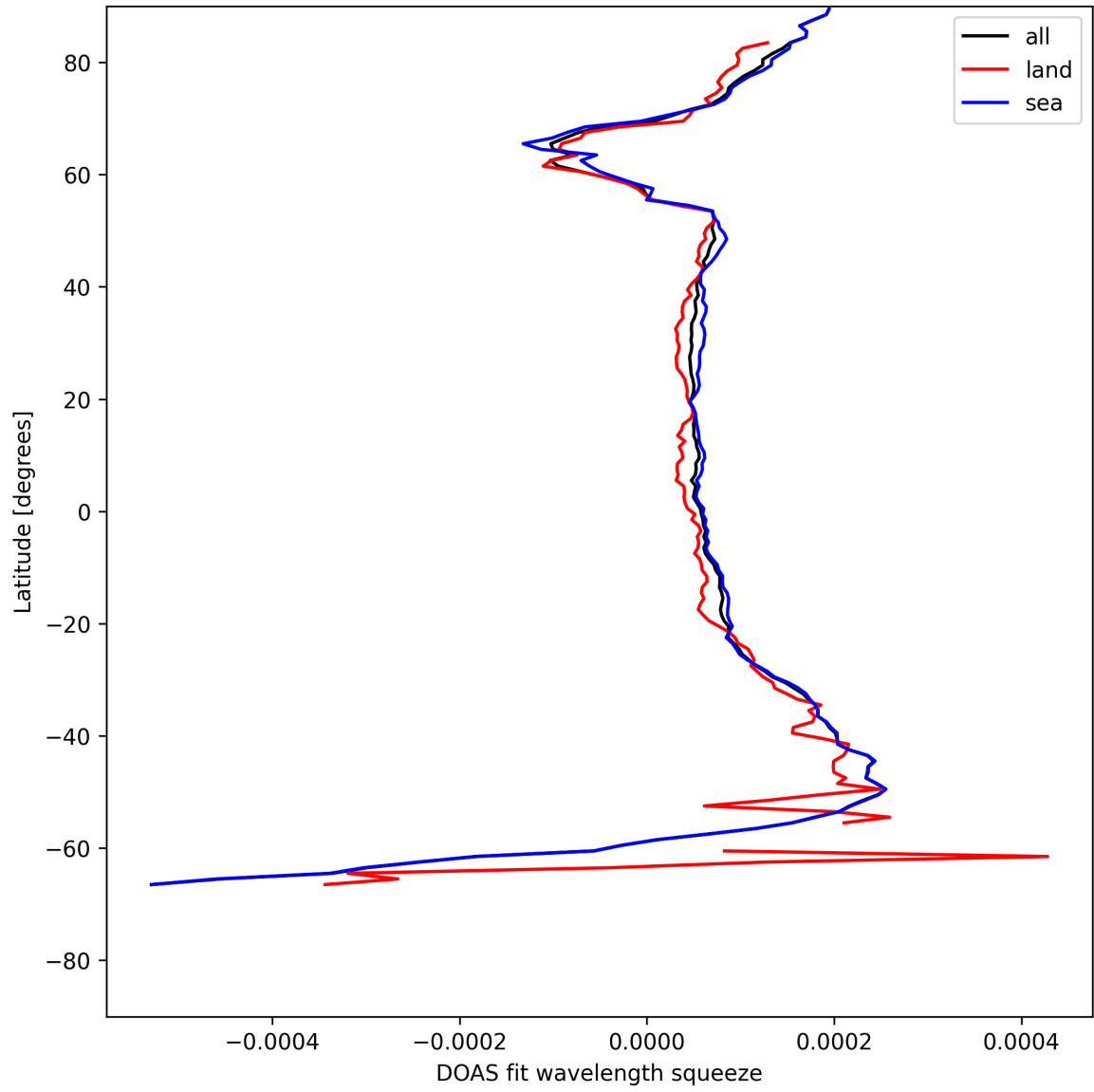
Figure 24: Zonal average of “DOAS fit wavelength squeeze” for 2025-06-01 to 2025-06-02.
