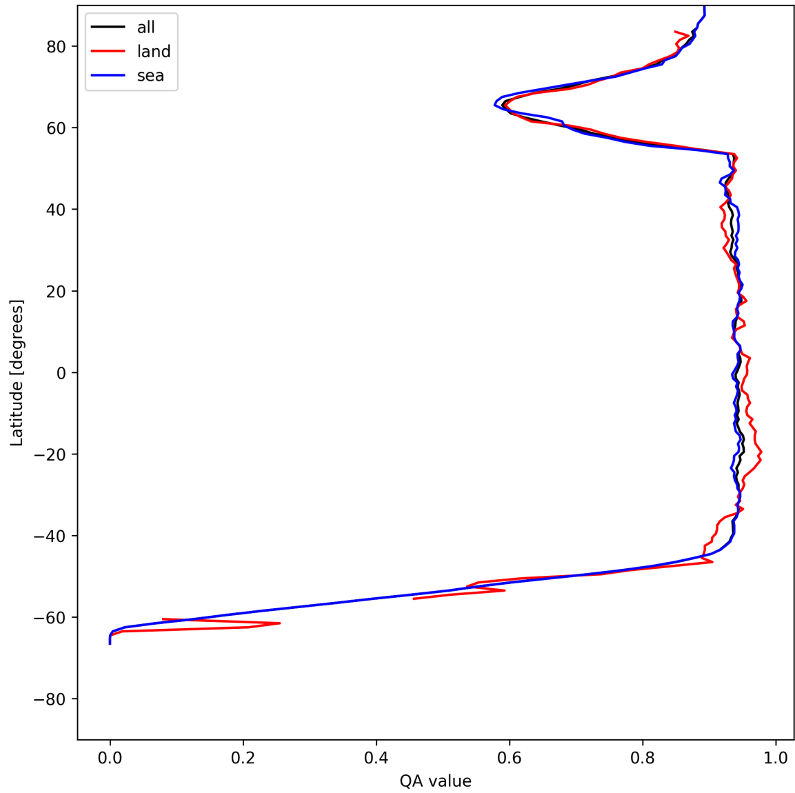
Figure 16: Zonal average of “QA value” for 2025-06-01 to 2025-06-02.
