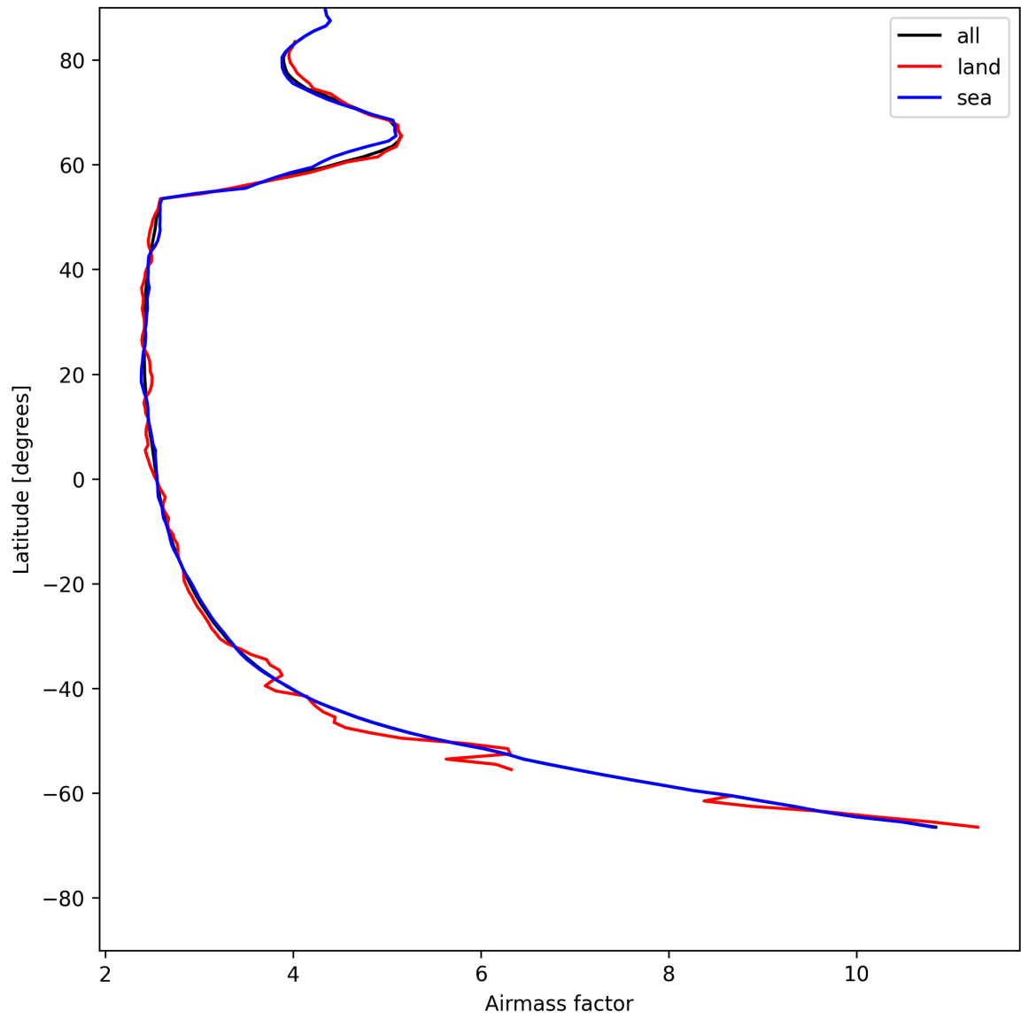
Figure 25: Zonal average of “Airmass factor” for 2025-06-01 to 2025-06-02.
