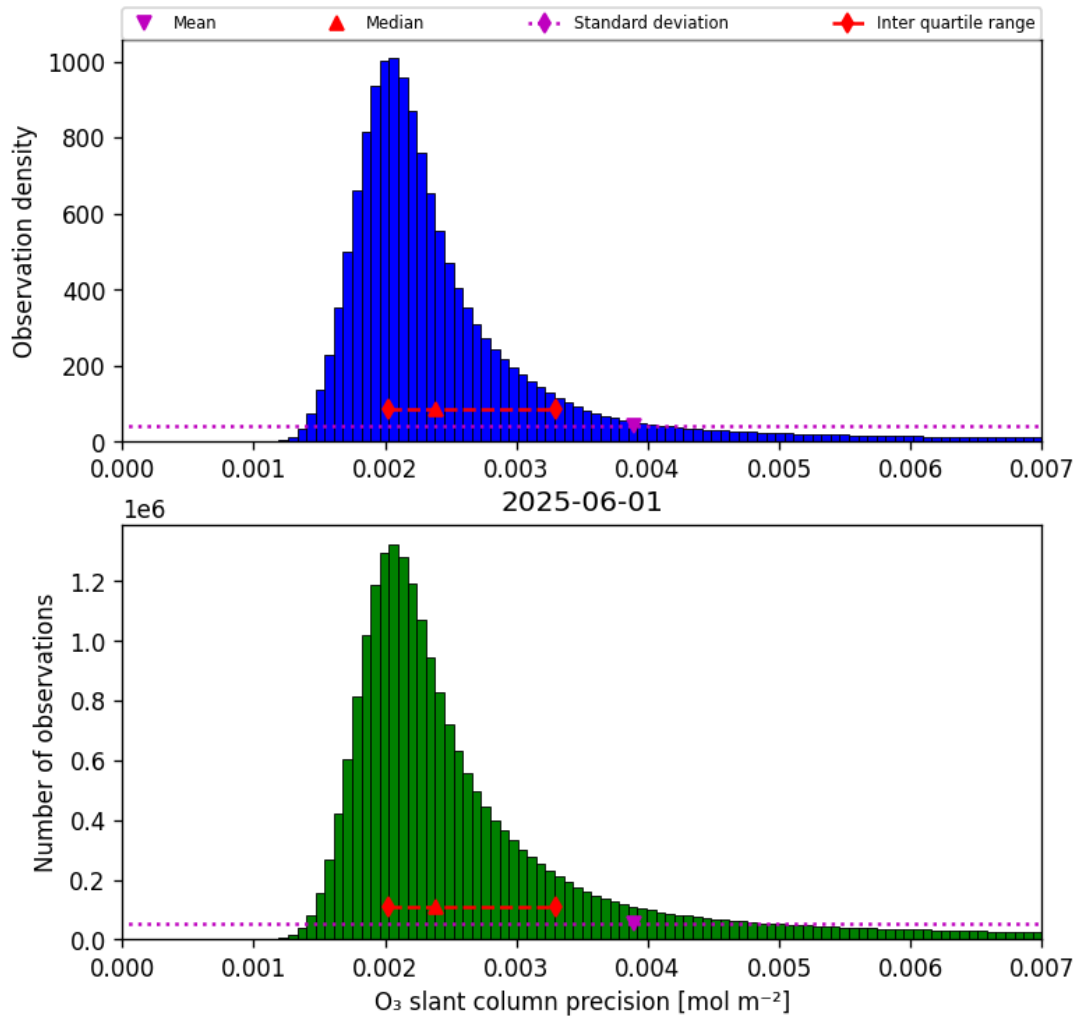
Figure 32: Histogram of “O 3 slant column precision” for 2025-06-01 to 2025-06-02
