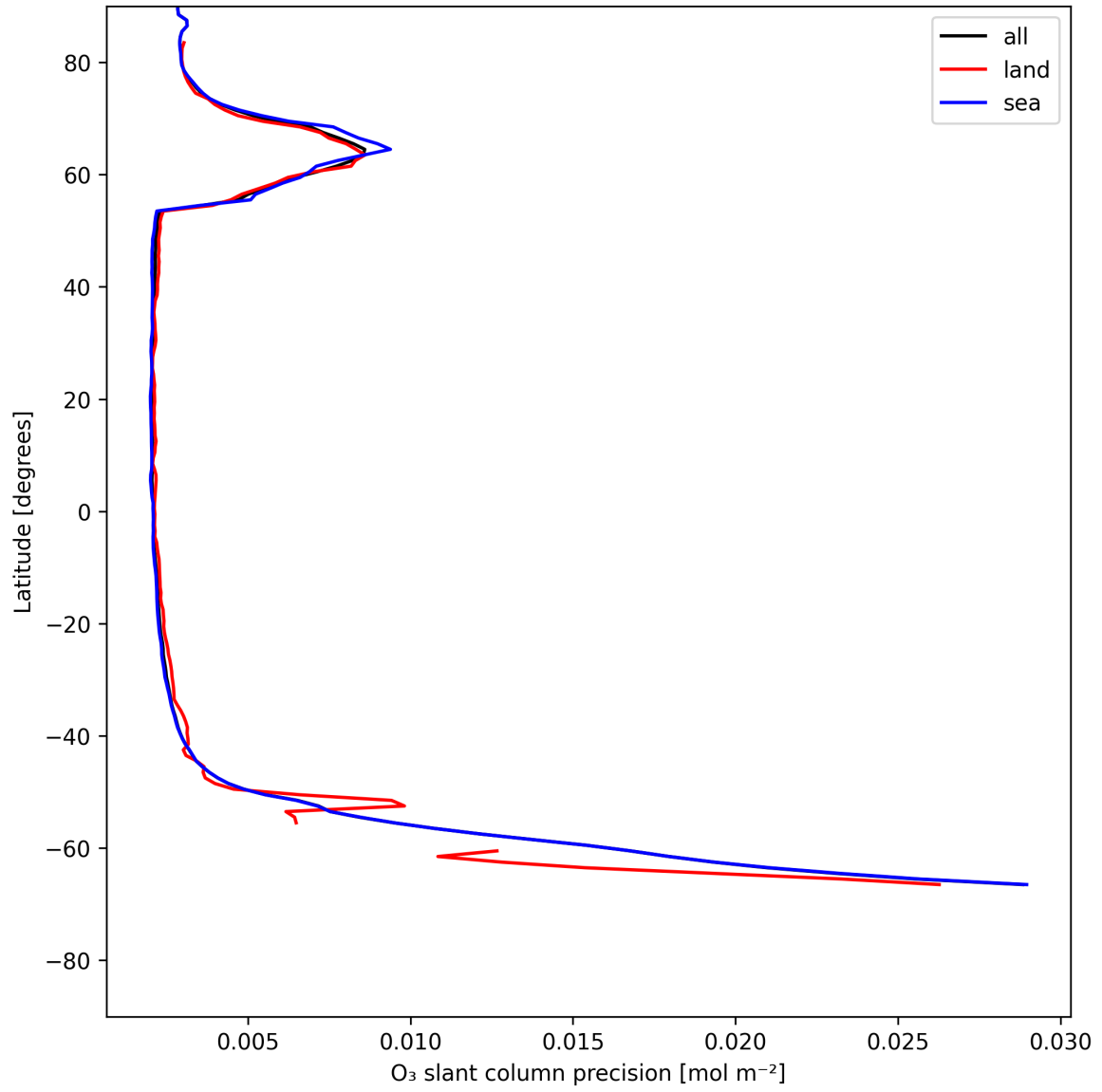
Figure 20: Zonal average of “O 3 slant column precision” for 2025-06-01 to 2025-06-02.
