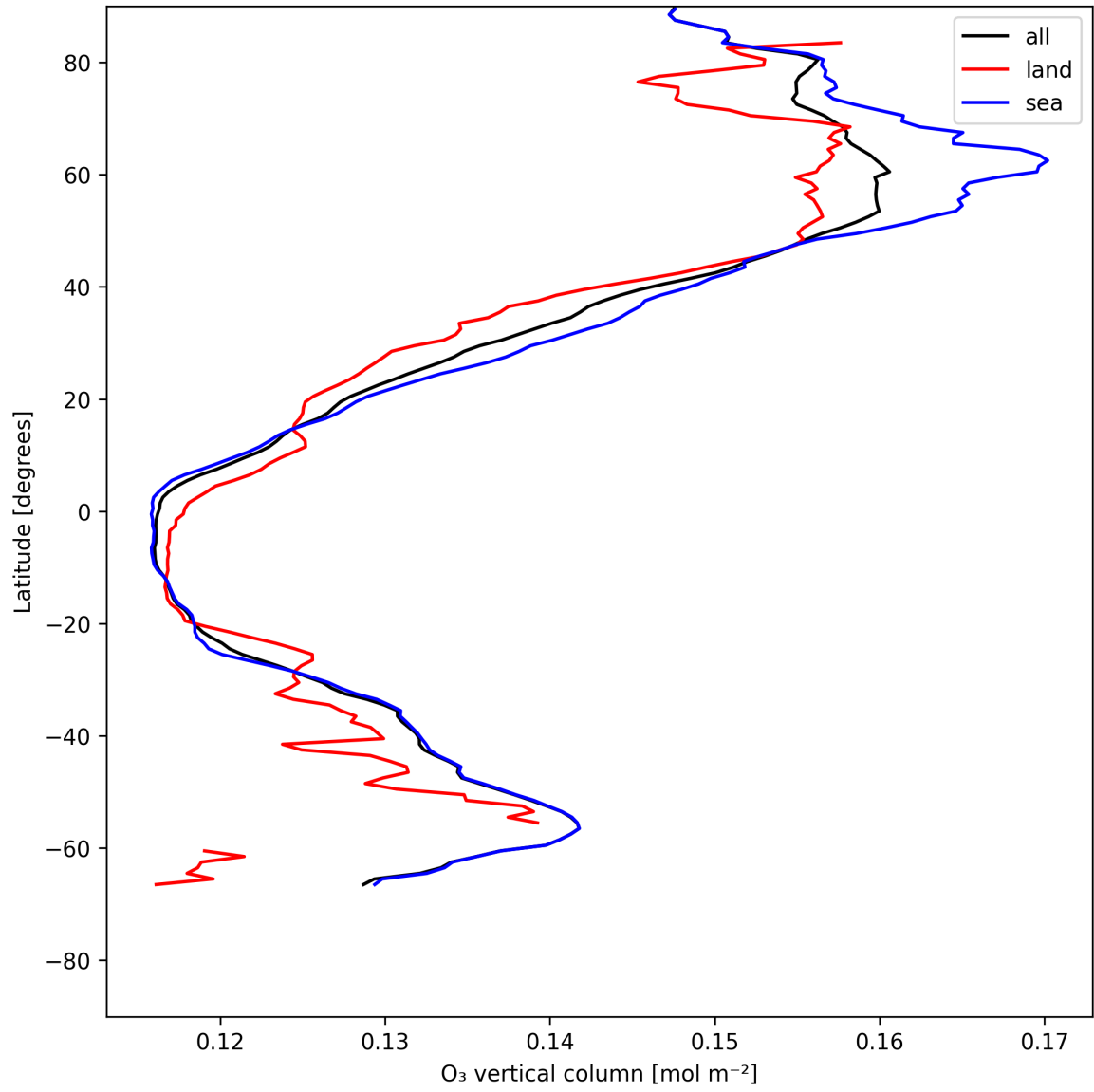
Figure 17: Zonal average of “O 3 vertical column” for 2025-06-01 to 2025-06-02.
