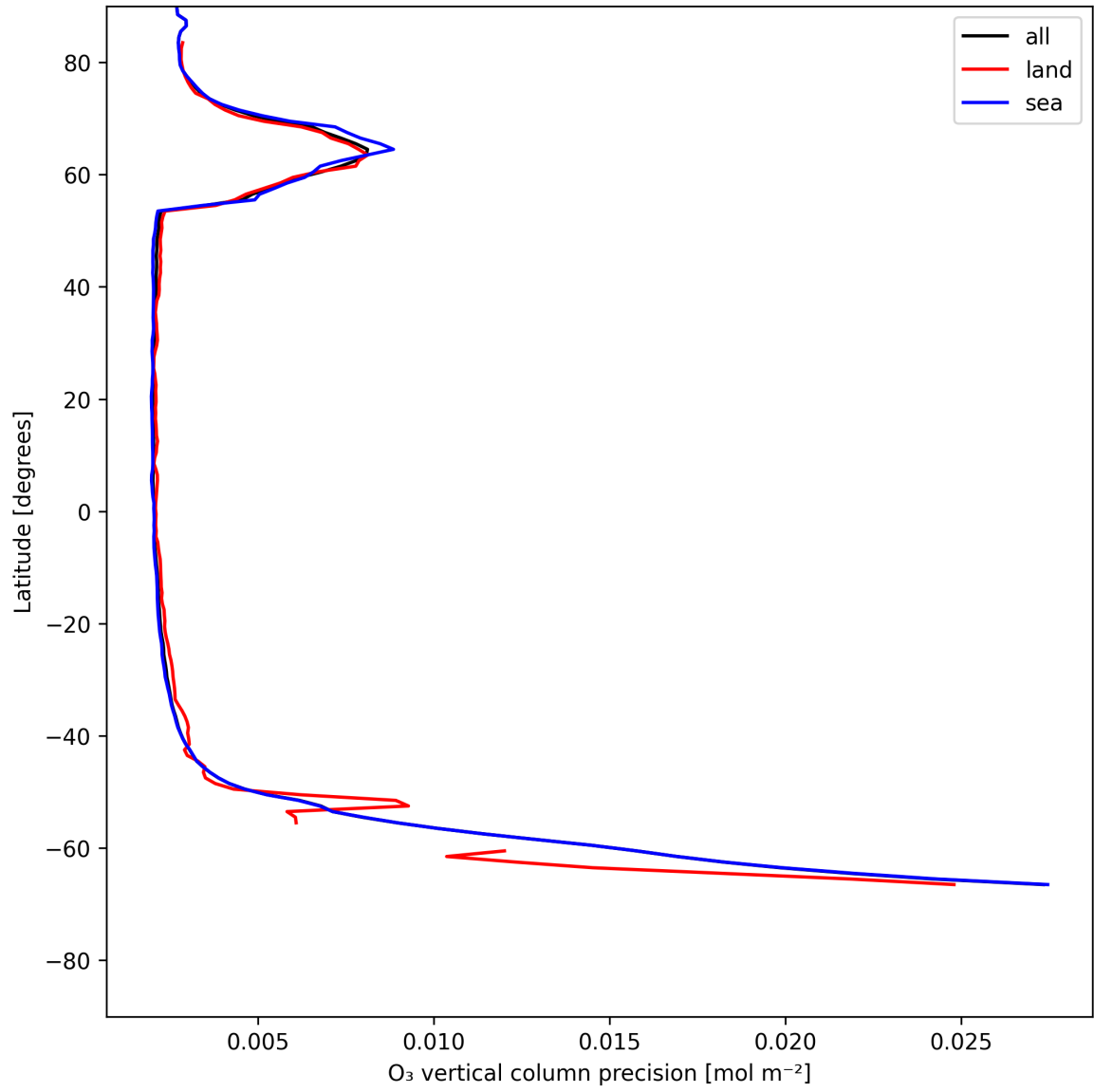
Figure 18: Zonal average of “O 3 vertical column precision” for 2025-06-01 to 2025-06-02.
