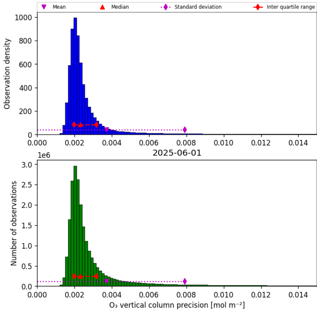
Figure 30: Histogram of “O 3 vertical column precision” for 2025-06-01 to 2025-06-02
