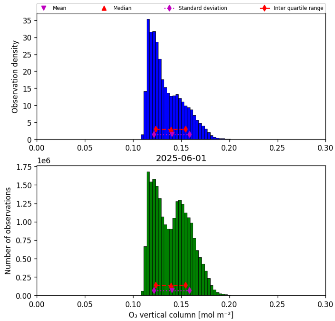
Figure 29: Histogram of “O 3 vertical column” for 2025-06-01 to 2025-06-02
