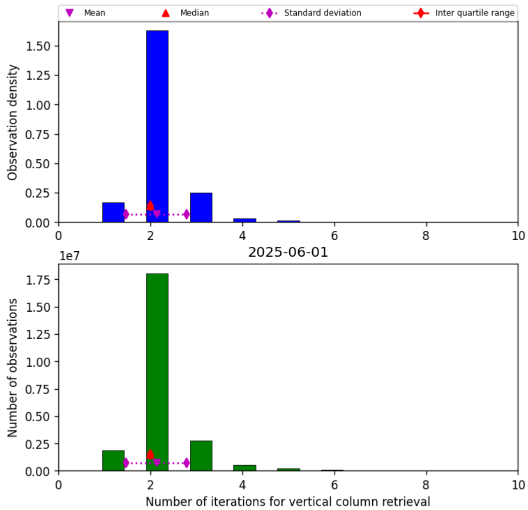
Figure 39: Histogram of “Number of iterations for vertical column retrieval” for 2025-06-01 to 2025-06-02
