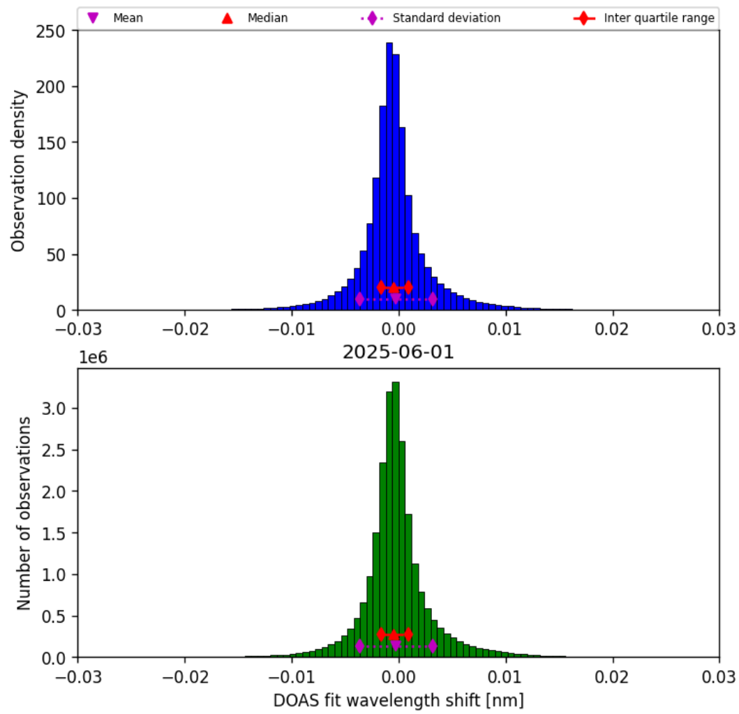
Figure 35: Histogram of “DOAS fit wavelength shift” for 2025-06-01 to 2025-06-02
