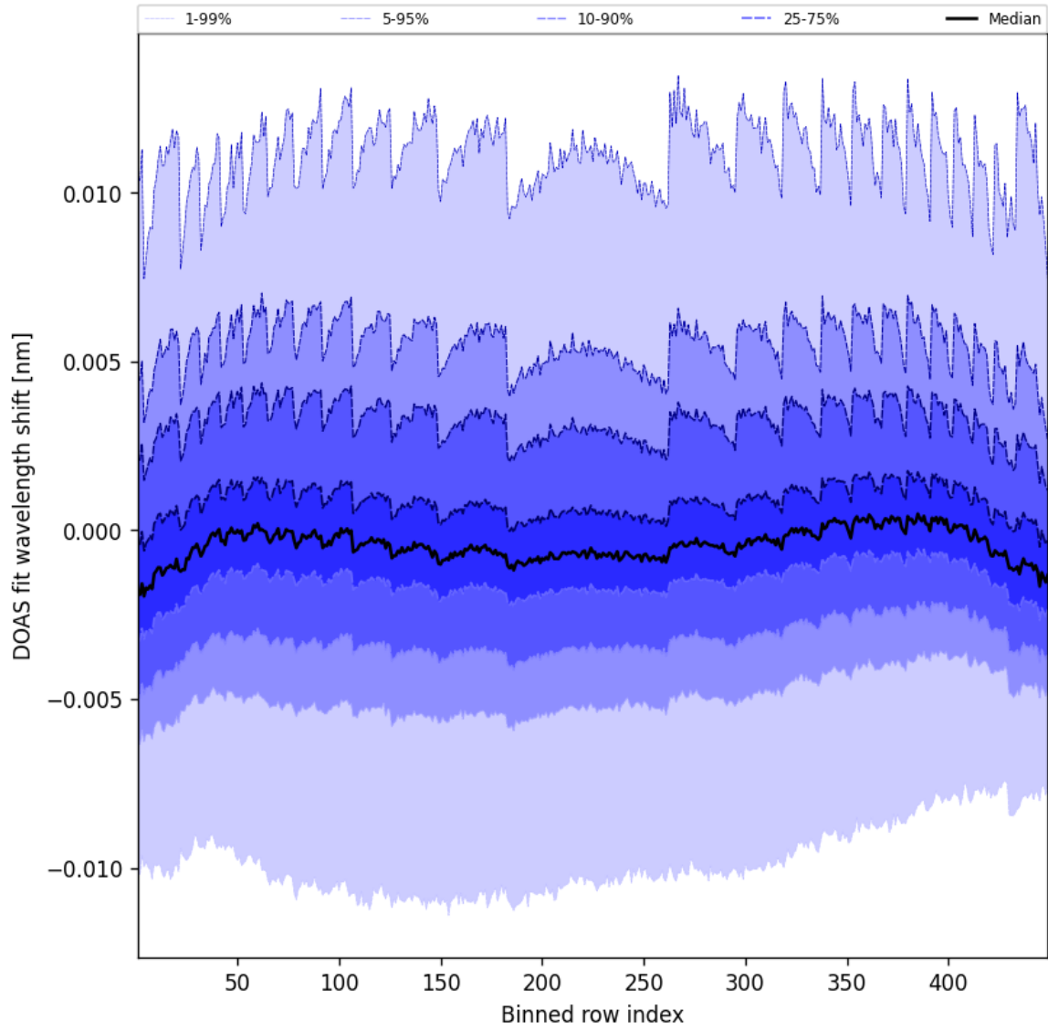
Figure 47: Along track statistics of “DOAS fit wavelength shift” for 2025-06-01 to 2025-06-02
