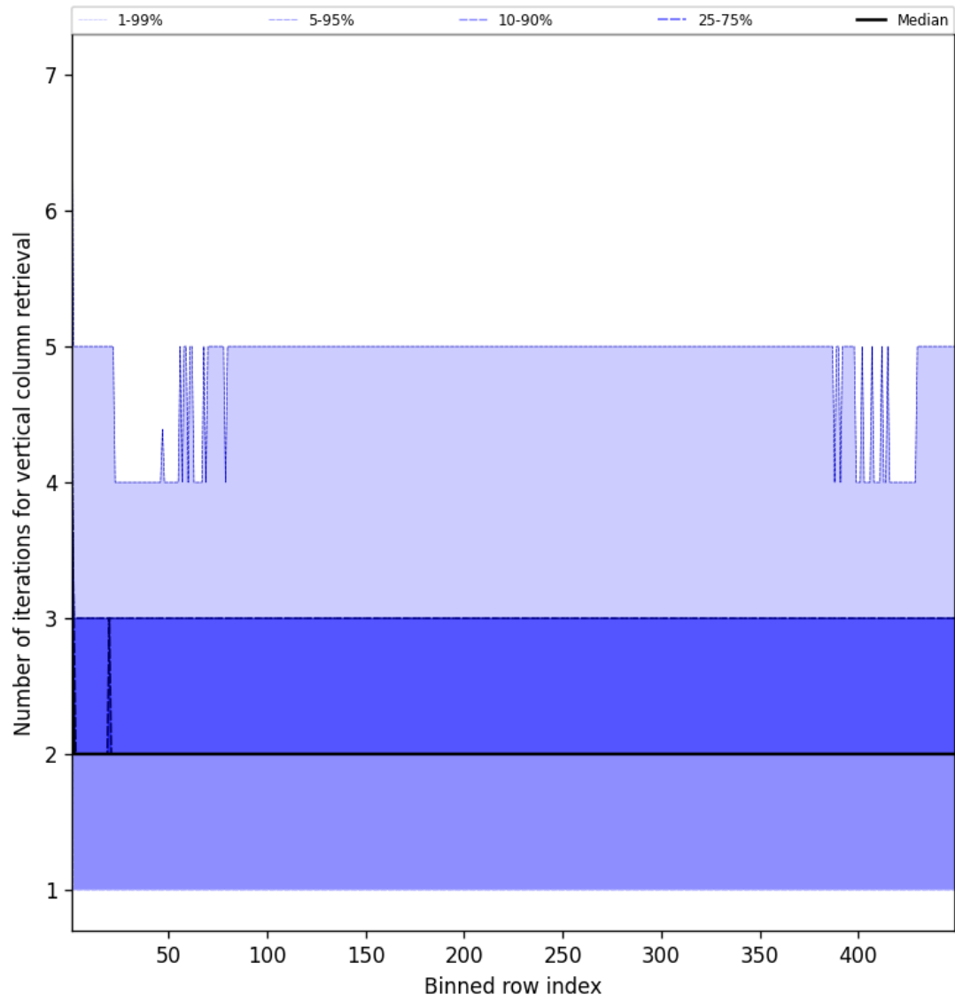
Figure 51: Along track statistics of “Number of iterations for vertical column retrieval” for 2025-06-01 to 2025-06-02
